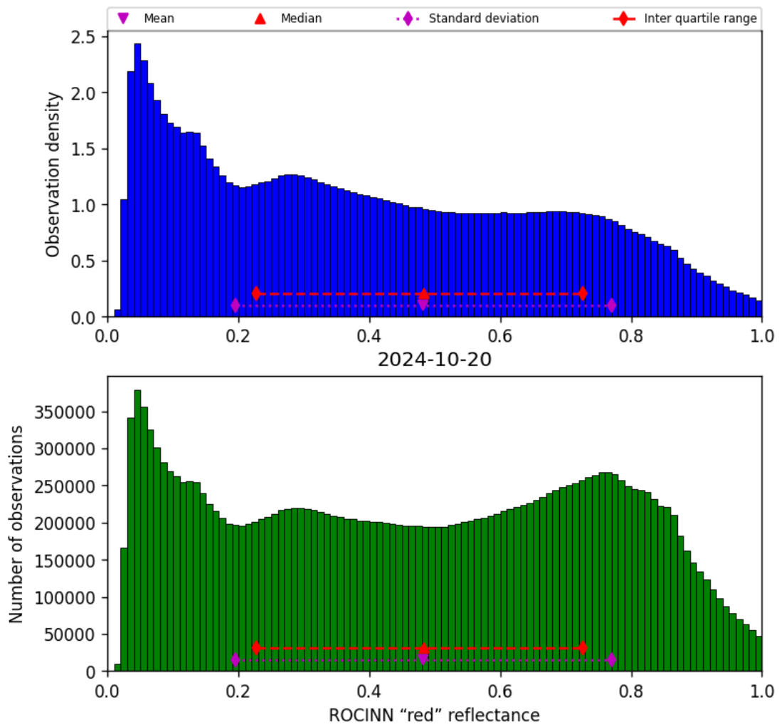
Figure 53: Histogram of “ROCINN “red” reflectance” for 2024-10-19 to 2024-10-21
