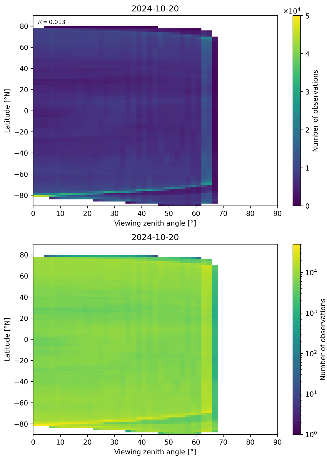
Figure 113: Scatter density plot of “Viewing zenith angle” against “Latitude” for 2024-10-19 to 2024-10-21.
