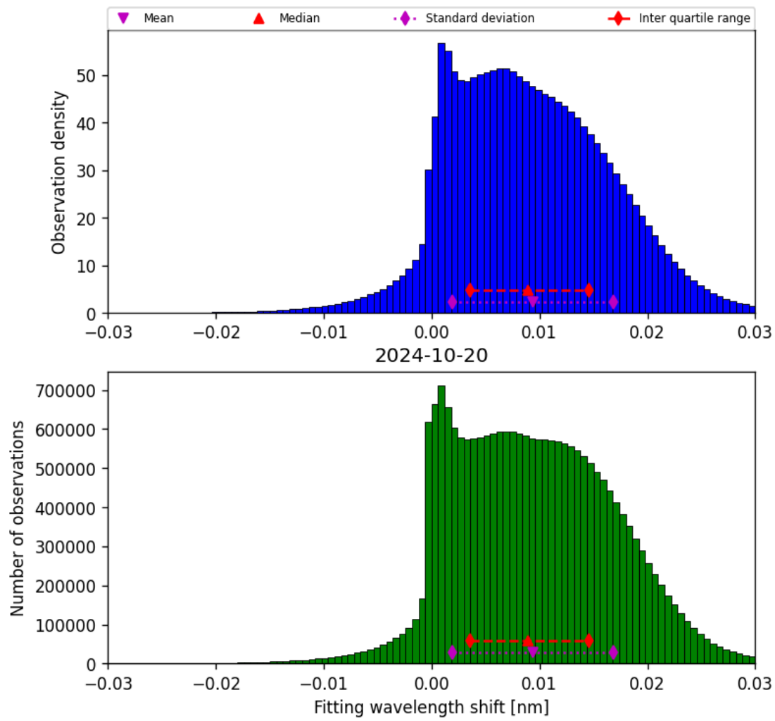
Figure 49: Histogram of “Fitting wavelength shift” for 2024-10-19 to 2024-10-21
