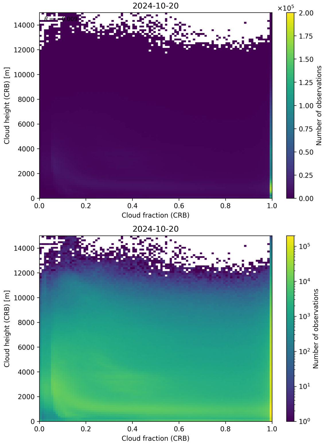
Figure 79: Scatter density plot of “Cloud fraction (CRB)” against “Cloud height (CRB)” for 2024-10-19 to 2024-10-21.
