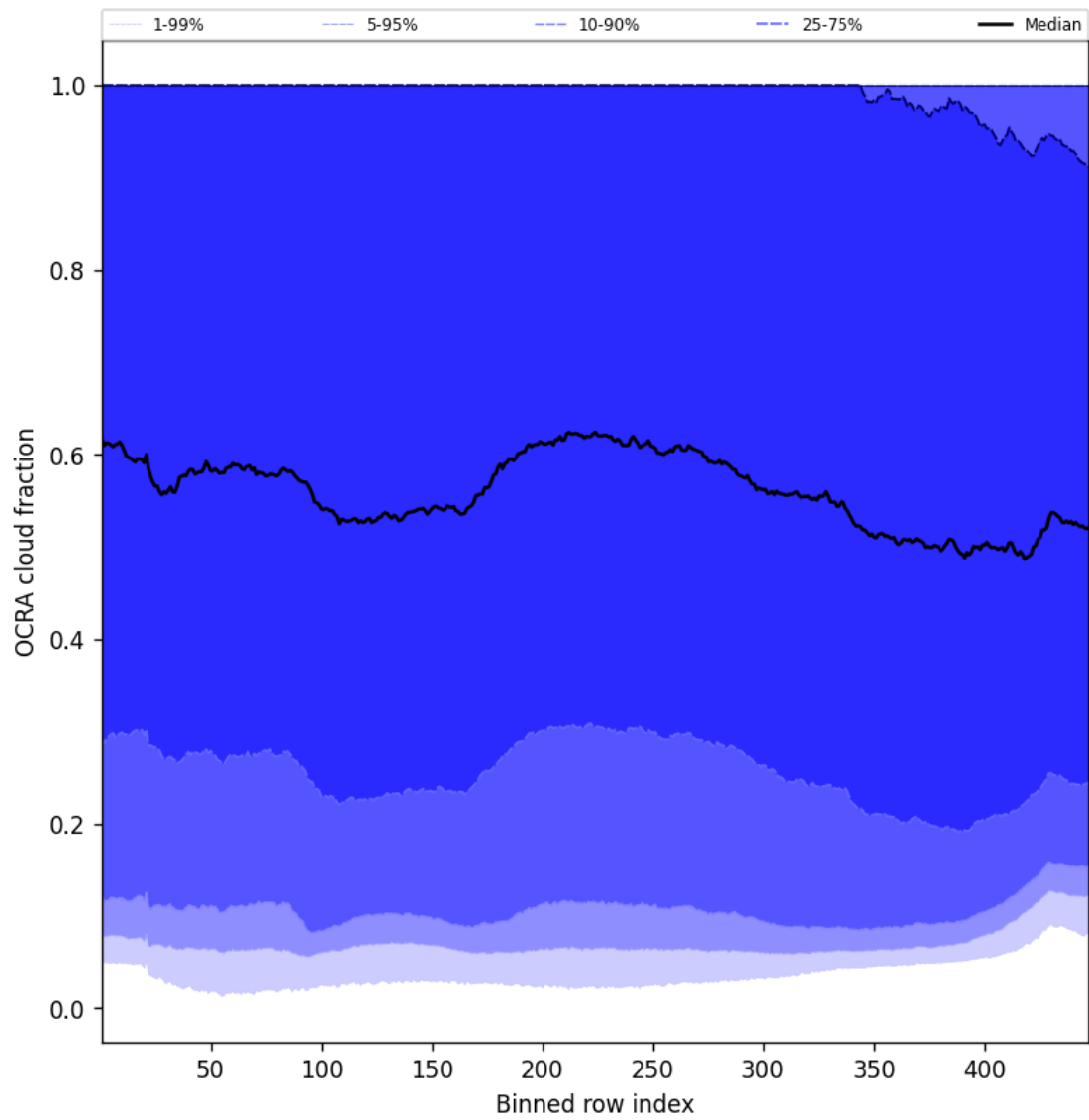
Figure 66: Along track statistics of “OCRA cloud fraction” for 2024-10-19 to 2024-10-21
