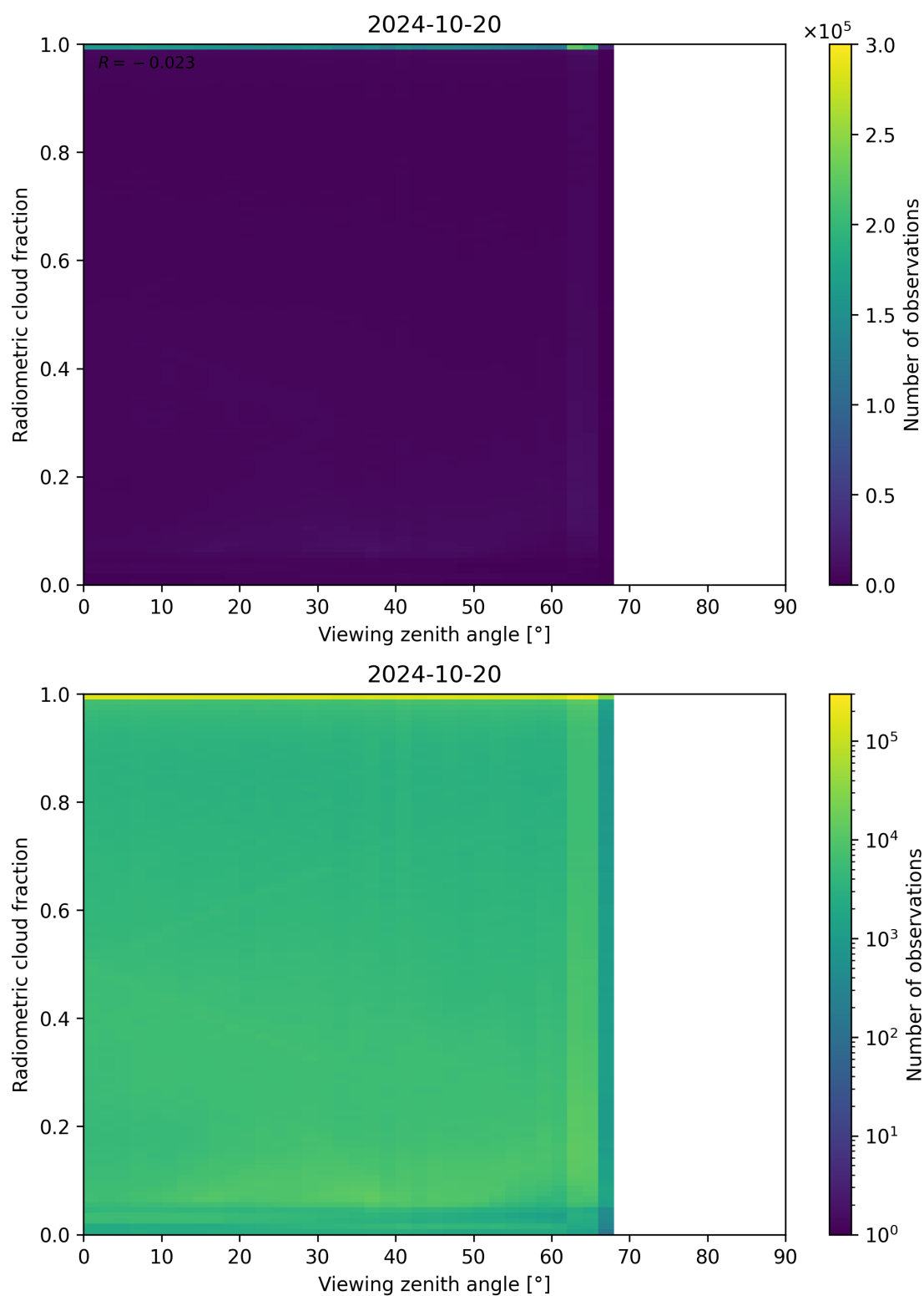
Figure 107: Scatter density plot of “Viewing zenith angle” against “Radiometric cloud fraction” for 2024-10-19 to 2024-10-21.
