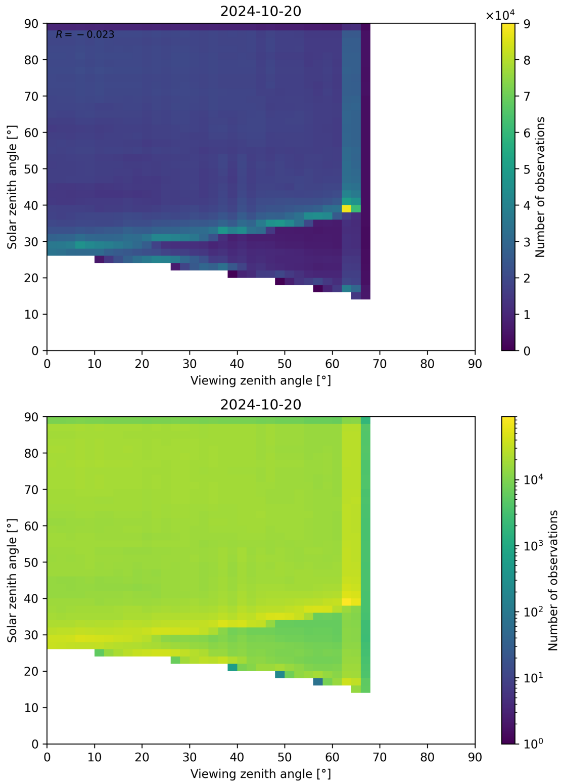
Figure 114: Scatter density plot of “Viewing zenith angle” against “Solar zenith angle” for 2024-10-19 to 2024-10-21.
