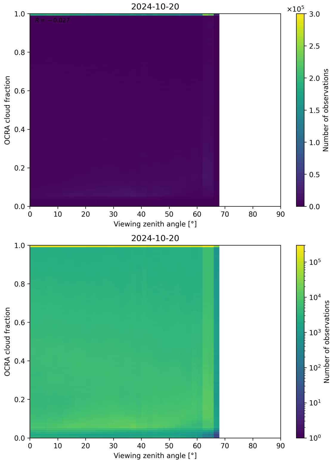
Figure 108: Scatter density plot of “Viewing zenith angle” against “OCRA cloud fraction” for 2024-10-19 to 2024-10-21.
