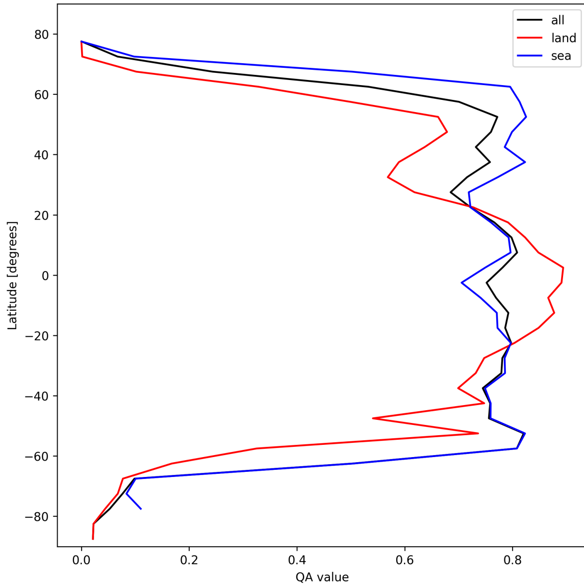
Figure 22: Zonal average of “QA value” for 2024-10-19 to 2024-10-21.
