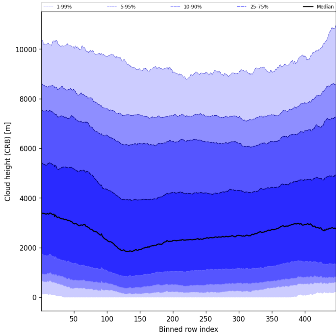
Figure 59: Along track statistics of “Cloud height (CRB)” for 2024-10-19 to 2024-10-21
