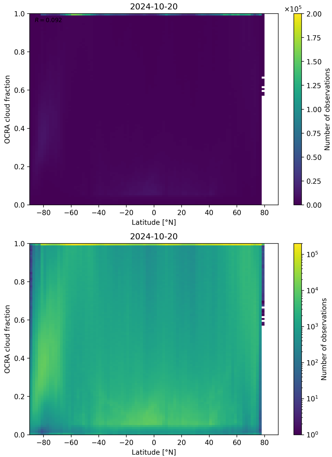
Figure 93: Scatter density plot of “Latitude” against “OCRA cloud fraction” for 2024-10-19 to 2024-10-21.
