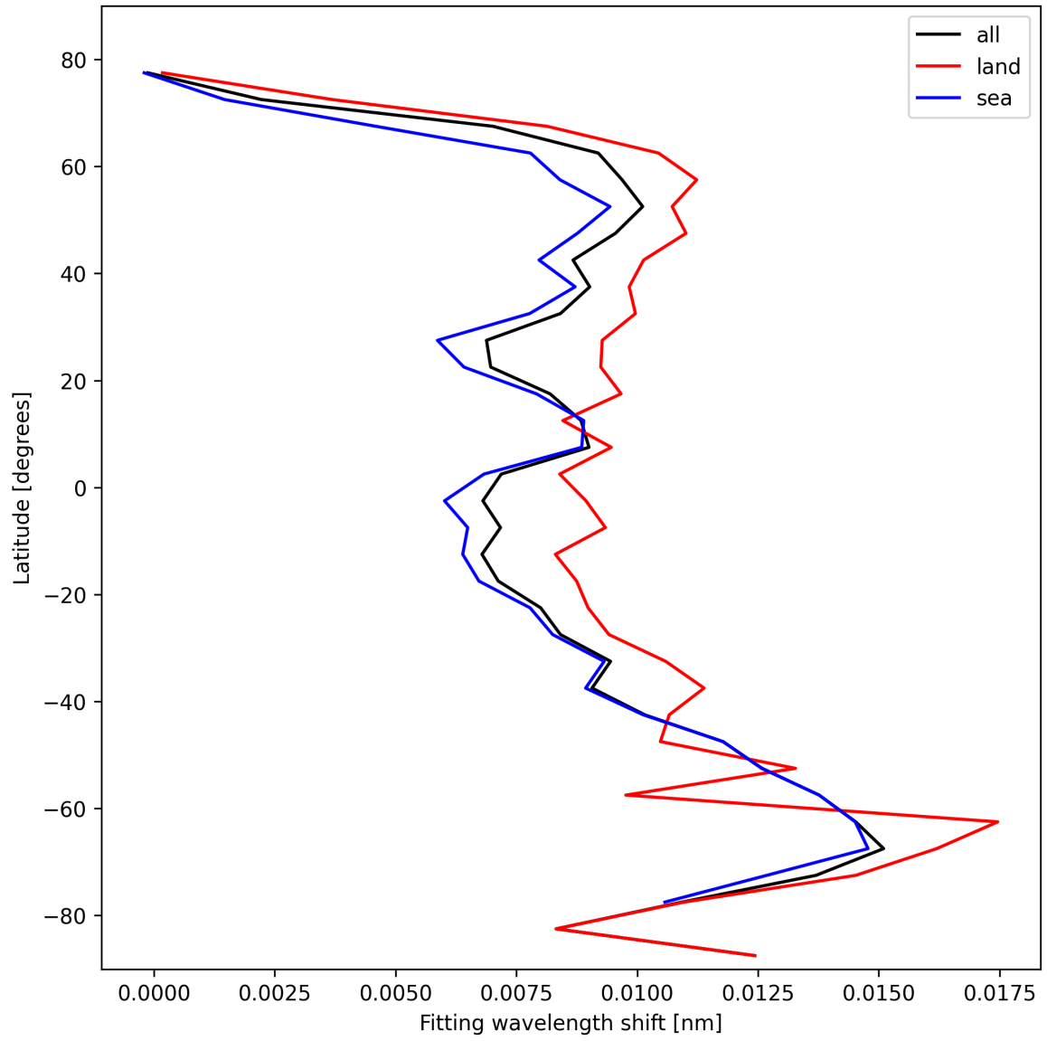
Figure 33: Zonal average of “Fitting wavelength shift” for 2024-10-19 to 2024-10-21.
