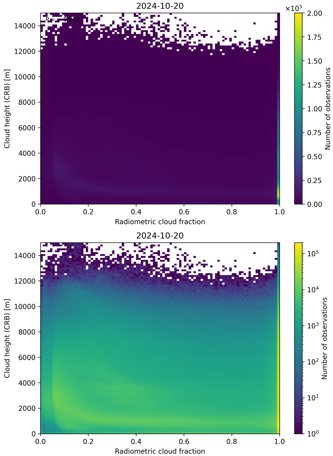
Figure 74: Scatter density plot of “Radiometric cloud fraction” against “Cloud height (CRB)” for 2024-10-19 to 2024-10-21.
