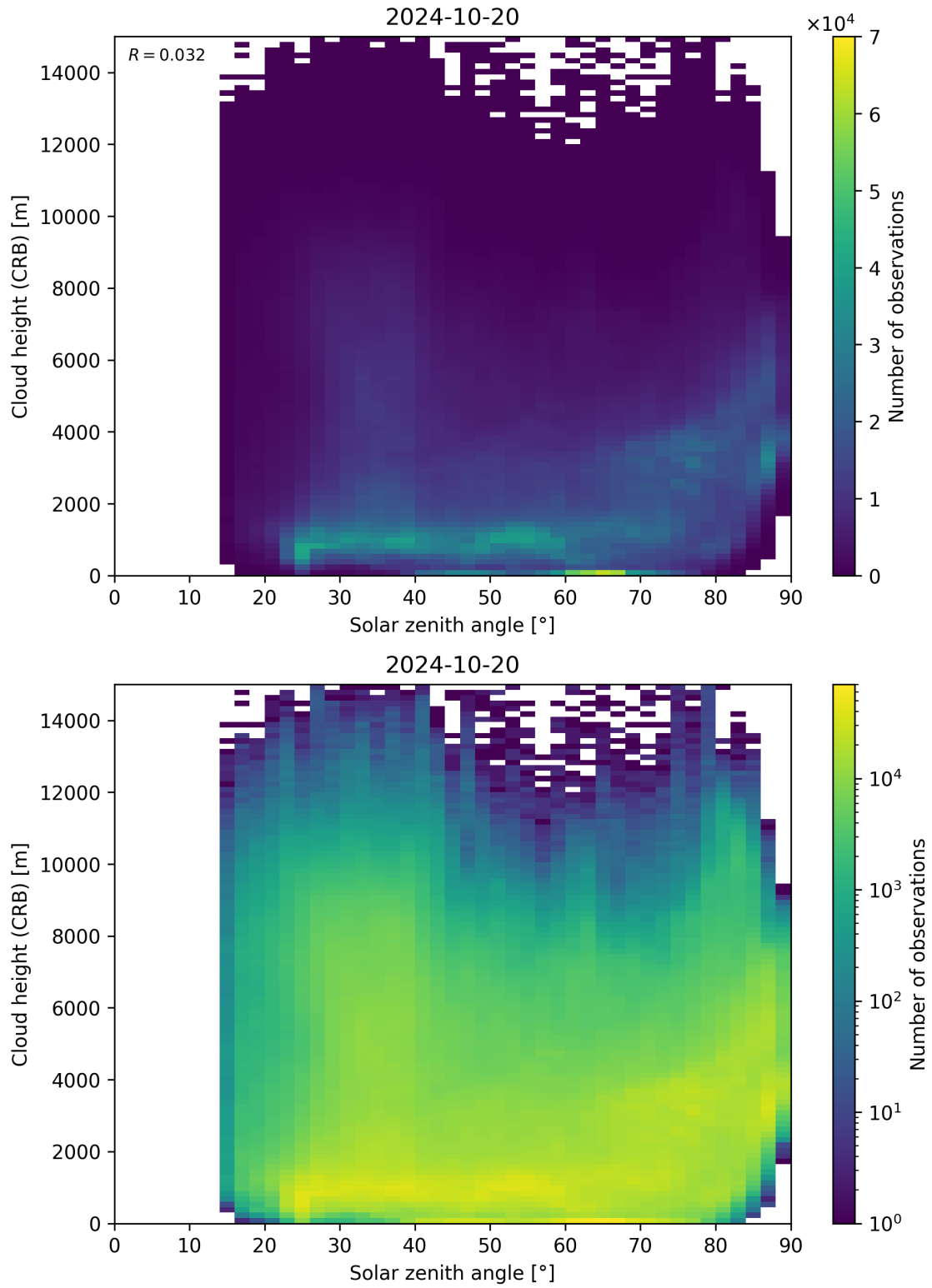
Figure 102: Scatter density plot of “Solar zenith angle” against “Cloud height (CRB)” for 2024-10-19 to 2024-10-21.
