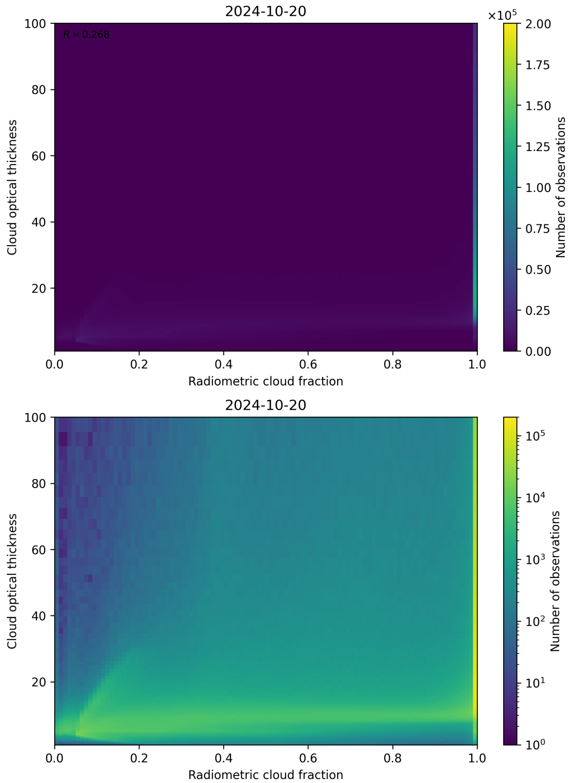
Figure 75: Scatter density plot of “Radiometric cloud fraction” against “Cloud optical thickness” for 2024-10-19 to 2024-10-21.
