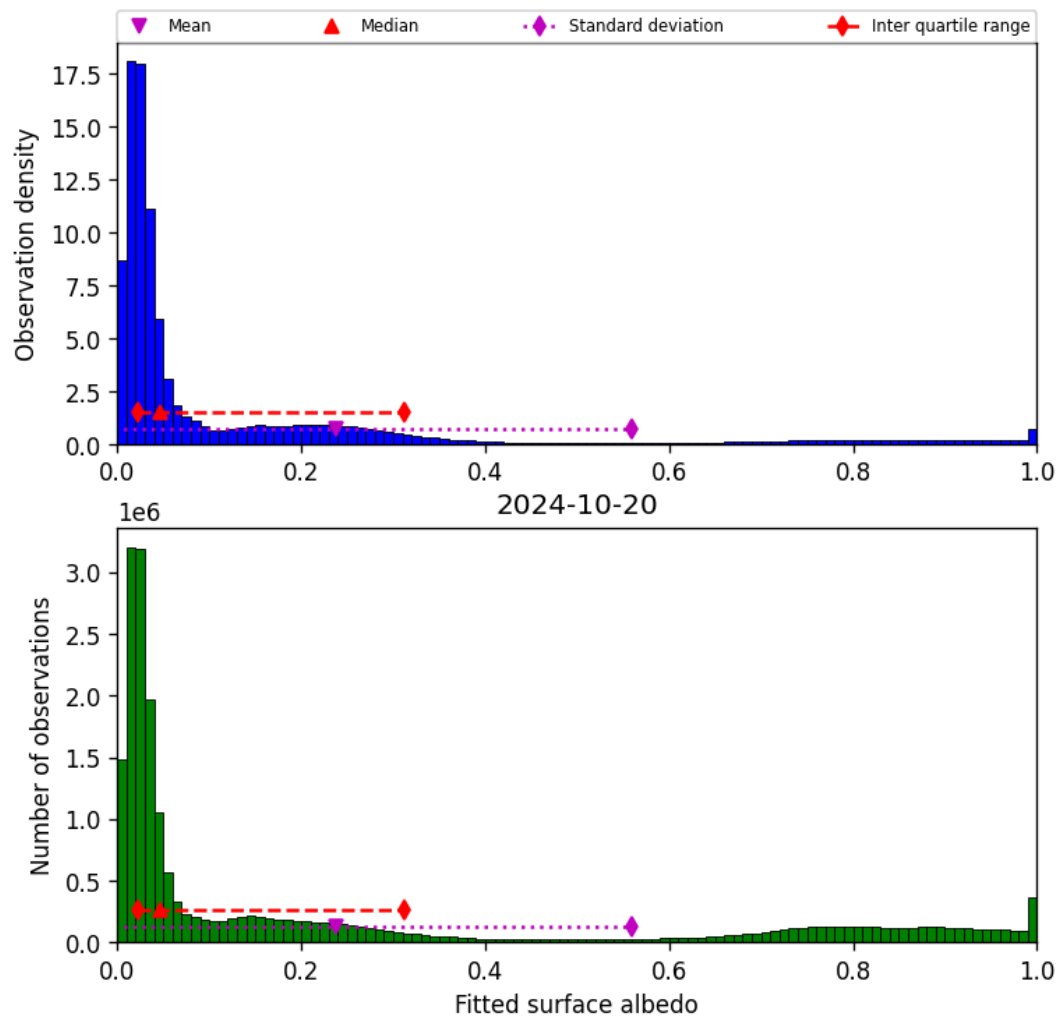
Figure 45: Histogram of “Fitted surface albedo” for 2024-10-19 to 2024-10-21
