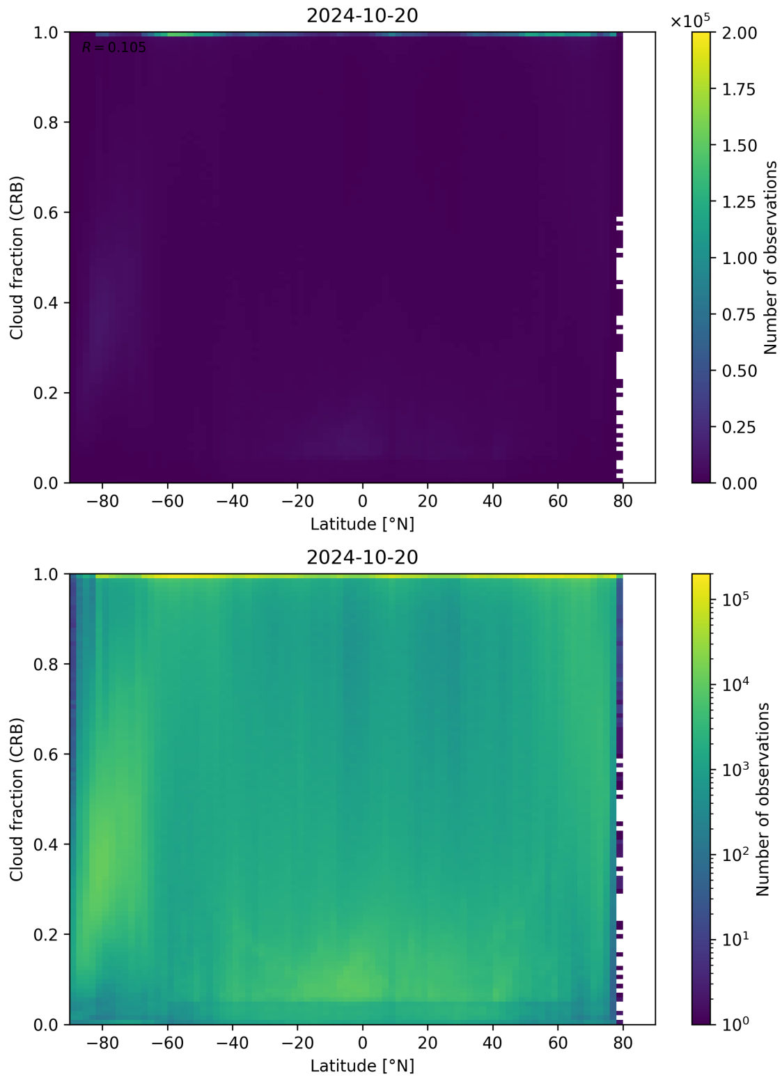
Figure 94: Scatter density plot of “Latitude” against “Cloud fraction (CRB)” for 2024-10-19 to 2024-10-21.
