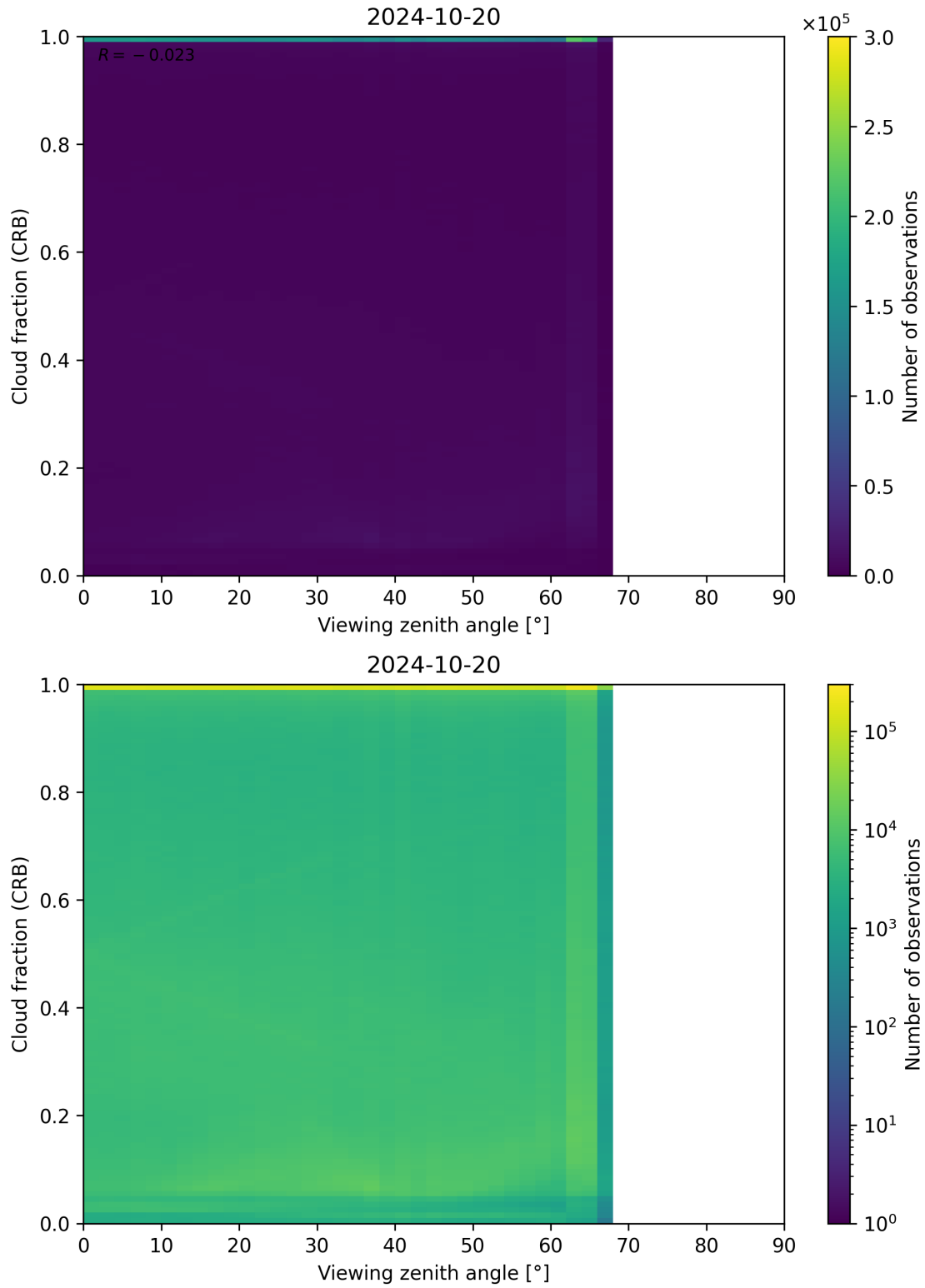
Figure 109: Scatter density plot of “Viewing zenith angle” against “Cloud fraction (CRB)” for 2024-10-19 to 2024-10-21.
