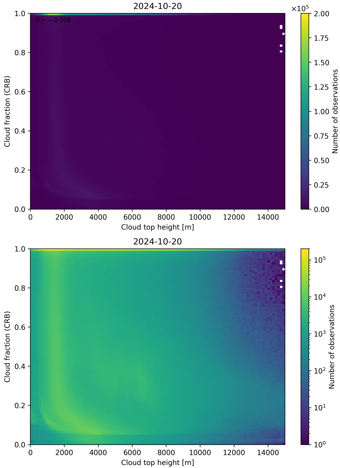
Figure 88: Scatter density plot of “Cloud top height” against “Cloud fraction (CRB)” for 2024-10-19 to 2024-10-21.
