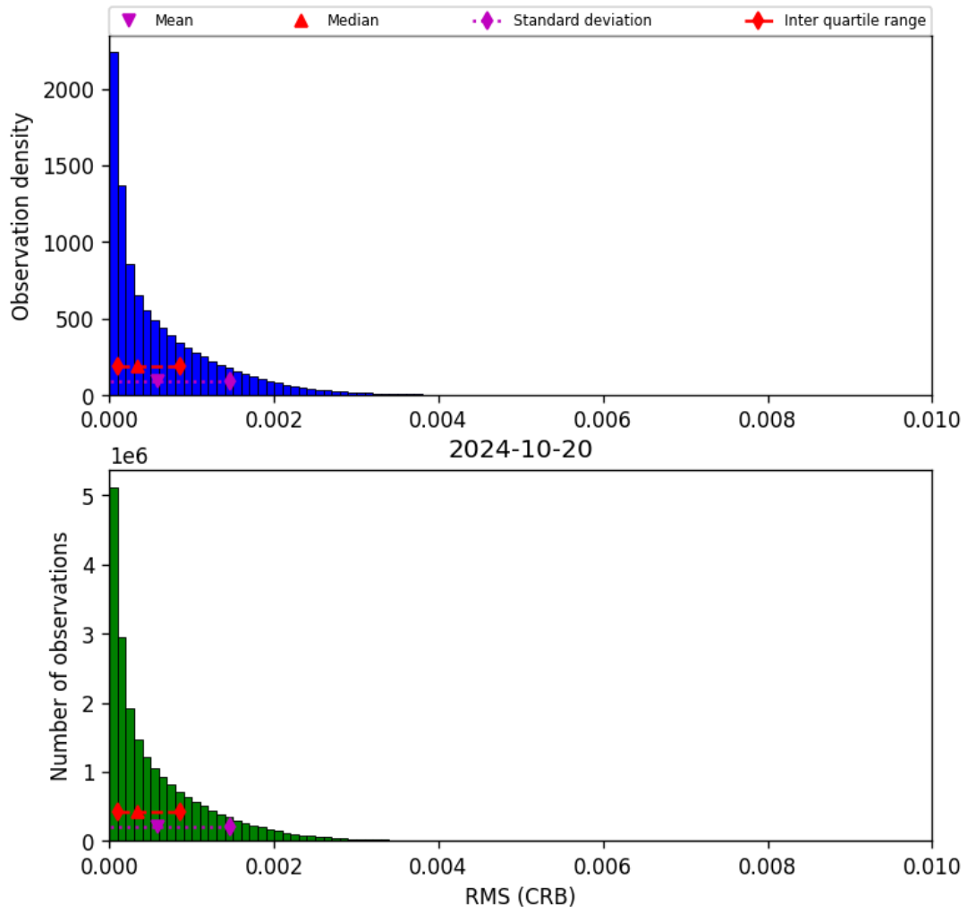
Figure 48: Histogram of “RMS (CRB)” for 2024-10-19 to 2024-10-21
