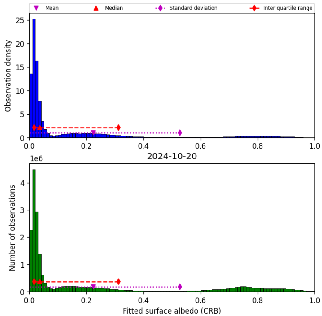
Figure 46: Histogram of “Fitted surface albedo (CRB)” for 2024-10-19 to 2024-10-21
