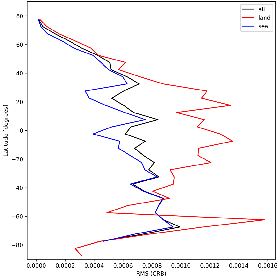
Figure 32: Zonal average of “RMS (CRB)” for 2024-10-19 to 2024-10-21.
