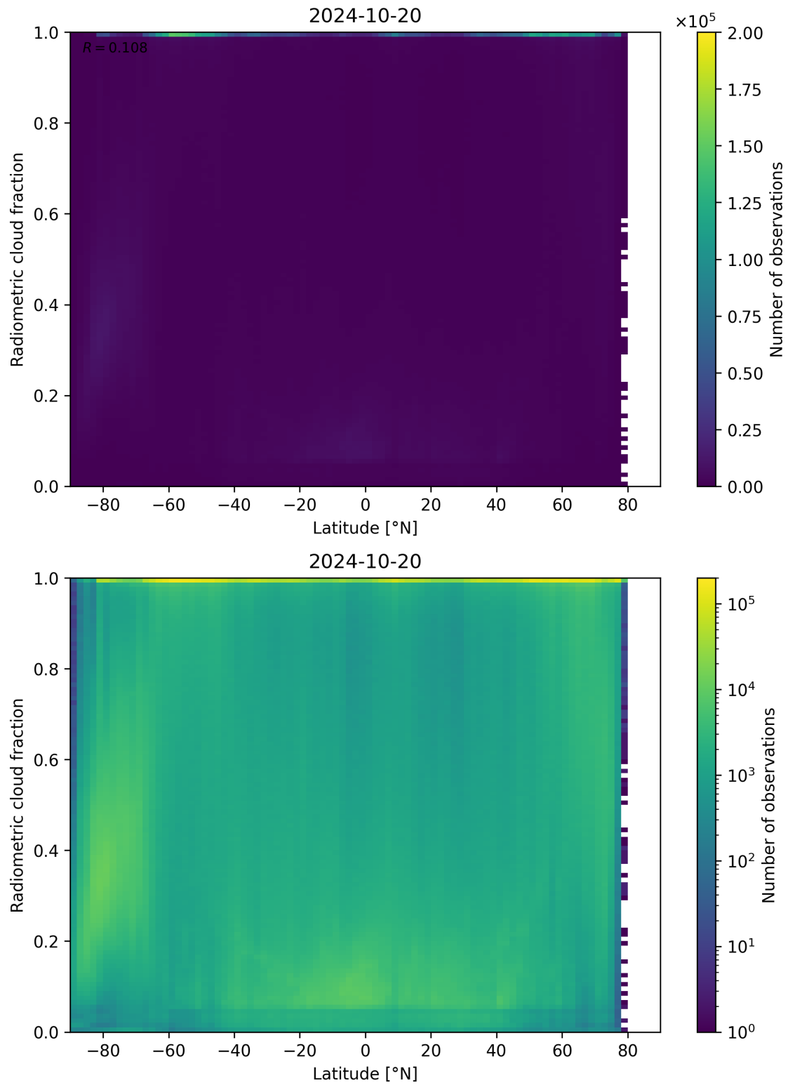
Figure 92: Scatter density plot of “Latitude” against “Radiometric cloud fraction” for 2024-10-19 to 2024-10-21.
