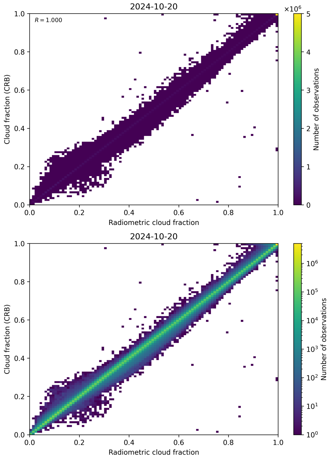
Figure 73: Scatter density plot of “Radiometric cloud fraction” against “Cloud fraction (CRB)” for 2024-10-19 to 2024-10-21.
