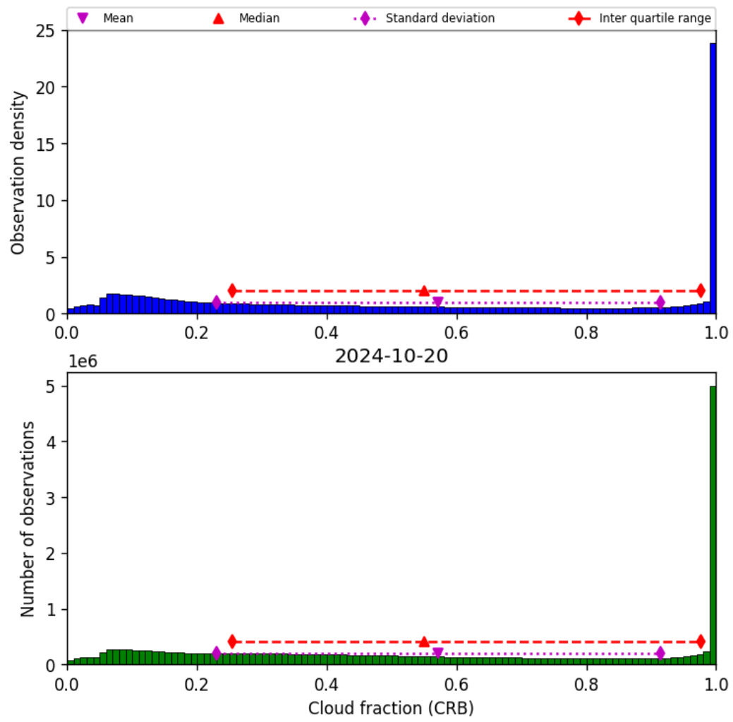
Figure 42: Histogram of “Cloud fraction (CRB)” for 2024-10-19 to 2024-10-21
