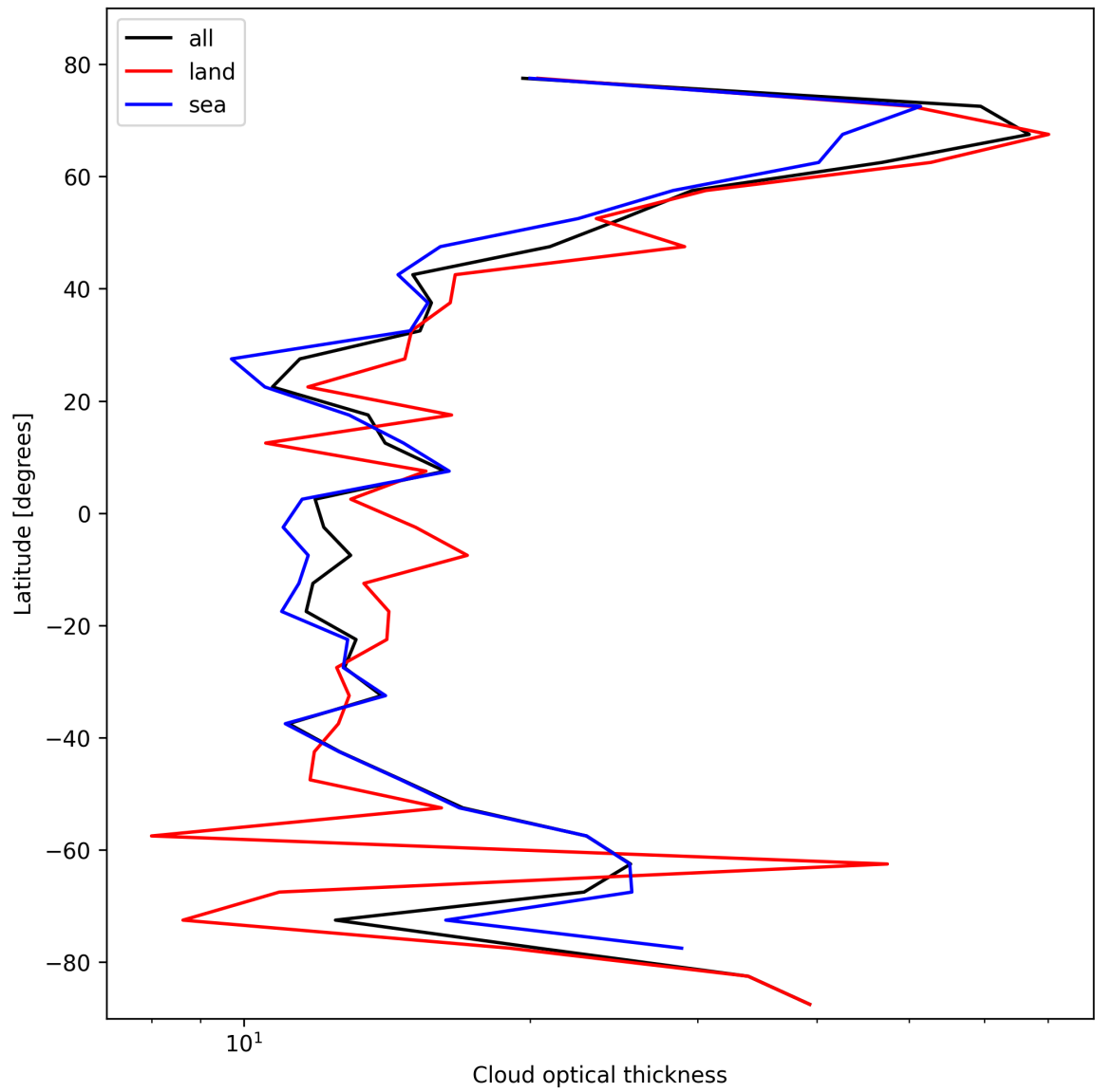
Figure 25: Zonal average of “Cloud optical thickness” for 2024-10-19 to 2024-10-21.
