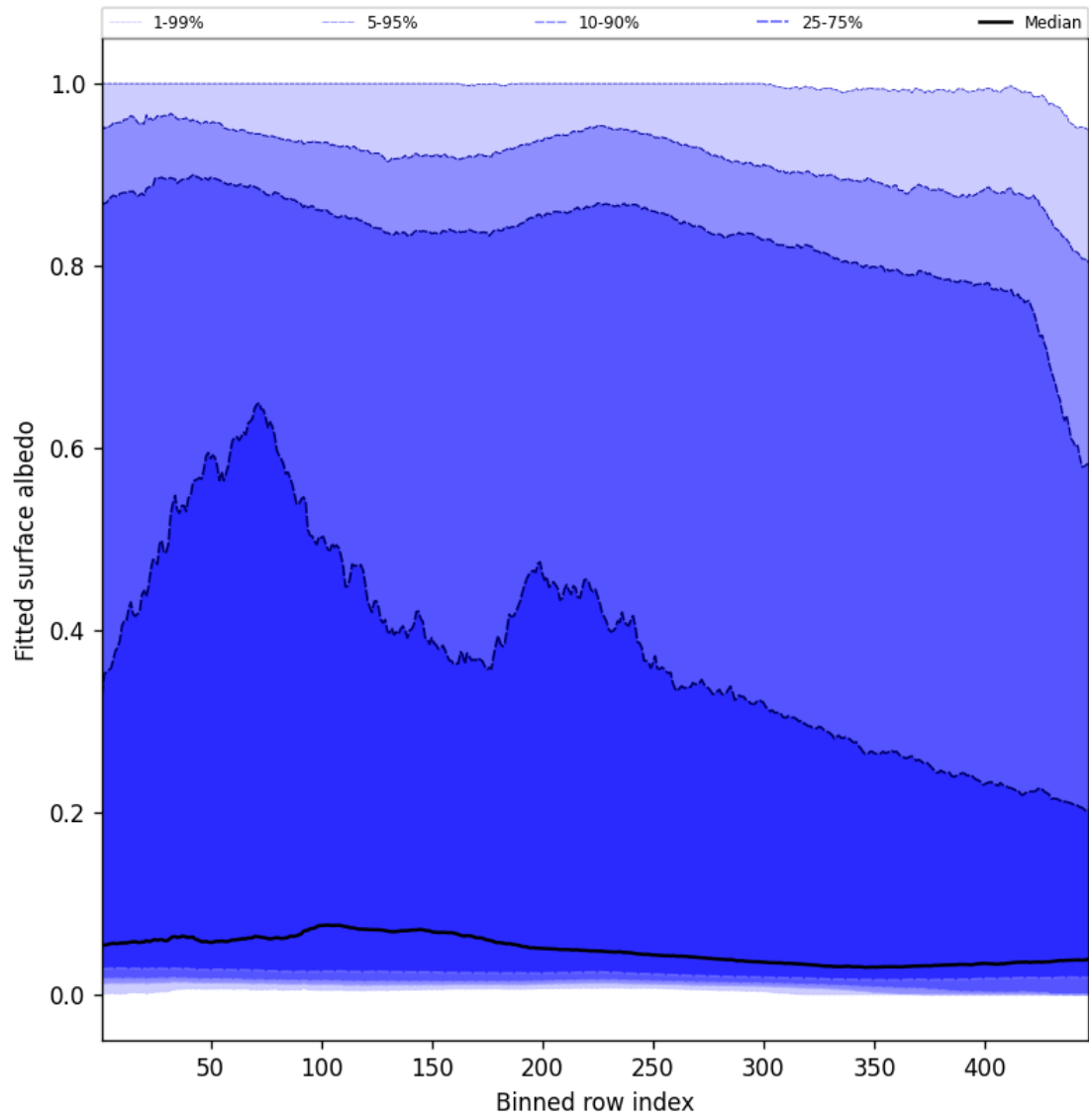
Figure 61: Along track statistics of “Fitted surface albedo” for 2024-10-19 to 2024-10-21
