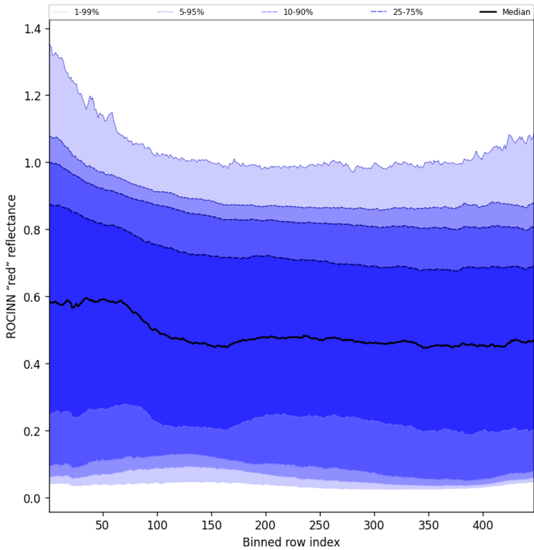
Figure 69: Along track statistics of “ROCINN “red” reflectance” for 2024-10-19 to 2024-10-21
