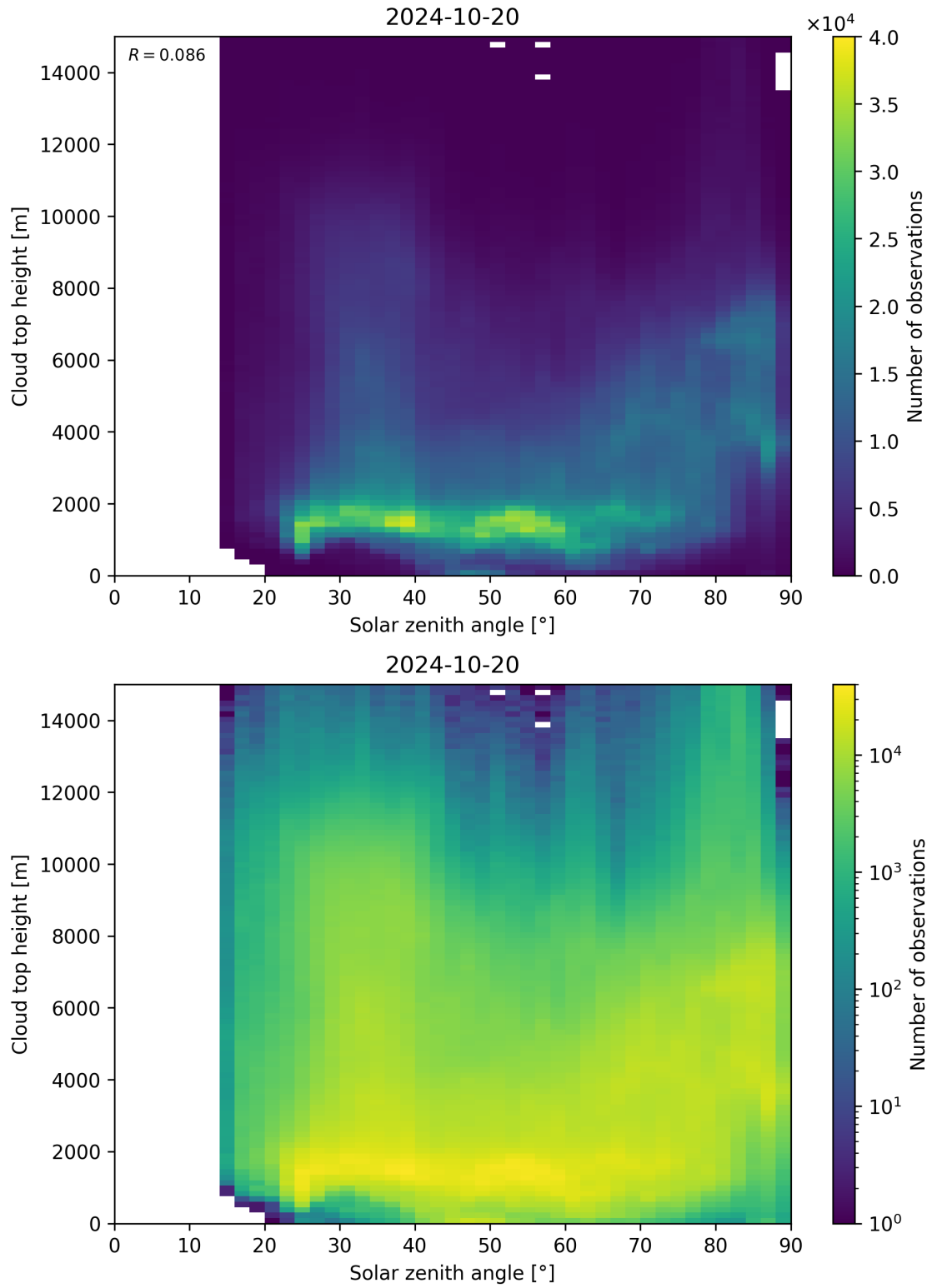
Figure 104: Scatter density plot of “Solar zenith angle” against “Cloud top height” for 2024-10-19 to 2024-10-21.
