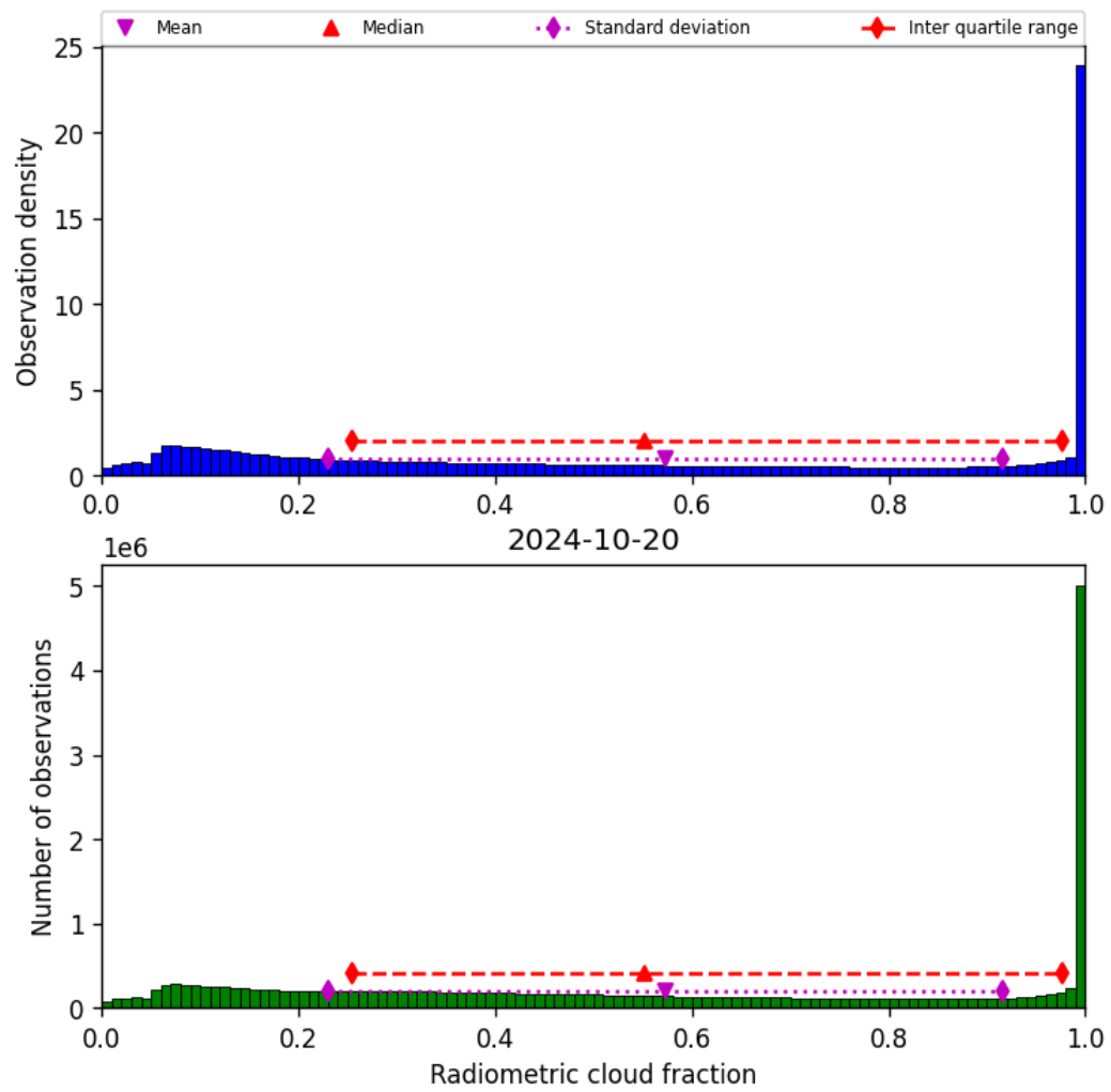
Figure 39: Histogram of “Radiometric cloud fraction” for 2024-10-19 to 2024-10-21
