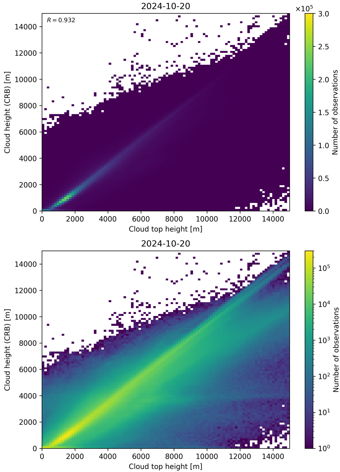
Figure 89: Scatter density plot of “Cloud top height” against “Cloud height (CRB)” for 2024-10-19 to 2024-10-21.
