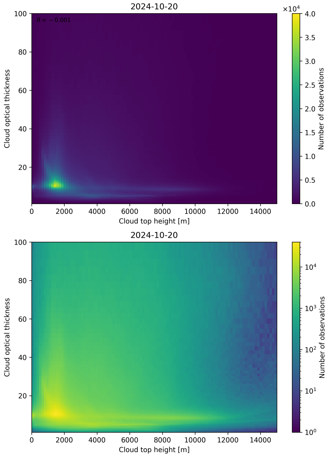
Figure 90: Scatter density plot of “Cloud top height” against “Cloud optical thickness” for 2024-10-19 to 2024-10-21.
