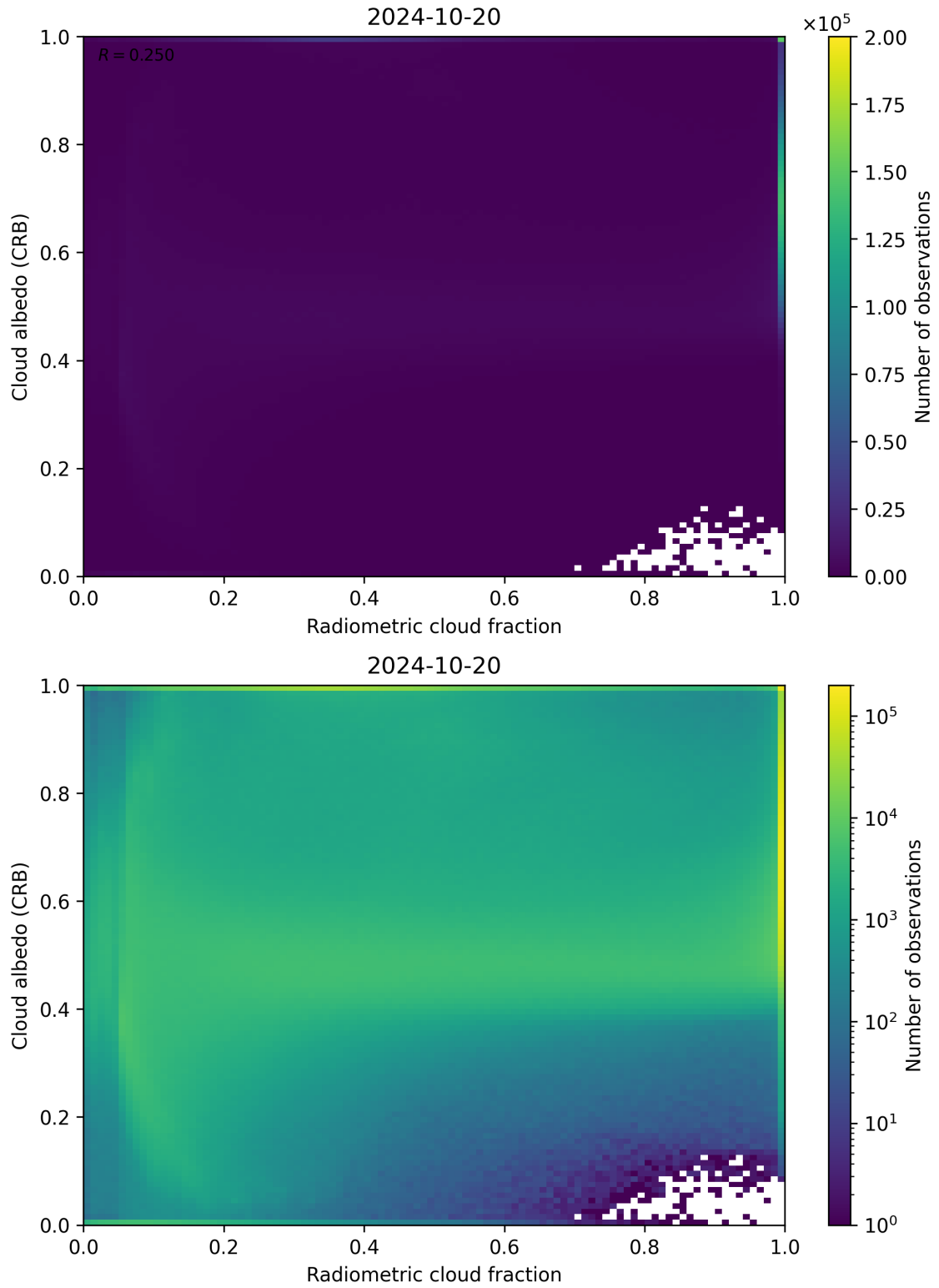
Figure 71: Scatter density plot of “Radiometric cloud fraction” against “Cloud albedo (CRB)” for 2024-10-19 to 2024-10-21.
