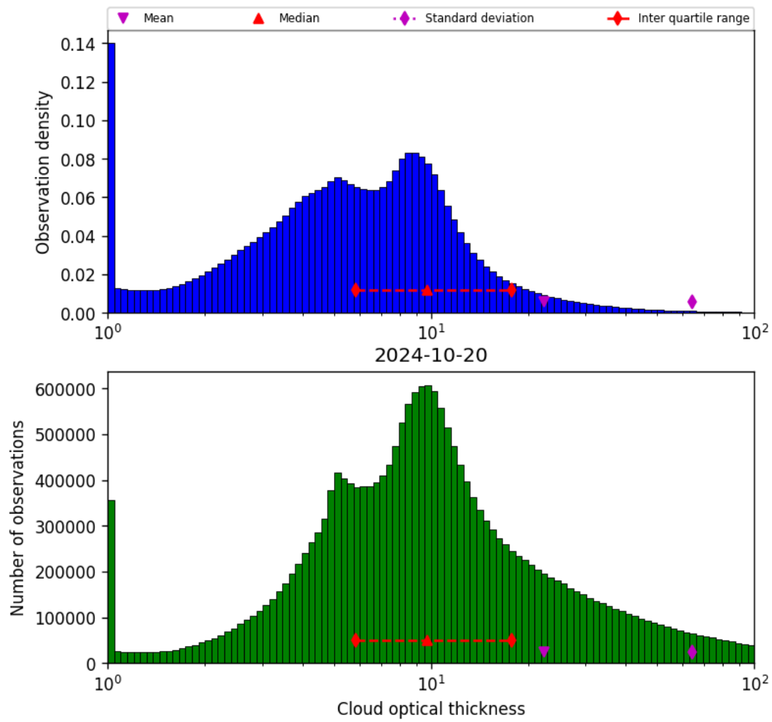
Figure 41: Histogram of “Cloud optical thickness” for 2024-10-19 to 2024-10-21
