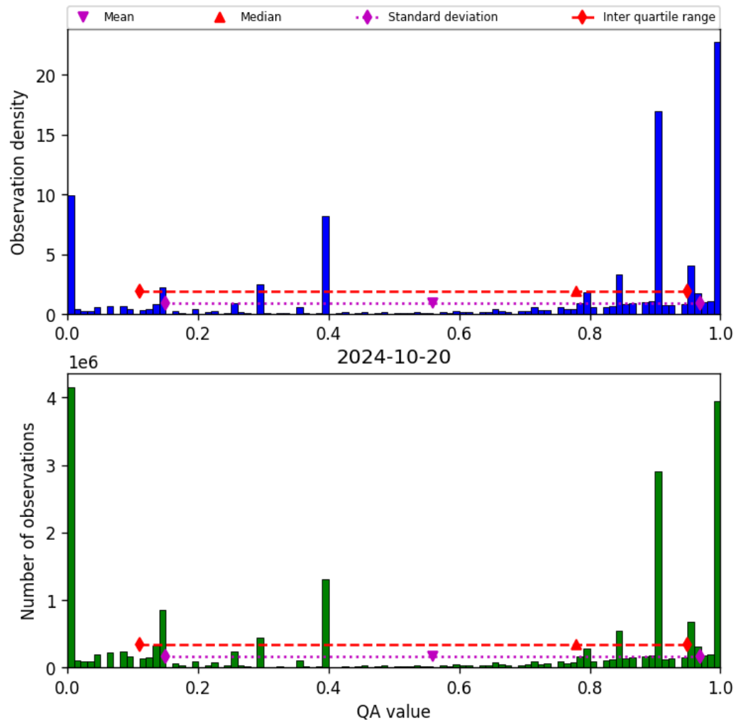
Figure 38: Histogram of “QA value” for 2024-10-19 to 2024-10-21
