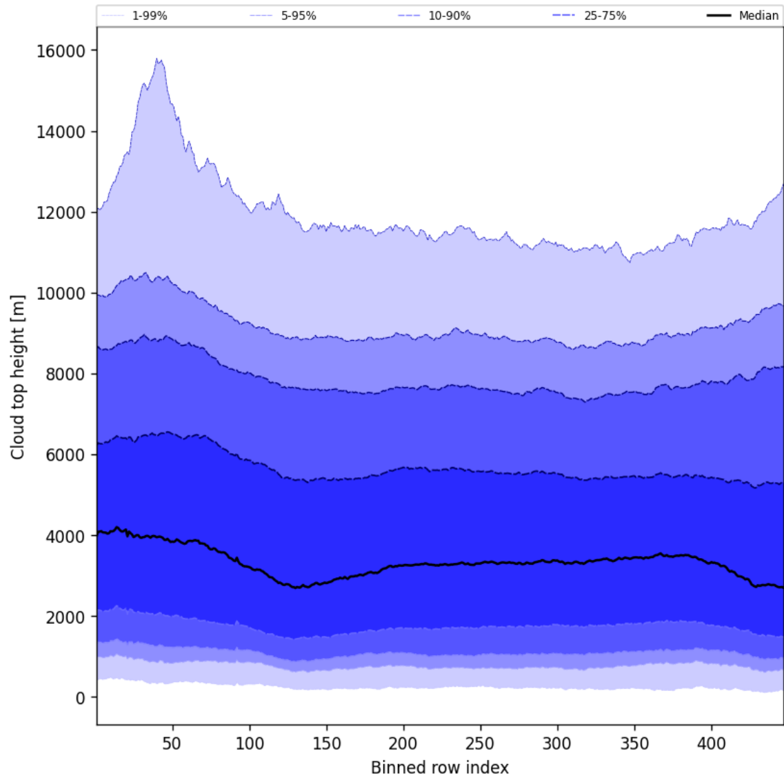
Figure 56: Along track statistics of “Cloud top height” for 2024-10-19 to 2024-10-21
