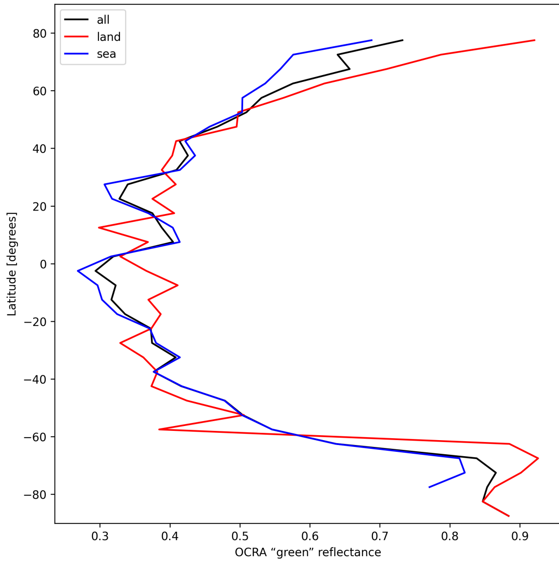
Figure 36: Zonal average of “OCRA “green” reflectance” for 2024-10-19 to 2024-10-21.
