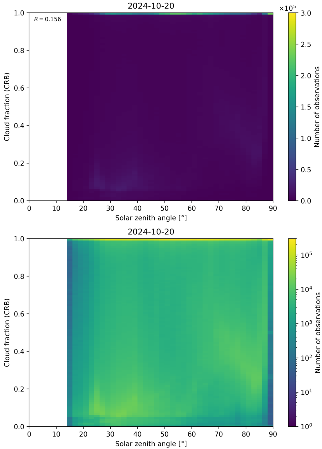
Figure 101: Scatter density plot of “Solar zenith angle” against “Cloud fraction (CRB)” for 2024-10-19 to 2024-10-21.
