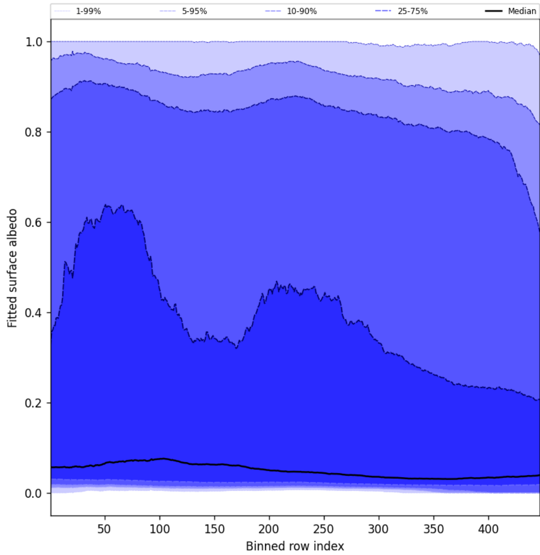
Figure 61: Along track statistics of “Fitted surface albedo” for 2024-10-20 to 2024-10-22
