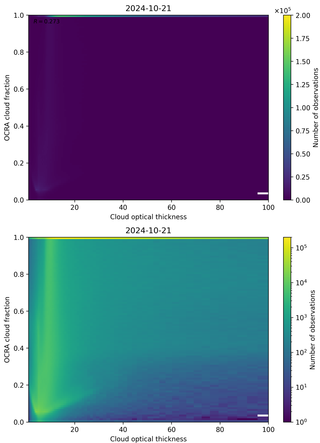
Figure 83: Scatter density plot of “Cloud optical thickness” against “OCRA cloud fraction” for 2024-10-20 to 2024-10-22.
