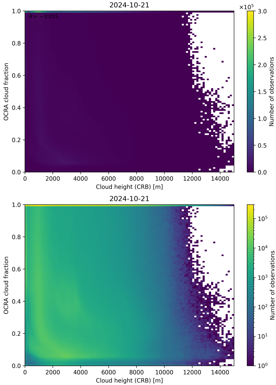
Figure 81: Scatter density plot of “Cloud height (CRB)” against “OCRA cloud fraction” for 2024-10-20 to 2024-10-22.
