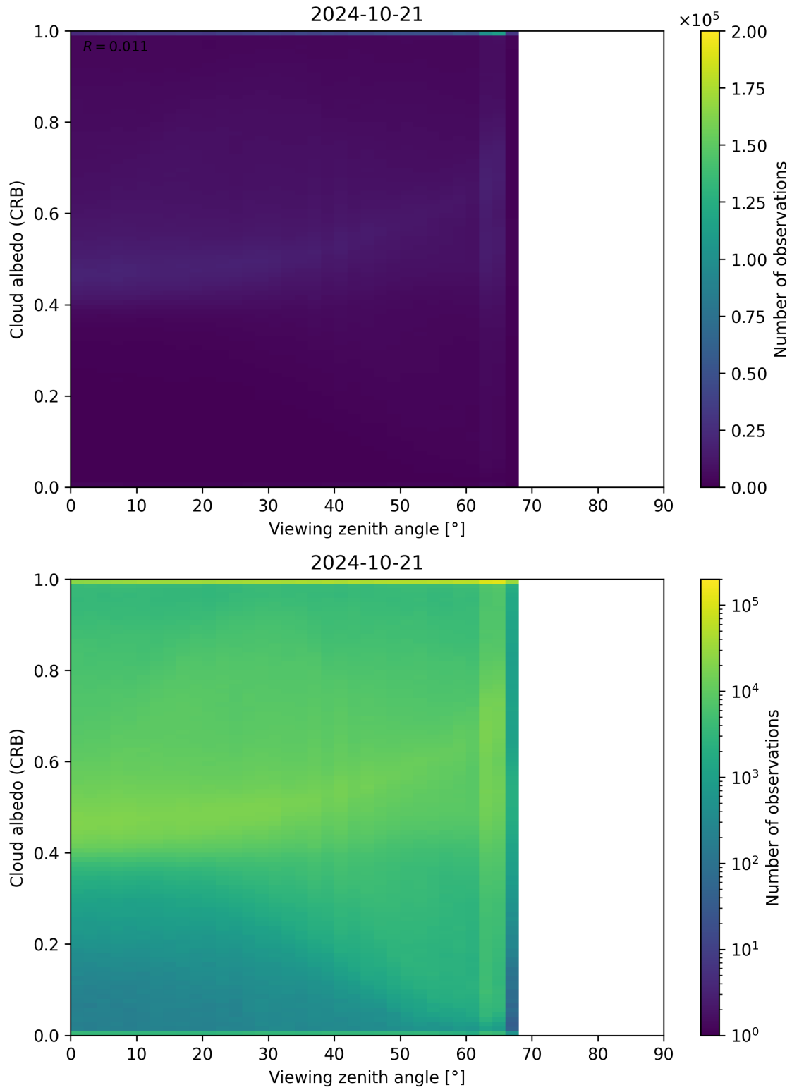
Figure 106: Scatter density plot of “Viewing zenith angle” against “Cloud albedo (CRB)” for 2024-10-20 to 2024-10-22.
