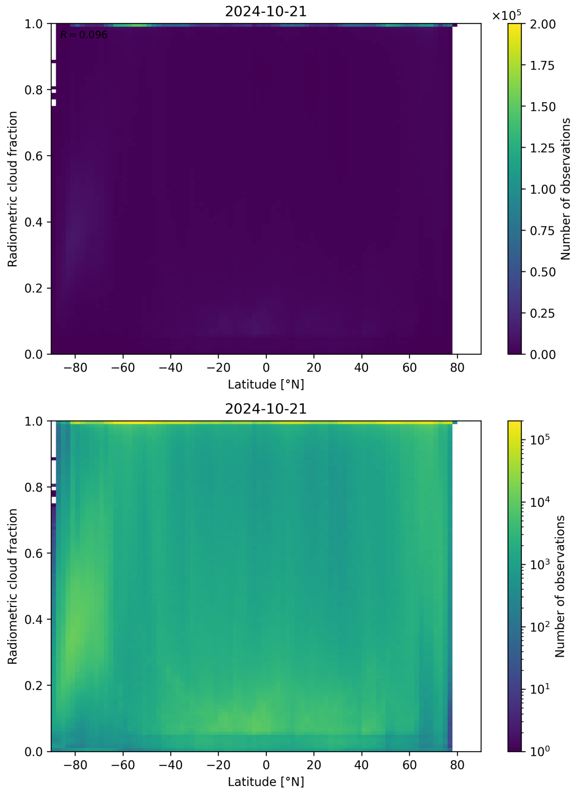
Figure 92: Scatter density plot of “Latitude” against “Radiometric cloud fraction” for 2024-10-20 to 2024-10-22.
