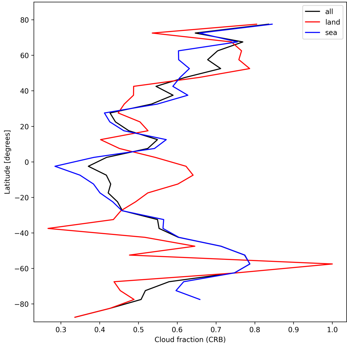
Figure 26: Zonal average of “Cloud fraction (CRB)” for 2024-10-20 to 2024-10-22.
