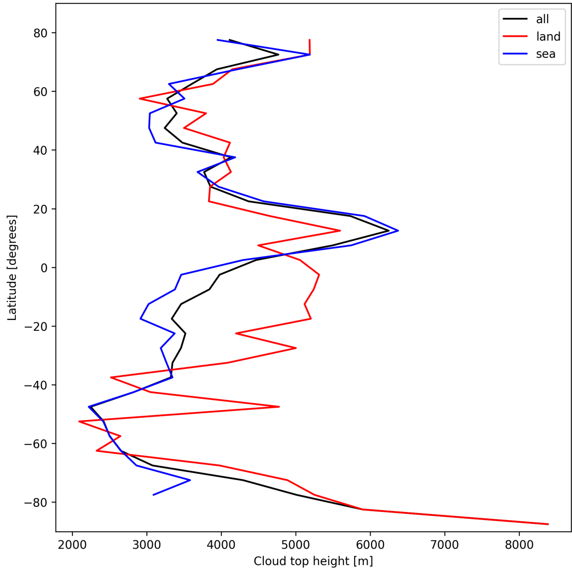
Figure 24: Zonal average of “Cloud top height” for 2024-10-20 to 2024-10-22.
