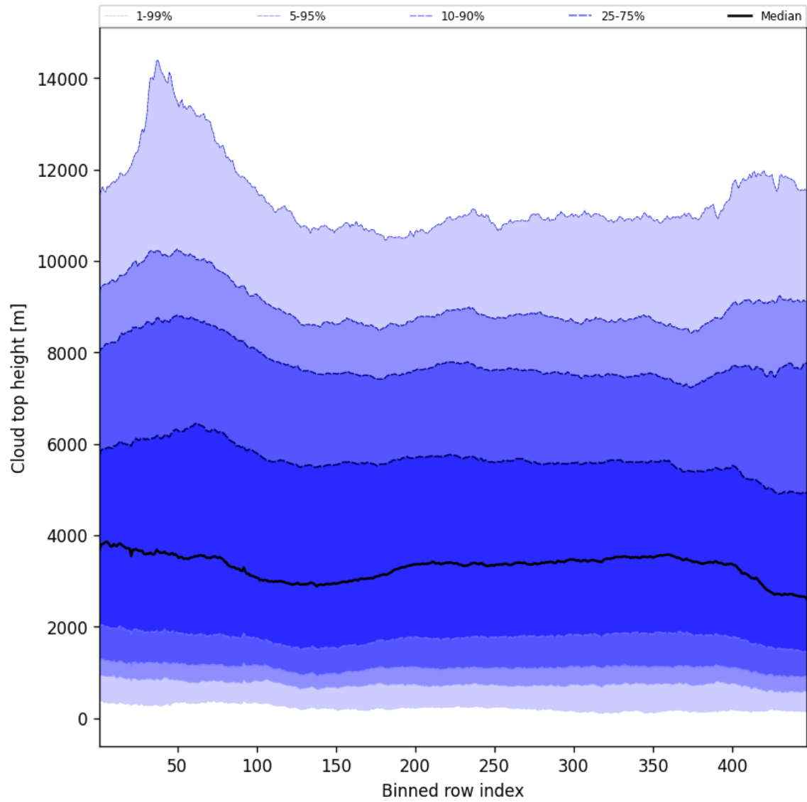
Figure 56: Along track statistics of “Cloud top height” for 2024-10-20 to 2024-10-22
