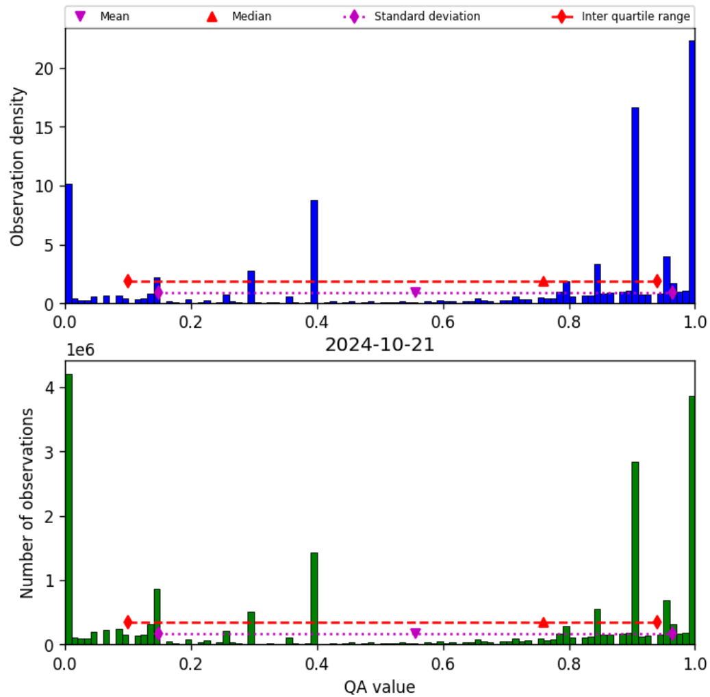
Figure 38: Histogram of “QA value” for 2024-10-20 to 2024-10-22
