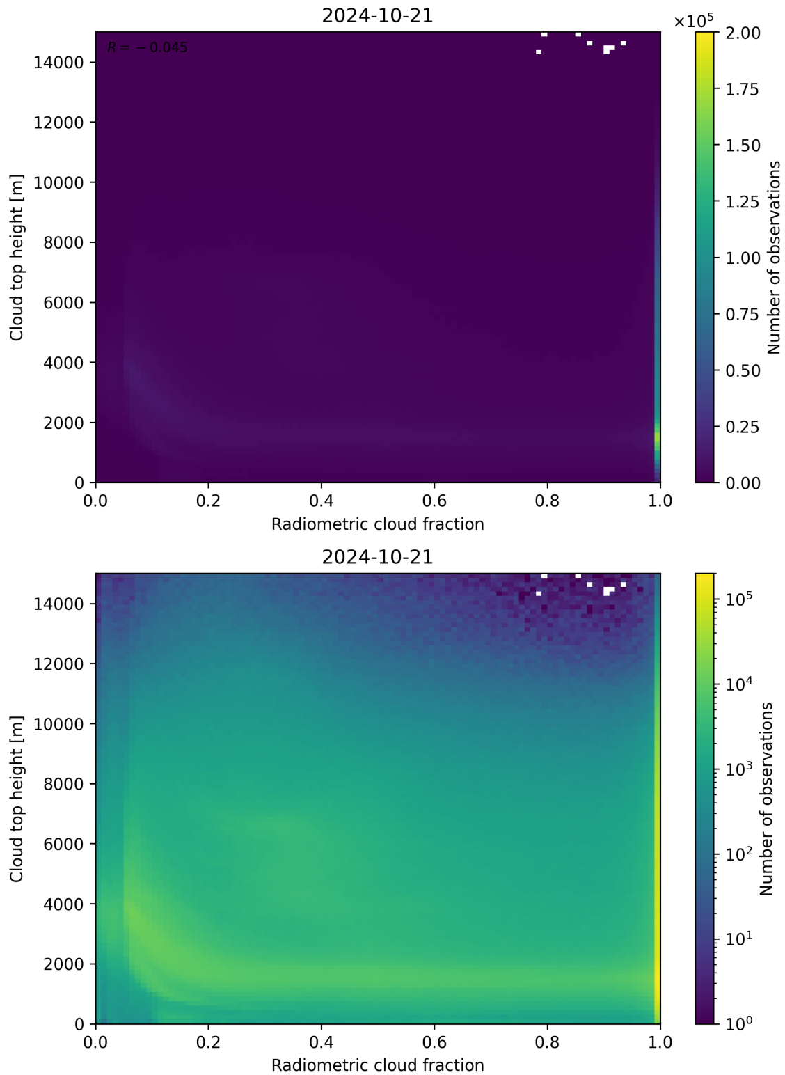
Figure 76: Scatter density plot of “Radiometric cloud fraction” against “Cloud top height” for 2024-10-20 to 2024-10-22.
