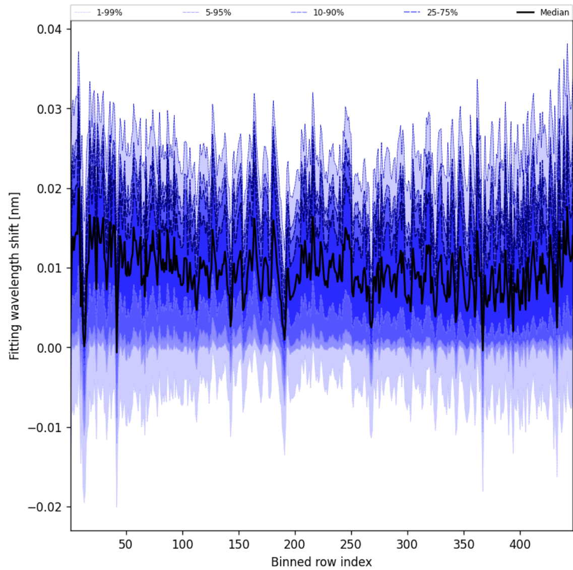
Figure 65: Along track statistics of “Fitting wavelength shift” for 2024-10-20 to 2024-10-22
