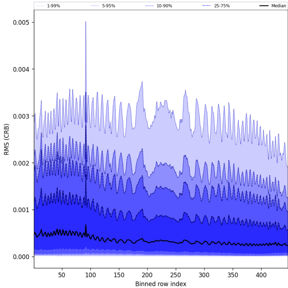
Figure 64: Along track statistics of “RMS (CRB)” for 2024-10-20 to 2024-10-22
