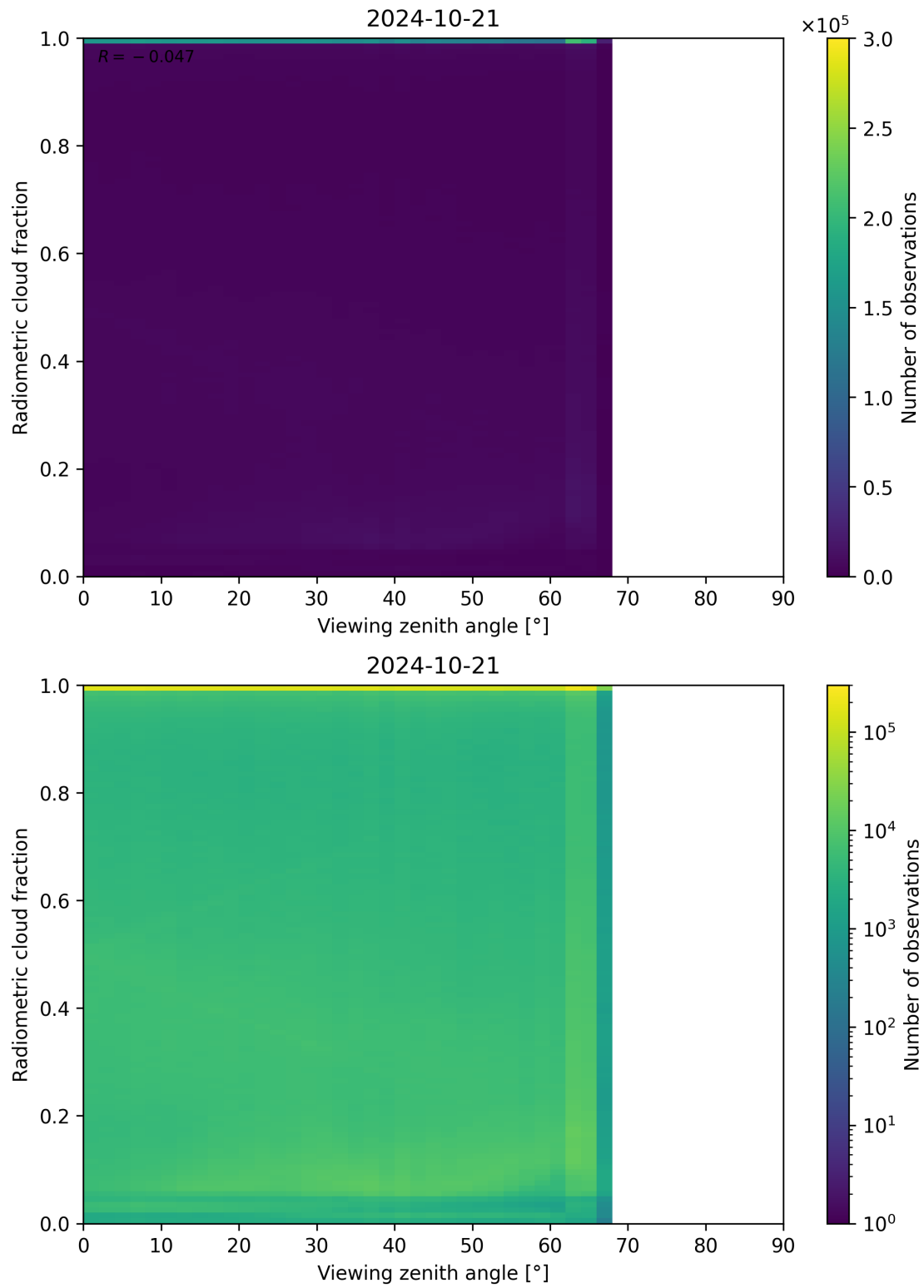
Figure 107: Scatter density plot of “Viewing zenith angle” against “Radiometric cloud fraction” for 2024-10-20 to 2024-10-22.
