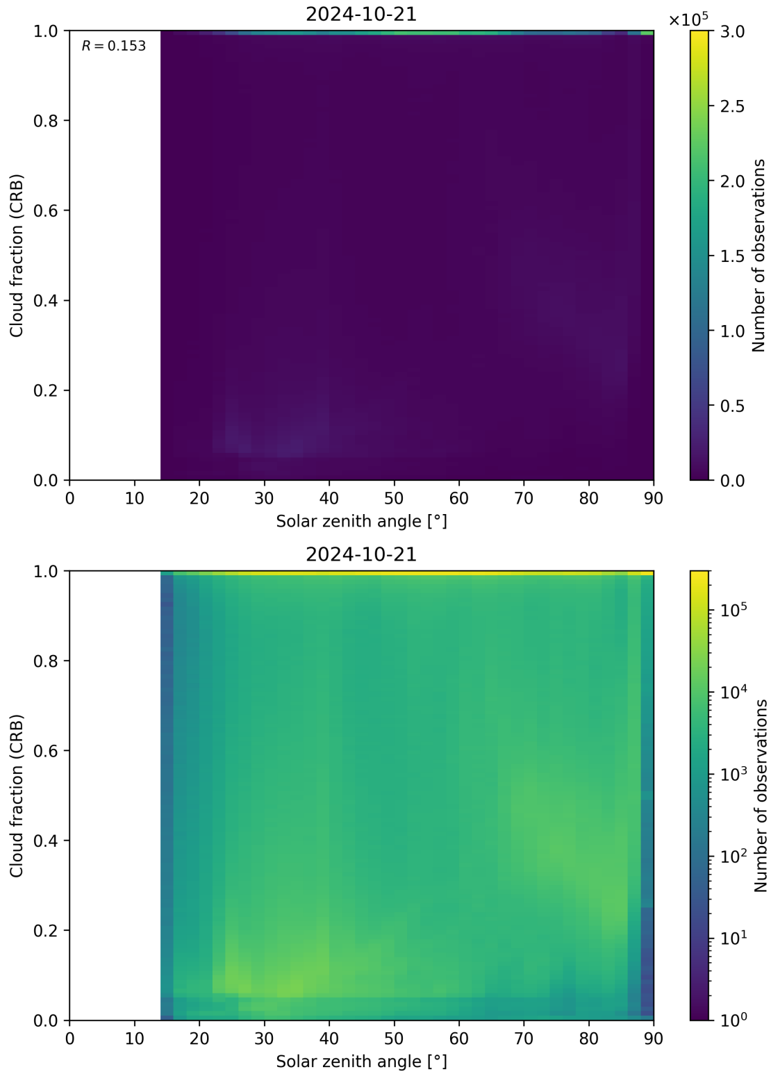
Figure 101: Scatter density plot of “Solar zenith angle” against “Cloud fraction (CRB)” for 2024-10-20 to 2024-10-22.
