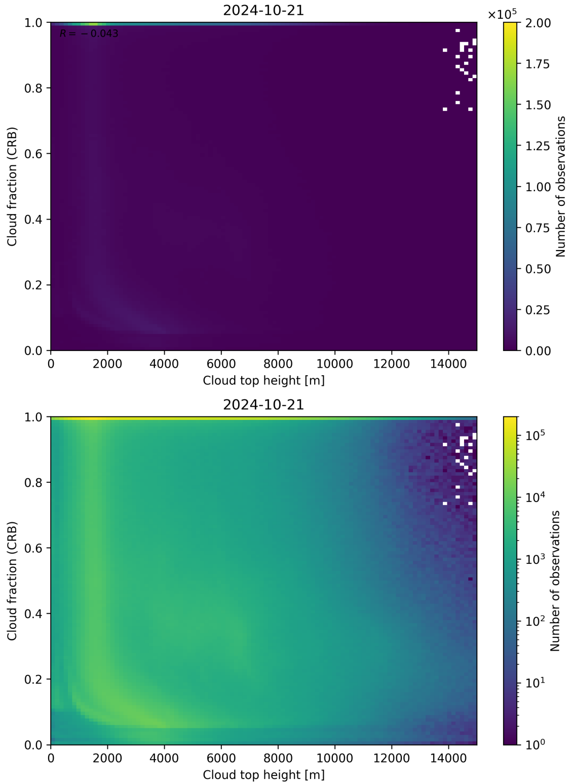
Figure 88: Scatter density plot of “Cloud top height” against “Cloud fraction (CRB)” for 2024-10-20 to 2024-10-22.
