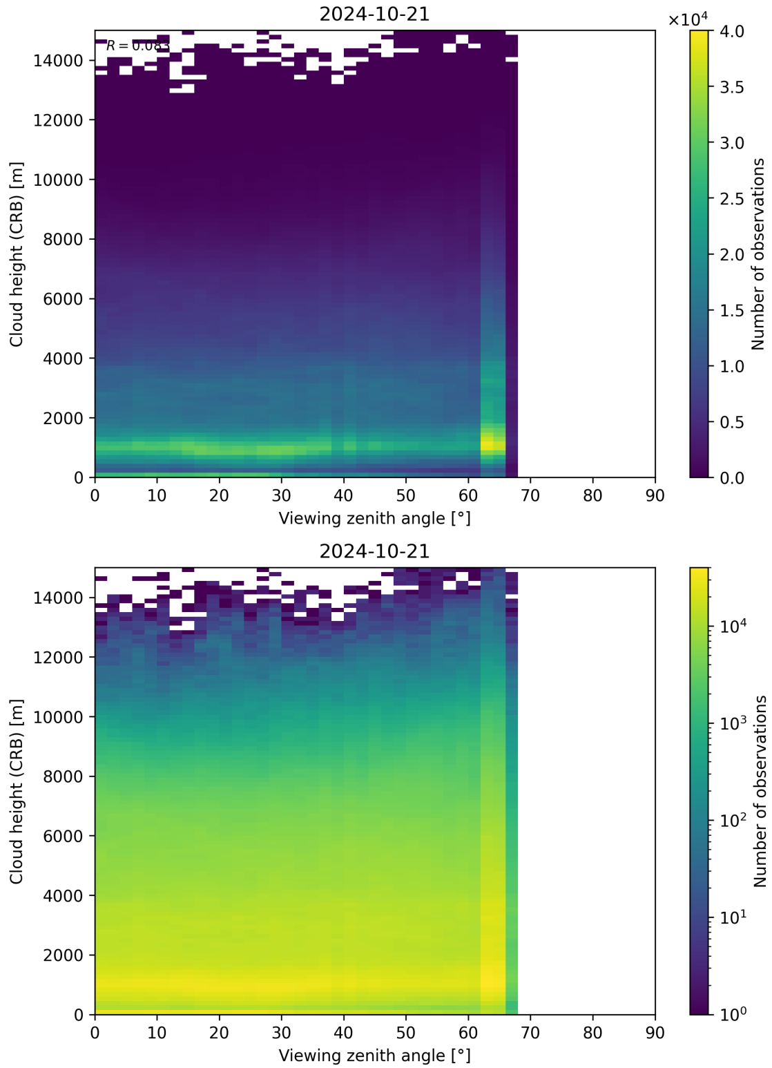
Figure 110: Scatter density plot of “Viewing zenith angle” against “Cloud height (CRB)” for 2024-10-20 to 2024-10-22.
