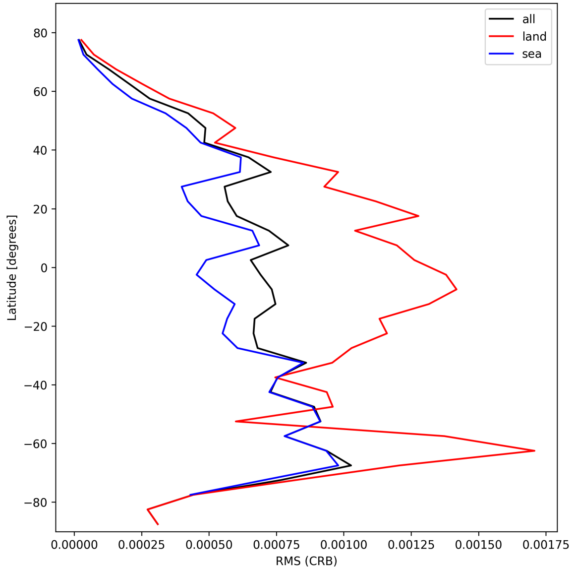
Figure 32: Zonal average of “RMS (CRB)” for 2024-10-20 to 2024-10-22.
