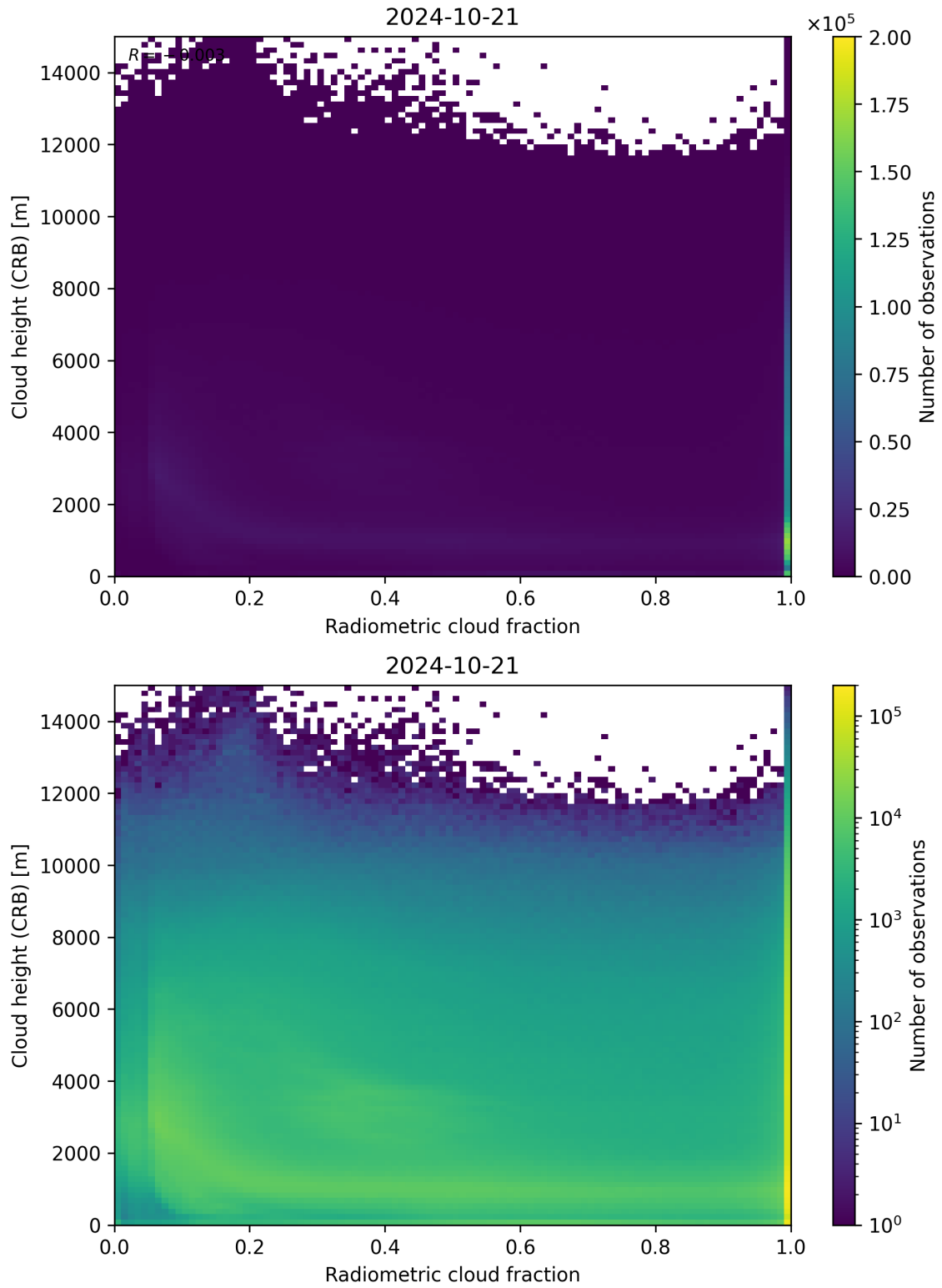
Figure 74: Scatter density plot of “Radiometric cloud fraction” against “Cloud height (CRB)” for 2024-10-20 to 2024-10-22.
