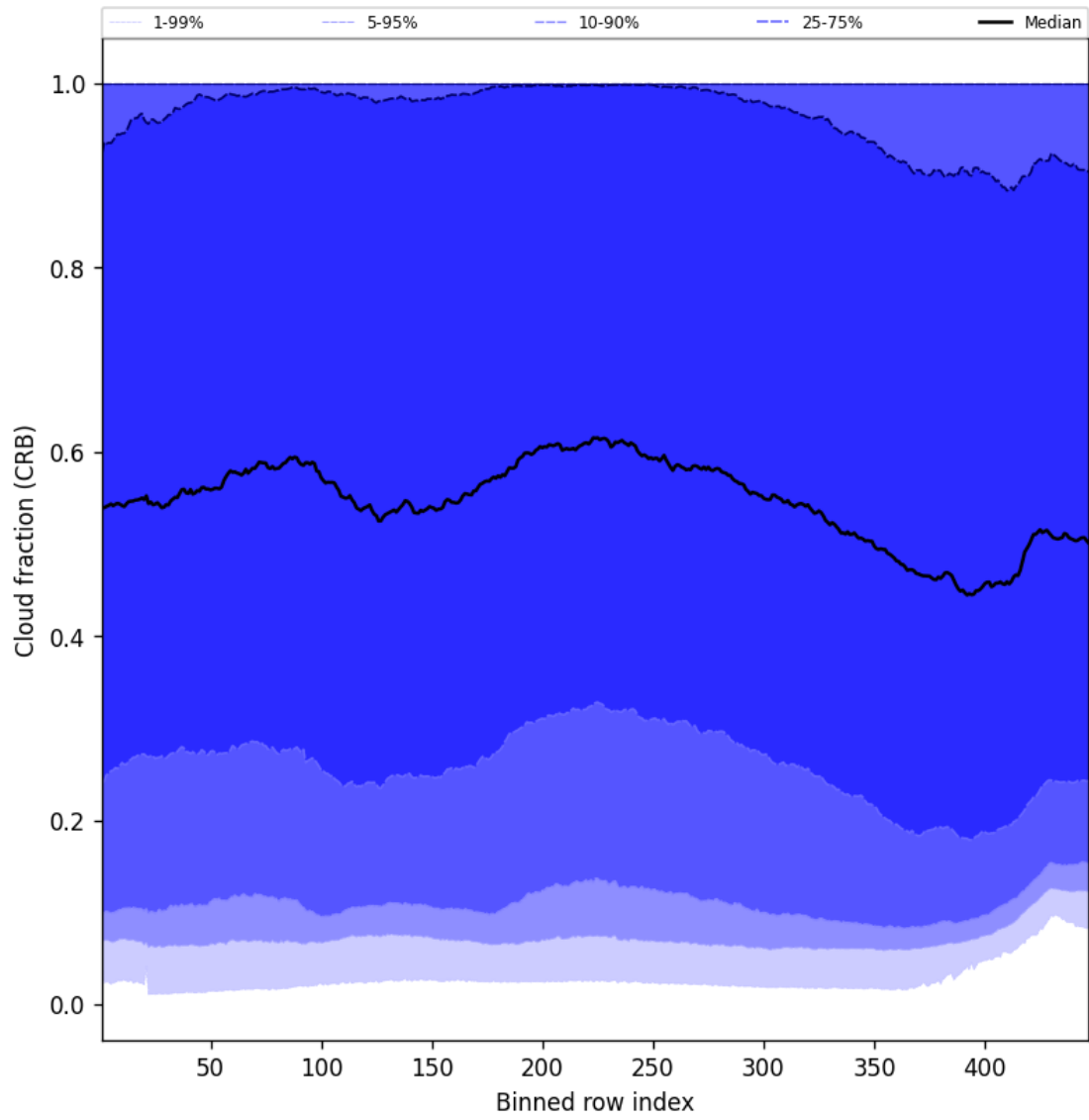
Figure 58: Along track statistics of “Cloud fraction (CRB)” for 2024-10-20 to 2024-10-22
