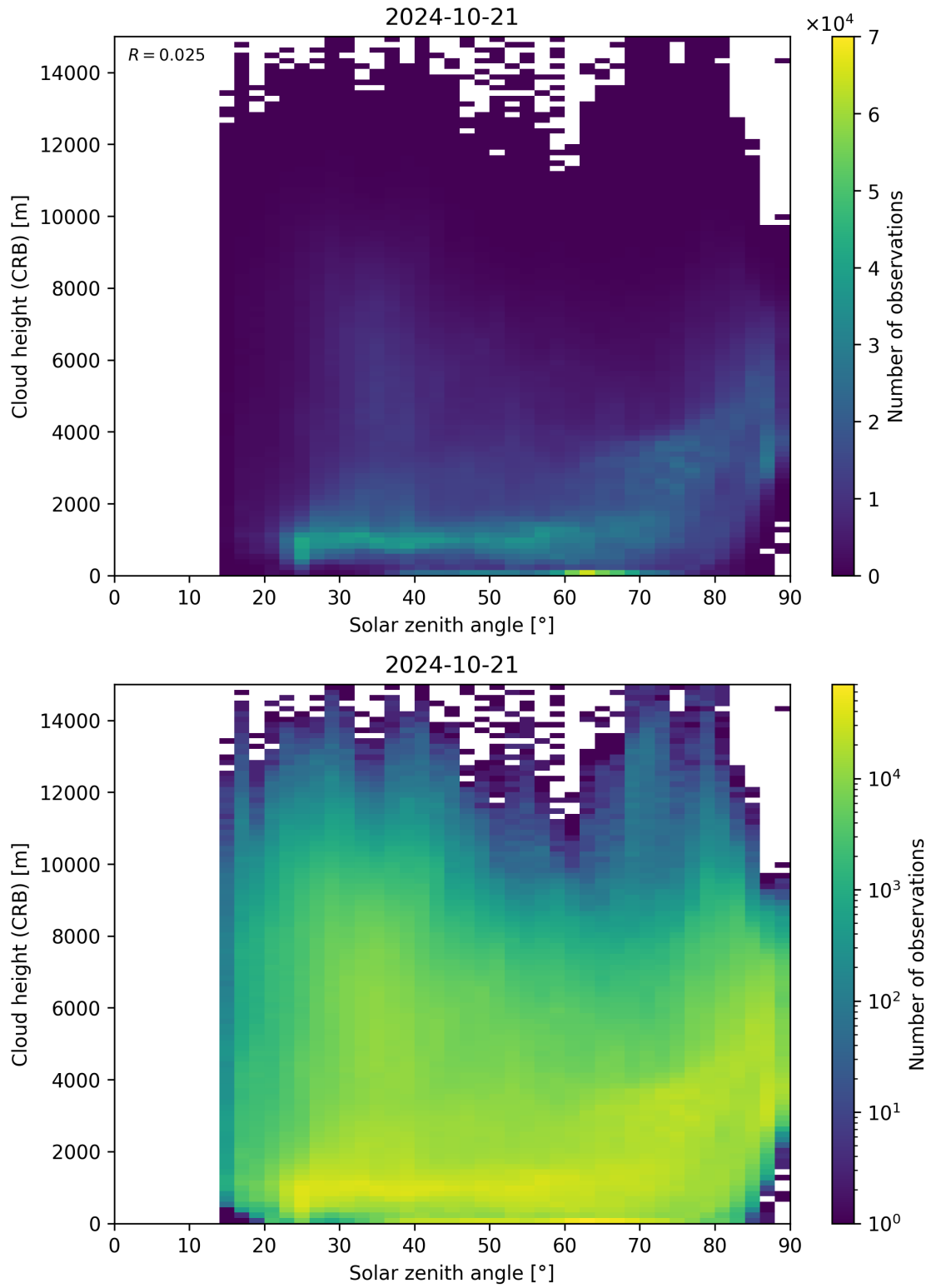
Figure 102: Scatter density plot of “Solar zenith angle” against “Cloud height (CRB)” for 2024-10-20 to 2024-10-22.
