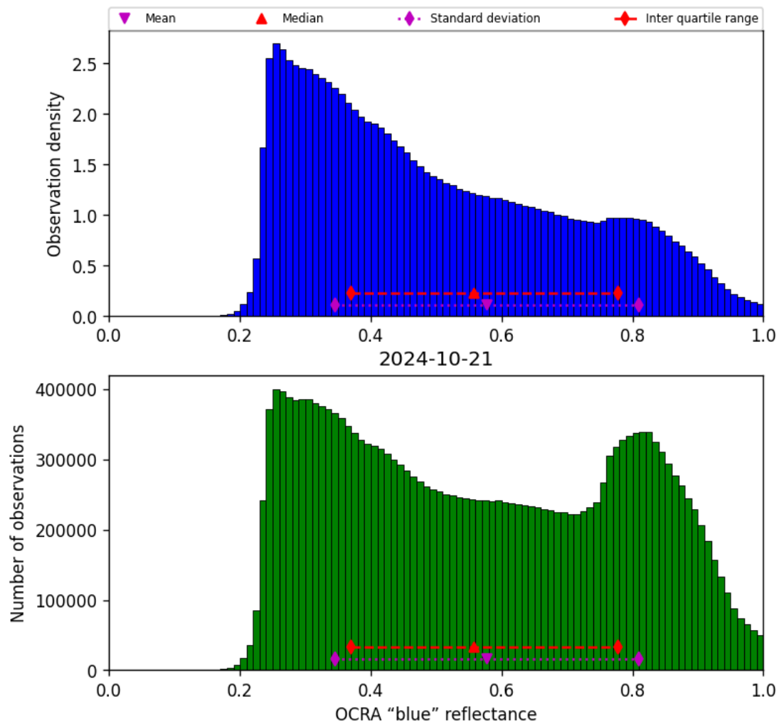
Figure 51: Histogram of “OCRA “blue” reflectance” for 2024-10-20 to 2024-10-22
