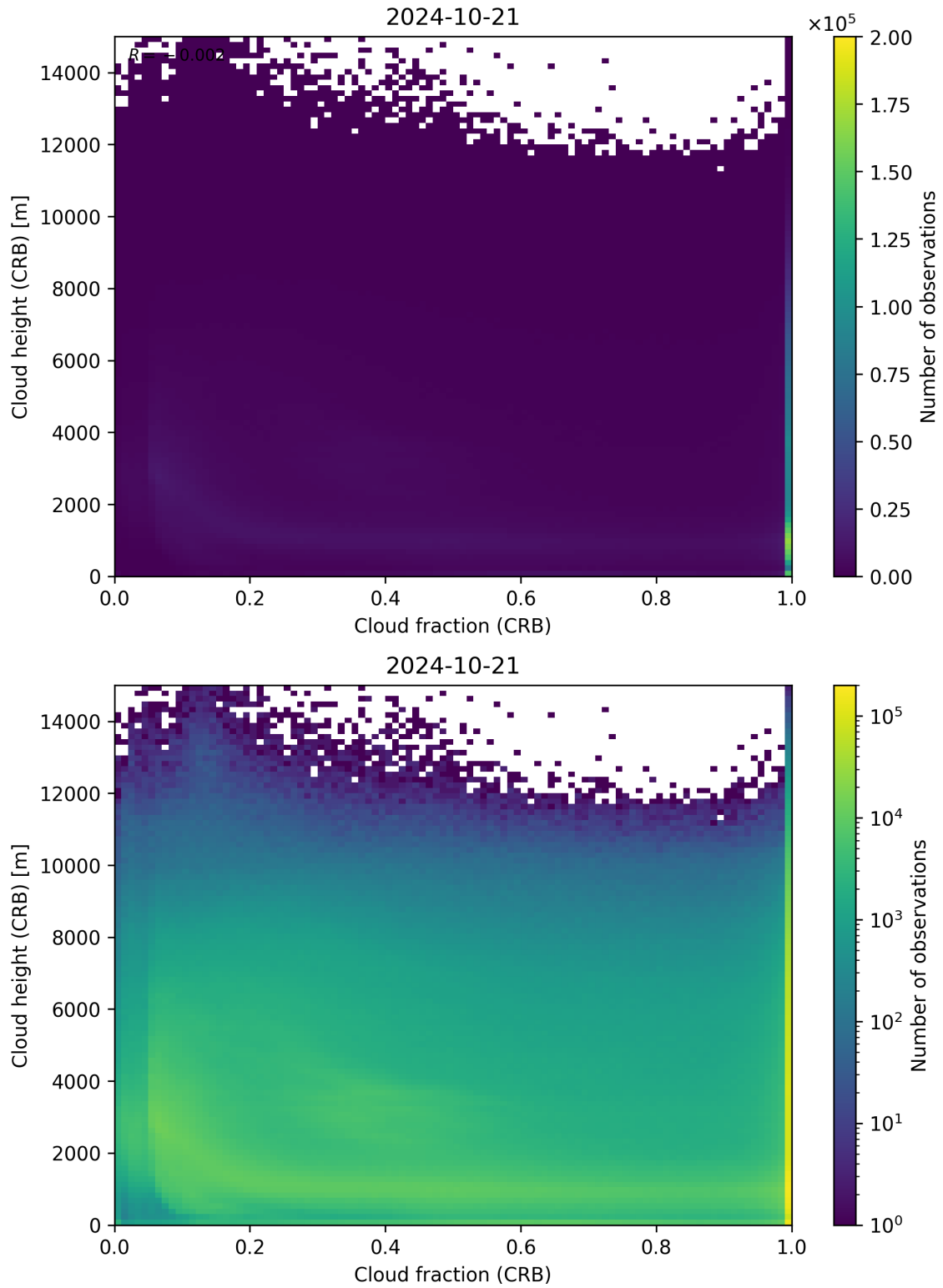
Figure 79: Scatter density plot of “Cloud fraction (CRB)” against “Cloud height (CRB)” for 2024-10-20 to 2024-10-22.
