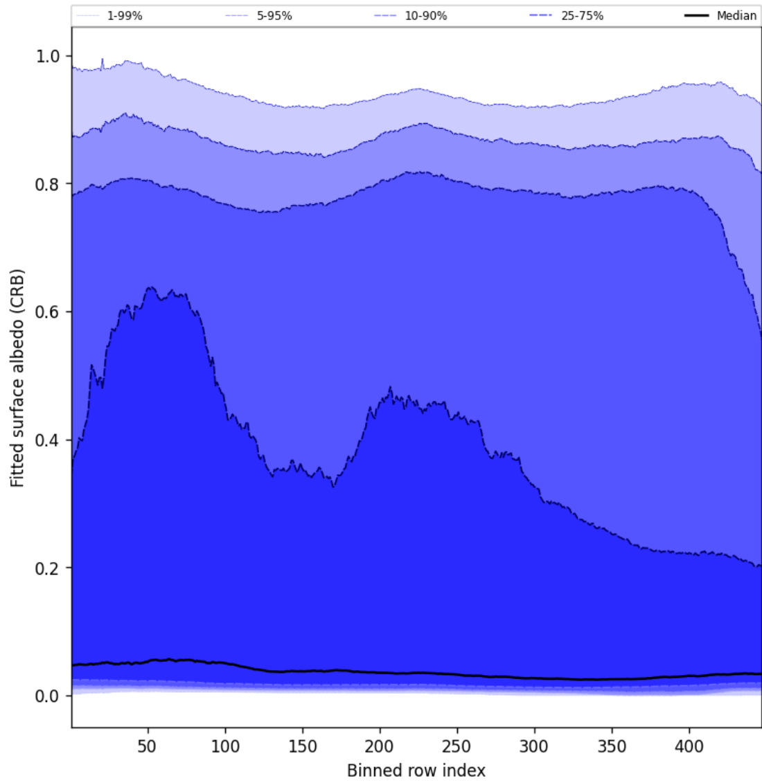
Figure 62: Along track statistics of “Fitted surface albedo (CRB)” for 2024-10-20 to 2024-10-22
