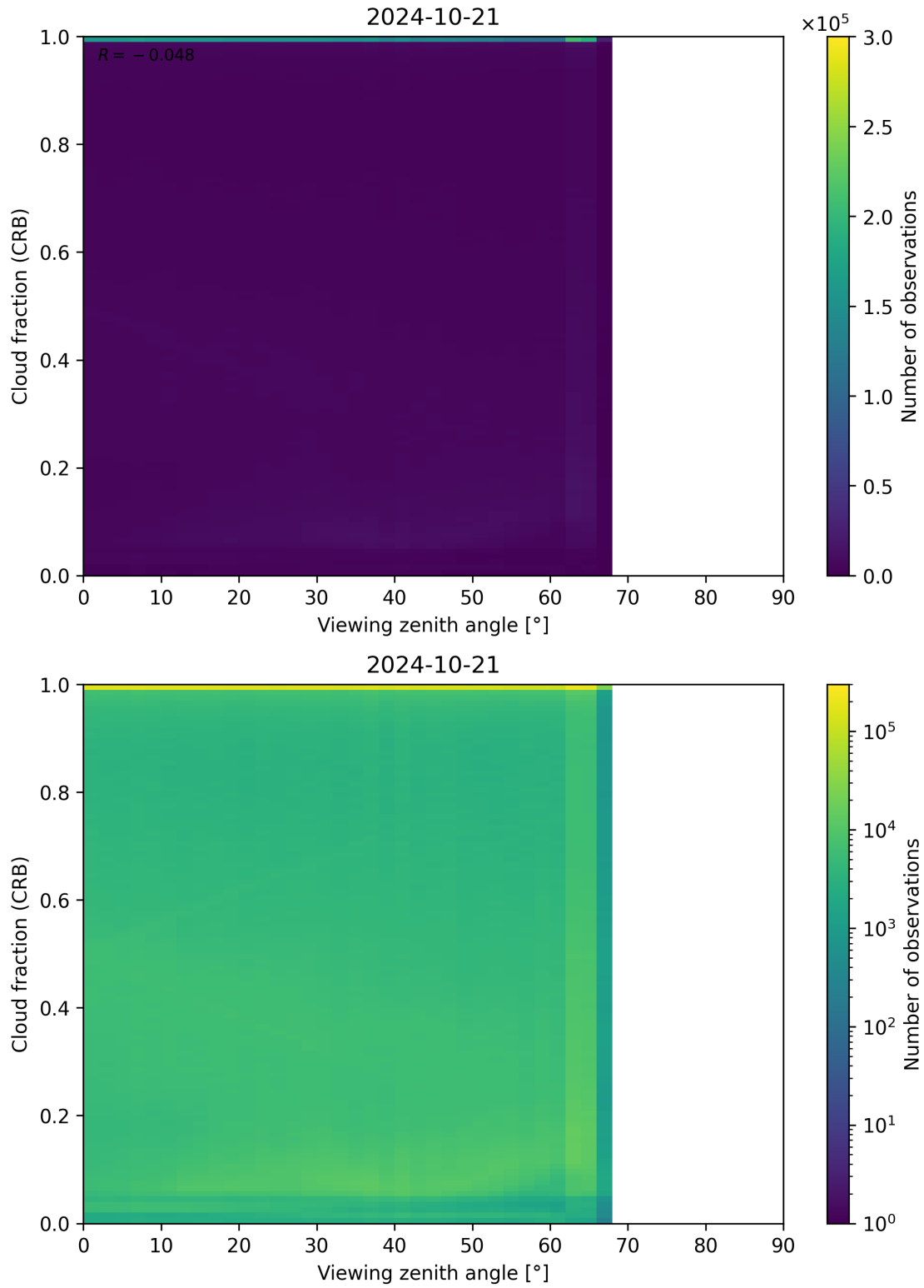
Figure 109: Scatter density plot of “Viewing zenith angle” against “Cloud fraction (CRB)” for 2024-10-20 to 2024-10-22.
