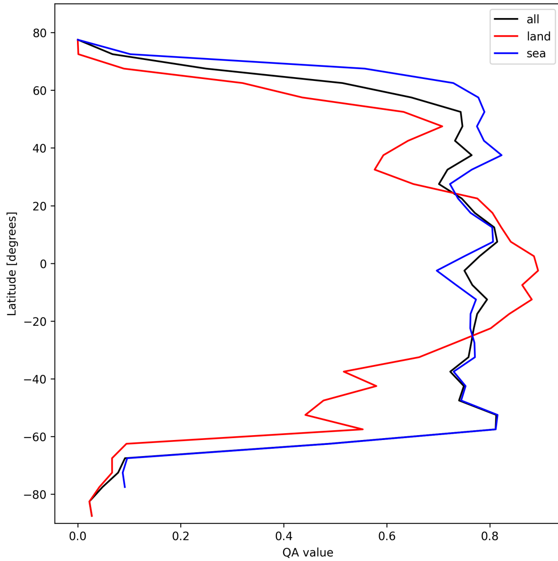
Figure 22: Zonal average of “QA value” for 2024-10-20 to 2024-10-22.
