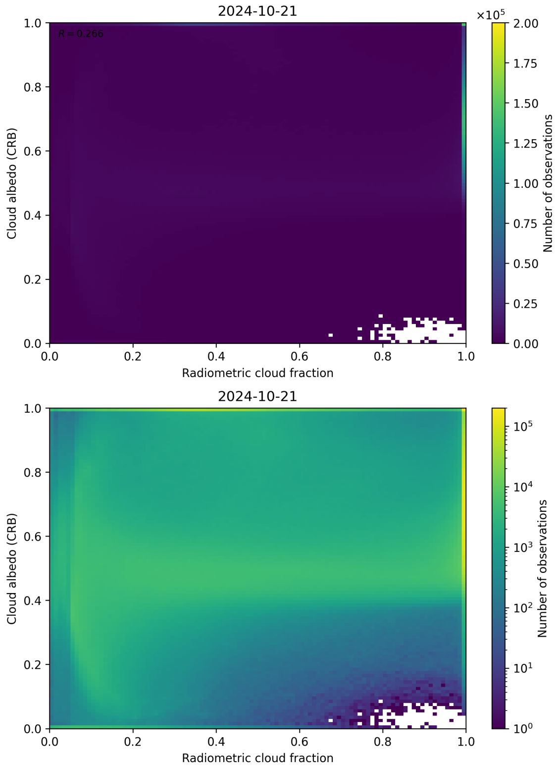
Figure 71: Scatter density plot of “Radiometric cloud fraction” against “Cloud albedo (CRB)” for 2024-10-20 to 2024-10-22.
