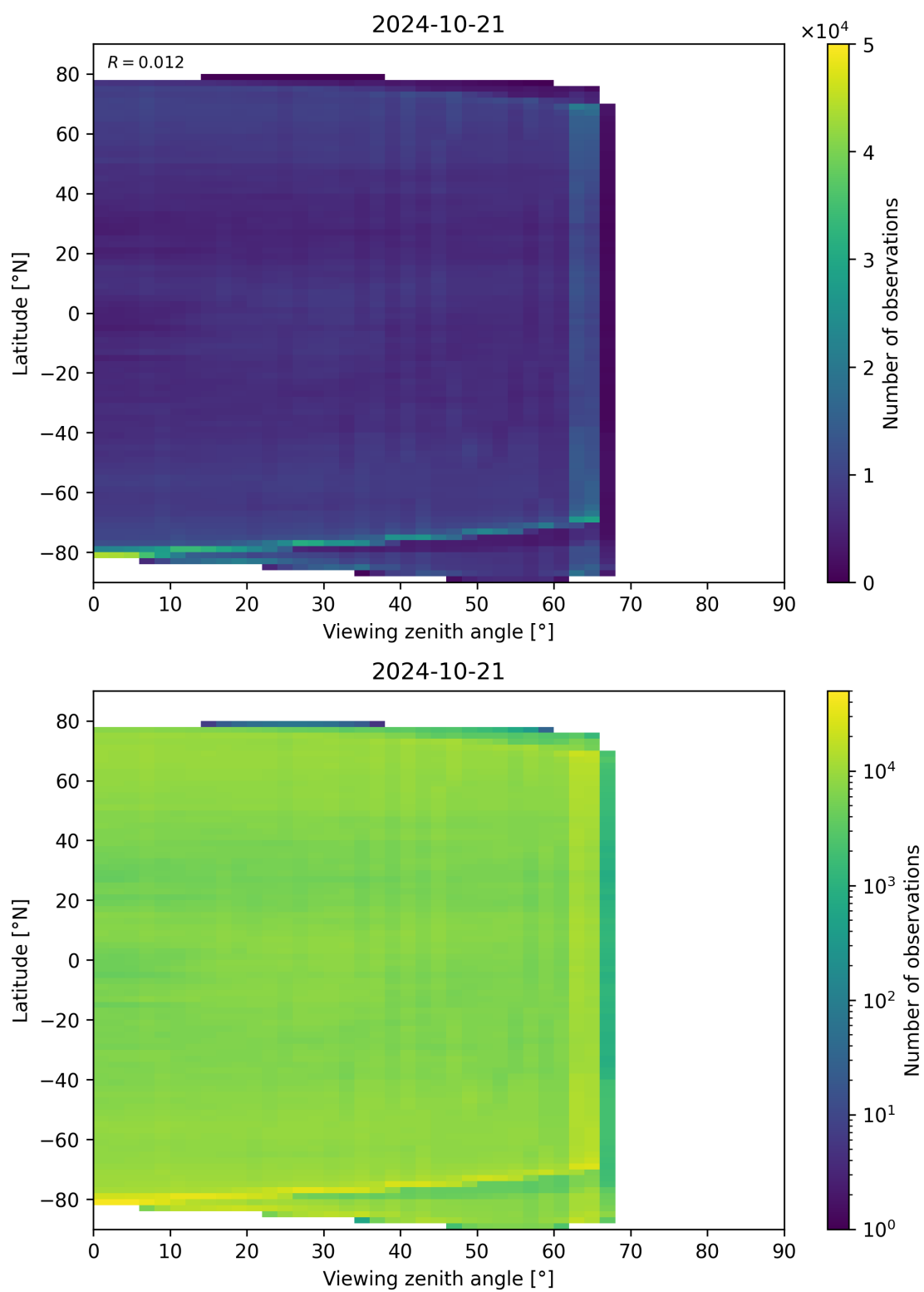
Figure 113: Scatter density plot of “Viewing zenith angle” against “Latitude” for 2024-10-20 to 2024-10-22.
