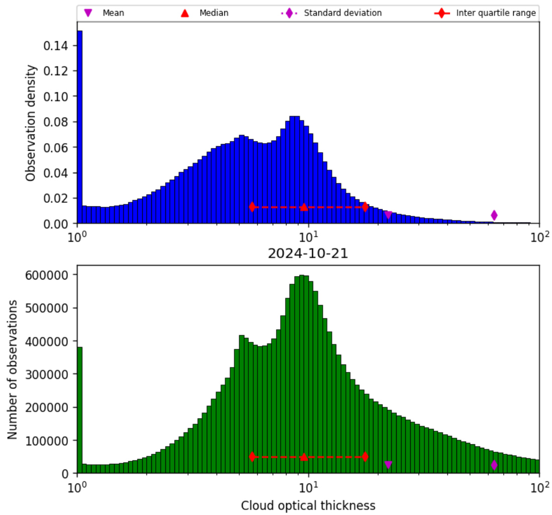
Figure 41: Histogram of “Cloud optical thickness” for 2024-10-20 to 2024-10-22
