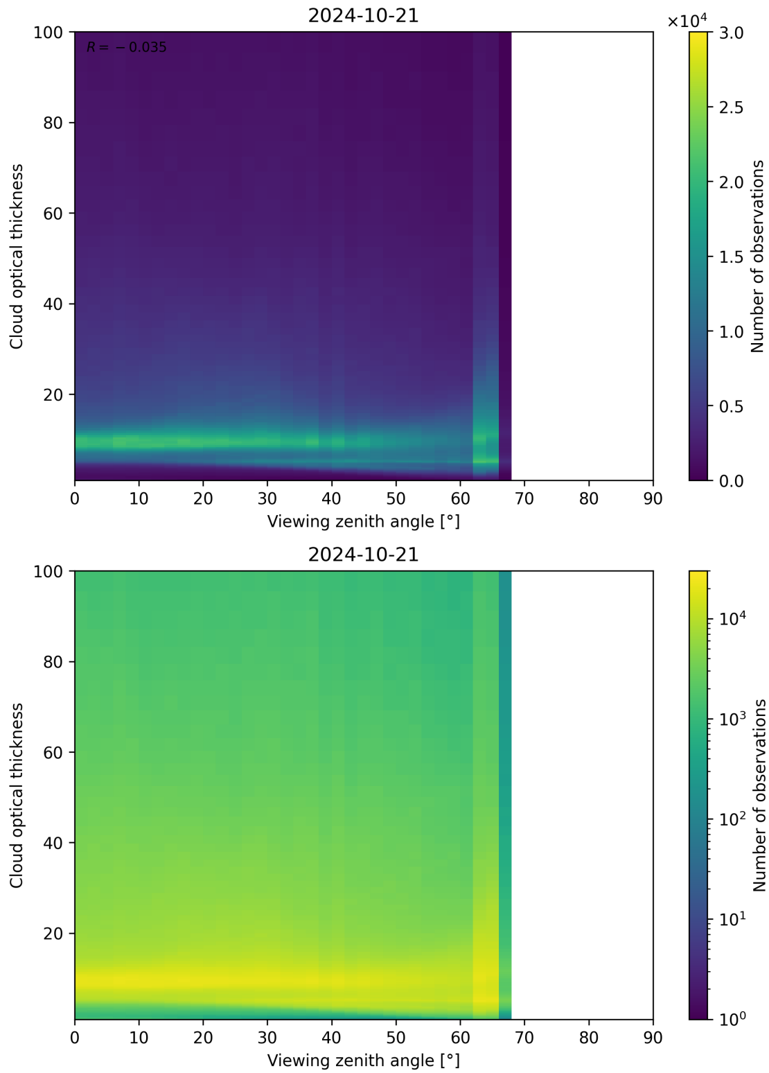
Figure 111: Scatter density plot of “Viewing zenith angle” against “Cloud optical thickness” for 2024-10-20 to 2024-10-22.
