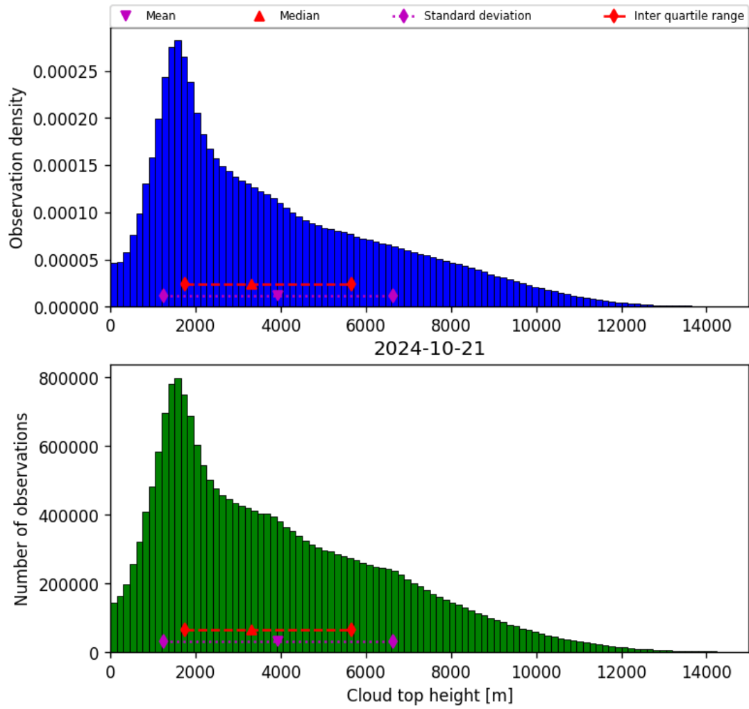
Figure 40: Histogram of “Cloud top height” for 2024-10-20 to 2024-10-22
