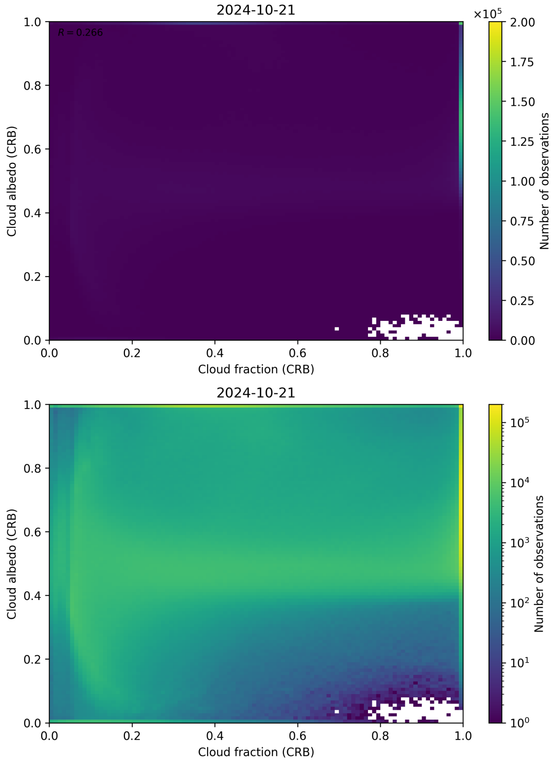
Figure 77: Scatter density plot of “Cloud fraction (CRB)” against “Cloud albedo (CRB)” for 2024-10-20 to 2024-10-22.
