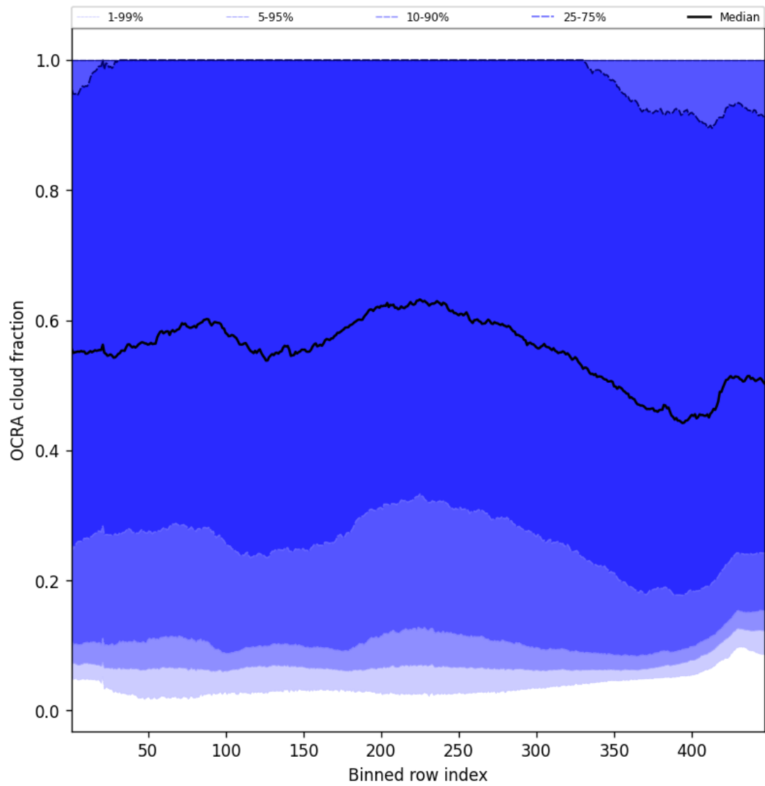
Figure 66: Along track statistics of “OCRA cloud fraction” for 2024-10-20 to 2024-10-22
