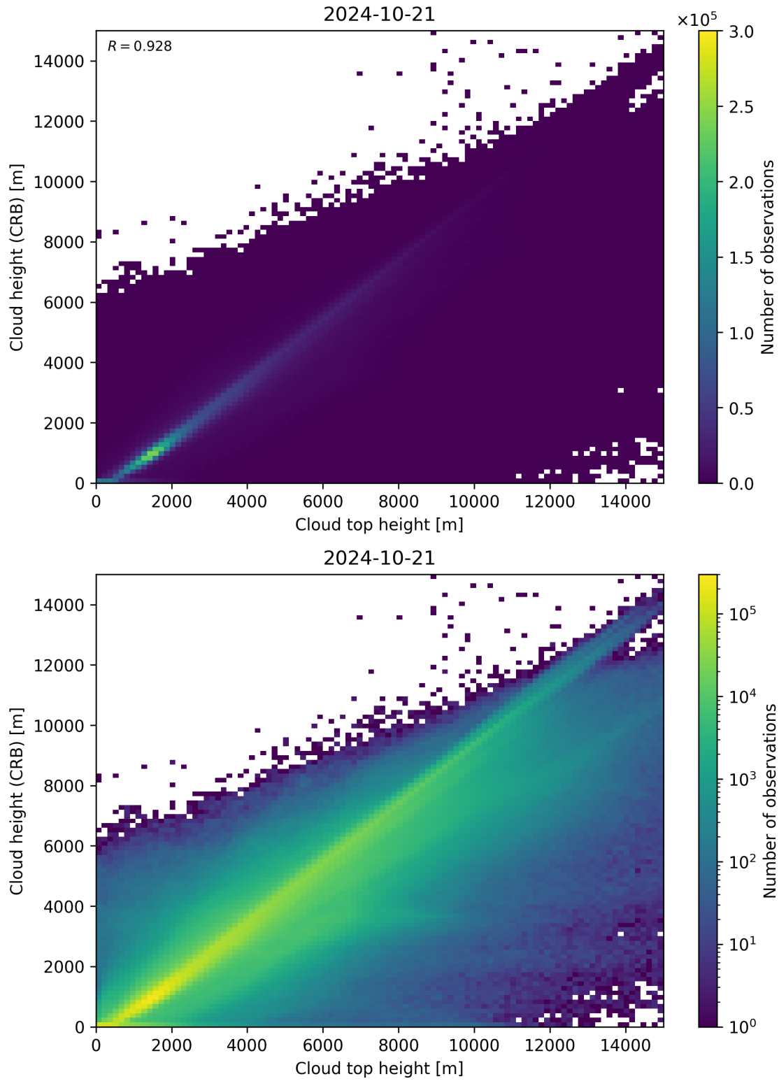
Figure 89: Scatter density plot of “Cloud top height” against “Cloud height (CRB)” for 2024-10-20 to 2024-10-22.
