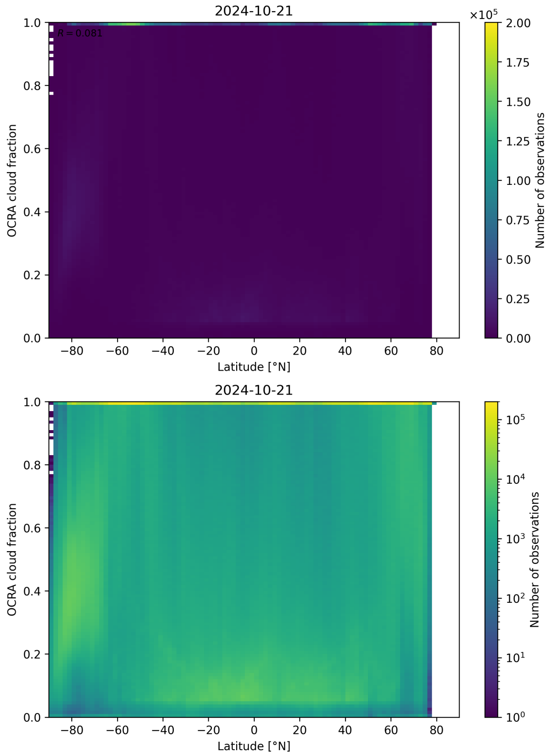
Figure 93: Scatter density plot of “Latitude” against “OCRA cloud fraction” for 2024-10-20 to 2024-10-22.
