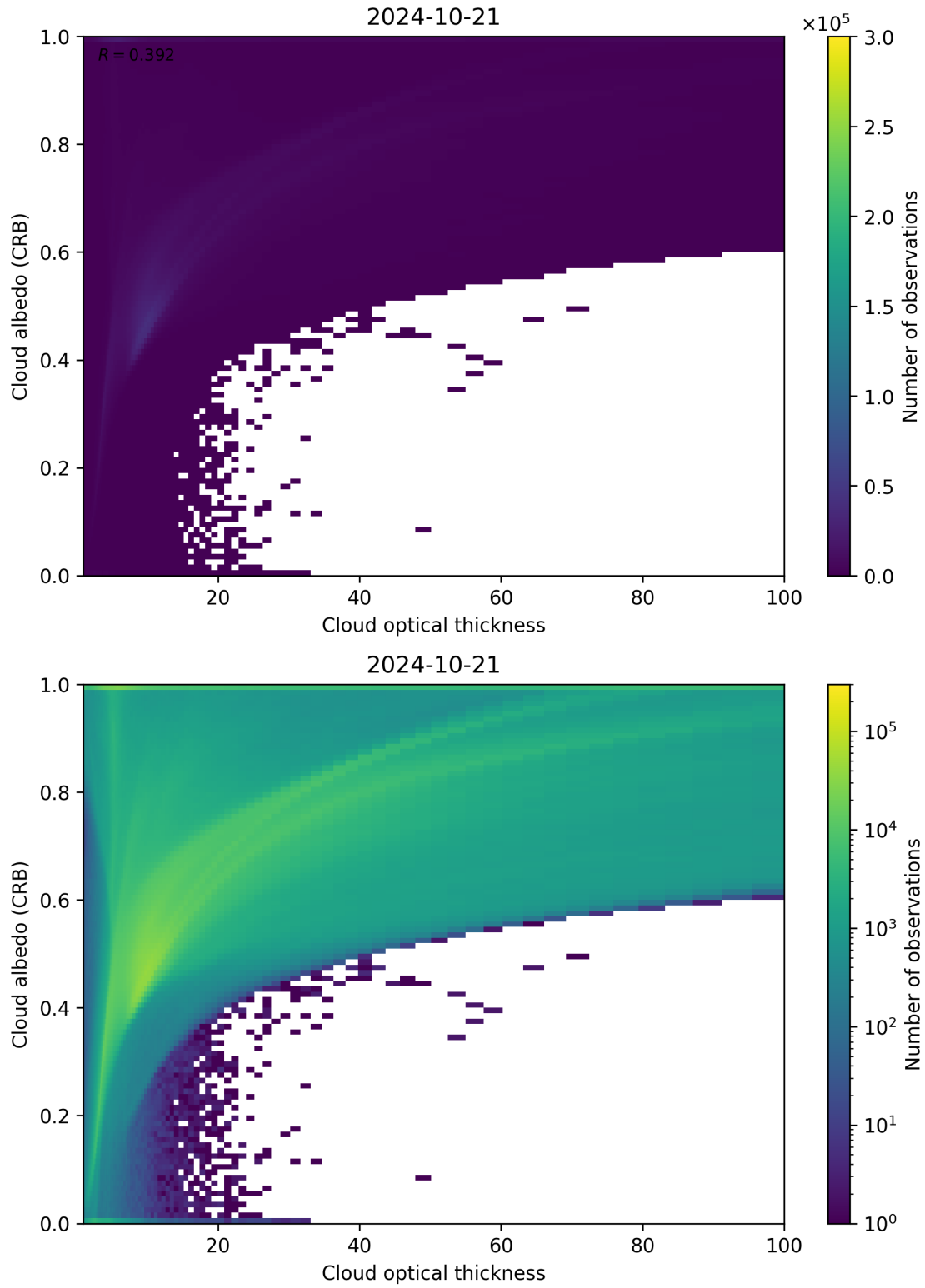
Figure 82: Scatter density plot of “Cloud optical thickness” against “Cloud albedo (CRB)” for 2024-10-20 to 2024-10-22.
