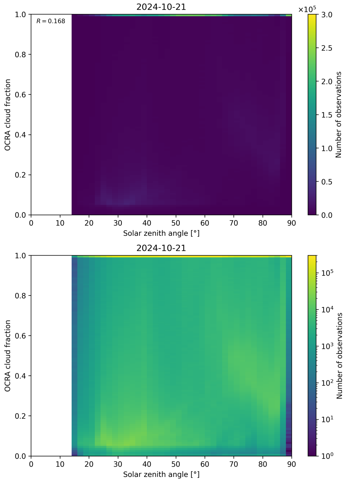
Figure 100: Scatter density plot of “Solar zenith angle” against “OCRA cloud fraction” for 2024-10-20 to 2024-10-22.
