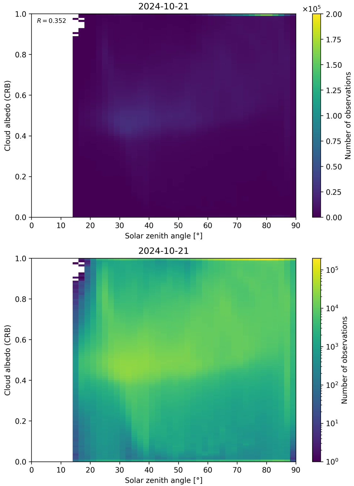
Figure 98: Scatter density plot of “Solar zenith angle” against “Cloud albedo (CRB)” for 2024-10-20 to 2024-10-22.
