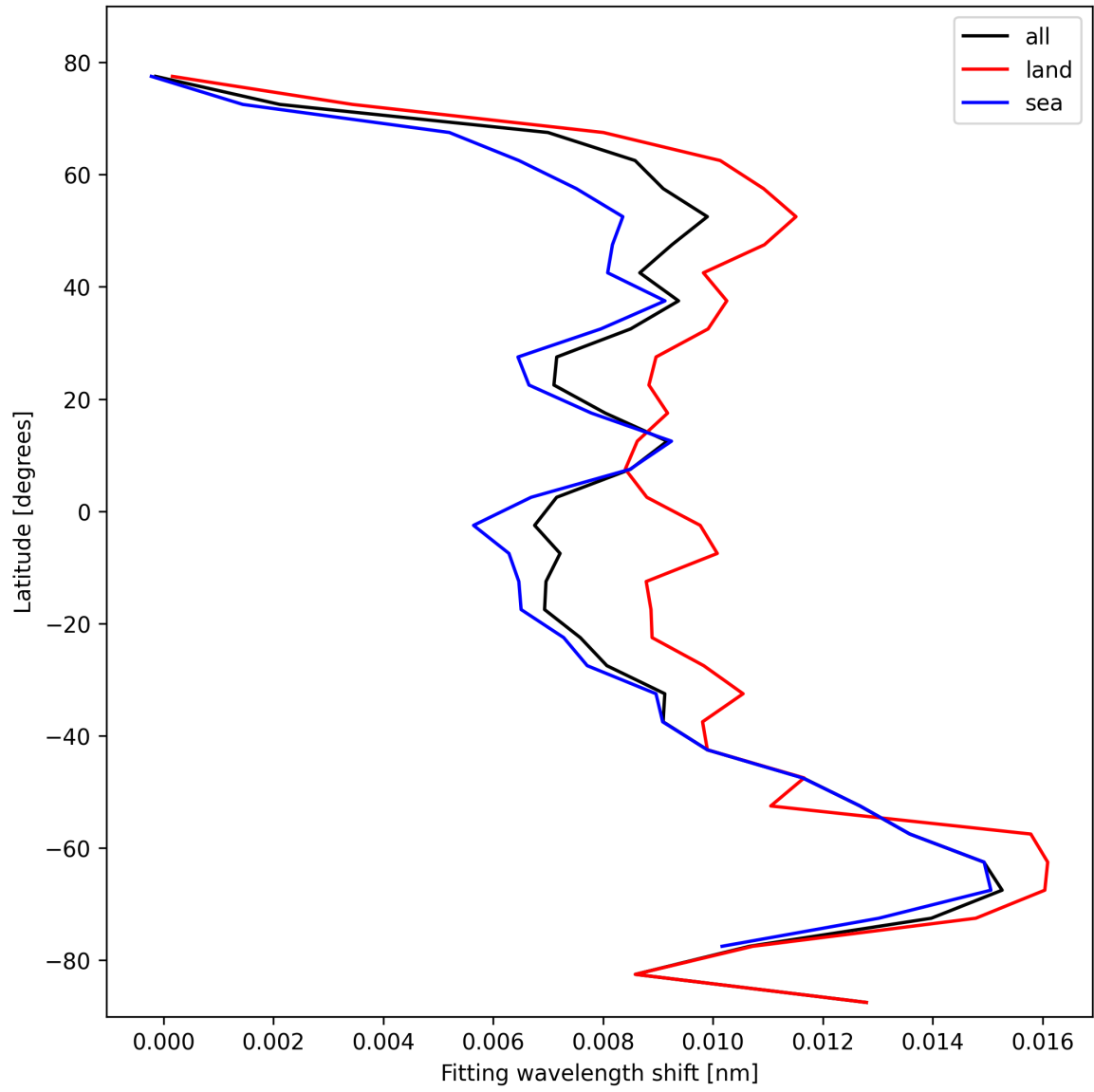
Figure 33: Zonal average of “Fitting wavelength shift” for 2024-10-20 to 2024-10-22.
