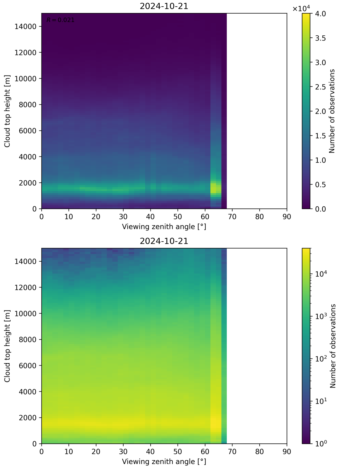
Figure 112: Scatter density plot of “Viewing zenith angle” against “Cloud top height” for 2024-10-20 to 2024-10-22.
