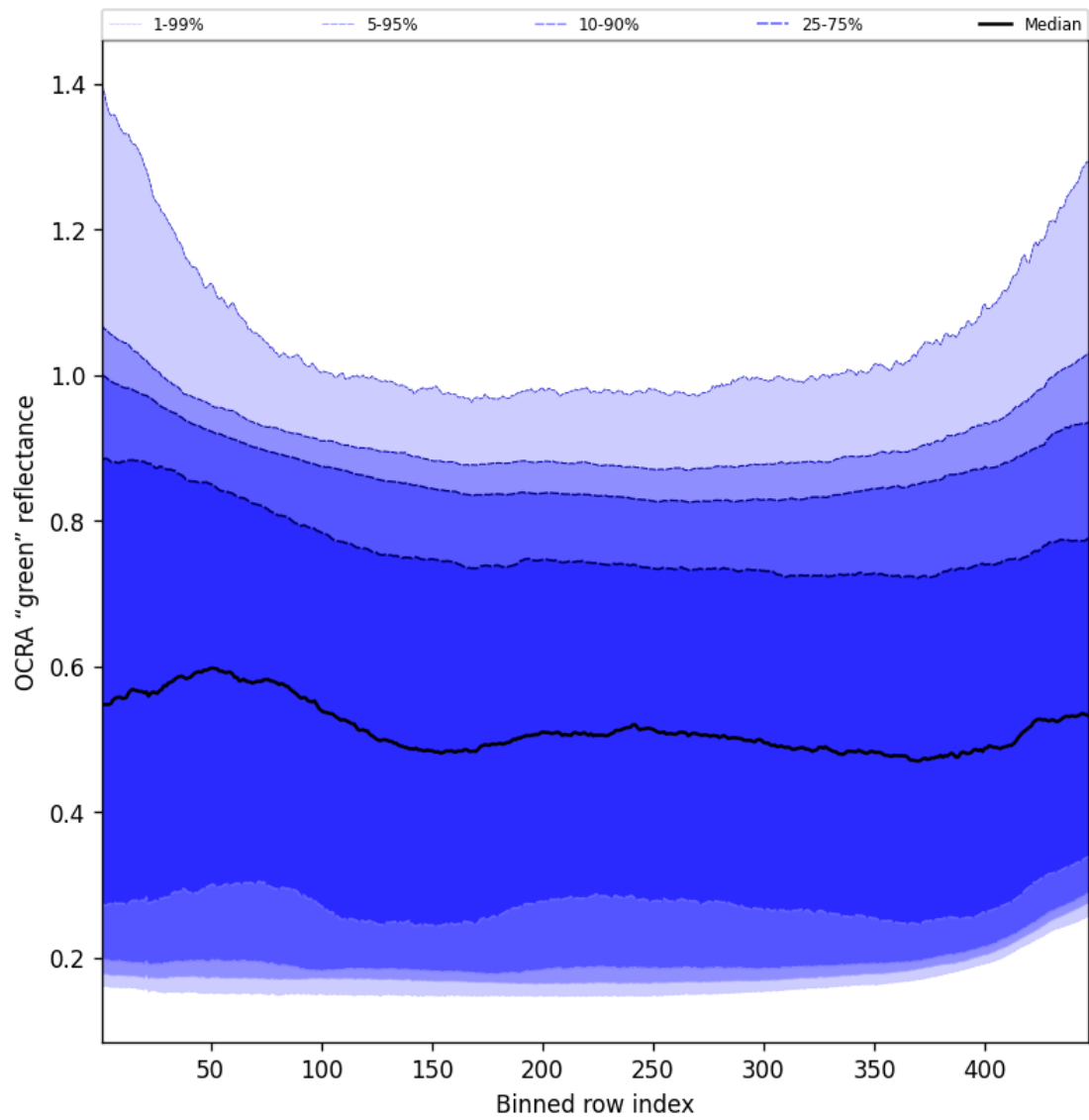
Figure 68: Along track statistics of “OCRA “green” reflectance” for 2024-10-20 to 2024-10-22
