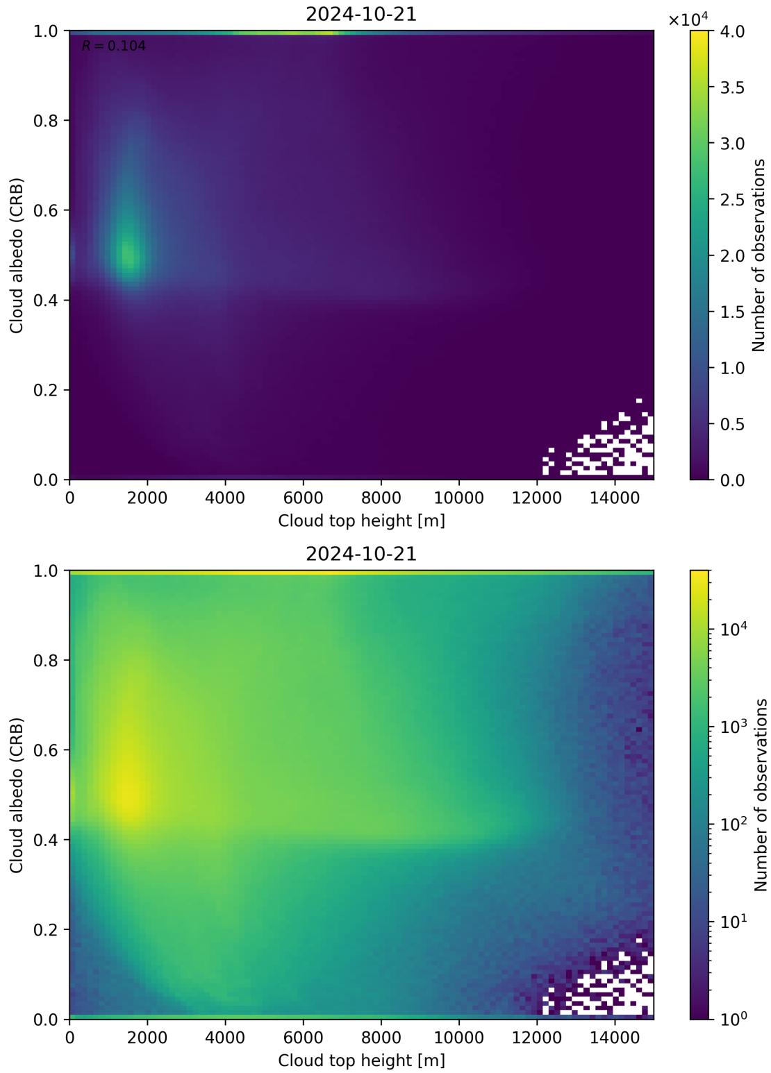
Figure 86: Scatter density plot of “Cloud top height” against “Cloud albedo (CRB)” for 2024-10-20 to 2024-10-22.
