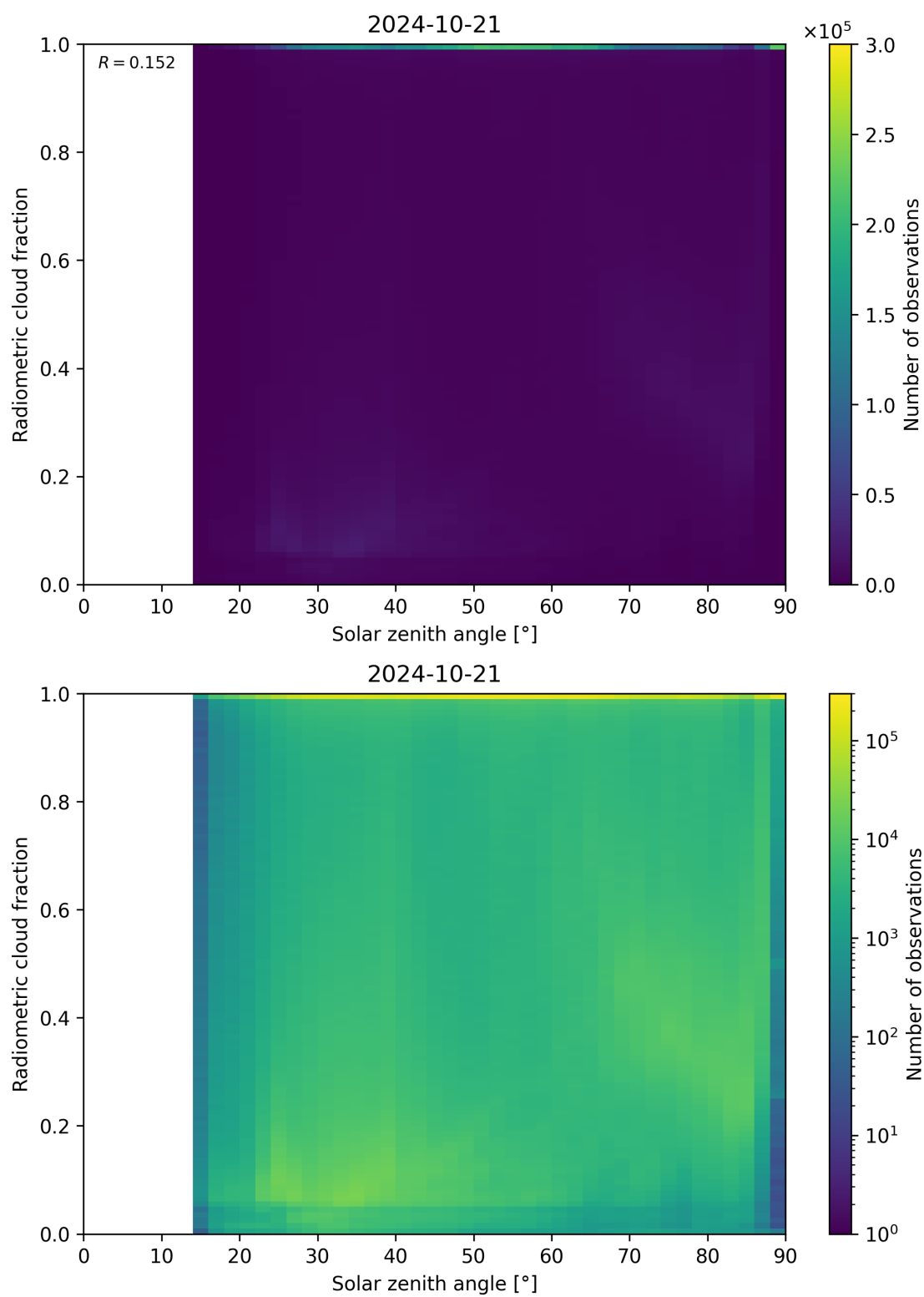
Figure 99: Scatter density plot of “Solar zenith angle” against “Radiometric cloud fraction” for 2024-10-20 to 2024-10-22.
