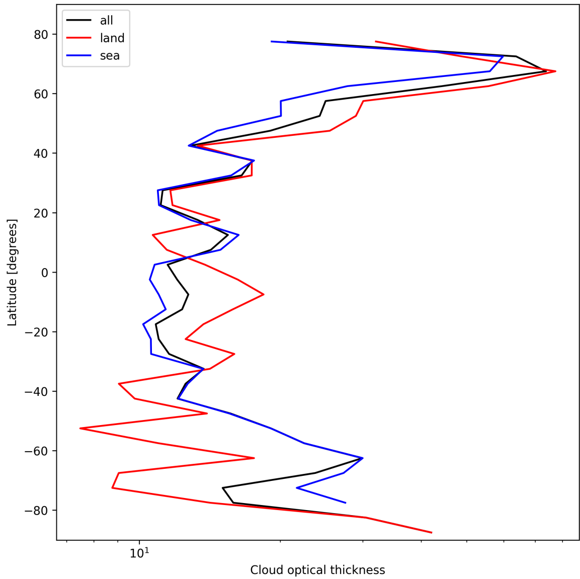
Figure 25: Zonal average of “Cloud optical thickness” for 2024-10-20 to 2024-10-22.
