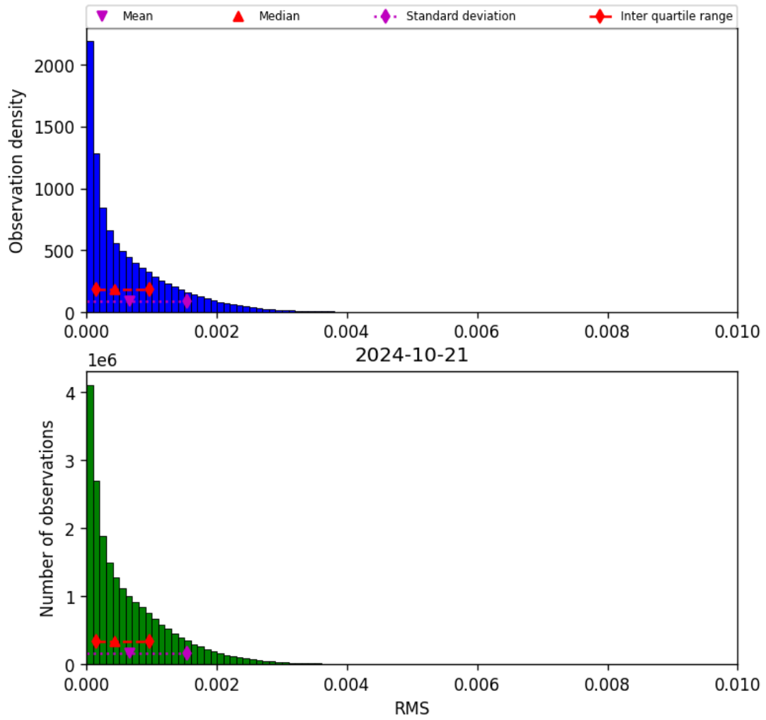
Figure 47: Histogram of “RMS” for 2024-10-20 to 2024-10-22
