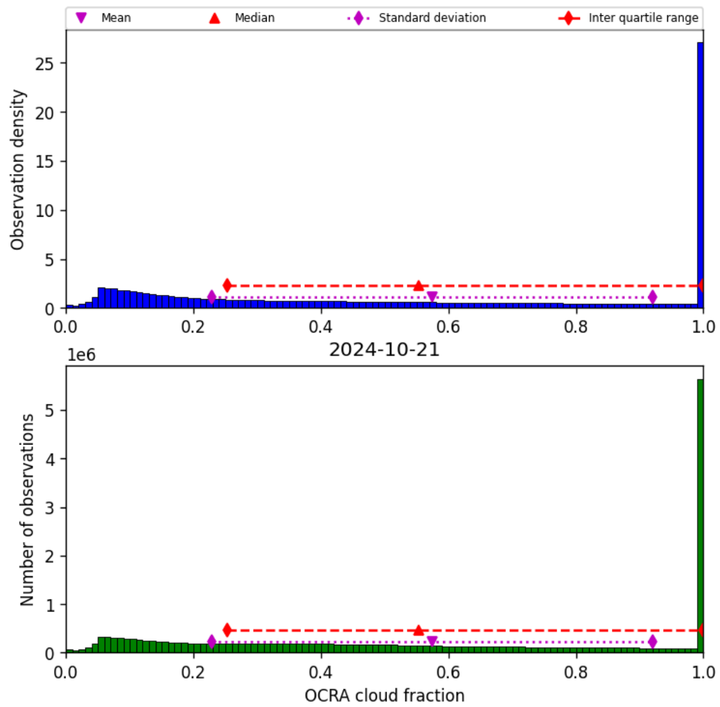
Figure 50: Histogram of “OCRA cloud fraction” for 2024-10-20 to 2024-10-22
