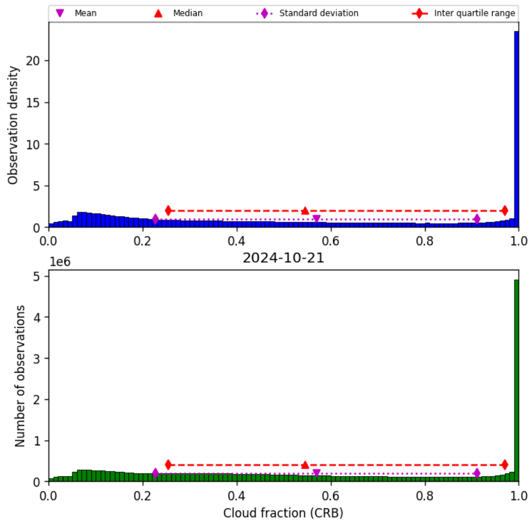
Figure 42: Histogram of “Cloud fraction (CRB)” for 2024-10-20 to 2024-10-22
