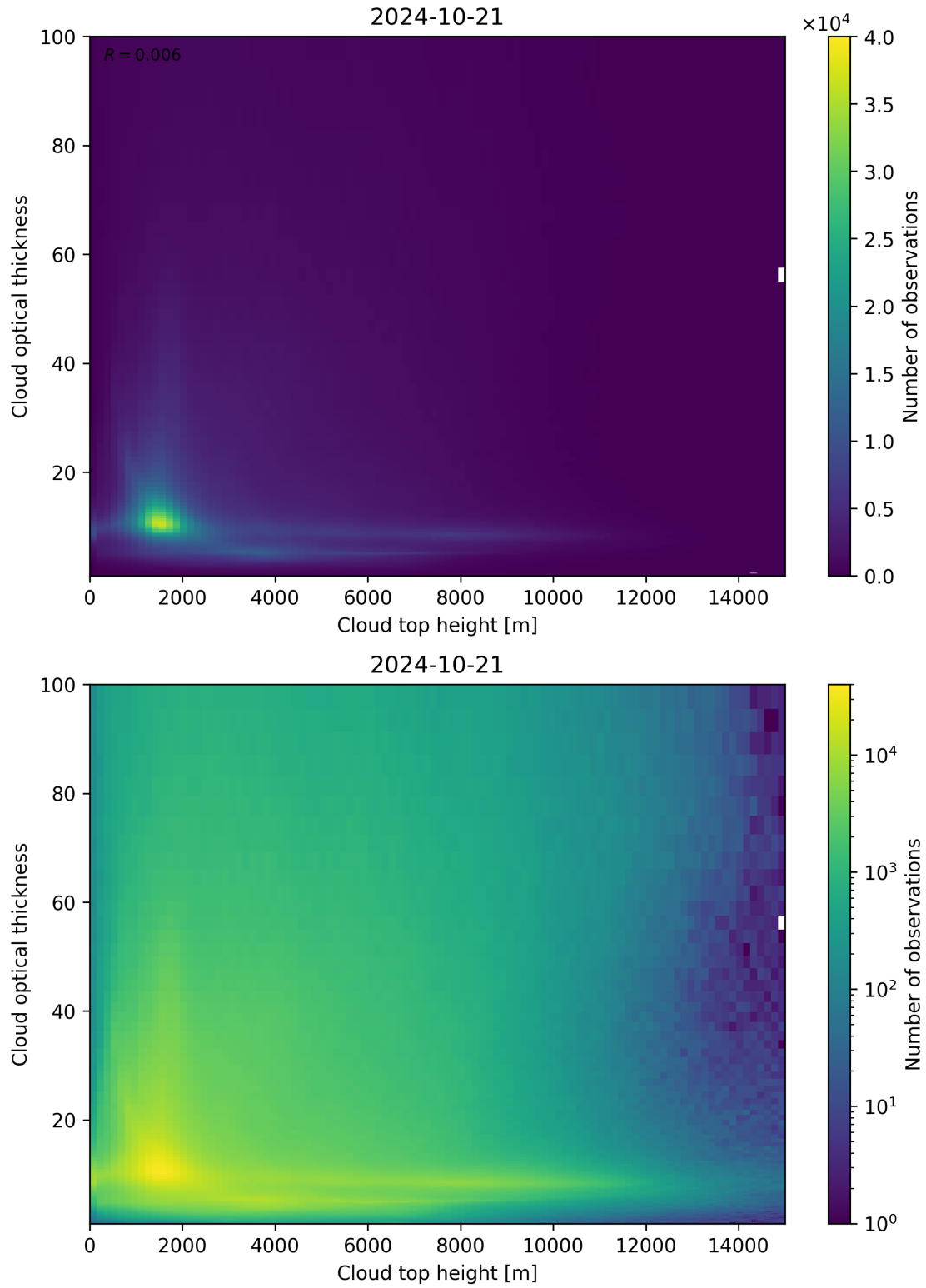
Figure 90: Scatter density plot of “Cloud top height” against “Cloud optical thickness” for 2024-10-20 to 2024-10-22.
