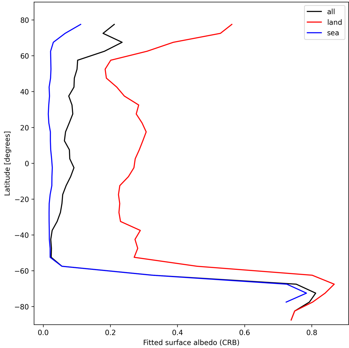
Figure 30: Zonal average of “Fitted surface albedo (CRB)” for 2024-10-20 to 2024-10-22.
