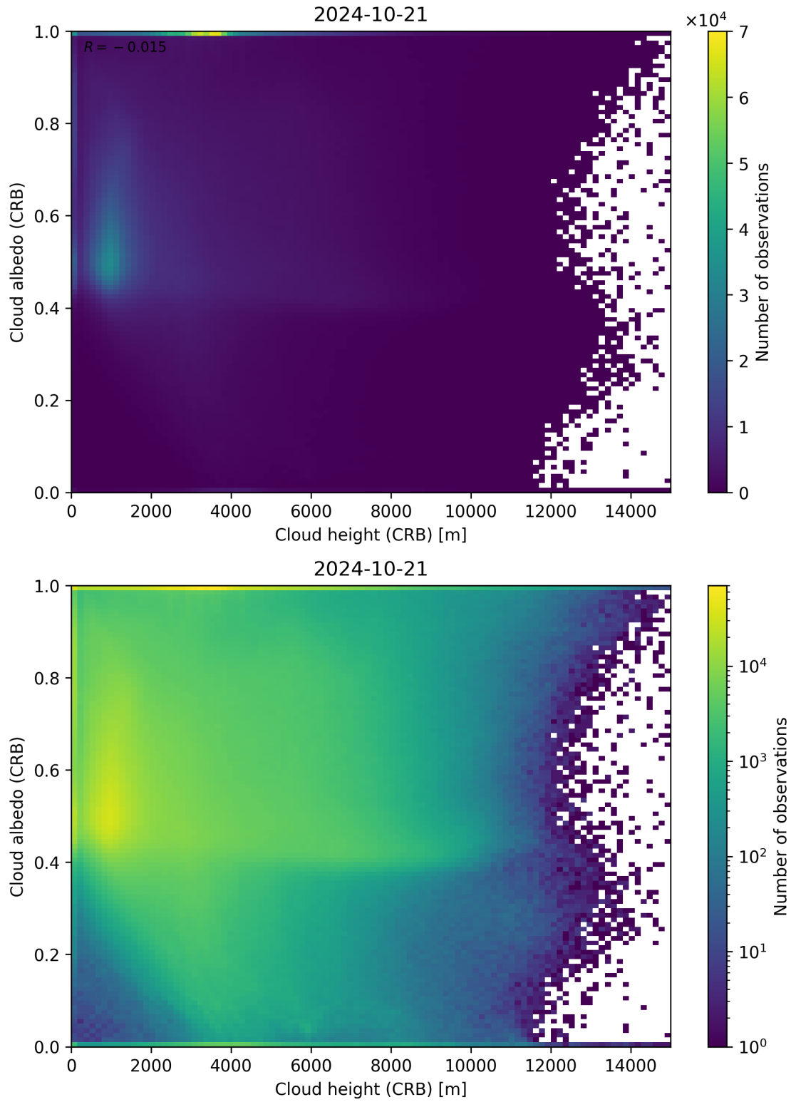
Figure 80: Scatter density plot of “Cloud height (CRB)” against “Cloud albedo (CRB)” for 2024-10-20 to 2024-10-22.
