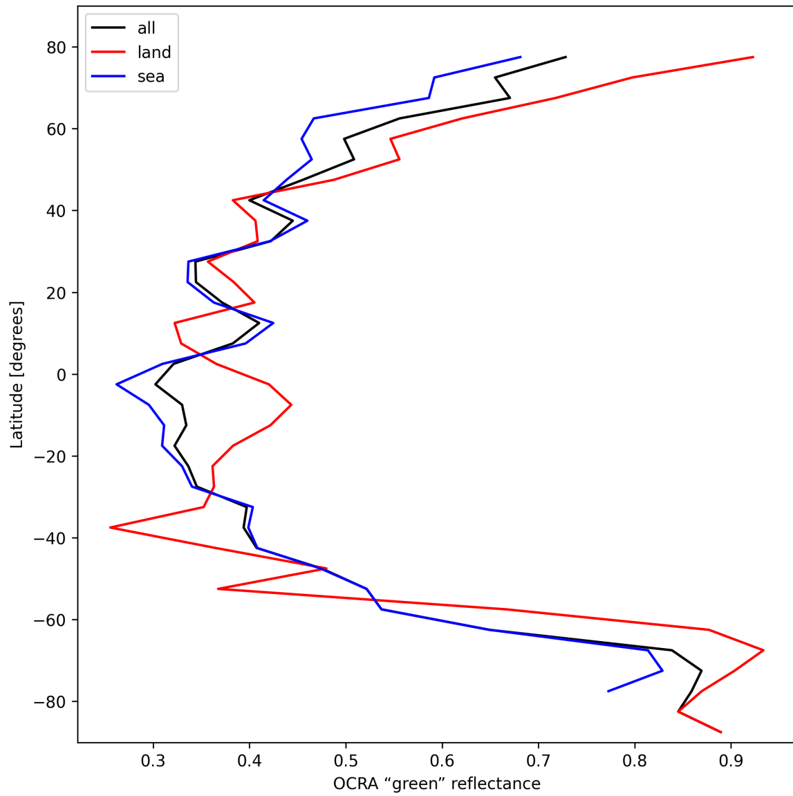
Figure 36: Zonal average of “OCRA “green” reflectance” for 2024-10-20 to 2024-10-22.
