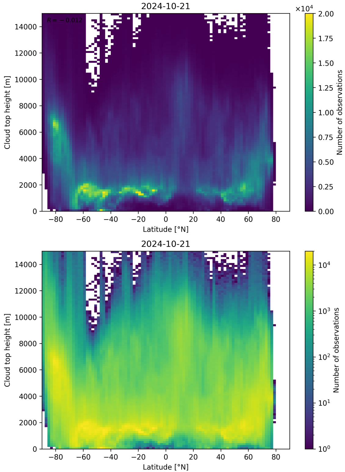
Figure 97: Scatter density plot of “Latitude” against “Cloud top height” for 2024-10-20 to 2024-10-22.
