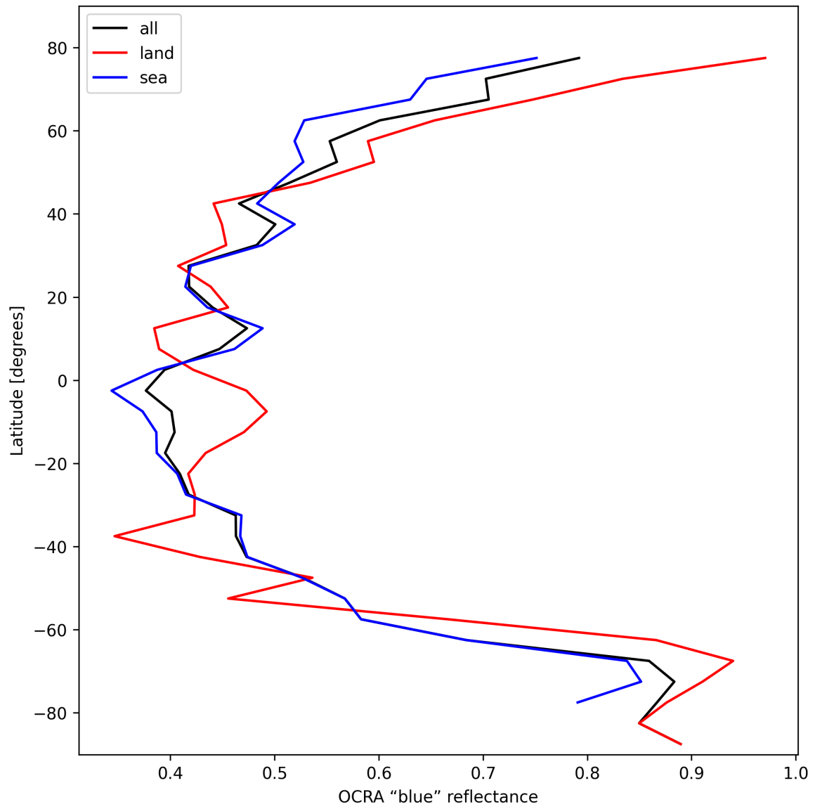
Figure 35: Zonal average of “OCRA “blue” reflectance” for 2024-10-20 to 2024-10-22.
