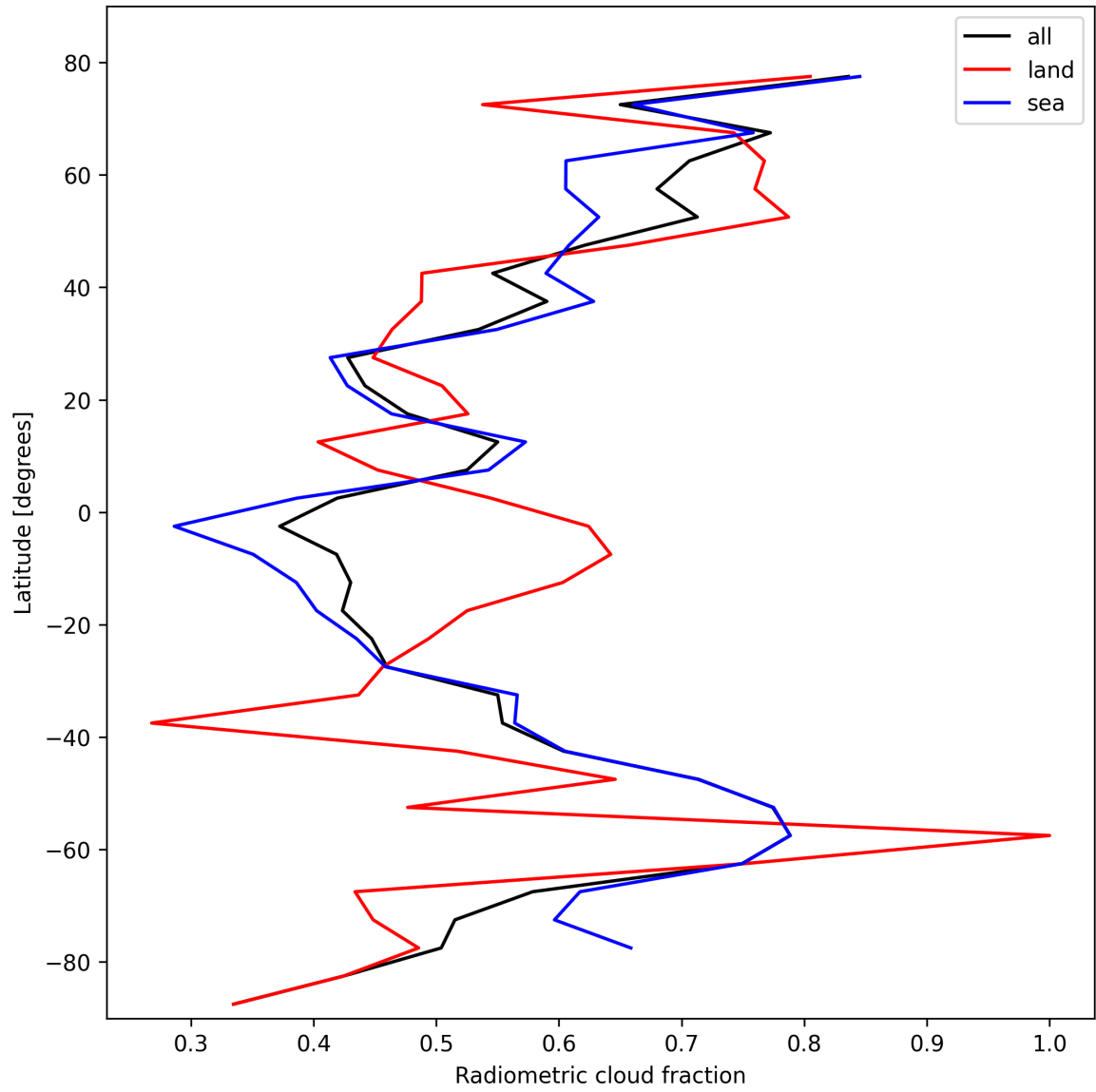
Figure 23: Zonal average of “Radiometric cloud fraction” for 2024-10-20 to 2024-10-22.
