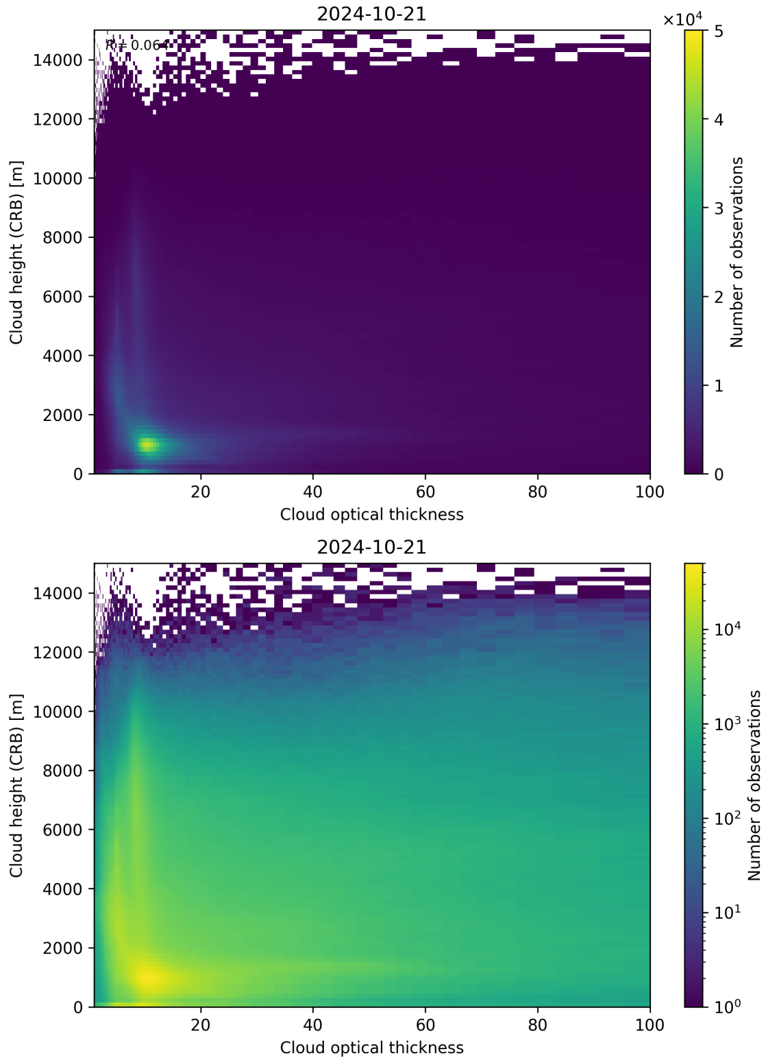
Figure 85: Scatter density plot of “Cloud optical thickness” against “Cloud height (CRB)” for 2024-10-20 to 2024-10-22.
