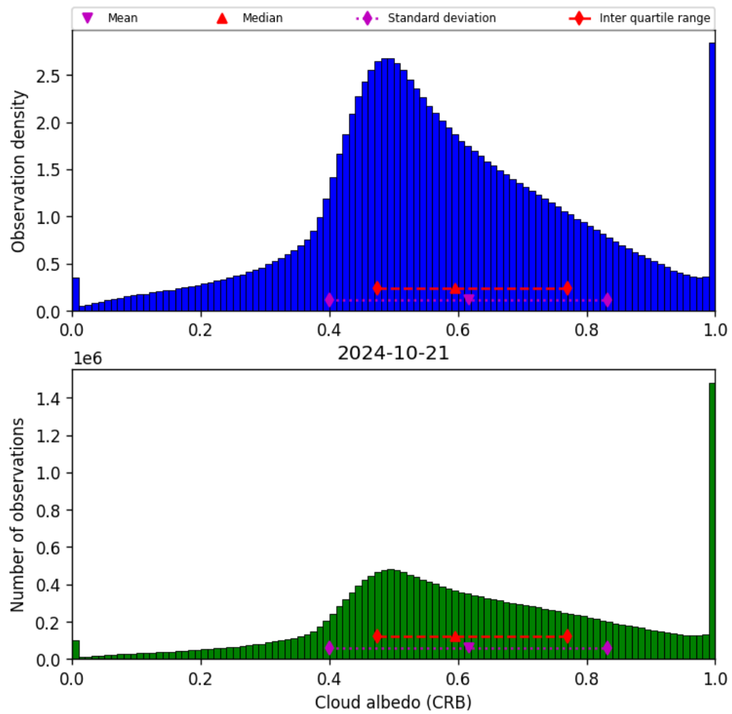
Figure 44: Histogram of “Cloud albedo (CRB)” for 2024-10-20 to 2024-10-22
