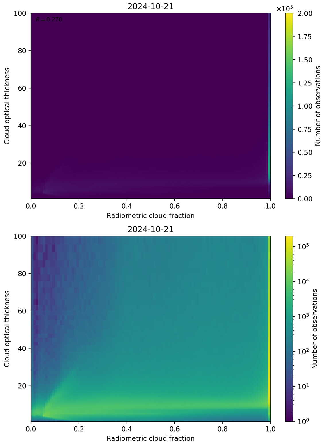
Figure 75: Scatter density plot of “Radiometric cloud fraction” against “Cloud optical thickness” for 2024-10-20 to 2024-10-22.
