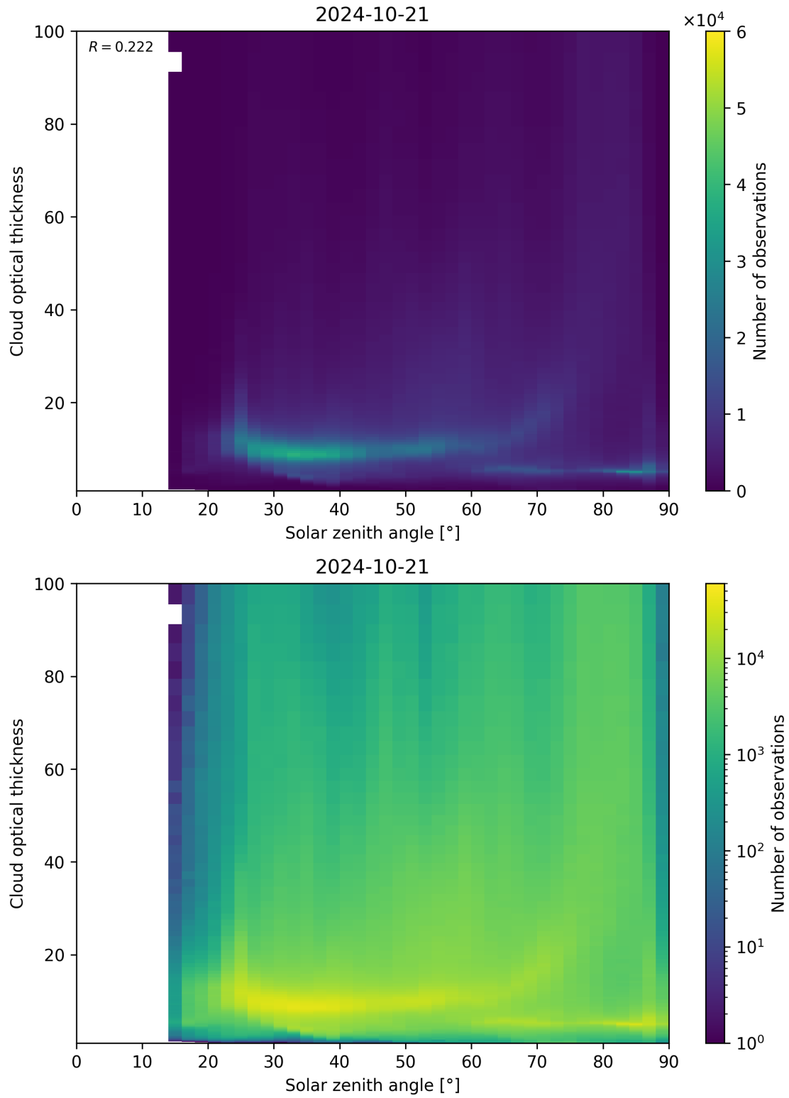
Figure 103: Scatter density plot of “Solar zenith angle” against “Cloud optical thickness” for 2024-10-20 to 2024-10-22.
