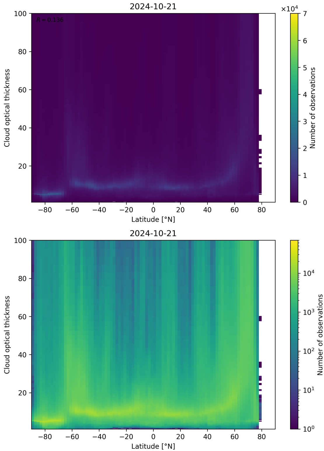
Figure 96: Scatter density plot of “Latitude” against “Cloud optical thickness” for 2024-10-20 to 2024-10-22.
