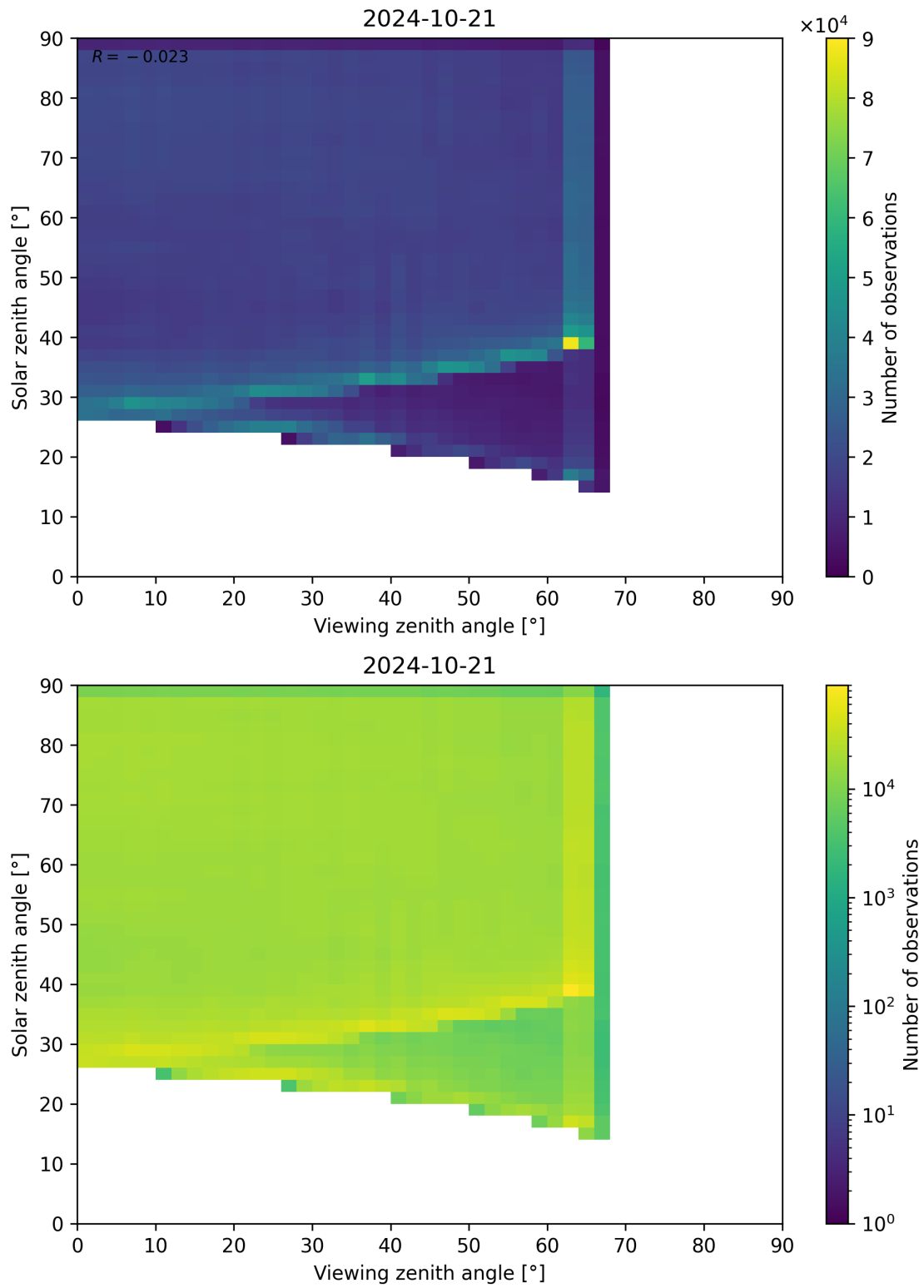
Figure 114: Scatter density plot of “Viewing zenith angle” against “Solar zenith angle” for 2024-10-20 to 2024-10-22.
