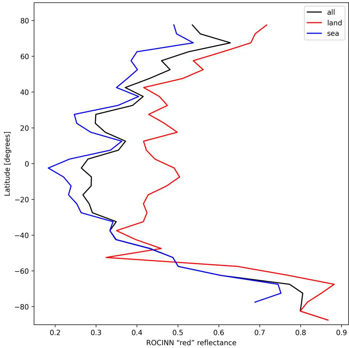
Figure 37: Zonal average of “ROCINN “red” reflectance” for 2024-10-20 to 2024-10-22.
