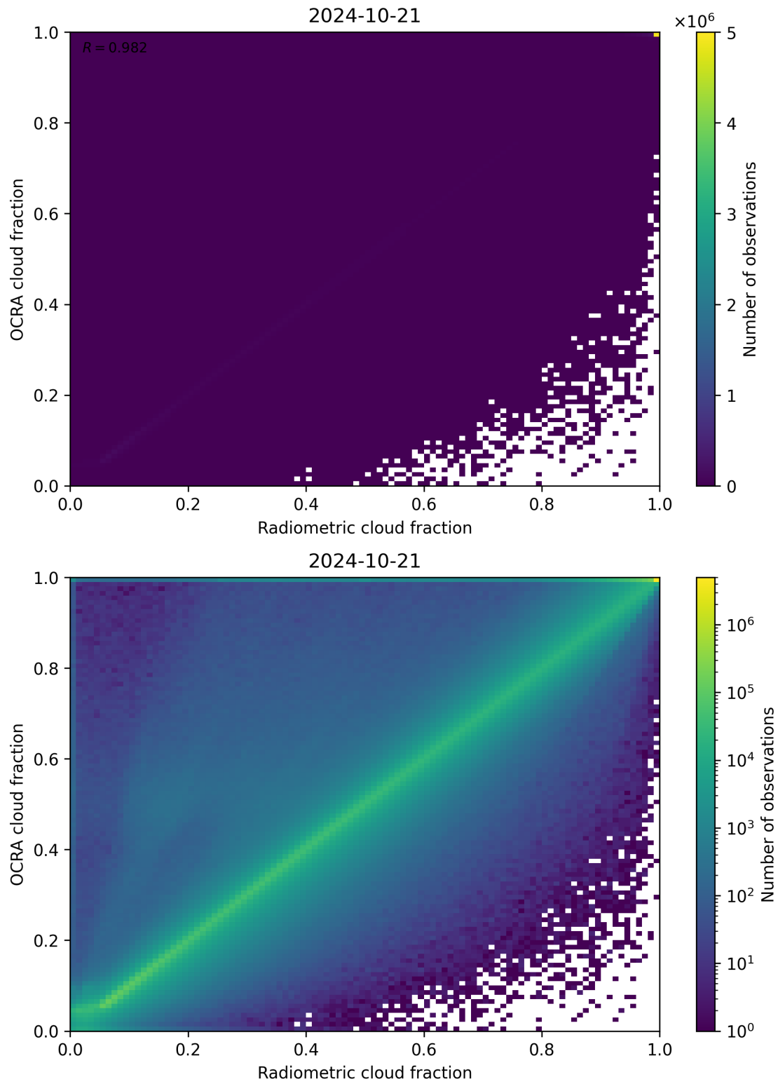
Figure 72: Scatter density plot of “Radiometric cloud fraction” against “OCRA cloud fraction” for 2024-10-20 to 2024-10-22.
