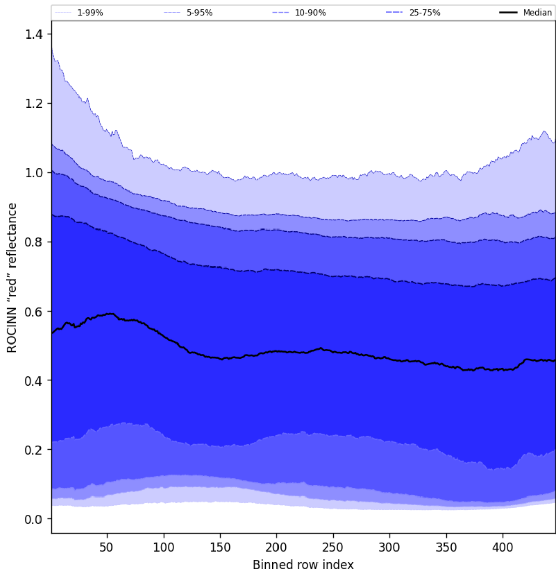
Figure 69: Along track statistics of “ROCINN “red” reflectance” for 2024-10-20 to 2024-10-22
