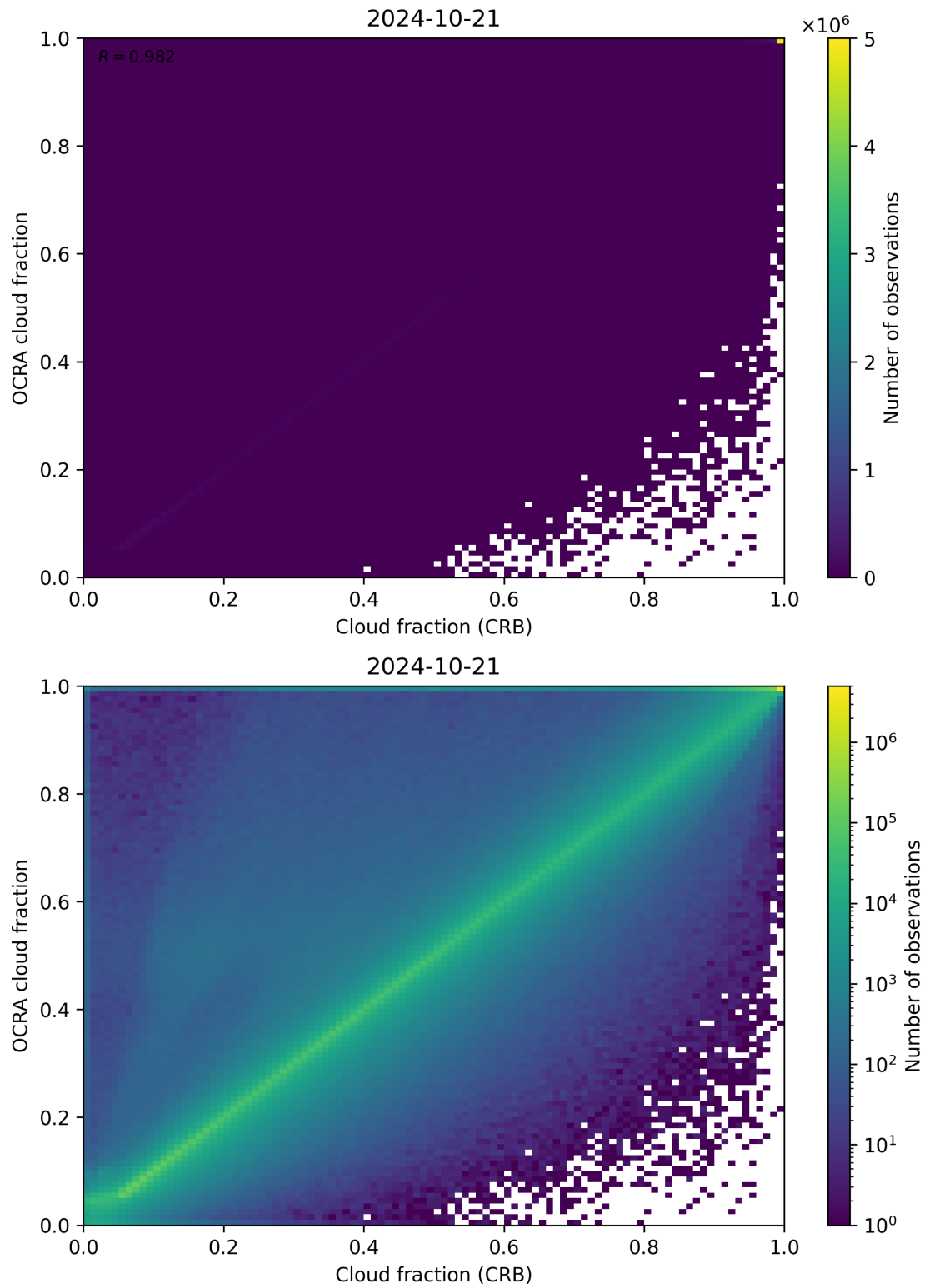
Figure 78: Scatter density plot of “Cloud fraction (CRB)” against “OCRA cloud fraction” for 2024-10-20 to 2024-10-22.
