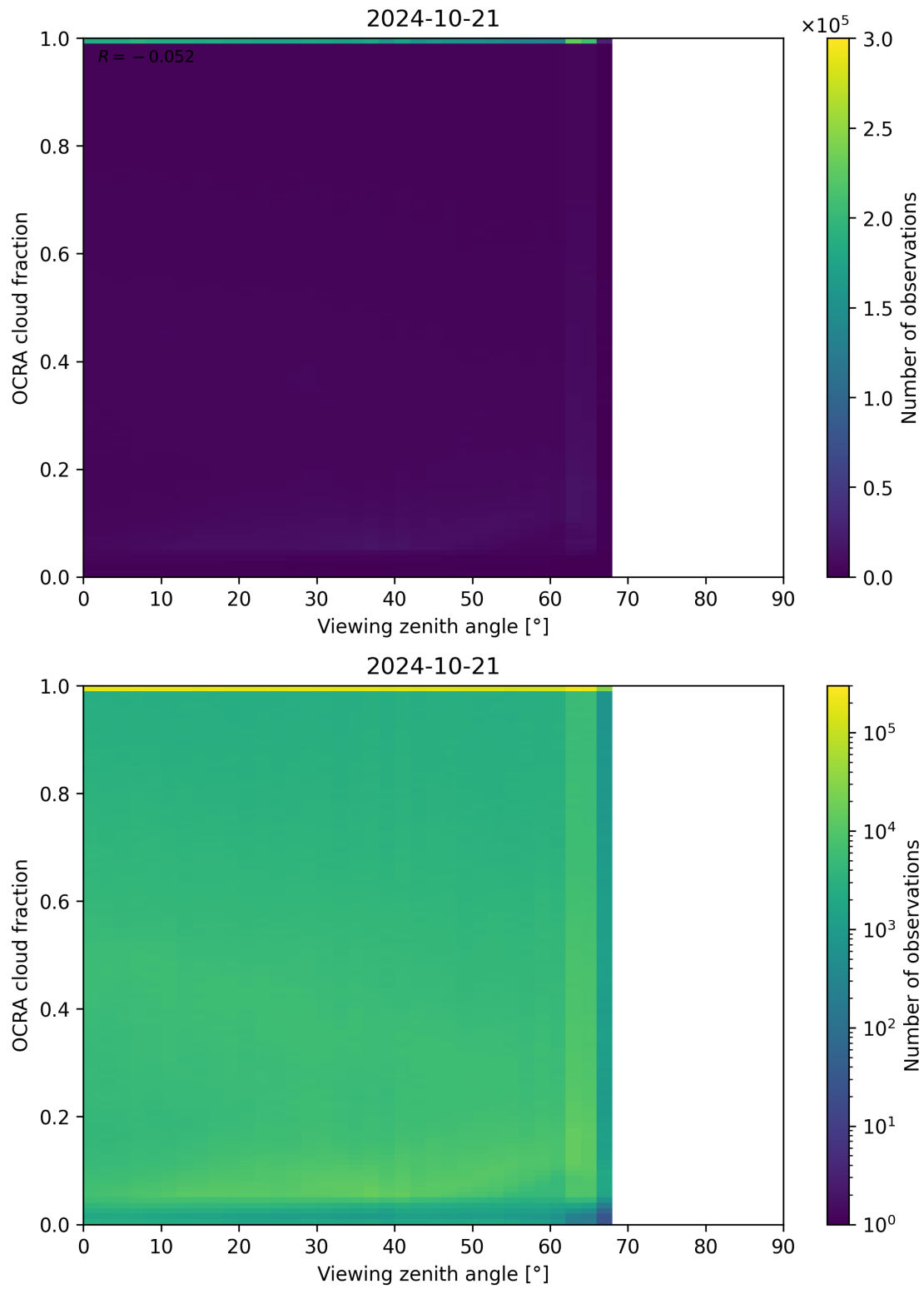
Figure 108: Scatter density plot of “Viewing zenith angle” against “OCRA cloud fraction” for 2024-10-20 to 2024-10-22.
