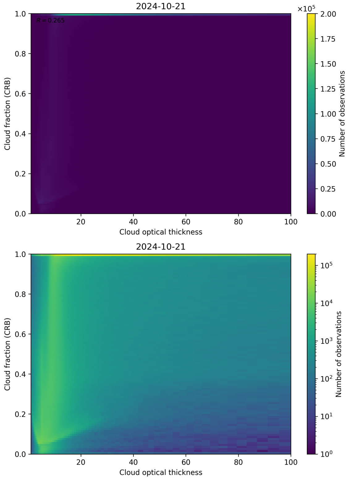
Figure 84: Scatter density plot of “Cloud optical thickness” against “Cloud fraction (CRB)” for 2024-10-20 to 2024-10-22.
