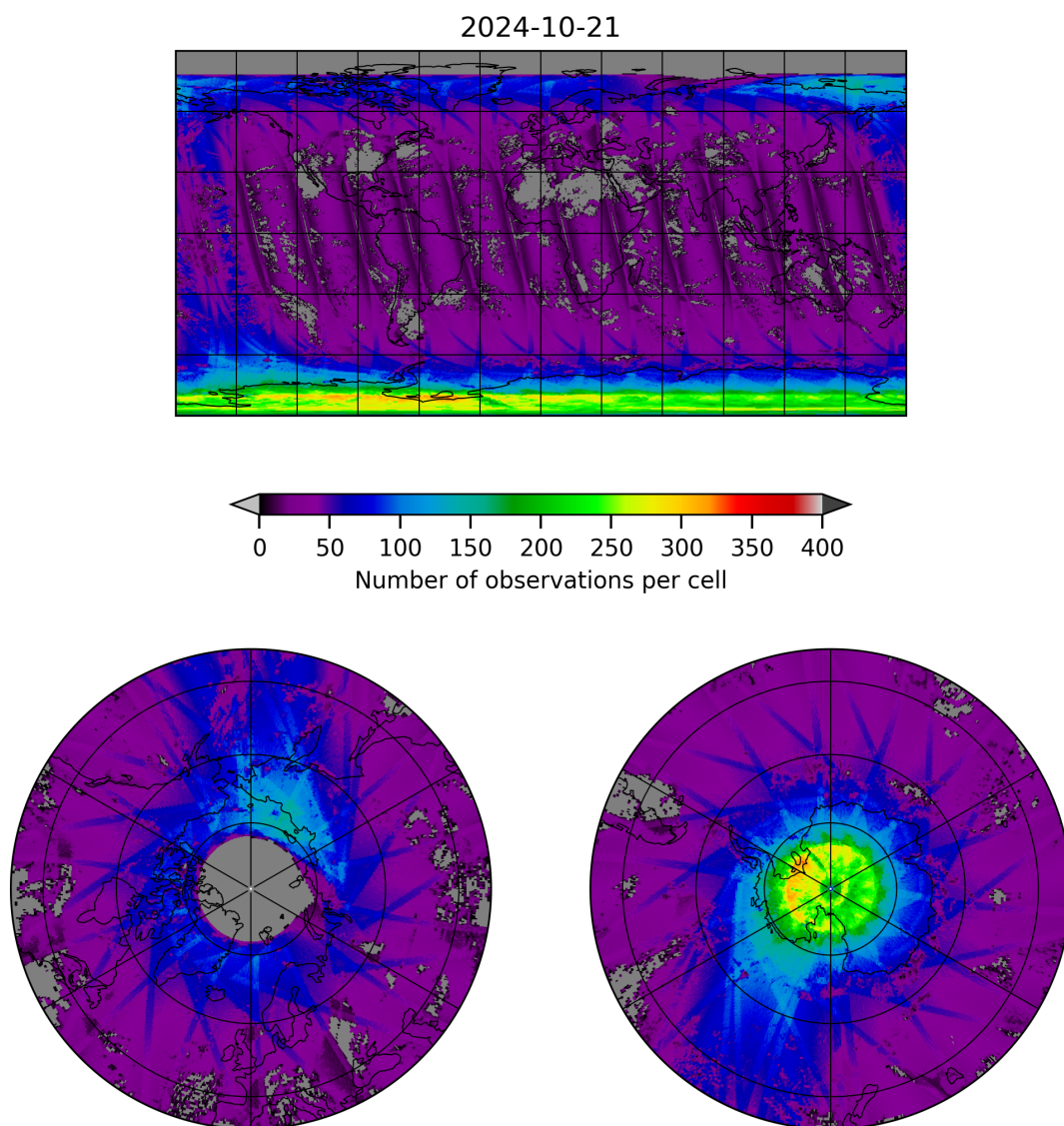
Figure 21: Map of the number of observations for 2024-10-20 to 2024-10-22
