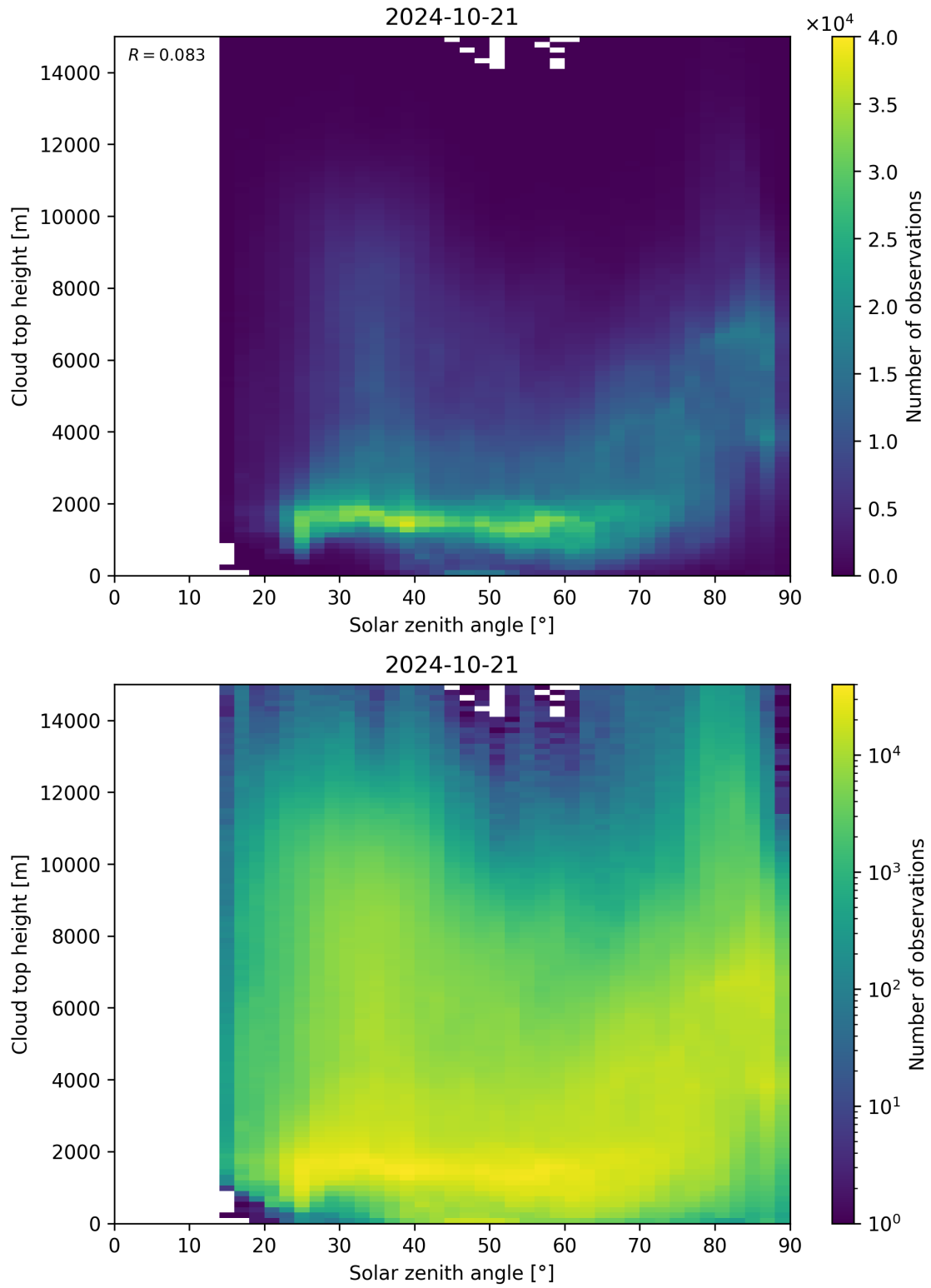
Figure 104: Scatter density plot of “Solar zenith angle” against “Cloud top height” for 2024-10-20 to 2024-10-22.
