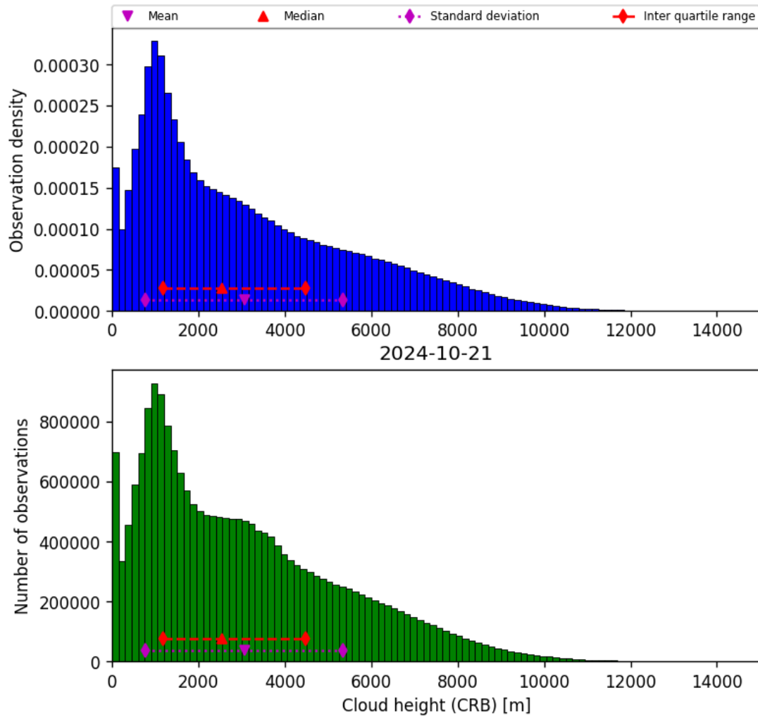
Figure 43: Histogram of “Cloud height (CRB)” for 2024-10-20 to 2024-10-22
