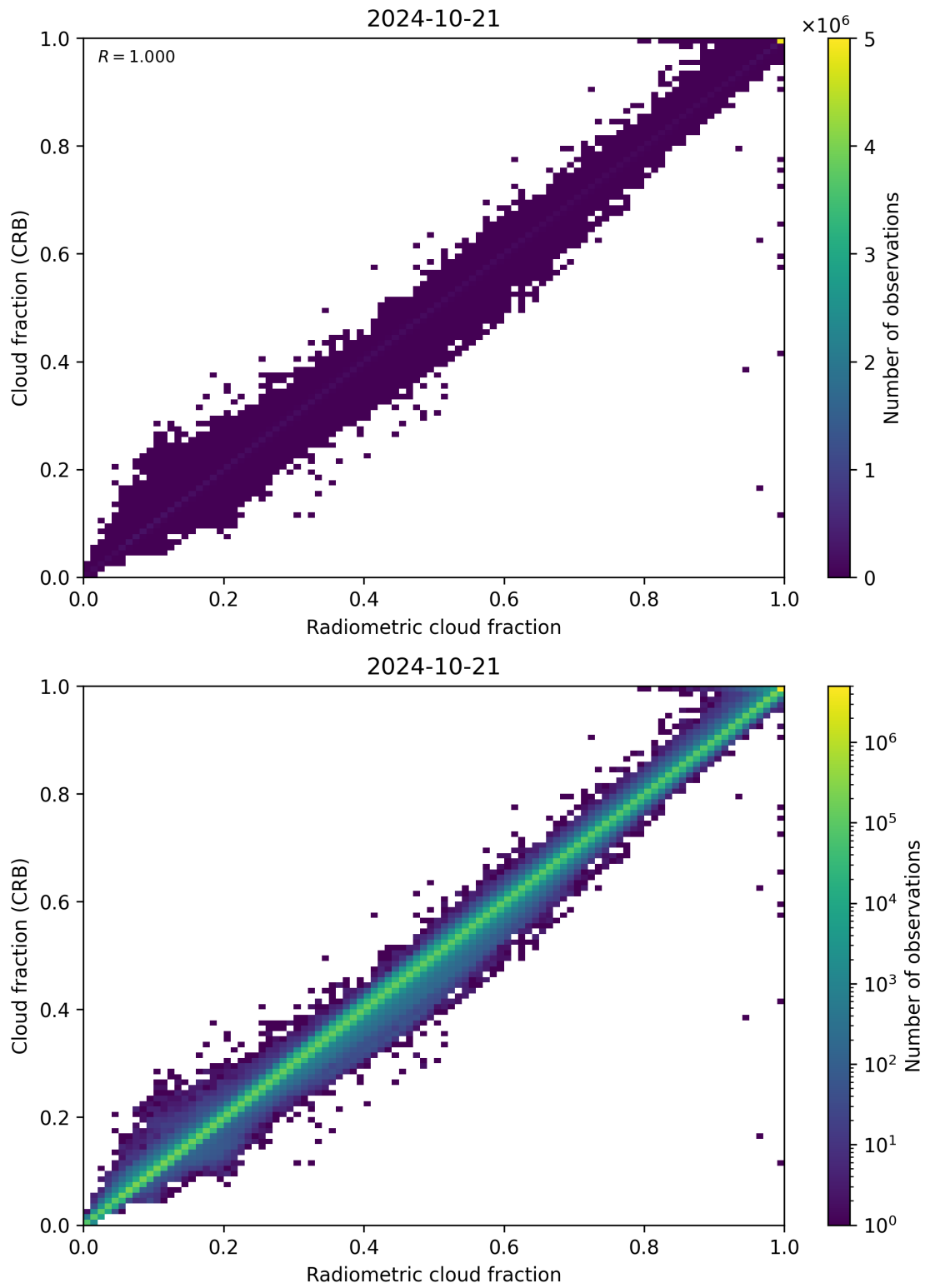
Figure 73: Scatter density plot of “Radiometric cloud fraction” against “Cloud fraction (CRB)” for 2024-10-20 to 2024-10-22.
