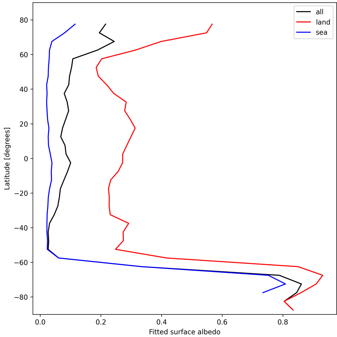
Figure 29: Zonal average of “Fitted surface albedo” for 2024-10-20 to 2024-10-22.
