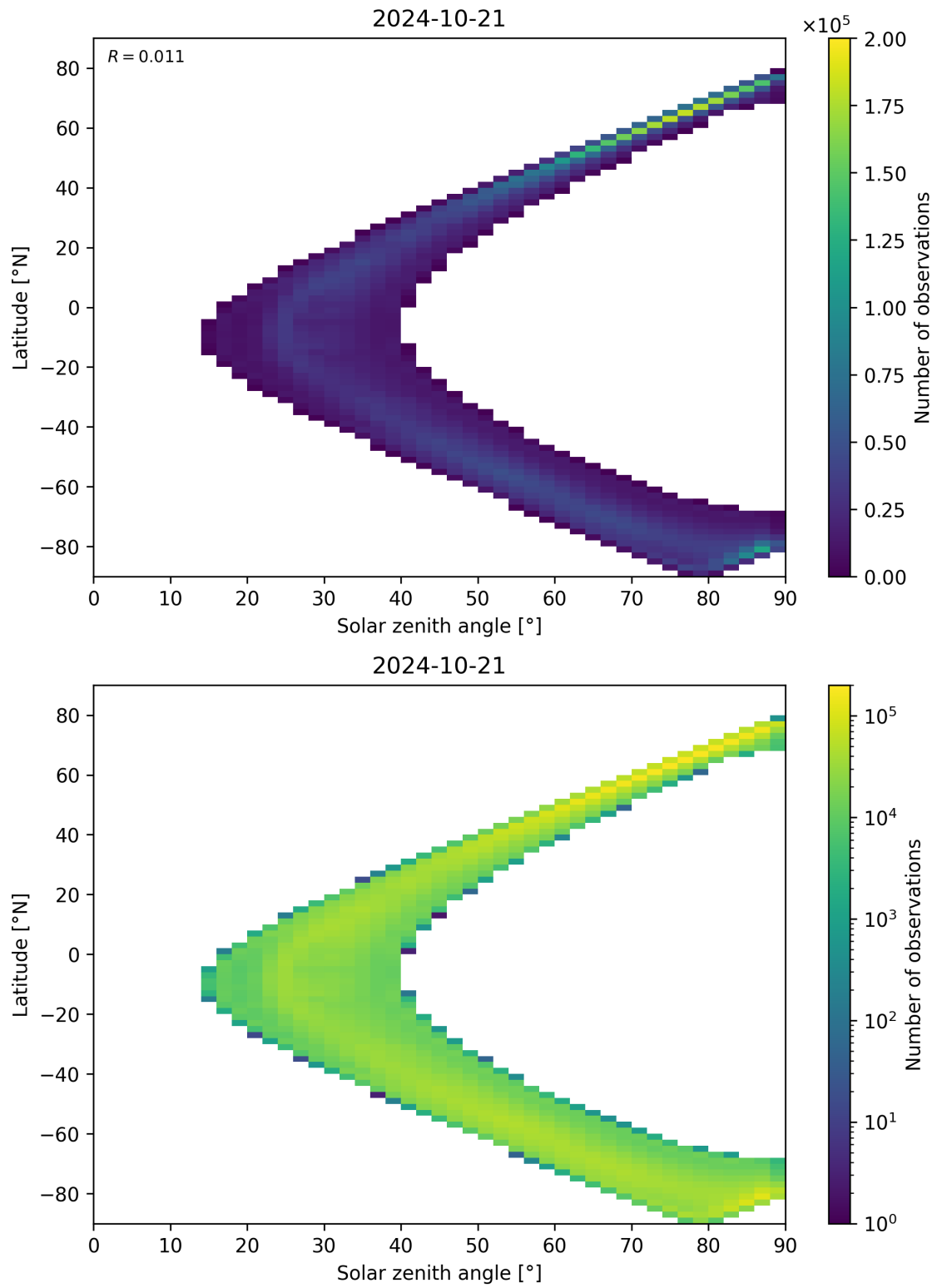
Figure 105: Scatter density plot of “Solar zenith angle” against “Latitude” for 2024-10-20 to 2024-10-22.
