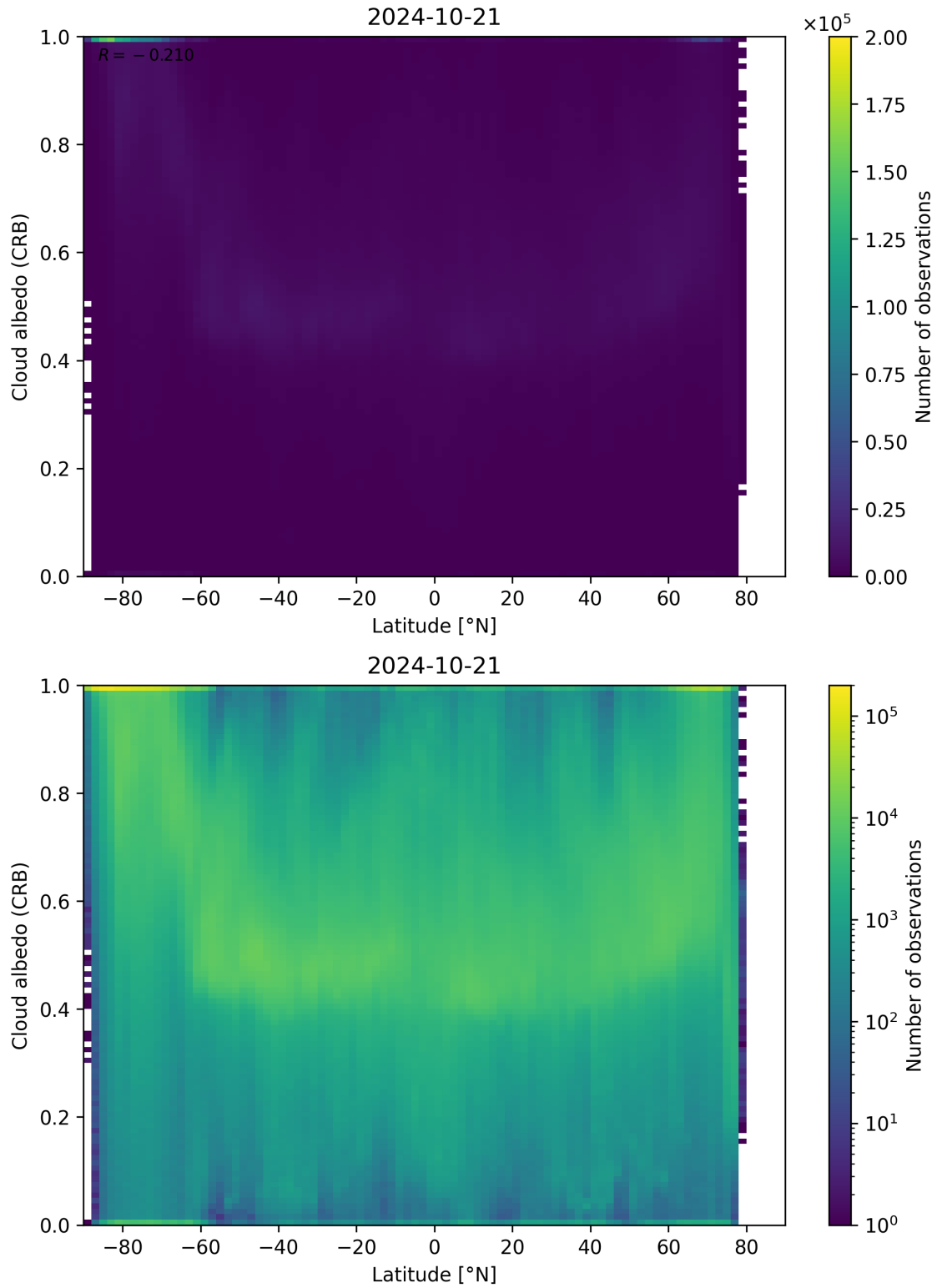
Figure 91: Scatter density plot of “Latitude” against “Cloud albedo (CRB)” for 2024-10-20 to 2024-10-22.
