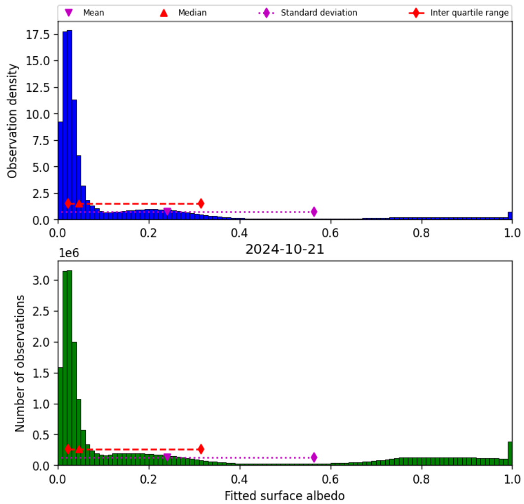
Figure 45: Histogram of “Fitted surface albedo” for 2024-10-20 to 2024-10-22
