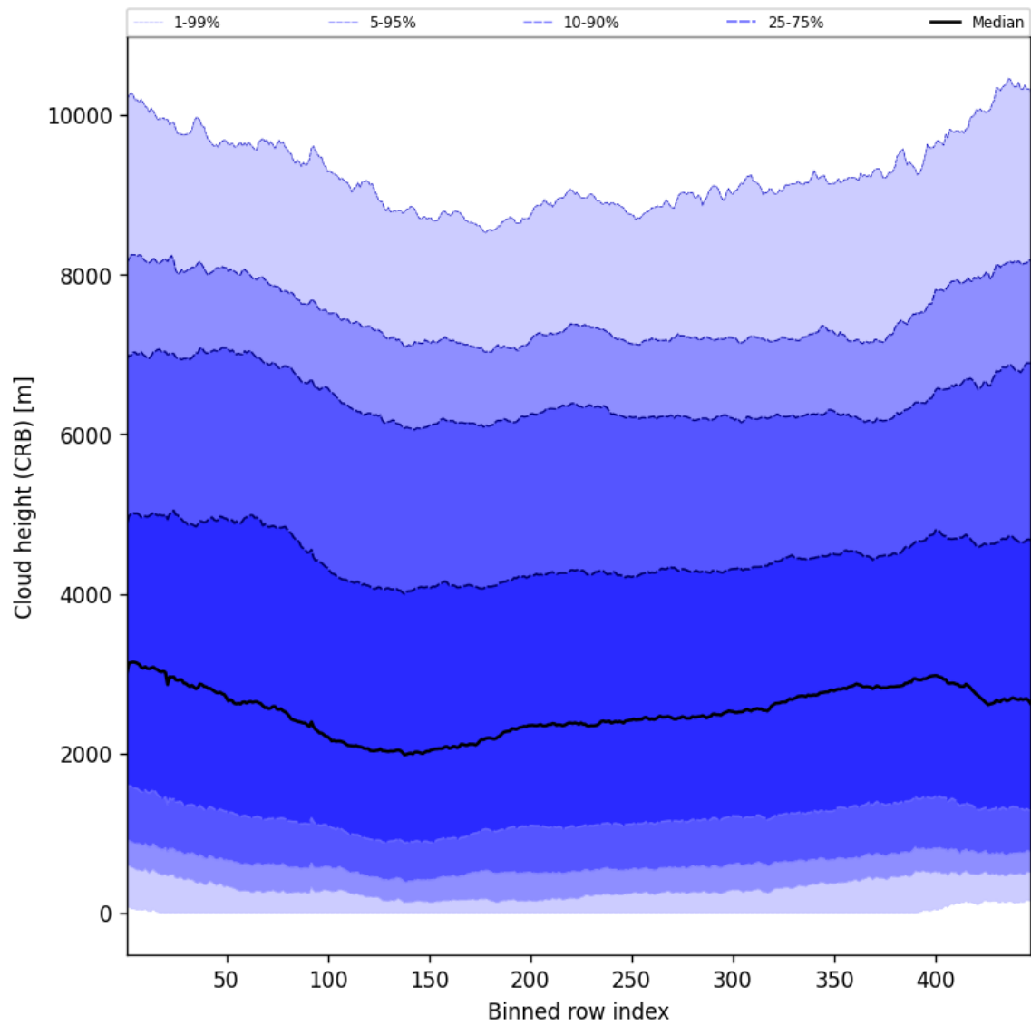
Figure 59: Along track statistics of “Cloud height (CRB)” for 2024-10-20 to 2024-10-22
