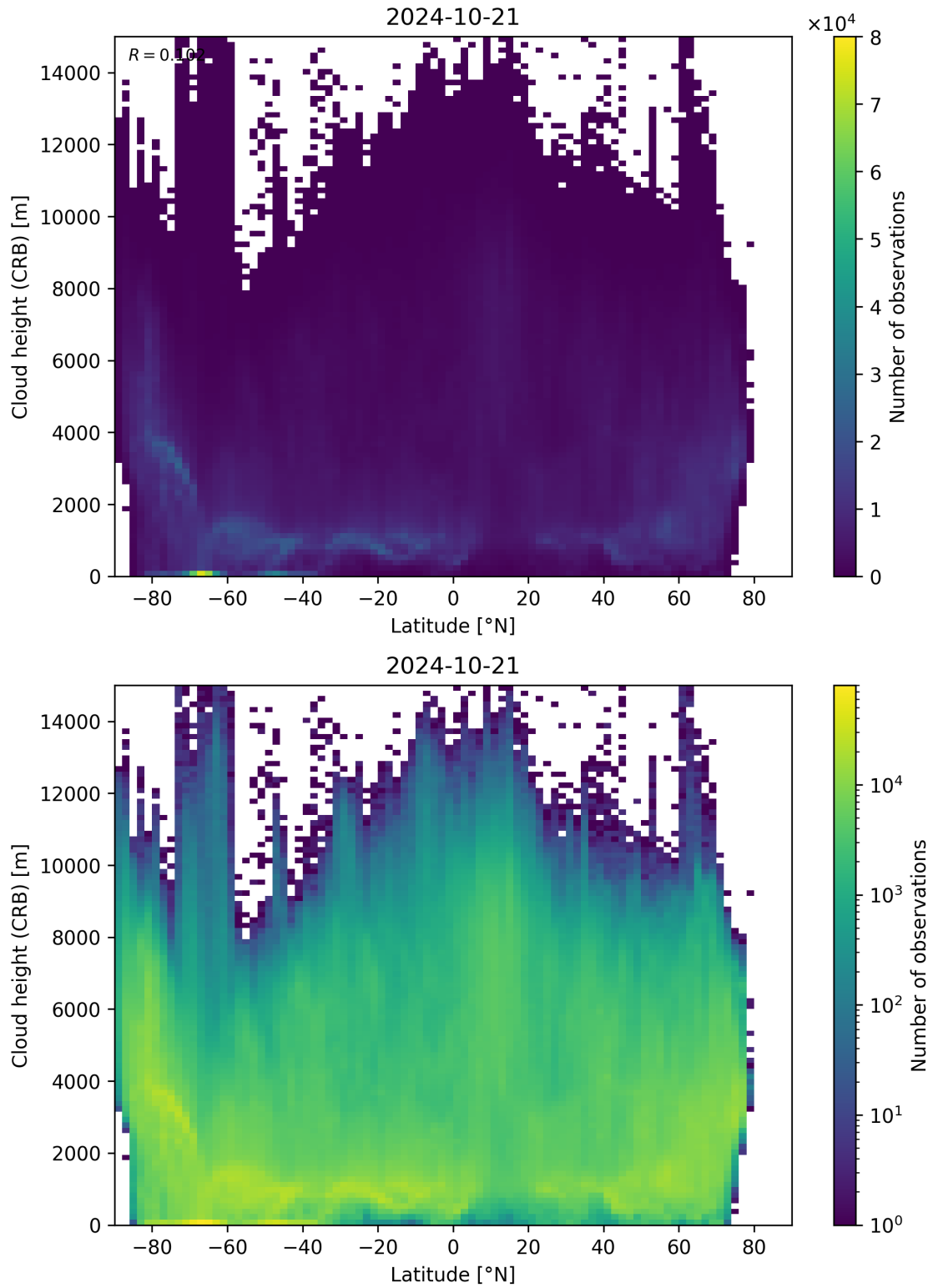
Figure 95: Scatter density plot of “Latitude” against “Cloud height (CRB)” for 2024-10-20 to 2024-10-22.
