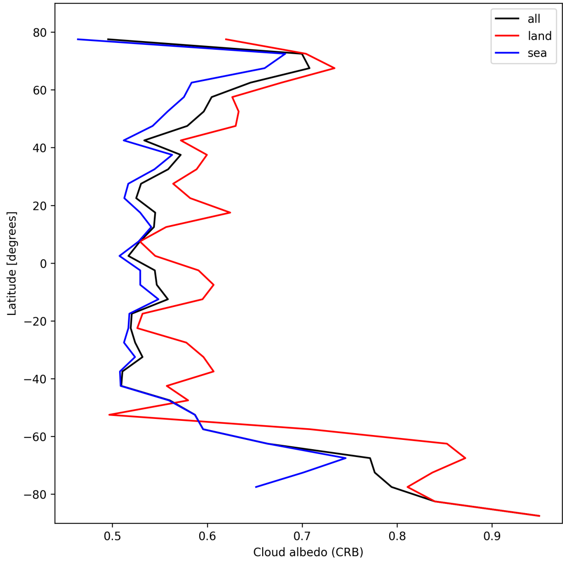
Figure 28: Zonal average of “Cloud albedo (CRB)” for 2024-10-20 to 2024-10-22.
