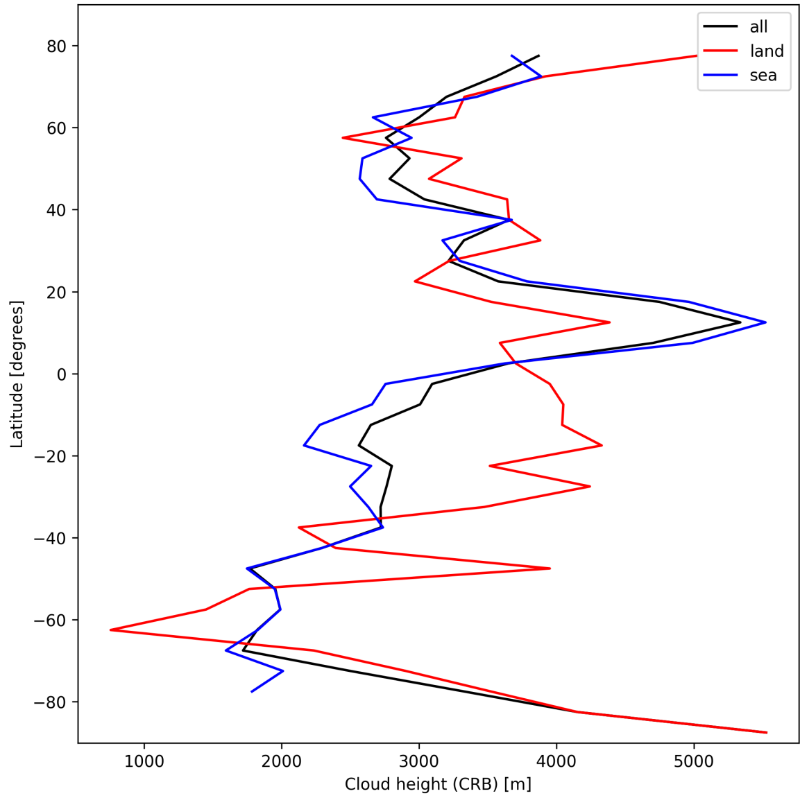
Figure 27: Zonal average of “Cloud height (CRB)” for 2024-10-20 to 2024-10-22.
