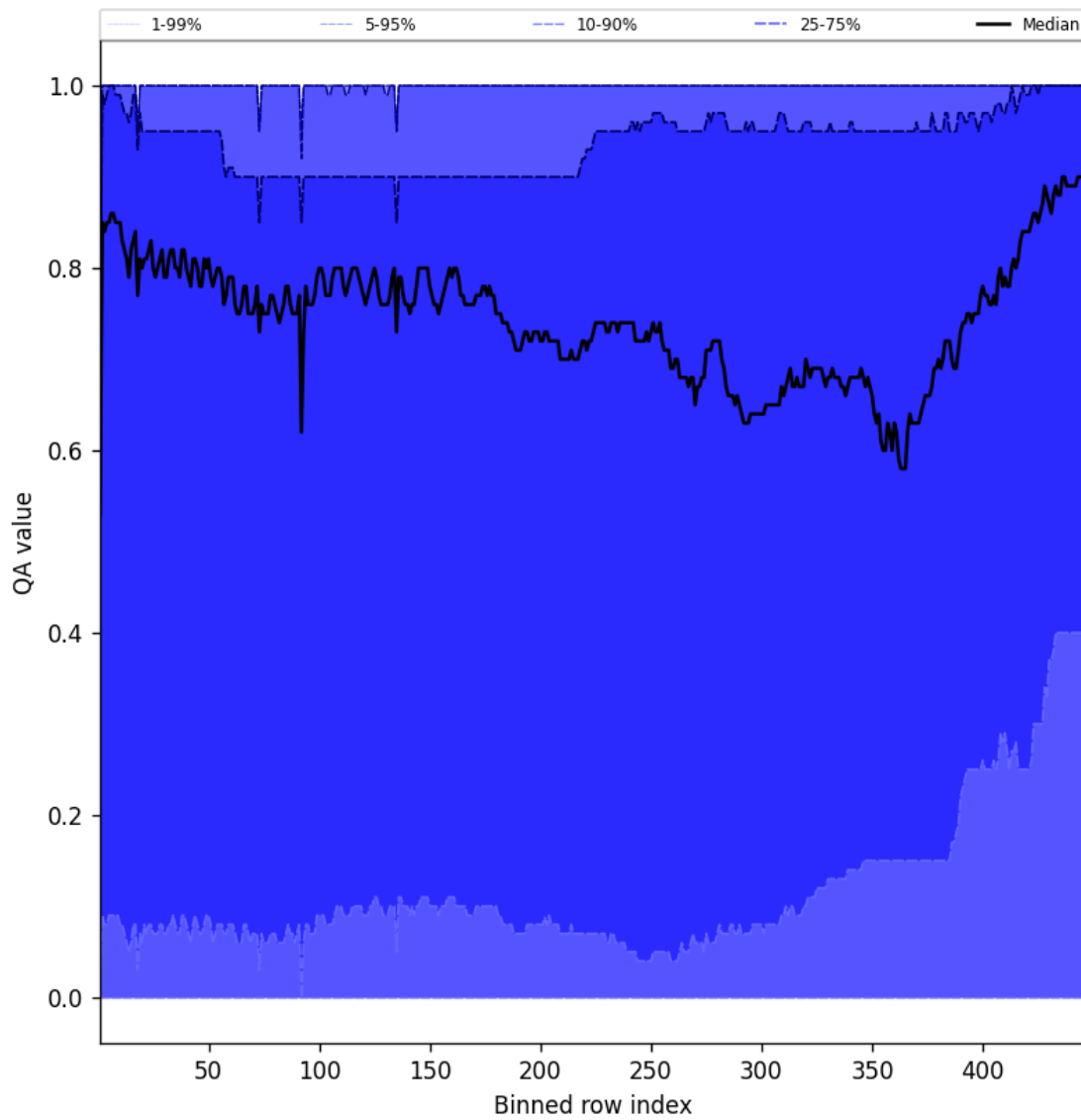
Figure 54: Along track statistics of “QA value” for 2024-10-20 to 2024-10-22
