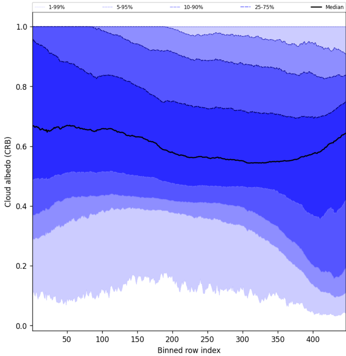
Figure 60: Along track statistics of “Cloud albedo (CRB)” for 2024-10-20 to 2024-10-22
