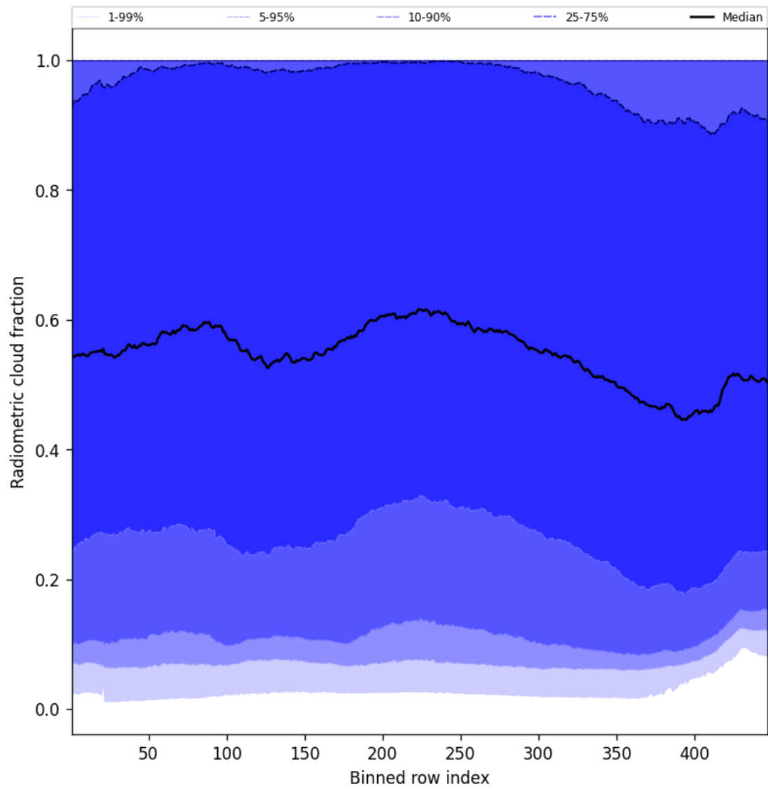
Figure 55: Along track statistics of “Radiometric cloud fraction” for 2024-10-20 to 2024-10-22
