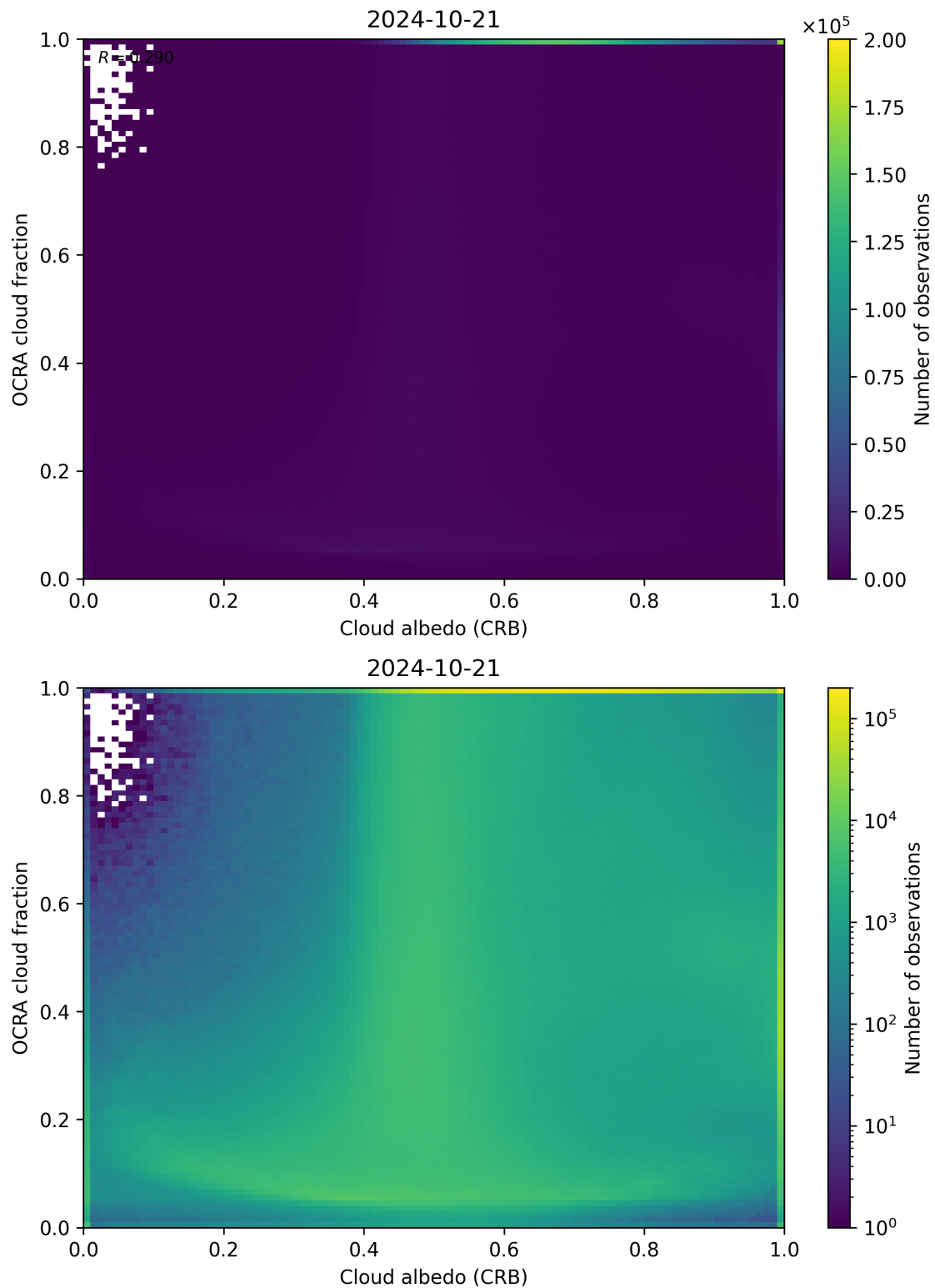
Figure 70: Scatter density plot of “Cloud albedo (CRB)” against “OCRA cloud fraction” for 2024-10-20 to 2024-10-22.
