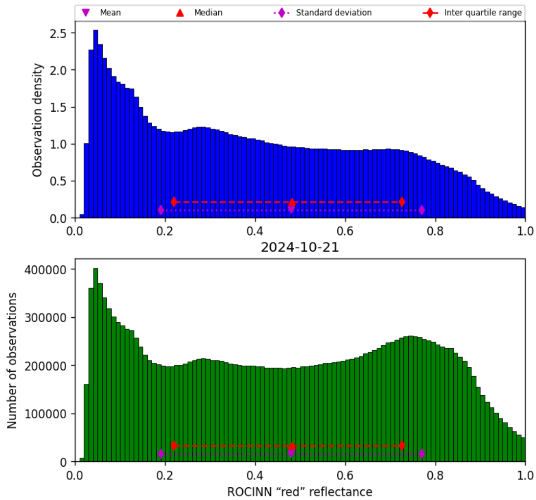
Figure 53: Histogram of “ROCINN “red” reflectance” for 2024-10-20 to 2024-10-22
