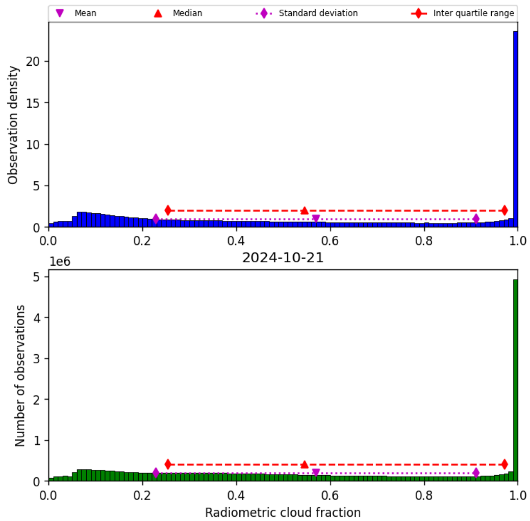
Figure 39: Histogram of “Radiometric cloud fraction” for 2024-10-20 to 2024-10-22
