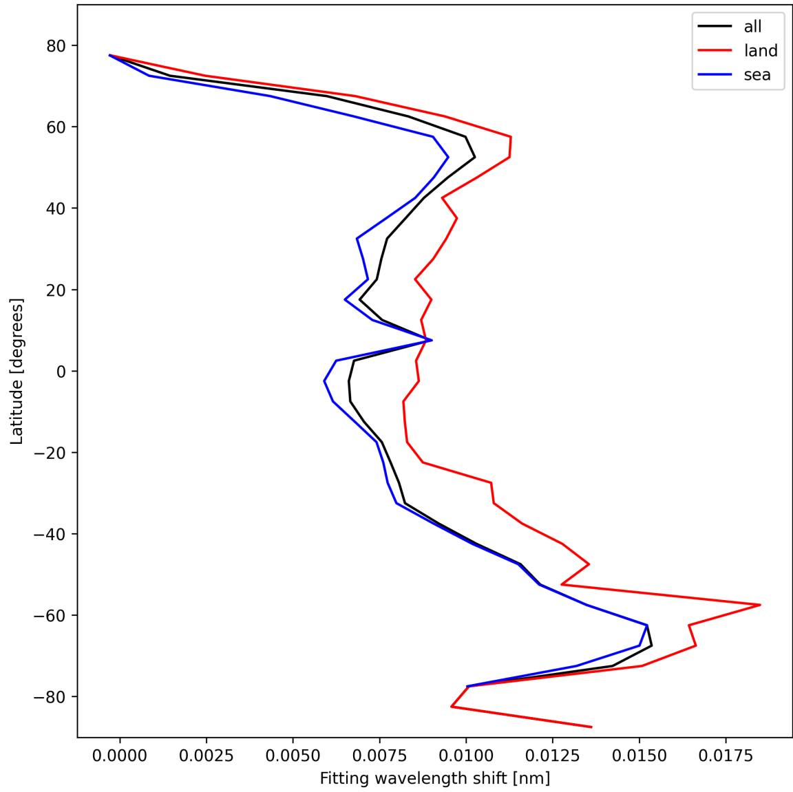
Figure 33: Zonal average of “Fitting wavelength shift” for 2024-10-24 to 2024-10-25.
