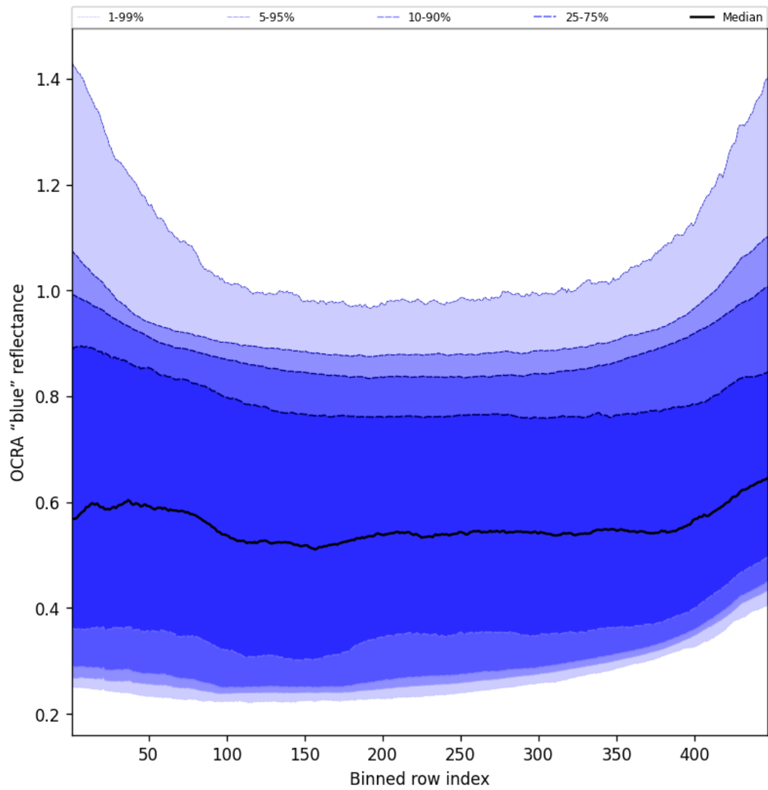
Figure 67: Along track statistics of “OCRA “blue” reflectance” for 2024-10-24 to 2024-10-25
