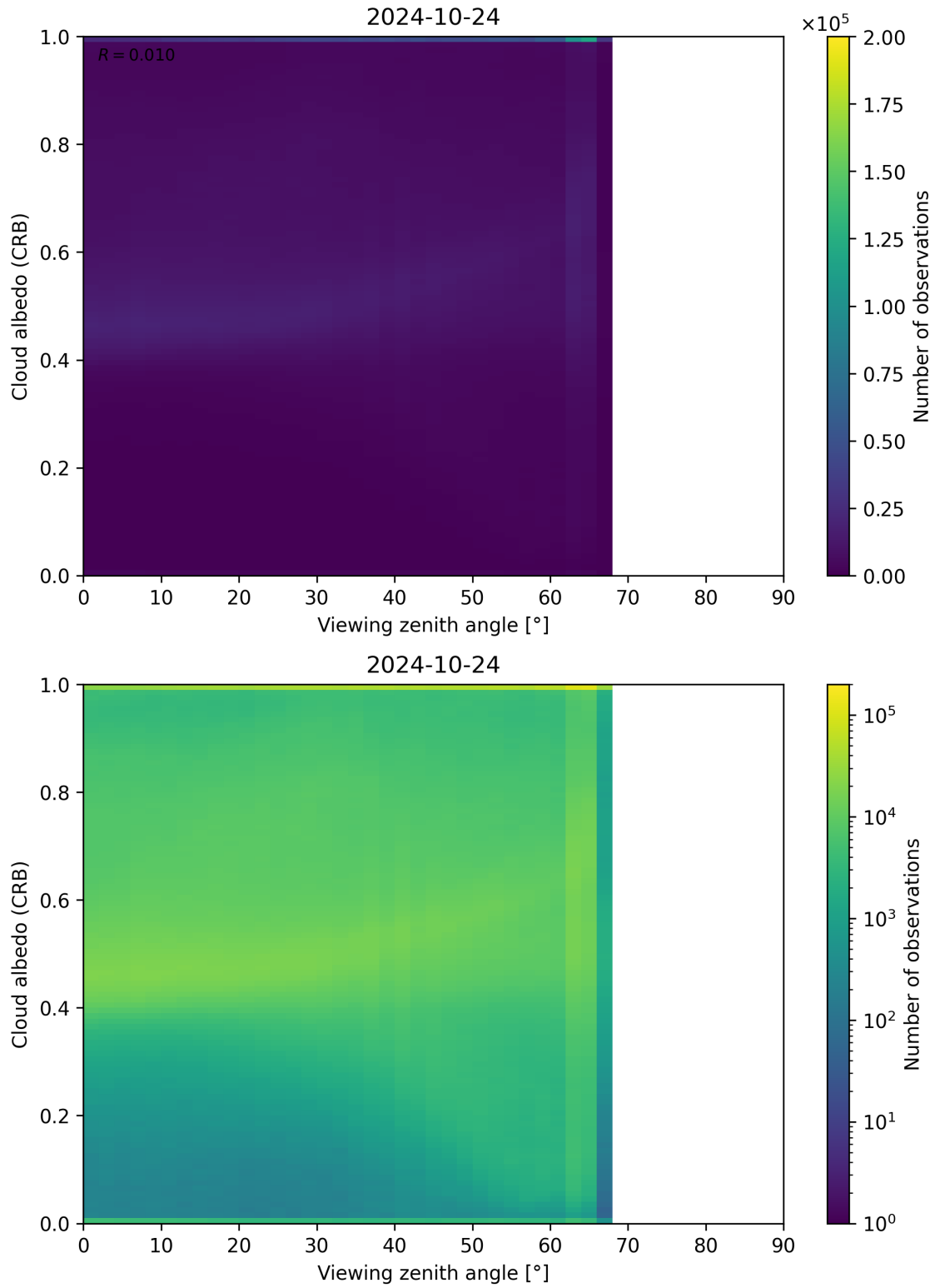
Figure 106: Scatter density plot of “Viewing zenith angle” against “Cloud albedo (CRB)” for 2024-10-24 to 2024-10-25.
