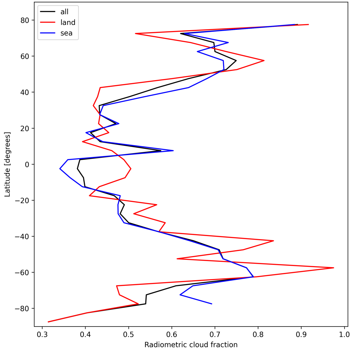
Figure 23: Zonal average of “Radiometric cloud fraction” for 2024-10-24 to 2024-10-25.
