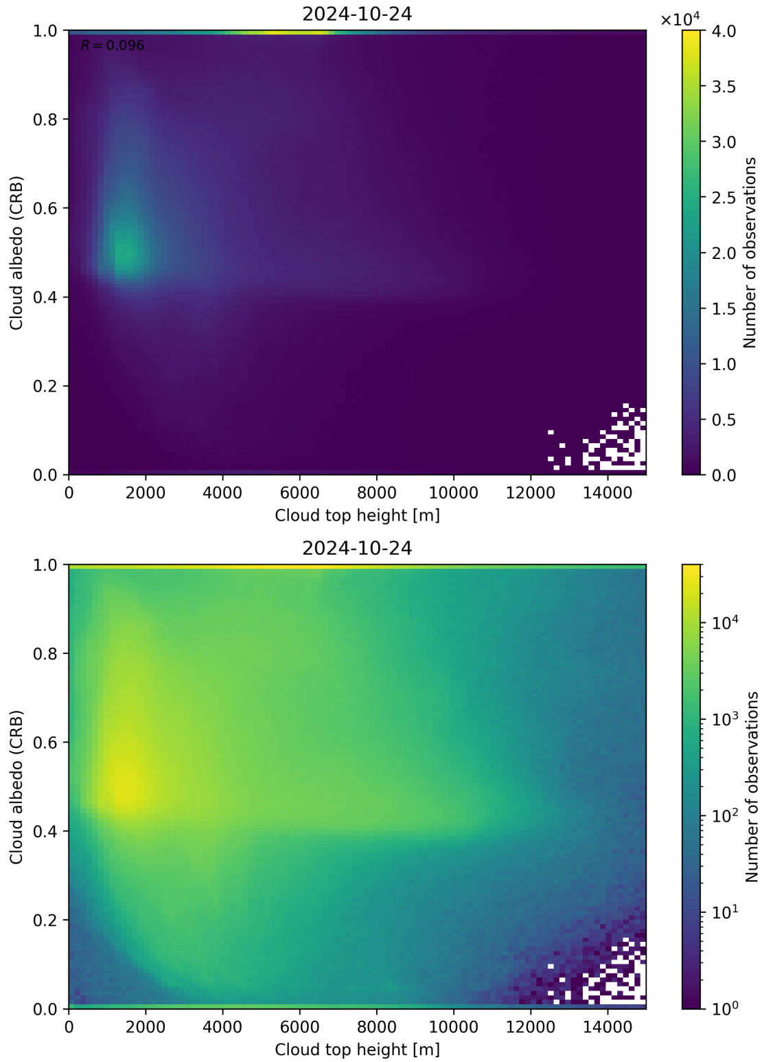
Figure 86: Scatter density plot of “Cloud top height” against “Cloud albedo (CRB)” for 2024-10-24 to 2024-10-25.
