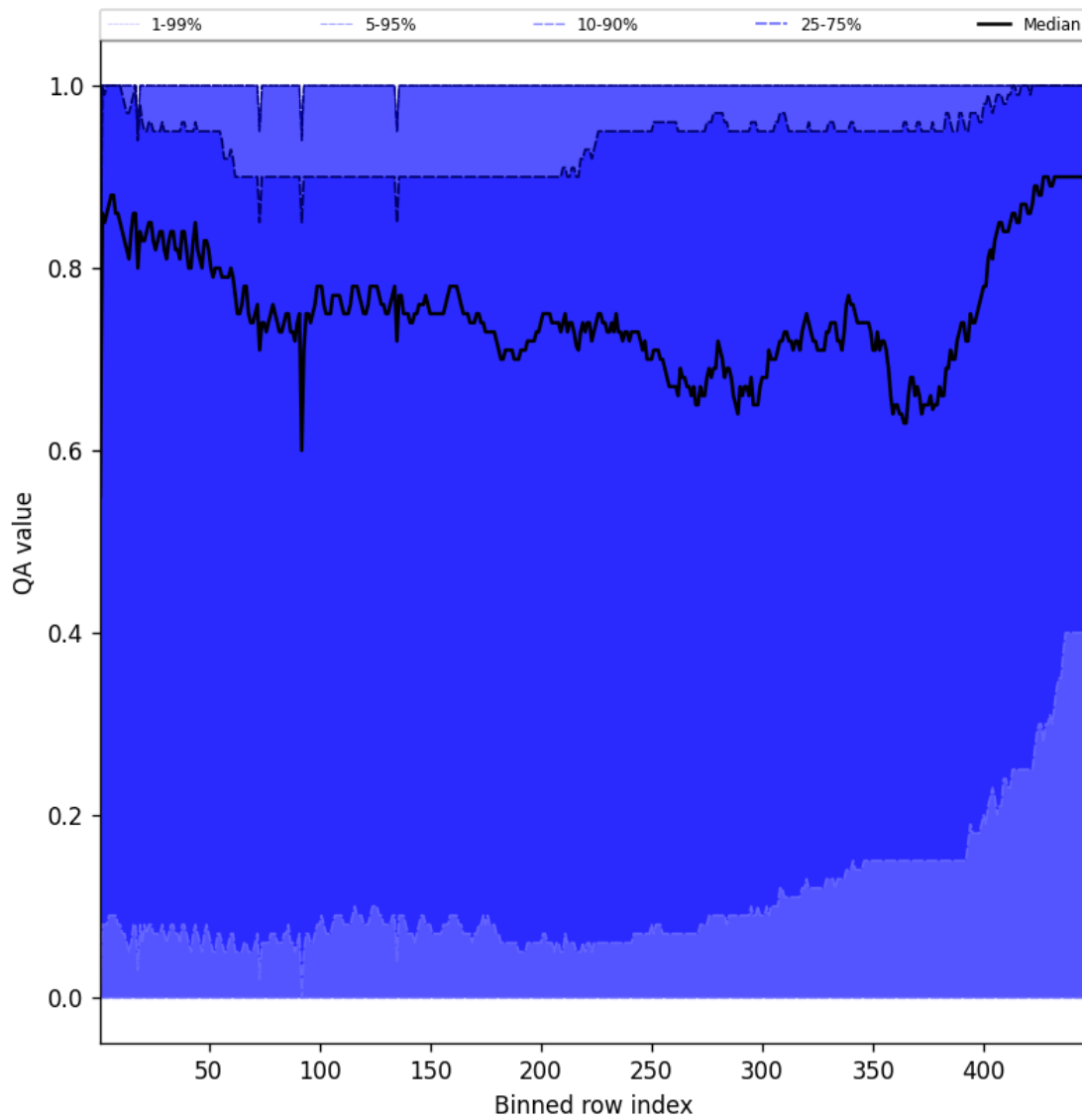
Figure 54: Along track statistics of “QA value” for 2024-10-24 to 2024-10-25
