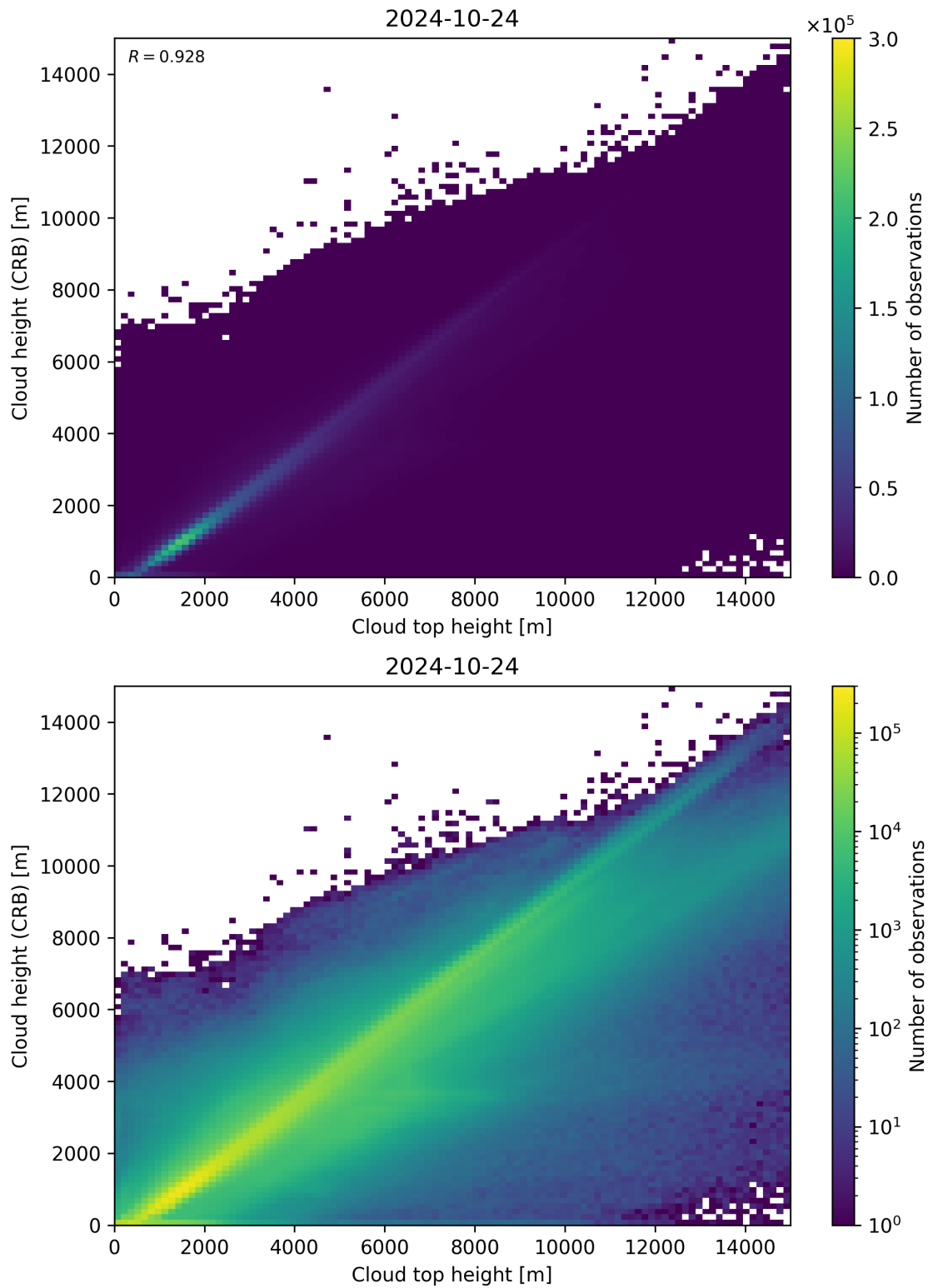
Figure 89: Scatter density plot of “Cloud top height” against “Cloud height (CRB)” for 2024-10-24 to 2024-10-25.
