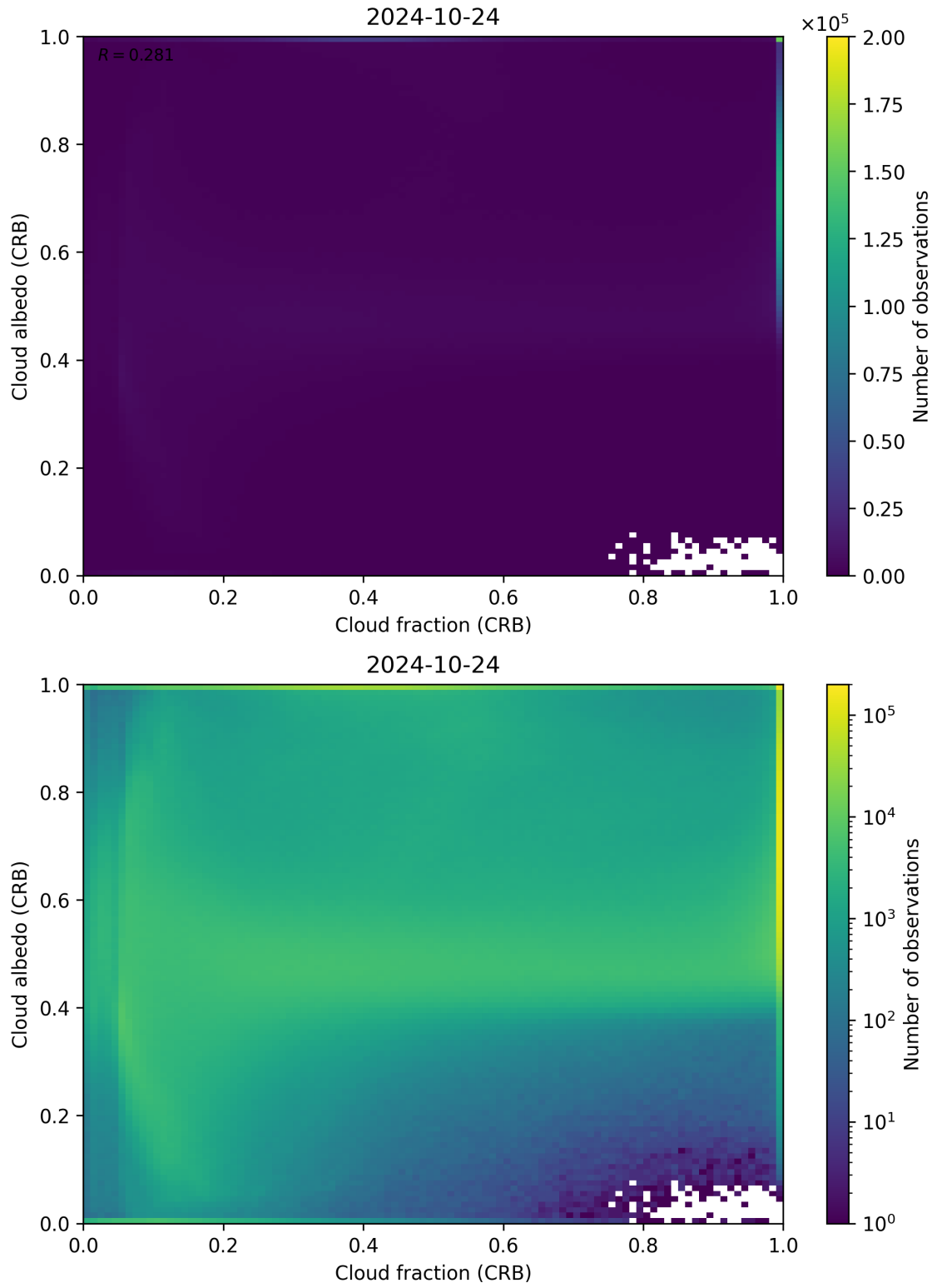
Figure 77: Scatter density plot of “Cloud fraction (CRB)” against “Cloud albedo (CRB)” for 2024-10-24 to 2024-10-25.
