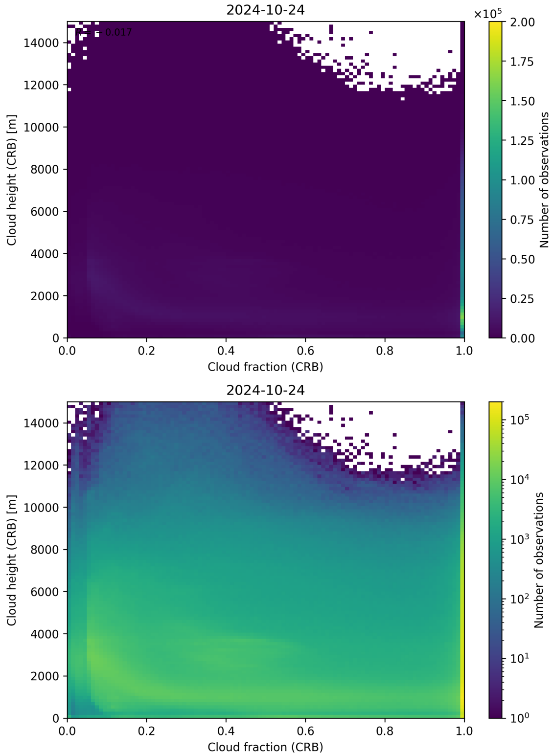
Figure 79: Scatter density plot of “Cloud fraction (CRB)” against “Cloud height (CRB)” for 2024-10-24 to 2024-10-25.
