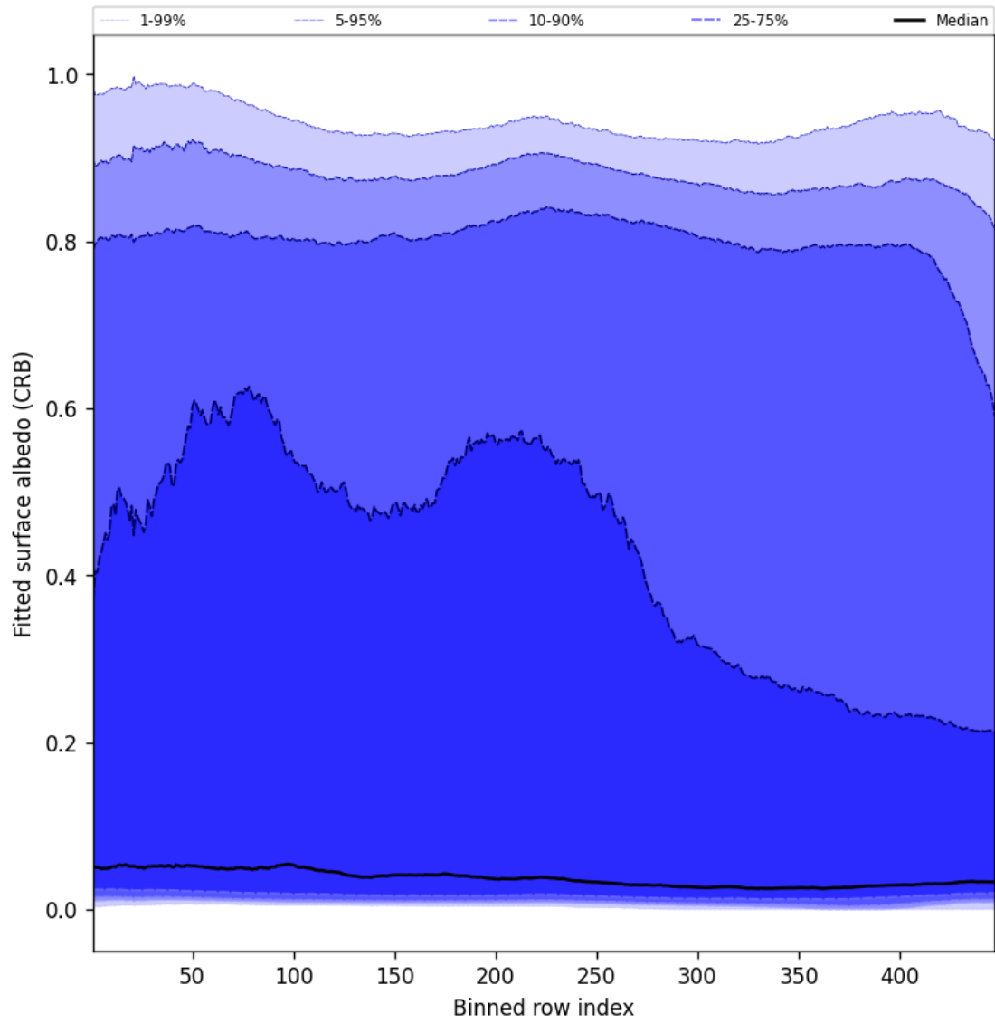
Figure 62: Along track statistics of “Fitted surface albedo (CRB)” for 2024-10-24 to 2024-10-25
