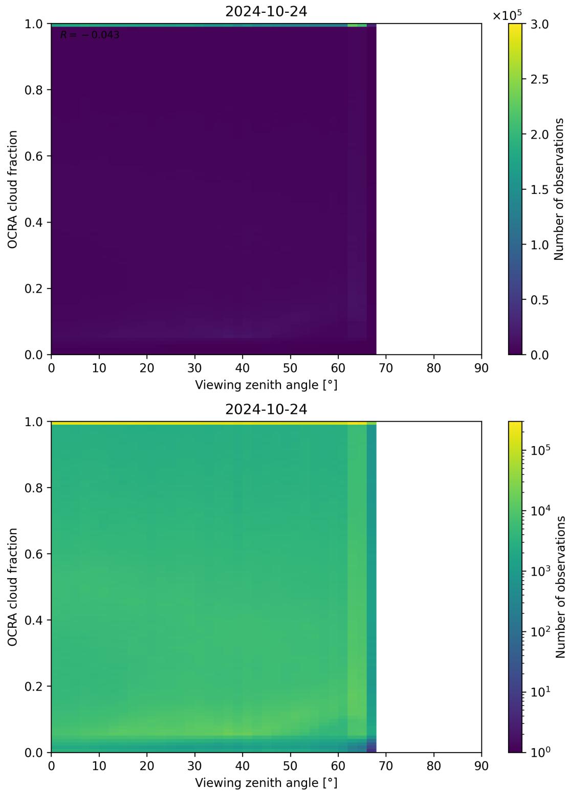
Figure 108: Scatter density plot of “Viewing zenith angle” against “OCRA cloud fraction” for 2024-10-24 to 2024-10-25.
