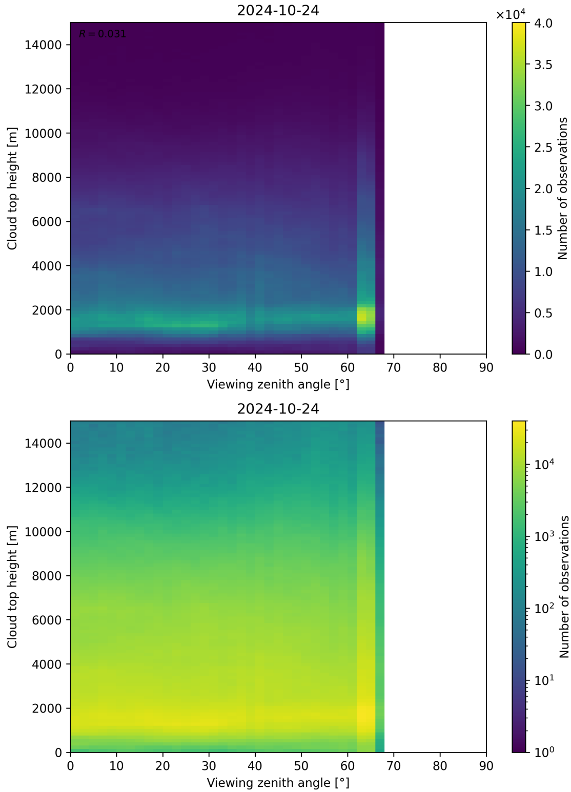
Figure 112: Scatter density plot of “Viewing zenith angle” against “Cloud top height” for 2024-10-24 to 2024-10-25.
