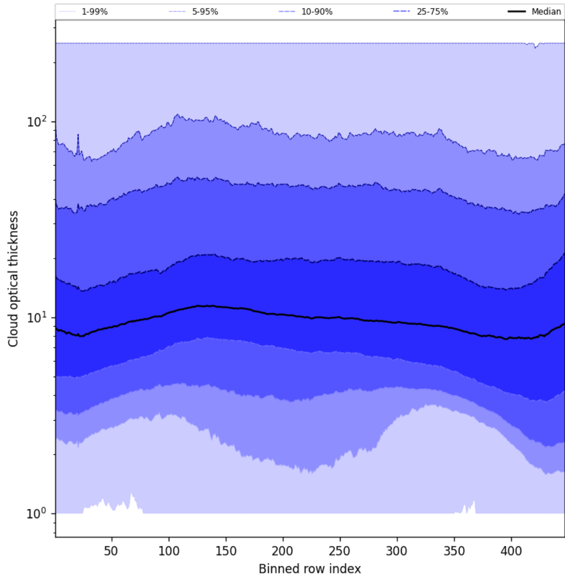
Figure 57: Along track statistics of “Cloud optical thickness” for 2024-10-24 to 2024-10-25
