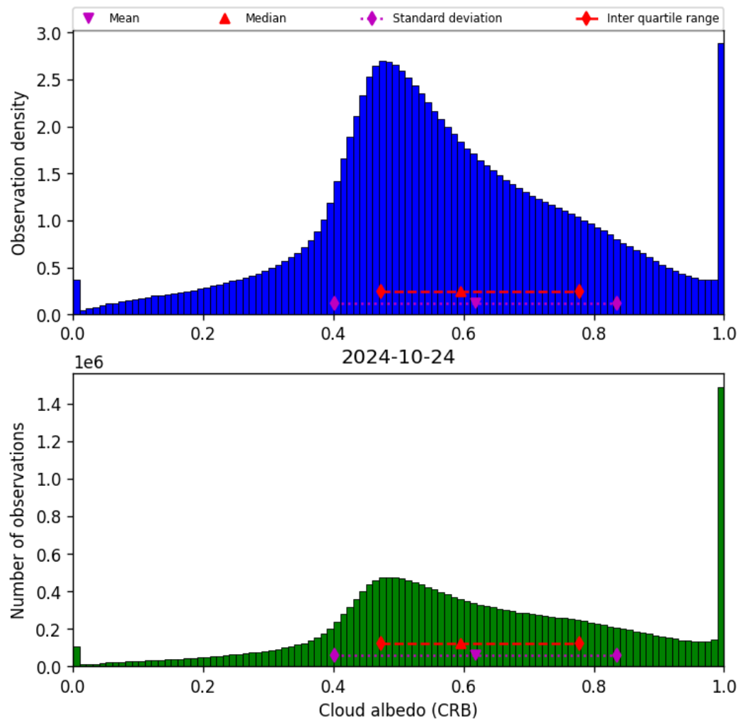
Figure 44: Histogram of “Cloud albedo (CRB)” for 2024-10-24 to 2024-10-25
