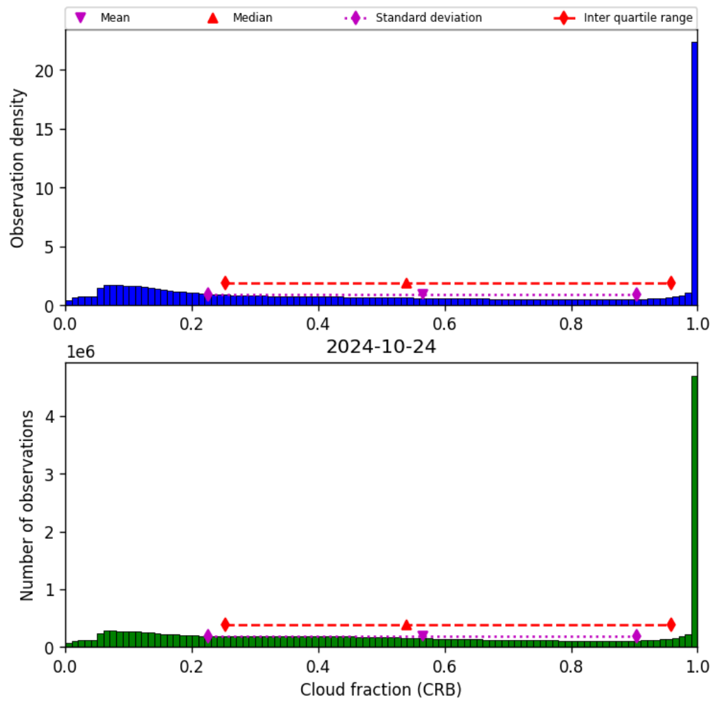
Figure 42: Histogram of “Cloud fraction (CRB)” for 2024-10-24 to 2024-10-25
