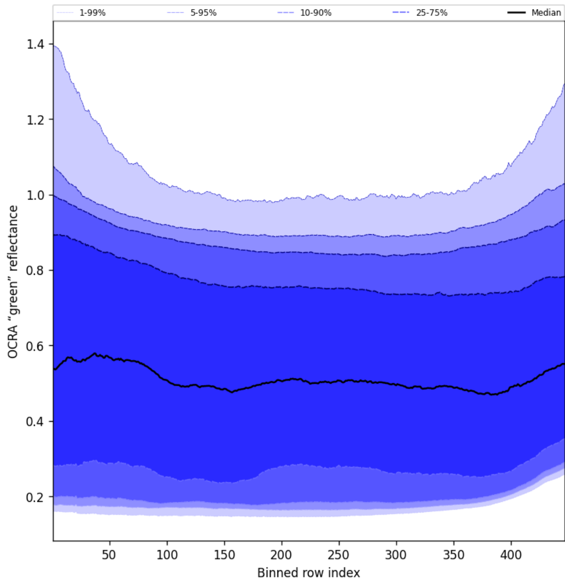
Figure 68: Along track statistics of “OCRA “green” reflectance” for 2024-10-24 to 2024-10-25
