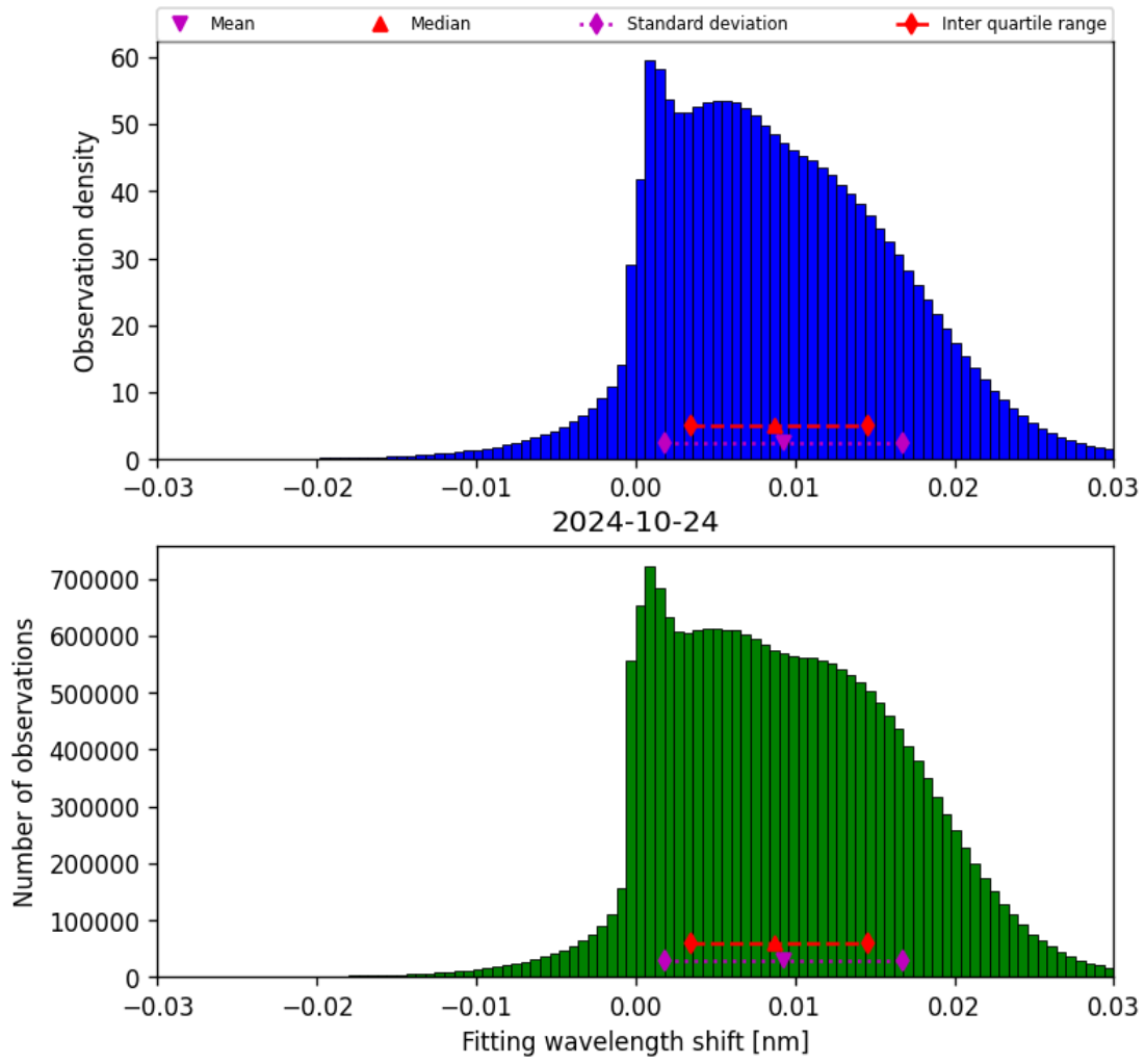
Figure 49: Histogram of “Fitting wavelength shift” for 2024-10-24 to 2024-10-25
