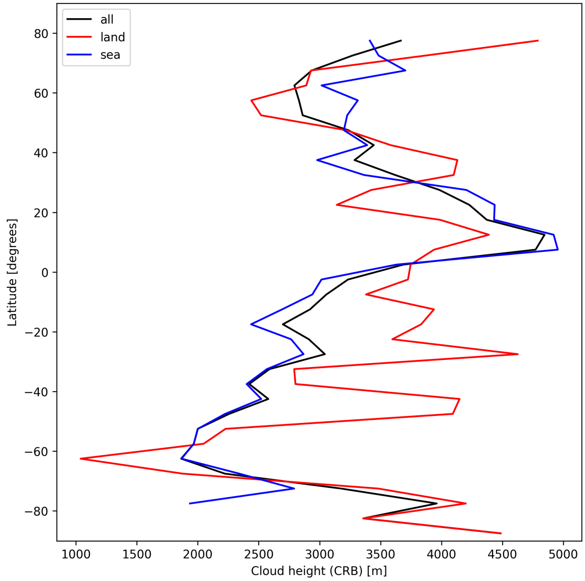
Figure 27: Zonal average of “Cloud height (CRB)” for 2024-10-24 to 2024-10-25.
