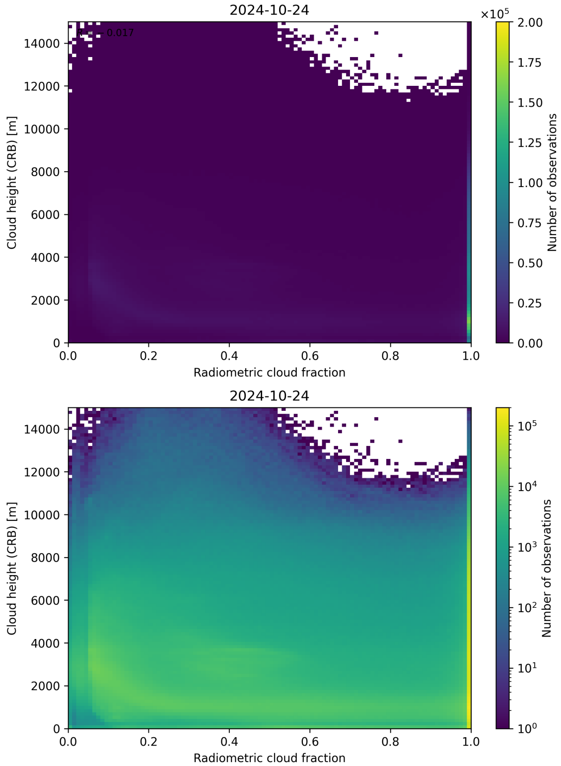
Figure 74: Scatter density plot of “Radiometric cloud fraction” against “Cloud height (CRB)” for 2024-10-24 to 2024-10-25.
