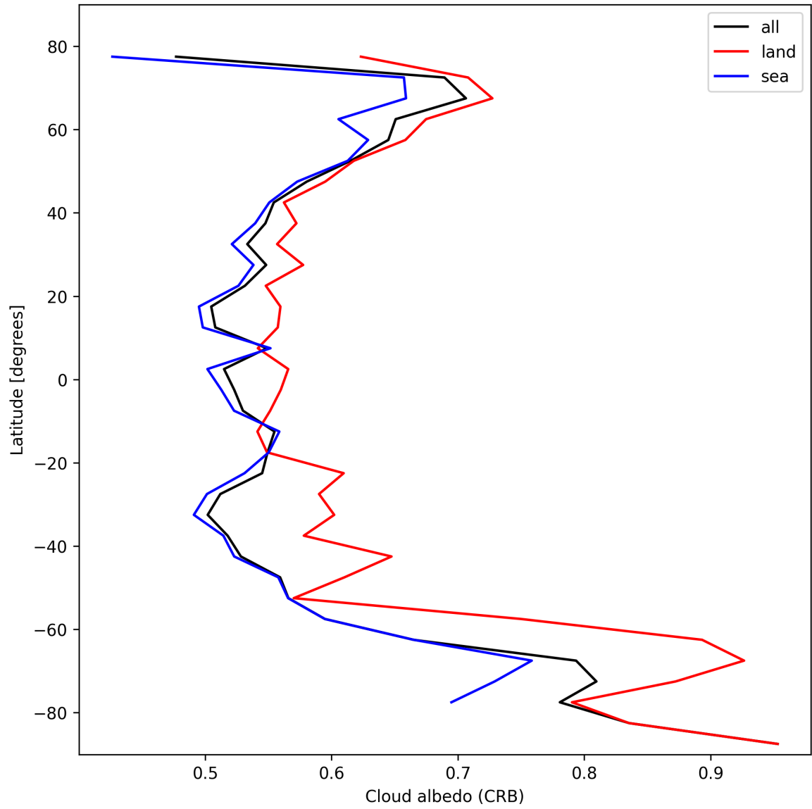
Figure 28: Zonal average of “Cloud albedo (CRB)” for 2024-10-24 to 2024-10-25.
