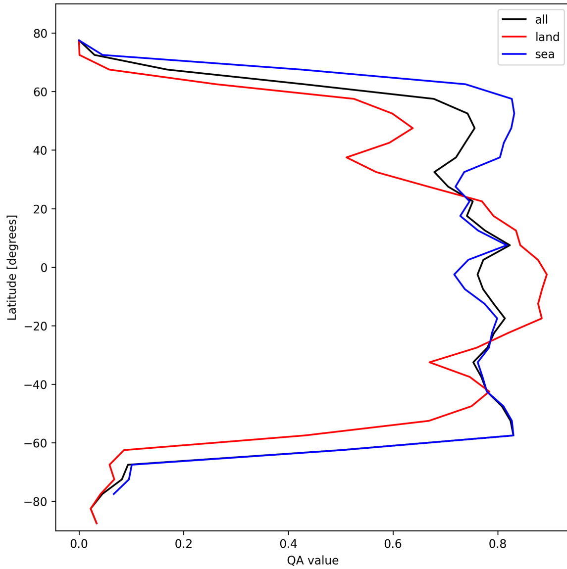
Figure 22: Zonal average of “QA value” for 2024-10-24 to 2024-10-25.
