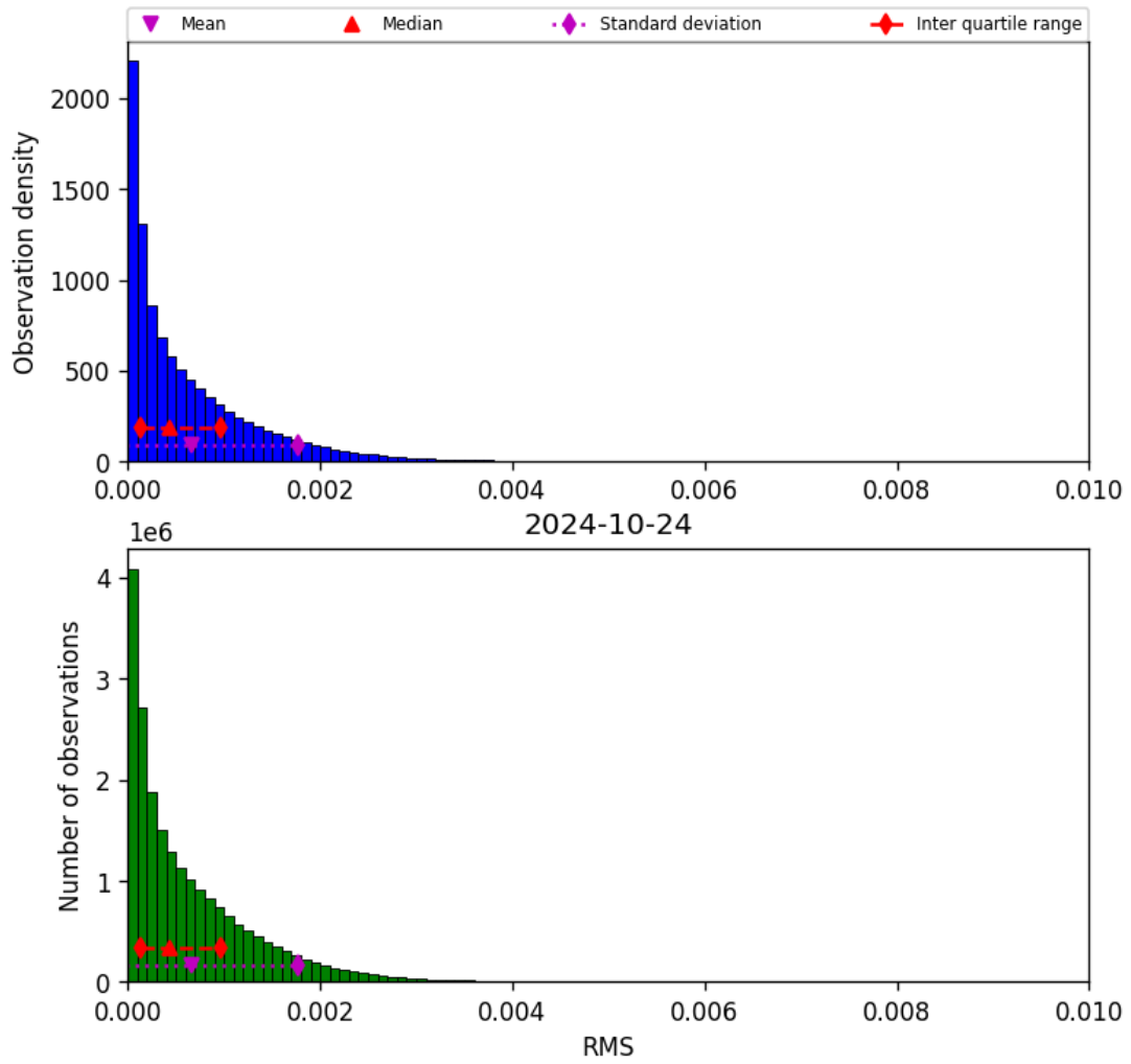
Figure 47: Histogram of “RMS” for 2024-10-24 to 2024-10-25
