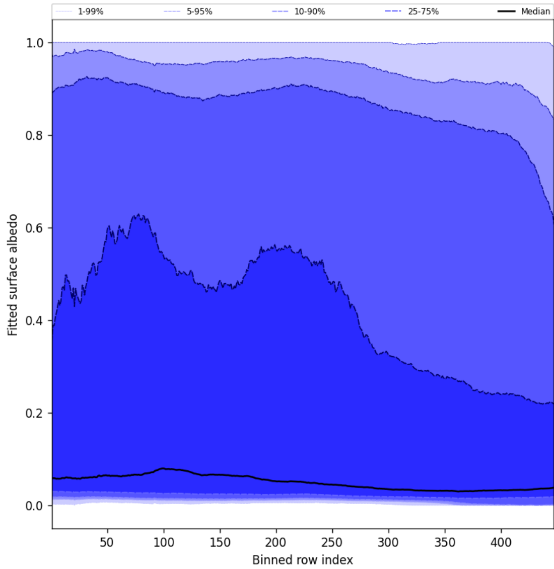
Figure 61: Along track statistics of “Fitted surface albedo” for 2024-10-24 to 2024-10-25
