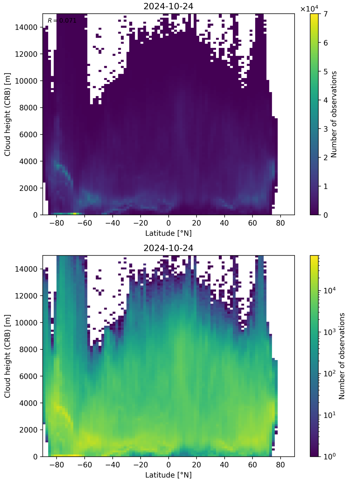
Figure 95: Scatter density plot of “Latitude” against “Cloud height (CRB)” for 2024-10-24 to 2024-10-25.
