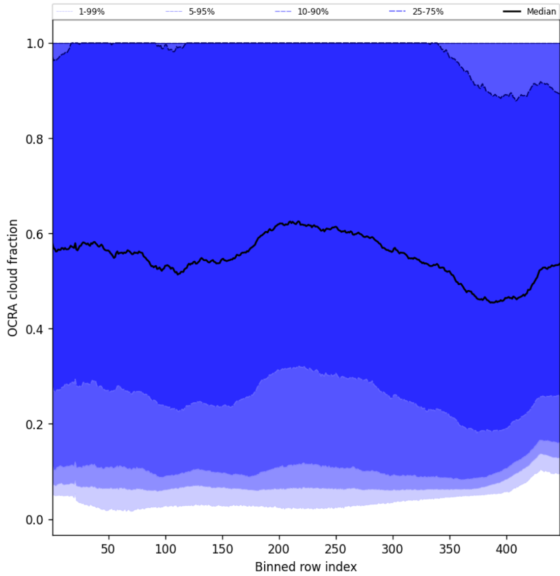
Figure 66: Along track statistics of “OCRA cloud fraction” for 2024-10-24 to 2024-10-25
