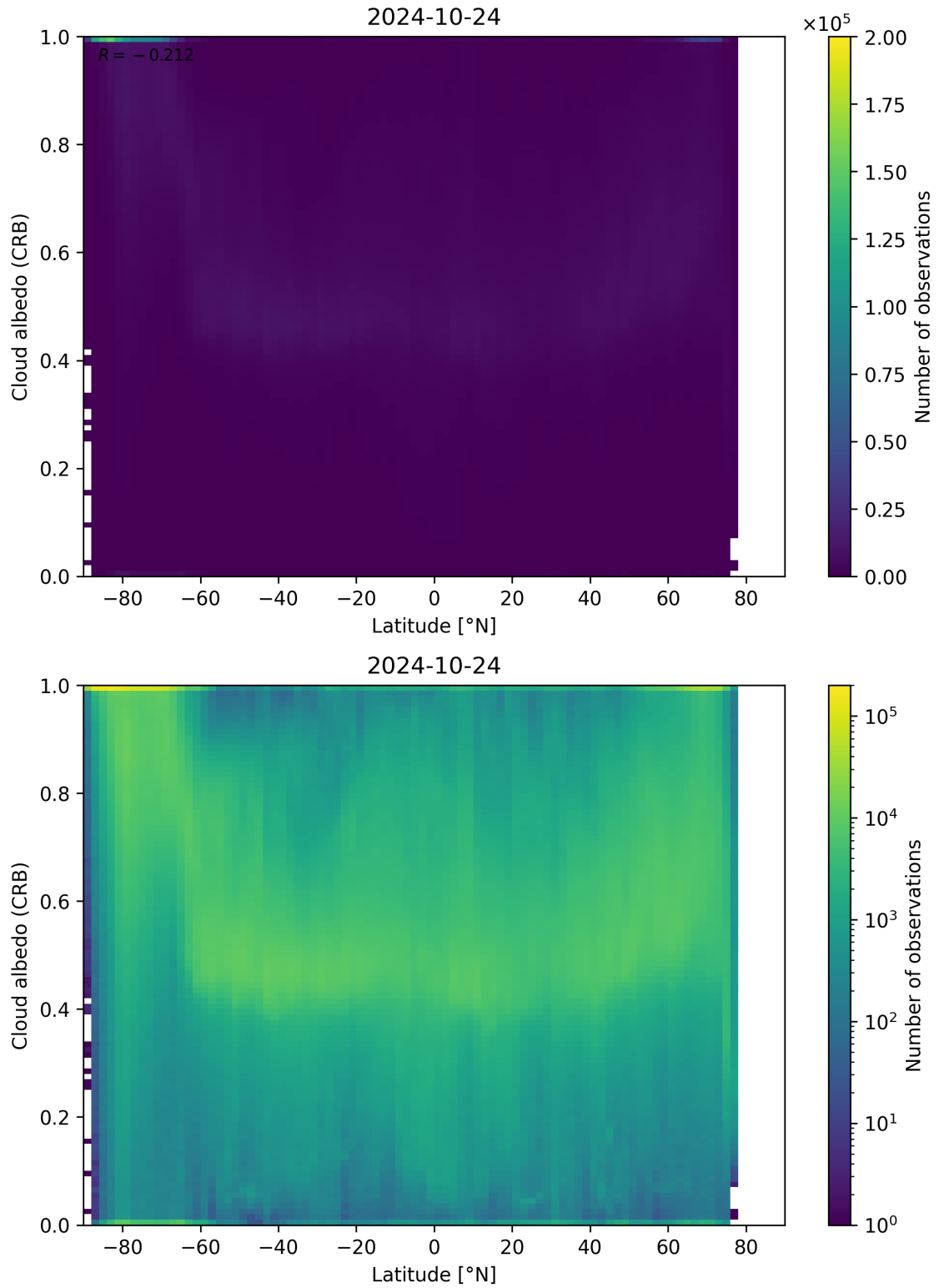
Figure 91: Scatter density plot of “Latitude” against “Cloud albedo (CRB)” for 2024-10-24 to 2024-10-25.
