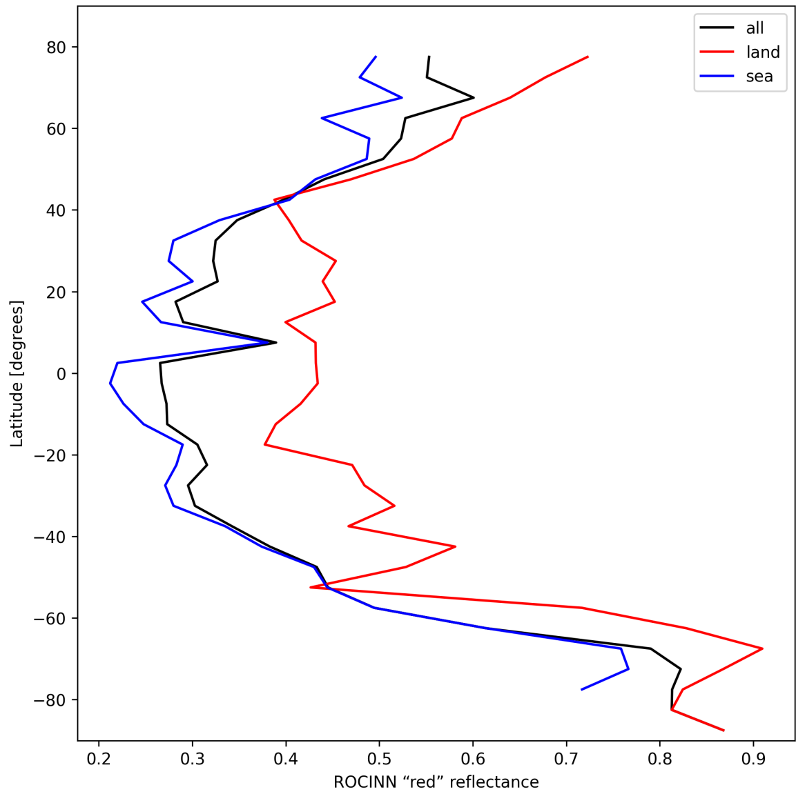
Figure 37: Zonal average of “ROCINN “red” reflectance” for 2024-10-24 to 2024-10-25.
