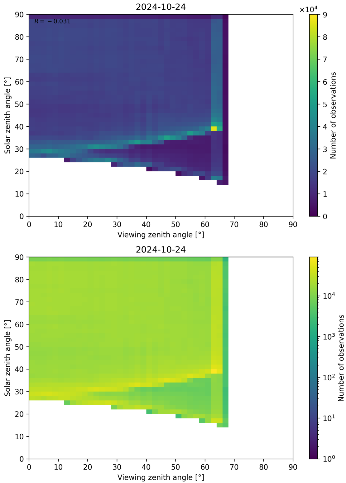
Figure 114: Scatter density plot of “Viewing zenith angle” against “Solar zenith angle” for 2024-10-24 to 2024-10-25.
