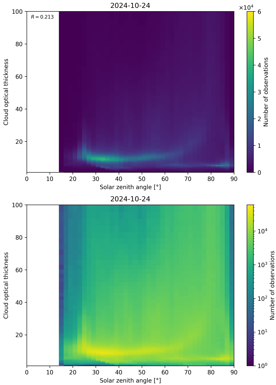
Figure 103: Scatter density plot of “Solar zenith angle” against “Cloud optical thickness” for 2024-10-24 to 2024-10-25.
