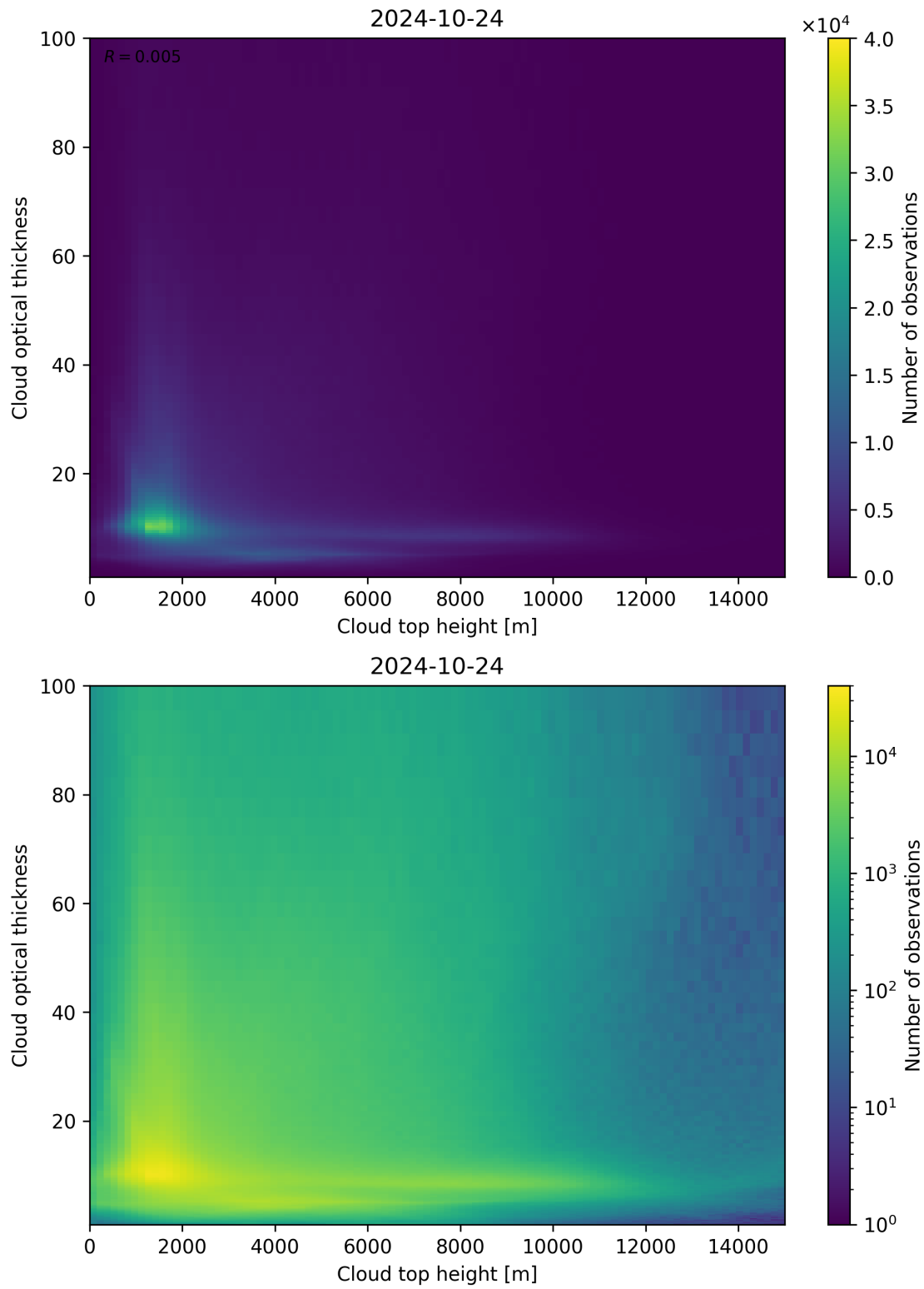
Figure 90: Scatter density plot of “Cloud top height” against “Cloud optical thickness” for 2024-10-24 to 2024-10-25.
