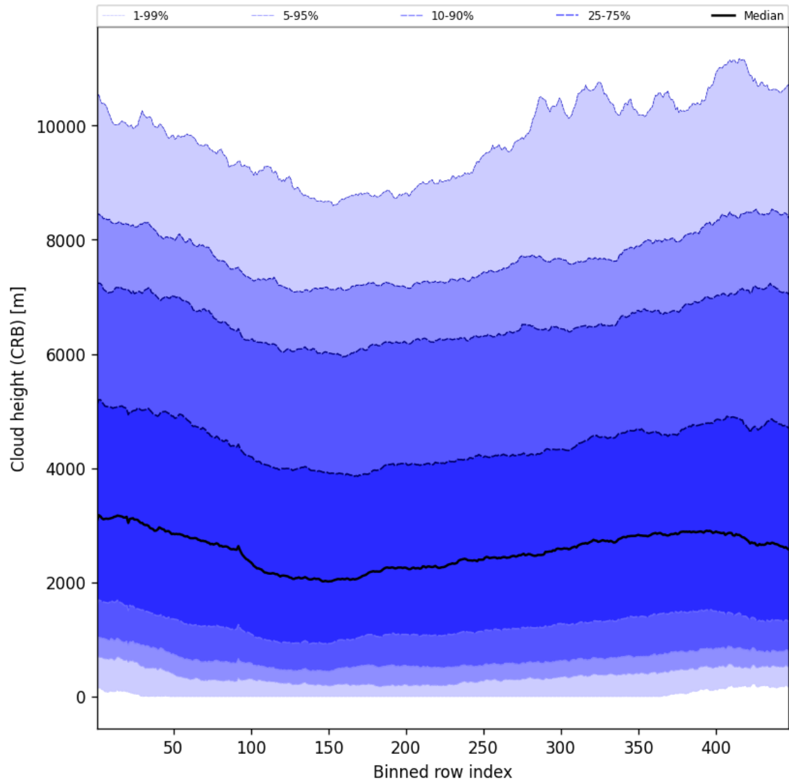
Figure 59: Along track statistics of “Cloud height (CRB)” for 2024-10-24 to 2024-10-25
