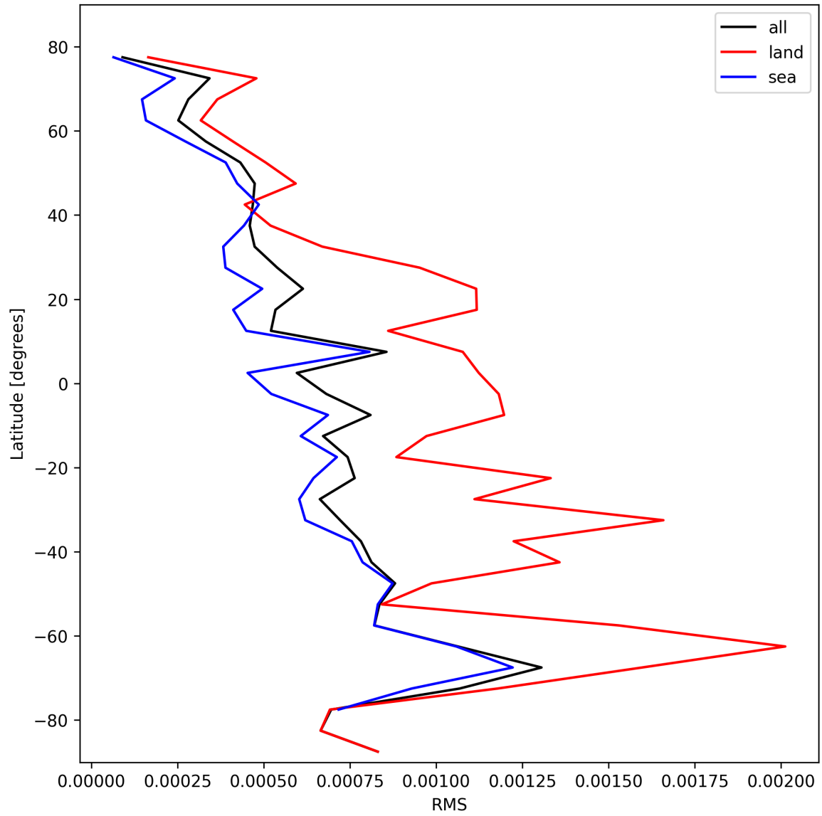
Figure 31: Zonal average of “RMS” for 2024-10-24 to 2024-10-25.
