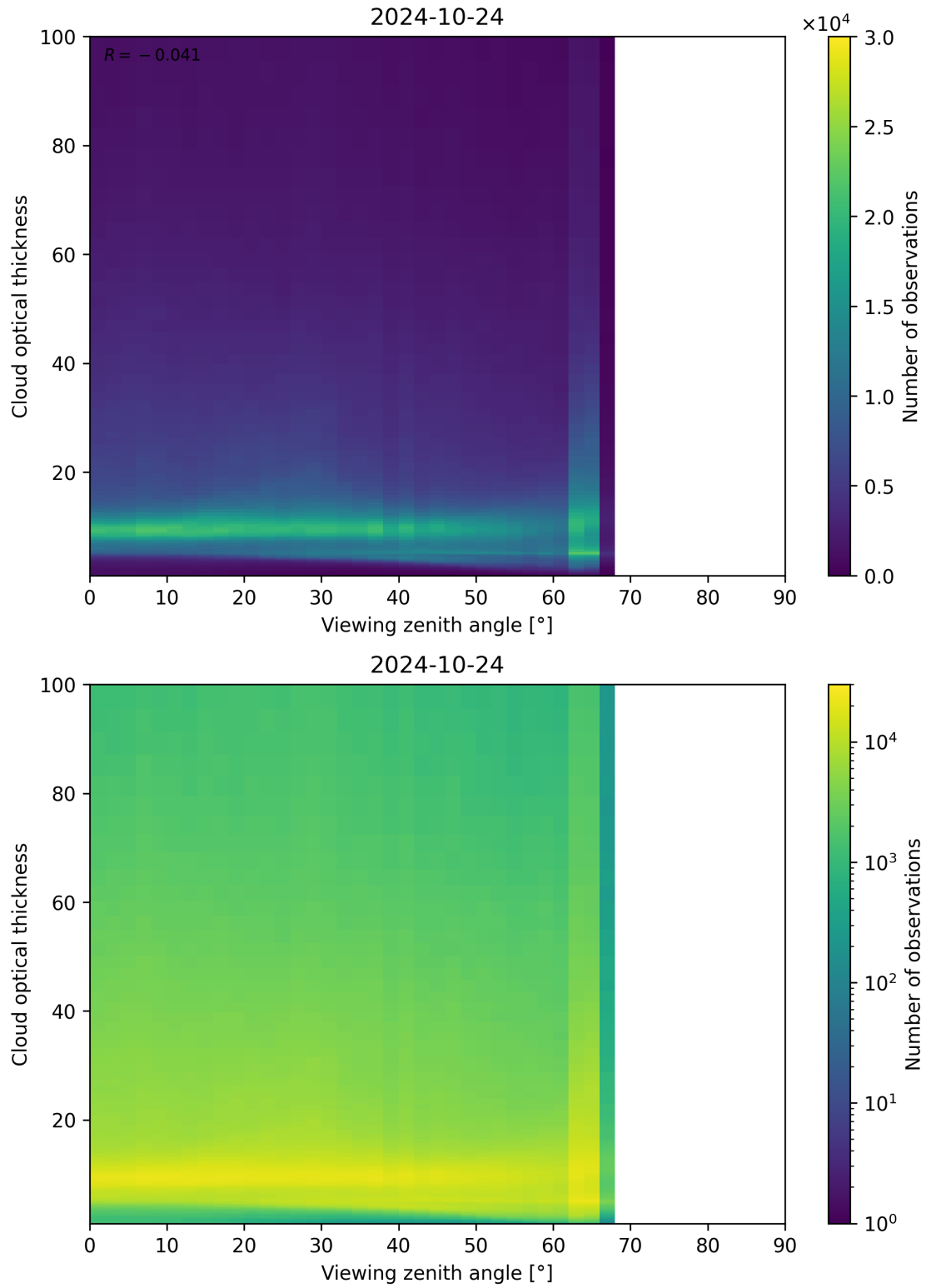
Figure 111: Scatter density plot of “Viewing zenith angle” against “Cloud optical thickness” for 2024-10-24 to 2024-10-25.
