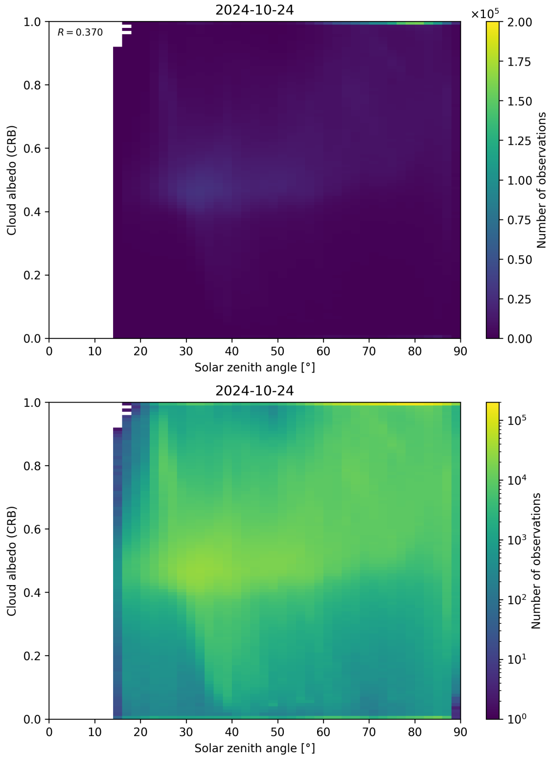
Figure 98: Scatter density plot of “Solar zenith angle” against “Cloud albedo (CRB)” for 2024-10-24 to 2024-10-25.
