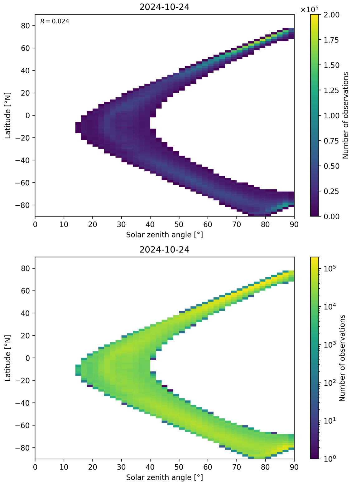
Figure 105: Scatter density plot of “Solar zenith angle” against “Latitude” for 2024-10-24 to 2024-10-25.
