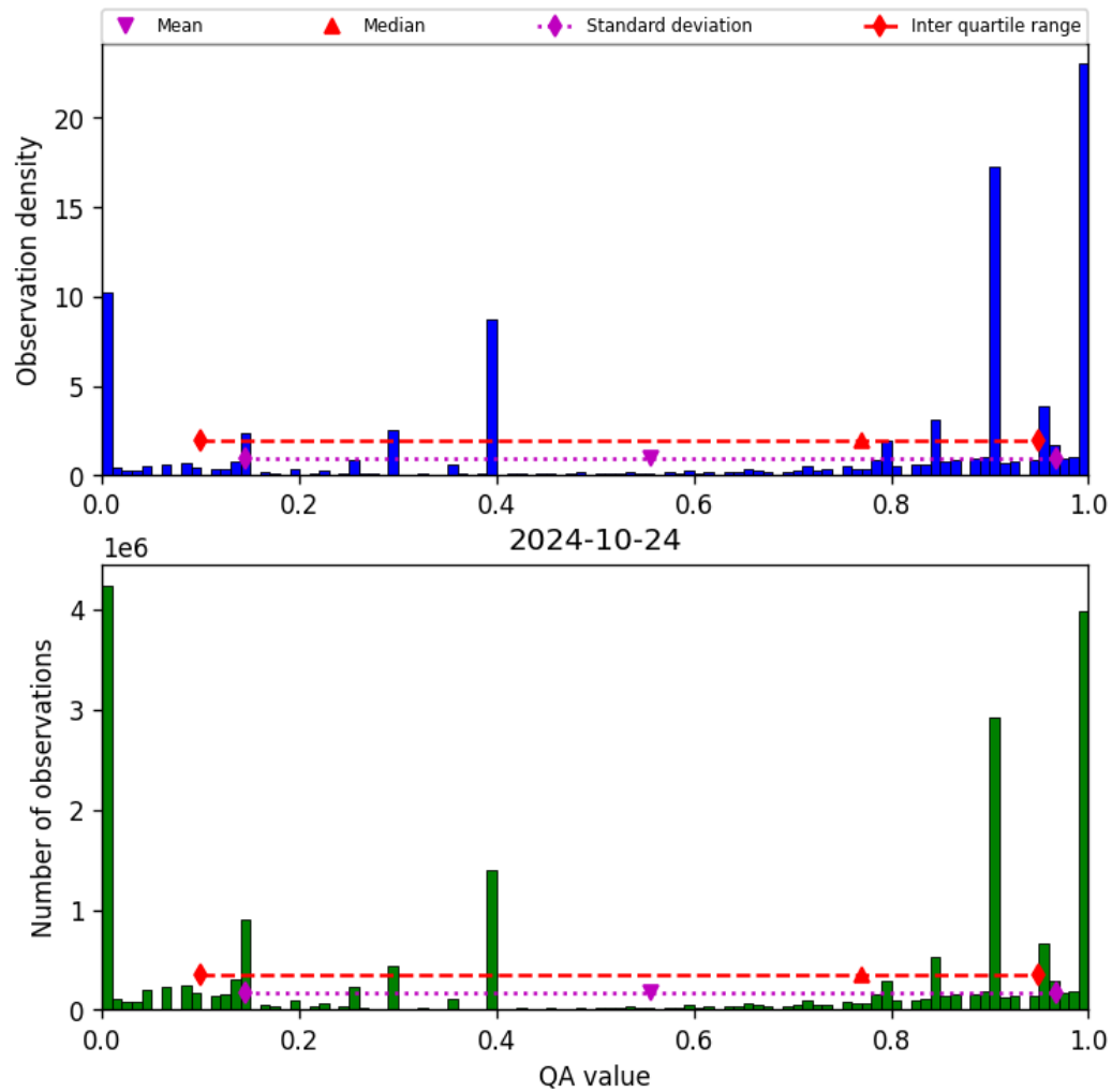
Figure 38: Histogram of “QA value” for 2024-10-24 to 2024-10-25
