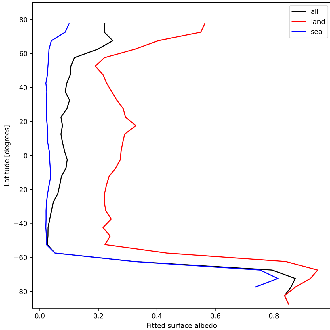
Figure 29: Zonal average of “Fitted surface albedo” for 2024-10-24 to 2024-10-25.
