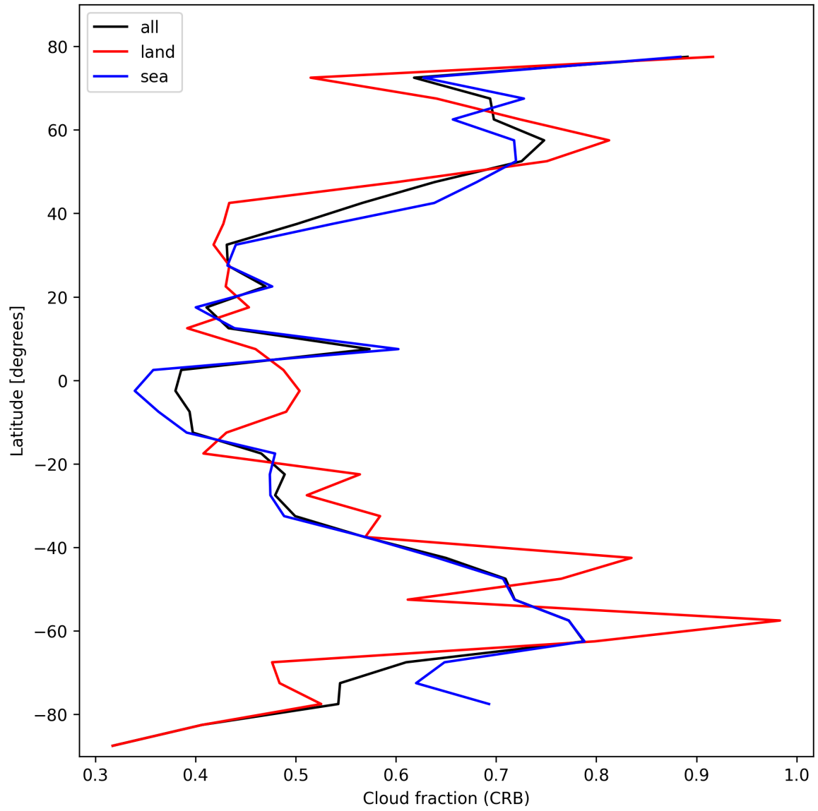
Figure 26: Zonal average of “Cloud fraction (CRB)” for 2024-10-24 to 2024-10-25.
