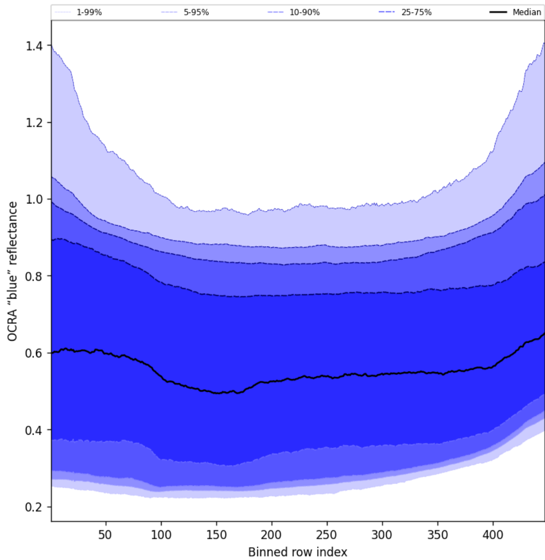
Figure 67: Along track statistics of “OCRA “blue” reflectance” for 2024-10-26 to 2024-10-28
