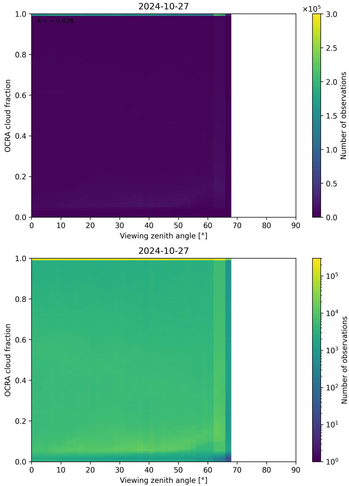
Figure 108: Scatter density plot of “Viewing zenith angle” against “OCRA cloud fraction” for 2024-10-26 to 2024-10-28.
