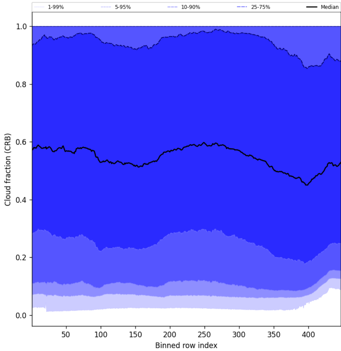
Figure 58: Along track statistics of “Cloud fraction (CRB)” for 2024-10-26 to 2024-10-28
