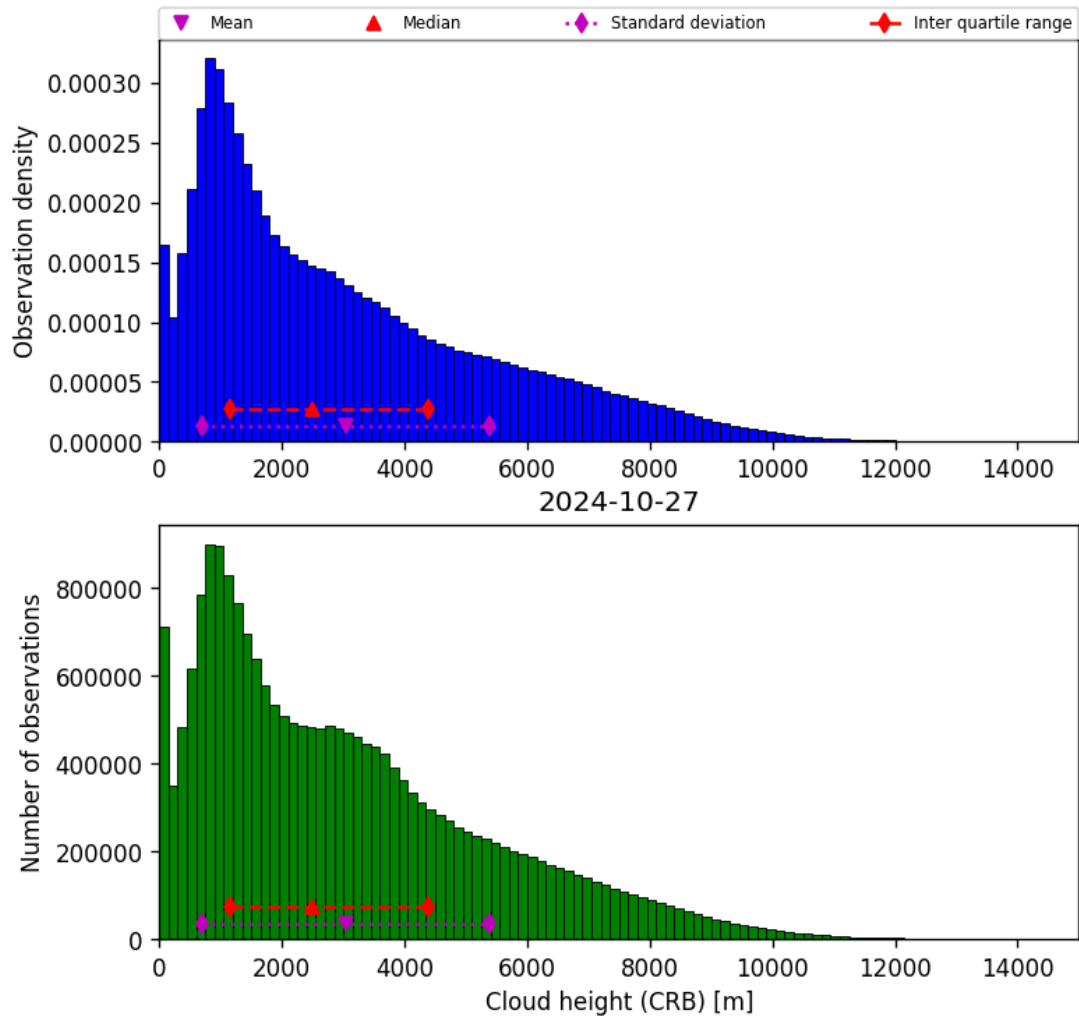
Figure 43: Histogram of “Cloud height (CRB)” for 2024-10-26 to 2024-10-28
