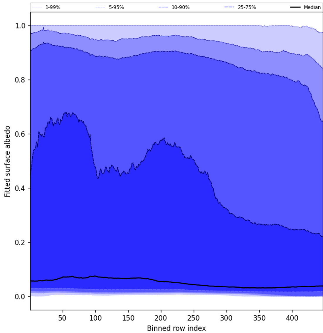
Figure 61: Along track statistics of “Fitted surface albedo” for 2024-10-26 to 2024-10-28
