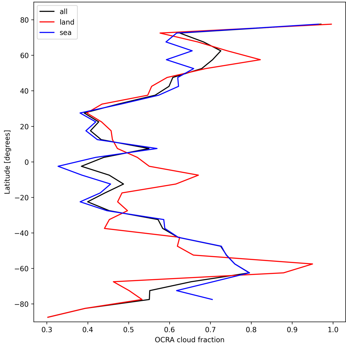
Figure 34: Zonal average of “OCRA cloud fraction” for 2024-10-26 to 2024-10-28.
