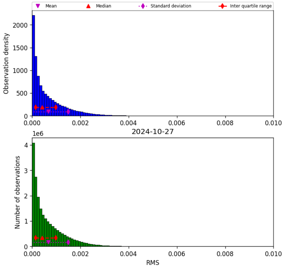
Figure 47: Histogram of “RMS” for 2024-10-26 to 2024-10-28
