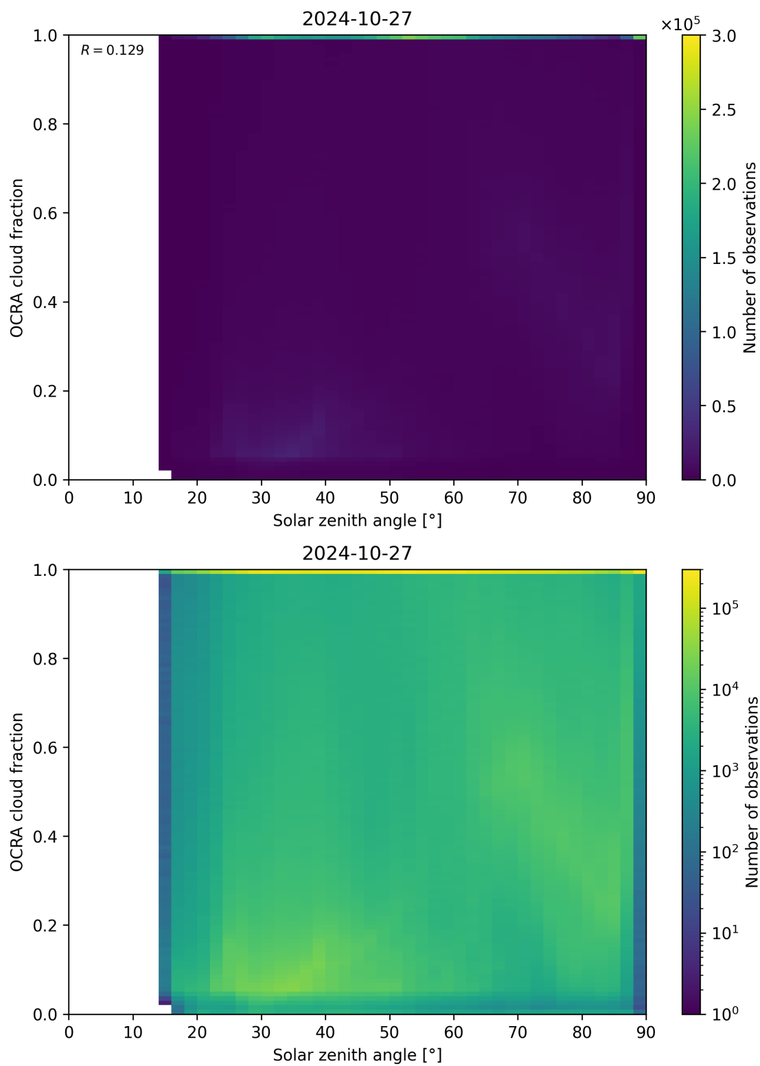
Figure 100: Scatter density plot of “Solar zenith angle” against “OCRA cloud fraction” for 2024-10-26 to 2024-10-28.
