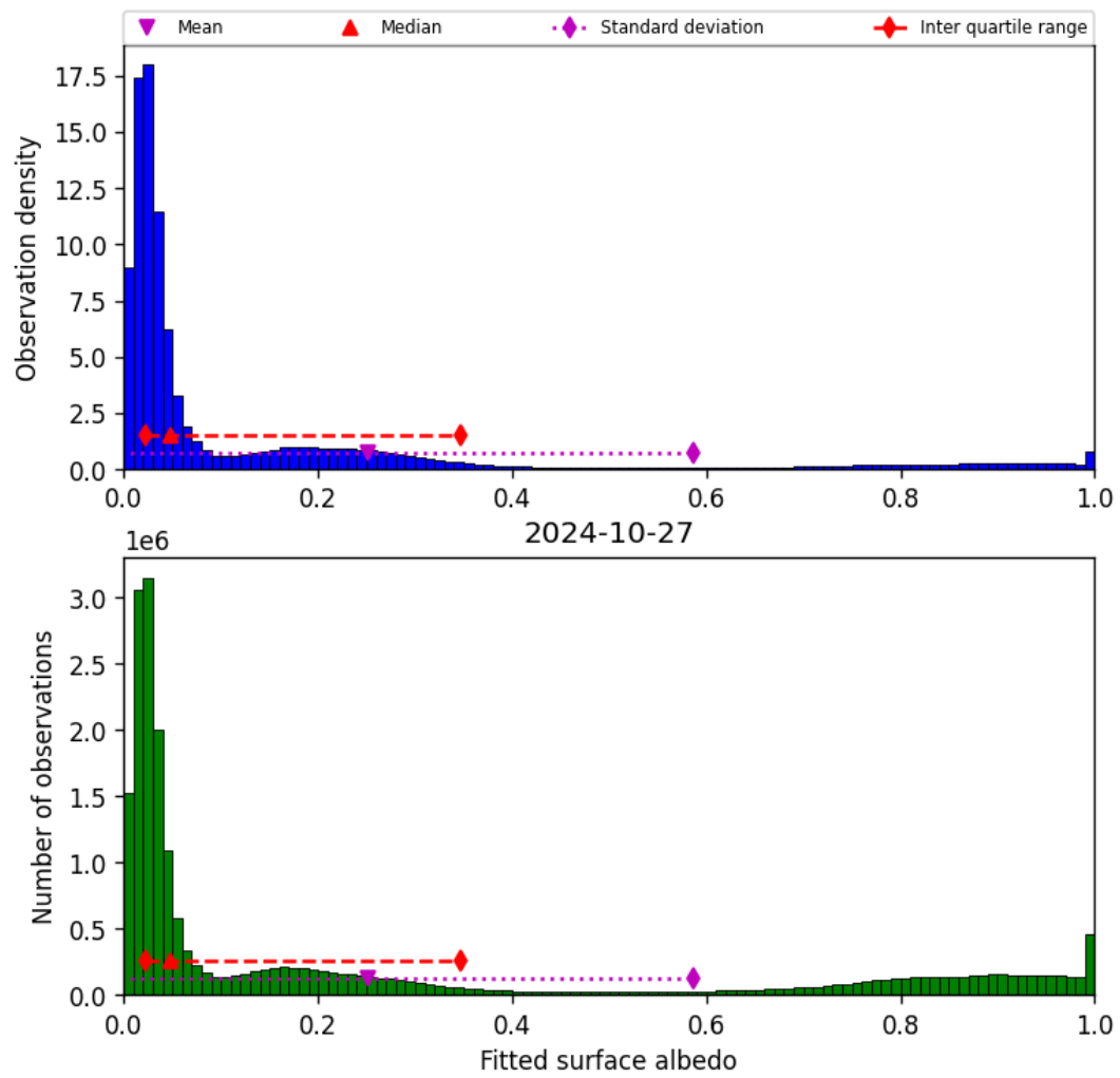
Figure 45: Histogram of “Fitted surface albedo” for 2024-10-26 to 2024-10-28
