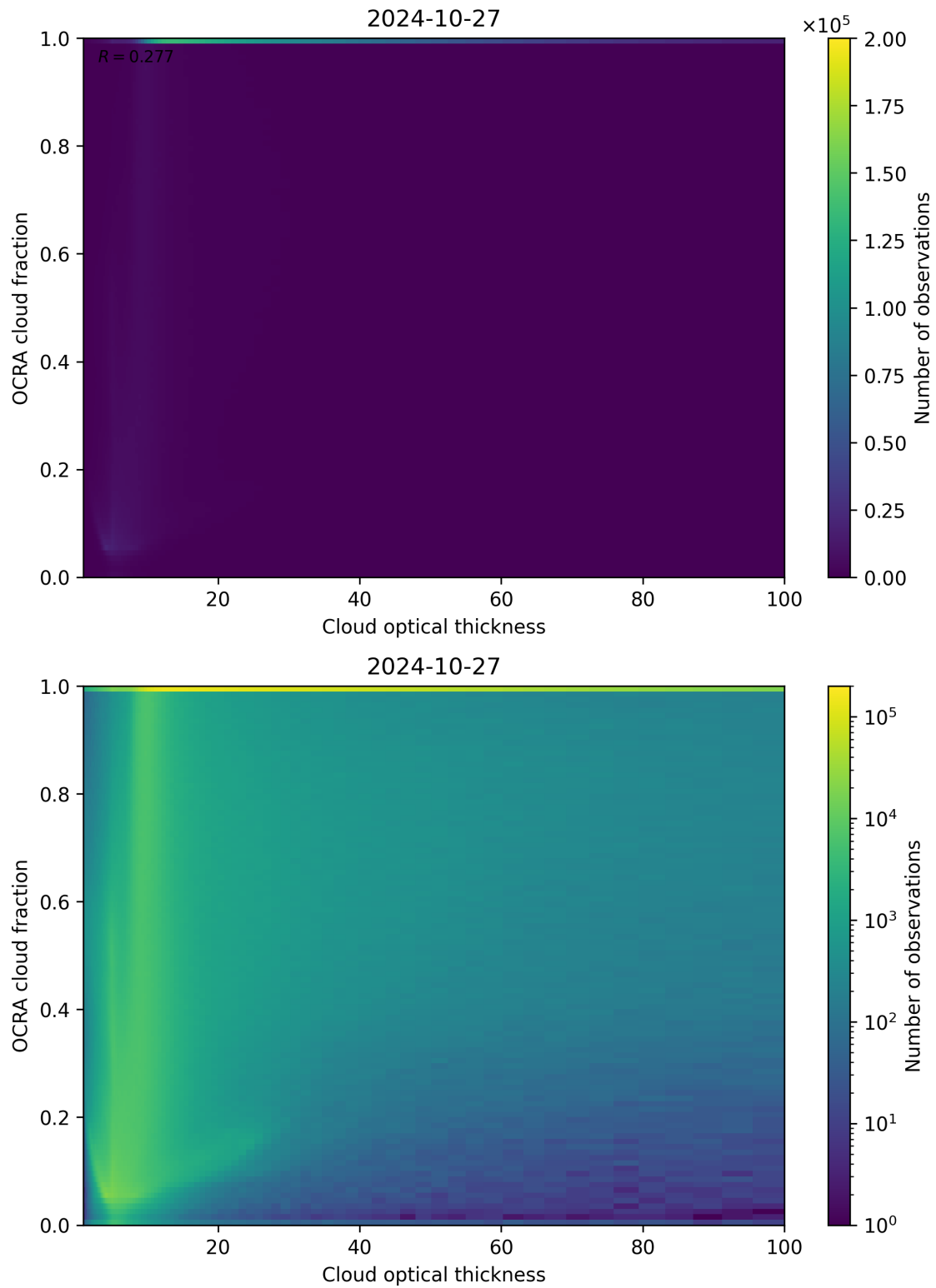
Figure 83: Scatter density plot of “Cloud optical thickness” against “OCRA cloud fraction” for 2024-10-26 to 2024-10-28.
