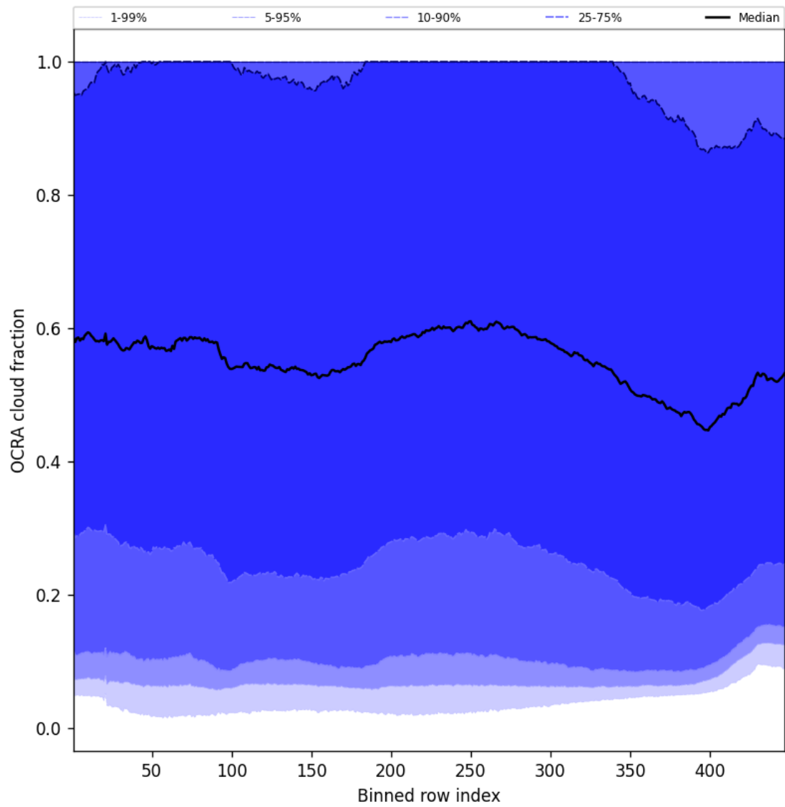
Figure 66: Along track statistics of “OCRA cloud fraction” for 2024-10-26 to 2024-10-28
