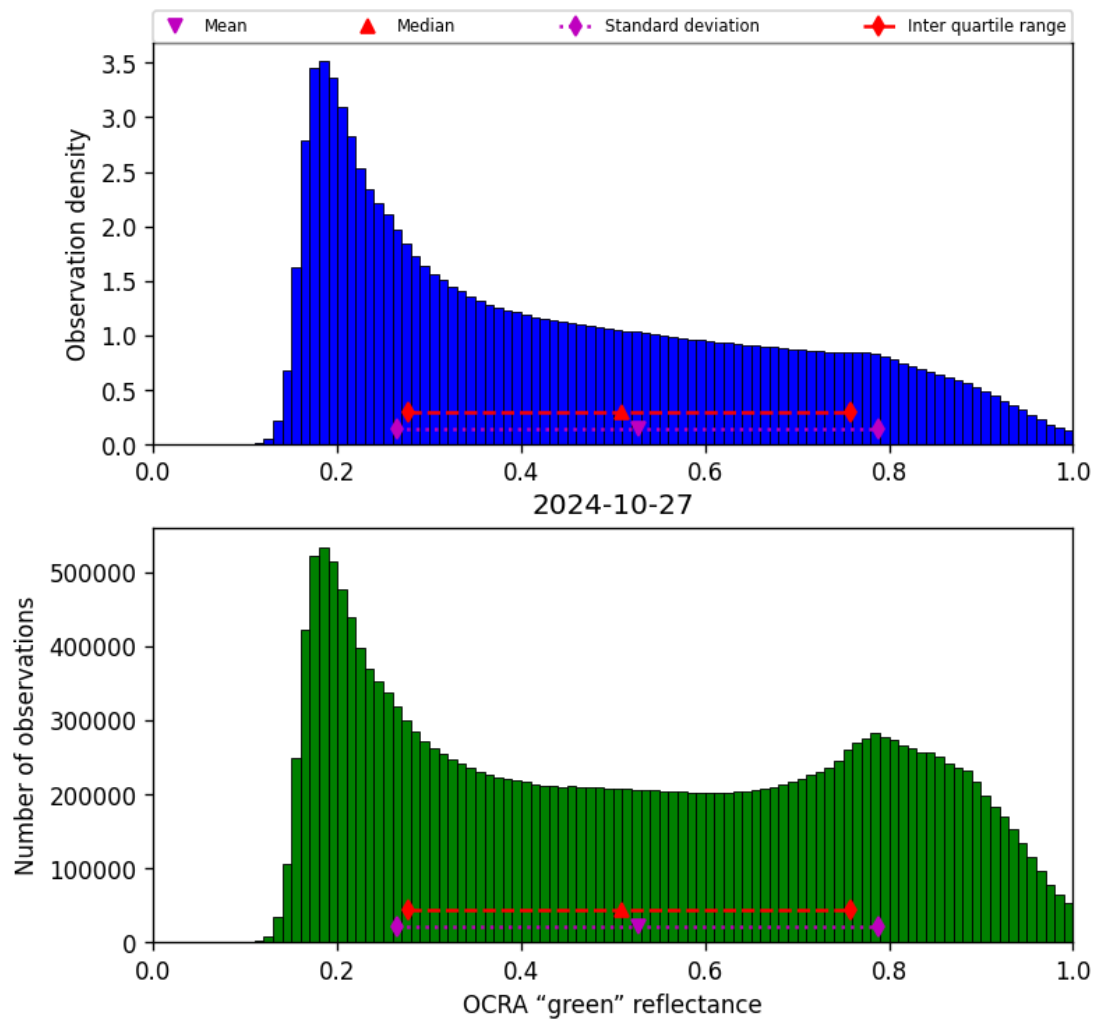
Figure 52: Histogram of “OCRA “green” reflectance” for 2024-10-26 to 2024-10-28
