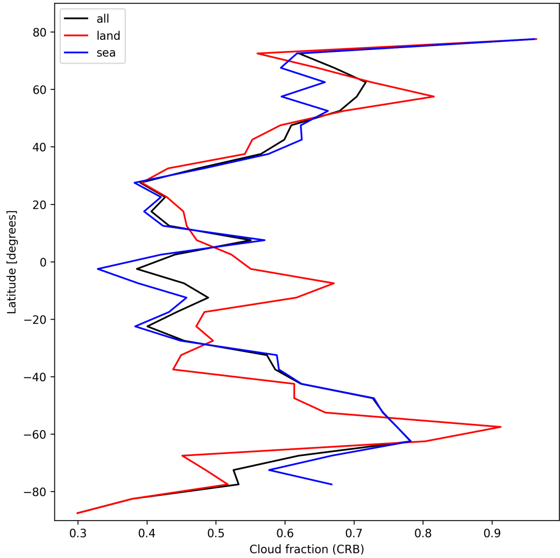
Figure 26: Zonal average of “Cloud fraction (CRB)” for 2024-10-26 to 2024-10-28.
