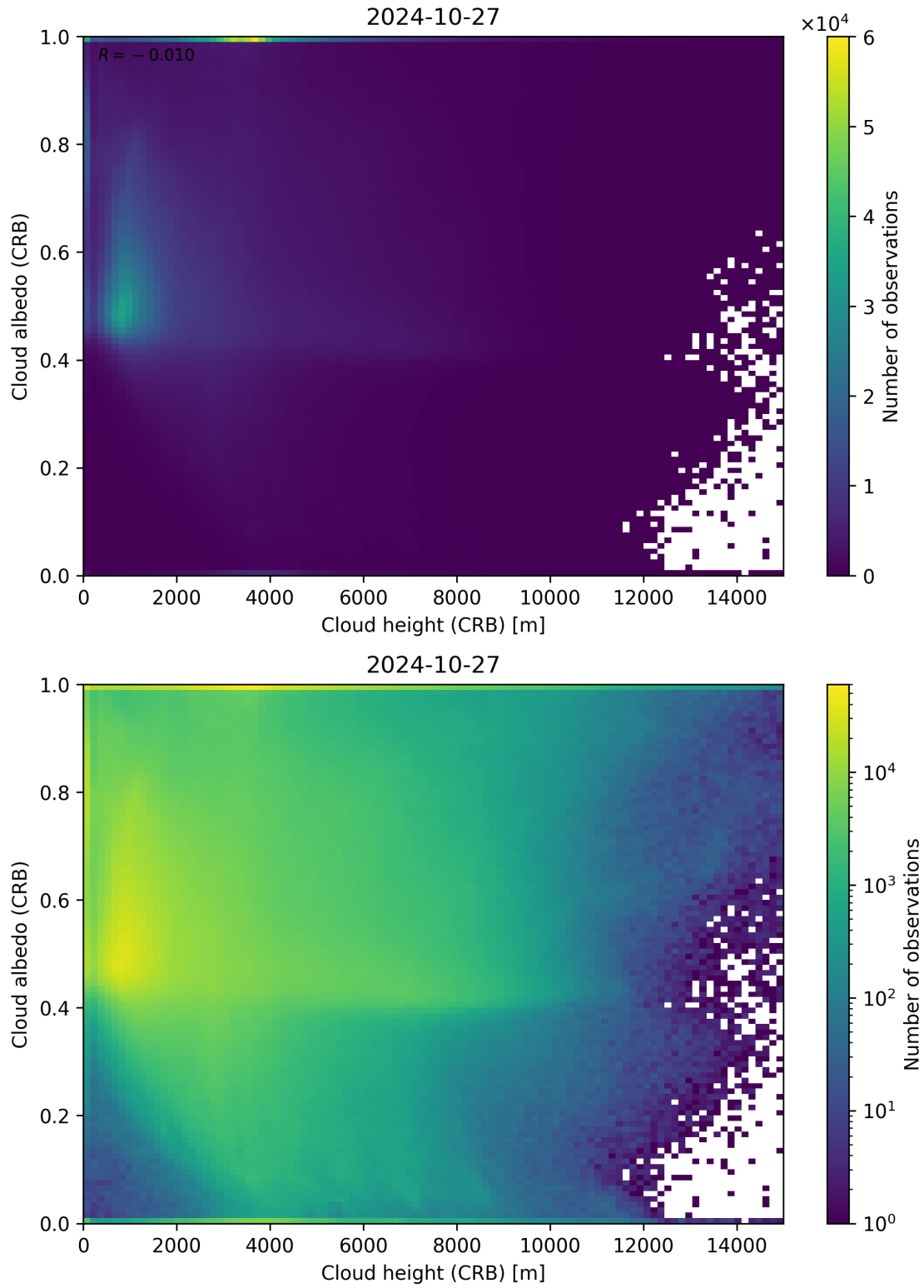
Figure 80: Scatter density plot of “Cloud height (CRB)” against “Cloud albedo (CRB)” for 2024-10-26 to 2024-10-28.
