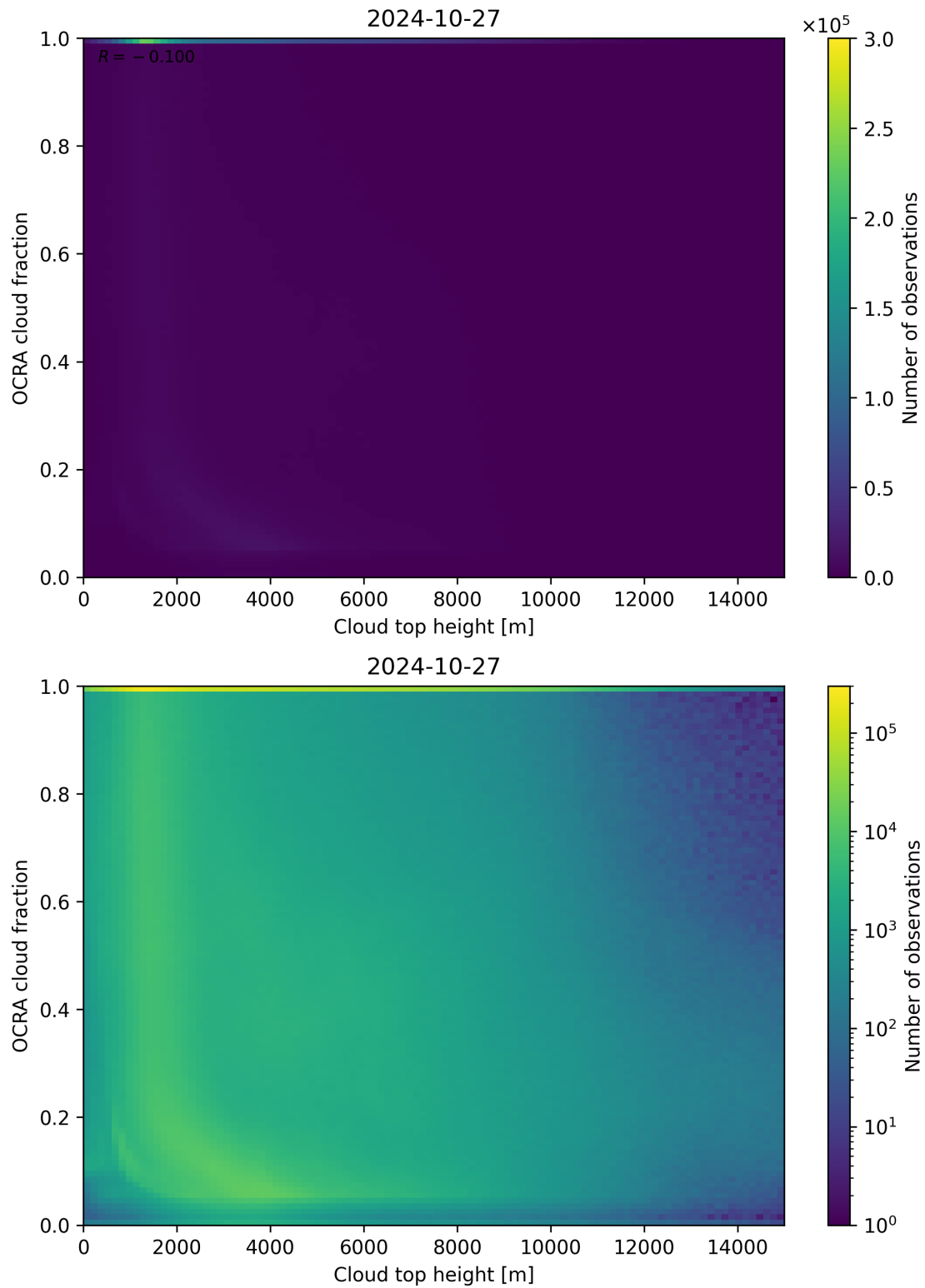
Figure 87: Scatter density plot of “Cloud top height” against “OCRA cloud fraction” for 2024-10-26 to 2024-10-28.
