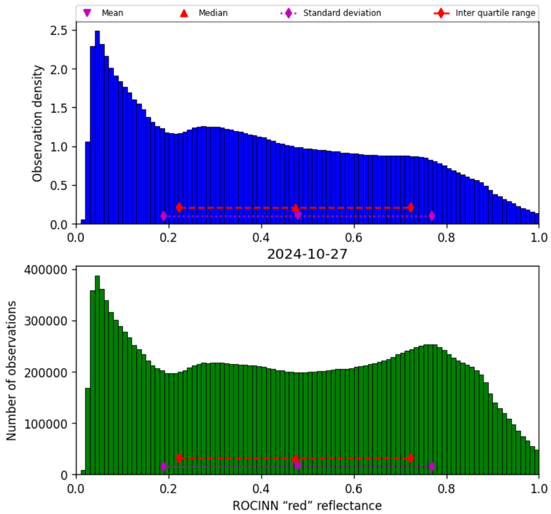
Figure 53: Histogram of “ROCINN “red” reflectance” for 2024-10-26 to 2024-10-28
