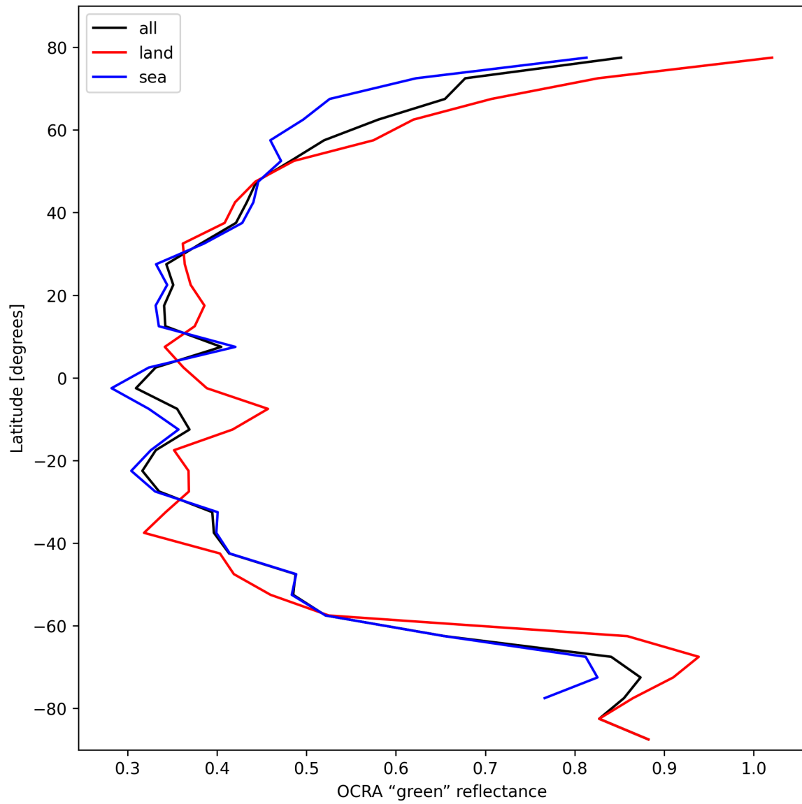
Figure 36: Zonal average of “OCRA “green” reflectance” for 2024-10-26 to 2024-10-28.
