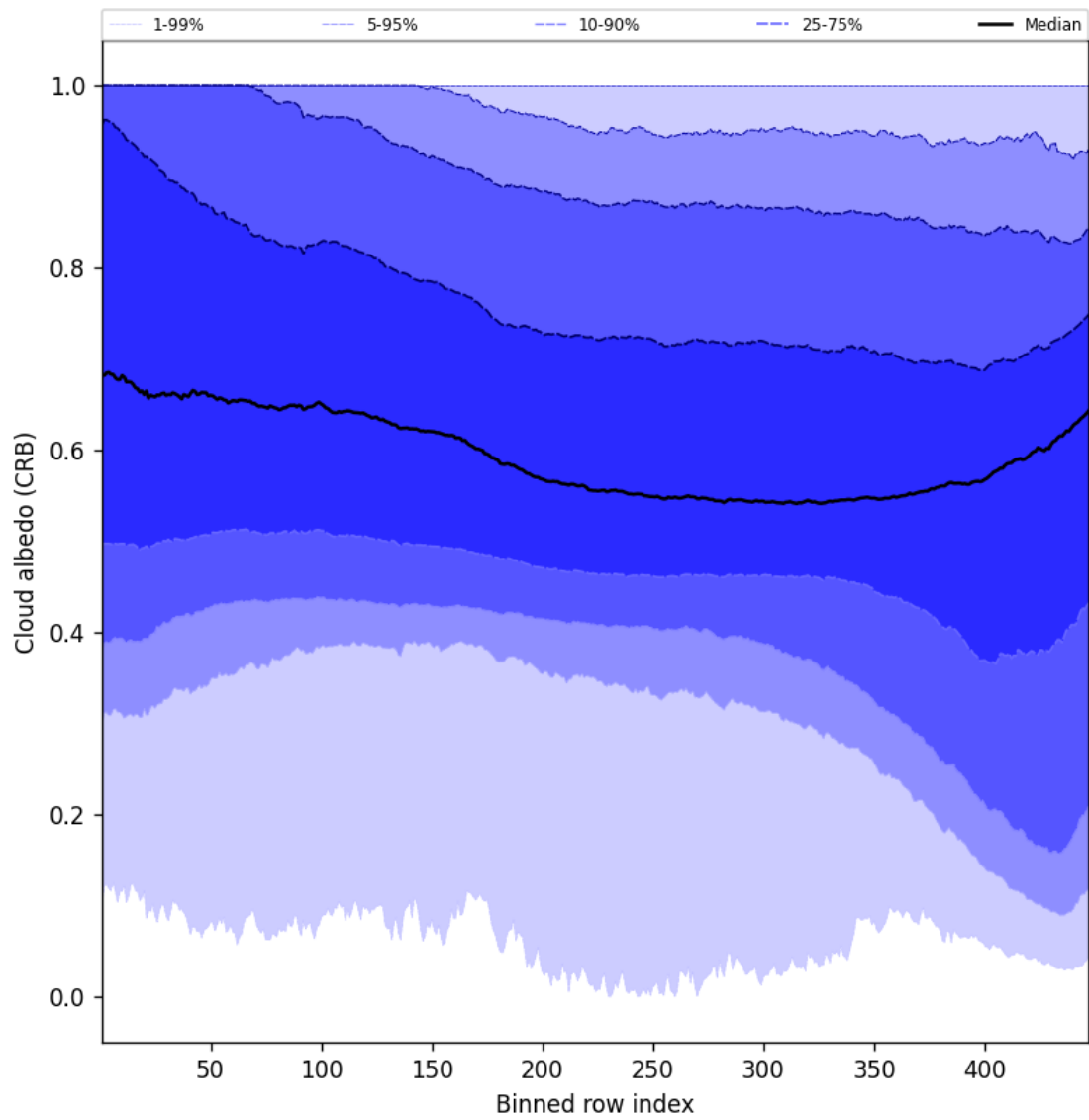
Figure 60: Along track statistics of “Cloud albedo (CRB)” for 2024-10-26 to 2024-10-28
