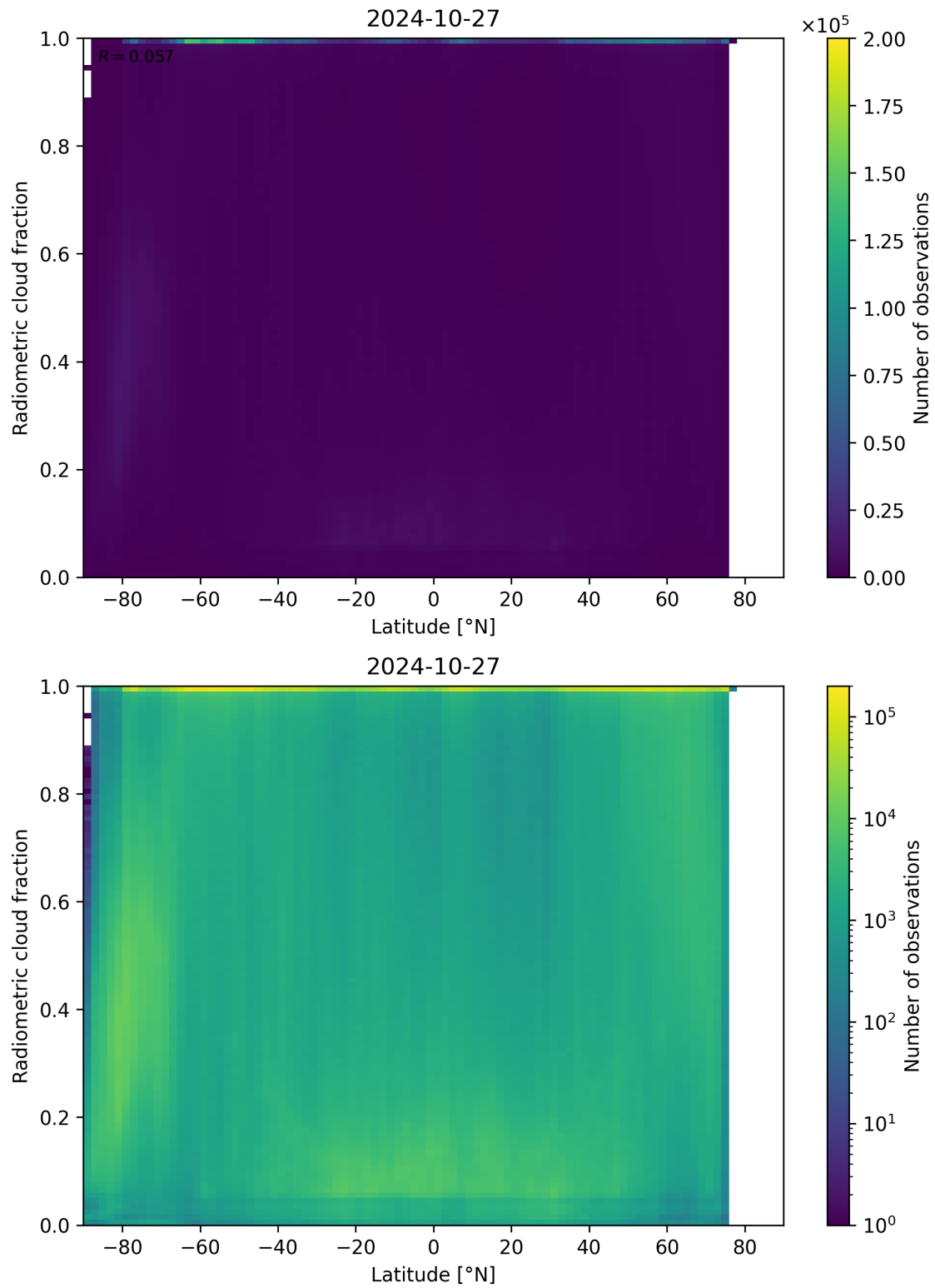
Figure 92: Scatter density plot of “Latitude” against “Radiometric cloud fraction” for 2024-10-26 to 2024-10-28.
