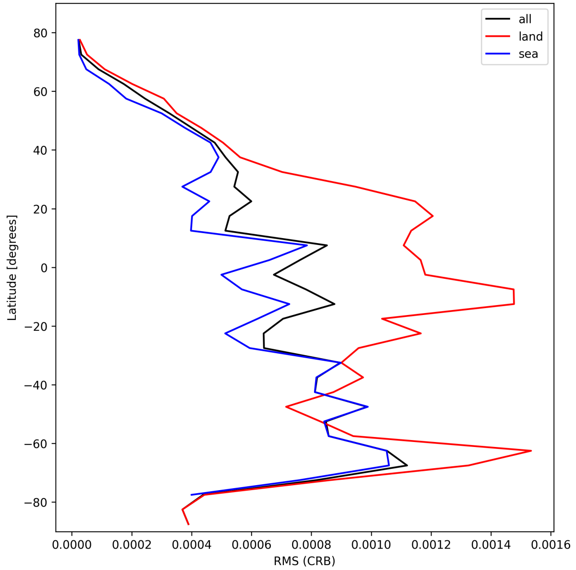
Figure 32: Zonal average of “RMS (CRB)” for 2024-10-26 to 2024-10-28.
