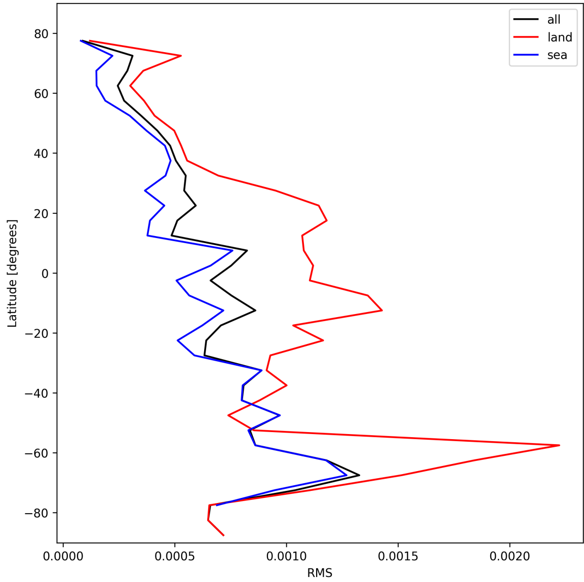
Figure 31: Zonal average of “RMS” for 2024-10-26 to 2024-10-28.
