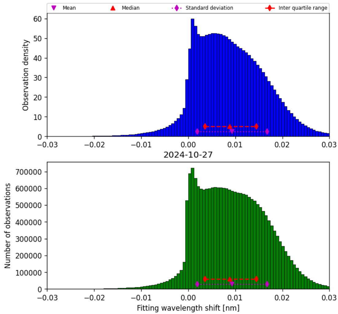
Figure 49: Histogram of “Fitting wavelength shift” for 2024-10-26 to 2024-10-28
