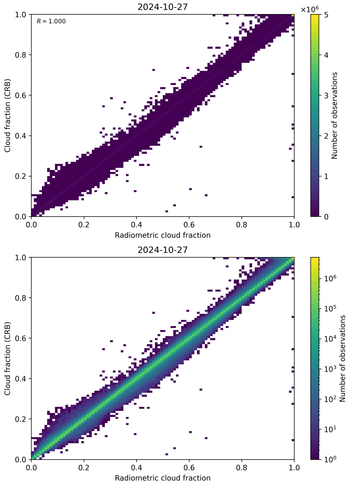
Figure 73: Scatter density plot of “Radiometric cloud fraction” against “Cloud fraction (CRB)” for 2024-10-26 to 2024-10-28.
