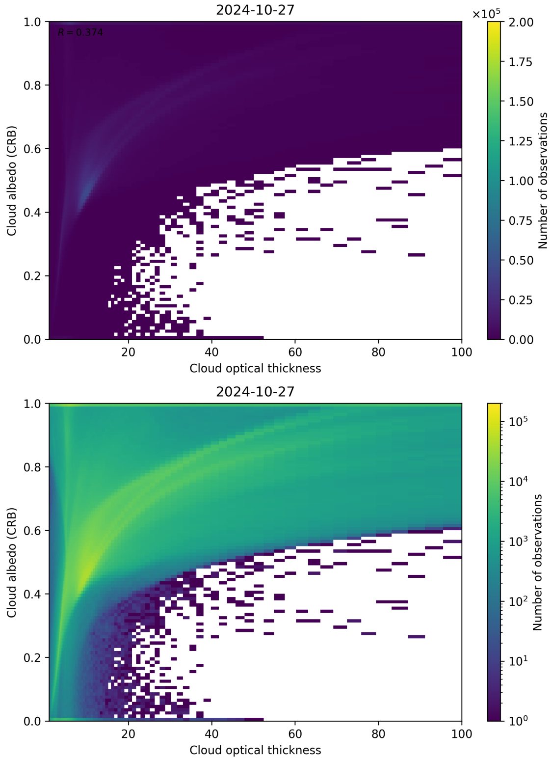
Figure 82: Scatter density plot of “Cloud optical thickness” against “Cloud albedo (CRB)” for 2024-10-26 to 2024-10-28.
