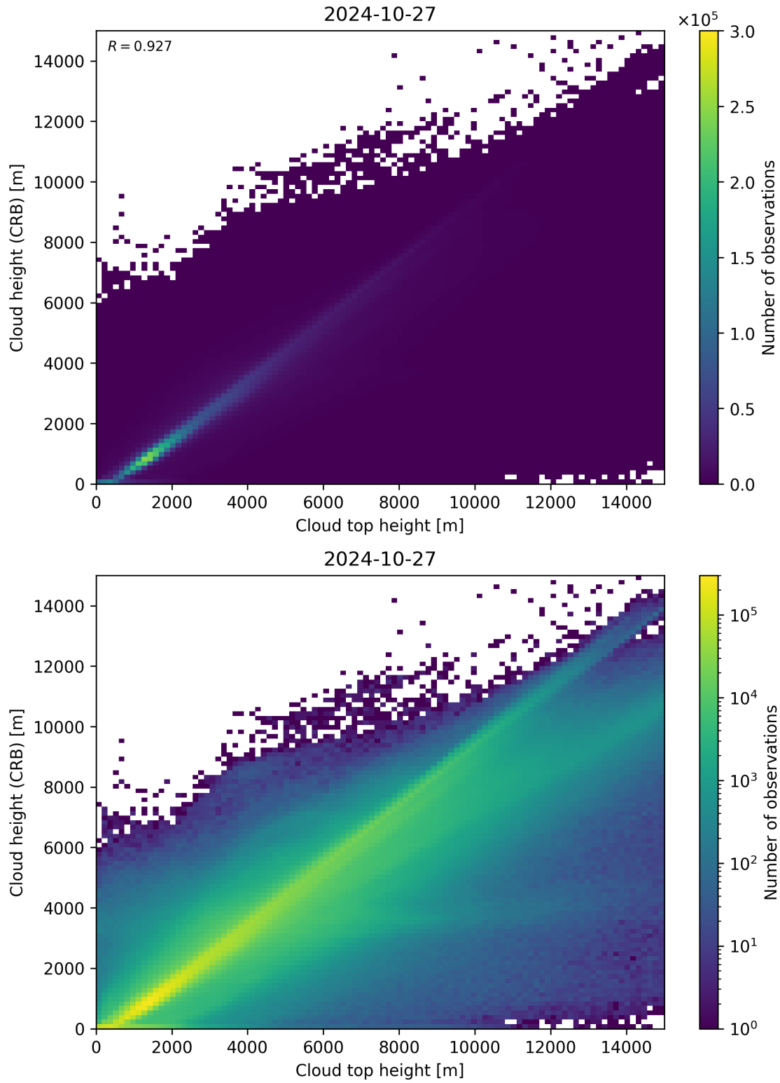
Figure 89: Scatter density plot of “Cloud top height” against “Cloud height (CRB)” for 2024-10-26 to 2024-10-28.
