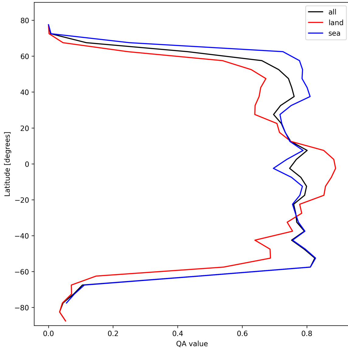
Figure 22: Zonal average of “QA value” for 2024-10-26 to 2024-10-28.
