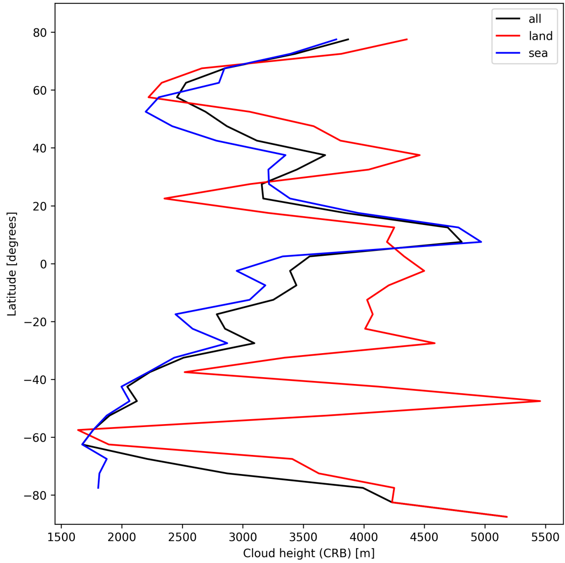
Figure 27: Zonal average of “Cloud height (CRB)” for 2024-10-26 to 2024-10-28.
