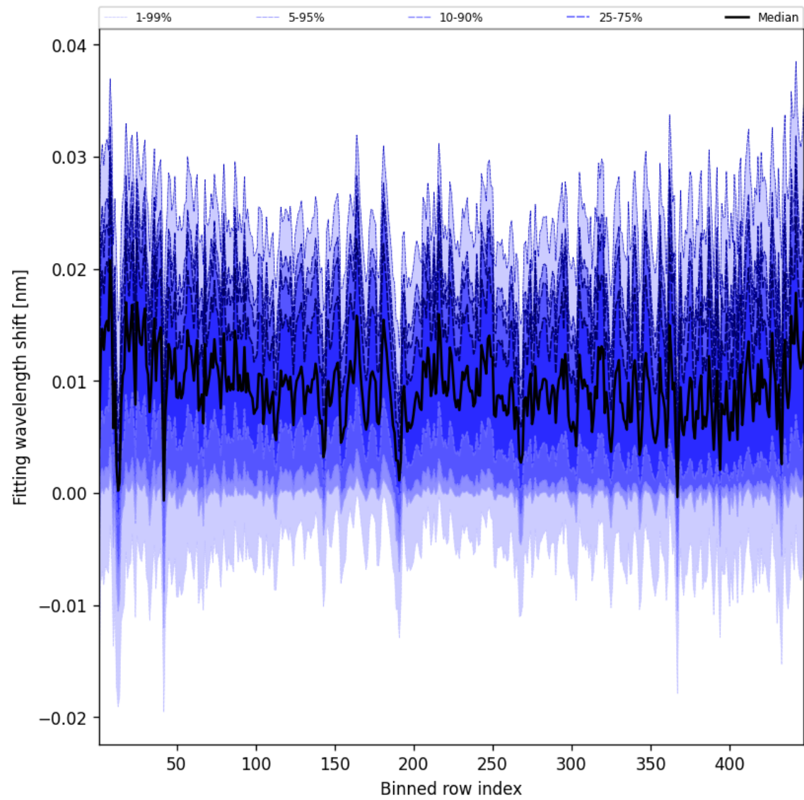
Figure 65: Along track statistics of “Fitting wavelength shift” for 2024-10-26 to 2024-10-28
