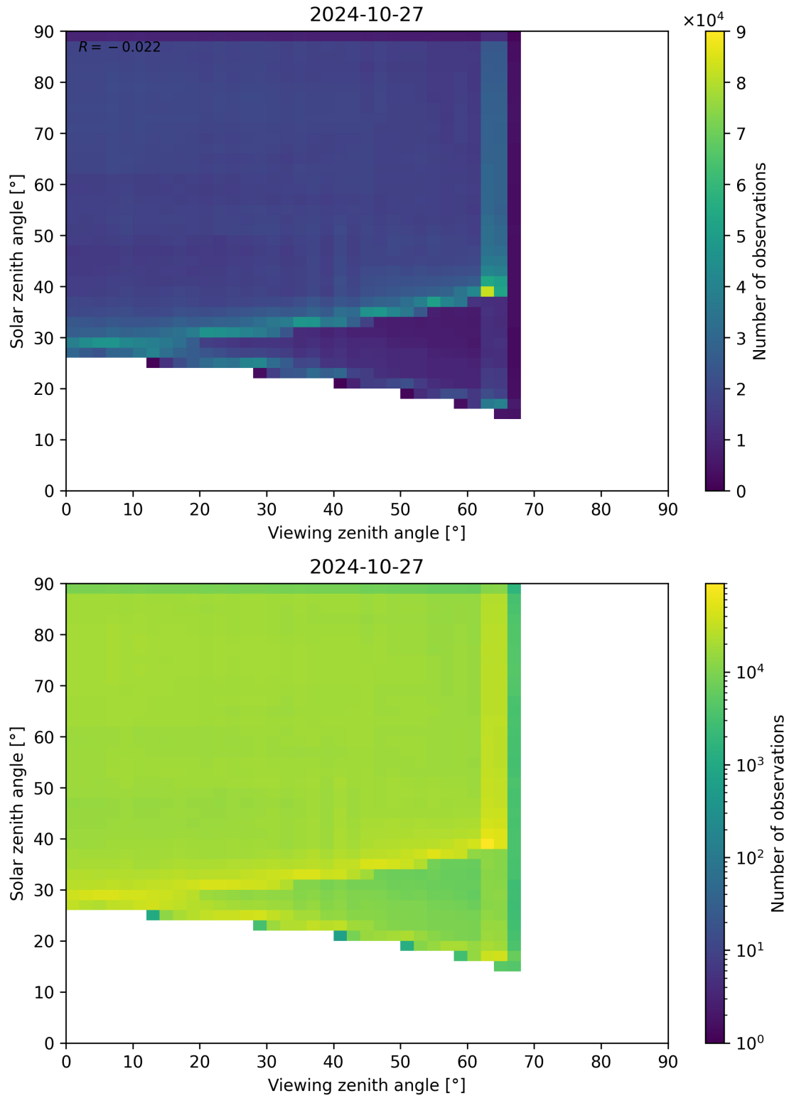
Figure 114: Scatter density plot of “Viewing zenith angle” against “Solar zenith angle” for 2024-10-26 to 2024-10-28.
