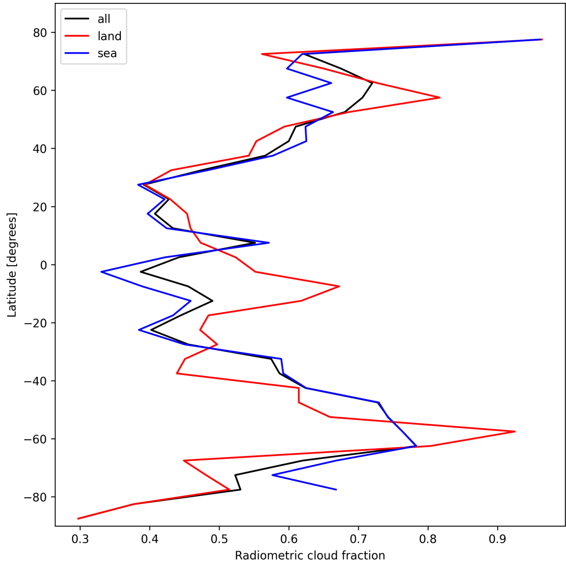
Figure 23: Zonal average of “Radiometric cloud fraction” for 2024-10-26 to 2024-10-28.
