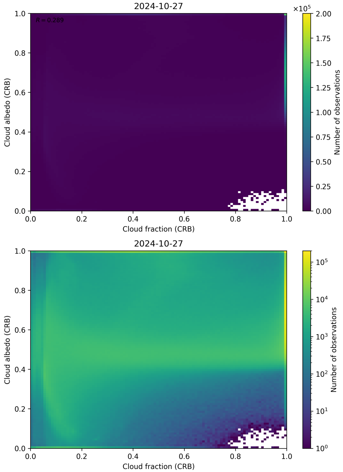
Figure 77: Scatter density plot of “Cloud fraction (CRB)” against “Cloud albedo (CRB)” for 2024-10-26 to 2024-10-28.
