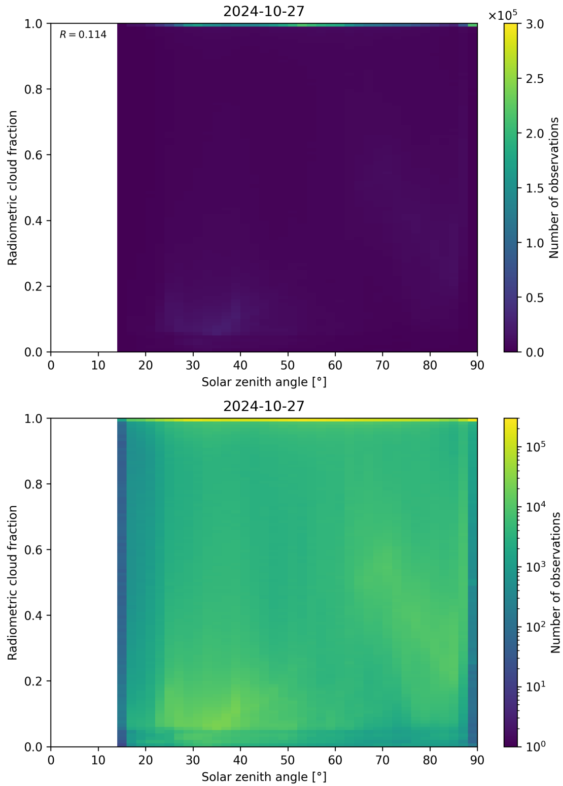
Figure 99: Scatter density plot of “Solar zenith angle” against “Radiometric cloud fraction” for 2024-10-26 to 2024-10-28.
