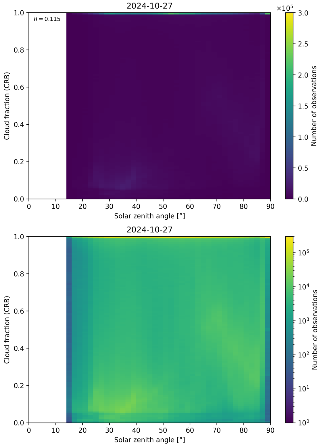
Figure 101: Scatter density plot of “Solar zenith angle” against “Cloud fraction (CRB)” for 2024-10-26 to 2024-10-28.
