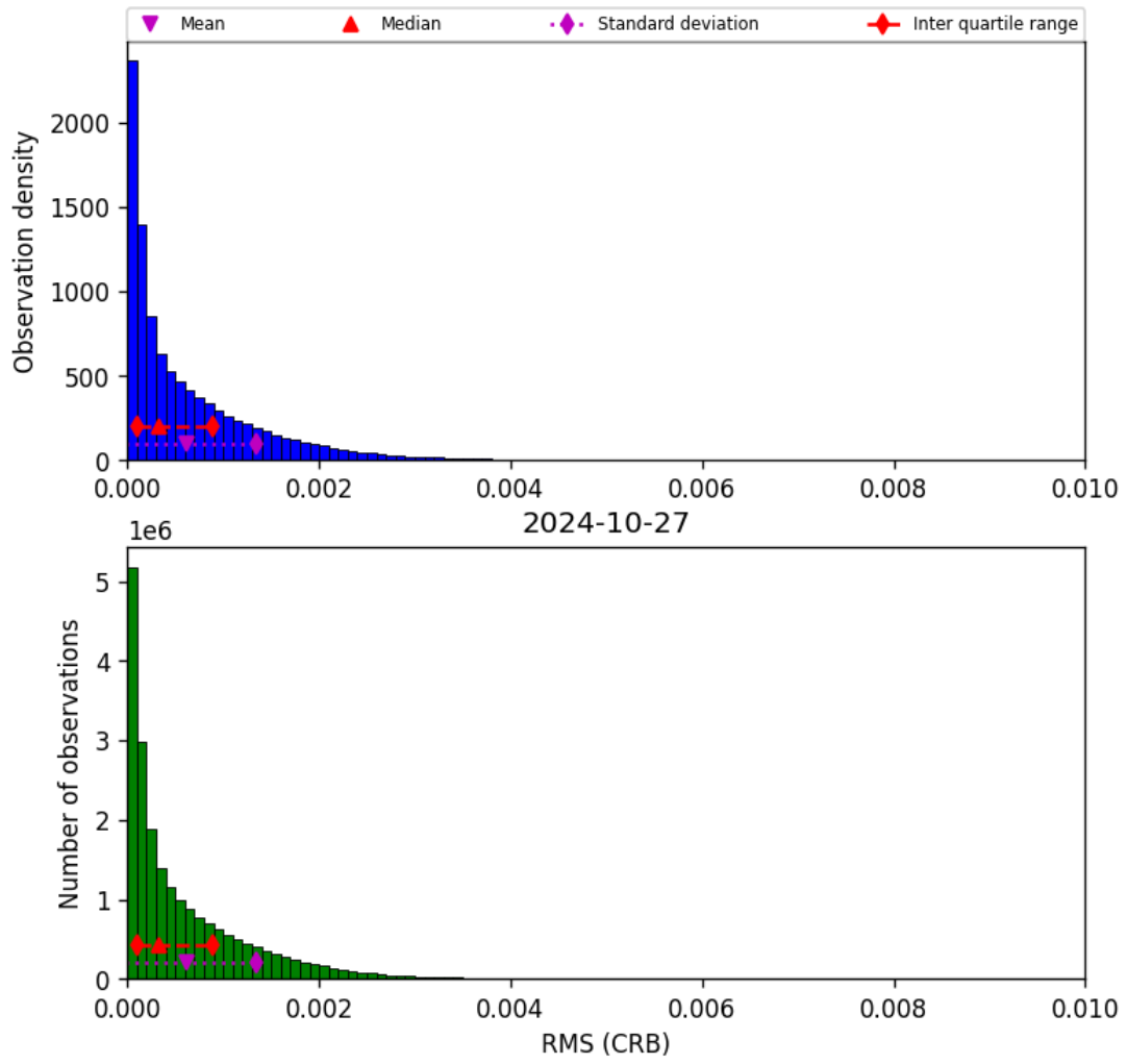
Figure 48: Histogram of “RMS (CRB)” for 2024-10-26 to 2024-10-28
