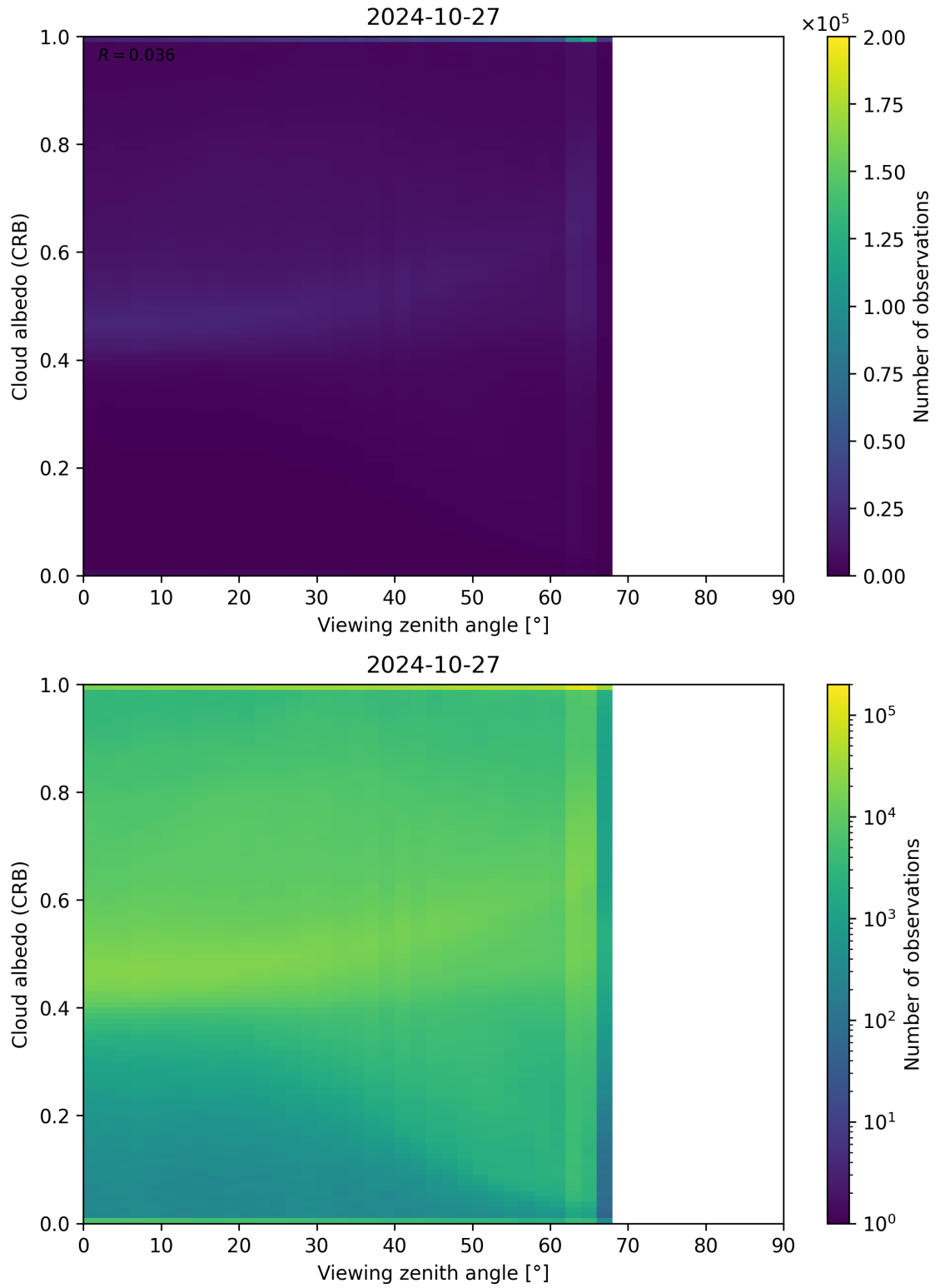
Figure 106: Scatter density plot of “Viewing zenith angle” against “Cloud albedo (CRB)” for 2024-10-26 to 2024-10-28.
