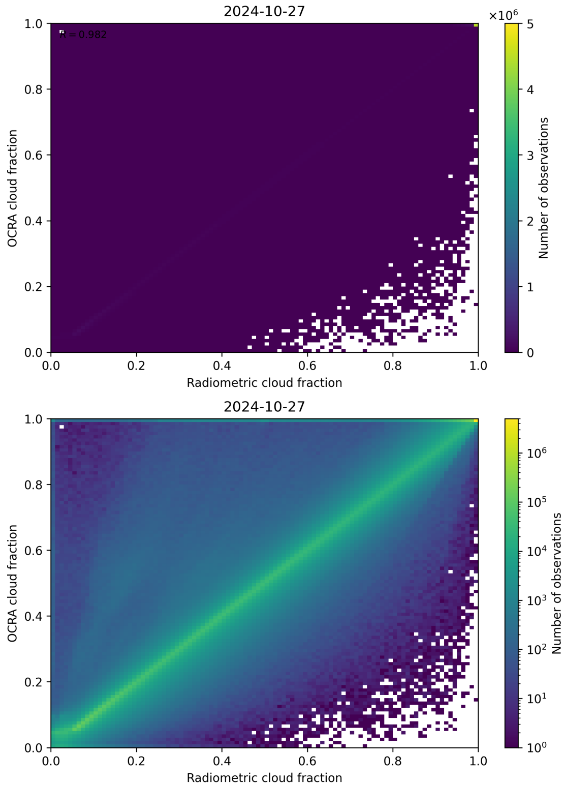
Figure 72: Scatter density plot of “Radiometric cloud fraction” against “OCRA cloud fraction” for 2024-10-26 to 2024-10-28.
