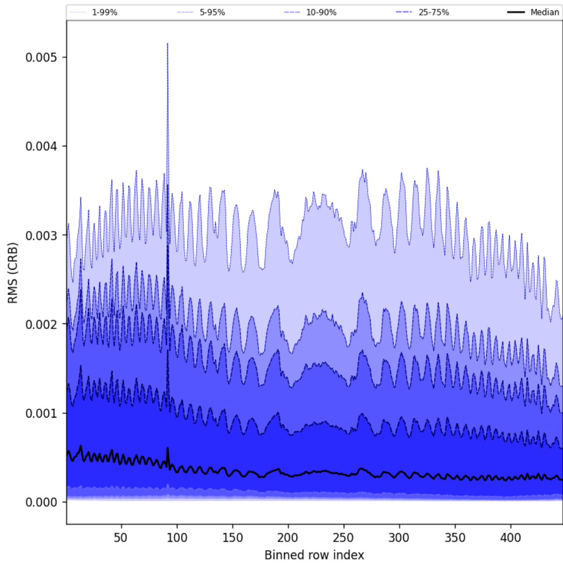
Figure 64: Along track statistics of “RMS (CRB)” for 2024-10-26 to 2024-10-28
