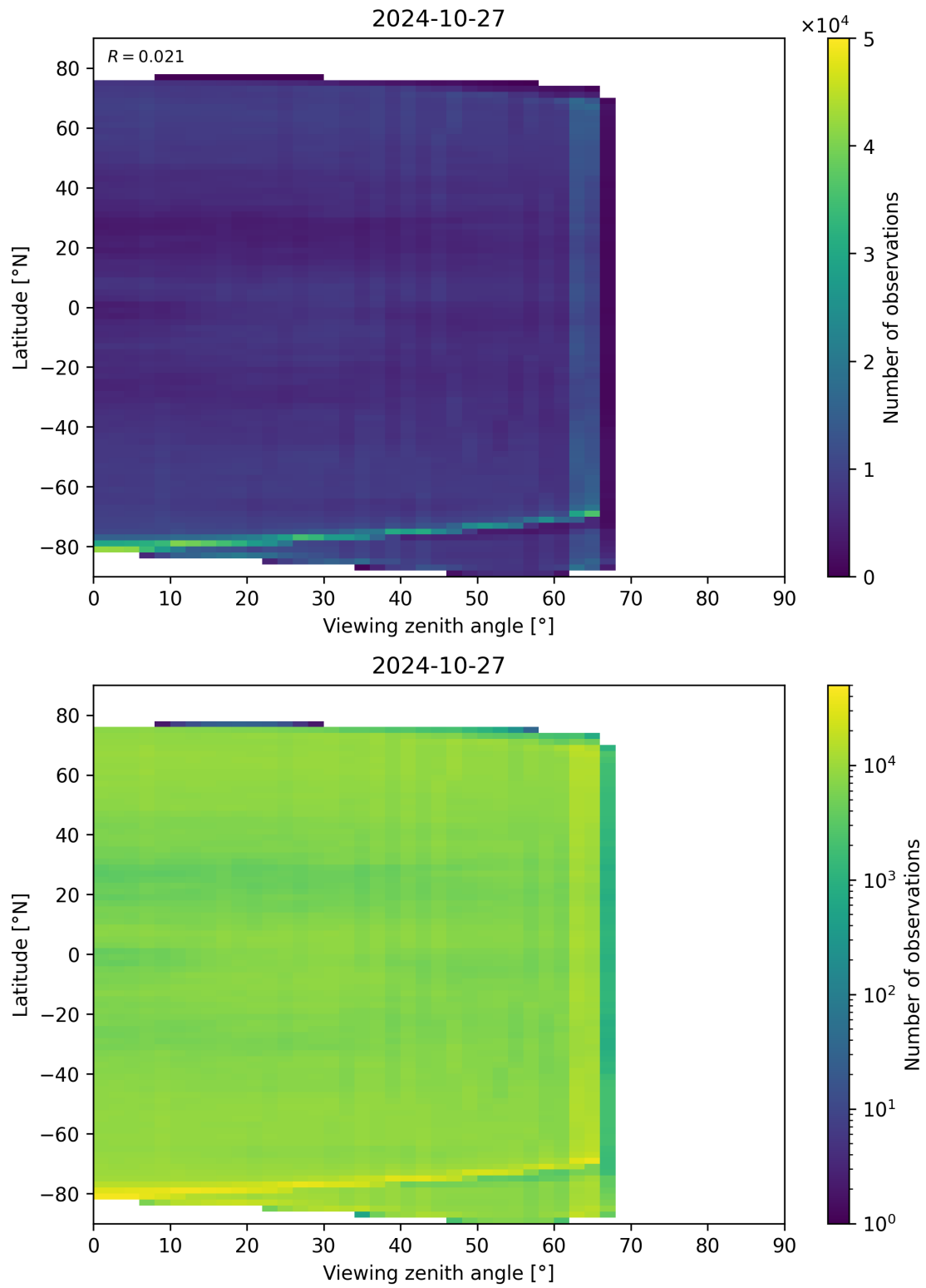
Figure 113: Scatter density plot of “Viewing zenith angle” against “Latitude” for 2024-10-26 to 2024-10-28.
