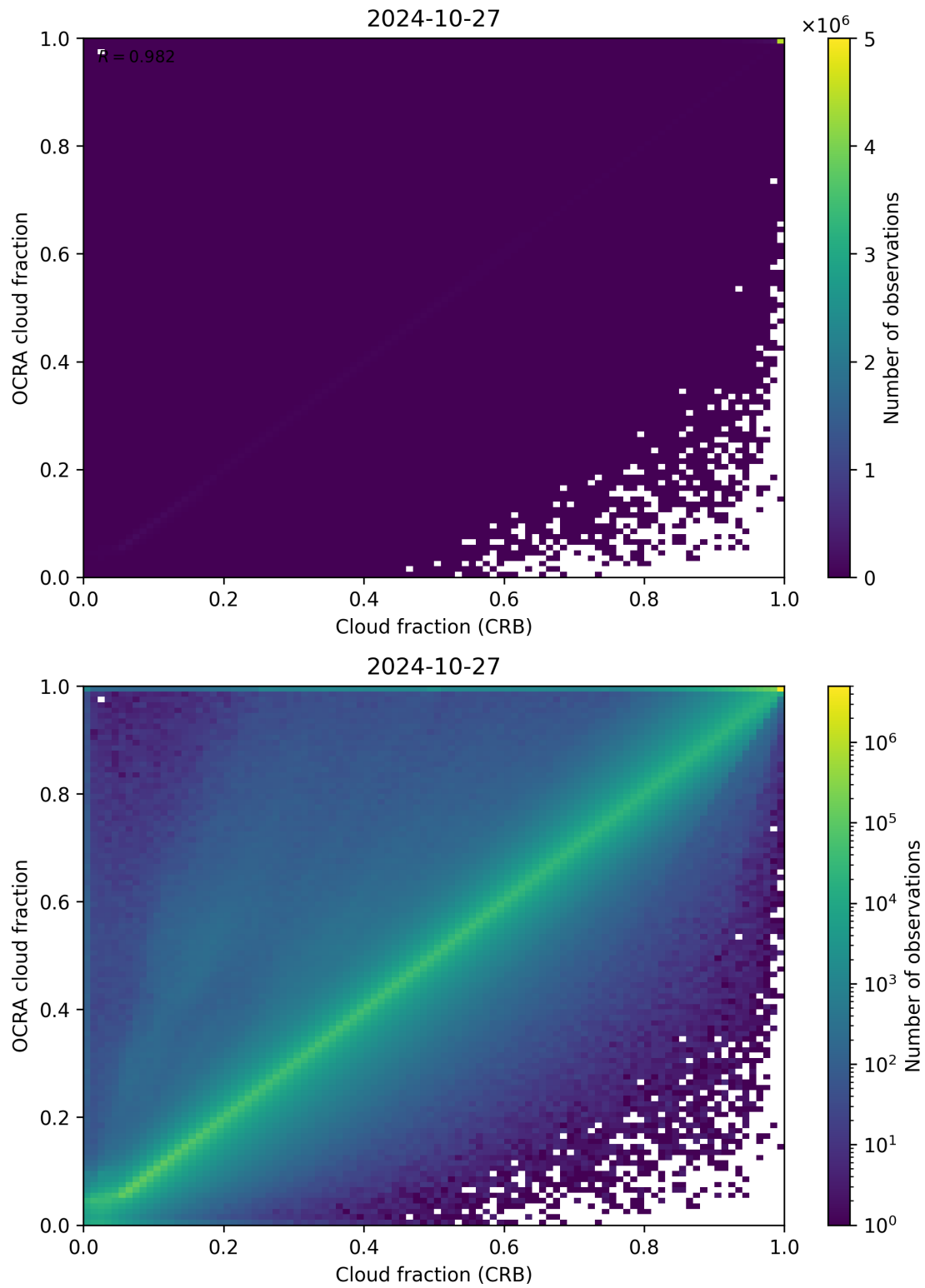
Figure 78: Scatter density plot of “Cloud fraction (CRB)” against “OCRA cloud fraction” for 2024-10-26 to 2024-10-28.
