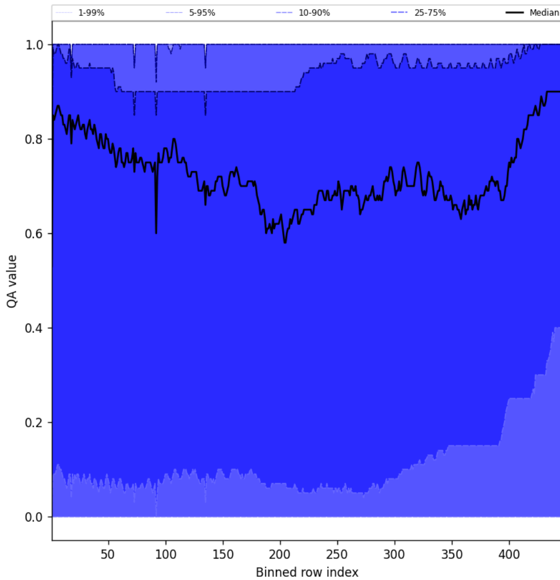
Figure 54: Along track statistics of “QA value” for 2024-10-26 to 2024-10-28
