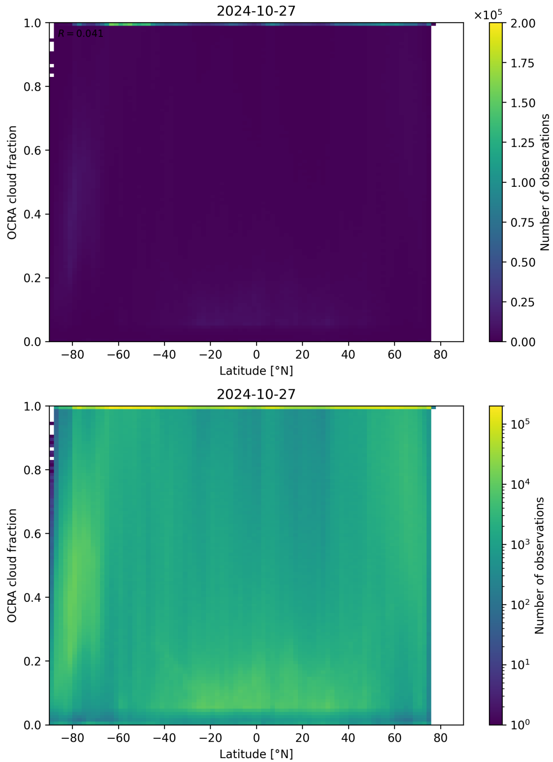
Figure 93: Scatter density plot of “Latitude” against “OCRA cloud fraction” for 2024-10-26 to 2024-10-28.
