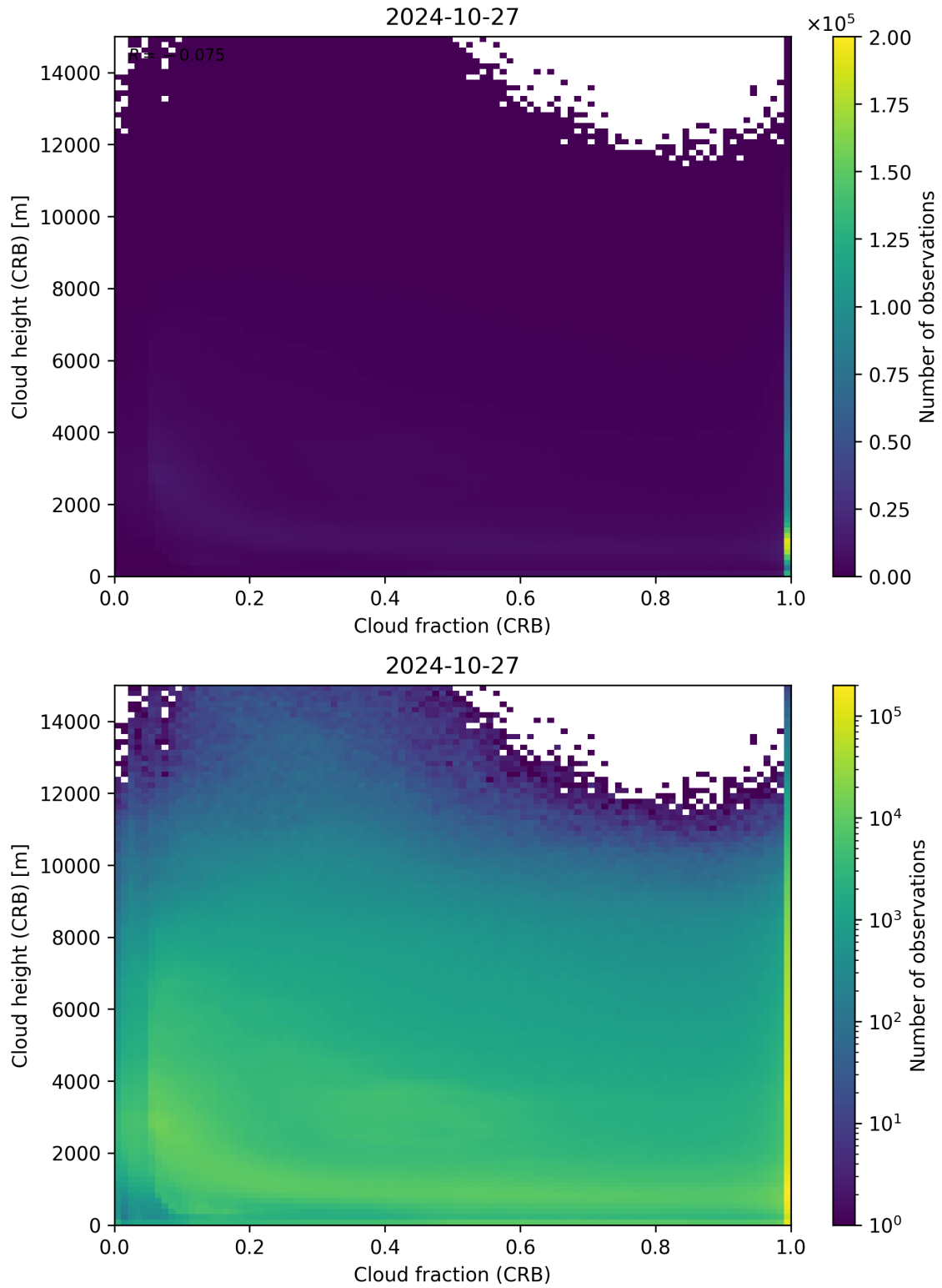
Figure 79: Scatter density plot of “Cloud fraction (CRB)” against “Cloud height (CRB)” for 2024-10-26 to 2024-10-28.
