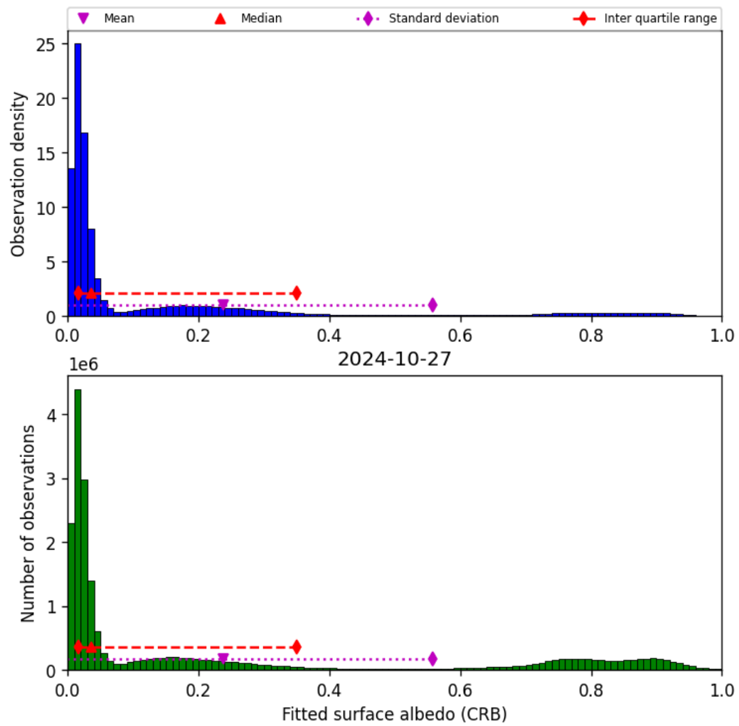
Figure 46: Histogram of “Fitted surface albedo (CRB)” for 2024-10-26 to 2024-10-28
