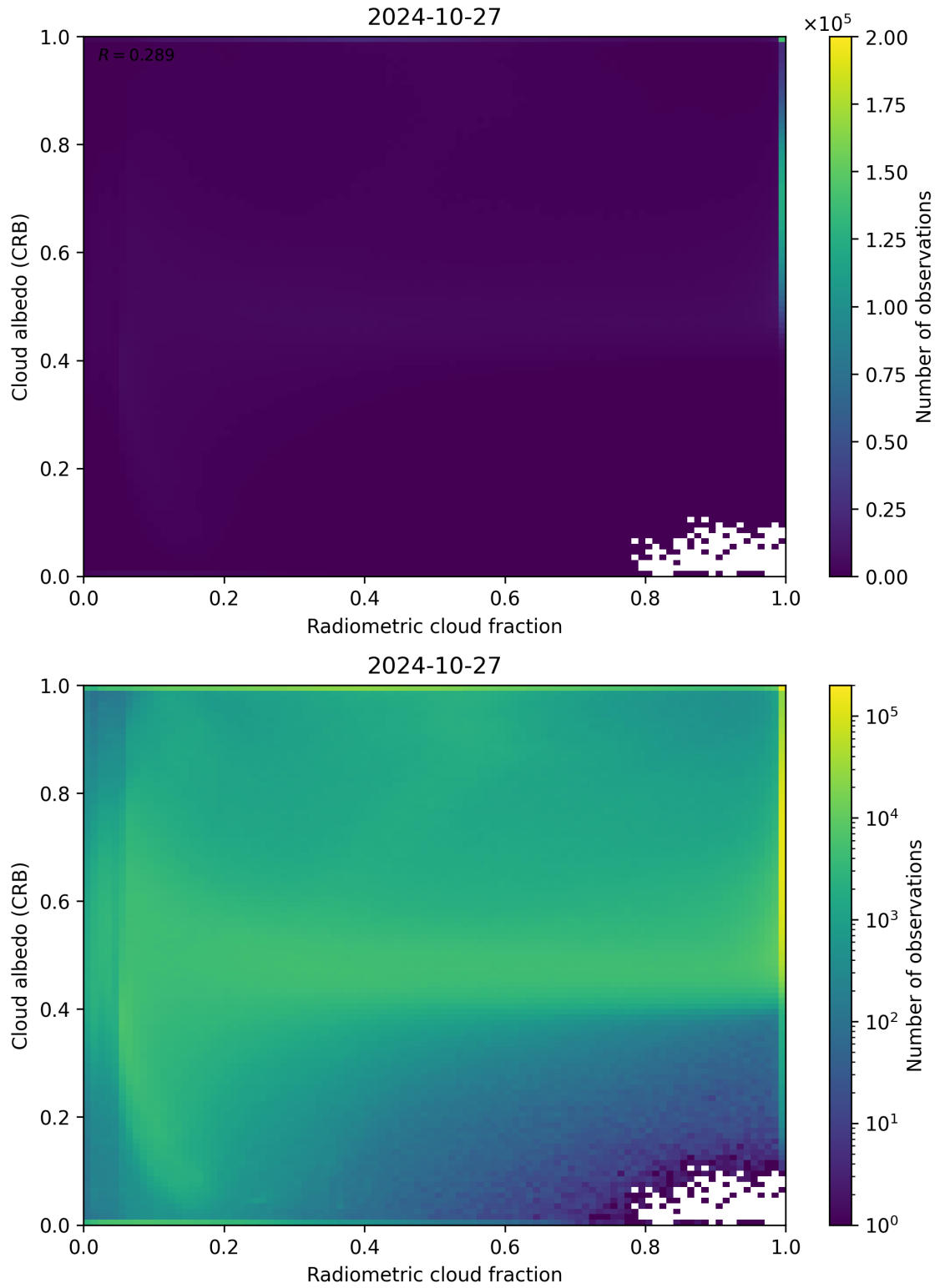
Figure 71: Scatter density plot of “Radiometric cloud fraction” against “Cloud albedo (CRB)” for 2024-10-26 to 2024-10-28.
