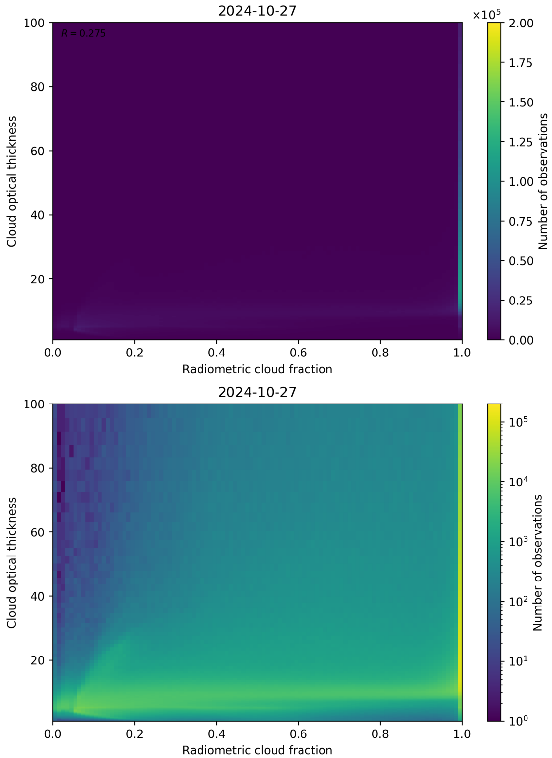
Figure 75: Scatter density plot of “Radiometric cloud fraction” against “Cloud optical thickness” for 2024-10-26 to 2024-10-28.
