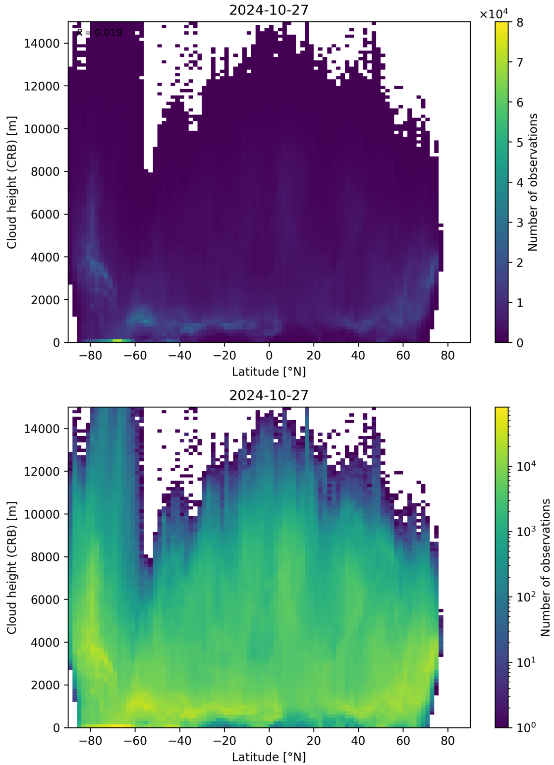
Figure 95: Scatter density plot of “Latitude” against “Cloud height (CRB)” for 2024-10-26 to 2024-10-28.
