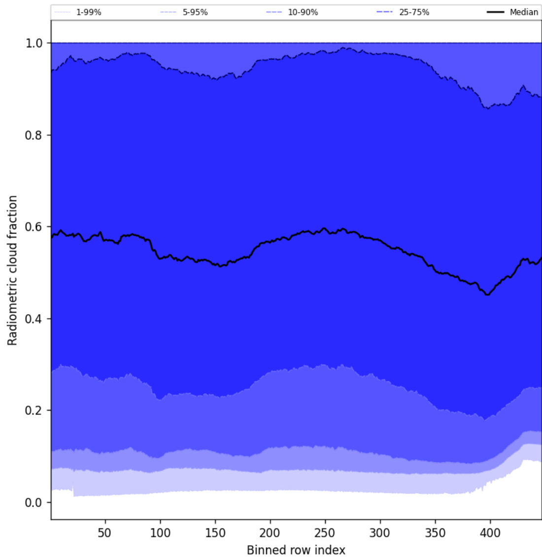
Figure 55: Along track statistics of “Radiometric cloud fraction” for 2024-10-26 to 2024-10-28
