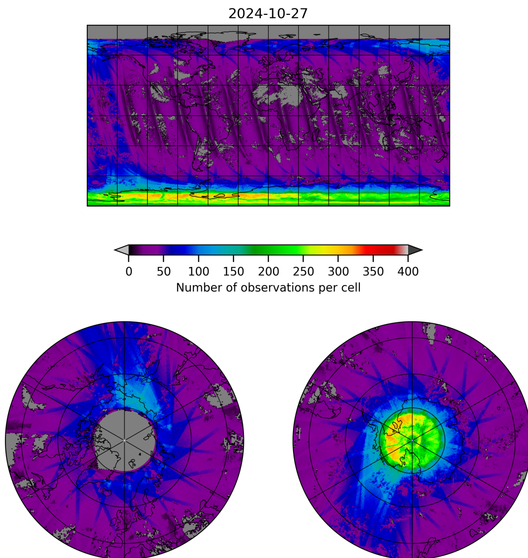
Figure 21: Map of the number of observations for 2024-10-26 to 2024-10-28
