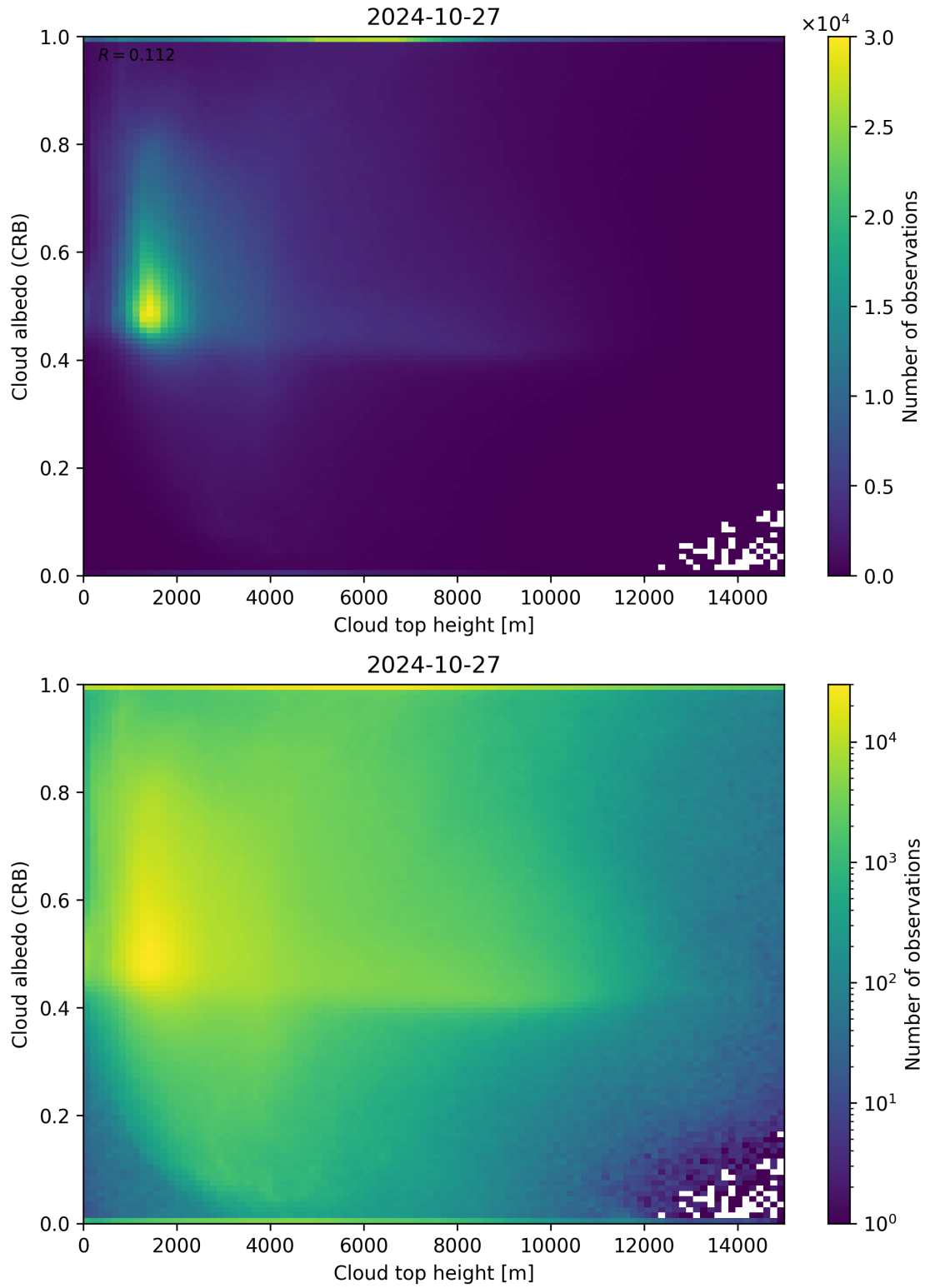
Figure 86: Scatter density plot of “Cloud top height” against “Cloud albedo (CRB)” for 2024-10-26 to 2024-10-28.
