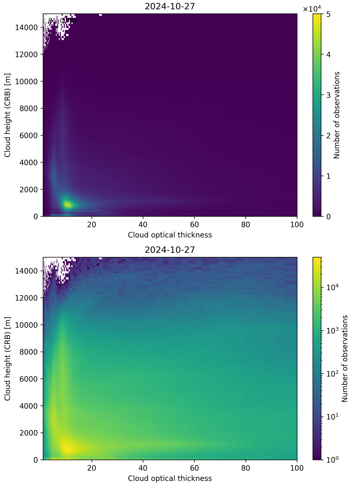
Figure 85: Scatter density plot of “Cloud optical thickness” against “Cloud height (CRB)” for 2024-10-26 to 2024-10-28.
