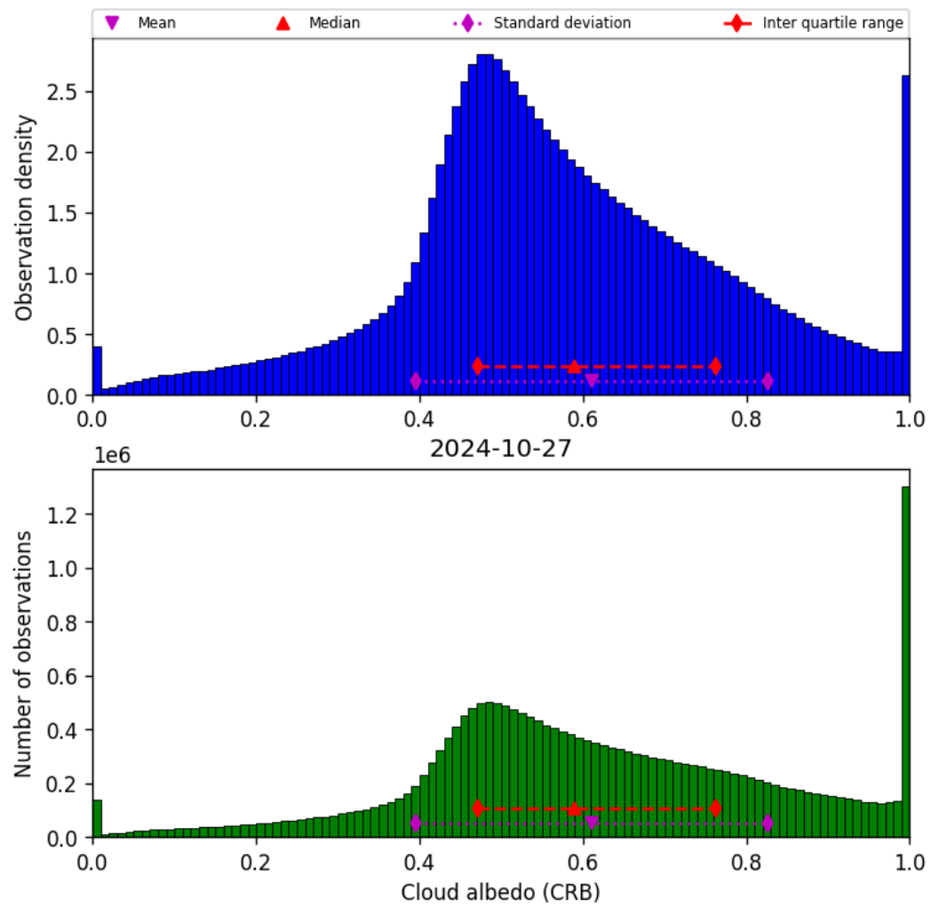
Figure 44: Histogram of “Cloud albedo (CRB)” for 2024-10-26 to 2024-10-28
