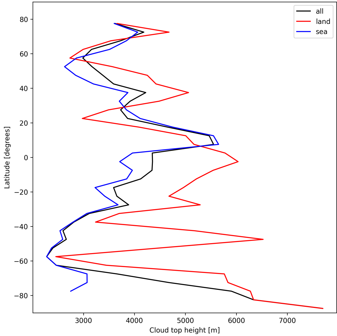
Figure 24: Zonal average of “Cloud top height” for 2024-10-26 to 2024-10-28.
