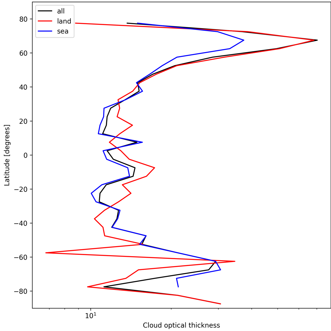
Figure 25: Zonal average of “Cloud optical thickness” for 2024-10-26 to 2024-10-28.
