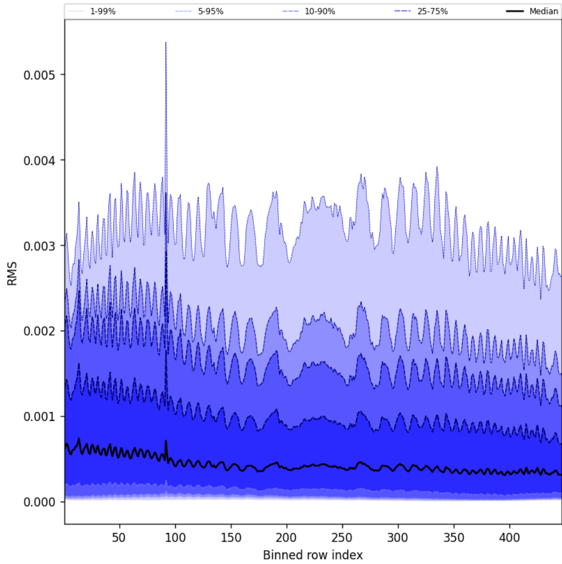
Figure 63: Along track statistics of “RMS” for 2024-10-26 to 2024-10-28
