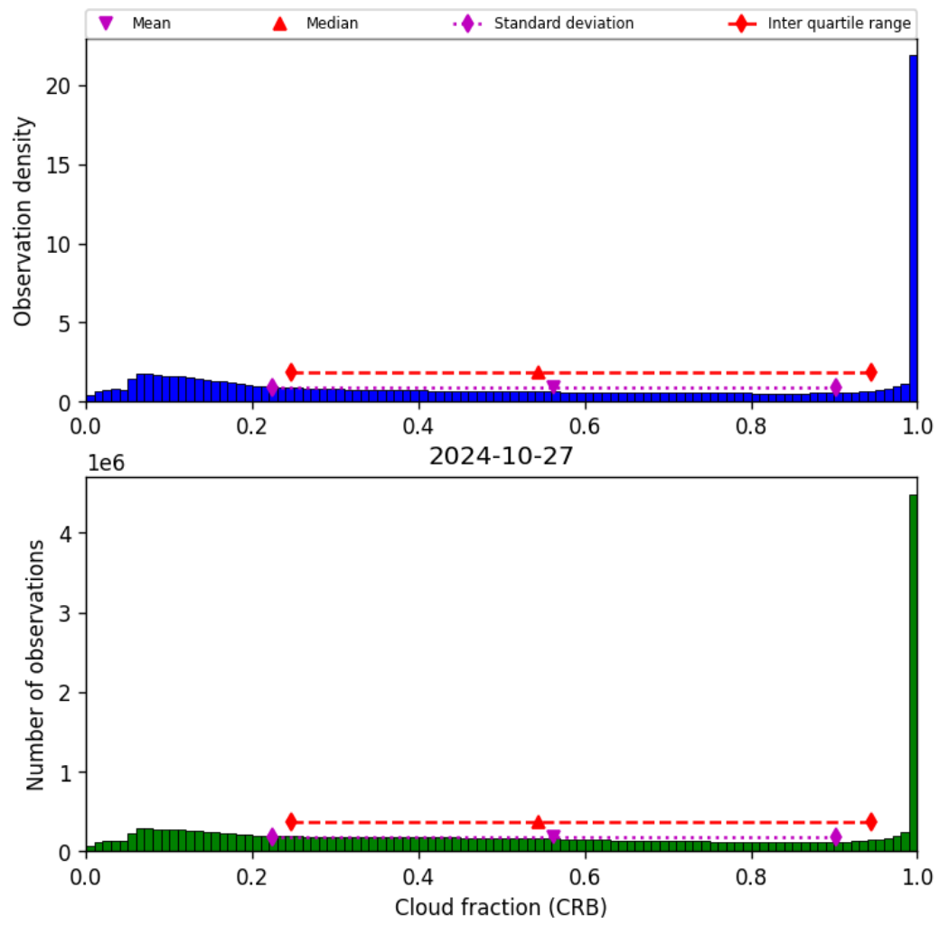
Figure 42: Histogram of “Cloud fraction (CRB)” for 2024-10-26 to 2024-10-28
