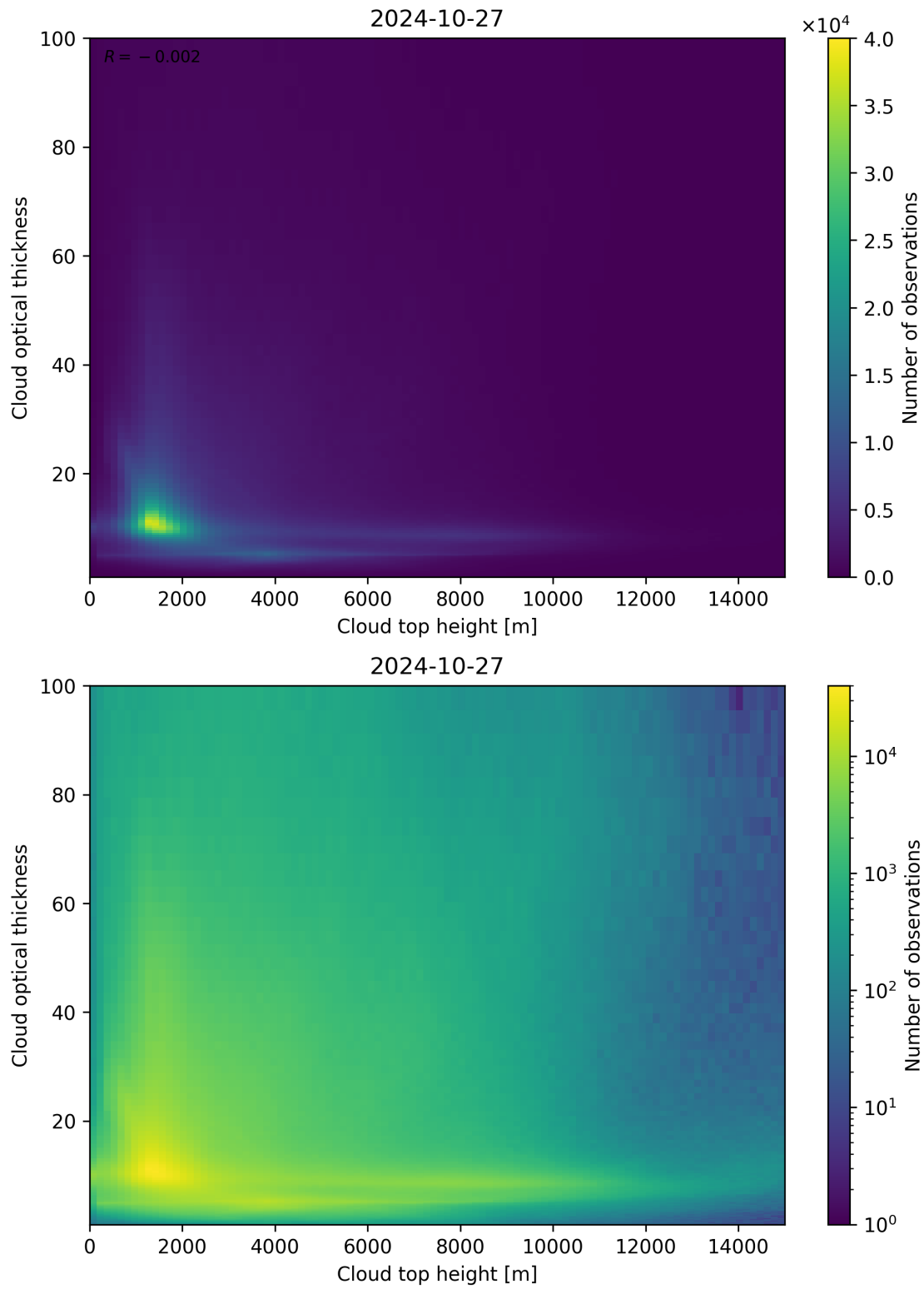
Figure 90: Scatter density plot of “Cloud top height” against “Cloud optical thickness” for 2024-10-26 to 2024-10-28.
