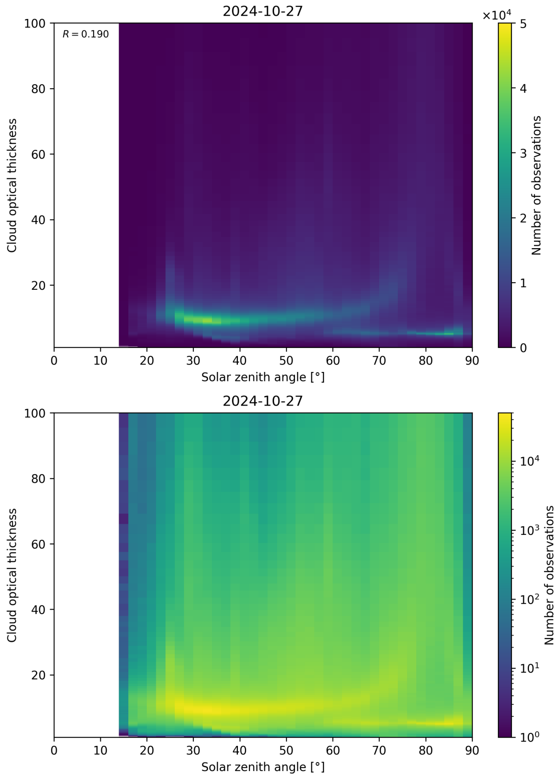
Figure 103: Scatter density plot of “Solar zenith angle” against “Cloud optical thickness” for 2024-10-26 to 2024-10-28.
