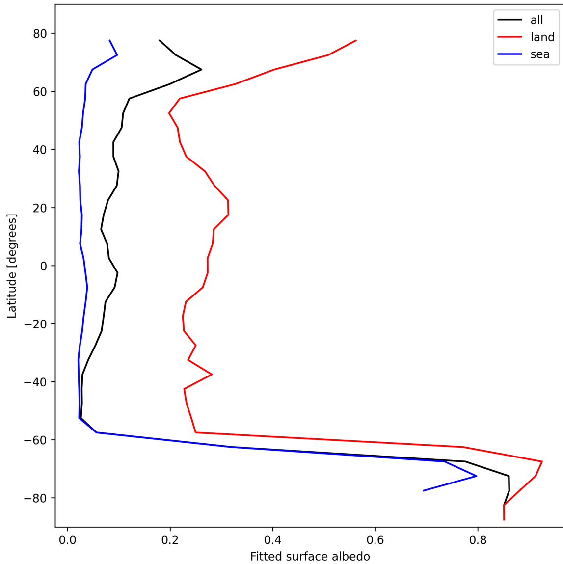
Figure 29: Zonal average of “Fitted surface albedo” for 2024-10-26 to 2024-10-28.
