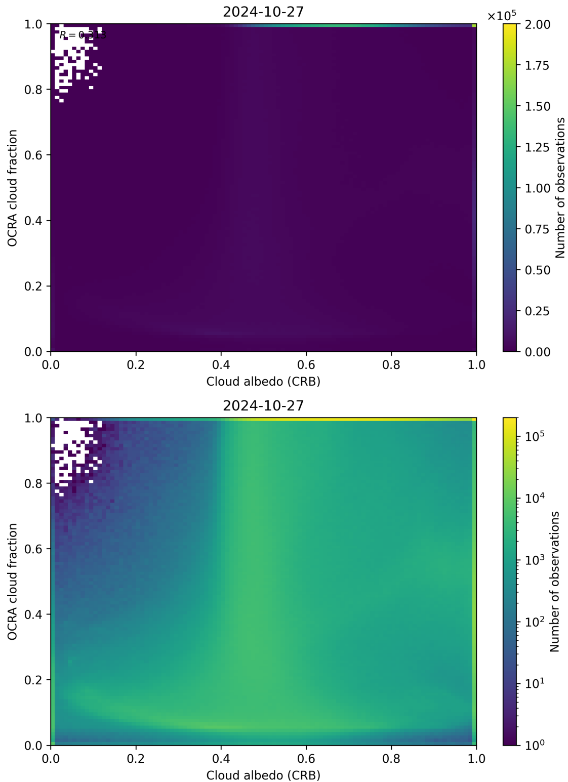
Figure 70: Scatter density plot of “Cloud albedo (CRB)” against “OCRA cloud fraction” for 2024-10-26 to 2024-10-28.
