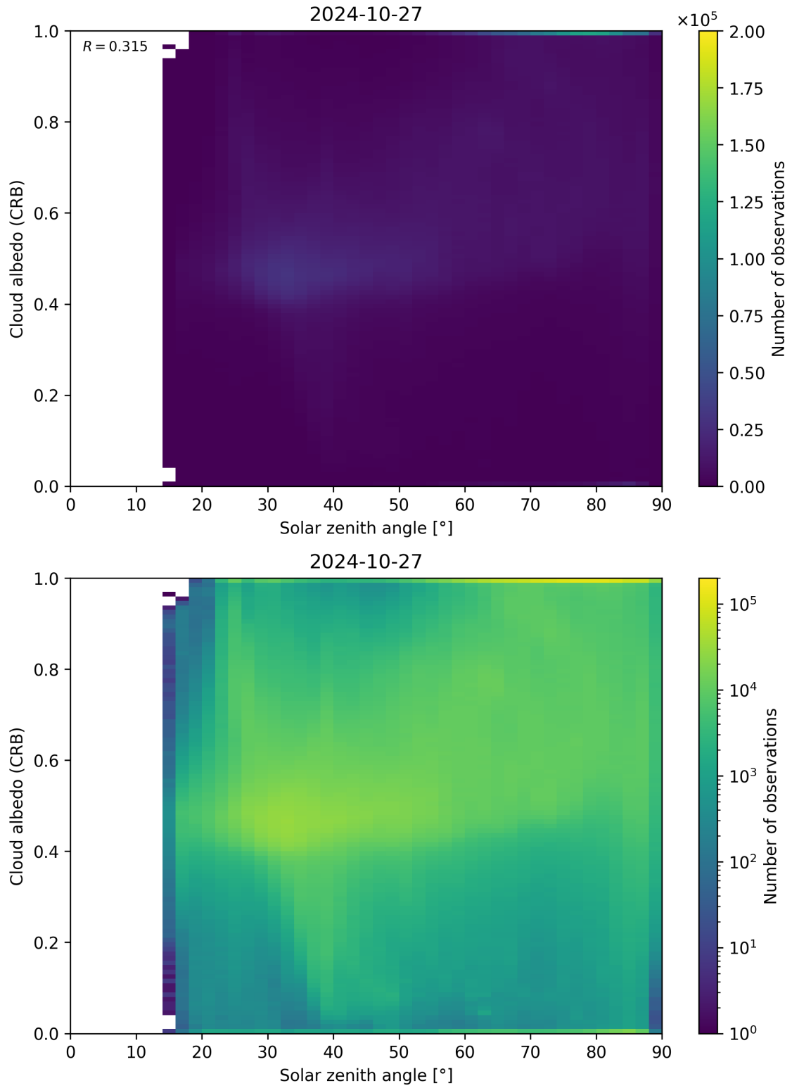
Figure 98: Scatter density plot of “Solar zenith angle” against “Cloud albedo (CRB)” for 2024-10-26 to 2024-10-28.
