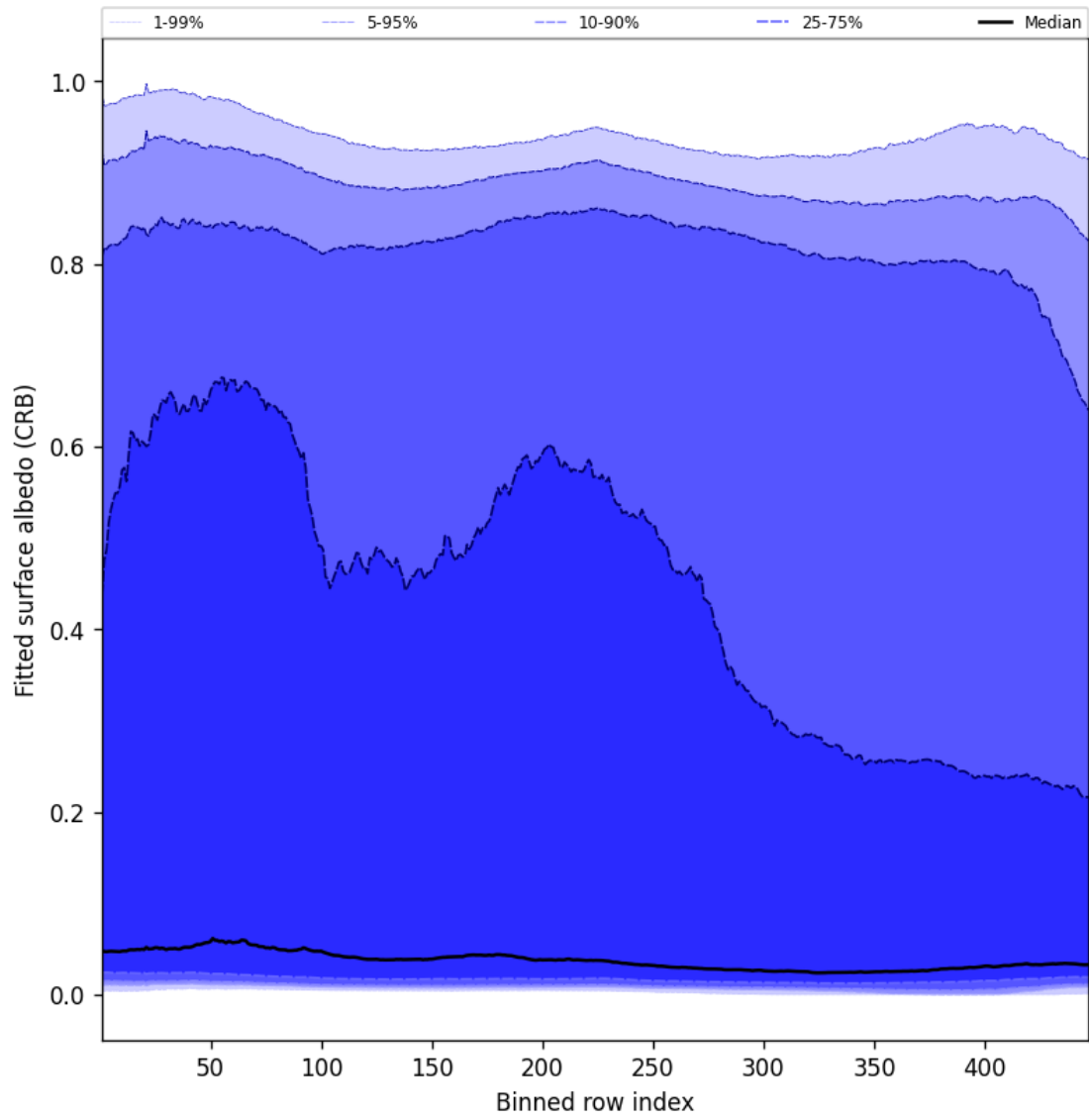
Figure 62: Along track statistics of “Fitted surface albedo (CRB)” for 2024-10-26 to 2024-10-28
