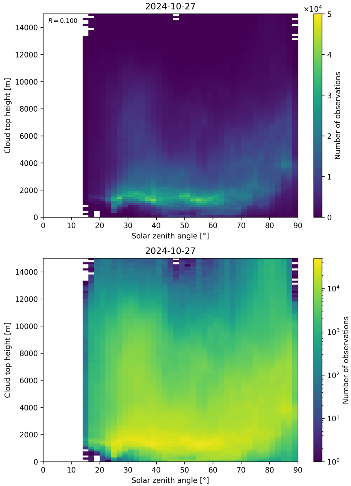
Figure 104: Scatter density plot of “Solar zenith angle” against “Cloud top height” for 2024-10-26 to 2024-10-28.
