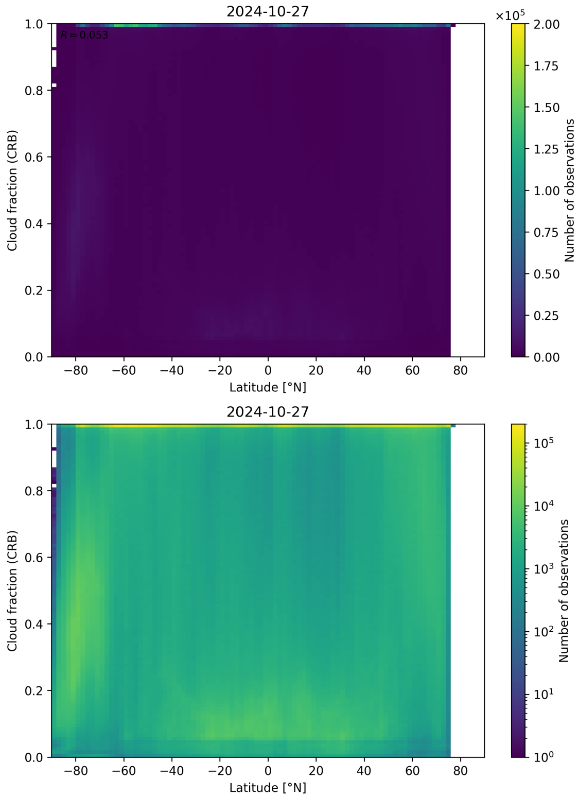
Figure 94: Scatter density plot of “Latitude” against “Cloud fraction (CRB)” for 2024-10-26 to 2024-10-28.
