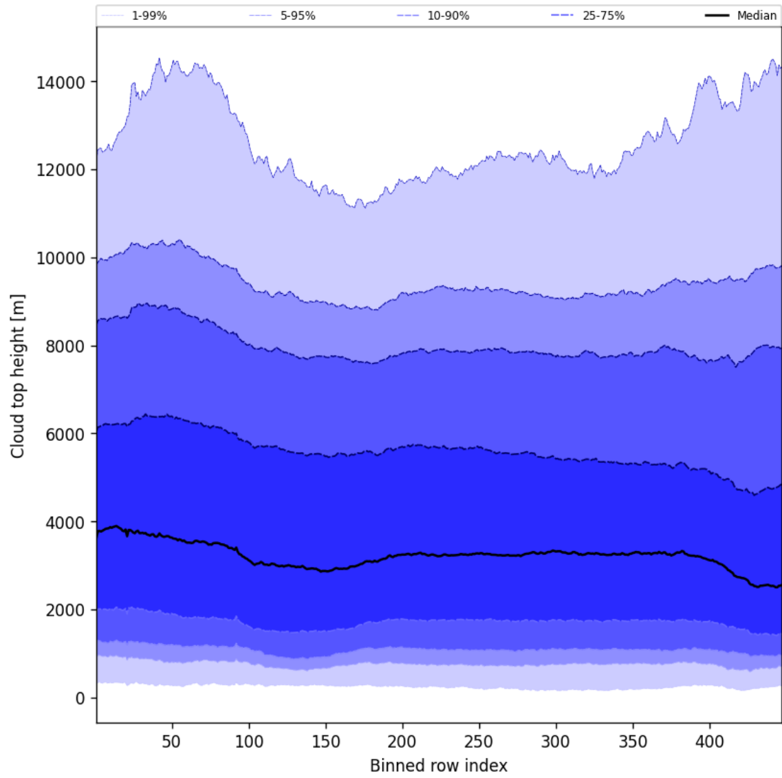
Figure 56: Along track statistics of “Cloud top height” for 2024-10-26 to 2024-10-28
