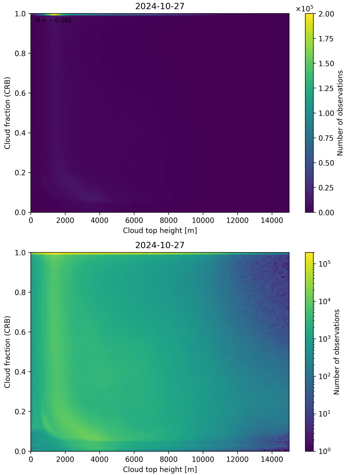
Figure 88: Scatter density plot of “Cloud top height” against “Cloud fraction (CRB)” for 2024-10-26 to 2024-10-28.
