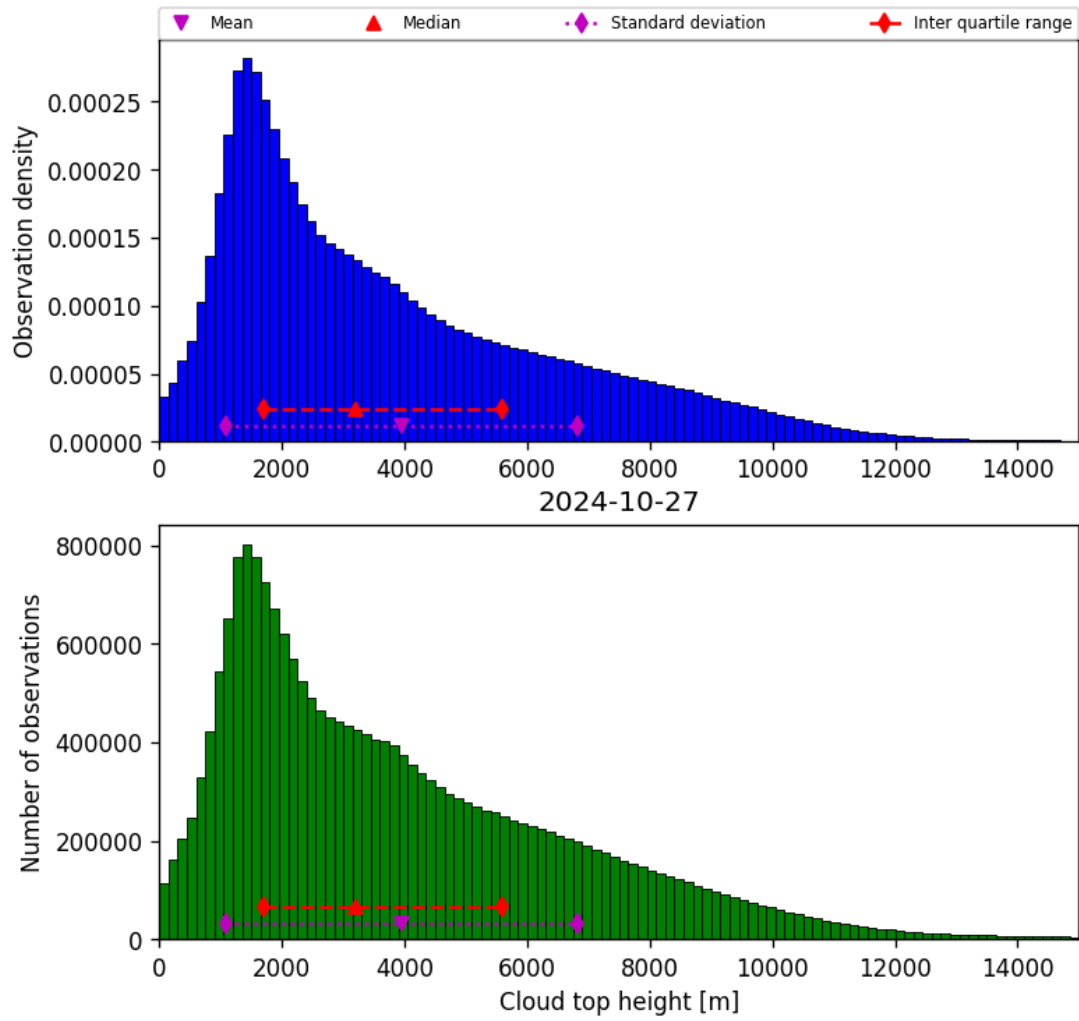
Figure 40: Histogram of “Cloud top height” for 2024-10-26 to 2024-10-28
