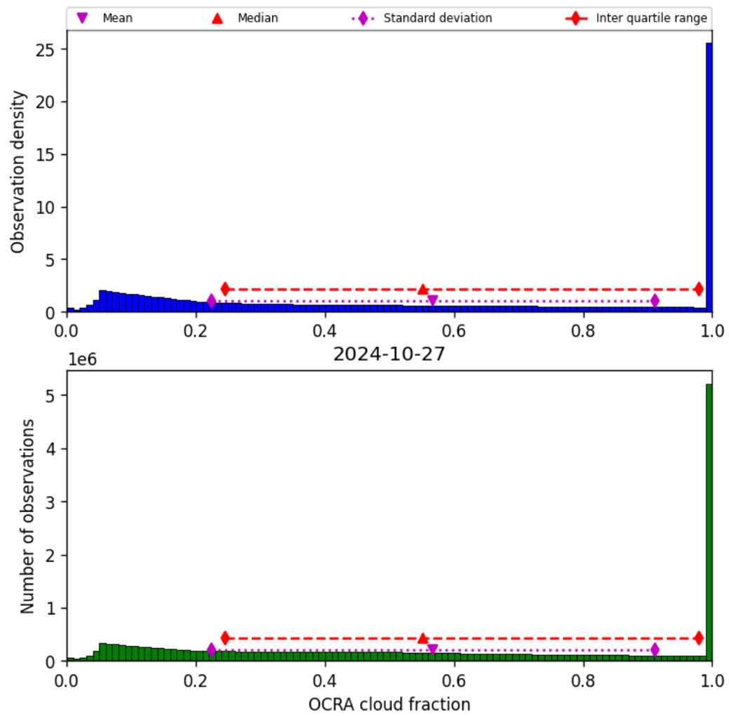
Figure 50: Histogram of “OCRA cloud fraction” for 2024-10-26 to 2024-10-28
