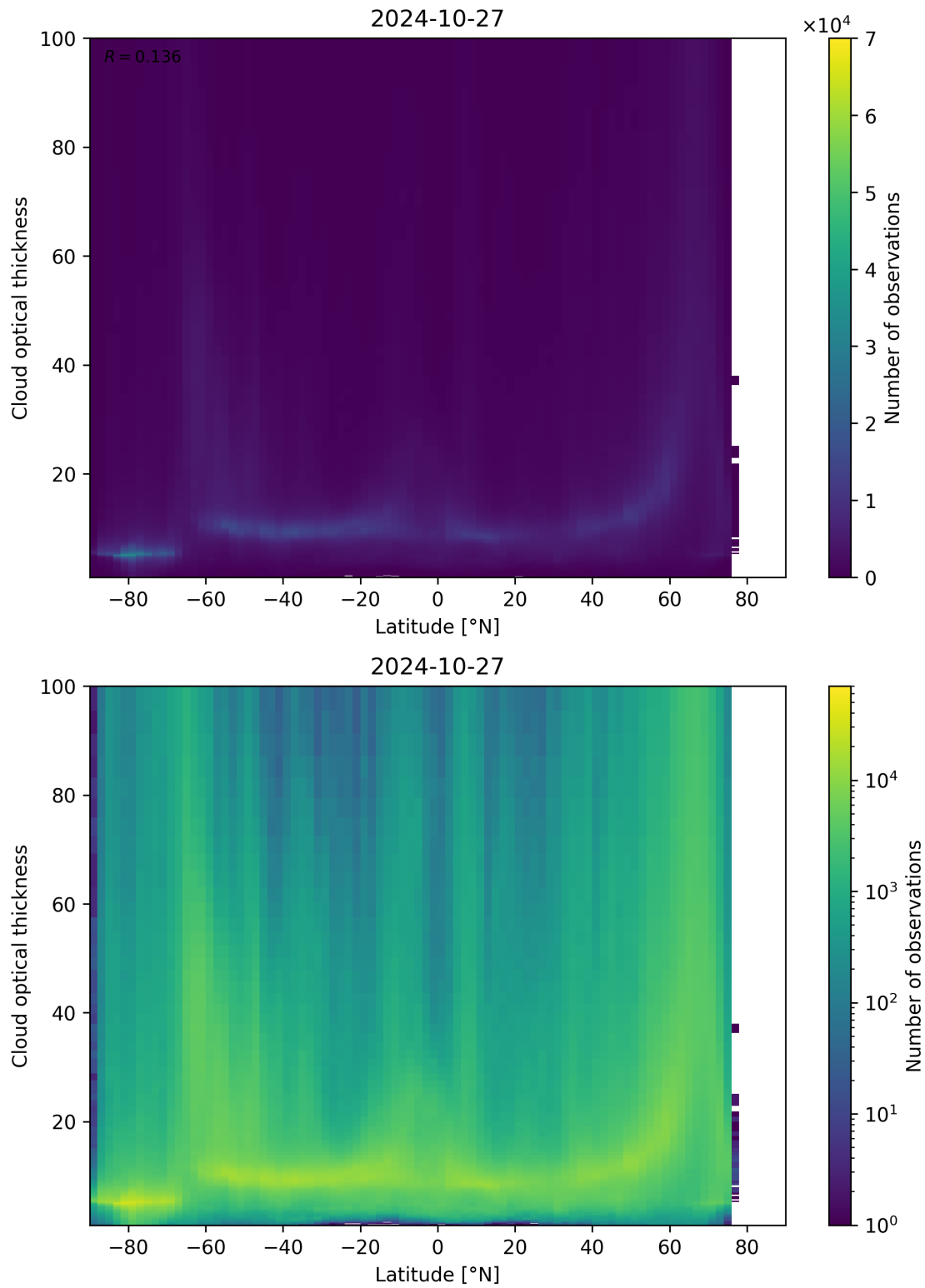
Figure 96: Scatter density plot of “Latitude” against “Cloud optical thickness” for 2024-10-26 to 2024-10-28.
