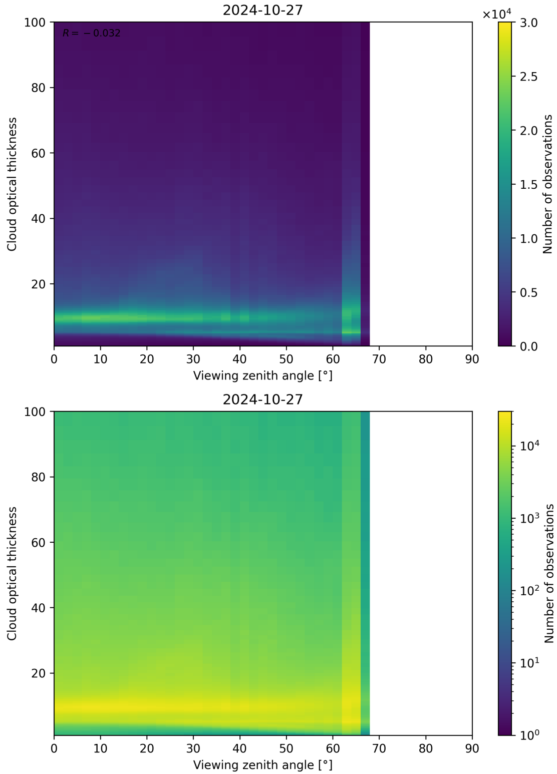
Figure 111: Scatter density plot of “Viewing zenith angle” against “Cloud optical thickness” for 2024-10-26 to 2024-10-28.
