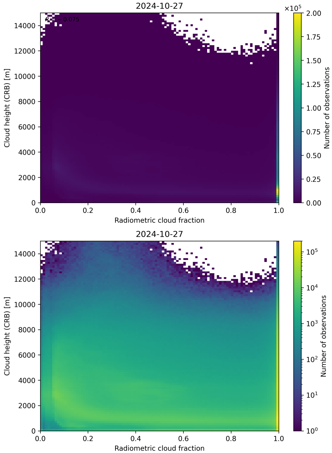
Figure 74: Scatter density plot of “Radiometric cloud fraction” against “Cloud height (CRB)” for 2024-10-26 to 2024-10-28.
