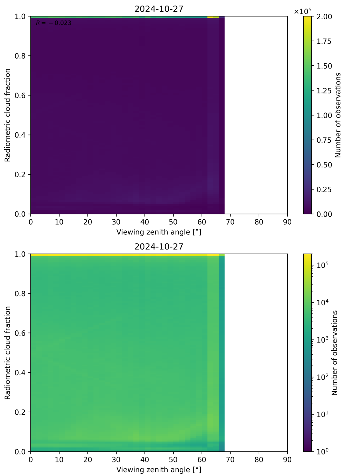
Figure 107: Scatter density plot of “Viewing zenith angle” against “Radiometric cloud fraction” for 2024-10-26 to 2024-10-28.
