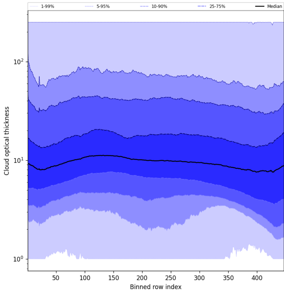
Figure 57: Along track statistics of “Cloud optical thickness” for 2024-10-26 to 2024-10-28
