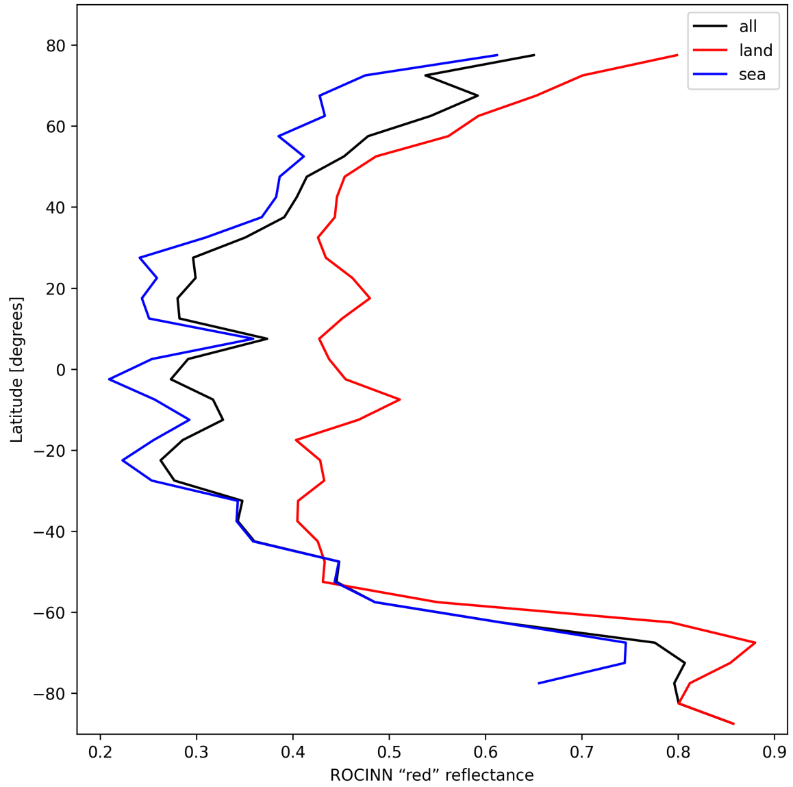
Figure 37: Zonal average of “ROCINN “red” reflectance” for 2024-10-26 to 2024-10-28.
