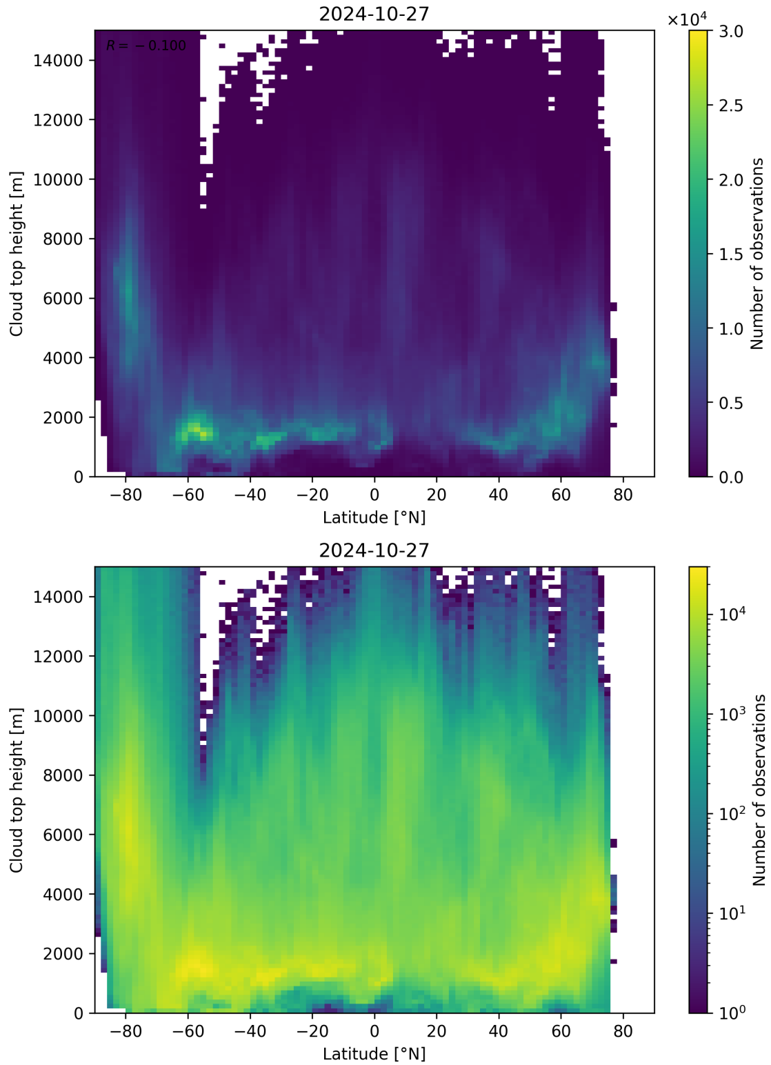
Figure 97: Scatter density plot of “Latitude” against “Cloud top height” for 2024-10-26 to 2024-10-28.
