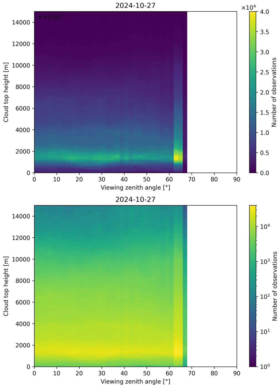
Figure 112: Scatter density plot of “Viewing zenith angle” against “Cloud top height” for 2024-10-26 to 2024-10-28.
