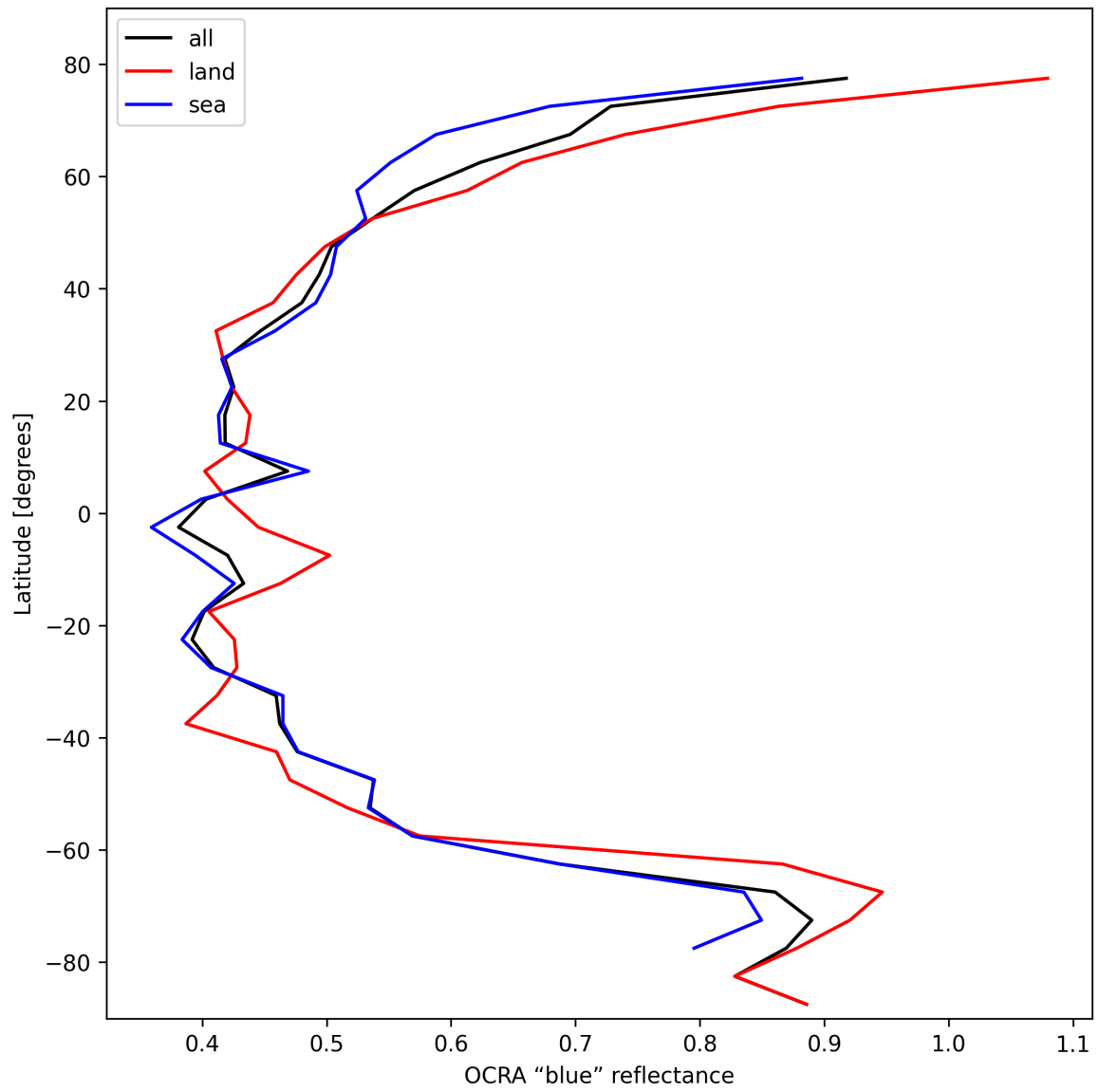
Figure 35: Zonal average of “OCRA “blue” reflectance” for 2024-10-26 to 2024-10-28.
