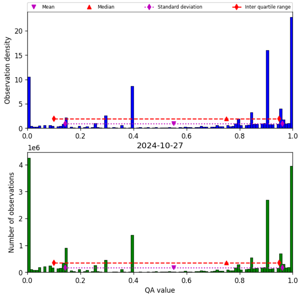
Figure 38: Histogram of “QA value” for 2024-10-26 to 2024-10-28
