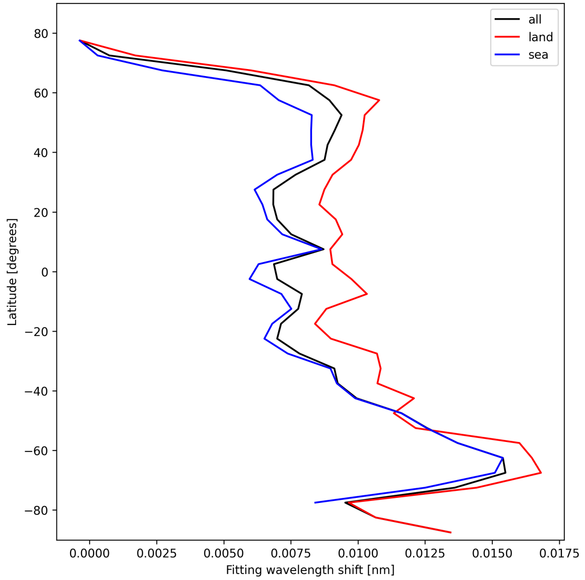
Figure 33: Zonal average of “Fitting wavelength shift” for 2024-10-26 to 2024-10-28.
