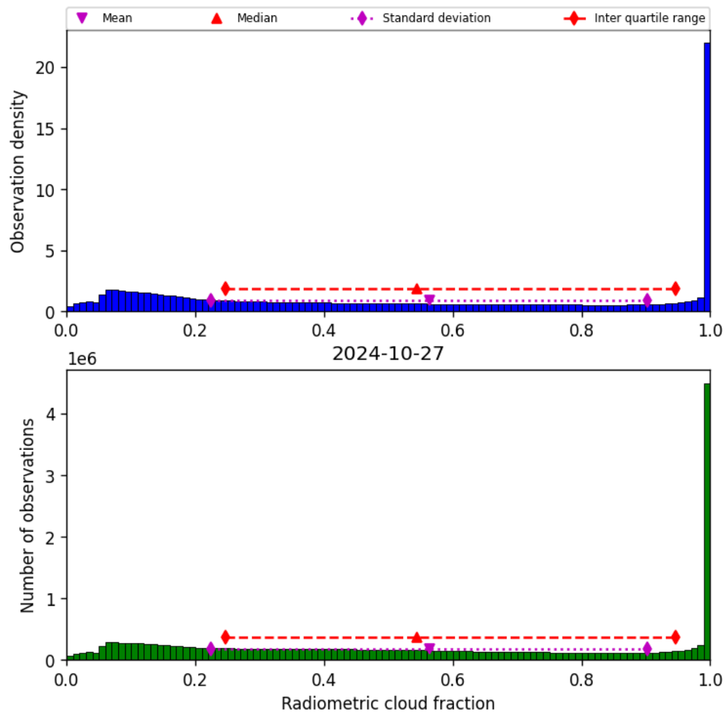
Figure 39: Histogram of “Radiometric cloud fraction” for 2024-10-26 to 2024-10-28
