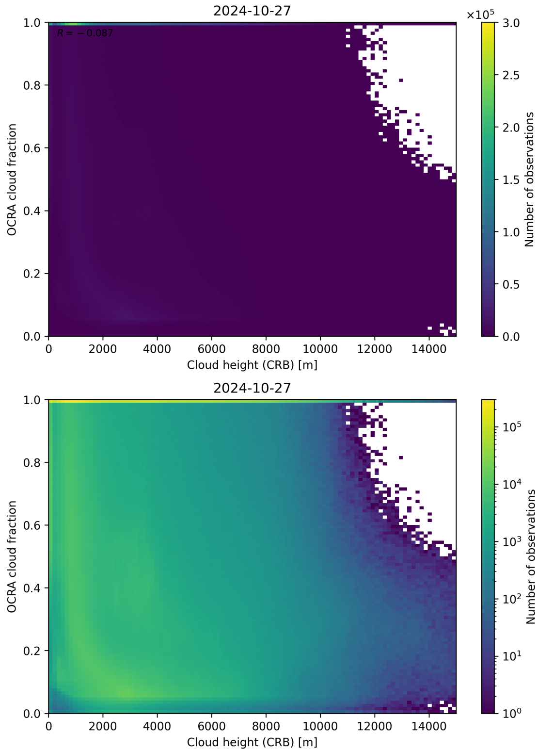
Figure 81: Scatter density plot of “Cloud height (CRB)” against “OCRA cloud fraction” for 2024-10-26 to 2024-10-28.
