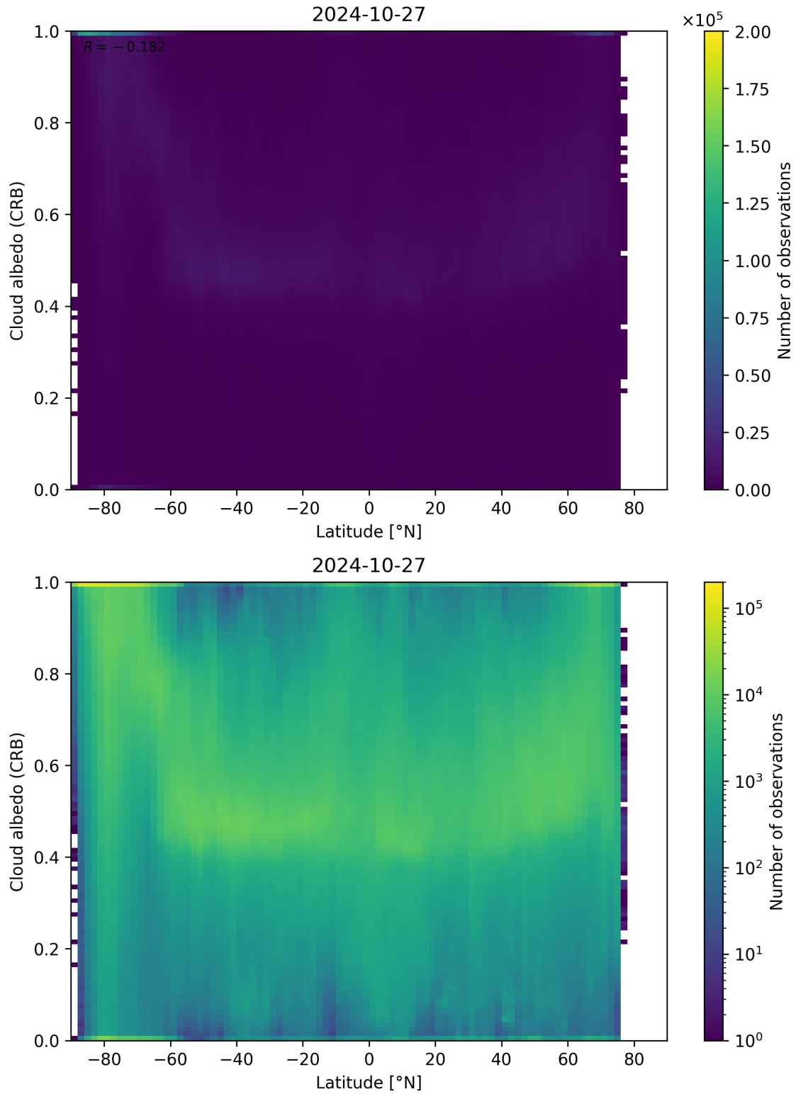
Figure 91: Scatter density plot of “Latitude” against “Cloud albedo (CRB)” for 2024-10-26 to 2024-10-28.
