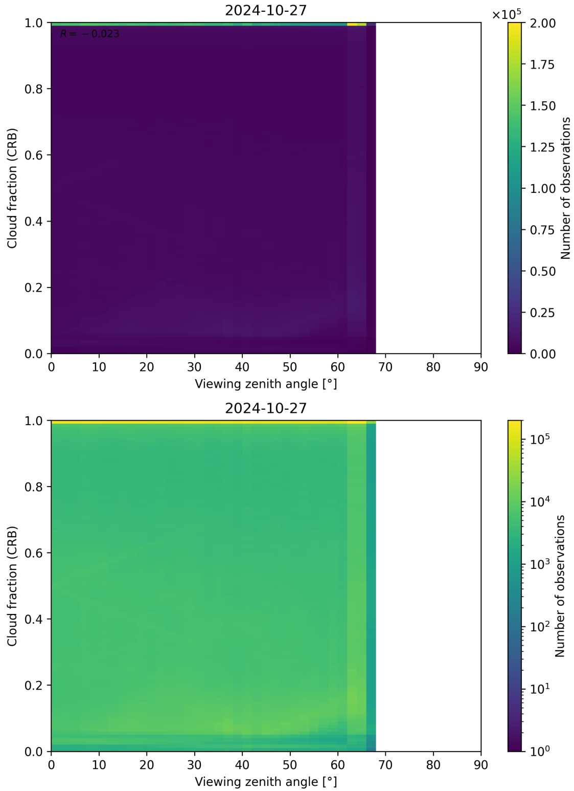
Figure 109: Scatter density plot of “Viewing zenith angle” against “Cloud fraction (CRB)” for 2024-10-26 to 2024-10-28.
