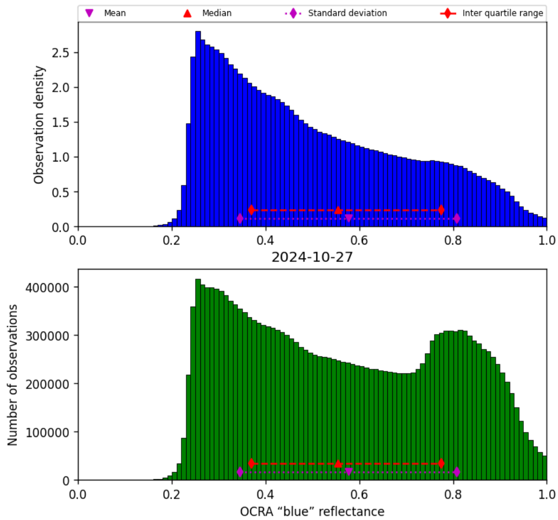
Figure 51: Histogram of “OCRA “blue” reflectance” for 2024-10-26 to 2024-10-28
