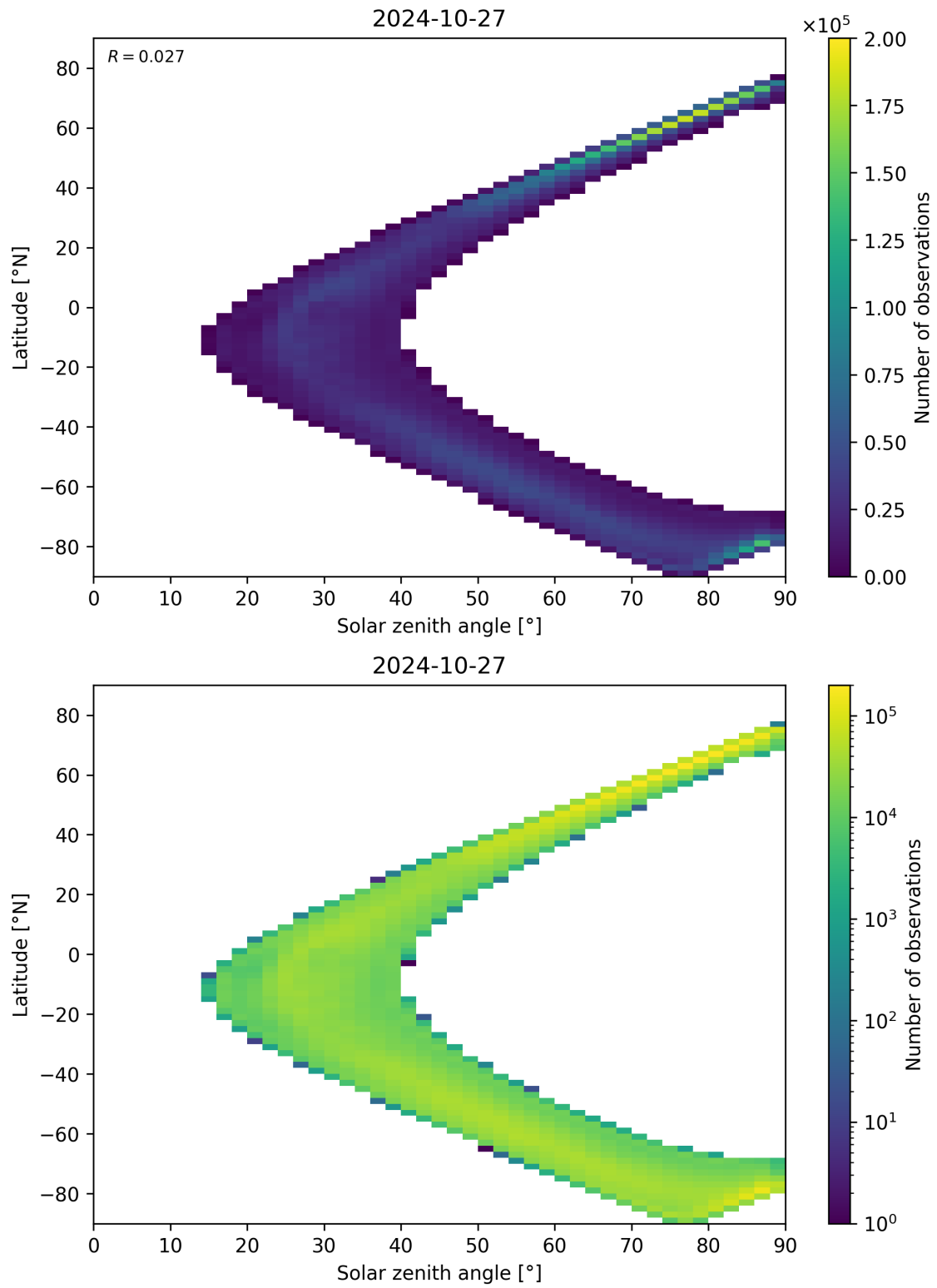
Figure 105: Scatter density plot of “Solar zenith angle” against “Latitude” for 2024-10-26 to 2024-10-28.
