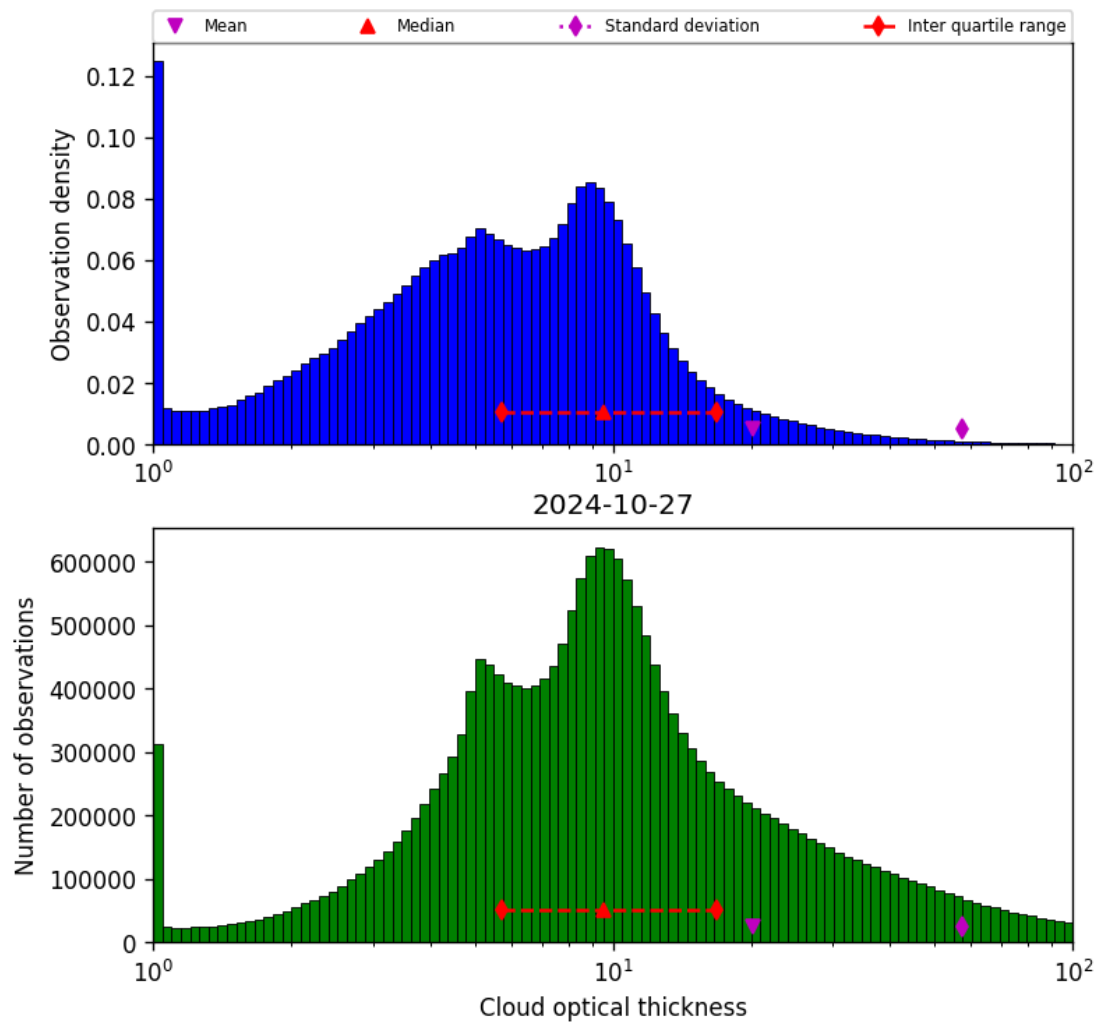
Figure 41: Histogram of “Cloud optical thickness” for 2024-10-26 to 2024-10-28
