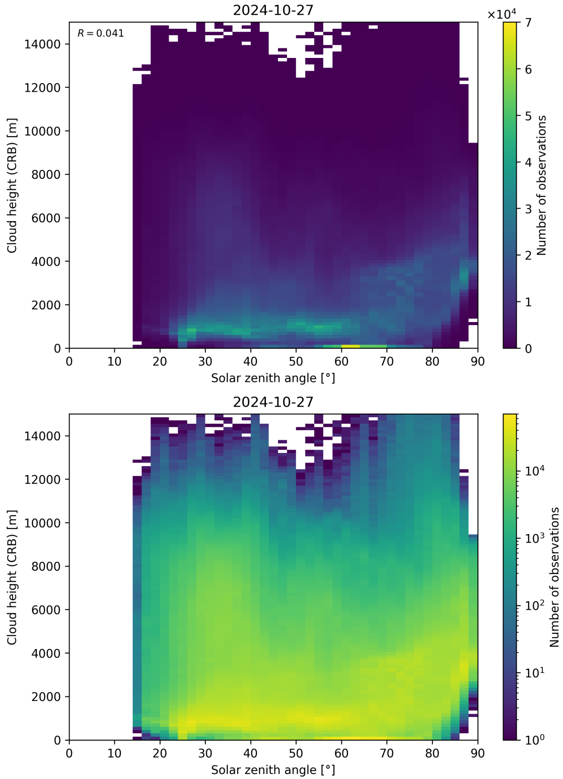
Figure 102: Scatter density plot of “Solar zenith angle” against “Cloud height (CRB)” for 2024-10-26 to 2024-10-28.
