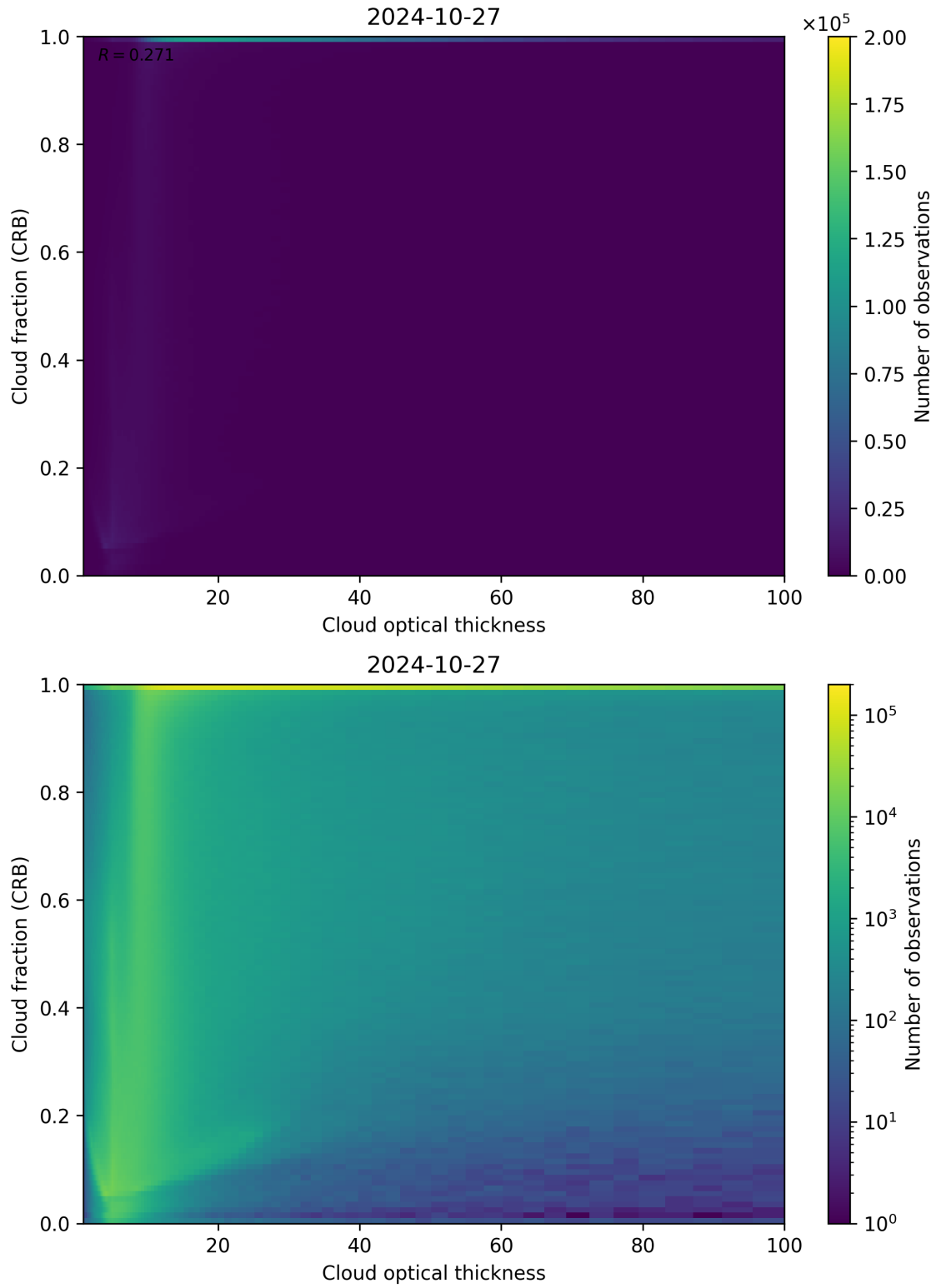
Figure 84: Scatter density plot of “Cloud optical thickness” against “Cloud fraction (CRB)” for 2024-10-26 to 2024-10-28.
