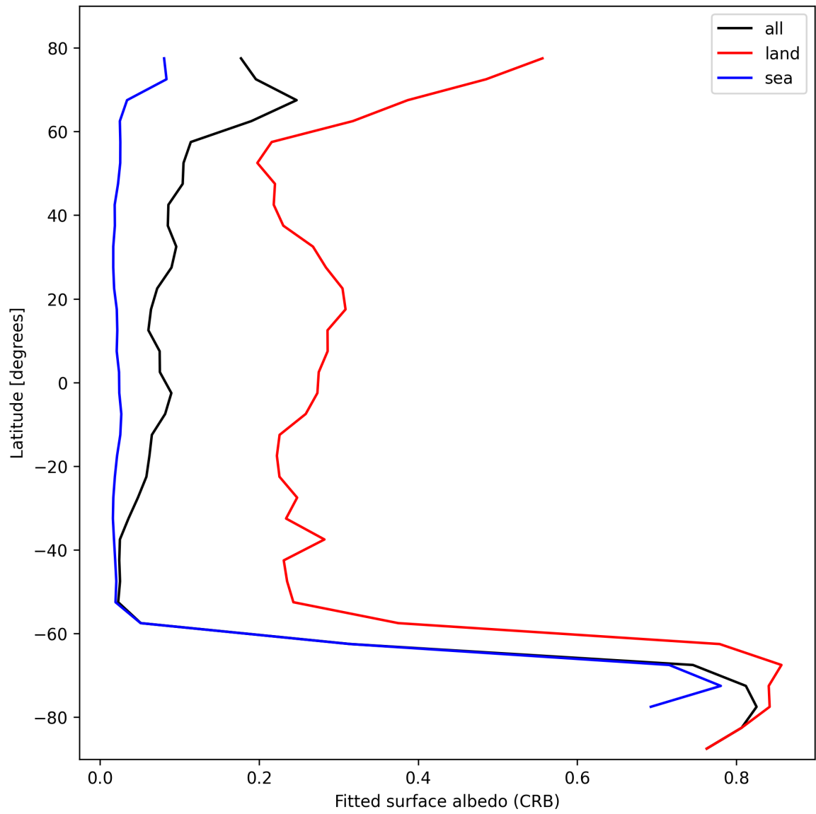
Figure 30: Zonal average of “Fitted surface albedo (CRB)” for 2024-10-26 to 2024-10-28.
