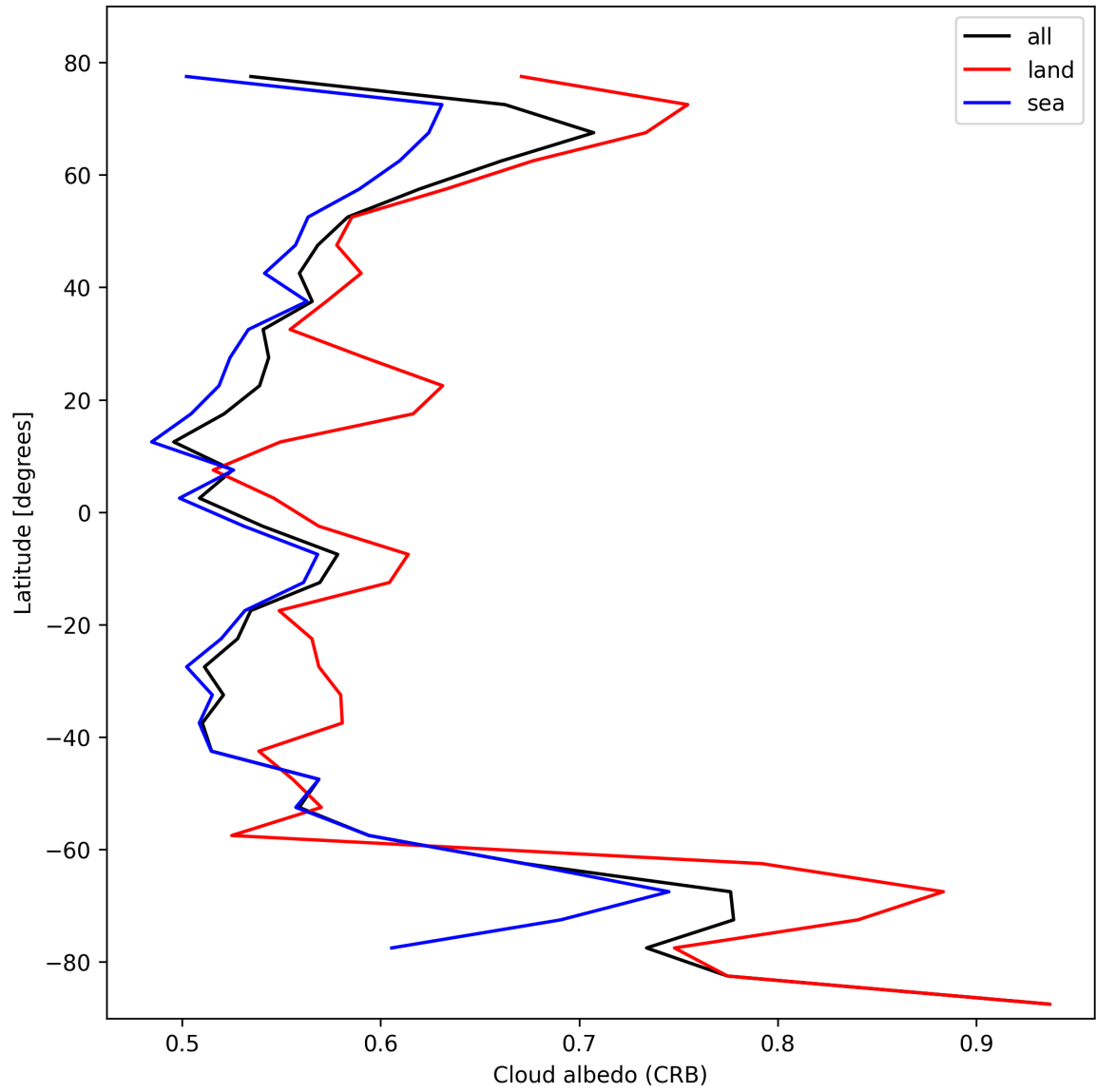
Figure 28: Zonal average of “Cloud albedo (CRB)” for 2024-10-26 to 2024-10-28.
