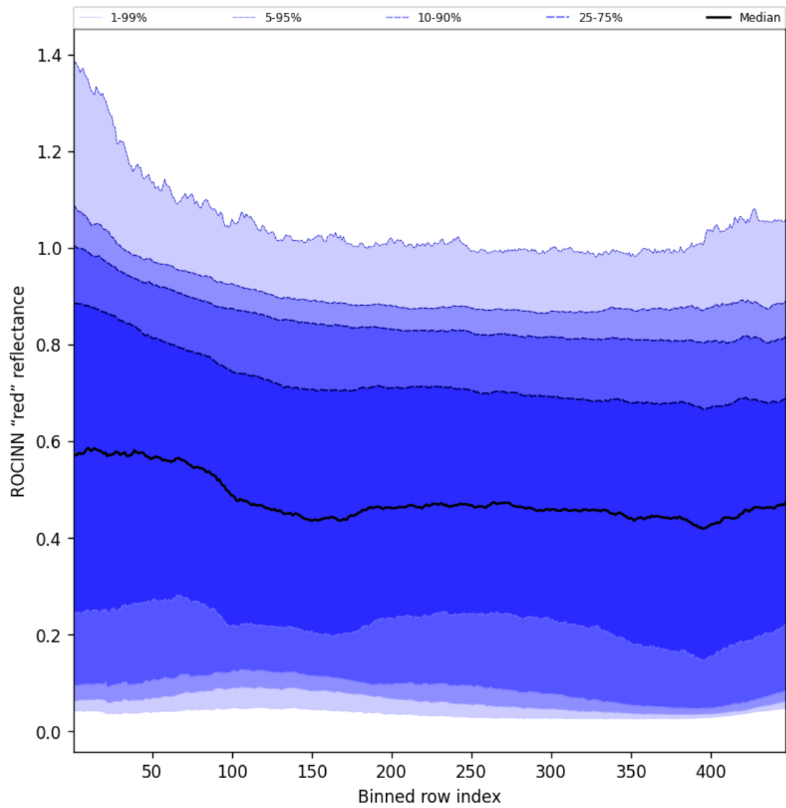
Figure 69: Along track statistics of “ROCINN “red” reflectance” for 2024-10-26 to 2024-10-28
