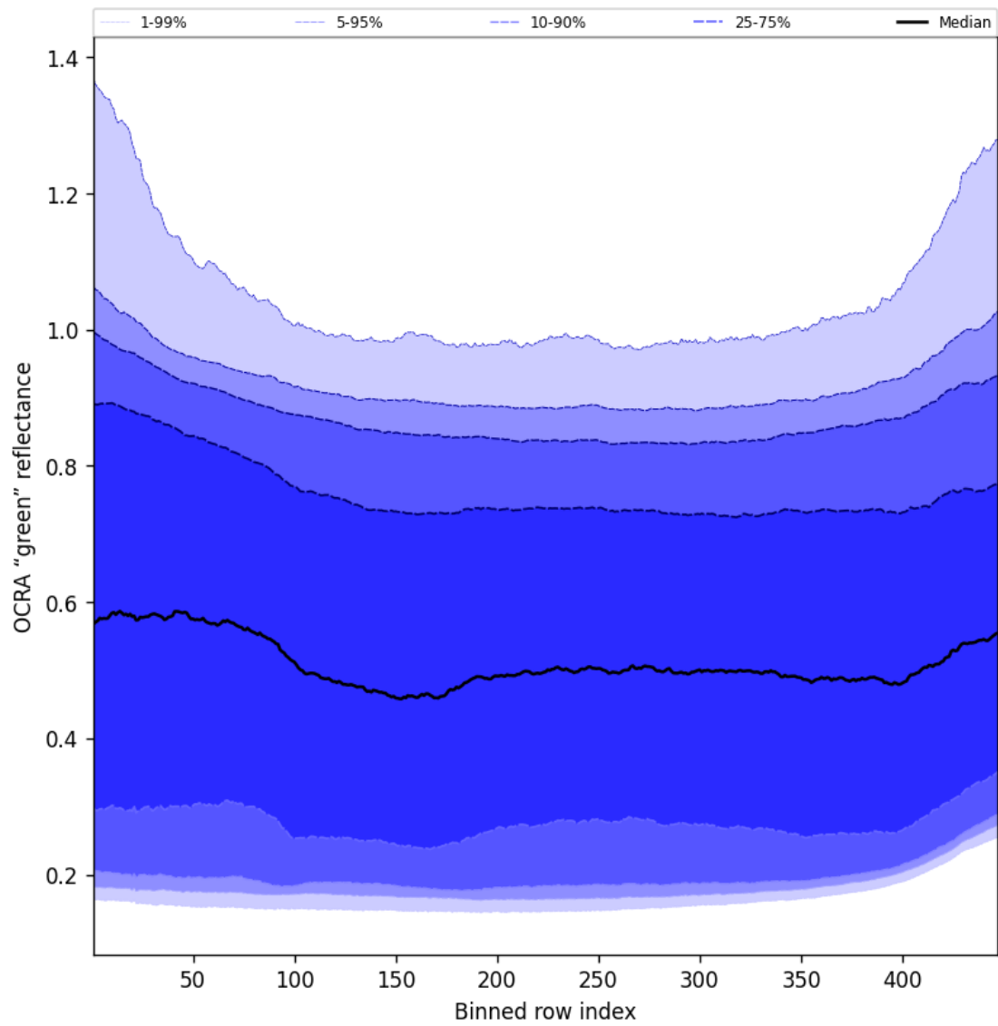
Figure 68: Along track statistics of "OCRA "green" reflectance" for 2024-10-26 to 2024-10-28
