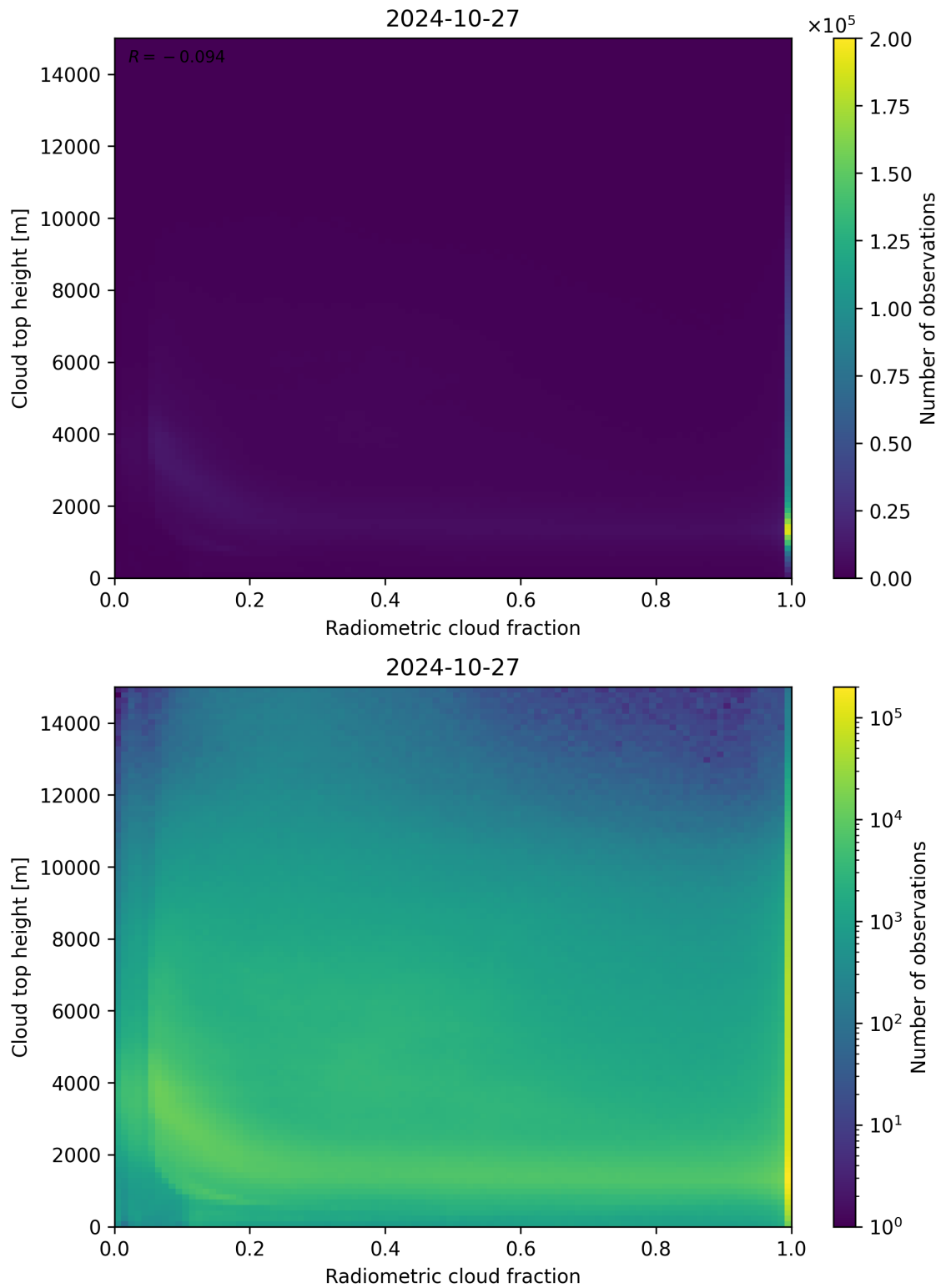
Figure 76: Scatter density plot of “Radiometric cloud fraction” against “Cloud top height” for 2024-10-26 to 2024-10-28.
