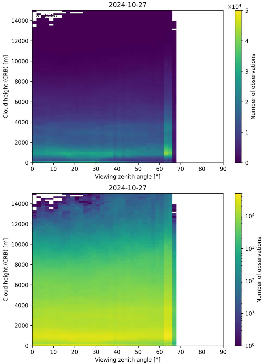
Figure 110: Scatter density plot of “Viewing zenith angle” against “Cloud height (CRB)” for 2024-10-26 to 2024-10-28.
