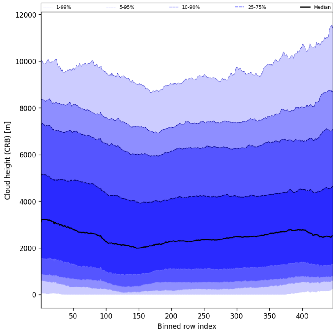
Figure 59: Along track statistics of “Cloud height (CRB)” for 2024-10-26 to 2024-10-28
