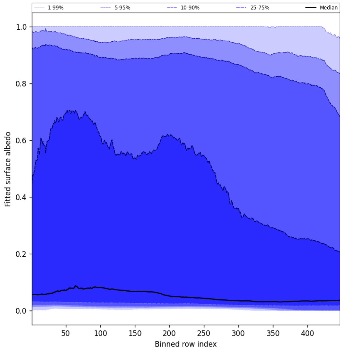
Figure 61: Along track statistics of “Fitted surface albedo” for 2024-10-27 to 2024-10-29
