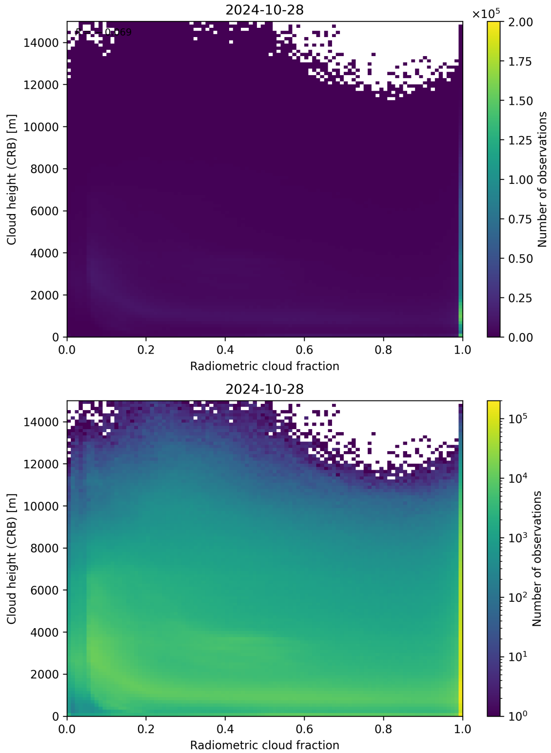
Figure 74: Scatter density plot of “Radiometric cloud fraction” against “Cloud height (CRB)” for 2024-10-27 to 2024-10-29.
