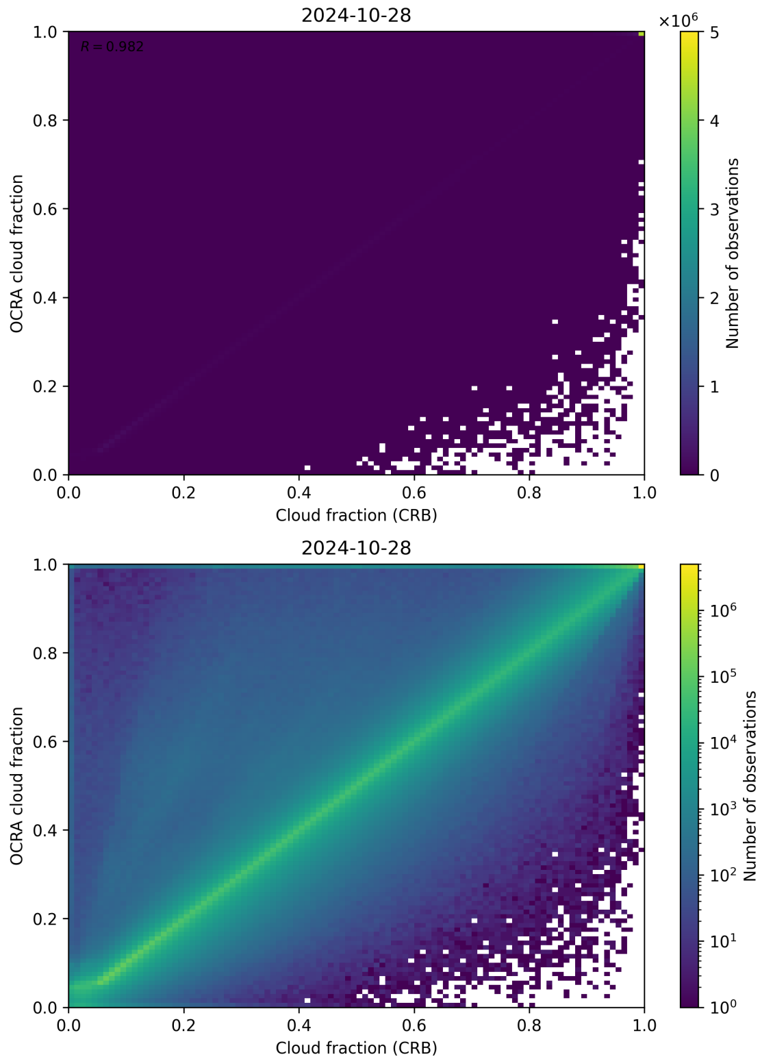
Figure 78: Scatter density plot of “Cloud fraction (CRB)” against “OCRA cloud fraction” for 2024-10-27 to 2024-10-29.
