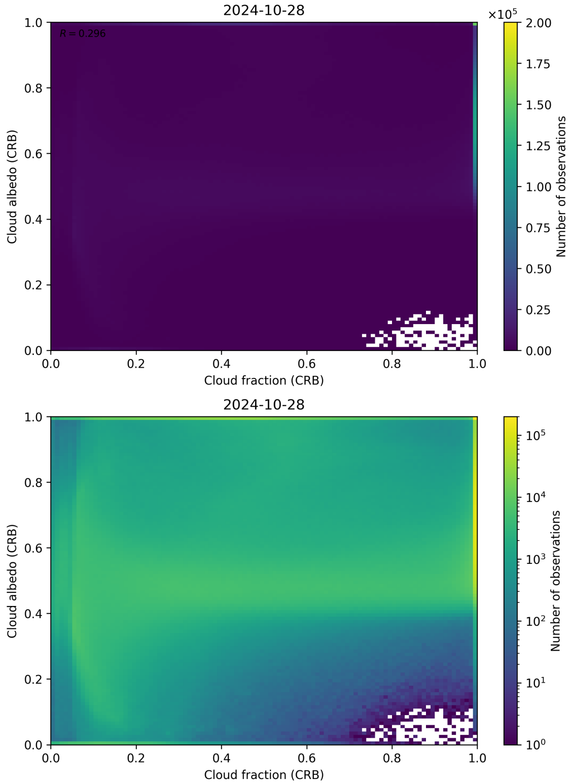
Figure 77: Scatter density plot of “Cloud fraction (CRB)” against “Cloud albedo (CRB)” for 2024-10-27 to 2024-10-29.
