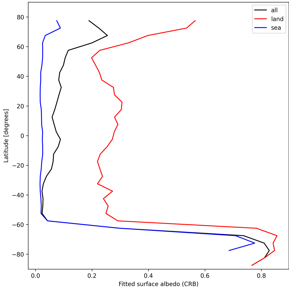
Figure 30: Zonal average of “Fitted surface albedo (CRB)” for 2024-10-27 to 2024-10-29.
