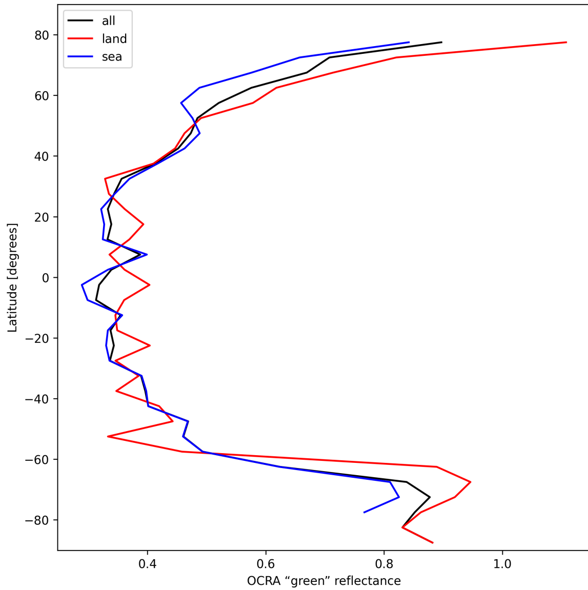
Figure 36: Zonal average of “OCRA “green” reflectance” for 2024-10-27 to 2024-10-29.
