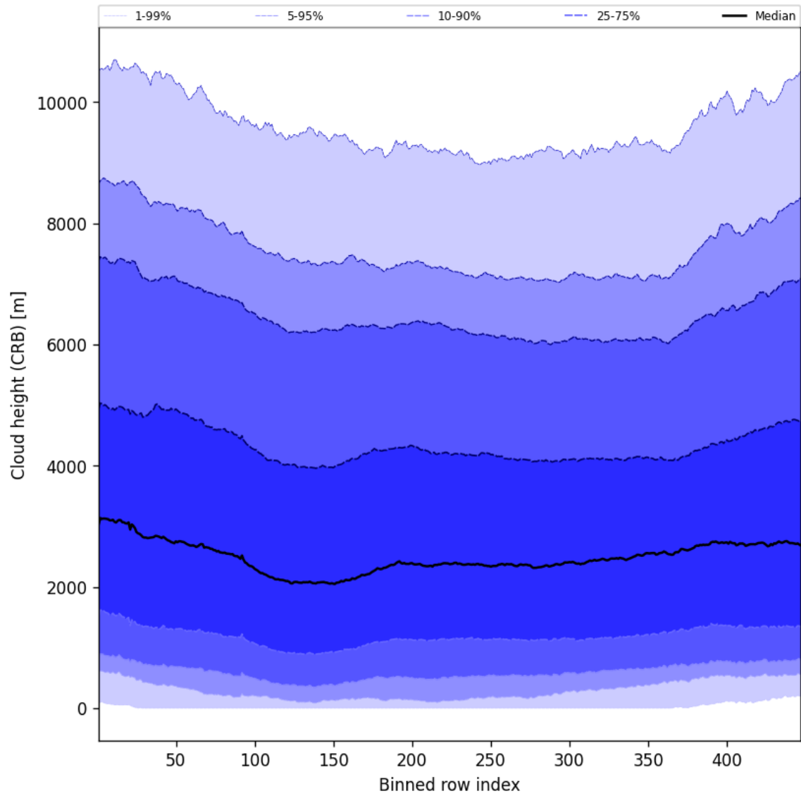
Figure 59: Along track statistics of “Cloud height (CRB)” for 2024-10-27 to 2024-10-29
