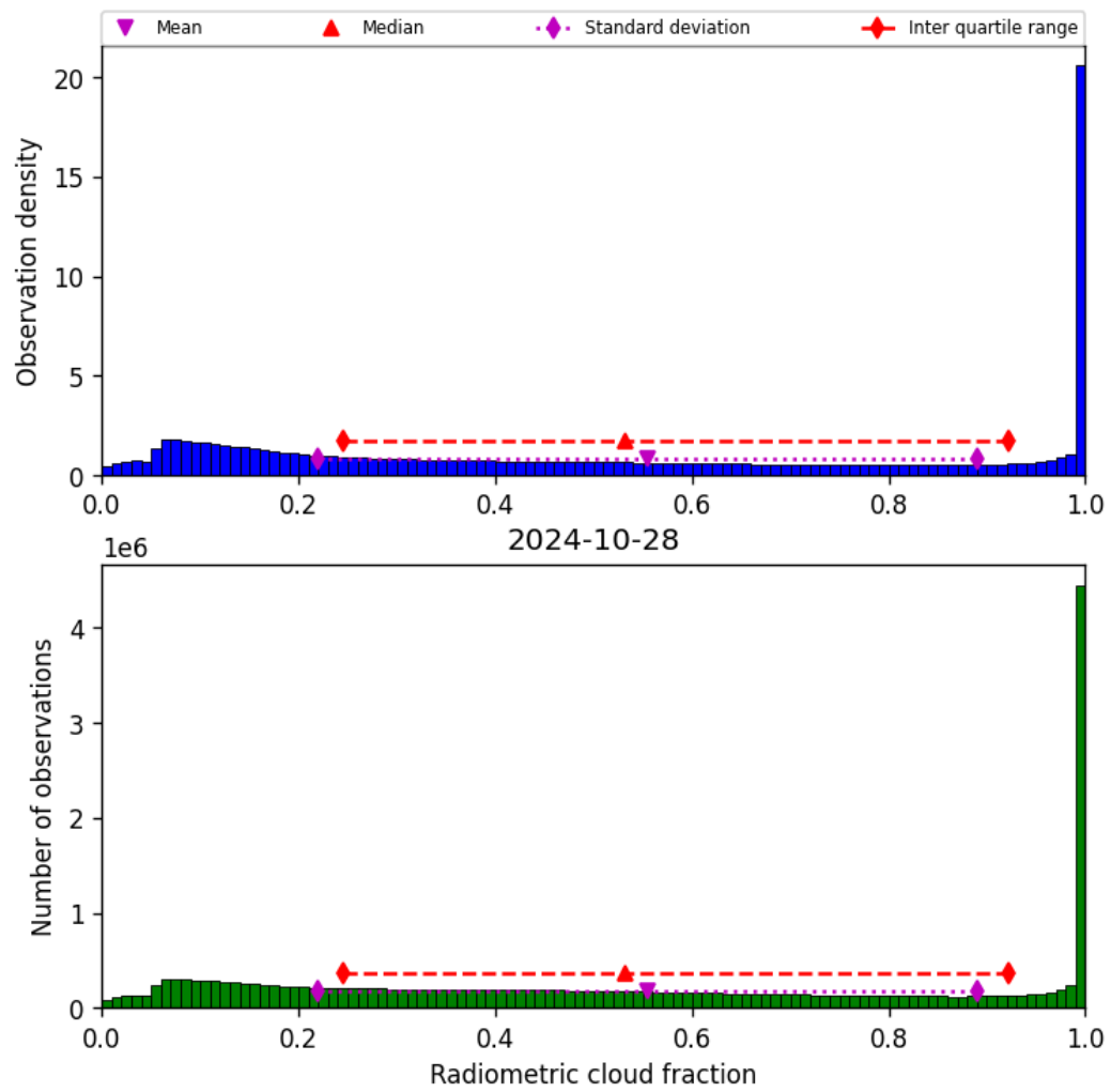
Figure 39: Histogram of “Radiometric cloud fraction” for 2024-10-27 to 2024-10-29
