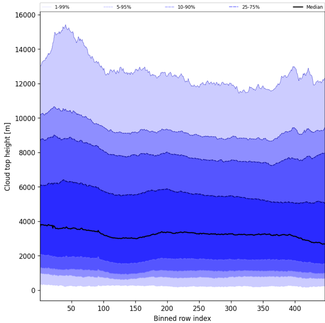
Figure 56: Along track statistics of “Cloud top height” for 2024-10-27 to 2024-10-29
