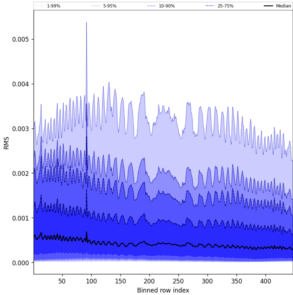
Figure 63: Along track statistics of “RMS” for 2024-10-27 to 2024-10-29
