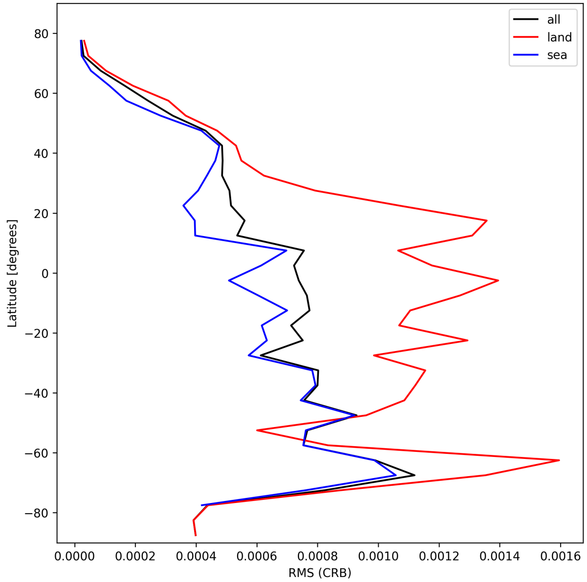
Figure 32: Zonal average of “RMS (CRB)” for 2024-10-27 to 2024-10-29.
