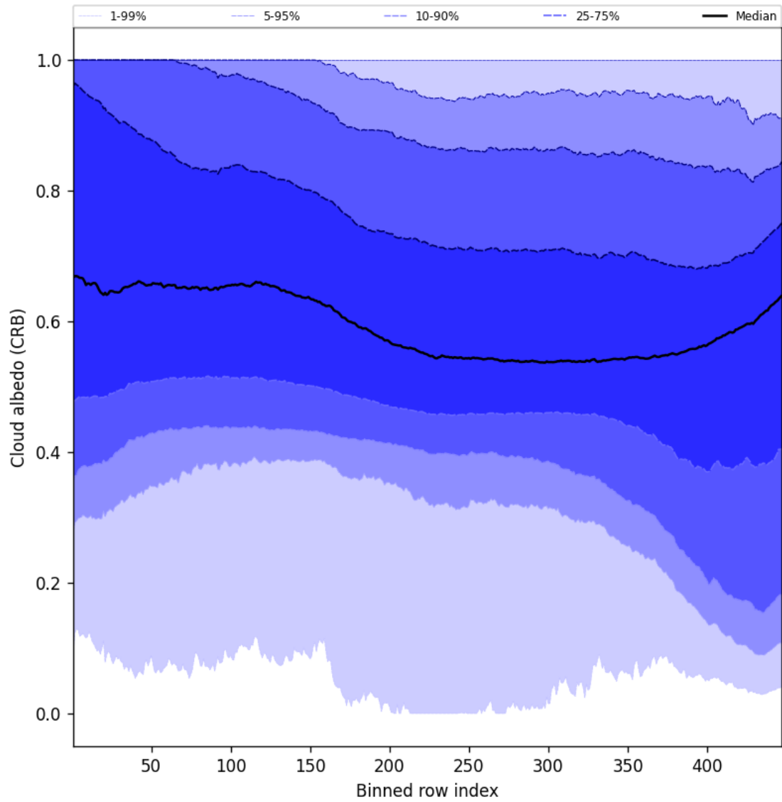
Figure 60: Along track statistics of “Cloud albedo (CRB)” for 2024-10-27 to 2024-10-29
