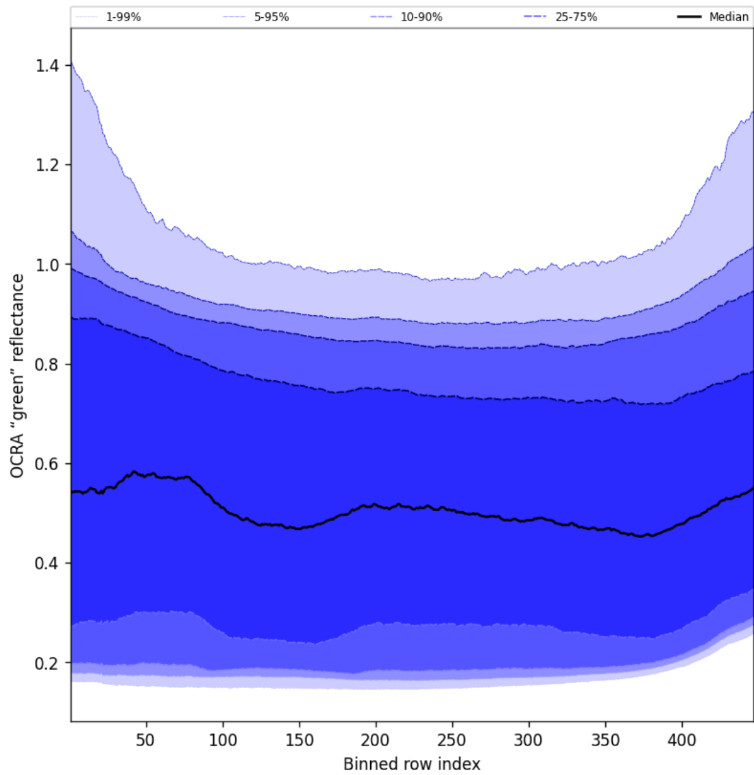
Figure 68: Along track statistics of "OCRA "green" reflectance" for 2024-10-27 to 2024-10-29
