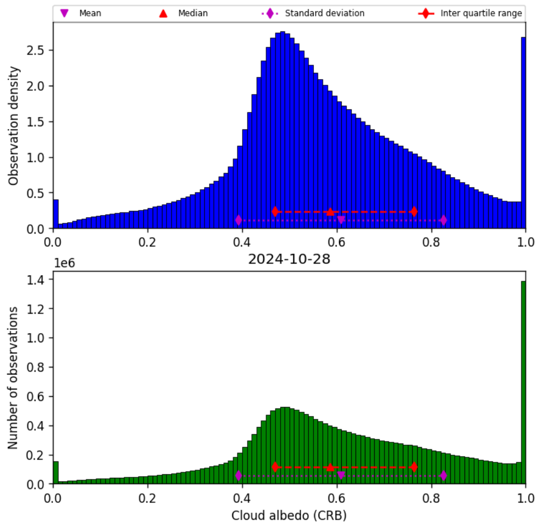
Figure 44: Histogram of “Cloud albedo (CRB)” for 2024-10-27 to 2024-10-29
