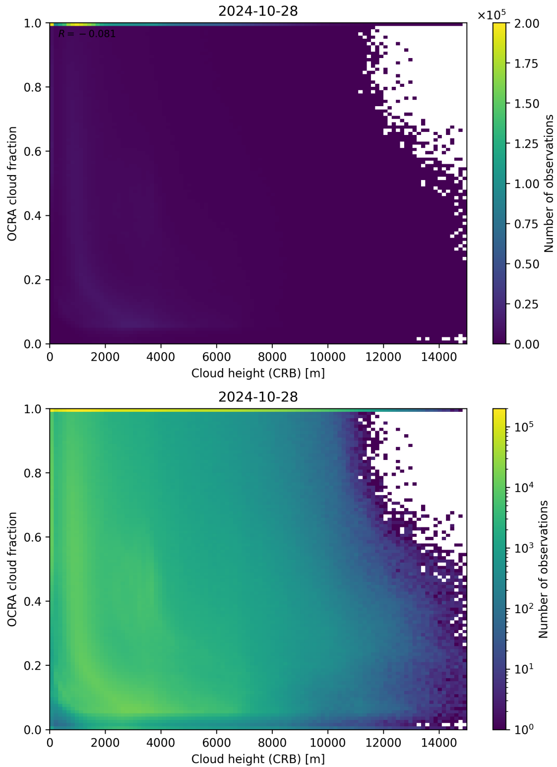
Figure 81: Scatter density plot of “Cloud height (CRB)” against “OCRA cloud fraction” for 2024-10-27 to 2024-10-29.
