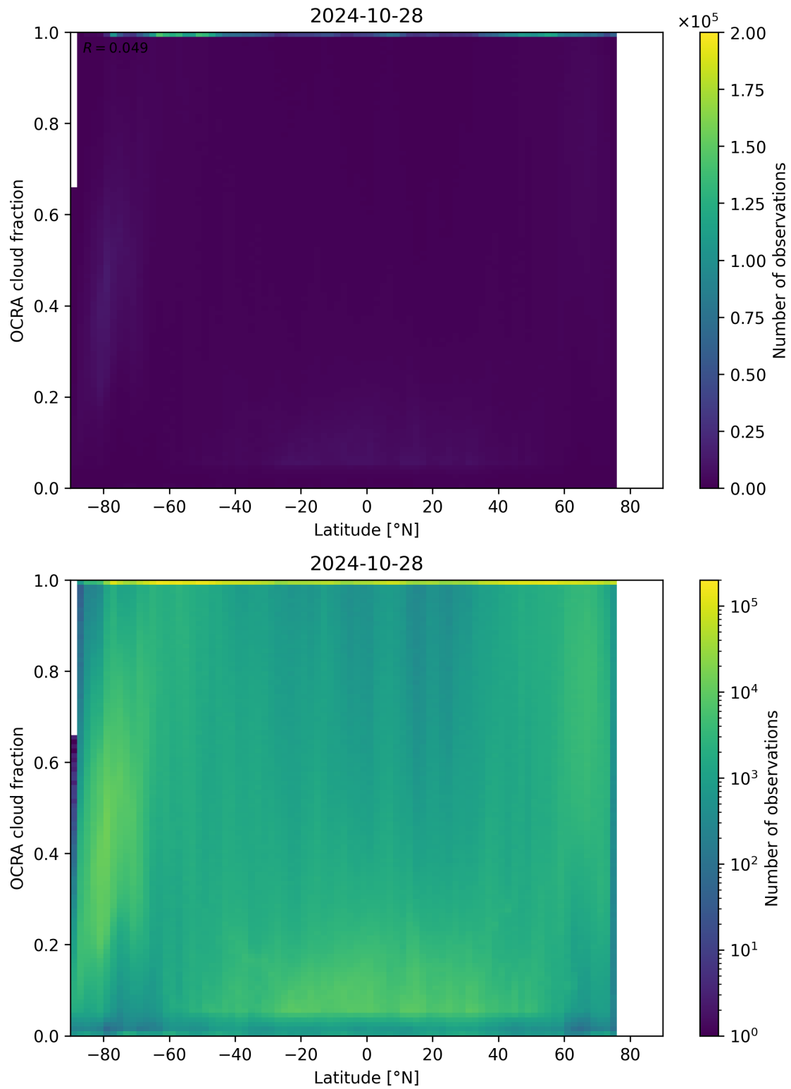
Figure 93: Scatter density plot of “Latitude” against “OCRA cloud fraction” for 2024-10-27 to 2024-10-29.
