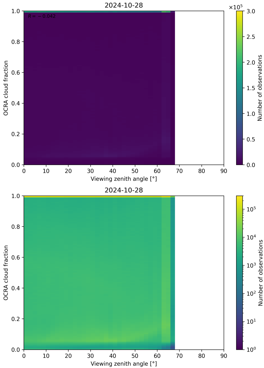
Figure 108: Scatter density plot of “Viewing zenith angle” against “OCRA cloud fraction” for 2024-10-27 to 2024-10-29.
