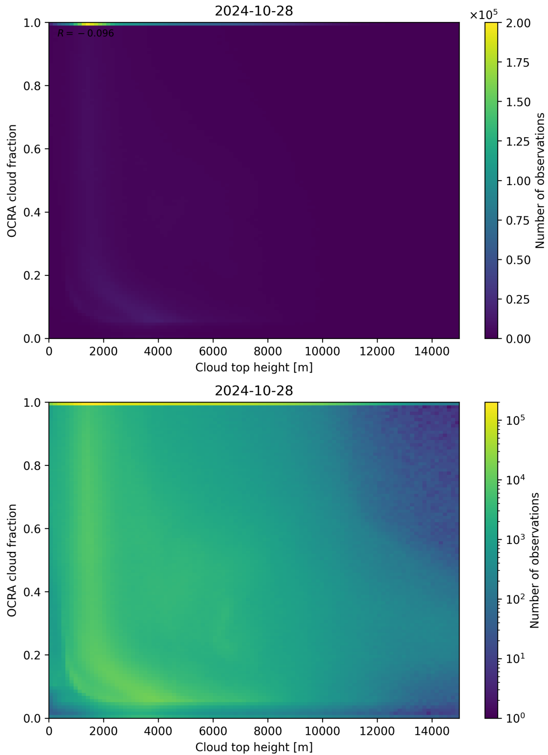
Figure 87: Scatter density plot of “Cloud top height” against “OCRA cloud fraction” for 2024-10-27 to 2024-10-29.
