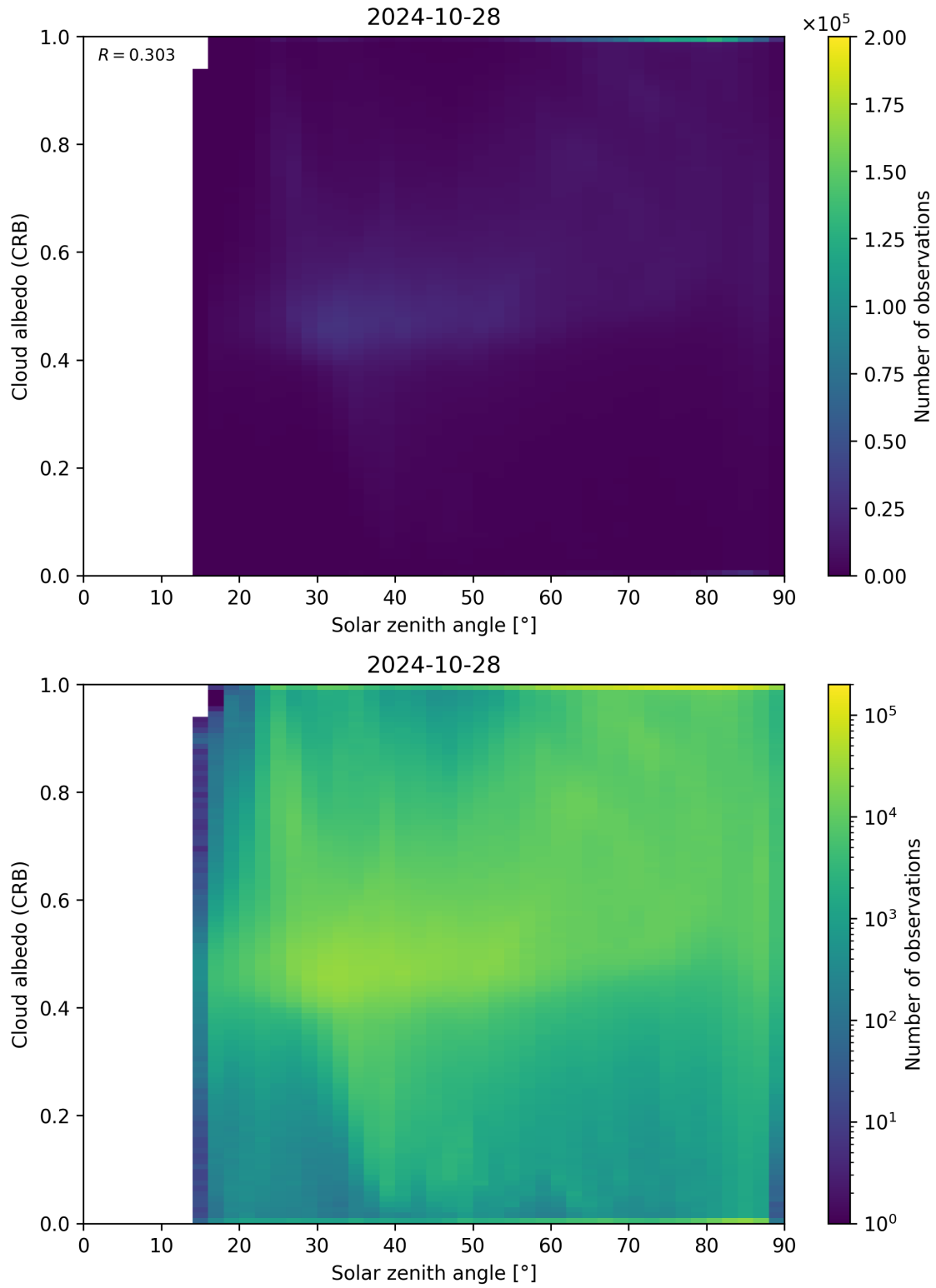
Figure 98: Scatter density plot of “Solar zenith angle” against “Cloud albedo (CRB)” for 2024-10-27 to 2024-10-29.
