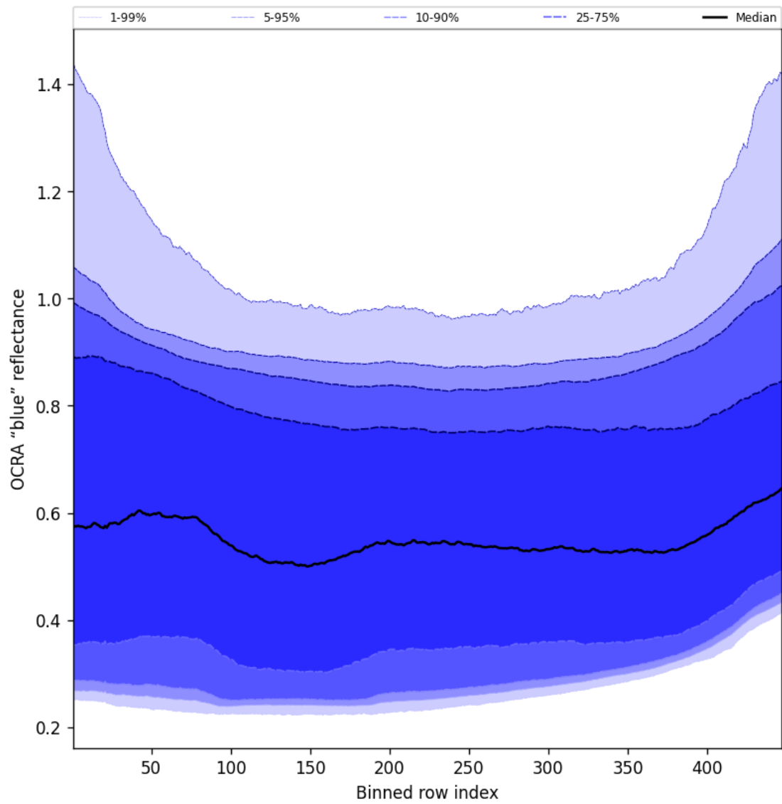
Figure 67: Along track statistics of “OCRA “blue” reflectance” for 2024-10-27 to 2024-10-29
