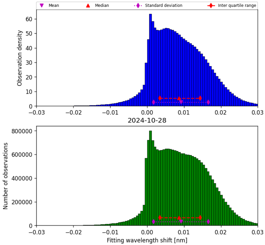
Figure 49: Histogram of “Fitting wavelength shift” for 2024-10-27 to 2024-10-29
