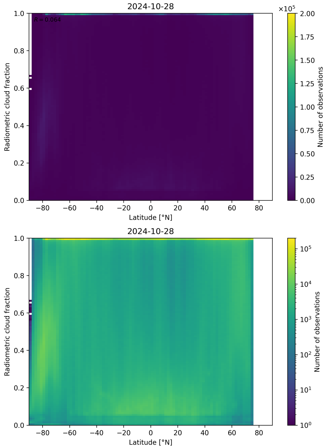
Figure 92: Scatter density plot of “Latitude” against “Radiometric cloud fraction” for 2024-10-27 to 2024-10-29.
