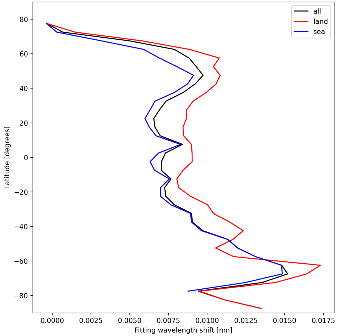
Figure 33: Zonal average of “Fitting wavelength shift” for 2024-10-27 to 2024-10-29.
