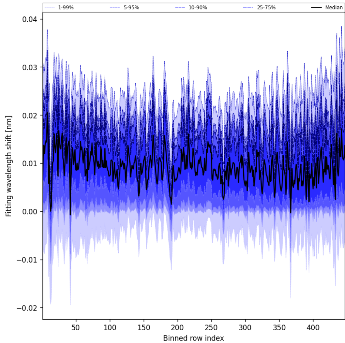
Figure 65: Along track statistics of “Fitting wavelength shift” for 2024-10-27 to 2024-10-29
