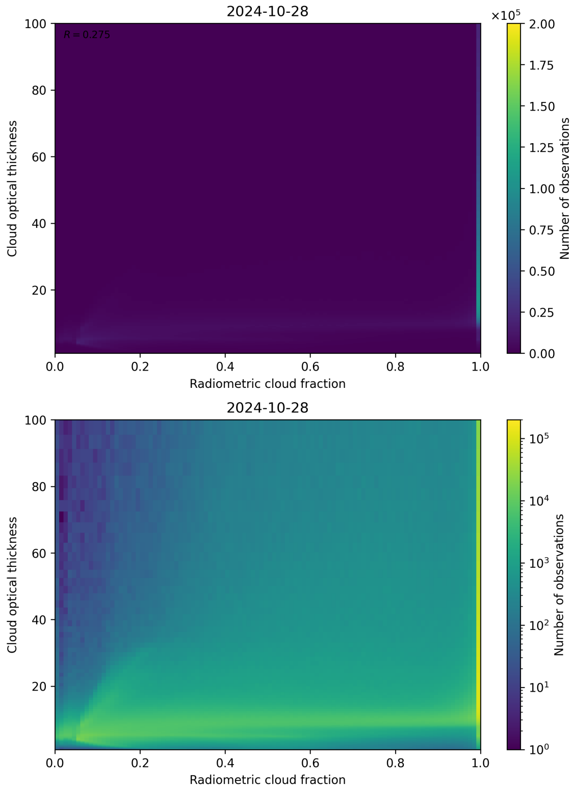
Figure 75: Scatter density plot of “Radiometric cloud fraction” against “Cloud optical thickness” for 2024-10-27 to 2024-10-29.
