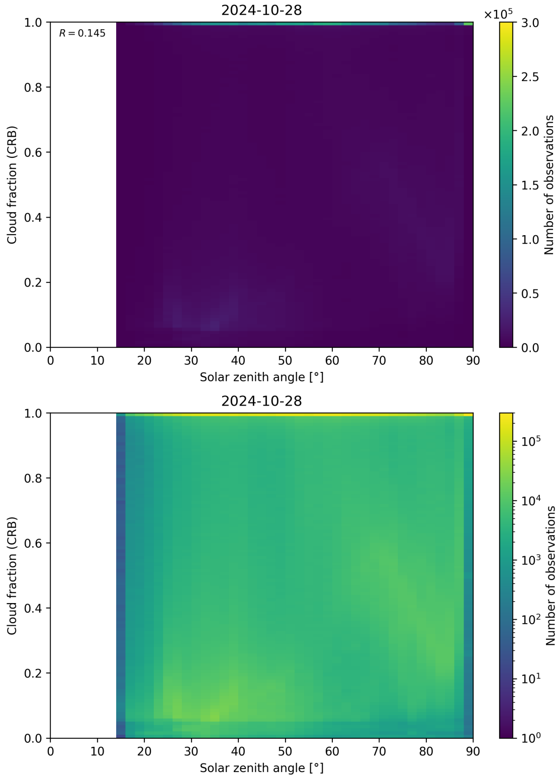
Figure 101: Scatter density plot of “Solar zenith angle” against “Cloud fraction (CRB)” for 2024-10-27 to 2024-10-29.
