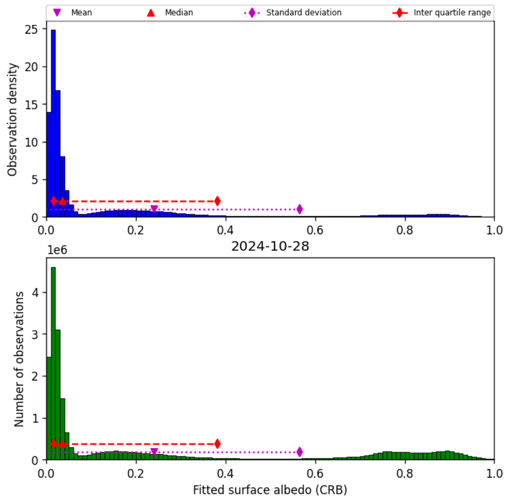
Figure 46: Histogram of “Fitted surface albedo (CRB)” for 2024-10-27 to 2024-10-29
