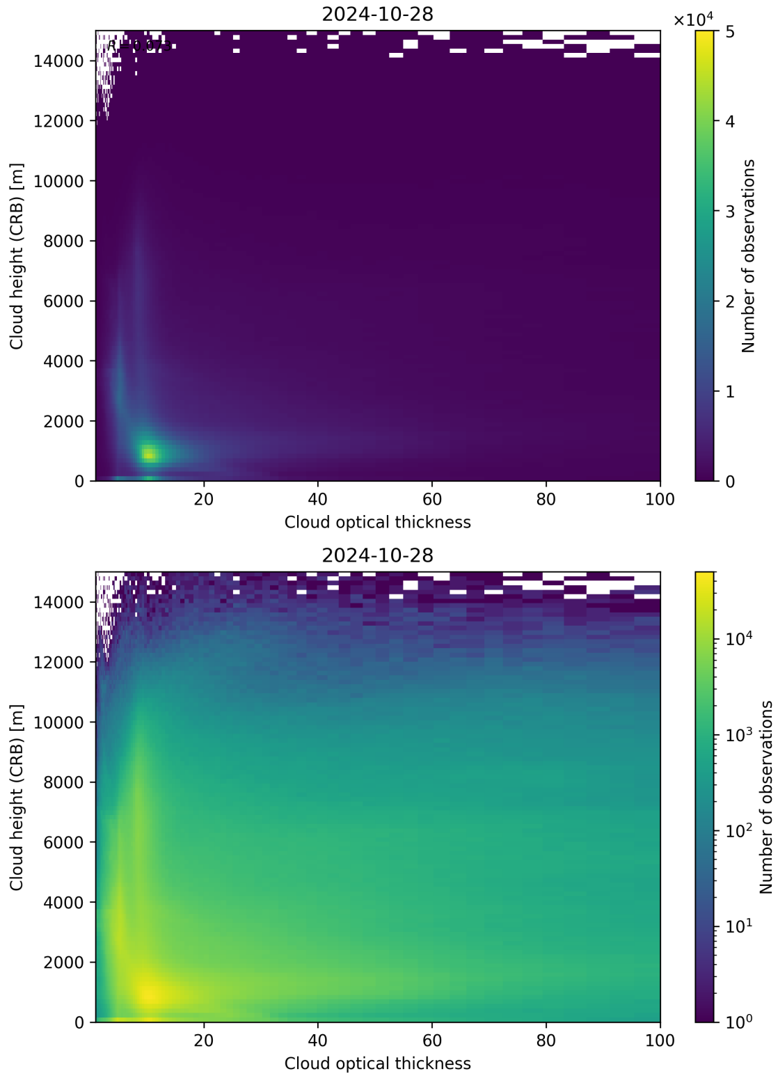
Figure 85: Scatter density plot of “Cloud optical thickness” against “Cloud height (CRB)” for 2024-10-27 to 2024-10-29.
