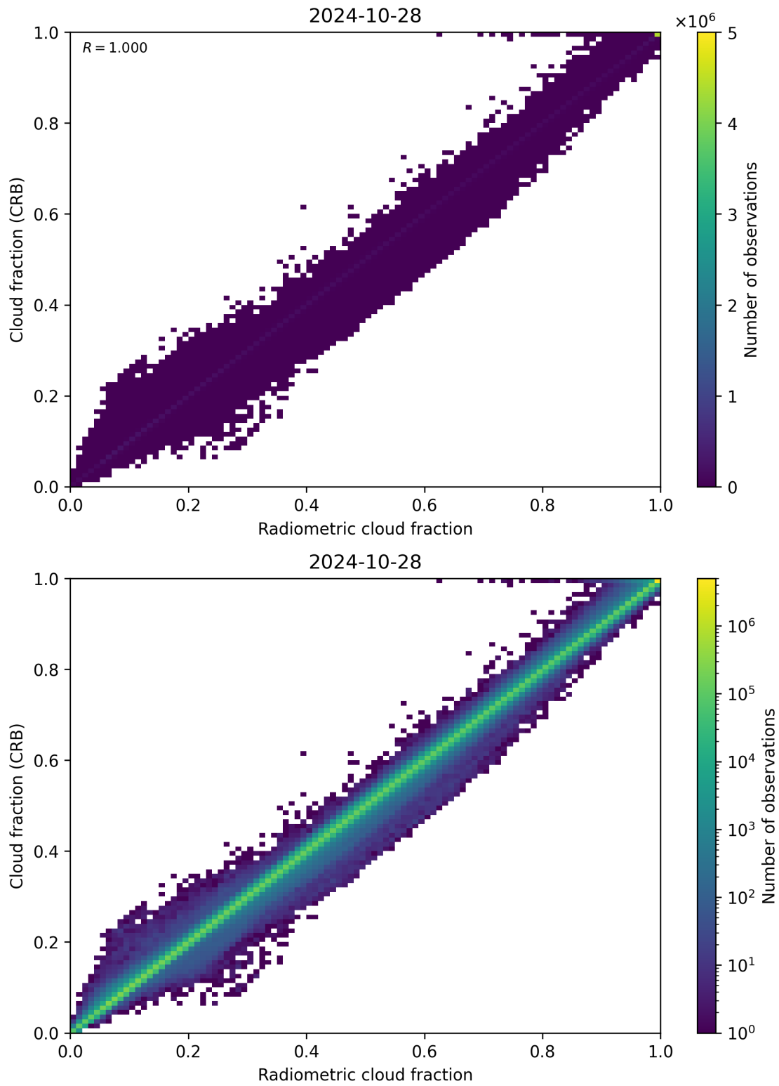
Figure 73: Scatter density plot of “Radiometric cloud fraction” against “Cloud fraction (CRB)” for 2024-10-27 to 2024-10-29.
