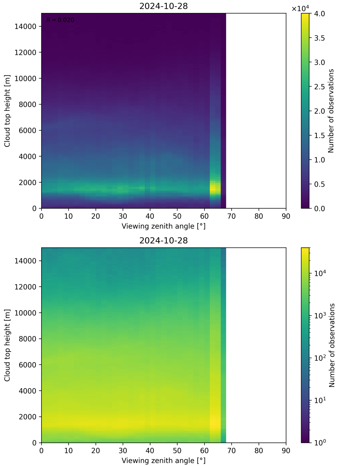
Figure 112: Scatter density plot of “Viewing zenith angle” against “Cloud top height” for 2024-10-27 to 2024-10-29.
