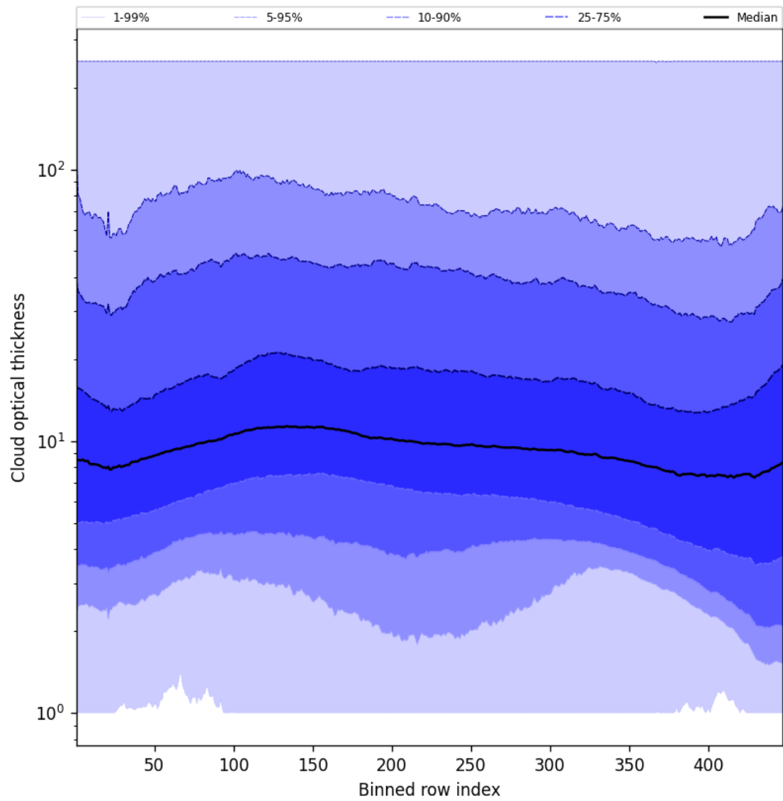
Figure 57: Along track statistics of “Cloud optical thickness” for 2024-10-27 to 2024-10-29
