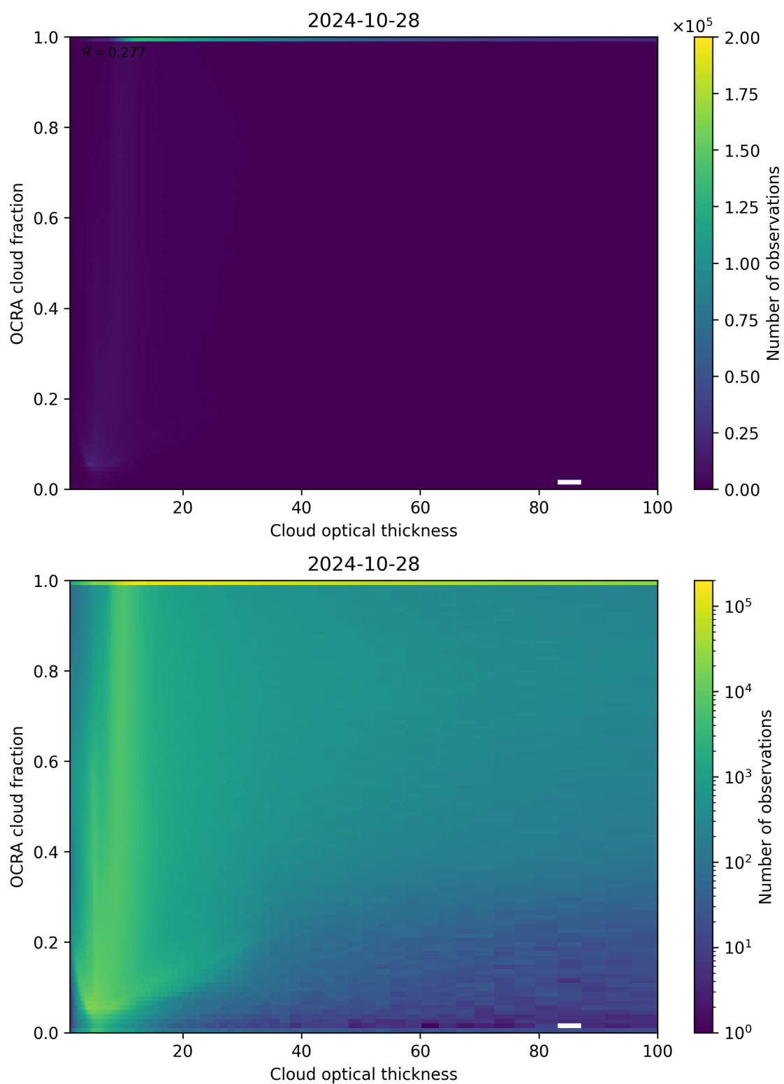
Figure 83: Scatter density plot of “Cloud optical thickness” against “OCRA cloud fraction” for 2024-10-27 to 2024-10-29.
