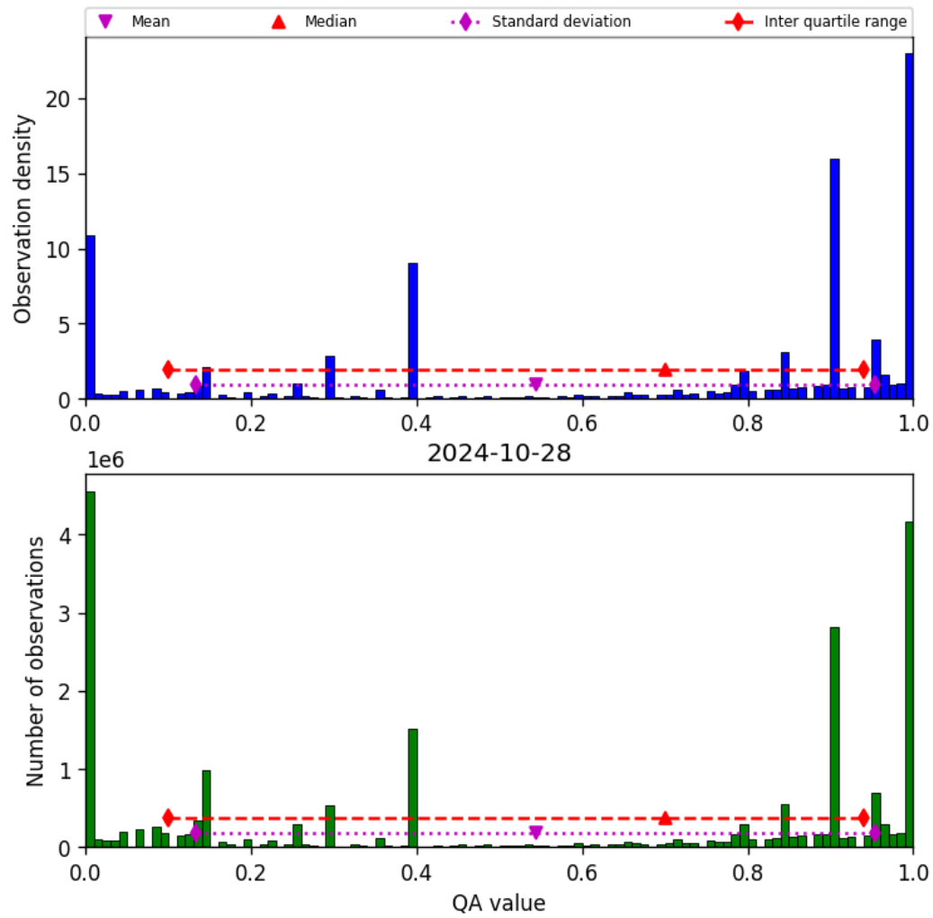
Figure 38: Histogram of “QA value” for 2024-10-27 to 2024-10-29
