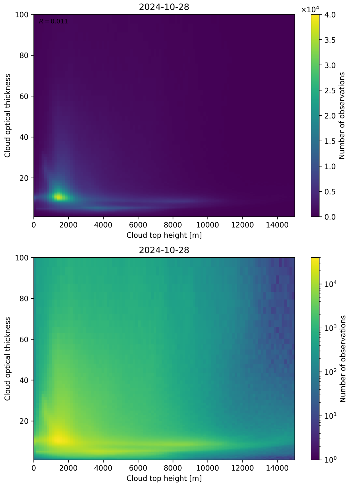
Figure 90: Scatter density plot of “Cloud top height” against “Cloud optical thickness” for 2024-10-27 to 2024-10-29.
