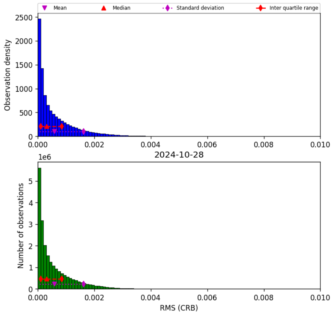
Figure 48: Histogram of “RMS (CRB)” for 2024-10-27 to 2024-10-29
