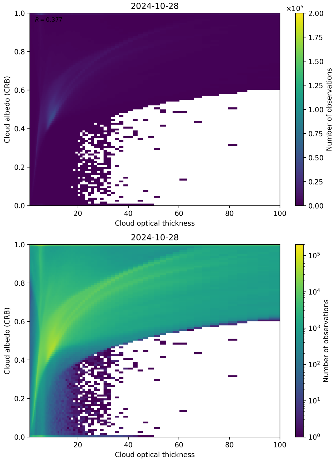
Figure 82: Scatter density plot of “Cloud optical thickness” against “Cloud albedo (CRB)” for 2024-10-27 to 2024-10-29.
