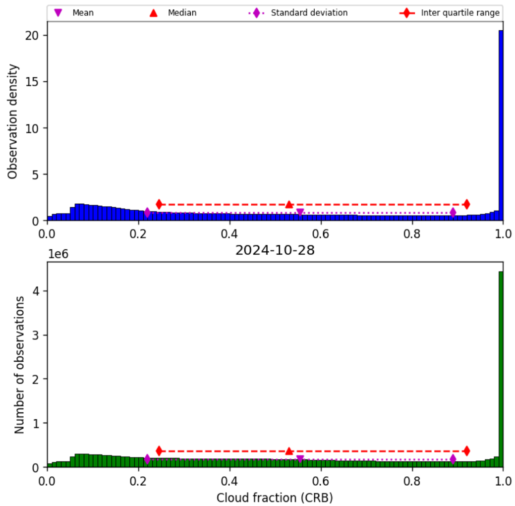
Figure 42: Histogram of “Cloud fraction (CRB)” for 2024-10-27 to 2024-10-29
