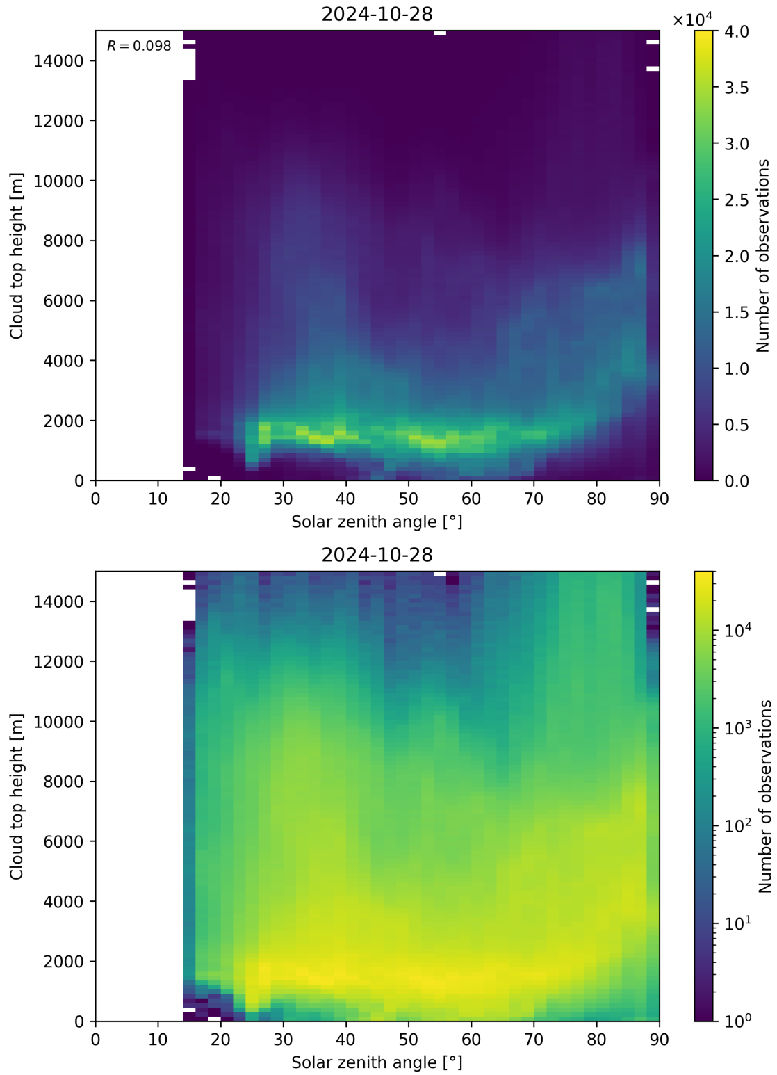
Figure 104: Scatter density plot of “Solar zenith angle” against “Cloud top height” for 2024-10-27 to 2024-10-29.
