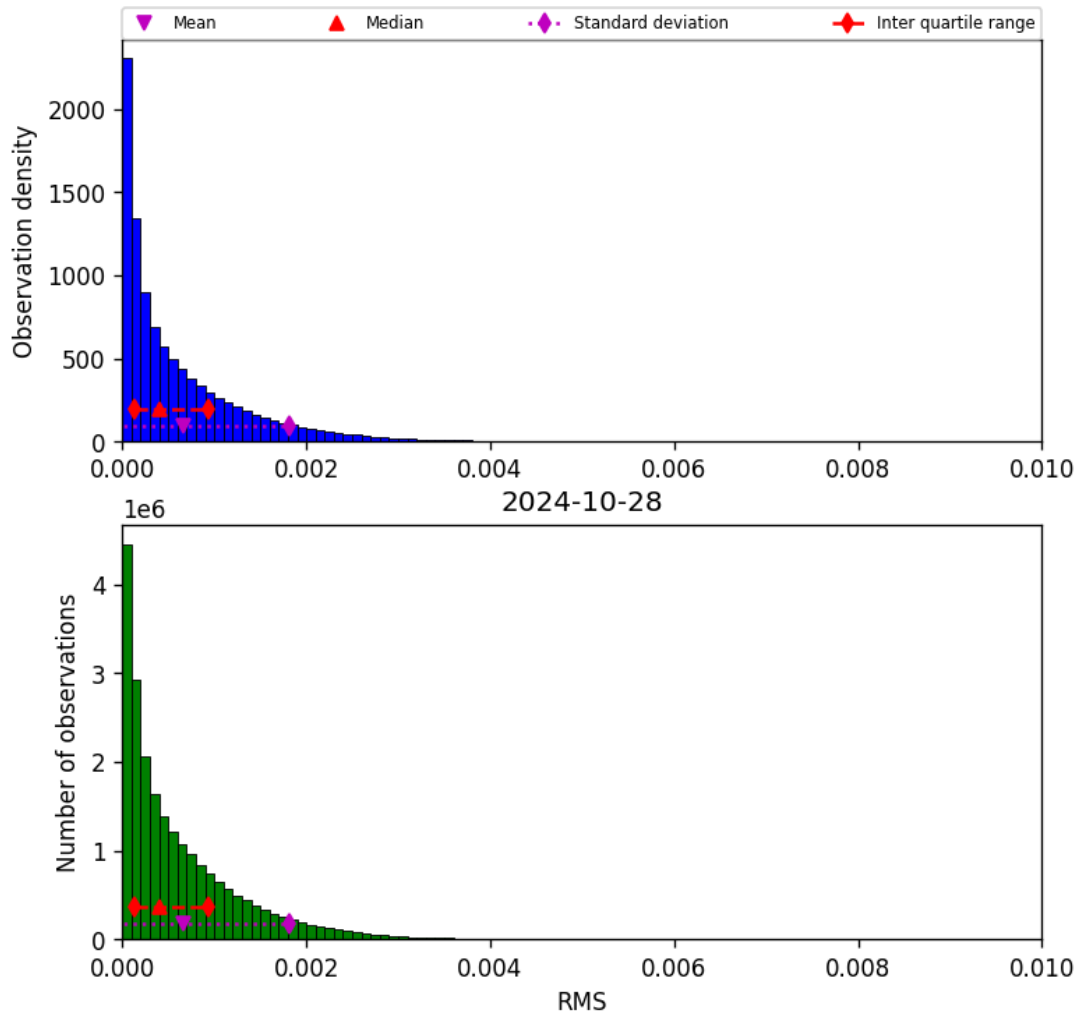
Figure 47: Histogram of “RMS” for 2024-10-27 to 2024-10-29
