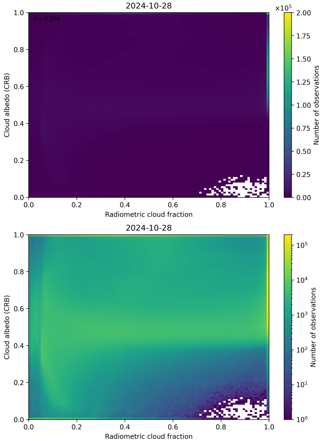
Figure 71: Scatter density plot of “Radiometric cloud fraction” against “Cloud albedo (CRB)” for 2024-10-27 to 2024-10-29.
