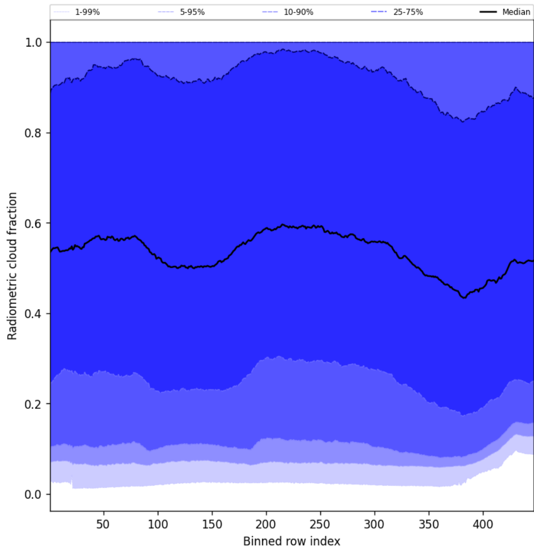
Figure 55: Along track statistics of “Radiometric cloud fraction” for 2024-10-27 to 2024-10-29
