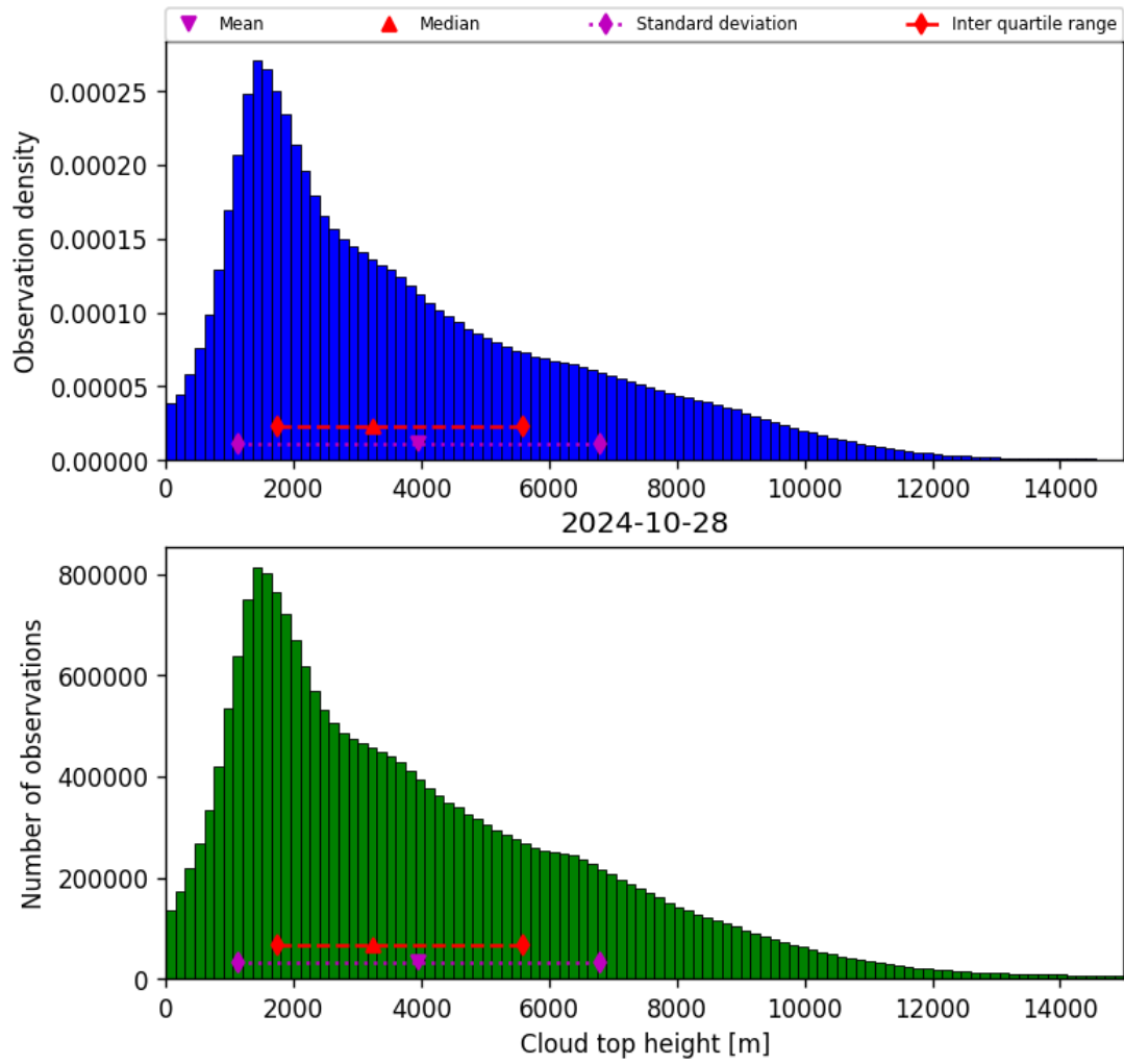
Figure 40: Histogram of “Cloud top height” for 2024-10-27 to 2024-10-29
