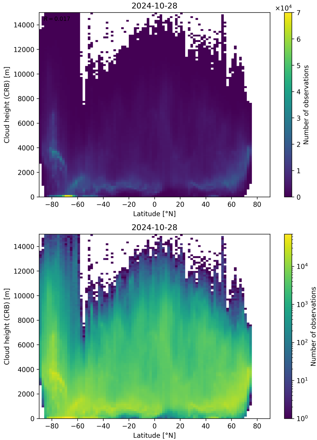
Figure 95: Scatter density plot of “Latitude” against “Cloud height (CRB)” for 2024-10-27 to 2024-10-29.
