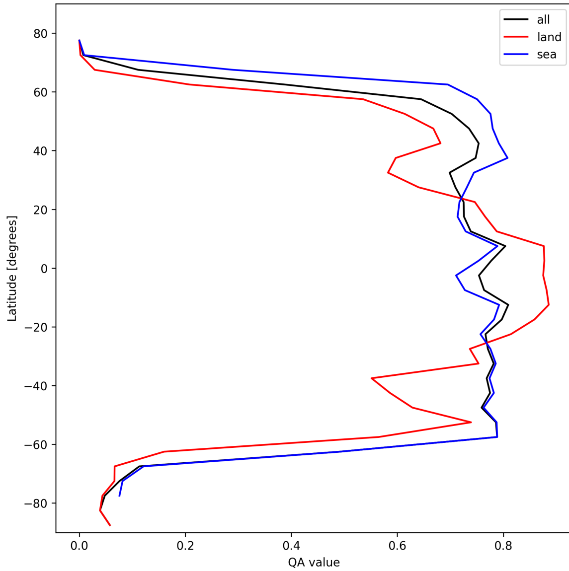
Figure 22: Zonal average of “QA value” for 2024-10-27 to 2024-10-29.
