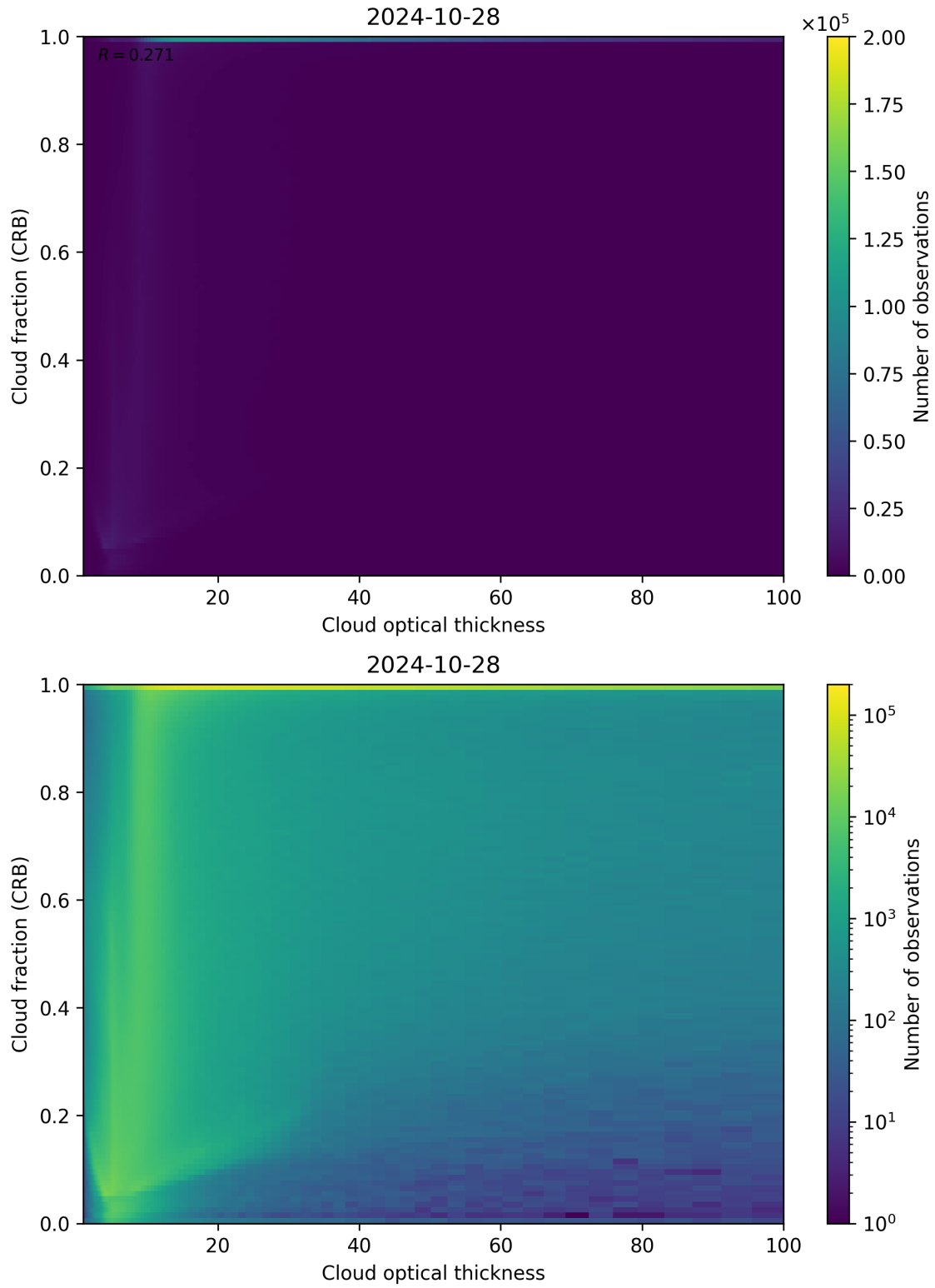
Figure 84: Scatter density plot of “Cloud optical thickness” against “Cloud fraction (CRB)” for 2024-10-27 to 2024-10-29.
