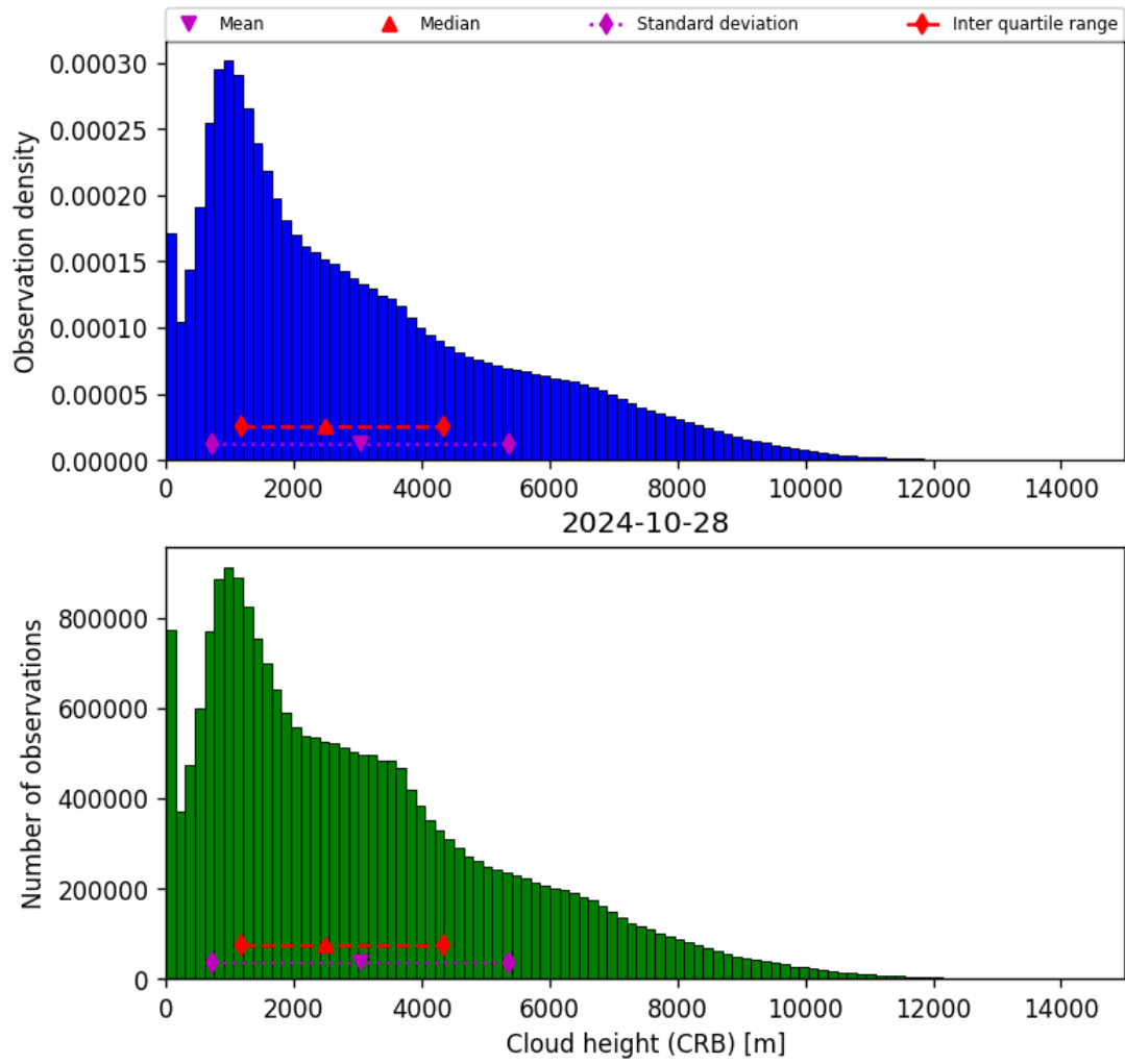
Figure 43: Histogram of “Cloud height (CRB)” for 2024-10-27 to 2024-10-29
