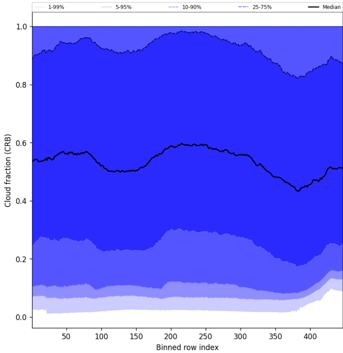
Figure 58: Along track statistics of “Cloud fraction (CRB)” for 2024-10-27 to 2024-10-29
