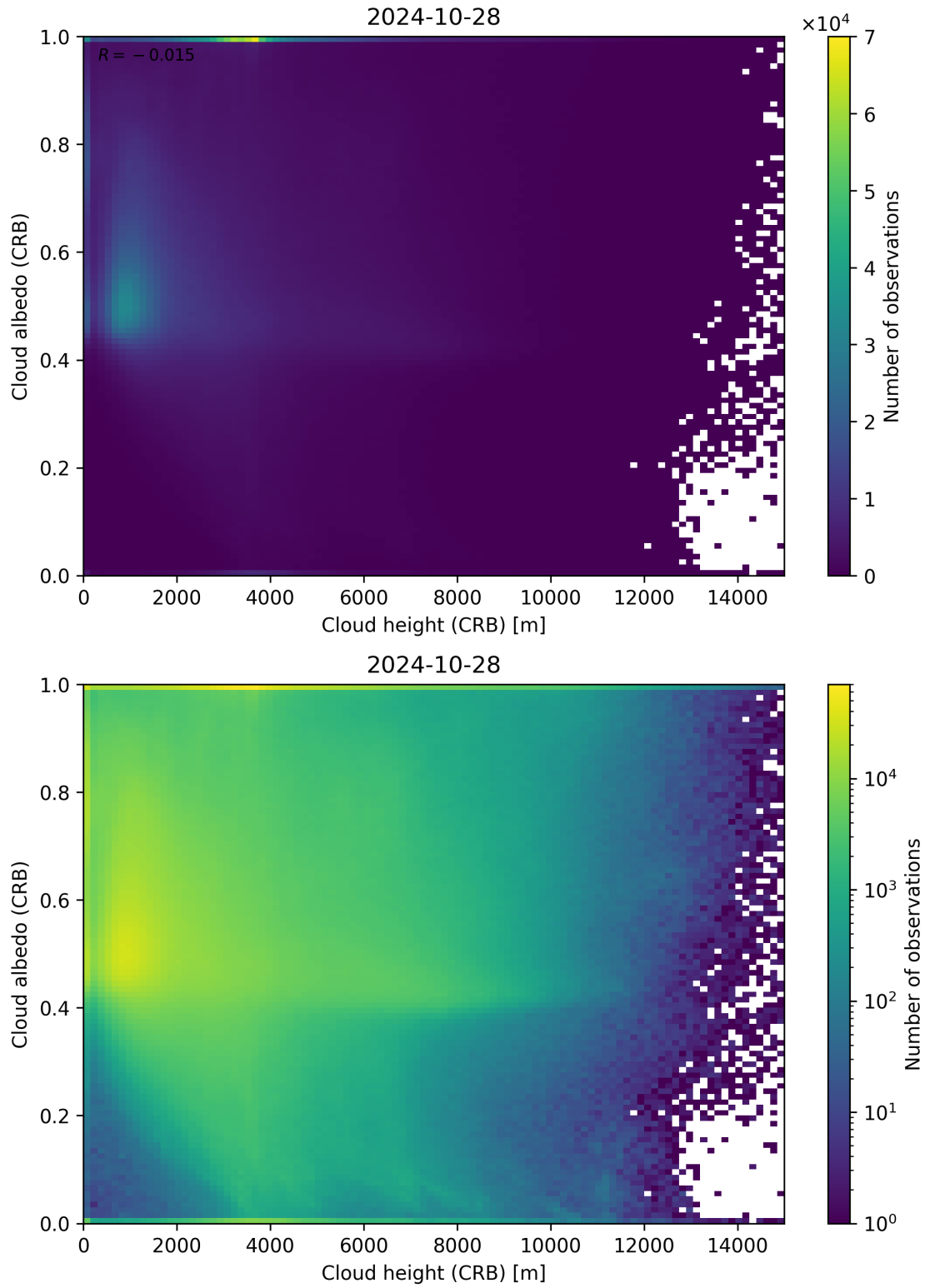
Figure 80: Scatter density plot of “Cloud height (CRB)” against “Cloud albedo (CRB)” for 2024-10-27 to 2024-10-29.
