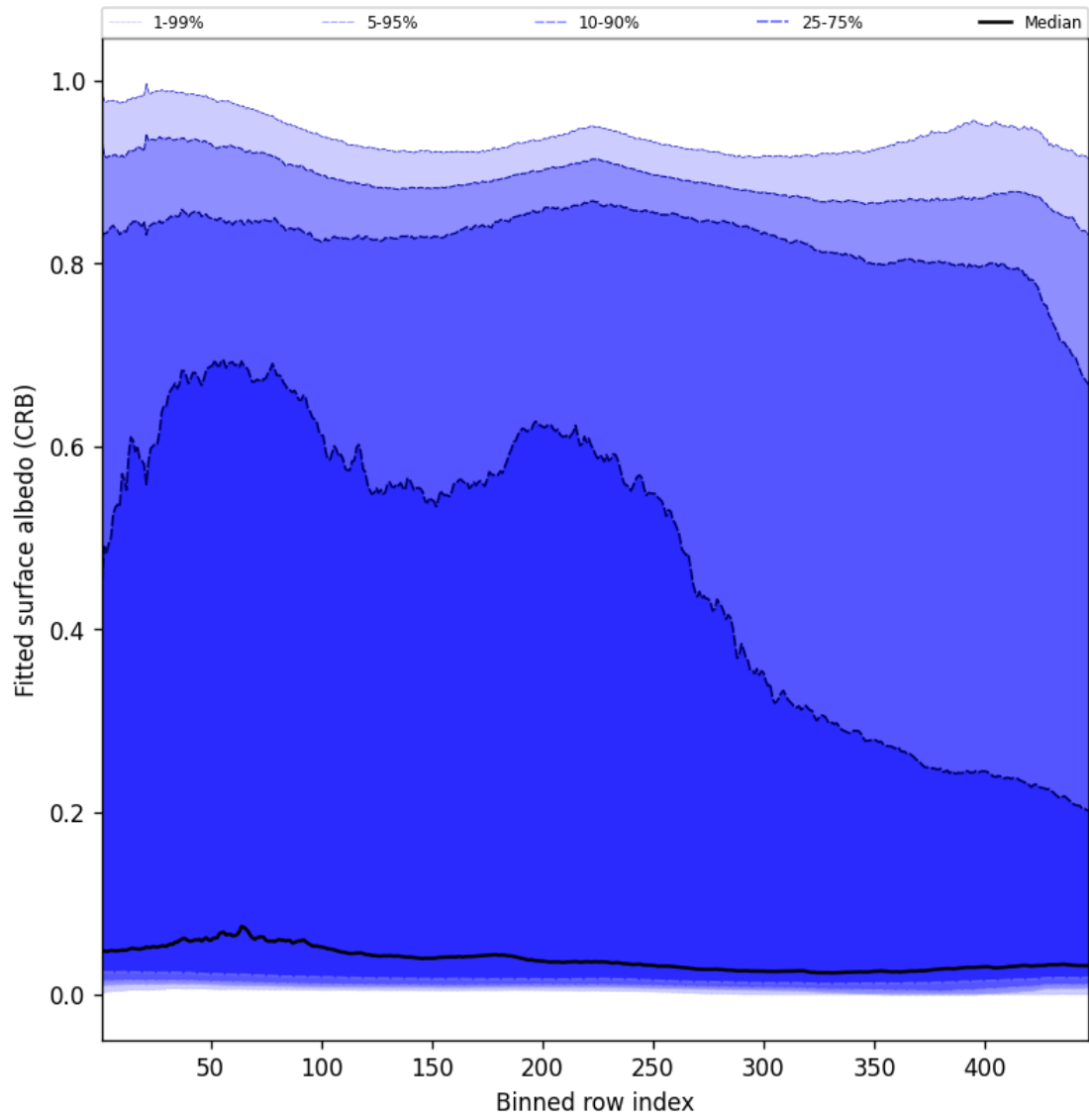
Figure 62: Along track statistics of “Fitted surface albedo (CRB)” for 2024-10-27 to 2024-10-29
