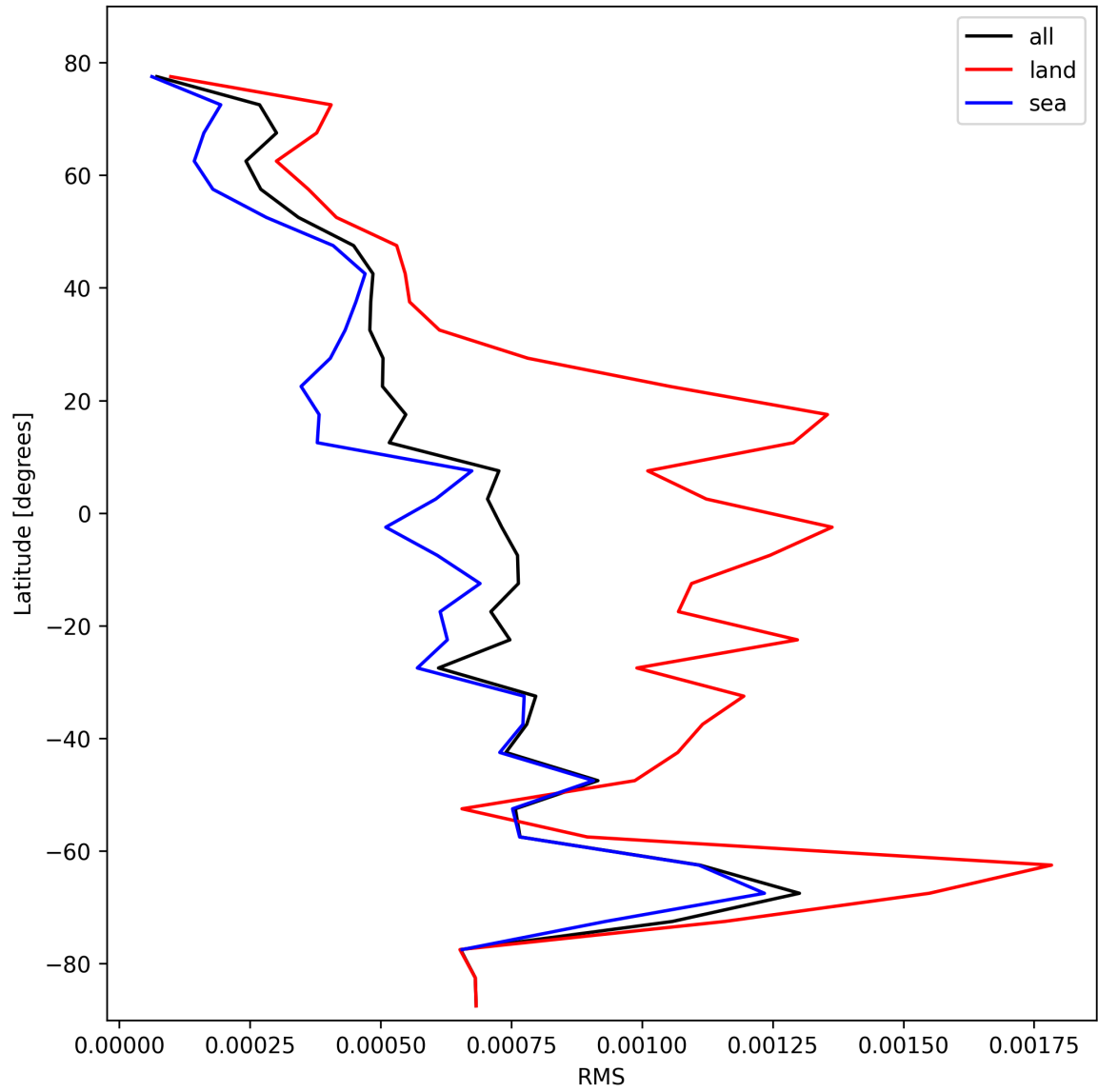
Figure 31: Zonal average of “RMS” for 2024-10-27 to 2024-10-29.
