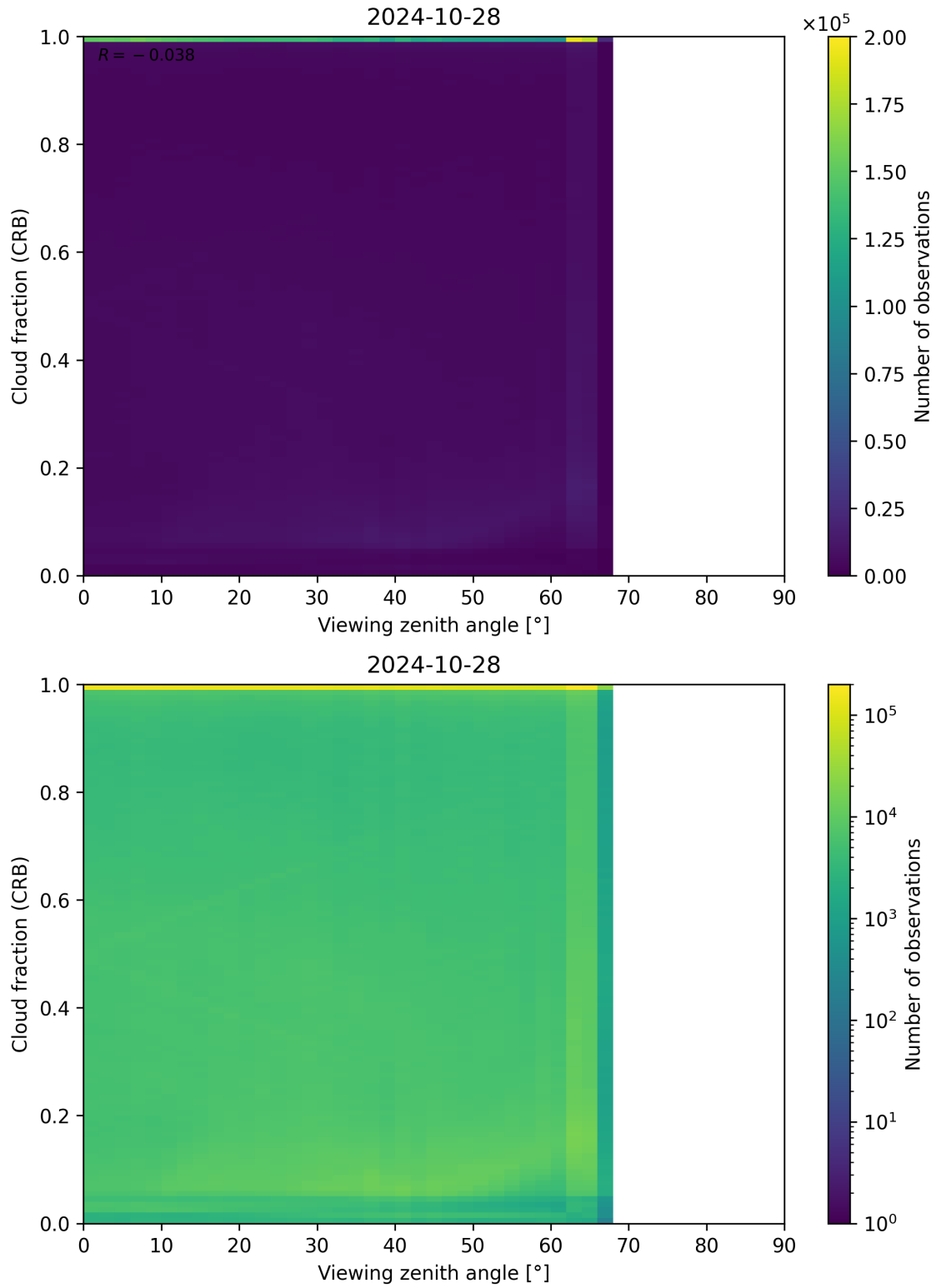
Figure 109: Scatter density plot of “Viewing zenith angle” against “Cloud fraction (CRB)” for 2024-10-27 to 2024-10-29.
