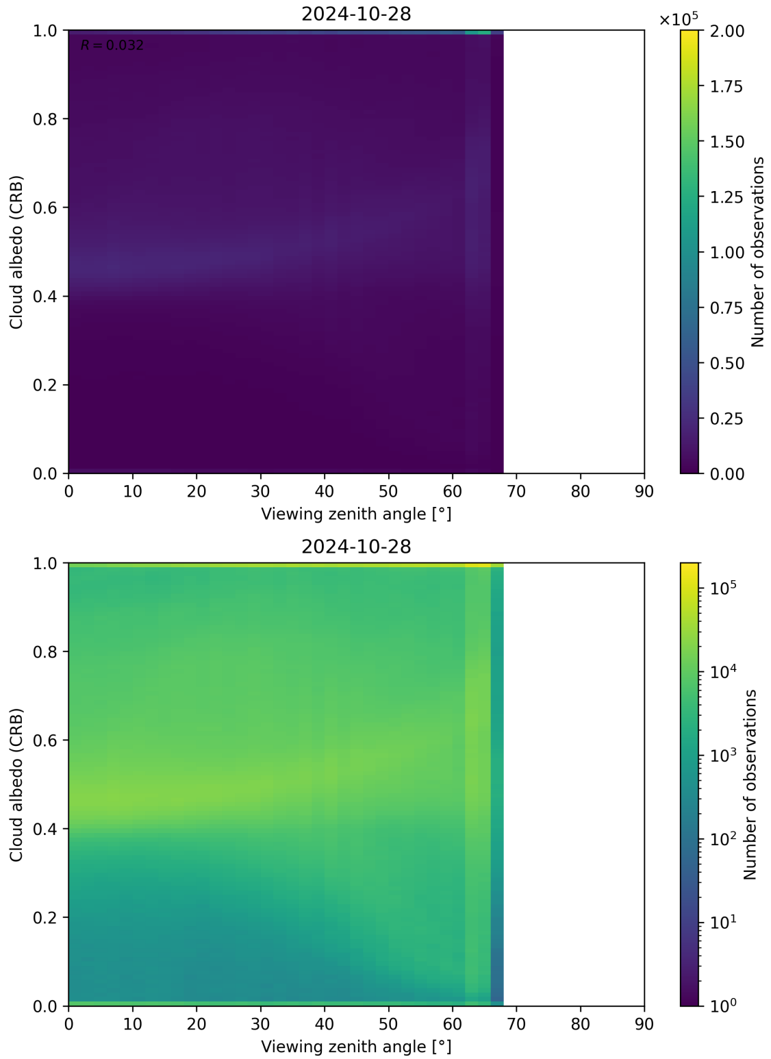
Figure 106: Scatter density plot of “Viewing zenith angle” against “Cloud albedo (CRB)” for 2024-10-27 to 2024-10-29.
