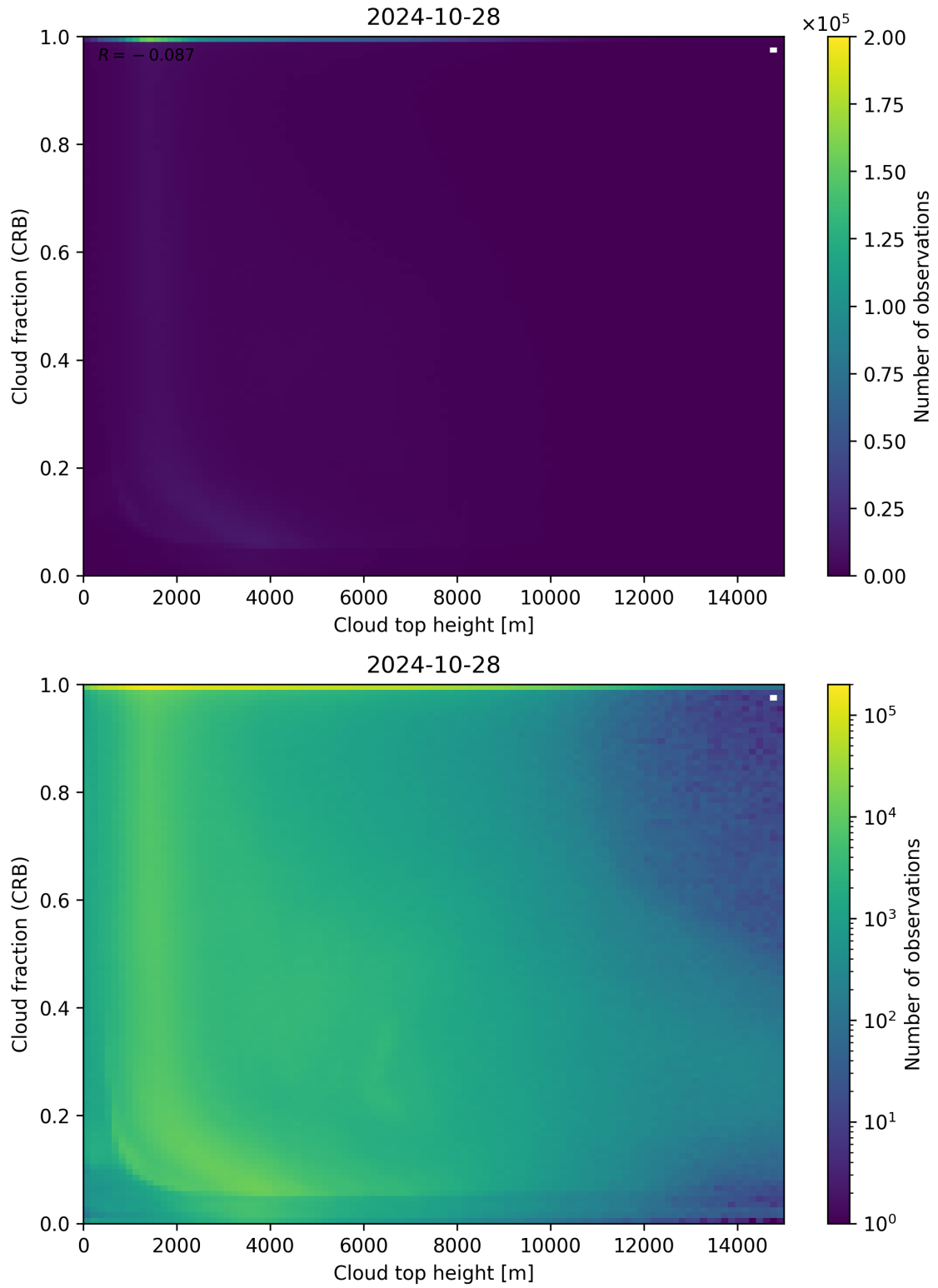
Figure 88: Scatter density plot of “Cloud top height” against “Cloud fraction (CRB)” for 2024-10-27 to 2024-10-29.
