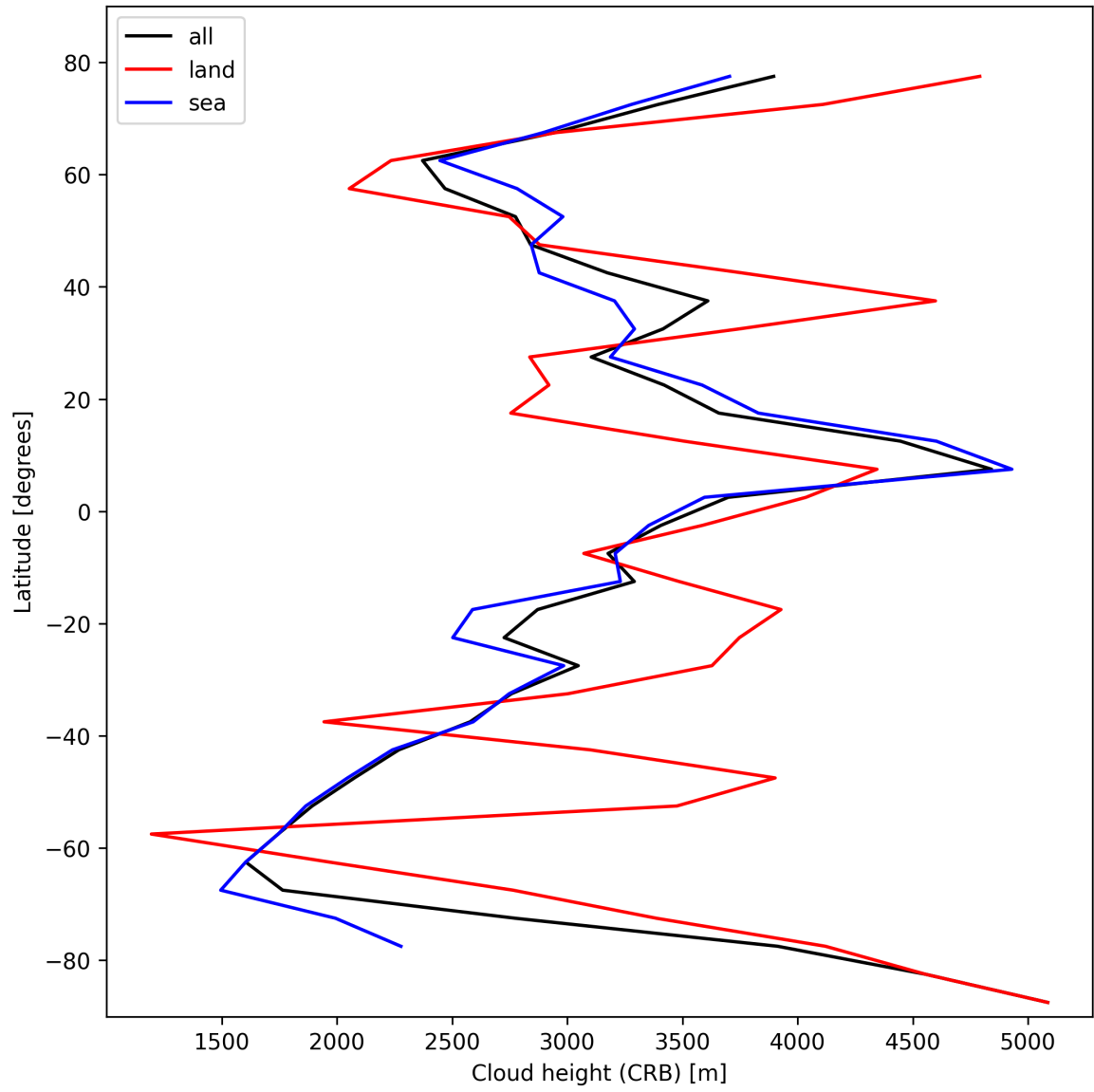
Figure 27: Zonal average of “Cloud height (CRB)” for 2024-10-27 to 2024-10-29.
