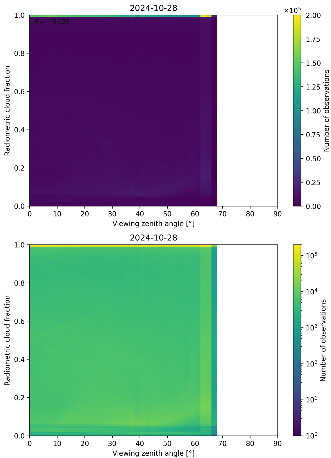
Figure 107: Scatter density plot of “Viewing zenith angle” against “Radiometric cloud fraction” for 2024-10-27 to 2024-10-29.
