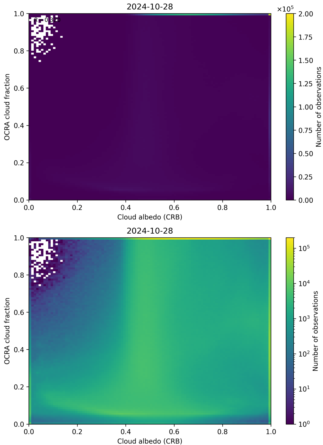
Figure 70: Scatter density plot of “Cloud albedo (CRB)” against “OCRA cloud fraction” for 2024-10-27 to 2024-10-29.
