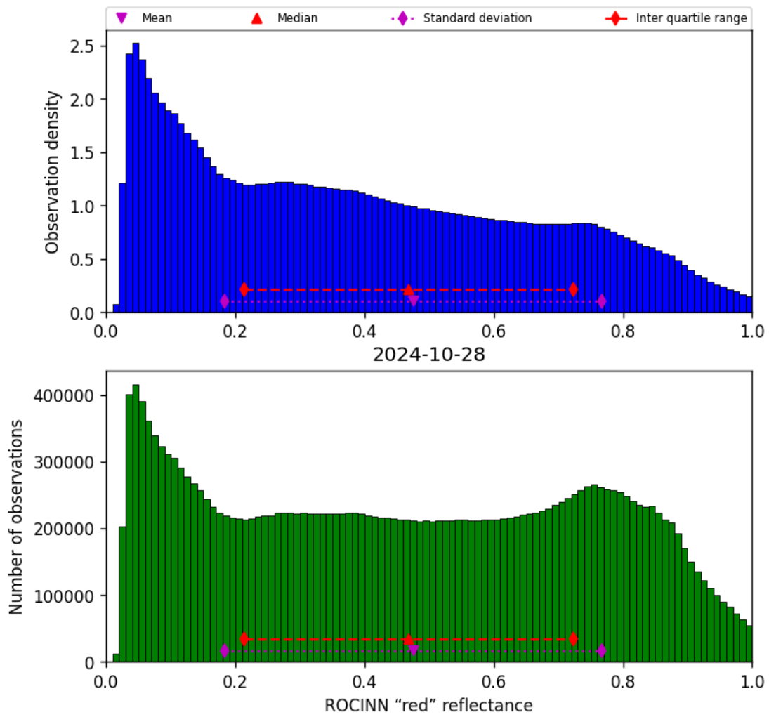
Figure 53: Histogram of “ROCINN “red” reflectance” for 2024-10-27 to 2024-10-29
