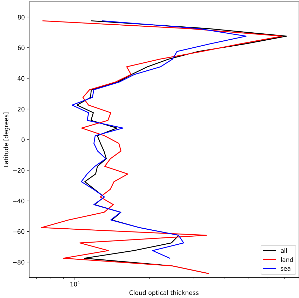
Figure 25: Zonal average of “Cloud optical thickness” for 2024-10-27 to 2024-10-29.
