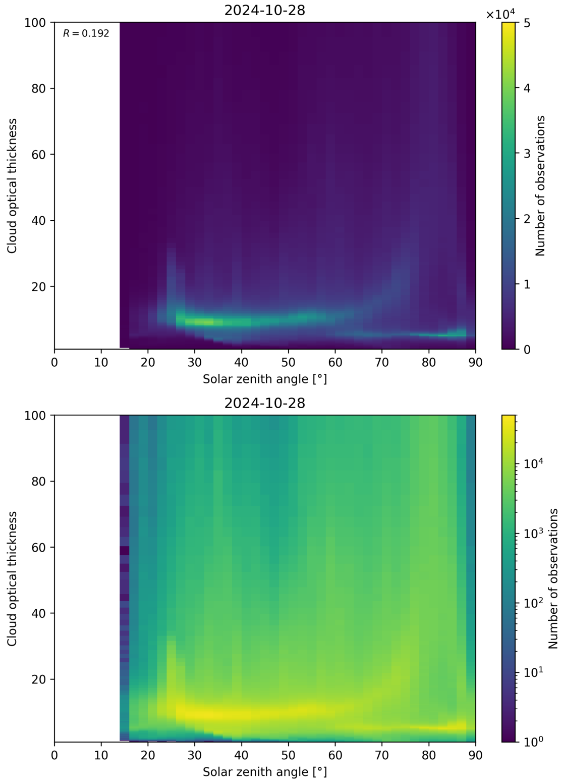
Figure 103: Scatter density plot of “Solar zenith angle” against “Cloud optical thickness” for 2024-10-27 to 2024-10-29.
