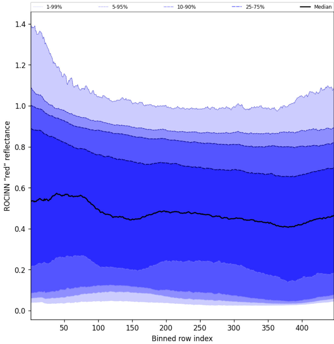
Figure 69: Along track statistics of "ROCINN "red" reflectance" for 2024-10-27 to 2024-10-29
