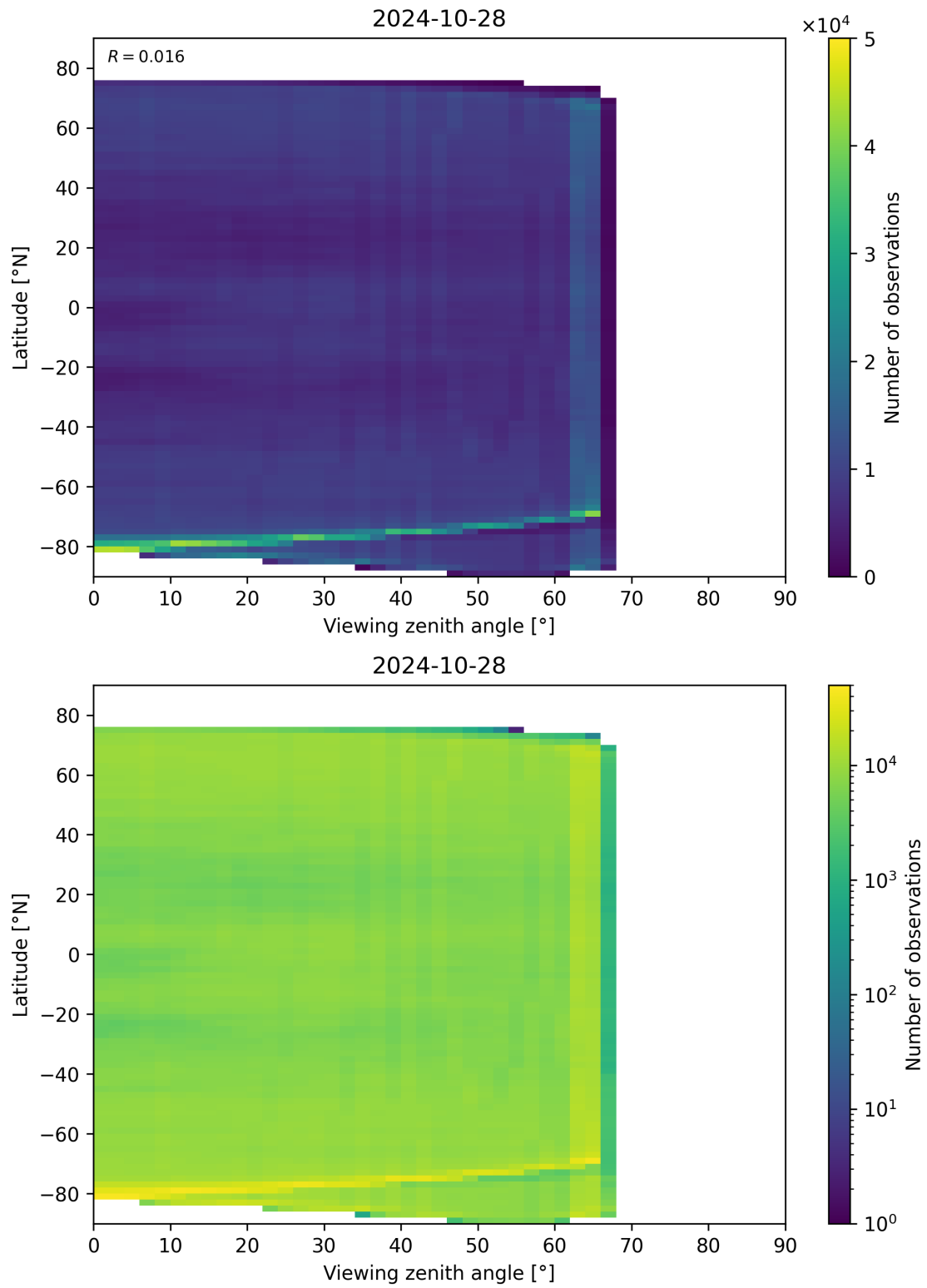
Figure 113: Scatter density plot of “Viewing zenith angle” against “Latitude” for 2024-10-27 to 2024-10-29.
