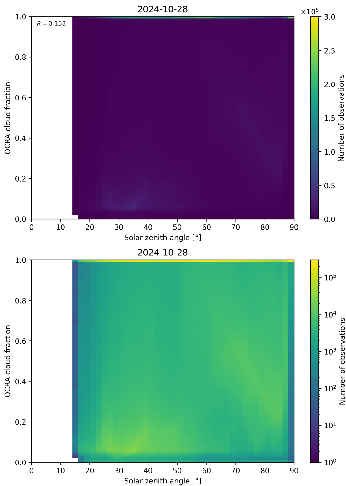
Figure 100: Scatter density plot of “Solar zenith angle” against “OCRA cloud fraction” for 2024-10-27 to 2024-10-29.
