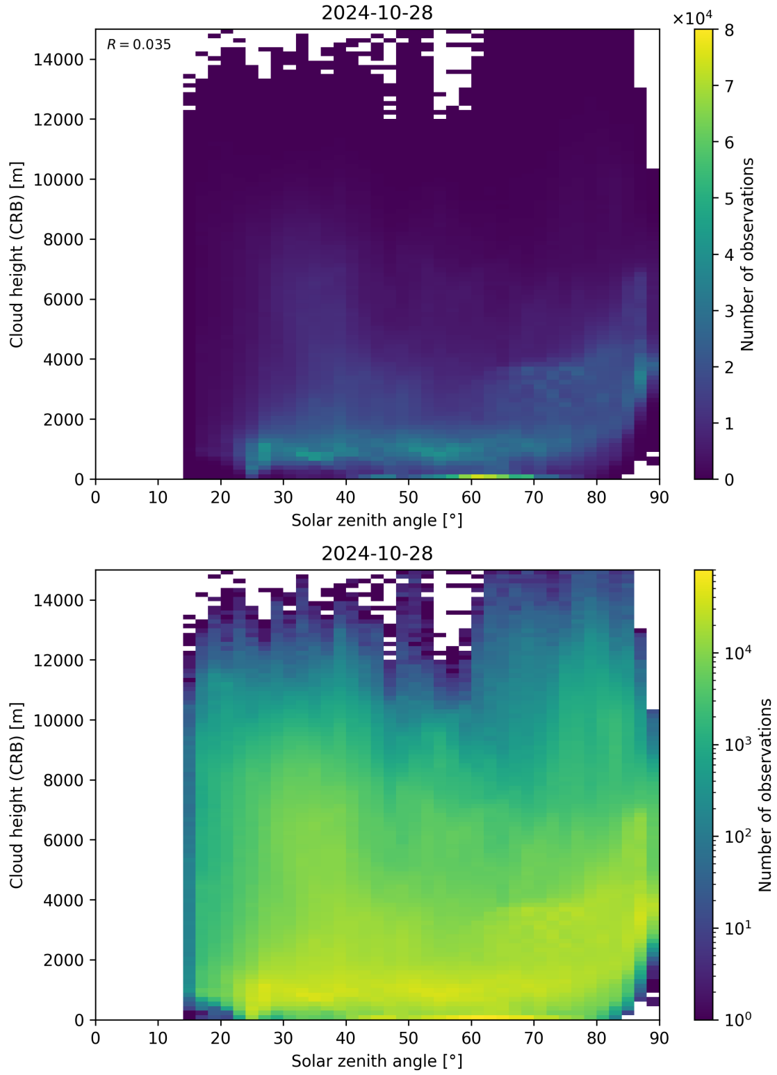
Figure 102: Scatter density plot of “Solar zenith angle” against “Cloud height (CRB)” for 2024-10-27 to 2024-10-29.
