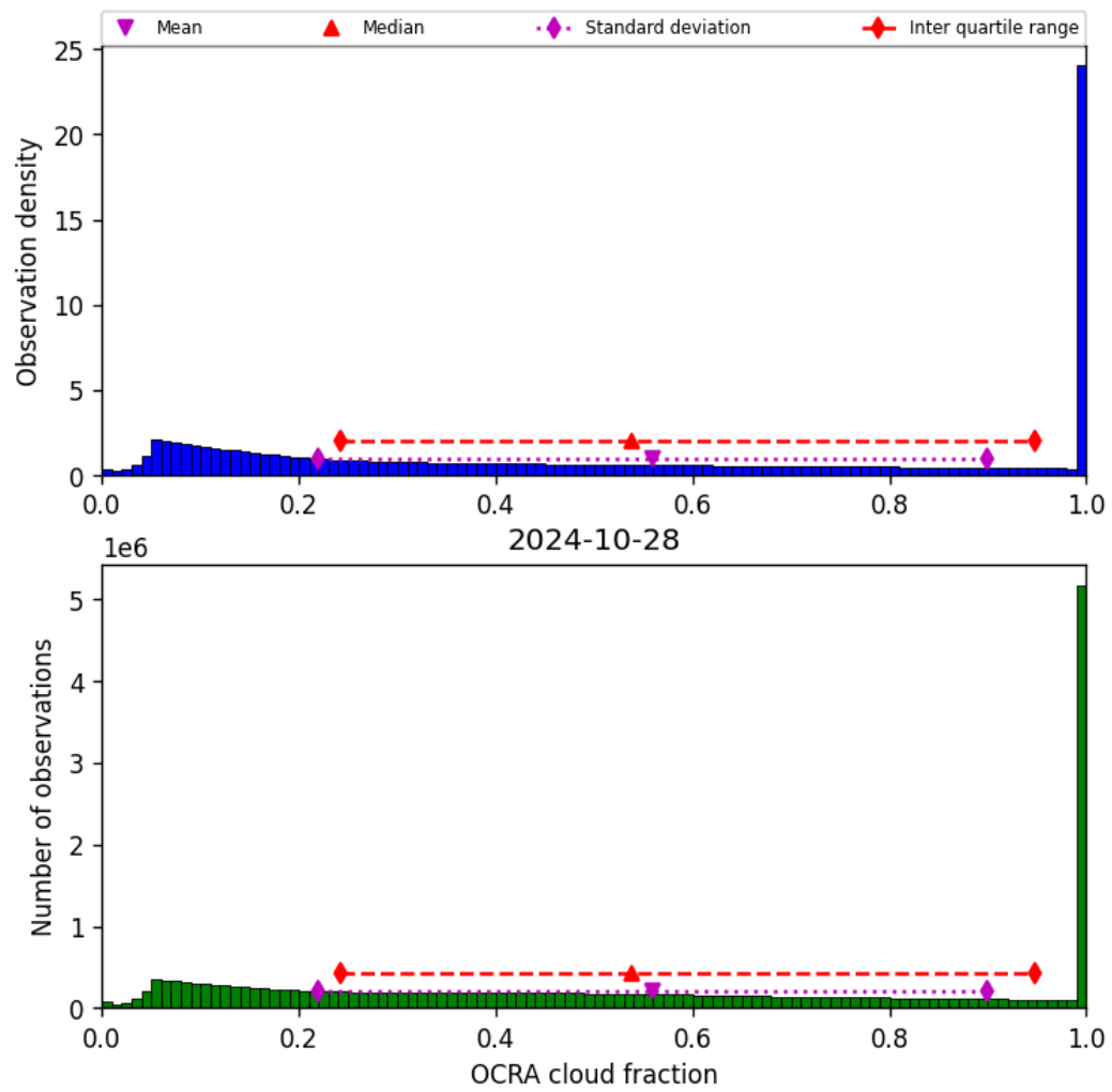
Figure 50: Histogram of “OCRA cloud fraction” for 2024-10-27 to 2024-10-29
