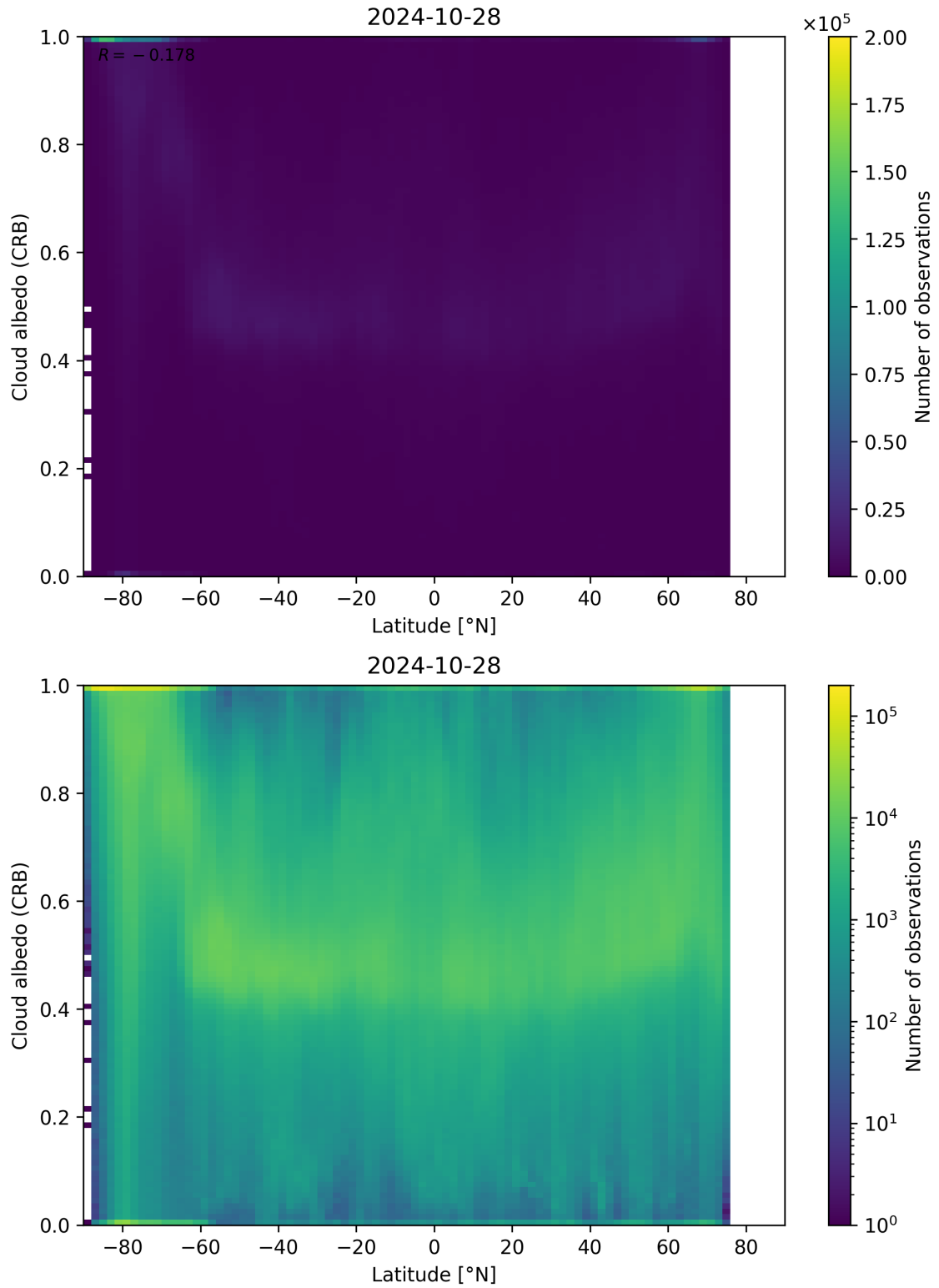
Figure 91: Scatter density plot of “Latitude” against “Cloud albedo (CRB)” for 2024-10-27 to 2024-10-29.
