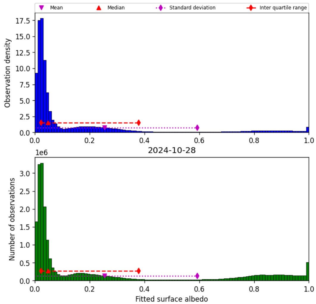
Figure 45: Histogram of “Fitted surface albedo” for 2024-10-27 to 2024-10-29
