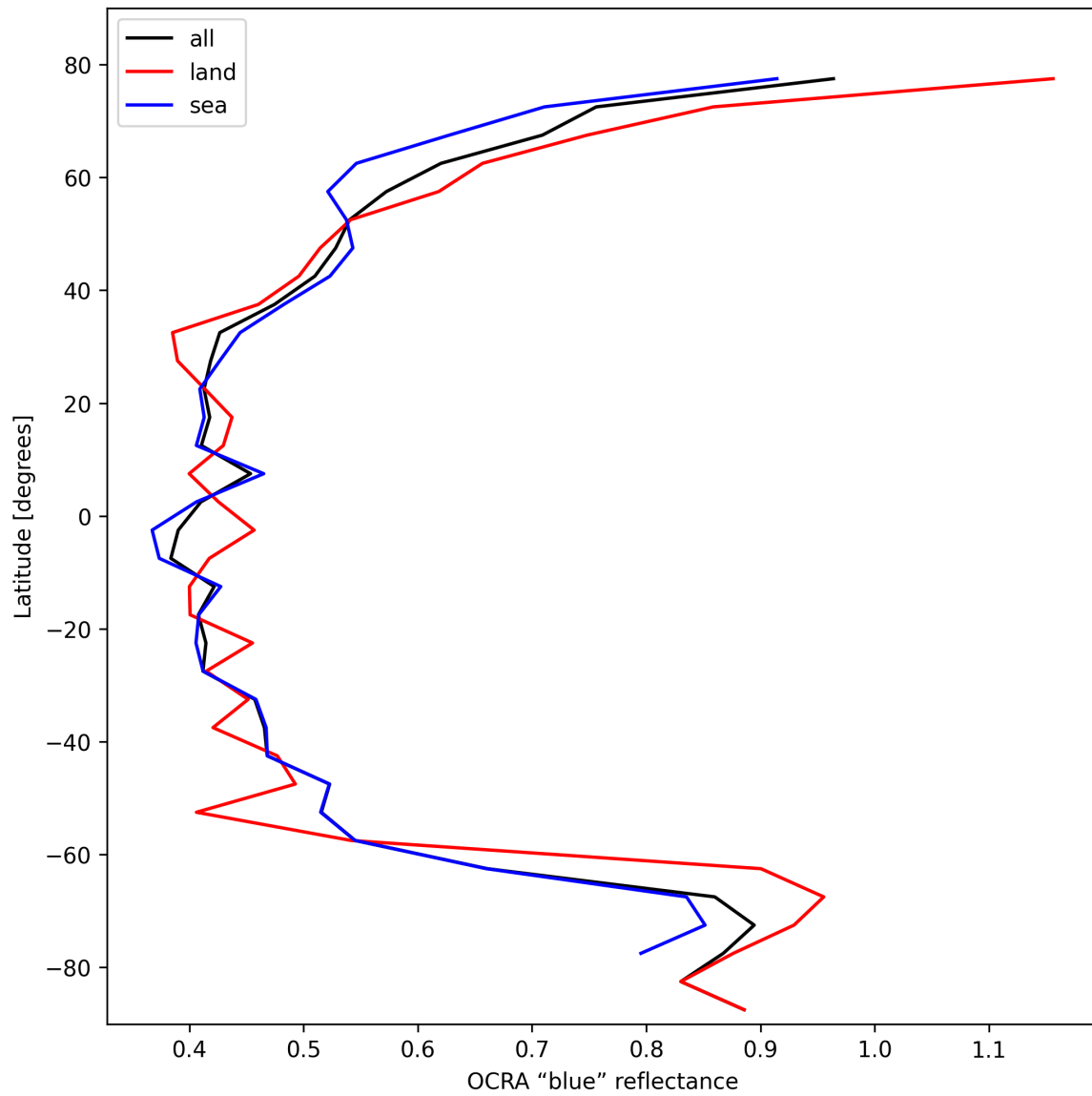
Figure 35: Zonal average of "OCRA "blue" reflectance" for 2024-10-27 to 2024-10-29.
