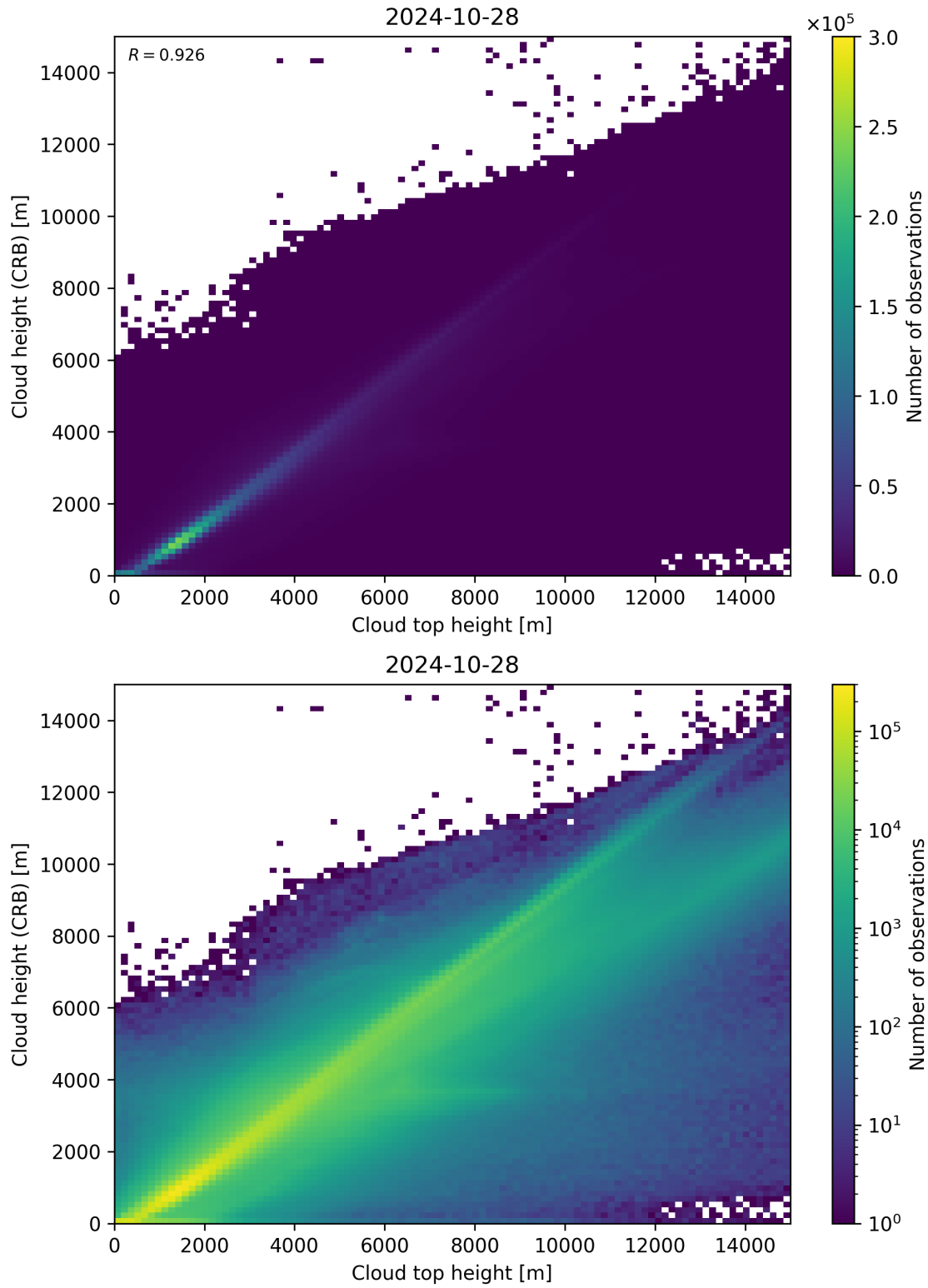
Figure 89: Scatter density plot of “Cloud top height” against “Cloud height (CRB)” for 2024-10-27 to 2024-10-29.
