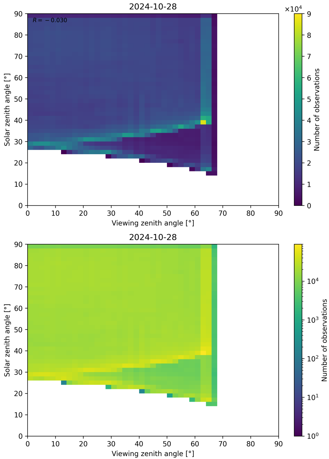
Figure 114: Scatter density plot of “Viewing zenith angle” against “Solar zenith angle” for 2024-10-27 to 2024-10-29.
