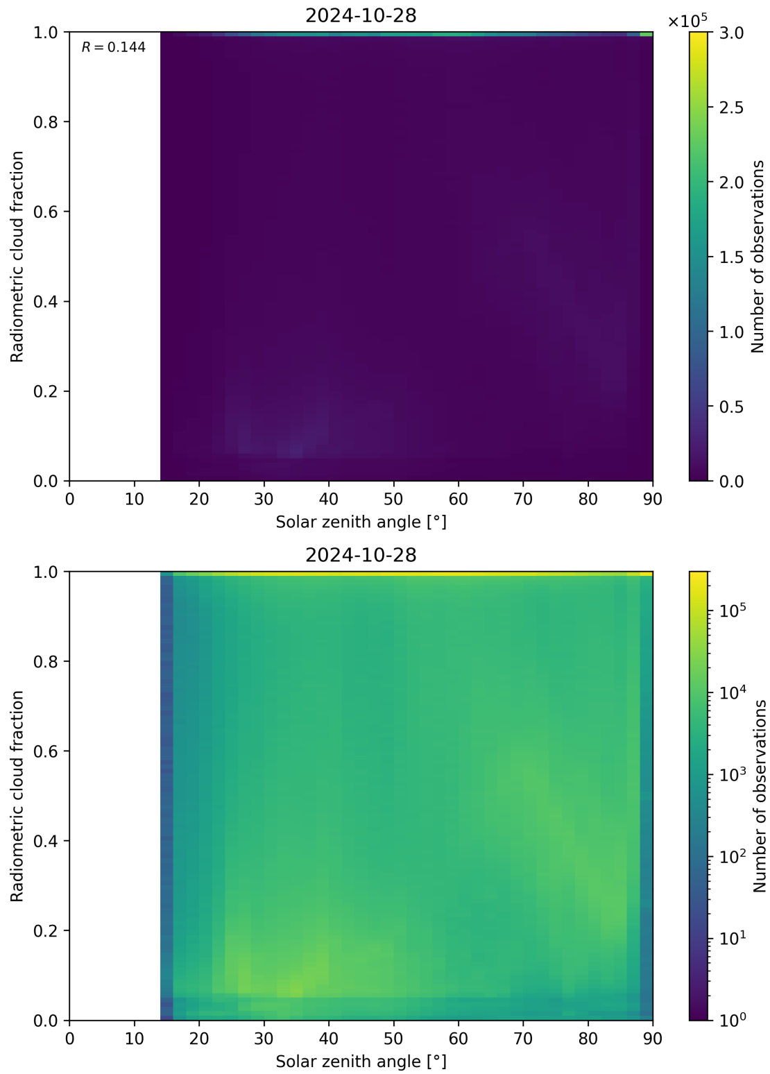
Figure 99: Scatter density plot of “Solar zenith angle” against “Radiometric cloud fraction” for 2024-10-27 to 2024-10-29.
