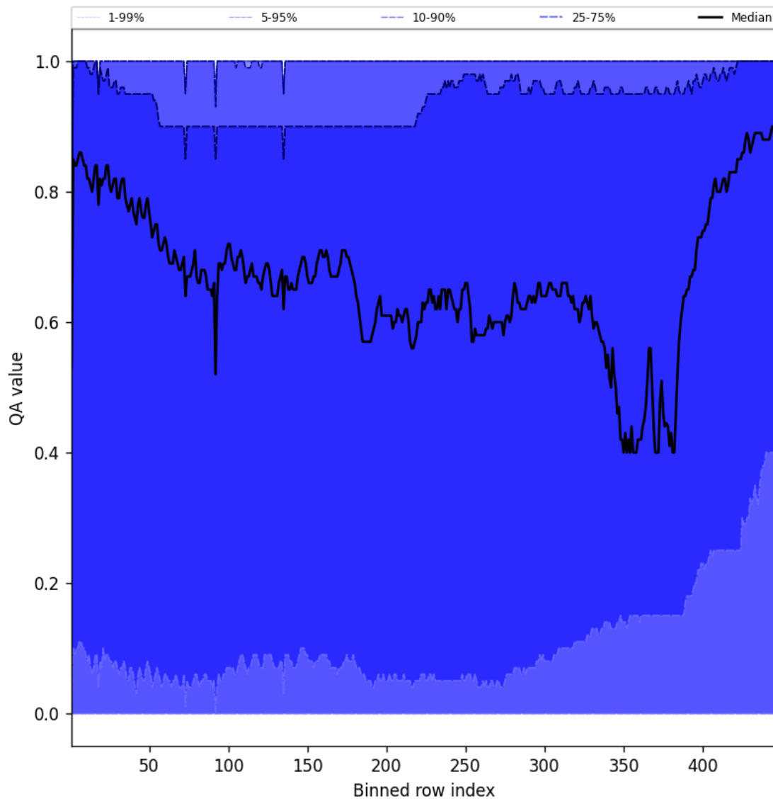
Figure 54: Along track statistics of “QA value” for 2024-10-27 to 2024-10-29
