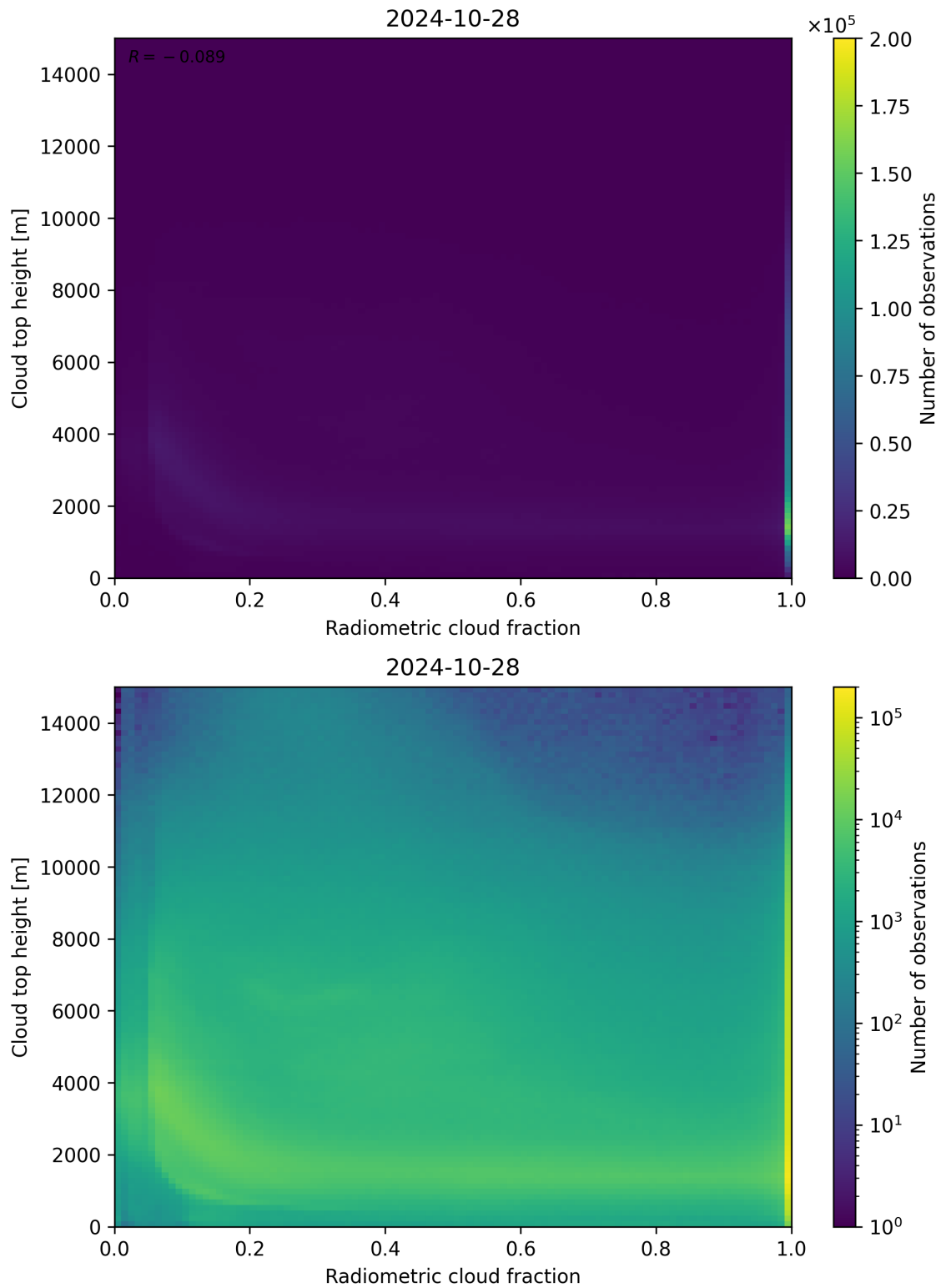
Figure 76: Scatter density plot of “Radiometric cloud fraction” against “Cloud top height” for 2024-10-27 to 2024-10-29.
