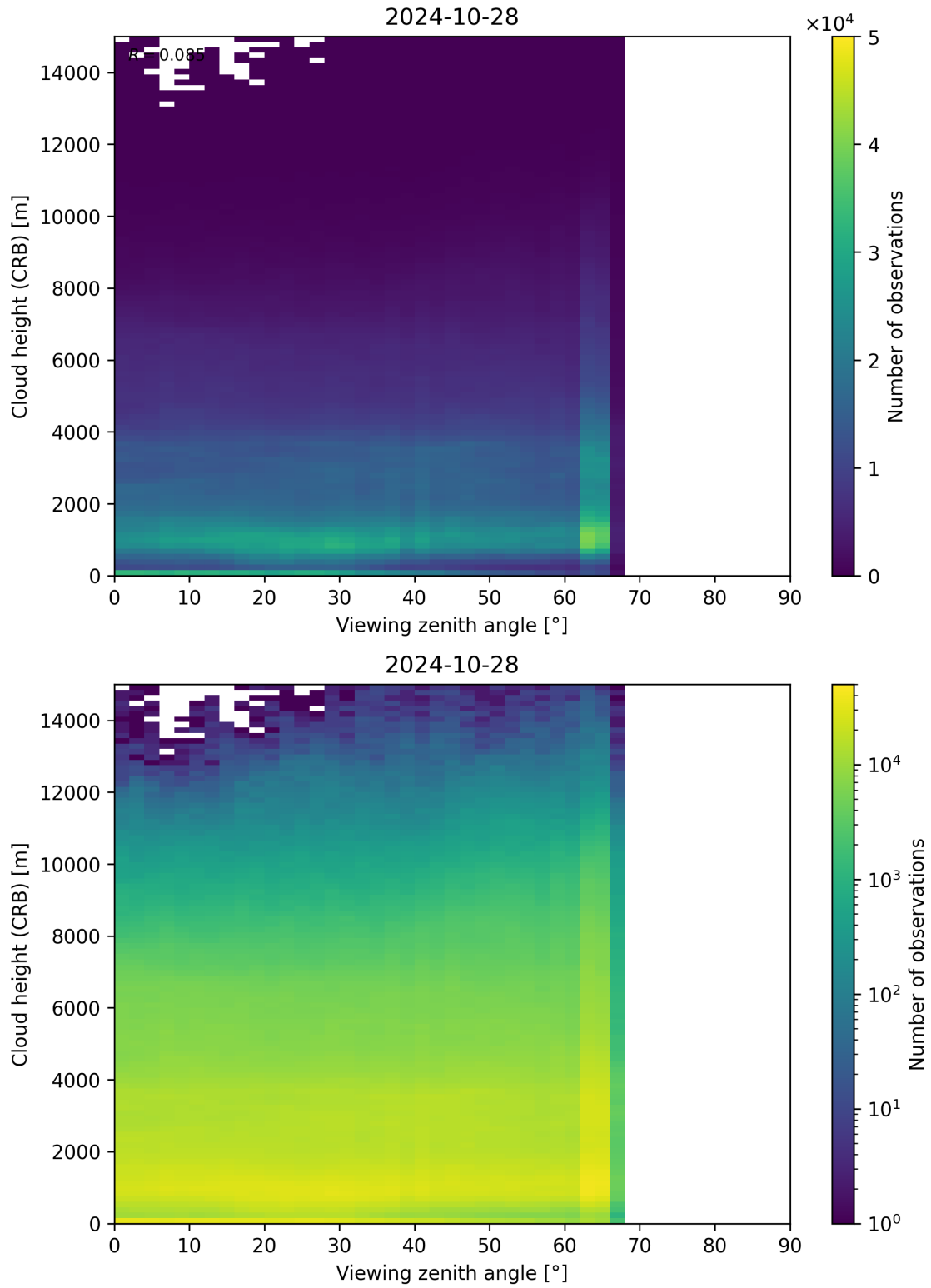
Figure 110: Scatter density plot of “Viewing zenith angle” against “Cloud height (CRB)” for 2024-10-27 to 2024-10-29.
