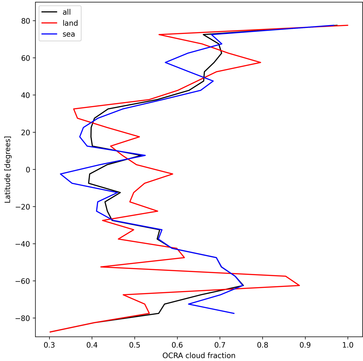
Figure 34: Zonal average of “OCRA cloud fraction” for 2024-10-27 to 2024-10-29.
