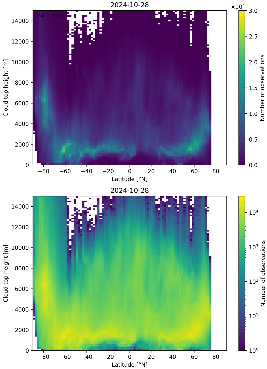
Figure 97: Scatter density plot of “Latitude” against “Cloud top height” for 2024-10-27 to 2024-10-29.
