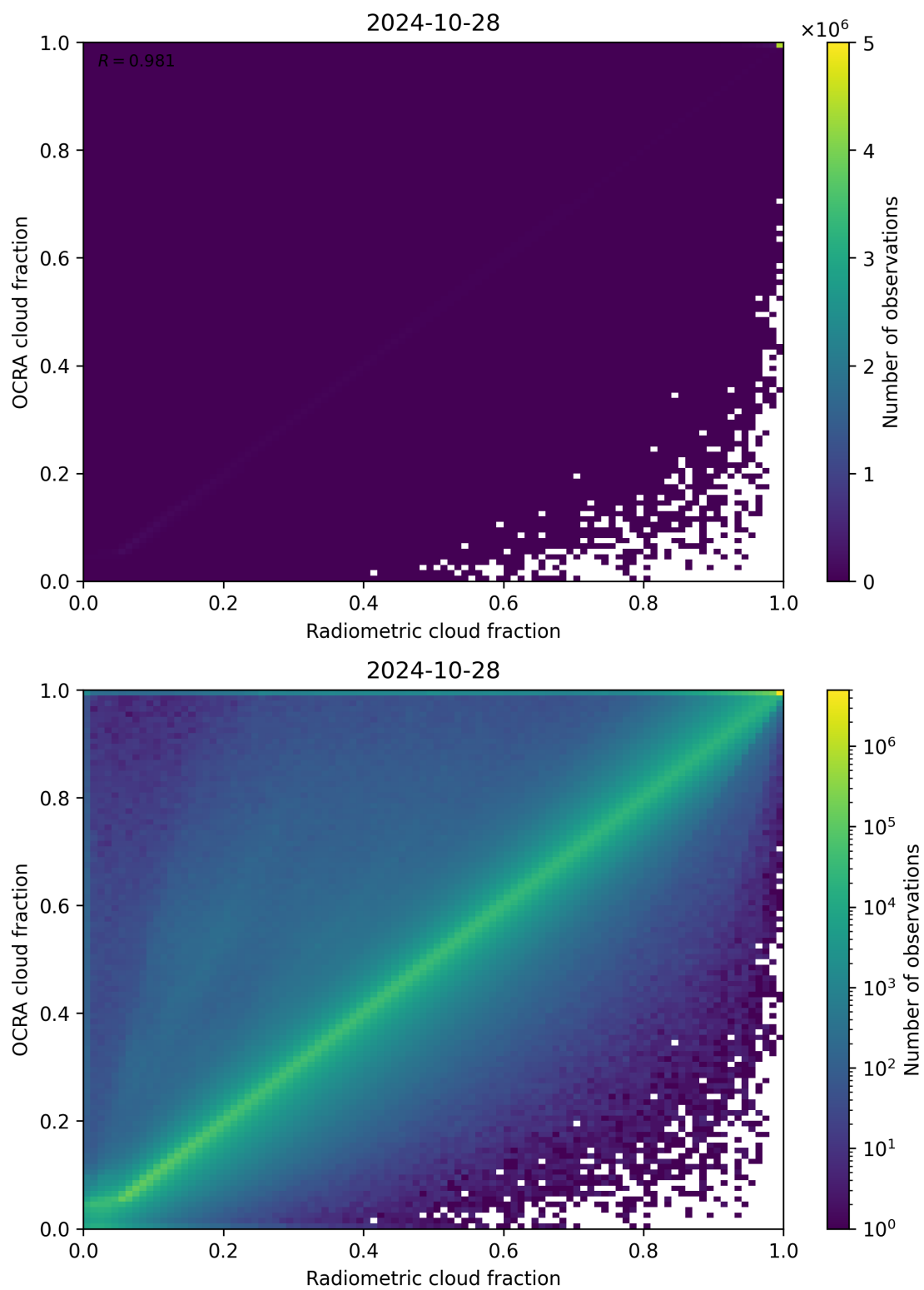
Figure 72: Scatter density plot of “Radiometric cloud fraction” against “OCRA cloud fraction” for 2024-10-27 to 2024-10-29.
