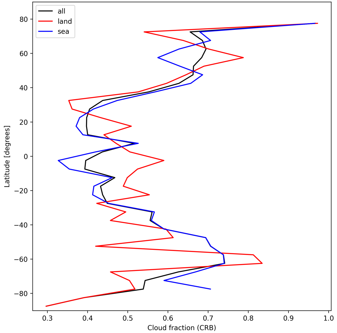
Figure 26: Zonal average of “Cloud fraction (CRB)” for 2024-10-27 to 2024-10-29.
