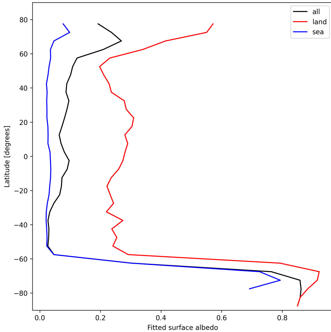
Figure 29: Zonal average of “Fitted surface albedo” for 2024-10-27 to 2024-10-29.
