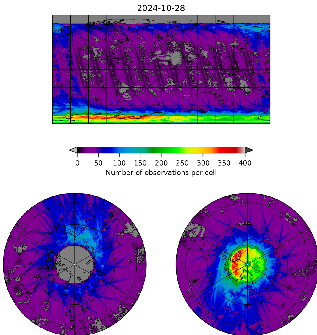
Figure 21: Map of the number of observations for 2024-10-27 to 2024-10-29
