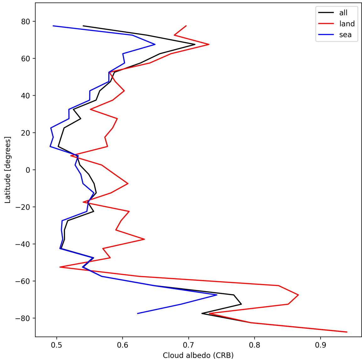
Figure 28: Zonal average of “Cloud albedo (CRB)” for 2024-10-27 to 2024-10-29.
