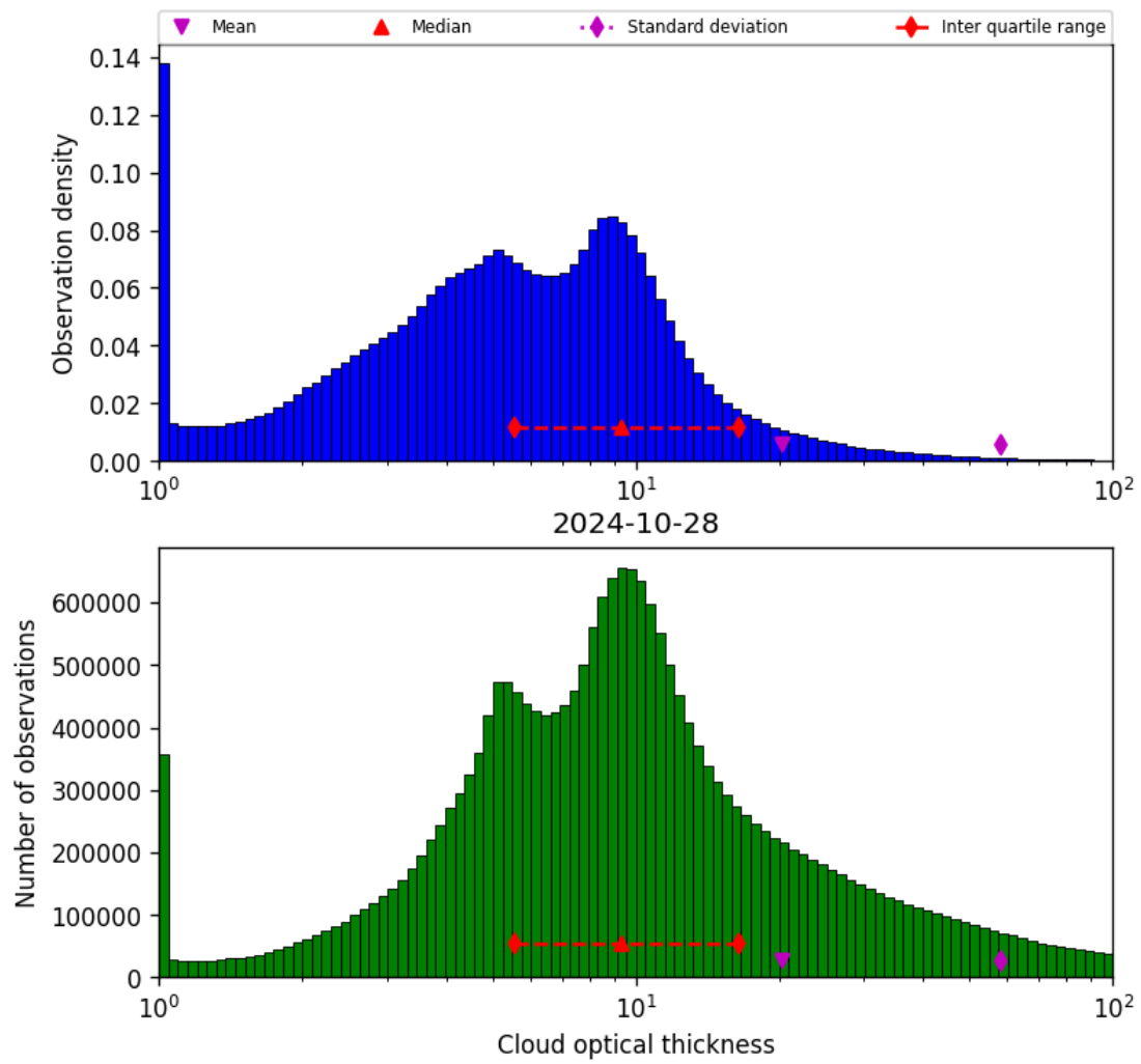
Figure 41: Histogram of “Cloud optical thickness” for 2024-10-27 to 2024-10-29
