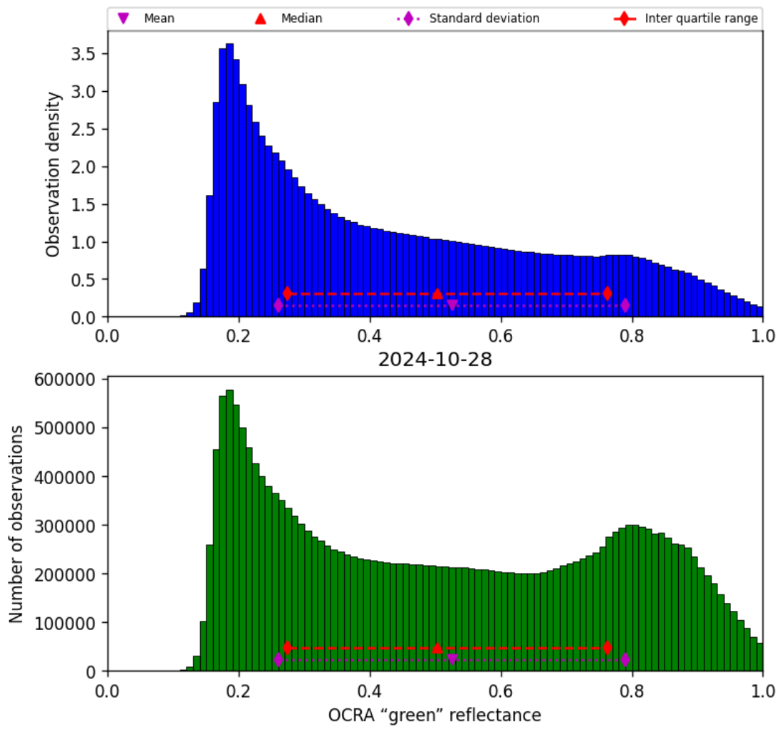
Figure 52: Histogram of “OCRA “green” reflectance” for 2024-10-27 to 2024-10-29
