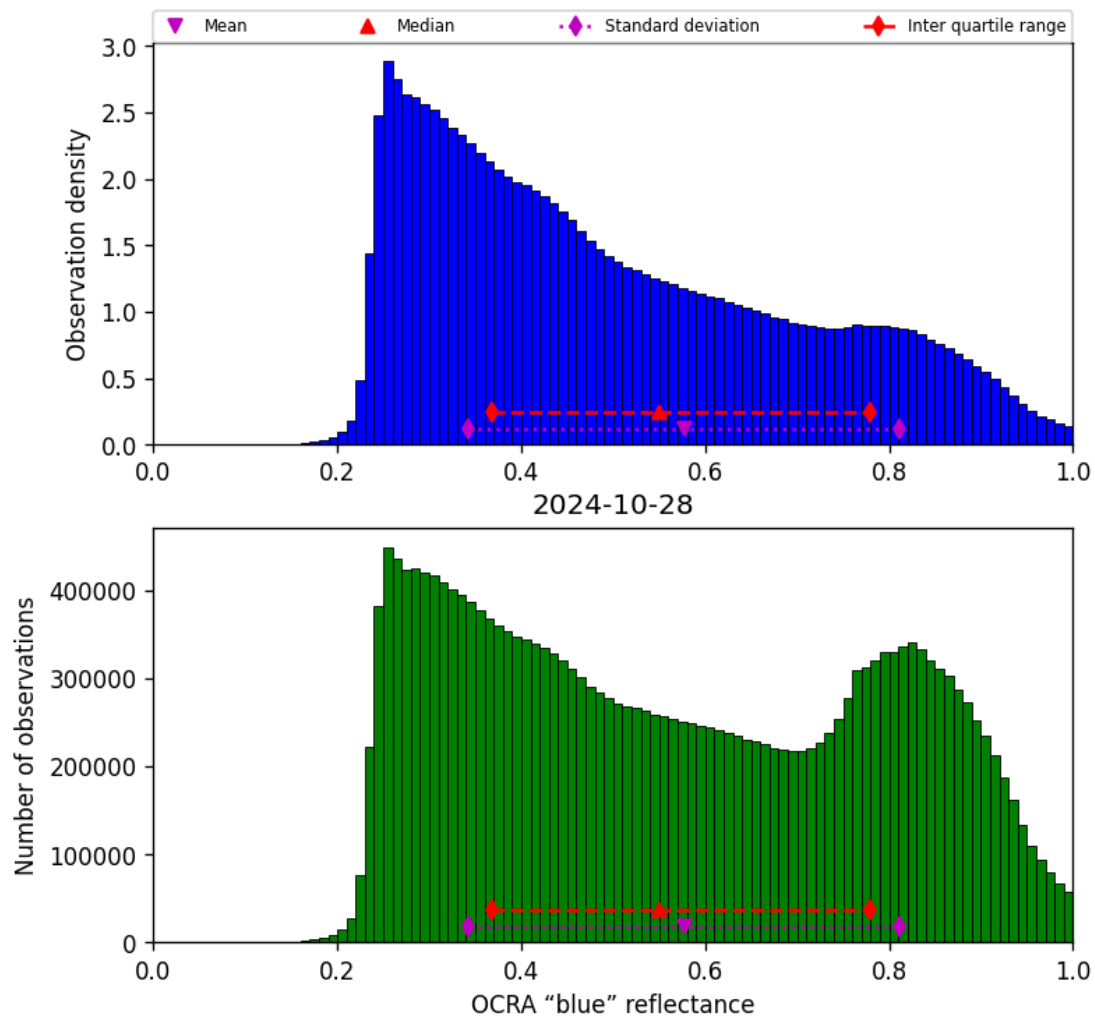
Figure 51: Histogram of “OCRA “blue” reflectance” for 2024-10-27 to 2024-10-29
