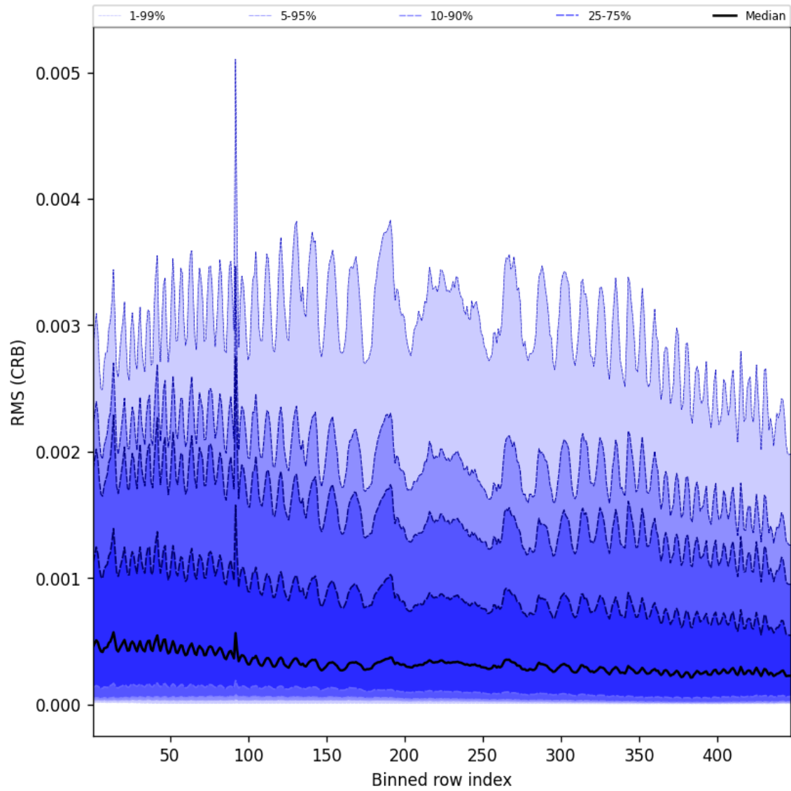
Figure 64: Along track statistics of “RMS (CRB)” for 2024-10-27 to 2024-10-29
