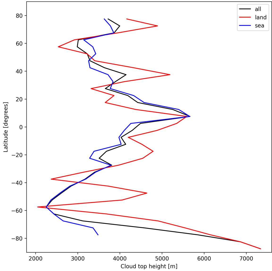
Figure 24: Zonal average of “Cloud top height” for 2024-10-27 to 2024-10-29.
