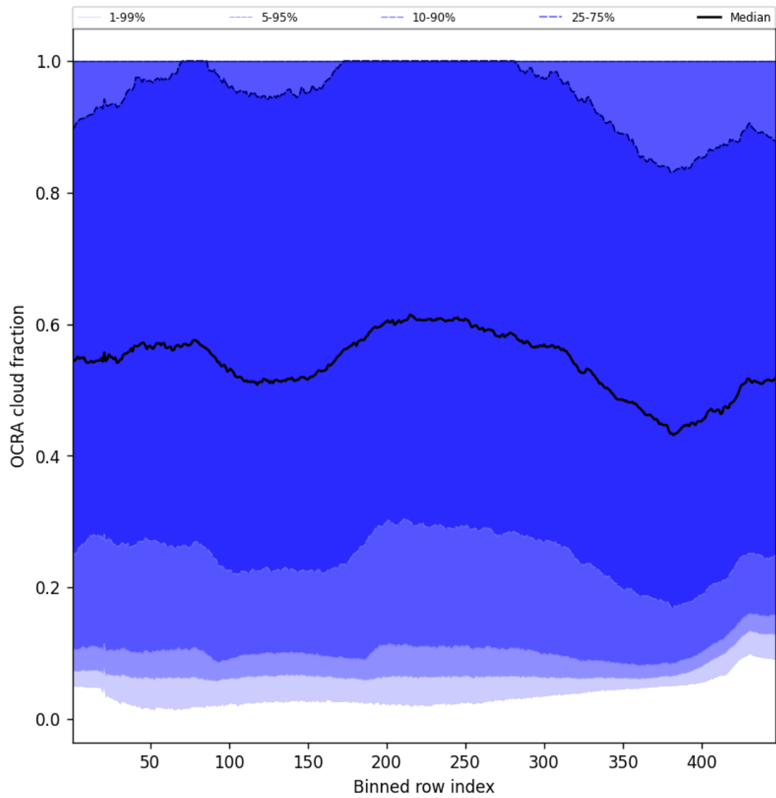
Figure 66: Along track statistics of “OCRA cloud fraction” for 2024-10-27 to 2024-10-29
