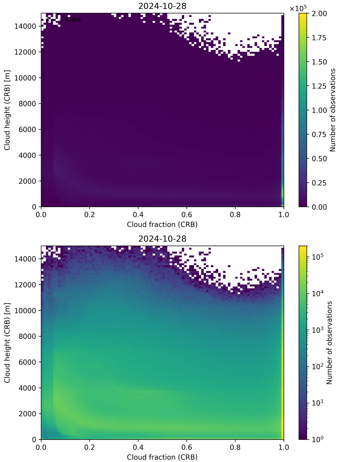
Figure 79: Scatter density plot of “Cloud fraction (CRB)” against “Cloud height (CRB)” for 2024-10-27 to 2024-10-29.
