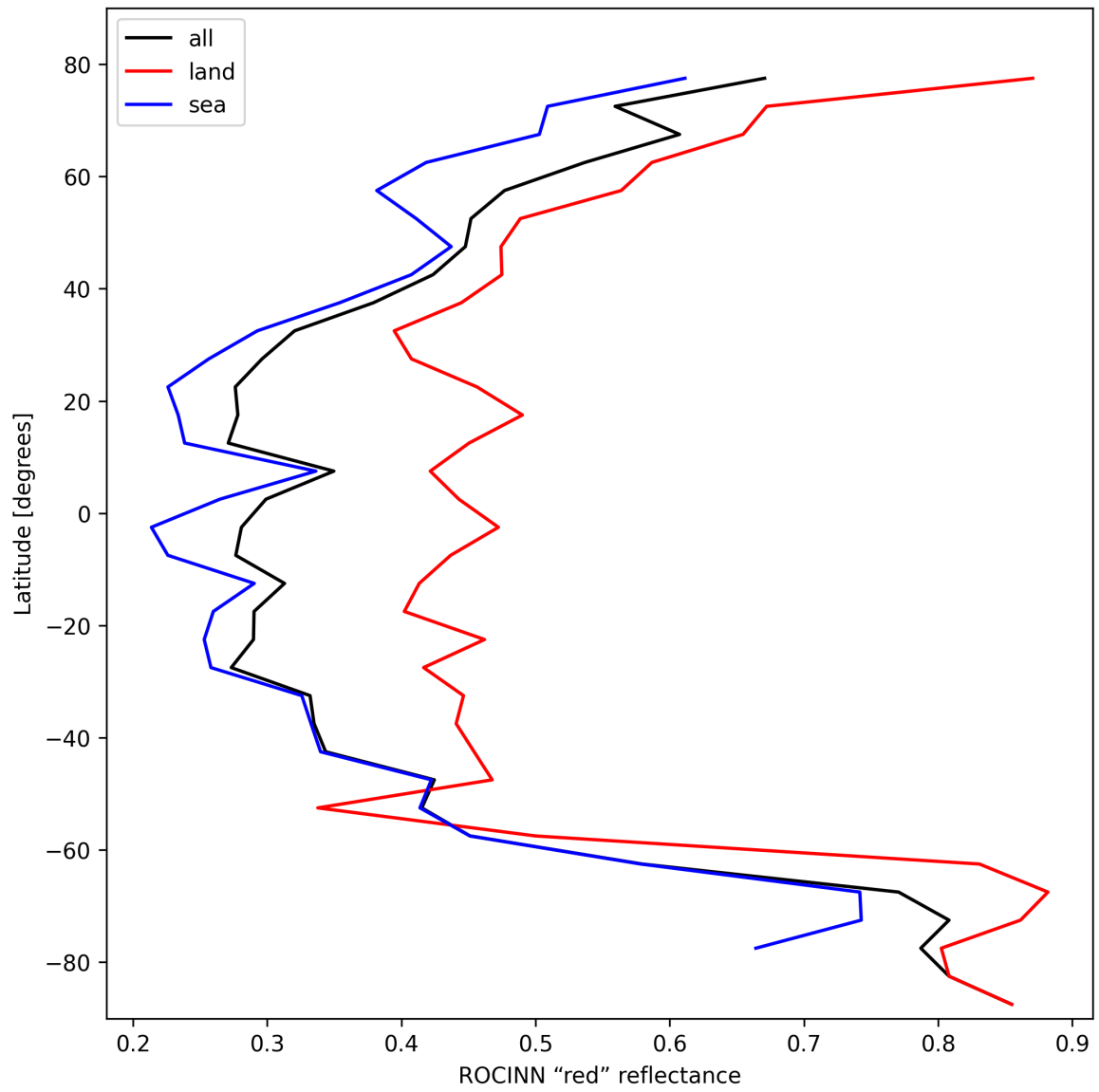
Figure 37: Zonal average of “ROCINN “red” reflectance” for 2024-10-27 to 2024-10-29.
