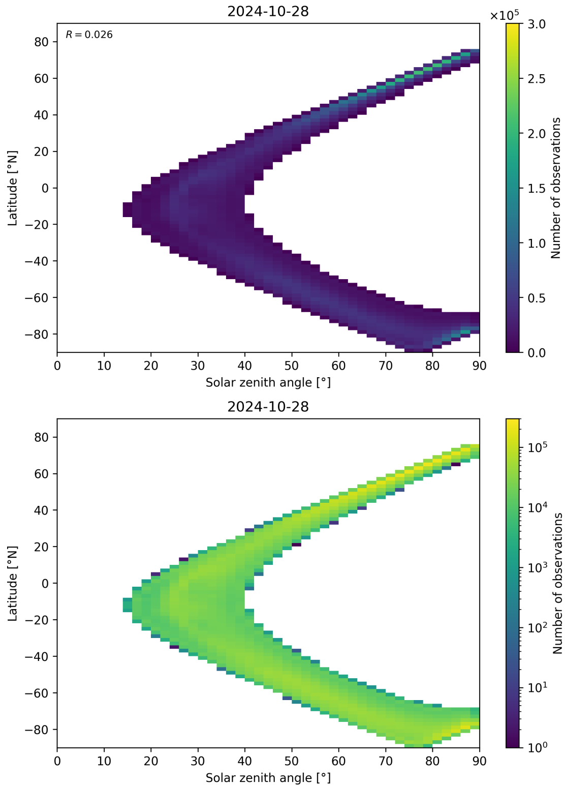
Figure 105: Scatter density plot of “Solar zenith angle” against “Latitude” for 2024-10-27 to 2024-10-29.
