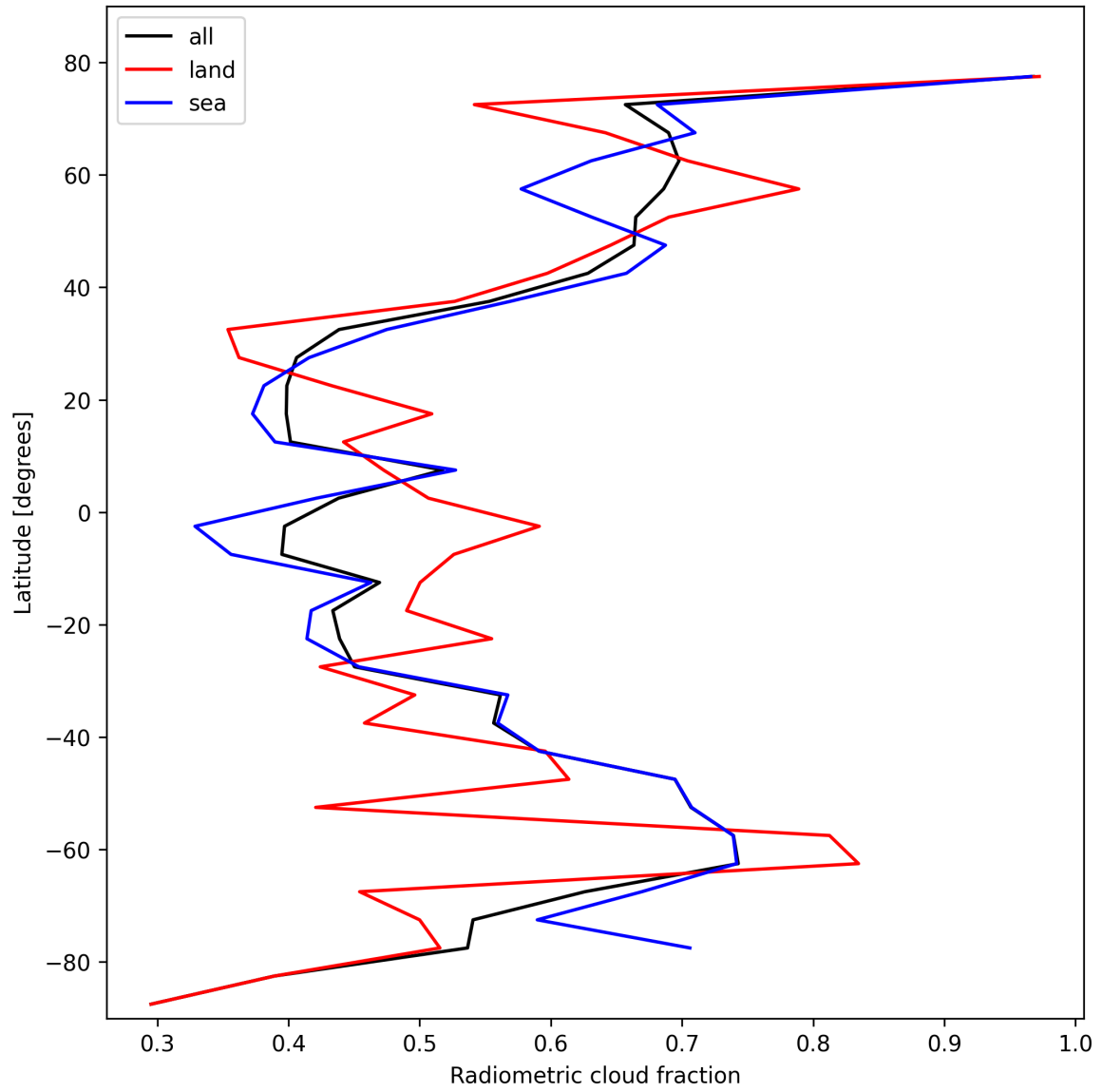
Figure 23: Zonal average of “Radiometric cloud fraction” for 2024-10-27 to 2024-10-29.
