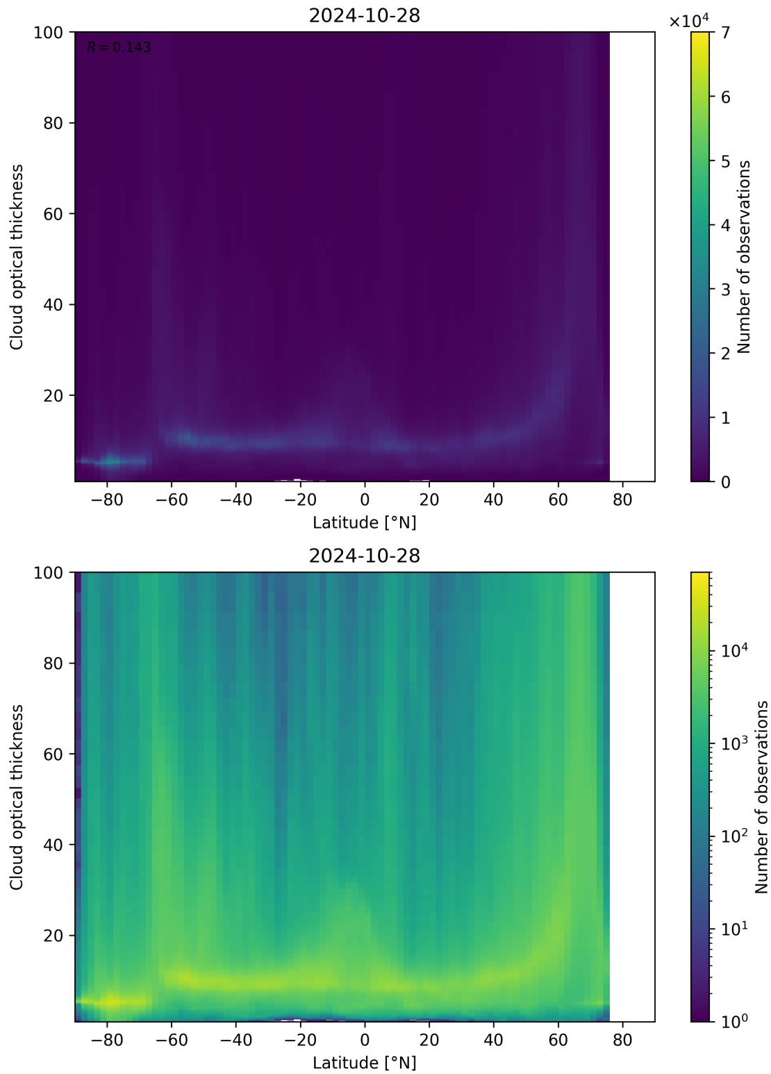
Figure 96: Scatter density plot of “Latitude” against “Cloud optical thickness” for 2024-10-27 to 2024-10-29.
