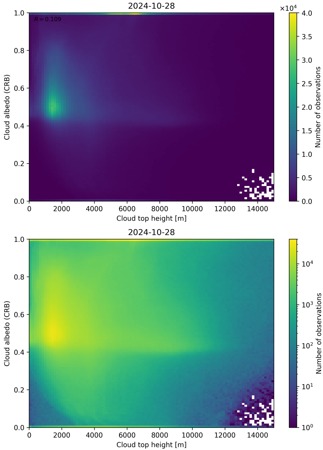
Figure 86: Scatter density plot of “Cloud top height” against “Cloud albedo (CRB)” for 2024-10-27 to 2024-10-29.
