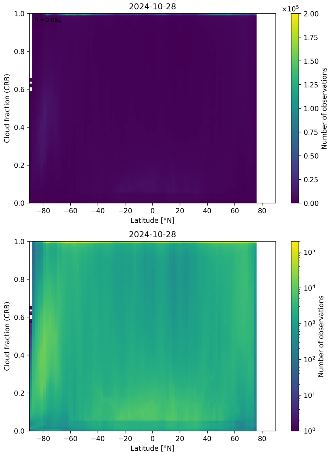
Figure 94: Scatter density plot of “Latitude” against “Cloud fraction (CRB)” for 2024-10-27 to 2024-10-29.
