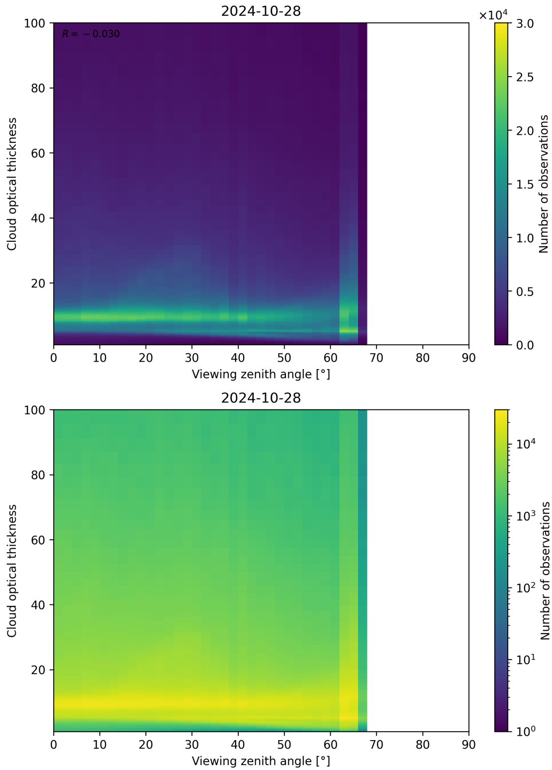
Figure 111: Scatter density plot of “Viewing zenith angle” against “Cloud optical thickness” for 2024-10-27 to 2024-10-29.
