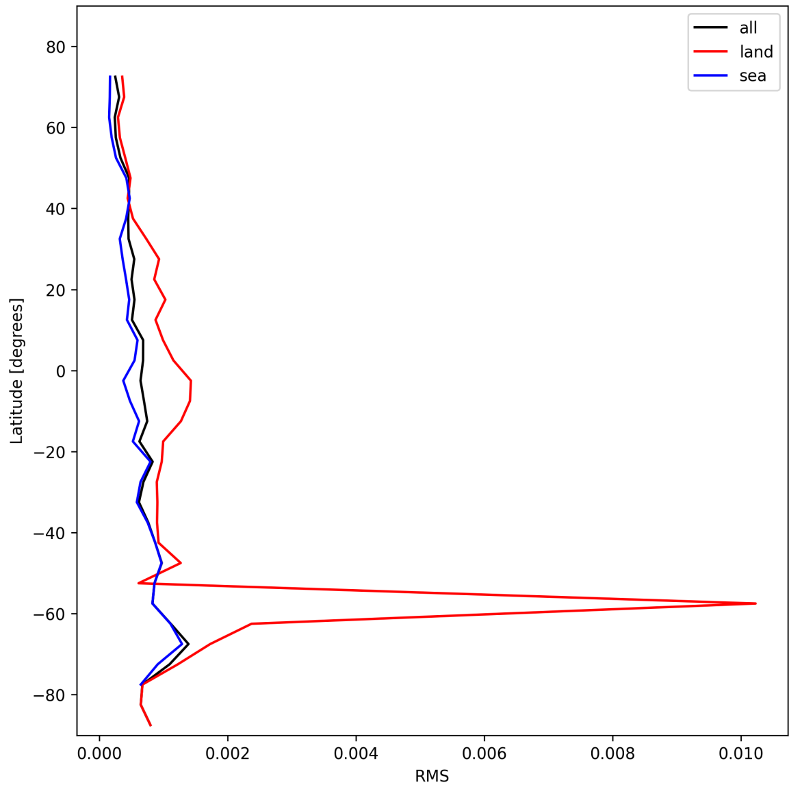
Figure 31: Zonal average of “RMS” for 2024-10-30 to 2024-11-01.
