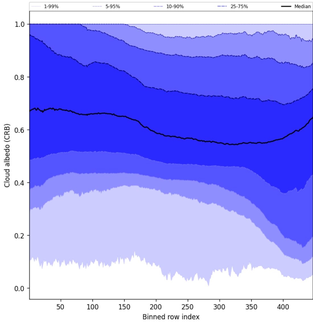
Figure 60: Along track statistics of “Cloud albedo (CRB)” for 2024-10-30 to 2024-11-01
