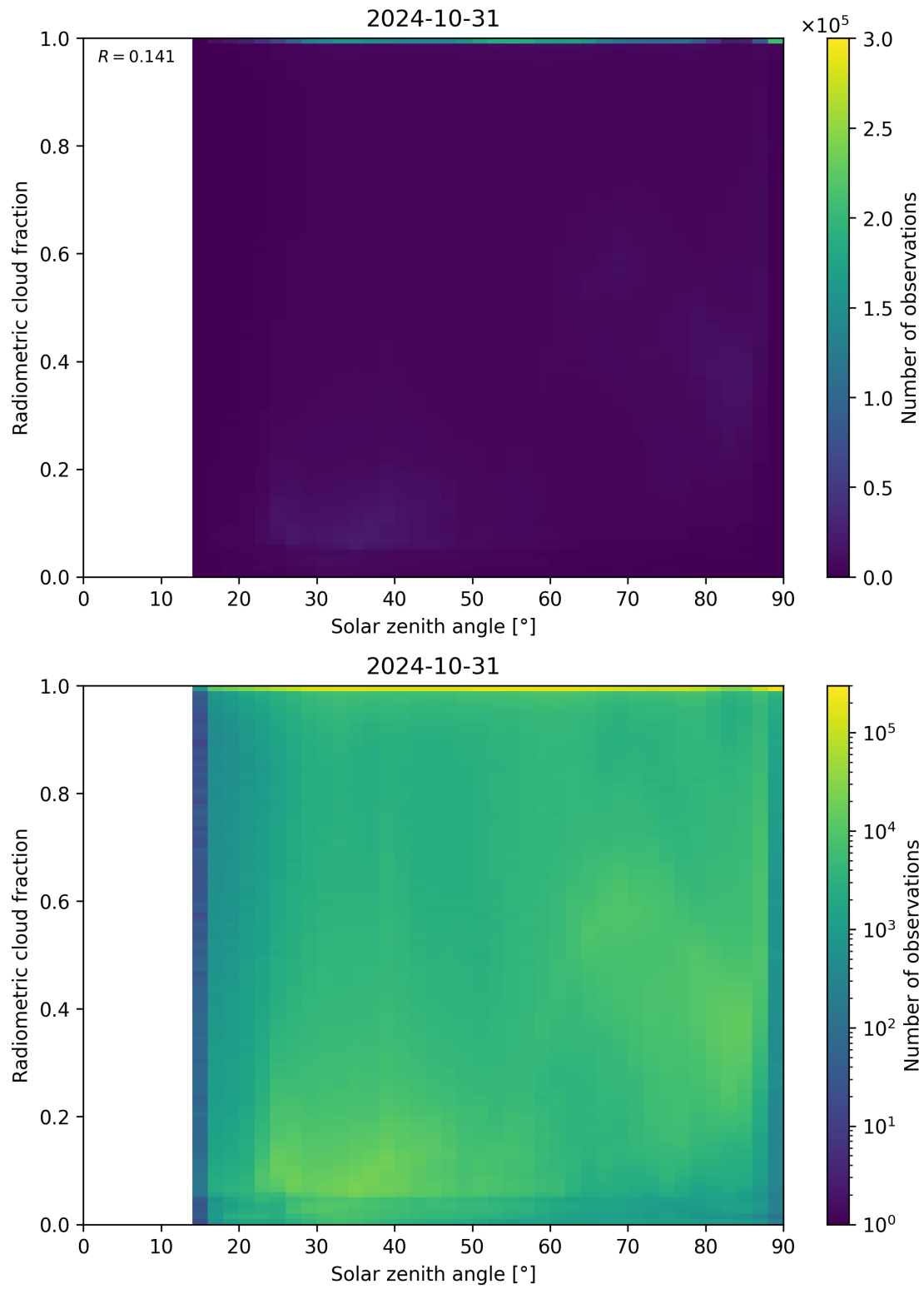
Figure 99: Scatter density plot of “Solar zenith angle” against “Radiometric cloud fraction” for 2024-10-30 to 2024-11-01.
