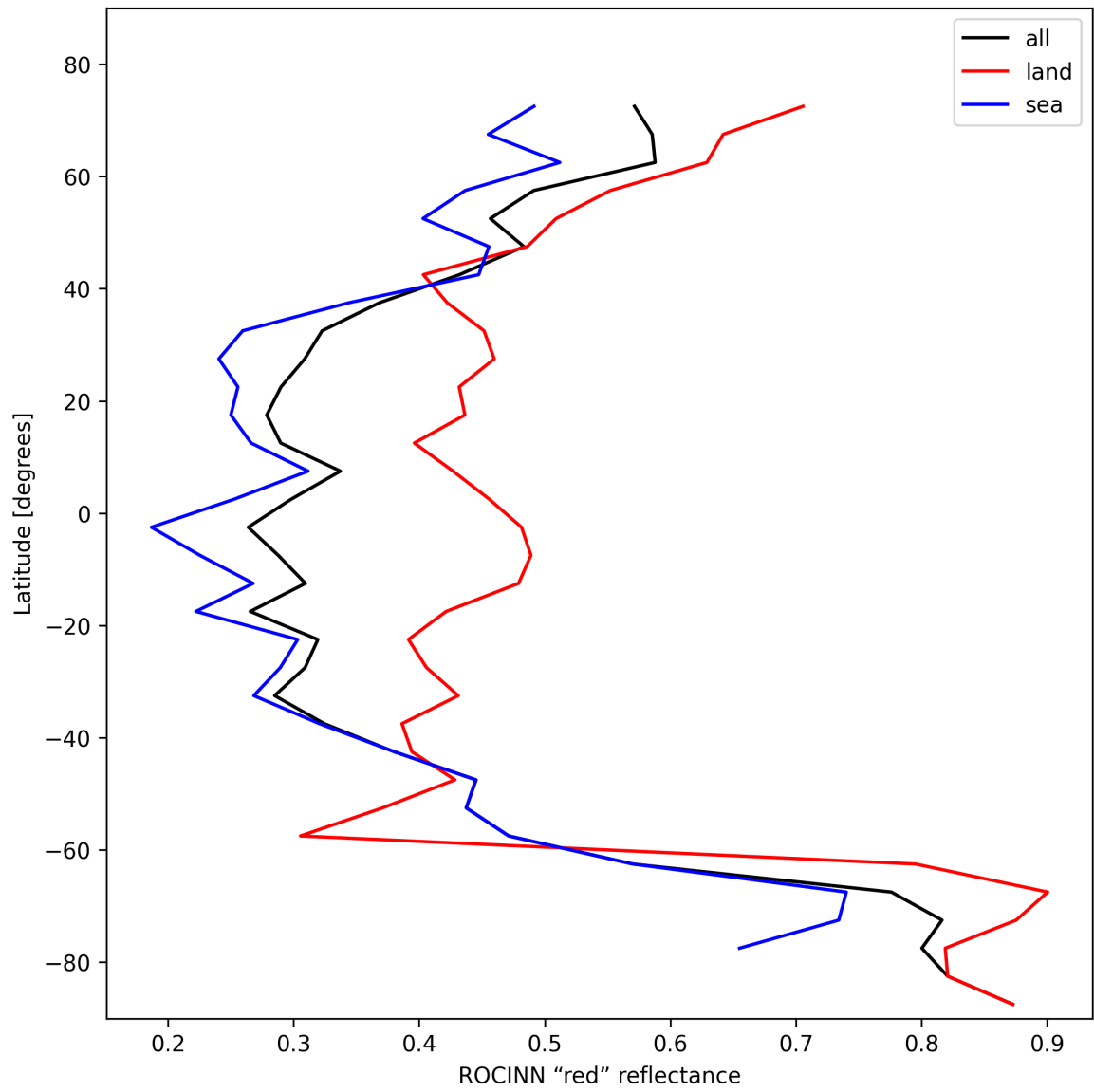
Figure 37: Zonal average of “ROCINN “red” reflectance” for 2024-10-30 to 2024-11-01.
