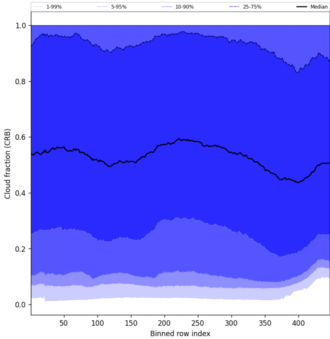
Figure 58: Along track statistics of “Cloud fraction (CRB)” for 2024-10-30 to 2024-11-01
