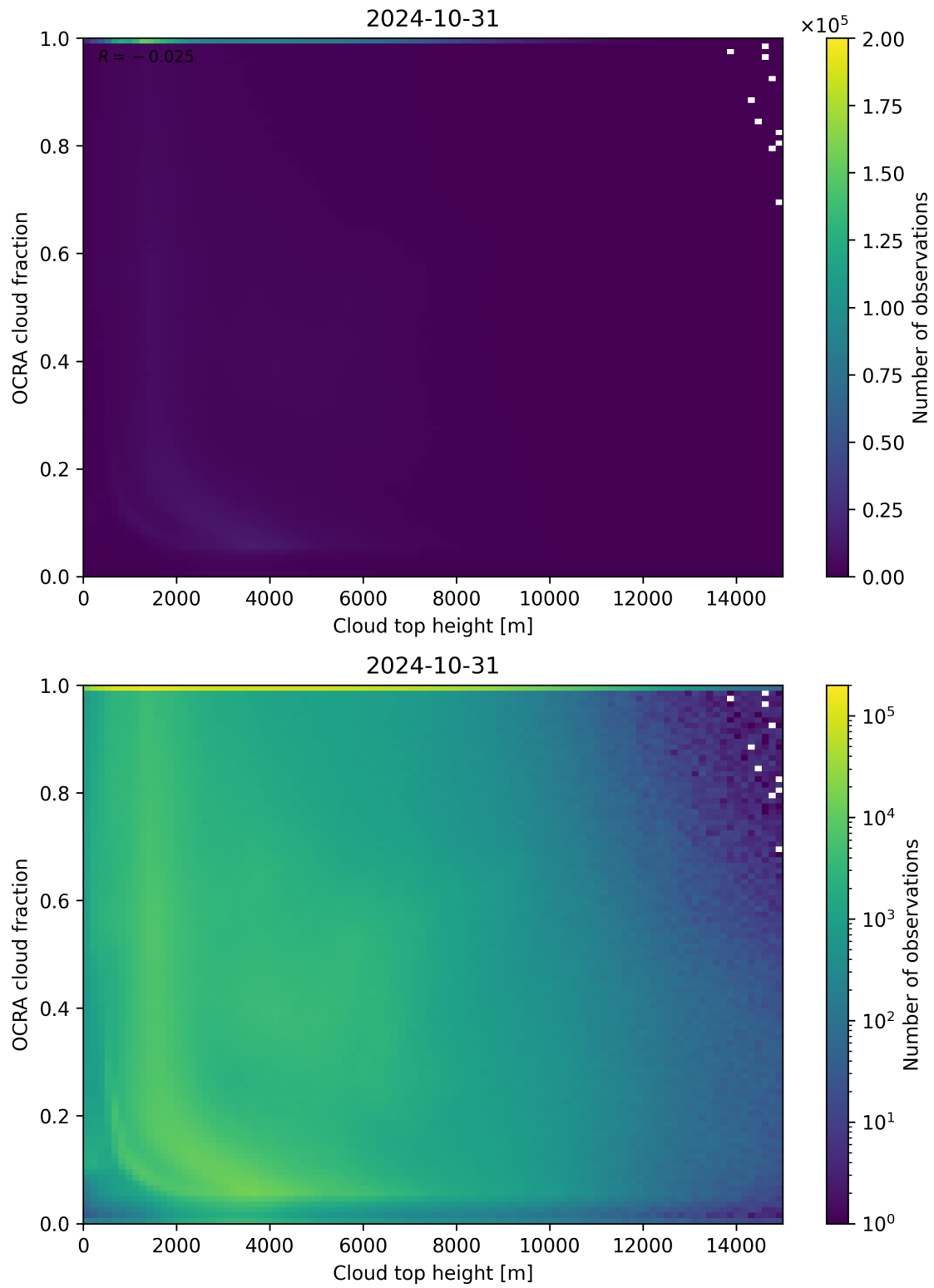
Figure 87: Scatter density plot of “Cloud top height” against “OCRA cloud fraction” for 2024-10-30 to 2024-11-01.
