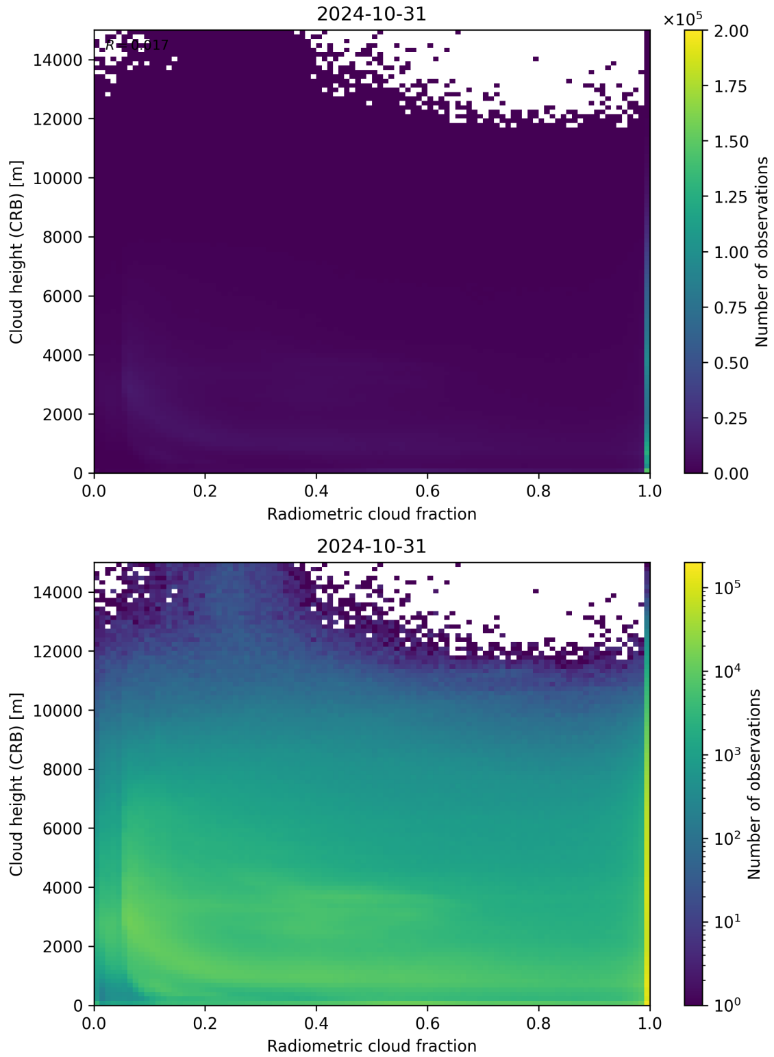
Figure 74: Scatter density plot of “Radiometric cloud fraction” against “Cloud height (CRB)” for 2024-10-30 to 2024-11-01.
