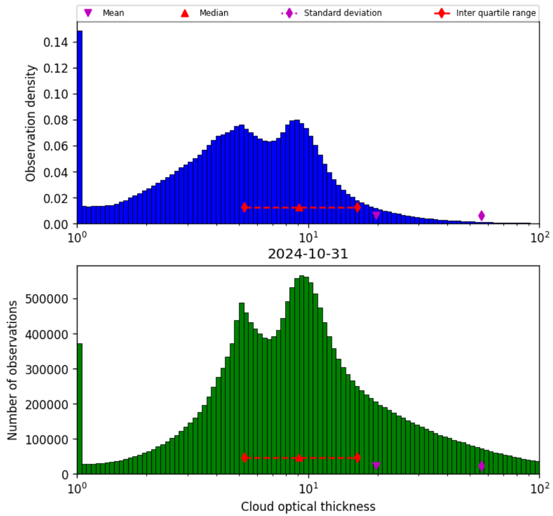
Figure 41: Histogram of “Cloud optical thickness” for 2024-10-30 to 2024-11-01
