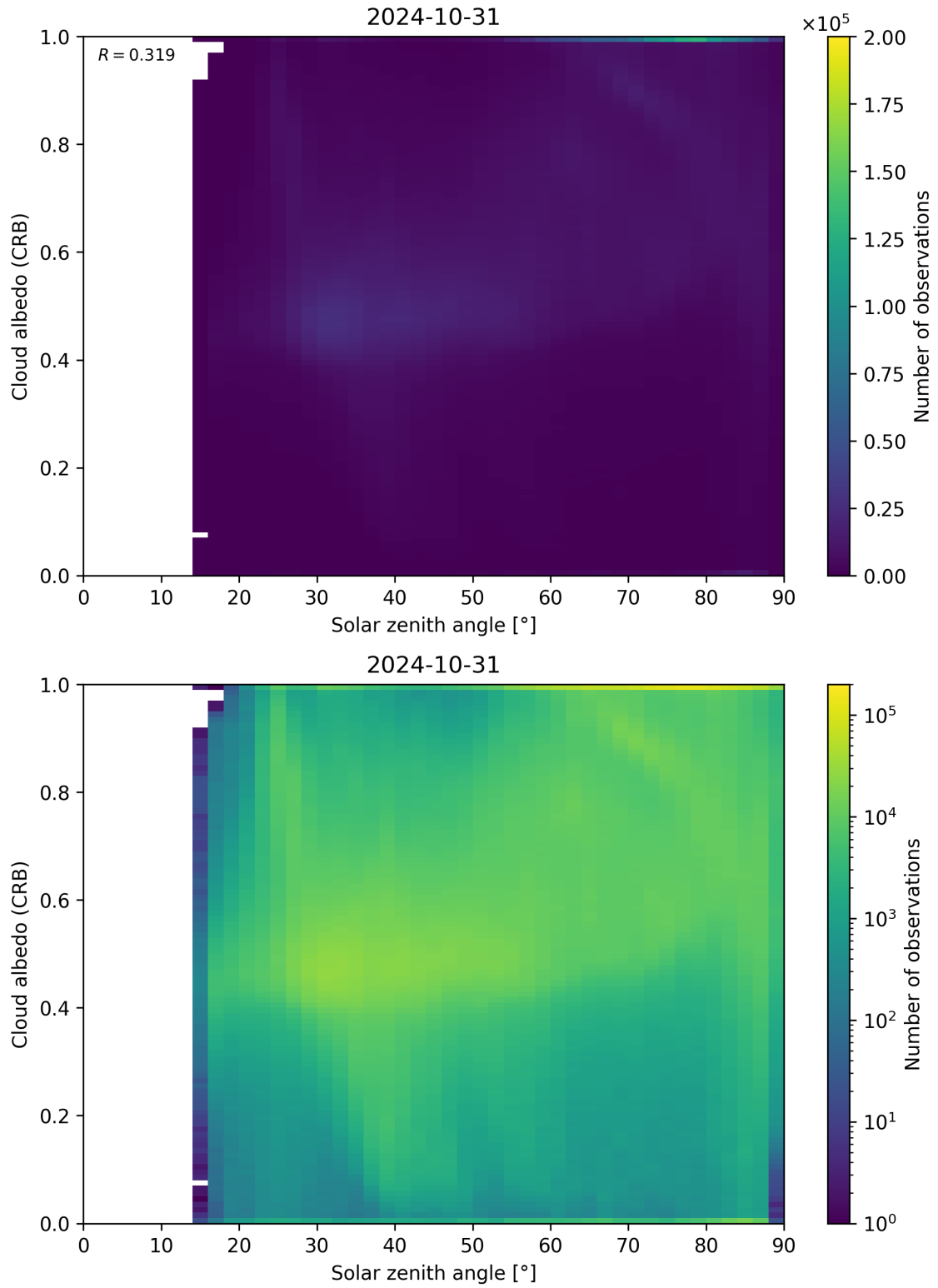
Figure 98: Scatter density plot of “Solar zenith angle” against “Cloud albedo (CRB)” for 2024-10-30 to 2024-11-01.
