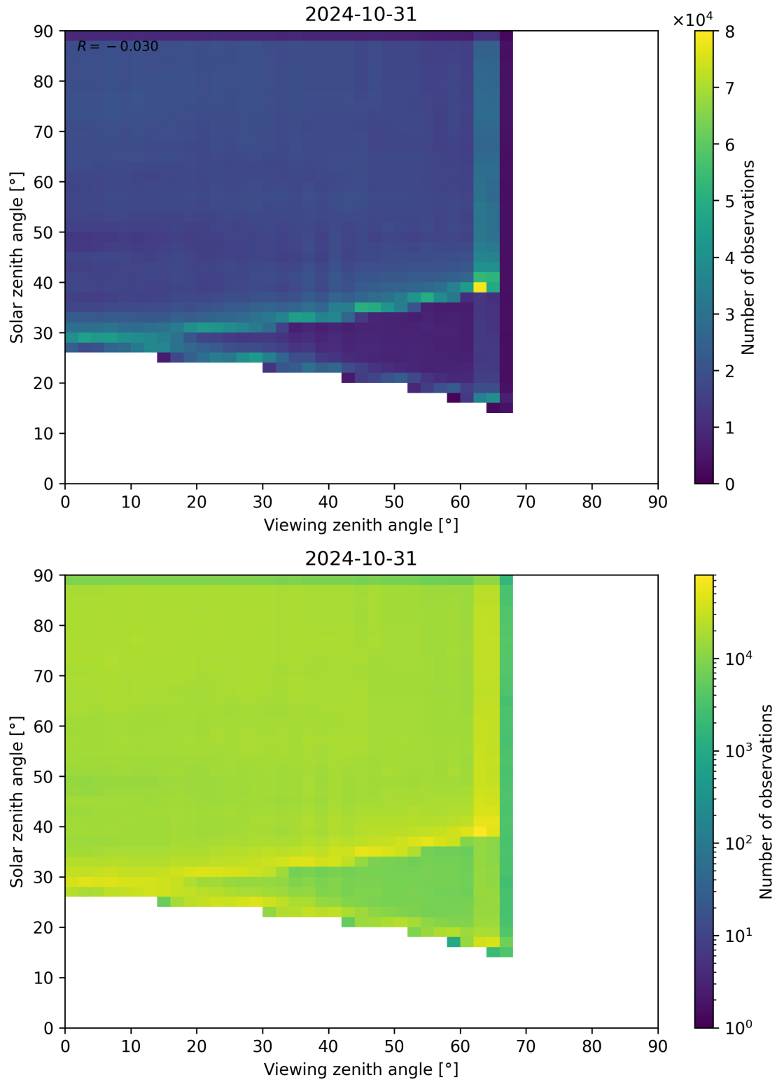
Figure 114: Scatter density plot of “Viewing zenith angle” against “Solar zenith angle” for 2024-10-30 to 2024-11-01.
