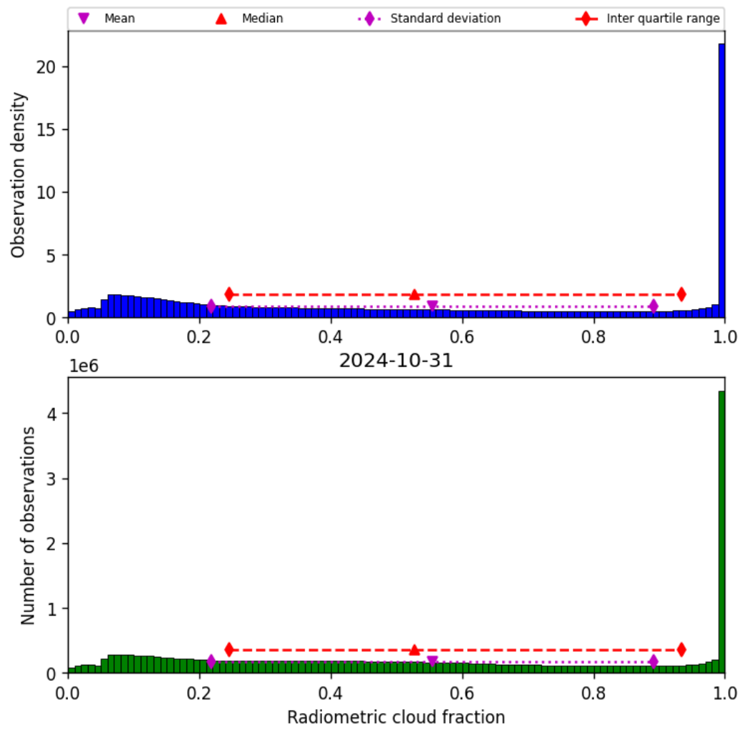
Figure 39: Histogram of “Radiometric cloud fraction” for 2024-10-30 to 2024-11-01
