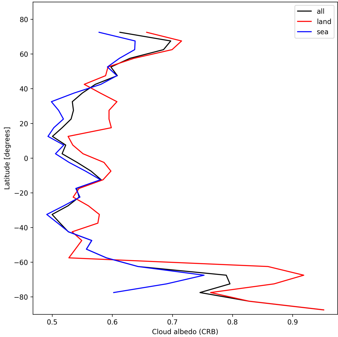
Figure 28: Zonal average of “Cloud albedo (CRB)” for 2024-10-30 to 2024-11-01.
