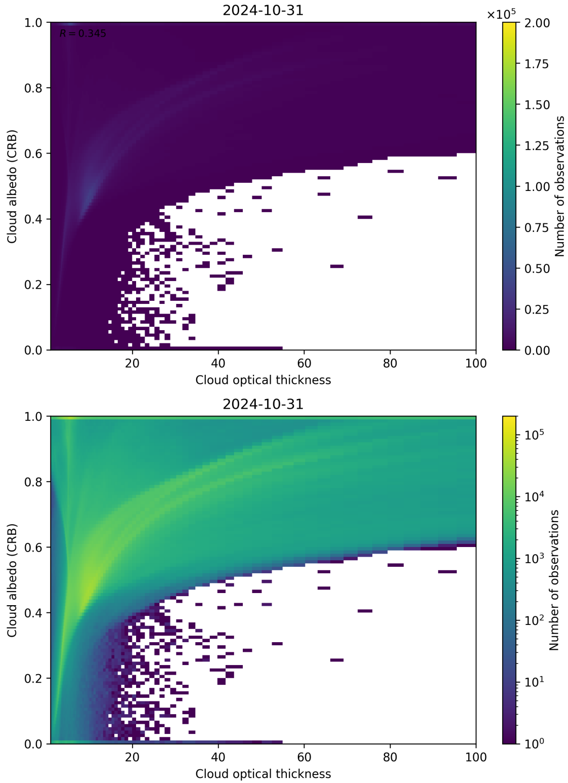
Figure 82: Scatter density plot of “Cloud optical thickness” against “Cloud albedo (CRB)” for 2024-10-30 to 2024-11-01.
