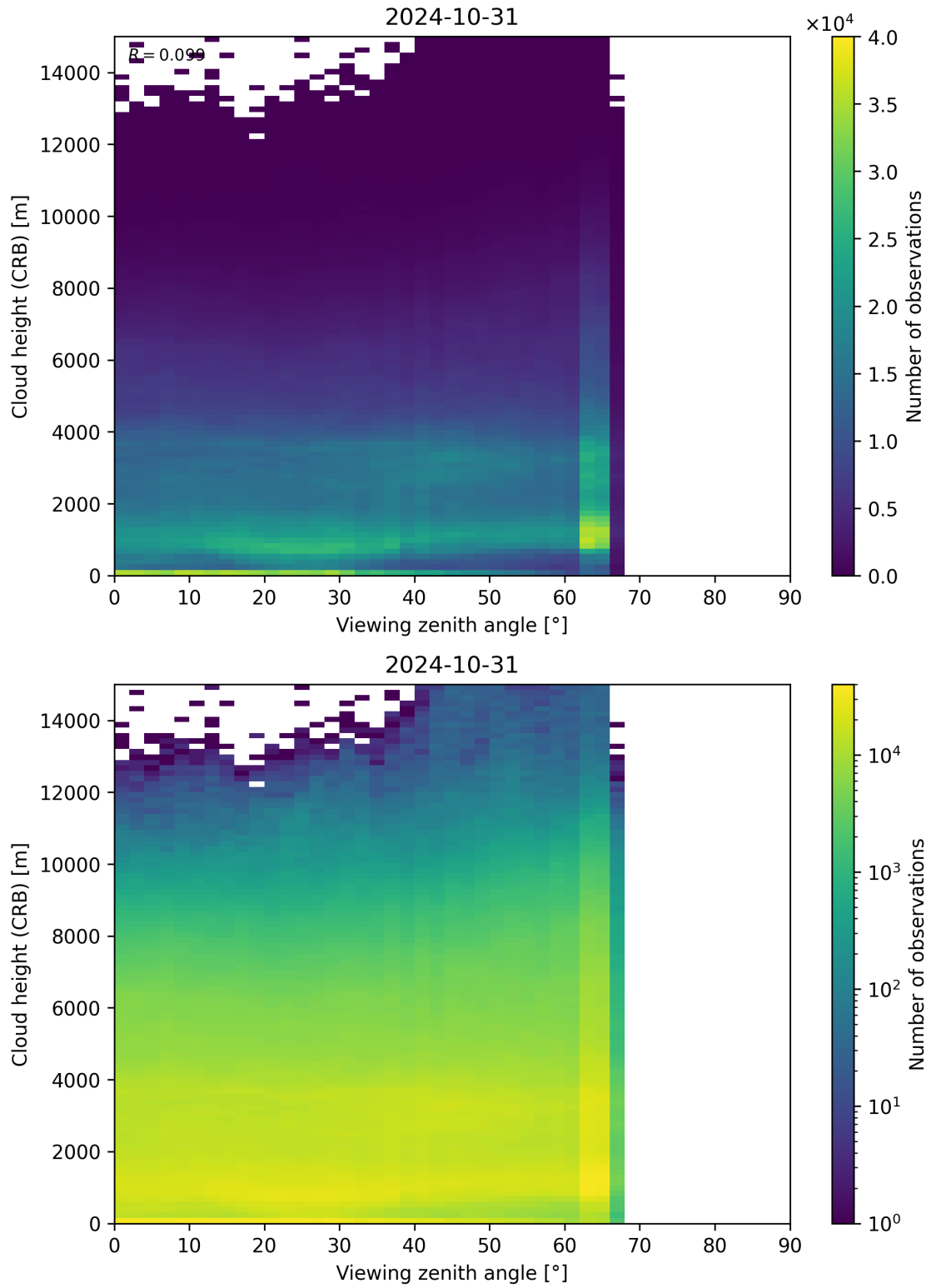
Figure 110: Scatter density plot of “Viewing zenith angle” against “Cloud height (CRB)” for 2024-10-30 to 2024-11-01.
