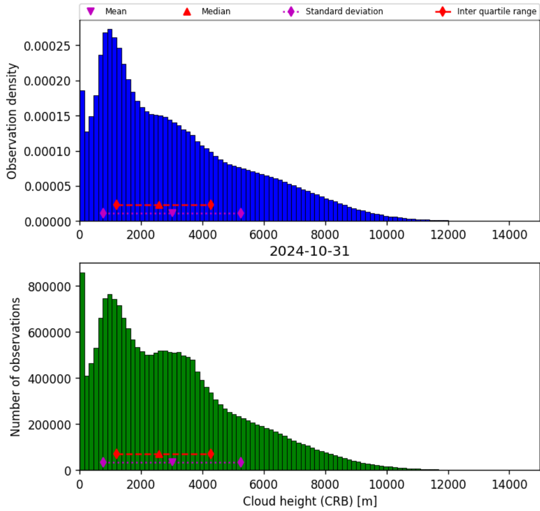
Figure 43: Histogram of “Cloud height (CRB)” for 2024-10-30 to 2024-11-01
