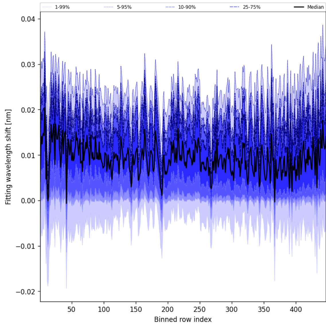
Figure 65: Along track statistics of “Fitting wavelength shift” for 2024-10-30 to 2024-11-01
