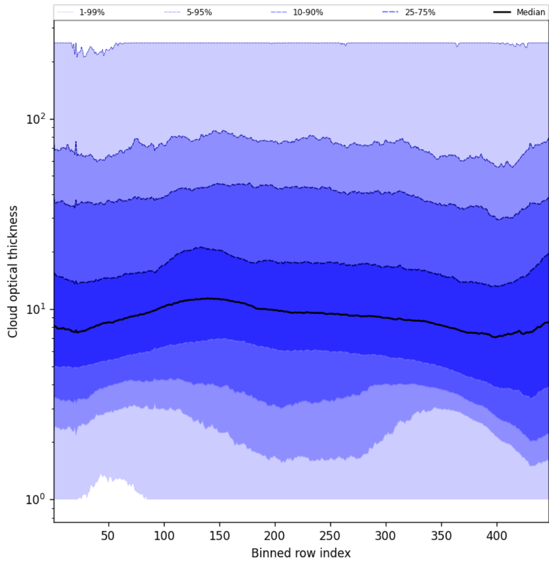
Figure 57: Along track statistics of “Cloud optical thickness” for 2024-10-30 to 2024-11-01
