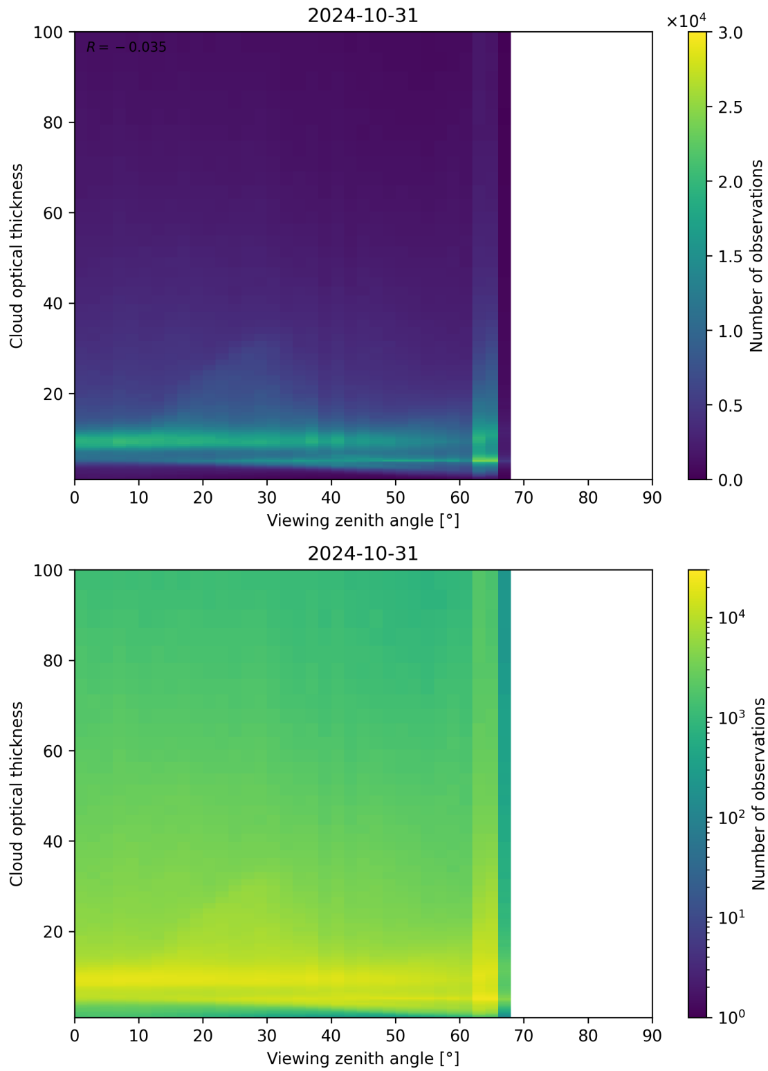
Figure 111: Scatter density plot of “Viewing zenith angle” against “Cloud optical thickness” for 2024-10-30 to 2024-11-01.
