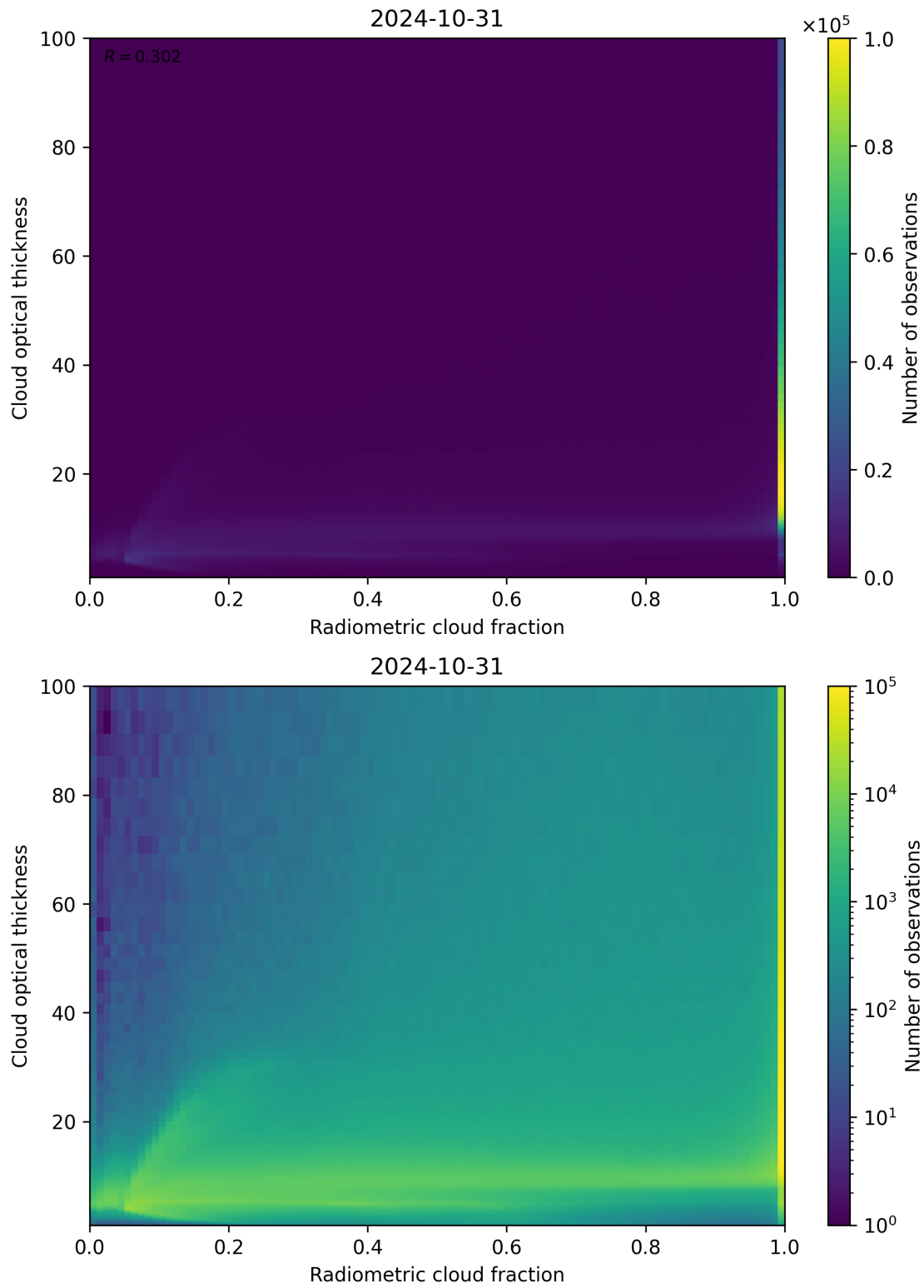
Figure 75: Scatter density plot of “Radiometric cloud fraction” against “Cloud optical thickness” for 2024-10-30 to 2024-11-01.
