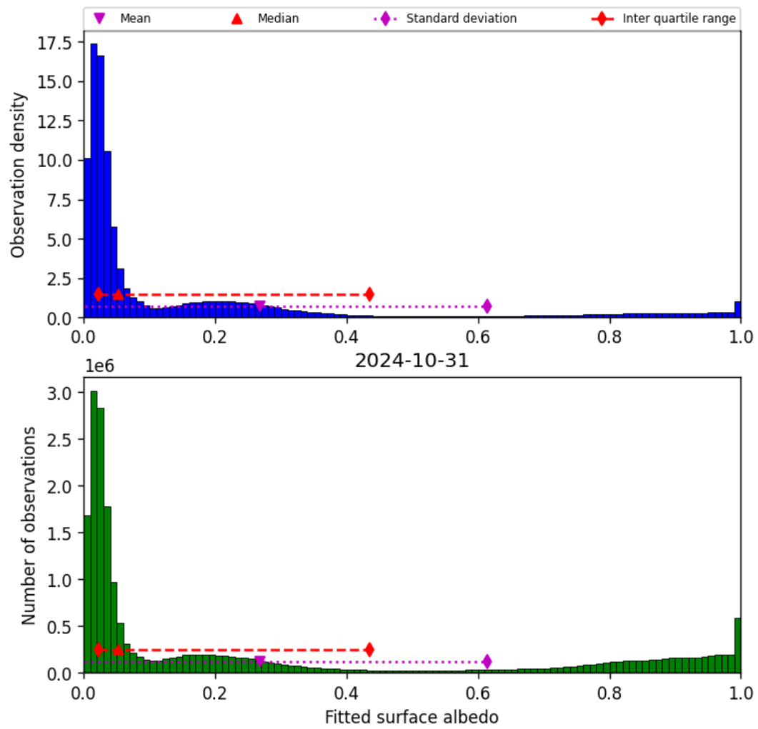
Figure 45: Histogram of “Fitted surface albedo” for 2024-10-30 to 2024-11-01
