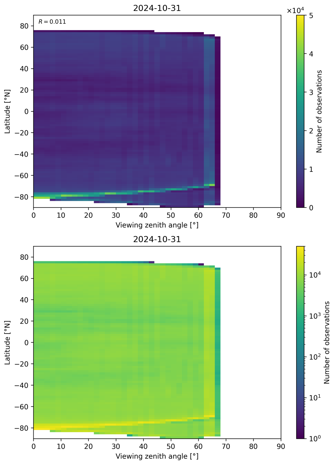
Figure 113: Scatter density plot of “Viewing zenith angle” against “Latitude” for 2024-10-30 to 2024-11-01.
