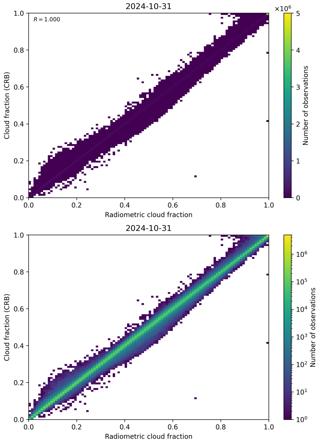
Figure 73: Scatter density plot of “Radiometric cloud fraction” against “Cloud fraction (CRB)” for 2024-10-30 to 2024-11-01.
