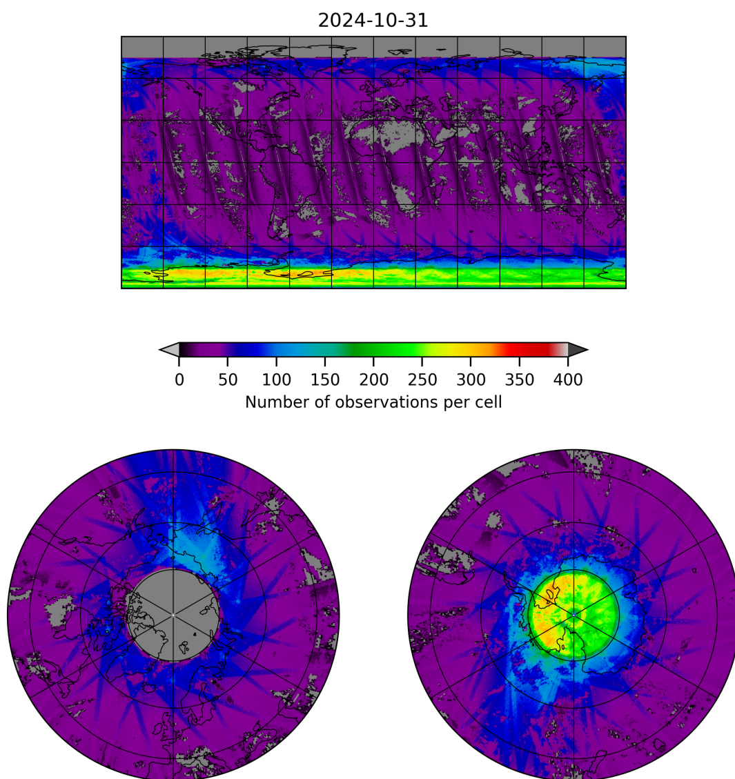
Figure 21: Map of the number of observations for 2024-10-30 to 2024-11-01
