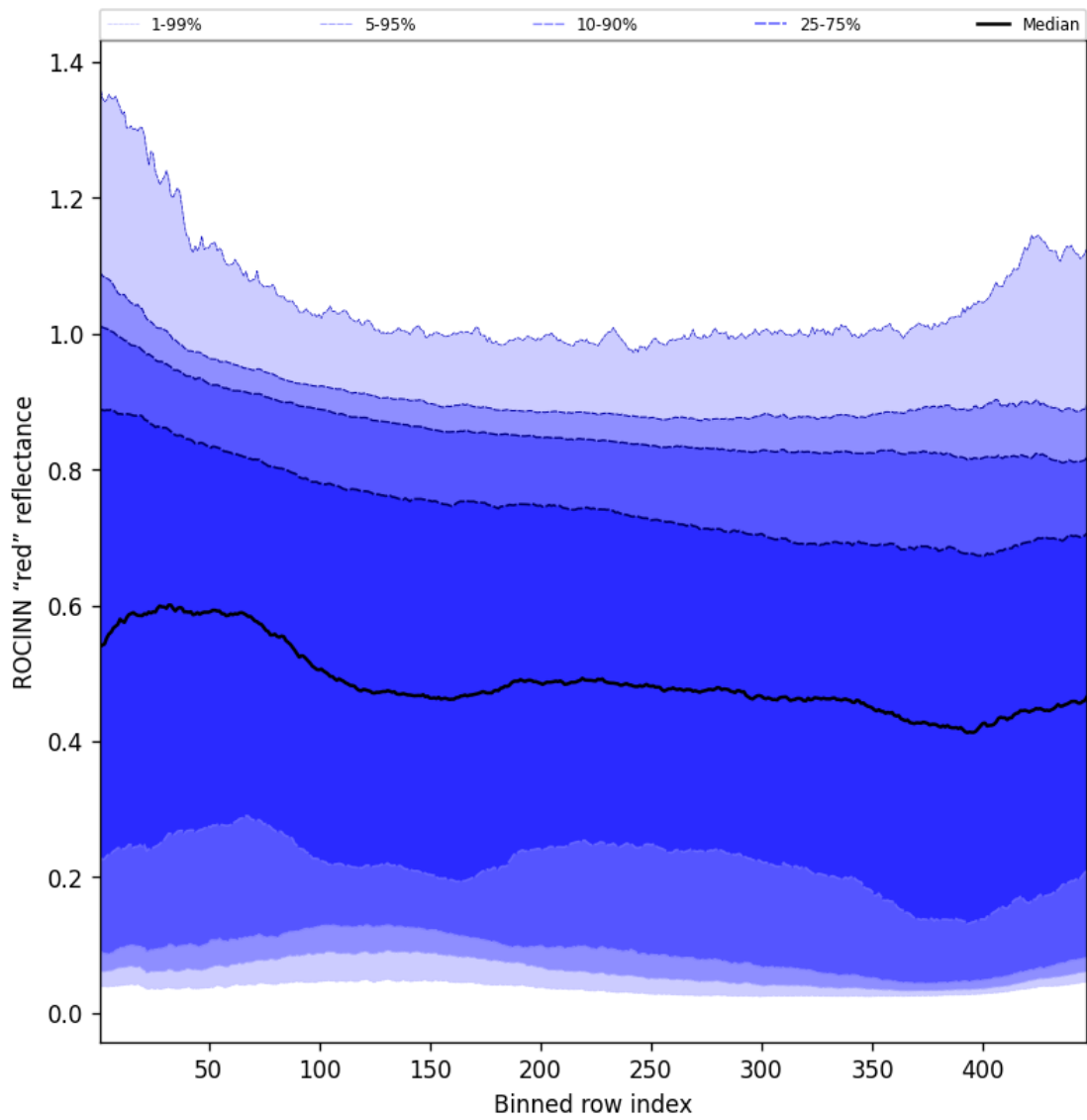
Figure 69: Along track statistics of “ROCINN “red” reflectance” for 2024-10-30 to 2024-11-01
