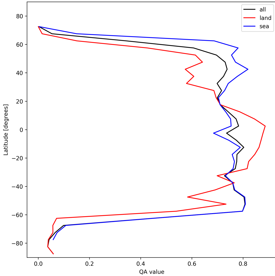
Figure 22: Zonal average of “QA value” for 2024-10-30 to 2024-11-01.
