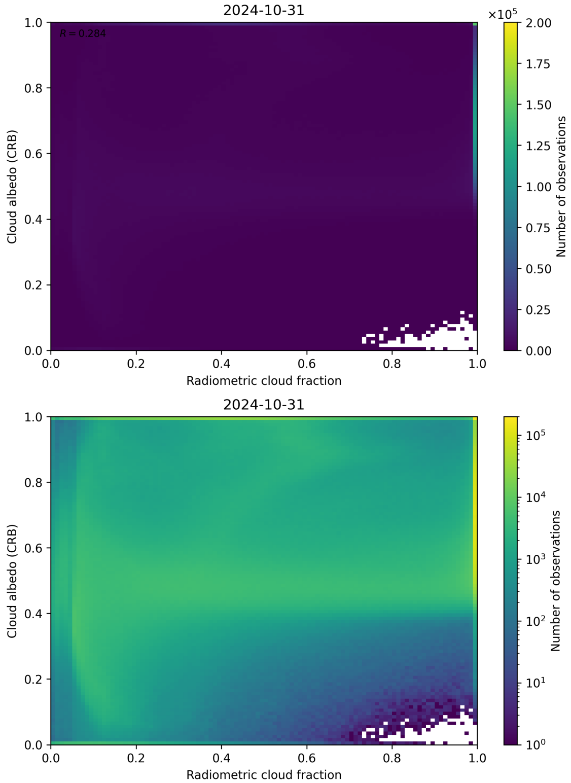
Figure 71: Scatter density plot of “Radiometric cloud fraction” against “Cloud albedo (CRB)” for 2024-10-30 to 2024-11-01.
