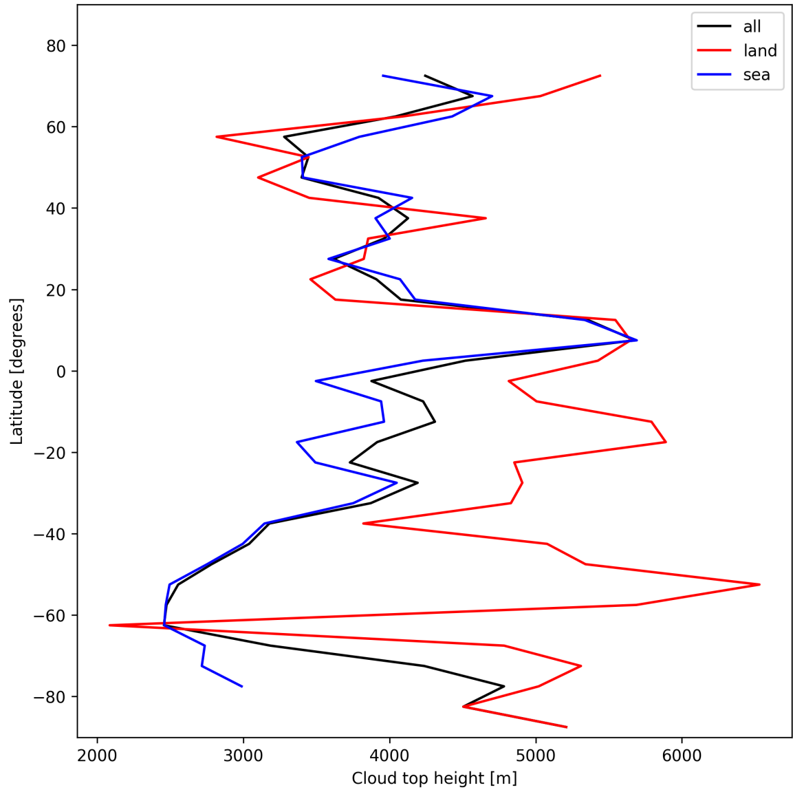
Figure 24: Zonal average of “Cloud top height” for 2024-10-30 to 2024-11-01.
