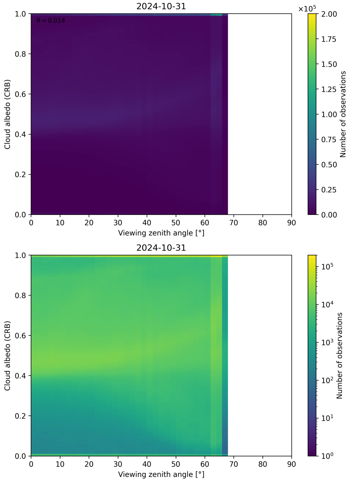
Figure 106: Scatter density plot of “Viewing zenith angle” against “Cloud albedo (CRB)” for 2024-10-30 to 2024-11-01.
