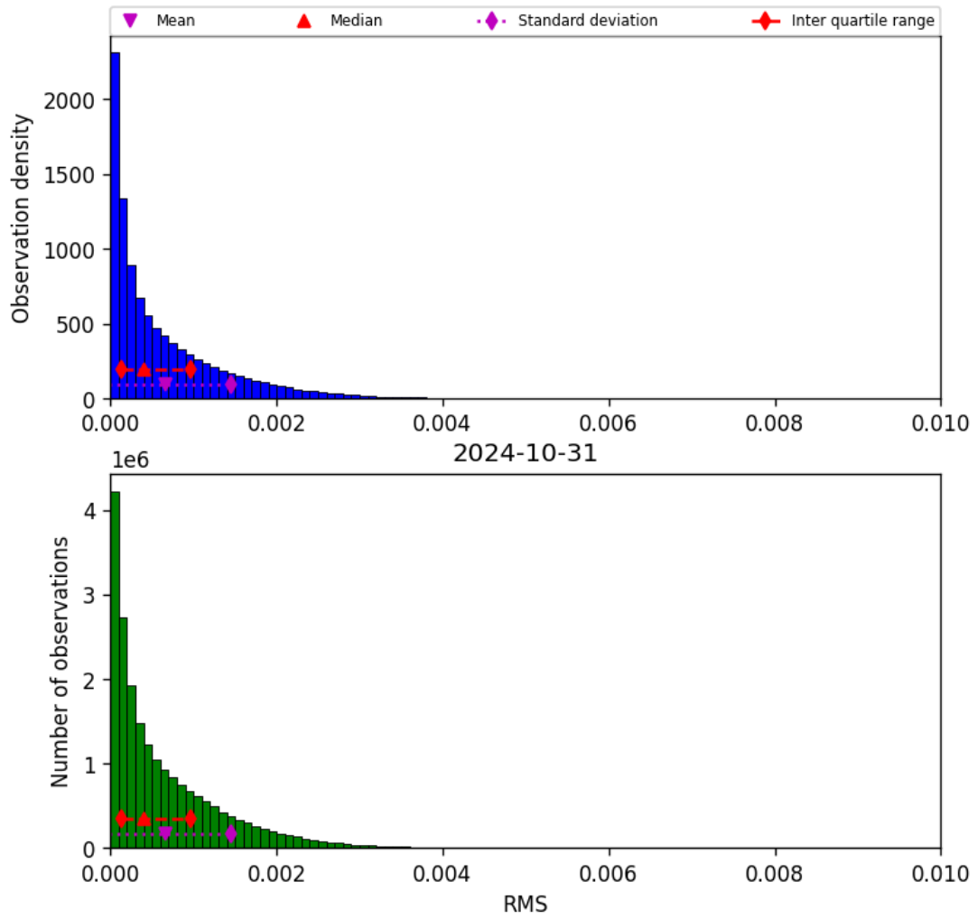
Figure 47: Histogram of “RMS” for 2024-10-30 to 2024-11-01
