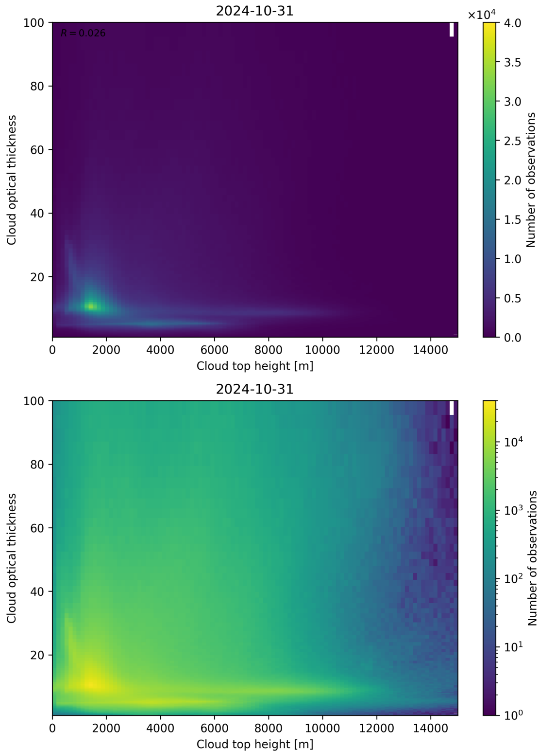
Figure 90: Scatter density plot of “Cloud top height” against “Cloud optical thickness” for 2024-10-30 to 2024-11-01.
