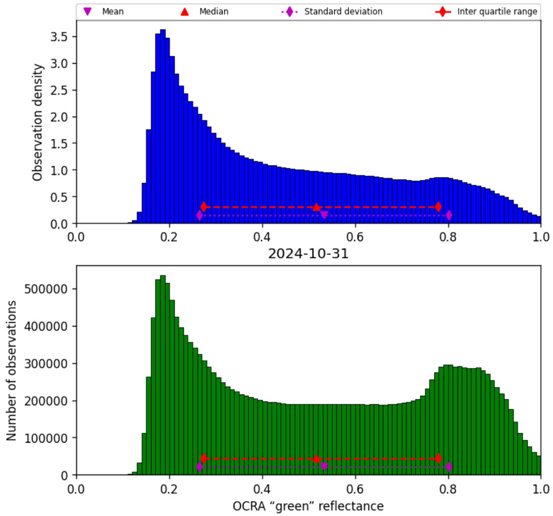
Figure 52: Histogram of “OCRA “green” reflectance” for 2024-10-30 to 2024-11-01
