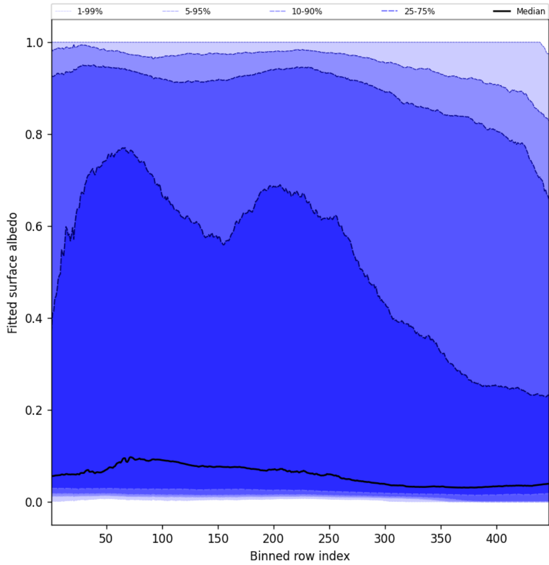
Figure 61: Along track statistics of “Fitted surface albedo” for 2024-10-30 to 2024-11-01
