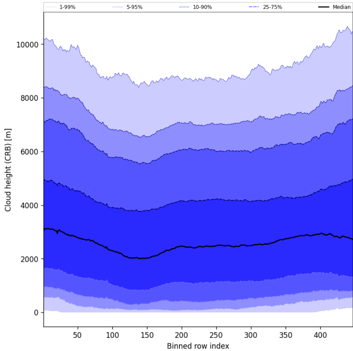
Figure 59: Along track statistics of “Cloud height (CRB)” for 2024-10-30 to 2024-11-01
