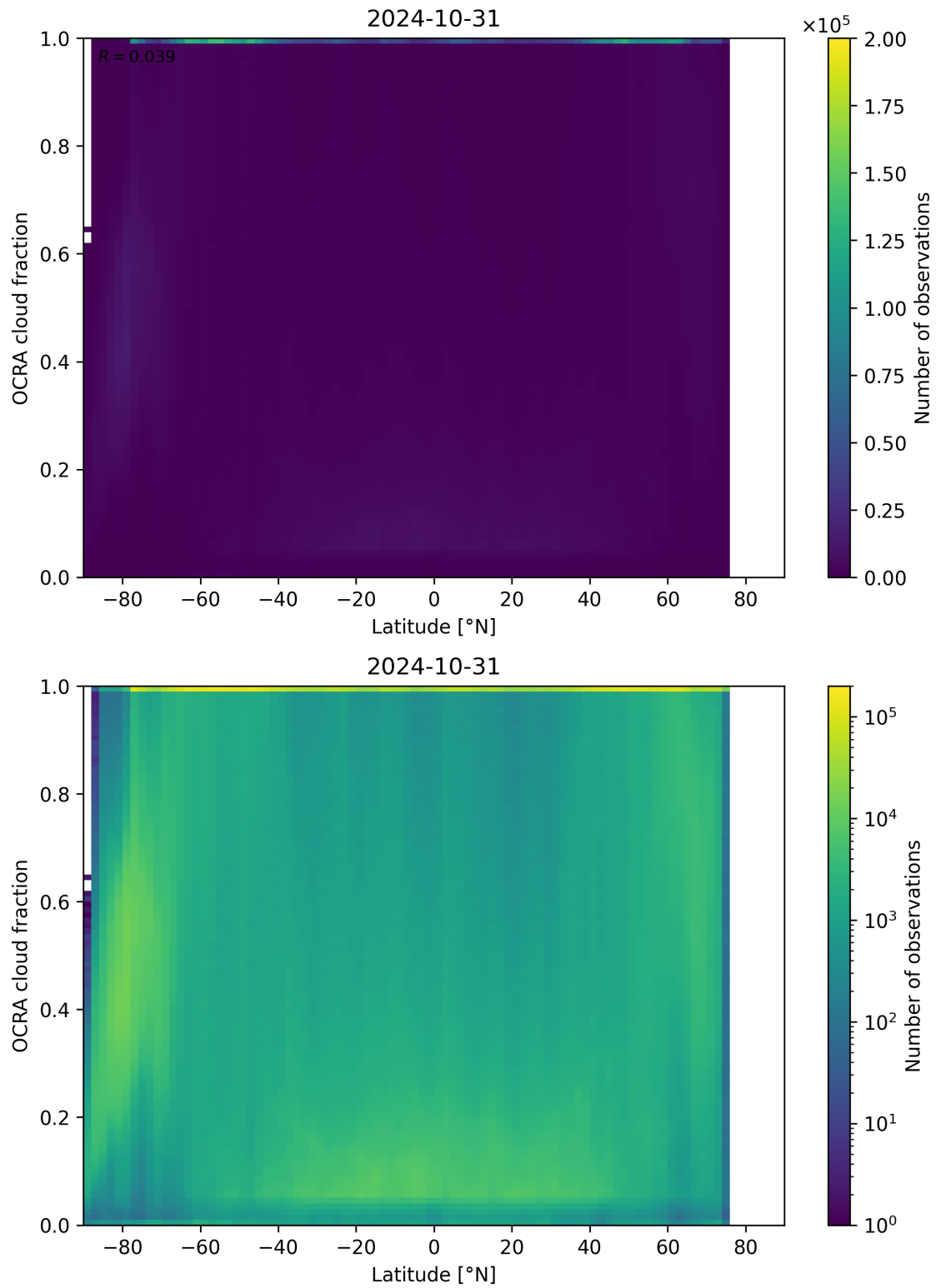
Figure 93: Scatter density plot of “Latitude” against “OCRA cloud fraction” for 2024-10-30 to 2024-11-01.
