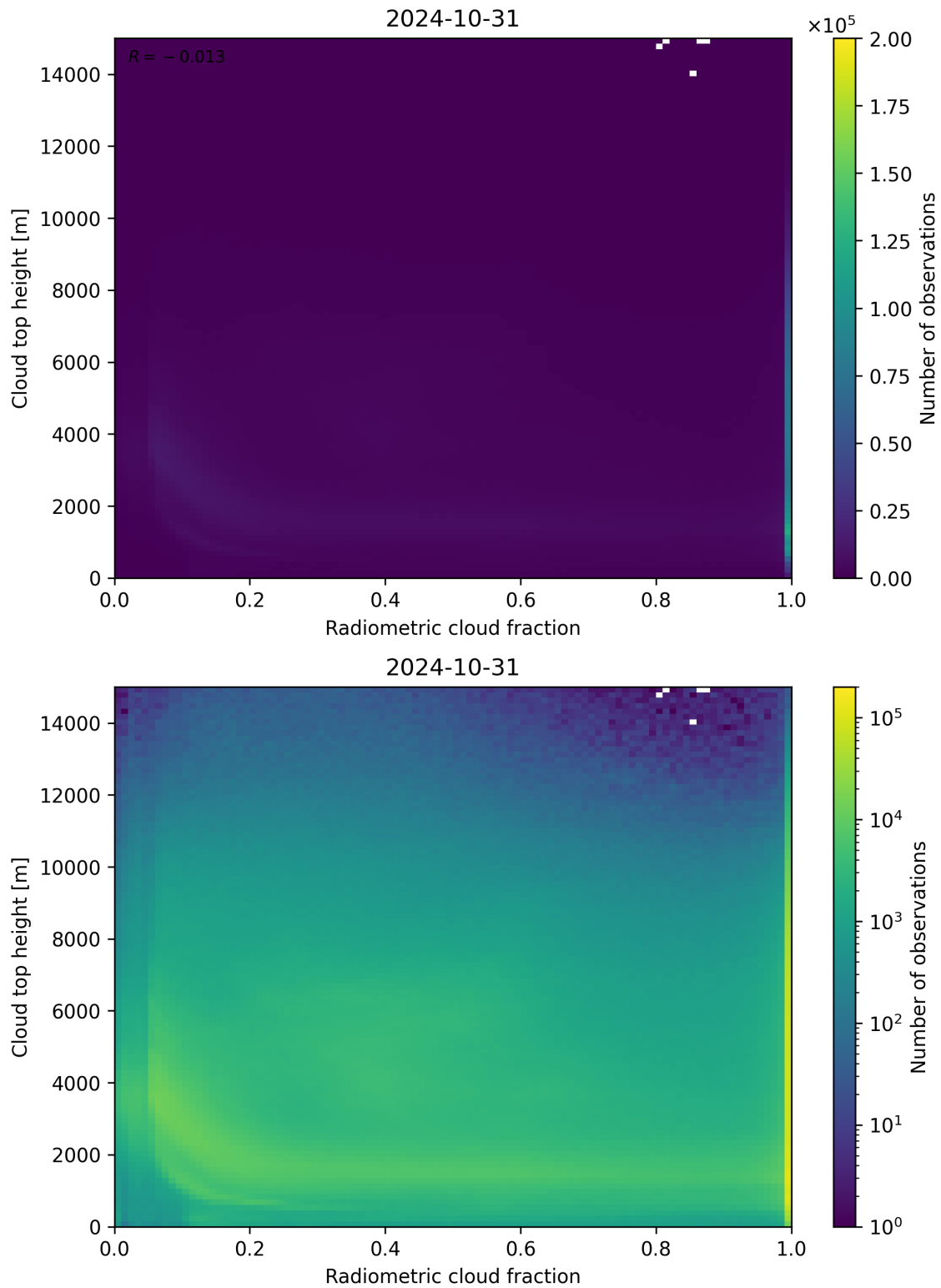
Figure 76: Scatter density plot of “Radiometric cloud fraction” against “Cloud top height” for 2024-10-30 to 2024-11-01.
