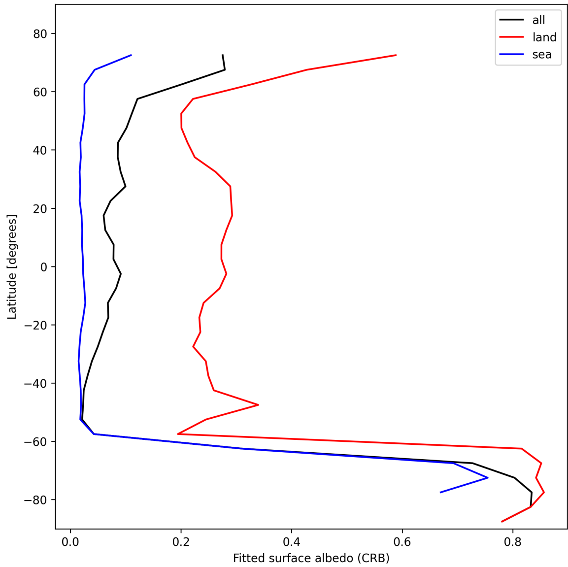
Figure 30: Zonal average of “Fitted surface albedo (CRB)” for 2024-10-30 to 2024-11-01.
