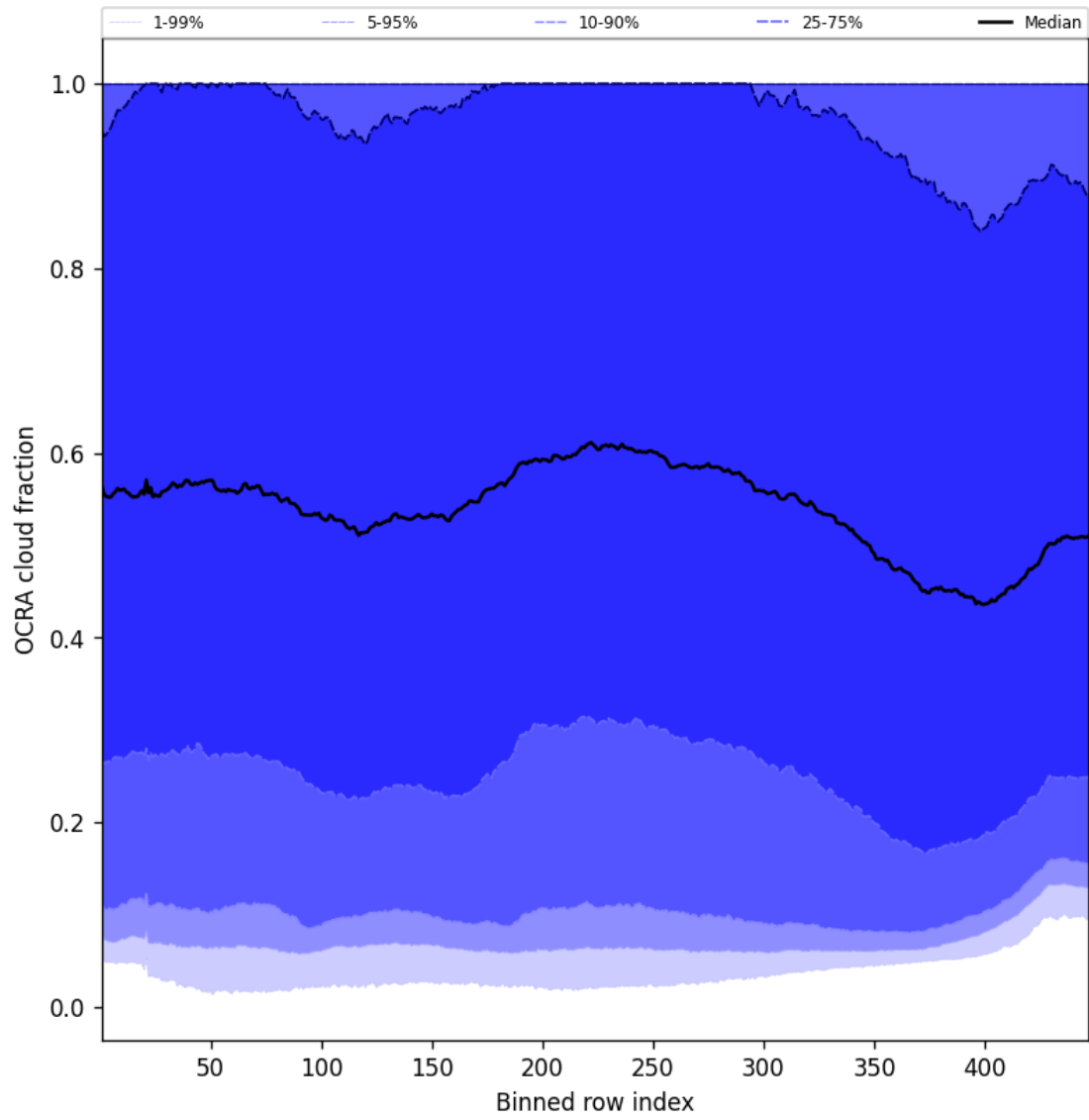
Figure 66: Along track statistics of “OCRA cloud fraction” for 2024-10-30 to 2024-11-01
