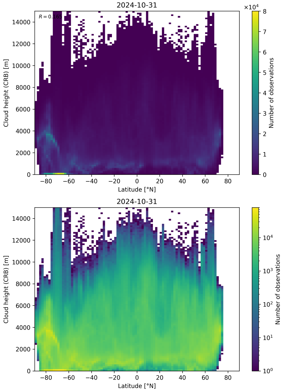
Figure 95: Scatter density plot of “Latitude” against “Cloud height (CRB)” for 2024-10-30 to 2024-11-01.
