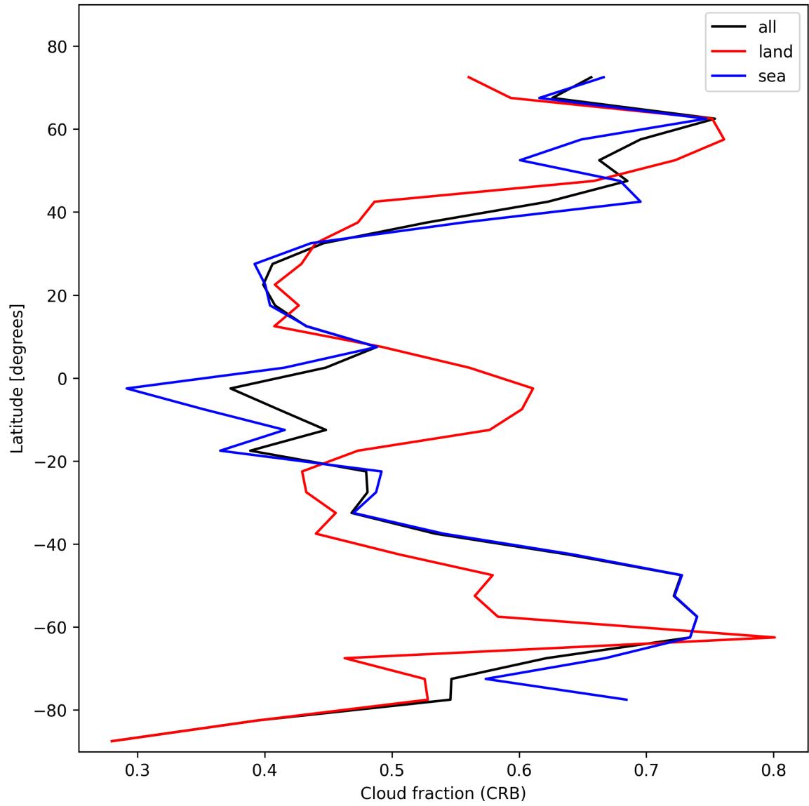
Figure 26: Zonal average of “Cloud fraction (CRB)” for 2024-10-30 to 2024-11-01.
