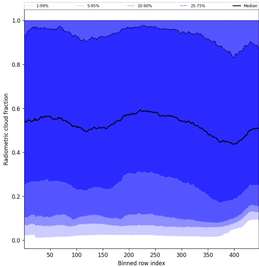
Figure 55: Along track statistics of “Radiometric cloud fraction” for 2024-10-30 to 2024-11-01
