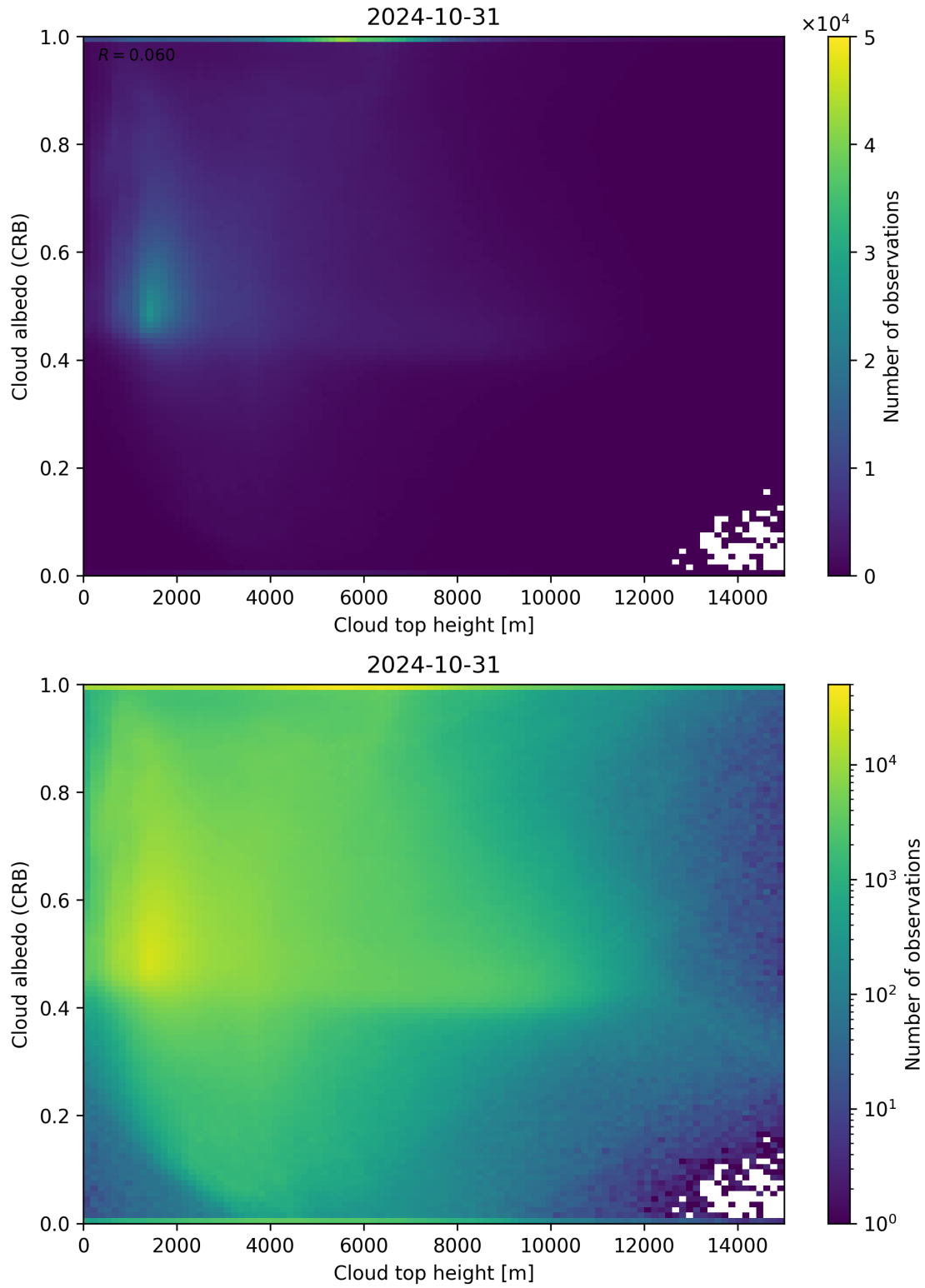
Figure 86: Scatter density plot of “Cloud top height” against “Cloud albedo (CRB)” for 2024-10-30 to 2024-11-01.
