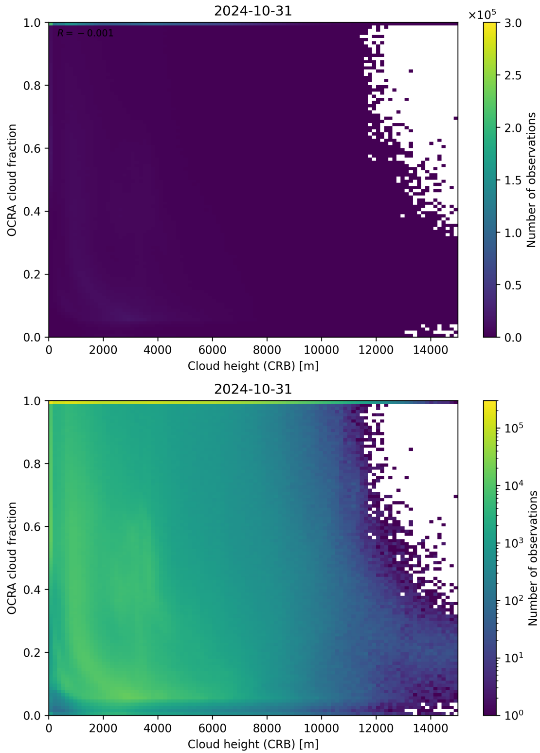
Figure 81: Scatter density plot of “Cloud height (CRB)” against “OCRA cloud fraction” for 2024-10-30 to 2024-11-01.
