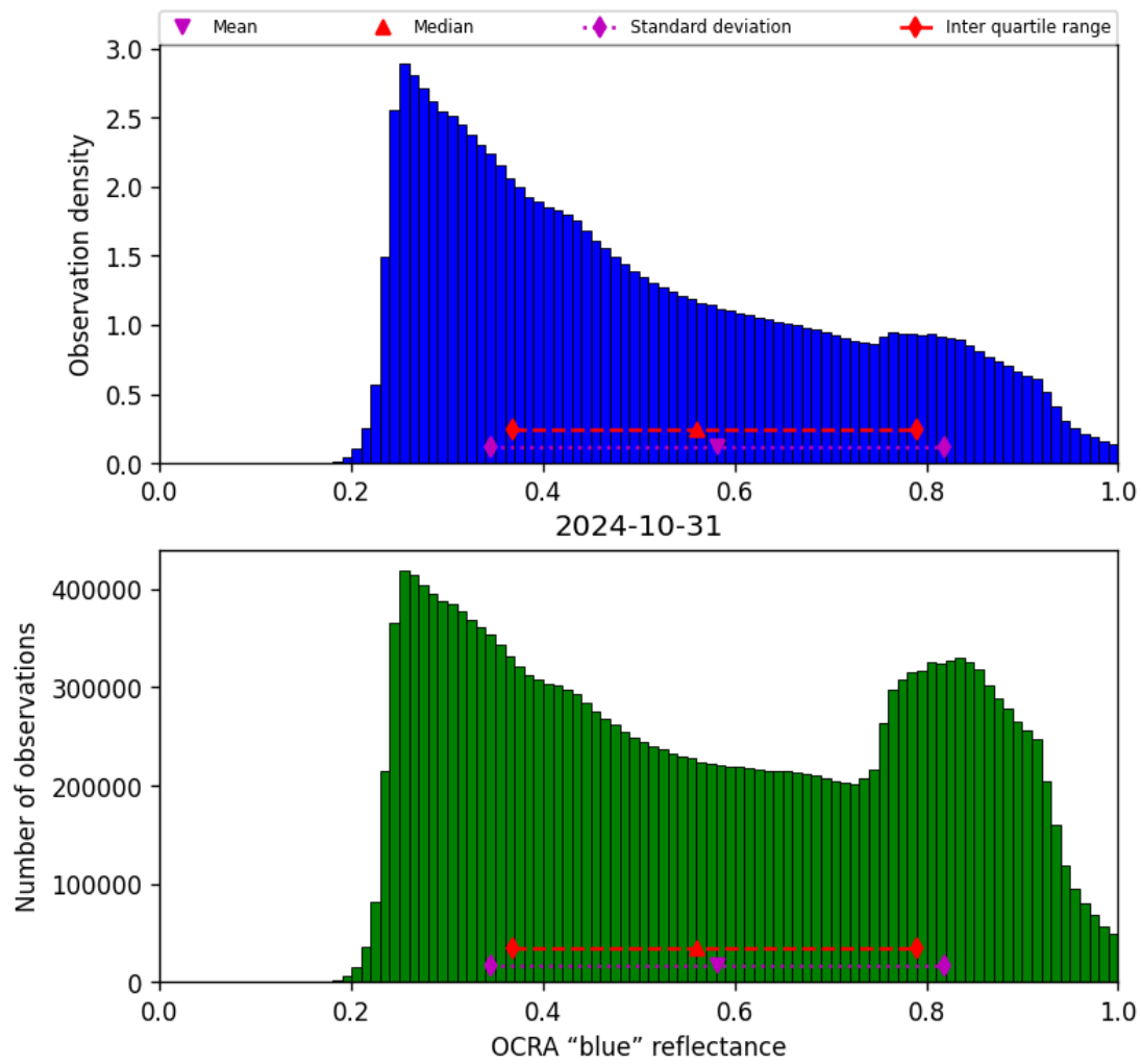
Figure 51: Histogram of “OCRA “blue” reflectance” for 2024-10-30 to 2024-11-01
