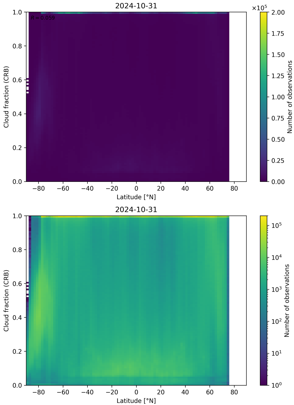
Figure 94: Scatter density plot of “Latitude” against “Cloud fraction (CRB)” for 2024-10-30 to 2024-11-01.
