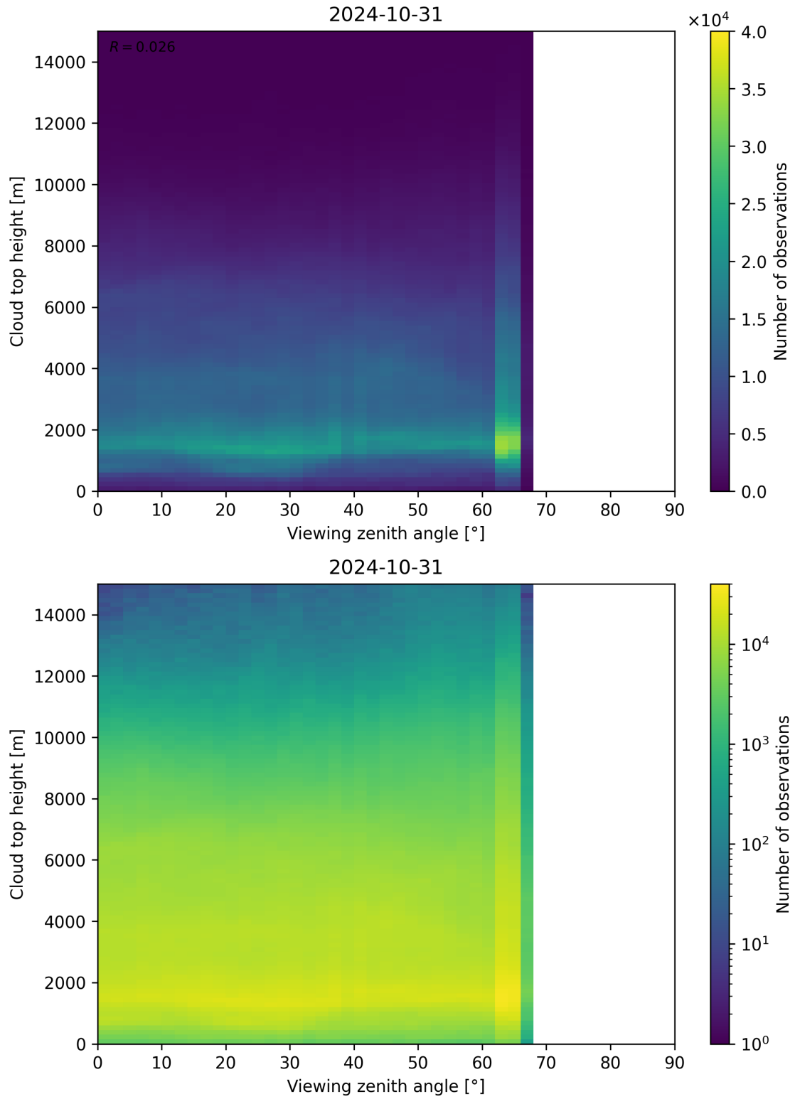
Figure 112: Scatter density plot of “Viewing zenith angle” against “Cloud top height” for 2024-10-30 to 2024-11-01.
