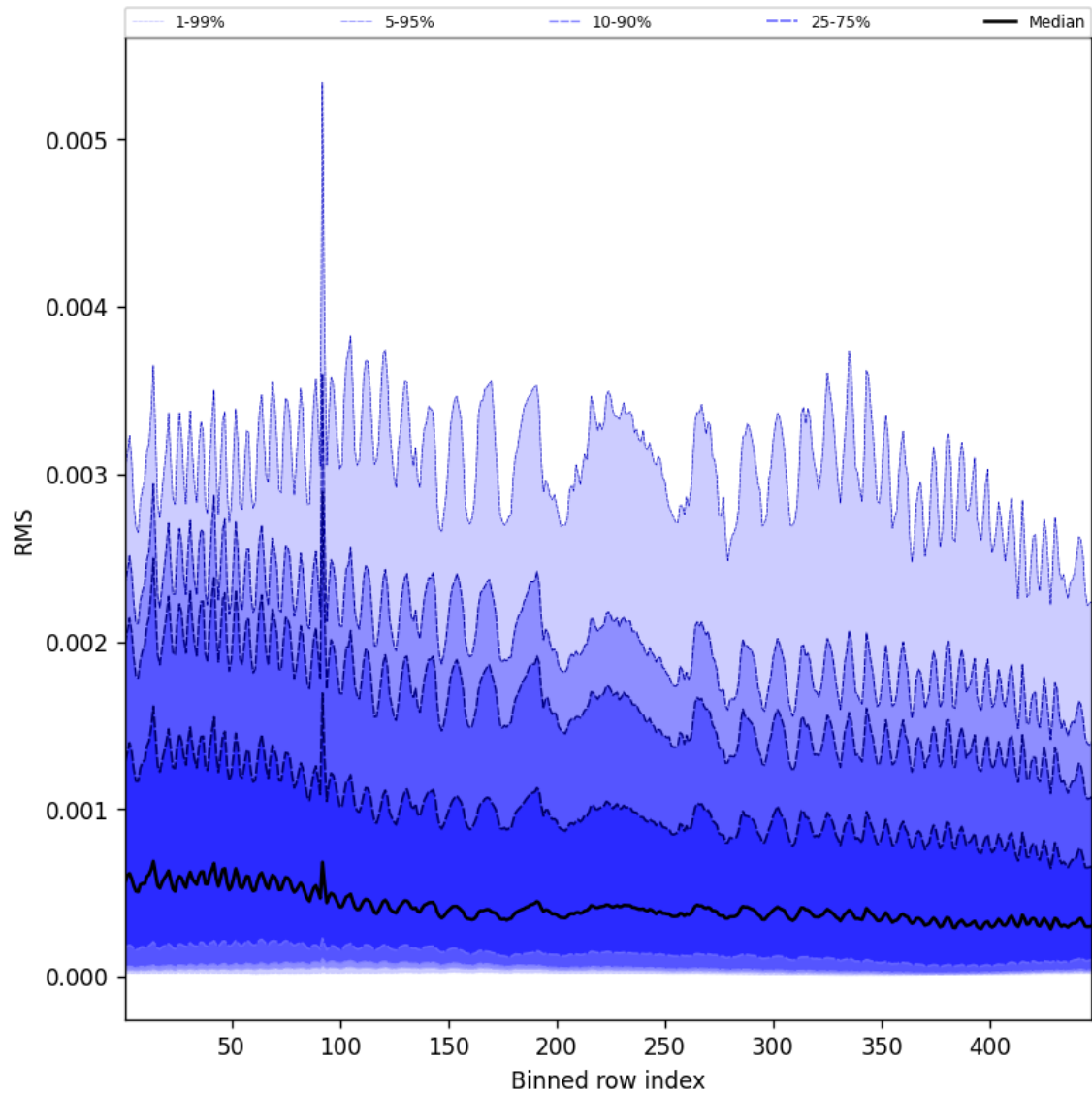
Figure 63: Along track statistics of “RMS” for 2024-10-30 to 2024-11-01
