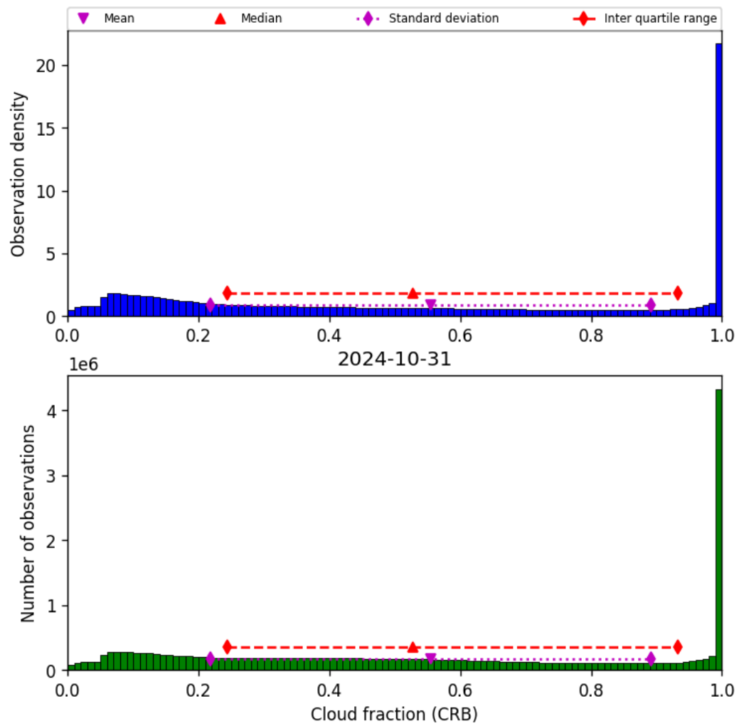
Figure 42: Histogram of “Cloud fraction (CRB)” for 2024-10-30 to 2024-11-01
