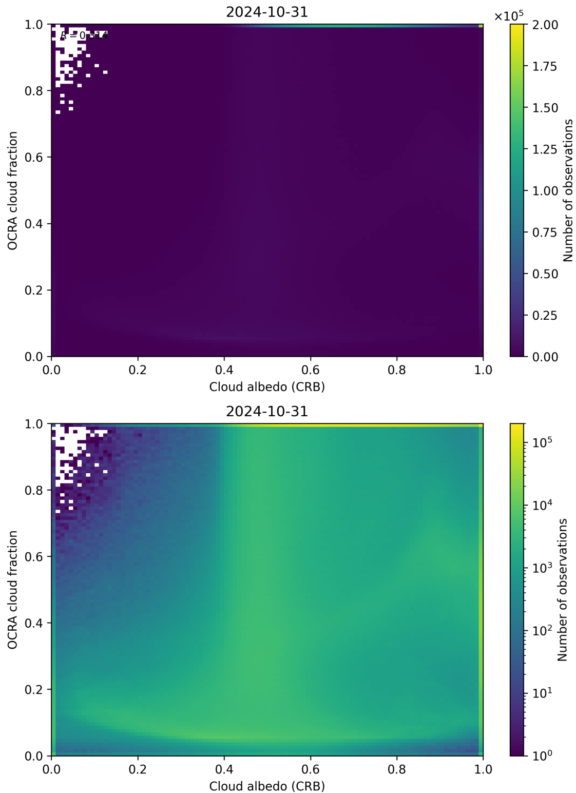
Figure 70: Scatter density plot of “Cloud albedo (CRB)” against “OCRA cloud fraction” for 2024-10-30 to 2024-11-01.
