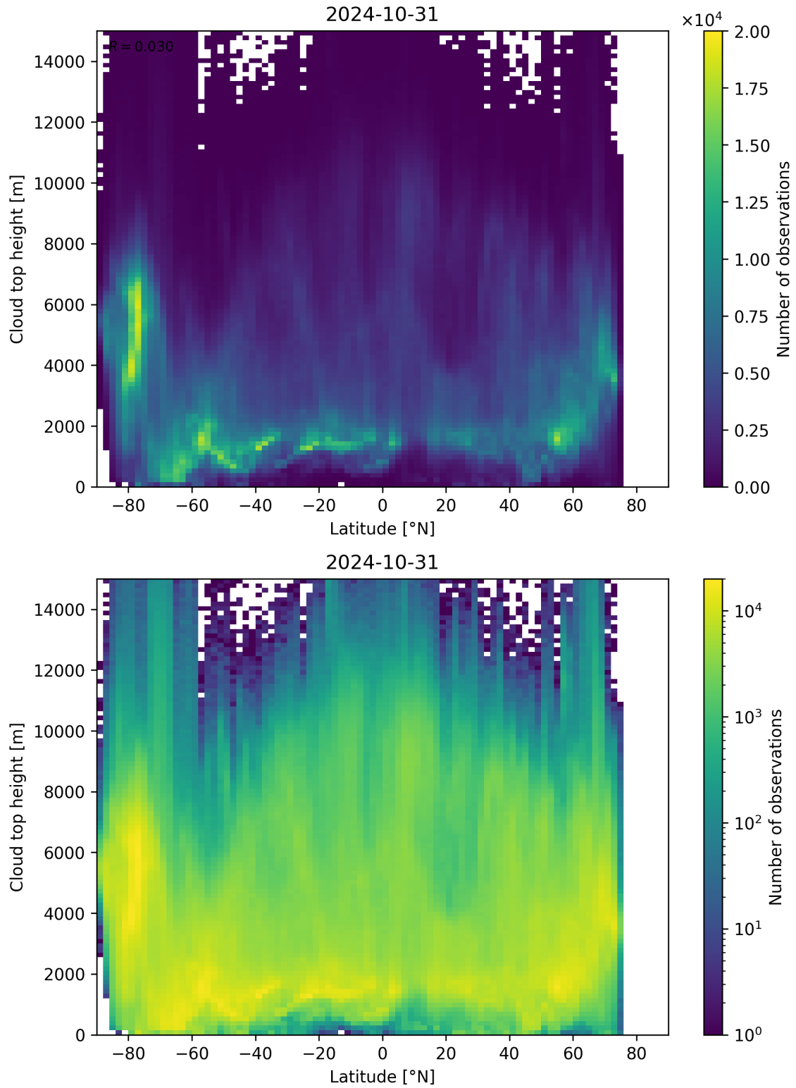
Figure 97: Scatter density plot of “Latitude” against “Cloud top height” for 2024-10-30 to 2024-11-01.
