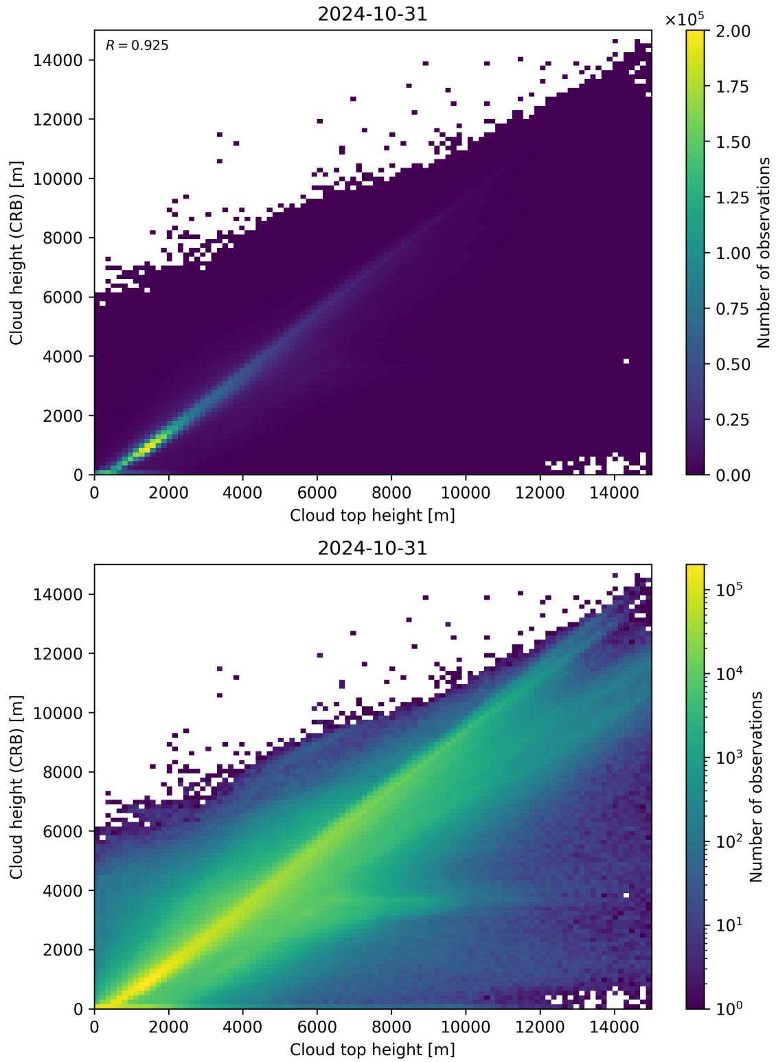
Figure 89: Scatter density plot of “Cloud top height” against “Cloud height (CRB)” for 2024-10-30 to 2024-11-01.
