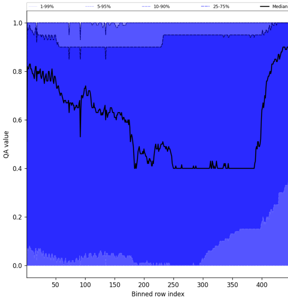
Figure 54: Along track statistics of “QA value” for 2024-10-30 to 2024-11-01
