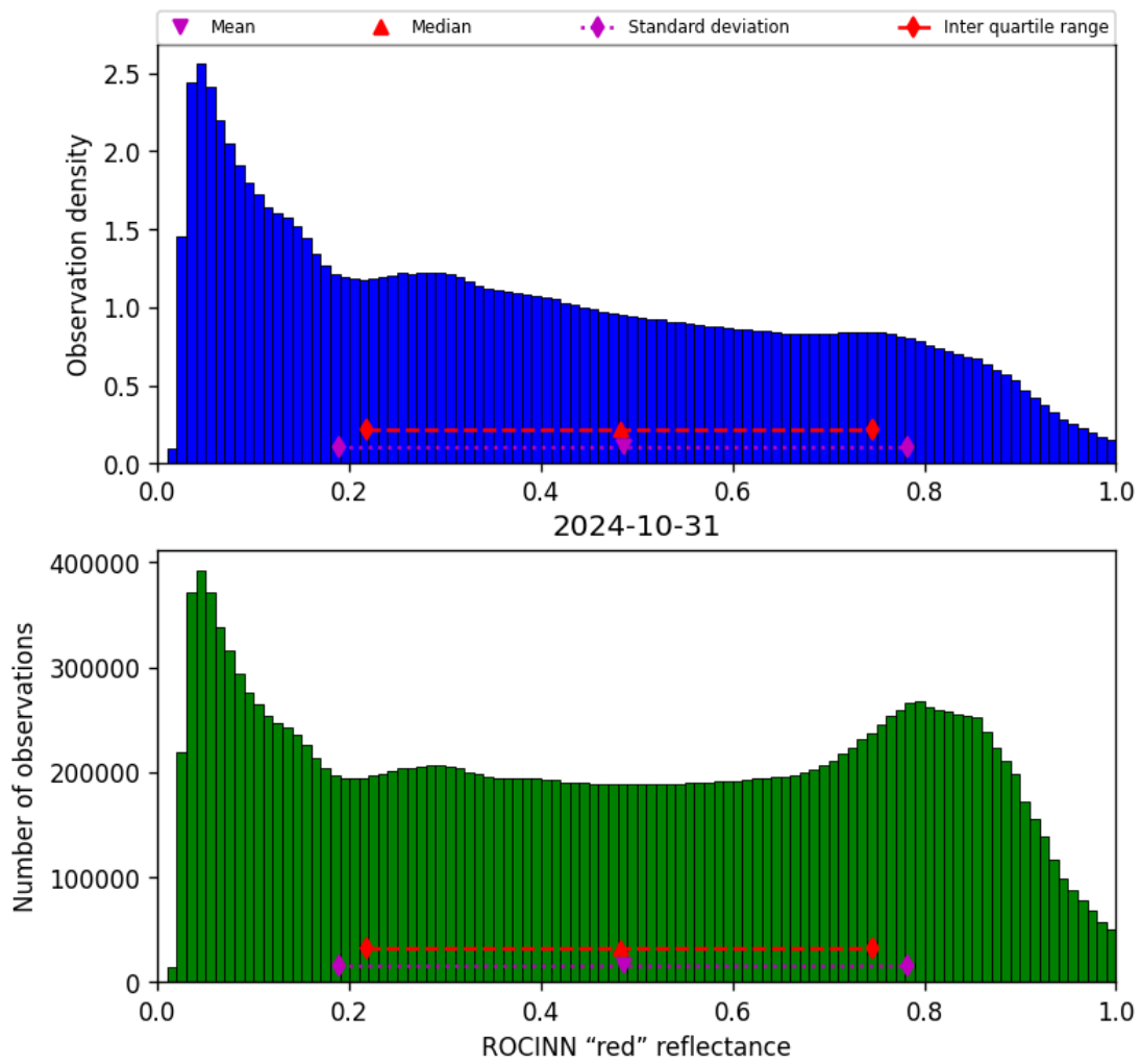
Figure 53: Histogram of “ROCINN “red” reflectance” for 2024-10-30 to 2024-11-01
