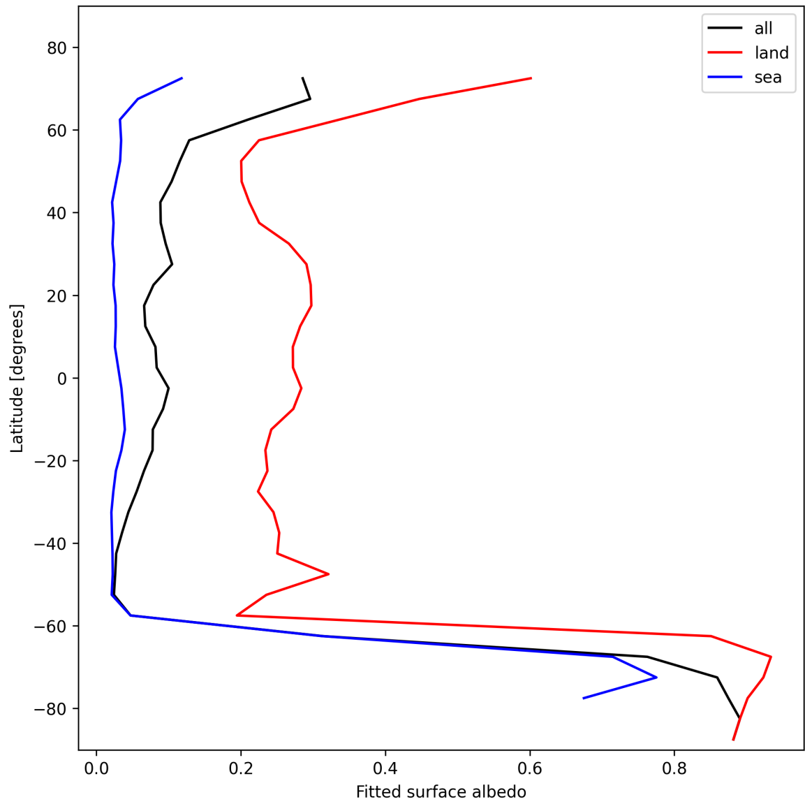
Figure 29: Zonal average of “Fitted surface albedo” for 2024-10-30 to 2024-11-01.
