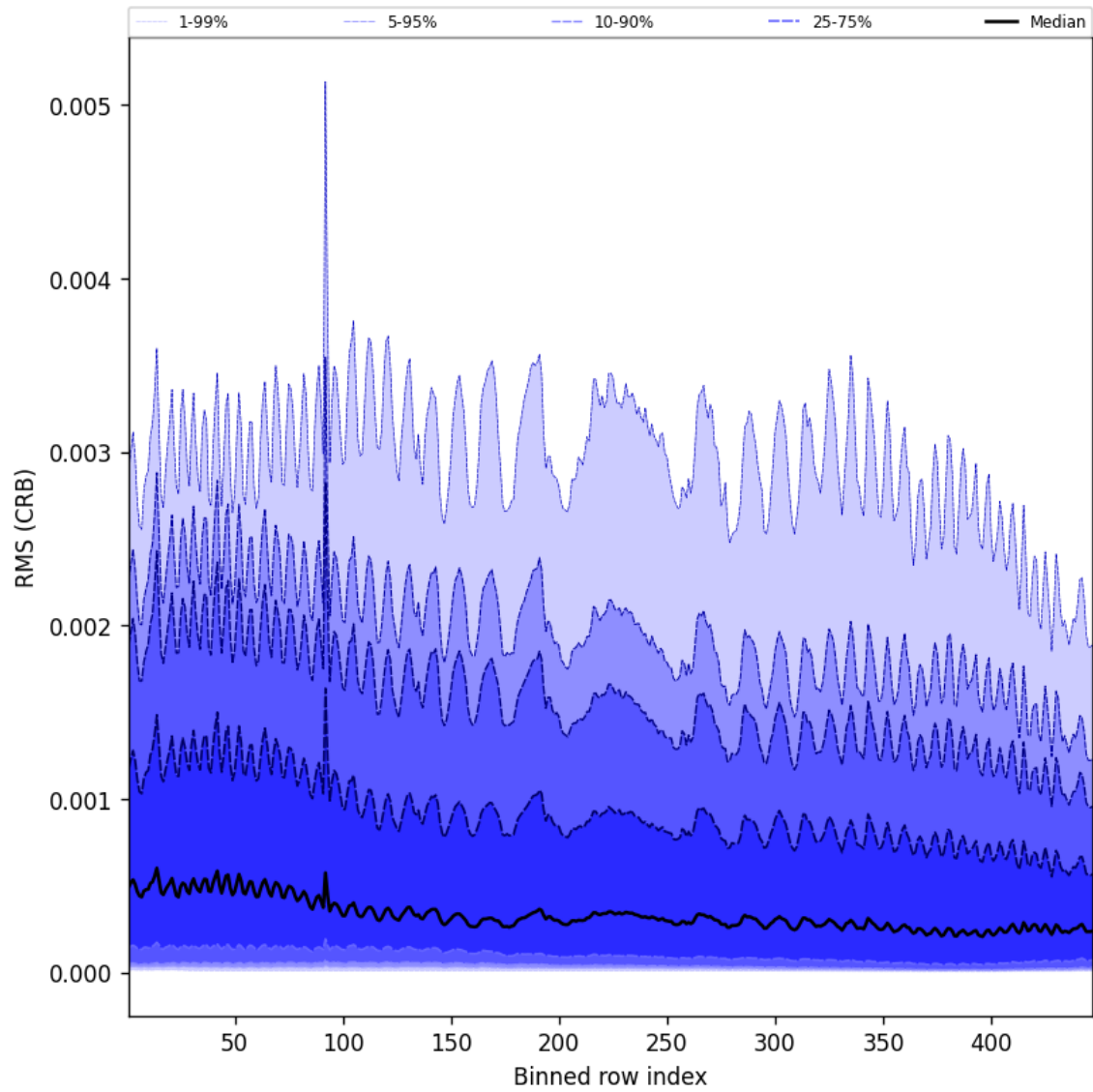
Figure 64: Along track statistics of “RMS (CRB)” for 2024-10-30 to 2024-11-01
