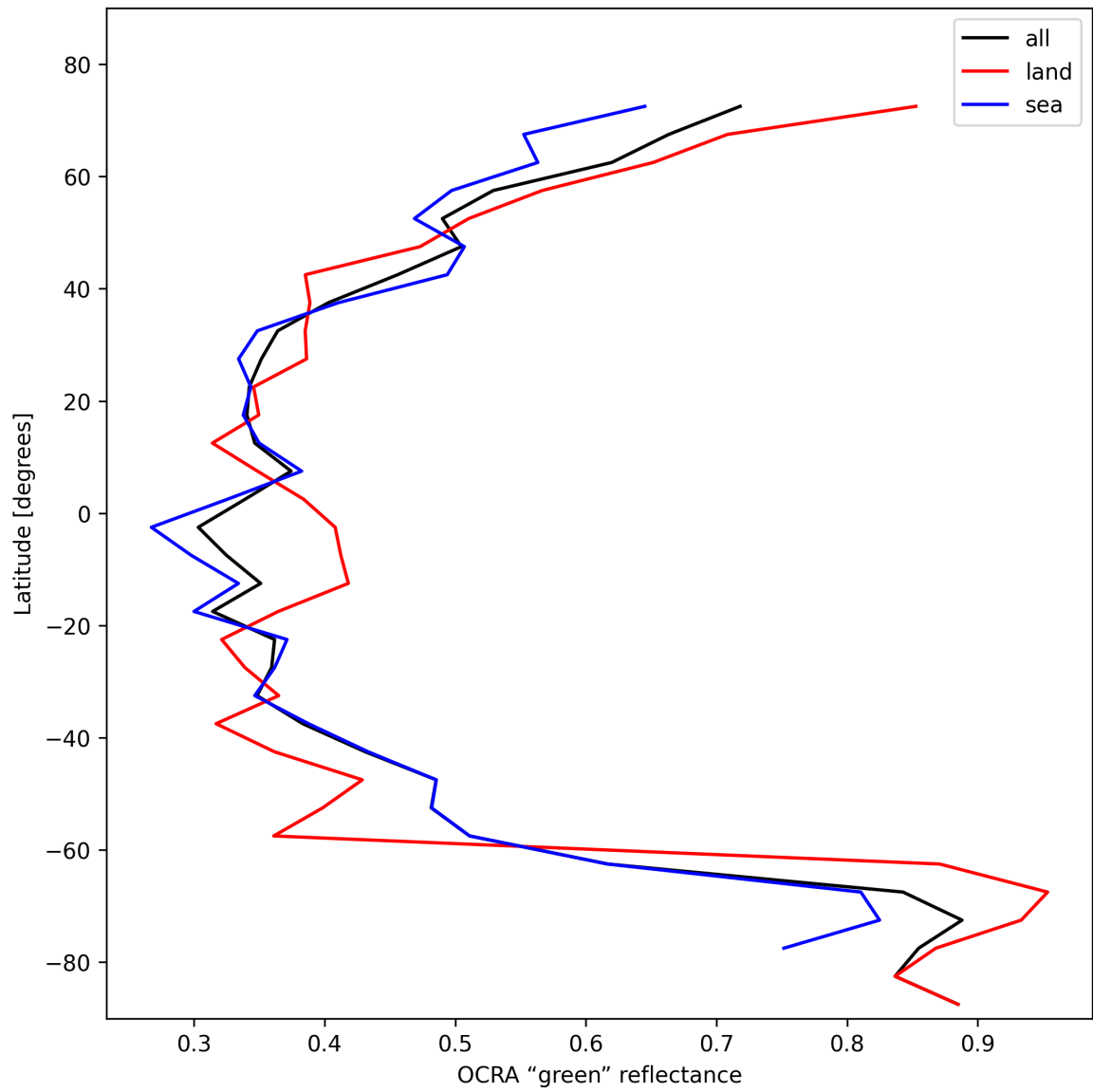
Figure 36: Zonal average of “OCRA “green” reflectance” for 2024-10-30 to 2024-11-01.
