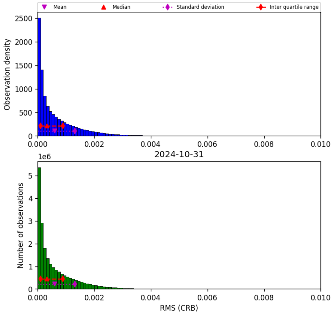
Figure 48: Histogram of “RMS (CRB)” for 2024-10-30 to 2024-11-01
