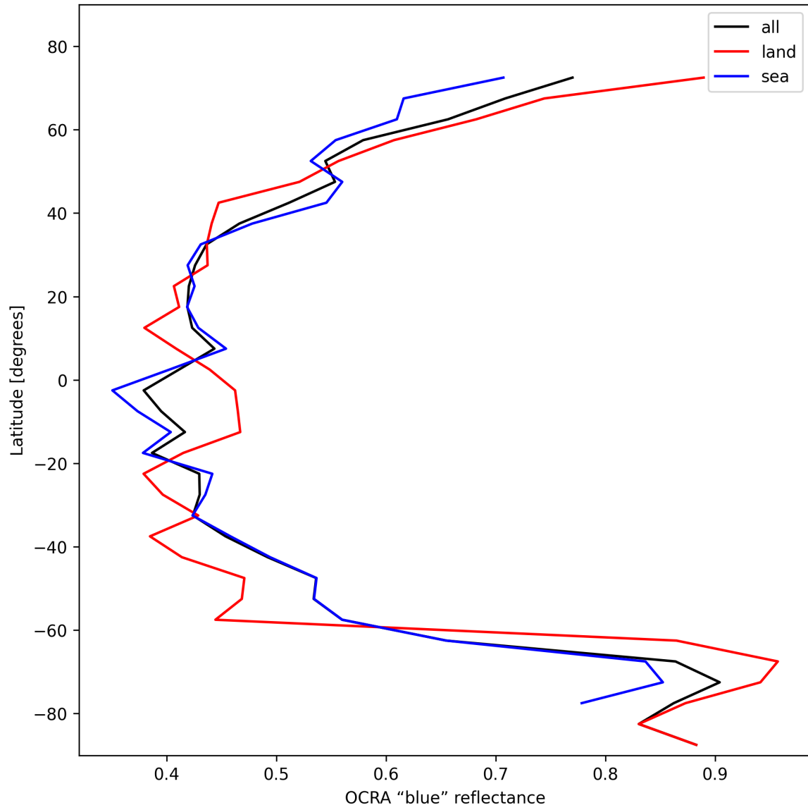
Figure 35: Zonal average of “OCRA “blue” reflectance” for 2024-10-30 to 2024-11-01.
