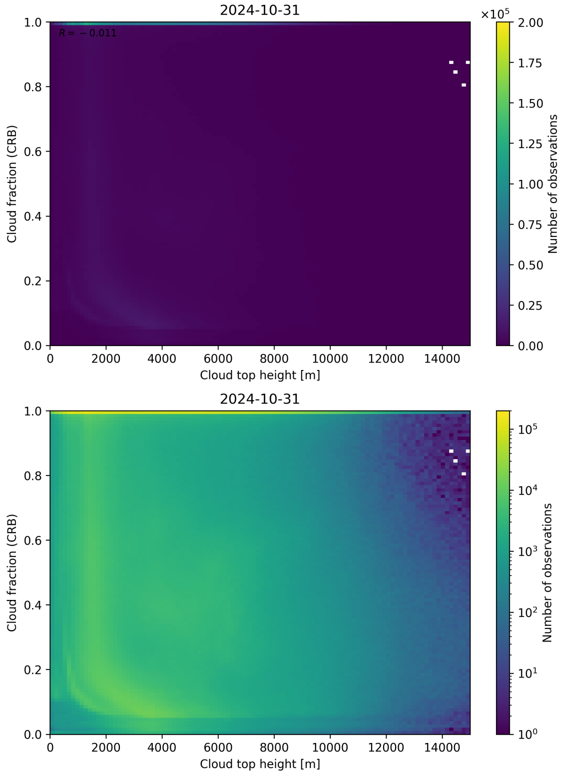
Figure 88: Scatter density plot of “Cloud top height” against “Cloud fraction (CRB)” for 2024-10-30 to 2024-11-01.
