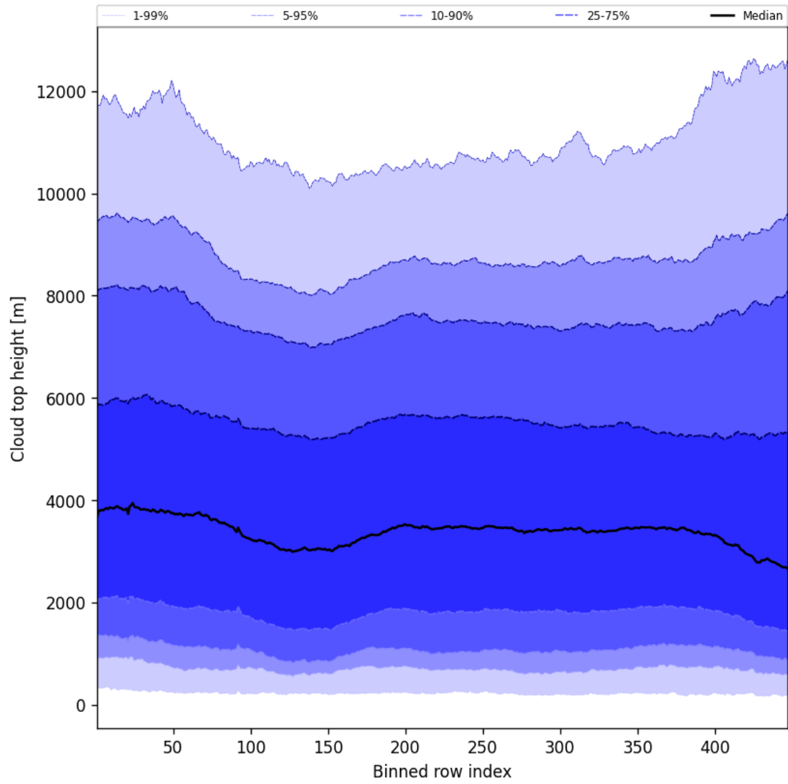
Figure 56: Along track statistics of “Cloud top height” for 2024-10-30 to 2024-11-01
