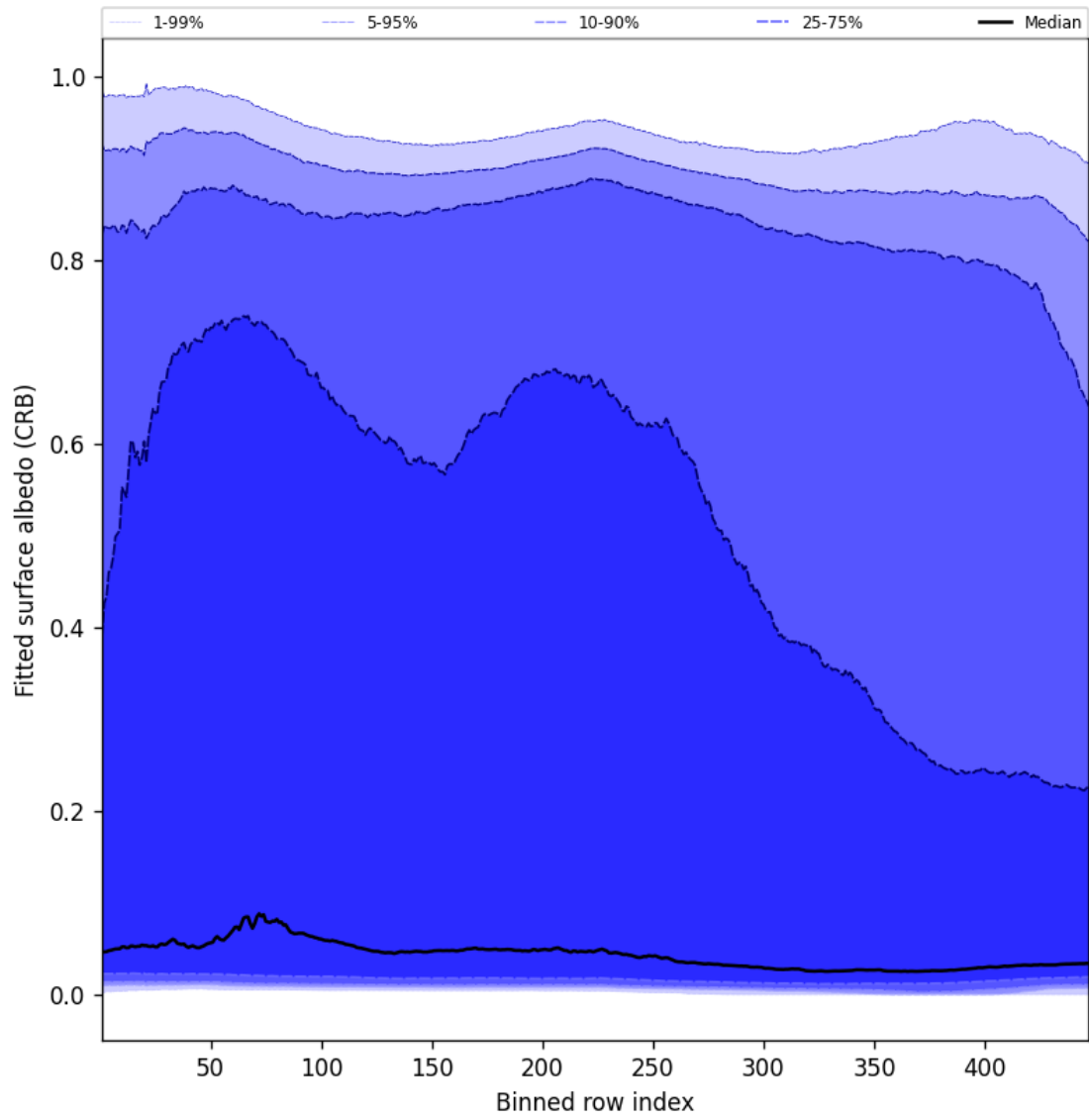
Figure 62: Along track statistics of “Fitted surface albedo (CRB)” for 2024-10-30 to 2024-11-01
