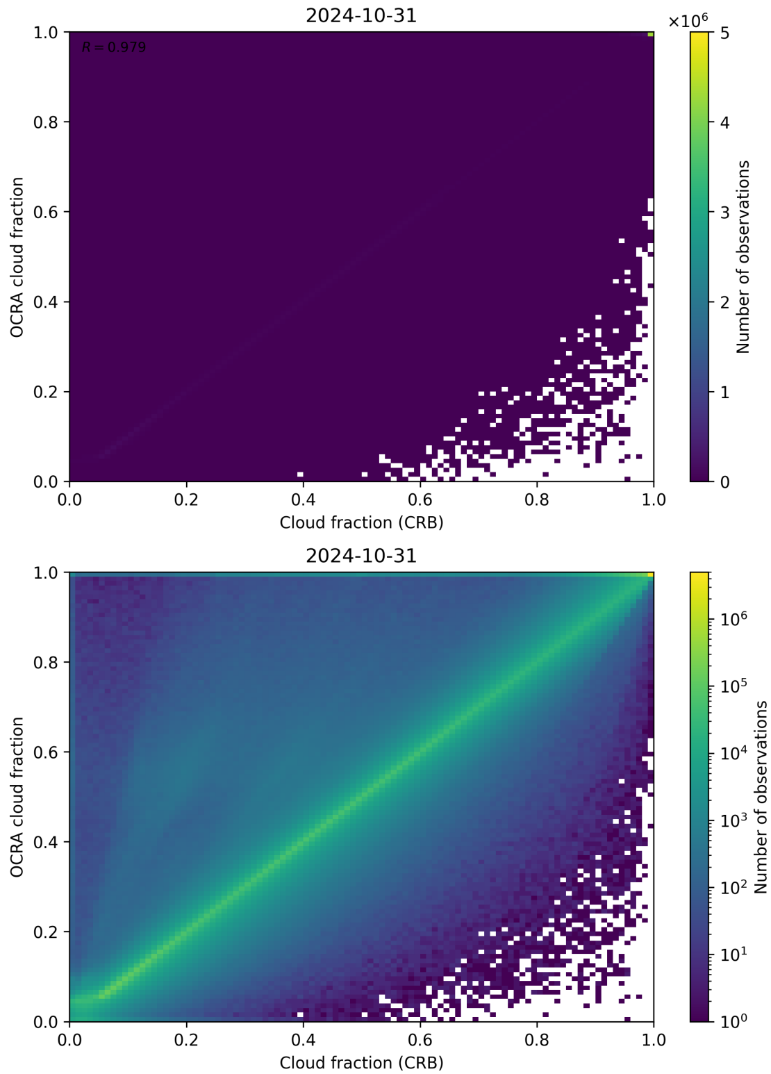
Figure 78: Scatter density plot of “Cloud fraction (CRB)” against “OCRA cloud fraction” for 2024-10-30 to 2024-11-01.
