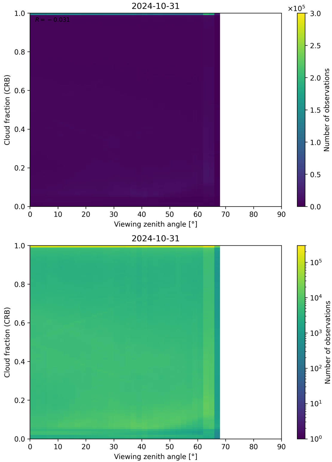
Figure 109: Scatter density plot of “Viewing zenith angle” against “Cloud fraction (CRB)” for 2024-10-30 to 2024-11-01.
