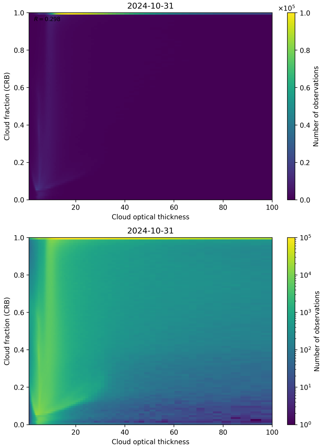
Figure 84: Scatter density plot of “Cloud optical thickness” against “Cloud fraction (CRB)” for 2024-10-30 to 2024-11-01.
