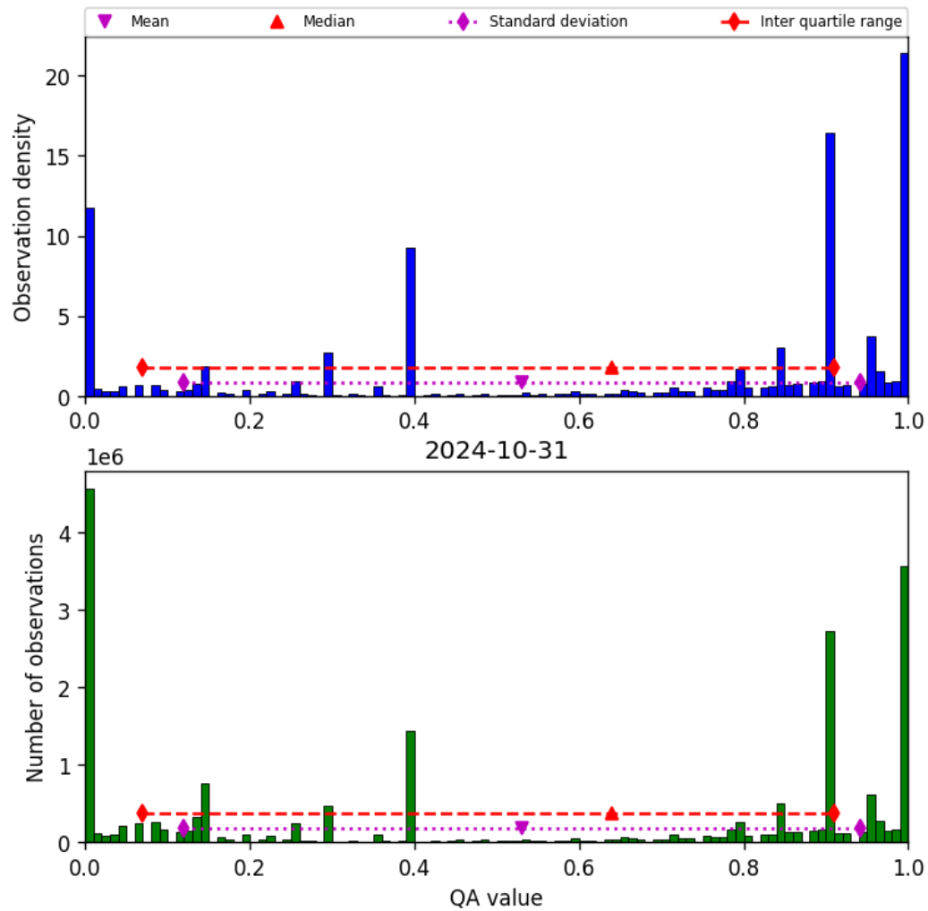
Figure 38: Histogram of “QA value” for 2024-10-30 to 2024-11-01
