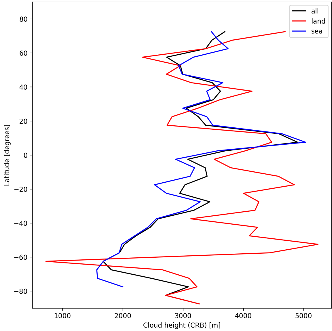
Figure 27: Zonal average of “Cloud height (CRB)” for 2024-10-30 to 2024-11-01.
