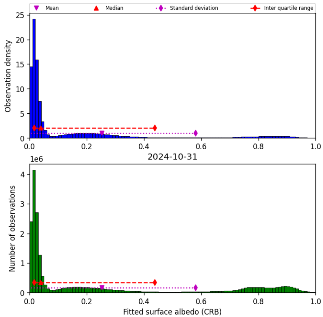
Figure 46: Histogram of “Fitted surface albedo (CRB)” for 2024-10-30 to 2024-11-01
