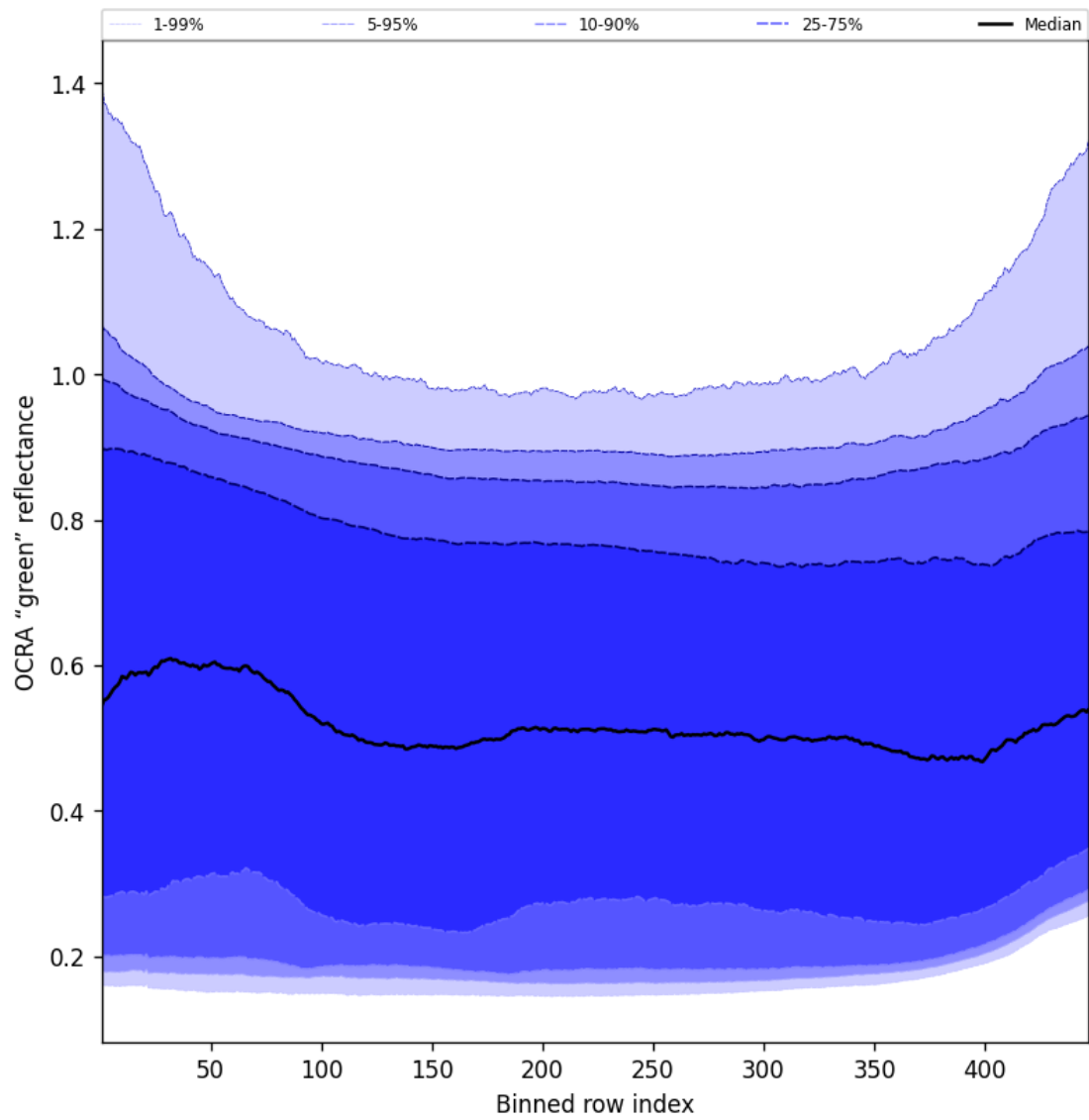
Figure 68: Along track statistics of “OCRA “green” reflectance” for 2024-10-30 to 2024-11-01
