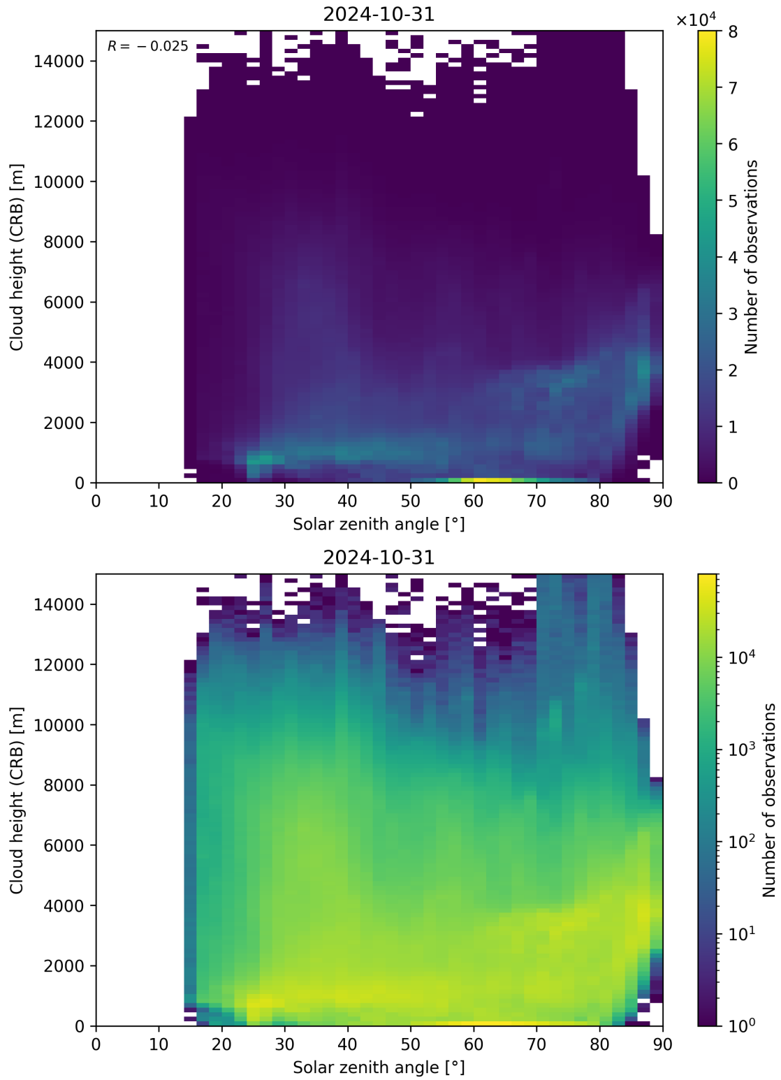
Figure 102: Scatter density plot of “Solar zenith angle” against “Cloud height (CRB)” for 2024-10-30 to 2024-11-01.
