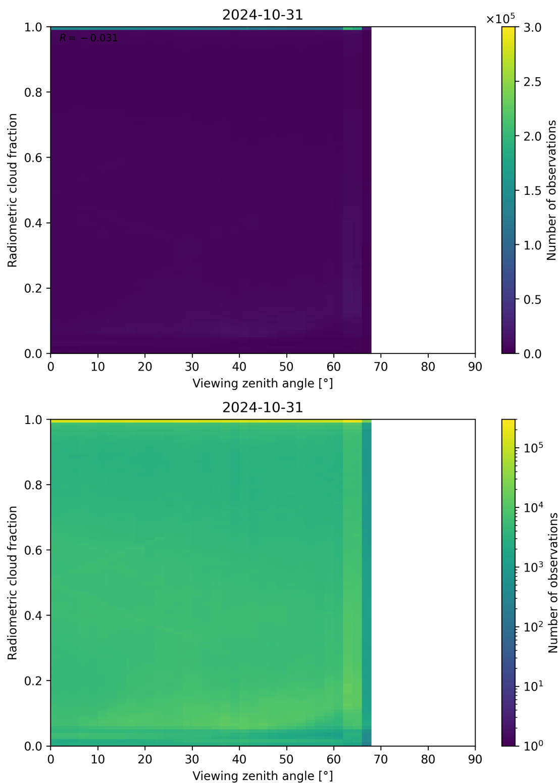
Figure 107: Scatter density plot of “Viewing zenith angle” against “Radiometric cloud fraction” for 2024-10-30 to 2024-11-01.
