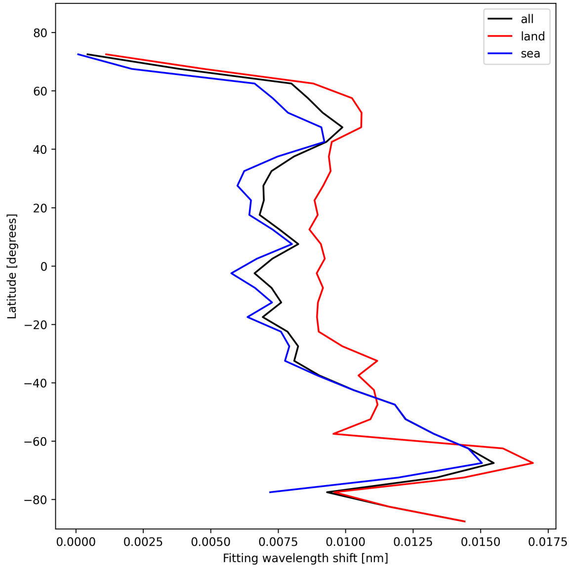
Figure 33: Zonal average of “Fitting wavelength shift” for 2024-10-30 to 2024-11-01.
