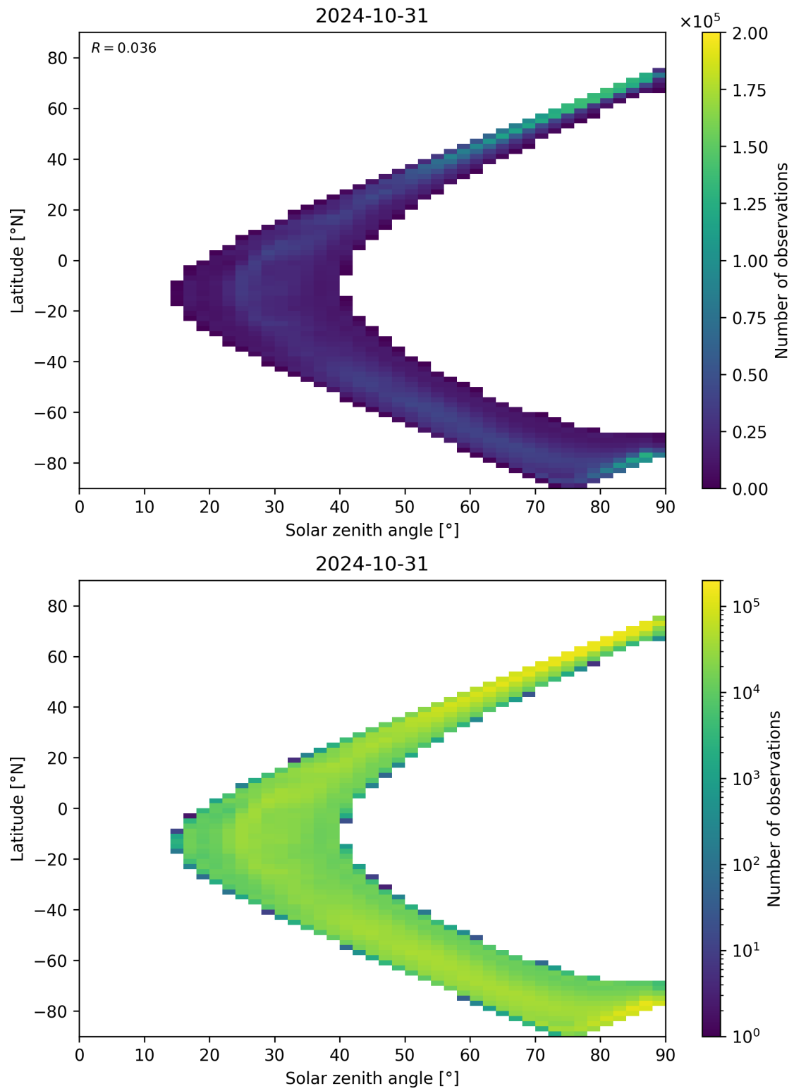
Figure 105: Scatter density plot of “Solar zenith angle” against “Latitude” for 2024-10-30 to 2024-11-01.
