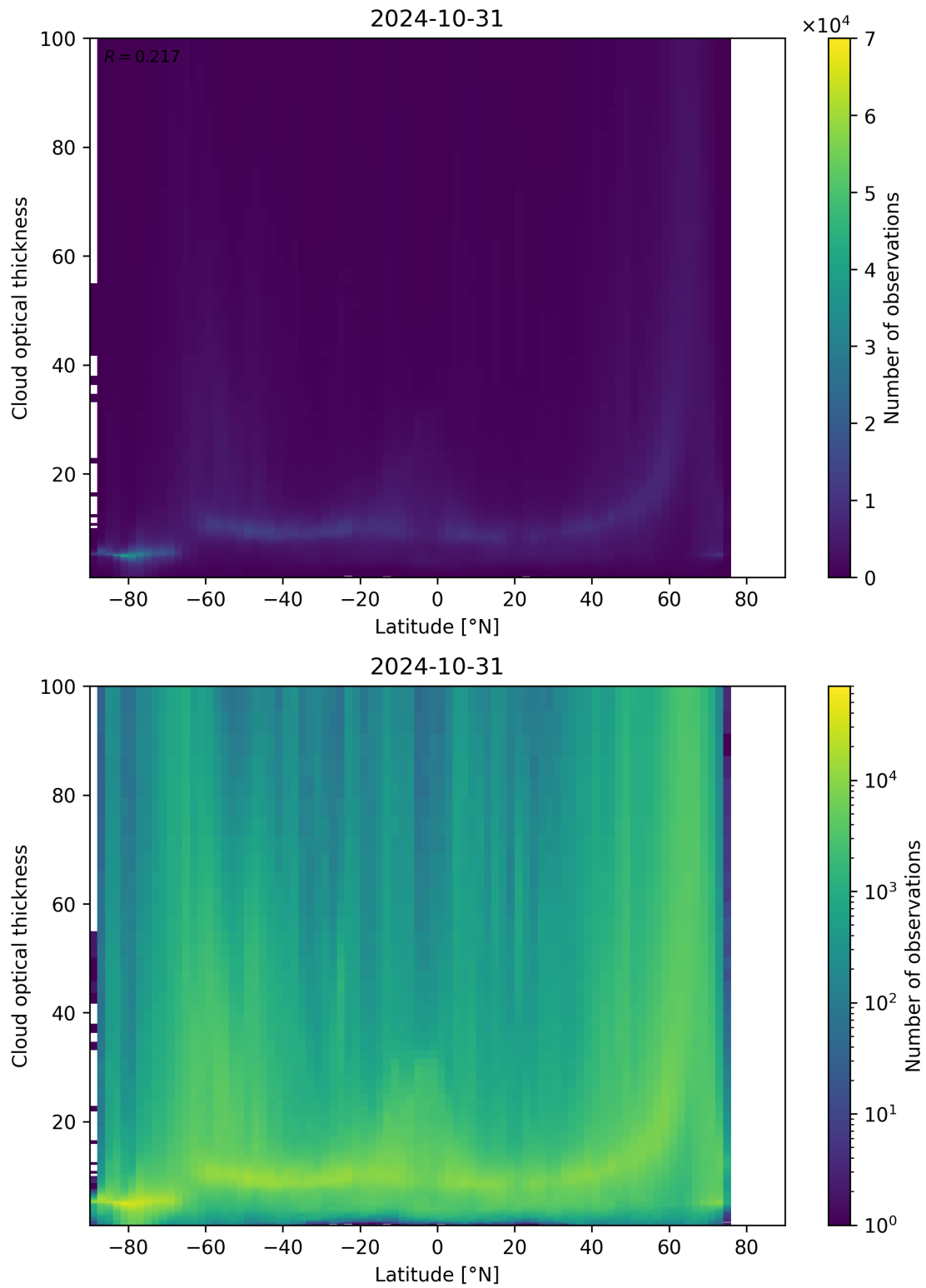
Figure 96: Scatter density plot of “Latitude” against “Cloud optical thickness” for 2024-10-30 to 2024-11-01.
