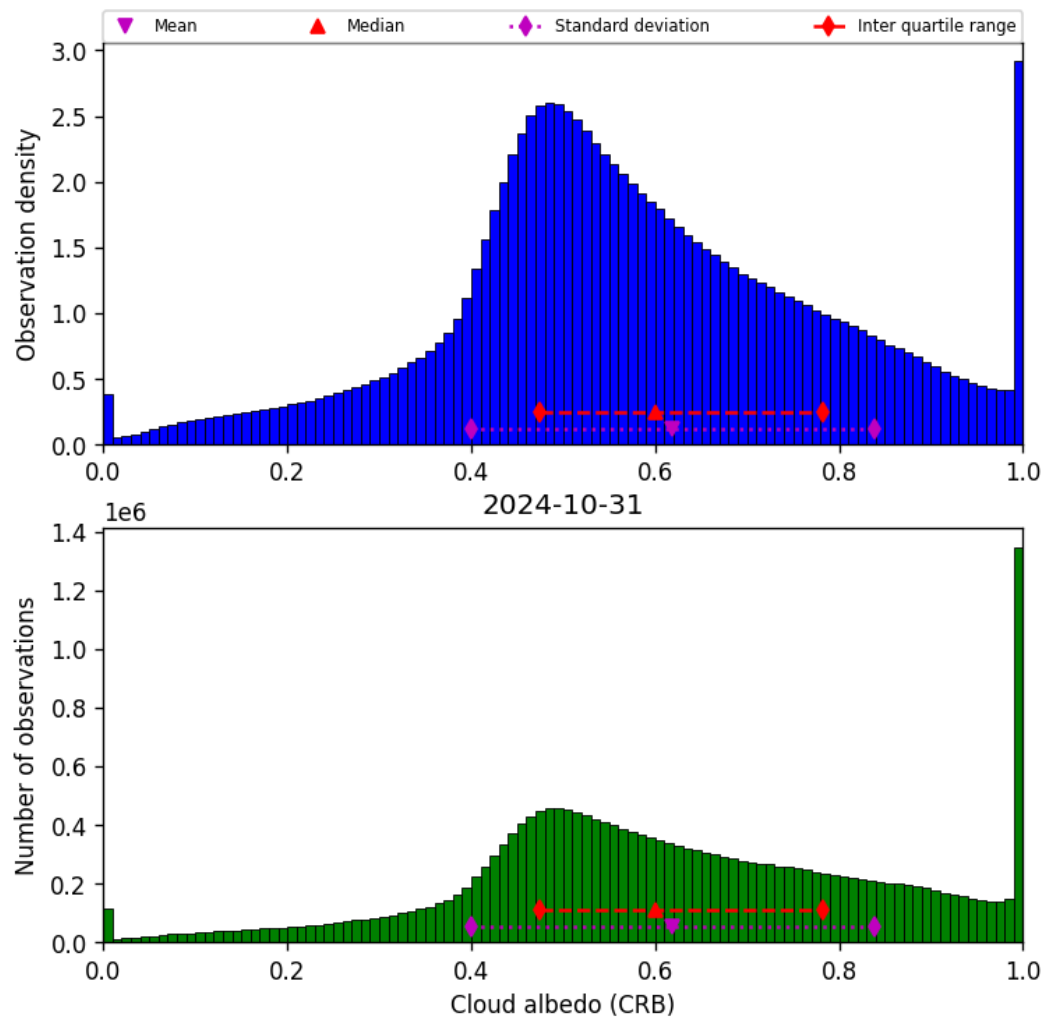
Figure 44: Histogram of “Cloud albedo (CRB)” for 2024-10-30 to 2024-11-01
