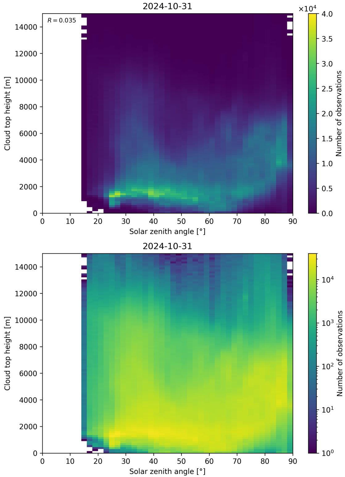
Figure 104: Scatter density plot of “Solar zenith angle” against “Cloud top height” for 2024-10-30 to 2024-11-01.
