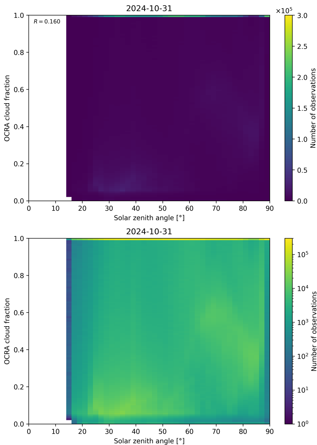
Figure 100: Scatter density plot of “Solar zenith angle” against “OCRA cloud fraction” for 2024-10-30 to 2024-11-01.
