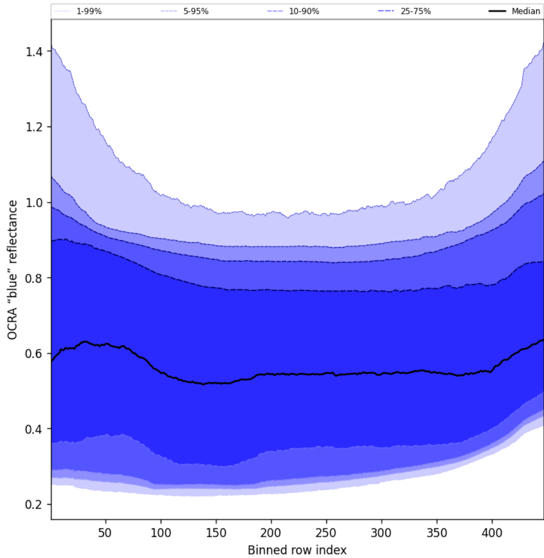
Figure 67: Along track statistics of “OCRA “blue” reflectance” for 2024-10-30 to 2024-11-01
