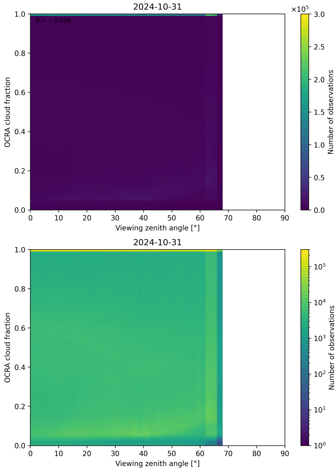
Figure 108: Scatter density plot of “Viewing zenith angle” against “OCRA cloud fraction” for 2024-10-30 to 2024-11-01.
