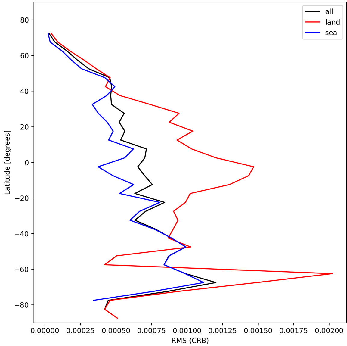
Figure 32: Zonal average of “RMS (CRB)” for 2024-10-30 to 2024-11-01.
