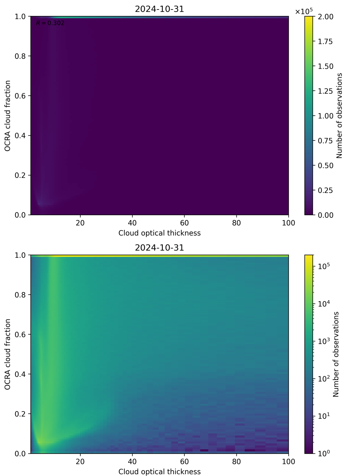
Figure 83: Scatter density plot of “Cloud optical thickness” against “OCRA cloud fraction” for 2024-10-30 to 2024-11-01.
