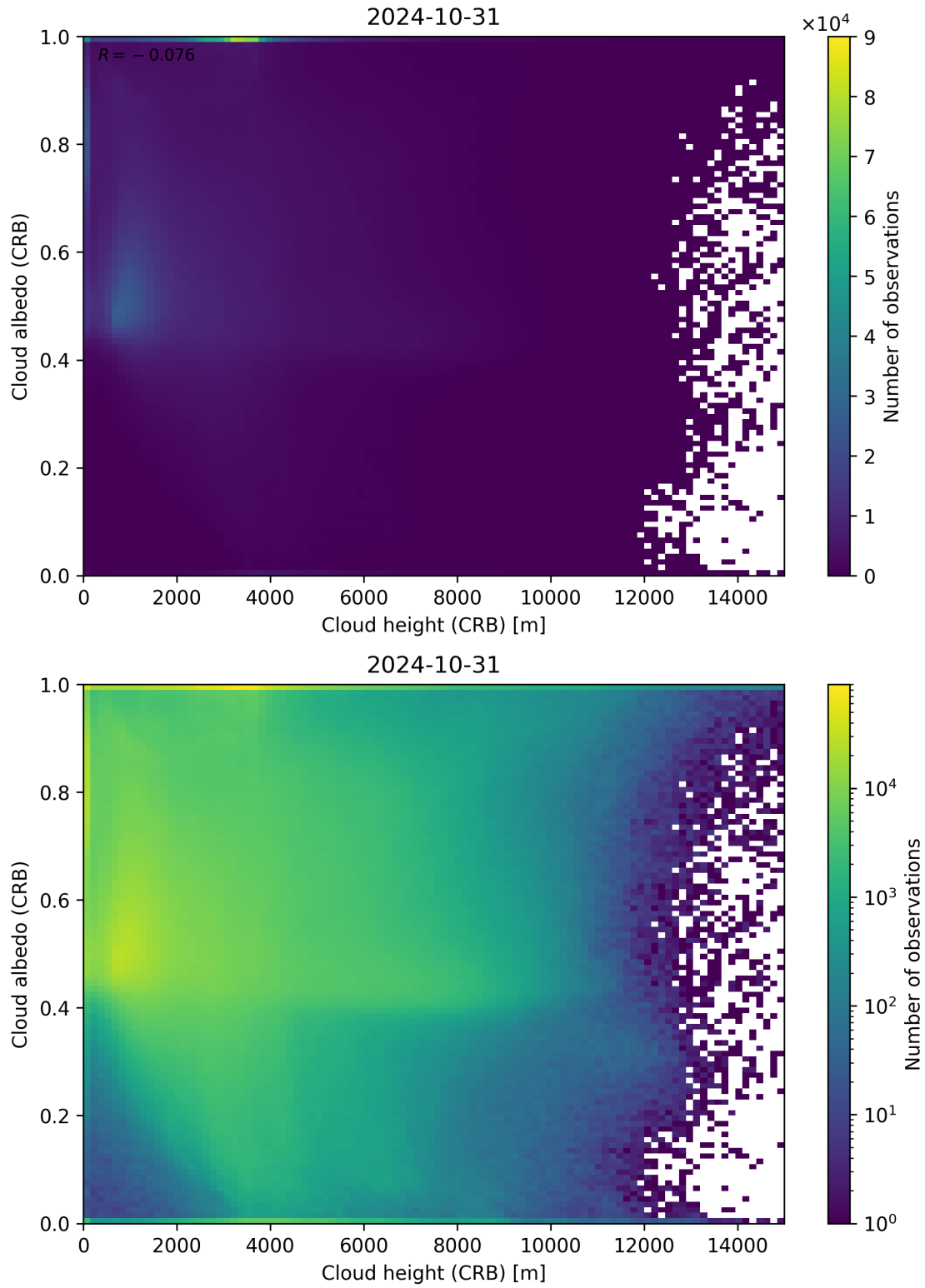
Figure 80: Scatter density plot of “Cloud height (CRB)” against “Cloud albedo (CRB)” for 2024-10-30 to 2024-11-01.
