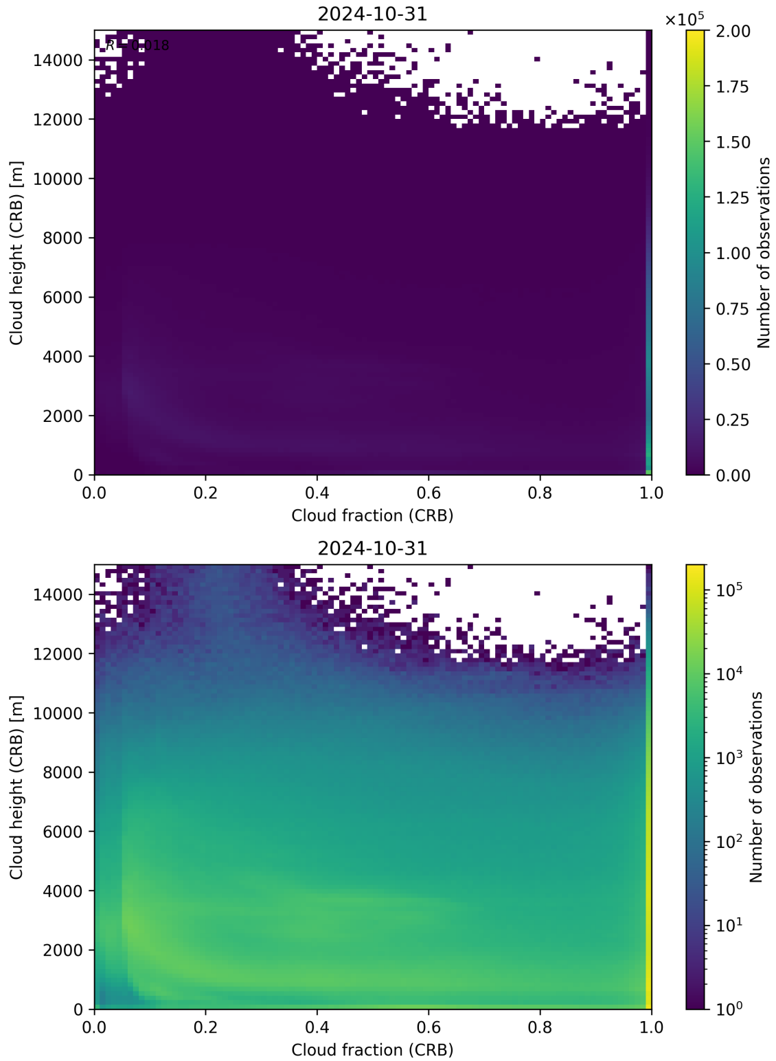
Figure 79: Scatter density plot of “Cloud fraction (CRB)” against “Cloud height (CRB)” for 2024-10-30 to 2024-11-01.
