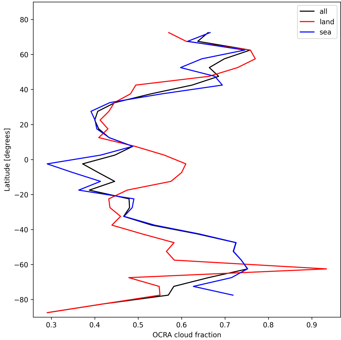
Figure 34: Zonal average of “OCRA cloud fraction” for 2024-10-30 to 2024-11-01.
