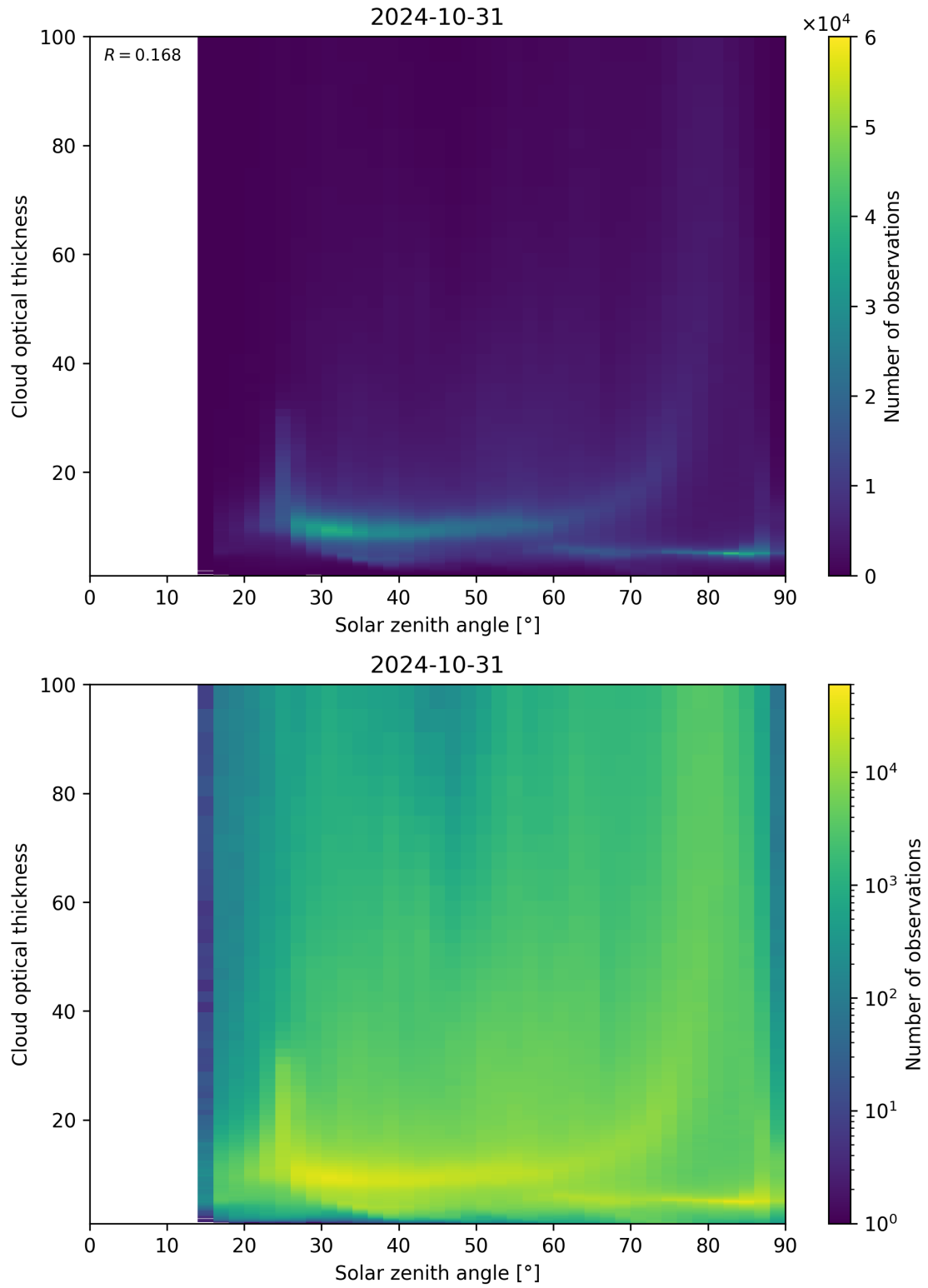
Figure 103: Scatter density plot of “Solar zenith angle” against “Cloud optical thickness” for 2024-10-30 to 2024-11-01.
