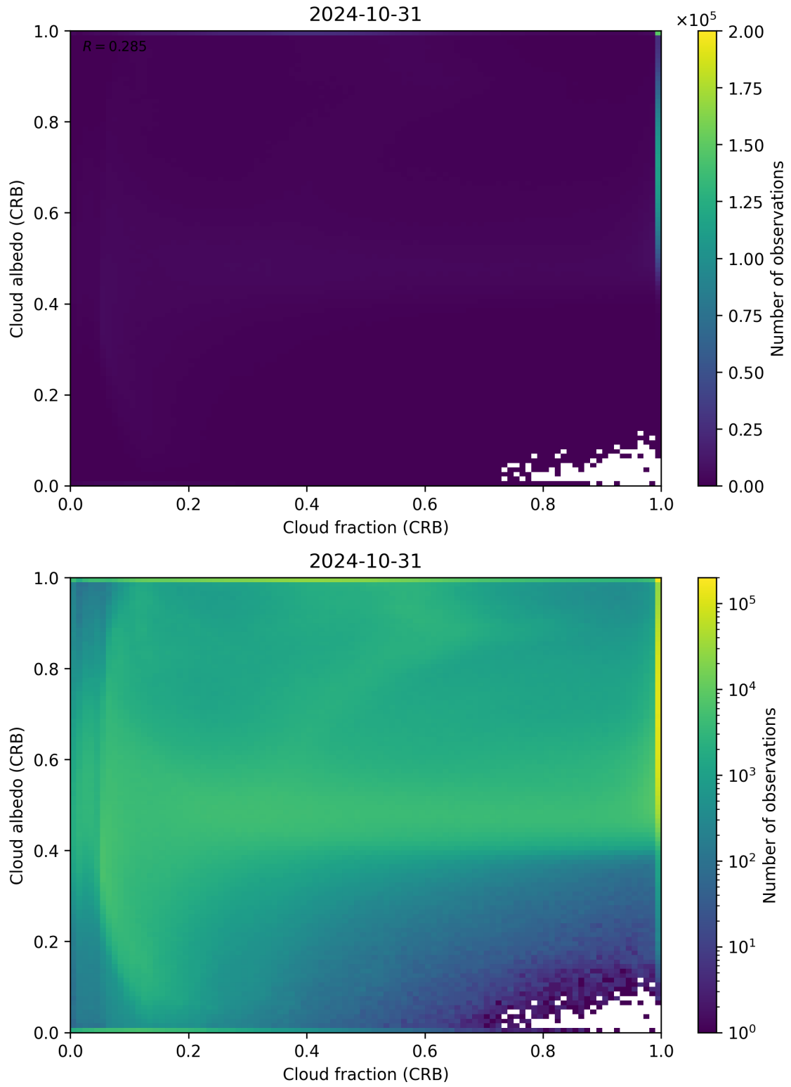
Figure 77: Scatter density plot of “Cloud fraction (CRB)” against “Cloud albedo (CRB)” for 2024-10-30 to 2024-11-01.
