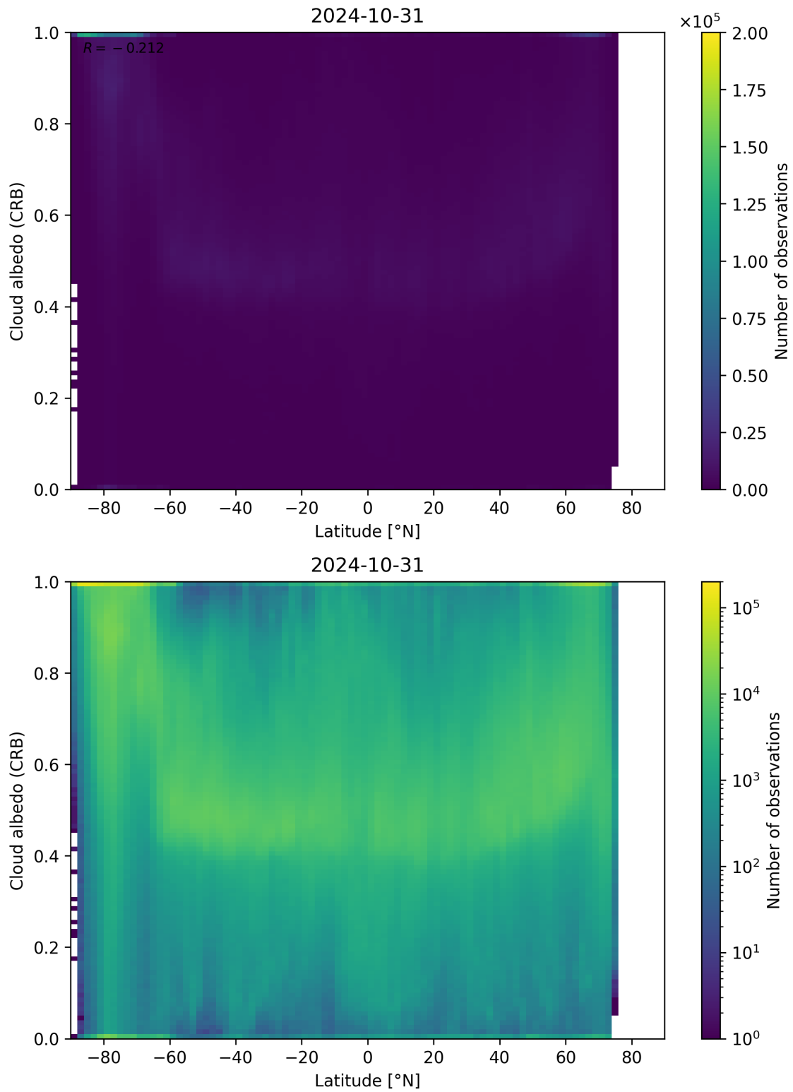
Figure 91: Scatter density plot of “Latitude” against “Cloud albedo (CRB)” for 2024-10-30 to 2024-11-01.
