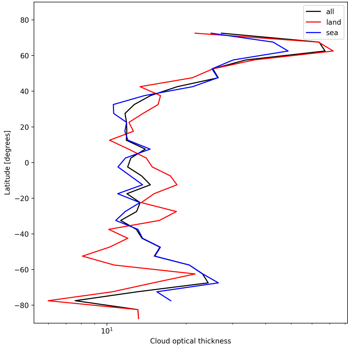
Figure 25: Zonal average of “Cloud optical thickness” for 2024-10-30 to 2024-11-01.
