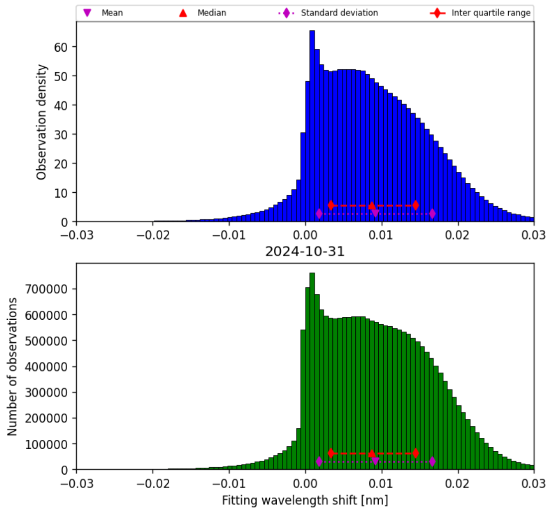
Figure 49: Histogram of “Fitting wavelength shift” for 2024-10-30 to 2024-11-01
