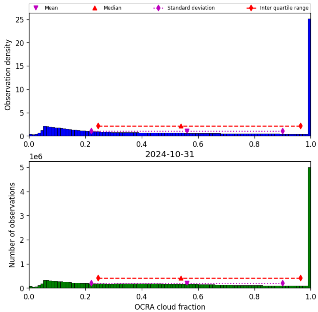
Figure 50: Histogram of “OCRA cloud fraction” for 2024-10-30 to 2024-11-01
