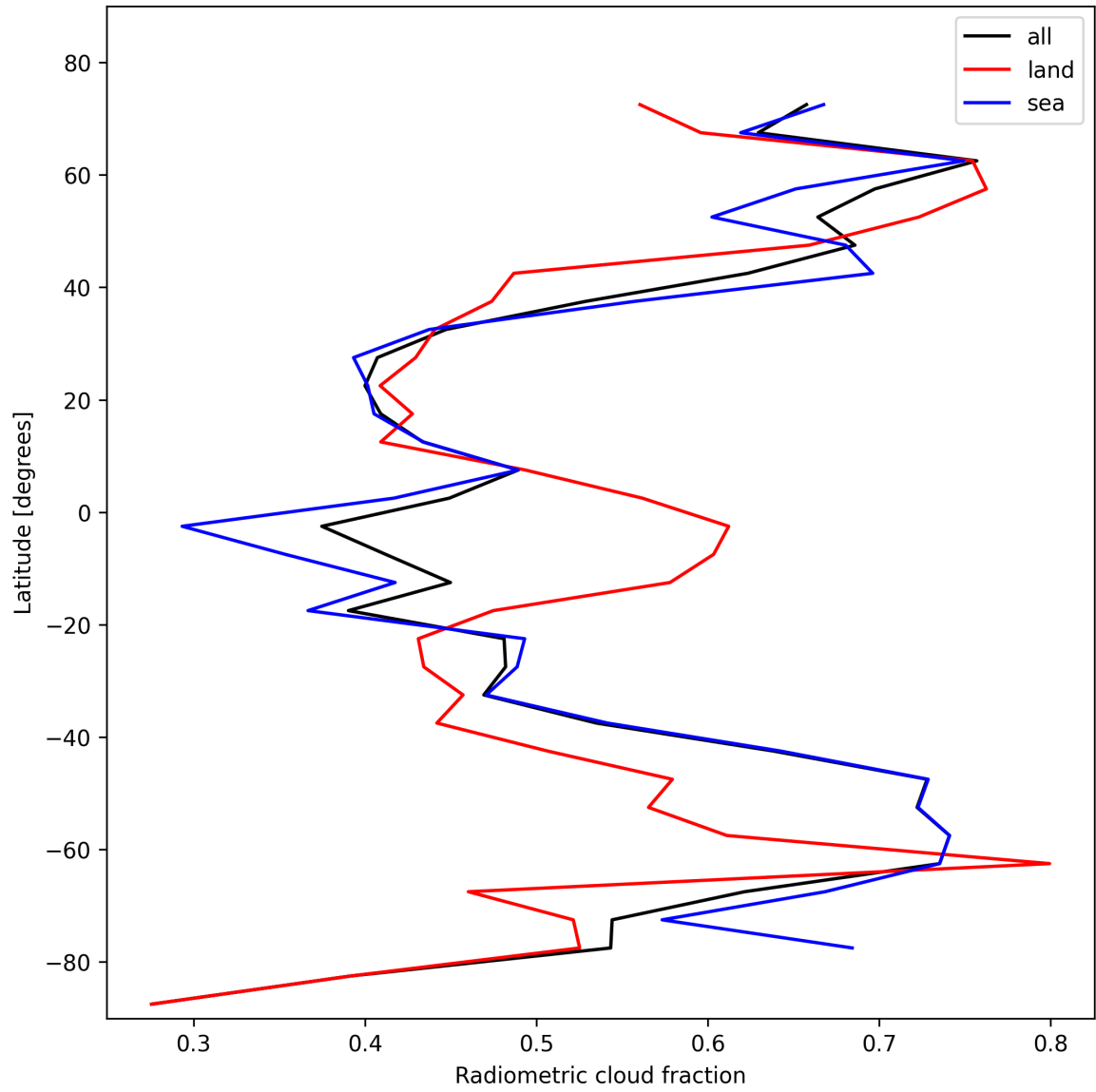
Figure 23: Zonal average of “Radiometric cloud fraction” for 2024-10-30 to 2024-11-01.
