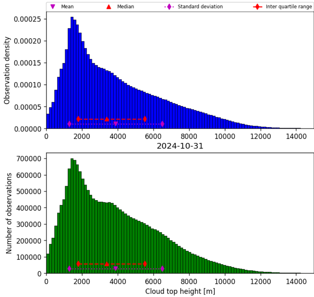
Figure 40: Histogram of “Cloud top height” for 2024-10-30 to 2024-11-01
