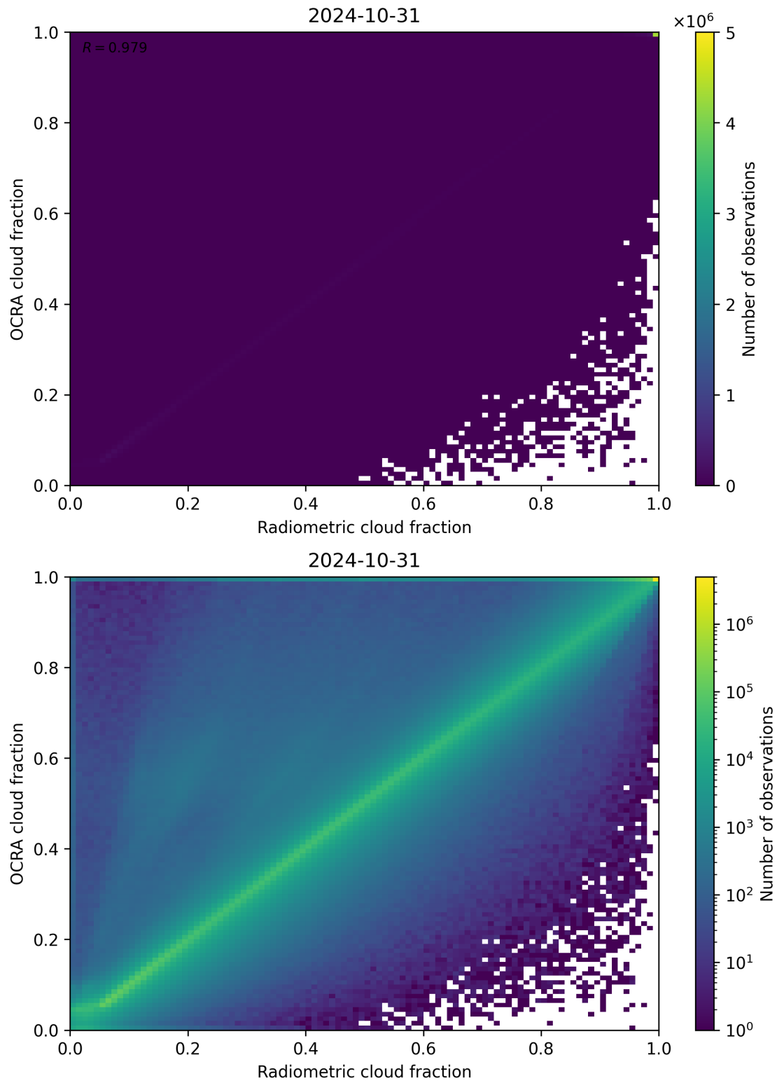
Figure 72: Scatter density plot of “Radiometric cloud fraction” against “OCRA cloud fraction” for 2024-10-30 to 2024-11-01.
