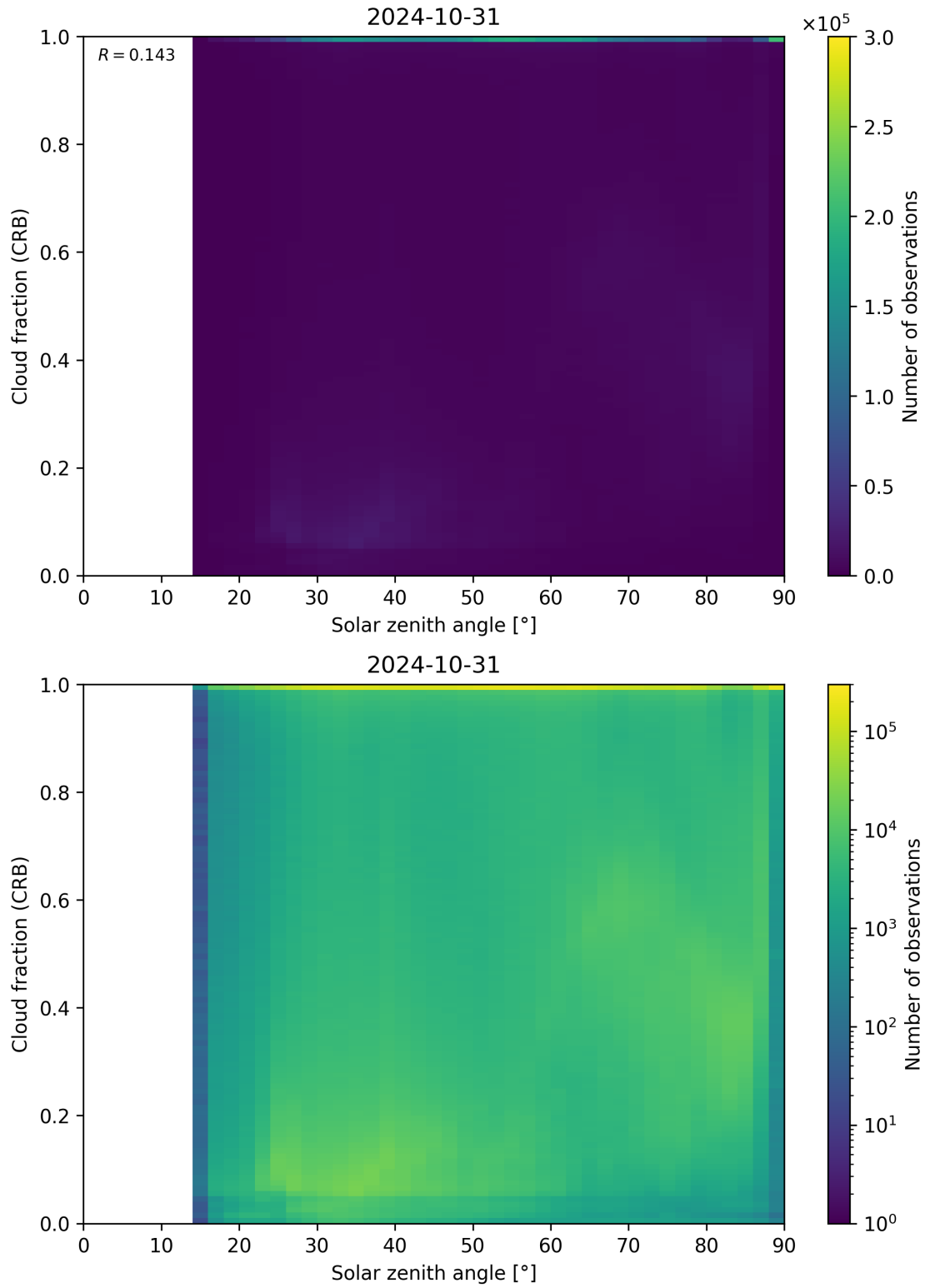
Figure 101: Scatter density plot of “Solar zenith angle” against “Cloud fraction (CRB)” for 2024-10-30 to 2024-11-01.
