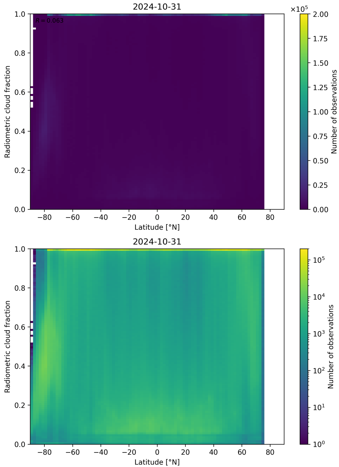
Figure 92: Scatter density plot of “Latitude” against “Radiometric cloud fraction” for 2024-10-30 to 2024-11-01.
