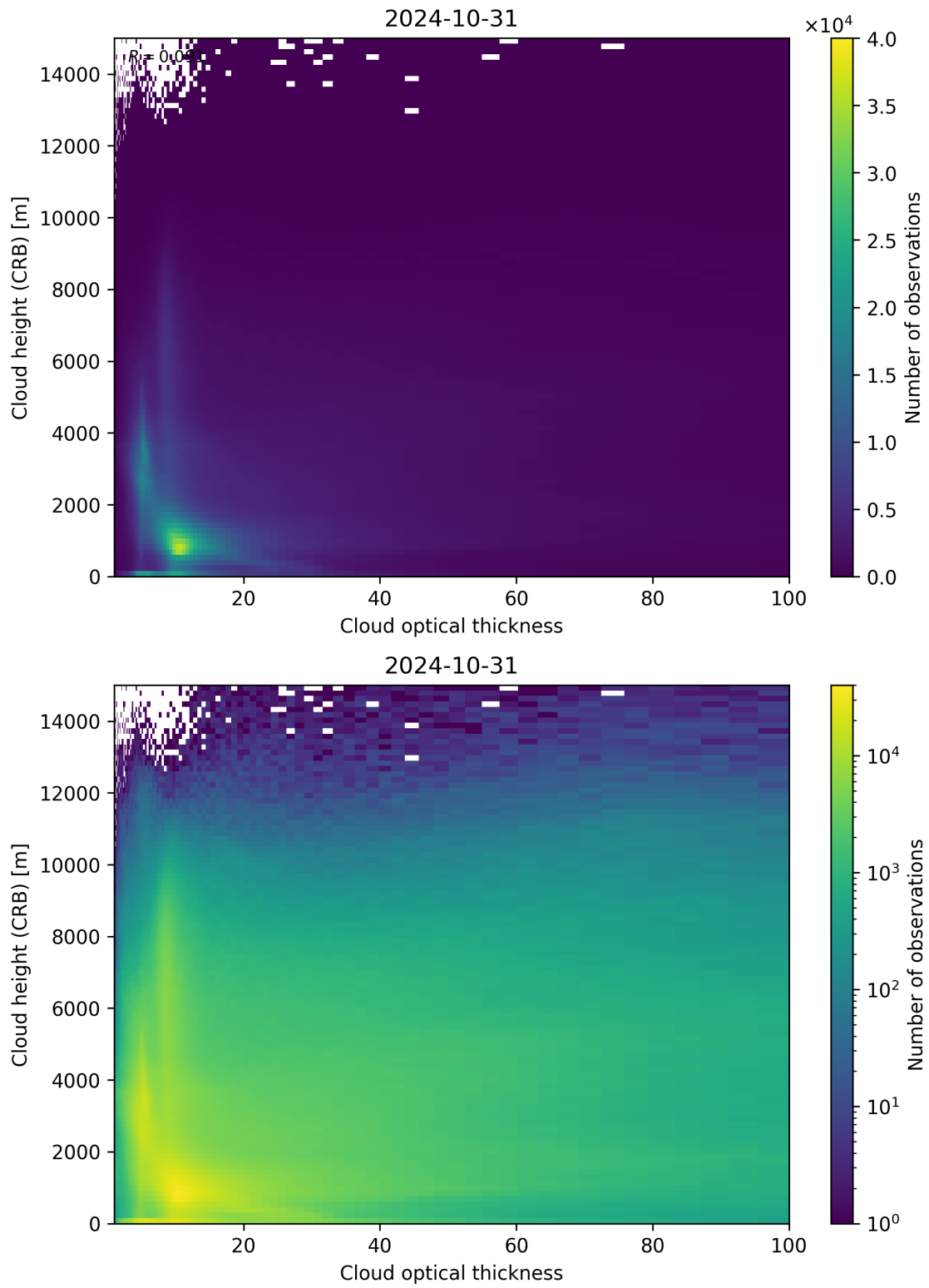
Figure 85: Scatter density plot of “Cloud optical thickness” against “Cloud height (CRB)” for 2024-10-30 to 2024-11-01.
