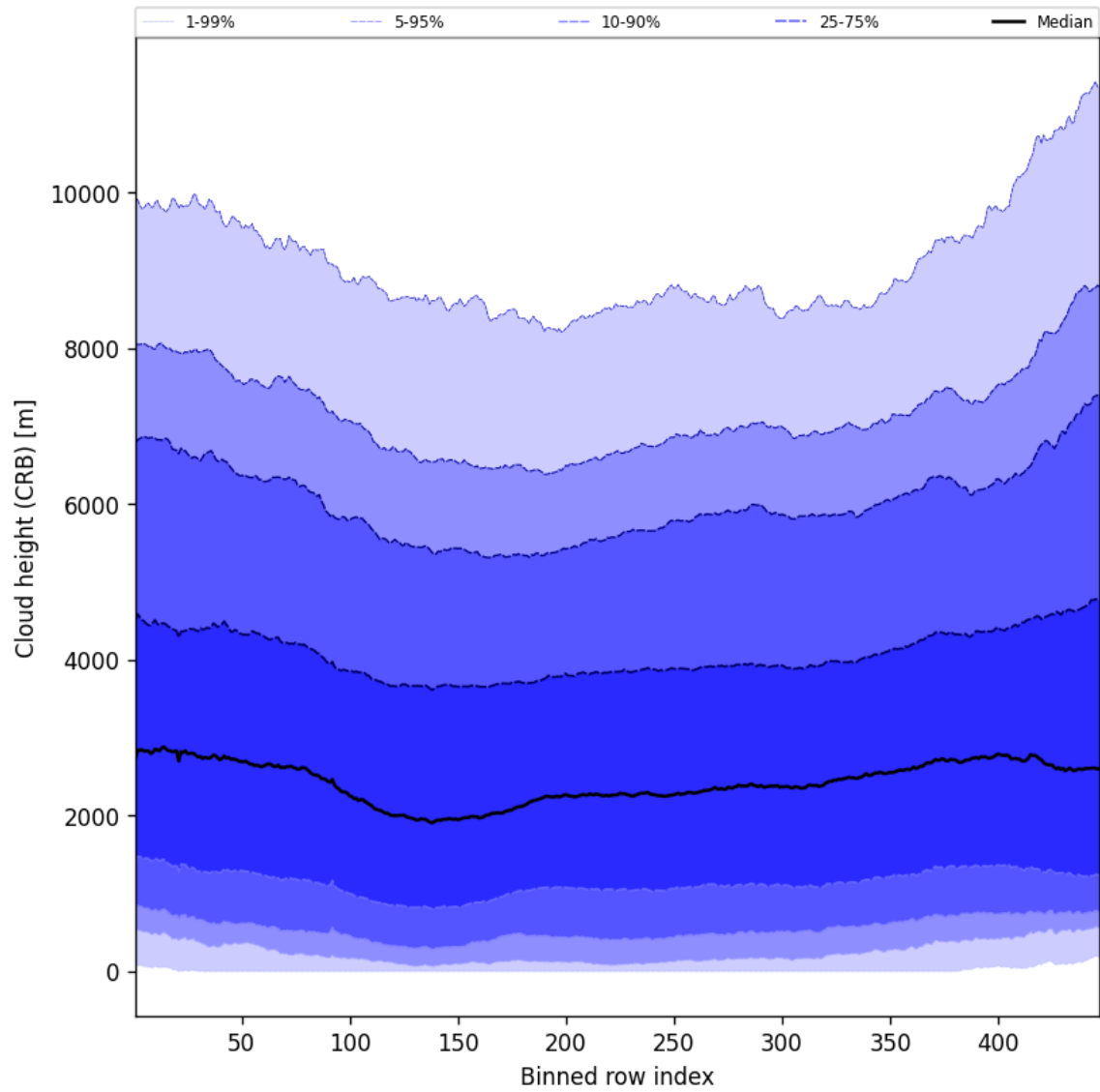
Figure 59: Along track statistics of “Cloud height (CRB)” for 2024-11-01 to 2024-11-03
