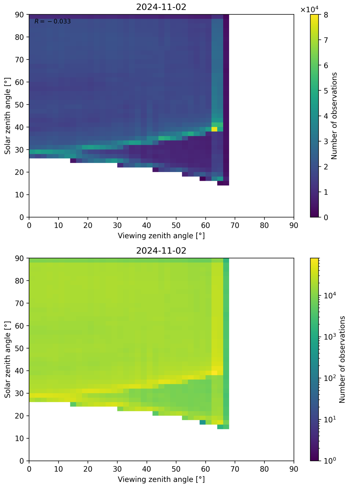
Figure 114: Scatter density plot of “Viewing zenith angle” against “Solar zenith angle” for 2024-11-01 to 2024-11-03.
