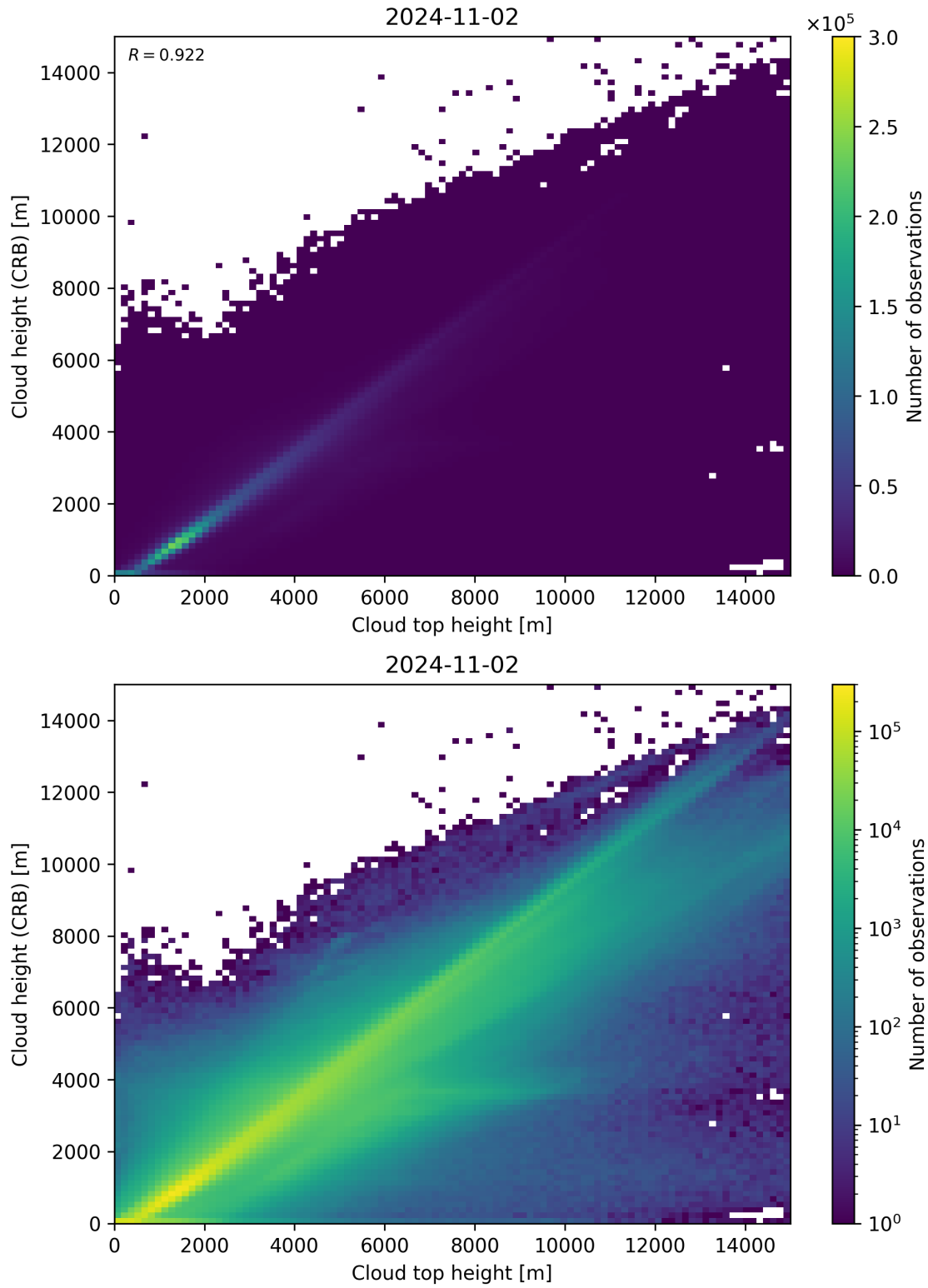
Figure 89: Scatter density plot of “Cloud top height” against “Cloud height (CRB)” for 2024-11-01 to 2024-11-03.
