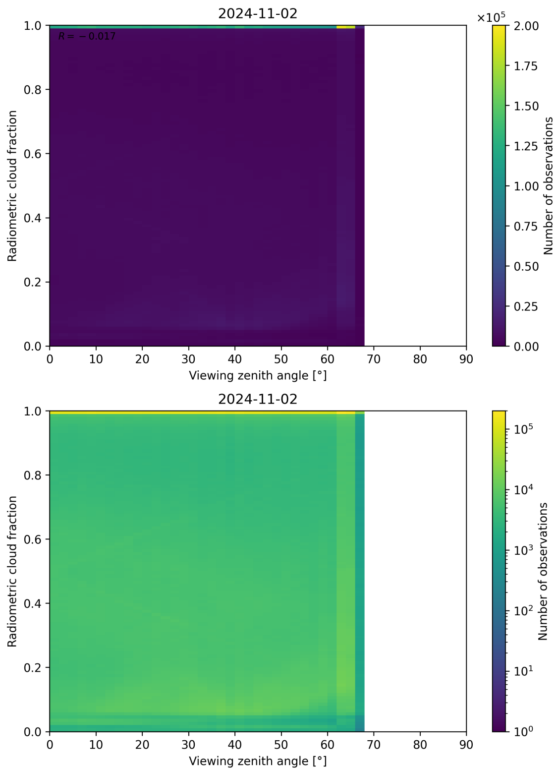
Figure 107: Scatter density plot of “Viewing zenith angle” against “Radiometric cloud fraction” for 2024-11-01 to 2024-11-03.
