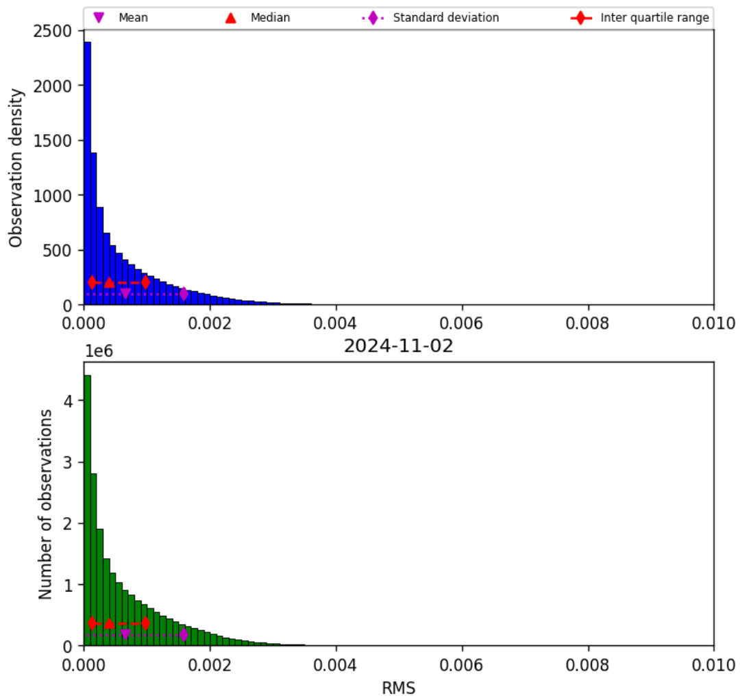
Figure 47: Histogram of “RMS” for 2024-11-01 to 2024-11-03
