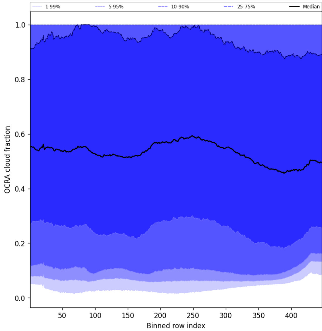
Figure 66: Along track statistics of “OCRA cloud fraction” for 2024-11-01 to 2024-11-03
