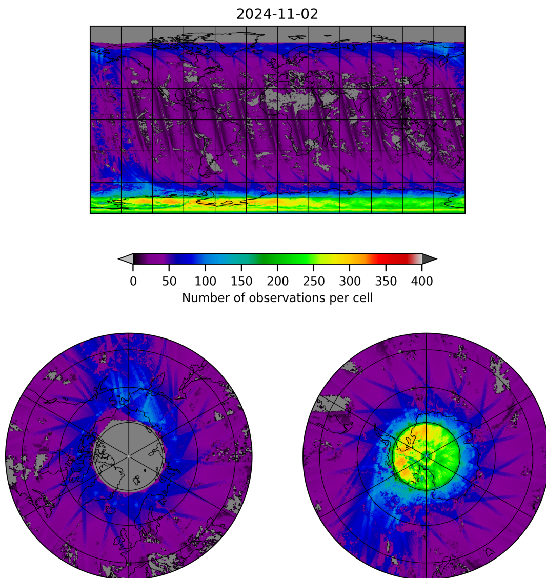
Figure 21: Map of the number of observations for 2024-11-01 to 2024-11-03
