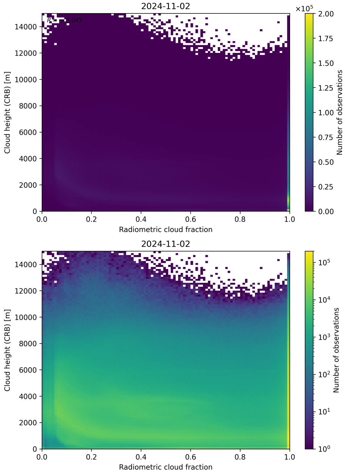
Figure 74: Scatter density plot of “Radiometric cloud fraction” against “Cloud height (CRB)” for 2024-11-01 to 2024-11-03.
