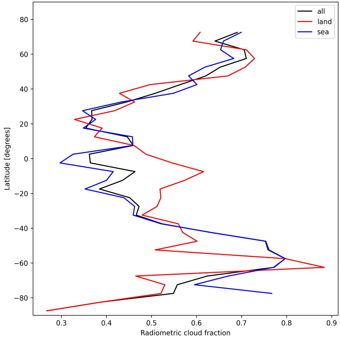
Figure 23: Zonal average of “Radiometric cloud fraction” for 2024-11-01 to 2024-11-03.
