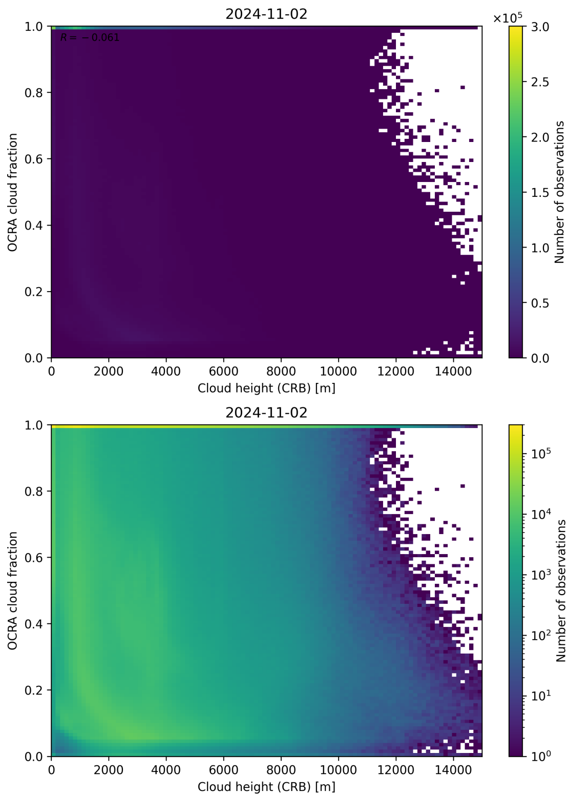
Figure 81: Scatter density plot of “Cloud height (CRB)” against “OCRA cloud fraction” for 2024-11-01 to 2024-11-03.
