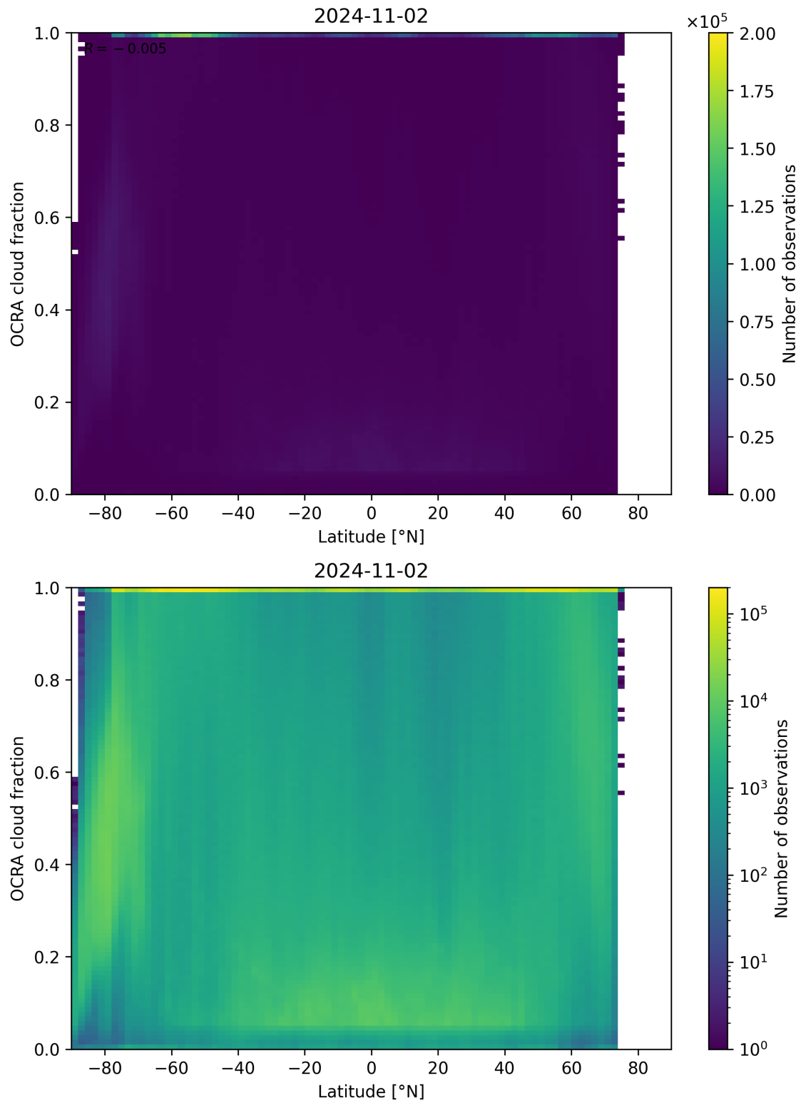
Figure 93: Scatter density plot of “Latitude” against “OCRA cloud fraction” for 2024-11-01 to 2024-11-03.
