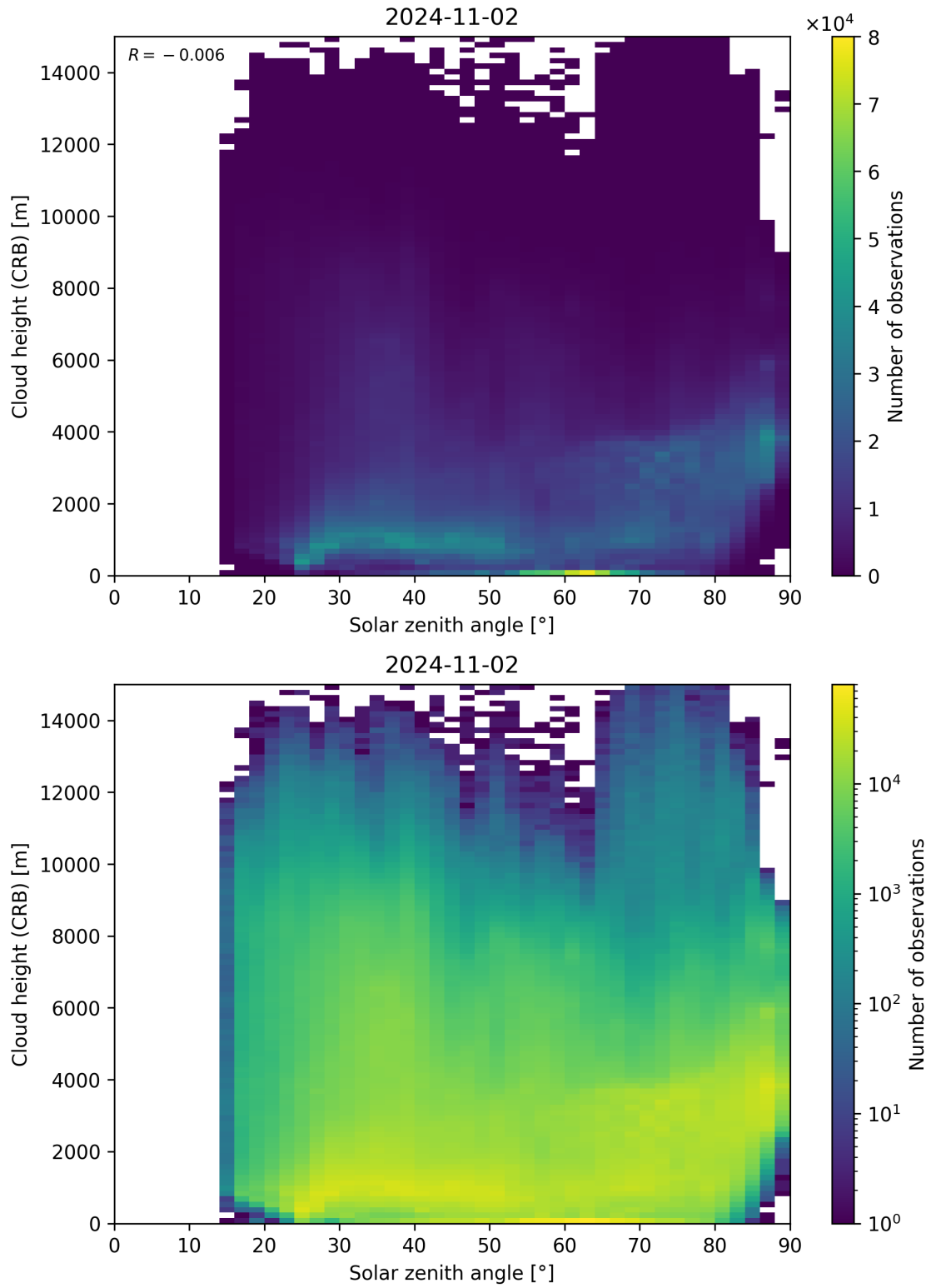
Figure 102: Scatter density plot of “Solar zenith angle” against “Cloud height (CRB)” for 2024-11-01 to 2024-11-03.
