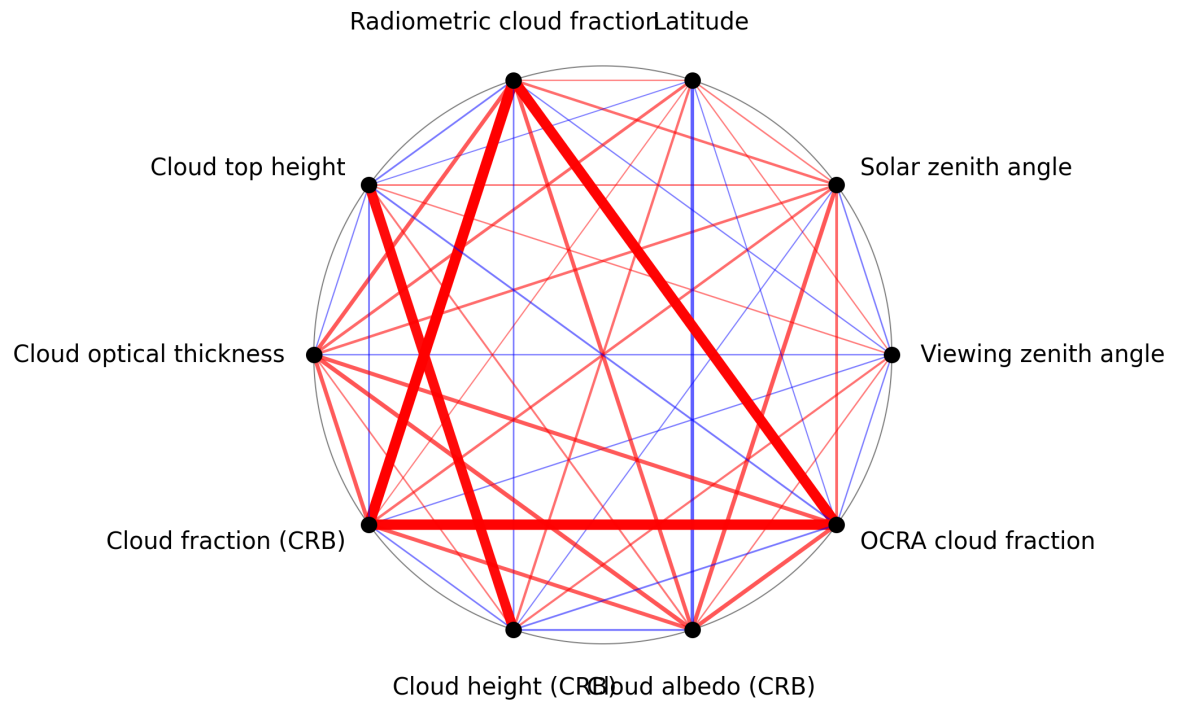
Figure 1: Map of correlation graph for 2024-11-01 to 2024-11-03.
