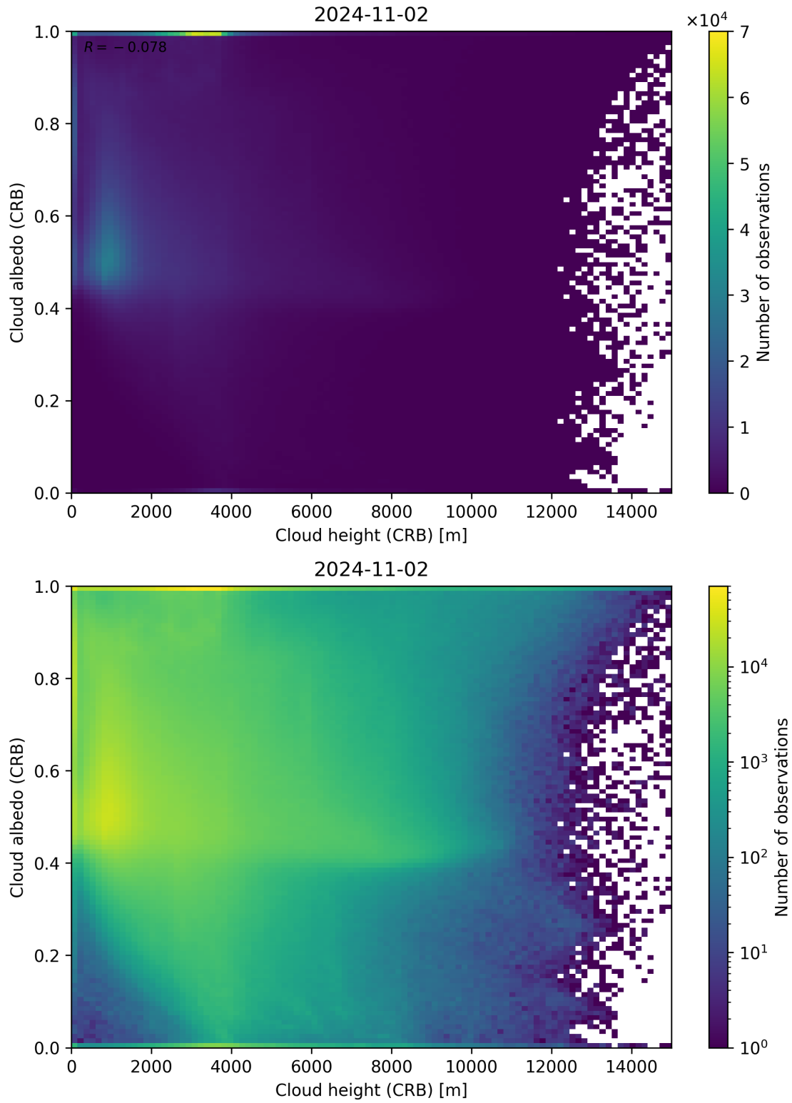
Figure 80: Scatter density plot of “Cloud height (CRB)” against “Cloud albedo (CRB)” for 2024-11-01 to 2024-11-03.
