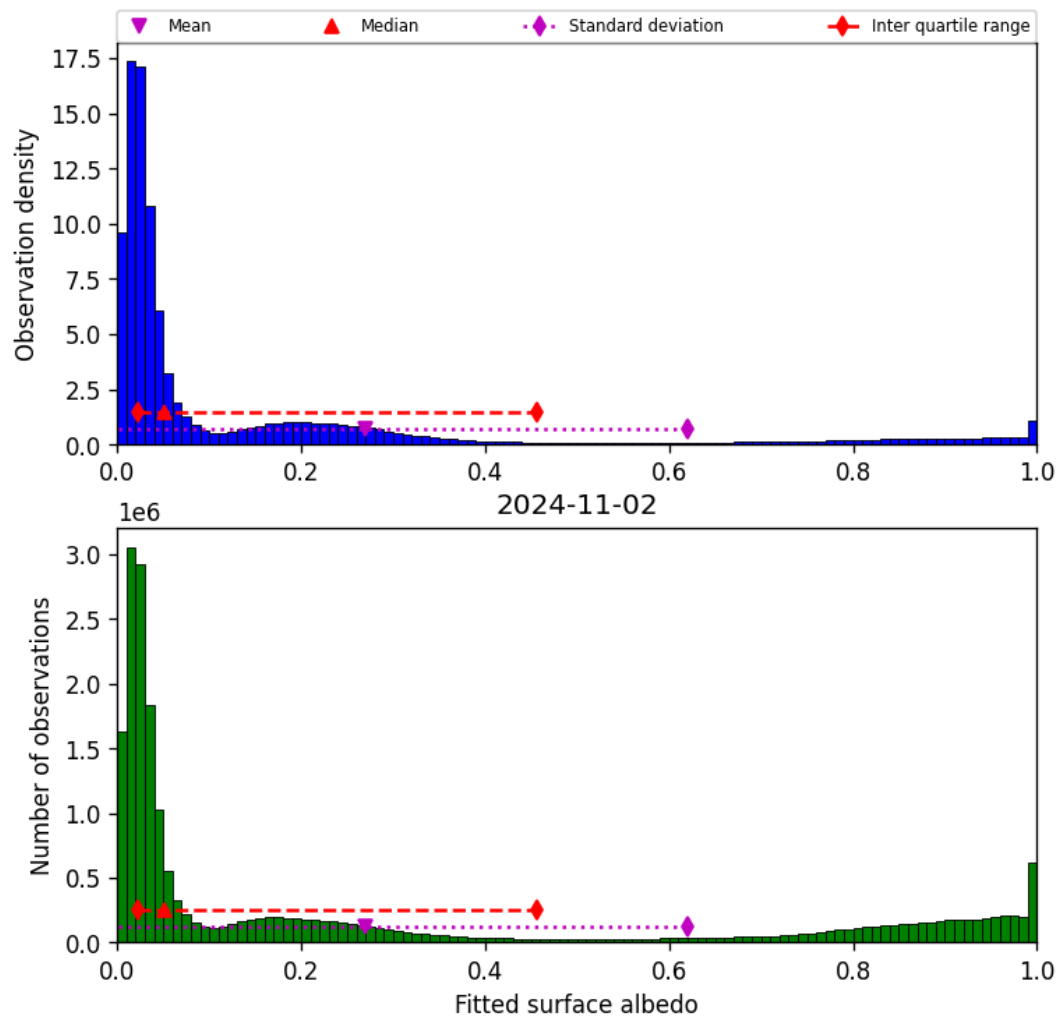
Figure 45: Histogram of “Fitted surface albedo” for 2024-11-01 to 2024-11-03
