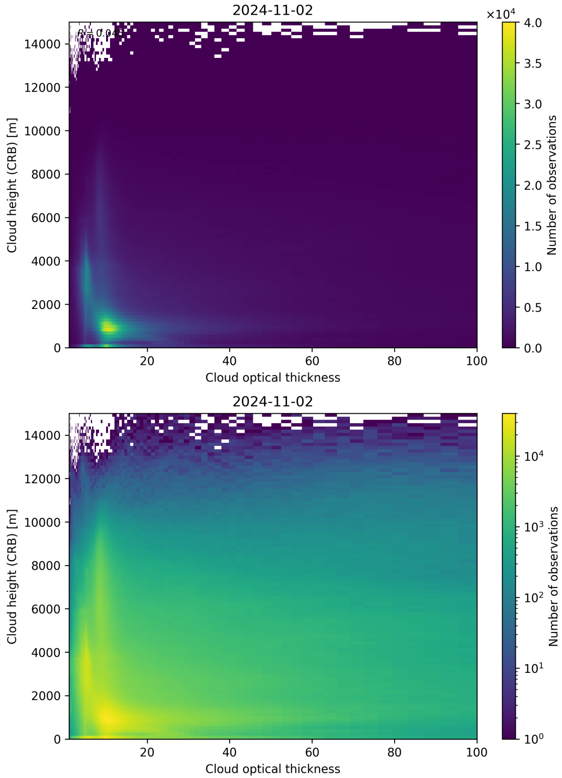
Figure 85: Scatter density plot of “Cloud optical thickness” against “Cloud height (CRB)” for 2024-11-01 to 2024-11-03.
