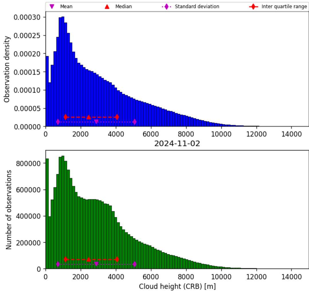
Figure 43: Histogram of “Cloud height (CRB)” for 2024-11-01 to 2024-11-03
