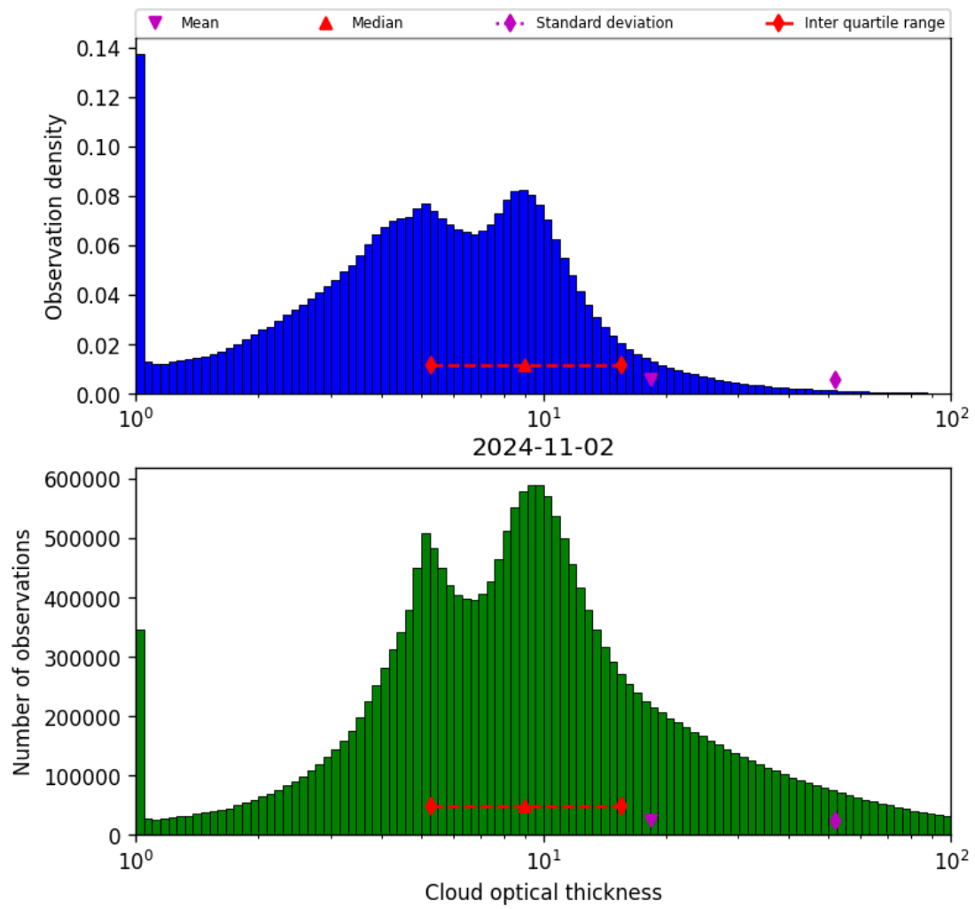
Figure 41: Histogram of “Cloud optical thickness” for 2024-11-01 to 2024-11-03
