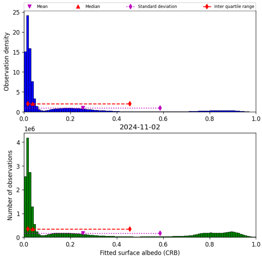
Figure 46: Histogram of “Fitted surface albedo (CRB)” for 2024-11-01 to 2024-11-03
