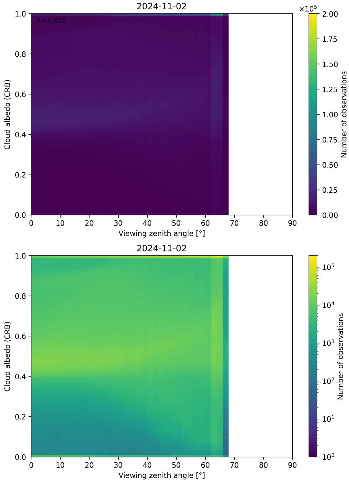
Figure 106: Scatter density plot of “Viewing zenith angle” against “Cloud albedo (CRB)” for 2024-11-01 to 2024-11-03.
