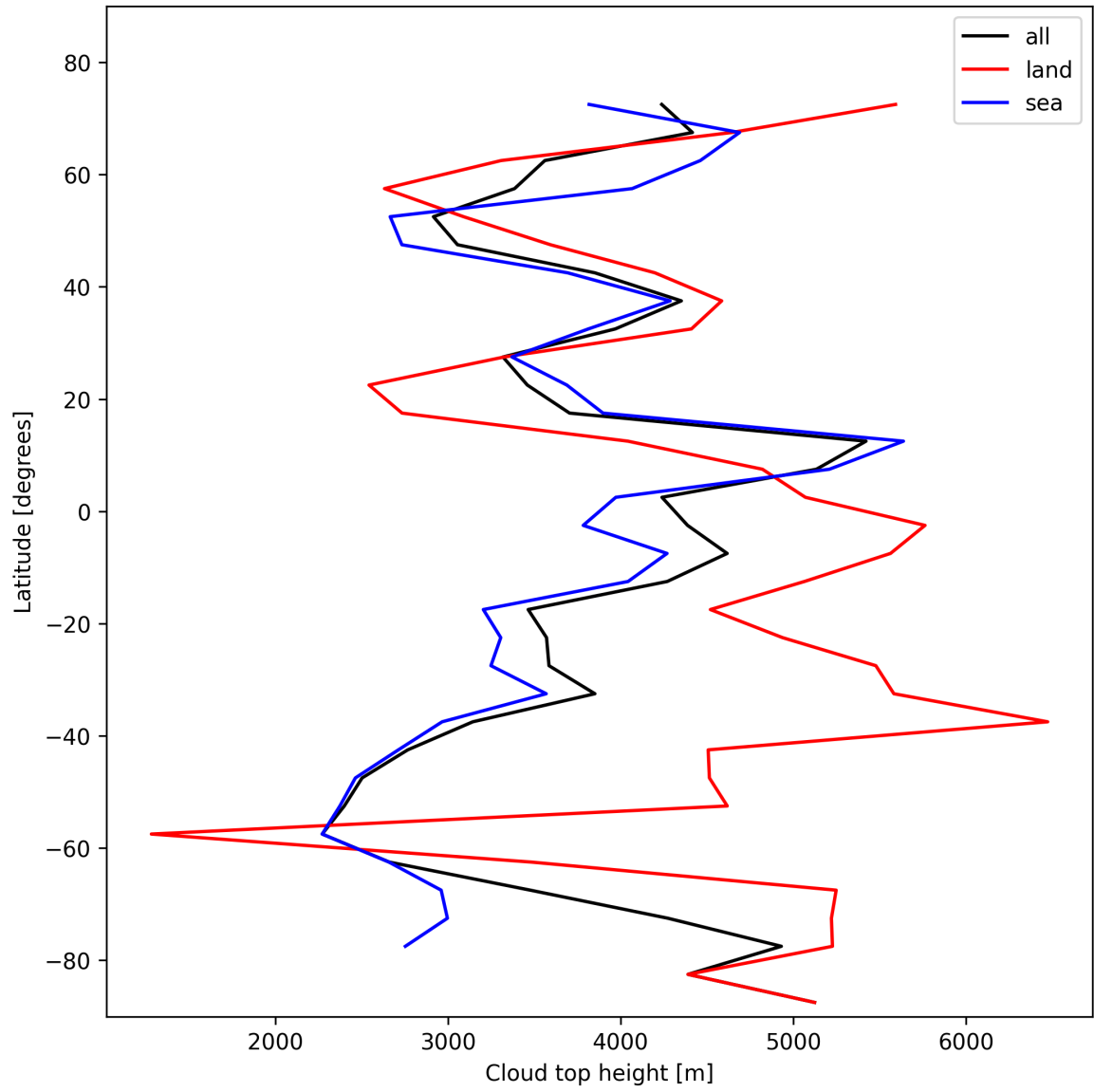
Figure 24: Zonal average of “Cloud top height” for 2024-11-01 to 2024-11-03.
