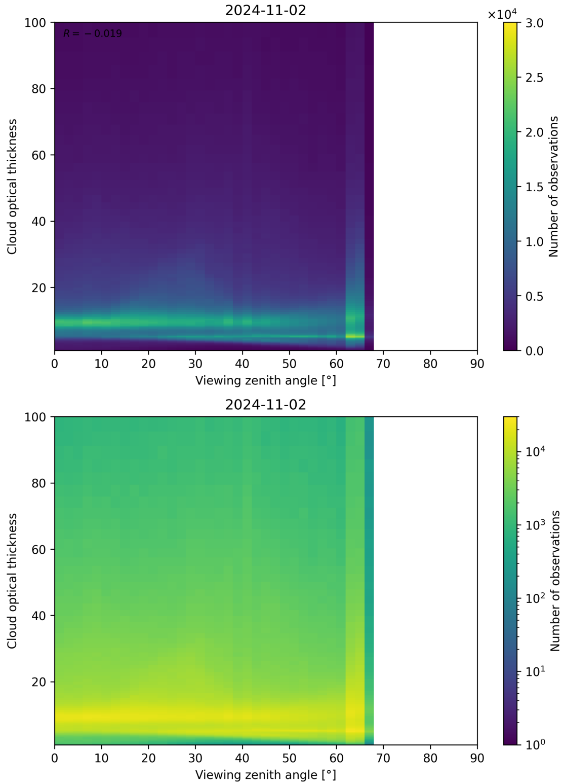
Figure 111: Scatter density plot of “Viewing zenith angle” against “Cloud optical thickness” for 2024-11-01 to 2024-11-03.
