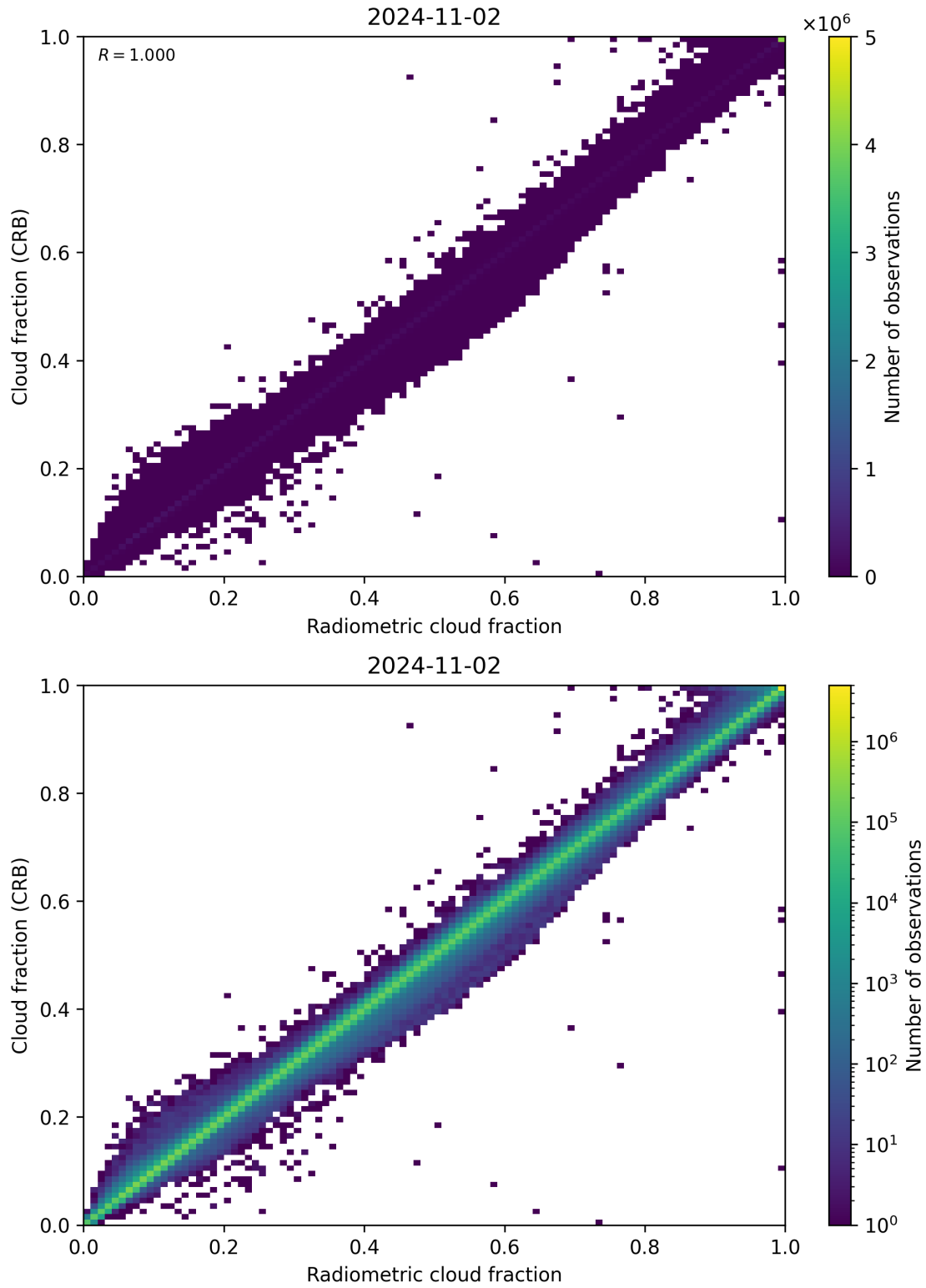
Figure 73: Scatter density plot of “Radiometric cloud fraction” against “Cloud fraction (CRB)” for 2024-11-01 to 2024-11-03.
