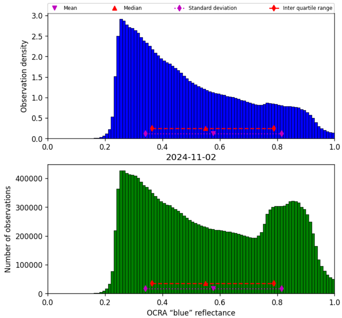
Figure 51: Histogram of “OCRA “blue” reflectance” for 2024-11-01 to 2024-11-03
