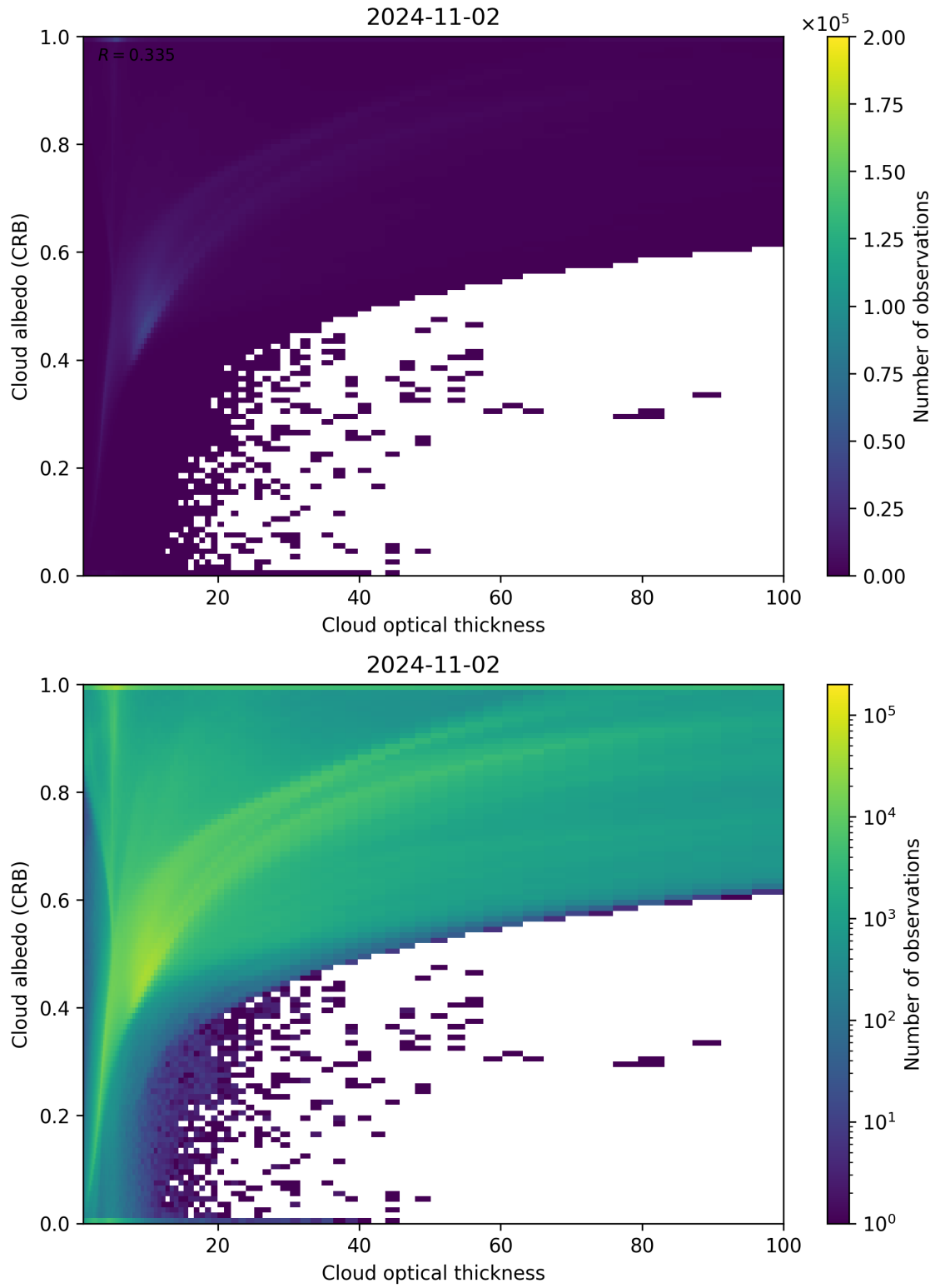
Figure 82: Scatter density plot of “Cloud optical thickness” against “Cloud albedo (CRB)” for 2024-11-01 to 2024-11-03.
