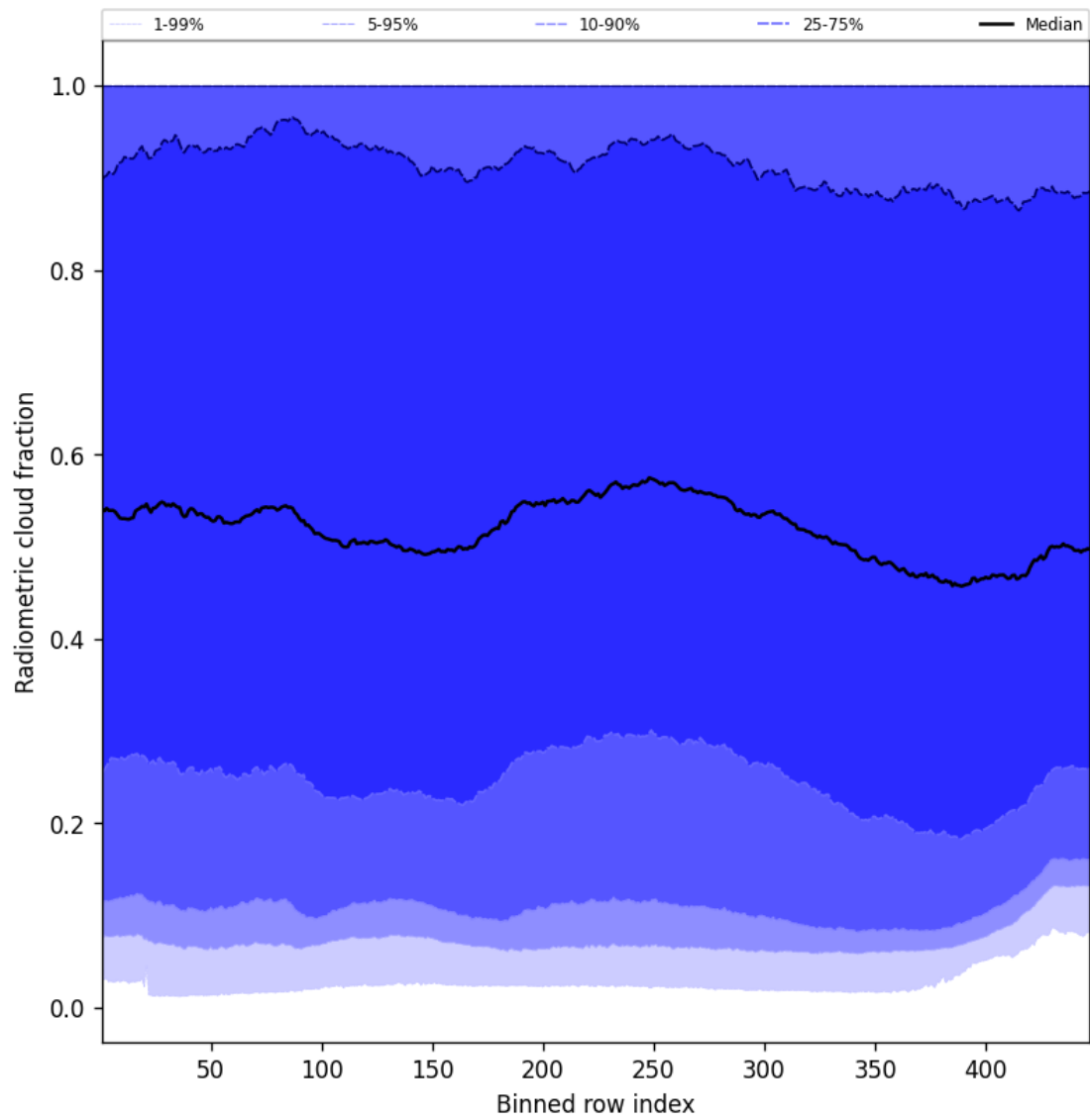
Figure 55: Along track statistics of “Radiometric cloud fraction” for 2024-11-01 to 2024-11-03
