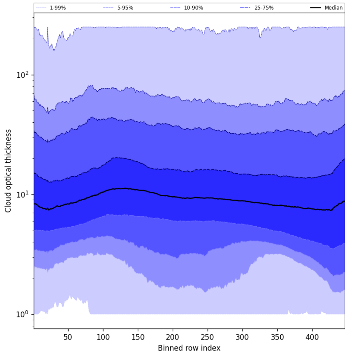
Figure 57: Along track statistics of “Cloud optical thickness” for 2024-11-01 to 2024-11-03
