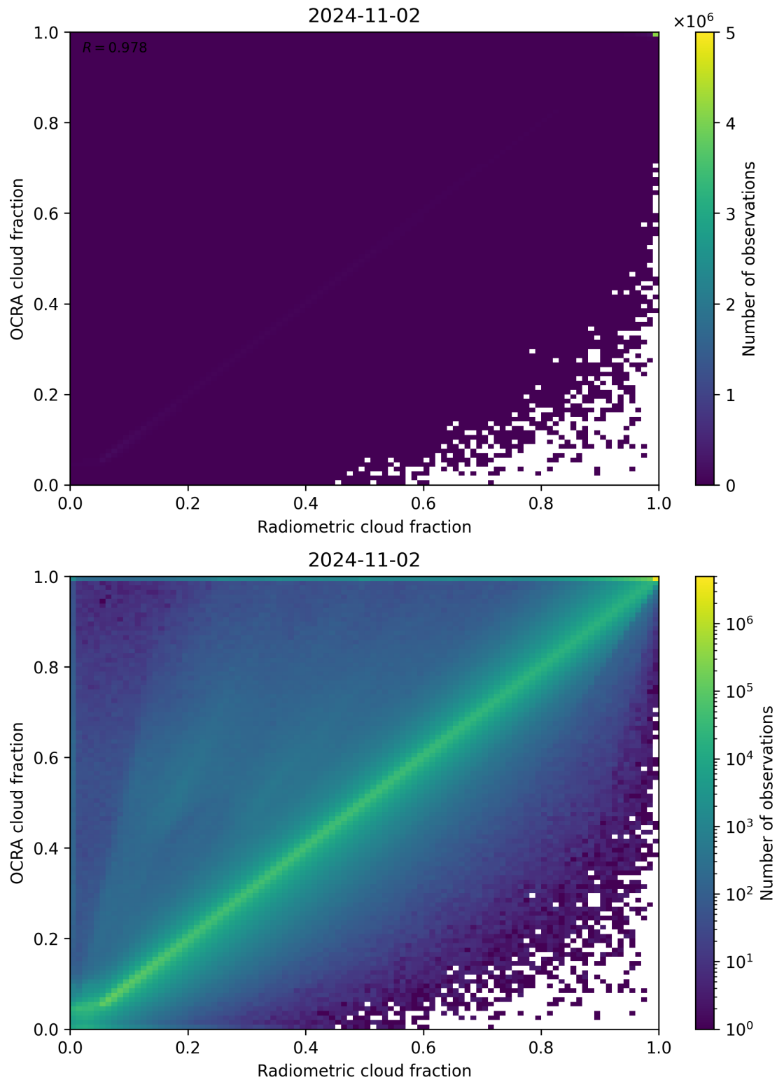
Figure 72: Scatter density plot of “Radiometric cloud fraction” against “OCRA cloud fraction” for 2024-11-01 to 2024-11-03.
