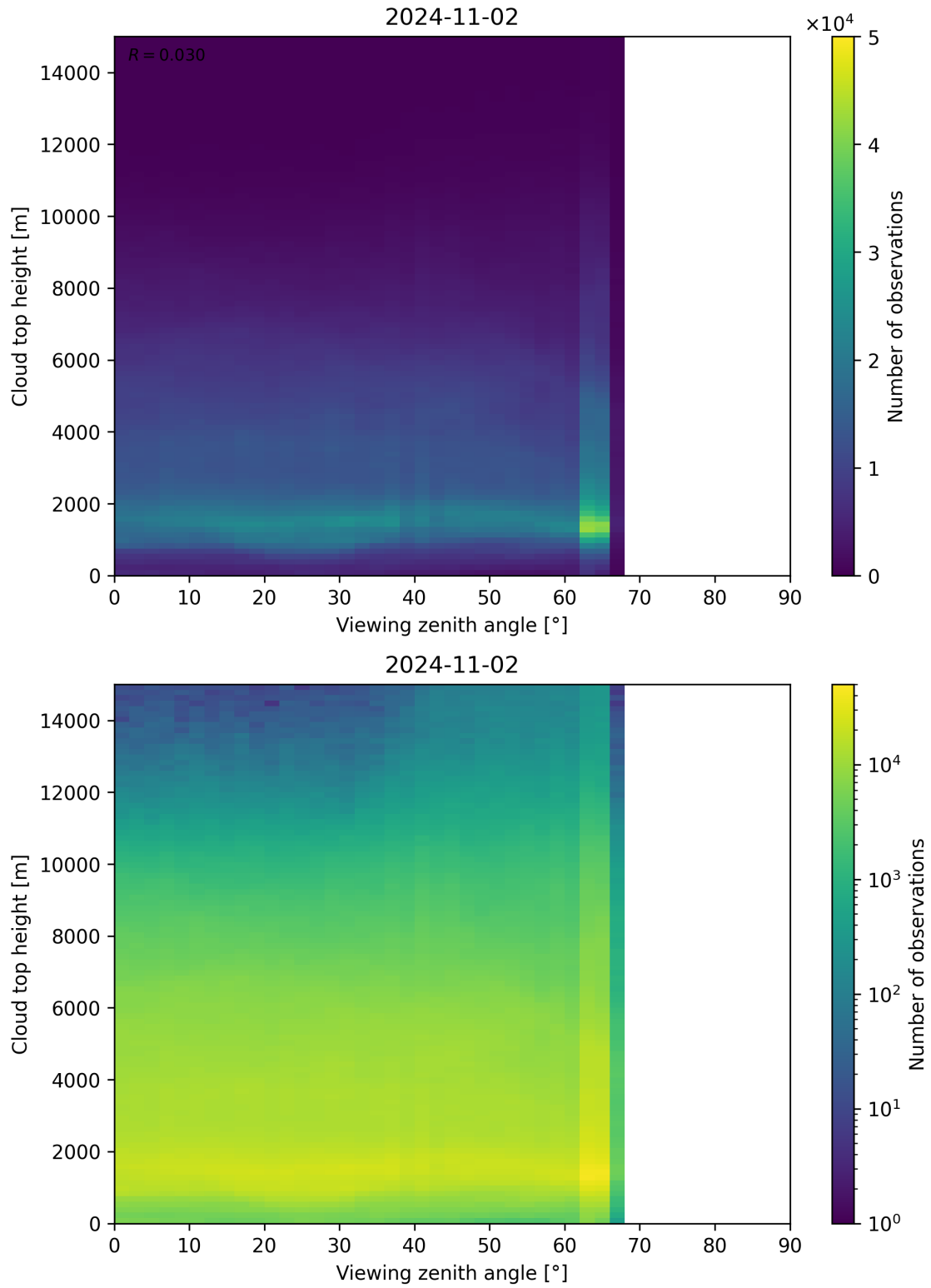
Figure 112: Scatter density plot of “Viewing zenith angle” against “Cloud top height” for 2024-11-01 to 2024-11-03.
