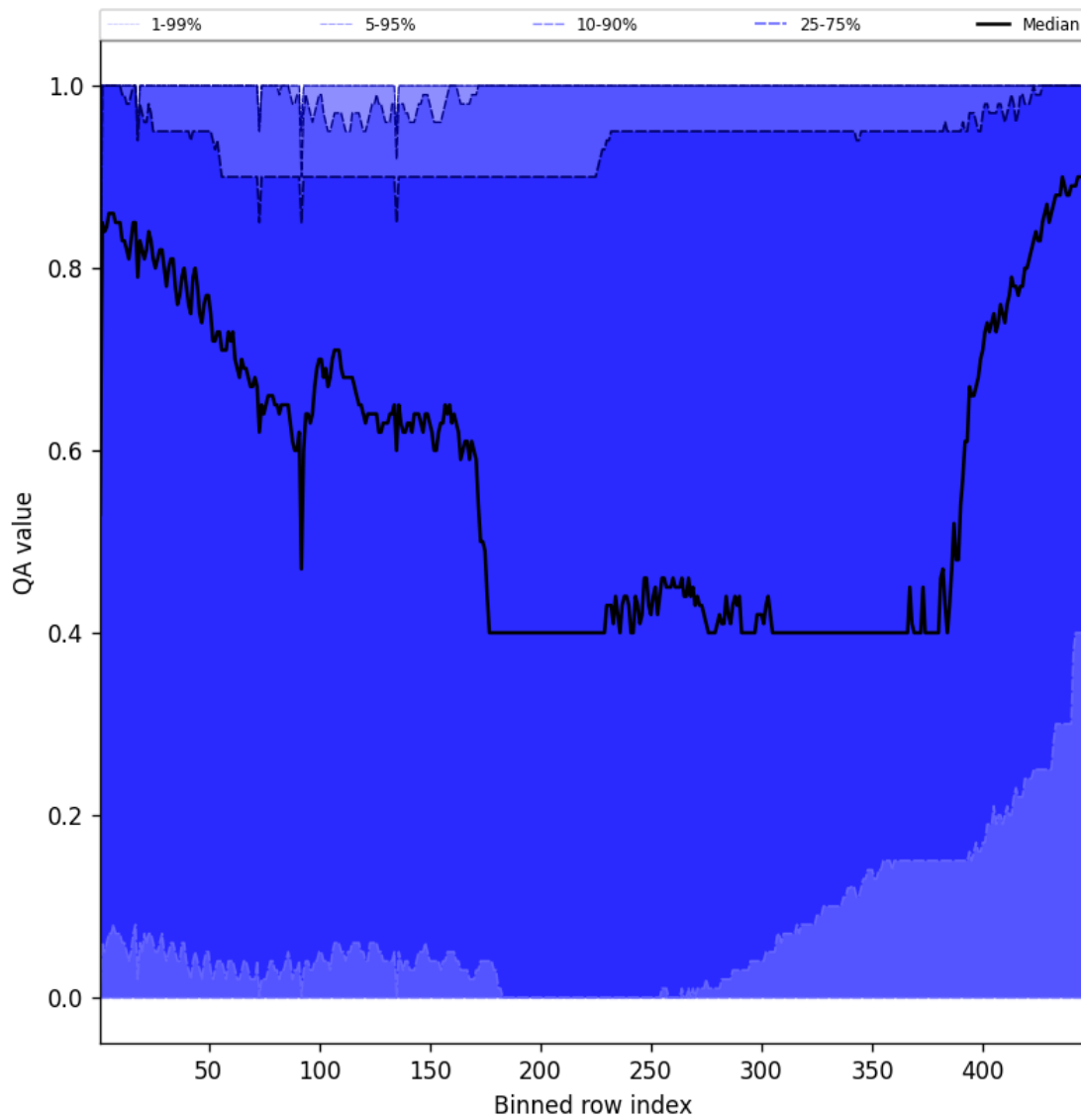
Figure 54: Along track statistics of “QA value” for 2024-11-01 to 2024-11-03
