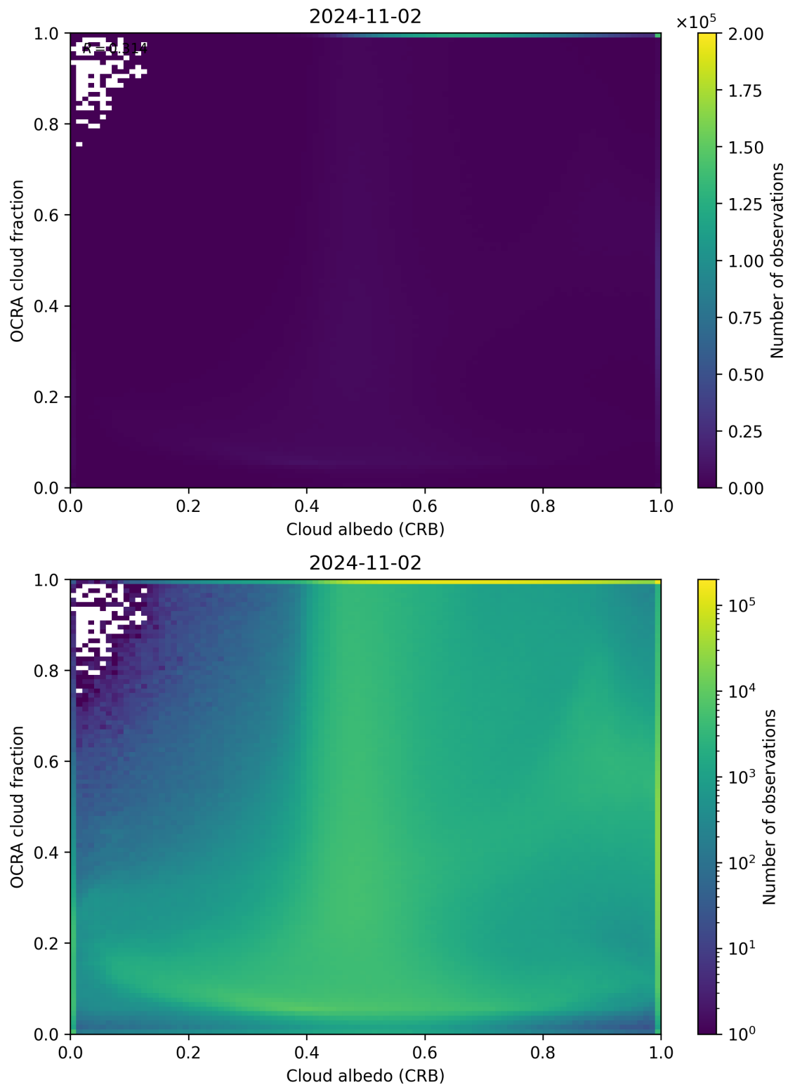
Figure 70: Scatter density plot of “Cloud albedo (CRB)” against “OCRA cloud fraction” for 2024-11-01 to 2024-11-03.
