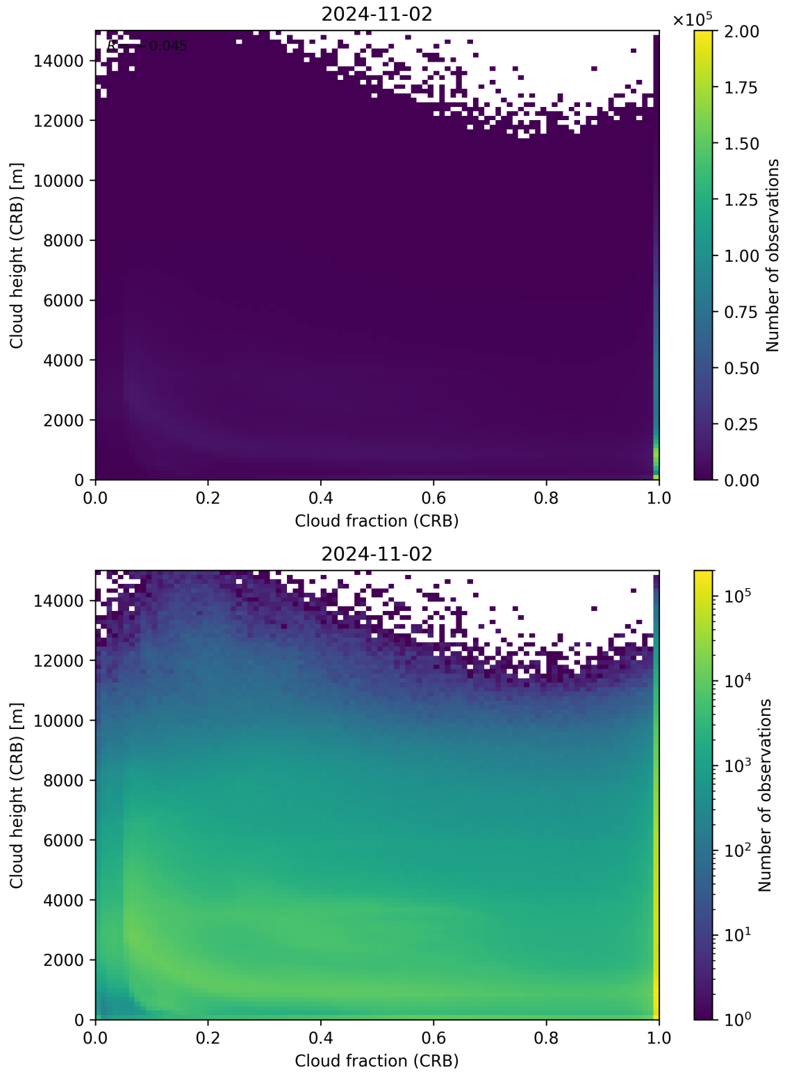
Figure 79: Scatter density plot of “Cloud fraction (CRB)” against “Cloud height (CRB)” for 2024-11-01 to 2024-11-03.
