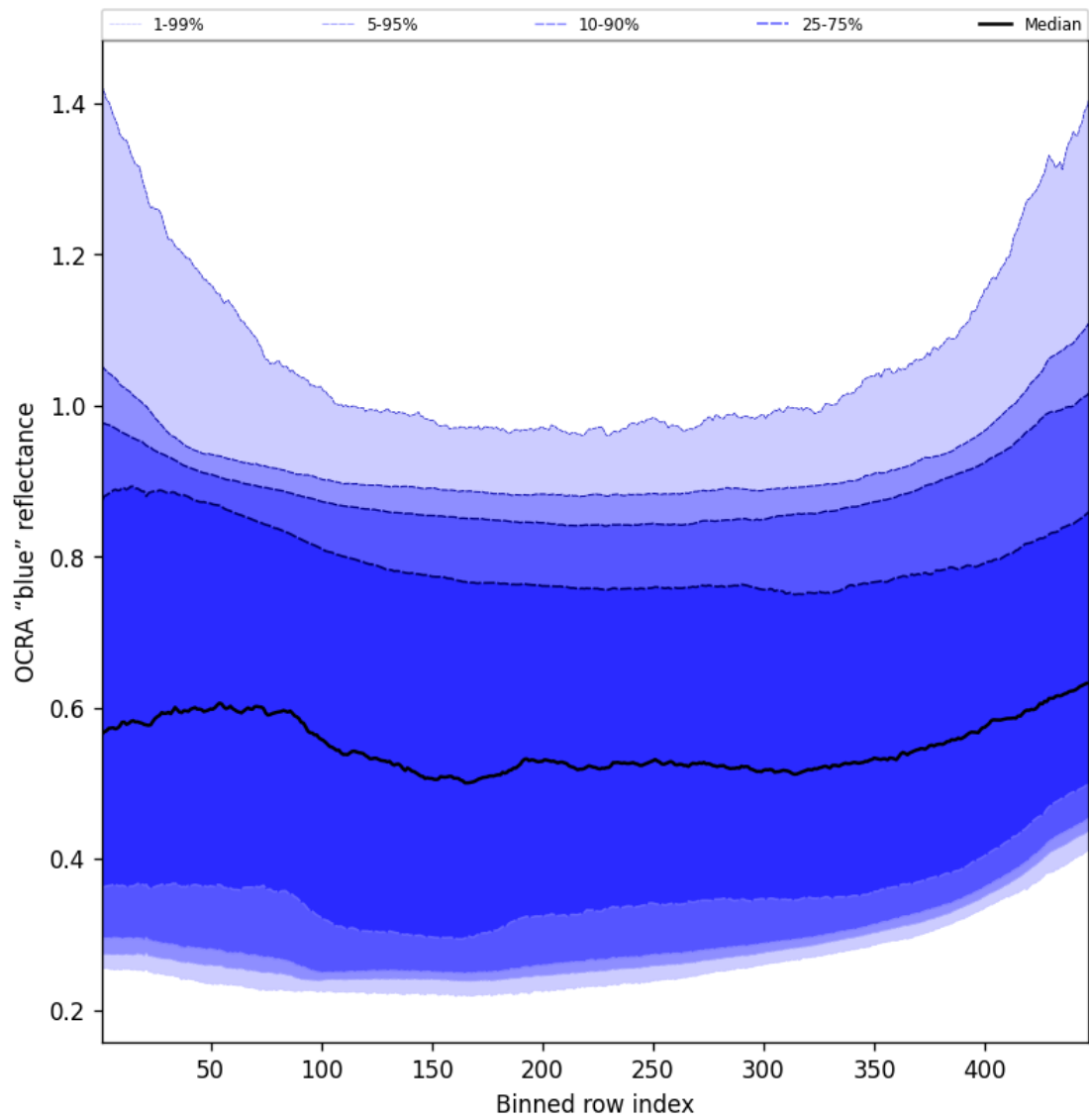
Figure 67: Along track statistics of “OCRA “blue” reflectance” for 2024-11-01 to 2024-11-03
