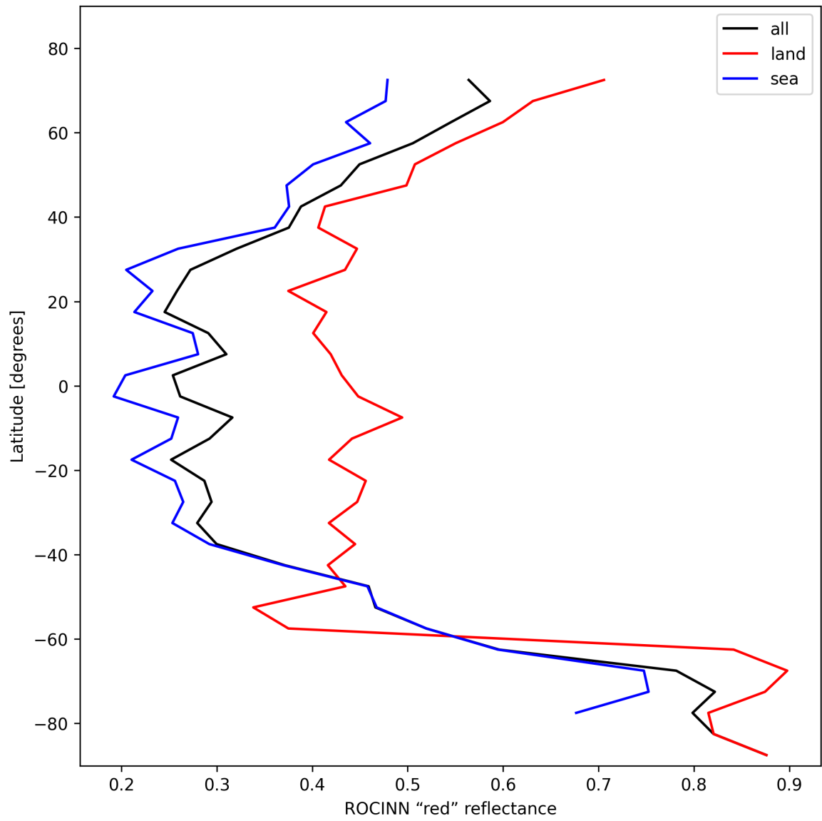
Figure 37: Zonal average of “ROCINN “red” reflectance” for 2024-11-01 to 2024-11-03.
