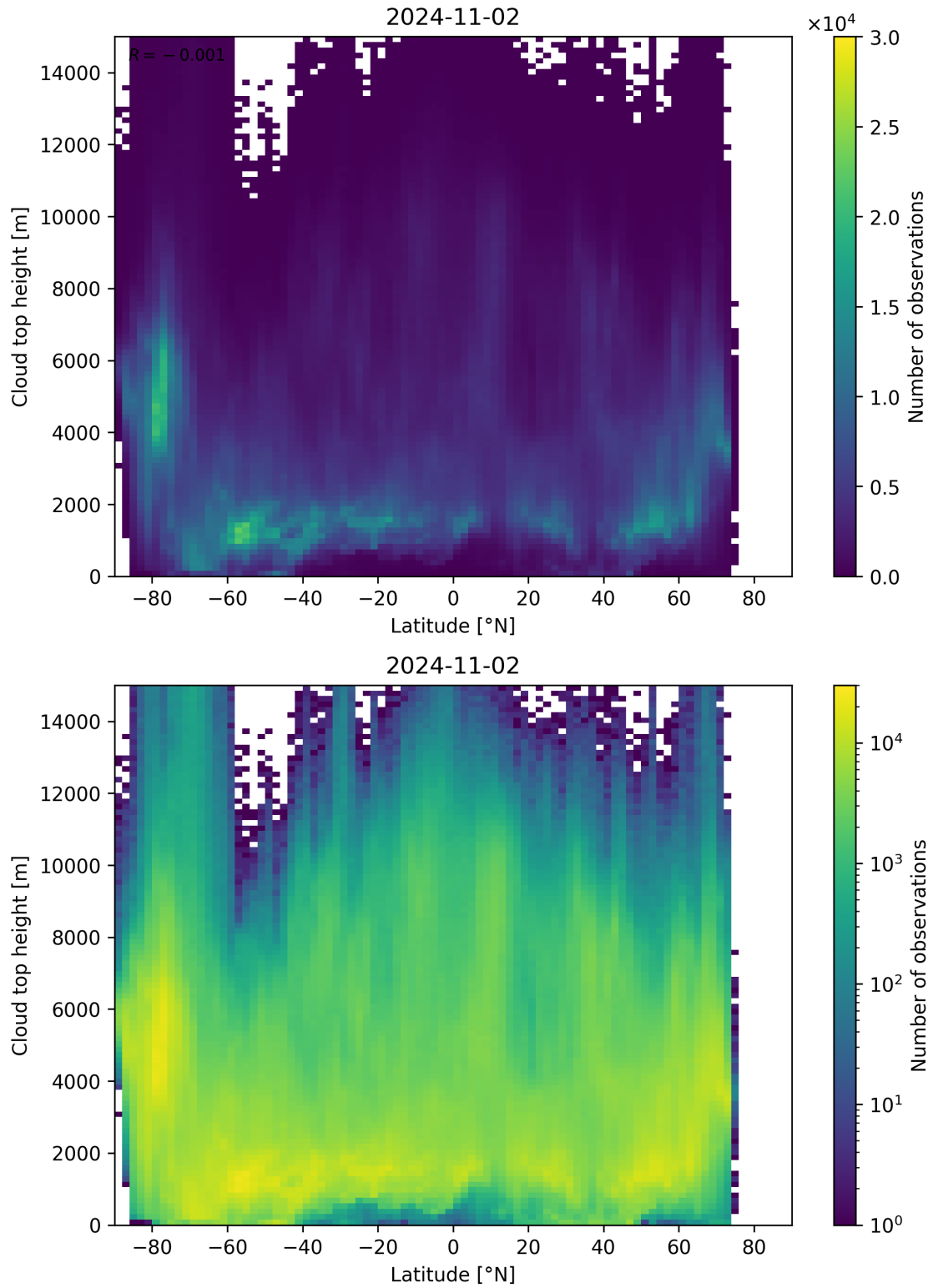
Figure 97: Scatter density plot of “Latitude” against “Cloud top height” for 2024-11-01 to 2024-11-03.
