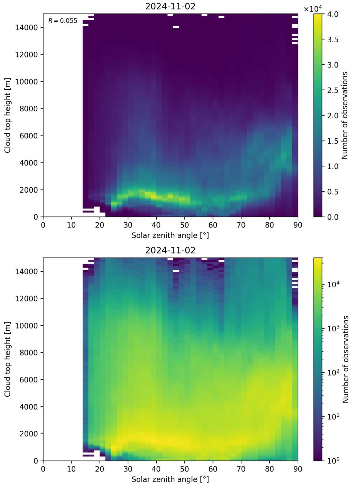
Figure 104: Scatter density plot of “Solar zenith angle” against “Cloud top height” for 2024-11-01 to 2024-11-03.
