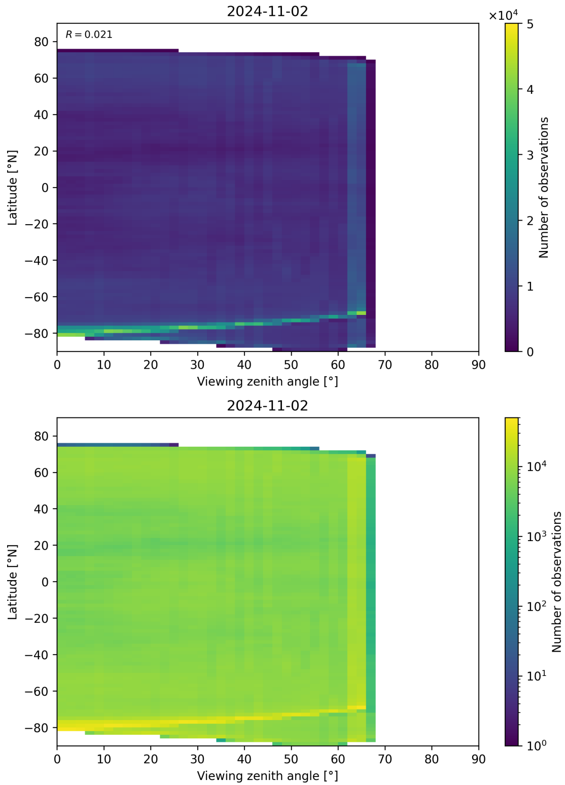
Figure 113: Scatter density plot of “Viewing zenith angle” against “Latitude” for 2024-11-01 to 2024-11-03.
