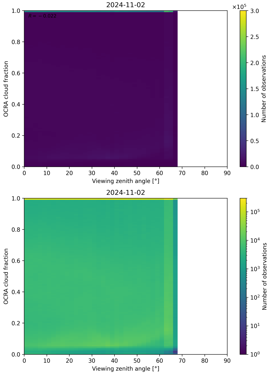
Figure 108: Scatter density plot of “Viewing zenith angle” against “OCRA cloud fraction” for 2024-11-01 to 2024-11-03.
