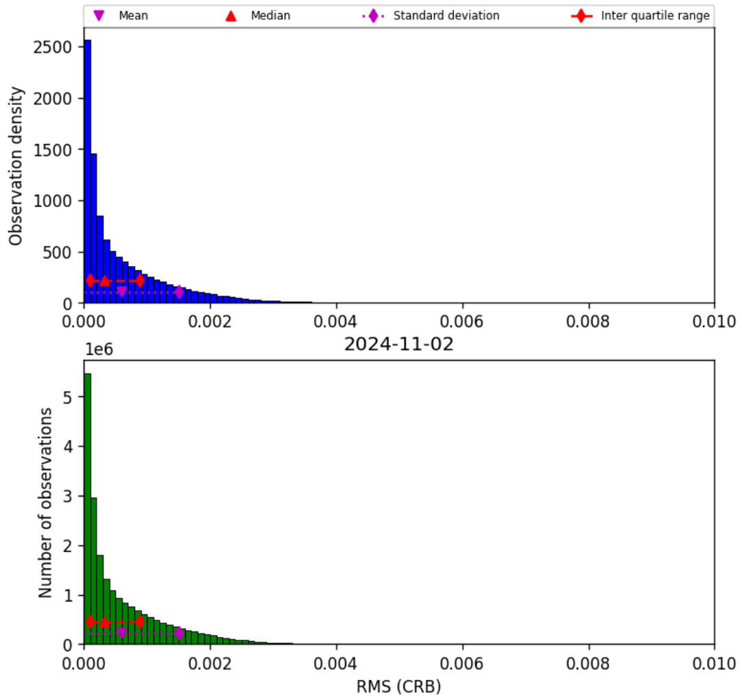
Figure 48: Histogram of “RMS (CRB)” for 2024-11-01 to 2024-11-03
