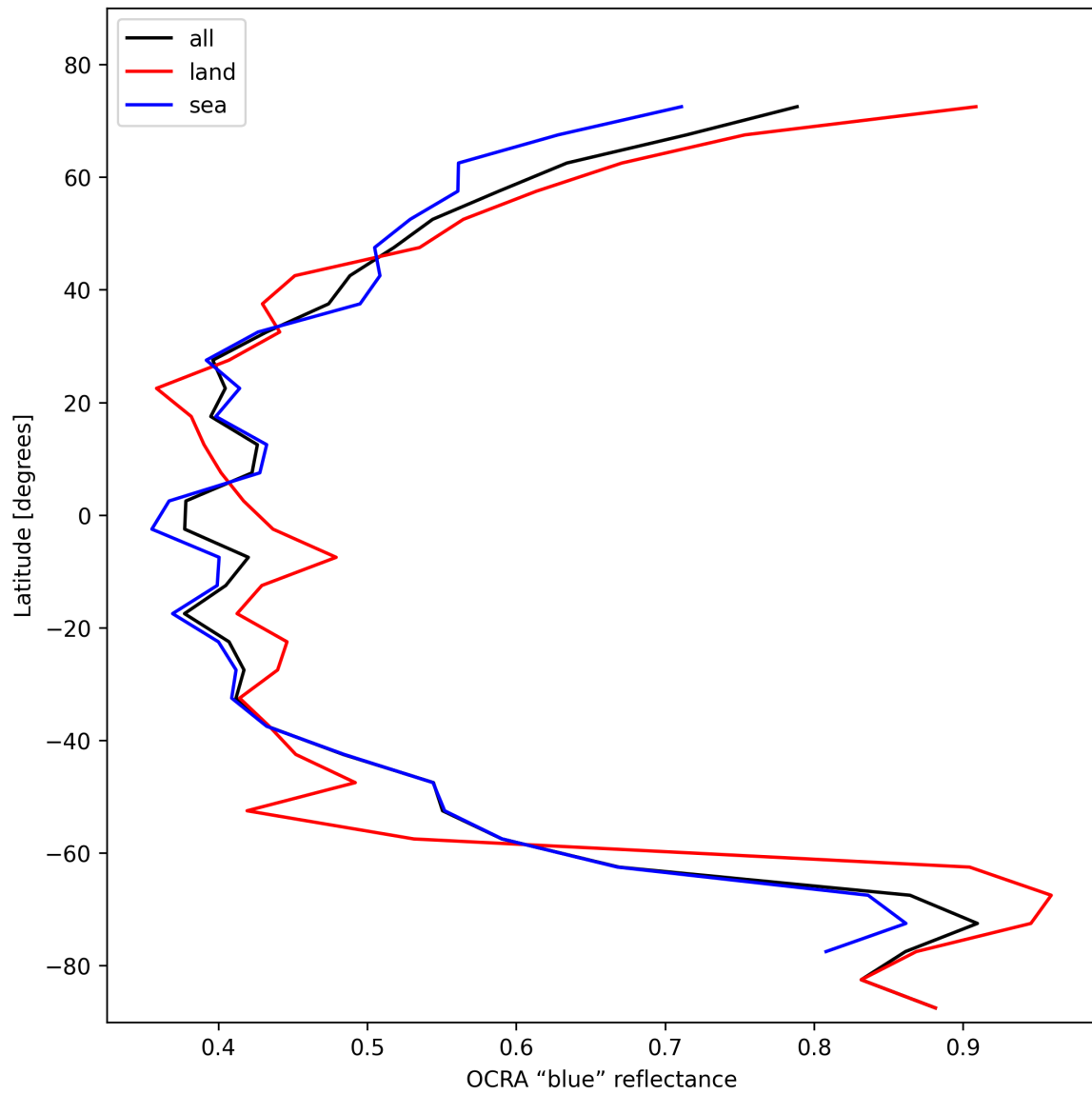
Figure 35: Zonal average of “OCRA “blue” reflectance” for 2024-11-01 to 2024-11-03.
