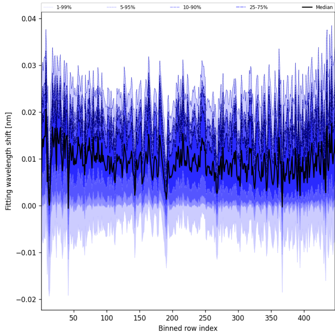
Figure 65: Along track statistics of “Fitting wavelength shift” for 2024-11-01 to 2024-11-03
