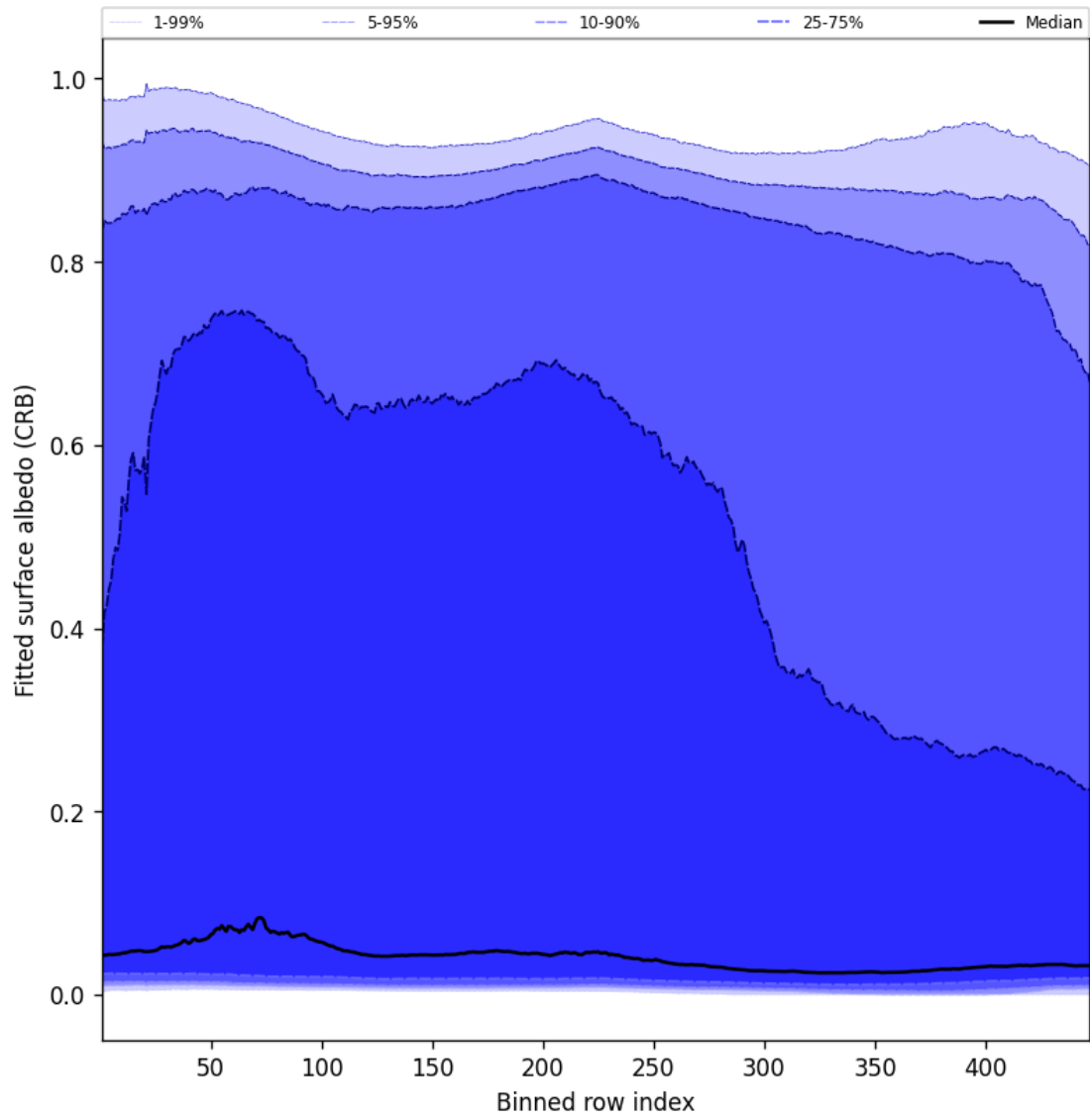
Figure 62: Along track statistics of “Fitted surface albedo (CRB)” for 2024-11-01 to 2024-11-03
