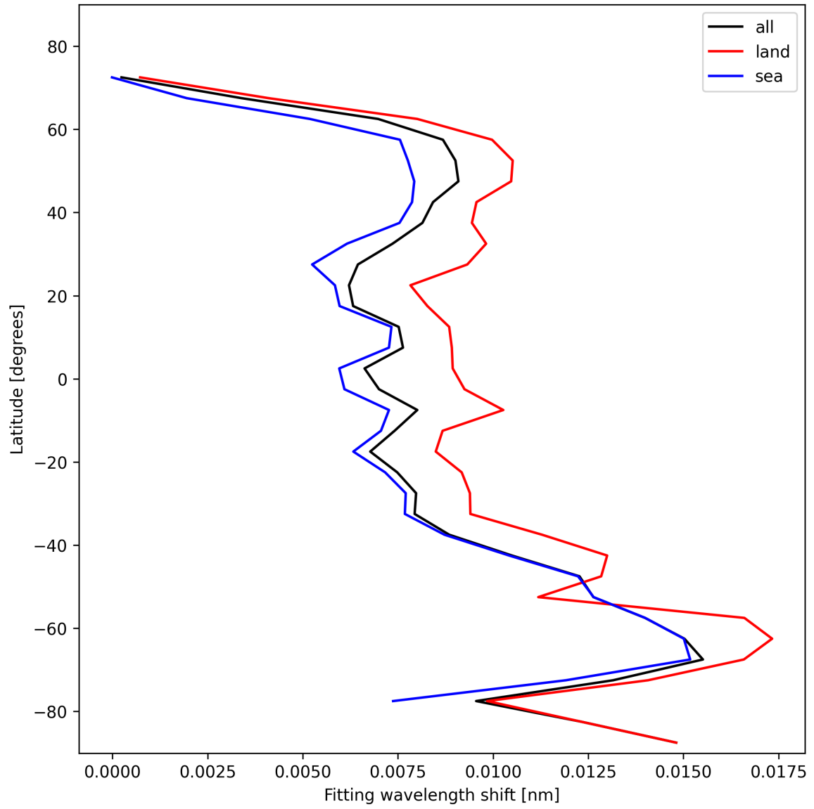
Figure 33: Zonal average of “Fitting wavelength shift” for 2024-11-01 to 2024-11-03.
