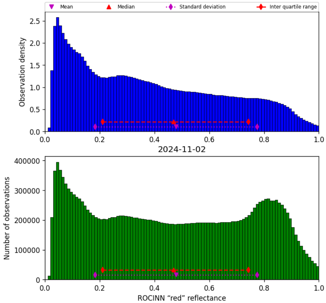
Figure 53: Histogram of “ROCINN “red” reflectance” for 2024-11-01 to 2024-11-03
