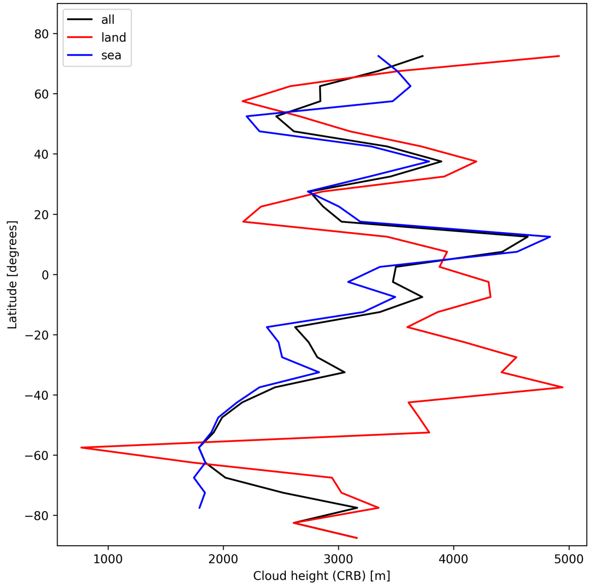
Figure 27: Zonal average of “Cloud height (CRB)” for 2024-11-01 to 2024-11-03.
