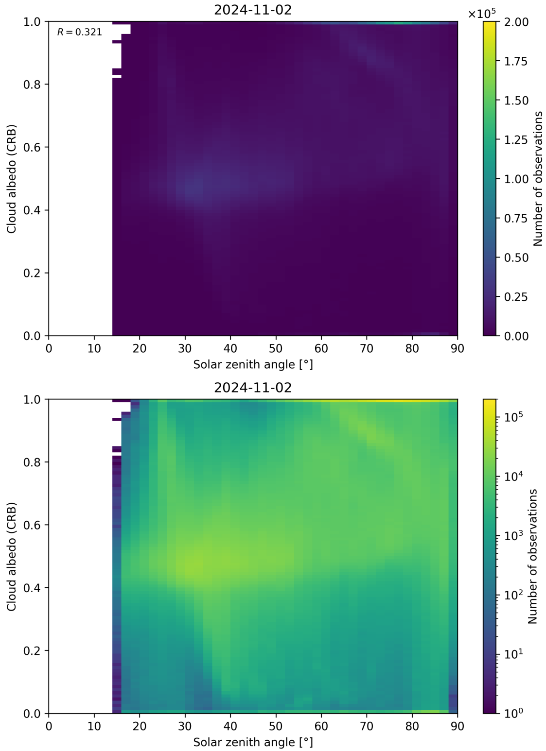
Figure 98: Scatter density plot of “Solar zenith angle” against “Cloud albedo (CRB)” for 2024-11-01 to 2024-11-03.
