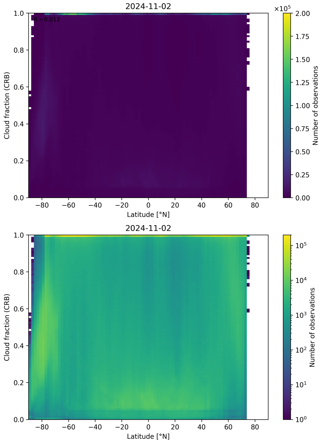
Figure 94: Scatter density plot of “Latitude” against “Cloud fraction (CRB)” for 2024-11-01 to 2024-11-03.
