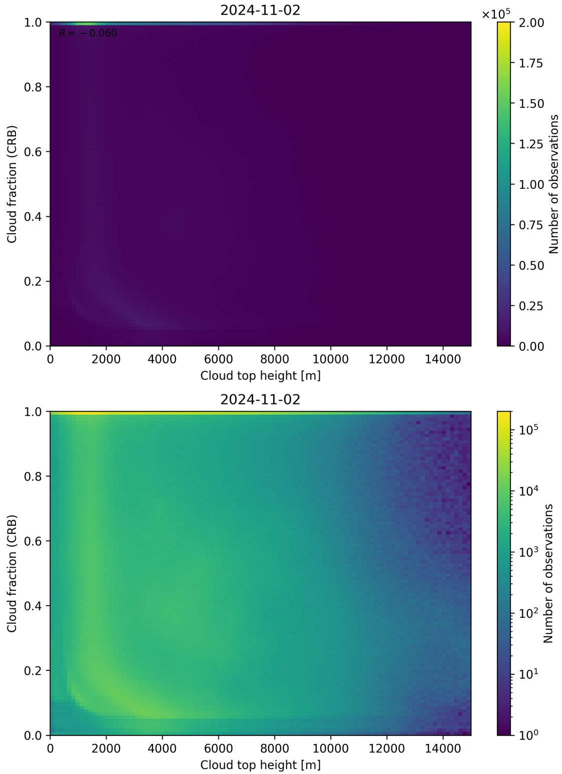
Figure 88: Scatter density plot of “Cloud top height” against “Cloud fraction (CRB)” for 2024-11-01 to 2024-11-03.
