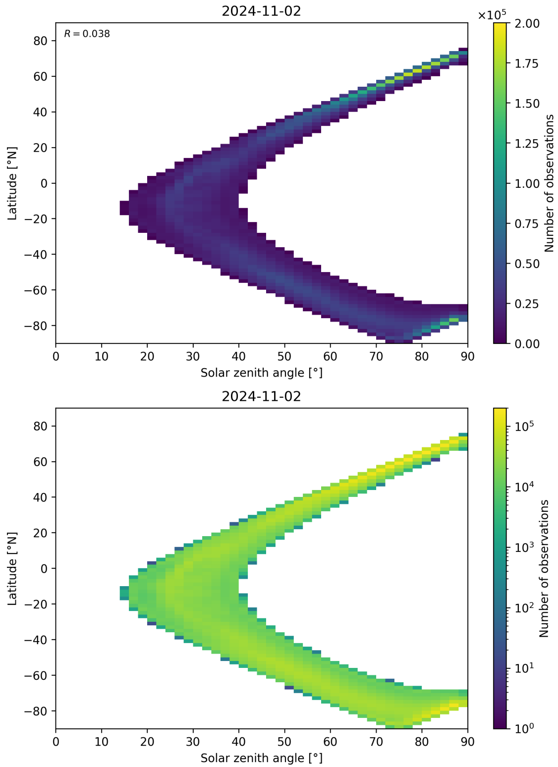
Figure 105: Scatter density plot of “Solar zenith angle” against “Latitude” for 2024-11-01 to 2024-11-03.
