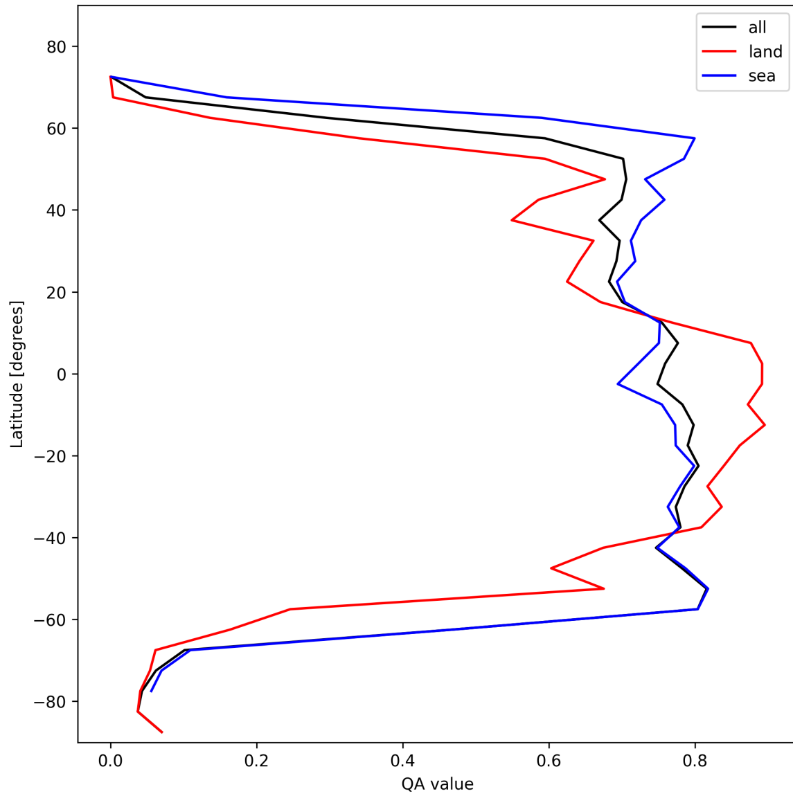
Figure 22: Zonal average of “QA value” for 2024-11-01 to 2024-11-03.
