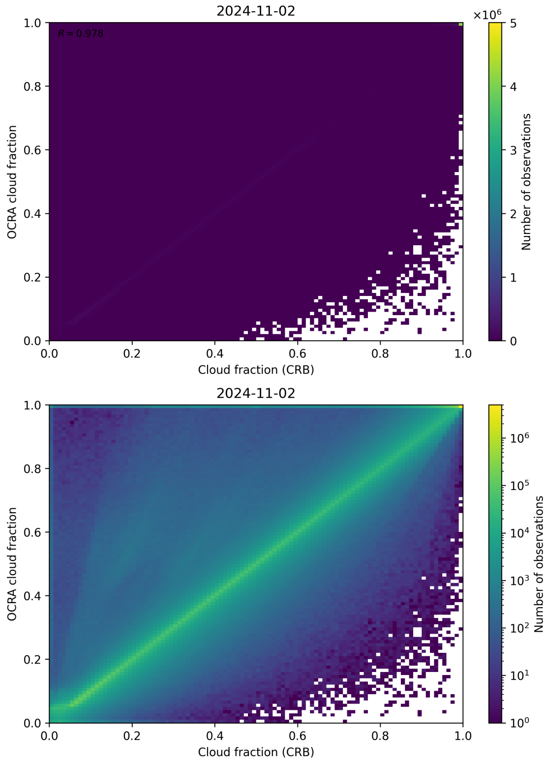
Figure 78: Scatter density plot of “Cloud fraction (CRB)” against “OCRA cloud fraction” for 2024-11-01 to 2024-11-03.
