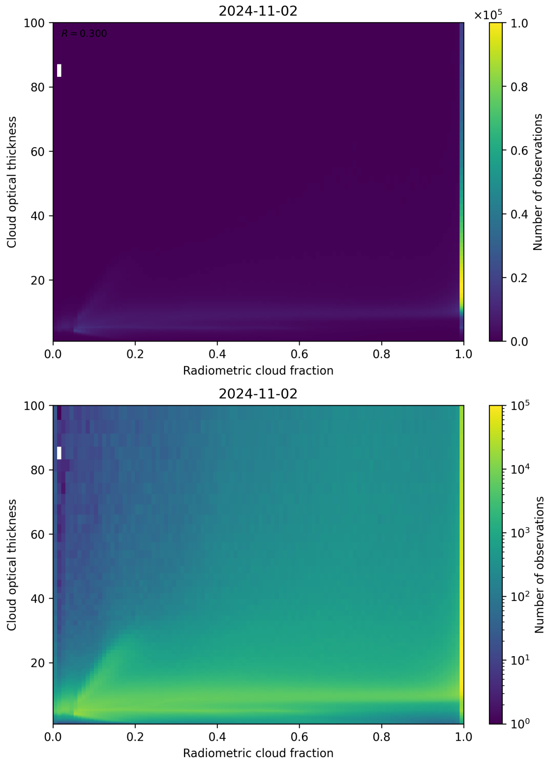
Figure 75: Scatter density plot of “Radiometric cloud fraction” against “Cloud optical thickness” for 2024-11-01 to 2024-11-03.
