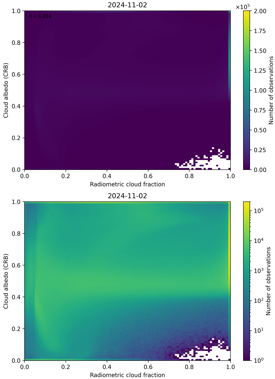
Figure 71: Scatter density plot of “Radiometric cloud fraction” against “Cloud albedo (CRB)” for 2024-11-01 to 2024-11-03.
