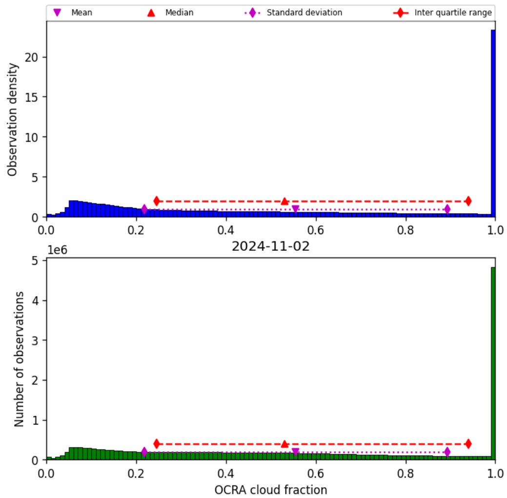
Figure 50: Histogram of “OCRA cloud fraction” for 2024-11-01 to 2024-11-03
