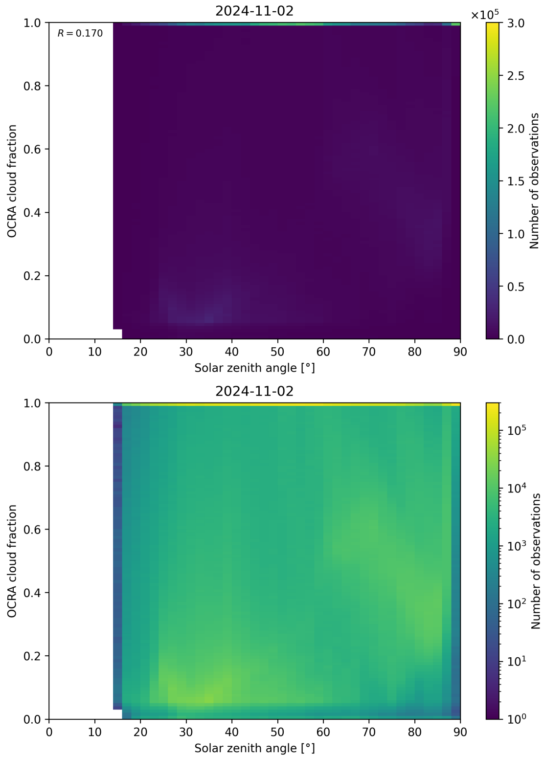
Figure 100: Scatter density plot of “Solar zenith angle” against “OCRA cloud fraction” for 2024-11-01 to 2024-11-03.
