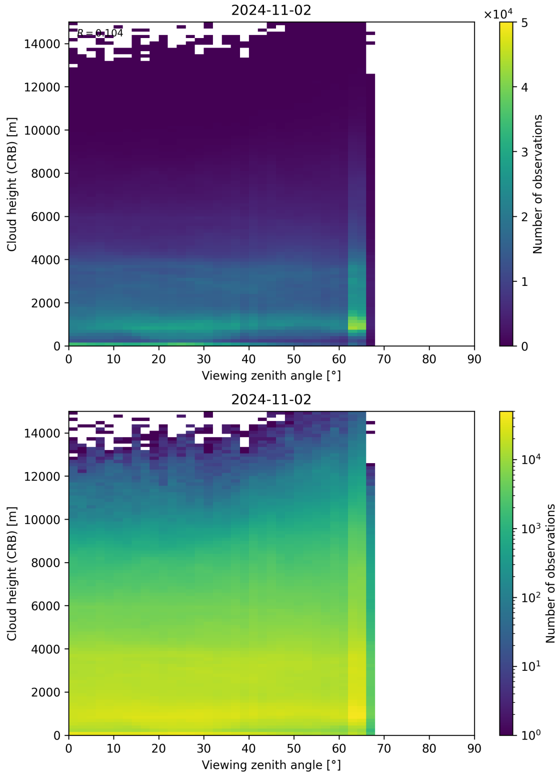
Figure 110: Scatter density plot of “Viewing zenith angle” against “Cloud height (CRB)” for 2024-11-01 to 2024-11-03.
