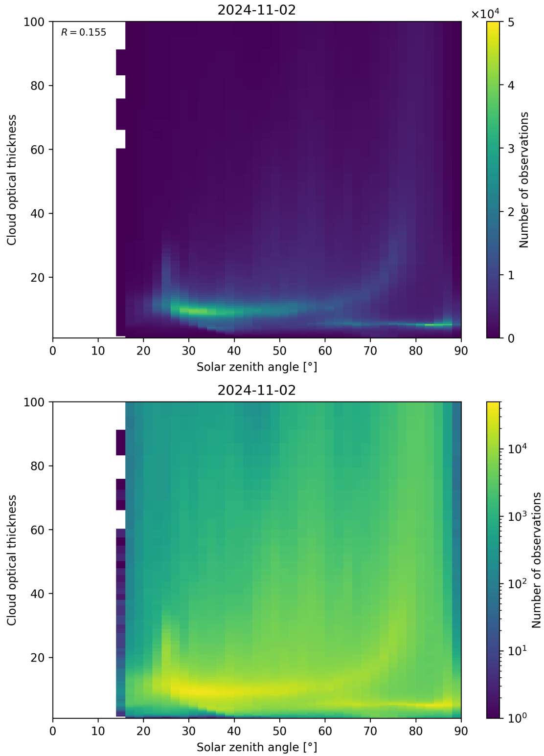
Figure 103: Scatter density plot of “Solar zenith angle” against “Cloud optical thickness” for 2024-11-01 to 2024-11-03.
