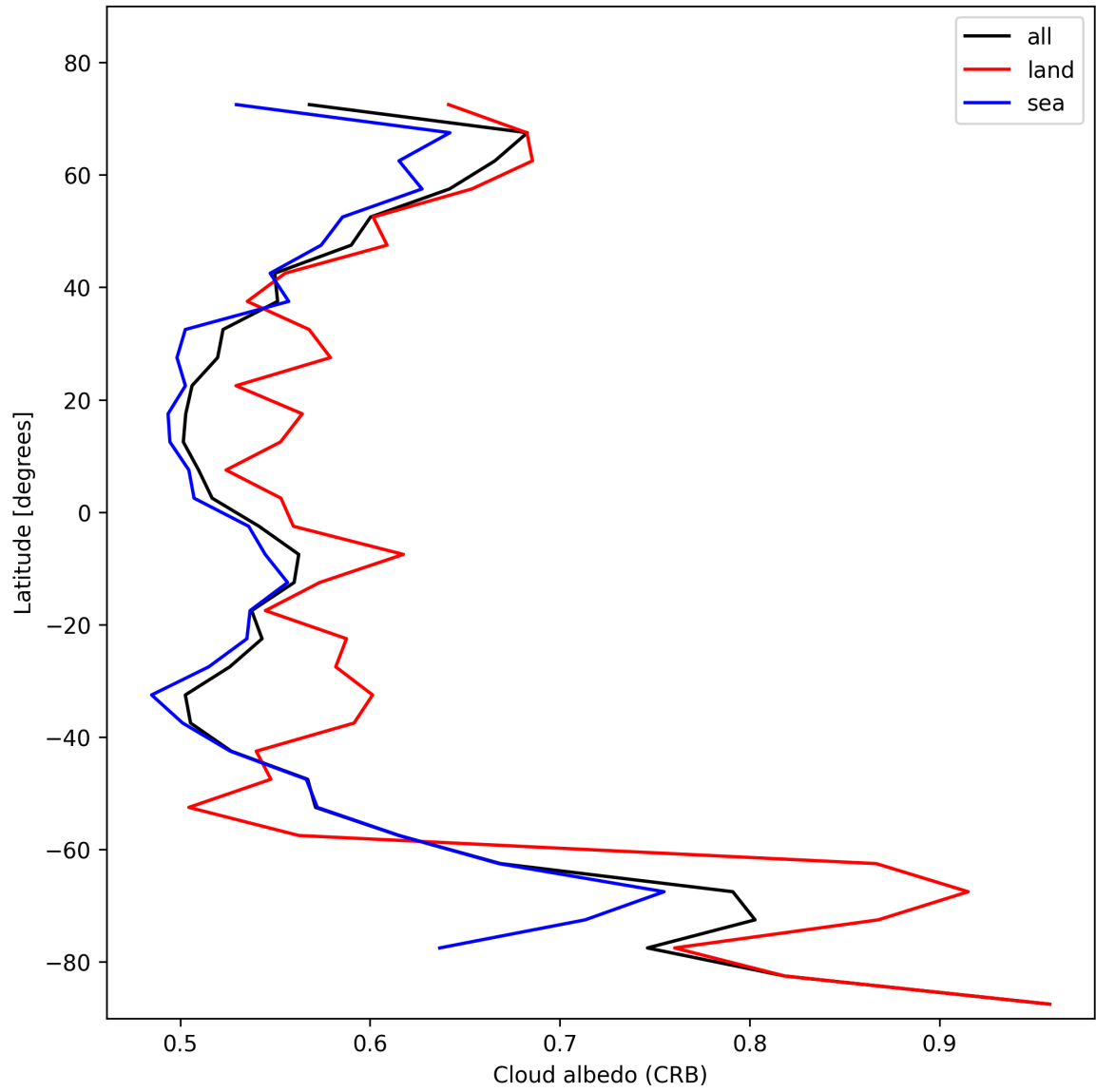
Figure 28: Zonal average of “Cloud albedo (CRB)” for 2024-11-01 to 2024-11-03.
