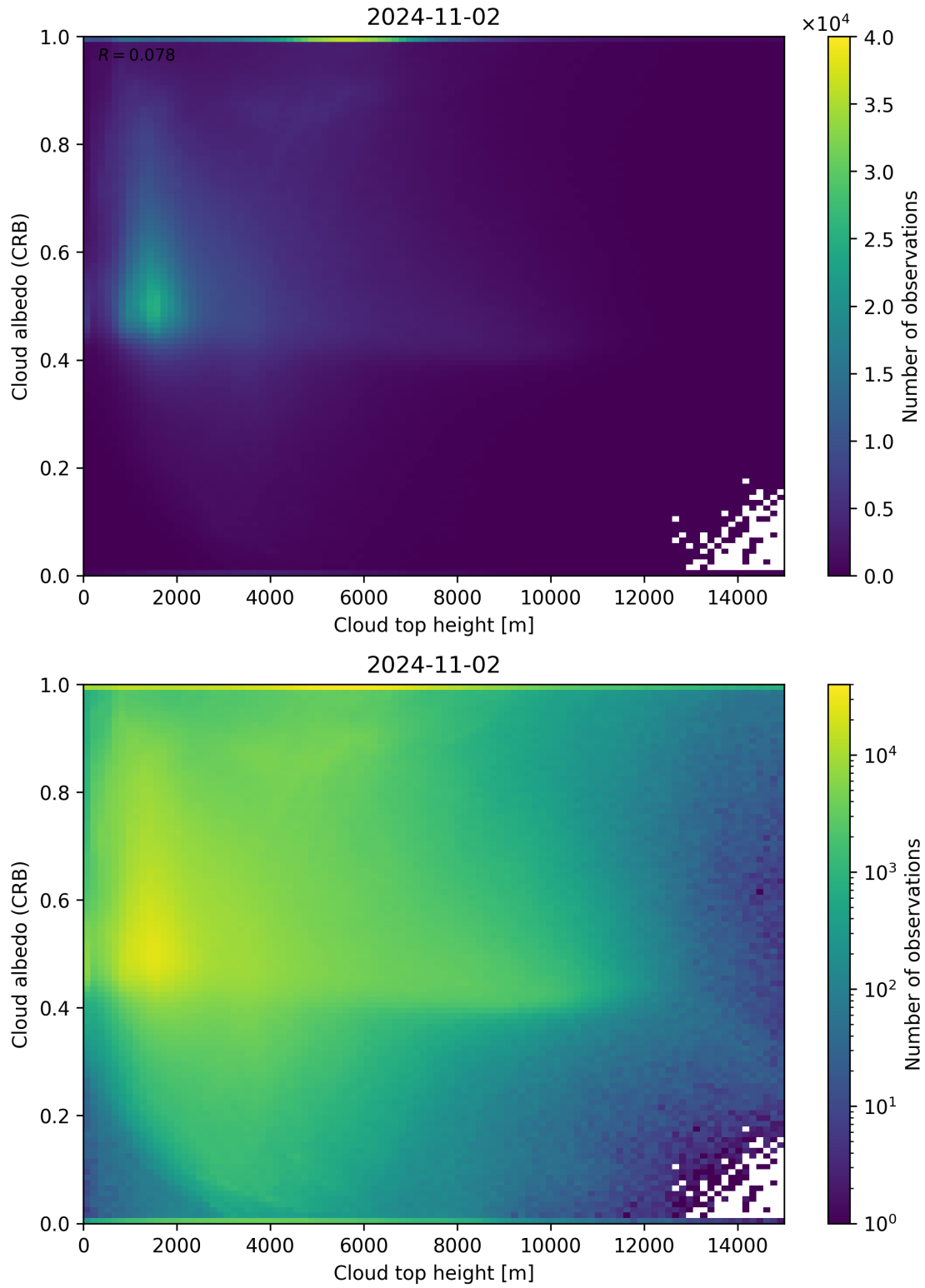
Figure 86: Scatter density plot of “Cloud top height” against “Cloud albedo (CRB)” for 2024-11-01 to 2024-11-03.
