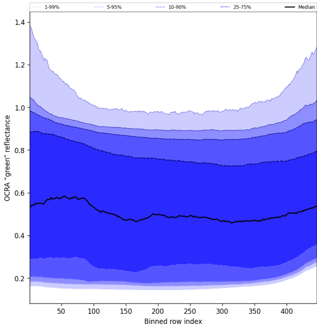
Figure 68: Along track statistics of “OCRA “green” reflectance” for 2024-11-01 to 2024-11-03
