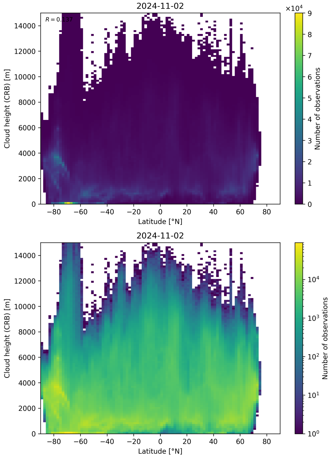
Figure 95: Scatter density plot of “Latitude” against “Cloud height (CRB)” for 2024-11-01 to 2024-11-03.
