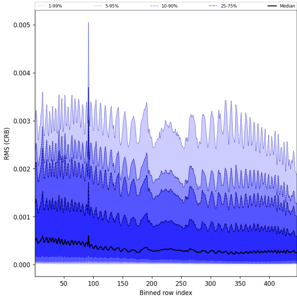
Figure 64: Along track statistics of “RMS (CRB)” for 2024-11-01 to 2024-11-03
