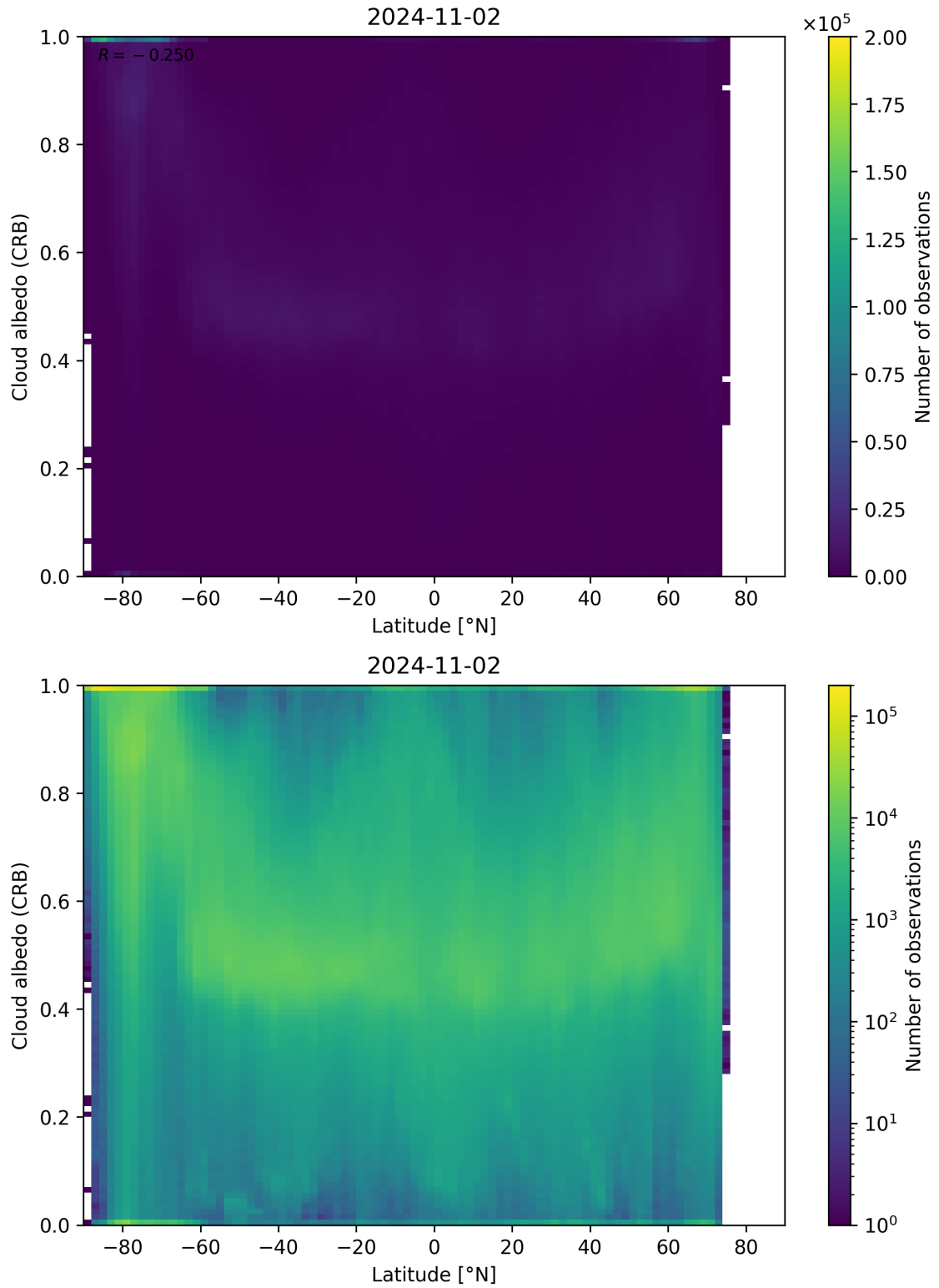
Figure 91: Scatter density plot of “Latitude” against “Cloud albedo (CRB)” for 2024-11-01 to 2024-11-03.
