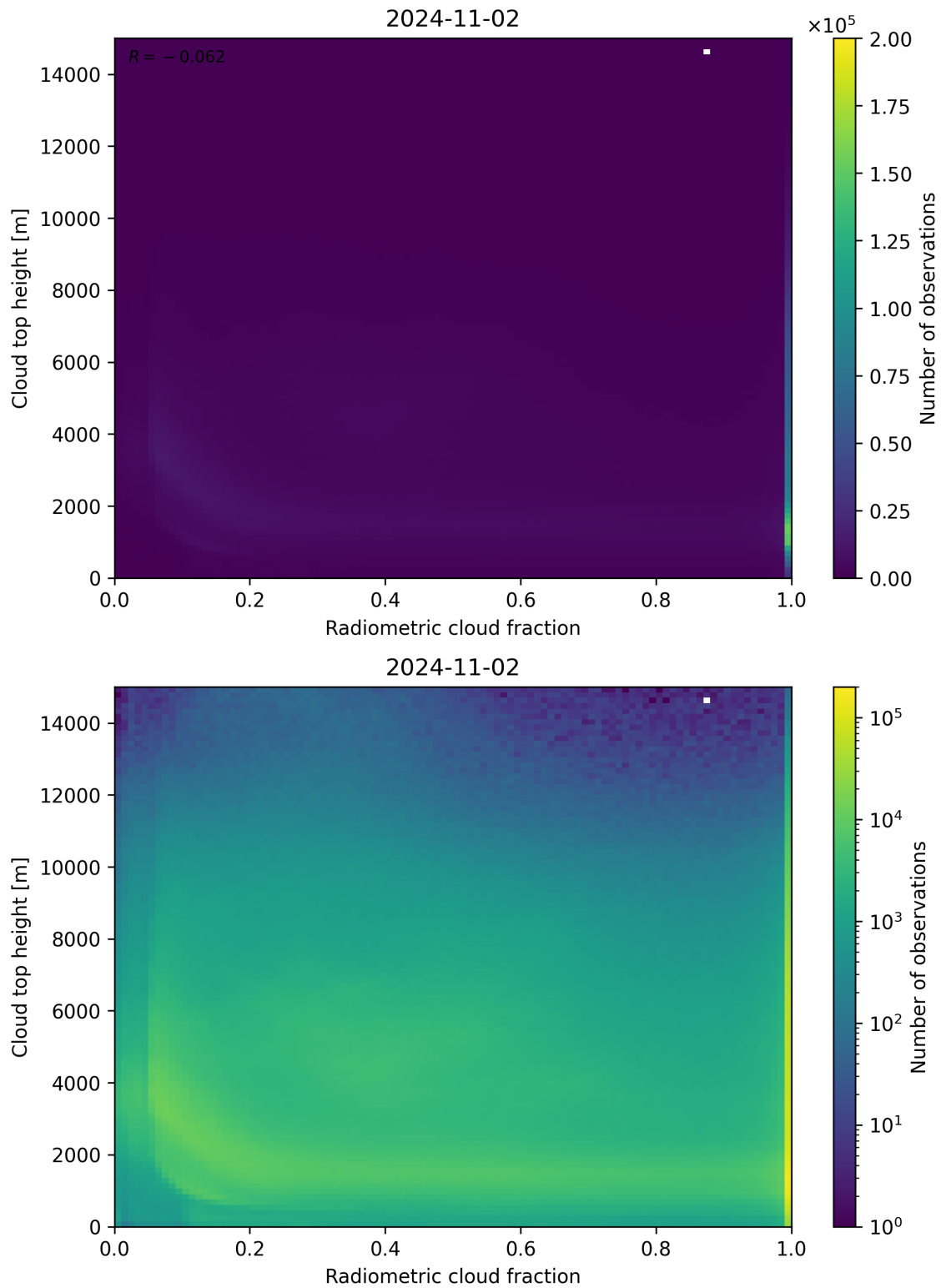
Figure 76: Scatter density plot of “Radiometric cloud fraction” against “Cloud top height” for 2024-11-01 to 2024-11-03.
