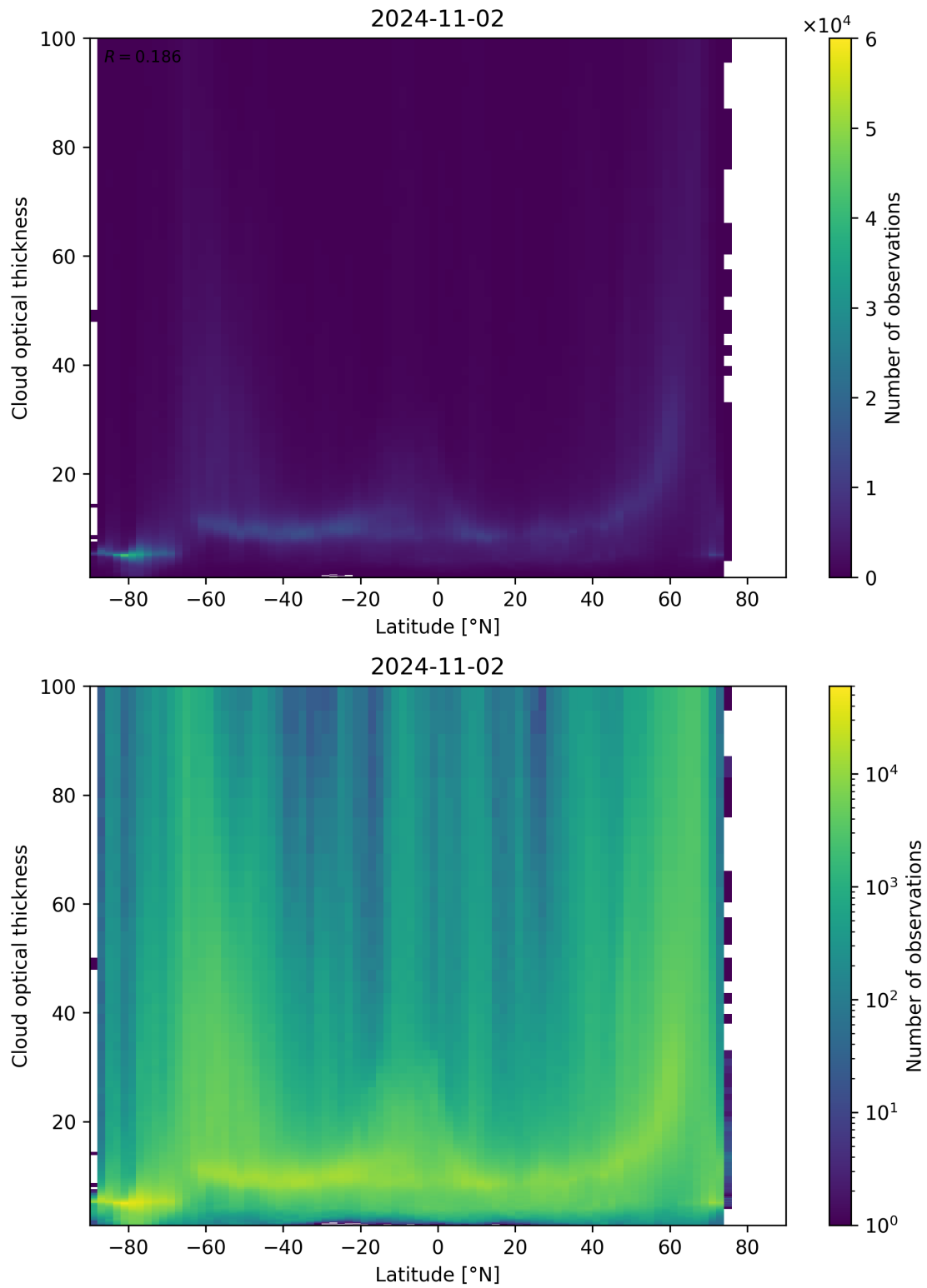
Figure 96: Scatter density plot of “Latitude” against “Cloud optical thickness” for 2024-11-01 to 2024-11-03.
