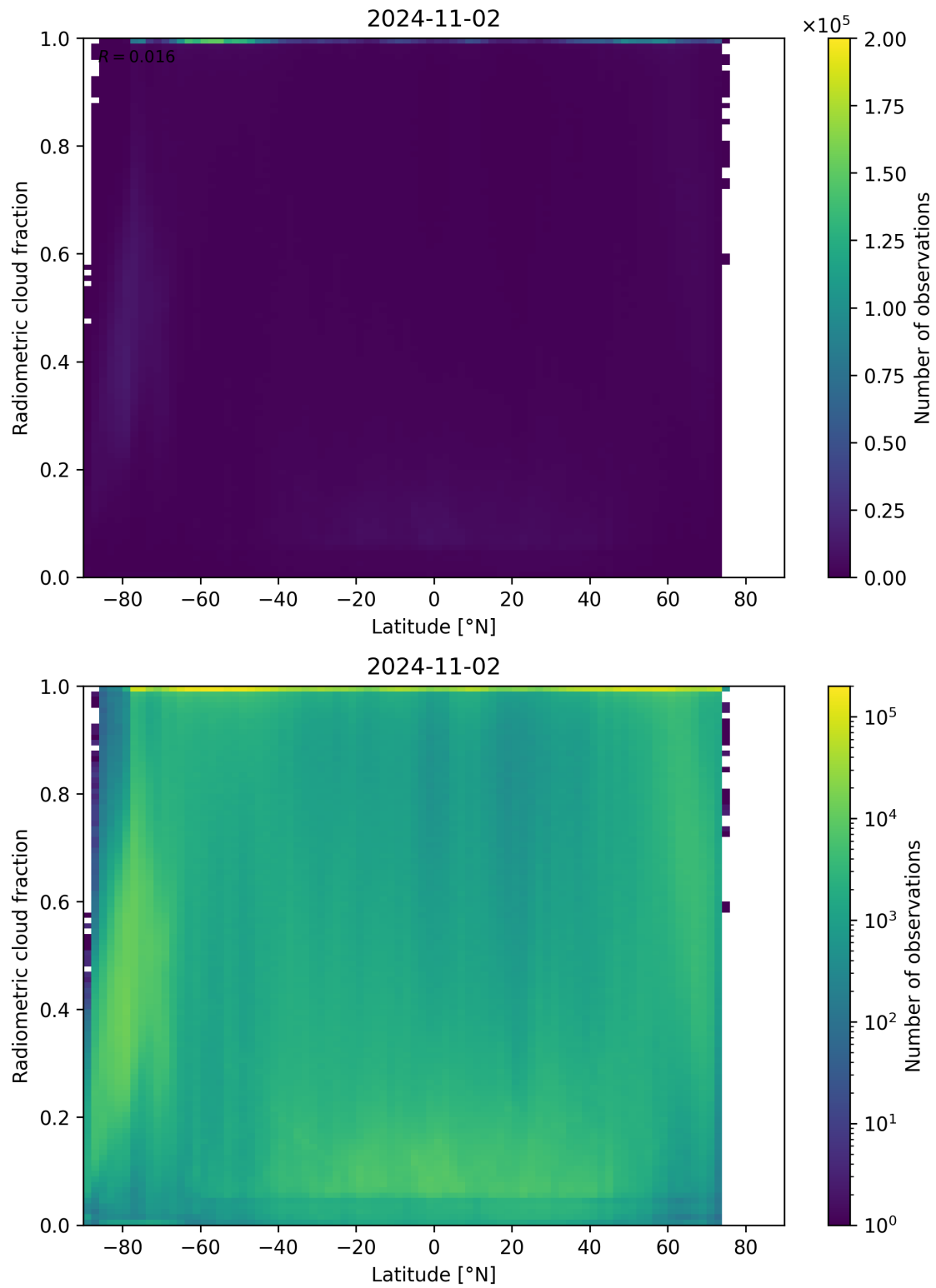
Figure 92: Scatter density plot of “Latitude” against “Radiometric cloud fraction” for 2024-11-01 to 2024-11-03.
