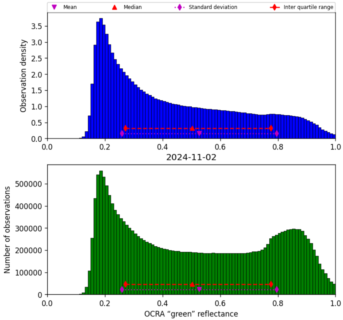
Figure 52: Histogram of “OCRA “green” reflectance” for 2024-11-01 to 2024-11-03
