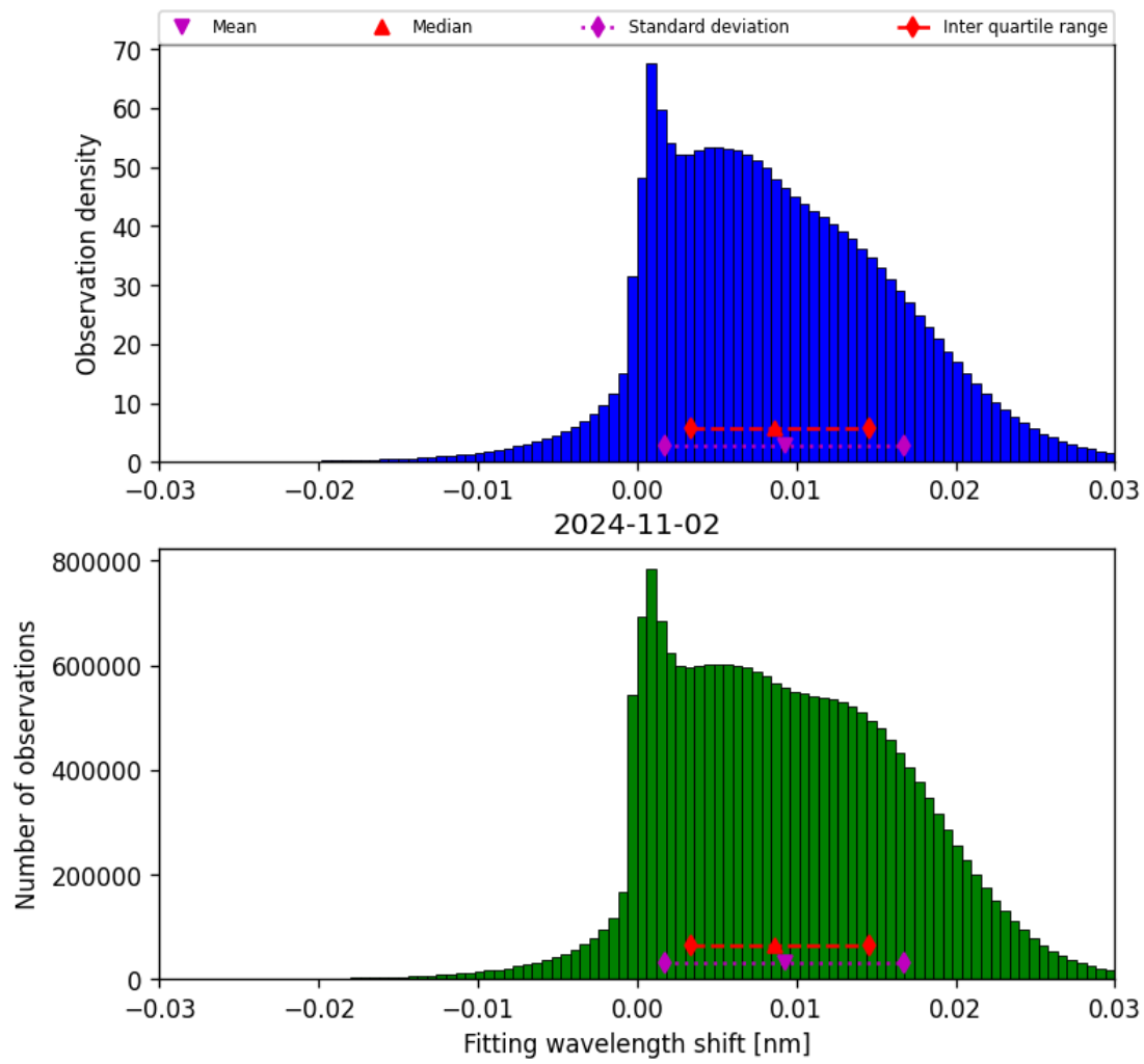
Figure 49: Histogram of “Fitting wavelength shift” for 2024-11-01 to 2024-11-03
