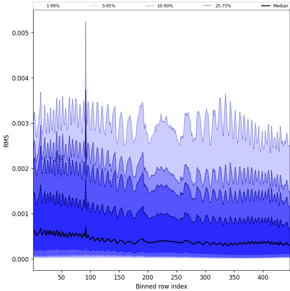
Figure 63: Along track statistics of “RMS” for 2024-11-01 to 2024-11-03
