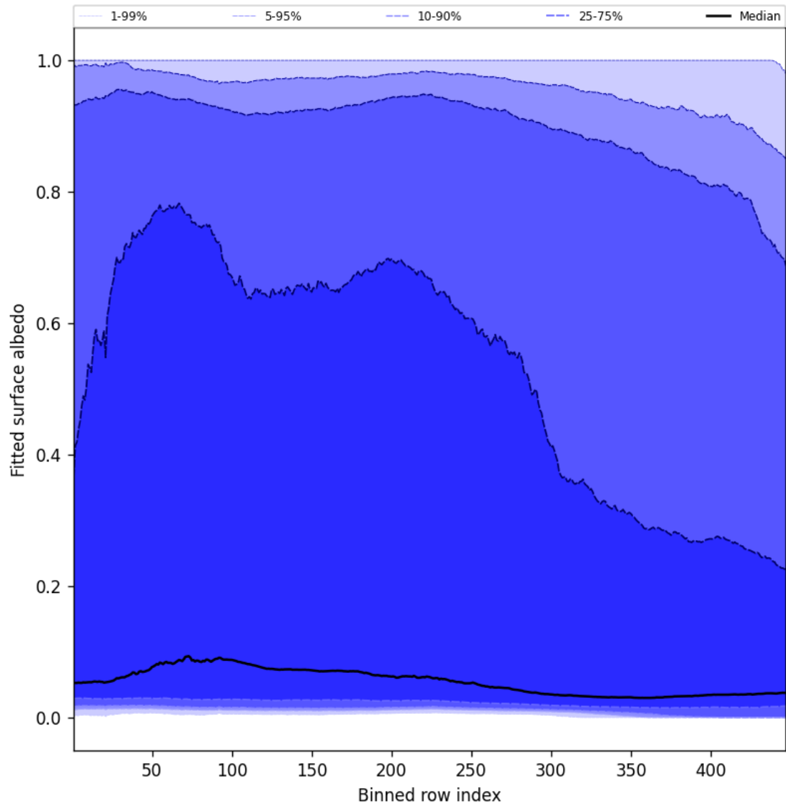
Figure 61: Along track statistics of “Fitted surface albedo” for 2024-11-01 to 2024-11-03
