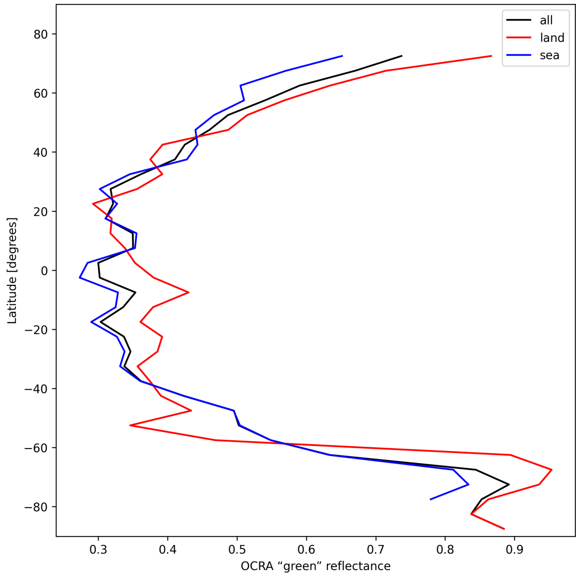
Figure 36: Zonal average of “OCRA “green” reflectance” for 2024-11-01 to 2024-11-03.
