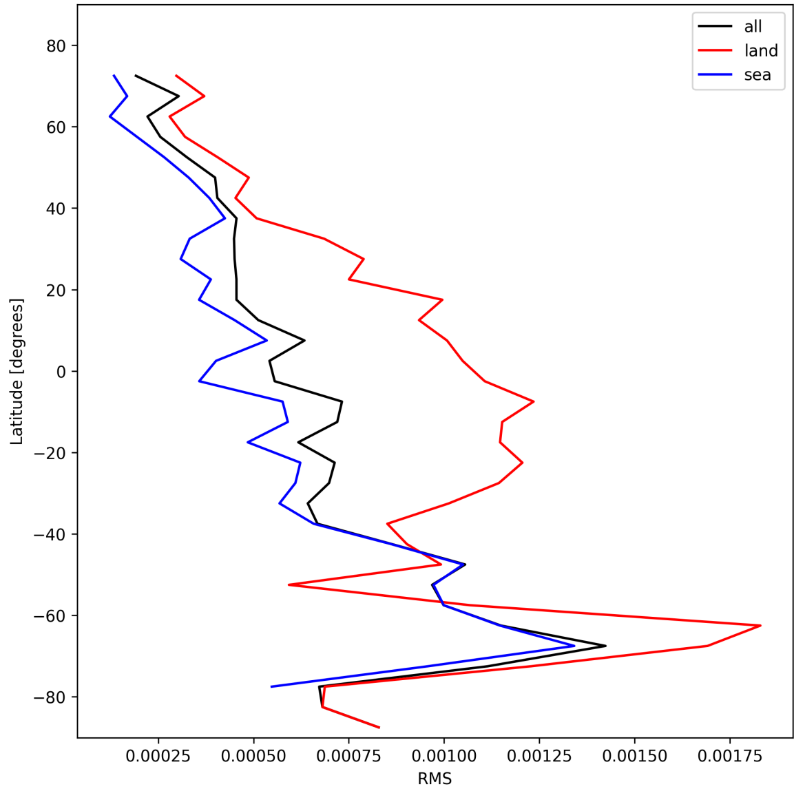
Figure 31: Zonal average of “RMS” for 2024-11-01 to 2024-11-03.
