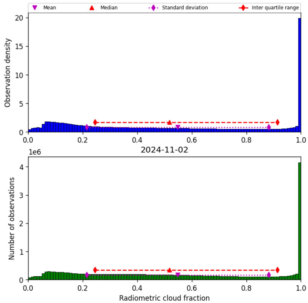
Figure 39: Histogram of “Radiometric cloud fraction” for 2024-11-01 to 2024-11-03
