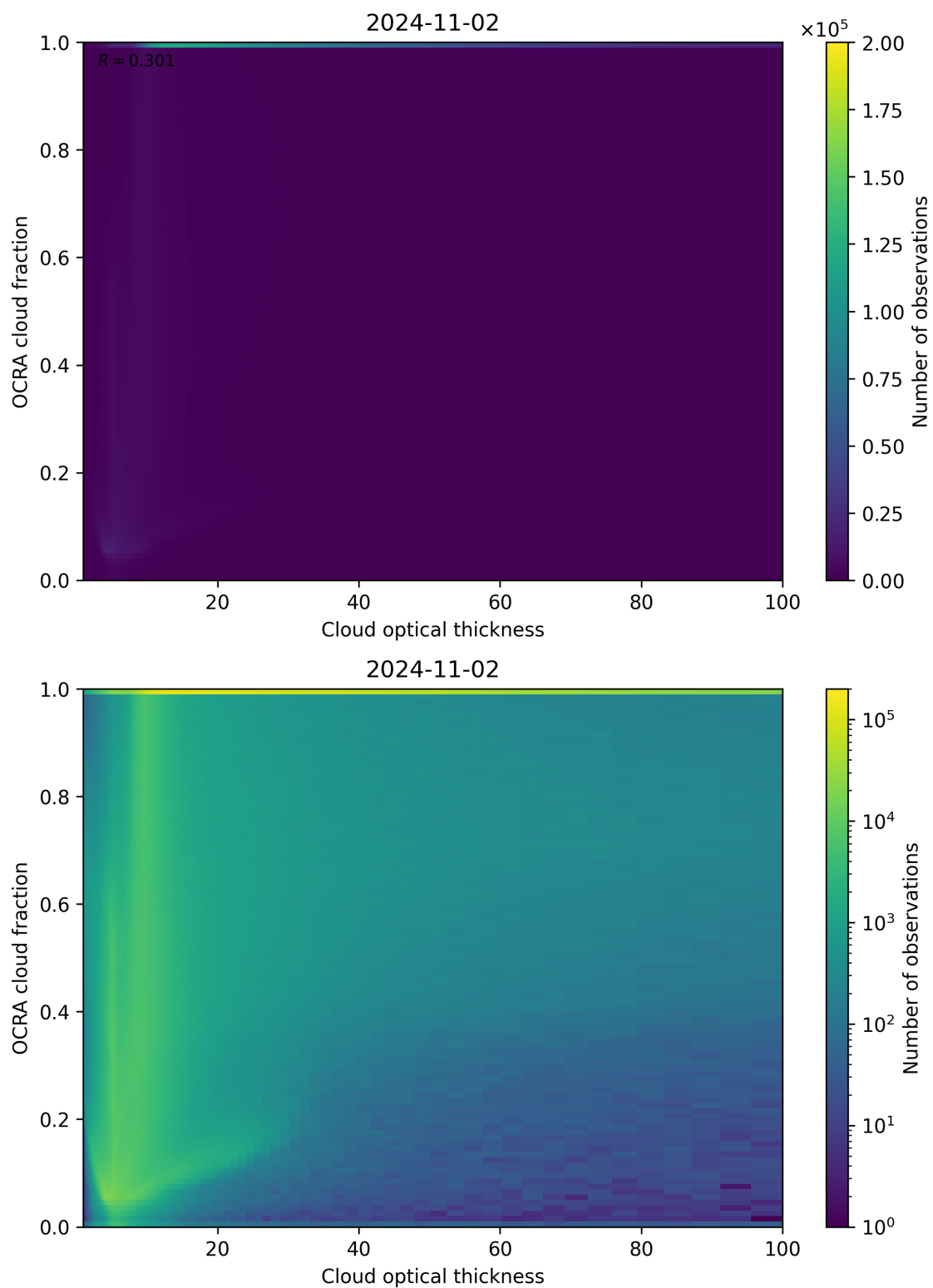
Figure 83: Scatter density plot of “Cloud optical thickness” against “OCRA cloud fraction” for 2024-11-01 to 2024-11-03.
