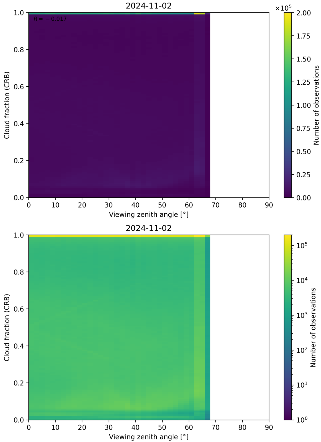
Figure 109: Scatter density plot of “Viewing zenith angle” against “Cloud fraction (CRB)” for 2024-11-01 to 2024-11-03.
