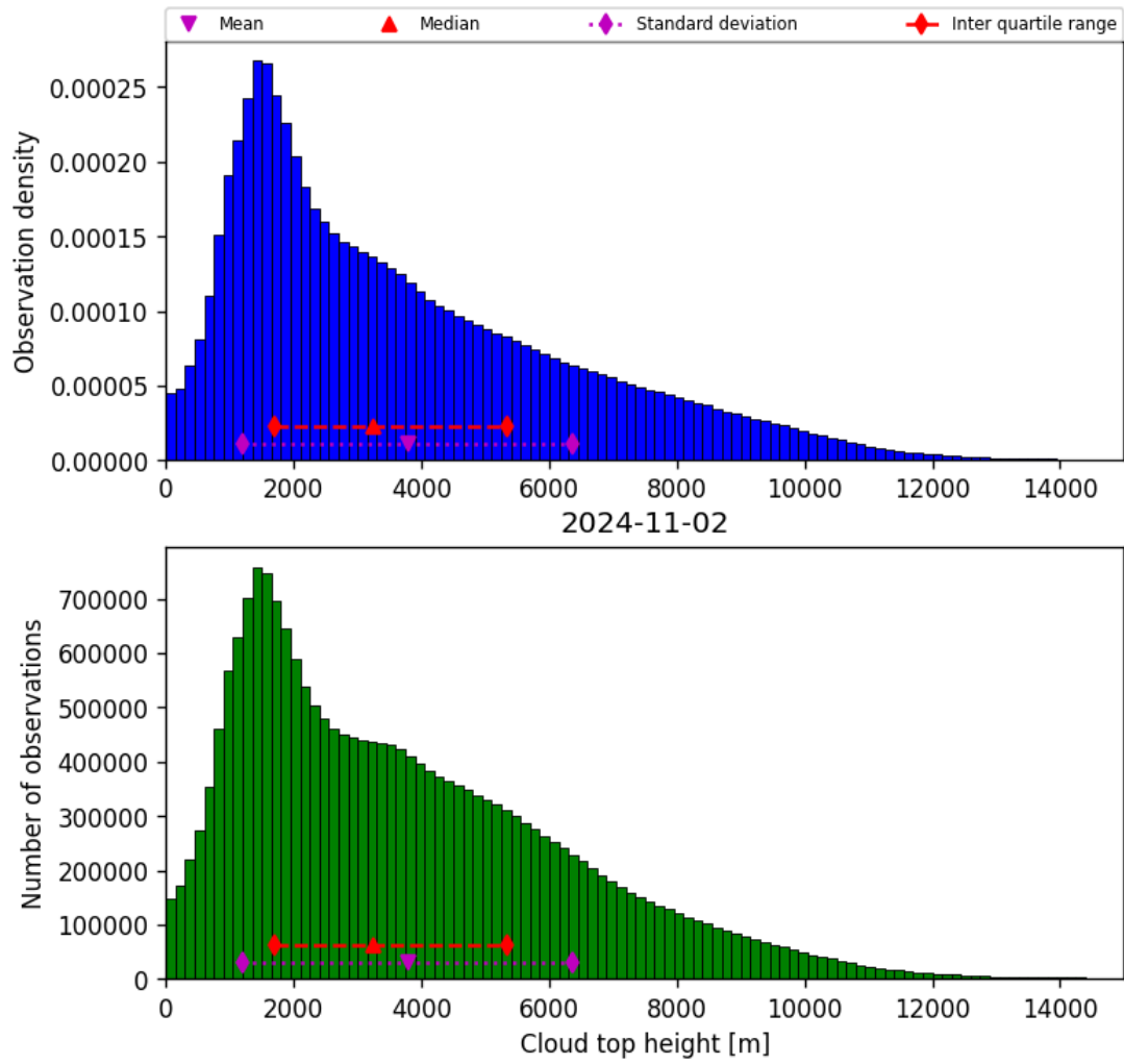
Figure 40: Histogram of “Cloud top height” for 2024-11-01 to 2024-11-03
