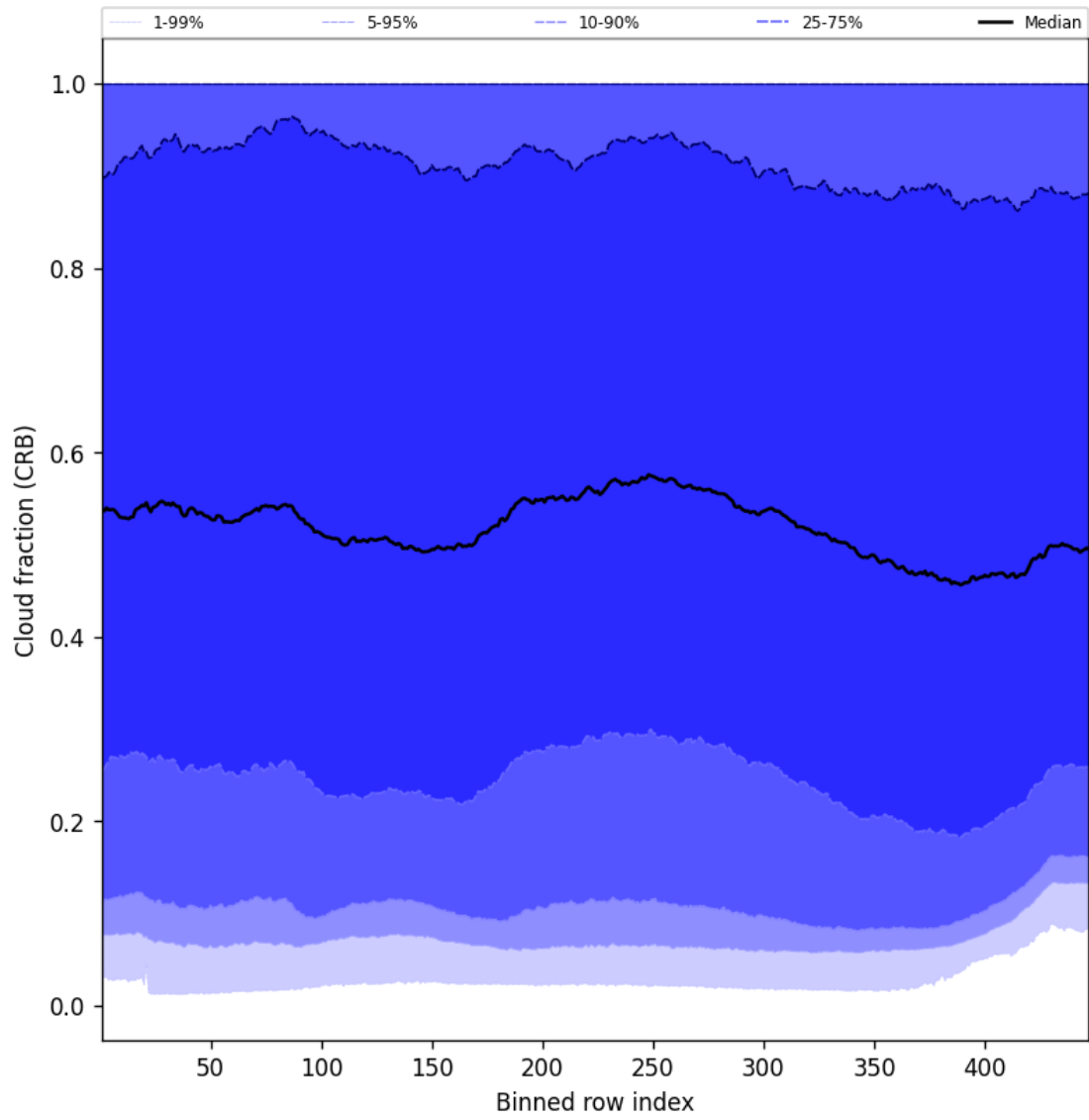
Figure 58: Along track statistics of “Cloud fraction (CRB)” for 2024-11-01 to 2024-11-03
