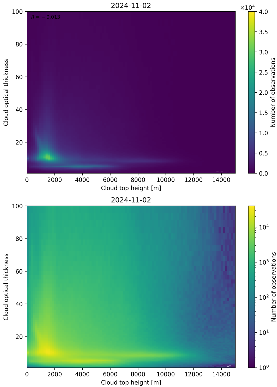
Figure 90: Scatter density plot of “Cloud top height” against “Cloud optical thickness” for 2024-11-01 to 2024-11-03.
