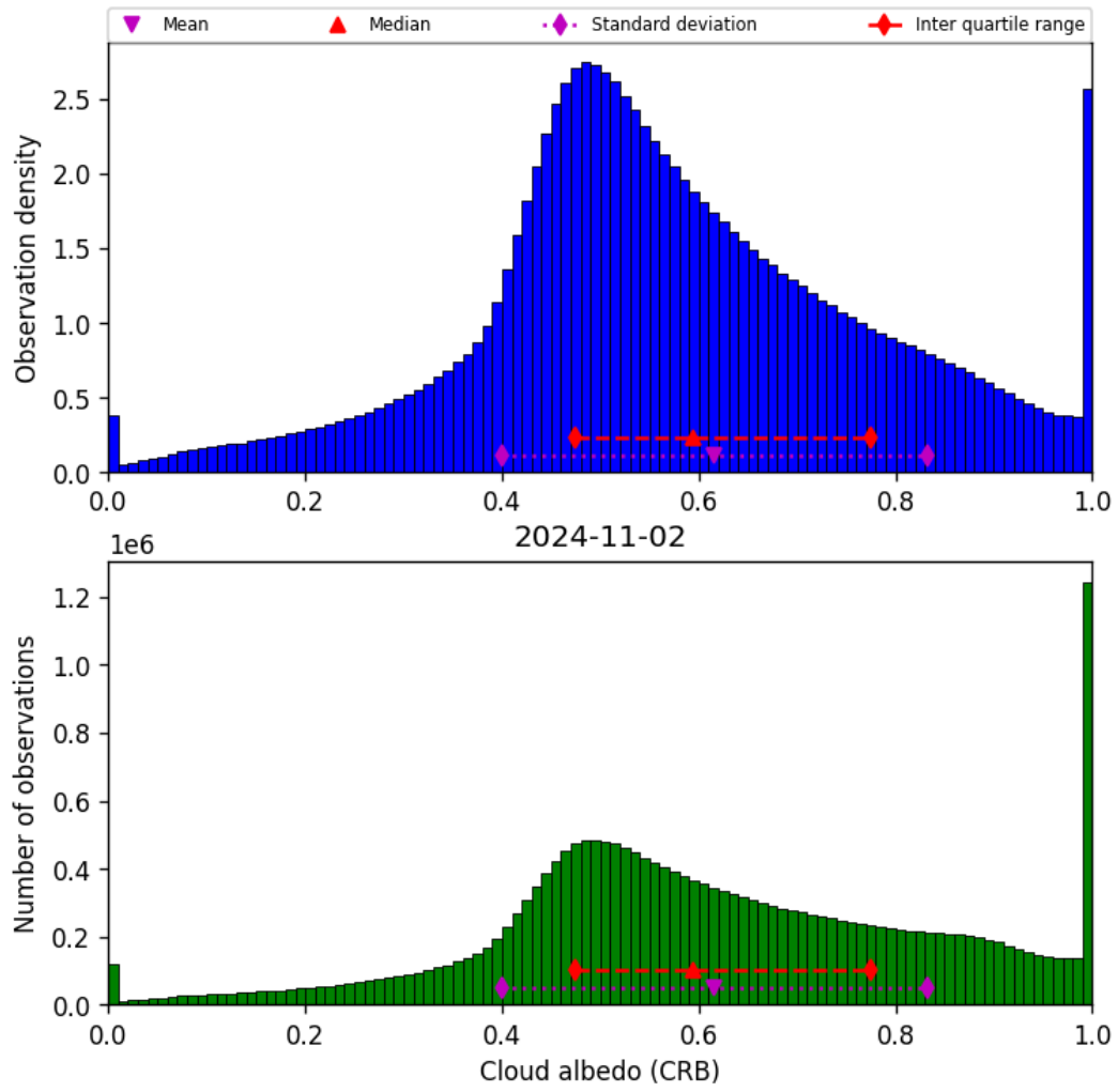
Figure 44: Histogram of “Cloud albedo (CRB)” for 2024-11-01 to 2024-11-03
