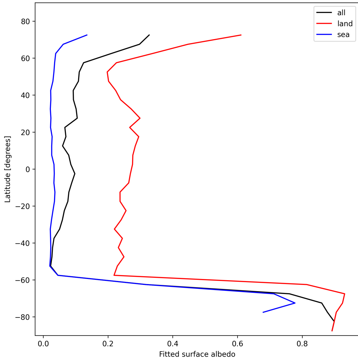
Figure 29: Zonal average of “Fitted surface albedo” for 2024-11-01 to 2024-11-03.
