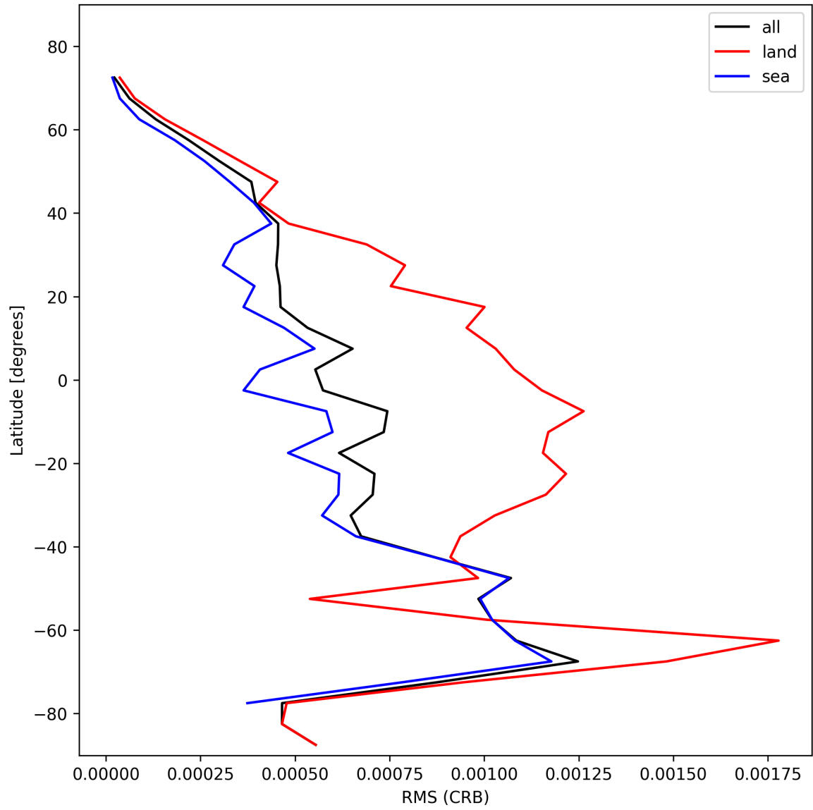
Figure 32: Zonal average of “RMS (CRB)” for 2024-11-01 to 2024-11-03.
