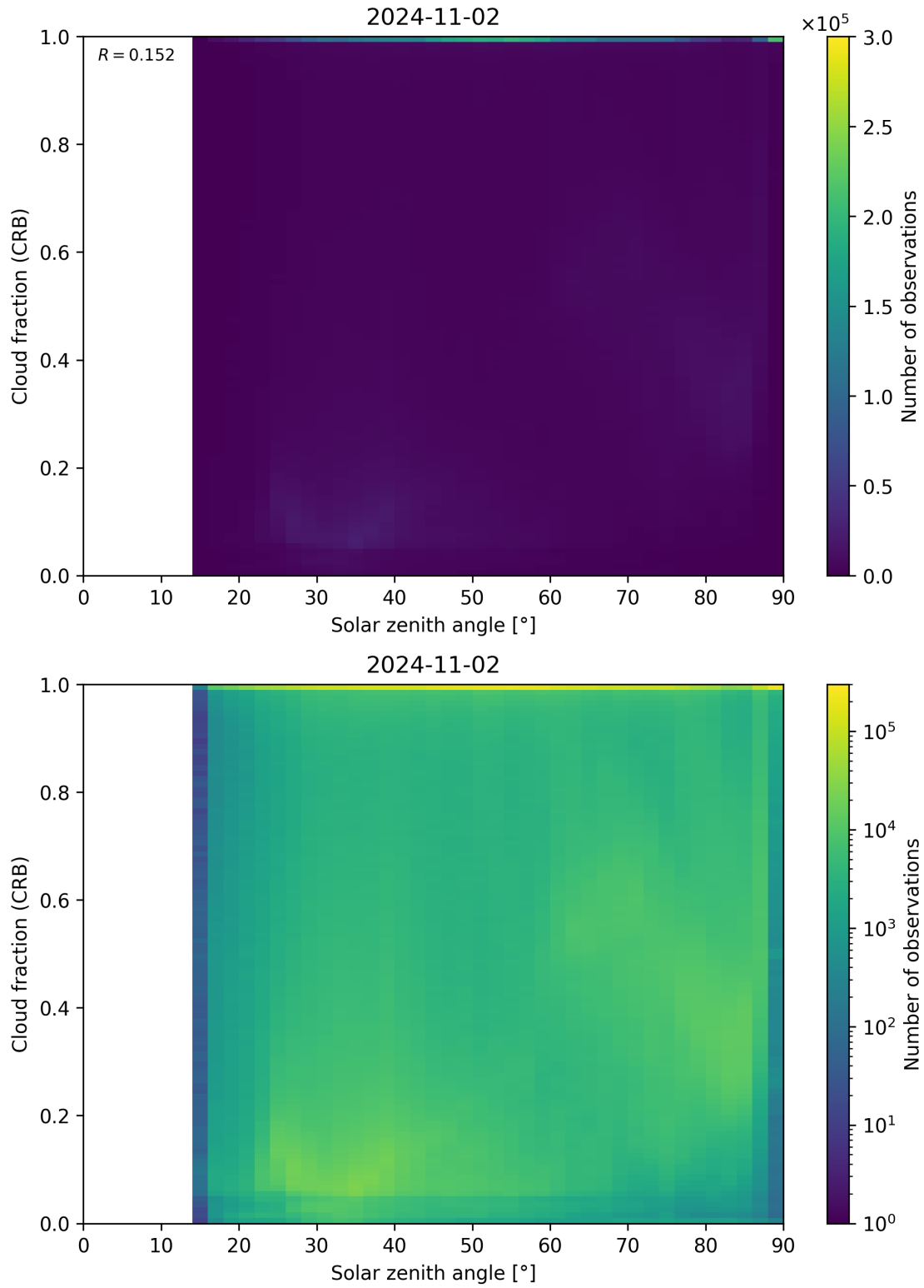
Figure 101: Scatter density plot of “Solar zenith angle” against “Cloud fraction (CRB)” for 2024-11-01 to 2024-11-03.
