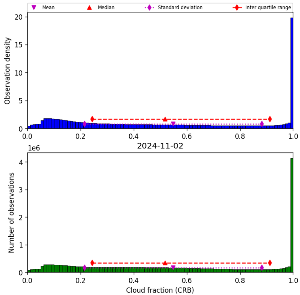
Figure 42: Histogram of “Cloud fraction (CRB)” for 2024-11-01 to 2024-11-03
