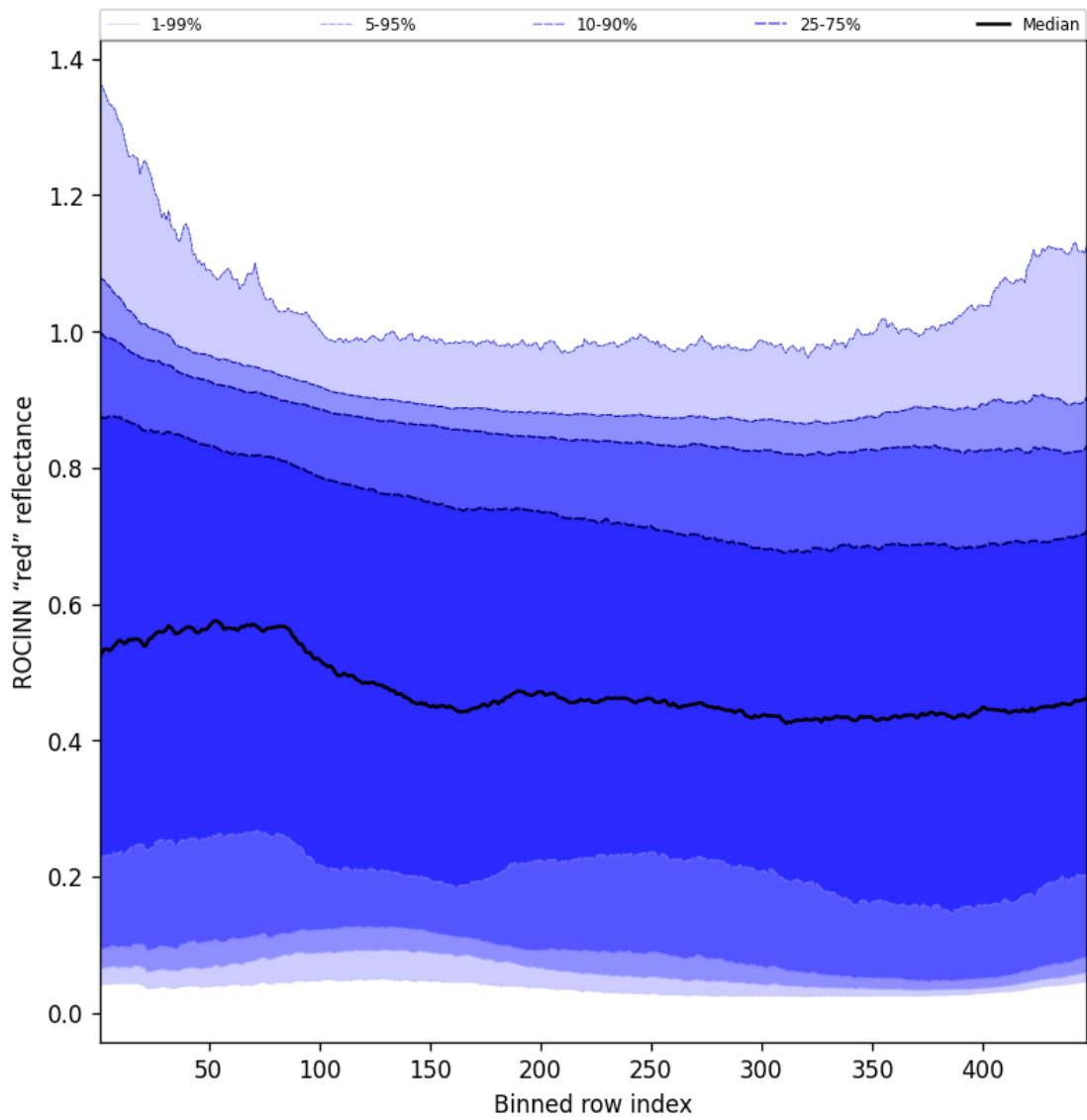
Figure 69: Along track statistics of “ROCINN “red” reflectance” for 2024-11-01 to 2024-11-03
