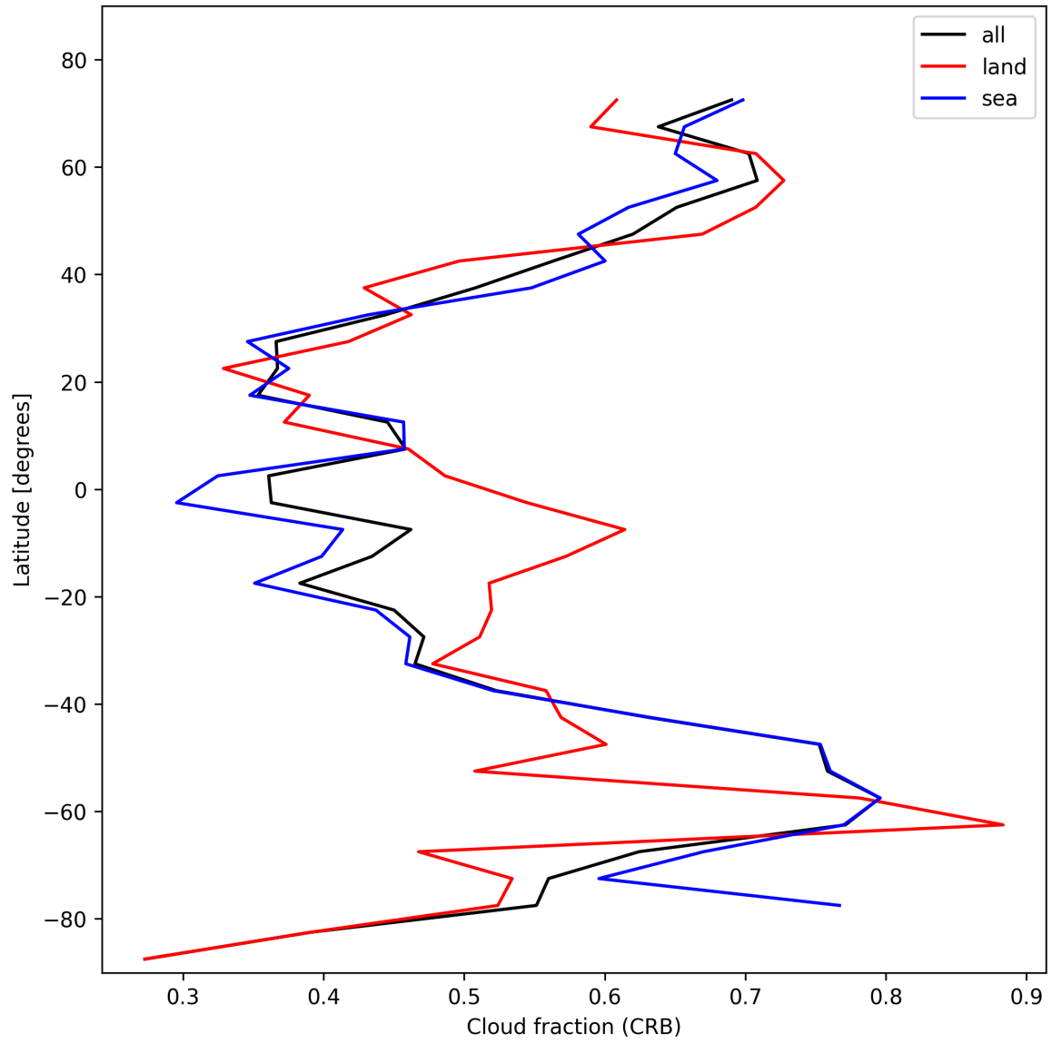
Figure 26: Zonal average of “Cloud fraction (CRB)” for 2024-11-01 to 2024-11-03.
