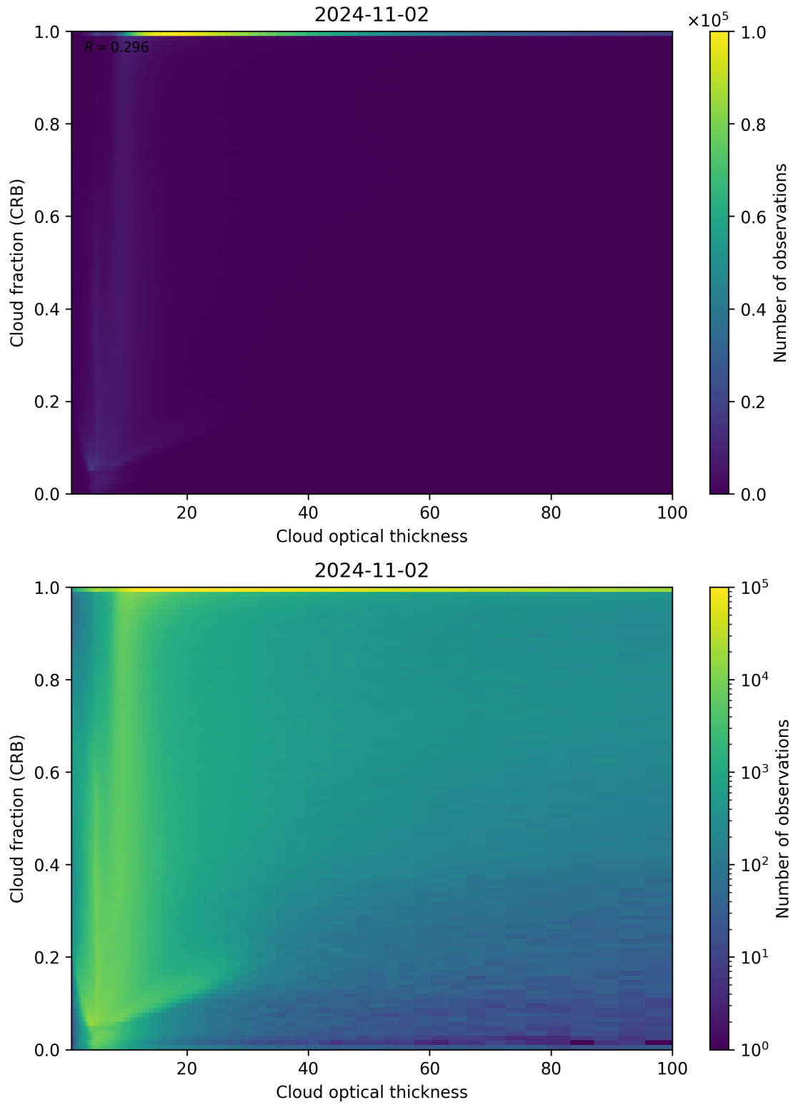
Figure 84: Scatter density plot of “Cloud optical thickness” against “Cloud fraction (CRB)” for 2024-11-01 to 2024-11-03.
