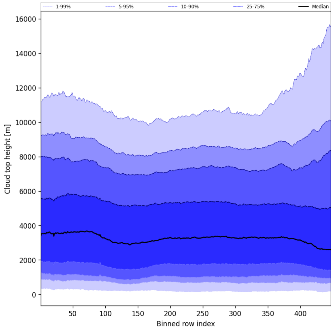
Figure 56: Along track statistics of “Cloud top height” for 2024-11-01 to 2024-11-03
