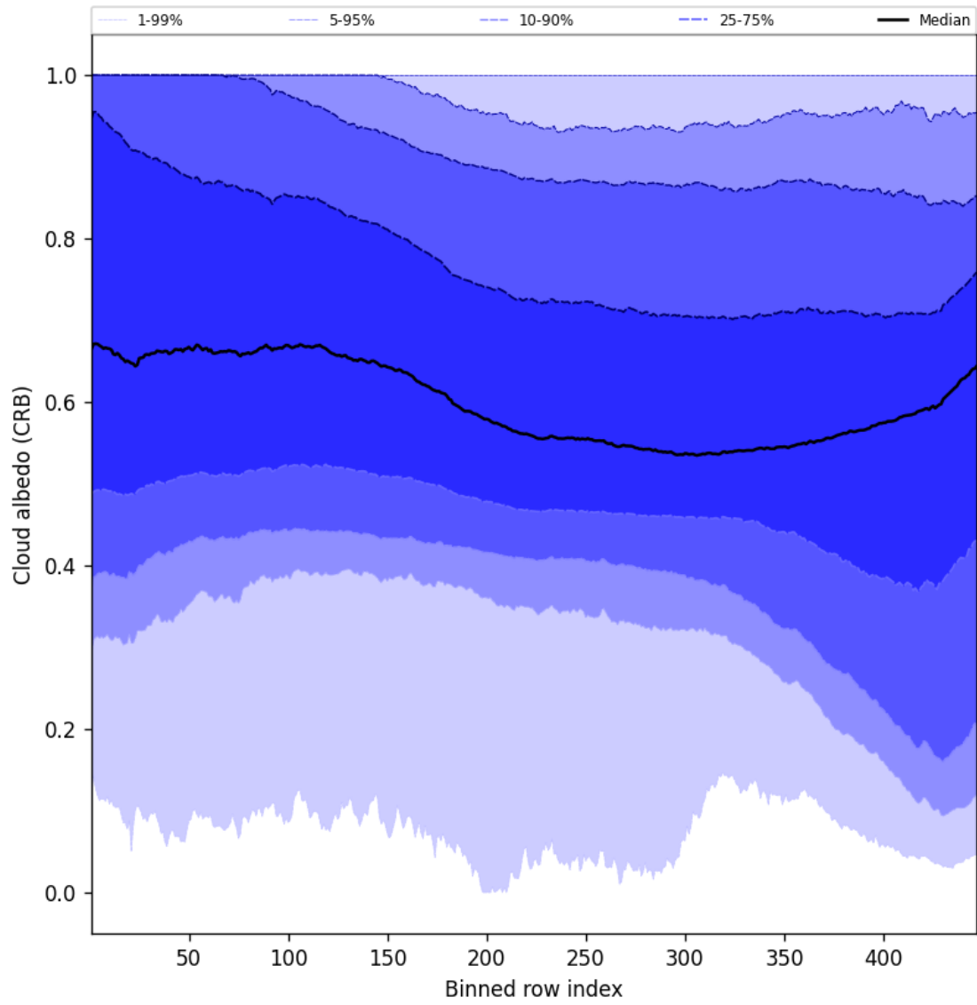
Figure 60: Along track statistics of “Cloud albedo (CRB)” for 2024-11-01 to 2024-11-03
