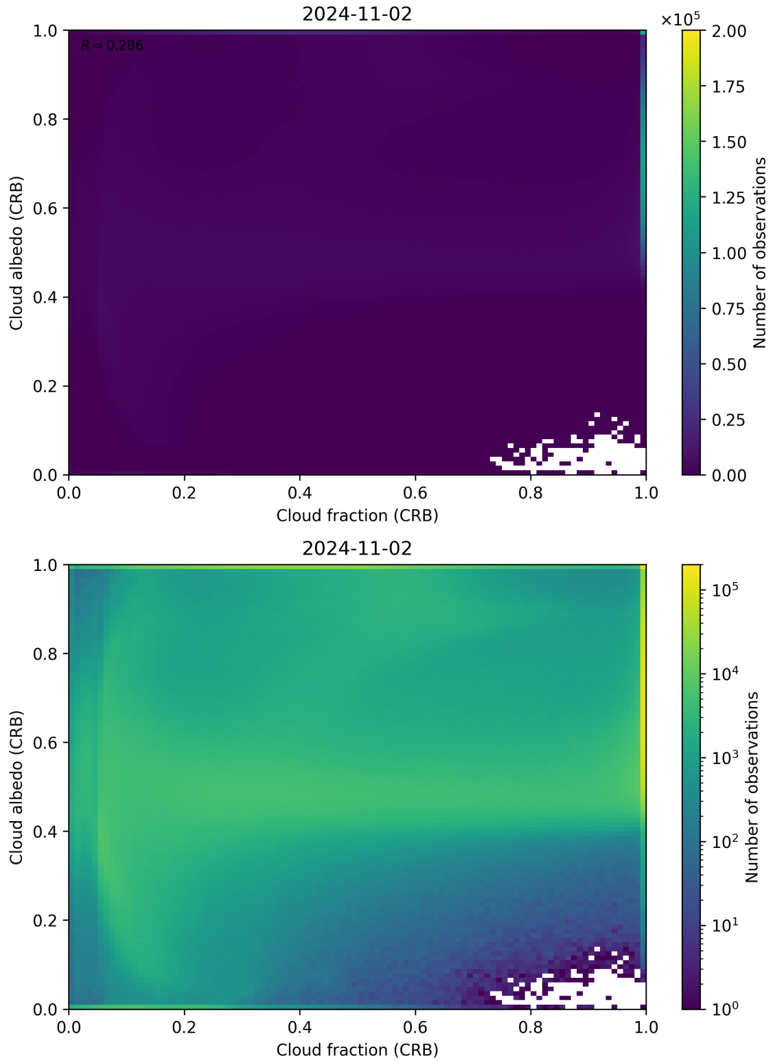
Figure 77: Scatter density plot of “Cloud fraction (CRB)” against “Cloud albedo (CRB)” for 2024-11-01 to 2024-11-03.
