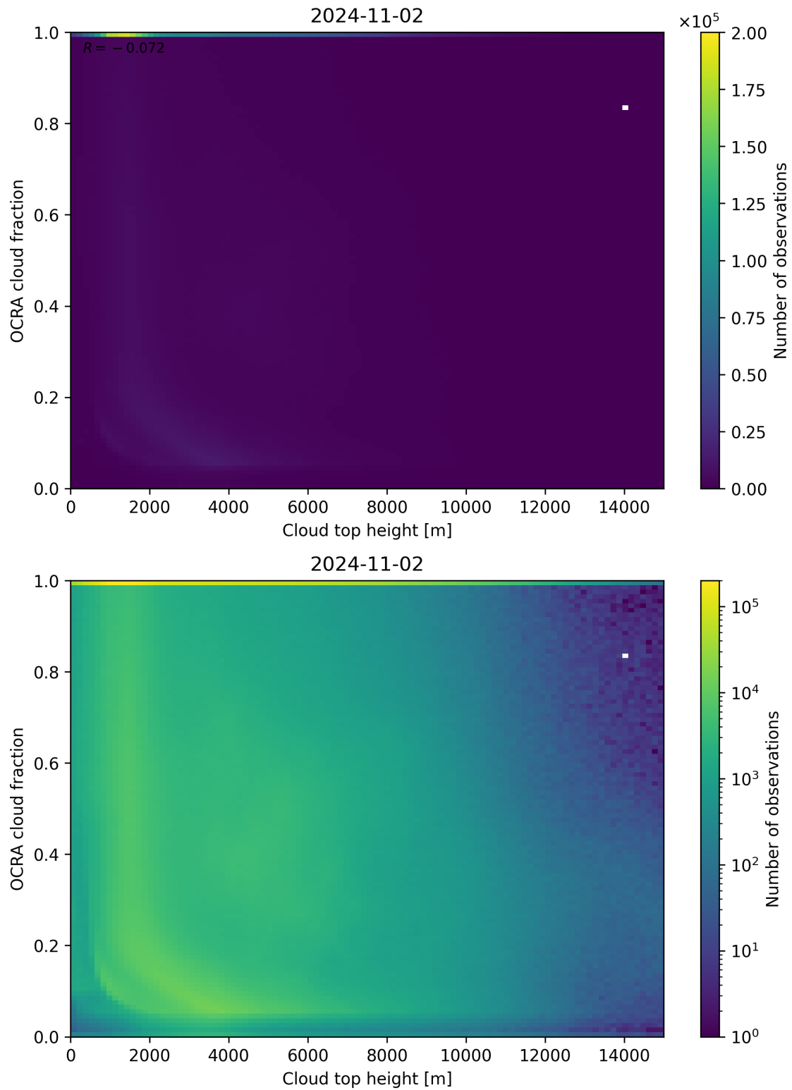
Figure 87: Scatter density plot of “Cloud top height” against “OCRA cloud fraction” for 2024-11-01 to 2024-11-03.
