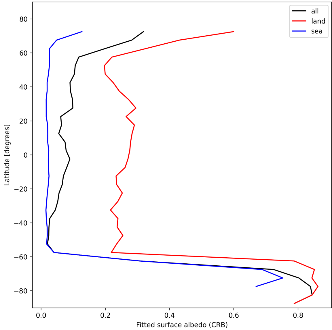
Figure 30: Zonal average of “Fitted surface albedo (CRB)” for 2024-11-01 to 2024-11-03.
