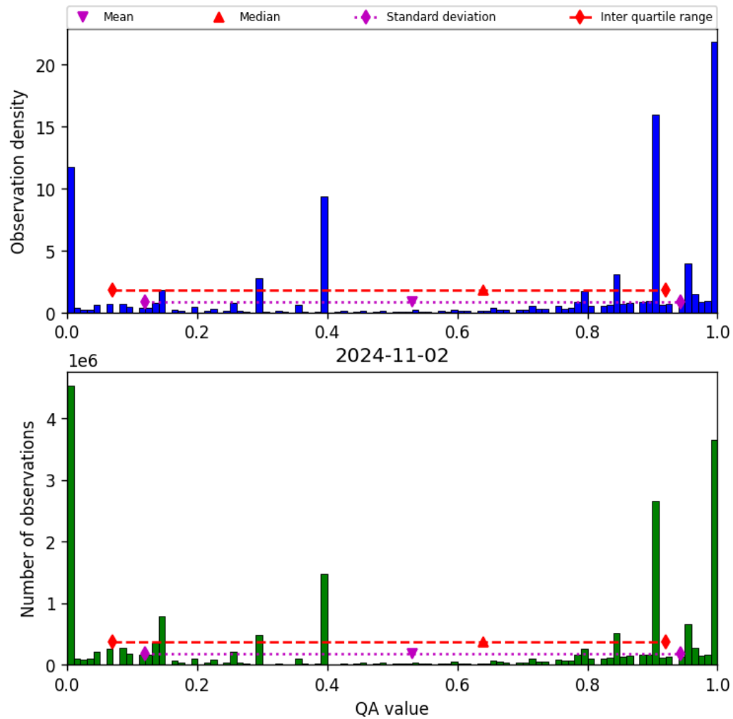
Figure 38: Histogram of “QA value” for 2024-11-01 to 2024-11-03
