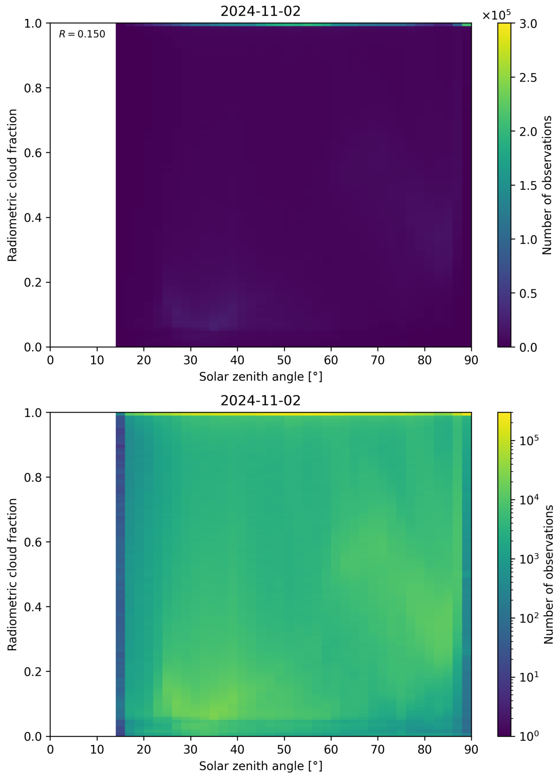
Figure 99: Scatter density plot of “Solar zenith angle” against “Radiometric cloud fraction” for 2024-11-01 to 2024-11-03.
