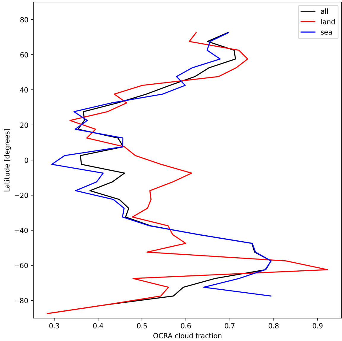
Figure 34: Zonal average of “OCRA cloud fraction” for 2024-11-01 to 2024-11-03.
