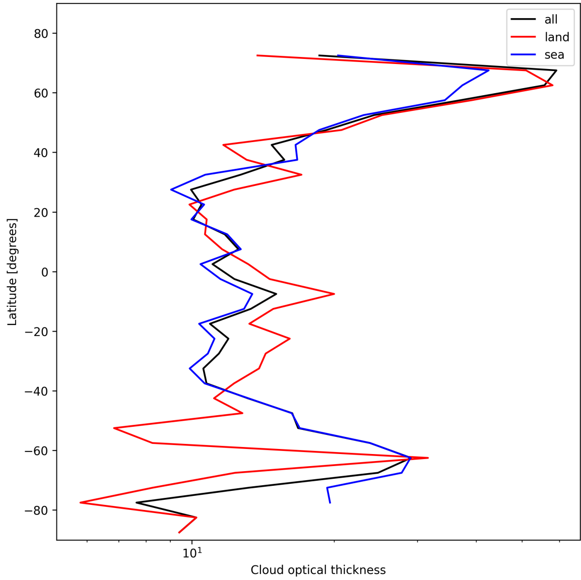
Figure 25: Zonal average of “Cloud optical thickness” for 2024-11-01 to 2024-11-03.
