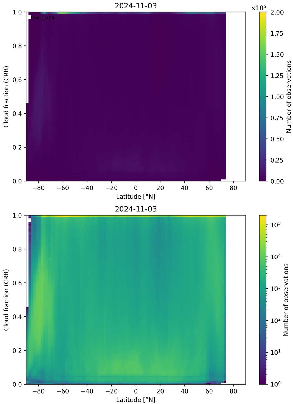
Figure 94: Scatter density plot of “Latitude” against “Cloud fraction (CRB)” for 2024-11-02 to 2024-11-04.
