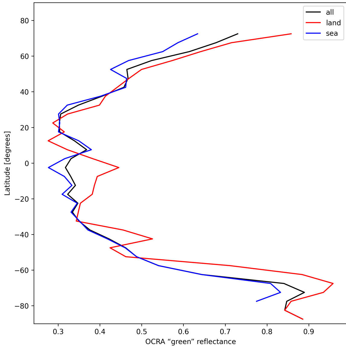
Figure 36: Zonal average of “OCRA “green” reflectance” for 2024-11-02 to 2024-11-04.
