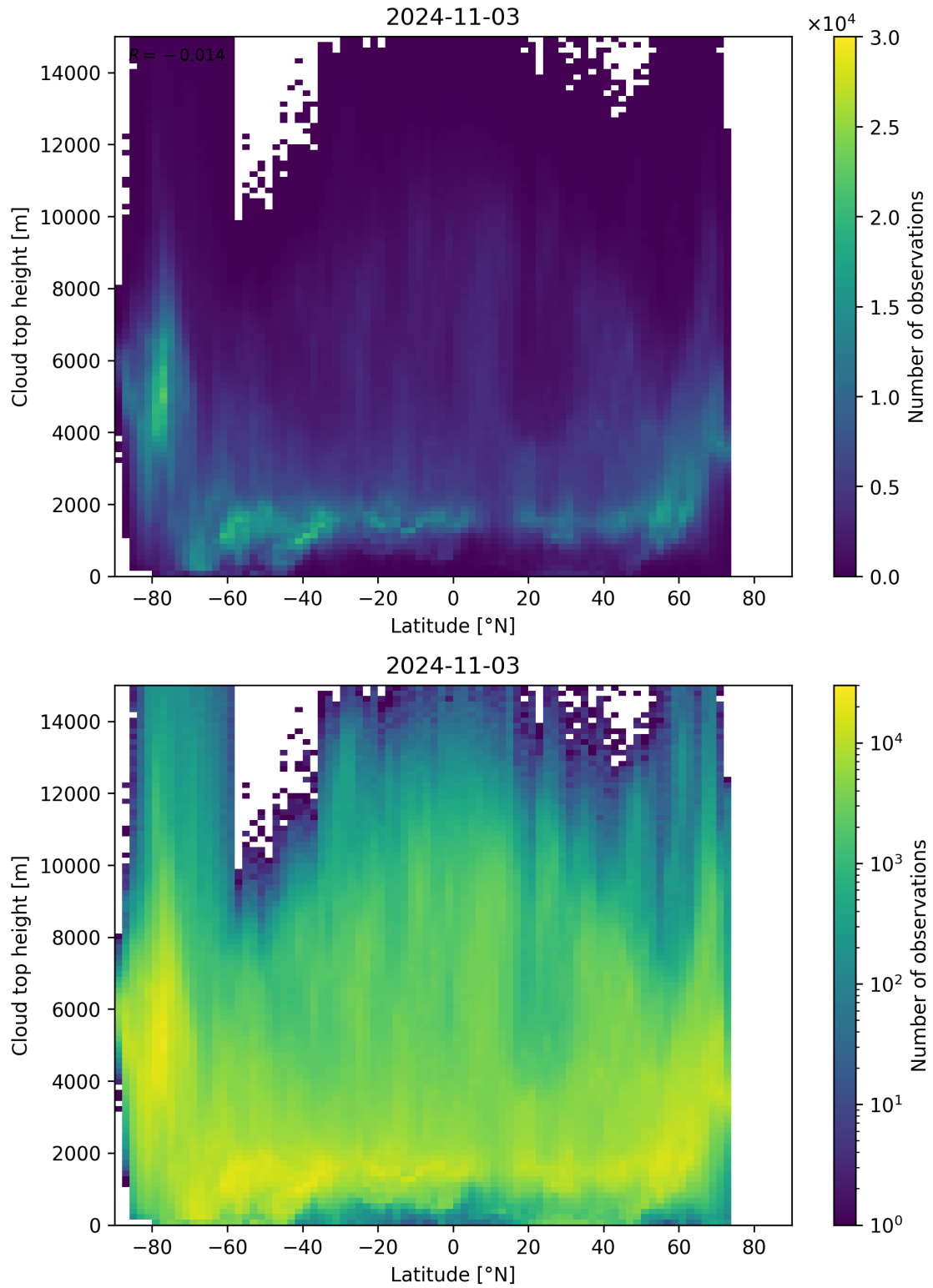
Figure 97: Scatter density plot of “Latitude” against “Cloud top height” for 2024-11-02 to 2024-11-04.
