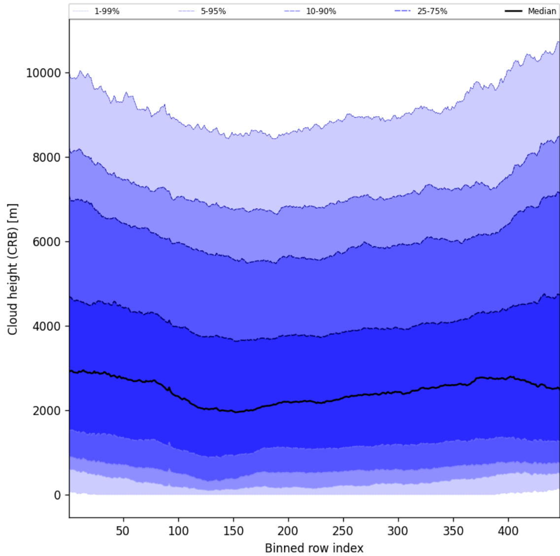
Figure 59: Along track statistics of “Cloud height (CRB)” for 2024-11-02 to 2024-11-04
