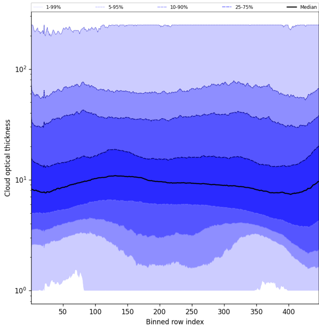
Figure 57: Along track statistics of “Cloud optical thickness” for 2024-11-02 to 2024-11-04
