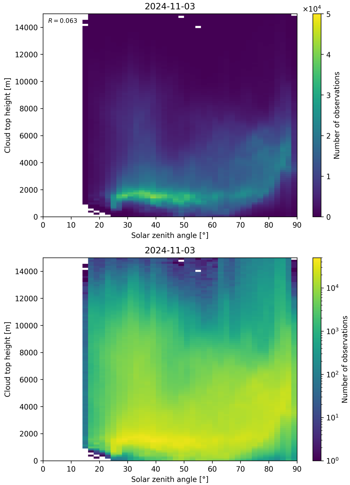
Figure 104: Scatter density plot of “Solar zenith angle” against “Cloud top height” for 2024-11-02 to 2024-11-04.
