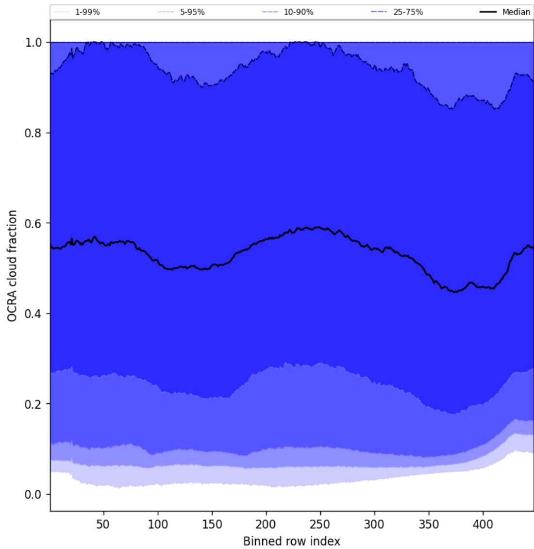
Figure 66: Along track statistics of “OCRA cloud fraction” for 2024-11-02 to 2024-11-04
