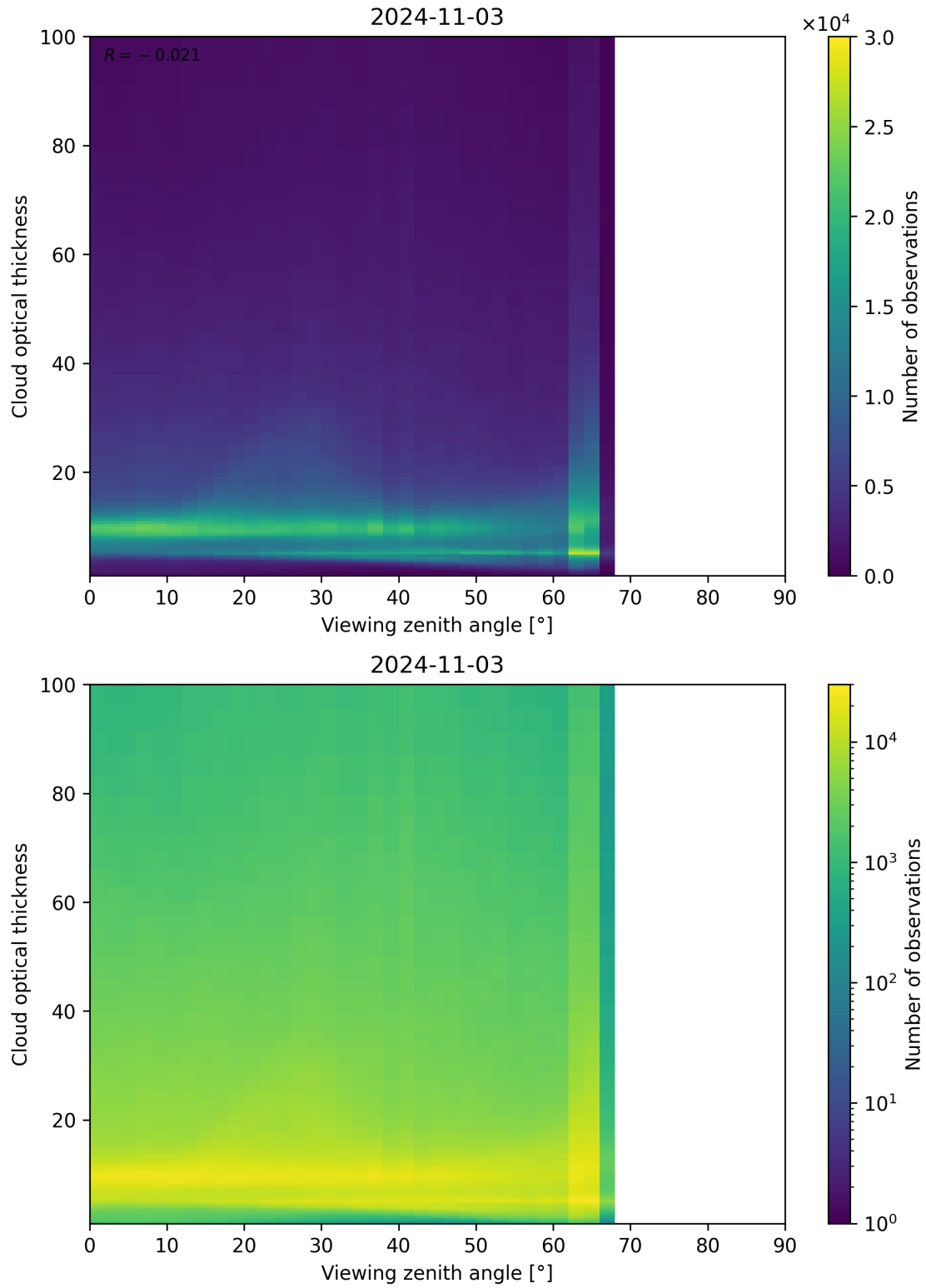
Figure 111: Scatter density plot of “Viewing zenith angle” against “Cloud optical thickness” for 2024-11-02 to 2024-11-04.
