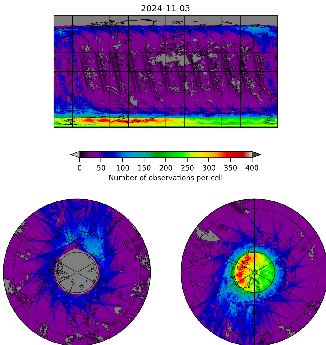
Figure 21: Map of the number of observations for 2024-11-02 to 2024-11-04
