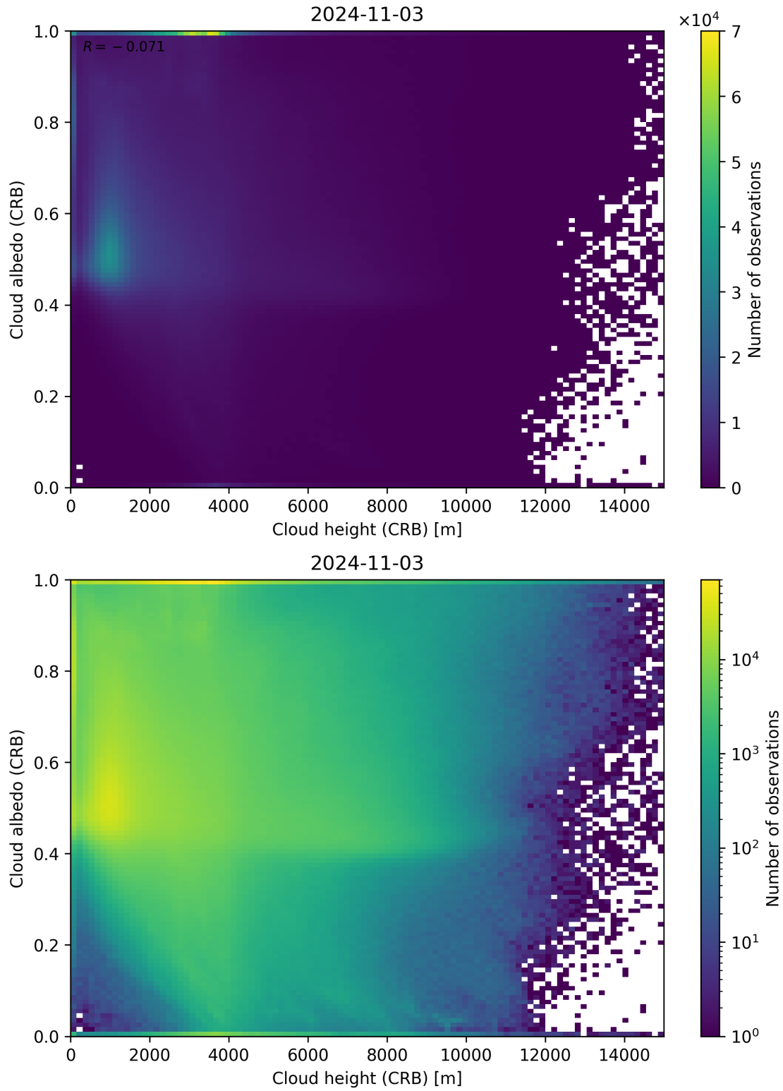
Figure 80: Scatter density plot of “Cloud height (CRB)” against “Cloud albedo (CRB)” for 2024-11-02 to 2024-11-04.
