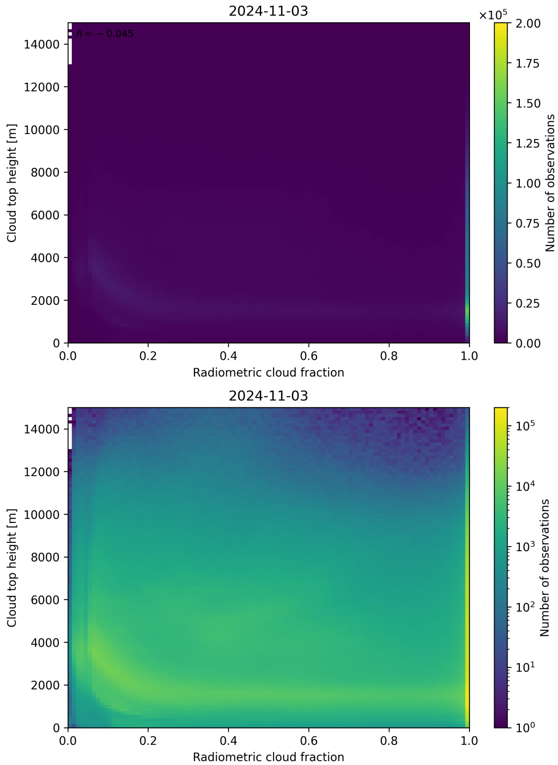
Figure 76: Scatter density plot of “Radiometric cloud fraction” against “Cloud top height” for 2024-11-02 to 2024-11-04.
