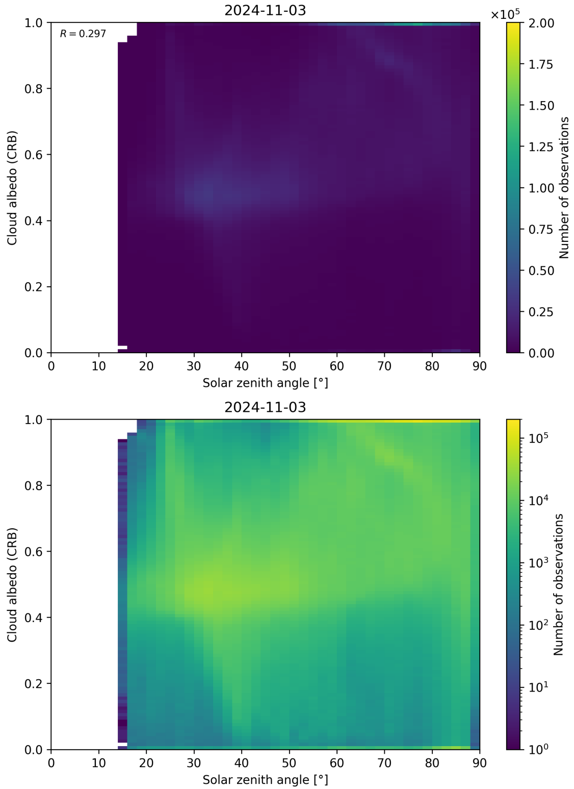
Figure 98: Scatter density plot of “Solar zenith angle” against “Cloud albedo (CRB)” for 2024-11-02 to 2024-11-04.
