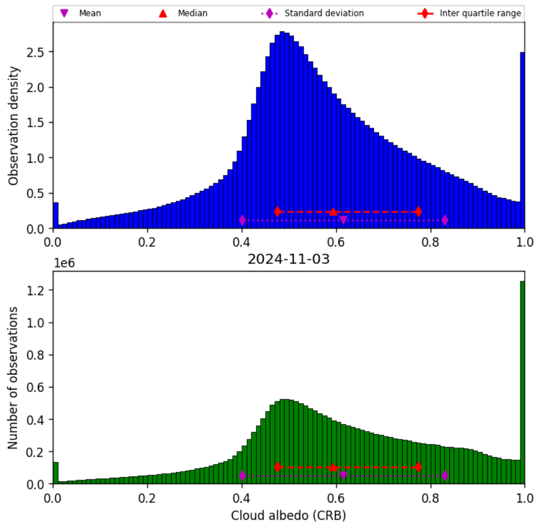
Figure 44: Histogram of “Cloud albedo (CRB)” for 2024-11-02 to 2024-11-04
