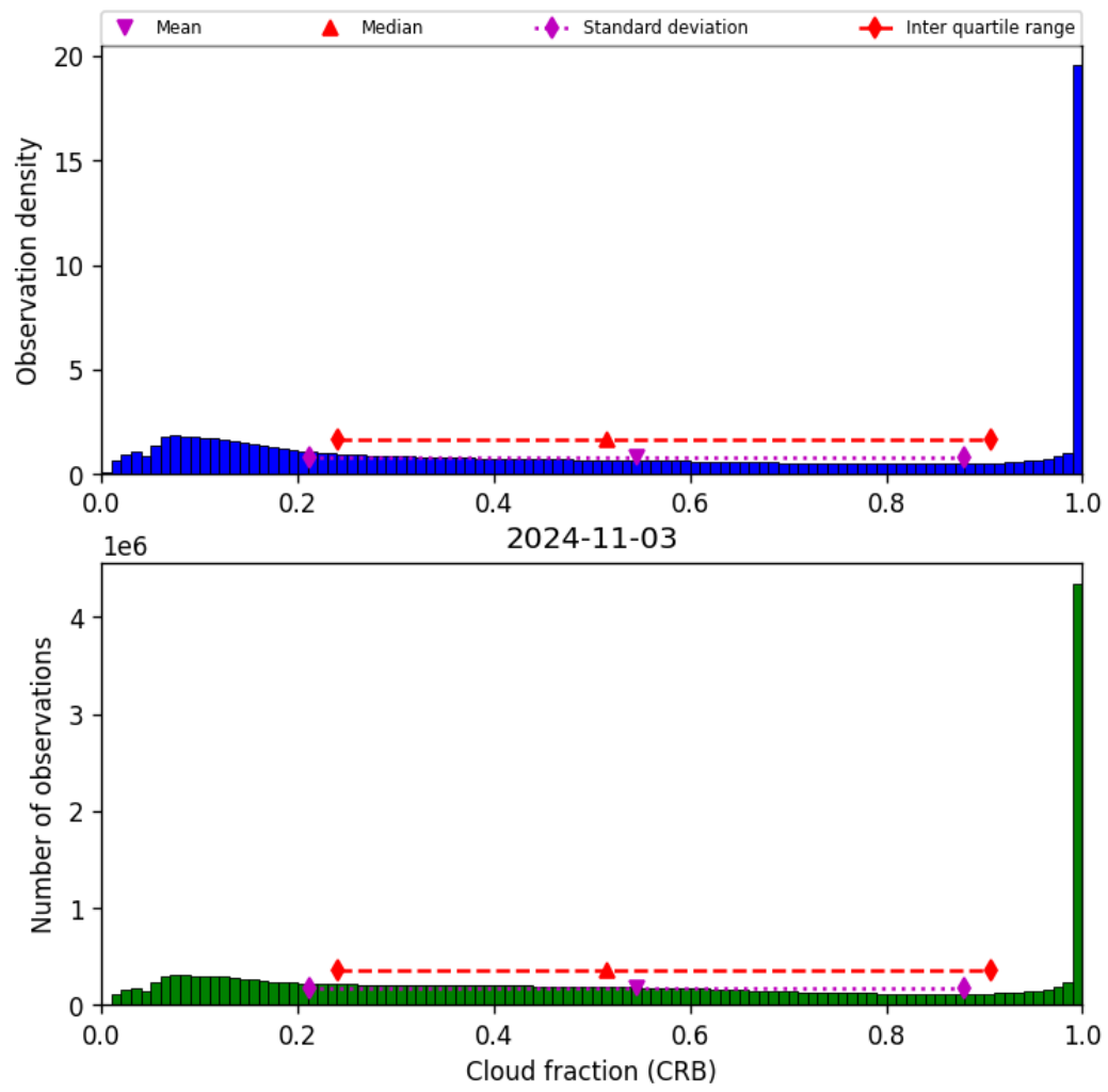
Figure 42: Histogram of “Cloud fraction (CRB)” for 2024-11-02 to 2024-11-04
