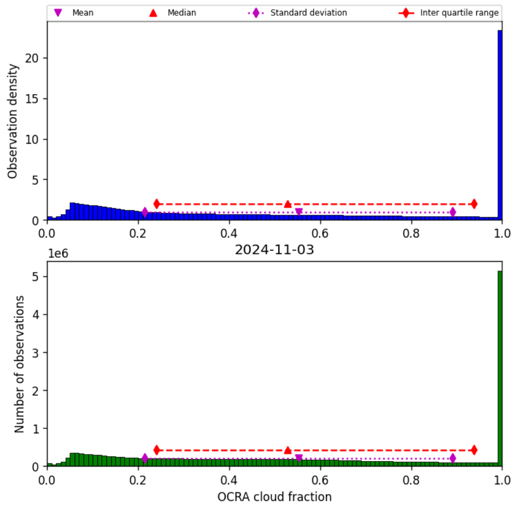
Figure 50: Histogram of “OCRA cloud fraction” for 2024-11-02 to 2024-11-04
