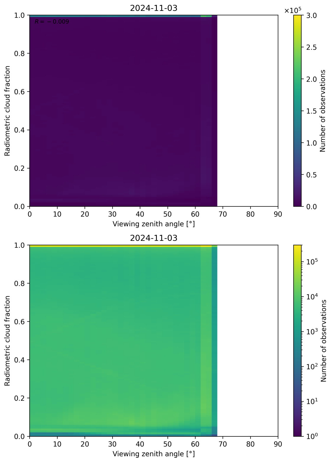
Figure 107: Scatter density plot of “Viewing zenith angle” against “Radiometric cloud fraction” for 2024-11-02 to 2024-11-04.
