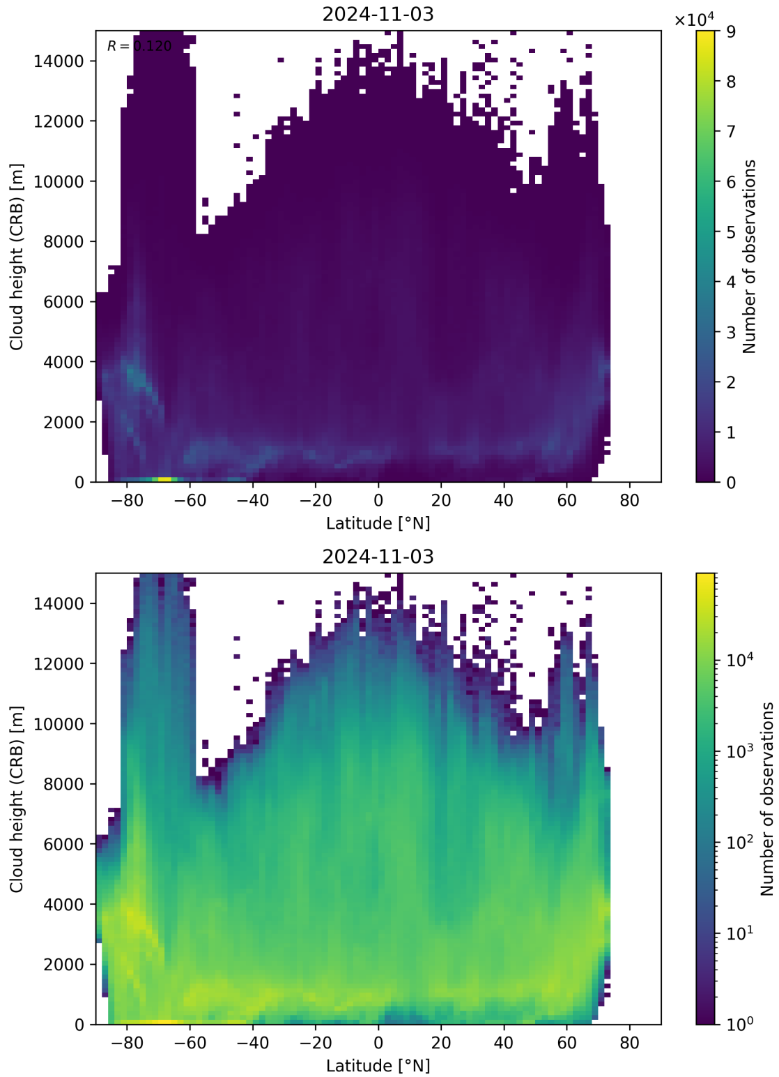
Figure 95: Scatter density plot of “Latitude” against “Cloud height (CRB)” for 2024-11-02 to 2024-11-04.
