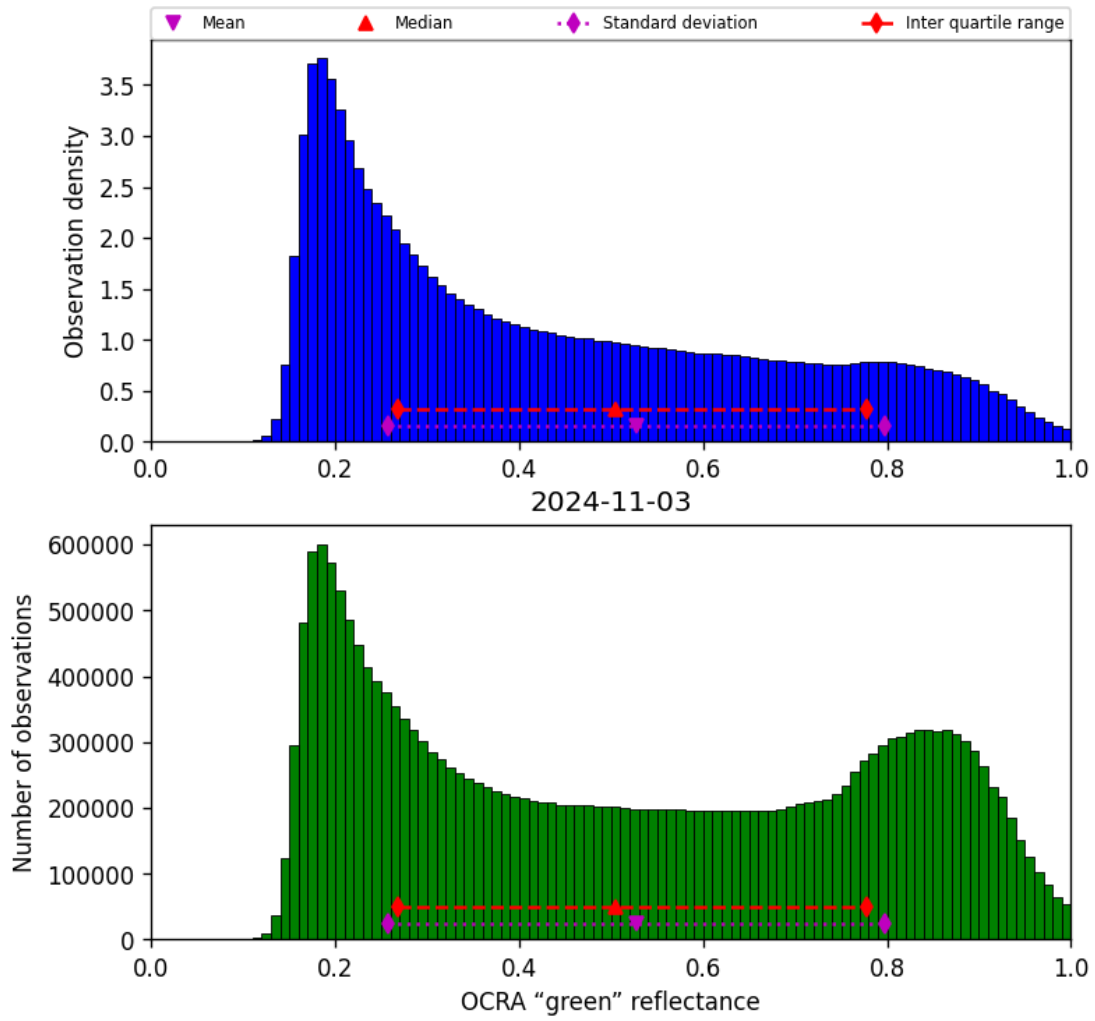
Figure 52: Histogram of “OCRA “green” reflectance” for 2024-11-02 to 2024-11-04
