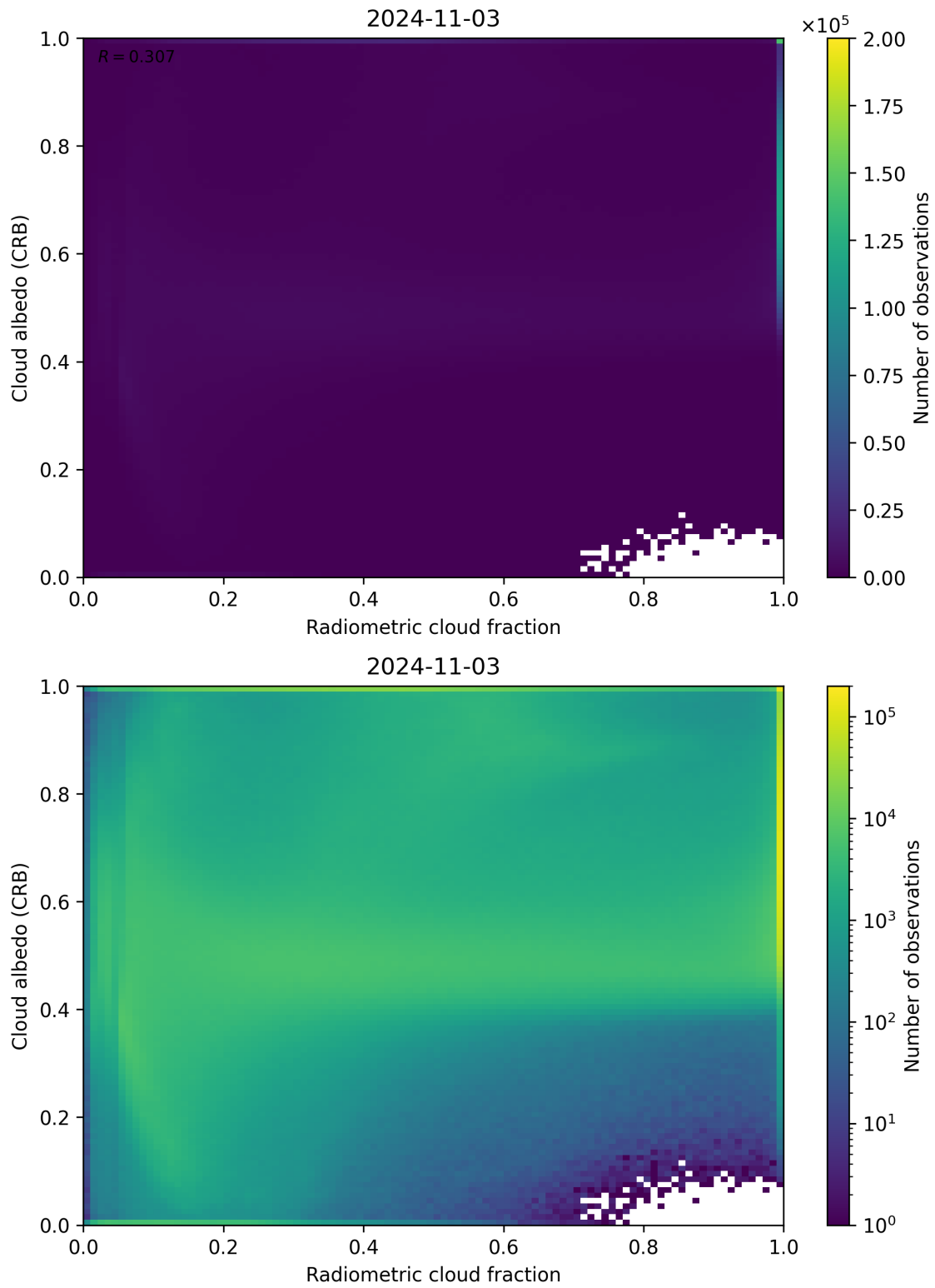
Figure 71: Scatter density plot of “Radiometric cloud fraction” against “Cloud albedo (CRB)” for 2024-11-02 to 2024-11-04.
