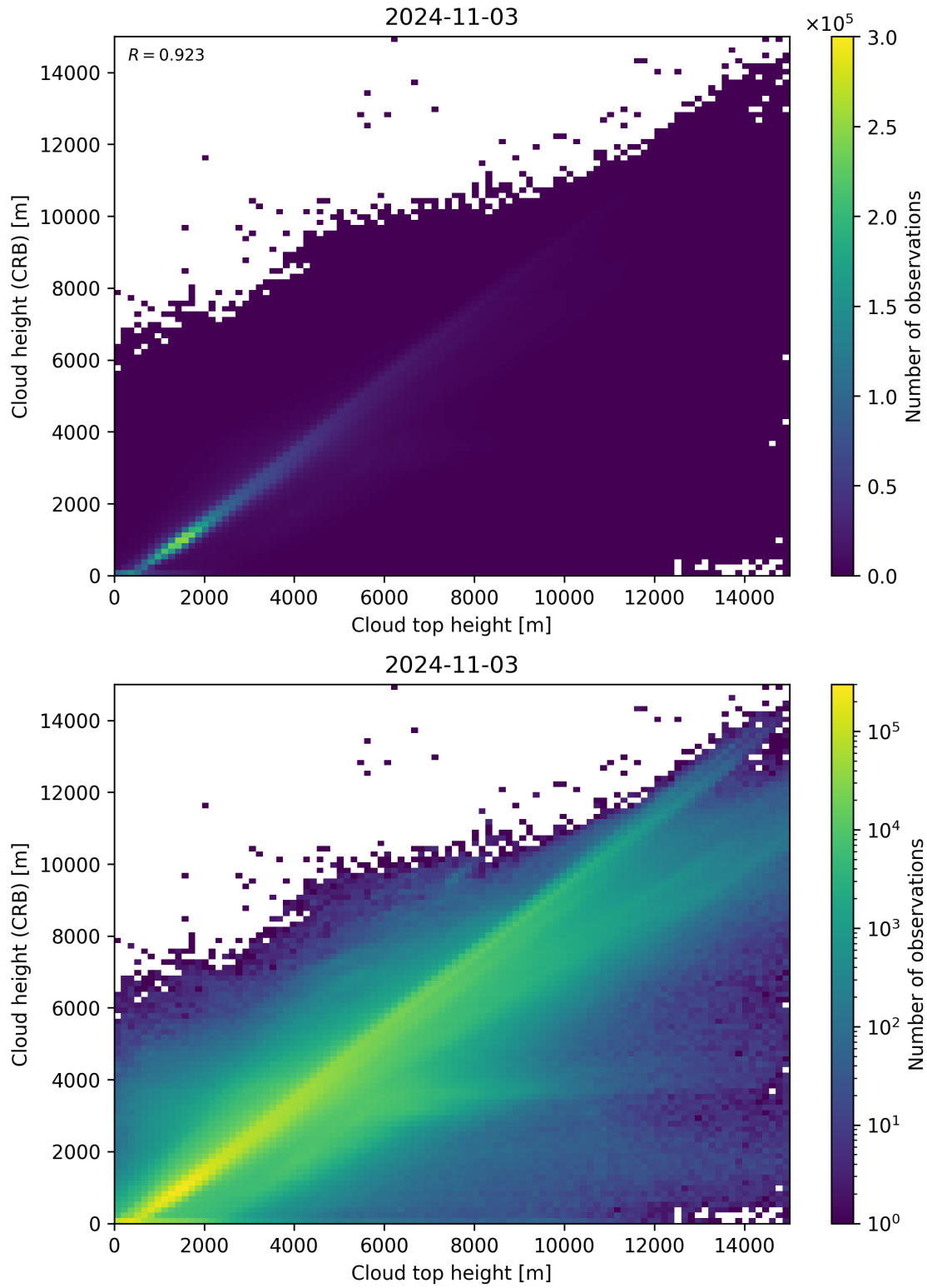
Figure 89: Scatter density plot of “Cloud top height” against “Cloud height (CRB)” for 2024-11-02 to 2024-11-04.
