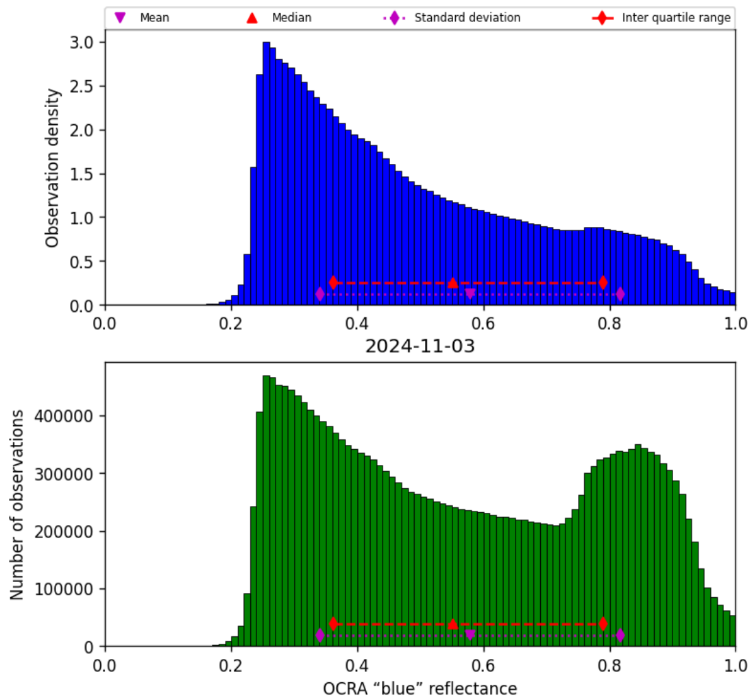
Figure 51: Histogram of “OCRA “blue” reflectance” for 2024-11-02 to 2024-11-04
