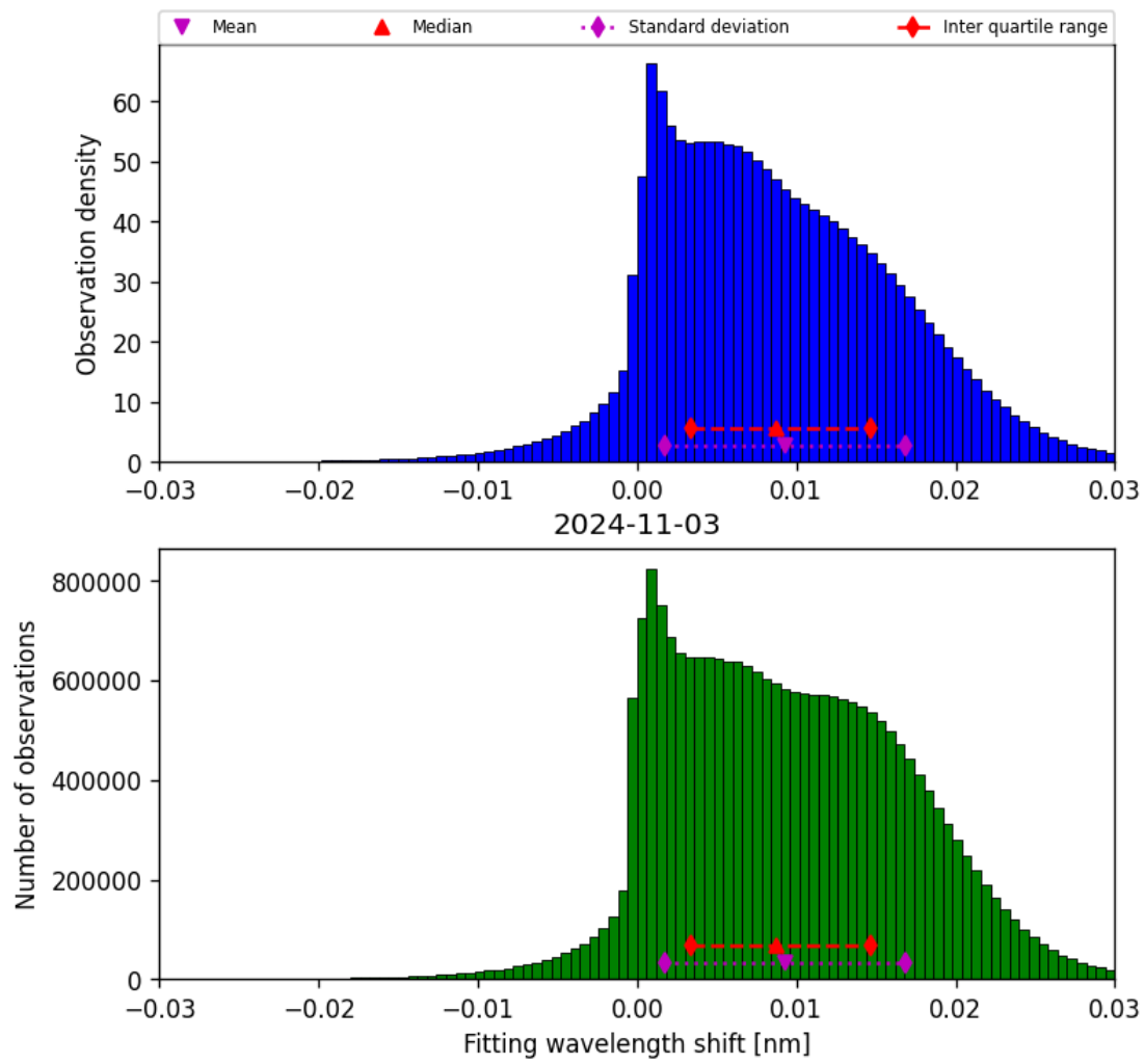
Figure 49: Histogram of “Fitting wavelength shift” for 2024-11-02 to 2024-11-04
