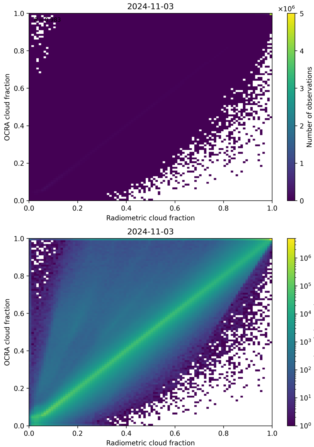
Figure 72: Scatter density plot of “Radiometric cloud fraction” against “OCRA cloud fraction” for 2024-11-02 to 2024-11-04.
