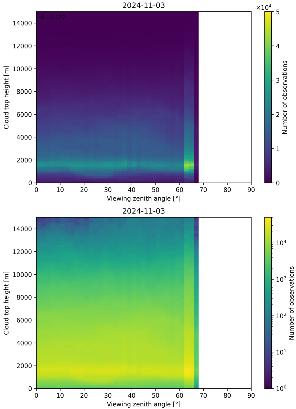
Figure 112: Scatter density plot of “Viewing zenith angle” against “Cloud top height” for 2024-11-02 to 2024-11-04.
