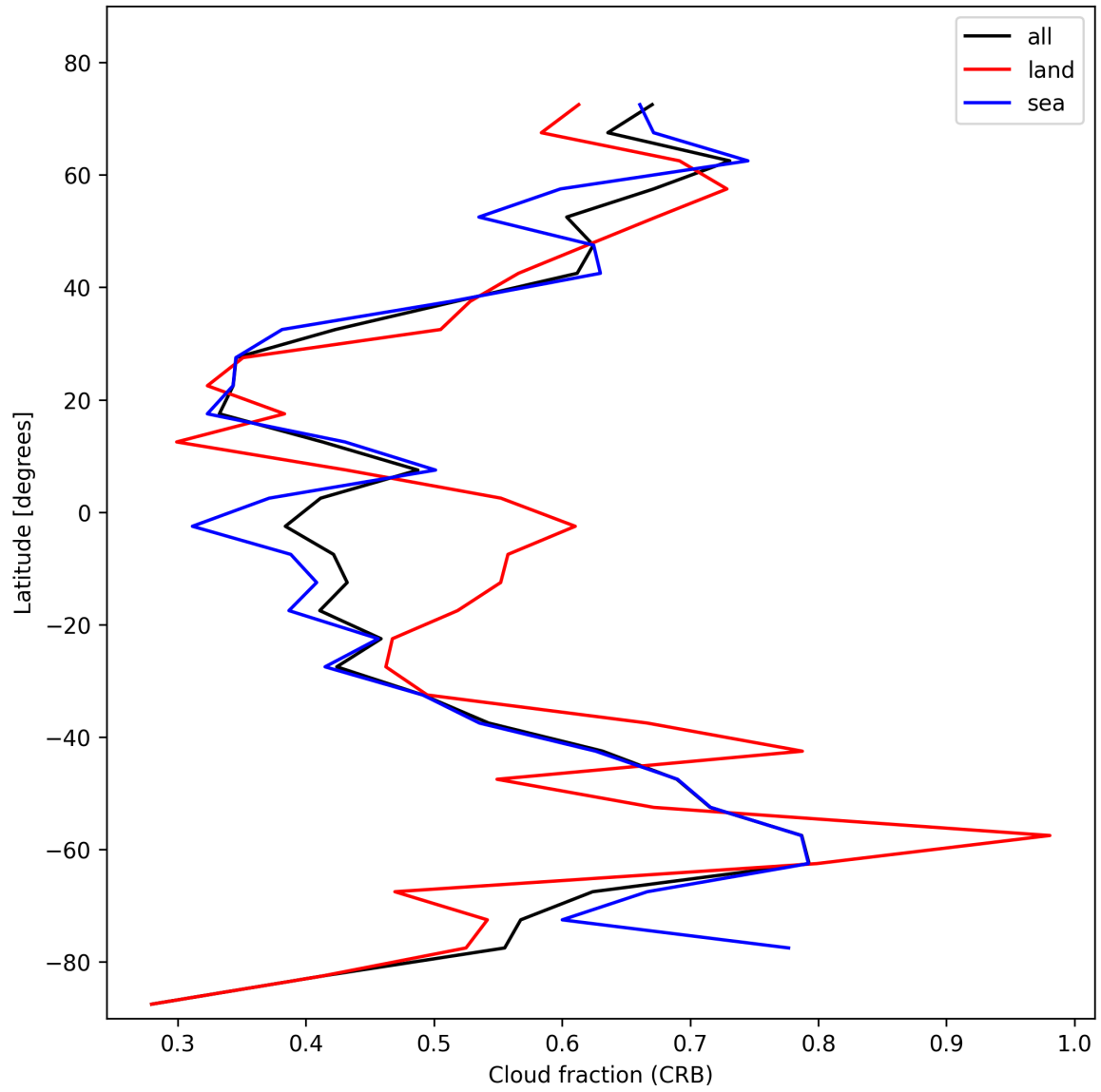
Figure 26: Zonal average of “Cloud fraction (CRB)” for 2024-11-02 to 2024-11-04.
