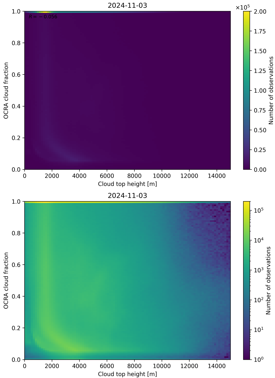
Figure 87: Scatter density plot of “Cloud top height” against “OCRA cloud fraction” for 2024-11-02 to 2024-11-04.
