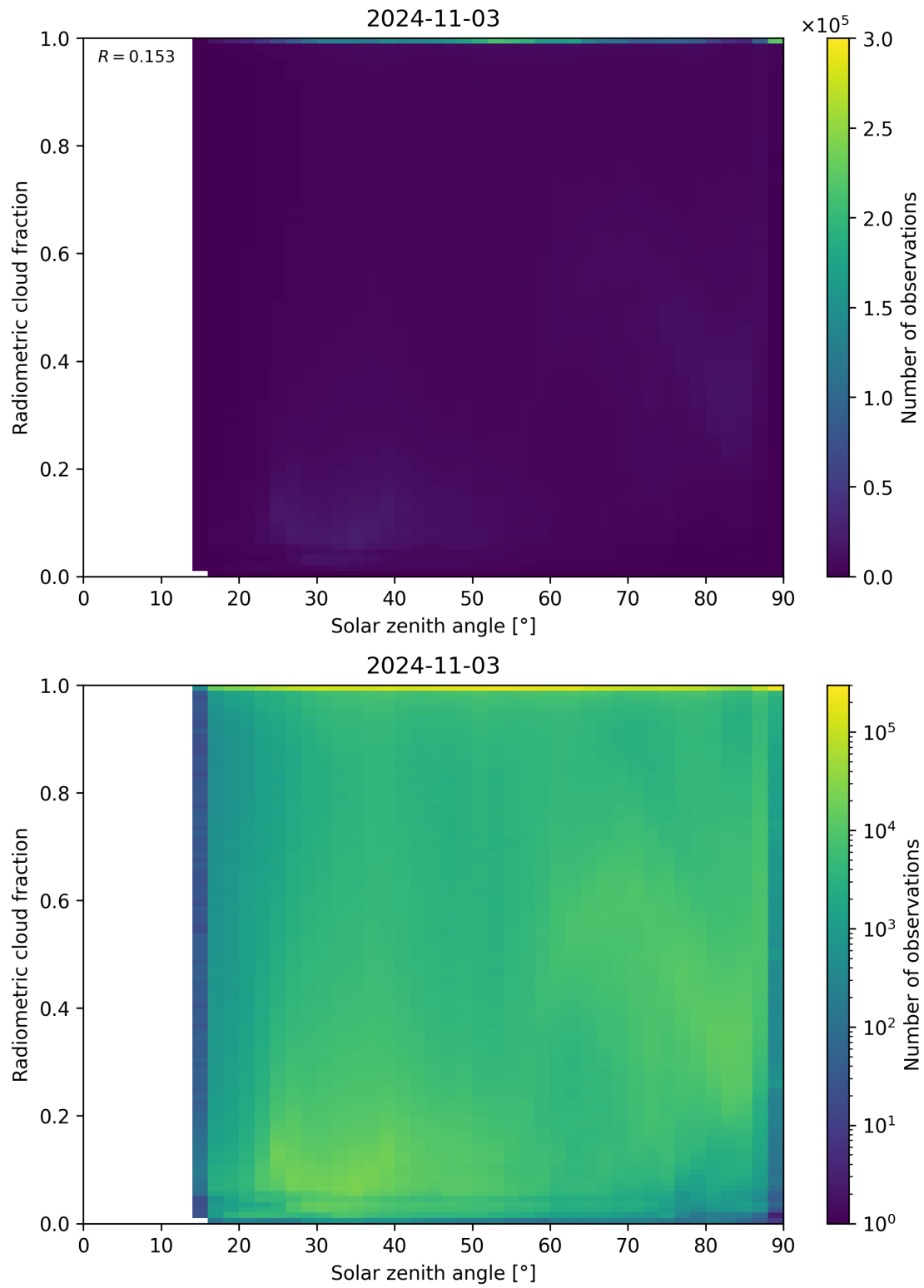
Figure 99: Scatter density plot of “Solar zenith angle” against “Radiometric cloud fraction” for 2024-11-02 to 2024-11-04.
