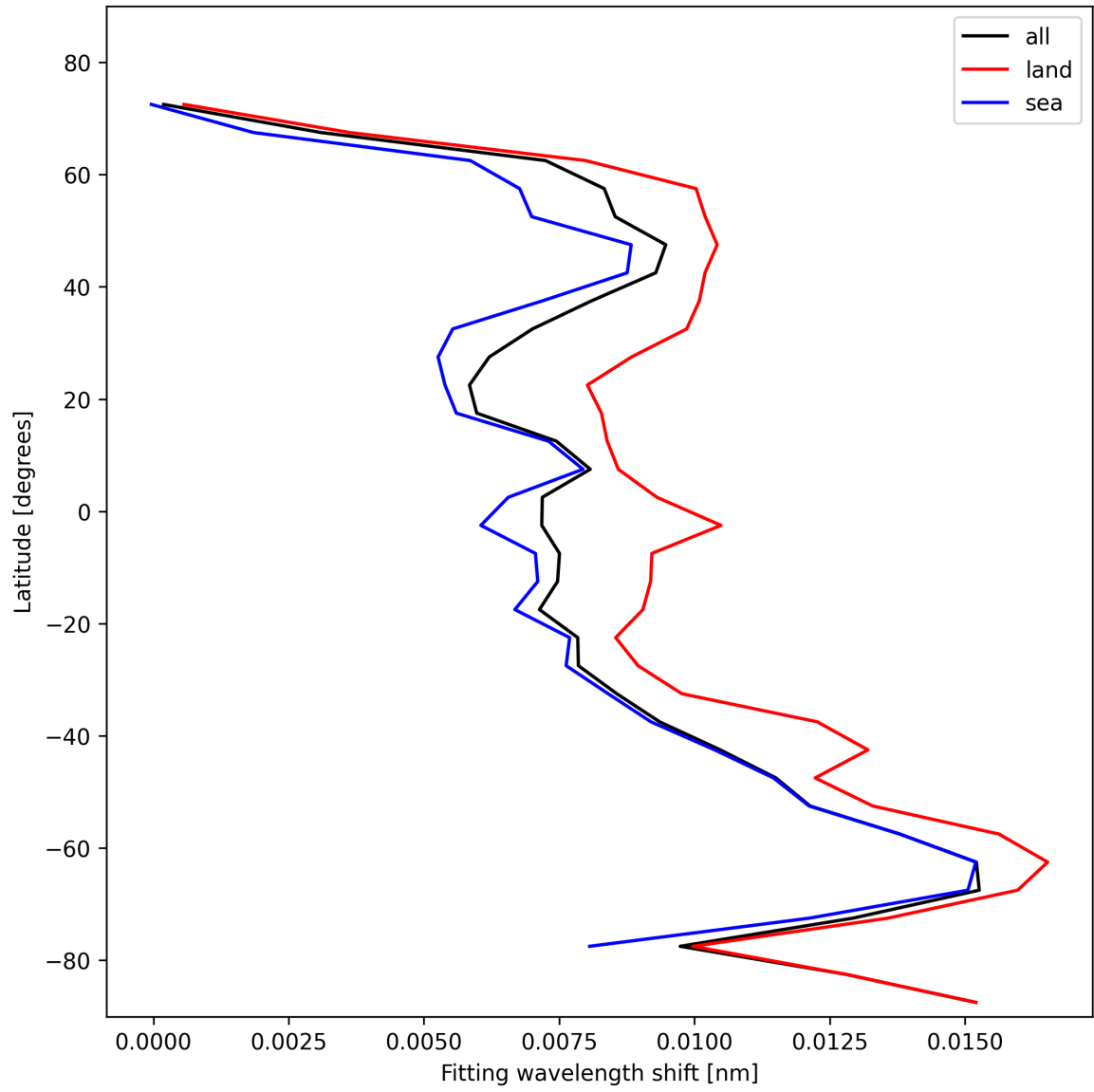
Figure 33: Zonal average of “Fitting wavelength shift” for 2024-11-02 to 2024-11-04.
