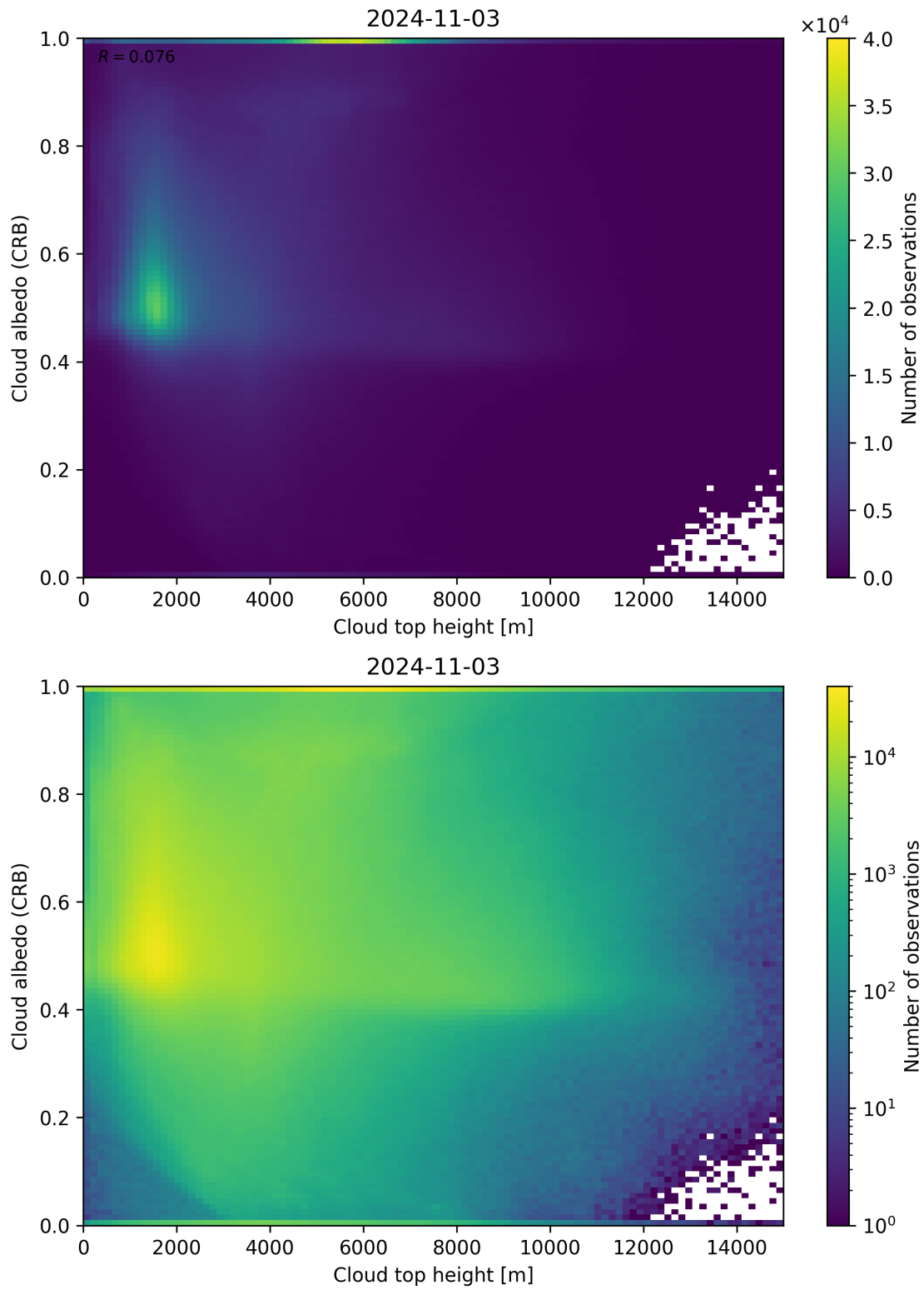
Figure 86: Scatter density plot of “Cloud top height” against “Cloud albedo (CRB)” for 2024-11-02 to 2024-11-04.
