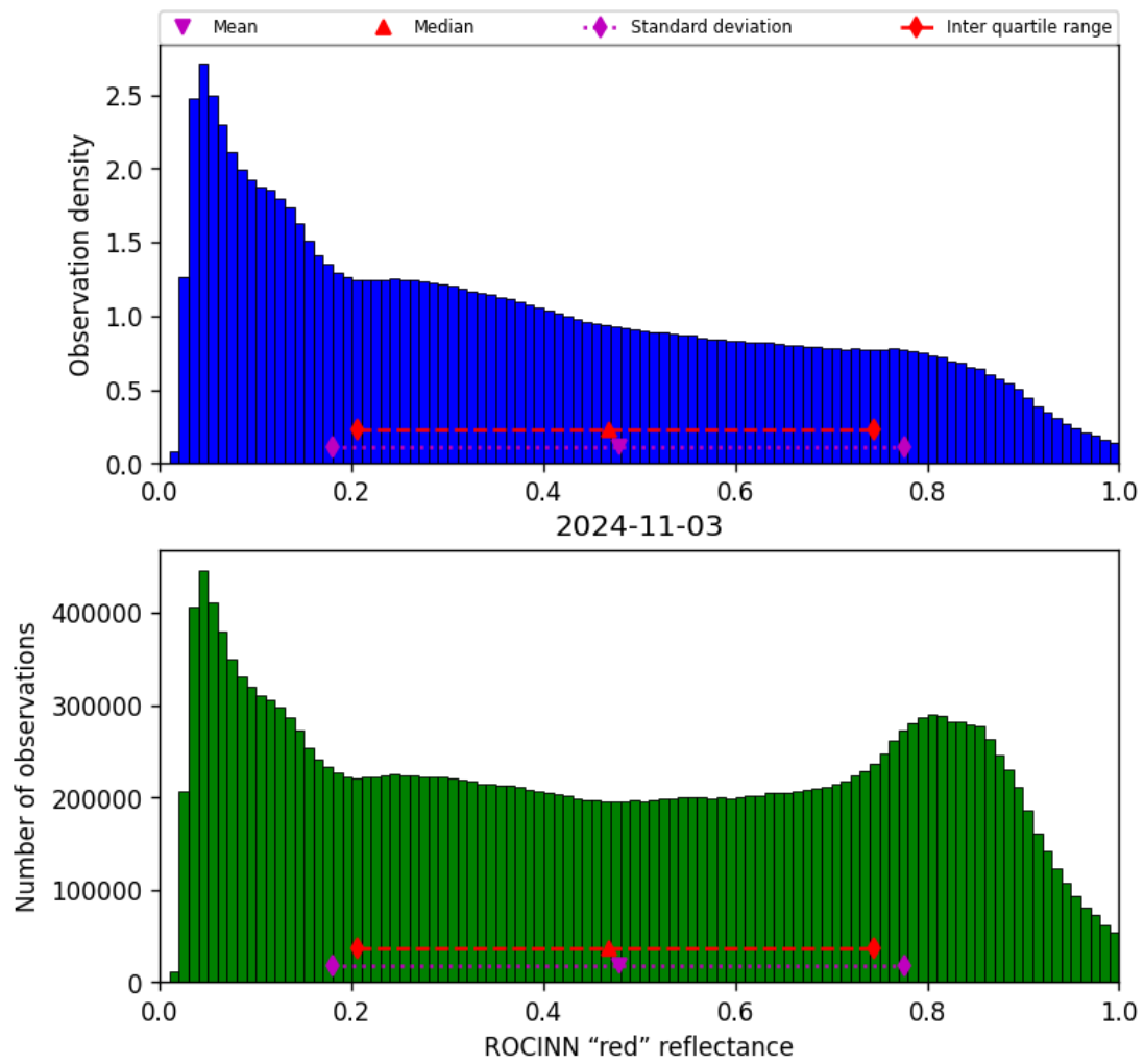
Figure 53: Histogram of “ROCINN “red” reflectance” for 2024-11-02 to 2024-11-04
