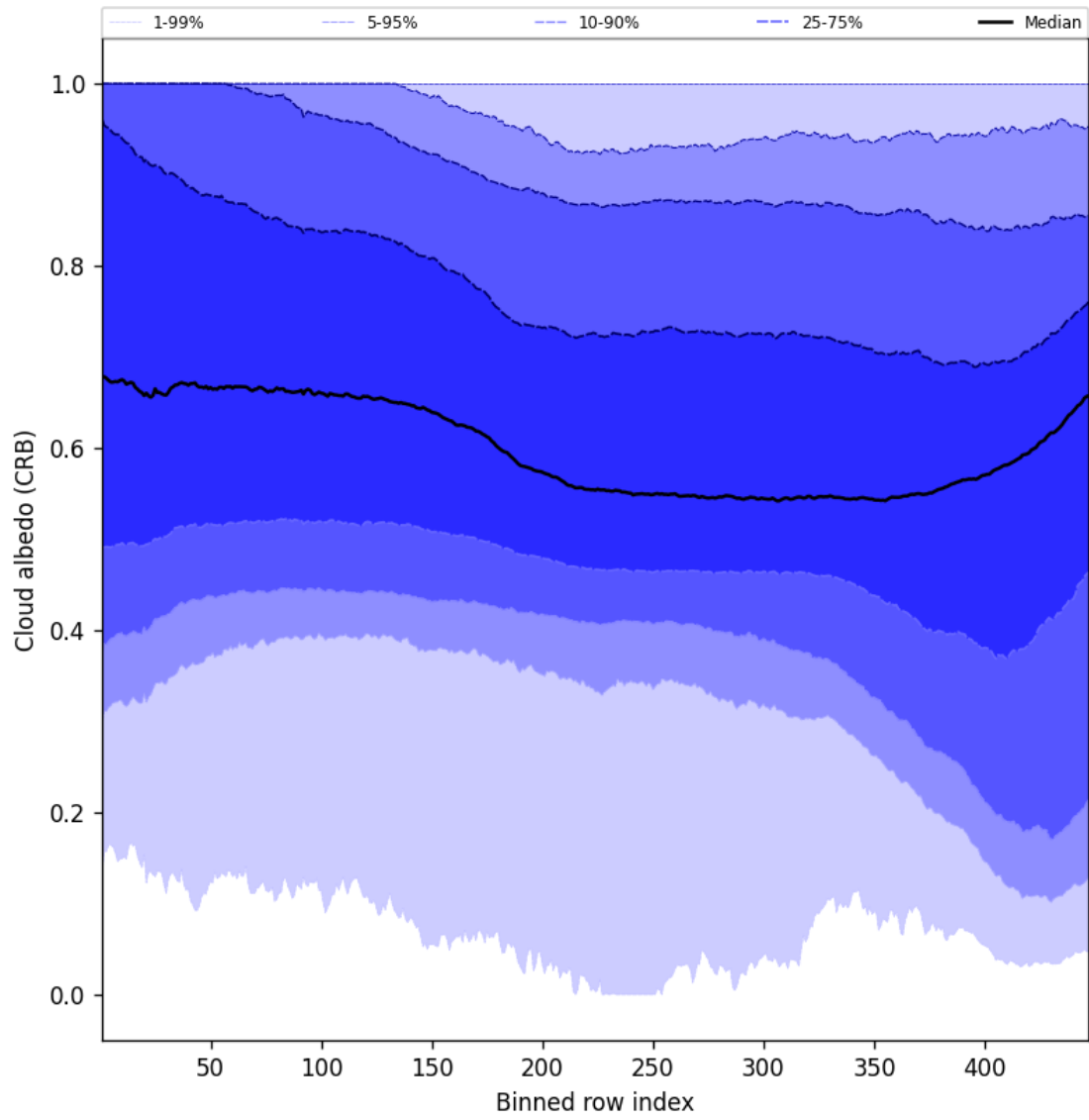
Figure 60: Along track statistics of “Cloud albedo (CRB)” for 2024-11-02 to 2024-11-04
