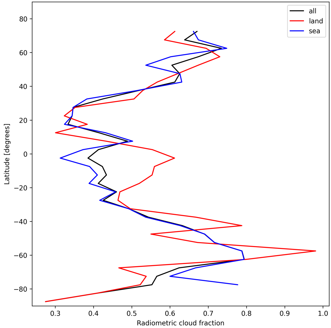
Figure 23: Zonal average of “Radiometric cloud fraction” for 2024-11-02 to 2024-11-04.
