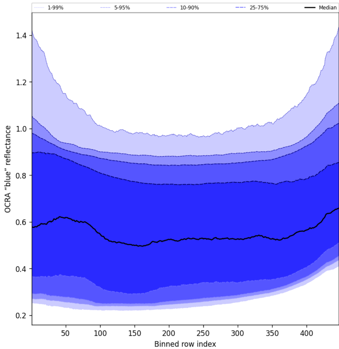
Figure 67: Along track statistics of “OCRA “blue” reflectance” for 2024-11-02 to 2024-11-04
