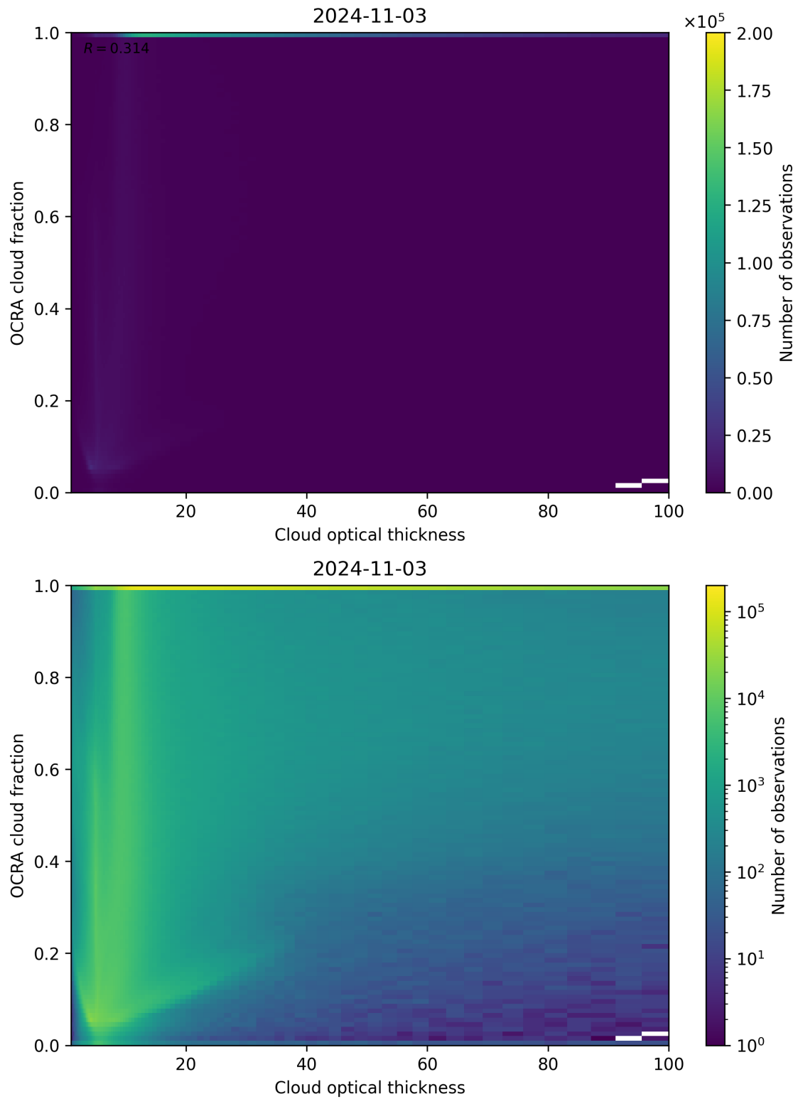
Figure 83: Scatter density plot of “Cloud optical thickness” against “OCRA cloud fraction” for 2024-11-02 to 2024-11-04.
