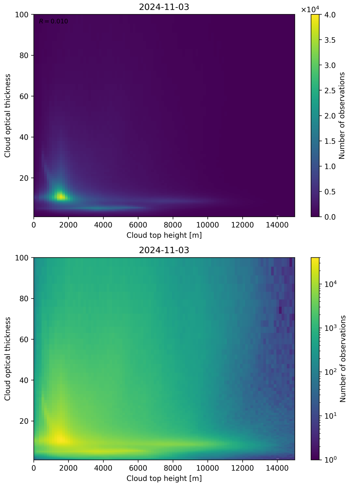
Figure 90: Scatter density plot of “Cloud top height” against “Cloud optical thickness” for 2024-11-02 to 2024-11-04.
