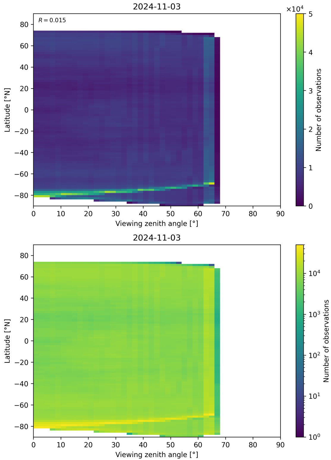
Figure 113: Scatter density plot of “Viewing zenith angle” against “Latitude” for 2024-11-02 to 2024-11-04.
