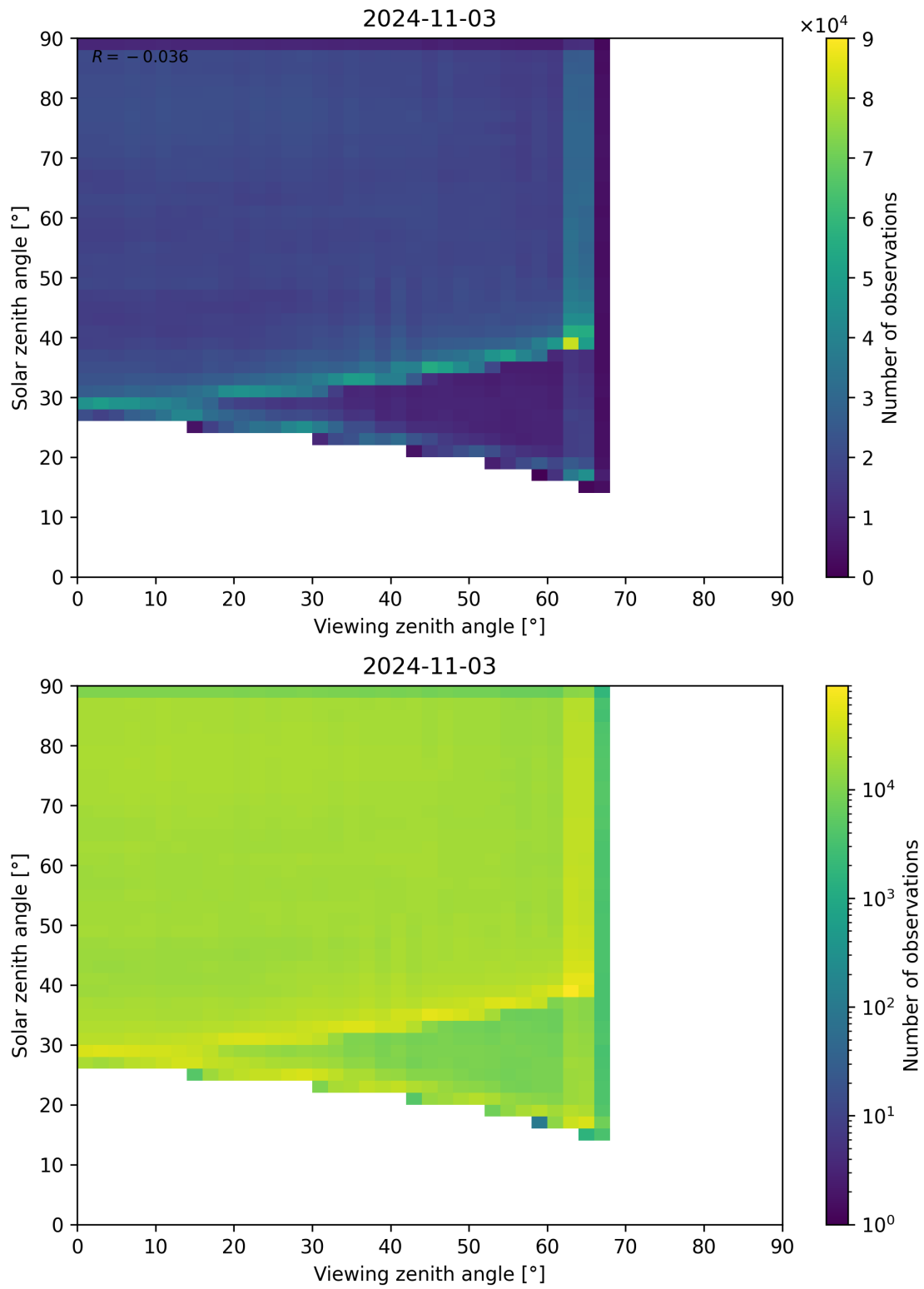
Figure 114: Scatter density plot of “Viewing zenith angle” against “Solar zenith angle” for 2024-11-02 to 2024-11-04.
