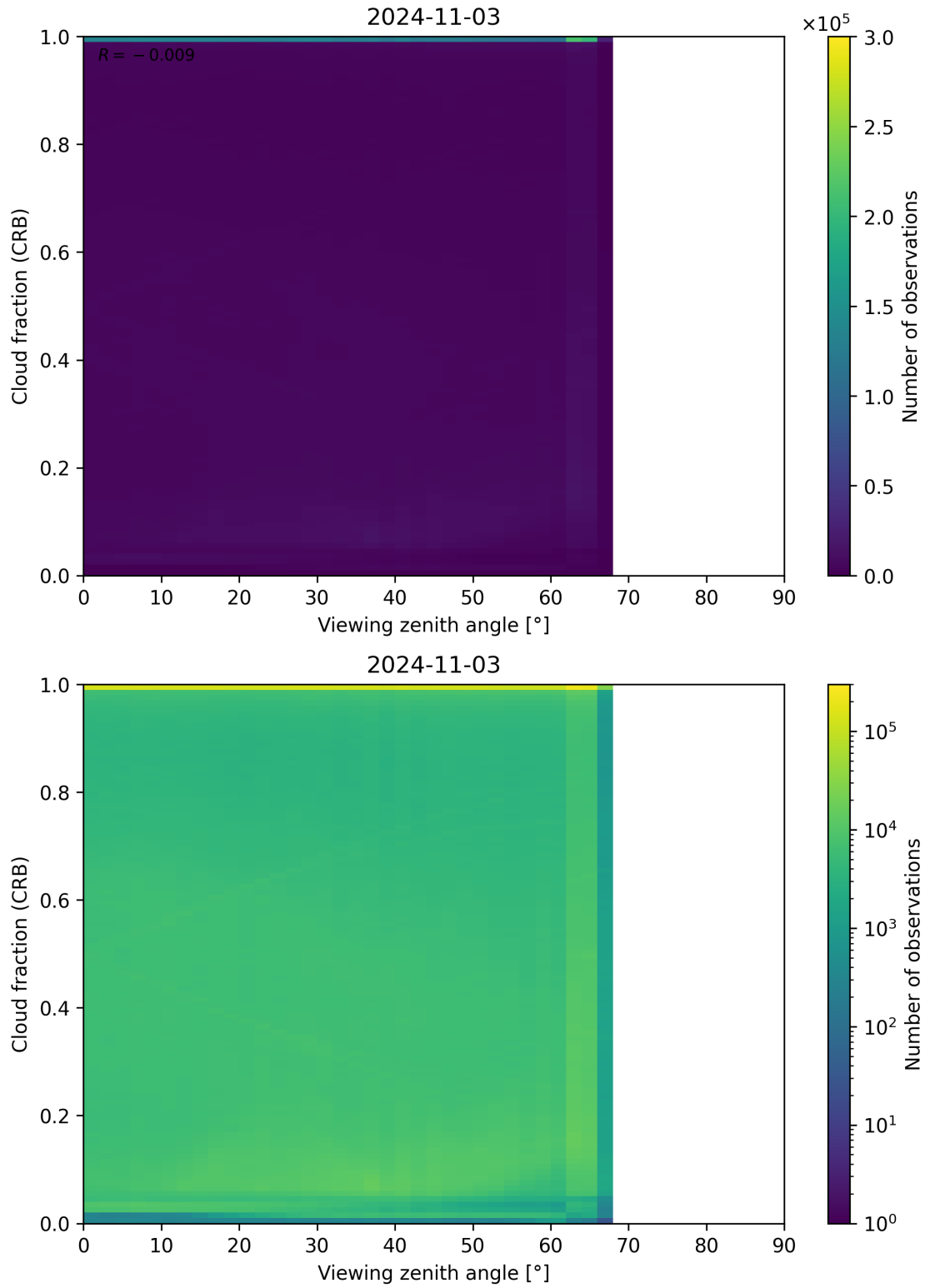
Figure 109: Scatter density plot of “Viewing zenith angle” against “Cloud fraction (CRB)” for 2024-11-02 to 2024-11-04.
