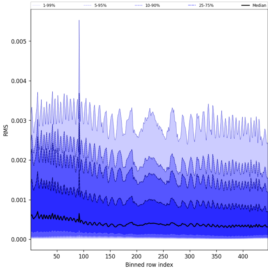
Figure 63: Along track statistics of “RMS” for 2024-11-02 to 2024-11-04
