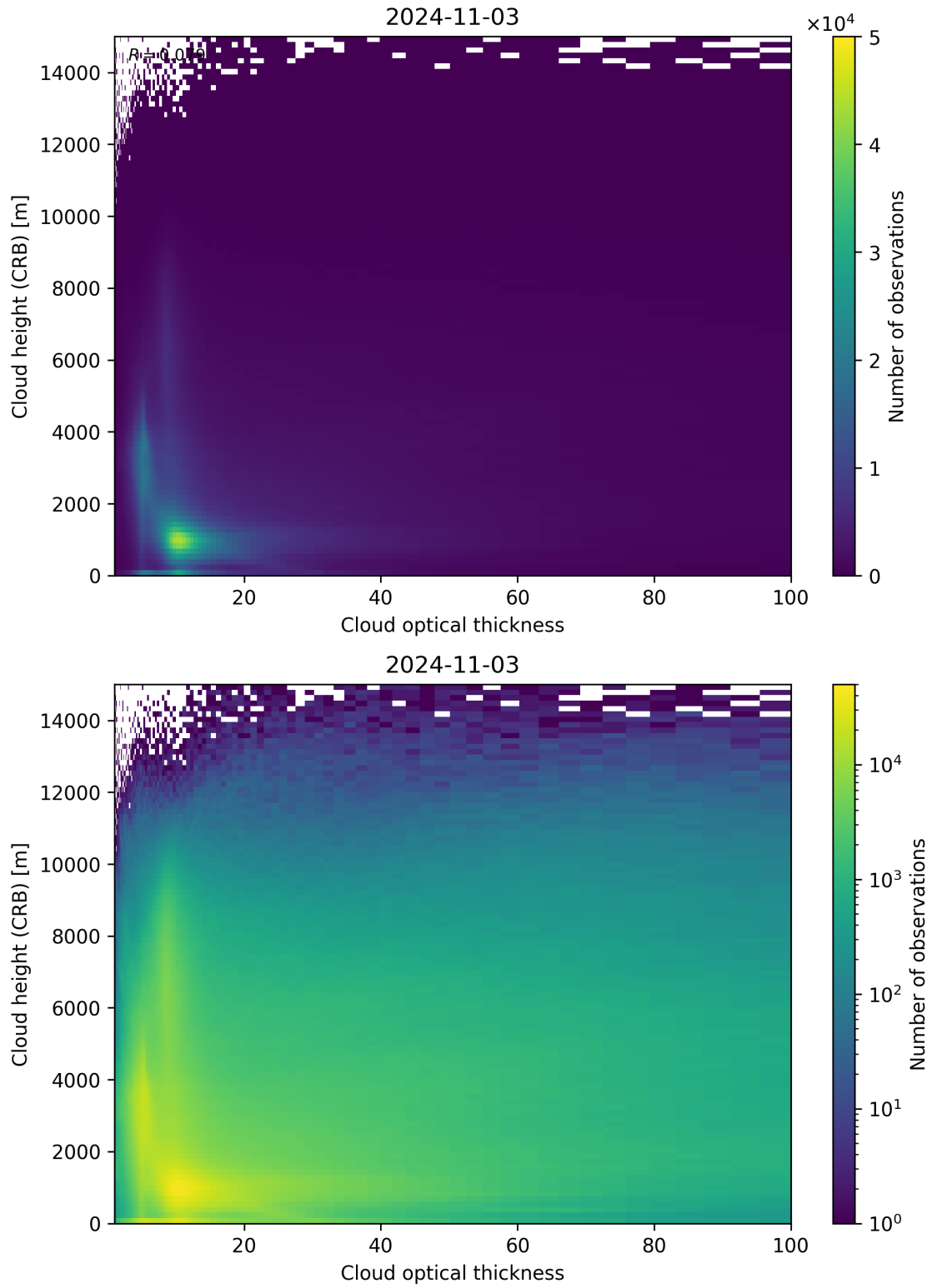
Figure 85: Scatter density plot of “Cloud optical thickness” against “Cloud height (CRB)” for 2024-11-02 to 2024-11-04.
