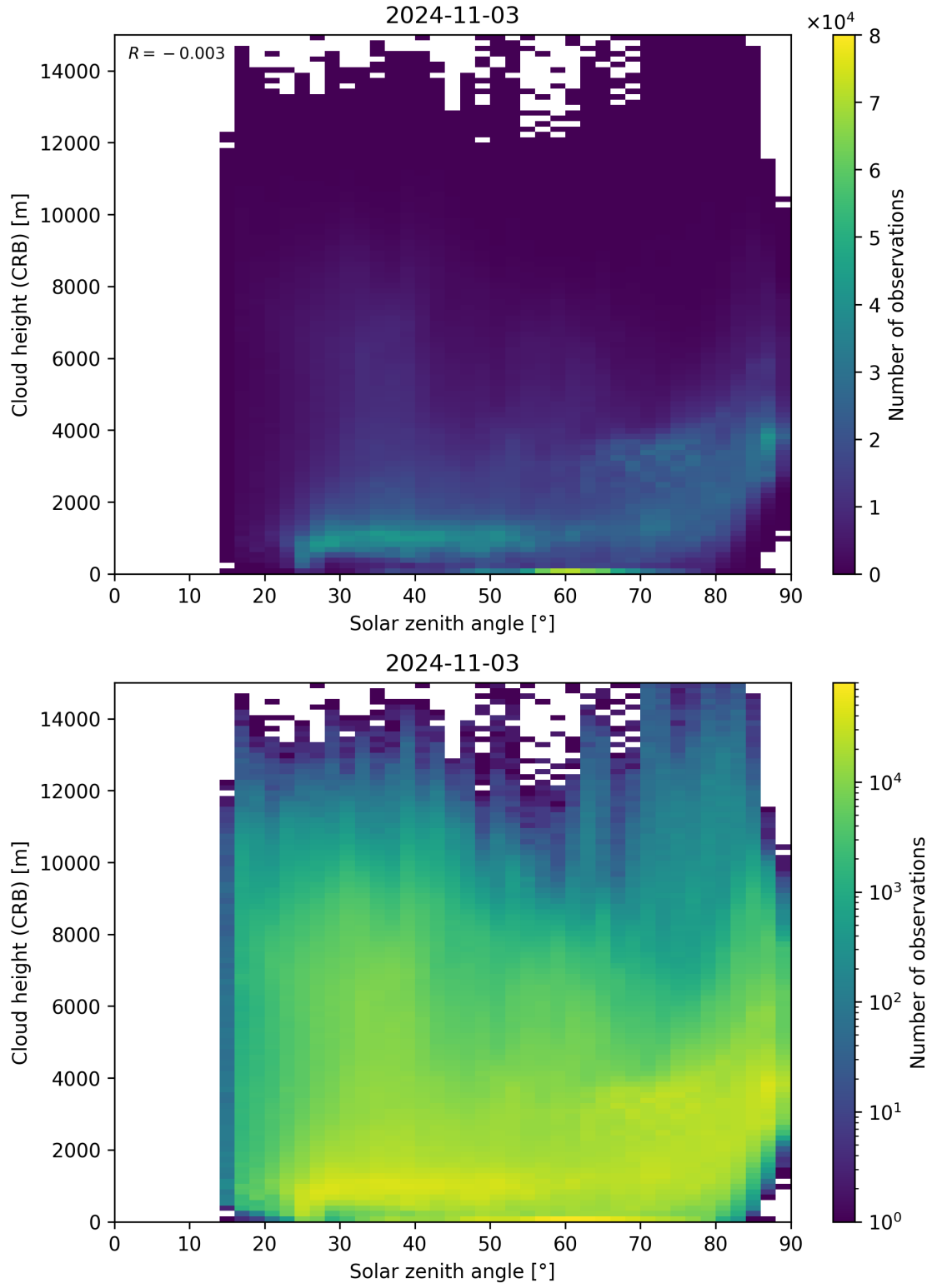
Figure 102: Scatter density plot of “Solar zenith angle” against “Cloud height (CRB)” for 2024-11-02 to 2024-11-04.
