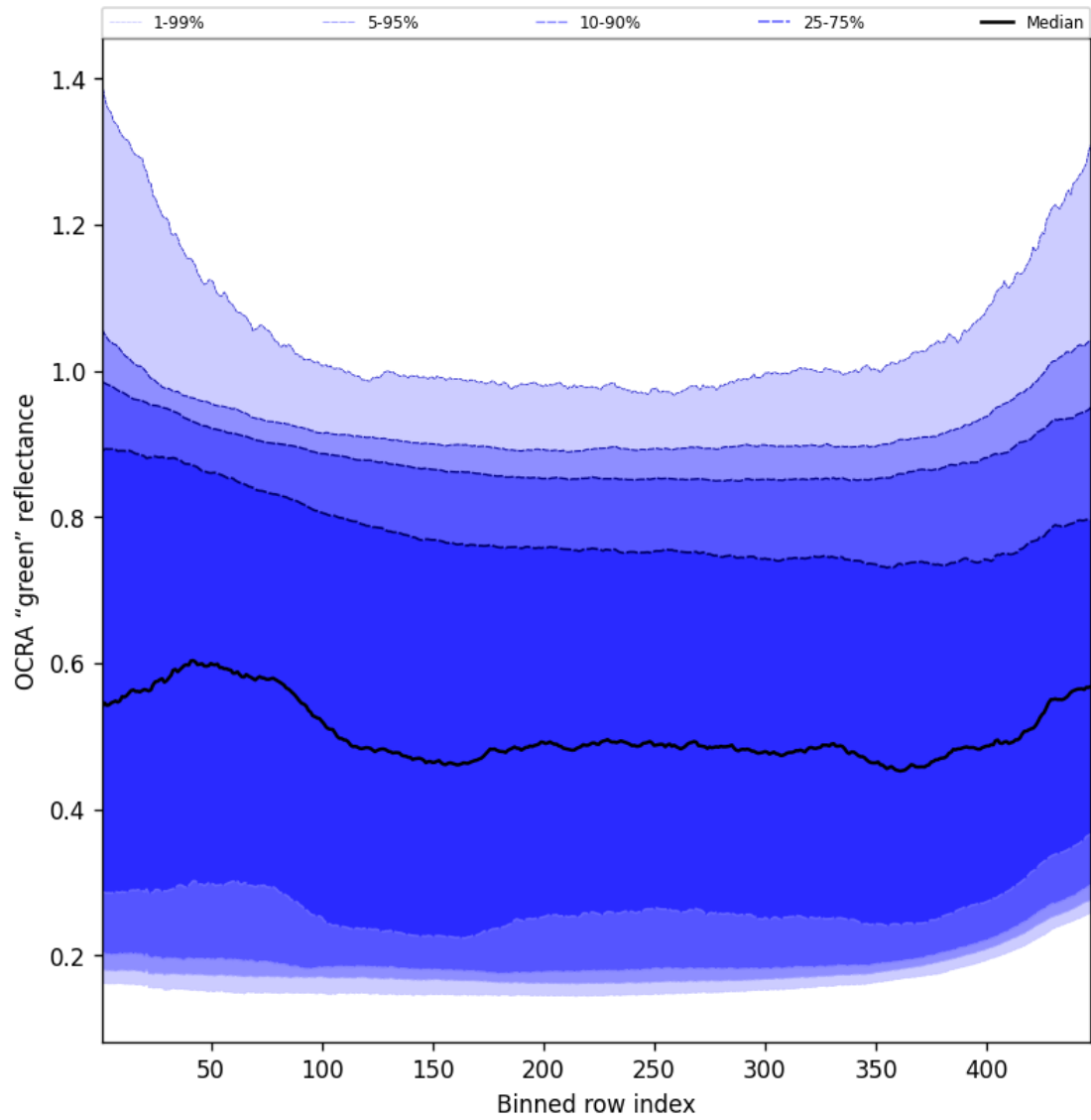
Figure 68: Along track statistics of “OCRA “green” reflectance” for 2024-11-02 to 2024-11-04
