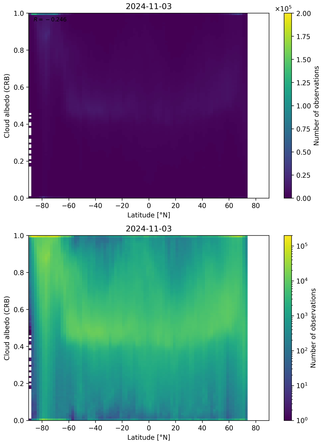
Figure 91: Scatter density plot of “Latitude” against “Cloud albedo (CRB)” for 2024-11-02 to 2024-11-04.
