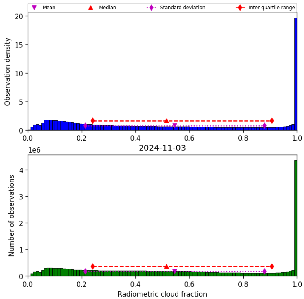
Figure 39: Histogram of “Radiometric cloud fraction” for 2024-11-02 to 2024-11-04
