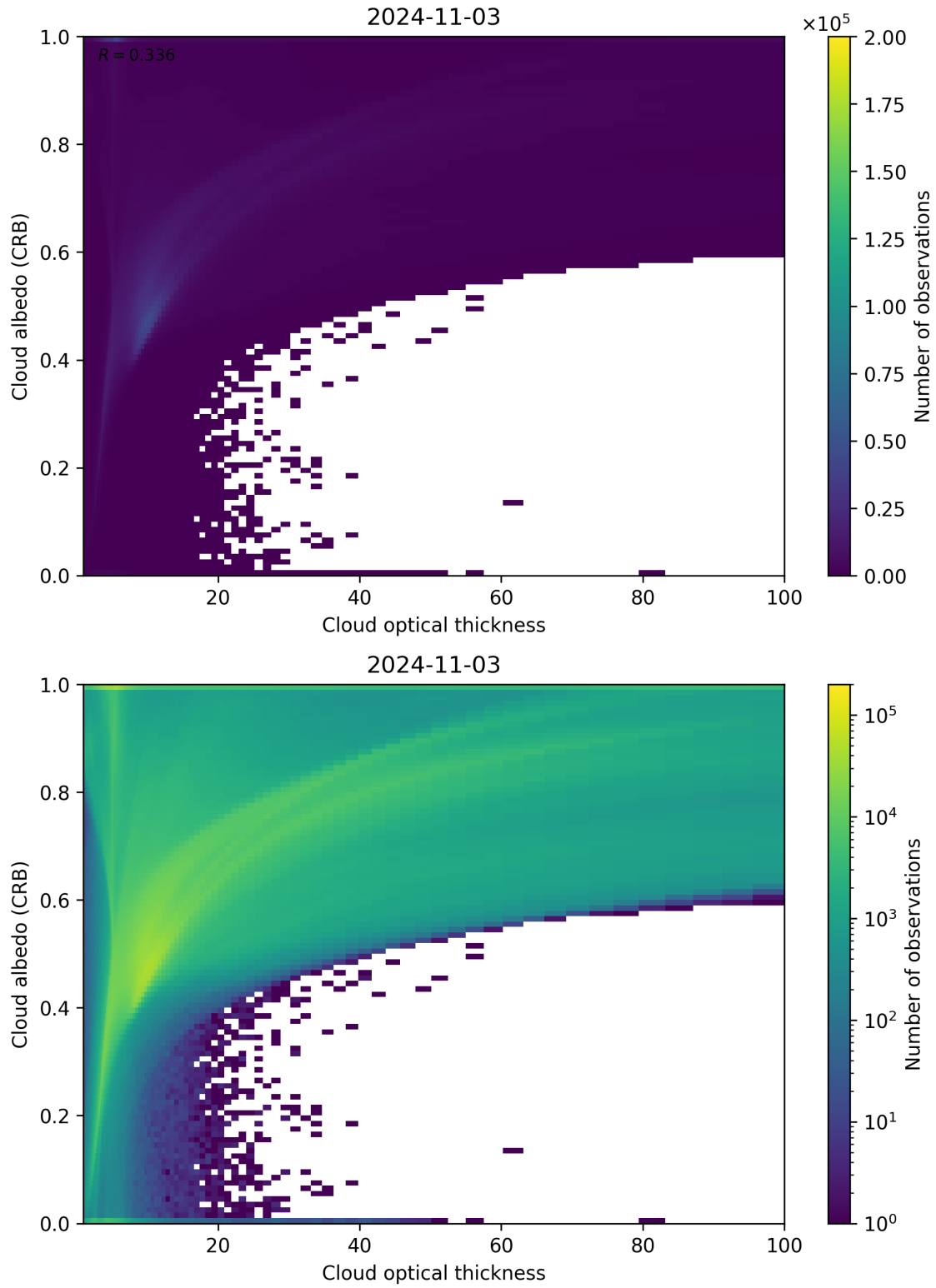
Figure 82: Scatter density plot of “Cloud optical thickness” against “Cloud albedo (CRB)” for 2024-11-02 to 2024-11-04.
