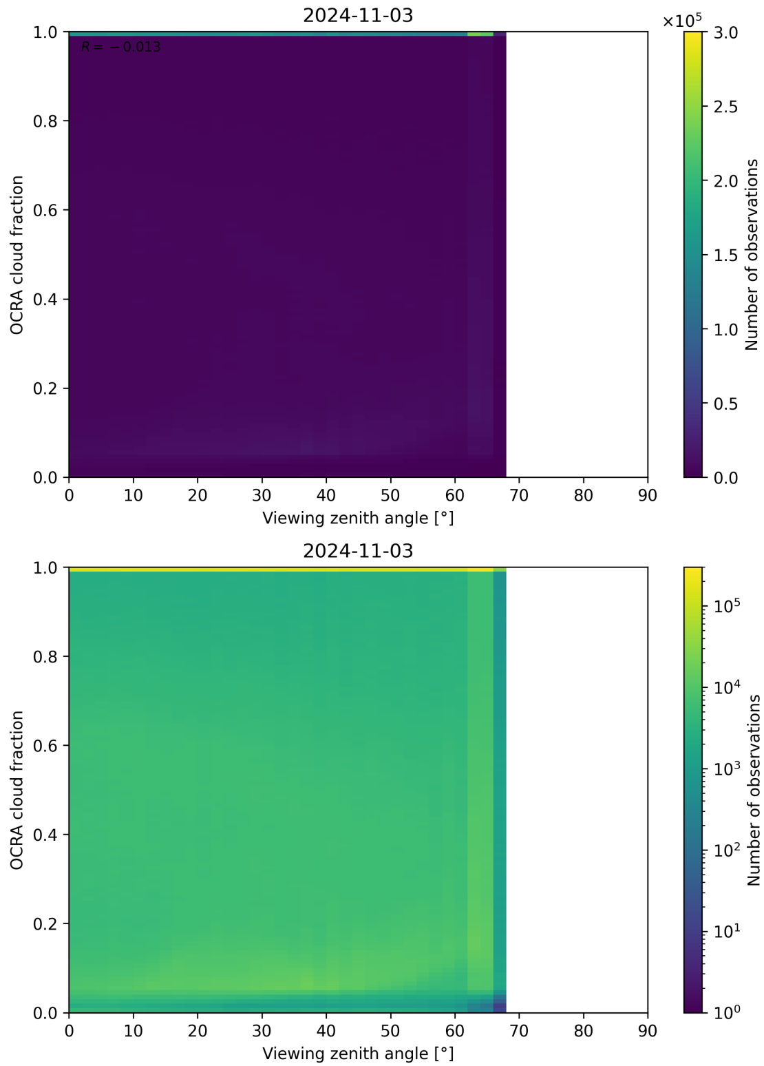
Figure 108: Scatter density plot of “Viewing zenith angle” against “OCRA cloud fraction” for 2024-11-02 to 2024-11-04.
