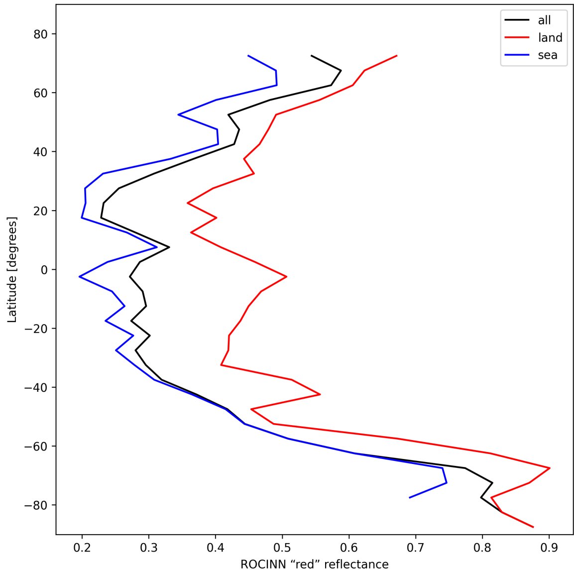
Figure 37: Zonal average of “ROCINN “red” reflectance” for 2024-11-02 to 2024-11-04.
