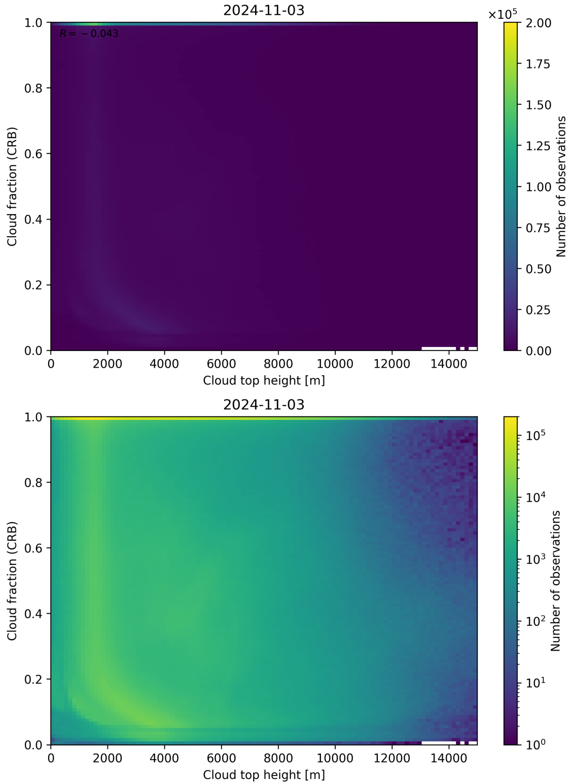
Figure 88: Scatter density plot of “Cloud top height” against “Cloud fraction (CRB)” for 2024-11-02 to 2024-11-04.
