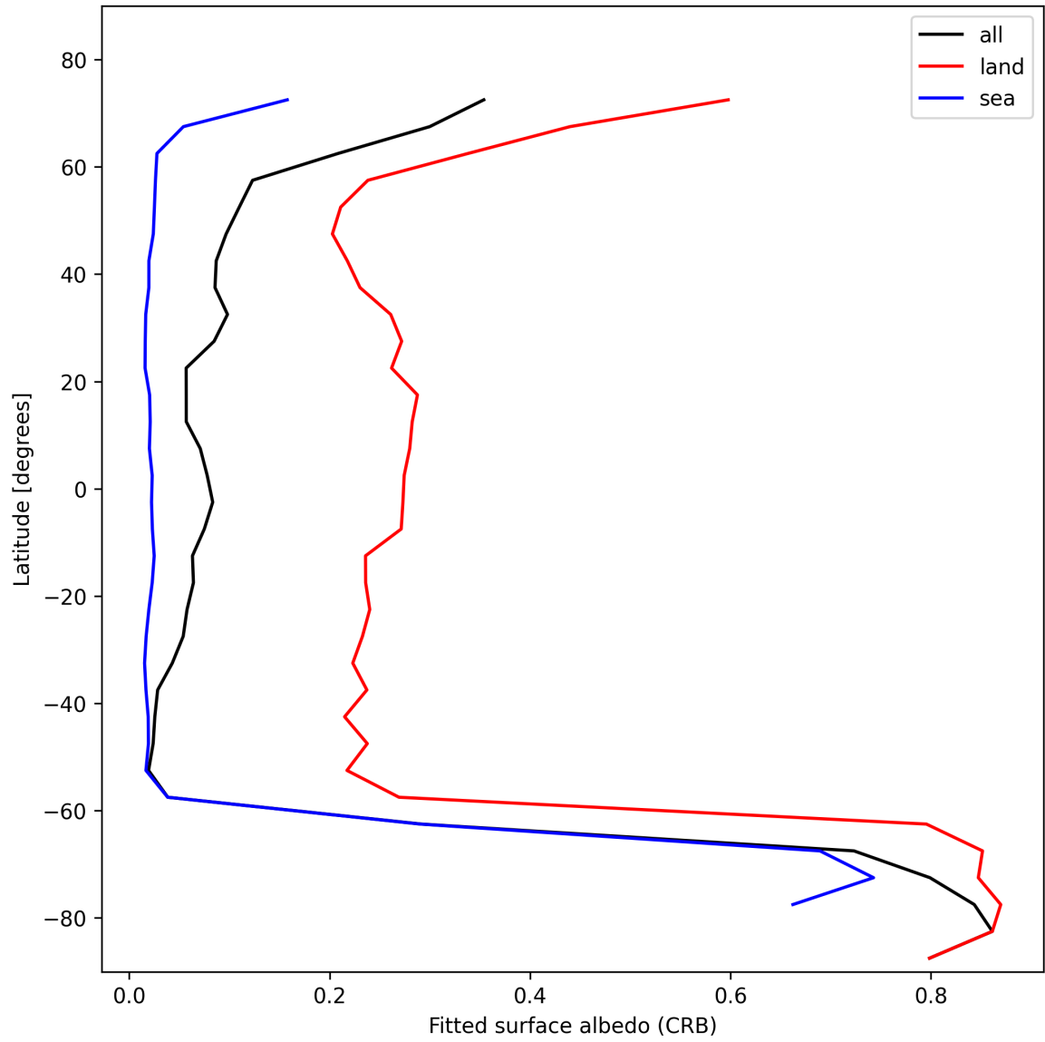
Figure 30: Zonal average of “Fitted surface albedo (CRB)” for 2024-11-02 to 2024-11-04.
