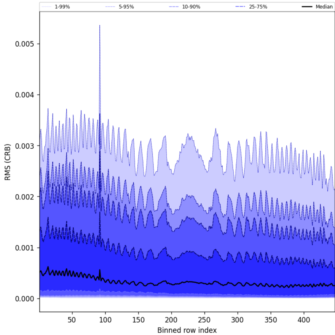
Figure 64: Along track statistics of “RMS (CRB)” for 2024-11-02 to 2024-11-04
