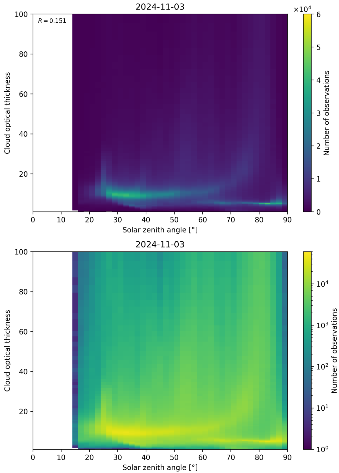
Figure 103: Scatter density plot of “Solar zenith angle” against “Cloud optical thickness” for 2024-11-02 to 2024-11-04.
