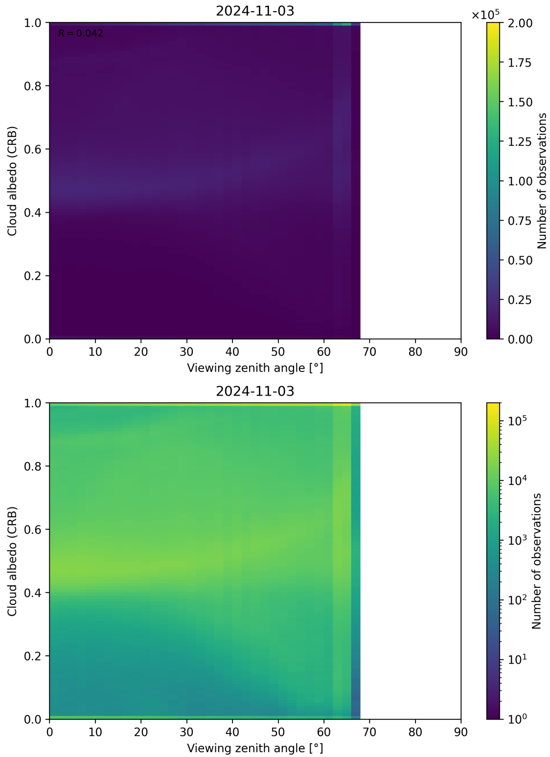
Figure 106: Scatter density plot of “Viewing zenith angle” against “Cloud albedo (CRB)” for 2024-11-02 to 2024-11-04.
