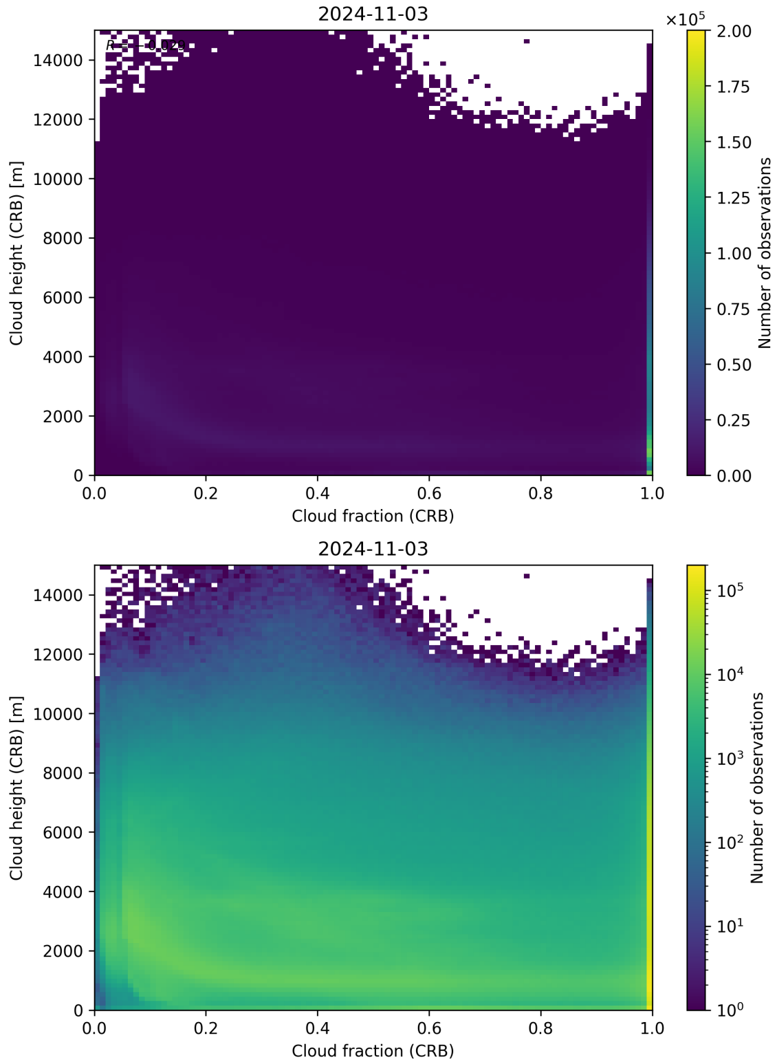
Figure 79: Scatter density plot of “Cloud fraction (CRB)” against “Cloud height (CRB)” for 2024-11-02 to 2024-11-04.
