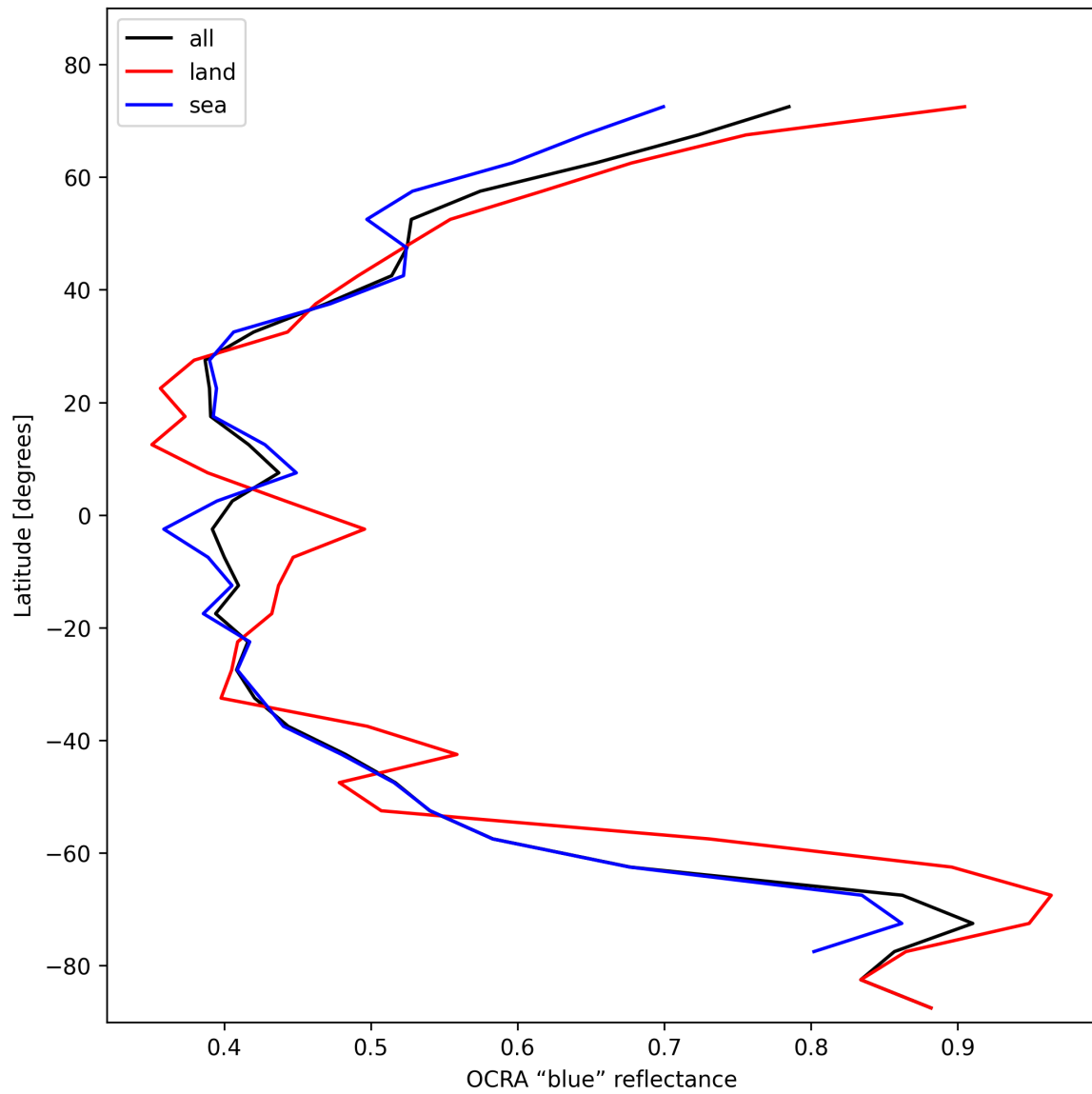
Figure 35: Zonal average of “OCRA “blue” reflectance” for 2024-11-02 to 2024-11-04.
