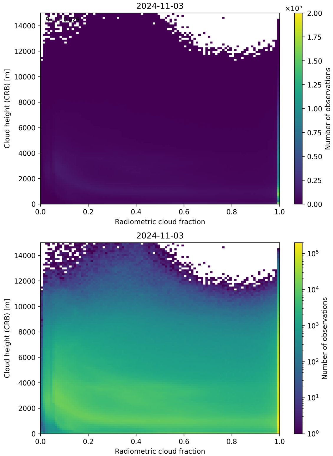
Figure 74: Scatter density plot of “Radiometric cloud fraction” against “Cloud height (CRB)” for 2024-11-02 to 2024-11-04.
