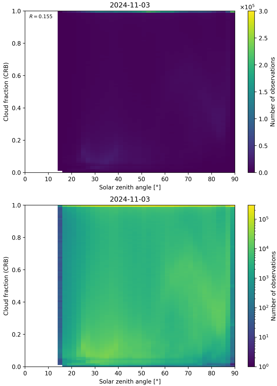
Figure 101: Scatter density plot of “Solar zenith angle” against “Cloud fraction (CRB)” for 2024-11-02 to 2024-11-04.
