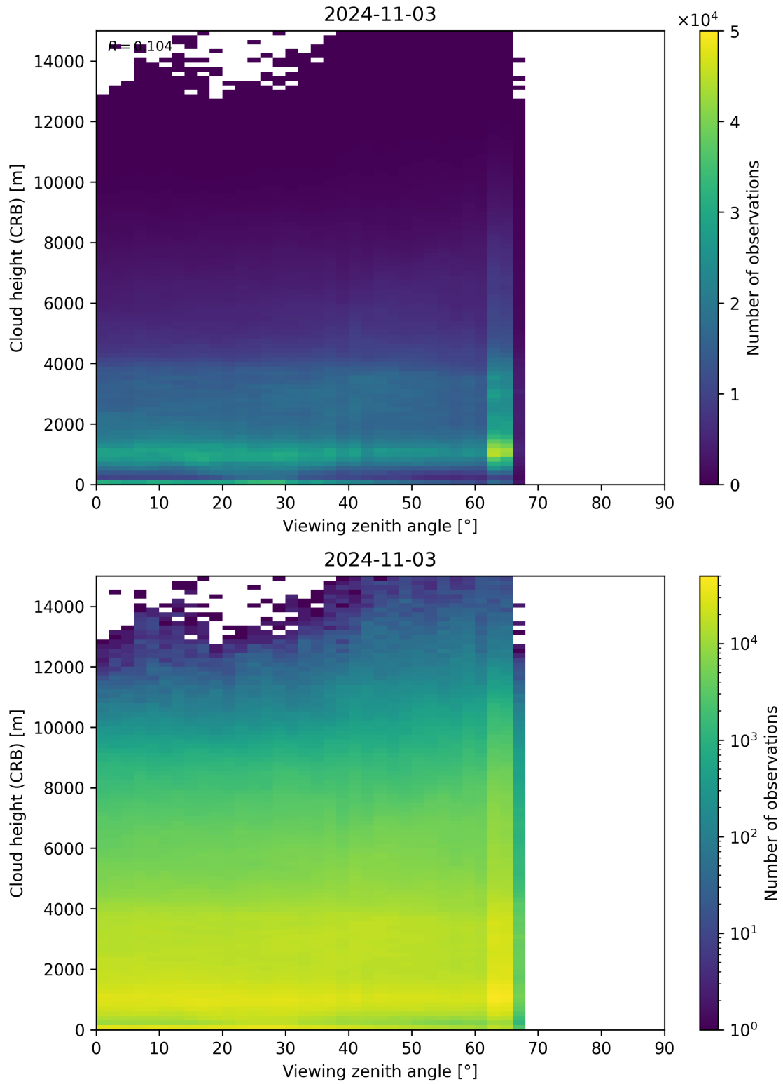
Figure 110: Scatter density plot of “Viewing zenith angle” against “Cloud height (CRB)” for 2024-11-02 to 2024-11-04.
