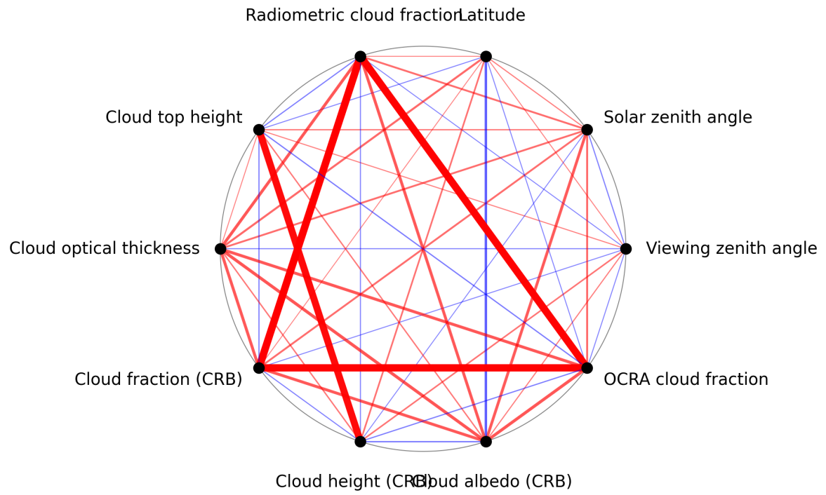
Figure 1: Map of correlation graph for 2024-11-02 to 2024-11-04.
