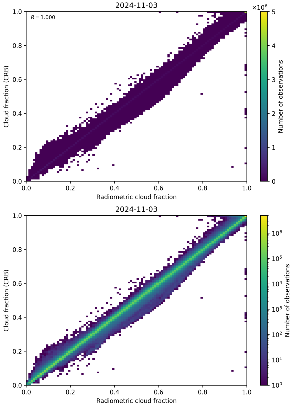
Figure 73: Scatter density plot of “Radiometric cloud fraction” against “Cloud fraction (CRB)” for 2024-11-02 to 2024-11-04.
