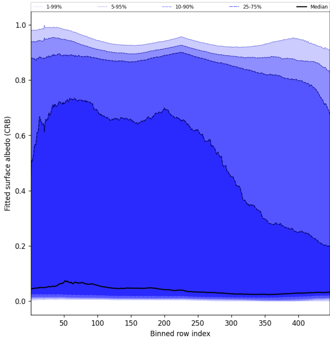
Figure 62: Along track statistics of “Fitted surface albedo (CRB)” for 2024-11-02 to 2024-11-04
