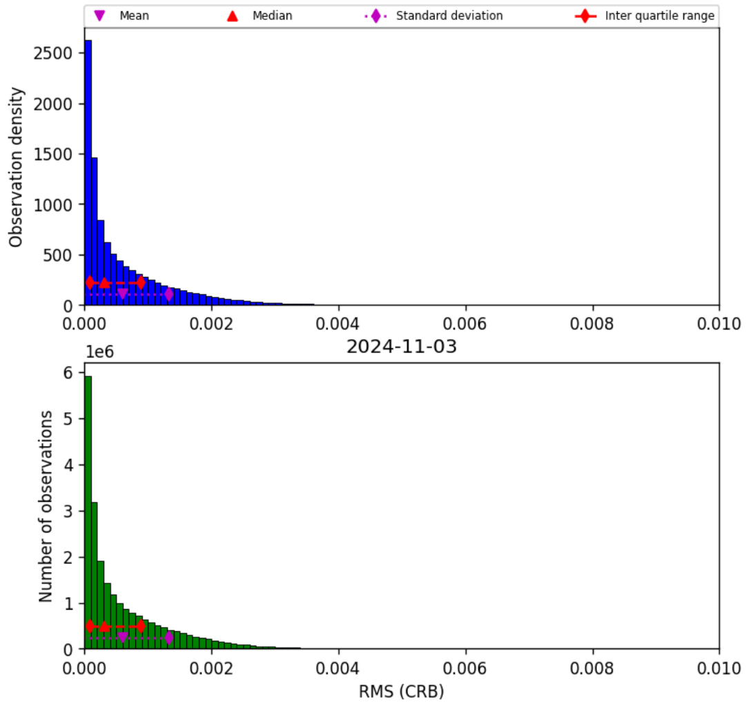
Figure 48: Histogram of “RMS (CRB)” for 2024-11-02 to 2024-11-04
