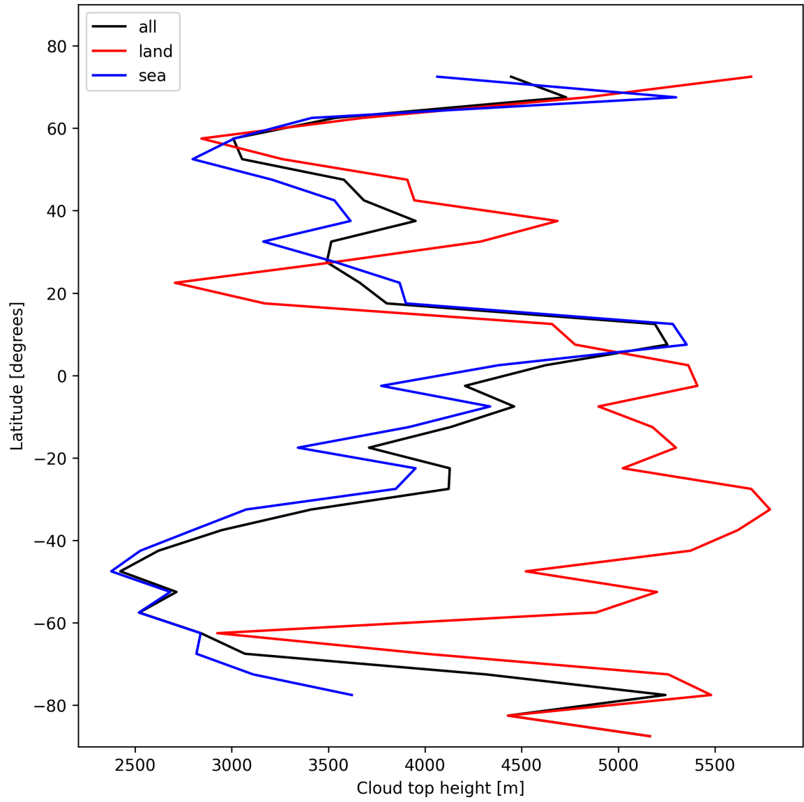
Figure 24: Zonal average of “Cloud top height” for 2024-11-02 to 2024-11-04.
