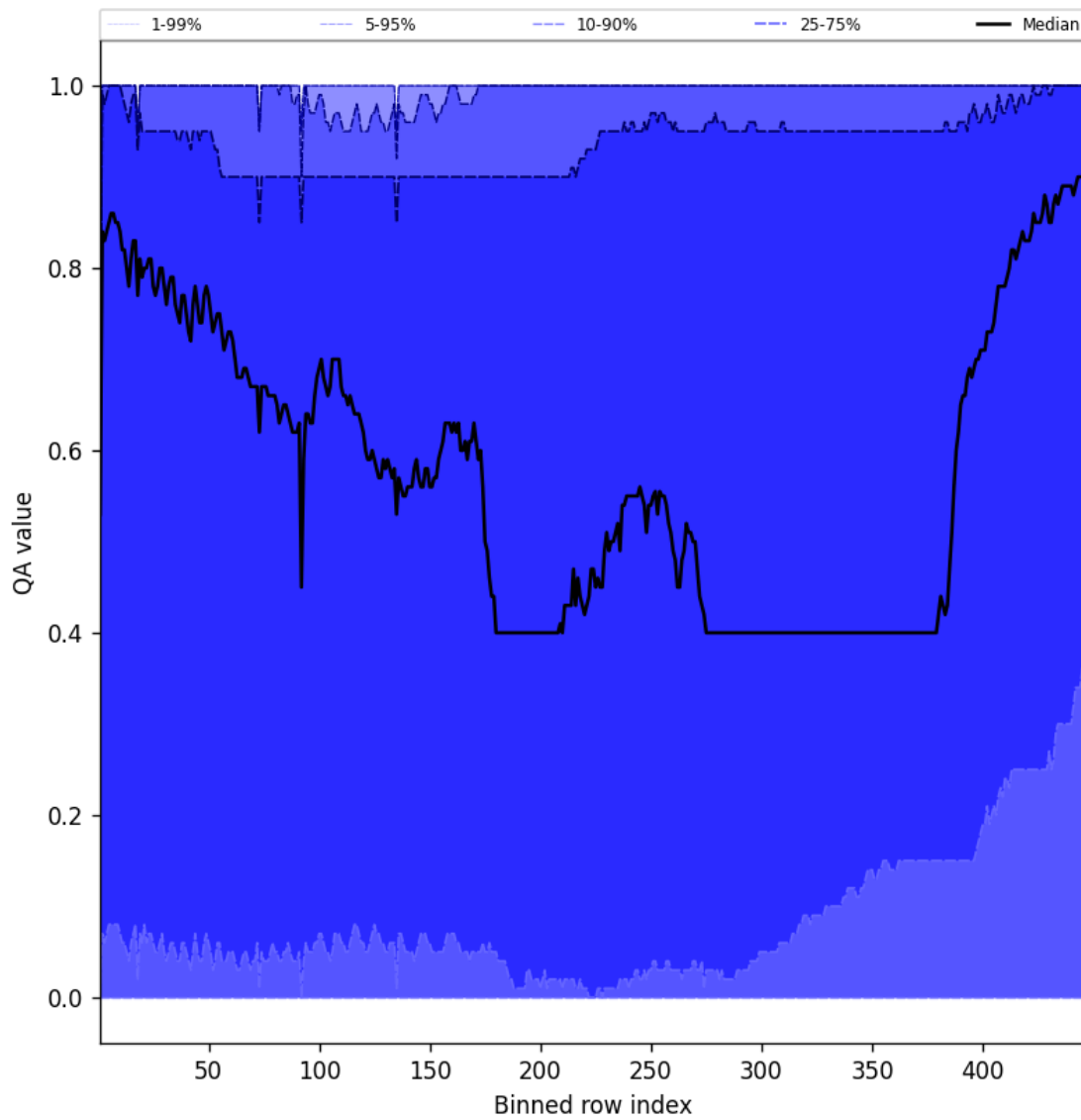
Figure 54: Along track statistics of “QA value” for 2024-11-02 to 2024-11-04
