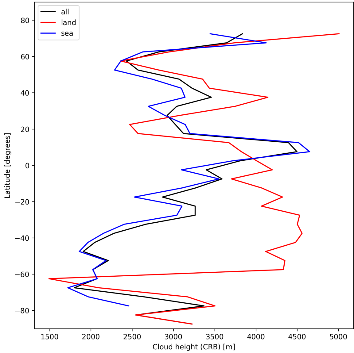
Figure 27: Zonal average of “Cloud height (CRB)” for 2024-11-02 to 2024-11-04.
