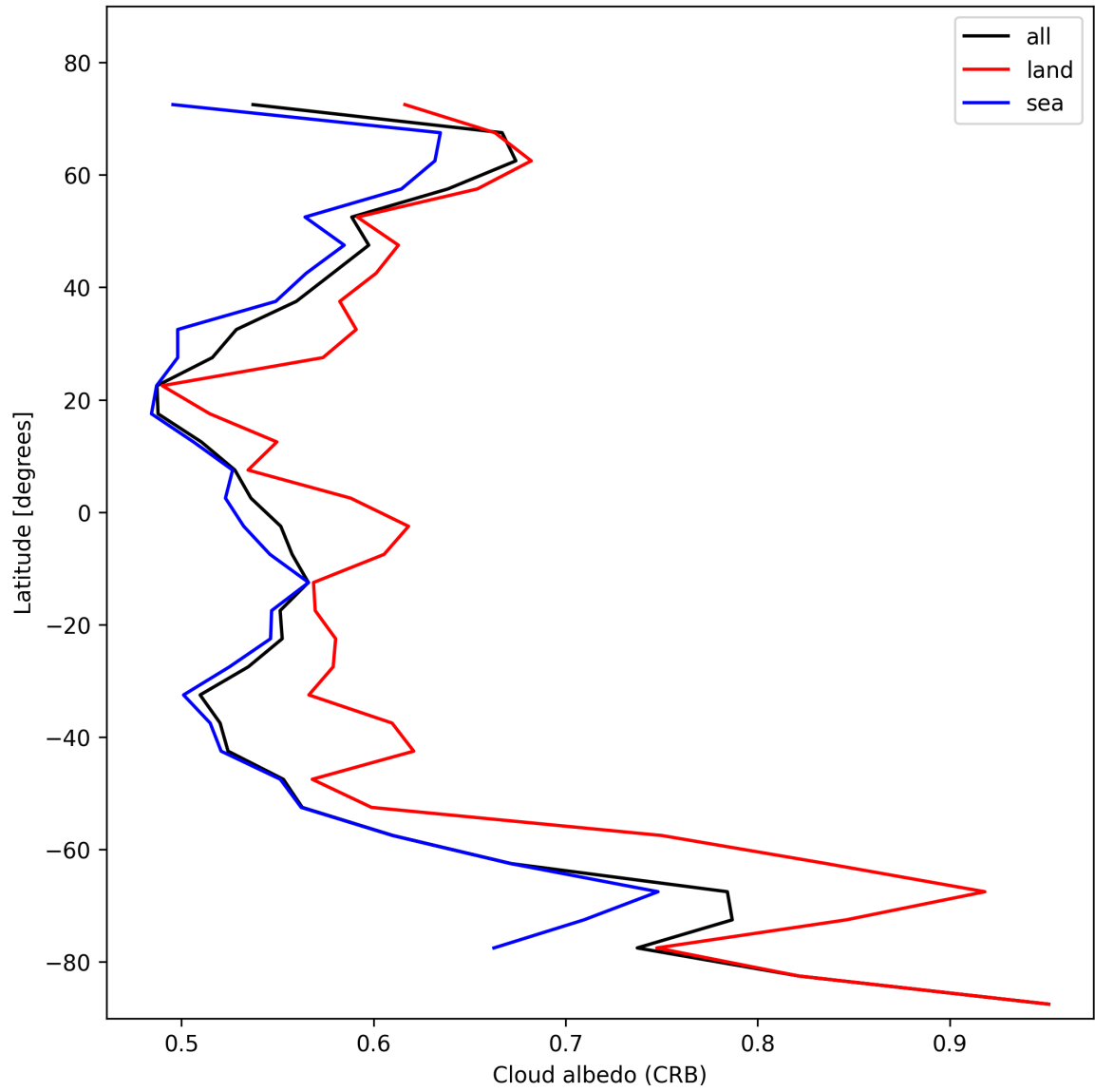
Figure 28: Zonal average of “Cloud albedo (CRB)” for 2024-11-02 to 2024-11-04.
