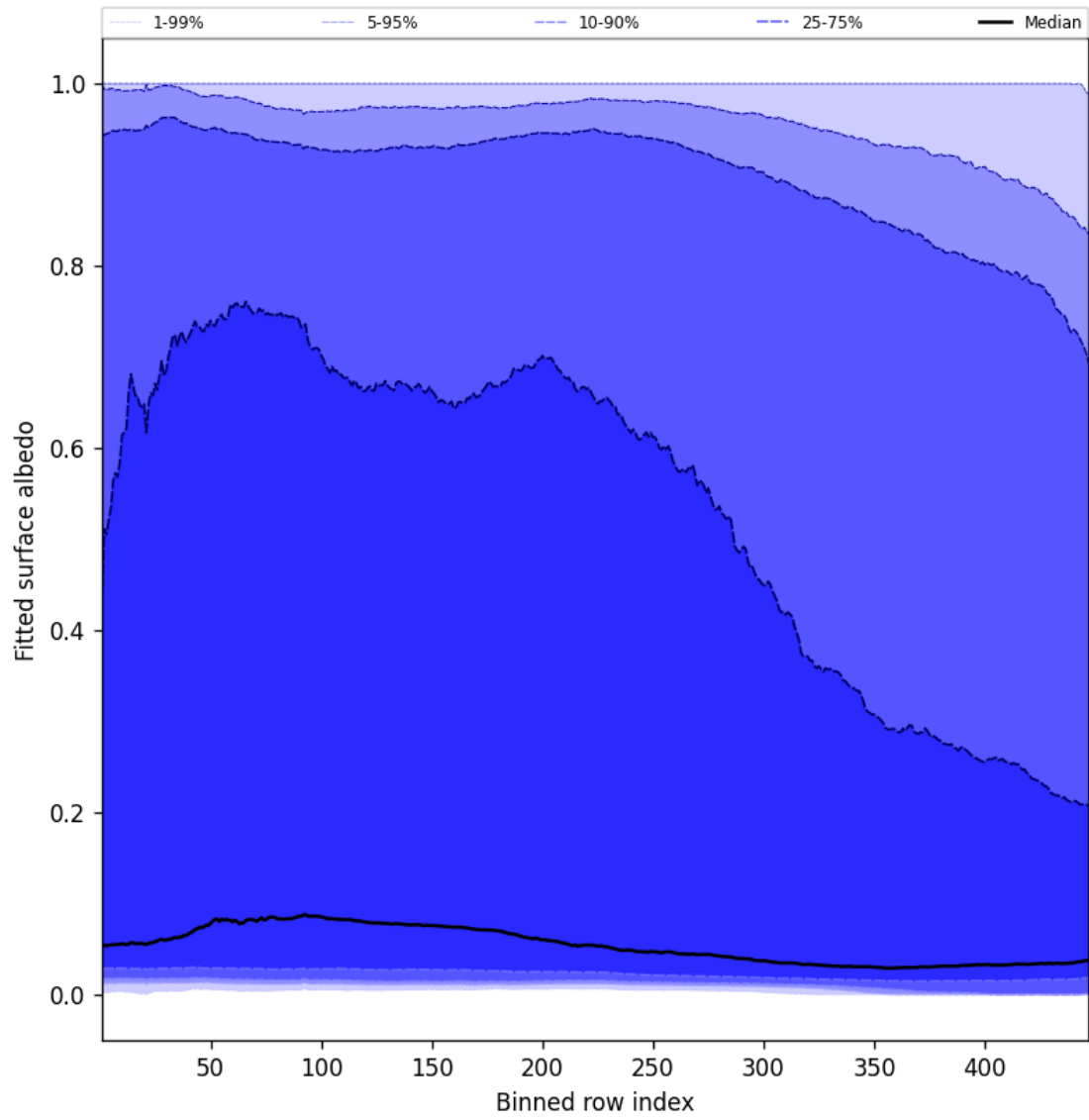
Figure 61: Along track statistics of “Fitted surface albedo” for 2024-11-02 to 2024-11-04
