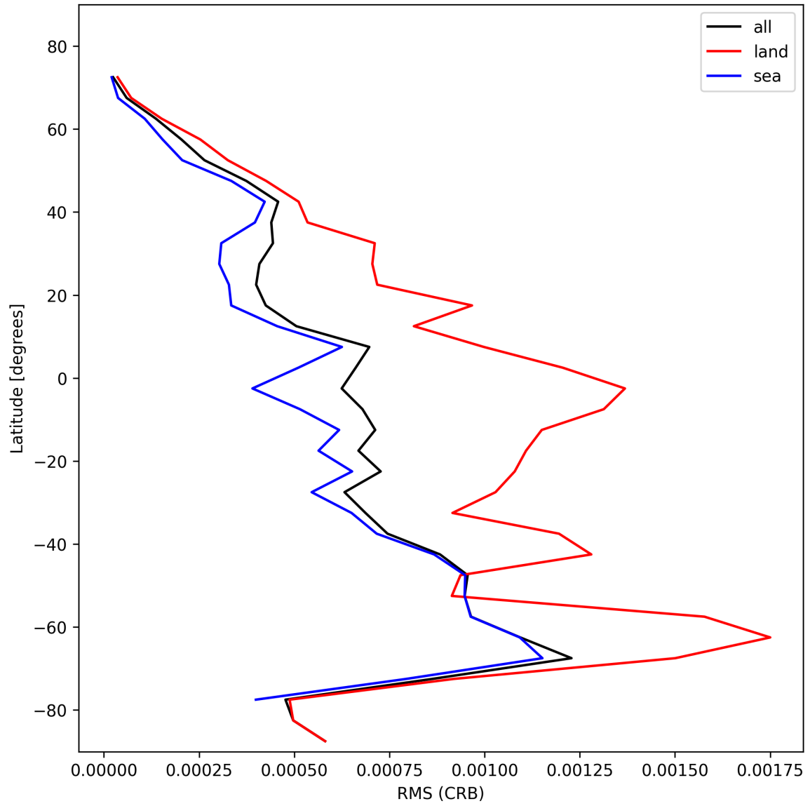
Figure 32: Zonal average of “RMS (CRB)” for 2024-11-02 to 2024-11-04.
