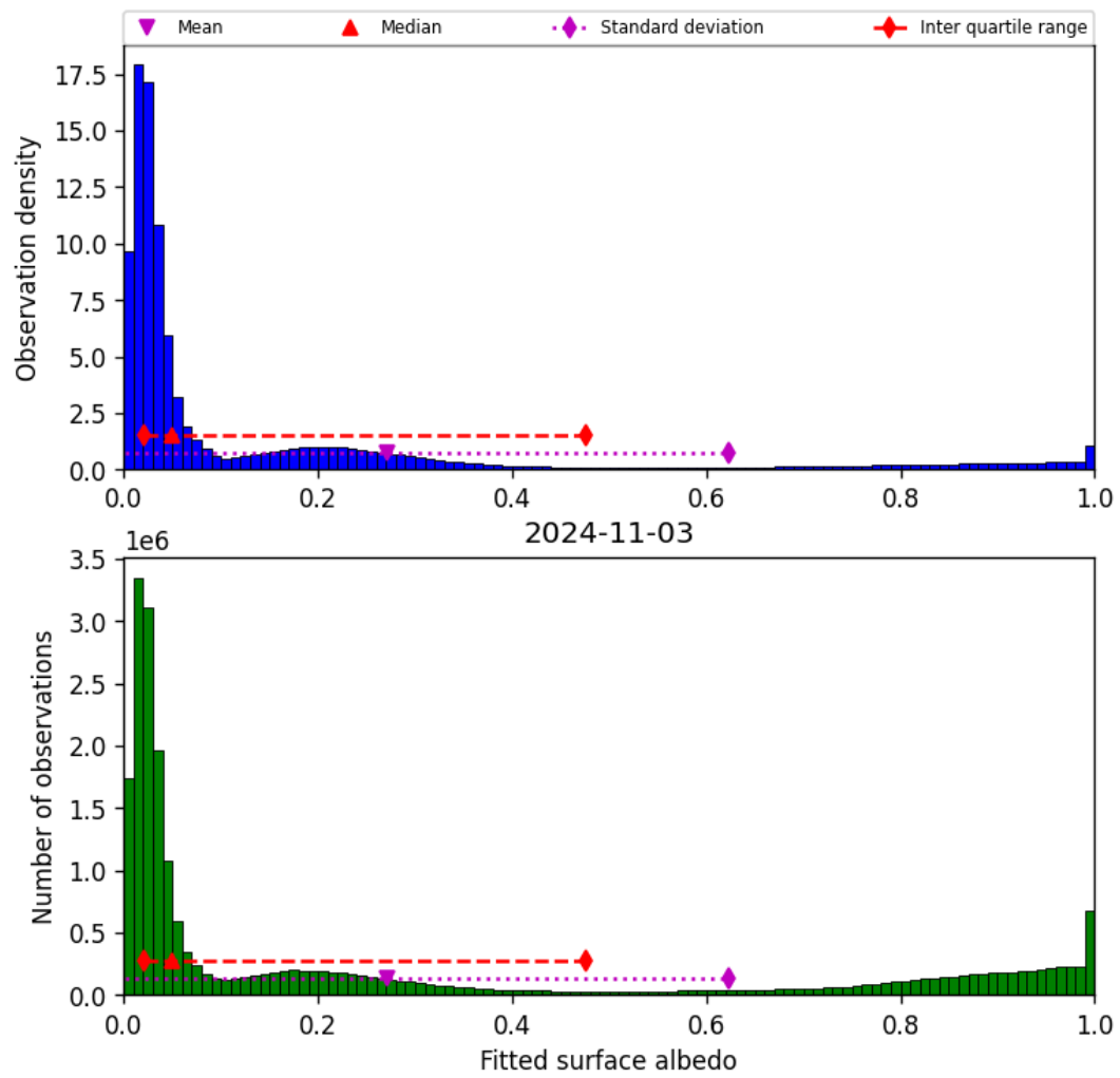
Figure 45: Histogram of “Fitted surface albedo” for 2024-11-02 to 2024-11-04
