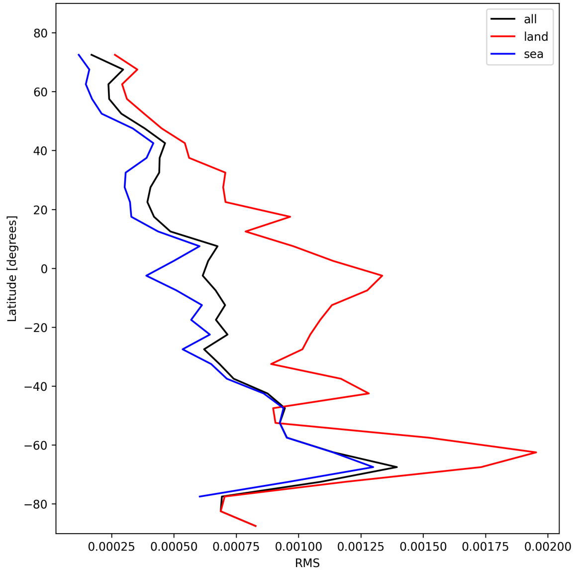
Figure 31: Zonal average of “RMS” for 2024-11-02 to 2024-11-04.
