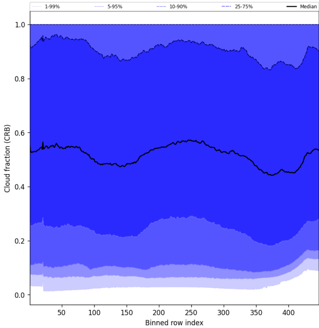
Figure 58: Along track statistics of “Cloud fraction (CRB)” for 2024-11-02 to 2024-11-04
