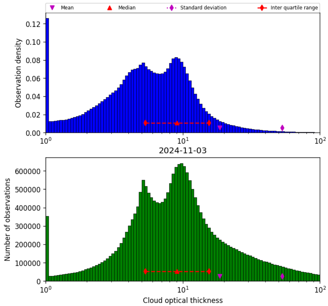
Figure 41: Histogram of “Cloud optical thickness” for 2024-11-02 to 2024-11-04
