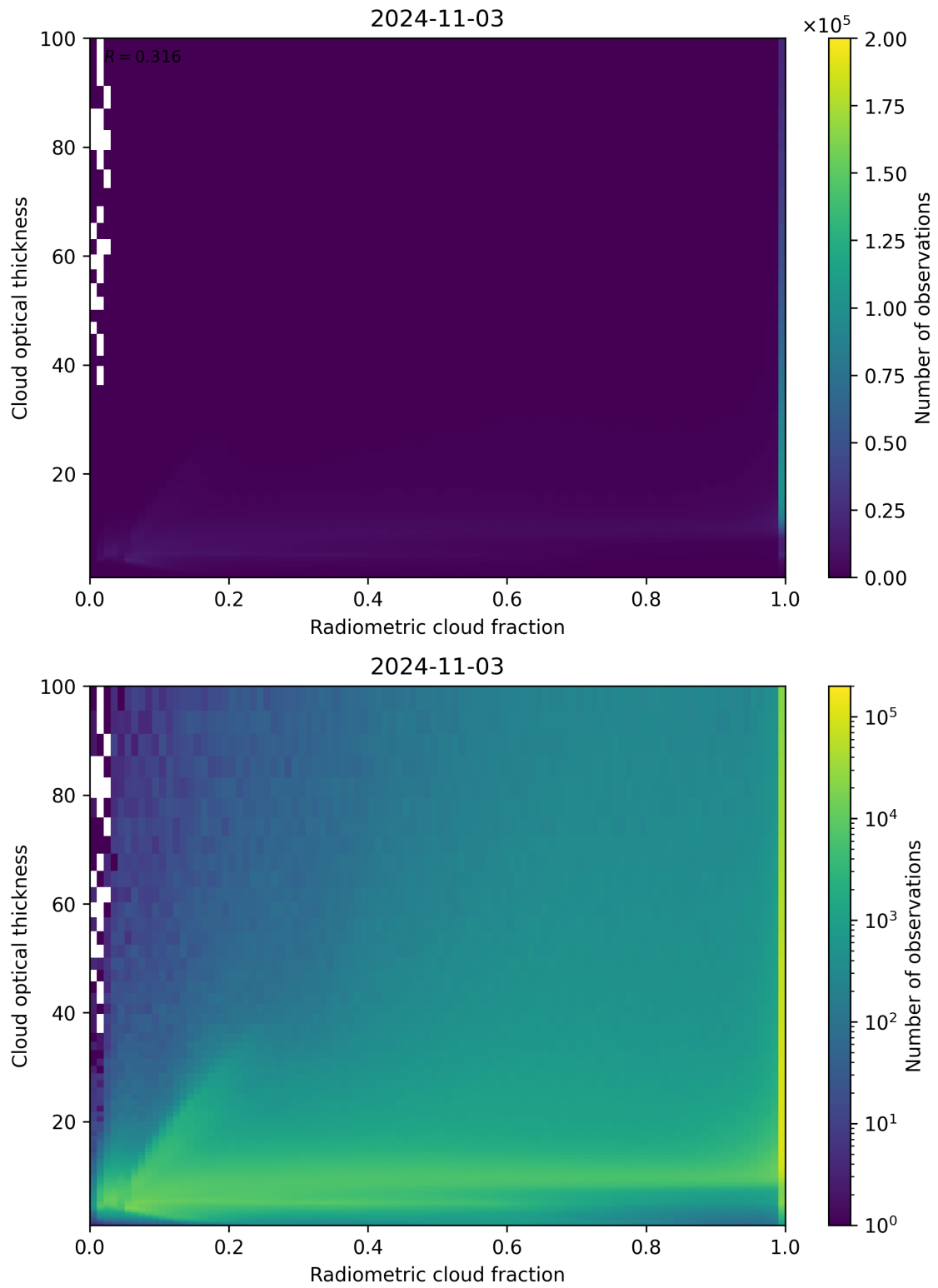
Figure 75: Scatter density plot of “Radiometric cloud fraction” against “Cloud optical thickness” for 2024-11-02 to 2024-11-04.
