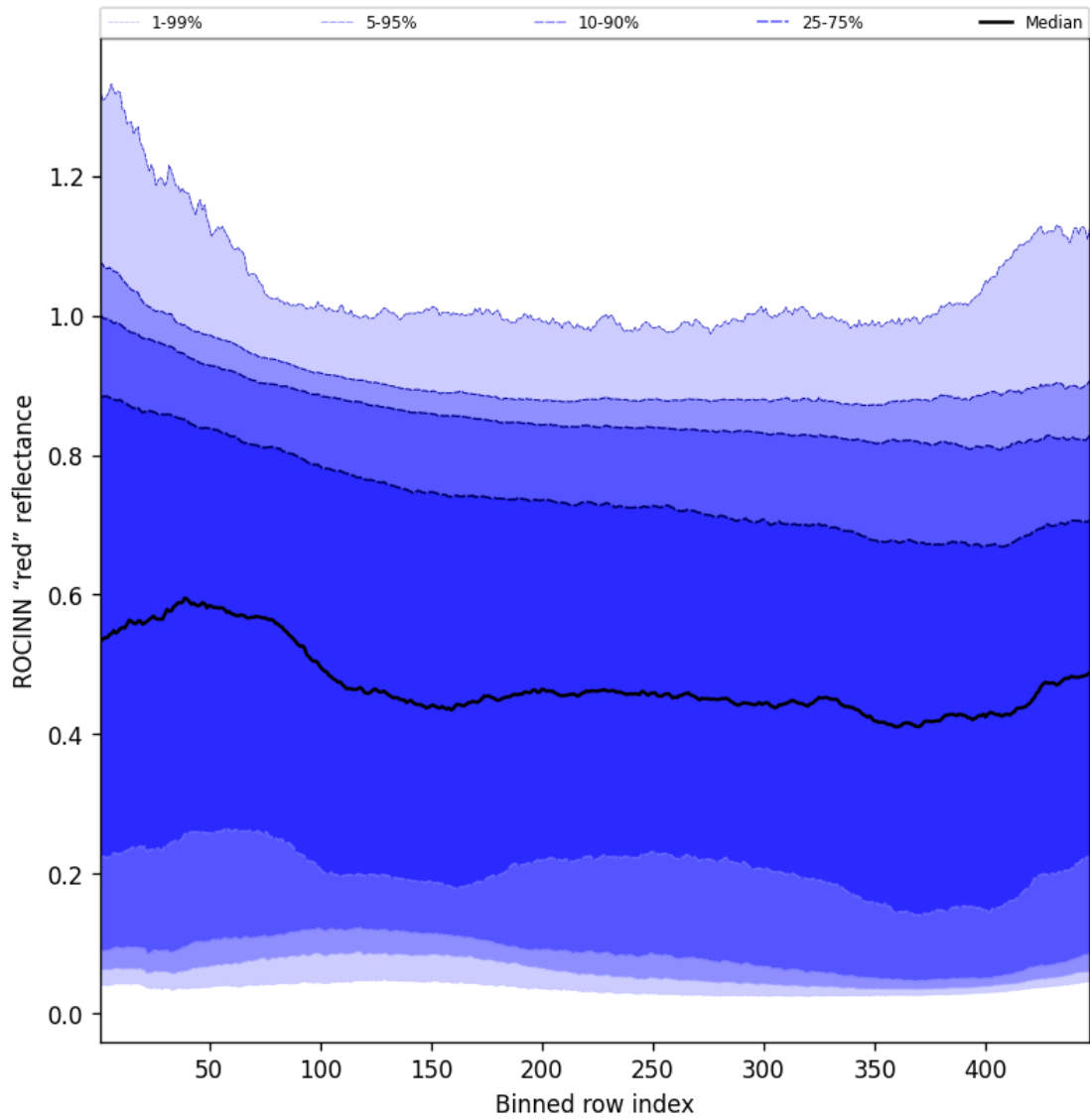
Figure 69: Along track statistics of “ROCINN “red” reflectance” for 2024-11-02 to 2024-11-04
