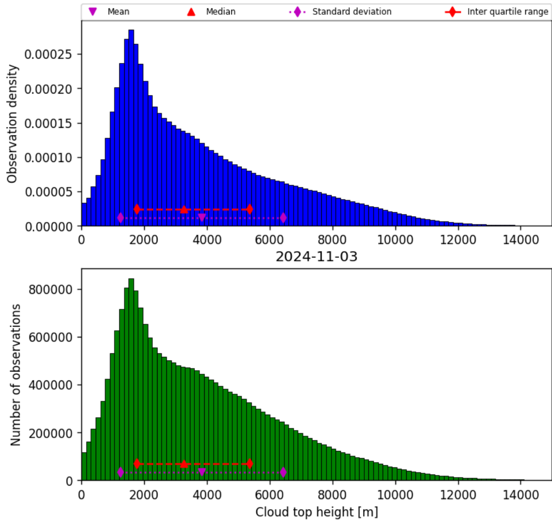
Figure 40: Histogram of “Cloud top height” for 2024-11-02 to 2024-11-04
