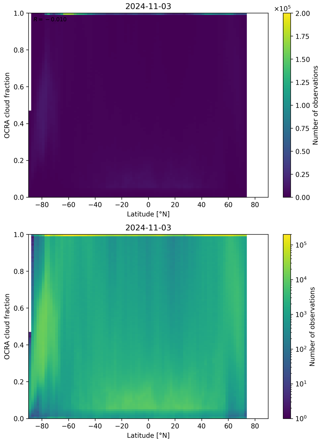
Figure 93: Scatter density plot of “Latitude” against “OCRA cloud fraction” for 2024-11-02 to 2024-11-04.
