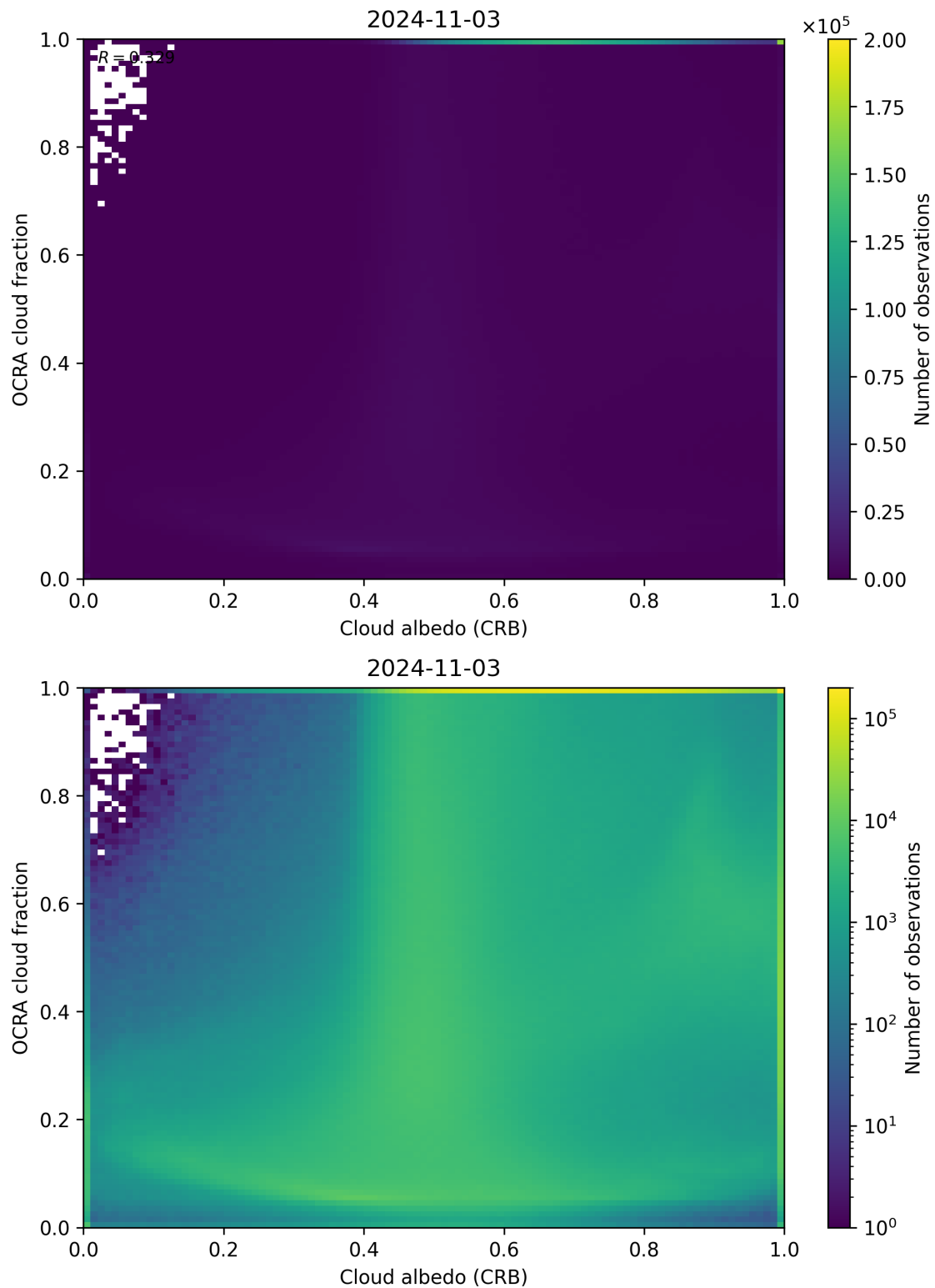
Figure 70: Scatter density plot of “Cloud albedo (CRB)” against “OCRA cloud fraction” for 2024-11-02 to 2024-11-04.
