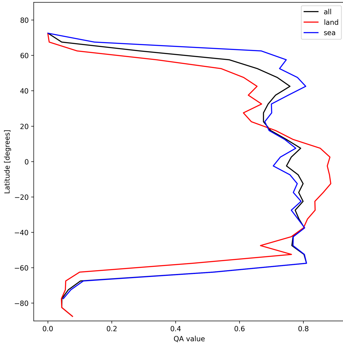
Figure 22: Zonal average of “QA value” for 2024-11-02 to 2024-11-04.
