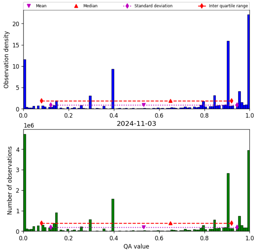
Figure 38: Histogram of “QA value” for 2024-11-02 to 2024-11-04
