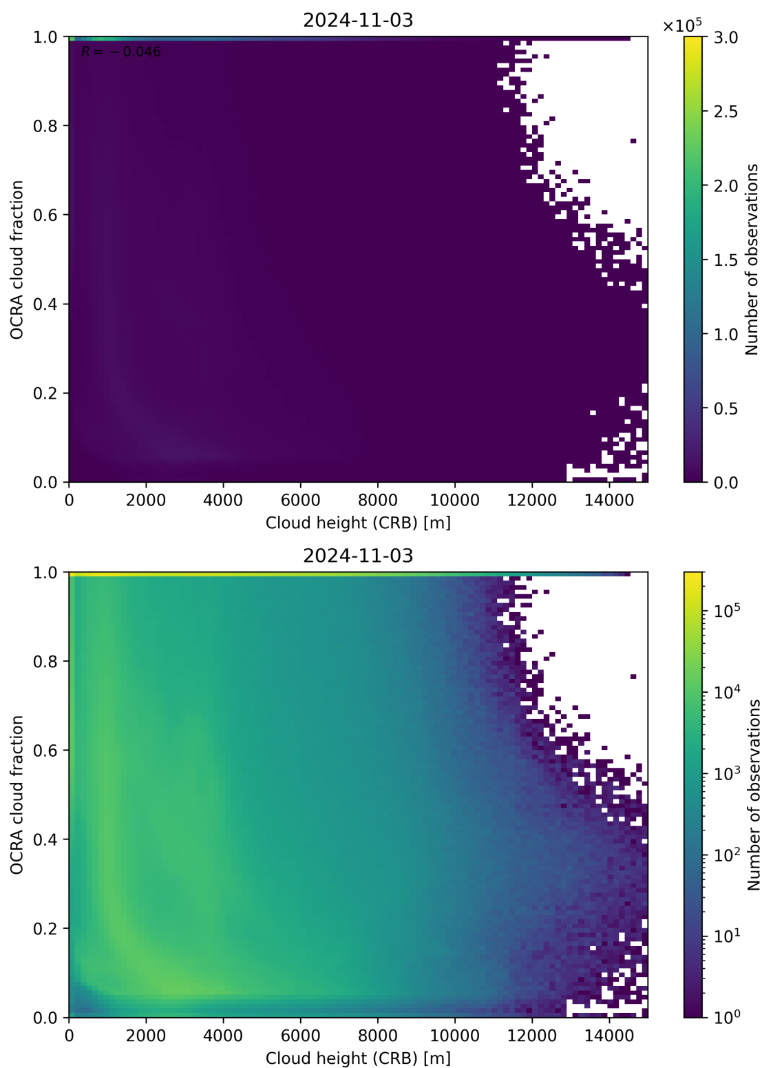
Figure 81: Scatter density plot of “Cloud height (CRB)” against “OCRA cloud fraction” for 2024-11-02 to 2024-11-04.
