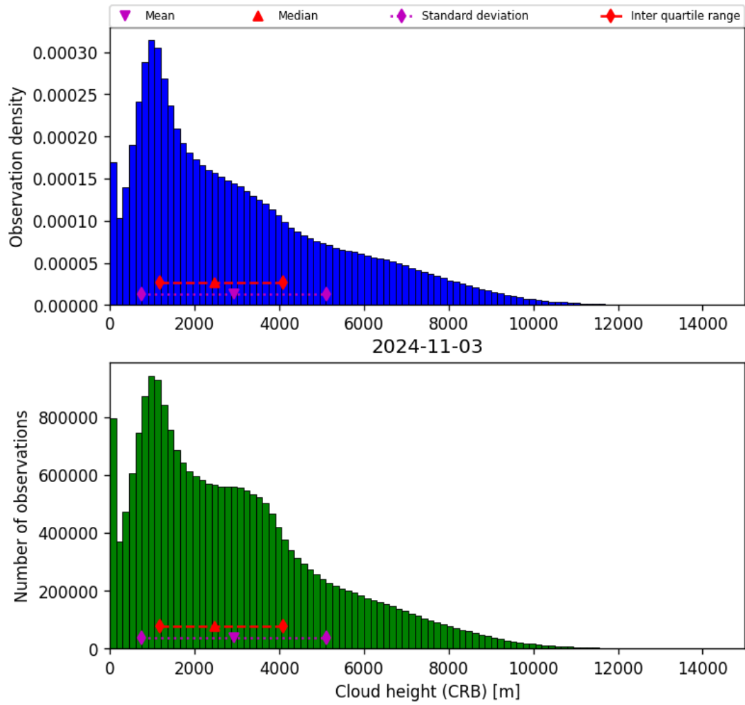
Figure 43: Histogram of “Cloud height (CRB)” for 2024-11-02 to 2024-11-04
