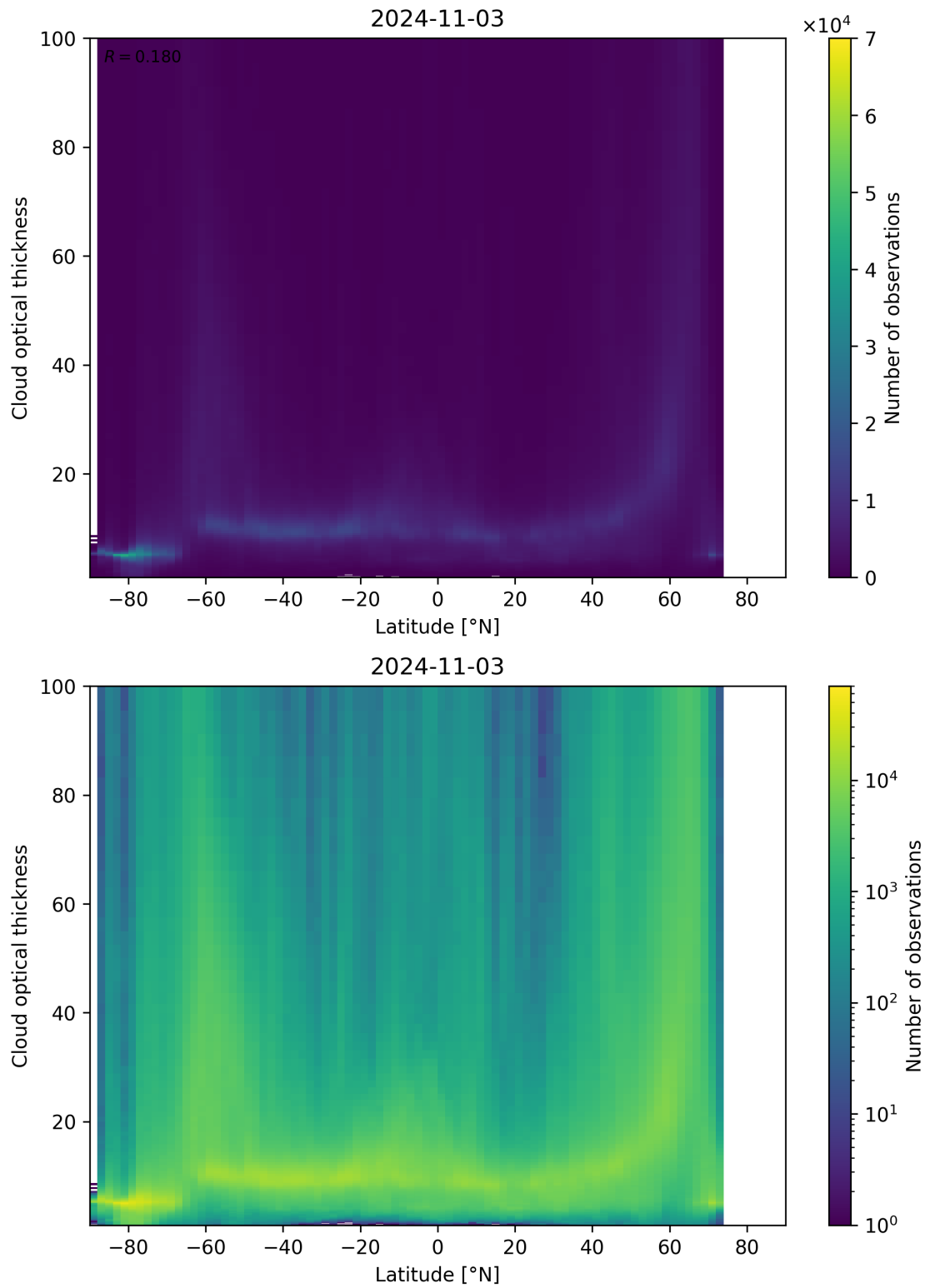
Figure 96: Scatter density plot of “Latitude” against “Cloud optical thickness” for 2024-11-02 to 2024-11-04.
