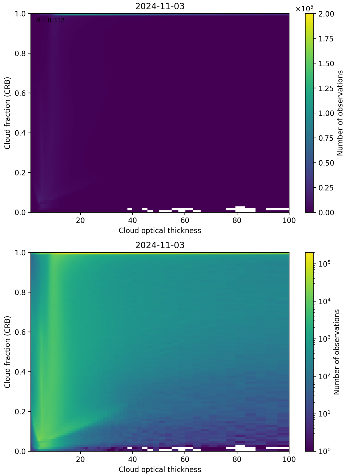
Figure 84: Scatter density plot of “Cloud optical thickness” against “Cloud fraction (CRB)” for 2024-11-02 to 2024-11-04.
