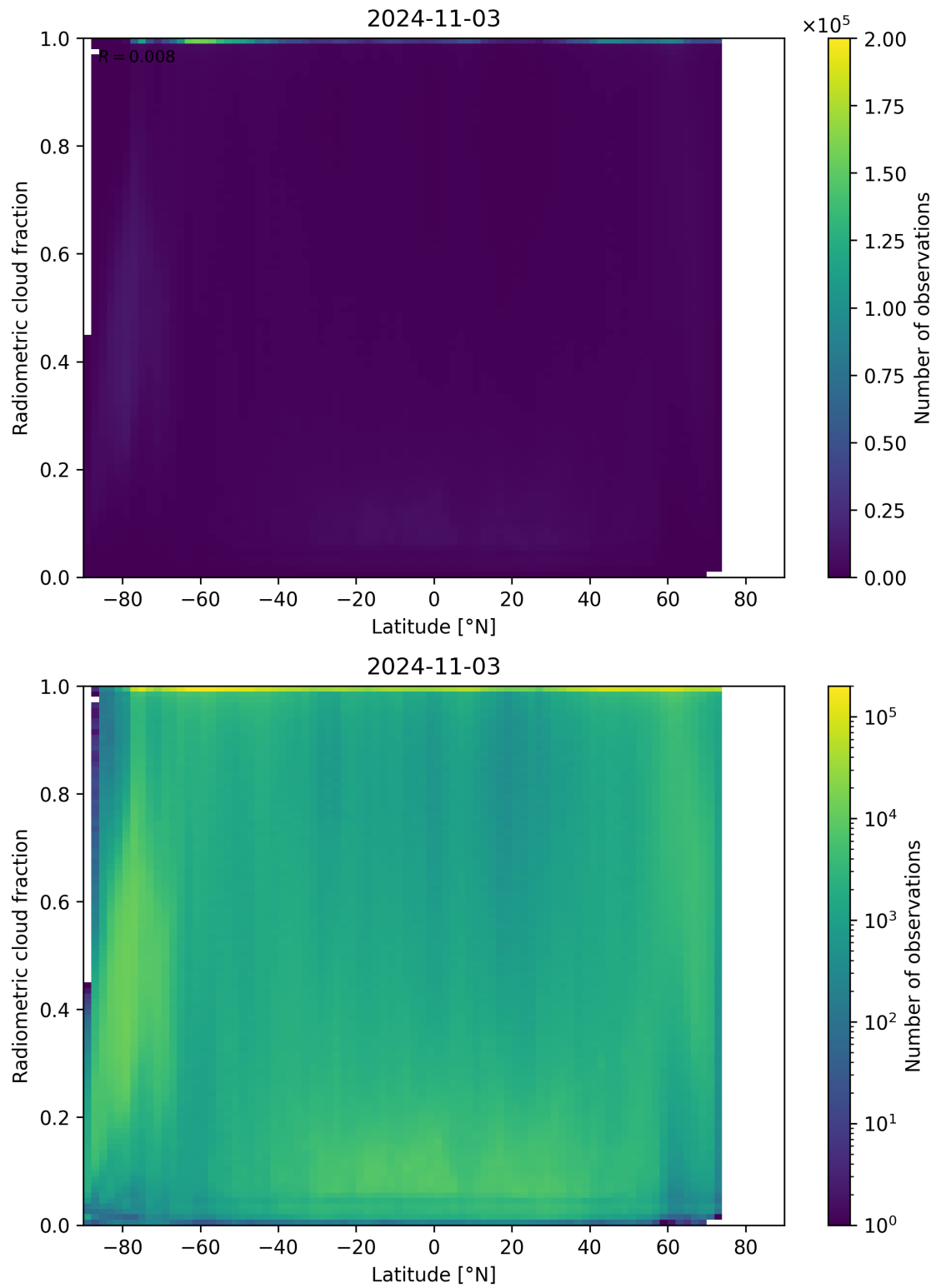
Figure 92: Scatter density plot of “Latitude” against “Radiometric cloud fraction” for 2024-11-02 to 2024-11-04.
