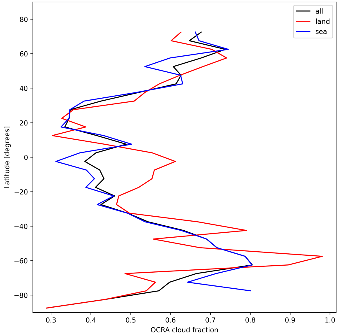
Figure 34: Zonal average of “OCRA cloud fraction” for 2024-11-02 to 2024-11-04.
