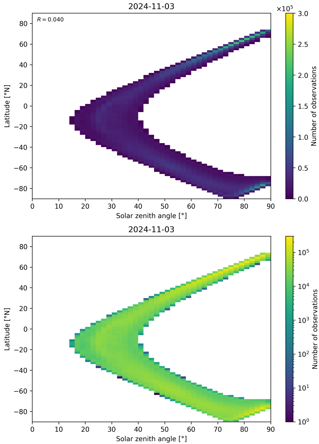
Figure 105: Scatter density plot of “Solar zenith angle” against “Latitude” for 2024-11-02 to 2024-11-04.
