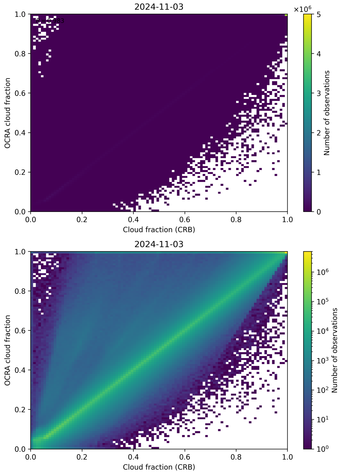
Figure 78: Scatter density plot of “Cloud fraction (CRB)” against “OCRA cloud fraction” for 2024-11-02 to 2024-11-04.
