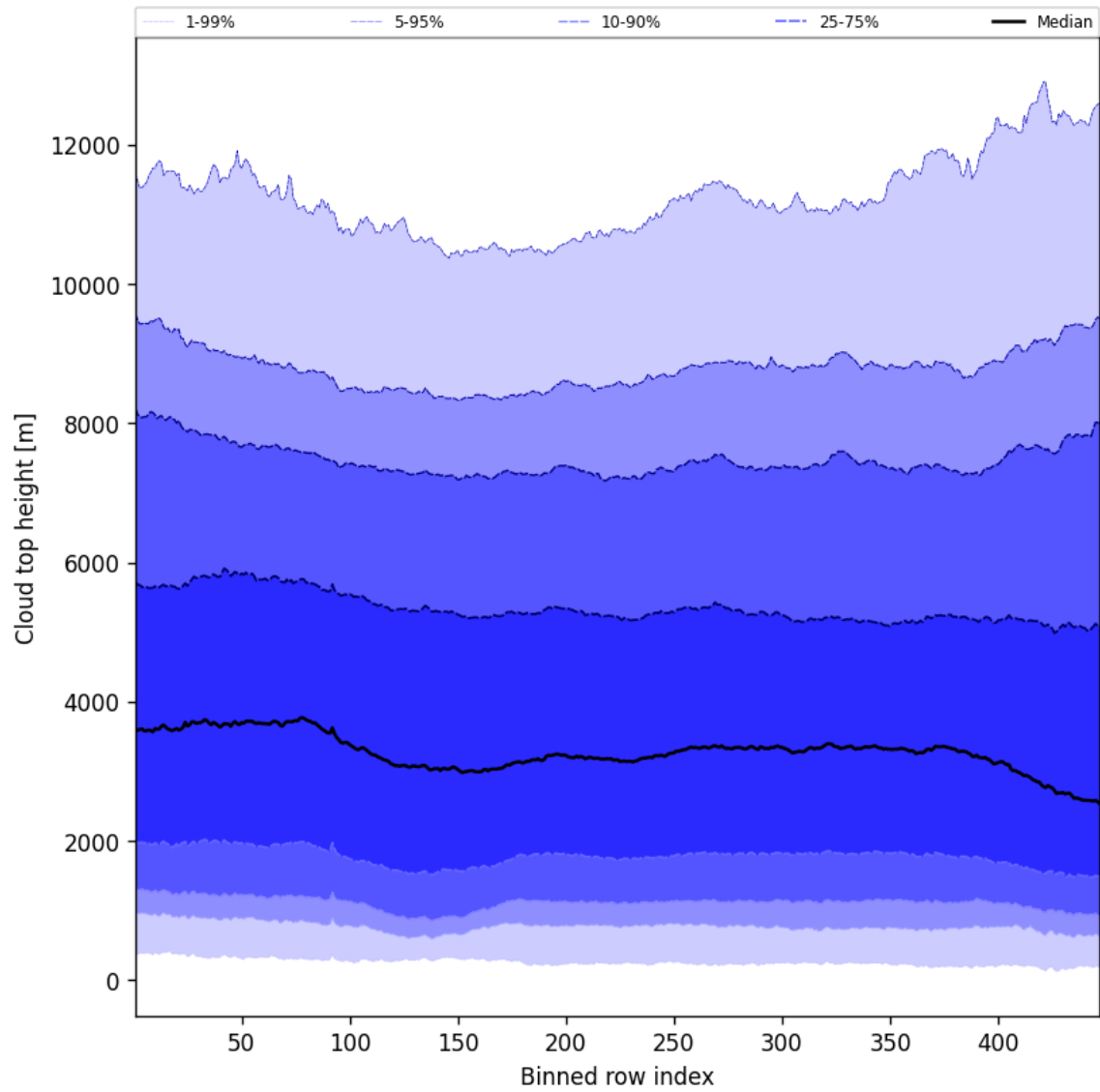
Figure 56: Along track statistics of “Cloud top height” for 2024-11-02 to 2024-11-04
