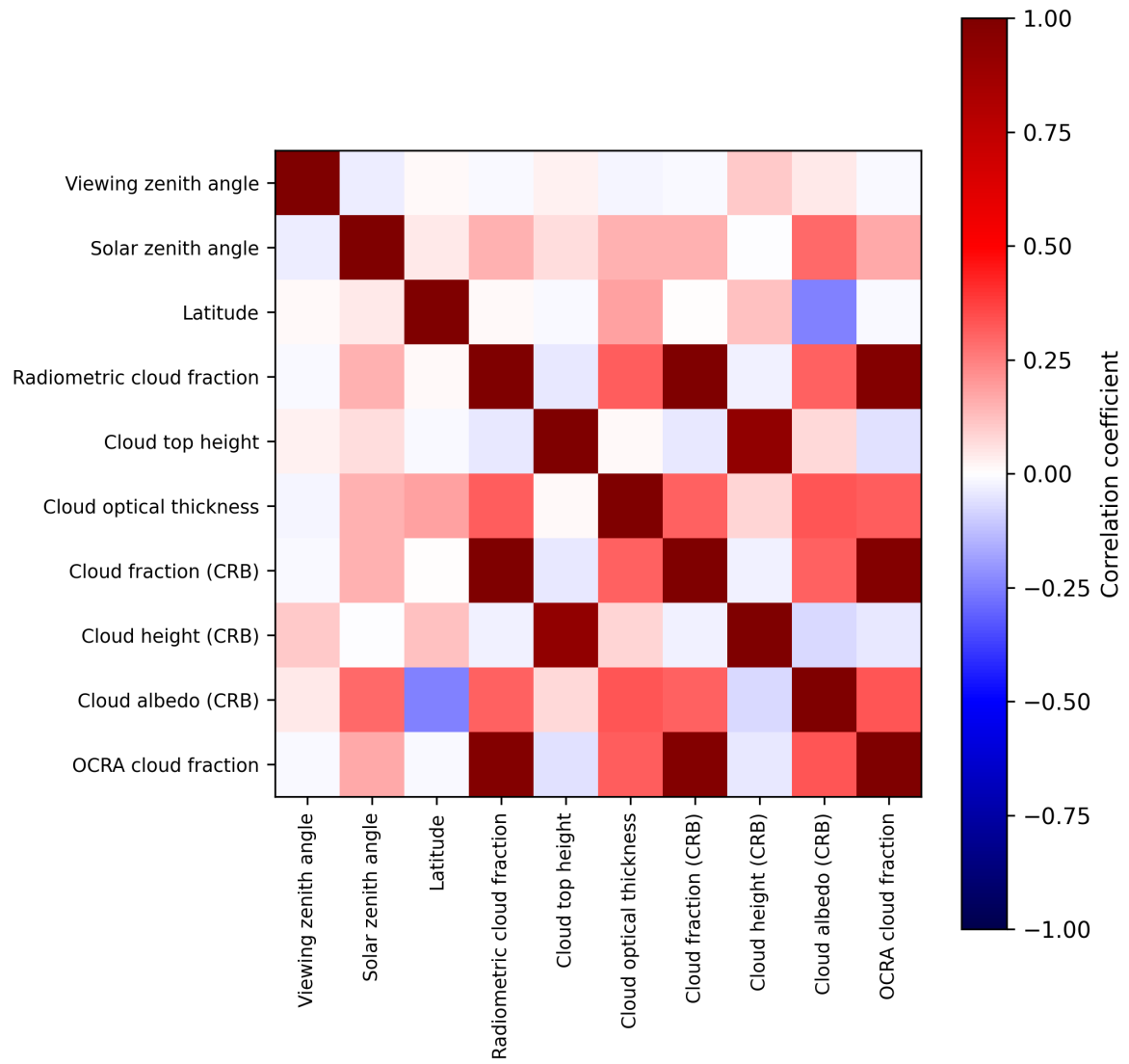
Figure 2: Map of correlation matrix for 2024-11-02 to 2024-11-04.
