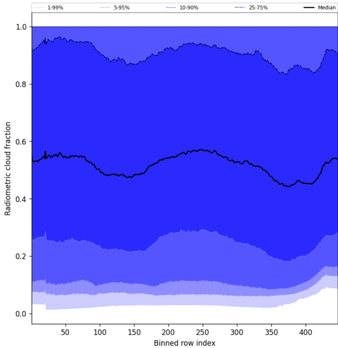
Figure 55: Along track statistics of “Radiometric cloud fraction” for 2024-11-02 to 2024-11-04
