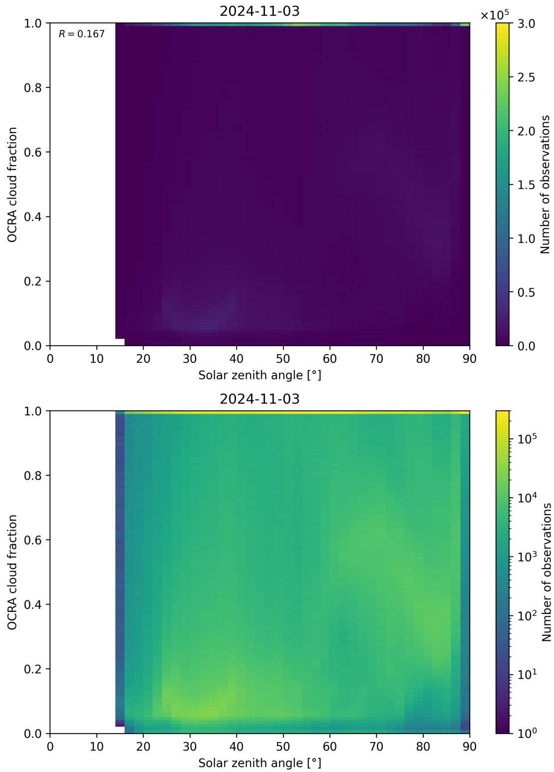
Figure 100: Scatter density plot of “Solar zenith angle” against “OCRA cloud fraction” for 2024-11-02 to 2024-11-04.
