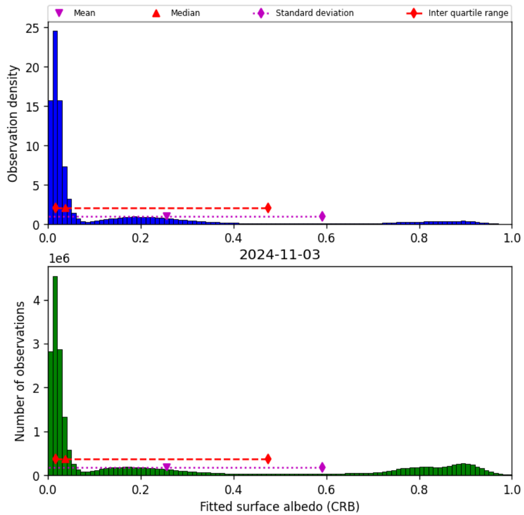
Figure 46: Histogram of “Fitted surface albedo (CRB)” for 2024-11-02 to 2024-11-04
