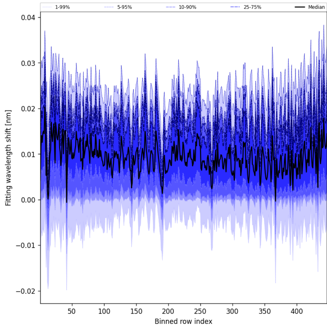
Figure 65: Along track statistics of “Fitting wavelength shift” for 2024-11-02 to 2024-11-04
