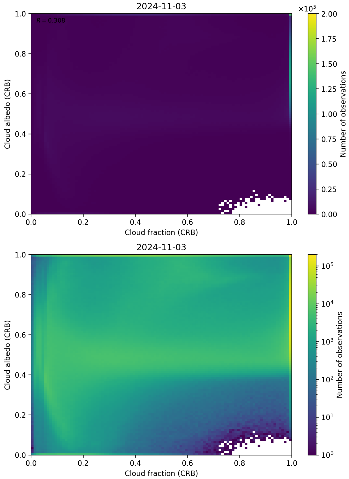
Figure 77: Scatter density plot of “Cloud fraction (CRB)” against “Cloud albedo (CRB)” for 2024-11-02 to 2024-11-04.
