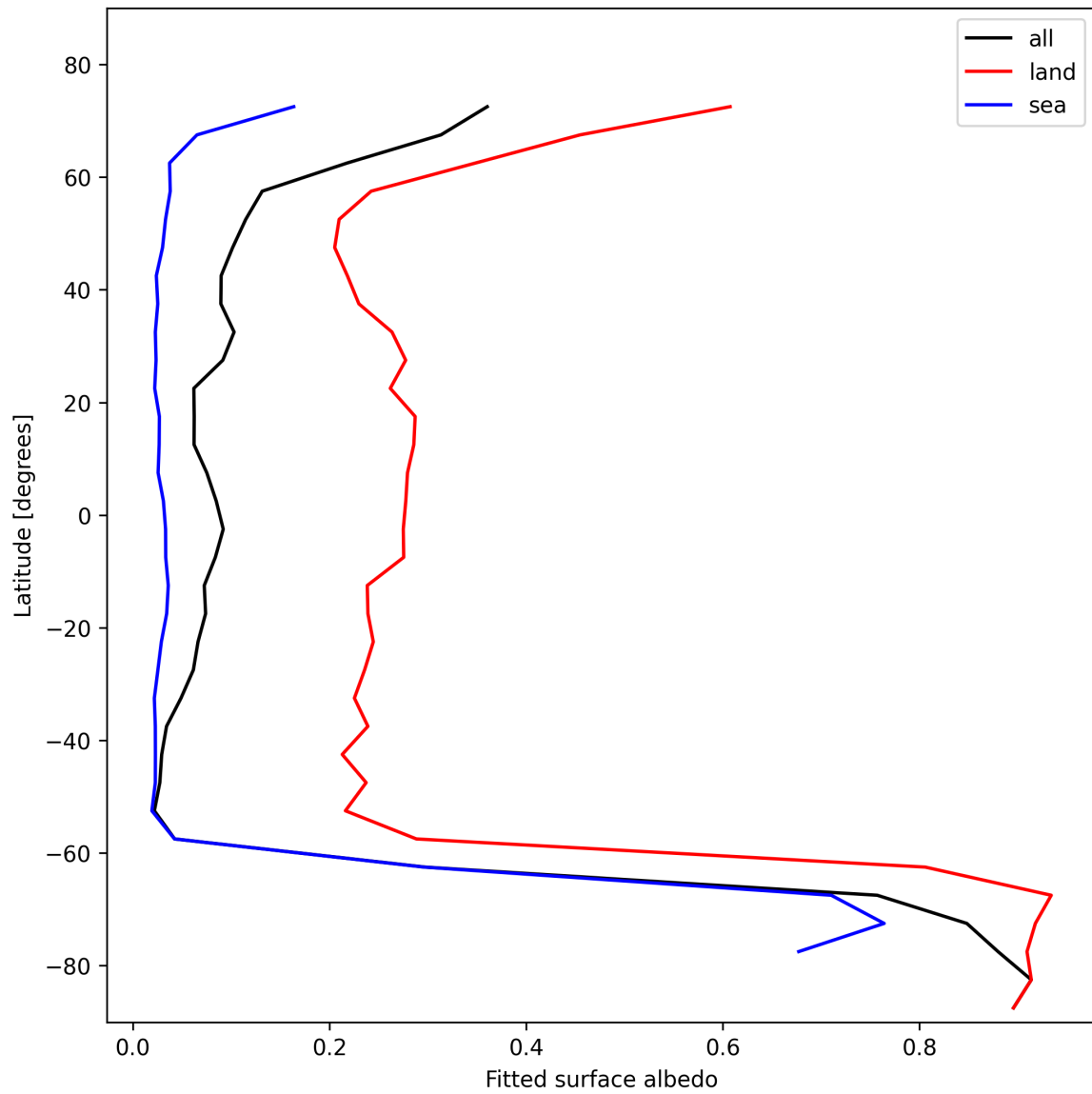
Figure 29: Zonal average of “Fitted surface albedo” for 2024-11-02 to 2024-11-04.
