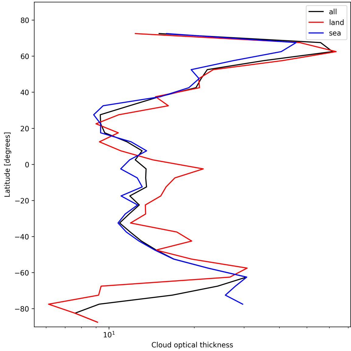
Figure 25: Zonal average of “Cloud optical thickness” for 2024-11-02 to 2024-11-04.
