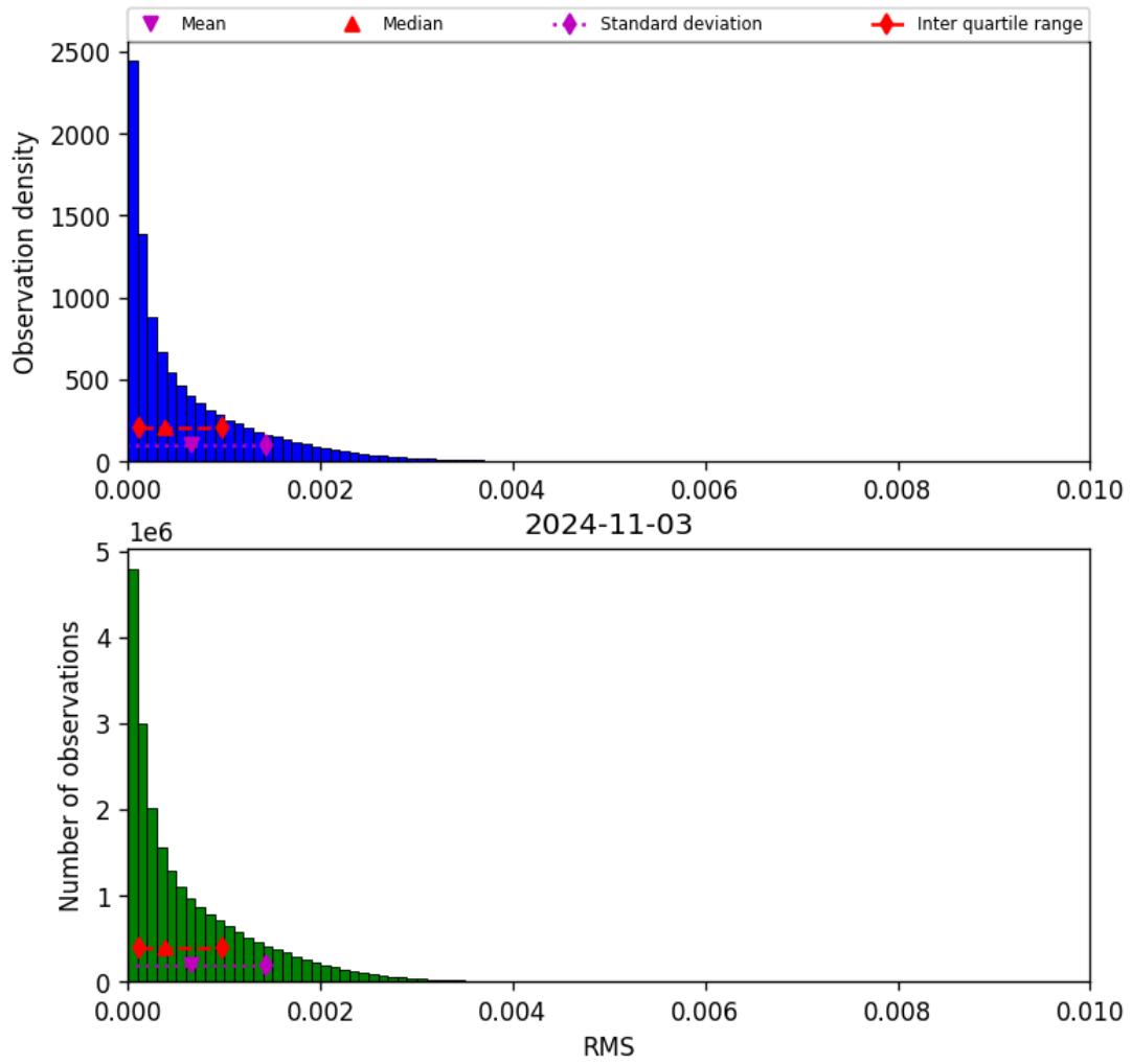
Figure 47: Histogram of “RMS” for 2024-11-02 to 2024-11-04
