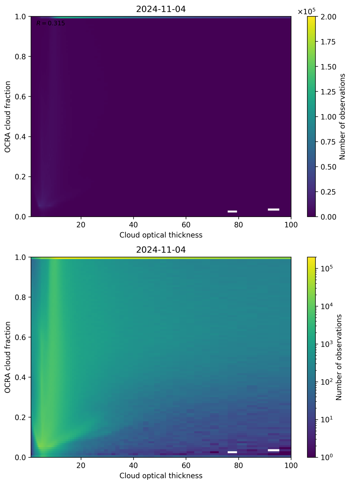
Figure 83: Scatter density plot of “Cloud optical thickness” against “OCRA cloud fraction” for 2024-11-04 to 2024-11-05.
