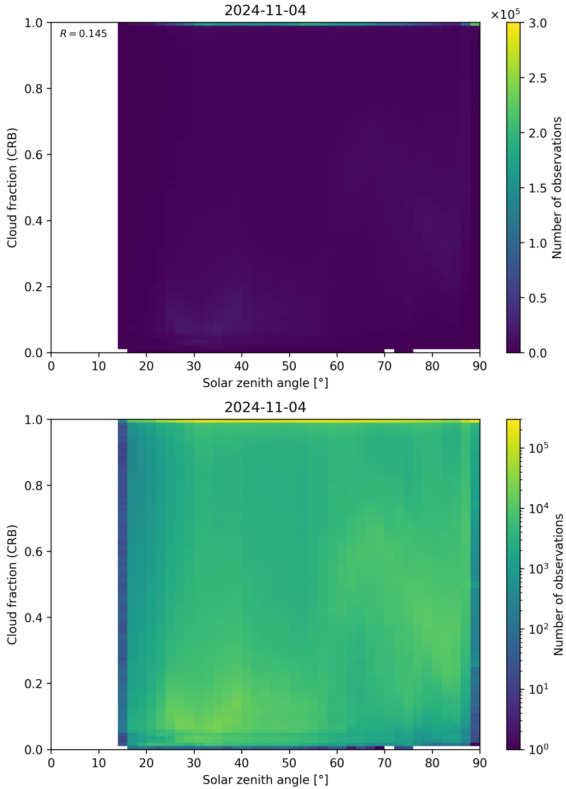
Figure 101: Scatter density plot of “Solar zenith angle” against “Cloud fraction (CRB)” for 2024-11-04 to 2024-11-05.
