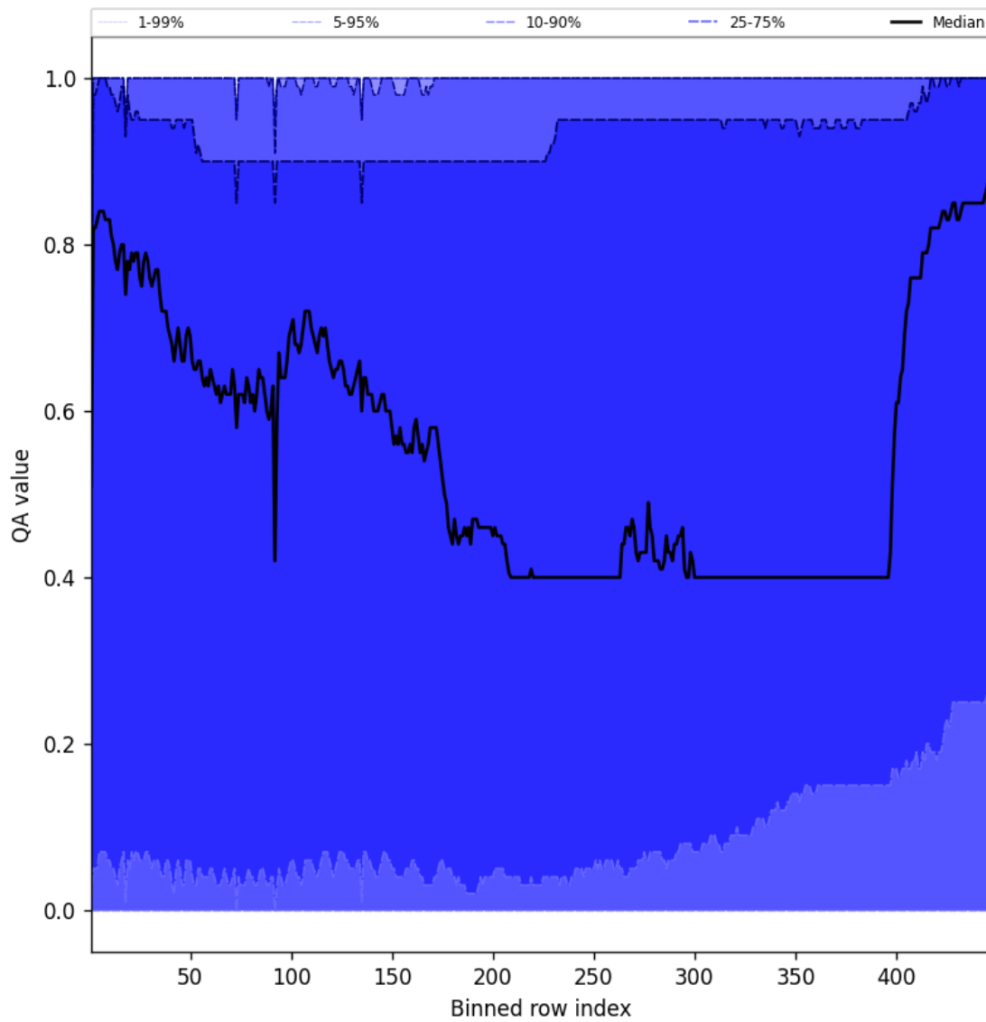
Figure 54: Along track statistics of “QA value” for 2024-11-04 to 2024-11-05
