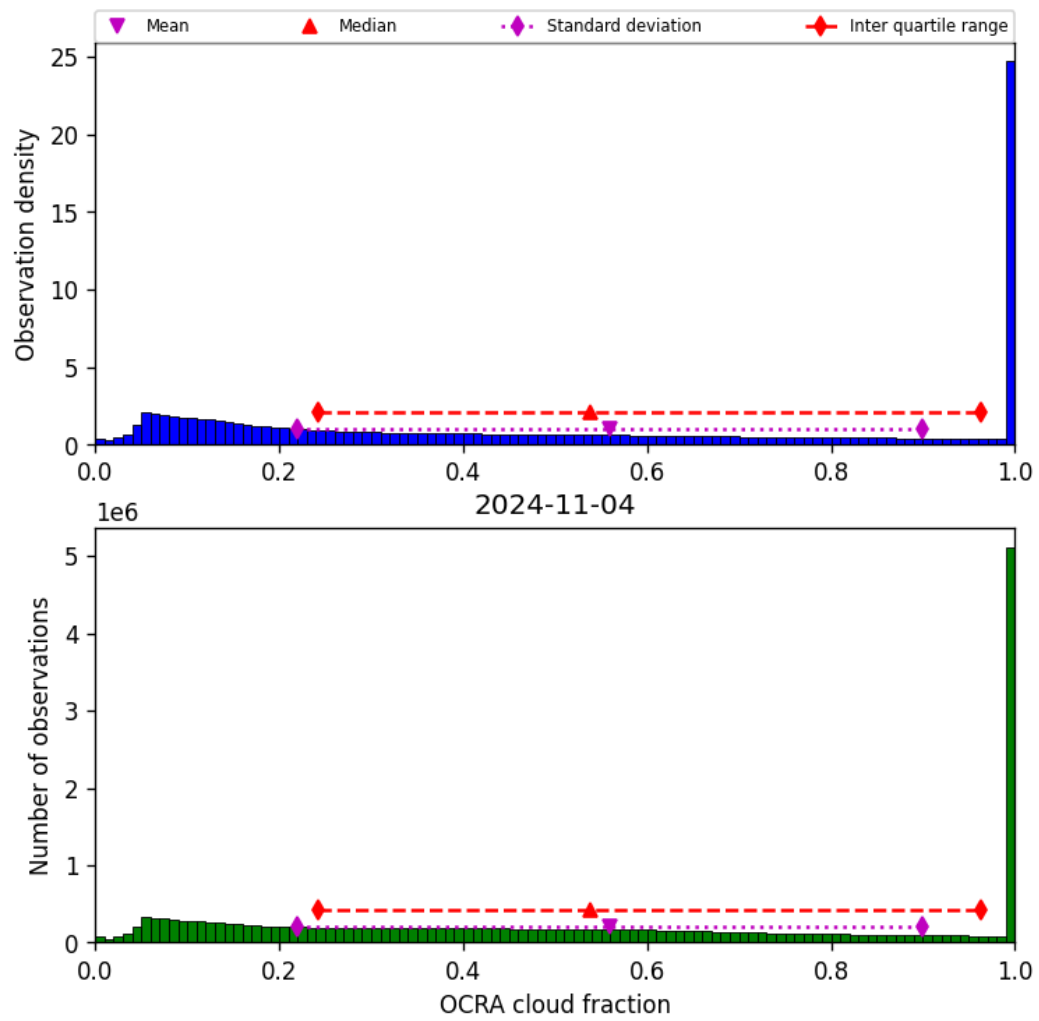
Figure 50: Histogram of “OCRA cloud fraction” for 2024-11-04 to 2024-11-05
