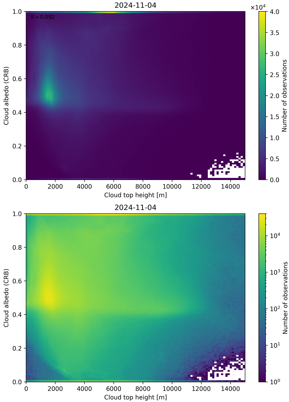
Figure 86: Scatter density plot of “Cloud top height” against “Cloud albedo (CRB)” for 2024-11-04 to 2024-11-05.
