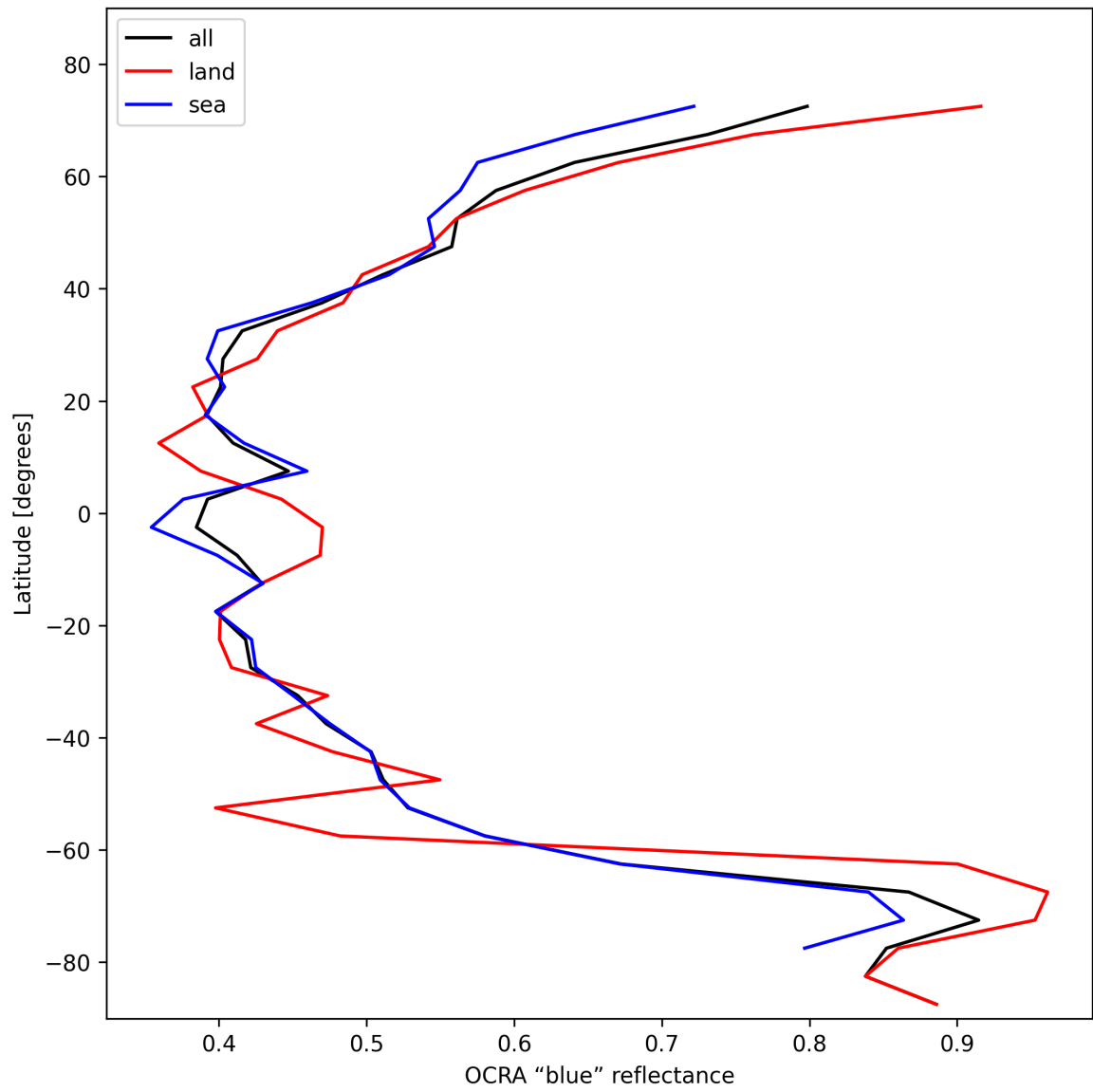
Figure 35: Zonal average of “OCRA “blue” reflectance” for 2024-11-04 to 2024-11-05.
