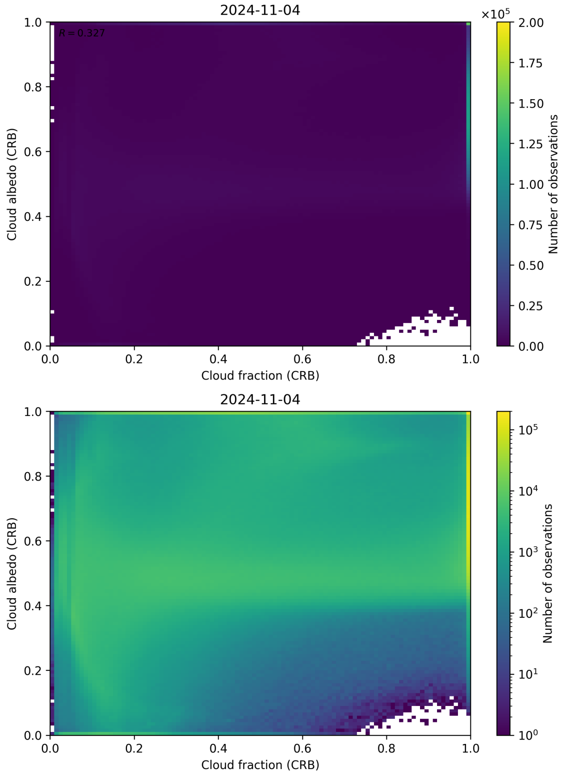
Figure 77: Scatter density plot of “Cloud fraction (CRB)” against “Cloud albedo (CRB)” for 2024-11-04 to 2024-11-05.
