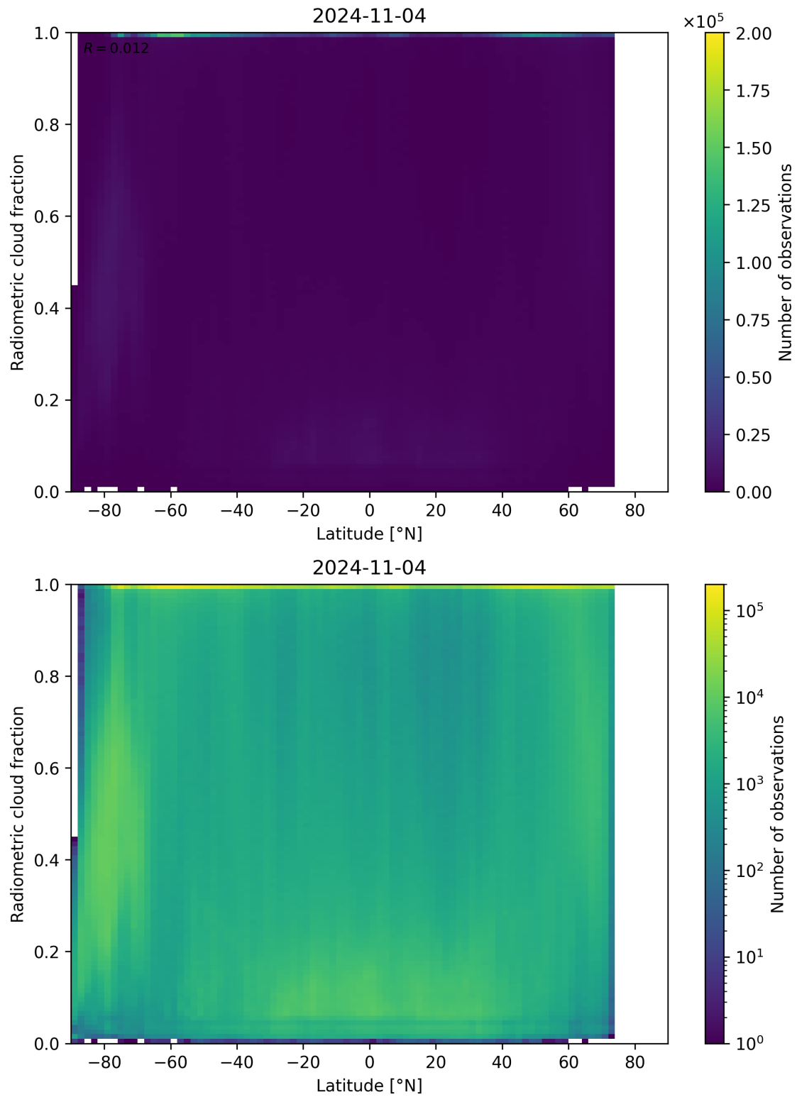
Figure 92: Scatter density plot of “Latitude” against “Radiometric cloud fraction” for 2024-11-04 to 2024-11-05.
