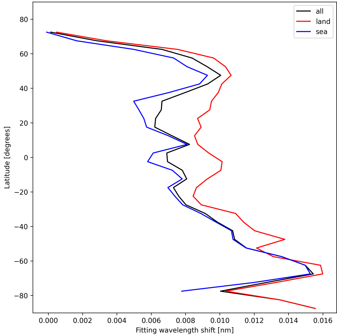
Figure 33: Zonal average of “Fitting wavelength shift” for 2024-11-04 to 2024-11-05.
