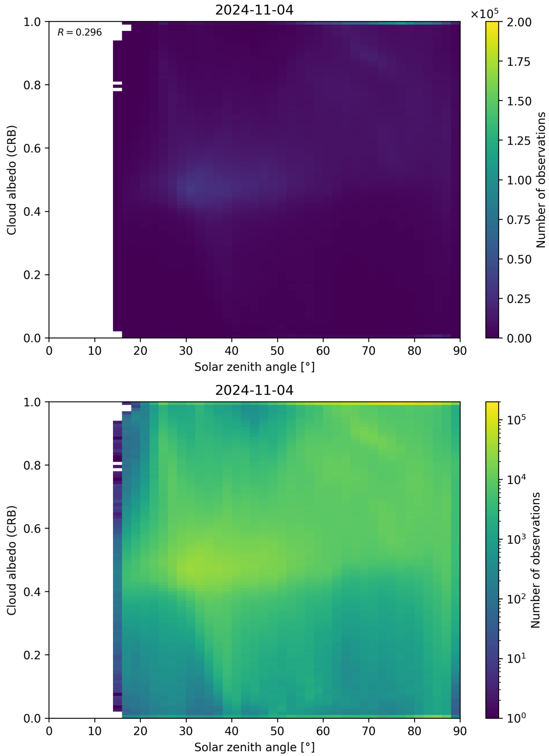
Figure 98: Scatter density plot of “Solar zenith angle” against “Cloud albedo (CRB)” for 2024-11-04 to 2024-11-05.
