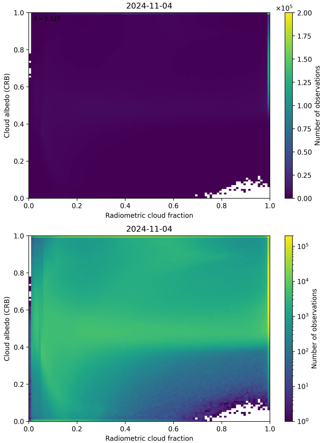
Figure 71: Scatter density plot of “Radiometric cloud fraction” against “Cloud albedo (CRB)” for 2024-11-04 to 2024-11-05.
