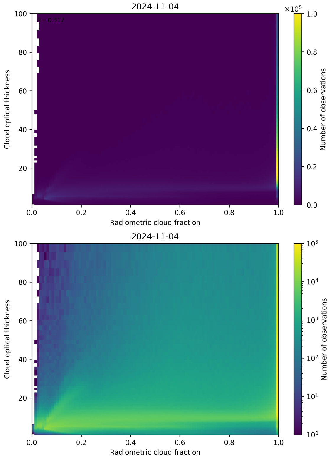
Figure 75: Scatter density plot of “Radiometric cloud fraction” against “Cloud optical thickness” for 2024-11-04 to 2024-11-05.
