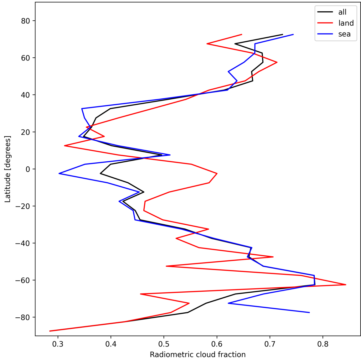
Figure 23: Zonal average of “Radiometric cloud fraction” for 2024-11-04 to 2024-11-05.
