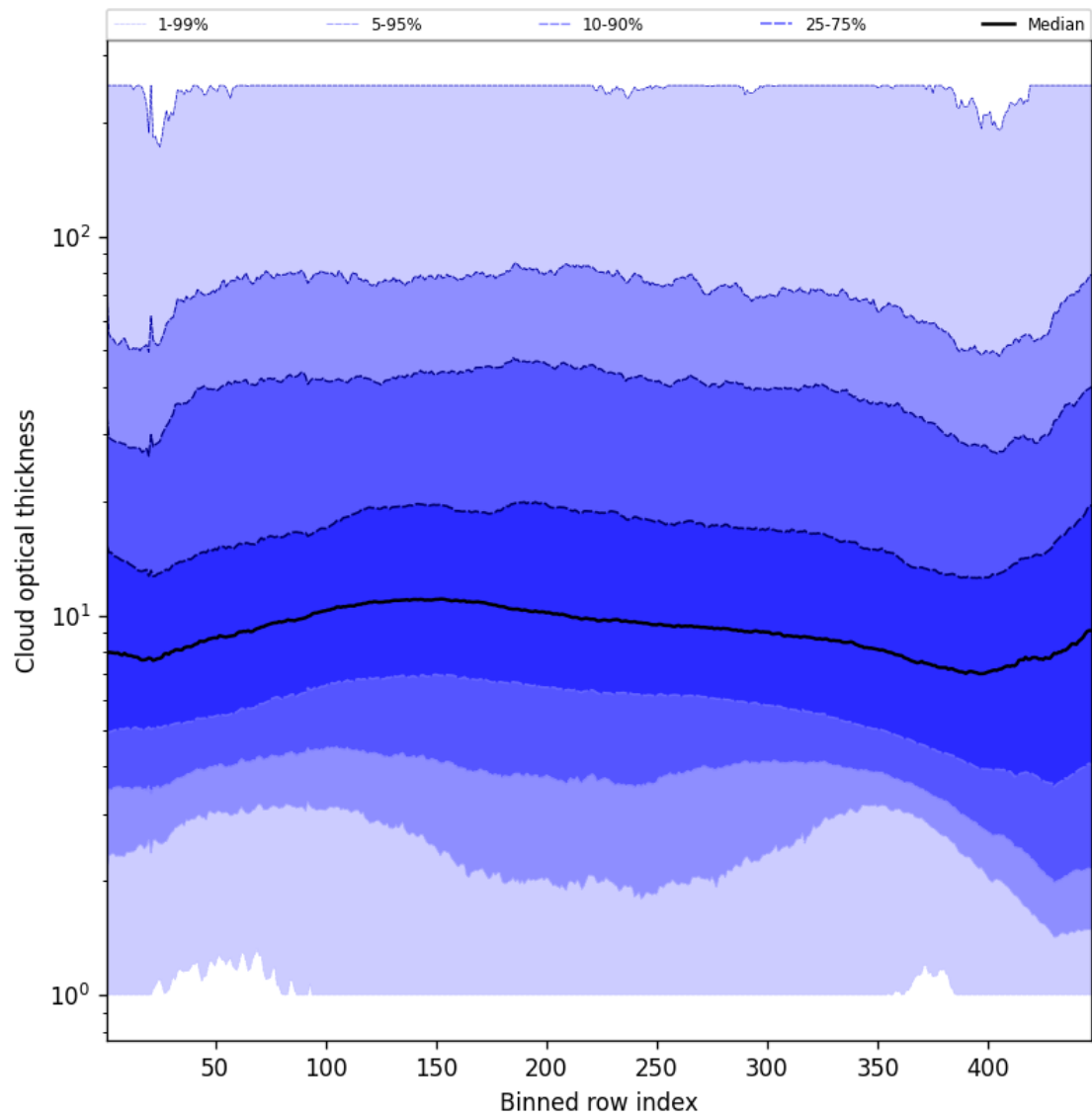
Figure 57: Along track statistics of “Cloud optical thickness” for 2024-11-04 to 2024-11-05
