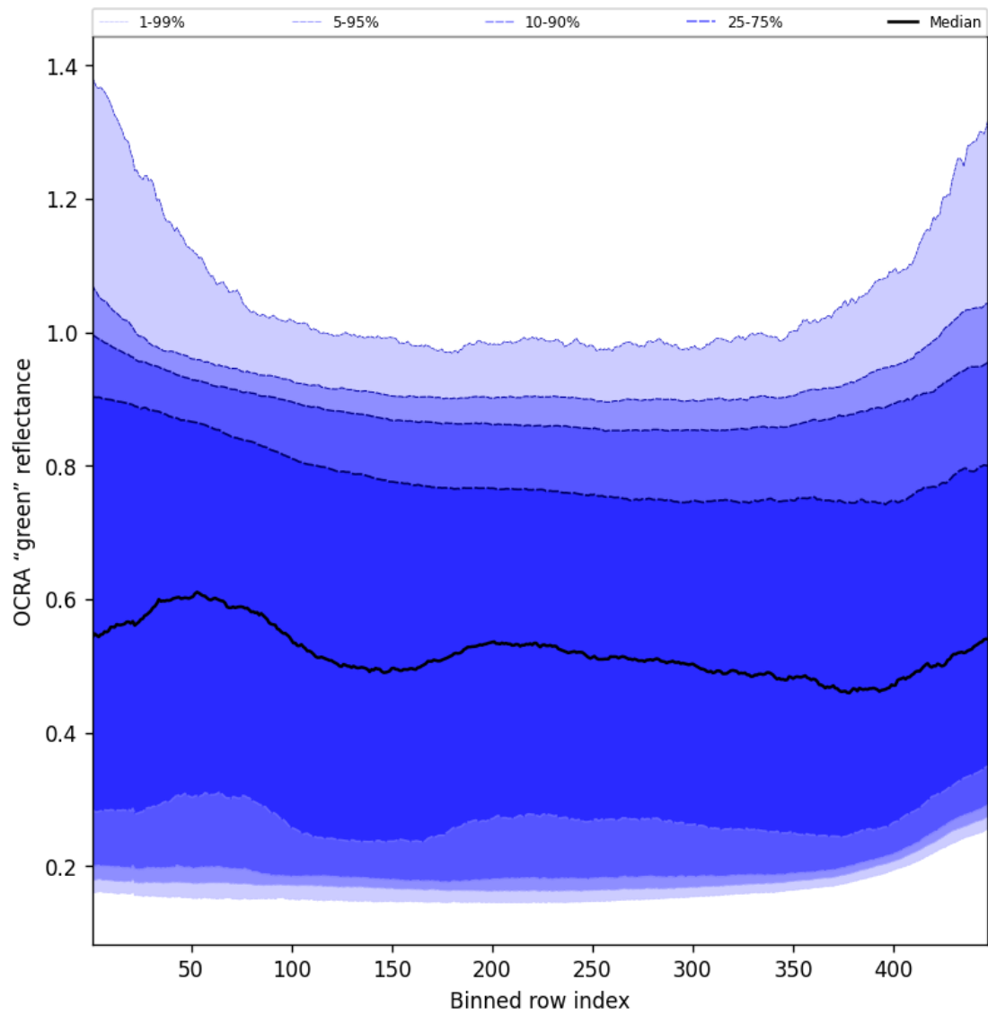
Figure 68: Along track statistics of “OCRA “green” reflectance” for 2024-11-04 to 2024-11-05
