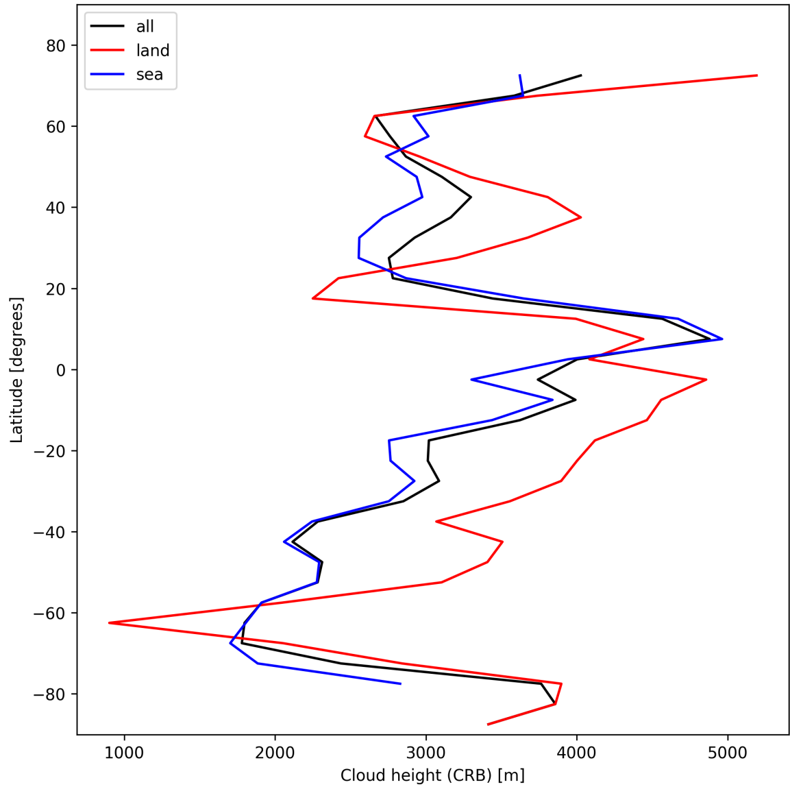
Figure 27: Zonal average of “Cloud height (CRB)” for 2024-11-04 to 2024-11-05.
