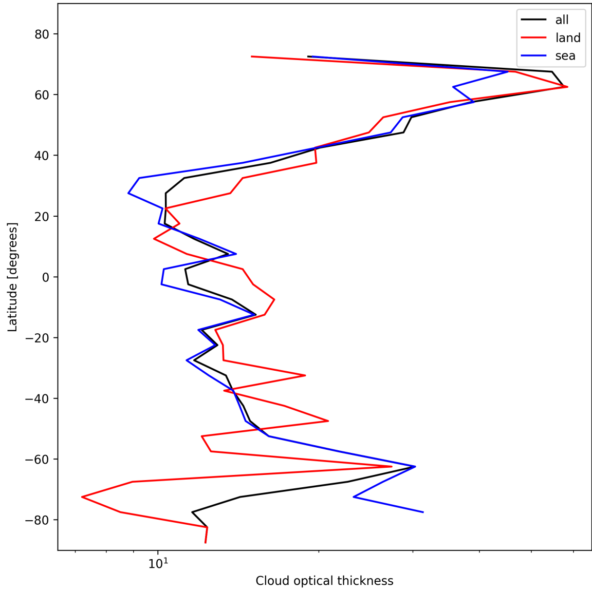
Figure 25: Zonal average of “Cloud optical thickness” for 2024-11-04 to 2024-11-05.
