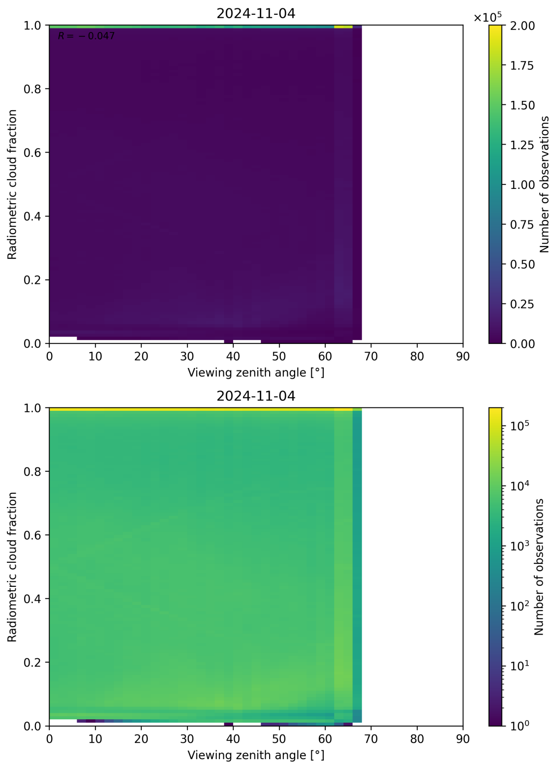
Figure 107: Scatter density plot of “Viewing zenith angle” against “Radiometric cloud fraction” for 2024-11-04 to 2024-11-05.
