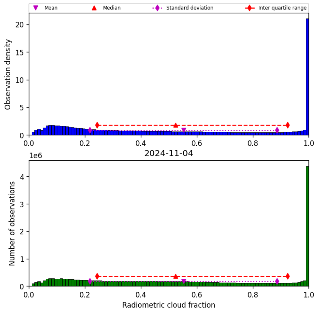
Figure 39: Histogram of “Radiometric cloud fraction” for 2024-11-04 to 2024-11-05
