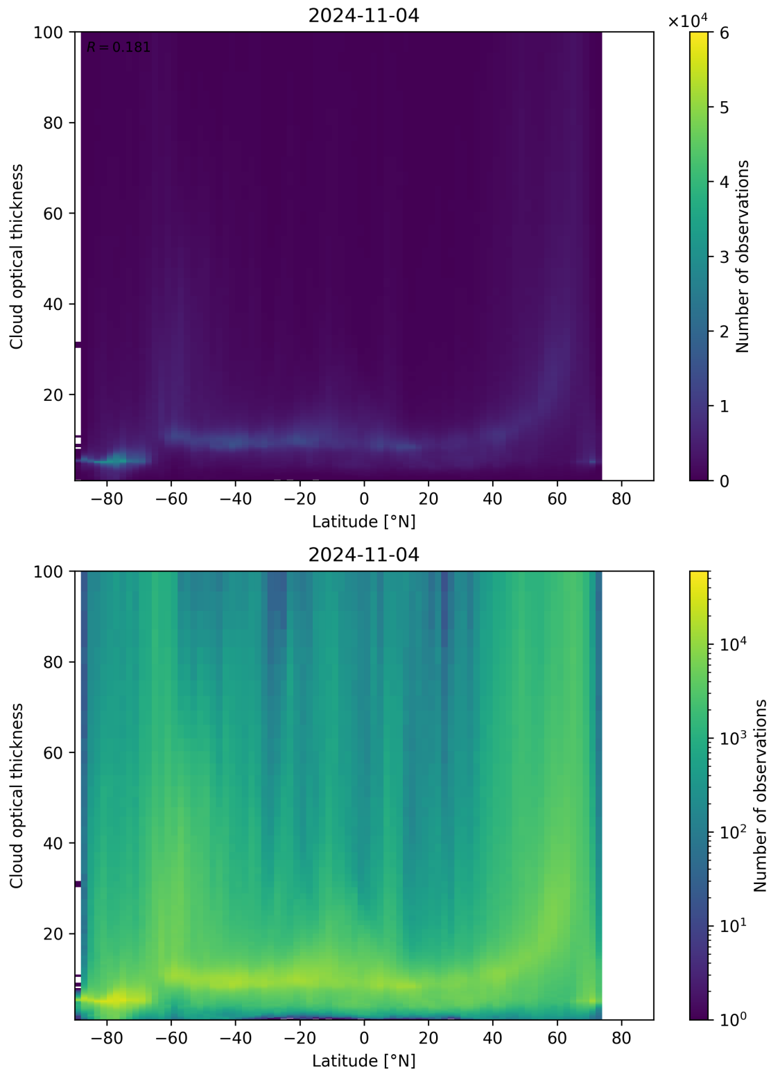
Figure 96: Scatter density plot of “Latitude” against “Cloud optical thickness” for 2024-11-04 to 2024-11-05.
