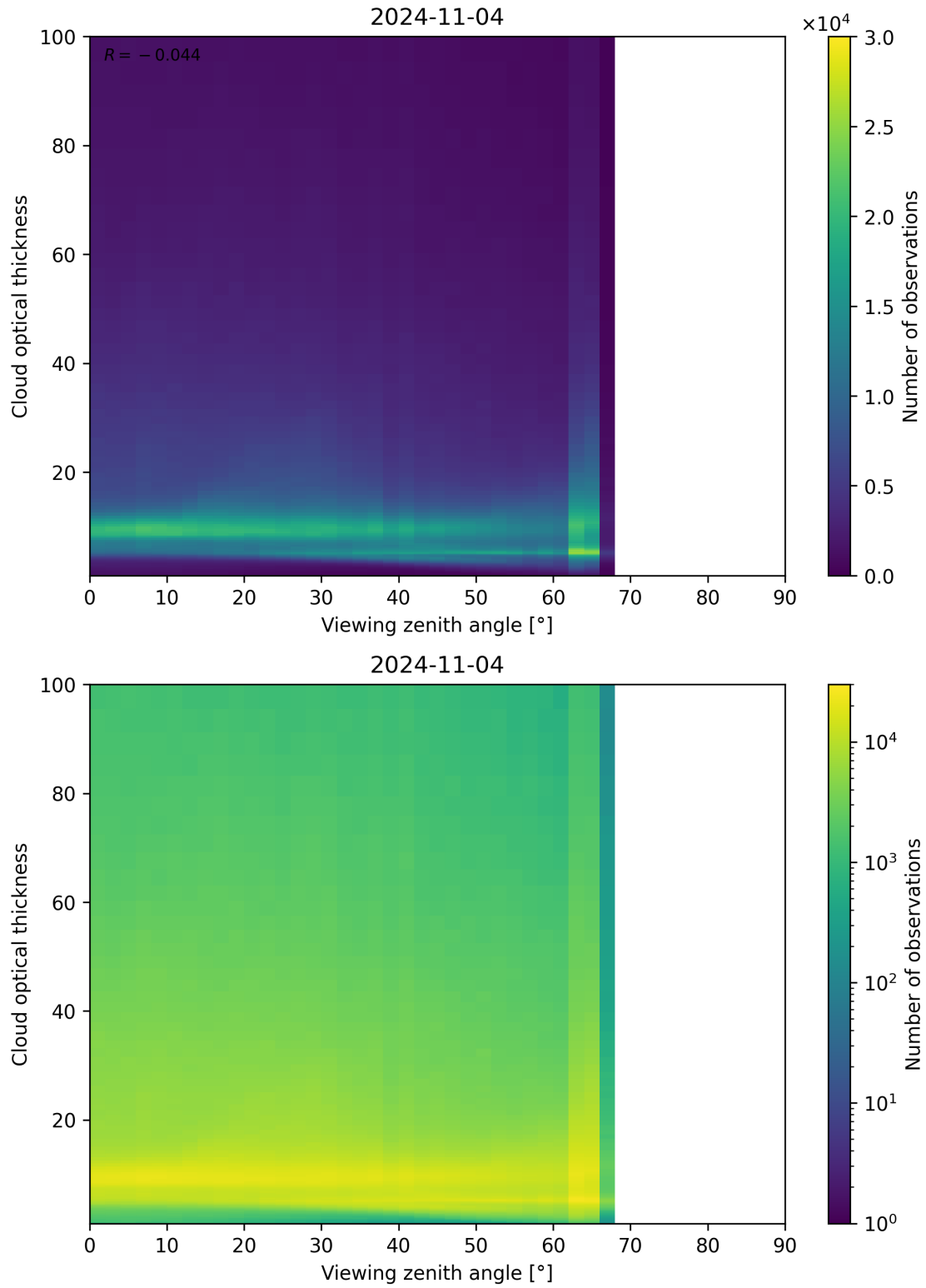
Figure 111: Scatter density plot of “Viewing zenith angle” against “Cloud optical thickness” for 2024-11-04 to 2024-11-05.
