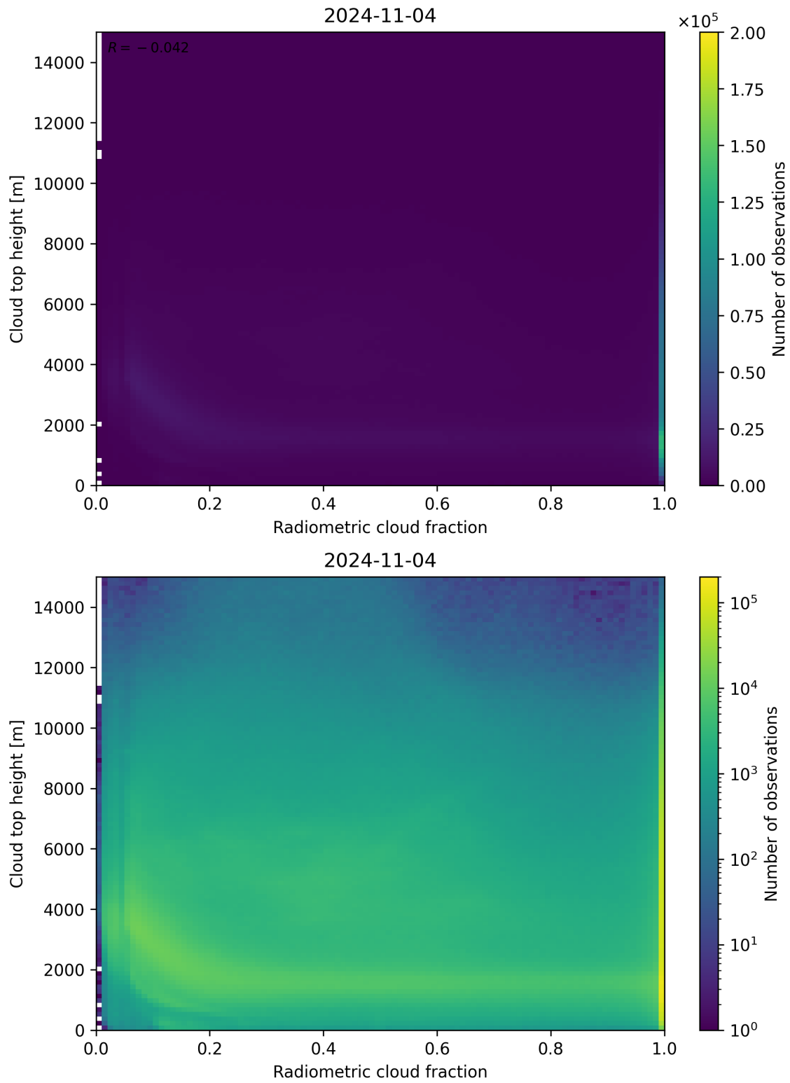
Figure 76: Scatter density plot of “Radiometric cloud fraction” against “Cloud top height” for 2024-11-04 to 2024-11-05.
