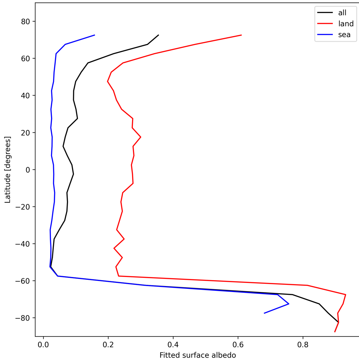
Figure 29: Zonal average of “Fitted surface albedo” for 2024-11-04 to 2024-11-05.
