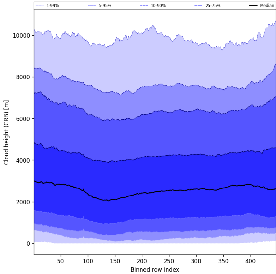
Figure 59: Along track statistics of “Cloud height (CRB)” for 2024-11-04 to 2024-11-05
