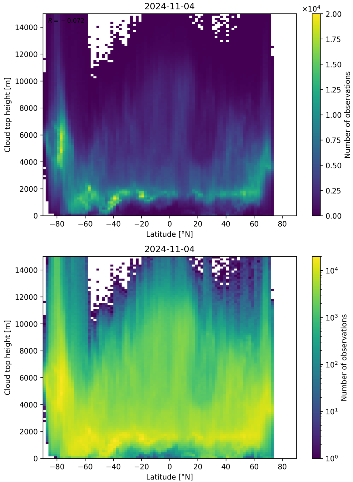
Figure 97: Scatter density plot of “Latitude” against “Cloud top height” for 2024-11-04 to 2024-11-05.
