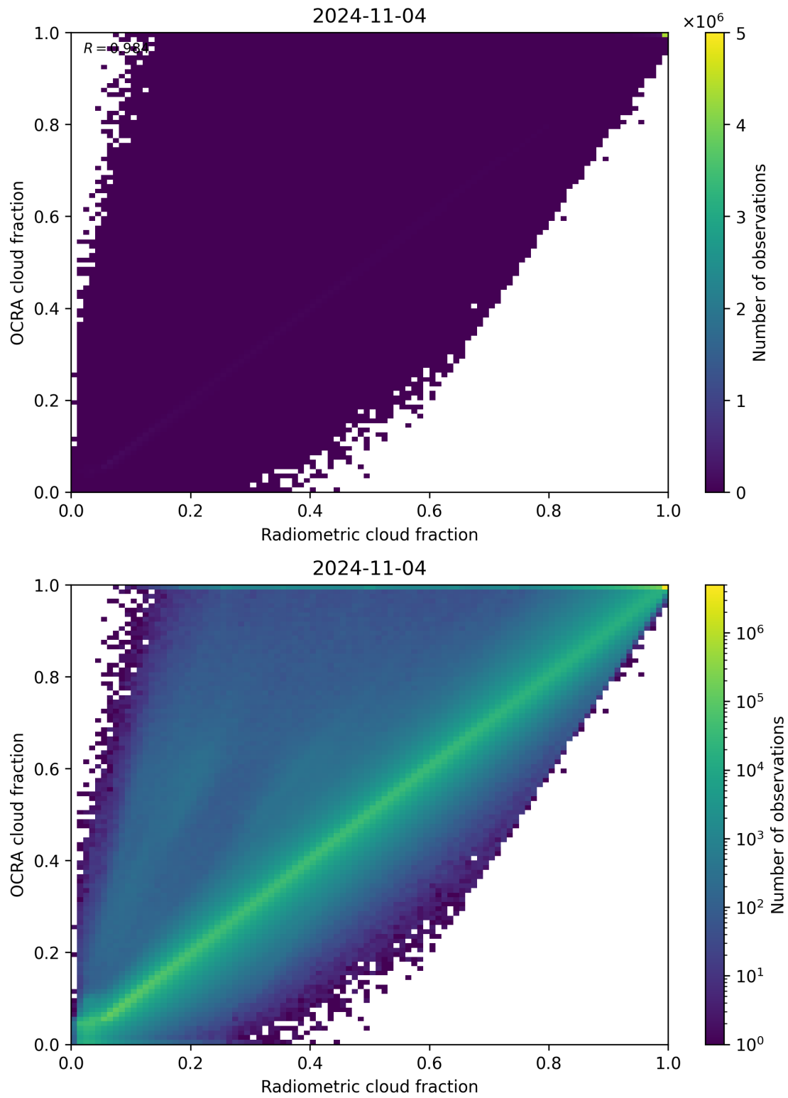
Figure 72: Scatter density plot of “Radiometric cloud fraction” against “OCRA cloud fraction” for 2024-11-04 to 2024-11-05.
