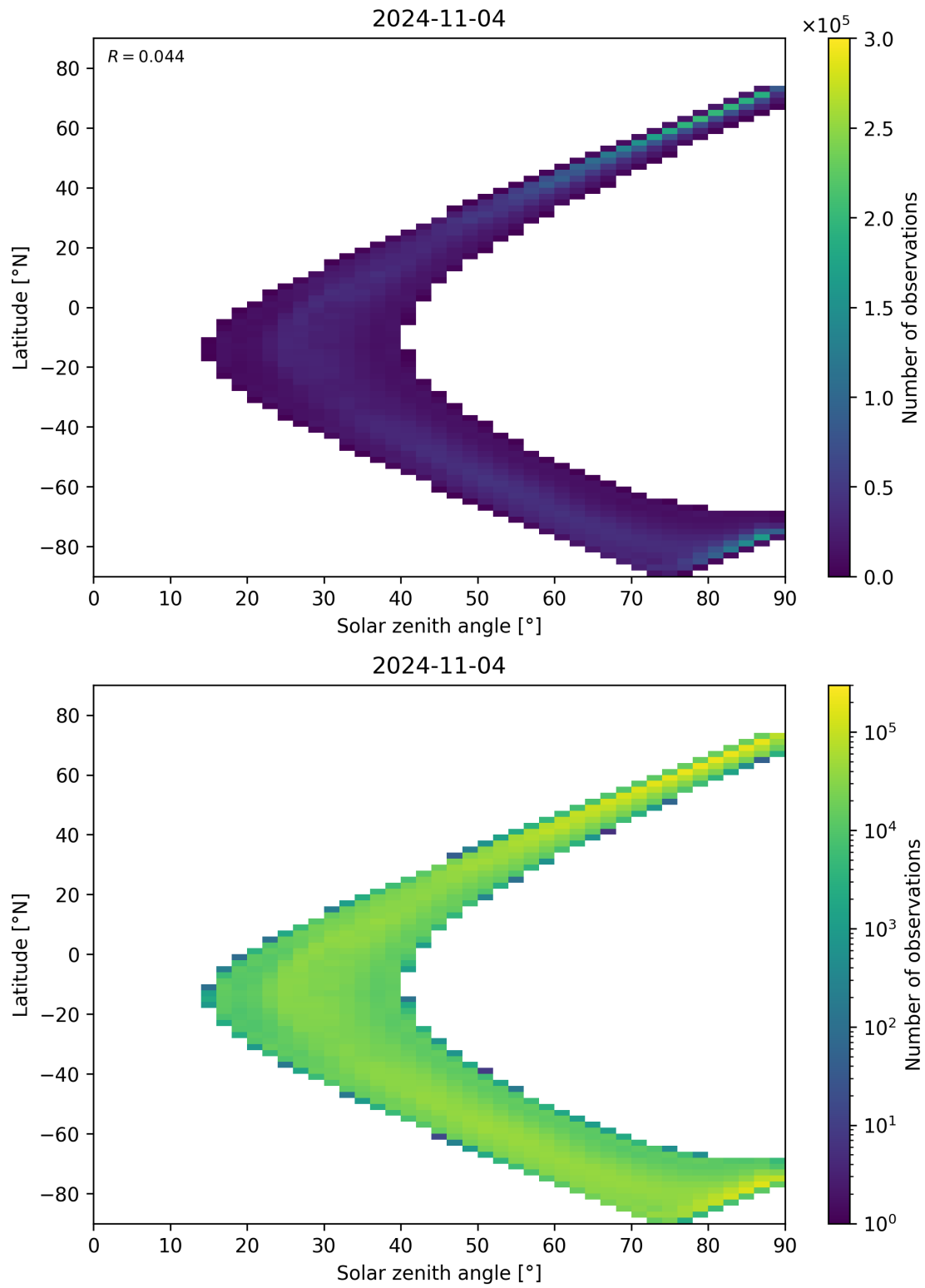
Figure 105: Scatter density plot of “Solar zenith angle” against “Latitude” for 2024-11-04 to 2024-11-05.
