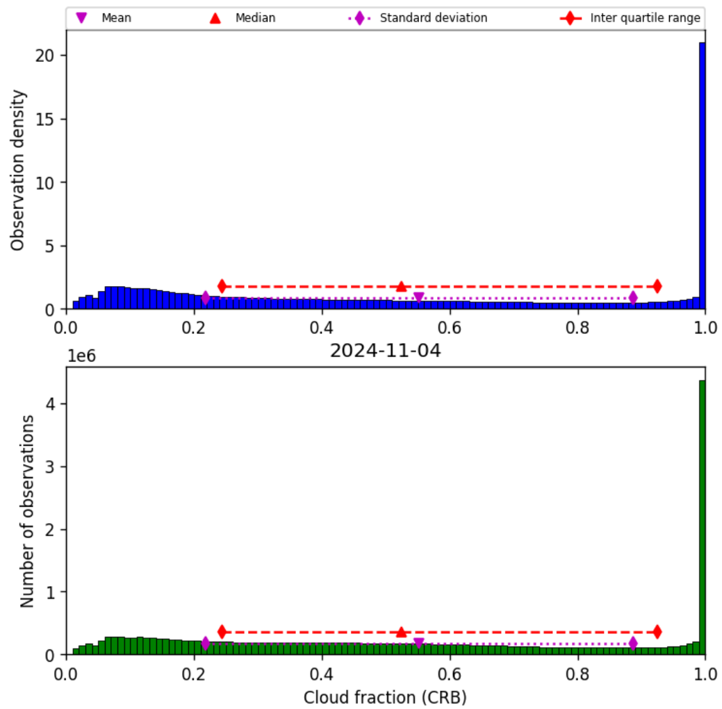
Figure 42: Histogram of “Cloud fraction (CRB)” for 2024-11-04 to 2024-11-05
