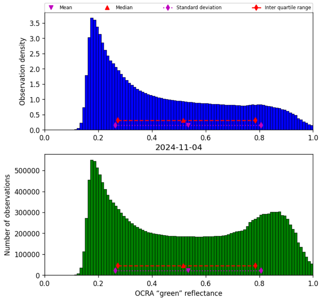
Figure 52: Histogram of “OCRA “green” reflectance” for 2024-11-04 to 2024-11-05
