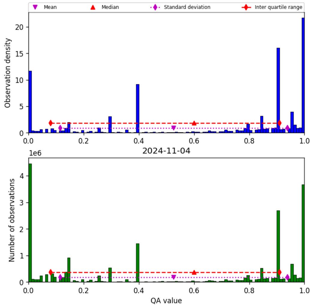
Figure 38: Histogram of “QA value” for 2024-11-04 to 2024-11-05
