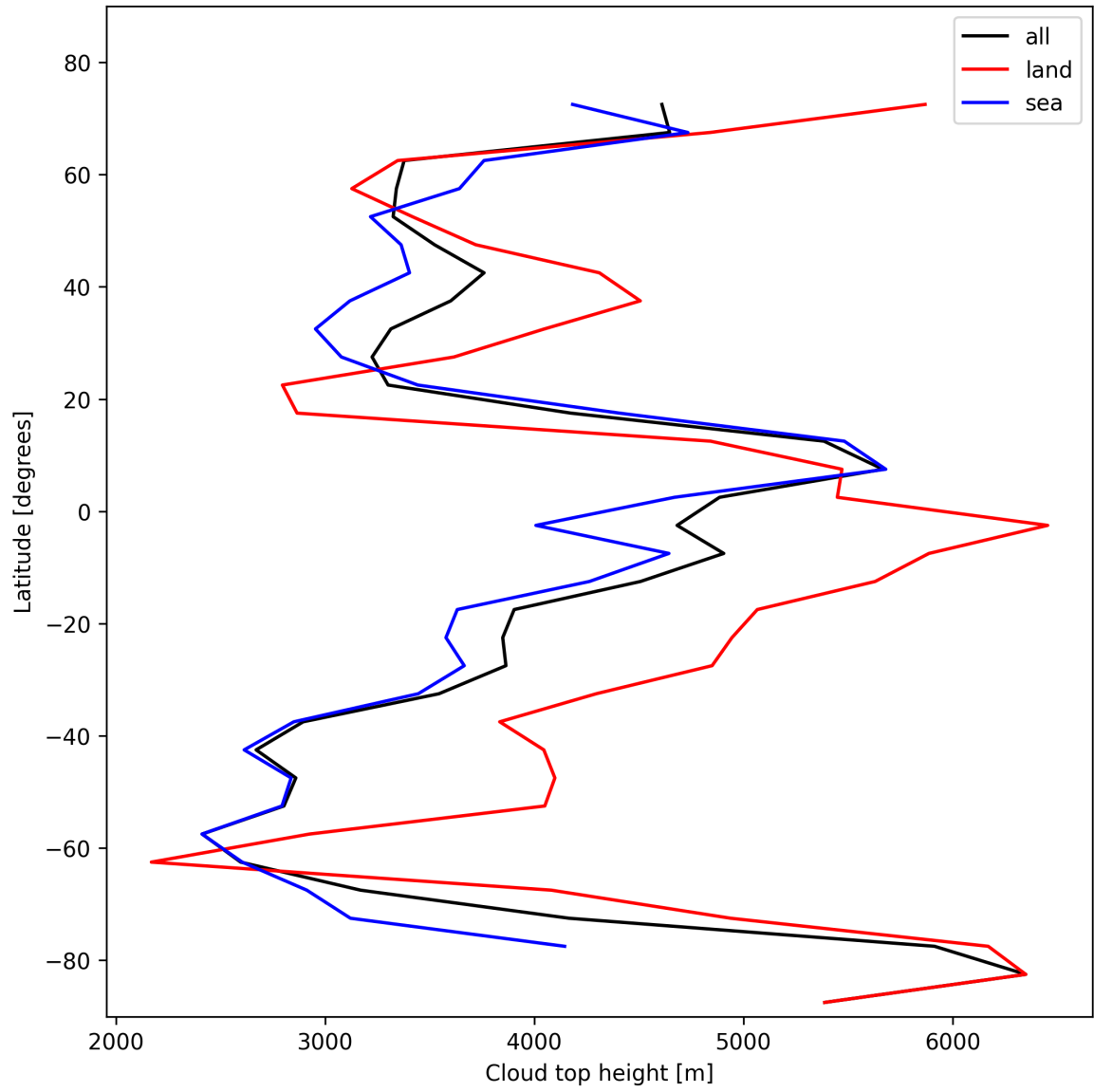
Figure 24: Zonal average of “Cloud top height” for 2024-11-04 to 2024-11-05.
