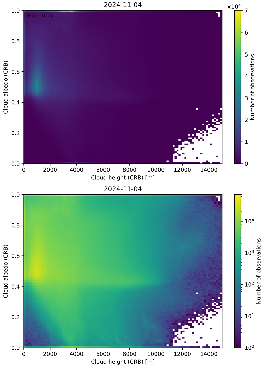
Figure 80: Scatter density plot of “Cloud height (CRB)” against “Cloud albedo (CRB)” for 2024-11-04 to 2024-11-05.
