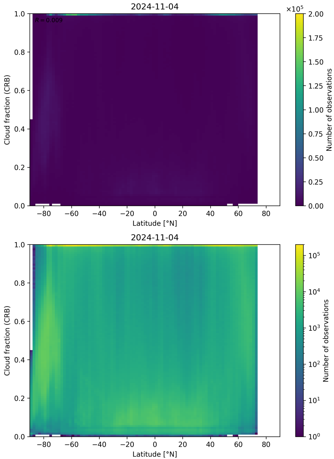
Figure 94: Scatter density plot of “Latitude” against “Cloud fraction (CRB)” for 2024-11-04 to 2024-11-05.
