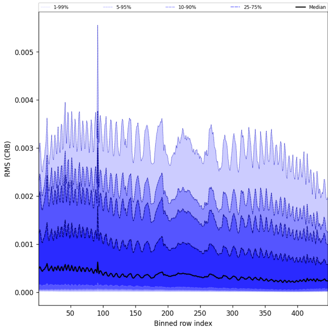
Figure 64: Along track statistics of “RMS (CRB)” for 2024-11-04 to 2024-11-05
