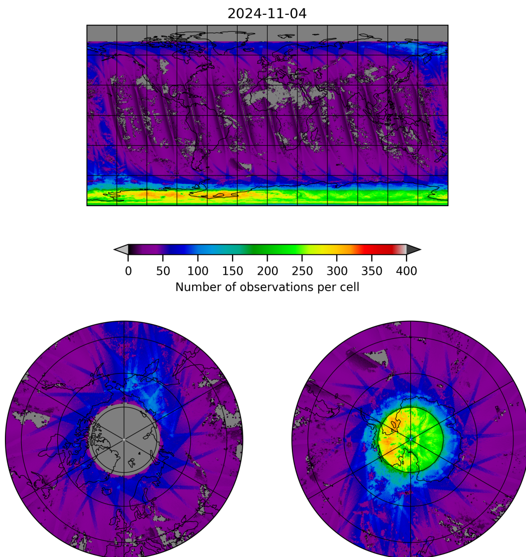
Figure 21: Map of the number of observations for 2024-11-04 to 2024-11-05
