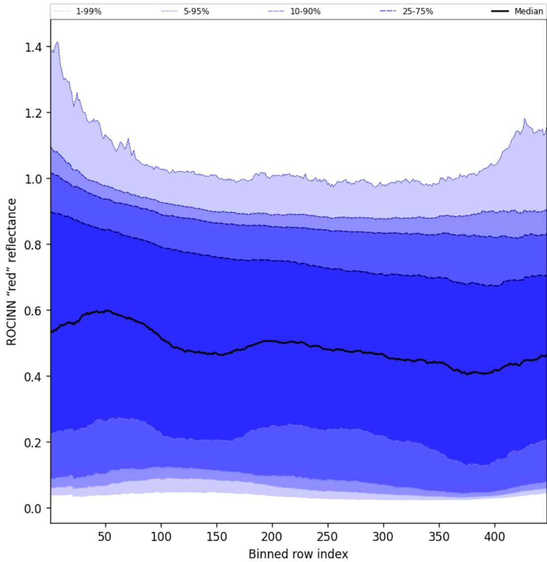
Figure 69: Along track statistics of “ROCINN “red” reflectance” for 2024-11-04 to 2024-11-05
