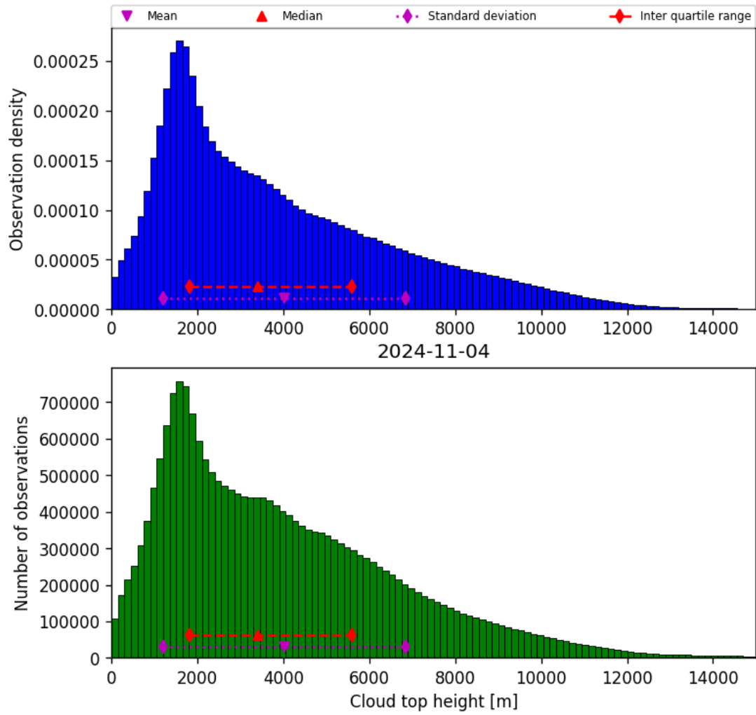
Figure 40: Histogram of “Cloud top height” for 2024-11-04 to 2024-11-05
