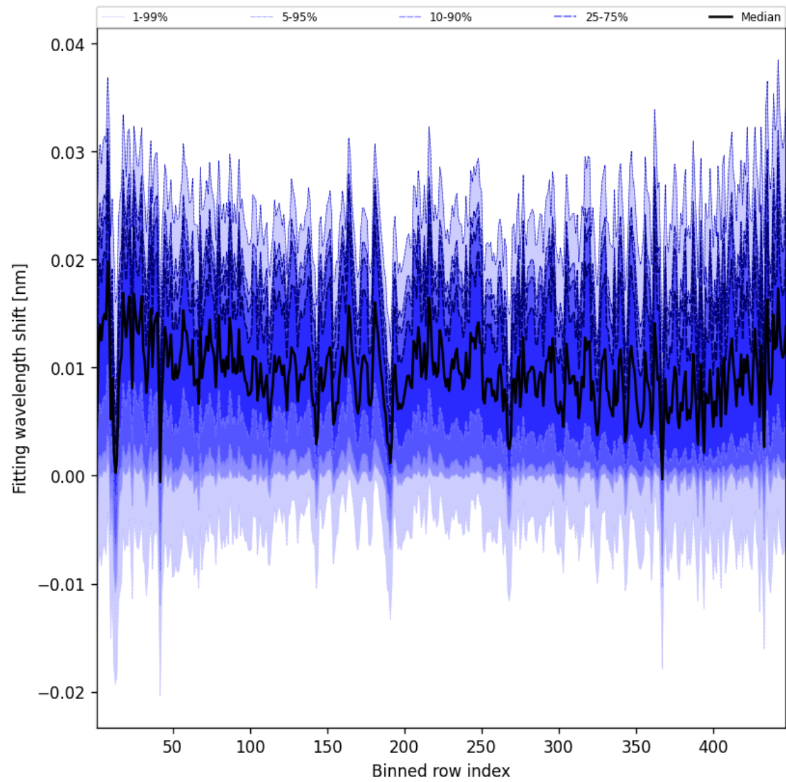
Figure 65: Along track statistics of “Fitting wavelength shift” for 2024-11-04 to 2024-11-05
