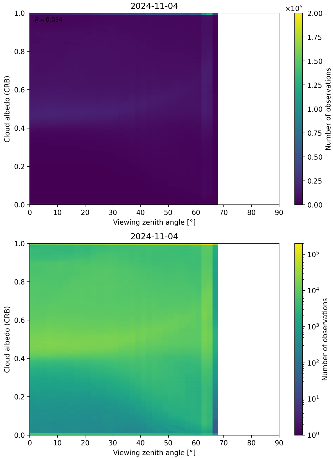
Figure 106: Scatter density plot of “Viewing zenith angle” against “Cloud albedo (CRB)” for 2024-11-04 to 2024-11-05.
