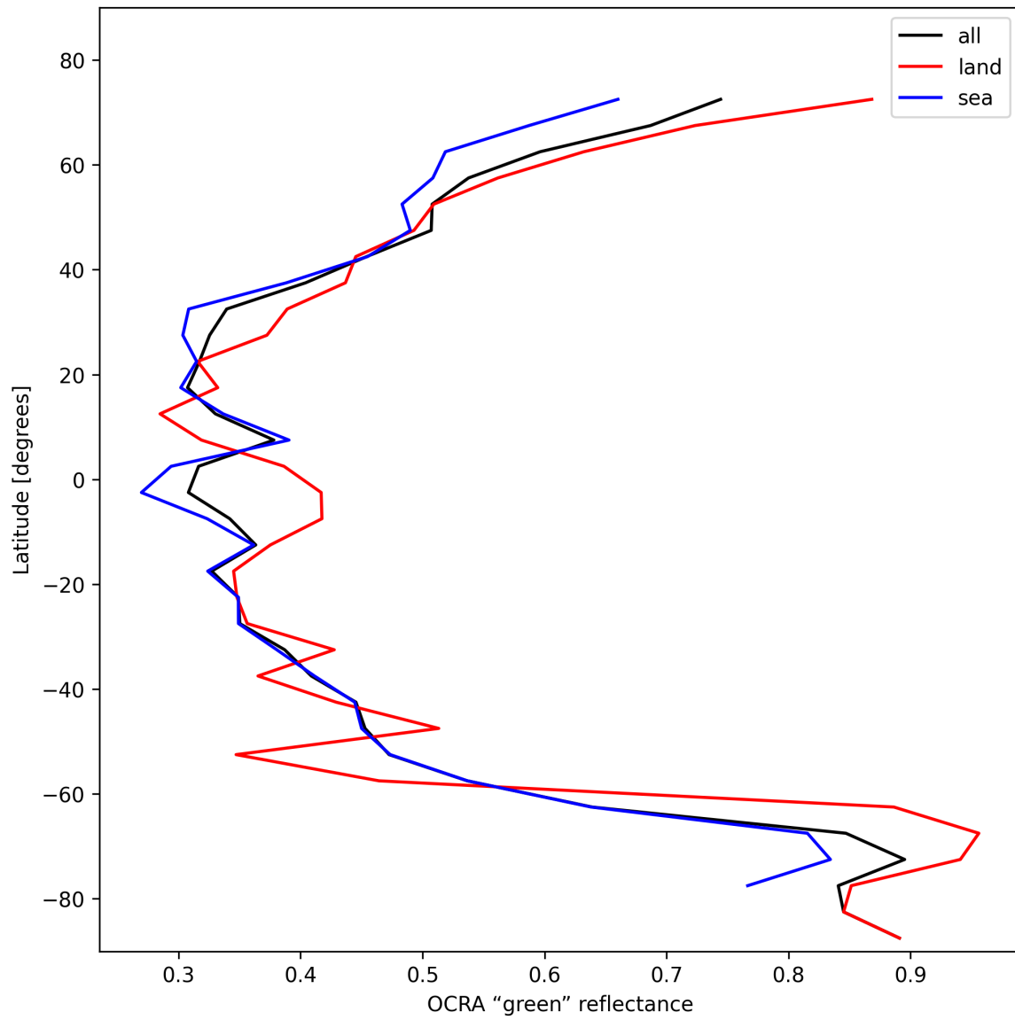
Figure 36: Zonal average of “OCRA “green” reflectance” for 2024-11-04 to 2024-11-05.
