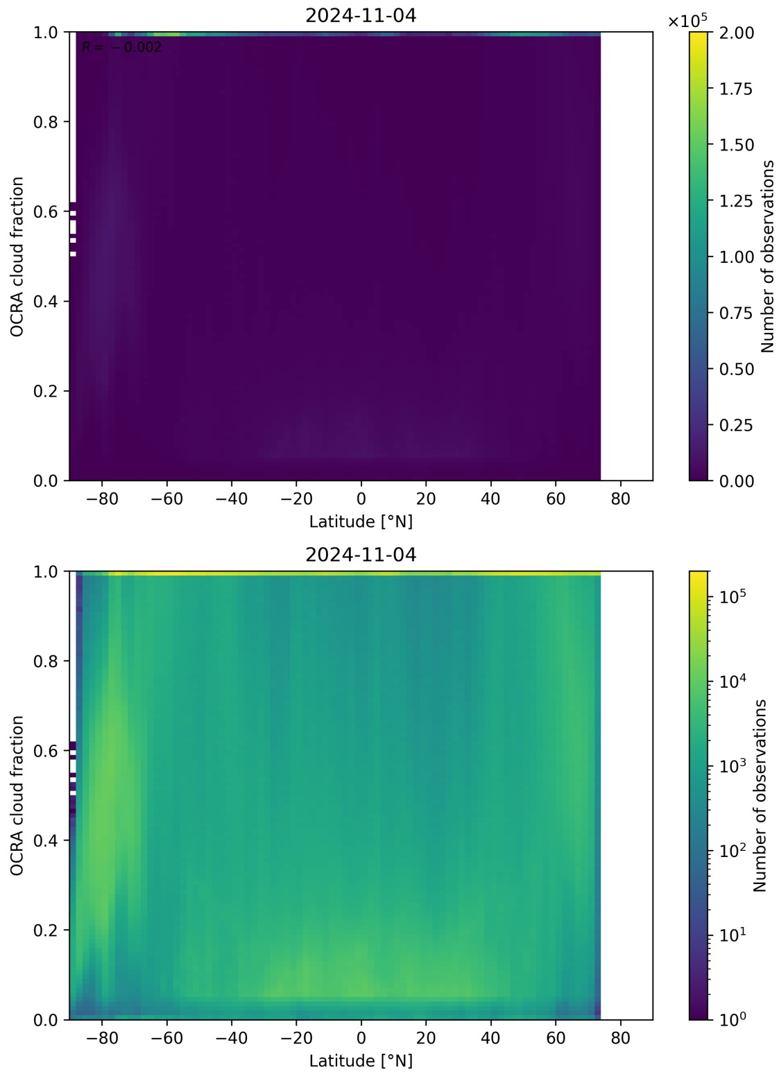
Figure 93: Scatter density plot of “Latitude” against “OCRA cloud fraction” for 2024-11-04 to 2024-11-05.
