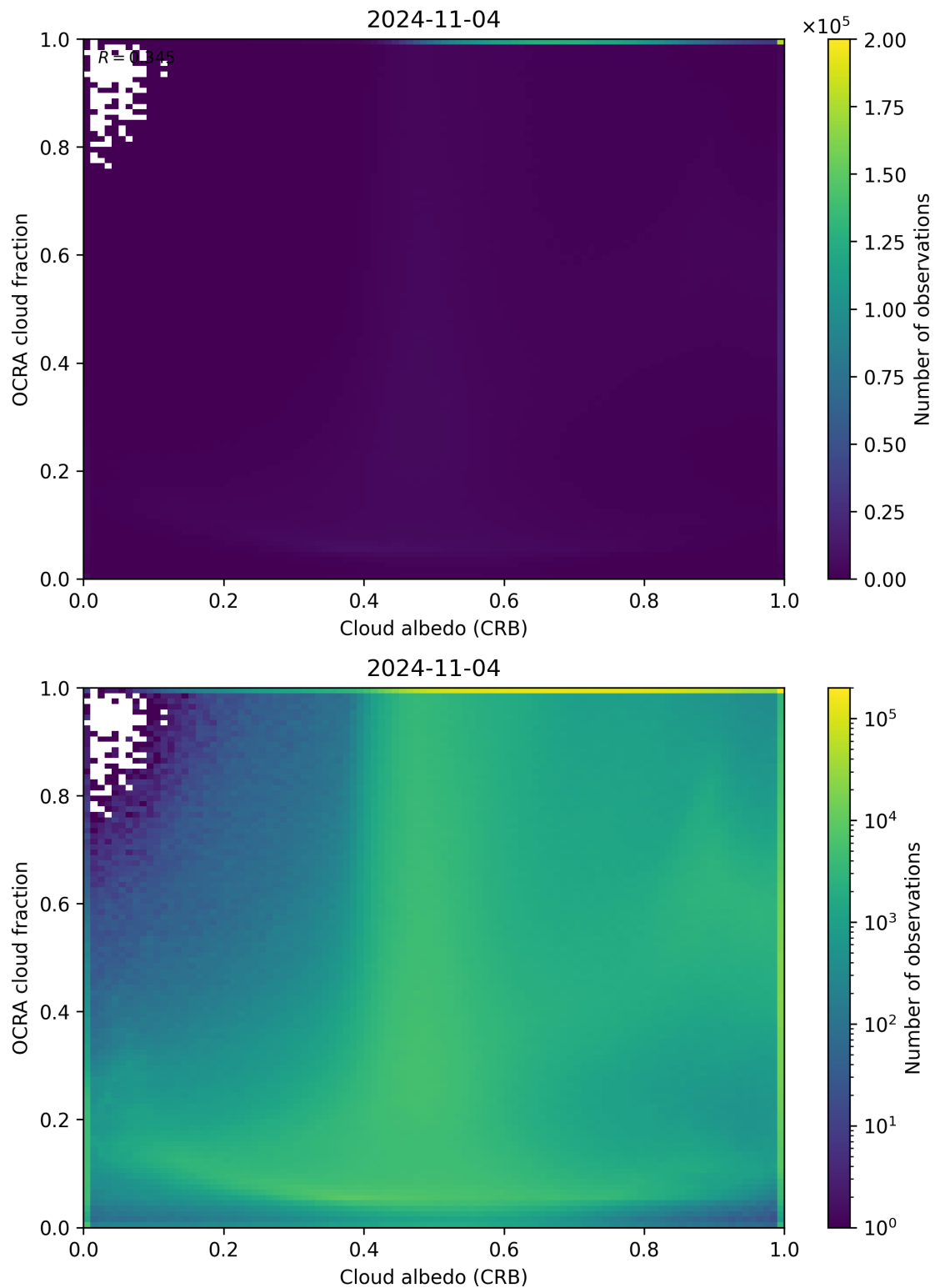
Figure 70: Scatter density plot of “Cloud albedo (CRB)” against “OCRA cloud fraction” for 2024-11-04 to 2024-11-05.
