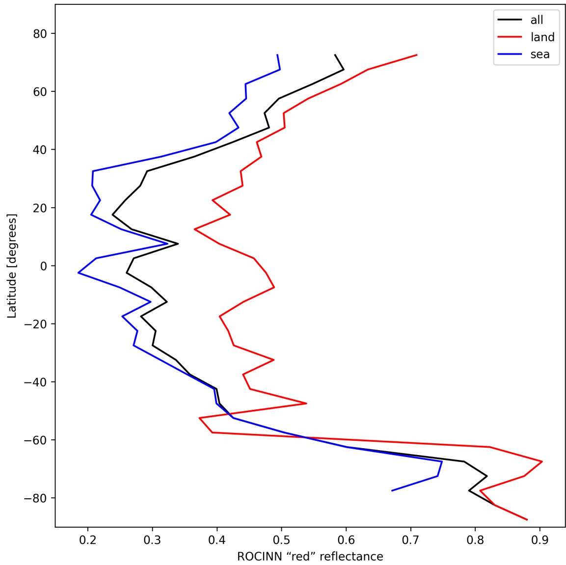
Figure 37: Zonal average of “ROCINN “red” reflectance” for 2024-11-04 to 2024-11-05.
