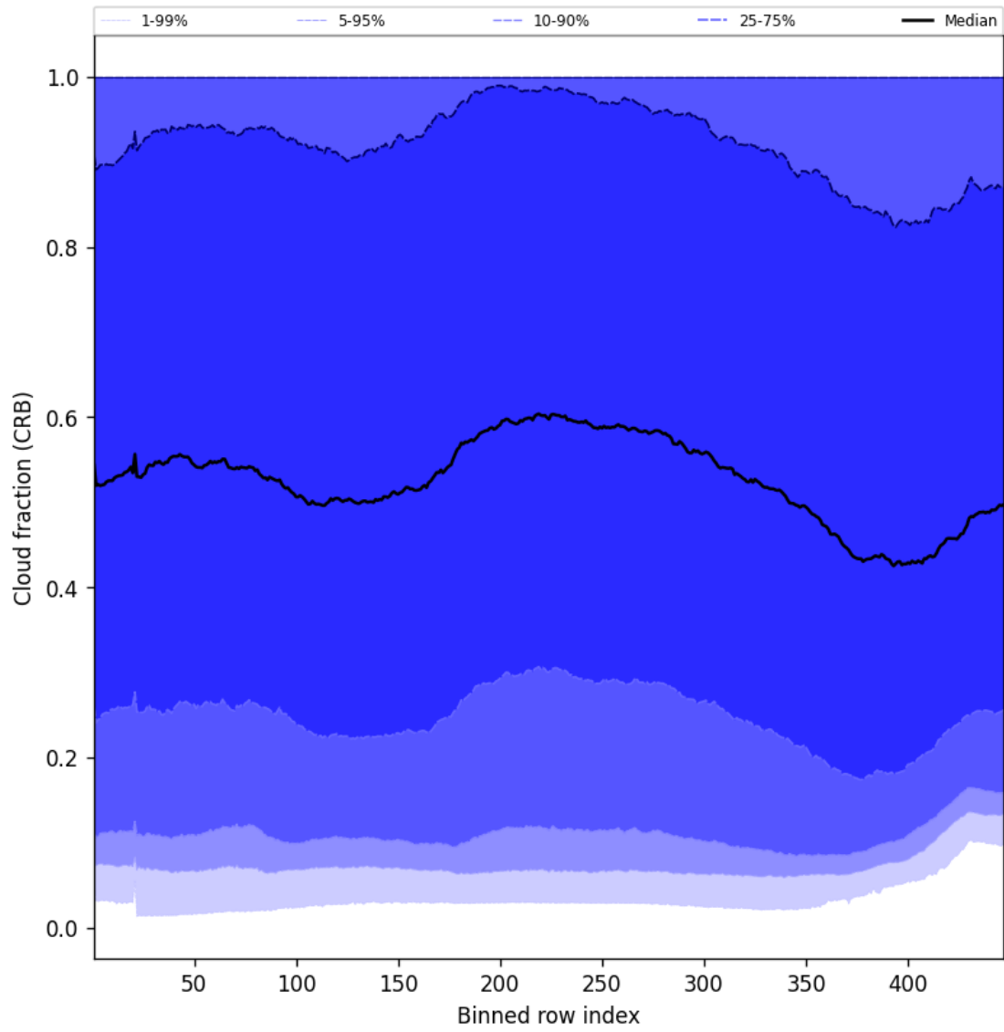
Figure 58: Along track statistics of “Cloud fraction (CRB)” for 2024-11-04 to 2024-11-05
