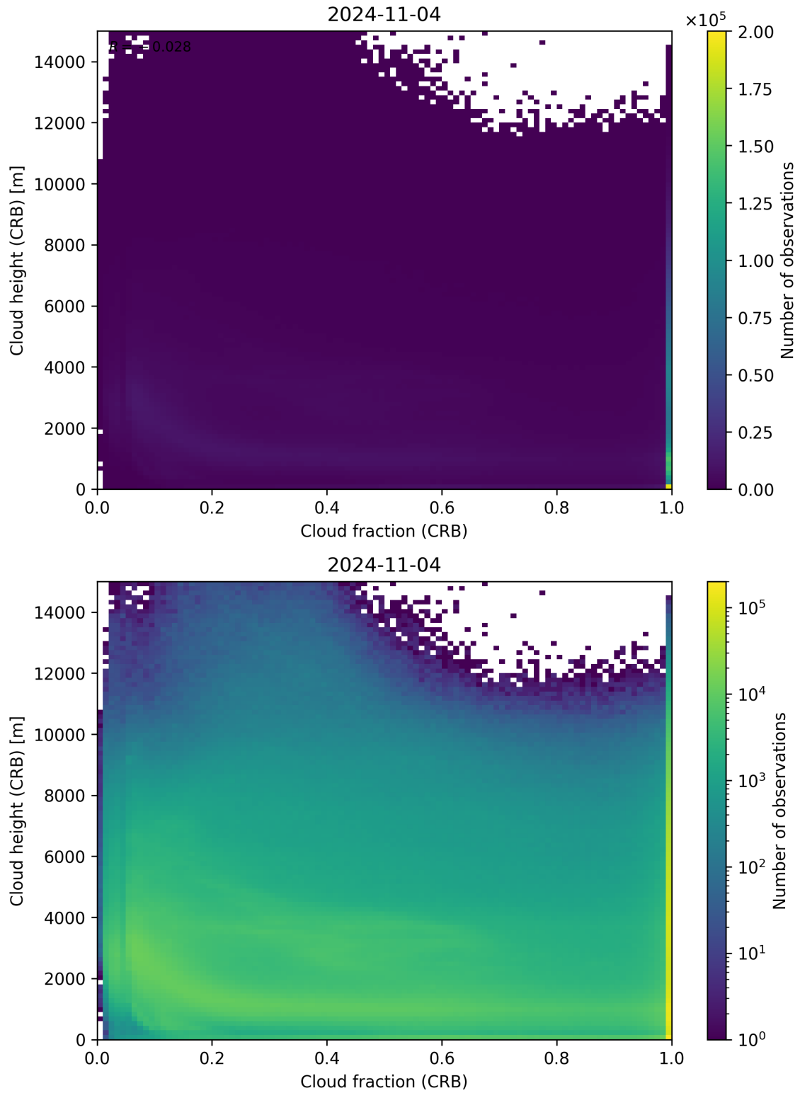
Figure 79: Scatter density plot of “Cloud fraction (CRB)” against “Cloud height (CRB)” for 2024-11-04 to 2024-11-05.
