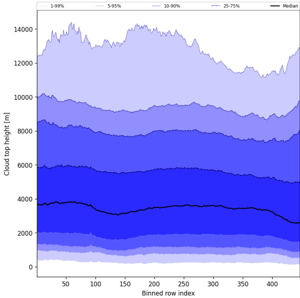
Figure 56: Along track statistics of “Cloud top height” for 2024-11-04 to 2024-11-05
