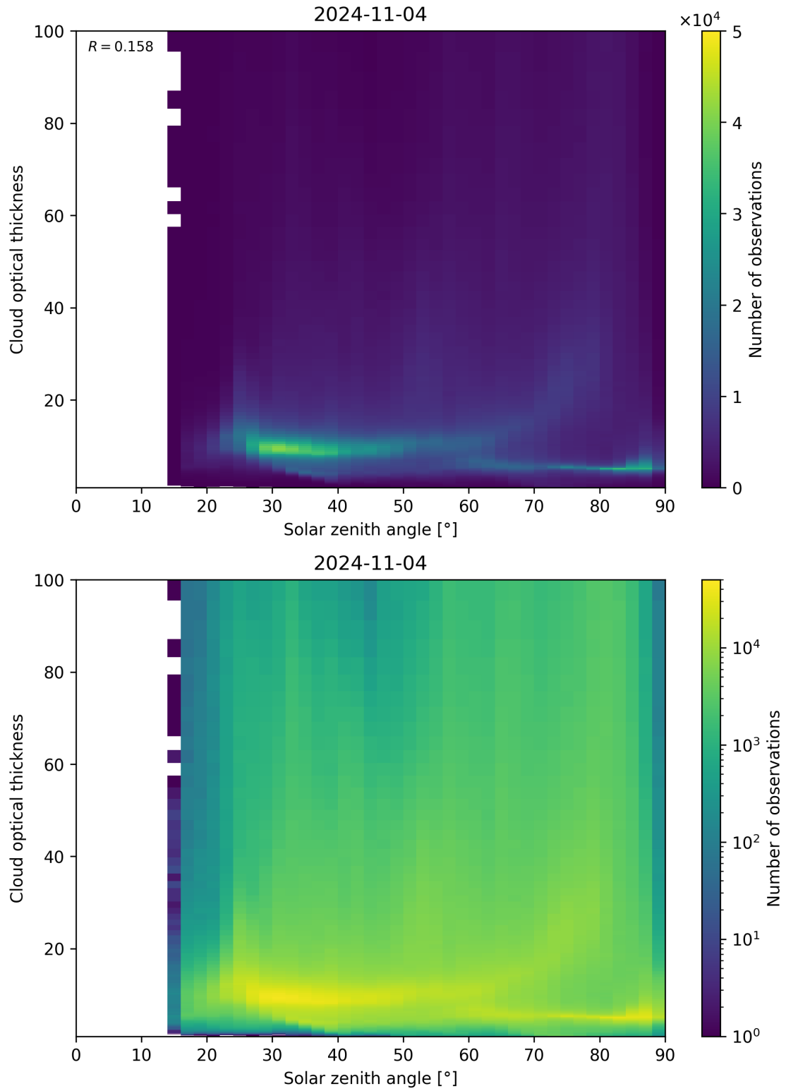
Figure 103: Scatter density plot of “Solar zenith angle” against “Cloud optical thickness” for 2024-11-04 to 2024-11-05.
