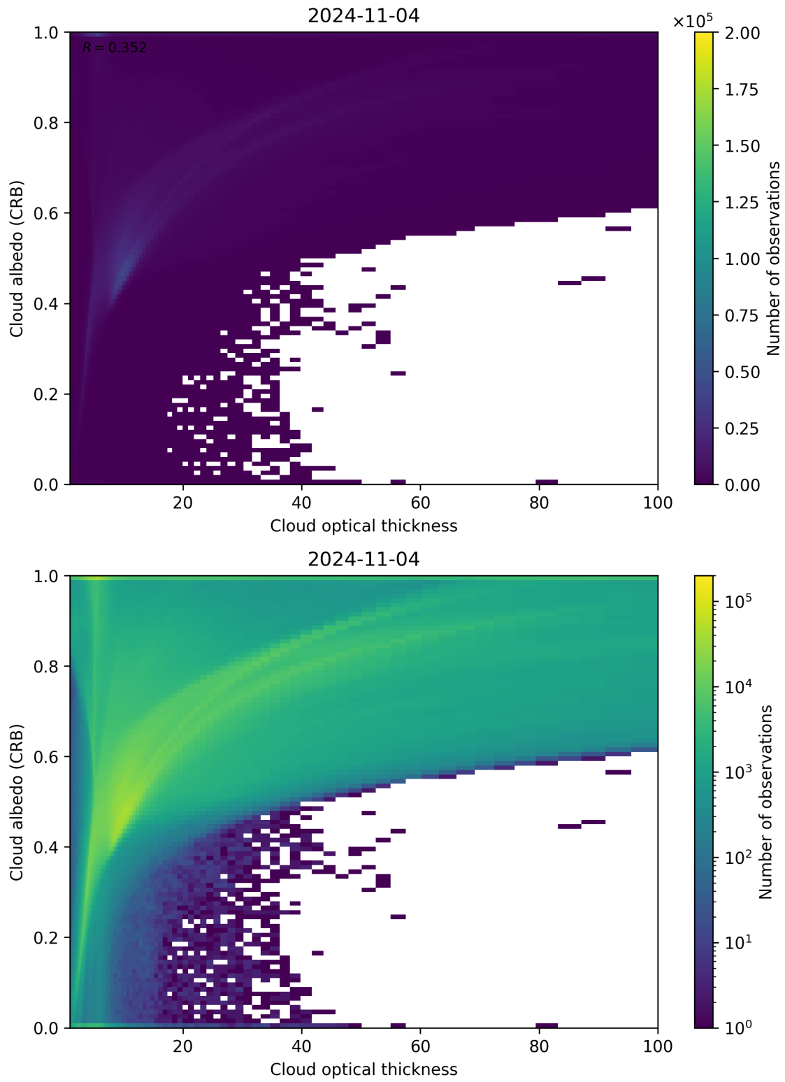
Figure 82: Scatter density plot of “Cloud optical thickness” against “Cloud albedo (CRB)” for 2024-11-04 to 2024-11-05.
