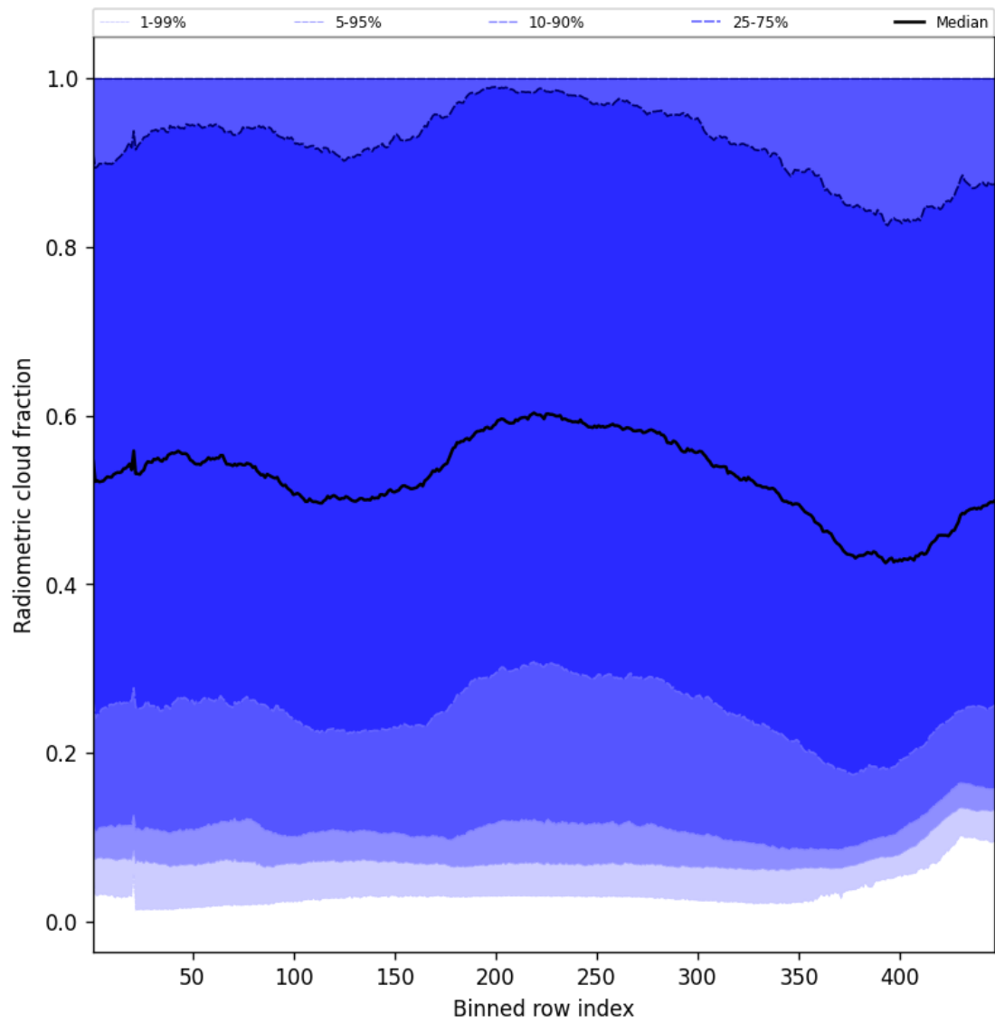
Figure 55: Along track statistics of “Radiometric cloud fraction” for 2024-11-04 to 2024-11-05
