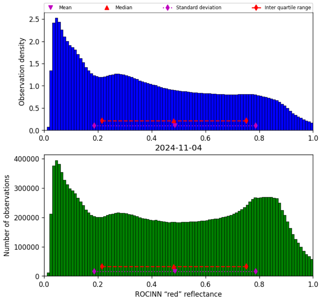
Figure 53: Histogram of “ROCINN “red” reflectance” for 2024-11-04 to 2024-11-05
