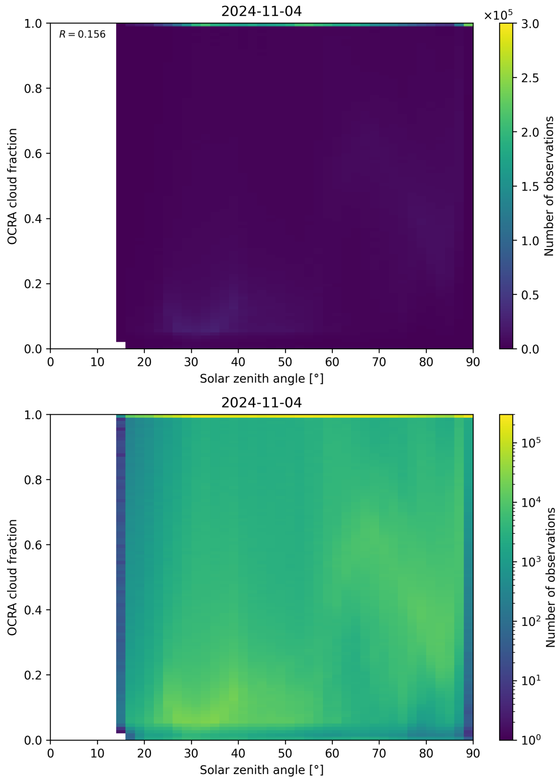
Figure 100: Scatter density plot of “Solar zenith angle” against “OCRA cloud fraction” for 2024-11-04 to 2024-11-05.
