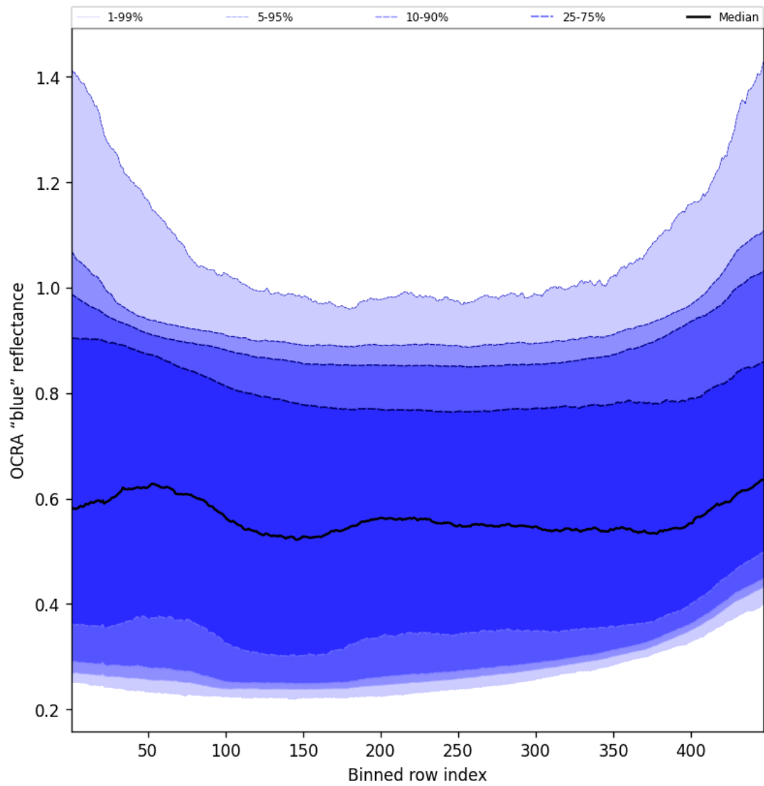
Figure 67: Along track statistics of “OCRA “blue” reflectance” for 2024-11-04 to 2024-11-05
