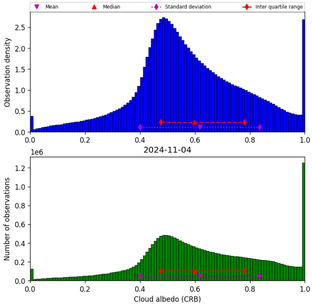
Figure 44: Histogram of “Cloud albedo (CRB)” for 2024-11-04 to 2024-11-05
