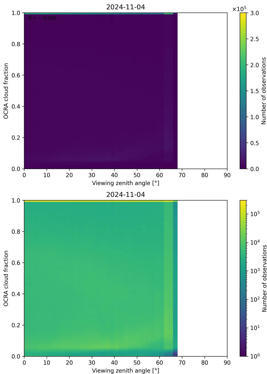
Figure 108: Scatter density plot of “Viewing zenith angle” against “OCRA cloud fraction” for 2024-11-04 to 2024-11-05.
