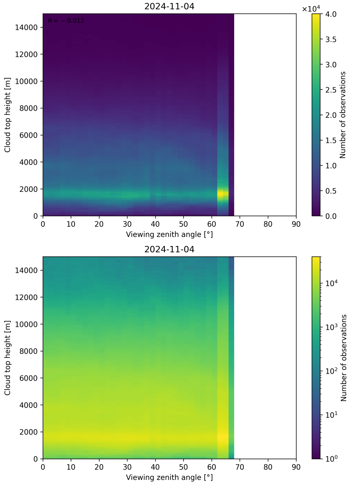
Figure 112: Scatter density plot of “Viewing zenith angle” against “Cloud top height” for 2024-11-04 to 2024-11-05.
