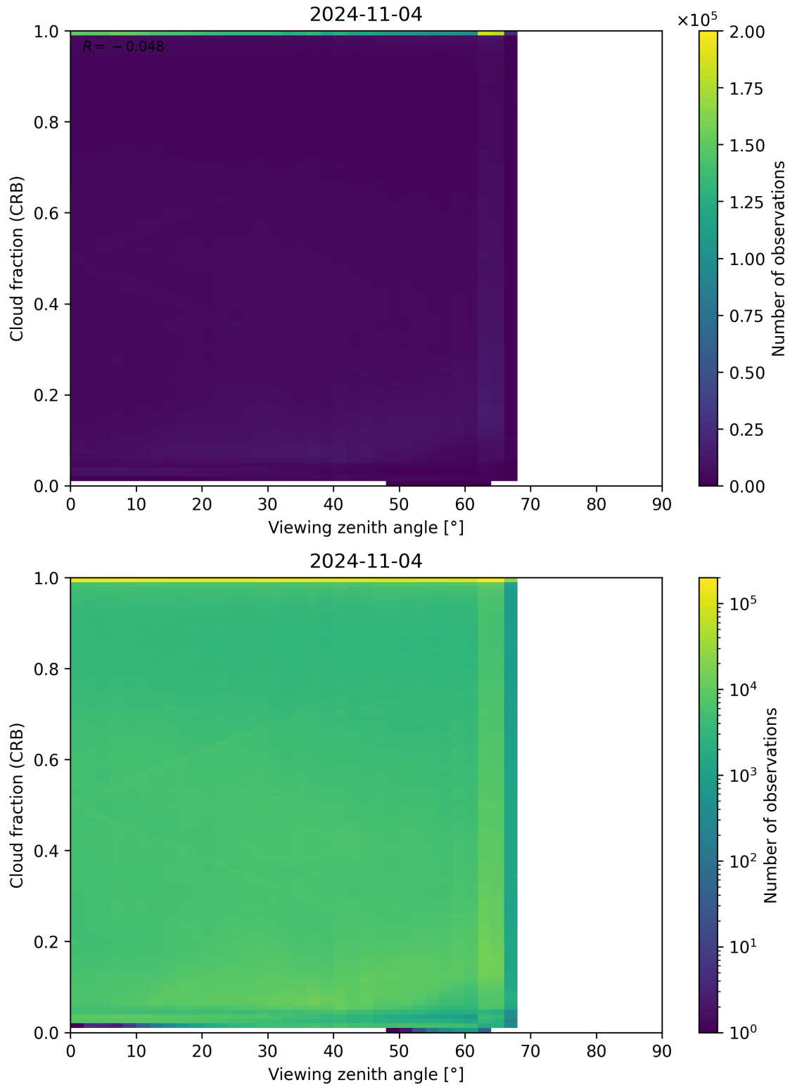
Figure 109: Scatter density plot of “Viewing zenith angle” against “Cloud fraction (CRB)” for 2024-11-04 to 2024-11-05.
