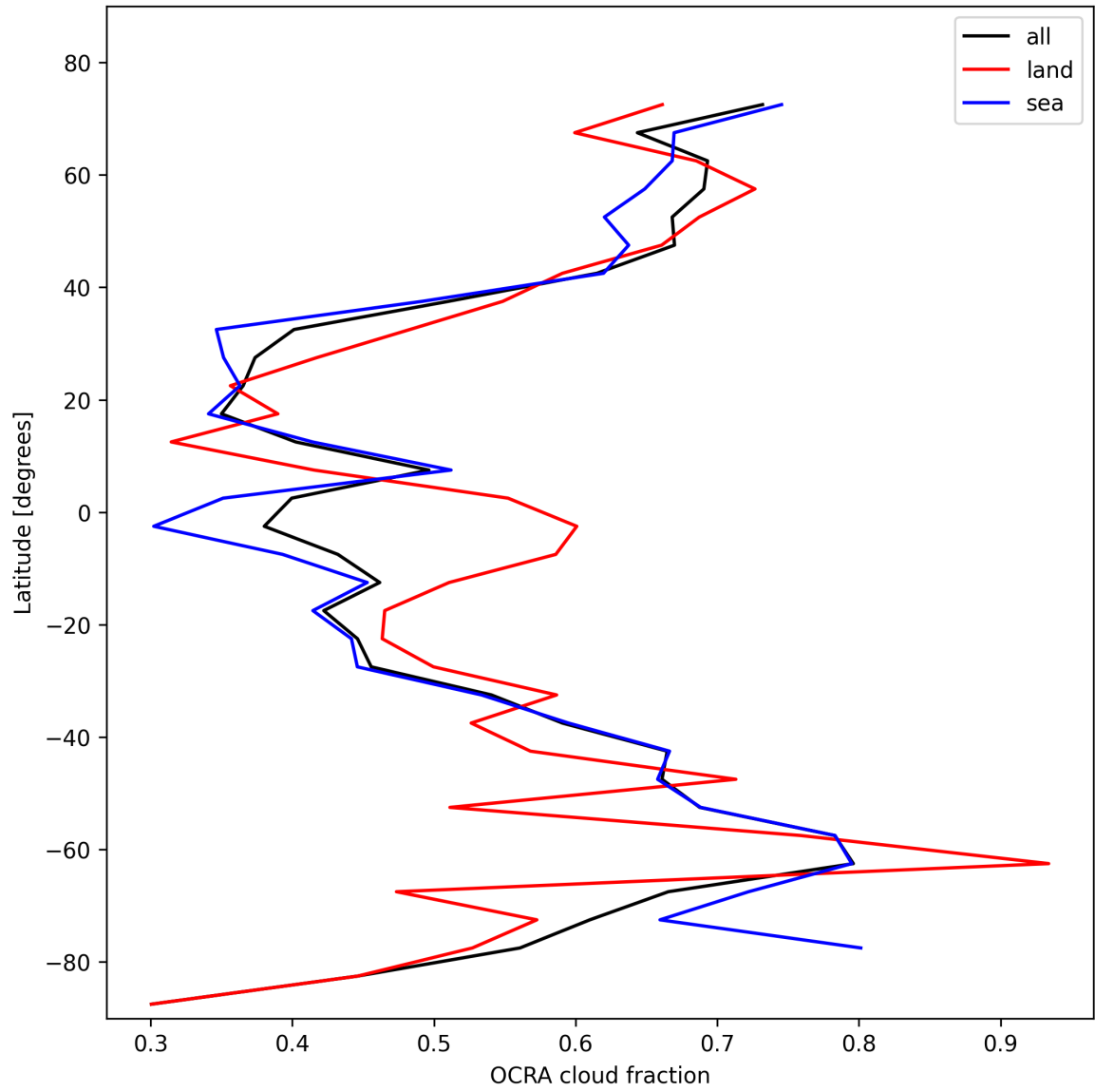
Figure 34: Zonal average of “OCRA cloud fraction” for 2024-11-04 to 2024-11-05.
