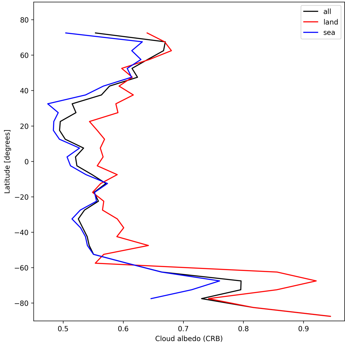
Figure 28: Zonal average of “Cloud albedo (CRB)” for 2024-11-04 to 2024-11-05.
