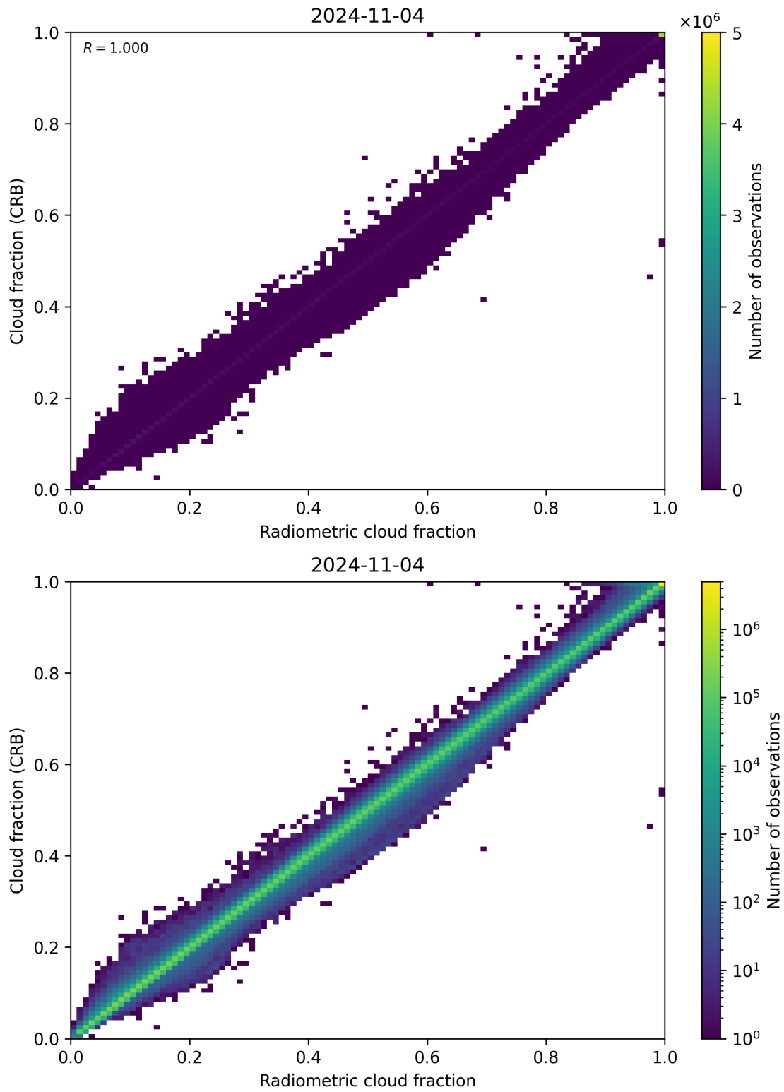
Figure 73: Scatter density plot of “Radiometric cloud fraction” against “Cloud fraction (CRB)” for 2024-11-04 to 2024-11-05.
