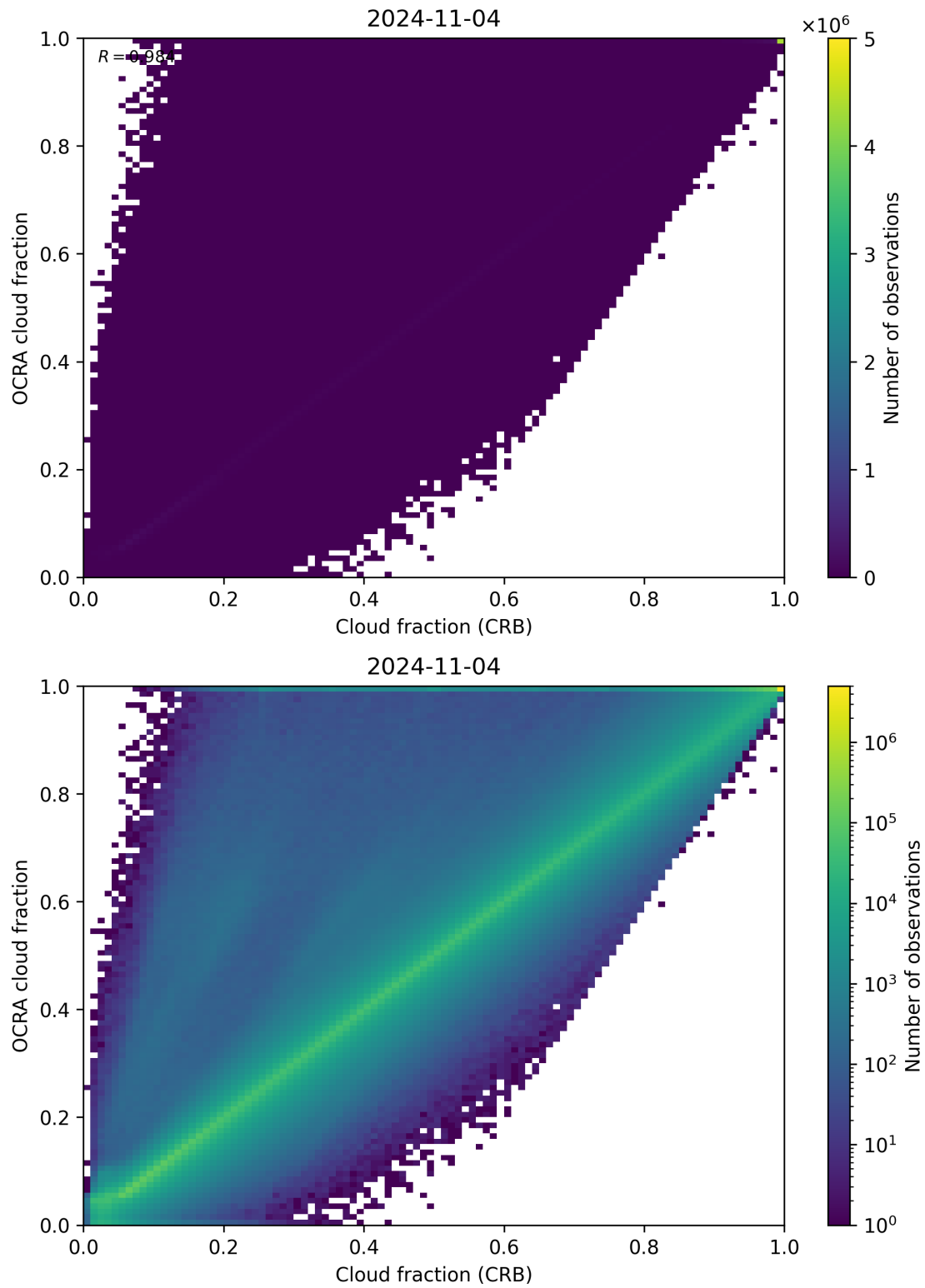
Figure 78: Scatter density plot of “Cloud fraction (CRB)” against “OCRA cloud fraction” for 2024-11-04 to 2024-11-05.
