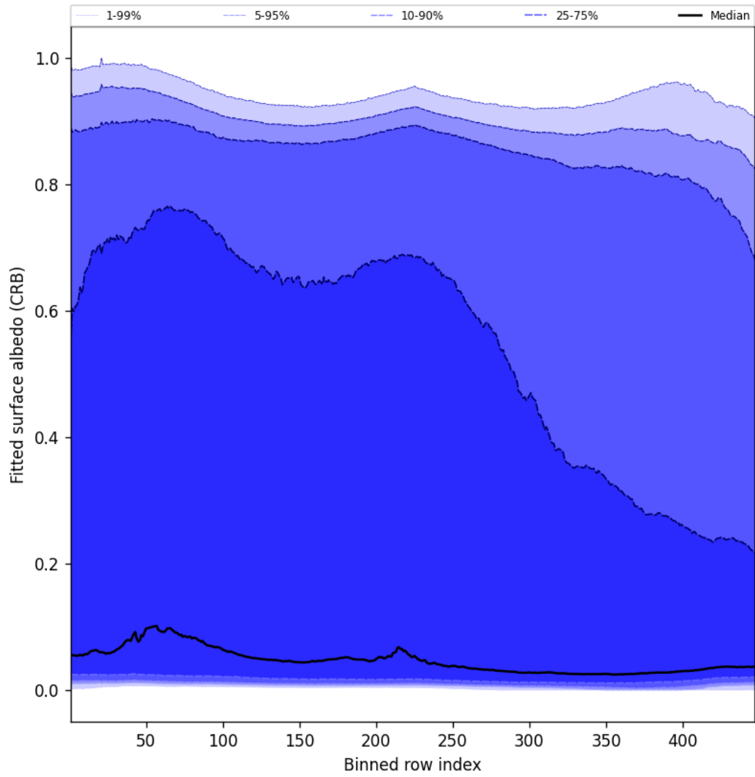
Figure 62: Along track statistics of “Fitted surface albedo (CRB)” for 2024-11-04 to 2024-11-05
