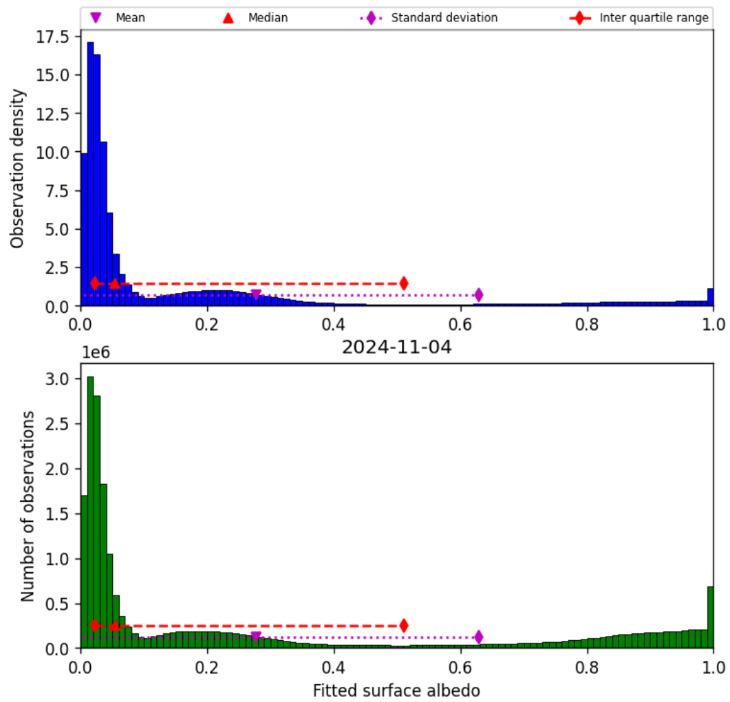
Figure 45: Histogram of “Fitted surface albedo” for 2024-11-04 to 2024-11-05
