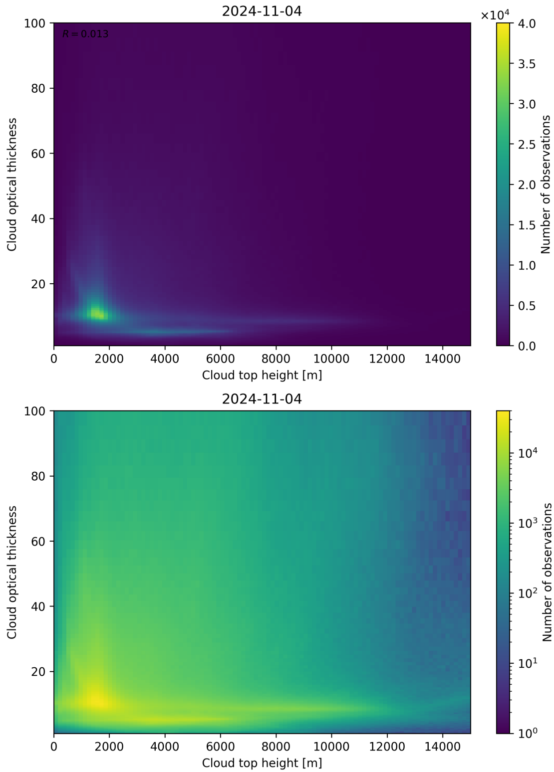
Figure 90: Scatter density plot of “Cloud top height” against “Cloud optical thickness” for 2024-11-04 to 2024-11-05.
