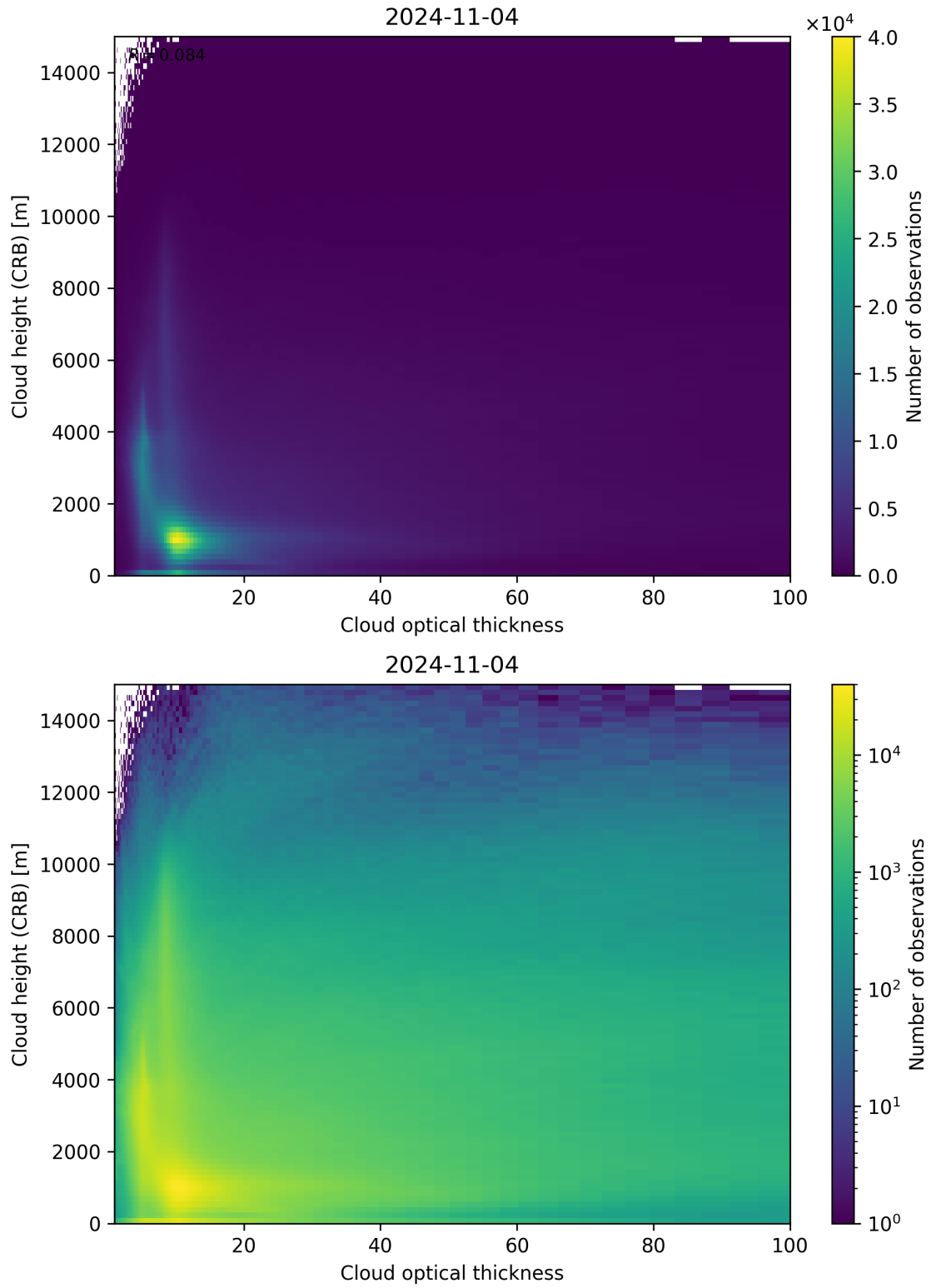
Figure 85: Scatter density plot of “Cloud optical thickness” against “Cloud height (CRB)” for 2024-11-04 to 2024-11-05.
