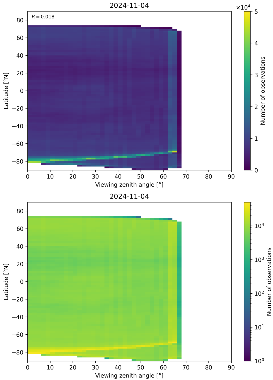
Figure 113: Scatter density plot of “Viewing zenith angle” against “Latitude” for 2024-11-04 to 2024-11-05.
