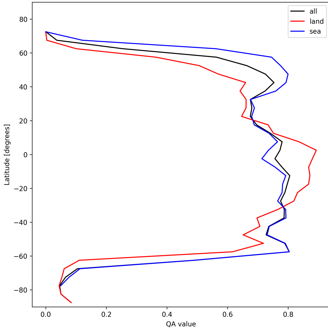
Figure 22: Zonal average of “QA value” for 2024-11-04 to 2024-11-05.
