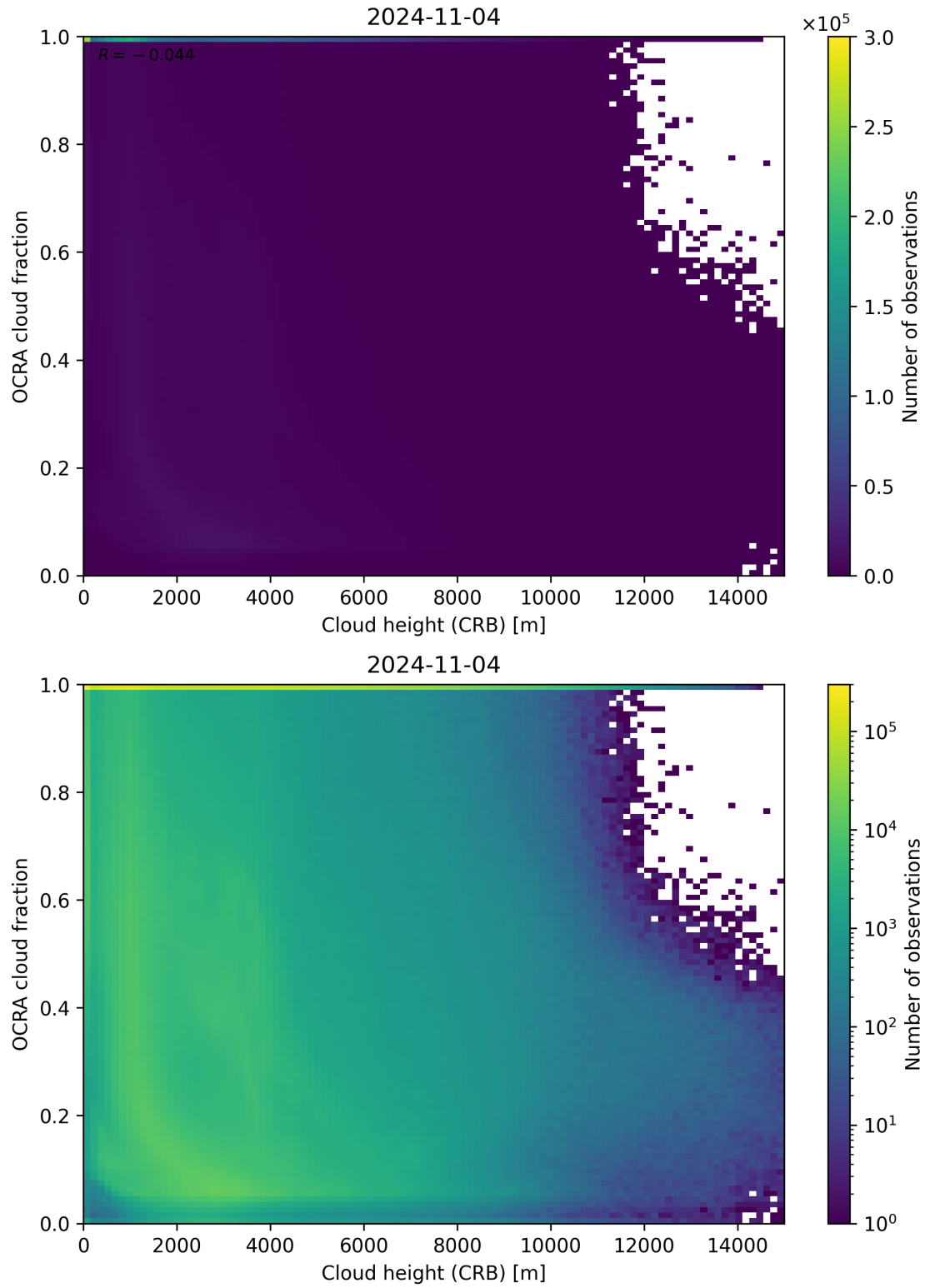
Figure 81: Scatter density plot of “Cloud height (CRB)” against “OCRA cloud fraction” for 2024-11-04 to 2024-11-05.
