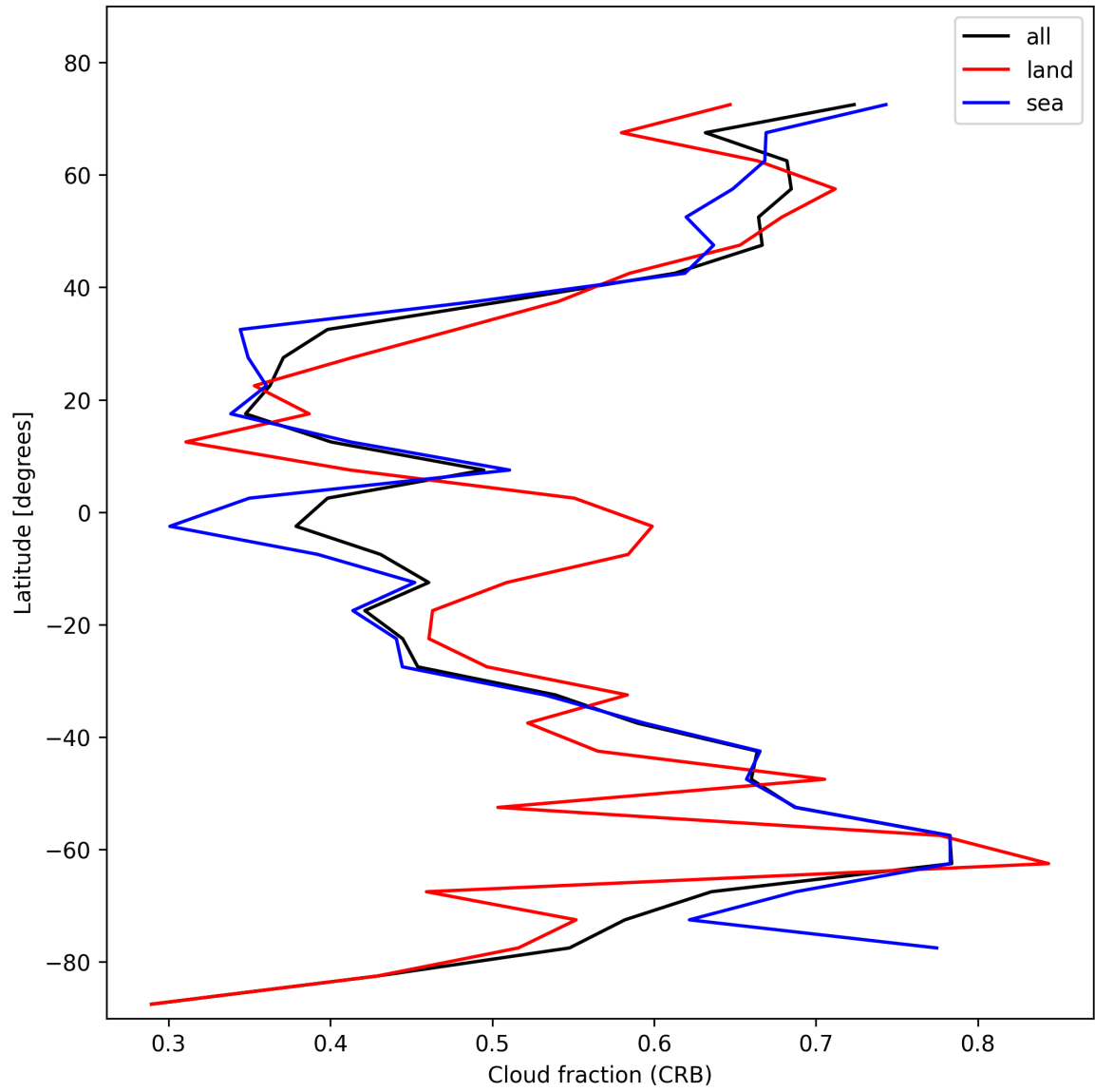
Figure 26: Zonal average of “Cloud fraction (CRB)” for 2024-11-04 to 2024-11-05.
