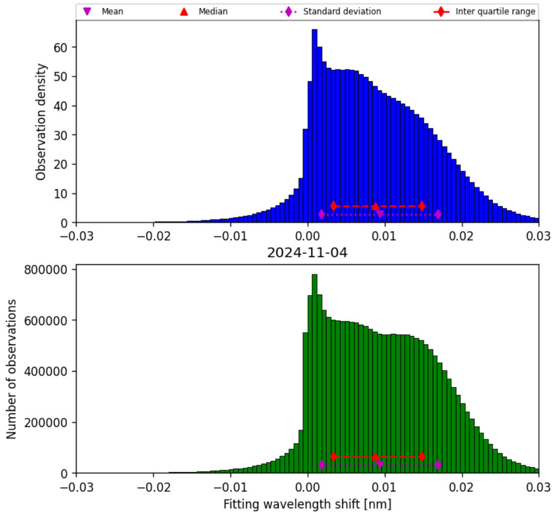
Figure 49: Histogram of “Fitting wavelength shift” for 2024-11-04 to 2024-11-05
