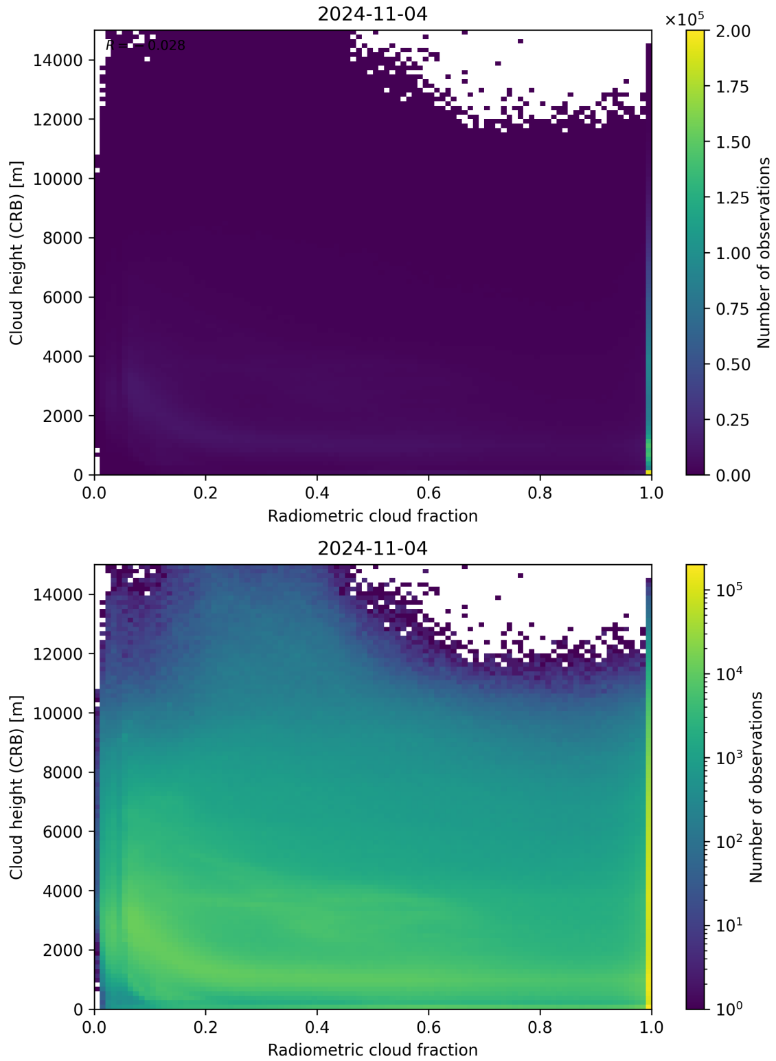
Figure 74: Scatter density plot of “Radiometric cloud fraction” against “Cloud height (CRB)” for 2024-11-04 to 2024-11-05.
