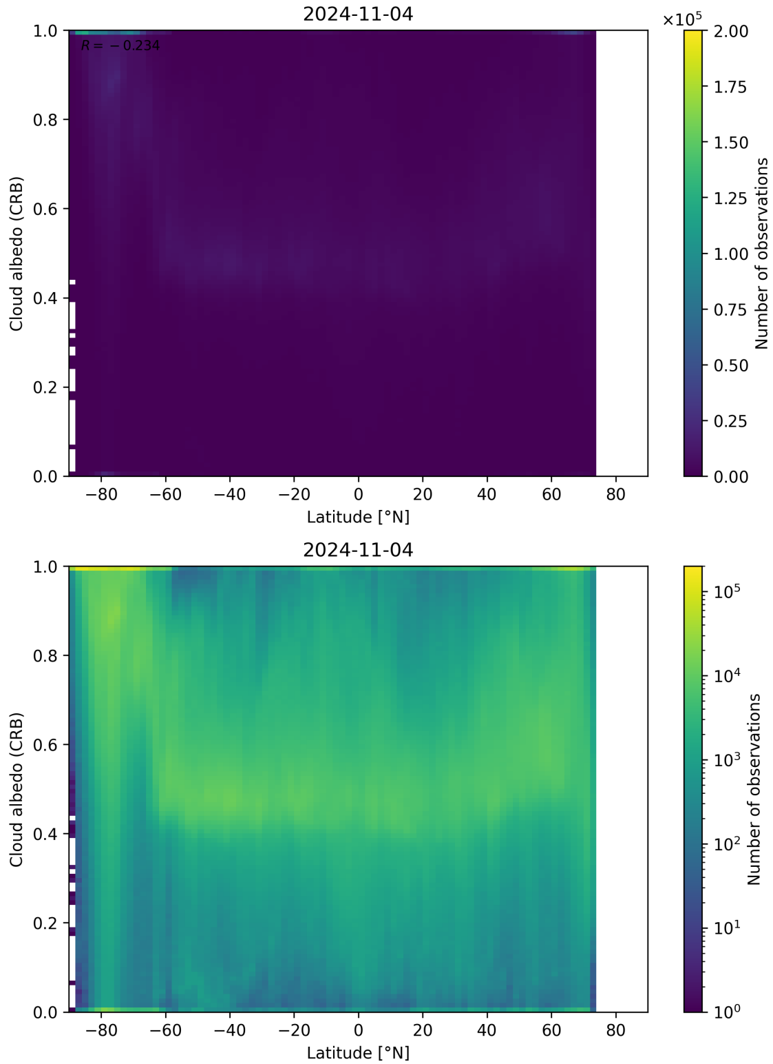
Figure 91: Scatter density plot of “Latitude” against “Cloud albedo (CRB)” for 2024-11-04 to 2024-11-05.
