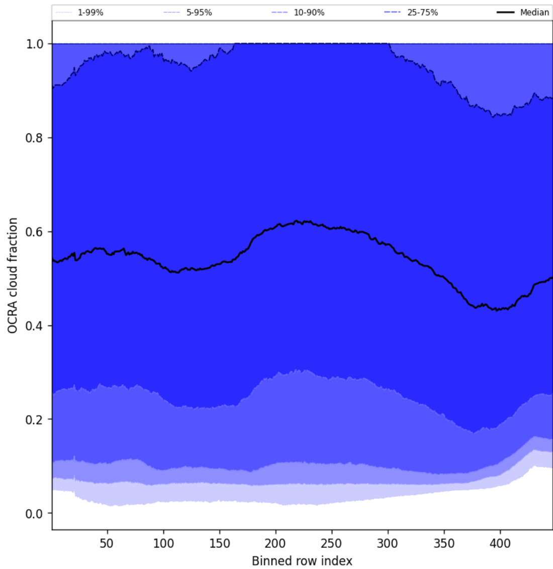
Figure 66: Along track statistics of “OCRA cloud fraction” for 2024-11-04 to 2024-11-05
