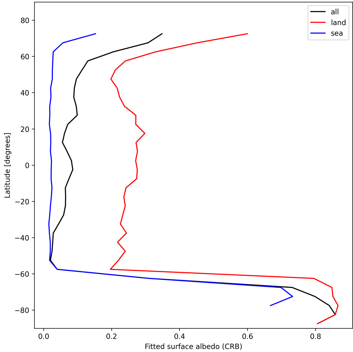
Figure 30: Zonal average of “Fitted surface albedo (CRB)” for 2024-11-04 to 2024-11-05.
