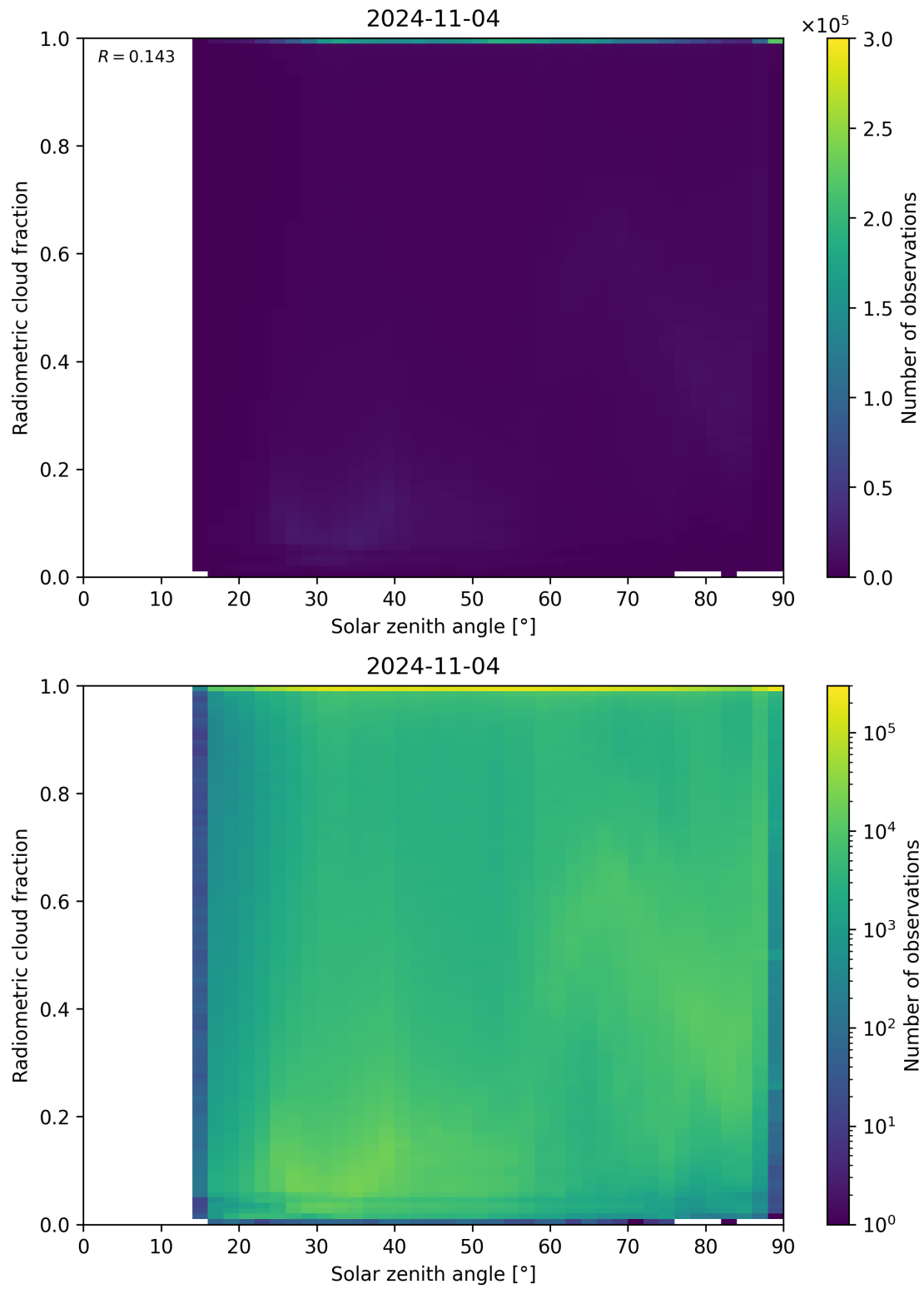
Figure 99: Scatter density plot of “Solar zenith angle” against “Radiometric cloud fraction” for 2024-11-04 to 2024-11-05.
