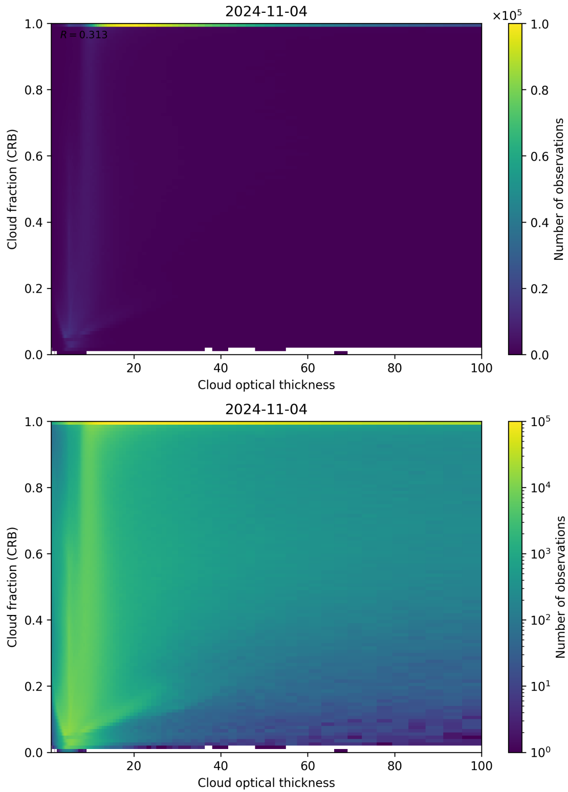
Figure 84: Scatter density plot of “Cloud optical thickness” against “Cloud fraction (CRB)” for 2024-11-04 to 2024-11-05.
