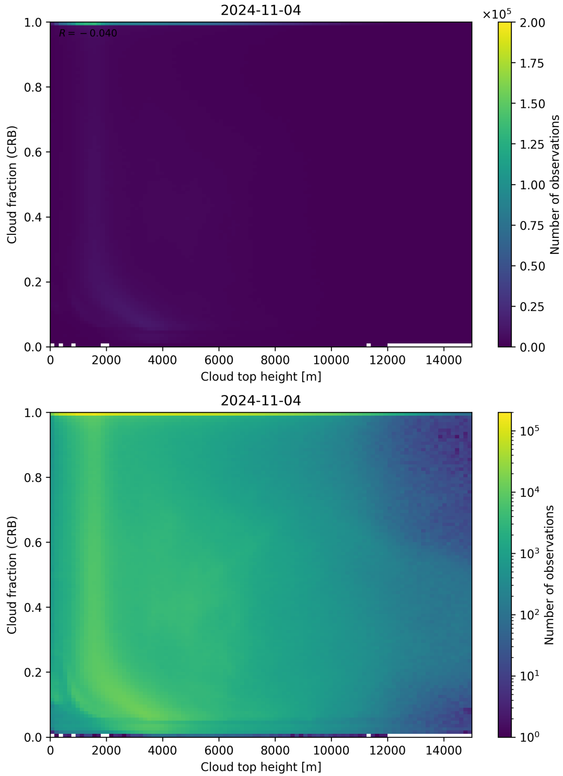
Figure 88: Scatter density plot of “Cloud top height” against “Cloud fraction (CRB)” for 2024-11-04 to 2024-11-05.
