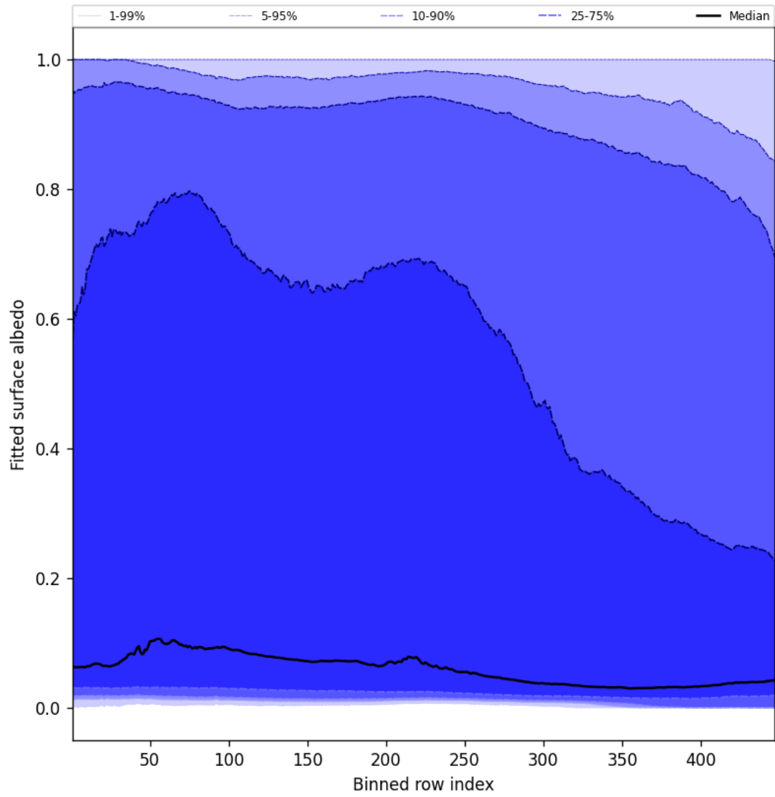
Figure 61: Along track statistics of “Fitted surface albedo” for 2024-11-04 to 2024-11-05
