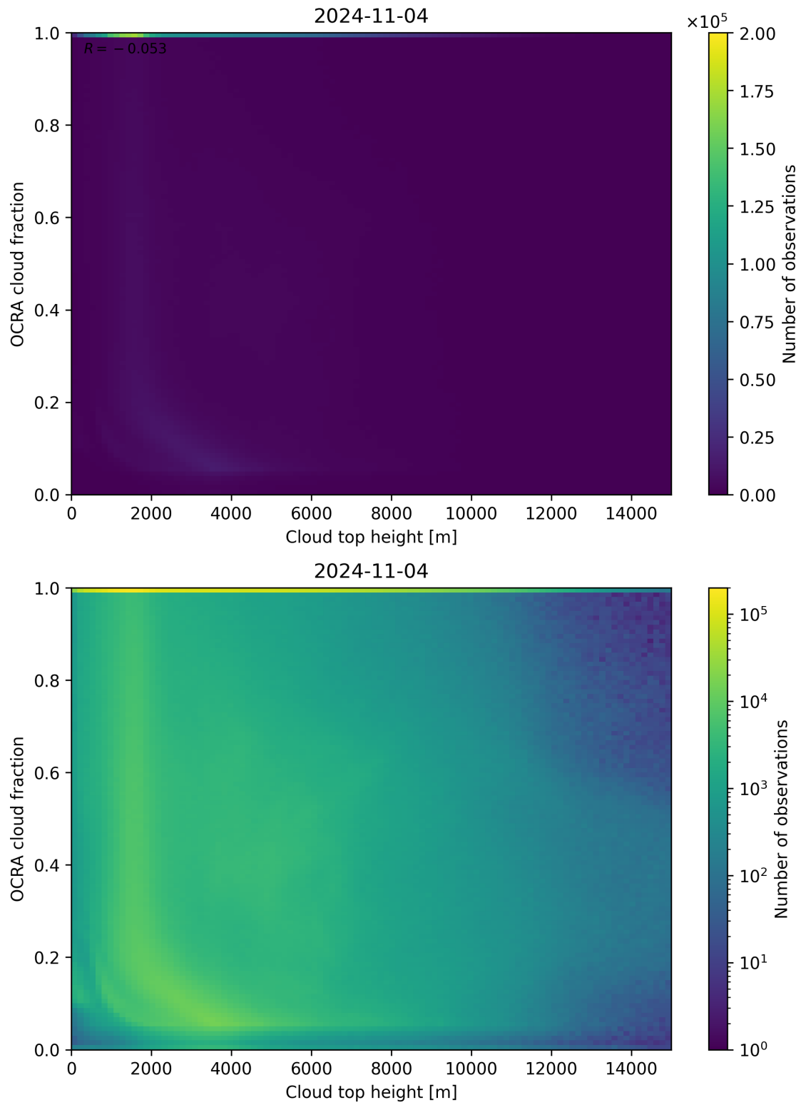
Figure 87: Scatter density plot of “Cloud top height” against “OCRA cloud fraction” for 2024-11-04 to 2024-11-05.
