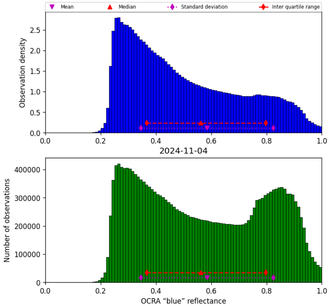
Figure 51: Histogram of “OCRA “blue” reflectance” for 2024-11-04 to 2024-11-05
