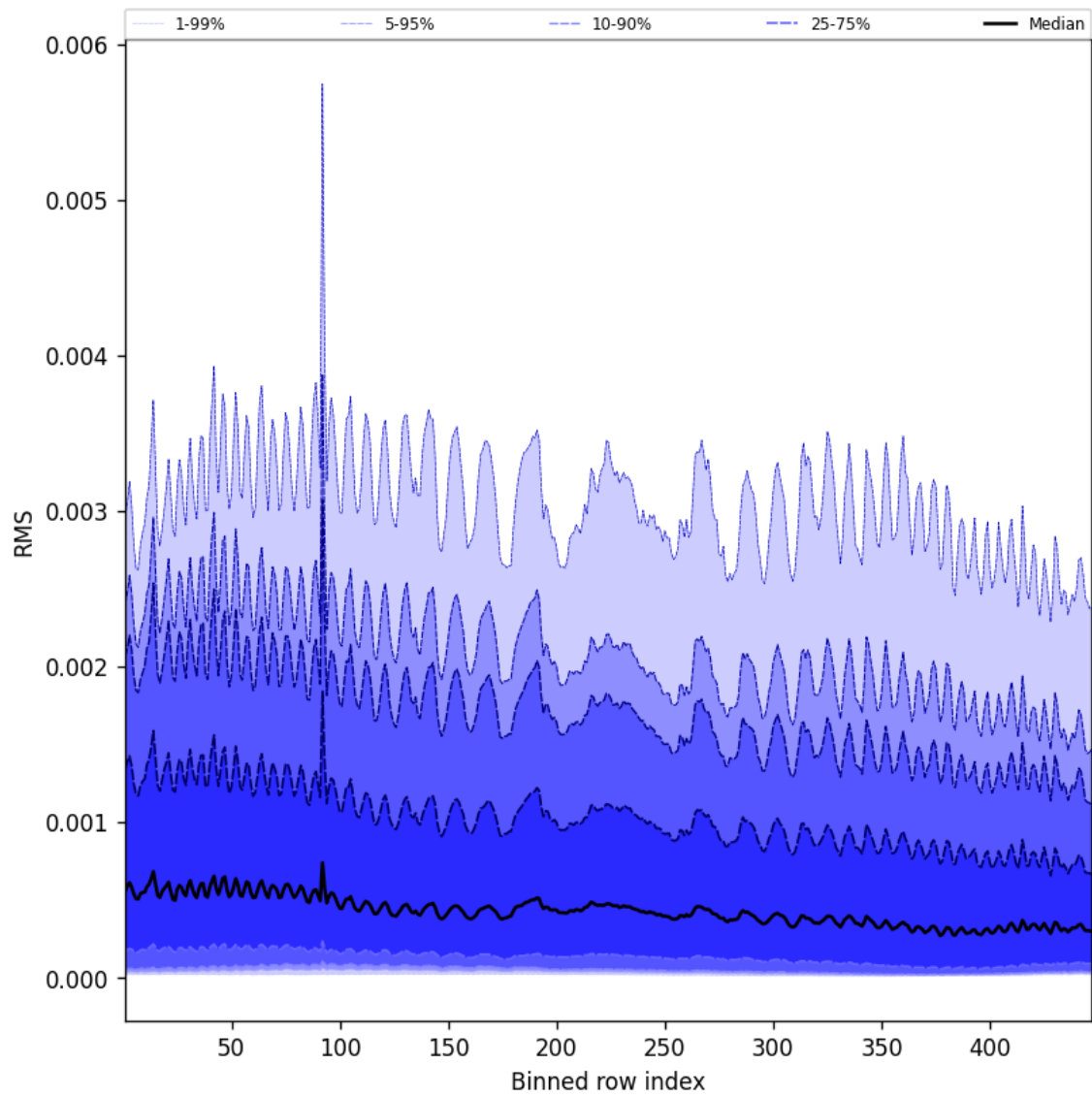
Figure 63: Along track statistics of “RMS” for 2024-11-04 to 2024-11-05
