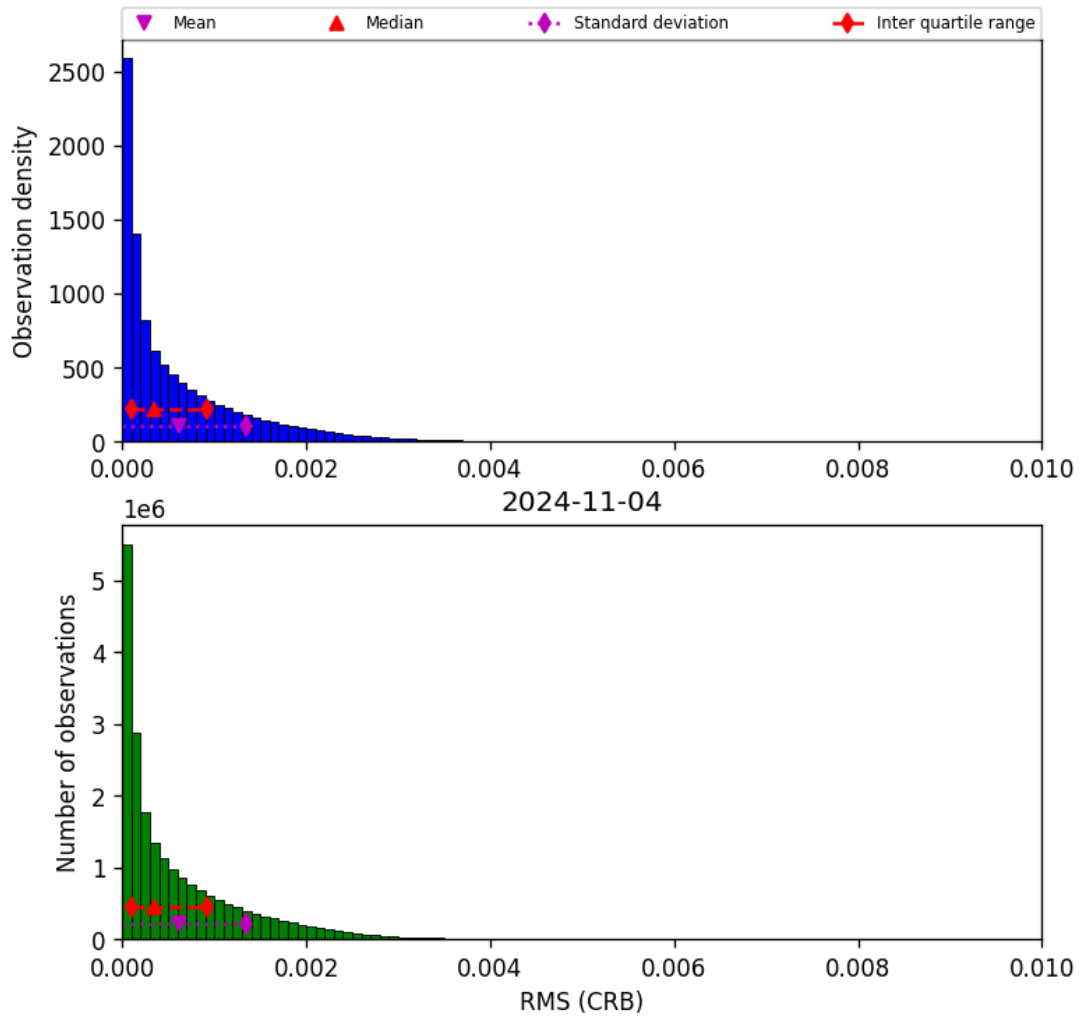
Figure 48: Histogram of “RMS (CRB)” for 2024-11-04 to 2024-11-05
