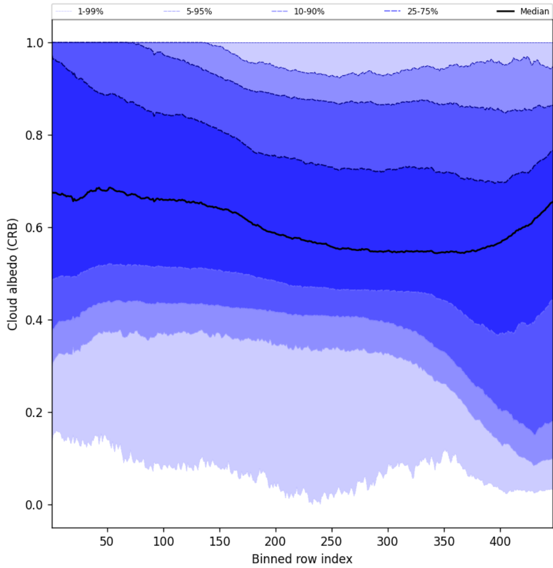
Figure 60: Along track statistics of “Cloud albedo (CRB)” for 2024-11-04 to 2024-11-05
