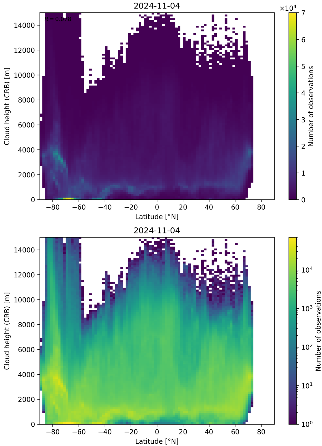
Figure 95: Scatter density plot of “Latitude” against “Cloud height (CRB)” for 2024-11-04 to 2024-11-05.
