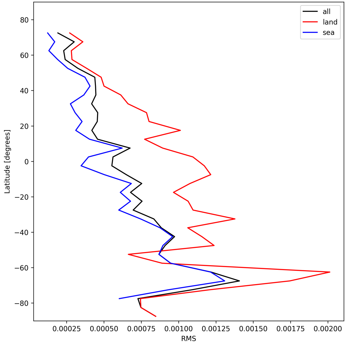
Figure 31: Zonal average of “RMS” for 2024-11-04 to 2024-11-05.
