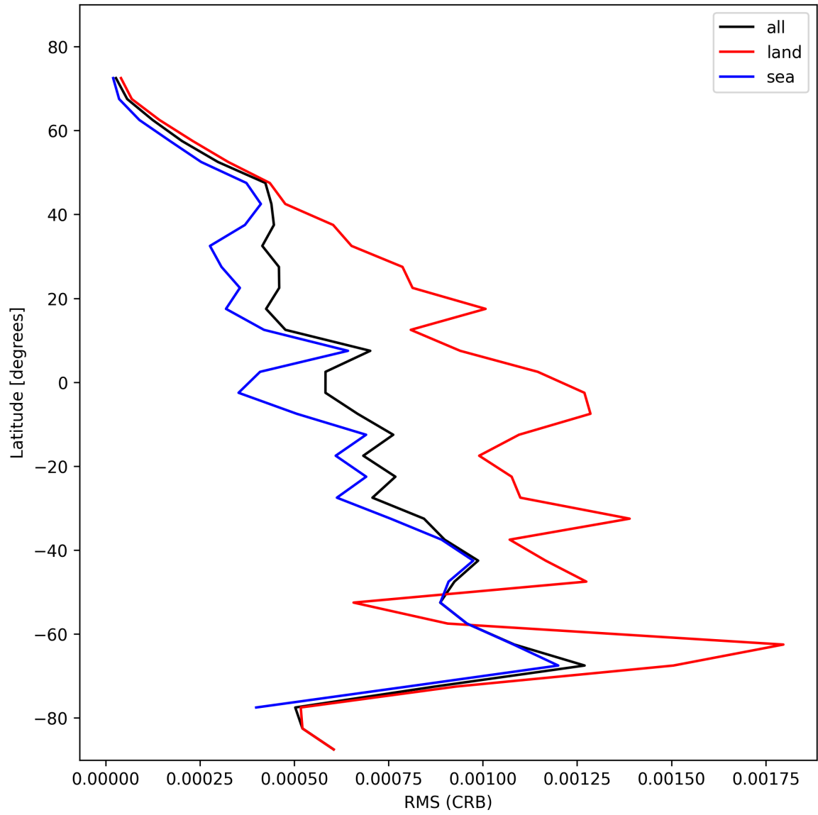
Figure 32: Zonal average of “RMS (CRB)” for 2024-11-04 to 2024-11-05.
