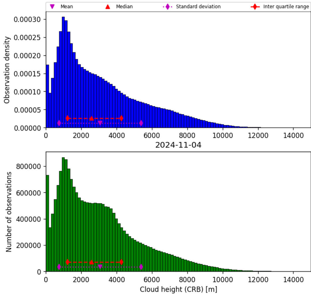
Figure 43: Histogram of “Cloud height (CRB)” for 2024-11-04 to 2024-11-05
