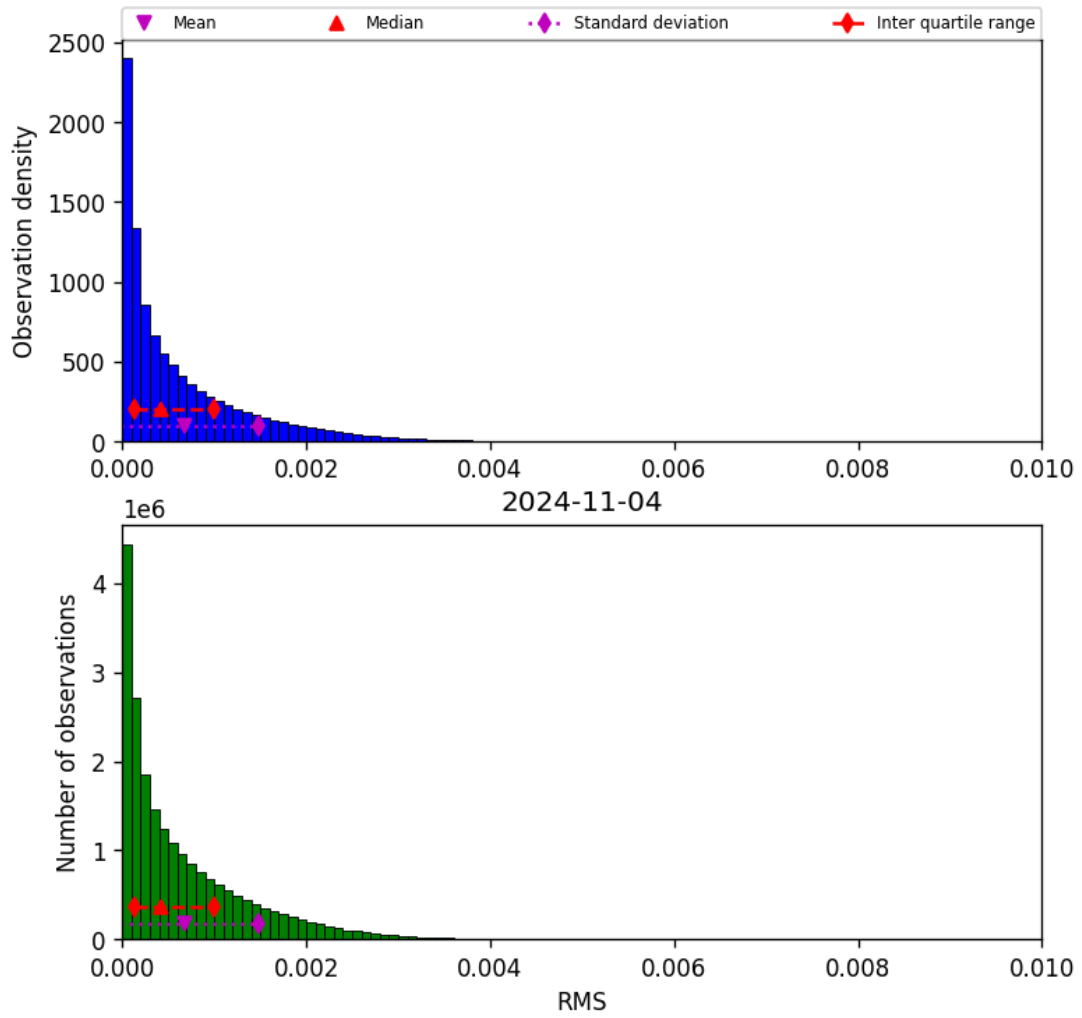
Figure 47: Histogram of “RMS” for 2024-11-04 to 2024-11-05
