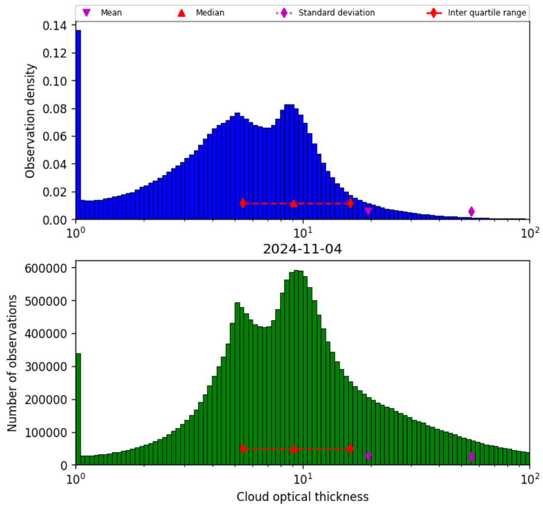
Figure 41: Histogram of “Cloud optical thickness” for 2024-11-04 to 2024-11-05
