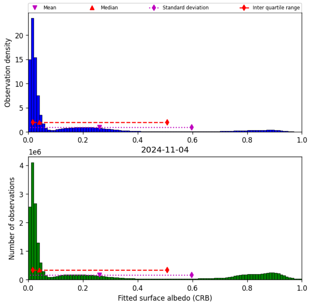
Figure 46: Histogram of “Fitted surface albedo (CRB)” for 2024-11-04 to 2024-11-05
