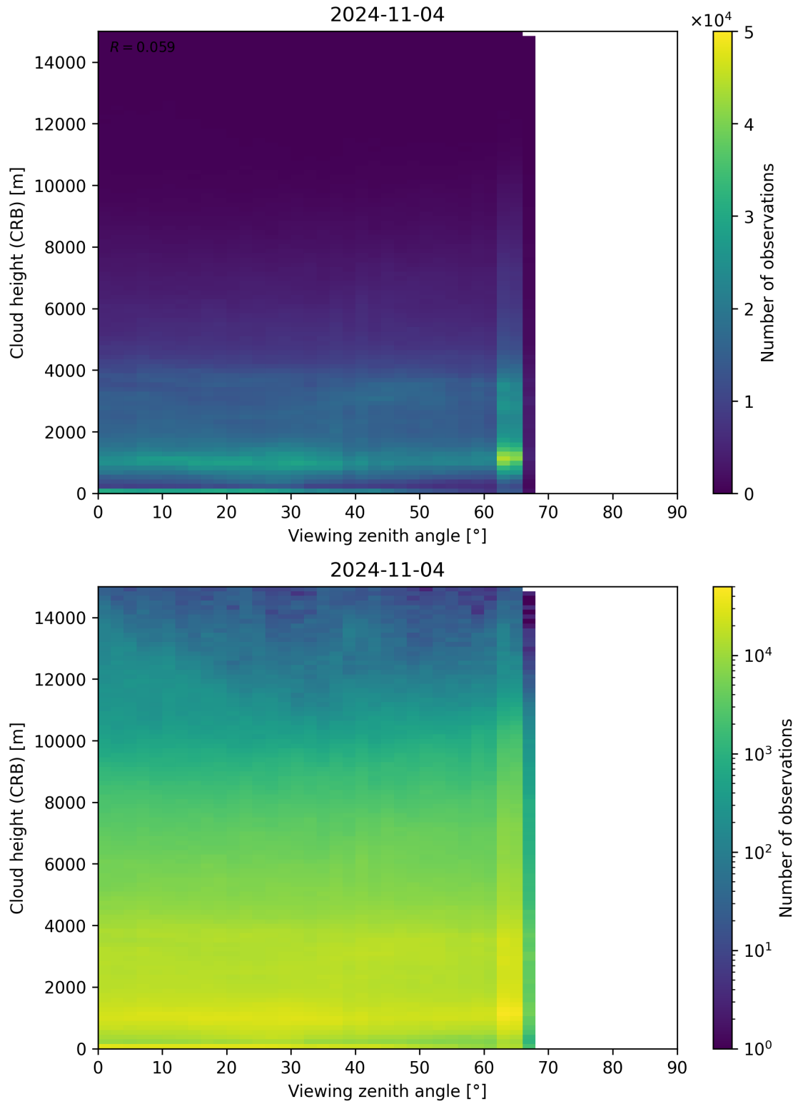
Figure 110: Scatter density plot of “Viewing zenith angle” against “Cloud height (CRB)” for 2024-11-04 to 2024-11-05.
