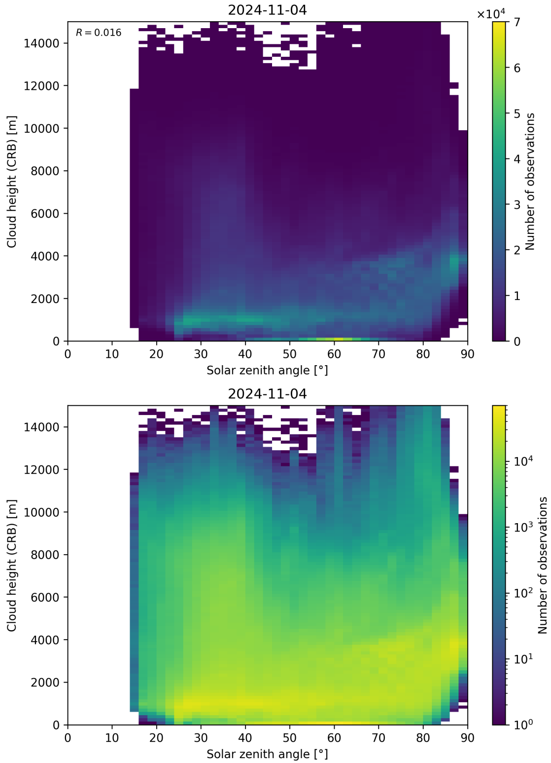
Figure 102: Scatter density plot of “Solar zenith angle” against “Cloud height (CRB)” for 2024-11-04 to 2024-11-05.
