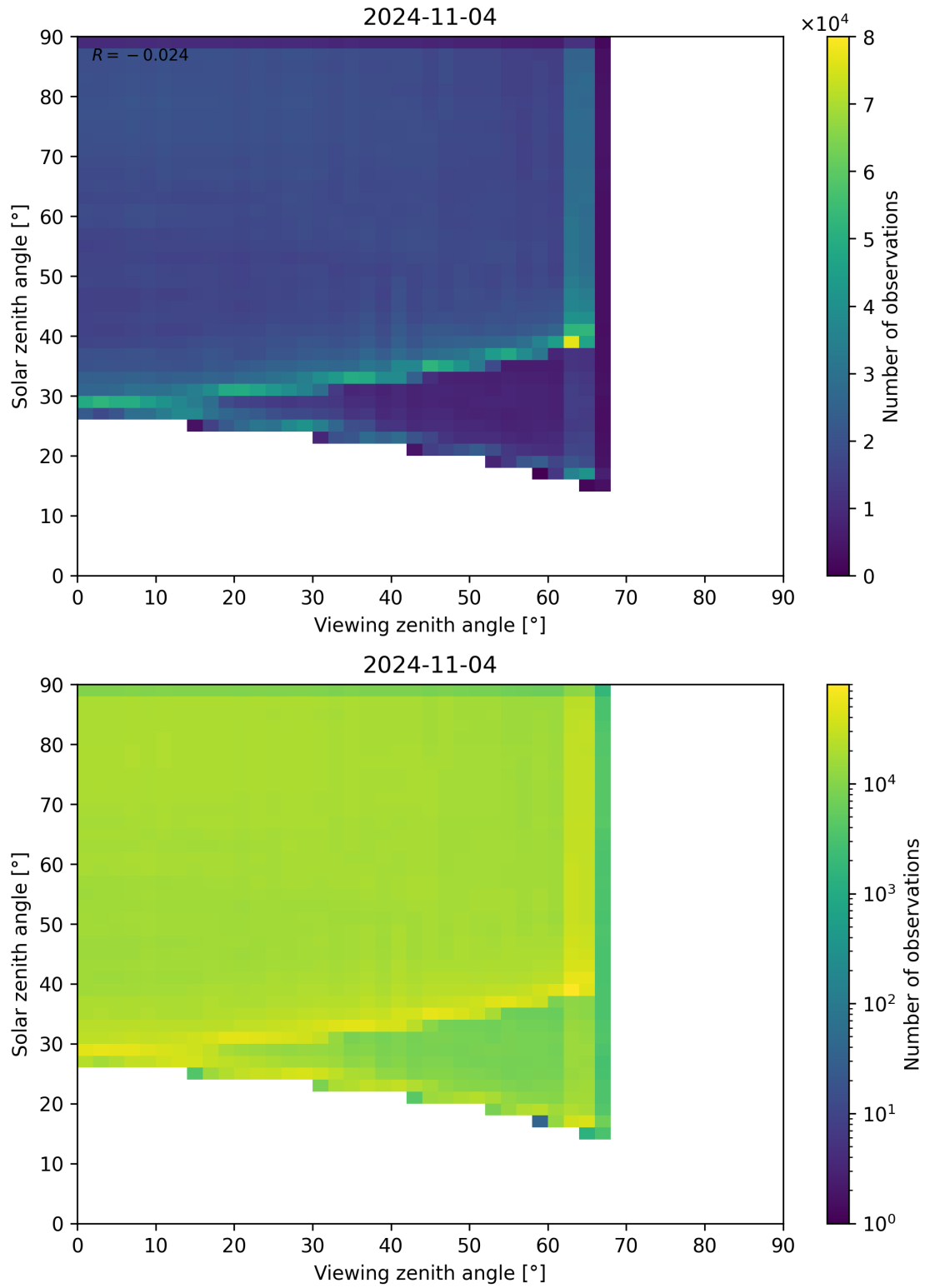
Figure 114: Scatter density plot of “Viewing zenith angle” against “Solar zenith angle” for 2024-11-04 to 2024-11-05.
