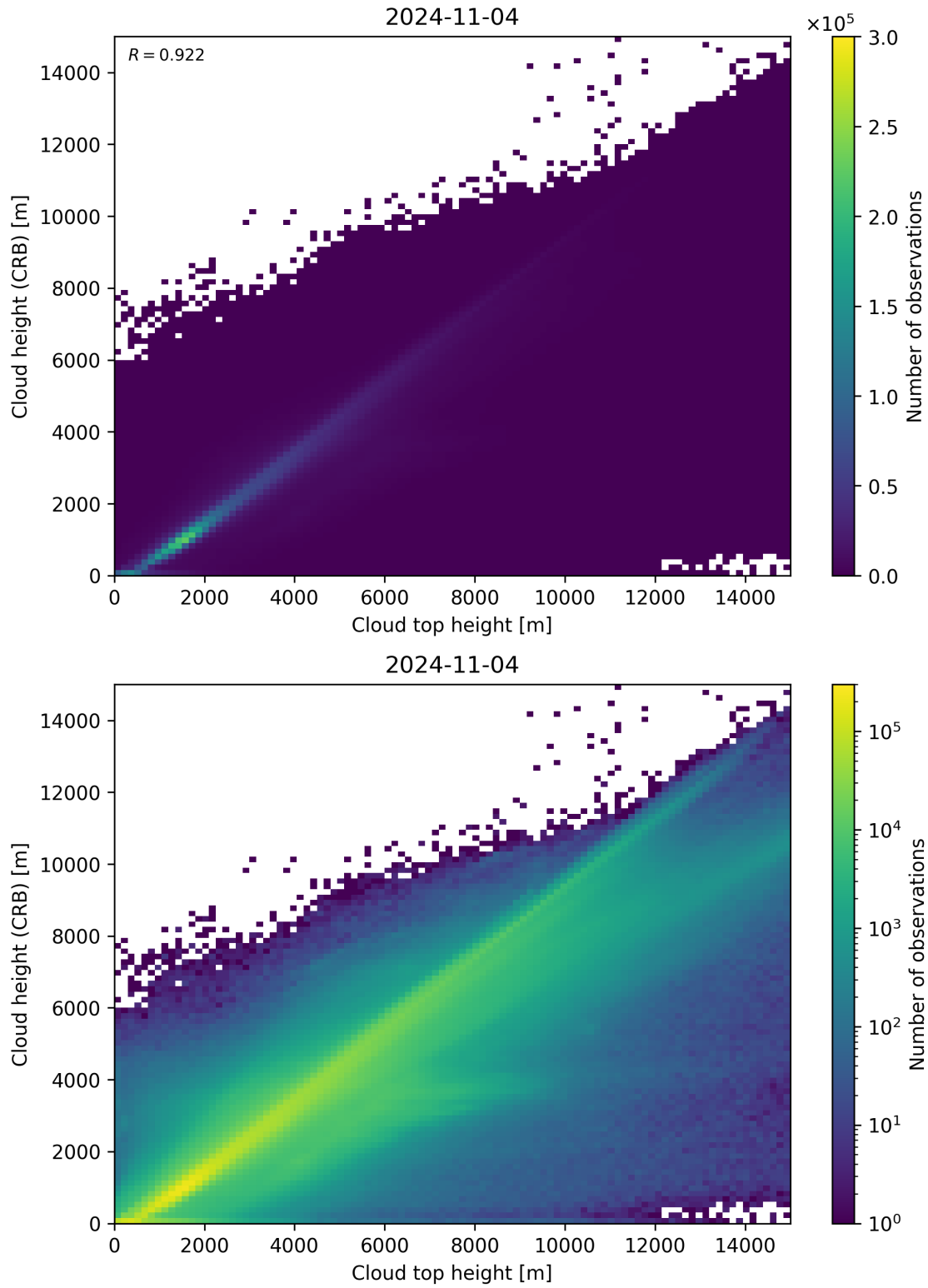
Figure 89: Scatter density plot of “Cloud top height” against “Cloud height (CRB)” for 2024-11-04 to 2024-11-05.
