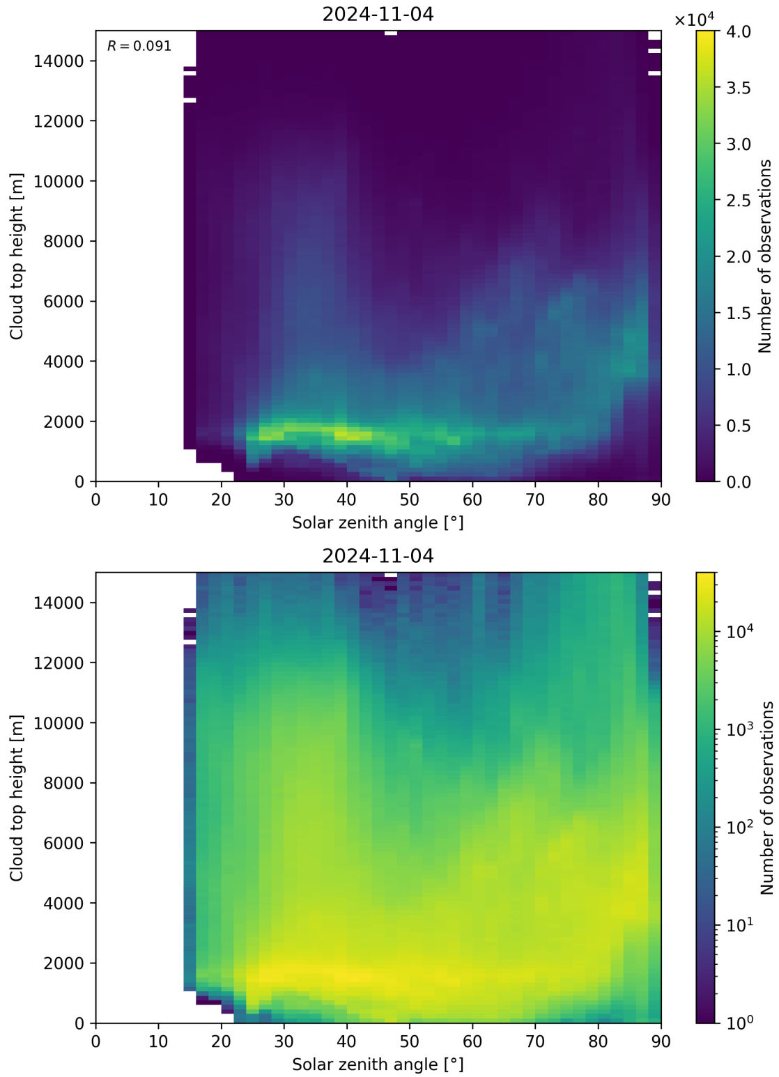
Figure 104: Scatter density plot of “Solar zenith angle” against “Cloud top height” for 2024-11-04 to 2024-11-05.
