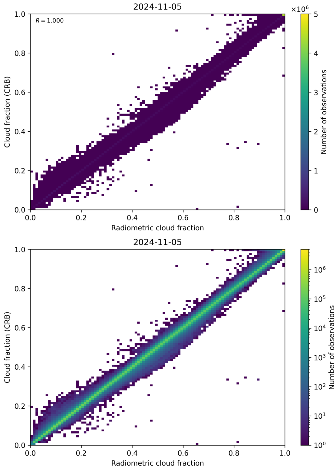
Figure 73: Scatter density plot of “Radiometric cloud fraction” against “Cloud fraction (CRB)” for 2024-11-04 to 2024-11-06.
