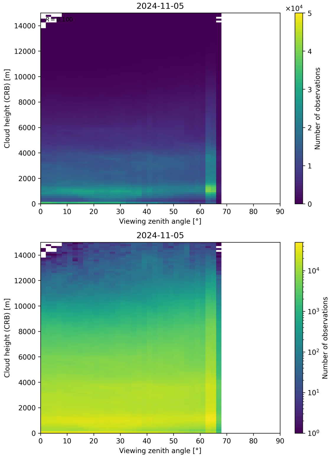
Figure 110: Scatter density plot of “Viewing zenith angle” against “Cloud height (CRB)” for 2024-11-04 to 2024-11-06.
