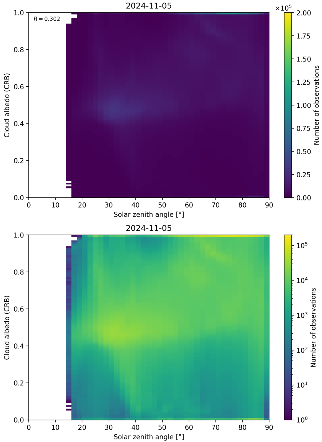
Figure 98: Scatter density plot of “Solar zenith angle” against “Cloud albedo (CRB)” for 2024-11-04 to 2024-11-06.
