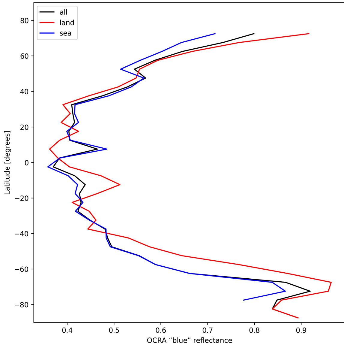
Figure 35: Zonal average of “OCRA “blue” reflectance” for 2024-11-04 to 2024-11-06.
