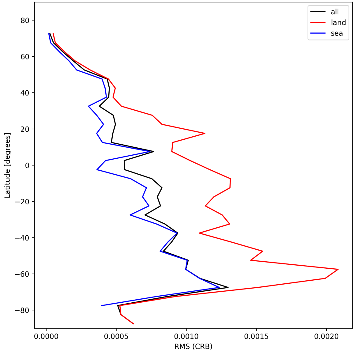
Figure 32: Zonal average of “RMS (CRB)” for 2024-11-04 to 2024-11-06.
