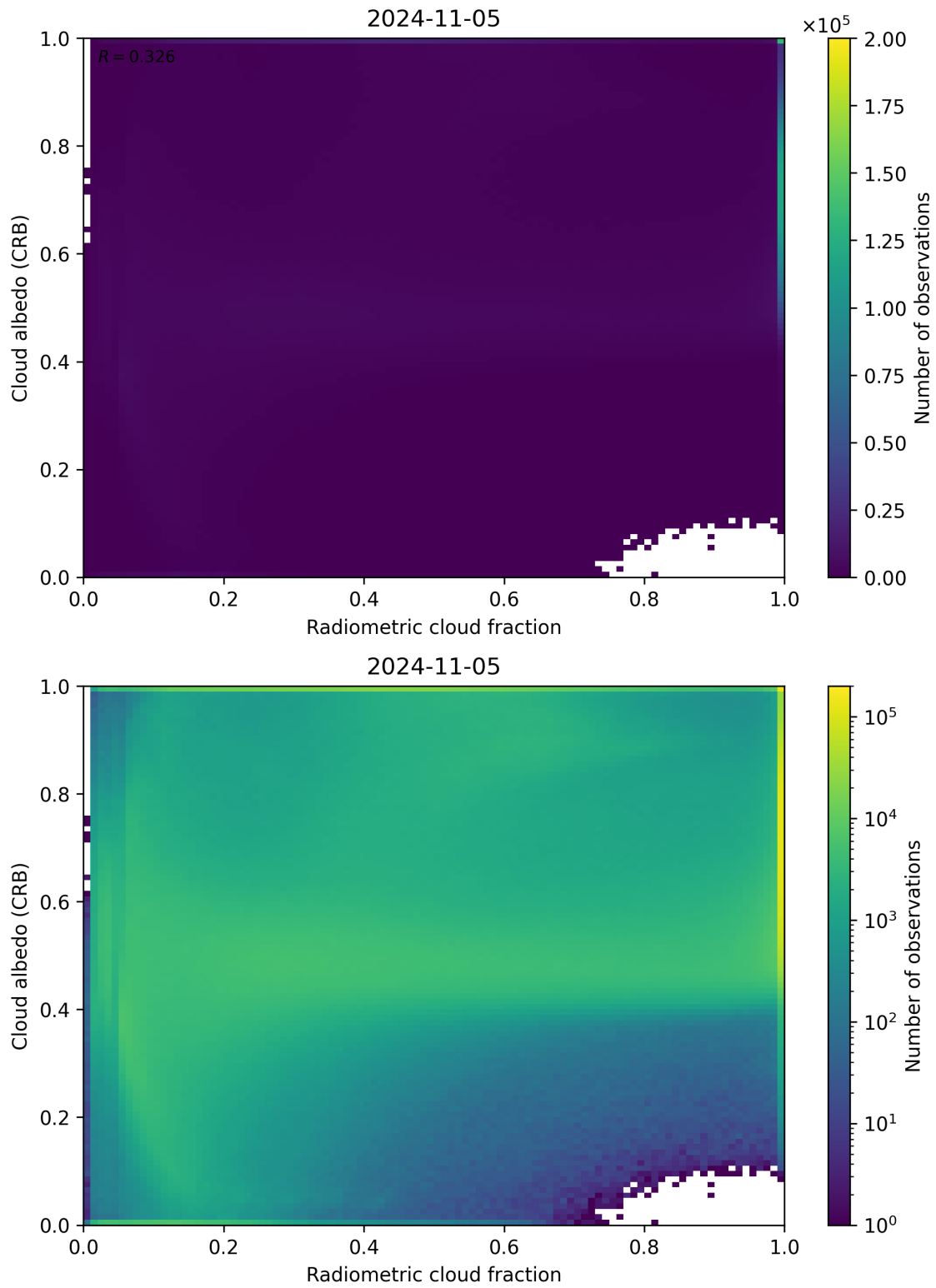
Figure 71: Scatter density plot of “Radiometric cloud fraction” against “Cloud albedo (CRB)” for 2024-11-04 to 2024-11-06.
