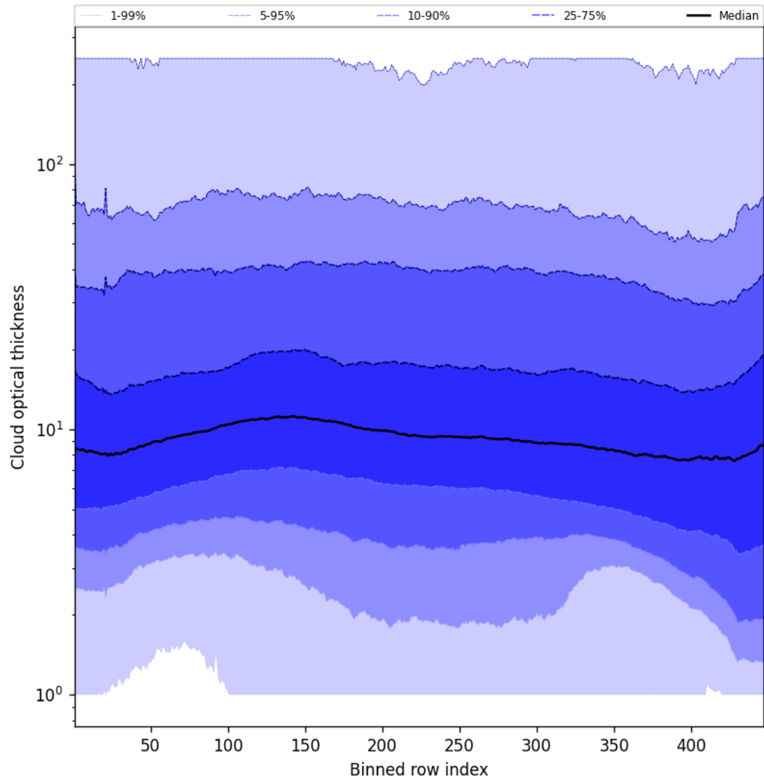
Figure 57: Along track statistics of “Cloud optical thickness” for 2024-11-04 to 2024-11-06
