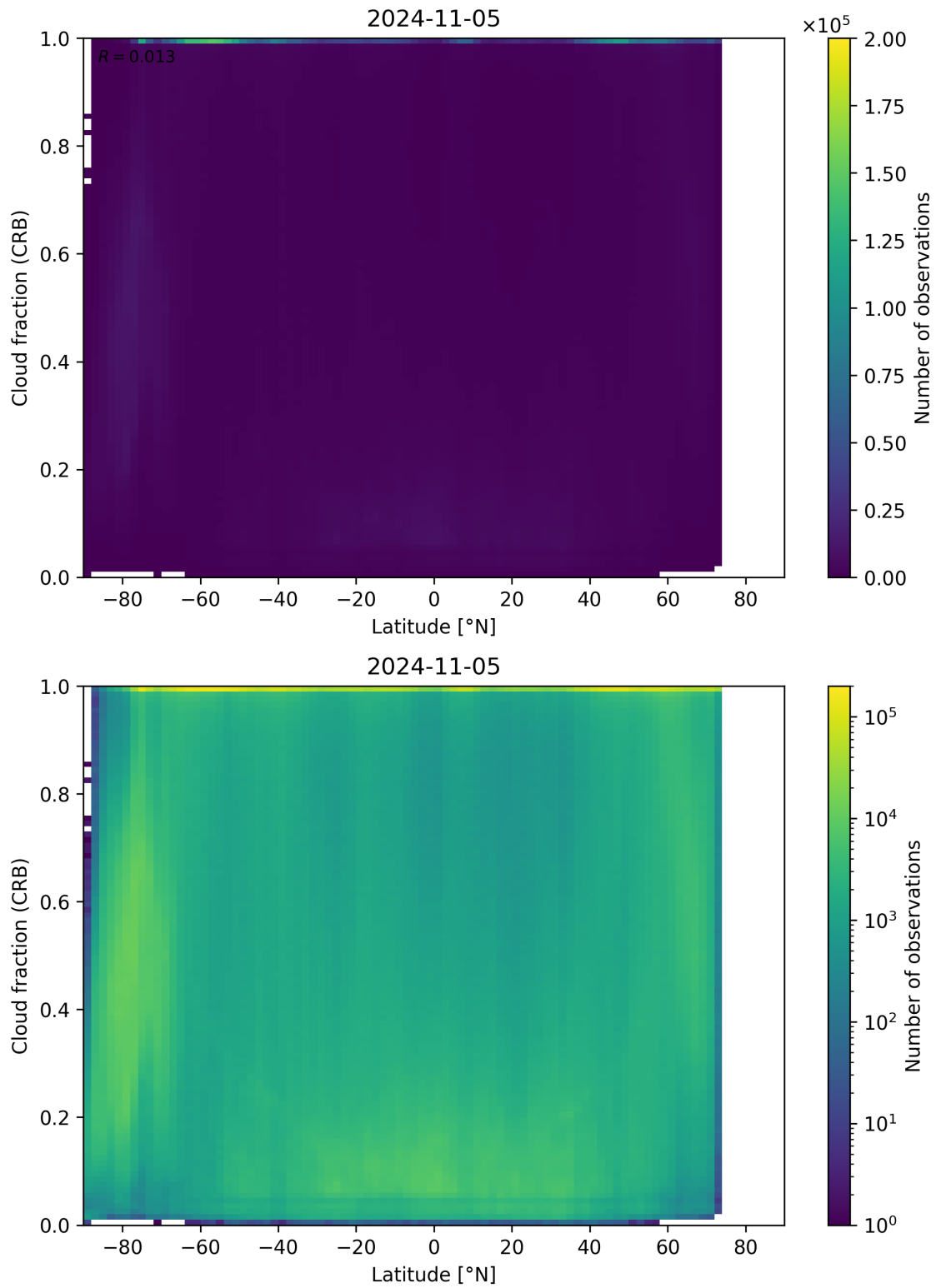
Figure 94: Scatter density plot of “Latitude” against “Cloud fraction (CRB)” for 2024-11-04 to 2024-11-06.
