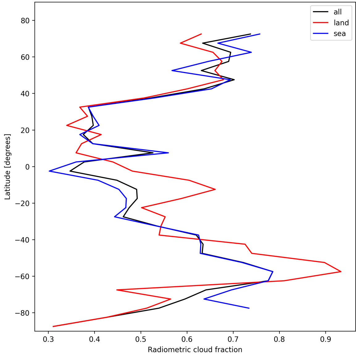
Figure 23: Zonal average of “Radiometric cloud fraction” for 2024-11-04 to 2024-11-06.
