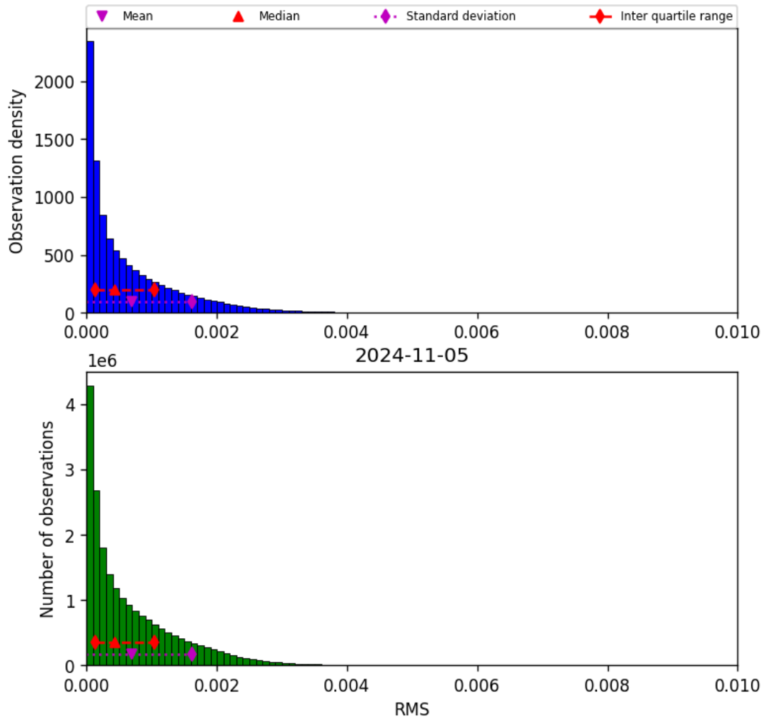
Figure 47: Histogram of “RMS” for 2024-11-04 to 2024-11-06
