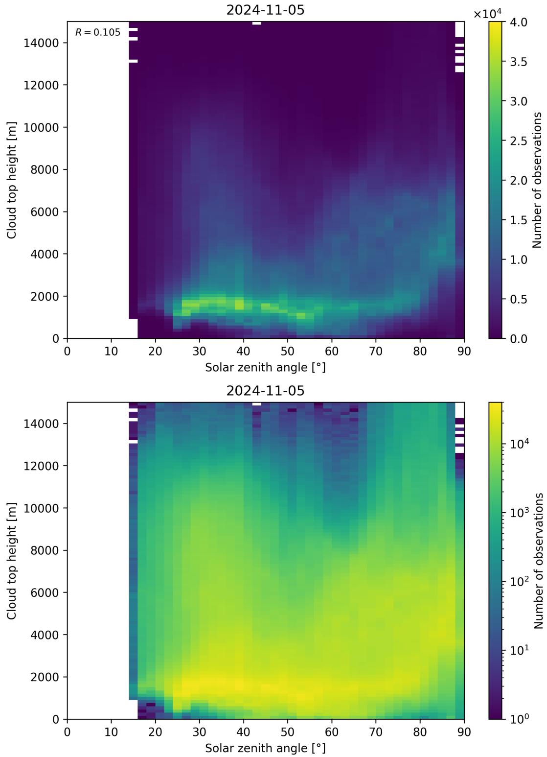
Figure 104: Scatter density plot of “Solar zenith angle” against “Cloud top height” for 2024-11-04 to 2024-11-06.
