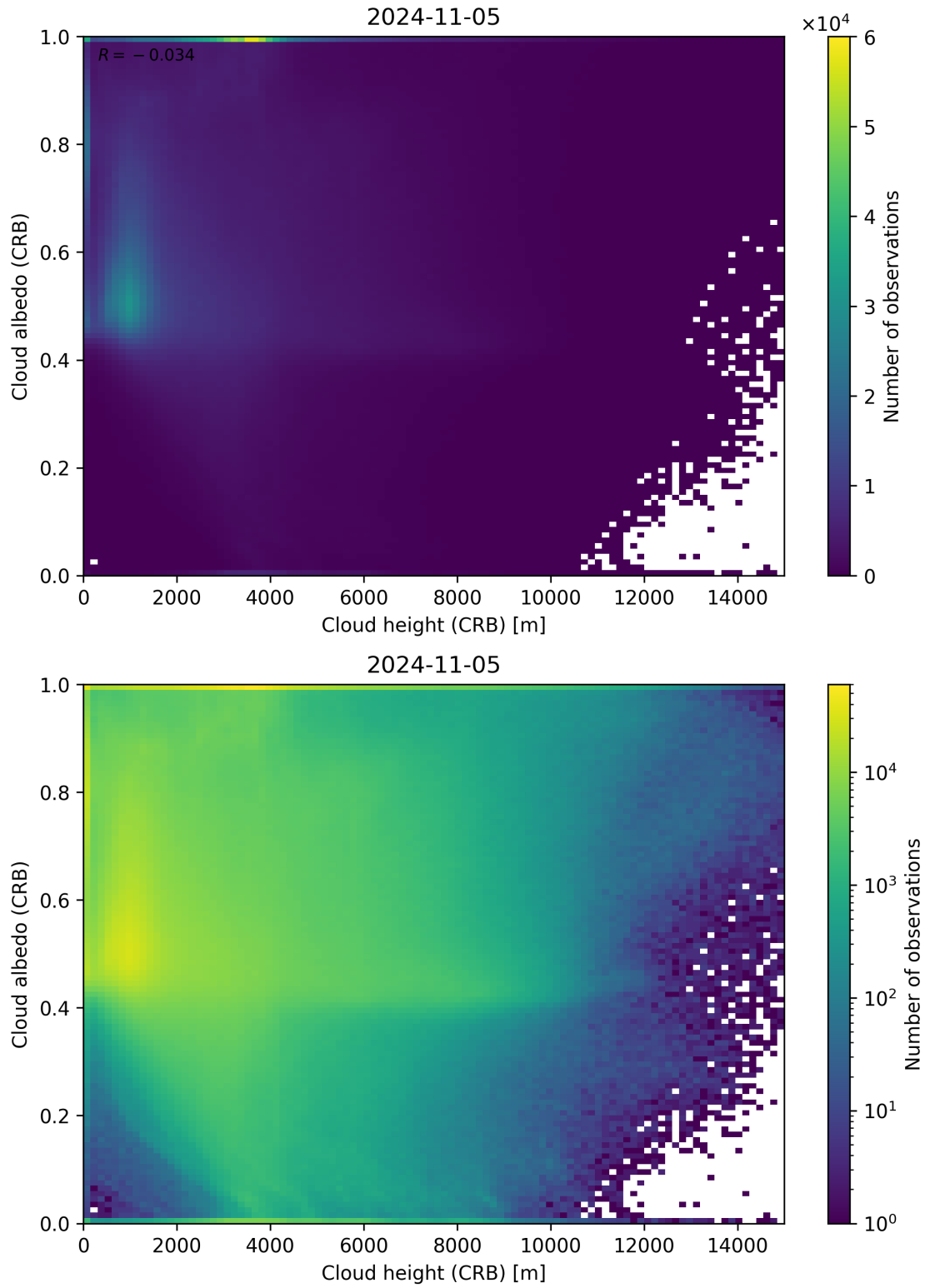
Figure 80: Scatter density plot of “Cloud height (CRB)” against “Cloud albedo (CRB)” for 2024-11-04 to 2024-11-06.
