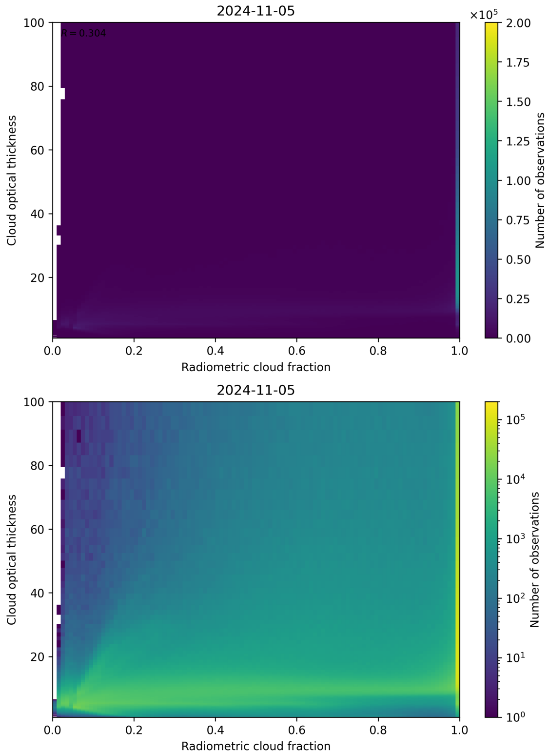
Figure 75: Scatter density plot of “Radiometric cloud fraction” against “Cloud optical thickness” for 2024-11-04 to 2024-11-06.
