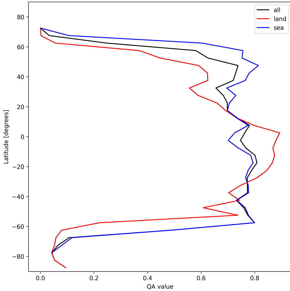
Figure 22: Zonal average of “QA value” for 2024-11-04 to 2024-11-06.
