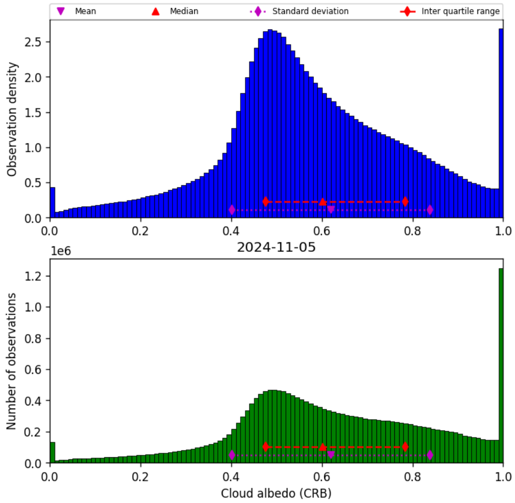
Figure 44: Histogram of “Cloud albedo (CRB)” for 2024-11-04 to 2024-11-06
