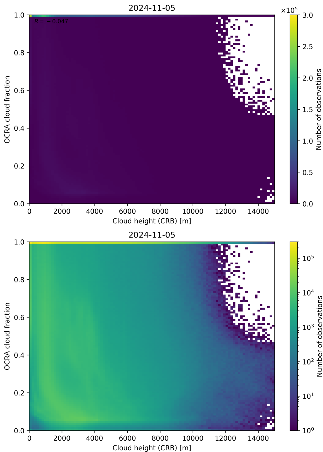
Figure 81: Scatter density plot of “Cloud height (CRB)” against “OCRA cloud fraction” for 2024-11-04 to 2024-11-06.
