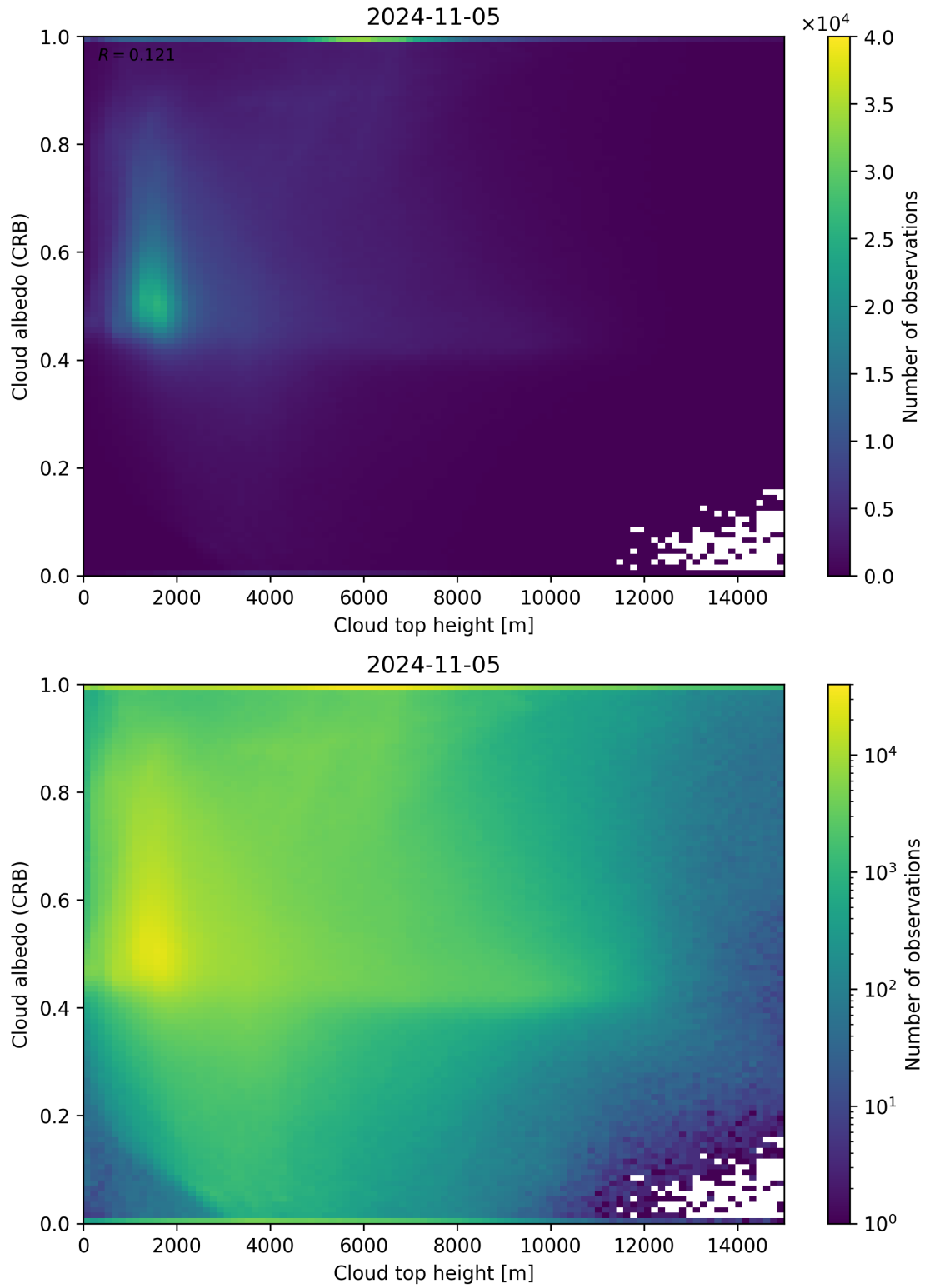
Figure 86: Scatter density plot of “Cloud top height” against “Cloud albedo (CRB)” for 2024-11-04 to 2024-11-06.
