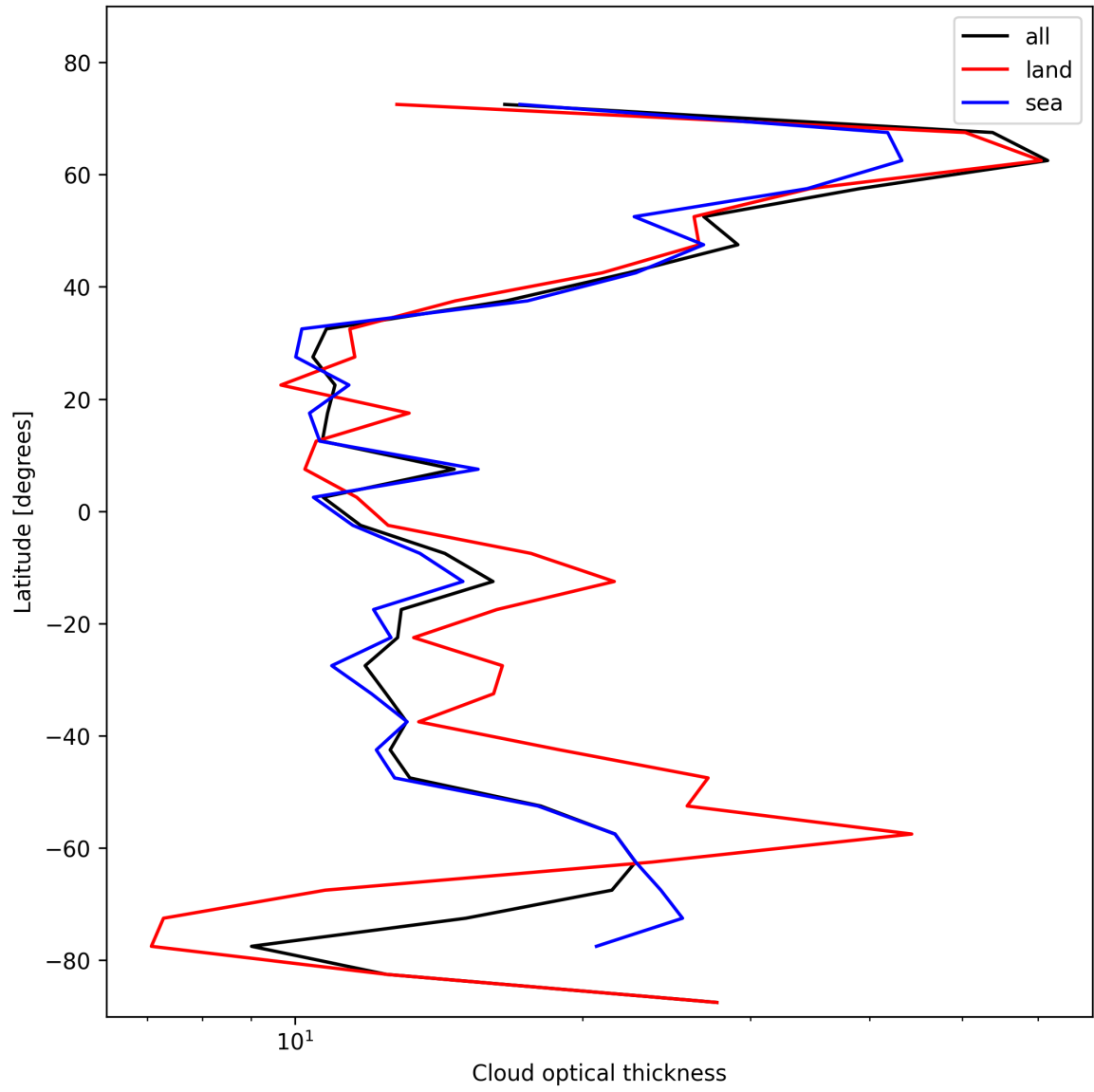
Figure 25: Zonal average of “Cloud optical thickness” for 2024-11-04 to 2024-11-06.
