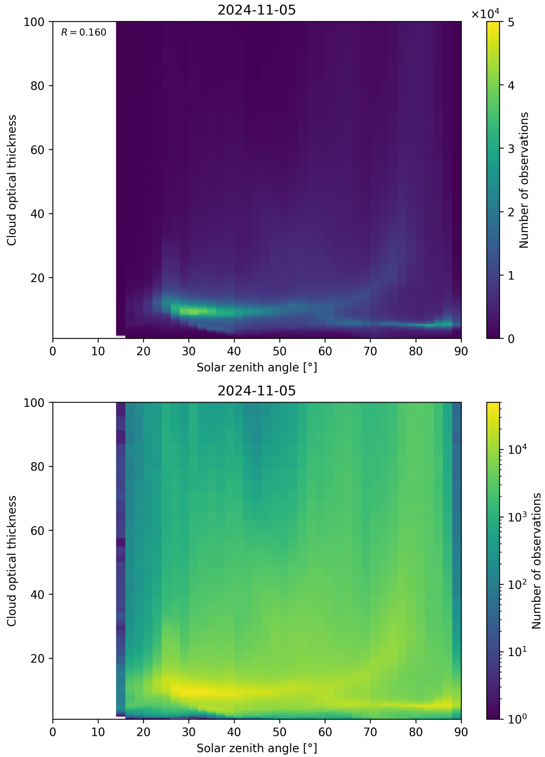
Figure 103: Scatter density plot of “Solar zenith angle” against “Cloud optical thickness” for 2024-11-04 to 2024-11-06.
