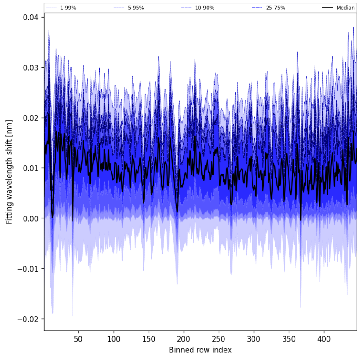
Figure 65: Along track statistics of “Fitting wavelength shift” for 2024-11-04 to 2024-11-06
