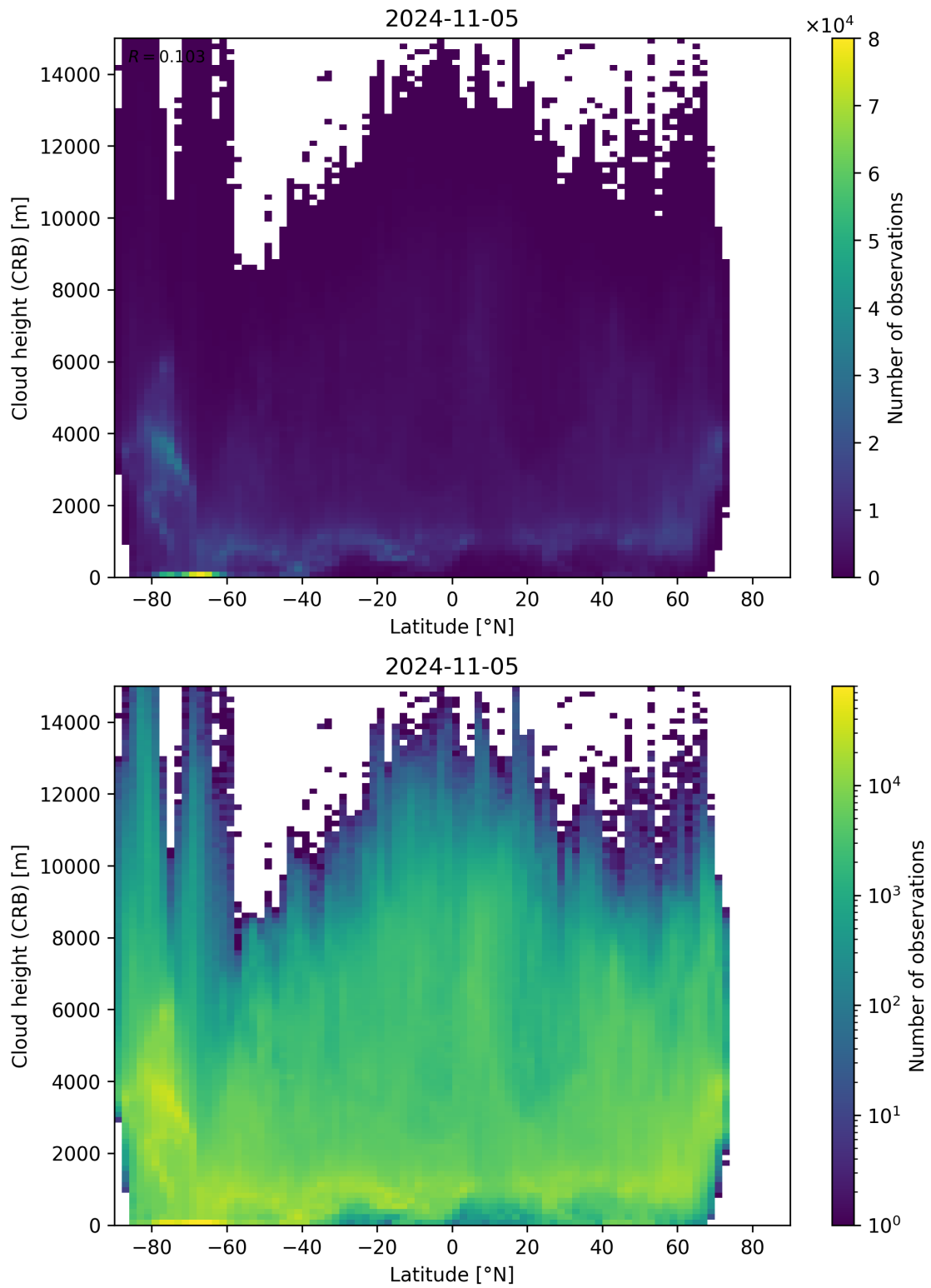
Figure 95: Scatter density plot of “Latitude” against “Cloud height (CRB)” for 2024-11-04 to 2024-11-06.
