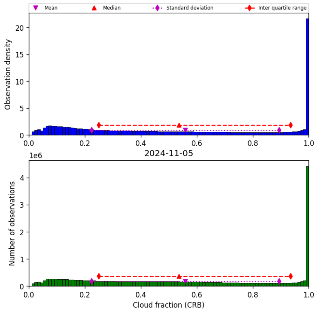
Figure 42: Histogram of “Cloud fraction (CRB)” for 2024-11-04 to 2024-11-06
