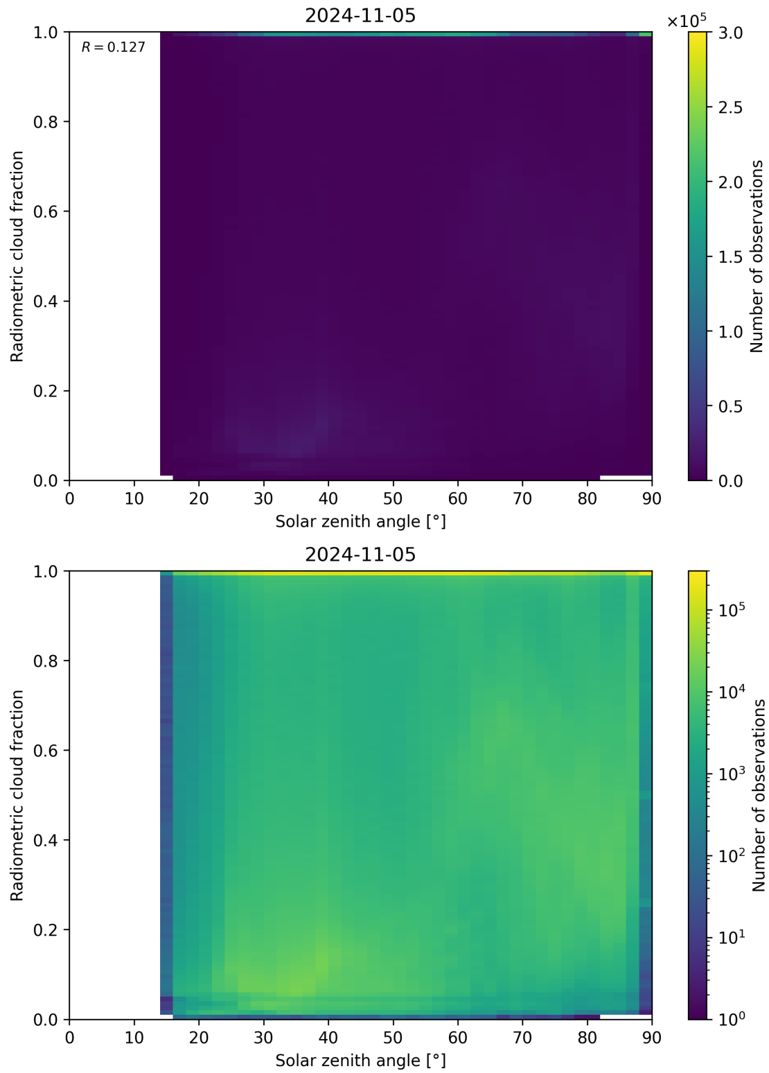
Figure 99: Scatter density plot of “Solar zenith angle” against “Radiometric cloud fraction” for 2024-11-04 to 2024-11-06.
