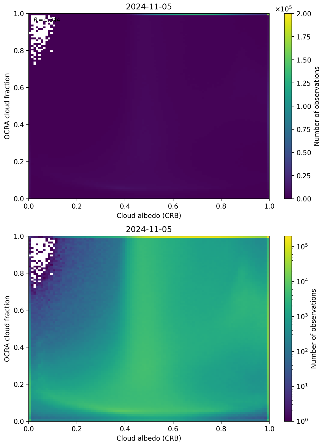
Figure 70: Scatter density plot of “Cloud albedo (CRB)” against “OCRA cloud fraction” for 2024-11-04 to 2024-11-06.
