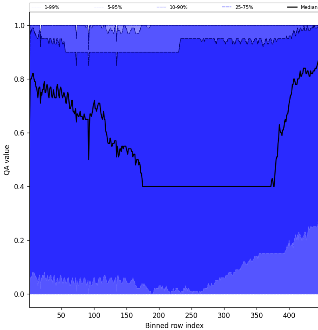
Figure 54: Along track statistics of “QA value” for 2024-11-04 to 2024-11-06
