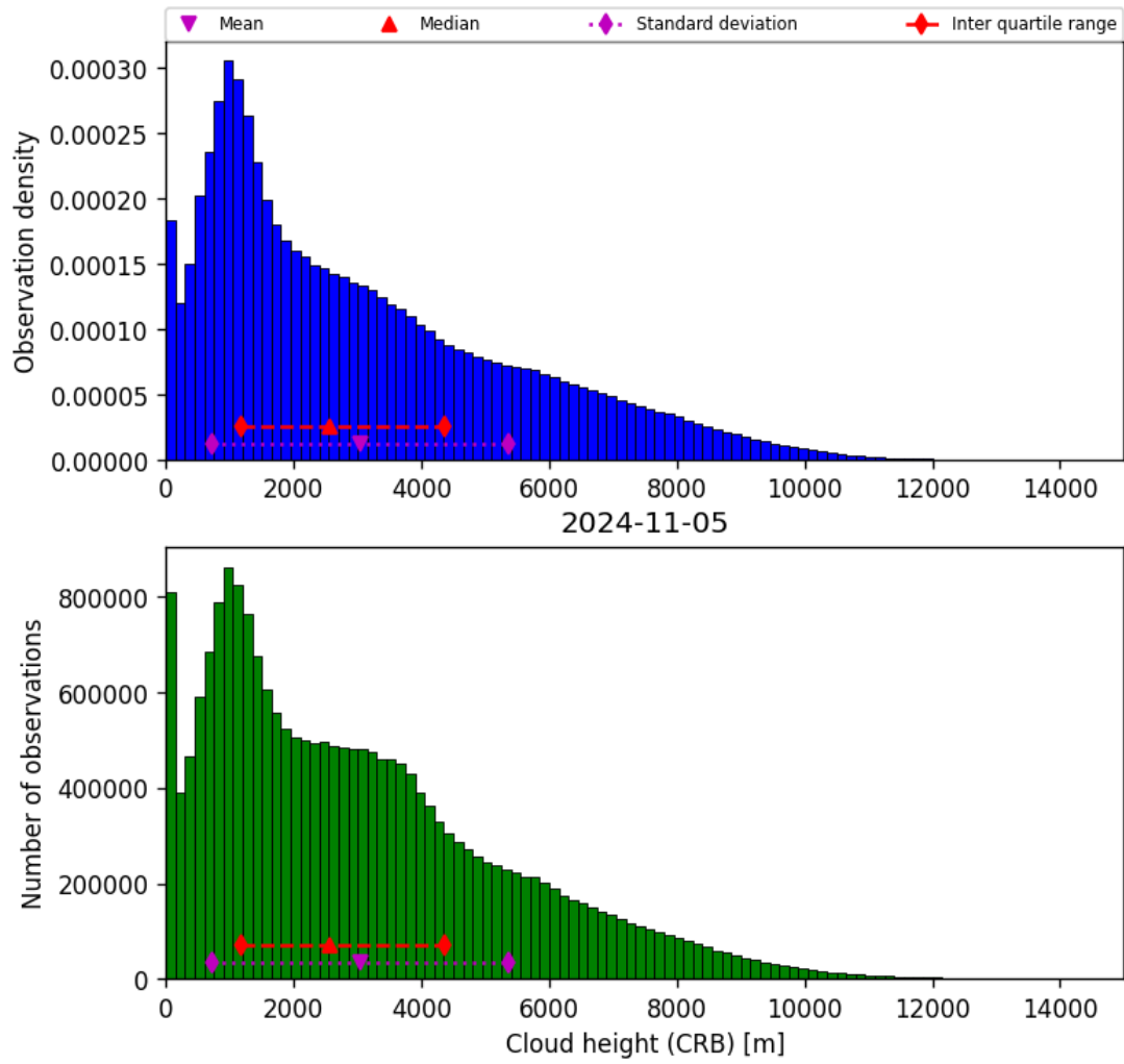
Figure 43: Histogram of “Cloud height (CRB)” for 2024-11-04 to 2024-11-06
