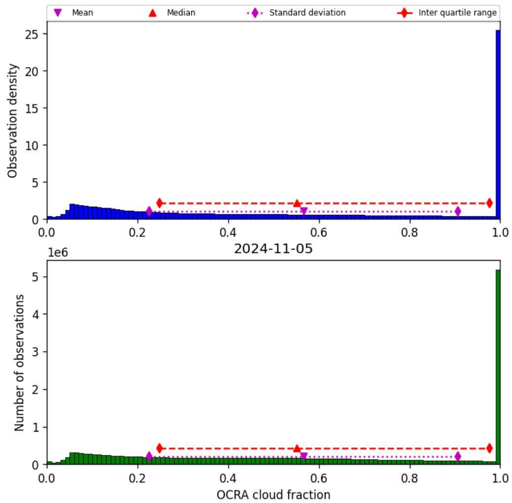
Figure 50: Histogram of “OCRA cloud fraction” for 2024-11-04 to 2024-11-06
