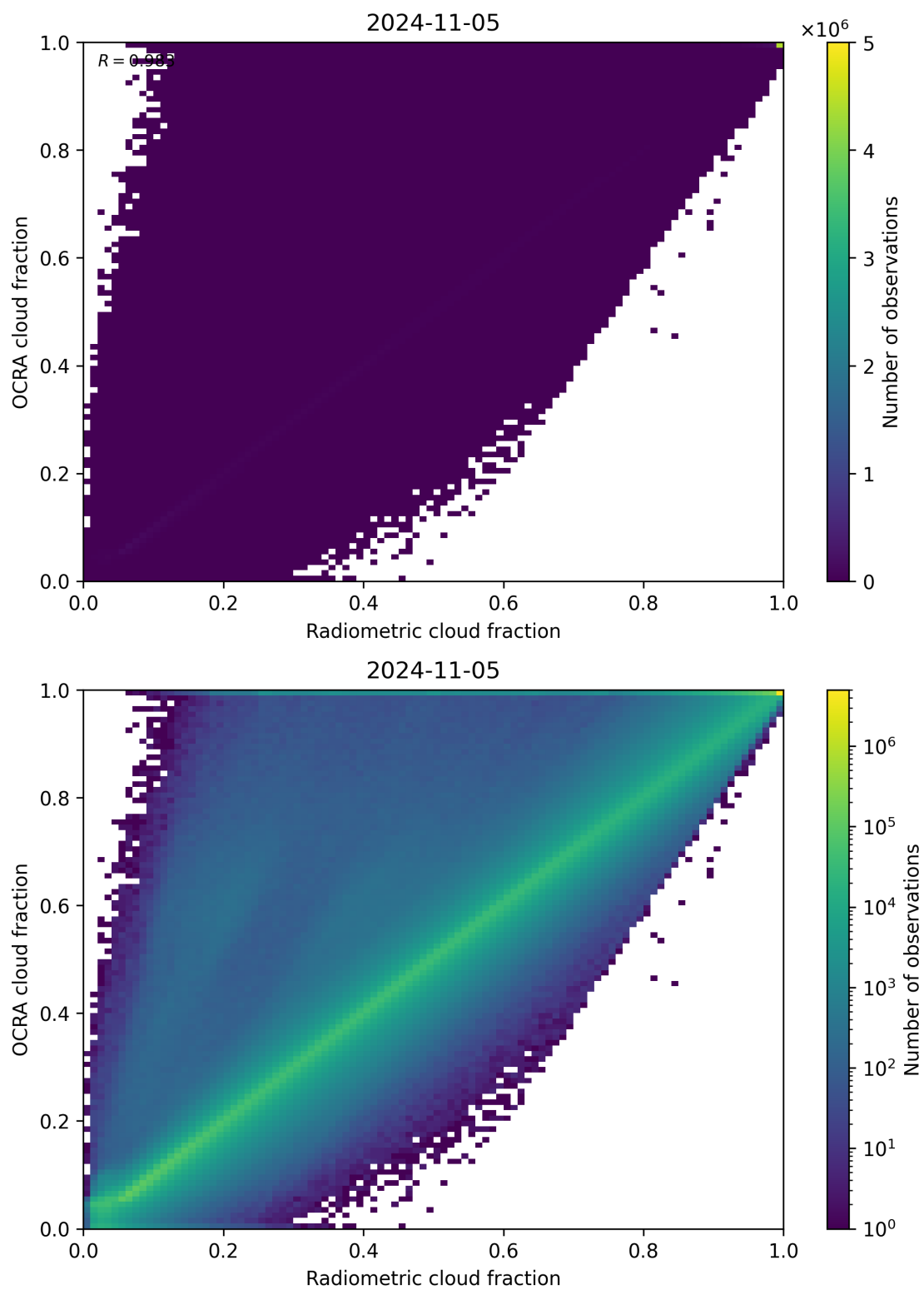
Figure 72: Scatter density plot of “Radiometric cloud fraction” against “OCRA cloud fraction” for 2024-11-04 to 2024-11-06.
