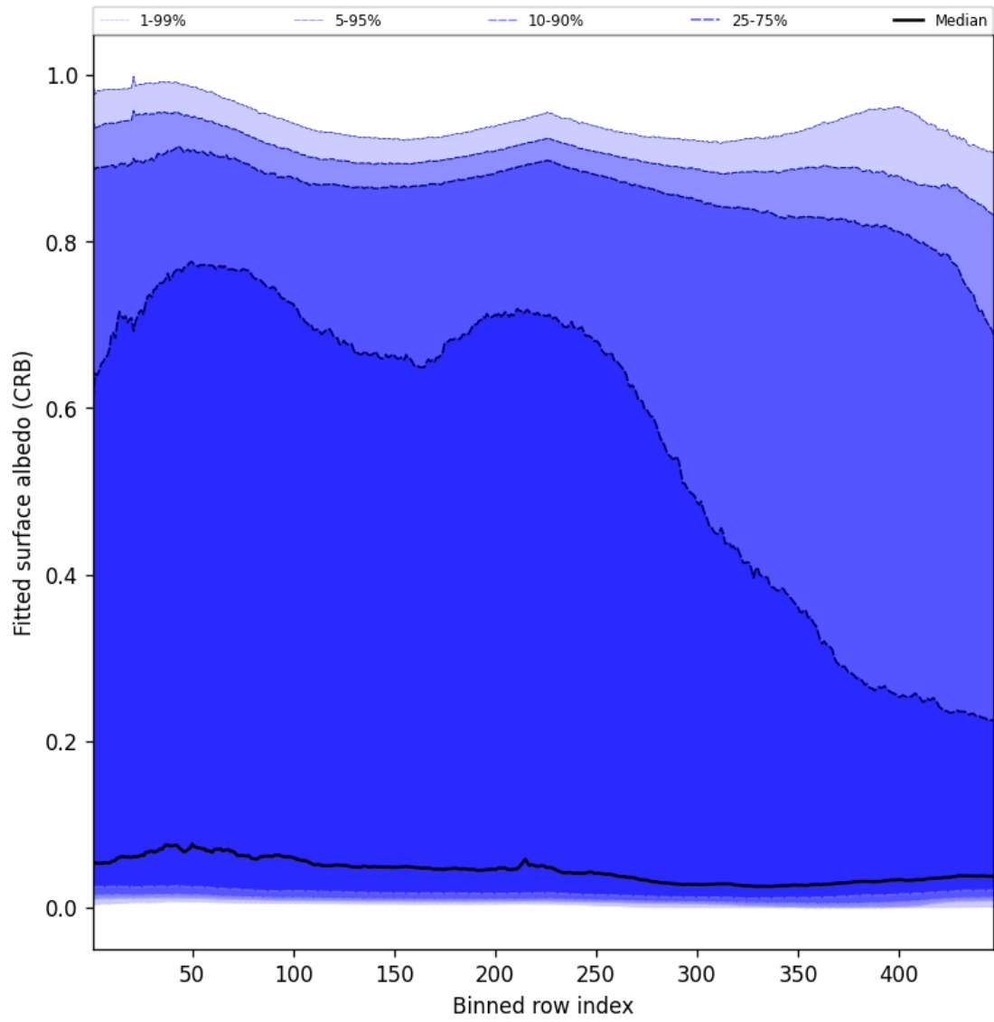
Figure 62: Along track statistics of “Fitted surface albedo (CRB)” for 2024-11-04 to 2024-11-06
