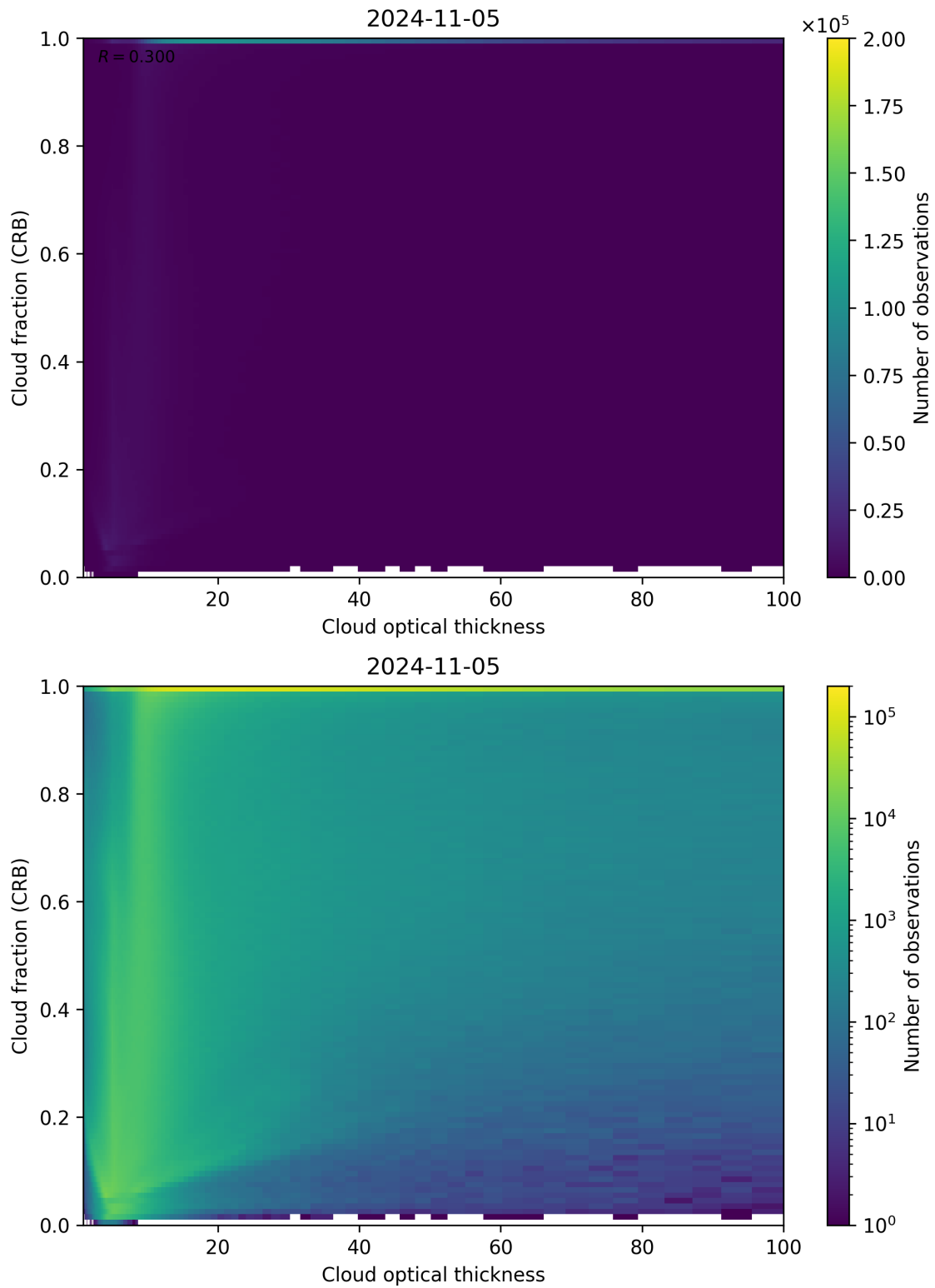
Figure 84: Scatter density plot of “Cloud optical thickness” against “Cloud fraction (CRB)” for 2024-11-04 to 2024-11-06.
