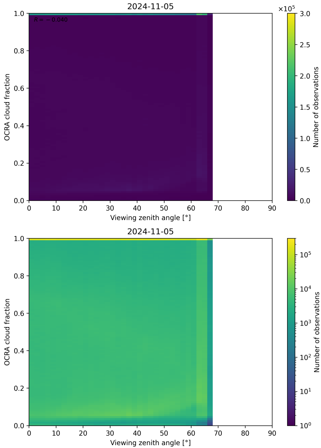
Figure 108: Scatter density plot of “Viewing zenith angle” against “OCRA cloud fraction” for 2024-11-04 to 2024-11-06.
