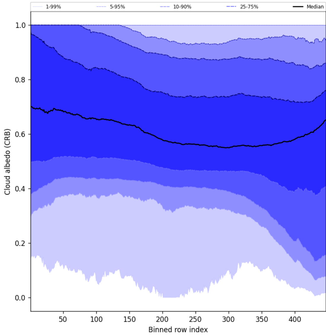
Figure 60: Along track statistics of “Cloud albedo (CRB)” for 2024-11-04 to 2024-11-06
