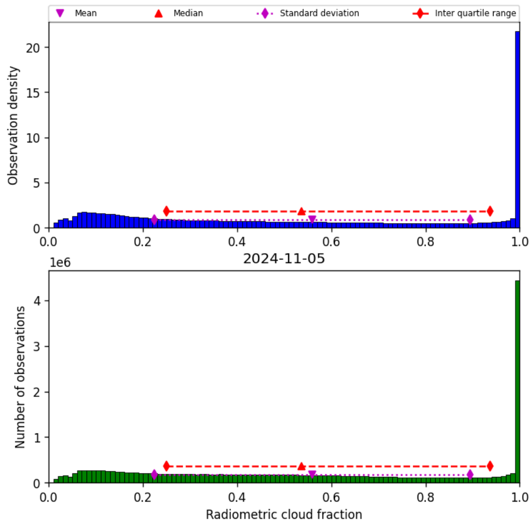
Figure 39: Histogram of “Radiometric cloud fraction” for 2024-11-04 to 2024-11-06
