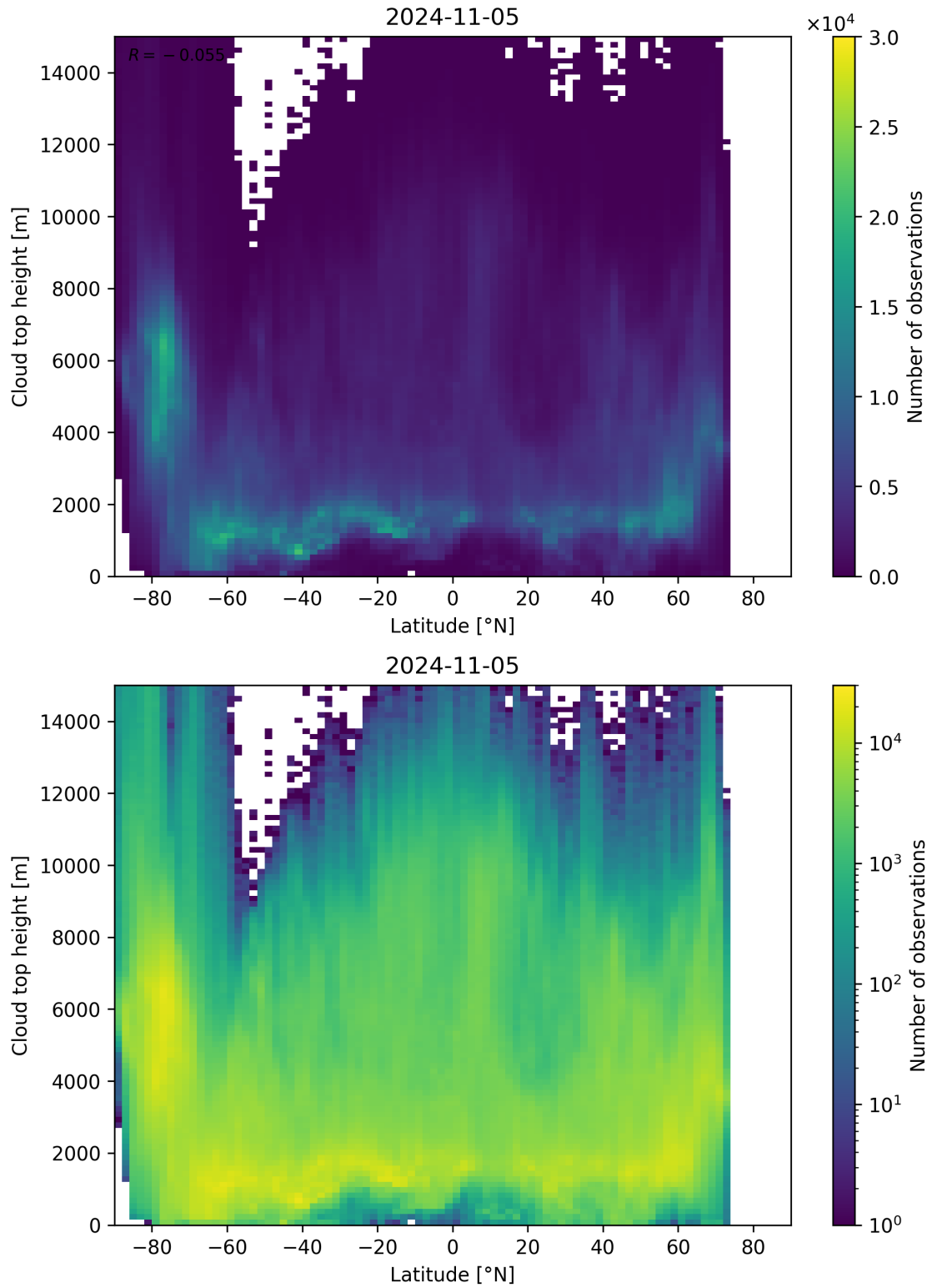
Figure 97: Scatter density plot of “Latitude” against “Cloud top height” for 2024-11-04 to 2024-11-06.
