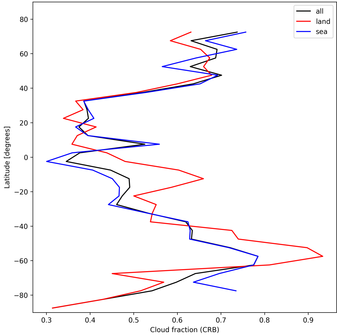
Figure 26: Zonal average of “Cloud fraction (CRB)” for 2024-11-04 to 2024-11-06.
