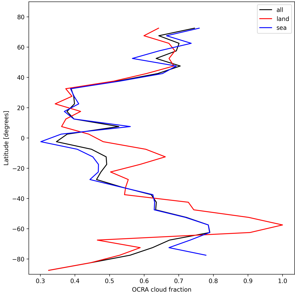
Figure 34: Zonal average of “OCRA cloud fraction” for 2024-11-04 to 2024-11-06.
