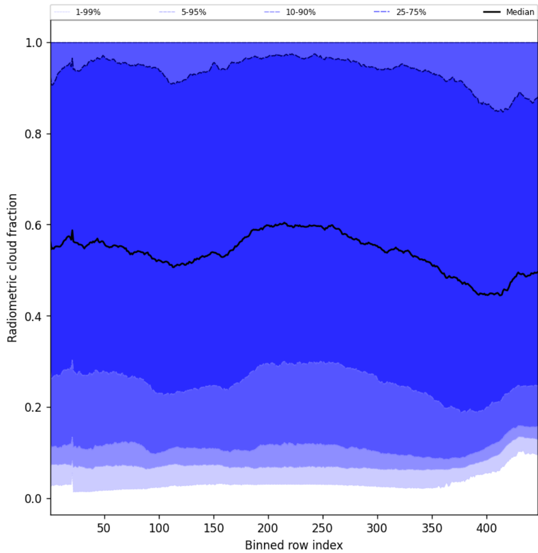
Figure 55: Along track statistics of “Radiometric cloud fraction” for 2024-11-04 to 2024-11-06
