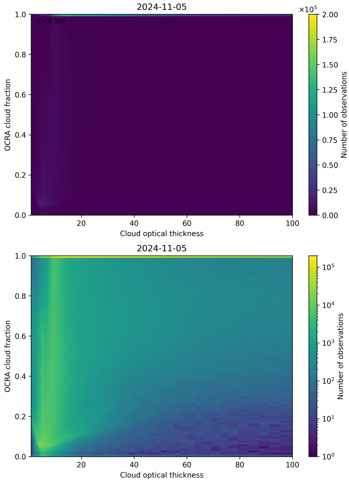
Figure 83: Scatter density plot of “Cloud optical thickness” against “OCRA cloud fraction” for 2024-11-04 to 2024-11-06.
