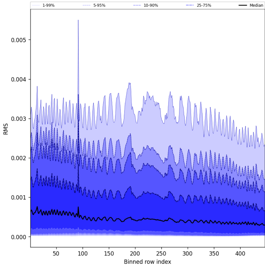
Figure 63: Along track statistics of “RMS” for 2024-11-04 to 2024-11-06
