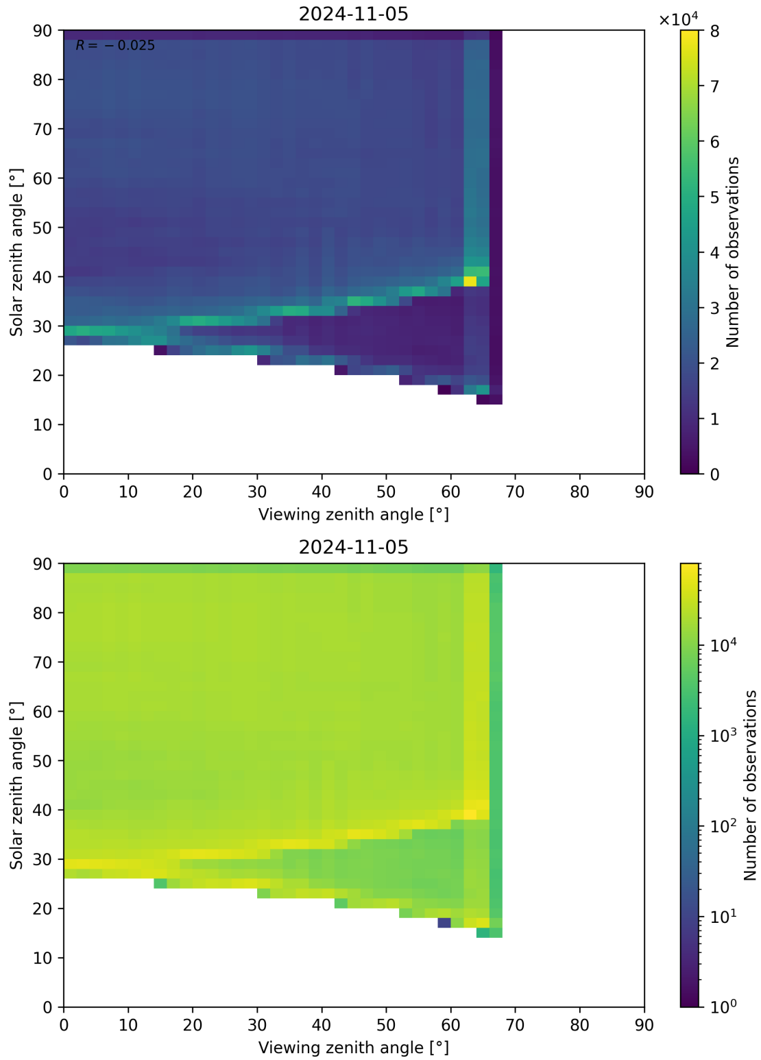
Figure 114: Scatter density plot of “Viewing zenith angle” against “Solar zenith angle” for 2024-11-04 to 2024-11-06.
