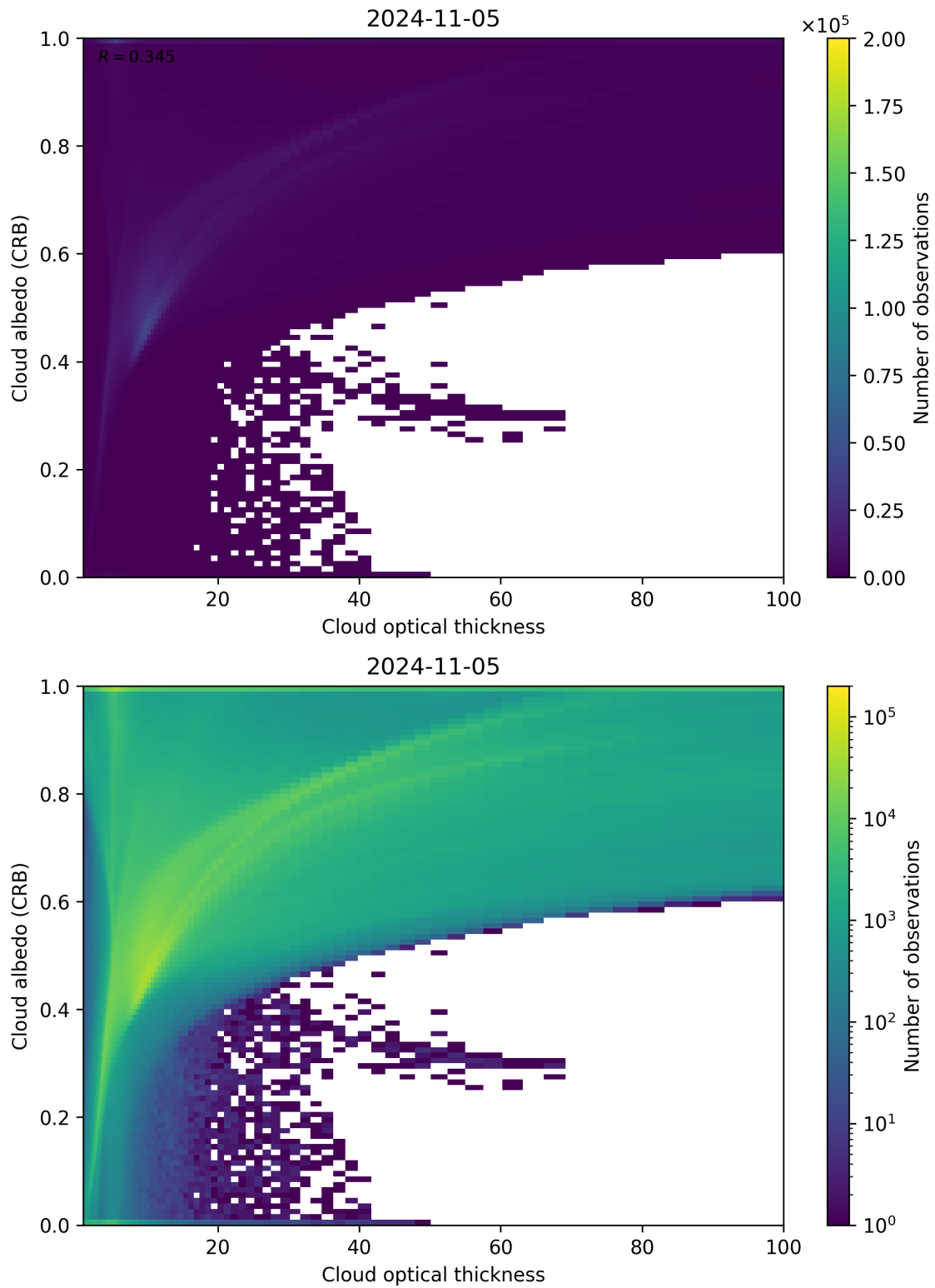
Figure 82: Scatter density plot of “Cloud optical thickness” against “Cloud albedo (CRB)” for 2024-11-04 to 2024-11-06.
