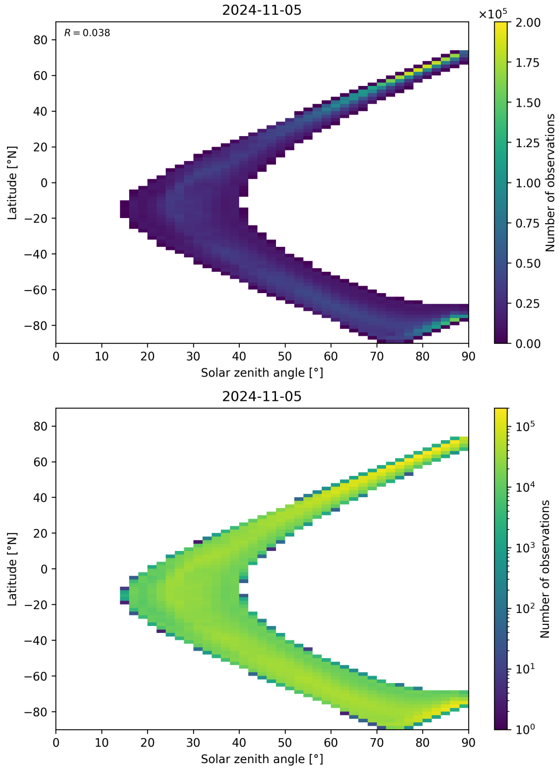
Figure 105: Scatter density plot of “Solar zenith angle” against “Latitude” for 2024-11-04 to 2024-11-06.
