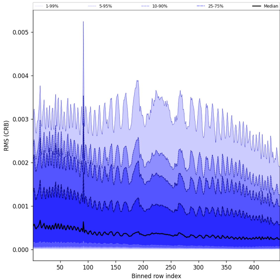
Figure 64: Along track statistics of “RMS (CRB)” for 2024-11-04 to 2024-11-06
