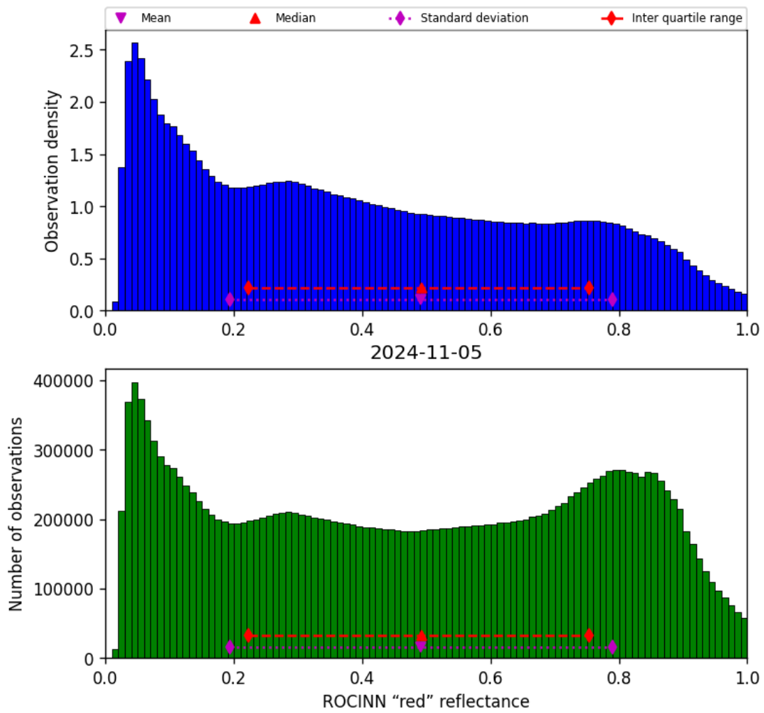
Figure 53: Histogram of “ROCINN “red” reflectance” for 2024-11-04 to 2024-11-06
