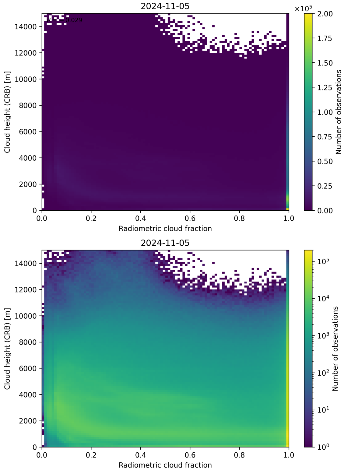
Figure 74: Scatter density plot of “Radiometric cloud fraction” against “Cloud height (CRB)” for 2024-11-04 to 2024-11-06.
