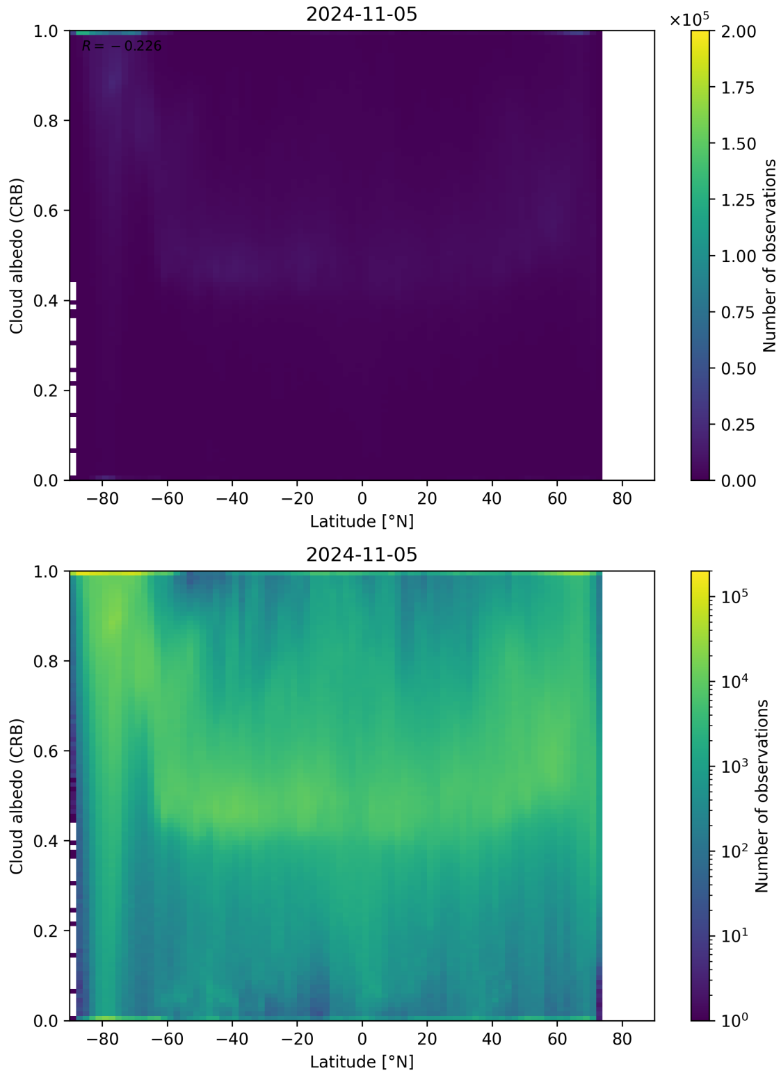
Figure 91: Scatter density plot of “Latitude” against “Cloud albedo (CRB)” for 2024-11-04 to 2024-11-06.
