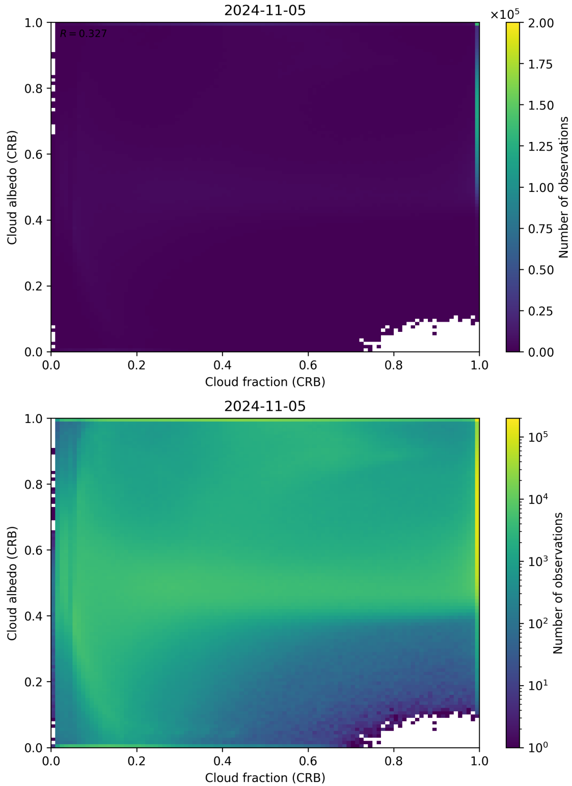
Figure 77: Scatter density plot of “Cloud fraction (CRB)” against “Cloud albedo (CRB)” for 2024-11-04 to 2024-11-06.
