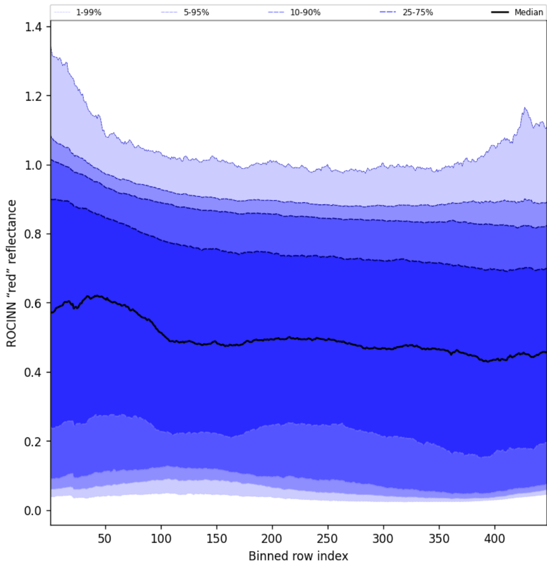
Figure 69: Along track statistics of “ROCINN “red” reflectance” for 2024-11-04 to 2024-11-06
