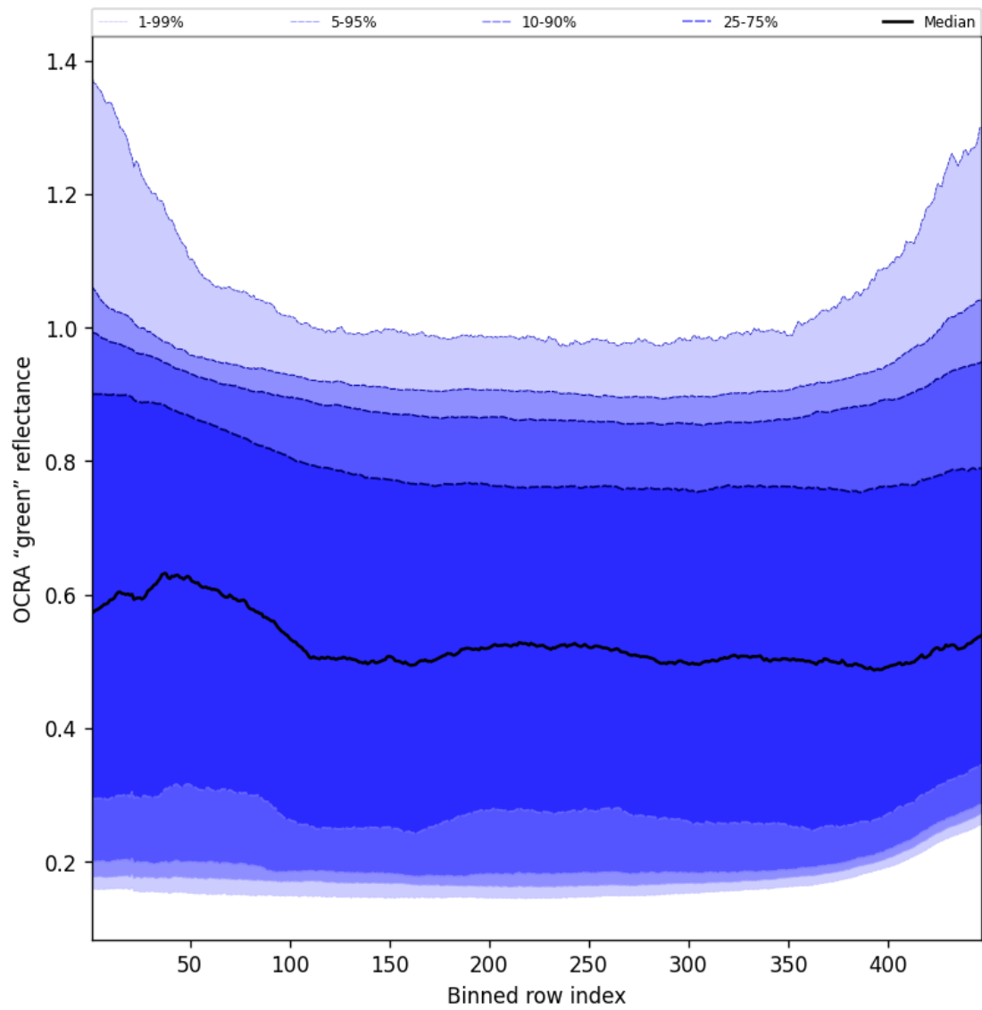
Figure 68: Along track statistics of “OCRA “green” reflectance” for 2024-11-04 to 2024-11-06
