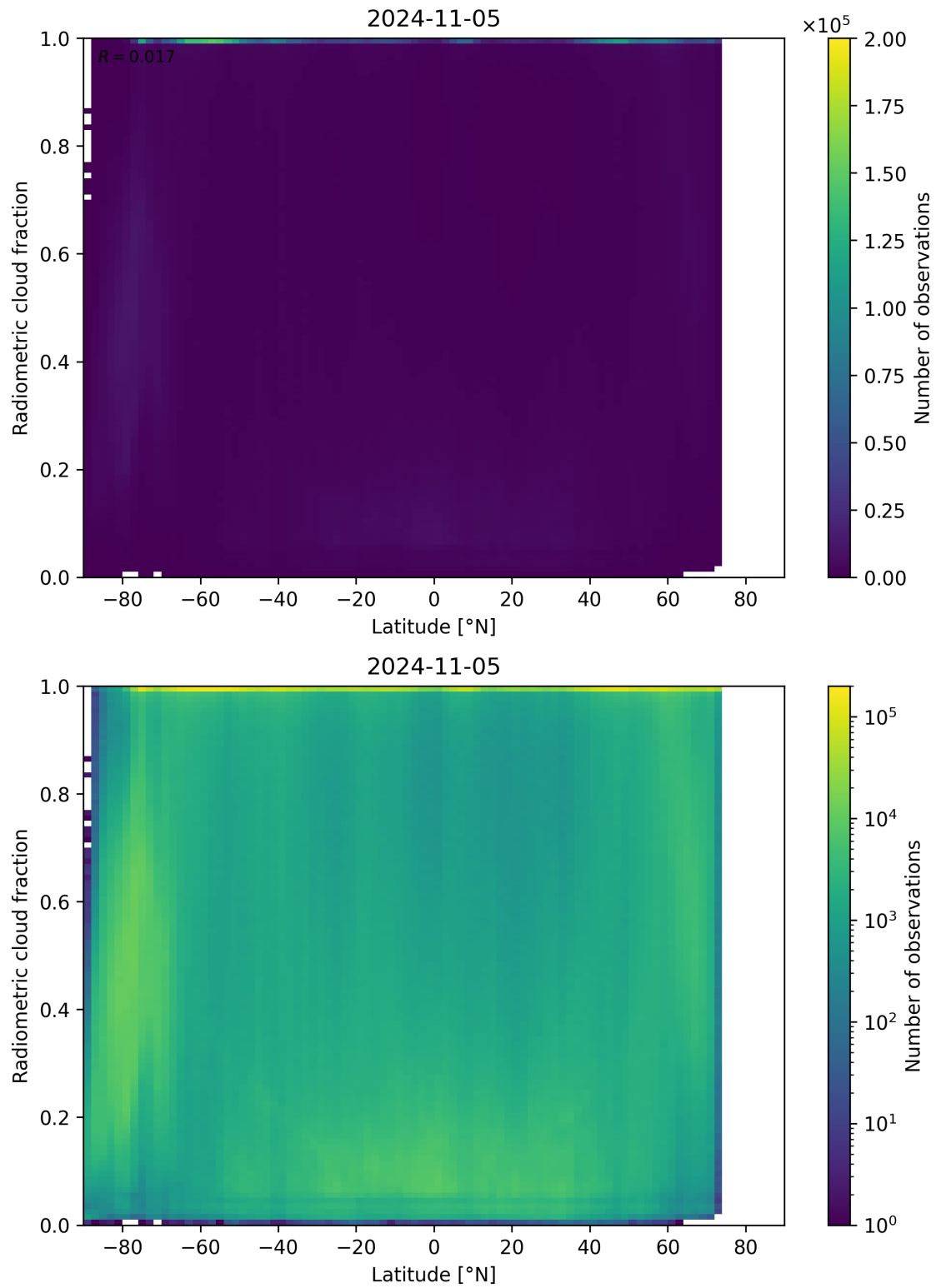
Figure 92: Scatter density plot of “Latitude” against “Radiometric cloud fraction” for 2024-11-04 to 2024-11-06.
