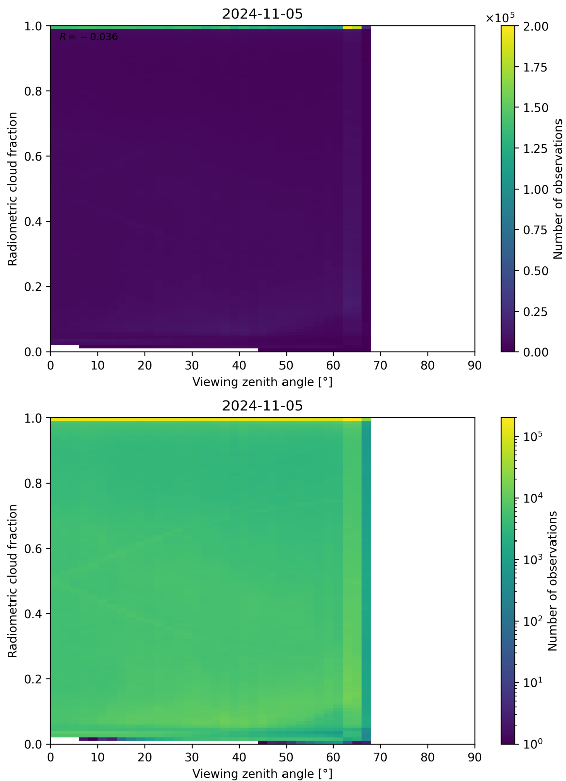
Figure 107: Scatter density plot of “Viewing zenith angle” against “Radiometric cloud fraction” for 2024-11-04 to 2024-11-06.
