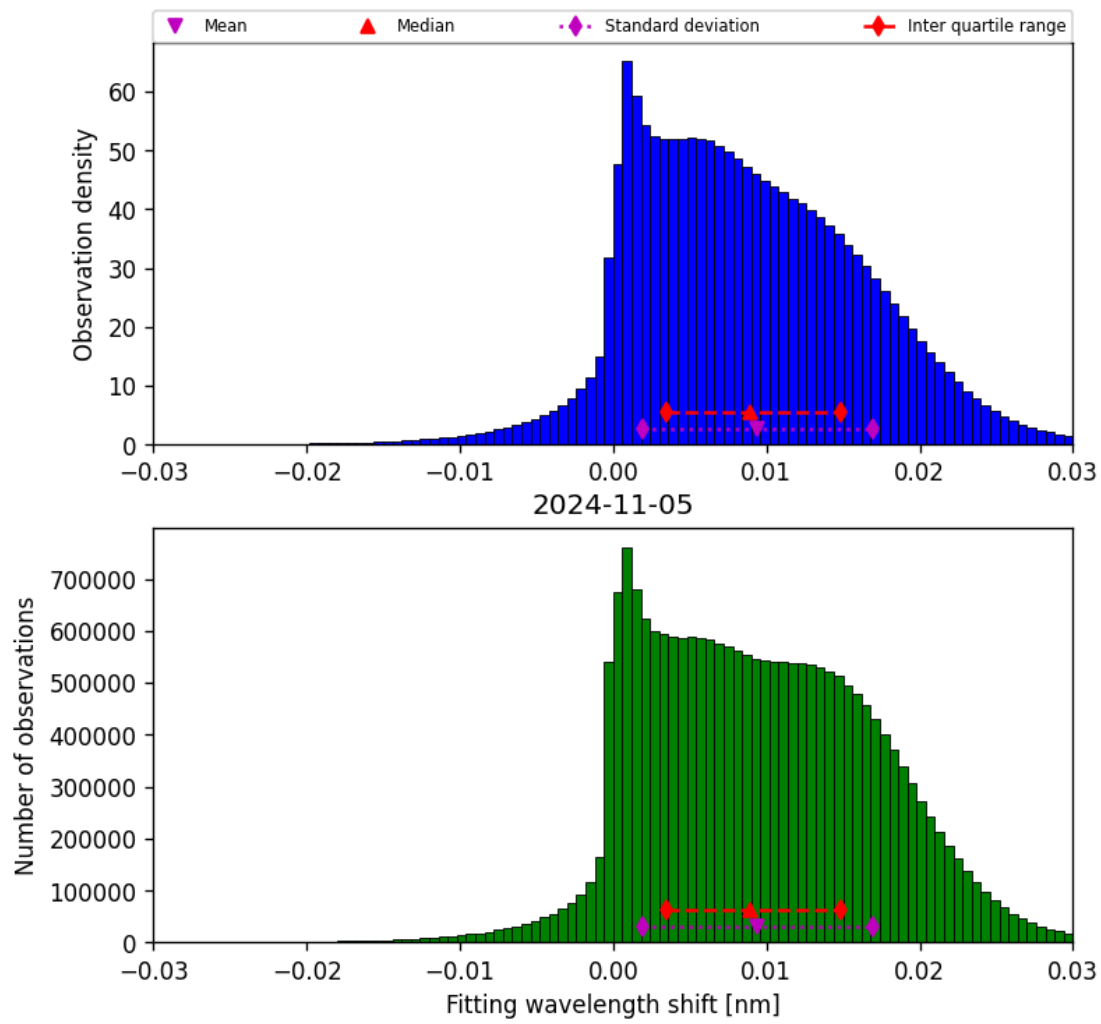
Figure 49: Histogram of “Fitting wavelength shift” for 2024-11-04 to 2024-11-06
