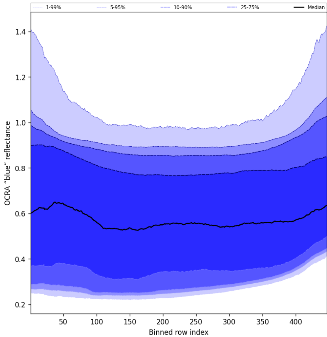
Figure 67: Along track statistics of “OCRA “blue” reflectance” for 2024-11-04 to 2024-11-06
