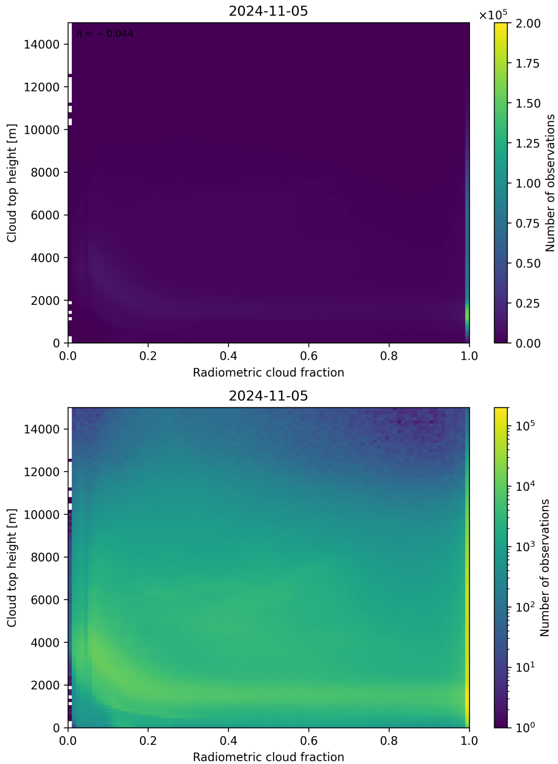
Figure 76: Scatter density plot of “Radiometric cloud fraction” against “Cloud top height” for 2024-11-04 to 2024-11-06.
