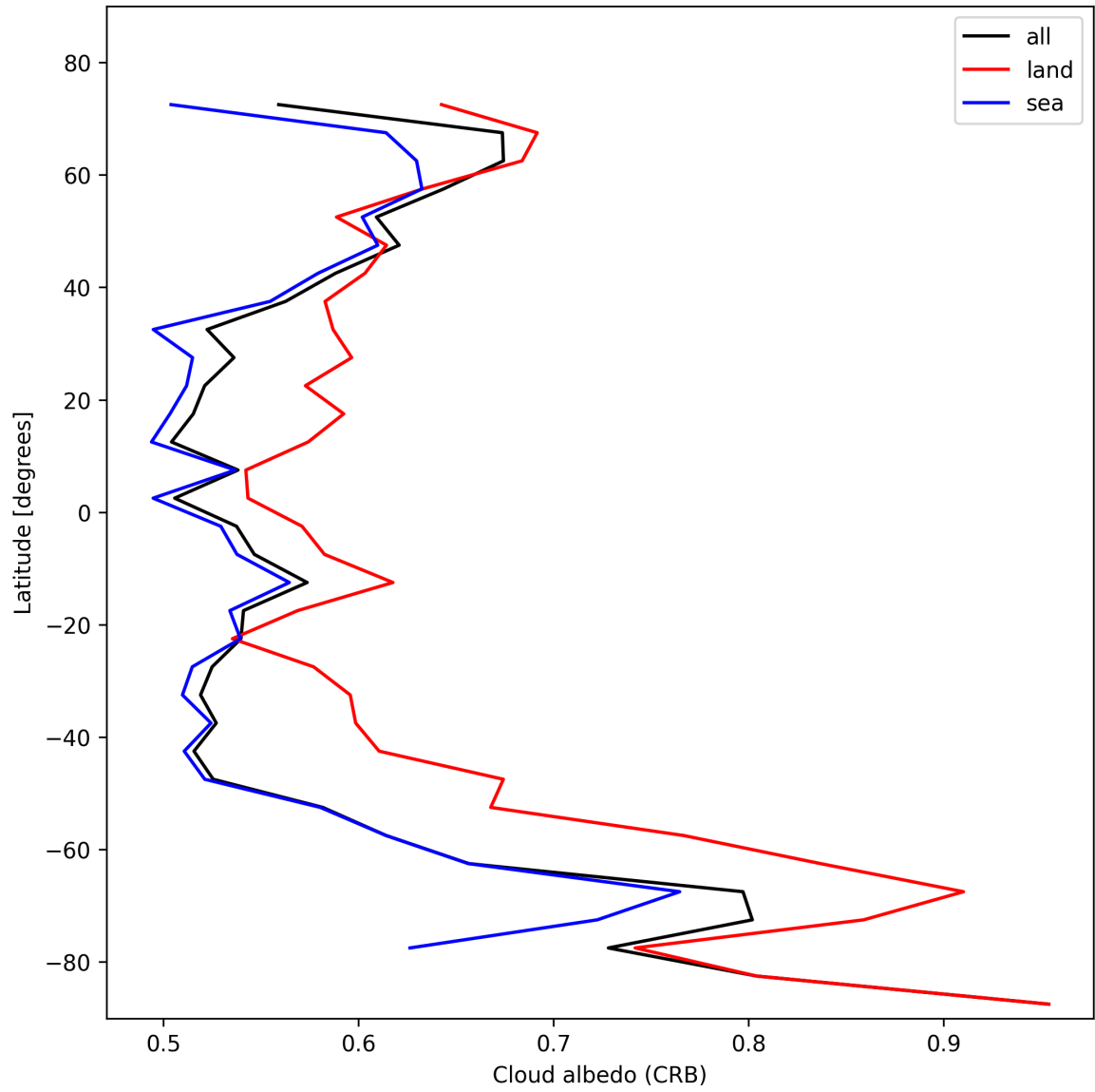
Figure 28: Zonal average of “Cloud albedo (CRB)” for 2024-11-04 to 2024-11-06.
