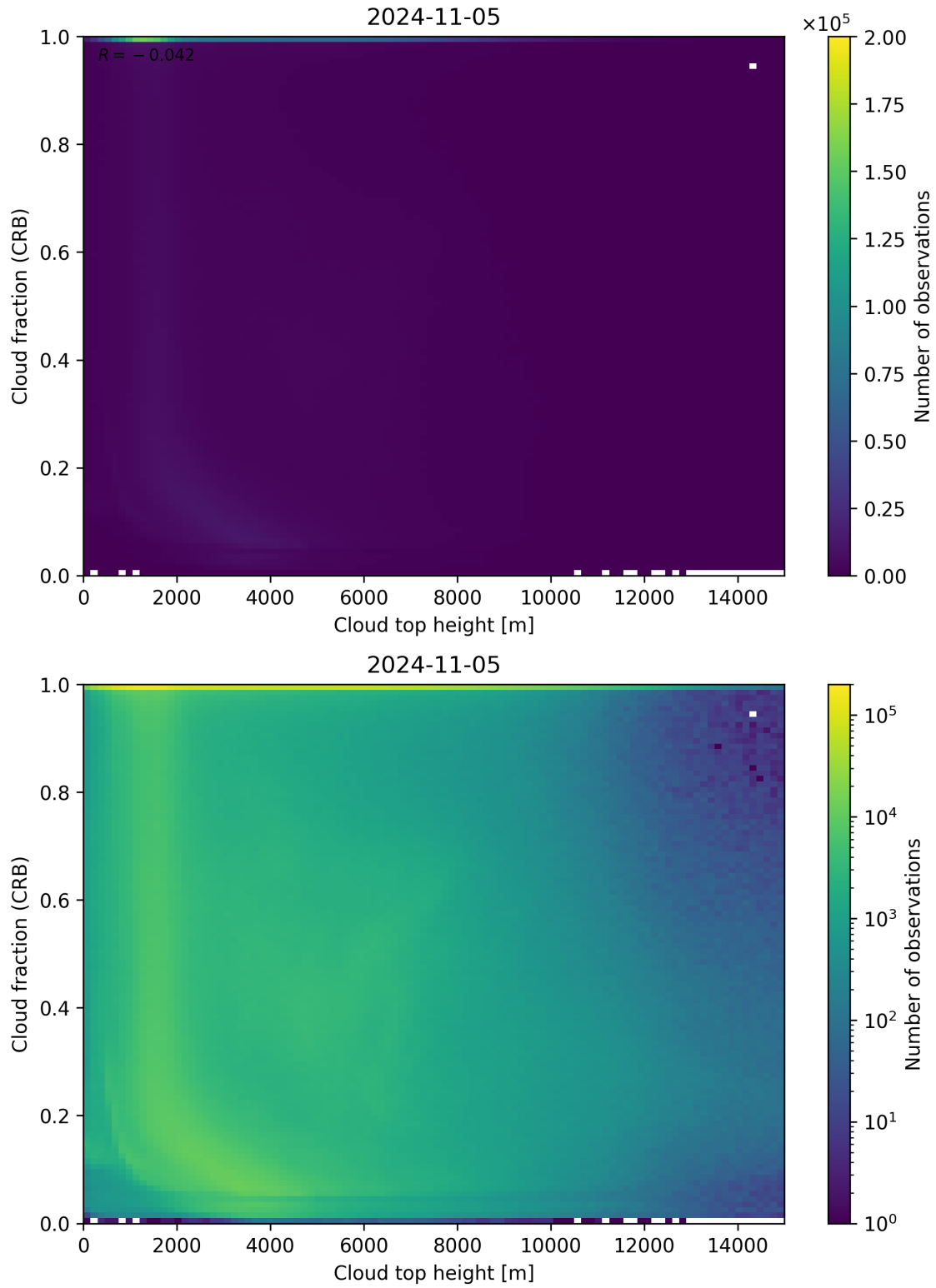
Figure 88: Scatter density plot of “Cloud top height” against “Cloud fraction (CRB)” for 2024-11-04 to 2024-11-06.
