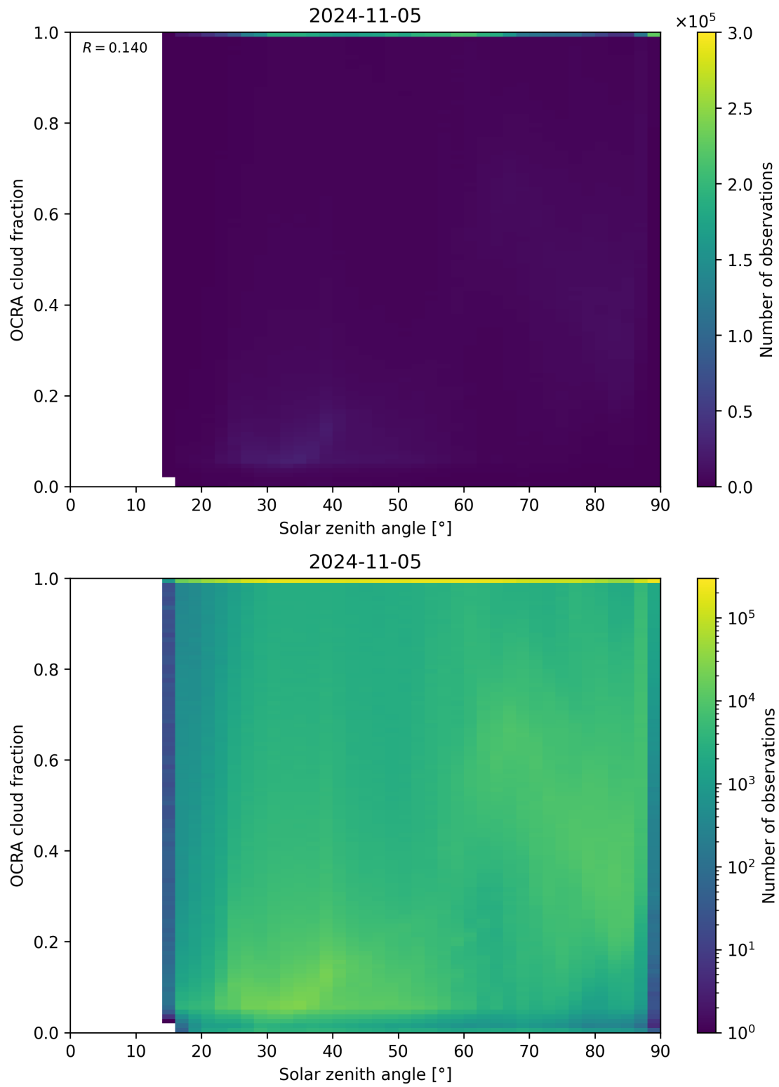
Figure 100: Scatter density plot of “Solar zenith angle” against “OCRA cloud fraction” for 2024-11-04 to 2024-11-06.
