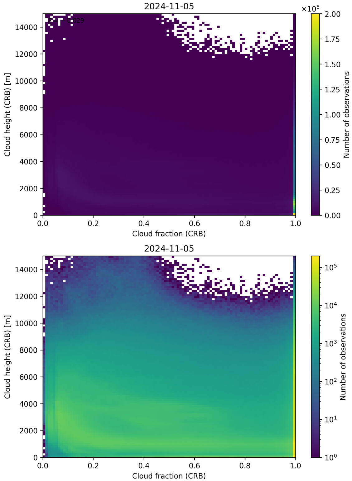
Figure 79: Scatter density plot of “Cloud fraction (CRB)” against “Cloud height (CRB)” for 2024-11-04 to 2024-11-06.
