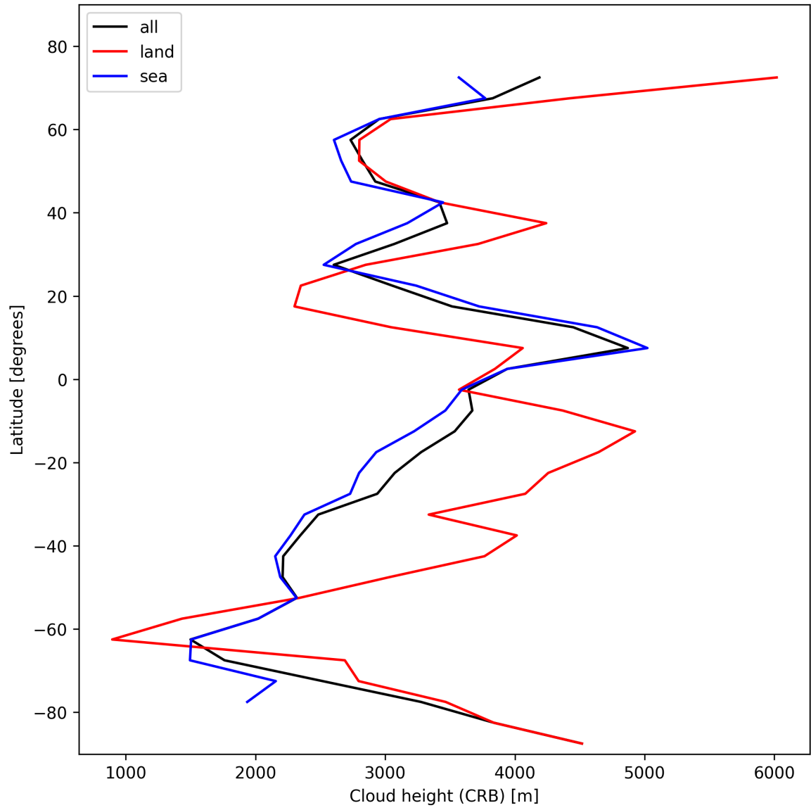
Figure 27: Zonal average of “Cloud height (CRB)” for 2024-11-04 to 2024-11-06.
