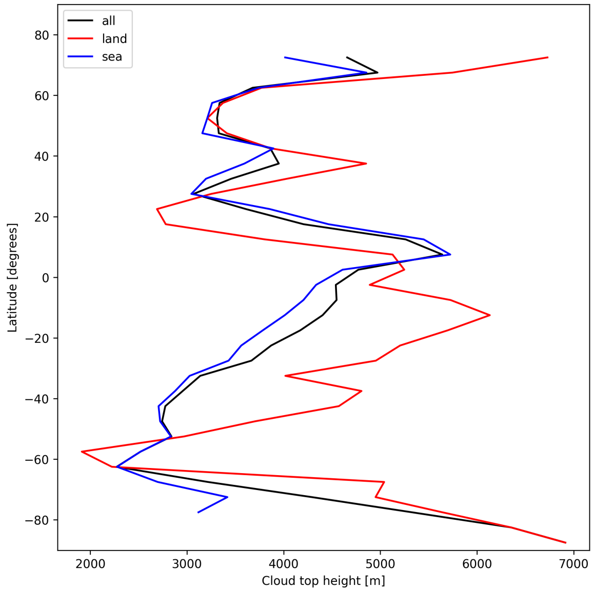
Figure 24: Zonal average of “Cloud top height” for 2024-11-04 to 2024-11-06.
