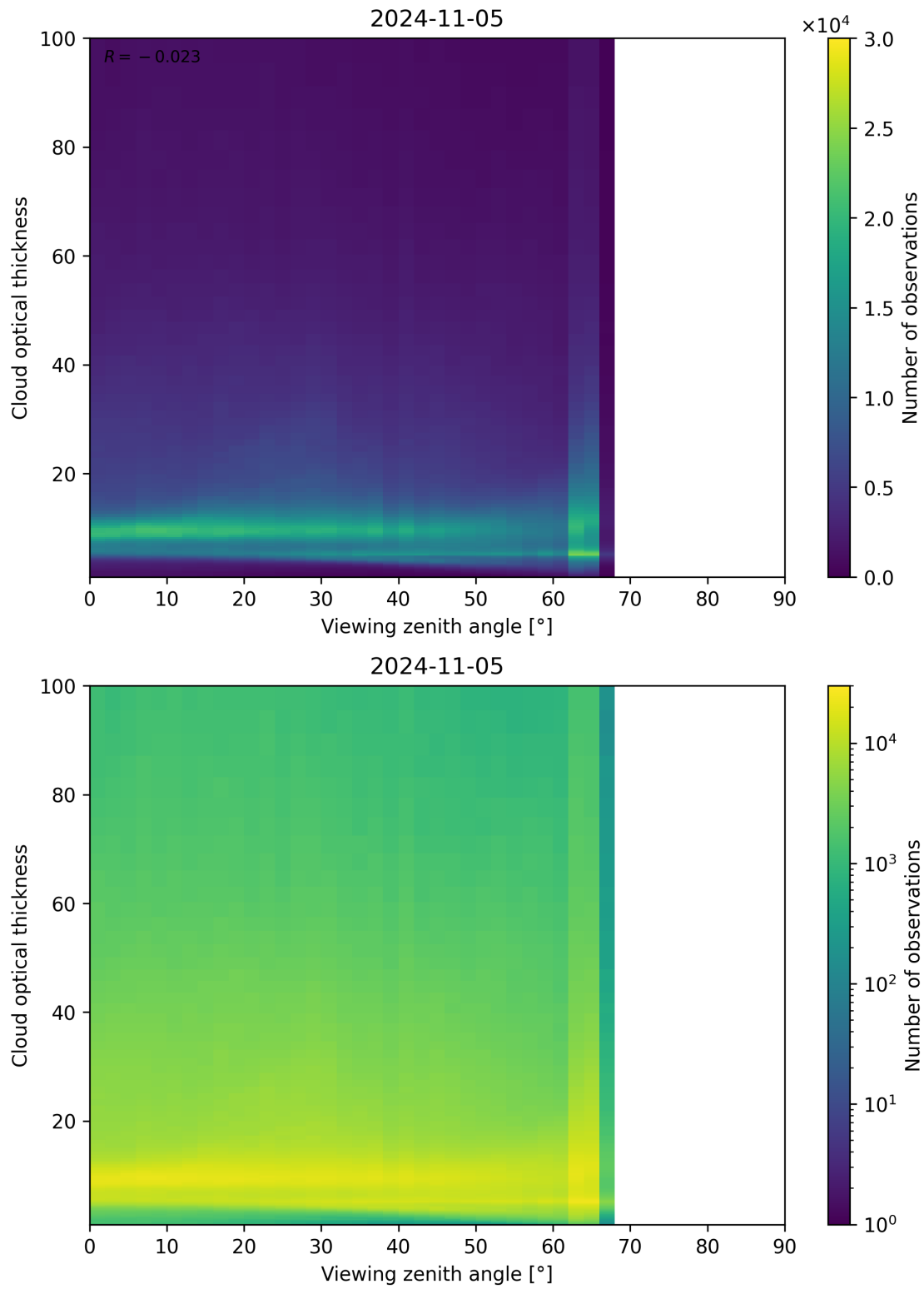
Figure 111: Scatter density plot of “Viewing zenith angle” against “Cloud optical thickness” for 2024-11-04 to 2024-11-06.
