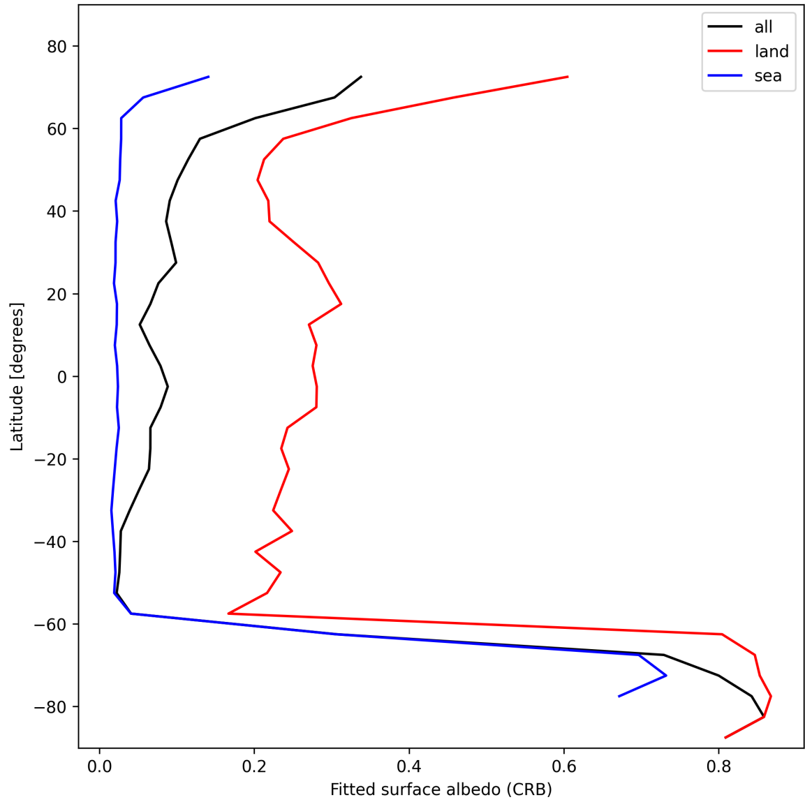
Figure 30: Zonal average of “Fitted surface albedo (CRB)” for 2024-11-04 to 2024-11-06.
