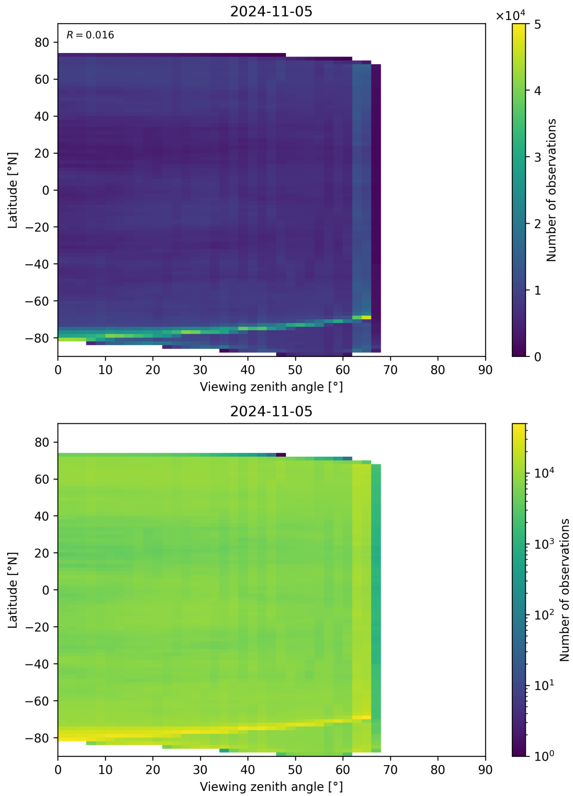
Figure 113: Scatter density plot of “Viewing zenith angle” against “Latitude” for 2024-11-04 to 2024-11-06.
