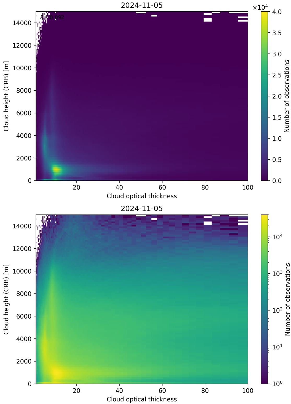
Figure 85: Scatter density plot of “Cloud optical thickness” against “Cloud height (CRB)” for 2024-11-04 to 2024-11-06.
