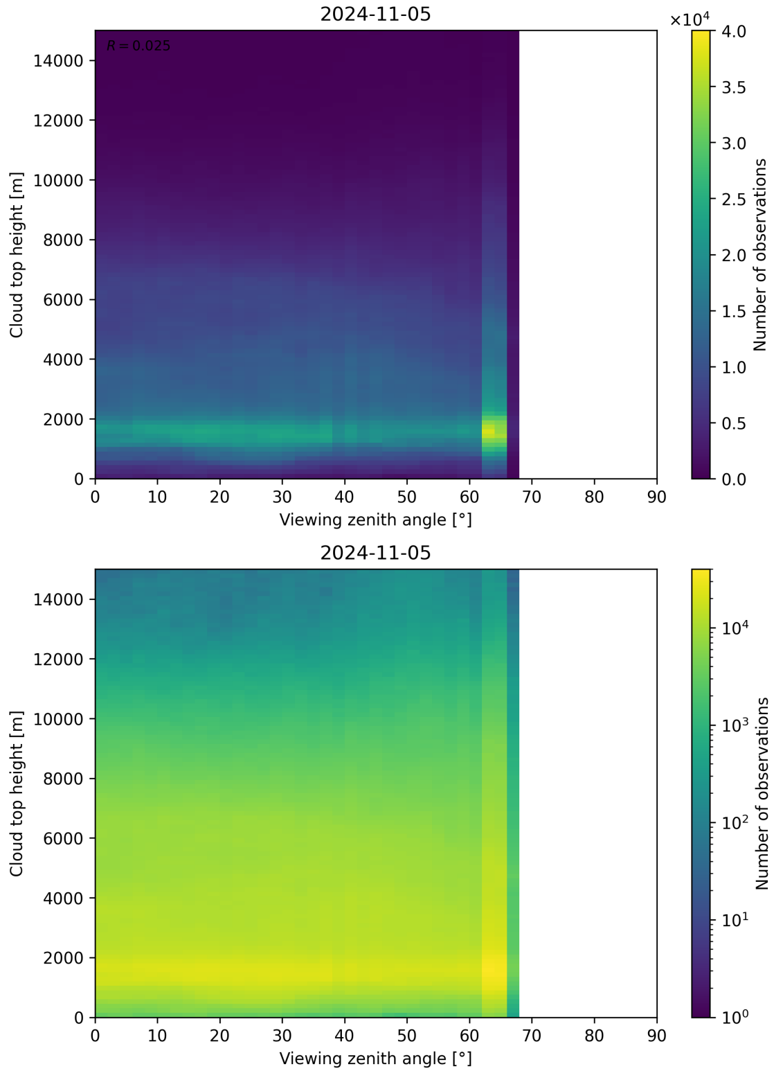
Figure 112: Scatter density plot of “Viewing zenith angle” against “Cloud top height” for 2024-11-04 to 2024-11-06.
