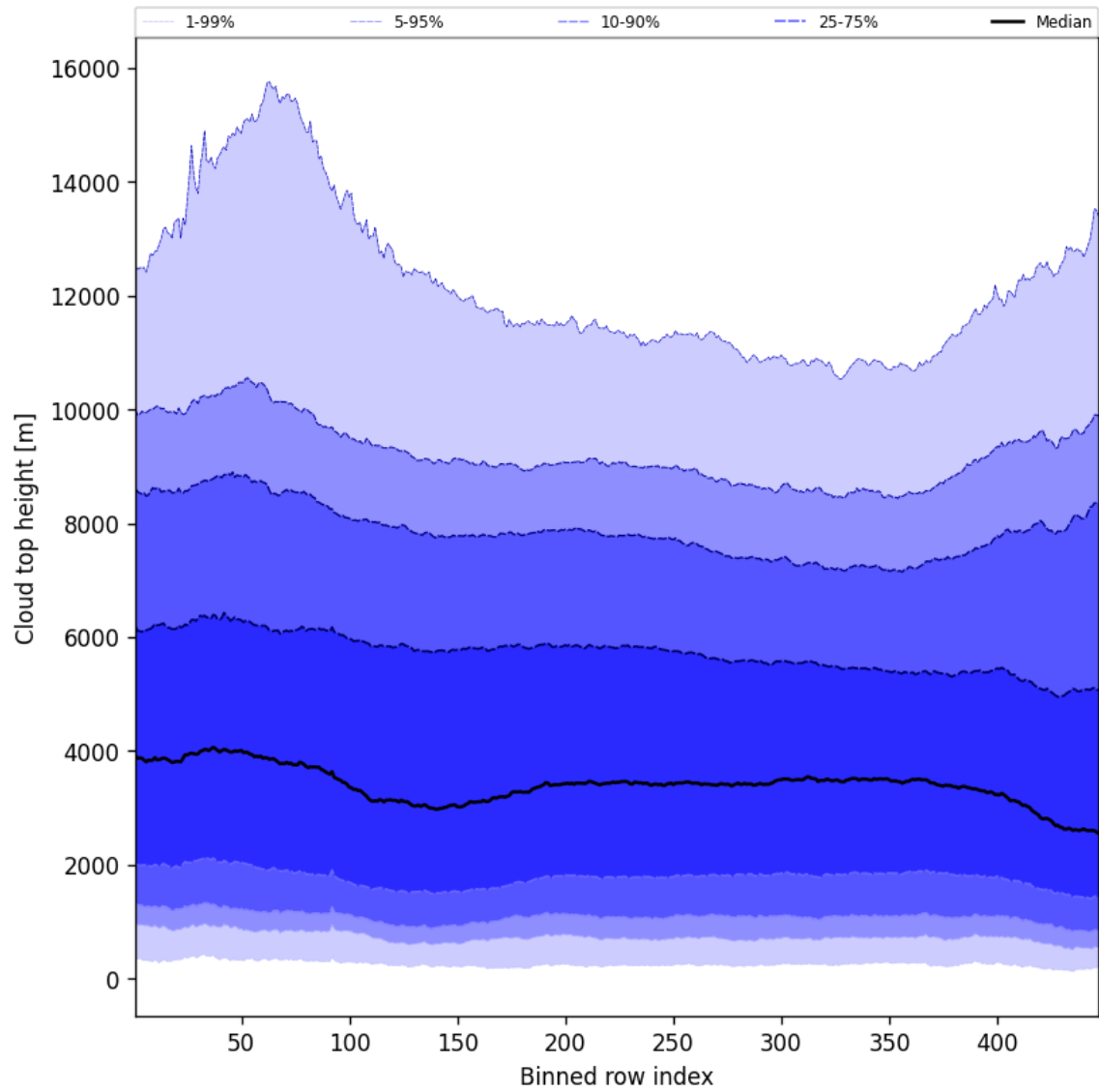
Figure 56: Along track statistics of “Cloud top height” for 2024-11-04 to 2024-11-06
