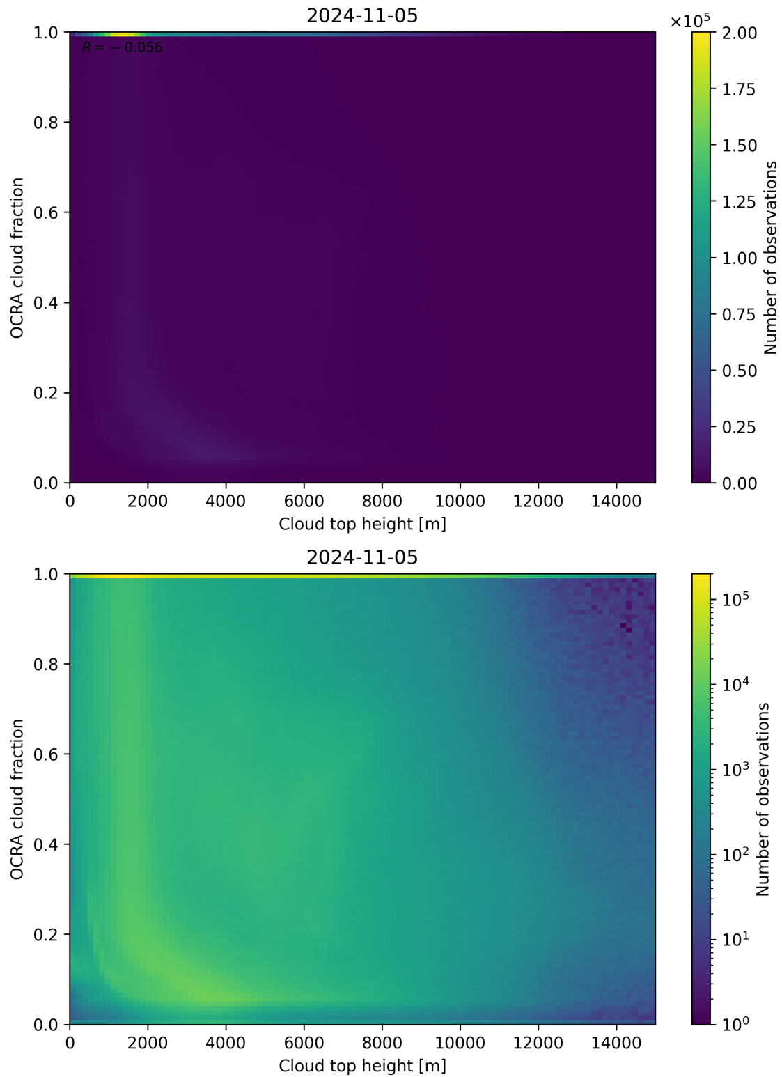
Figure 87: Scatter density plot of “Cloud top height” against “OCRA cloud fraction” for 2024-11-04 to 2024-11-06.
