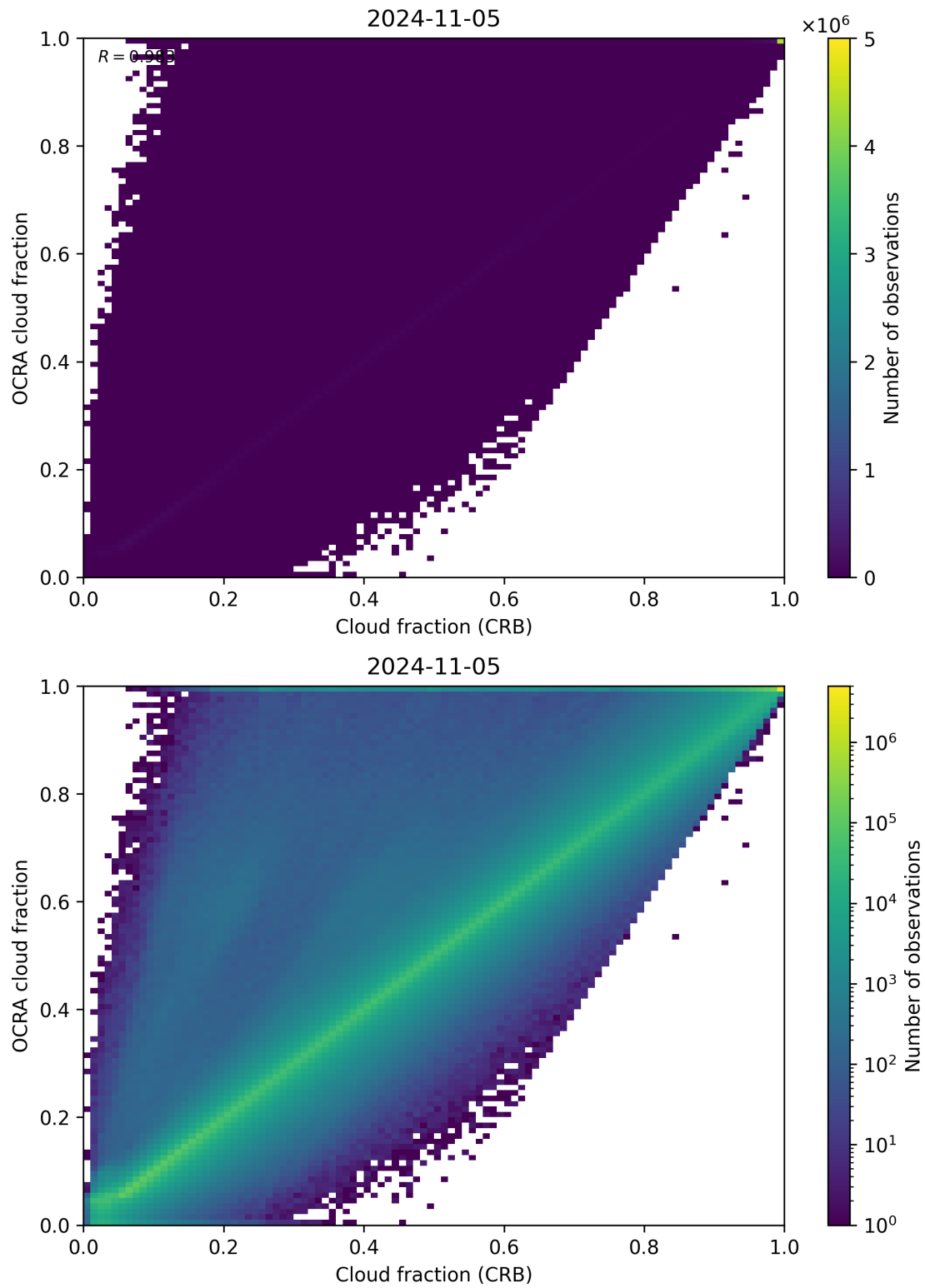
Figure 78: Scatter density plot of “Cloud fraction (CRB)” against “OCRA cloud fraction” for 2024-11-04 to 2024-11-06.
