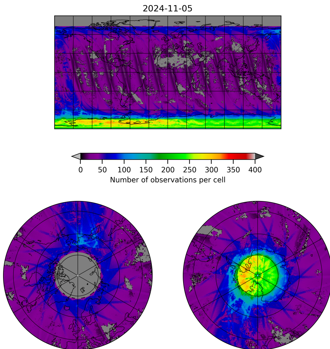
Figure 21: Map of the number of observations for 2024-11-04 to 2024-11-06
