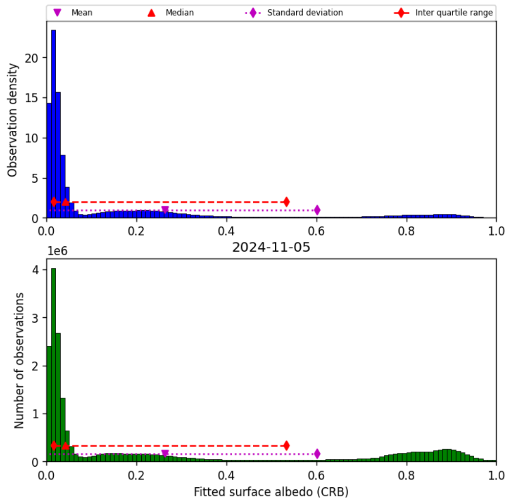
Figure 46: Histogram of “Fitted surface albedo (CRB)” for 2024-11-04 to 2024-11-06
