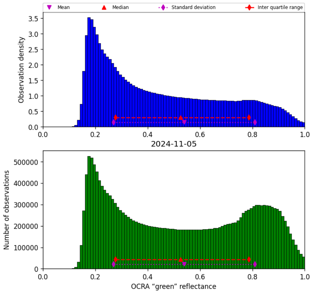
Figure 52: Histogram of “OCRA “green” reflectance” for 2024-11-04 to 2024-11-06
