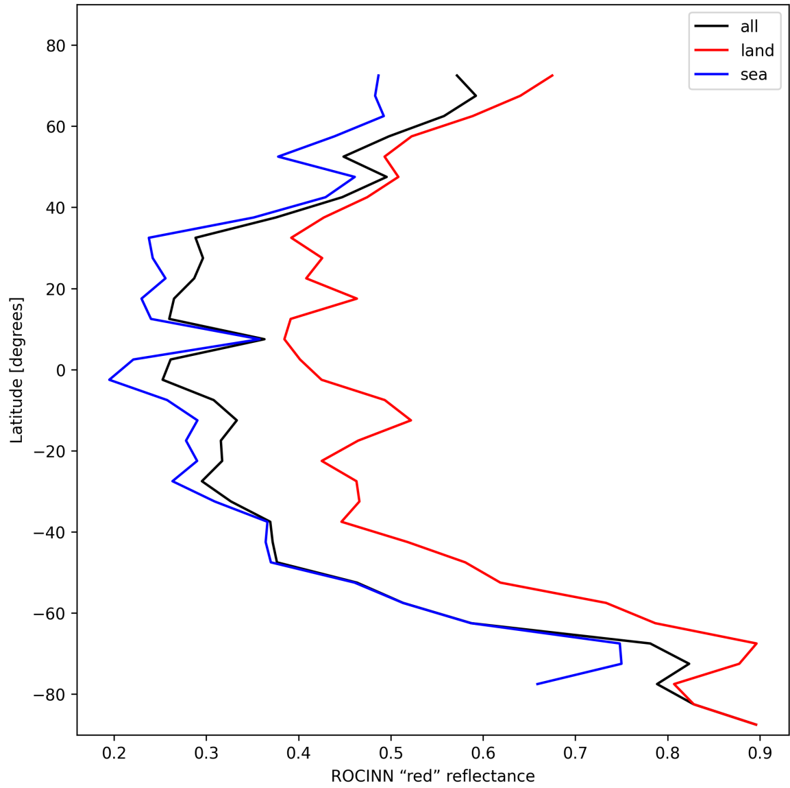
Figure 37: Zonal average of "ROCINN "red" reflectance" for 2024-11-04 to 2024-11-06.
