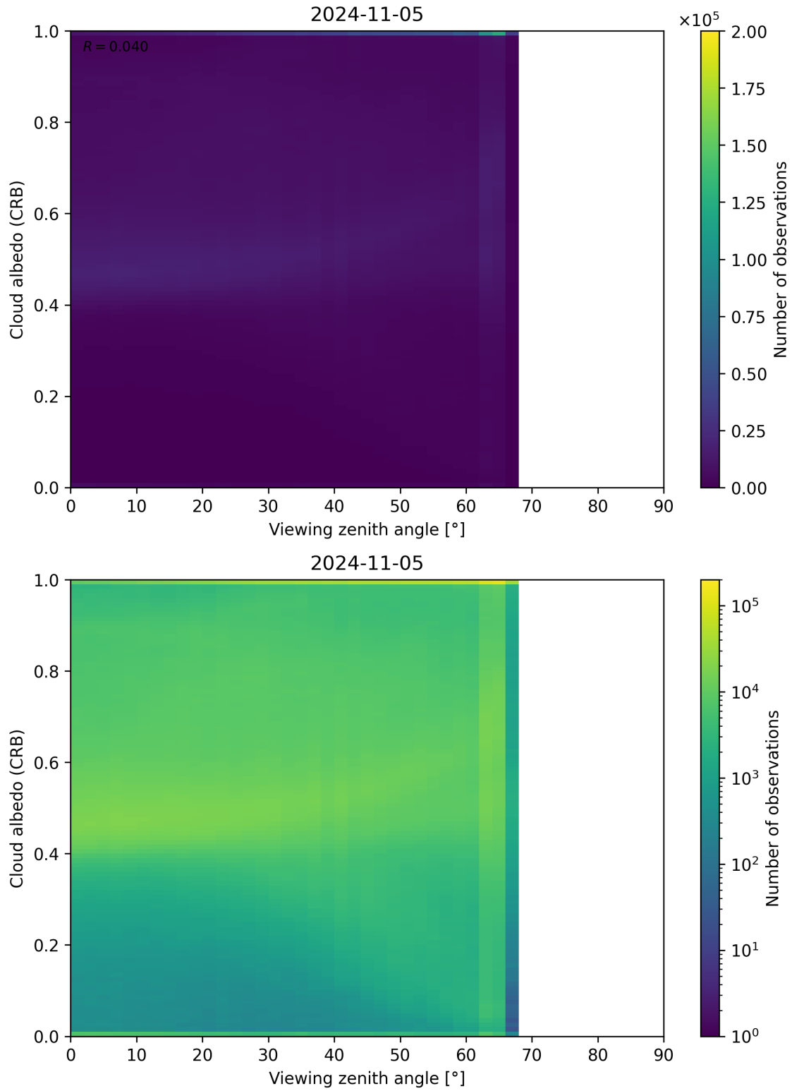
Figure 106: Scatter density plot of “Viewing zenith angle” against “Cloud albedo (CRB)” for 2024-11-04 to 2024-11-06.
