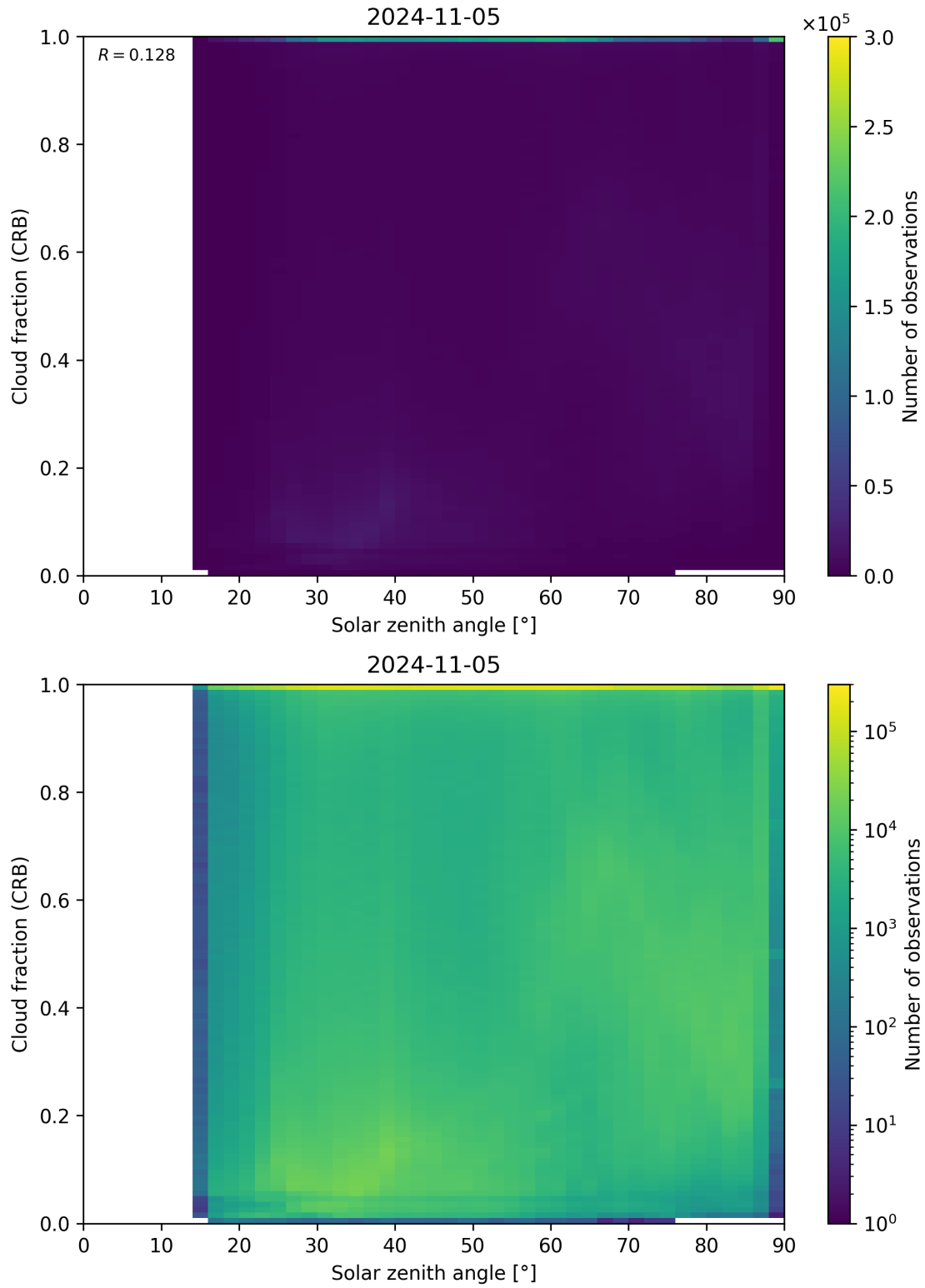
Figure 101: Scatter density plot of “Solar zenith angle” against “Cloud fraction (CRB)” for 2024-11-04 to 2024-11-06.
