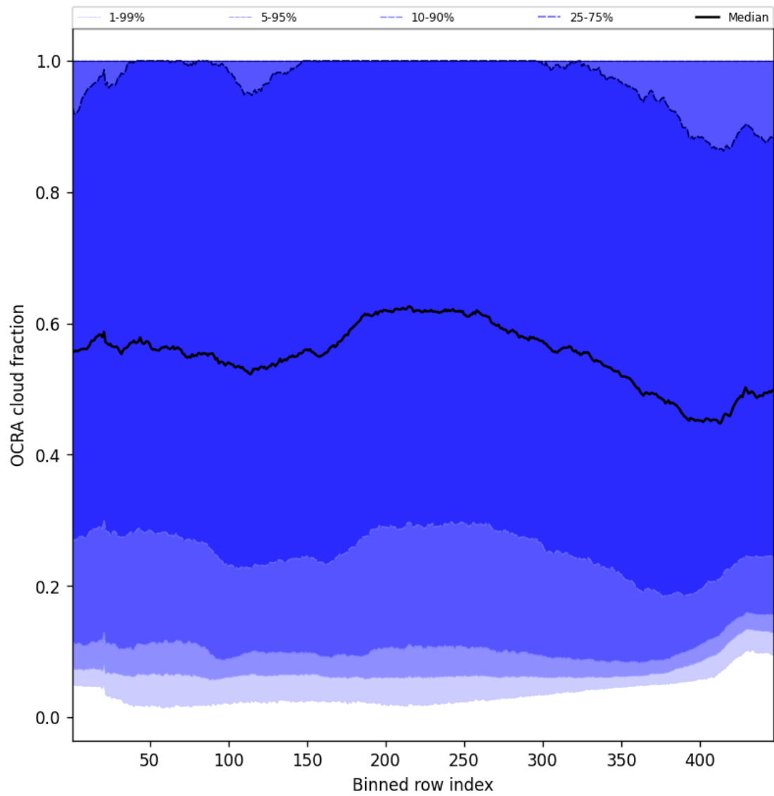
Figure 66: Along track statistics of “OCRA cloud fraction” for 2024-11-04 to 2024-11-06
