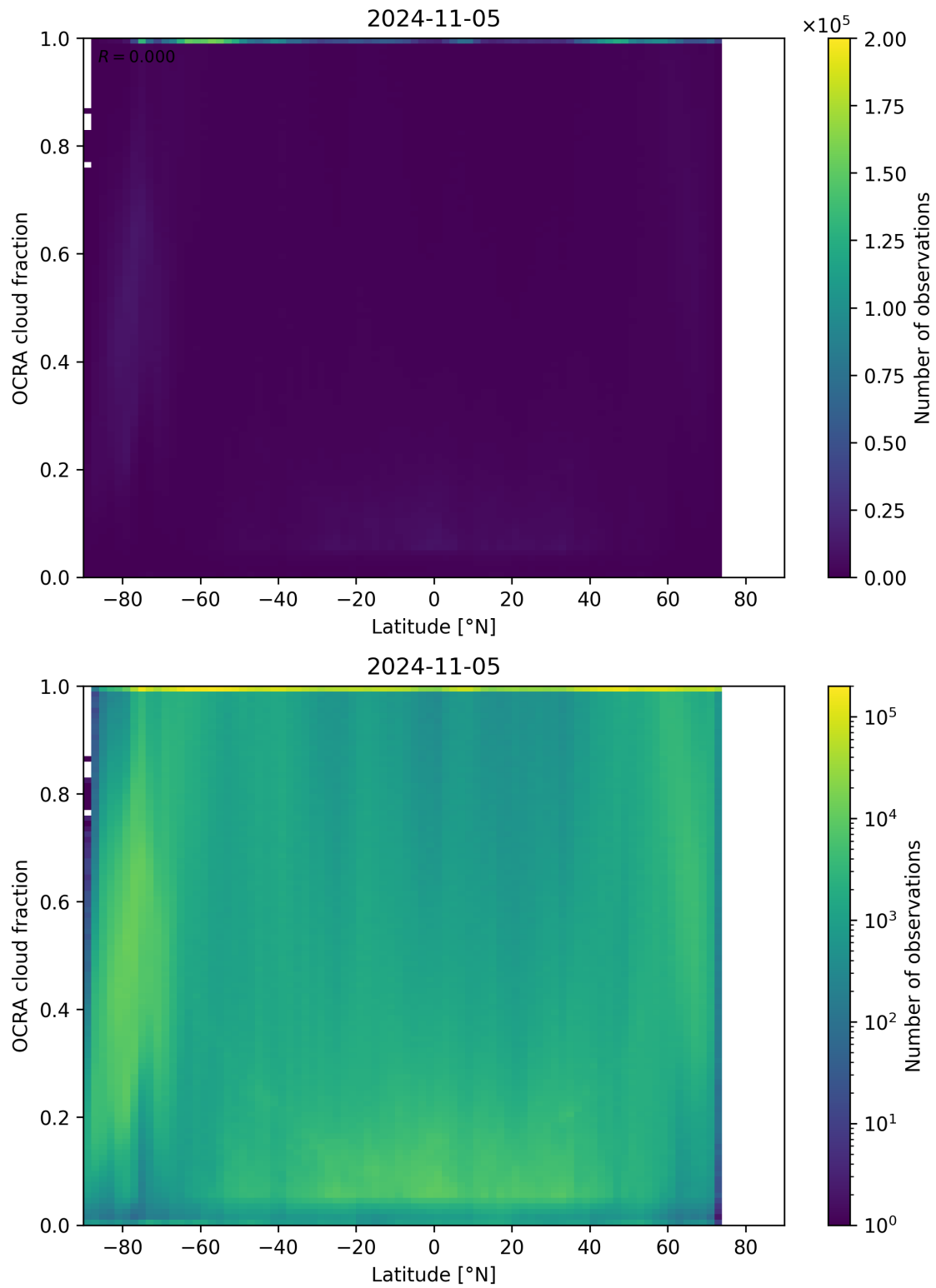
Figure 93: Scatter density plot of “Latitude” against “OCRA cloud fraction” for 2024-11-04 to 2024-11-06.
