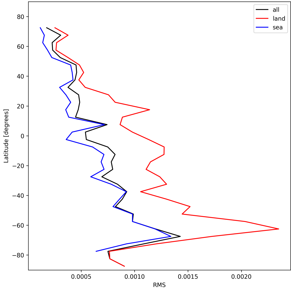
Figure 31: Zonal average of “RMS” for 2024-11-04 to 2024-11-06.
