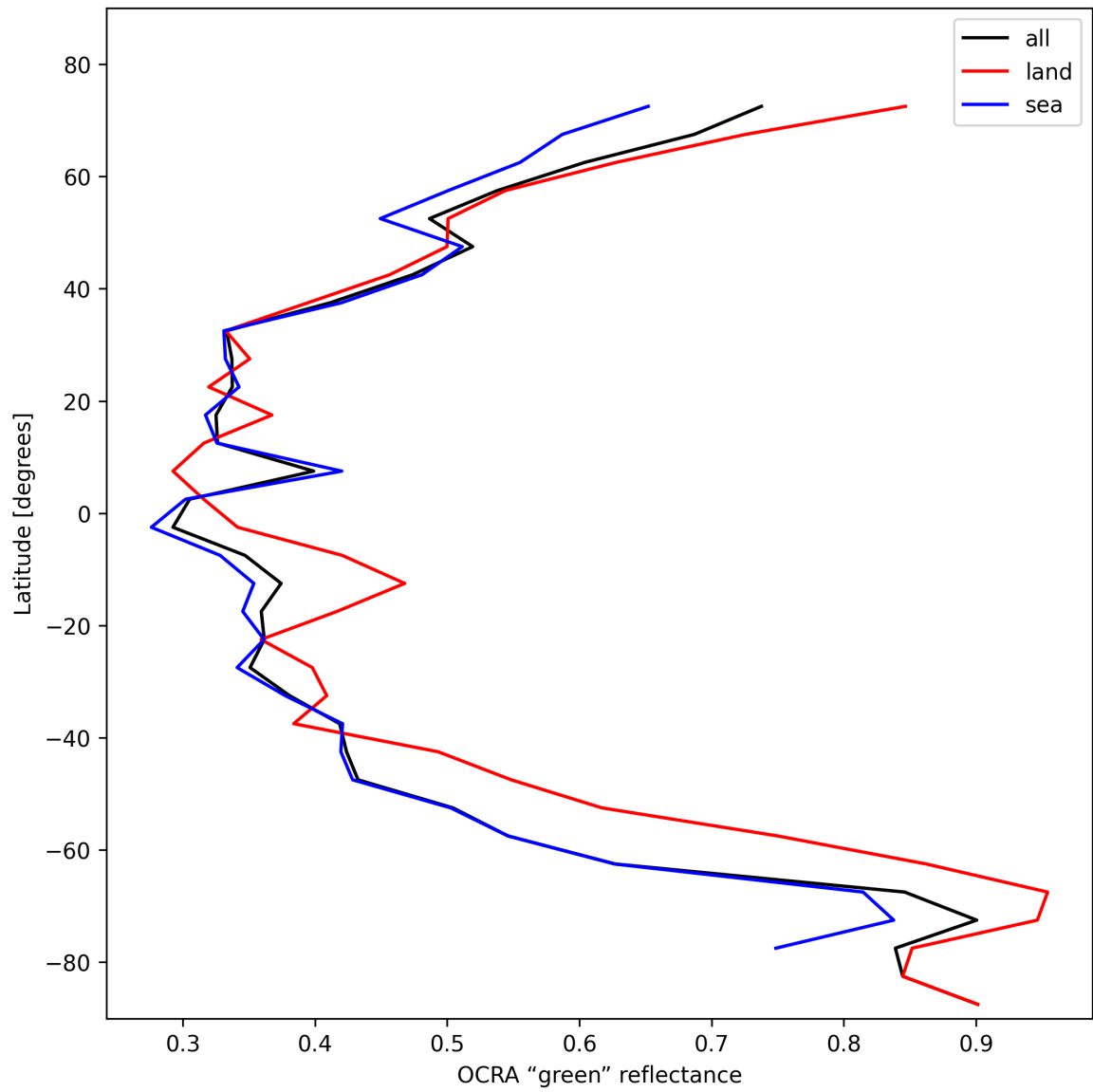
Figure 36: Zonal average of “OCRA “green” reflectance” for 2024-11-04 to 2024-11-06.
