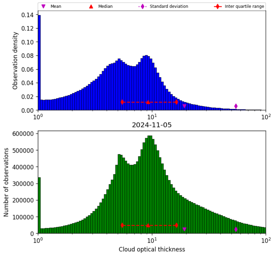
Figure 41: Histogram of “Cloud optical thickness” for 2024-11-04 to 2024-11-06
