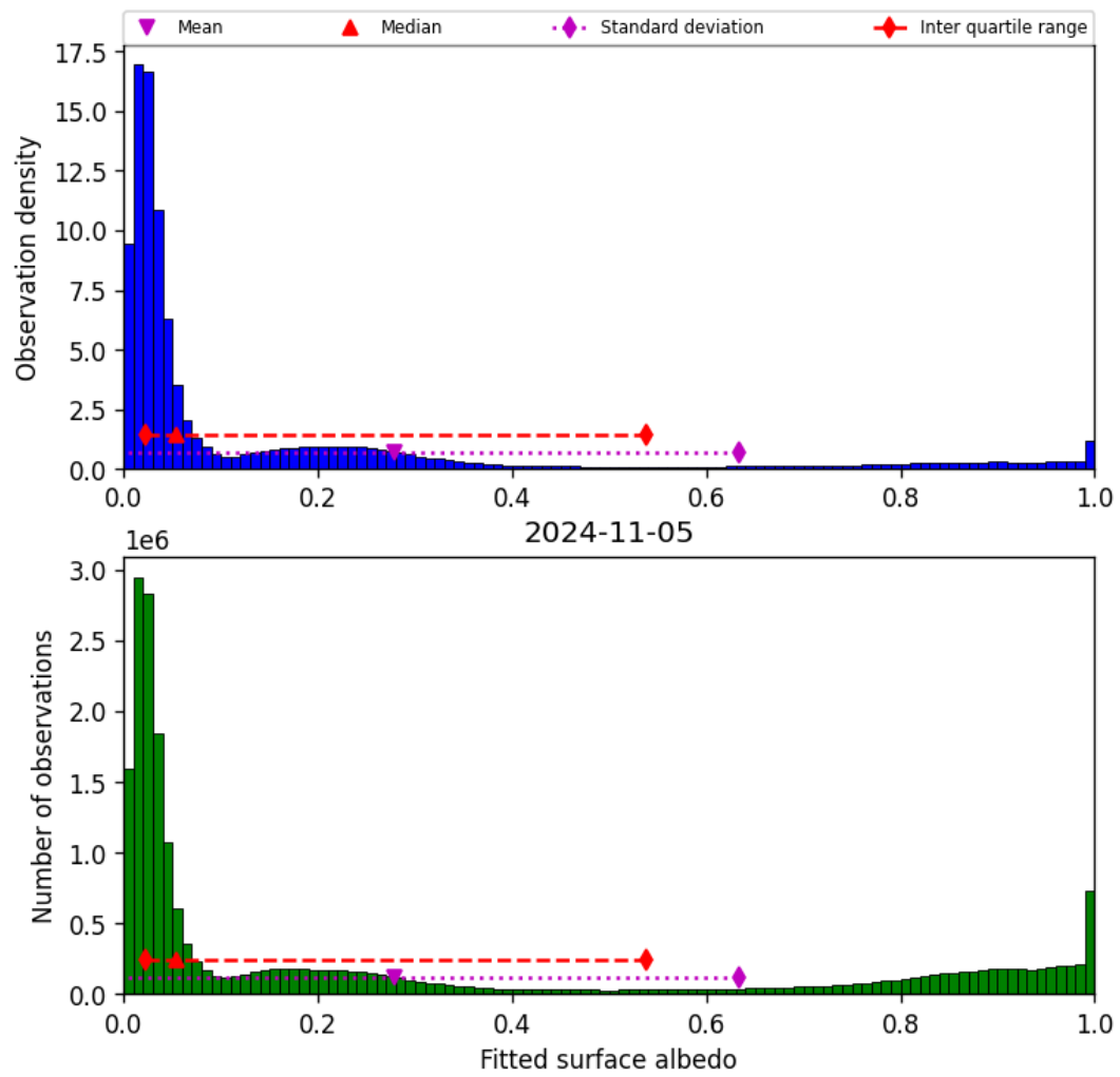
Figure 45: Histogram of “Fitted surface albedo” for 2024-11-04 to 2024-11-06
