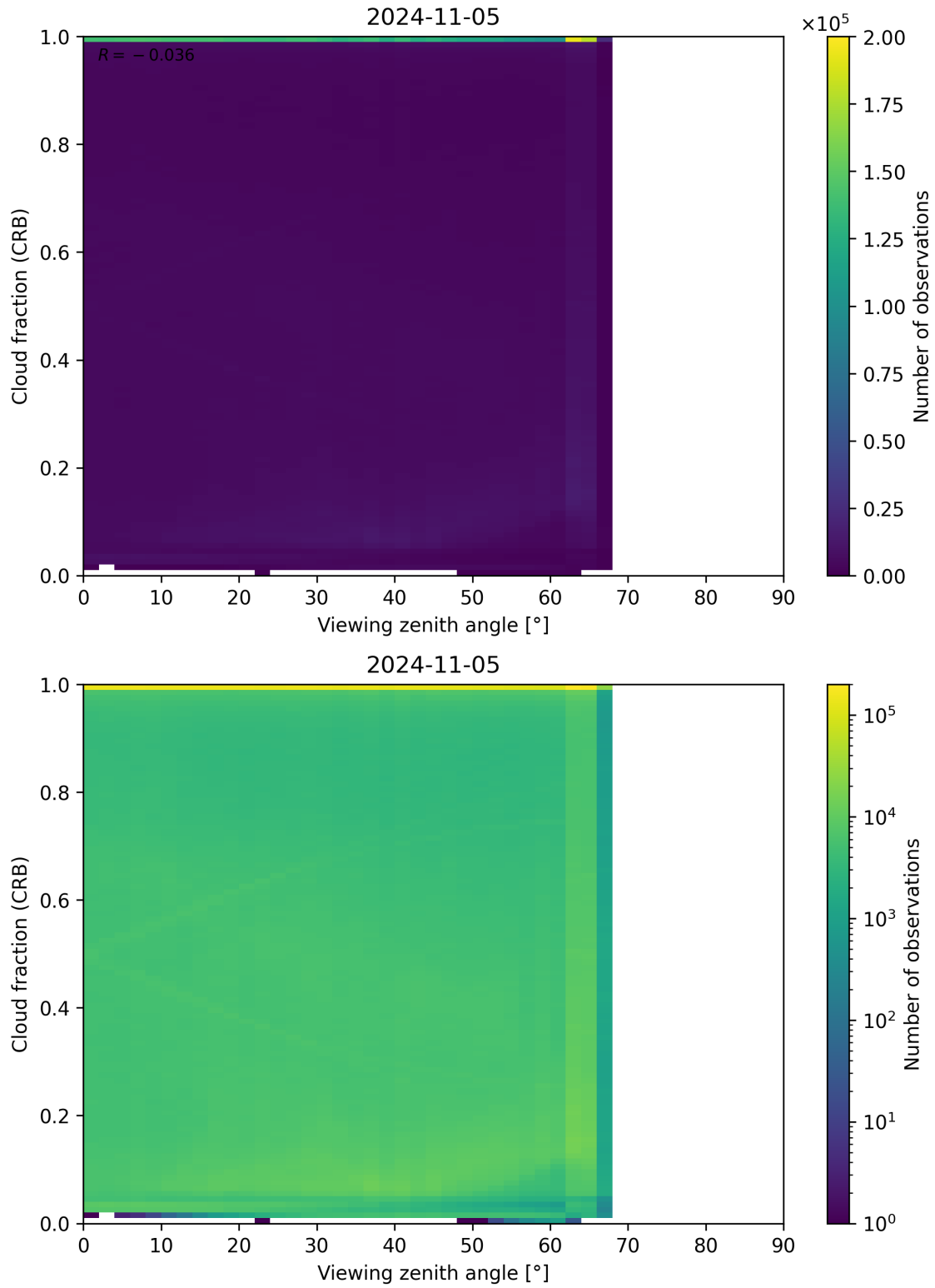
Figure 109: Scatter density plot of “Viewing zenith angle” against “Cloud fraction (CRB)” for 2024-11-04 to 2024-11-06.
