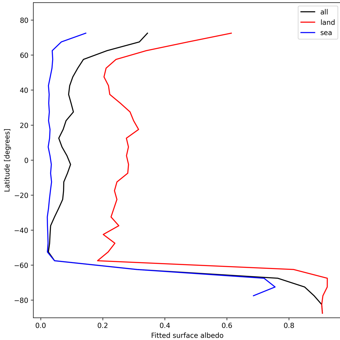
Figure 29: Zonal average of “Fitted surface albedo” for 2024-11-04 to 2024-11-06.
