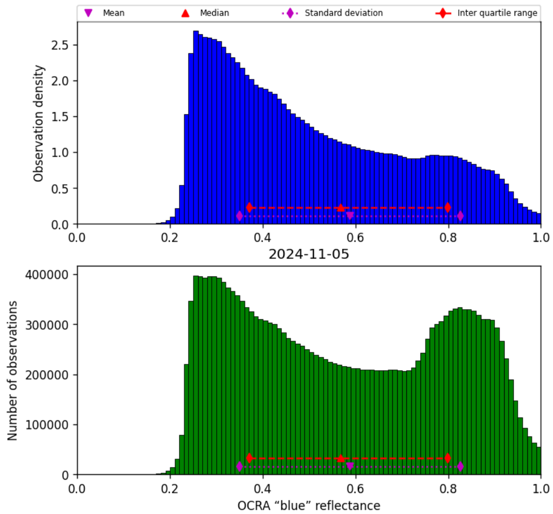
Figure 51: Histogram of “OCRA “blue” reflectance” for 2024-11-04 to 2024-11-06
