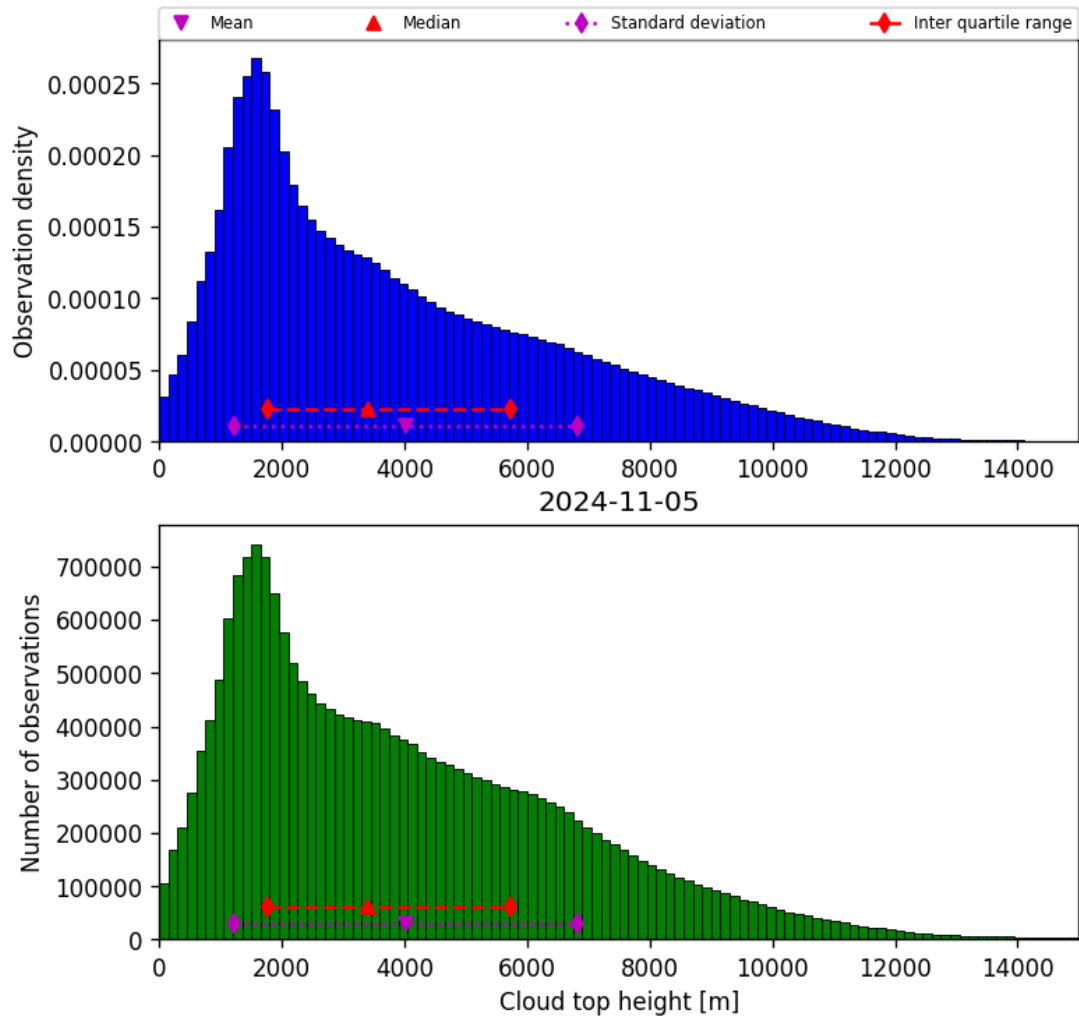
Figure 40: Histogram of “Cloud top height” for 2024-11-04 to 2024-11-06
