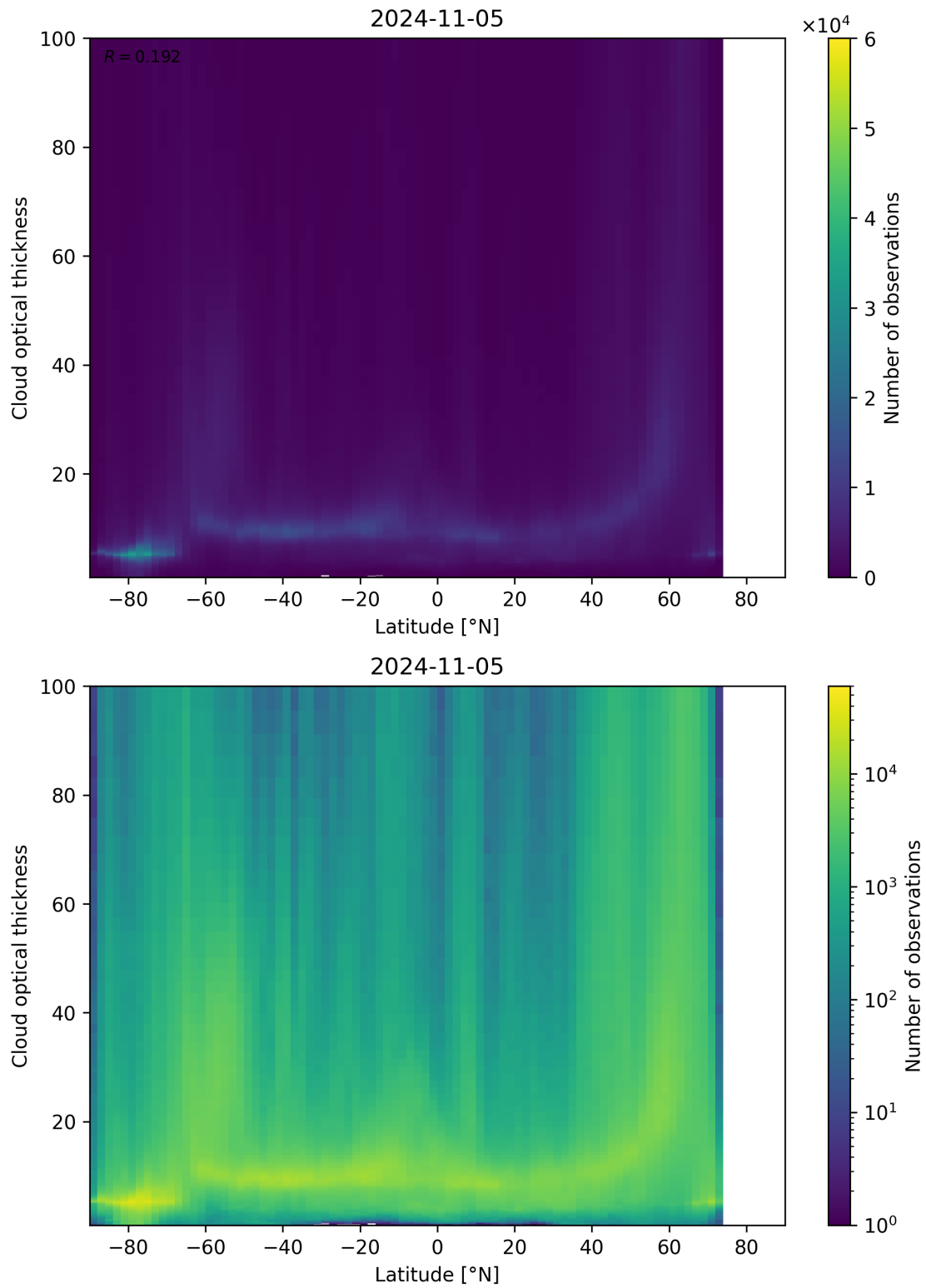
Figure 96: Scatter density plot of “Latitude” against “Cloud optical thickness” for 2024-11-04 to 2024-11-06.
