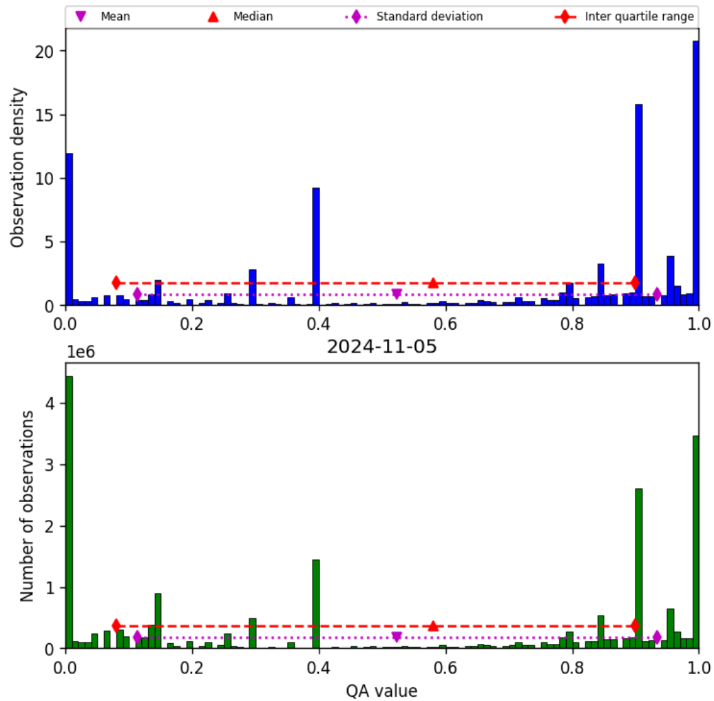
Figure 38: Histogram of “QA value” for 2024-11-04 to 2024-11-06
