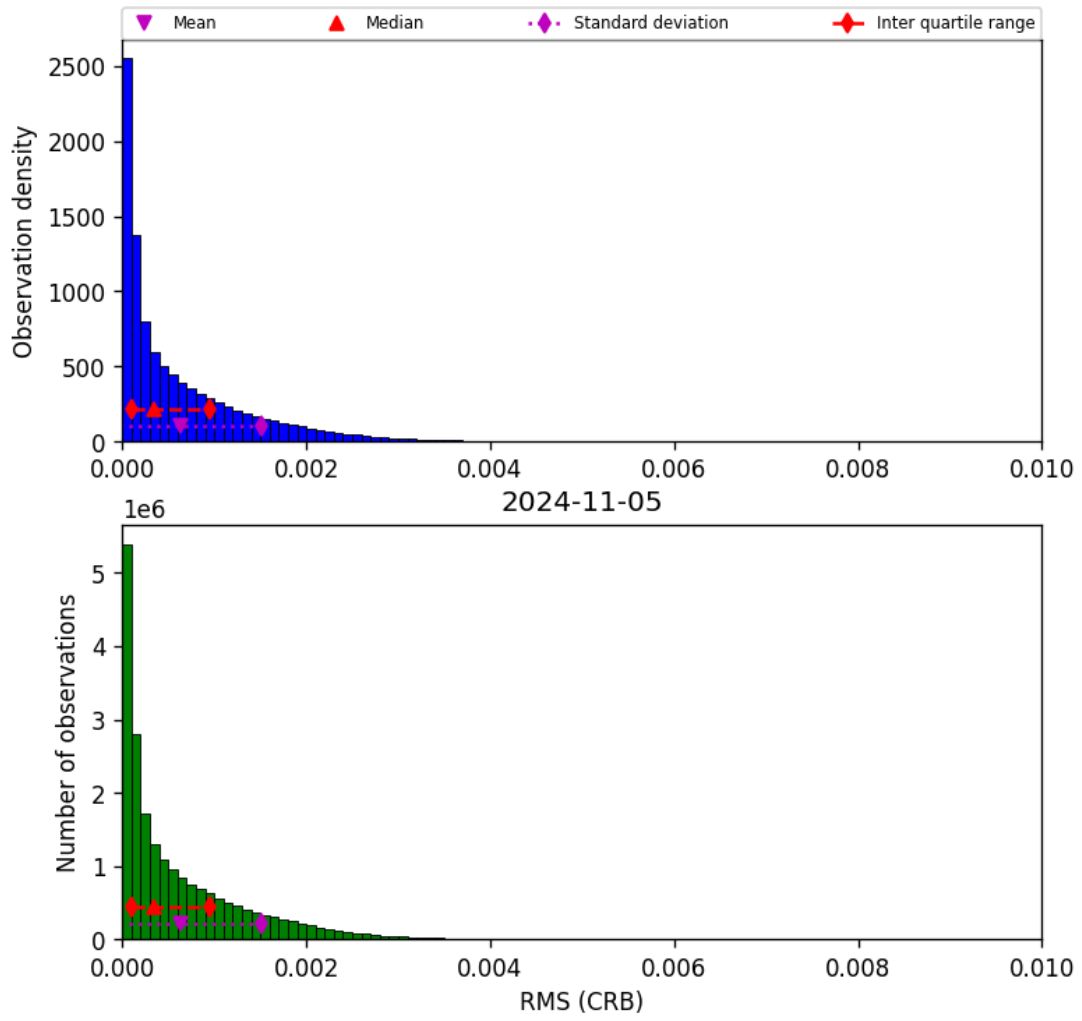
Figure 48: Histogram of “RMS (CRB)” for 2024-11-04 to 2024-11-06
