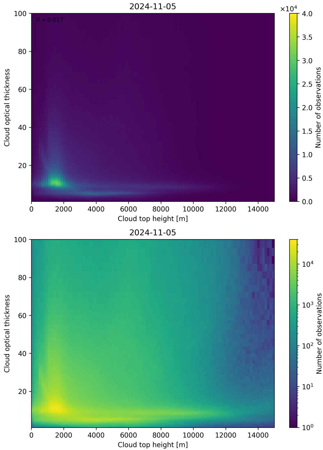
Figure 90: Scatter density plot of “Cloud top height” against “Cloud optical thickness” for 2024-11-04 to 2024-11-06.
