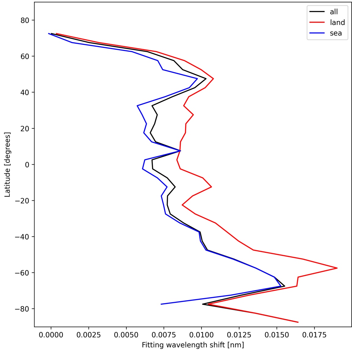
Figure 33: Zonal average of “Fitting wavelength shift” for 2024-11-04 to 2024-11-06.
