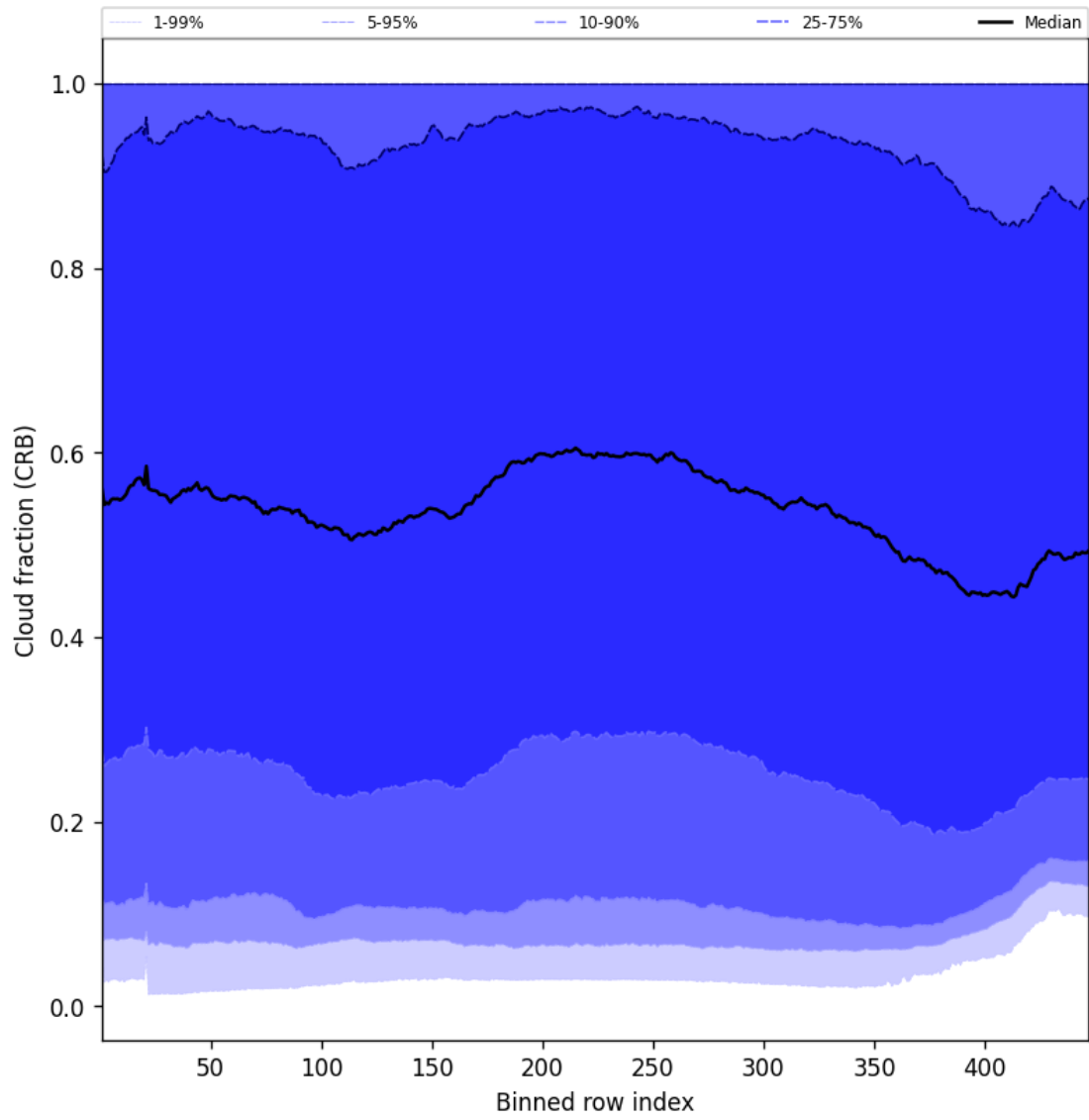
Figure 58: Along track statistics of “Cloud fraction (CRB)” for 2024-11-04 to 2024-11-06
