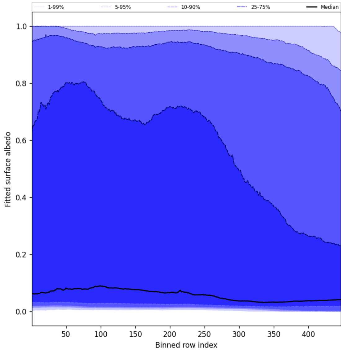
Figure 61: Along track statistics of “Fitted surface albedo” for 2024-11-04 to 2024-11-06
