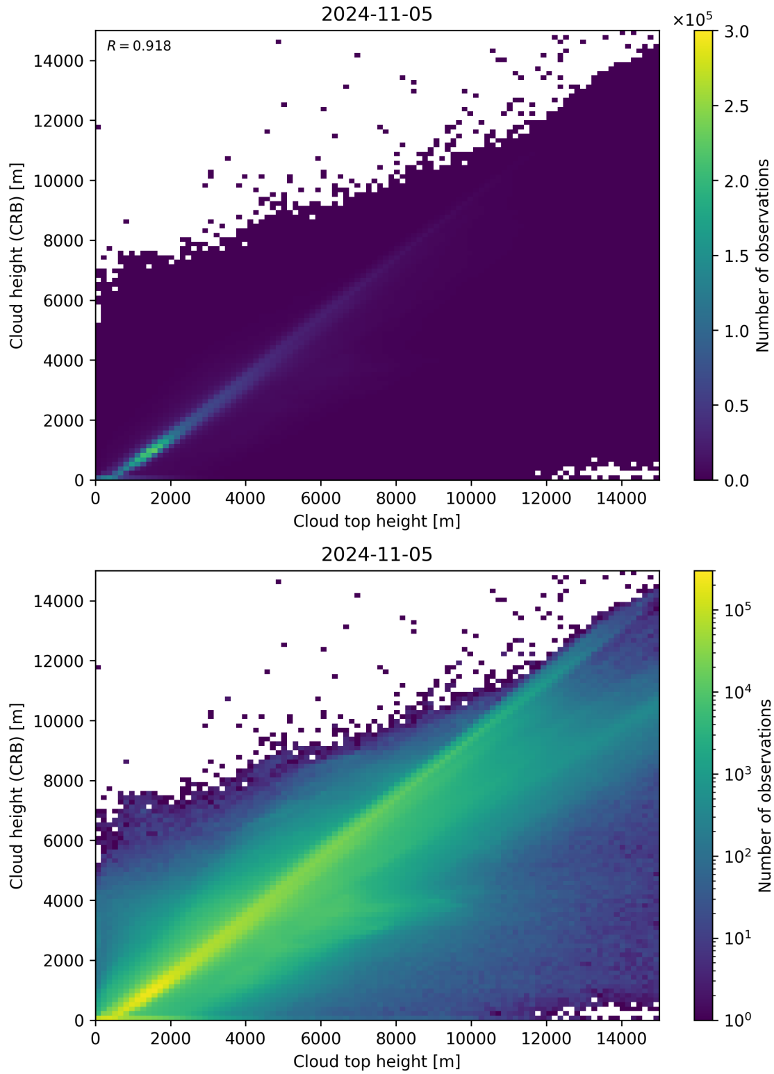
Figure 89: Scatter density plot of “Cloud top height” against “Cloud height (CRB)” for 2024-11-04 to 2024-11-06.
