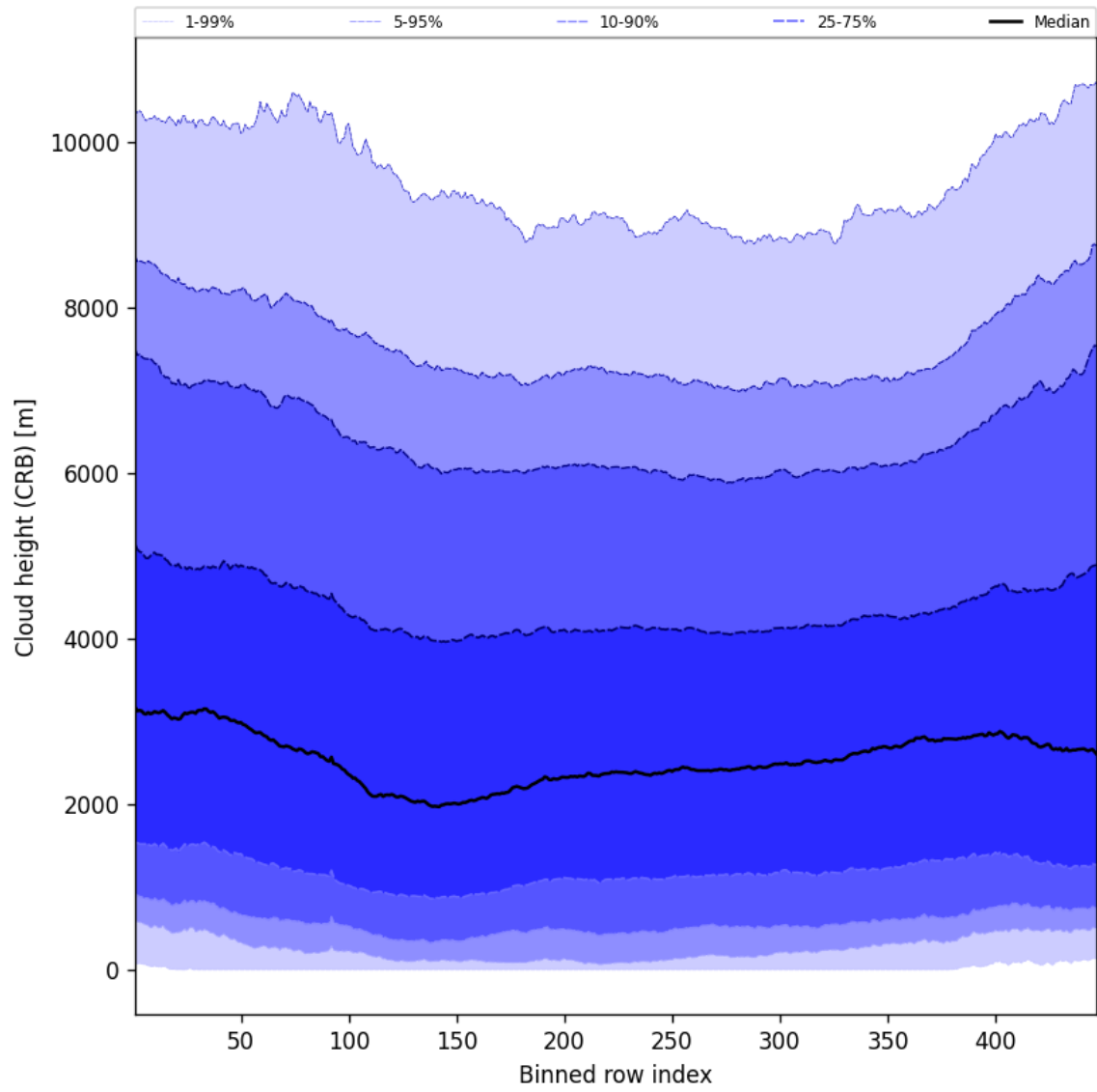
Figure 59: Along track statistics of “Cloud height (CRB)” for 2024-11-04 to 2024-11-06
