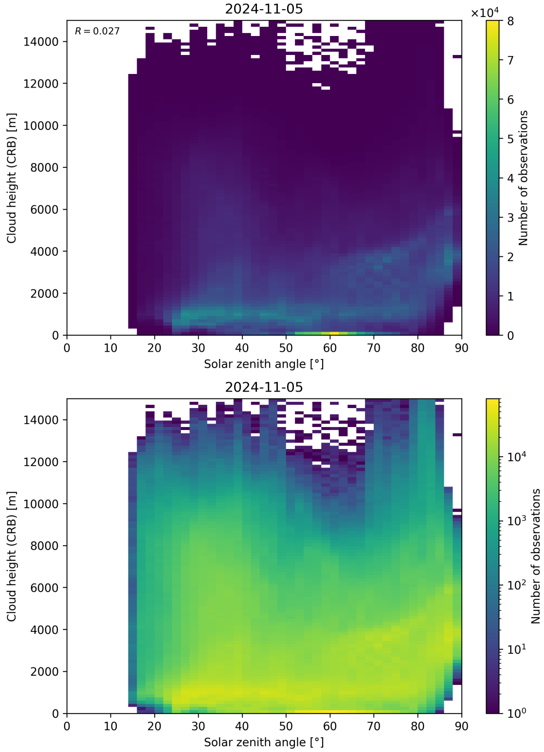
Figure 102: Scatter density plot of “Solar zenith angle” against “Cloud height (CRB)” for 2024-11-04 to 2024-11-06.
