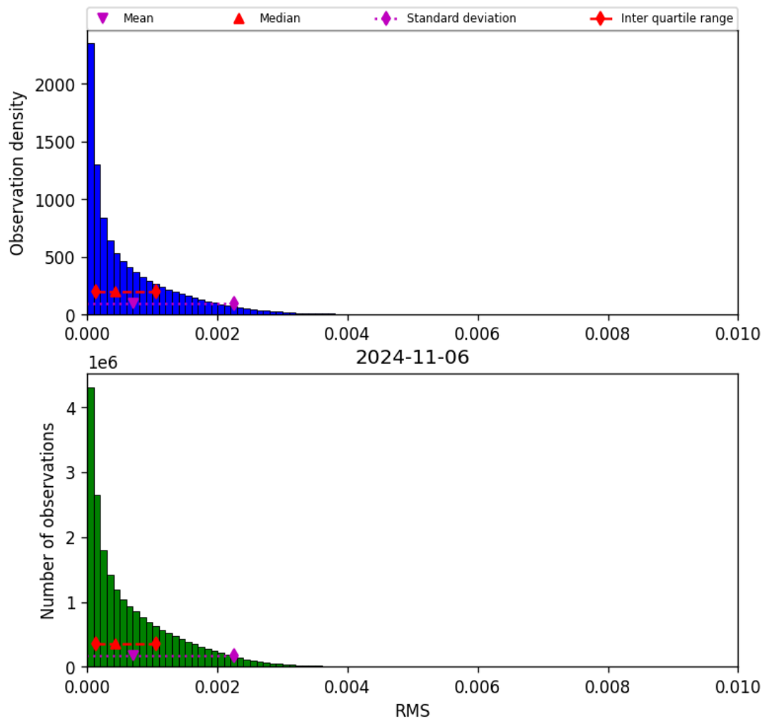
Figure 47: Histogram of “RMS” for 2024-11-05 to 2024-11-07
