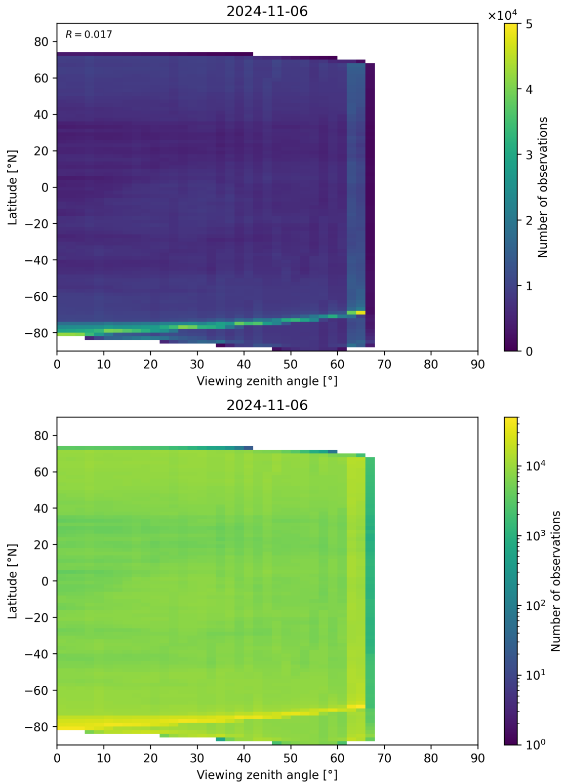
Figure 113: Scatter density plot of “Viewing zenith angle” against “Latitude” for 2024-11-05 to 2024-11-07.
