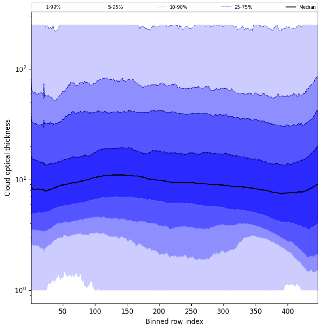
Figure 57: Along track statistics of “Cloud optical thickness” for 2024-11-05 to 2024-11-07
