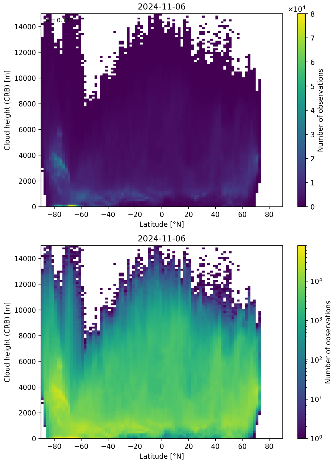
Figure 95: Scatter density plot of “Latitude” against “Cloud height (CRB)” for 2024-11-05 to 2024-11-07.
