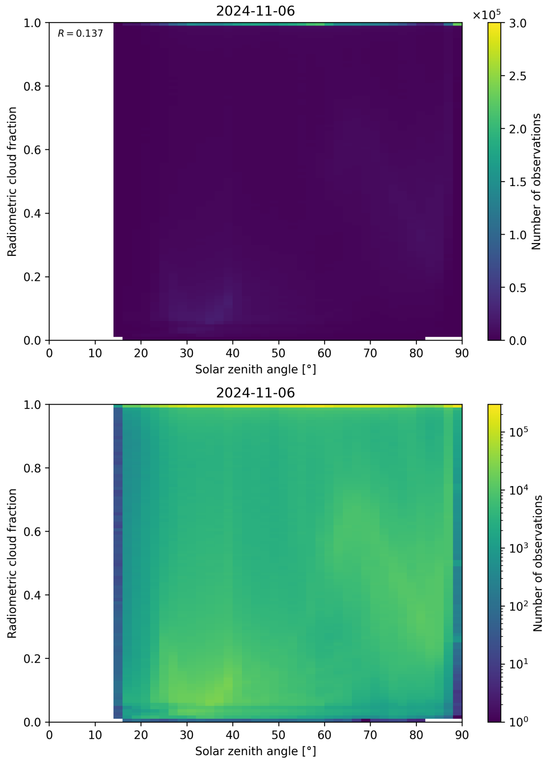
Figure 99: Scatter density plot of “Solar zenith angle” against “Radiometric cloud fraction” for 2024-11-05 to 2024-11-07.
