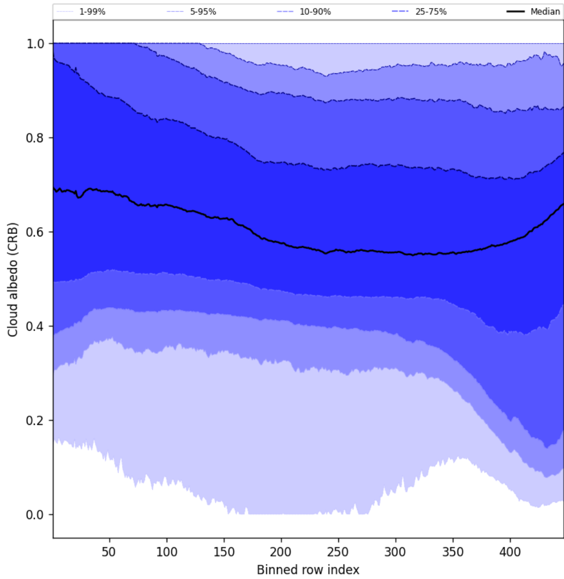
Figure 60: Along track statistics of “Cloud albedo (CRB)” for 2024-11-05 to 2024-11-07
