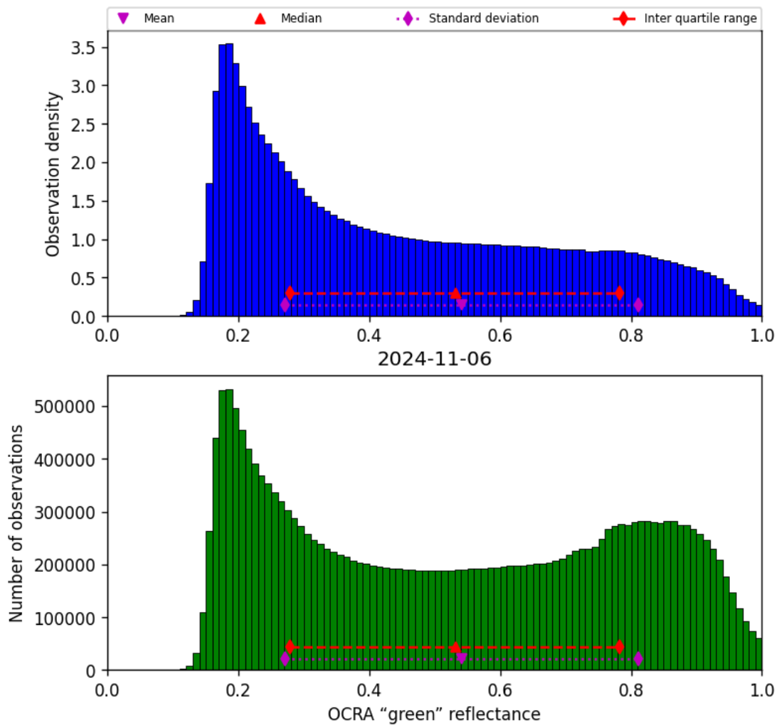
Figure 52: Histogram of “OCRA “green” reflectance” for 2024-11-05 to 2024-11-07
