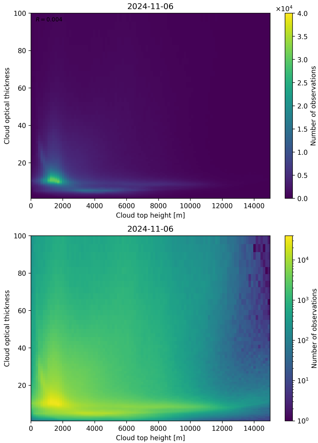
Figure 90: Scatter density plot of “Cloud top height” against “Cloud optical thickness” for 2024-11-05 to 2024-11-07.
