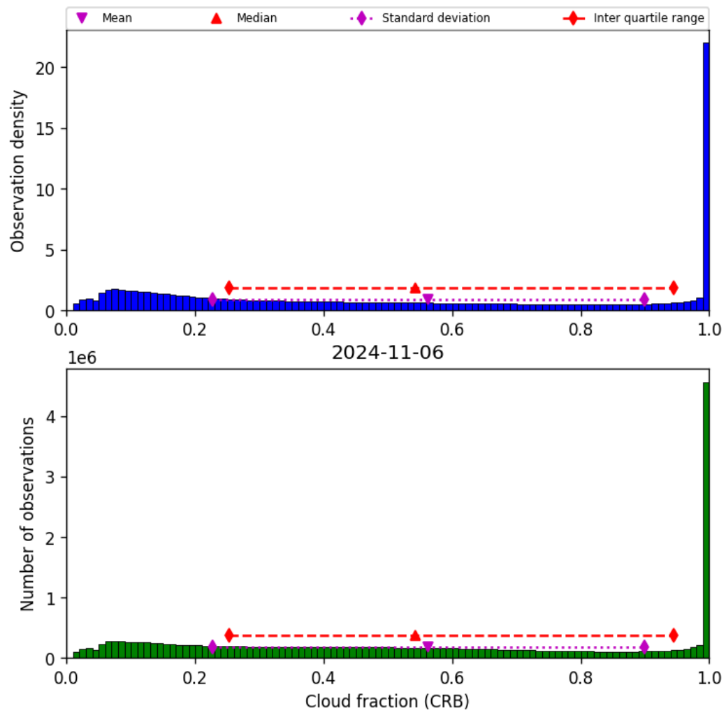
Figure 42: Histogram of “Cloud fraction (CRB)” for 2024-11-05 to 2024-11-07
