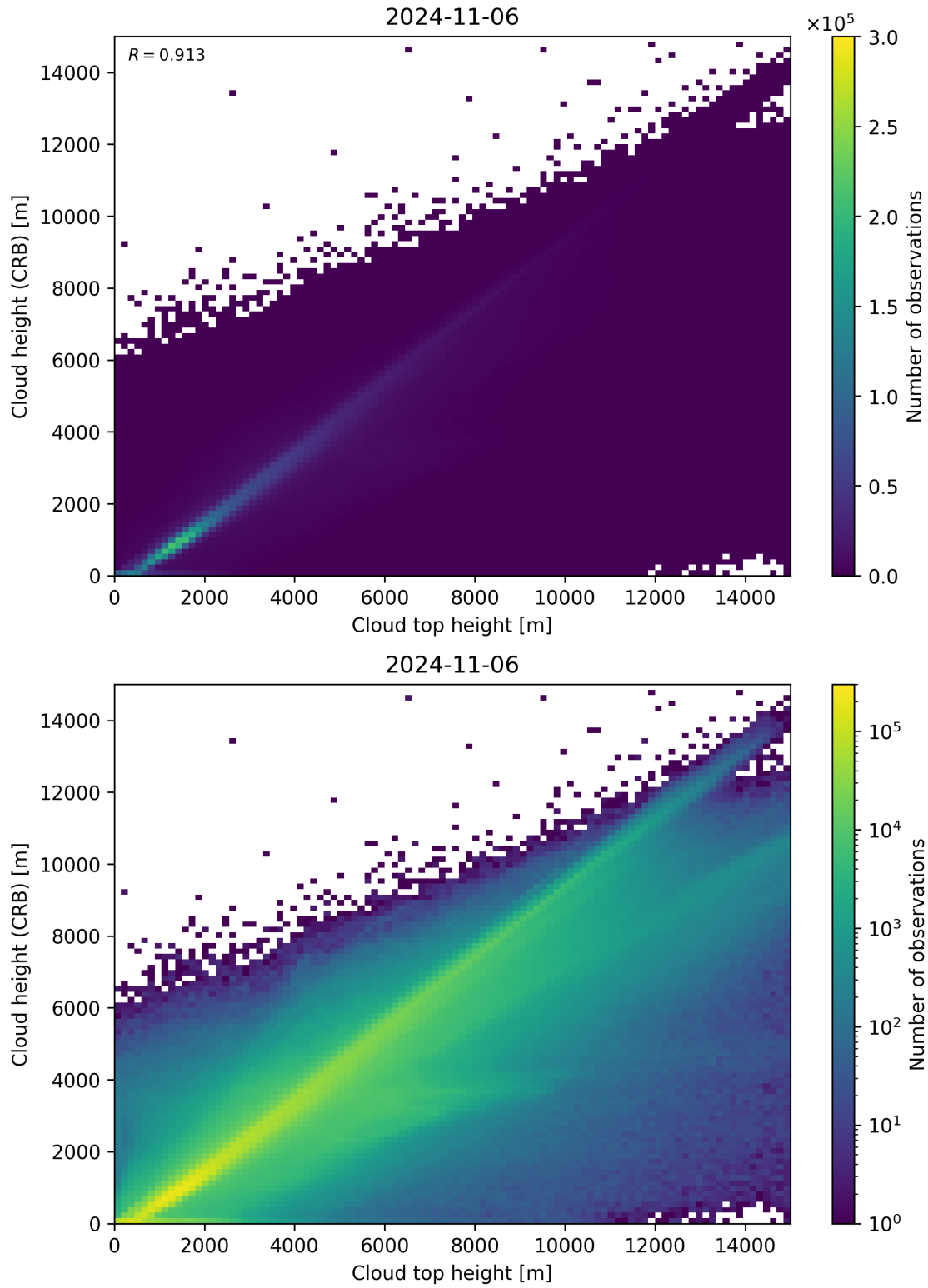
Figure 89: Scatter density plot of “Cloud top height” against “Cloud height (CRB)” for 2024-11-05 to 2024-11-07.
