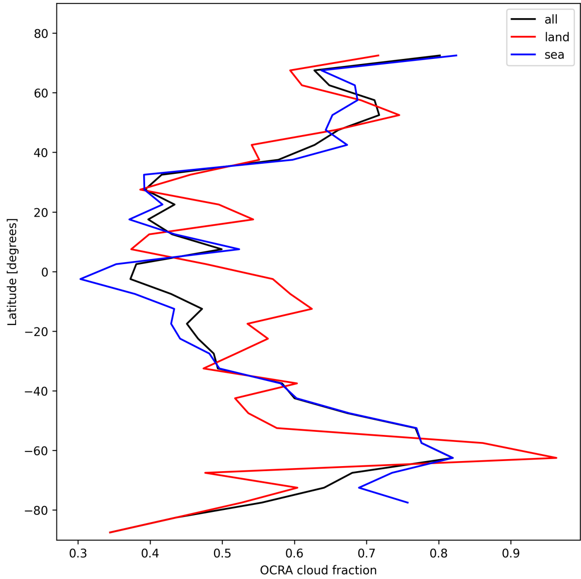
Figure 34: Zonal average of “OCRA cloud fraction” for 2024-11-05 to 2024-11-07.
