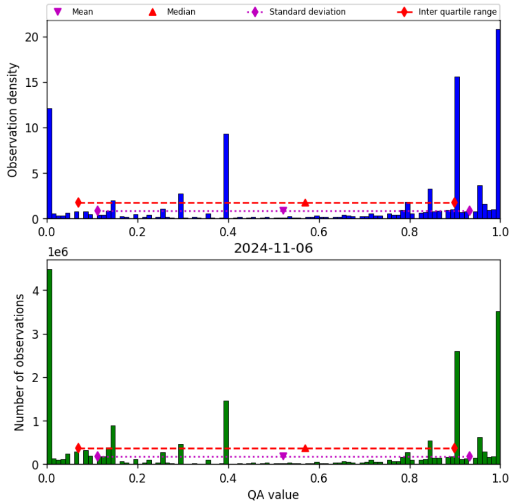
Figure 38: Histogram of “QA value” for 2024-11-05 to 2024-11-07
