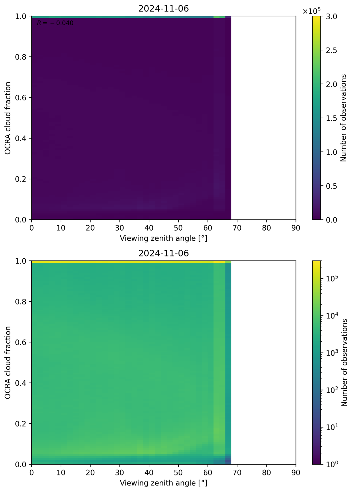
Figure 108: Scatter density plot of “Viewing zenith angle” against “OCRA cloud fraction” for 2024-11-05 to 2024-11-07.
