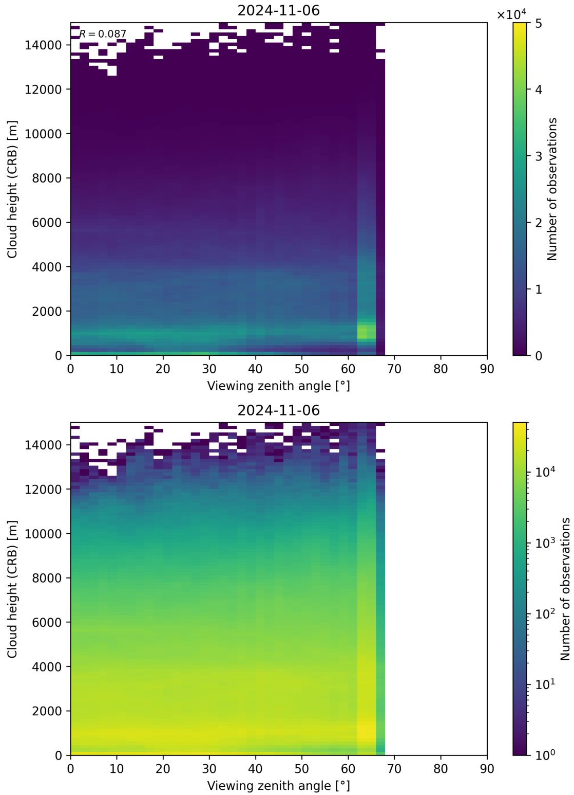
Figure 110: Scatter density plot of “Viewing zenith angle” against “Cloud height (CRB)” for 2024-11-05 to 2024-11-07.
