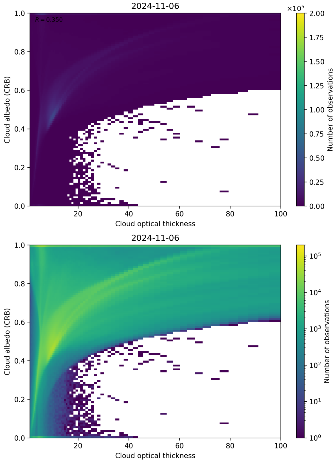
Figure 82: Scatter density plot of “Cloud optical thickness” against “Cloud albedo (CRB)” for 2024-11-05 to 2024-11-07.
