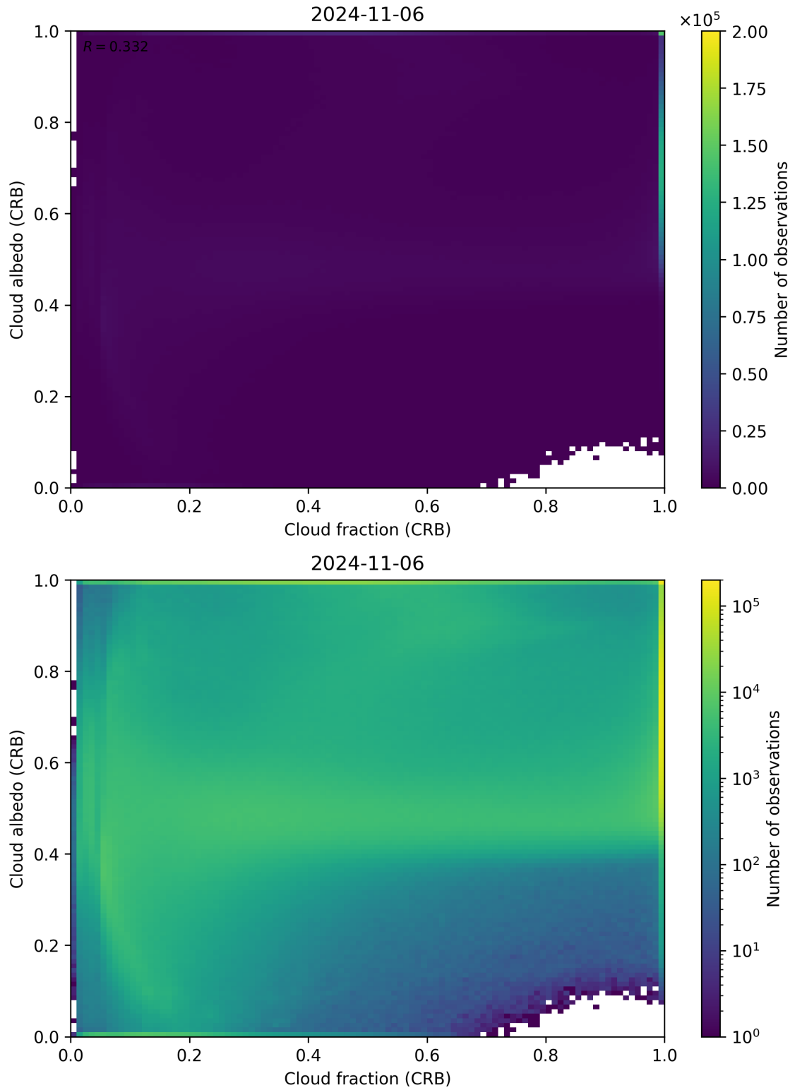
Figure 77: Scatter density plot of “Cloud fraction (CRB)” against “Cloud albedo (CRB)” for 2024-11-05 to 2024-11-07.
