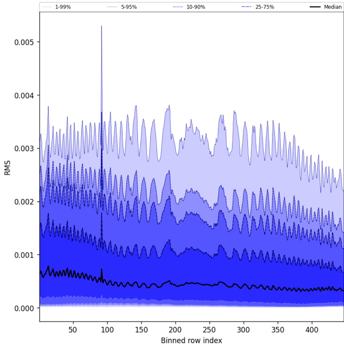
Figure 63: Along track statistics of “RMS” for 2024-11-05 to 2024-11-07
