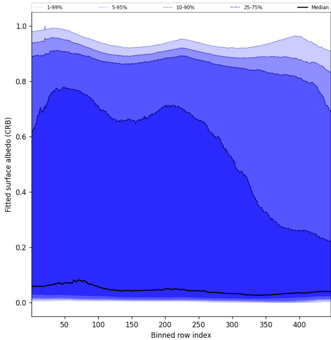
Figure 62: Along track statistics of “Fitted surface albedo (CRB)” for 2024-11-05 to 2024-11-07
