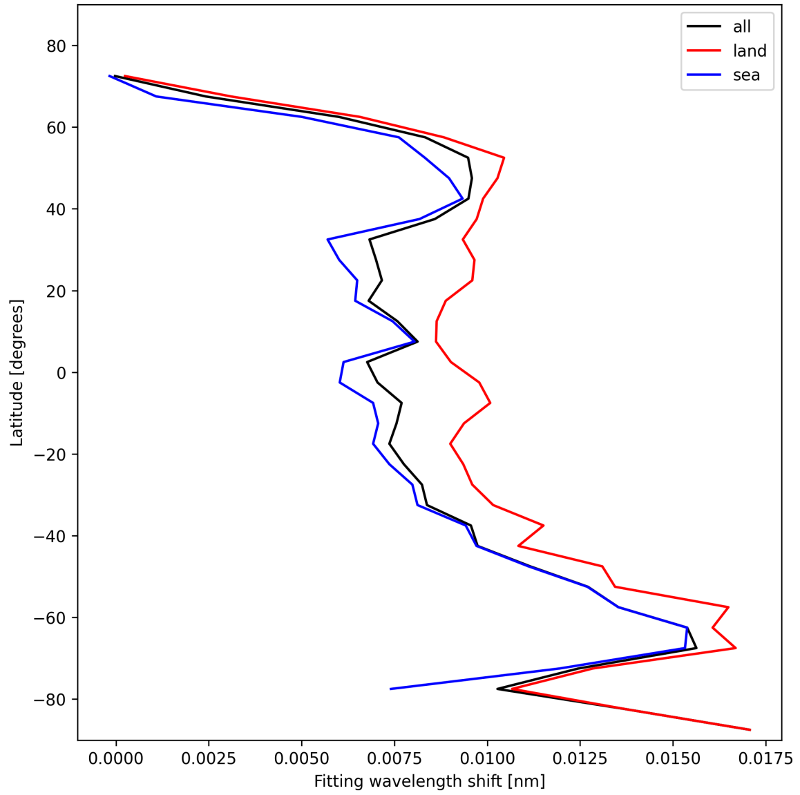
Figure 33: Zonal average of “Fitting wavelength shift” for 2024-11-05 to 2024-11-07.
