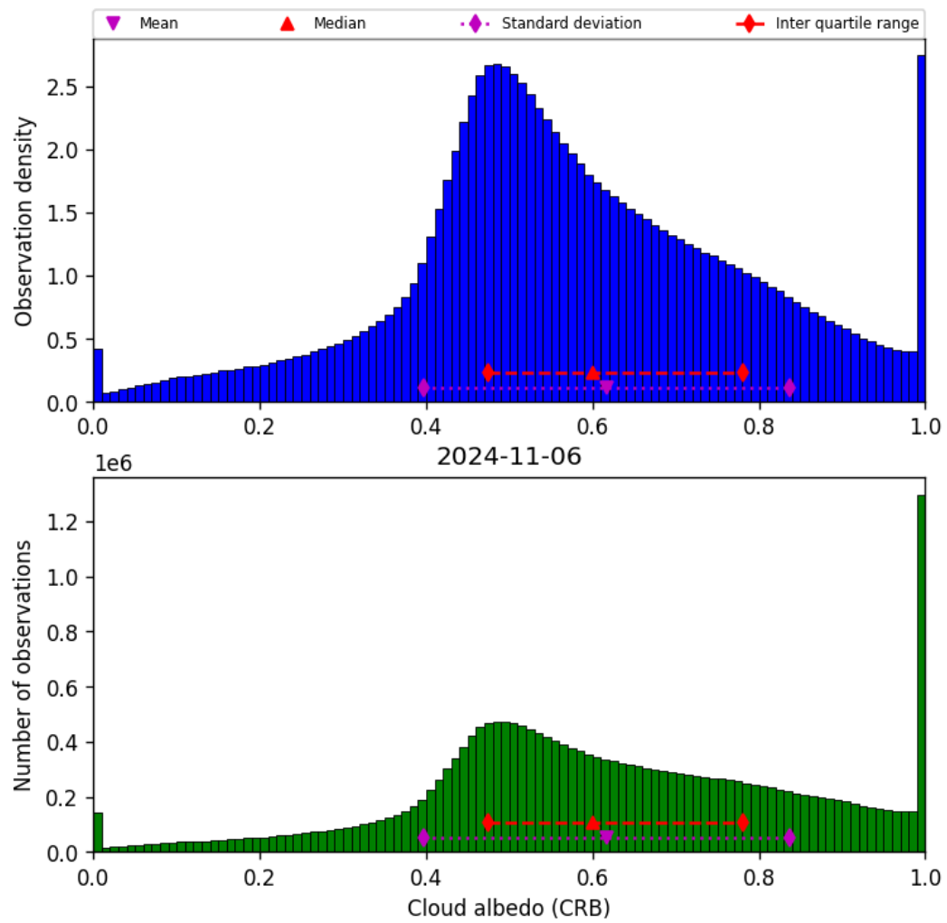
Figure 44: Histogram of “Cloud albedo (CRB)” for 2024-11-05 to 2024-11-07
