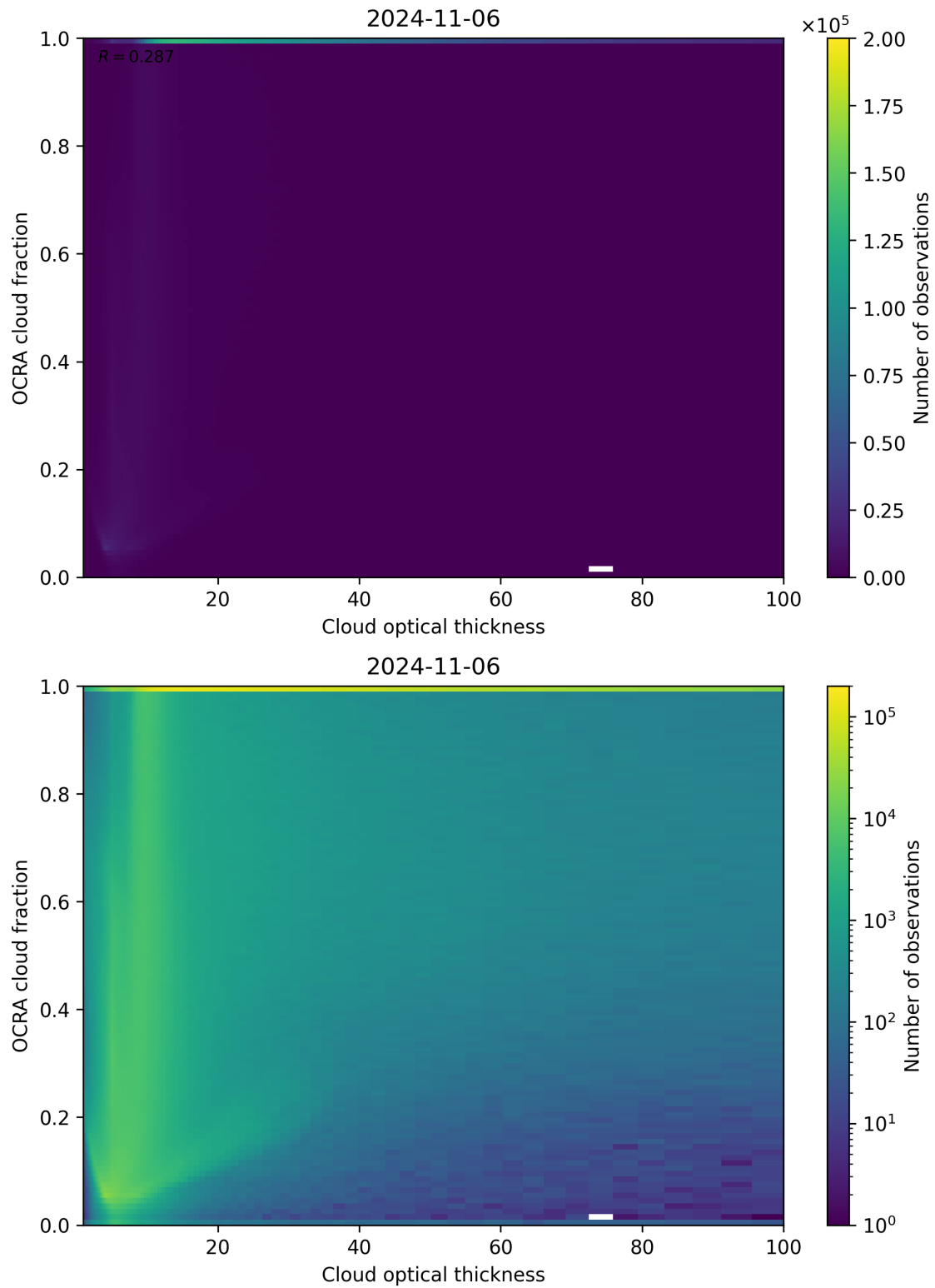
Figure 83: Scatter density plot of “Cloud optical thickness” against “OCRA cloud fraction” for 2024-11-05 to 2024-11-07.
