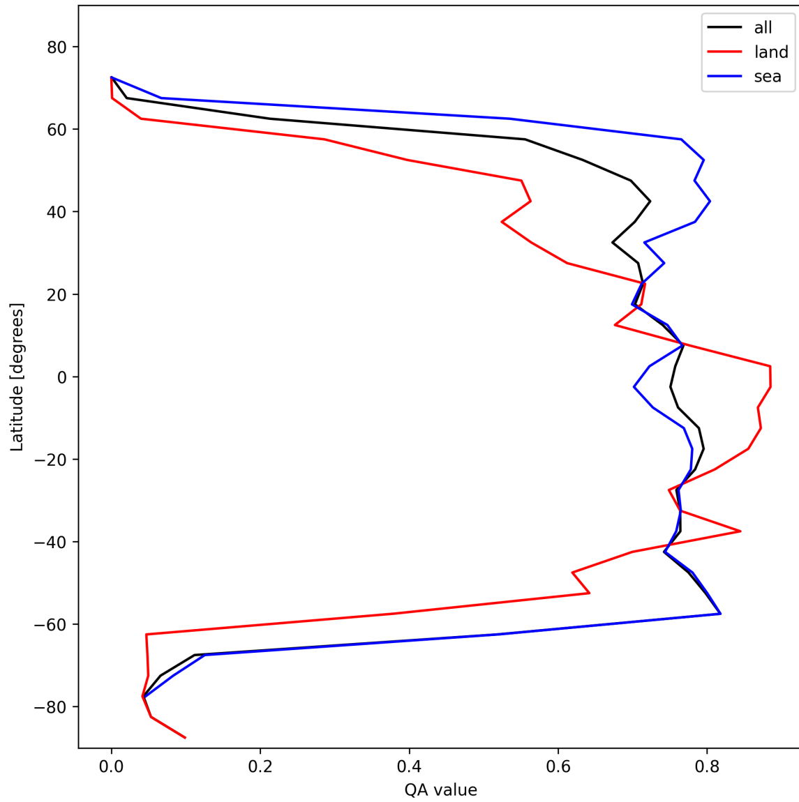
Figure 22: Zonal average of “QA value” for 2024-11-05 to 2024-11-07.
