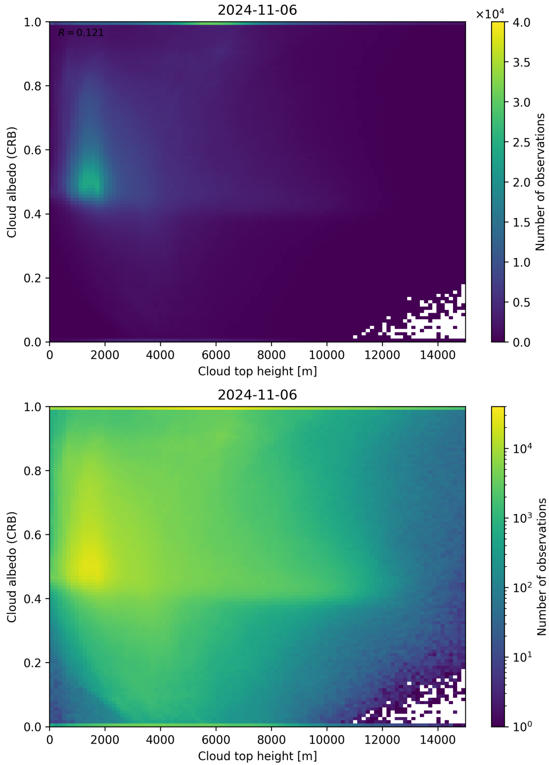
Figure 86: Scatter density plot of “Cloud top height” against “Cloud albedo (CRB)” for 2024-11-05 to 2024-11-07.
