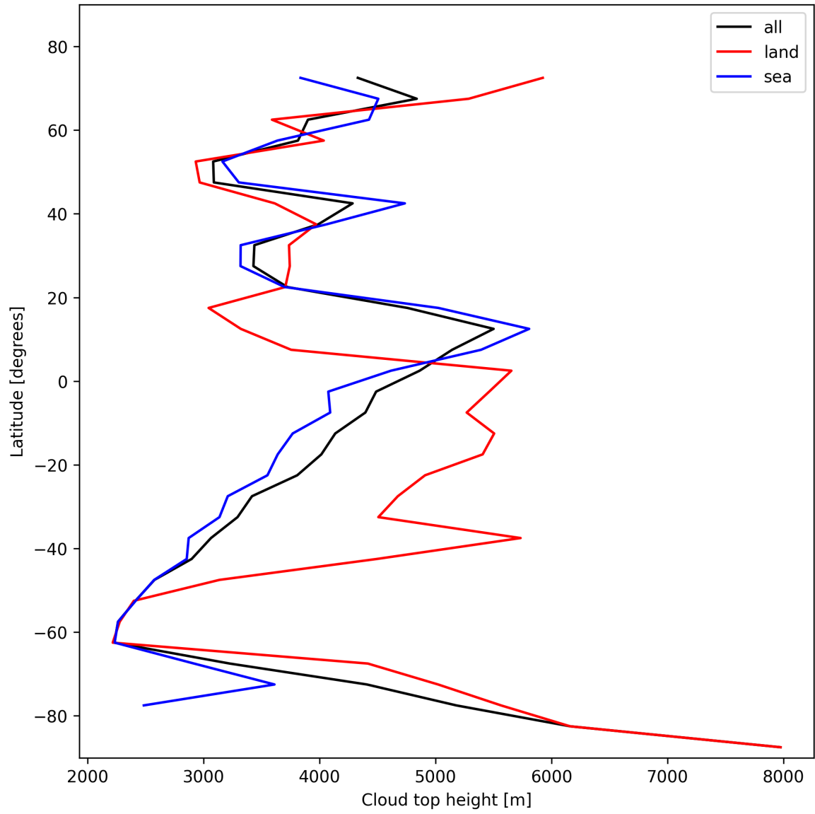
Figure 24: Zonal average of “Cloud top height” for 2024-11-05 to 2024-11-07.
