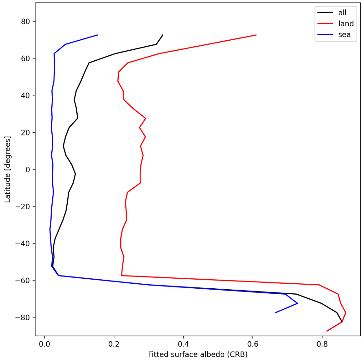
Figure 30: Zonal average of “Fitted surface albedo (CRB)” for 2024-11-05 to 2024-11-07.
