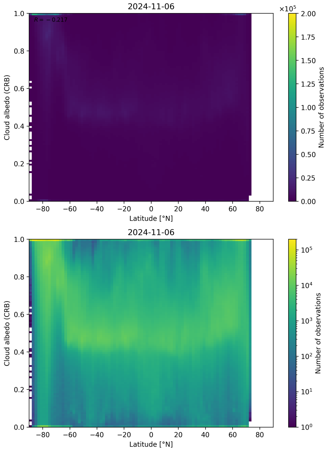
Figure 91: Scatter density plot of “Latitude” against “Cloud albedo (CRB)” for 2024-11-05 to 2024-11-07.
