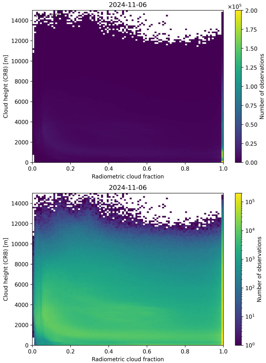
Figure 74: Scatter density plot of “Radiometric cloud fraction” against “Cloud height (CRB)” for 2024-11-05 to 2024-11-07.
