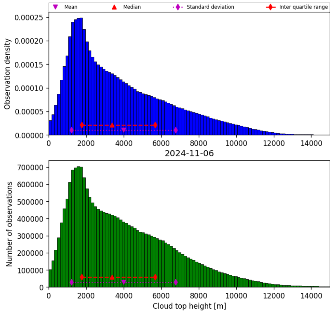
Figure 40: Histogram of “Cloud top height” for 2024-11-05 to 2024-11-07
