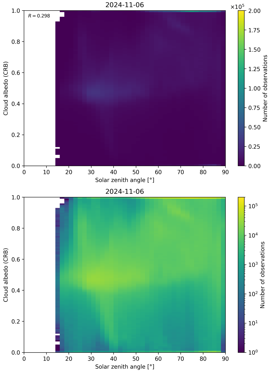
Figure 98: Scatter density plot of “Solar zenith angle” against “Cloud albedo (CRB)” for 2024-11-05 to 2024-11-07.
