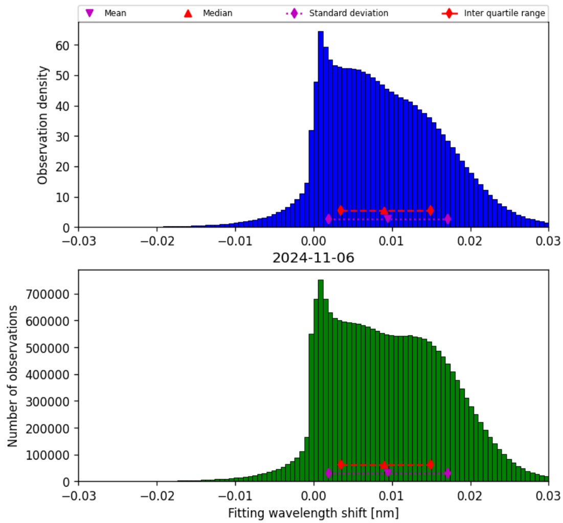
Figure 49: Histogram of “Fitting wavelength shift” for 2024-11-05 to 2024-11-07
