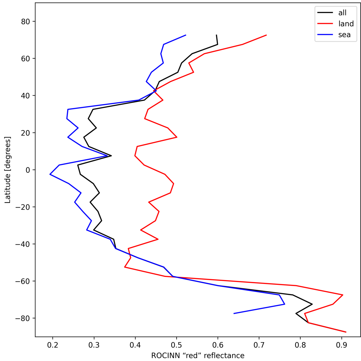
Figure 37: Zonal average of "ROCINN "red" reflectance" for 2024-11-05 to 2024-11-07.
