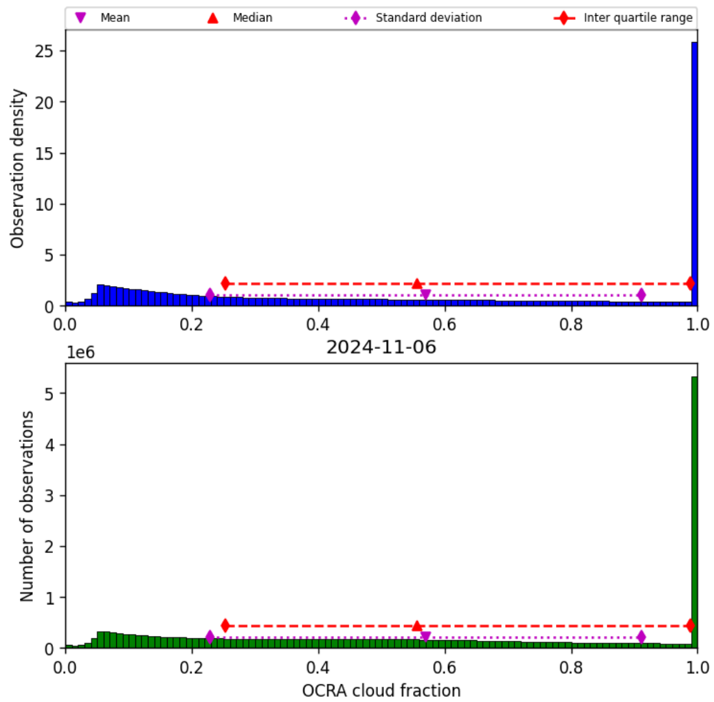
Figure 50: Histogram of “OCRA cloud fraction” for 2024-11-05 to 2024-11-07
