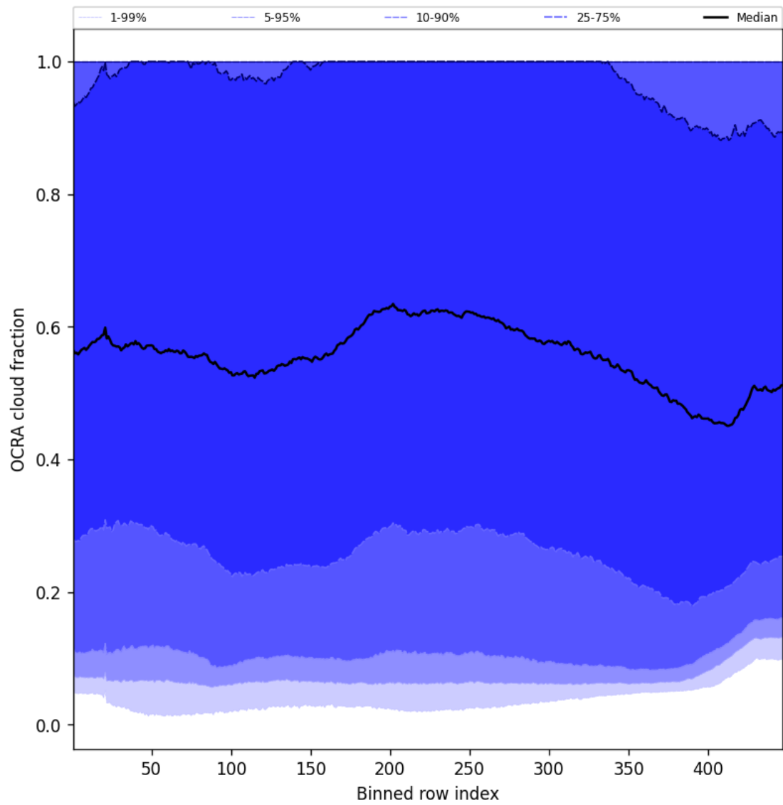
Figure 66: Along track statistics of “OCRA cloud fraction” for 2024-11-05 to 2024-11-07
