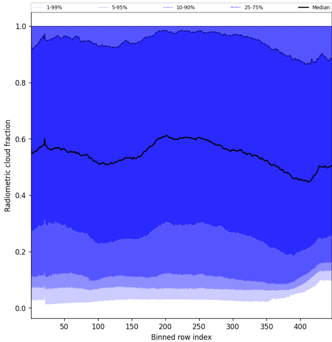
Figure 55: Along track statistics of “Radiometric cloud fraction” for 2024-11-05 to 2024-11-07
