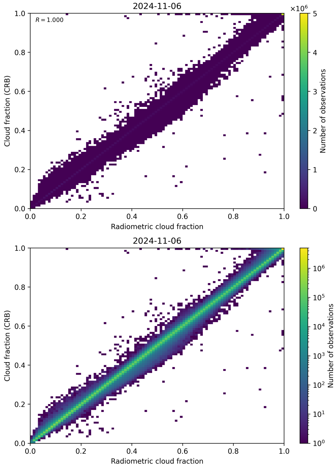
Figure 73: Scatter density plot of “Radiometric cloud fraction” against “Cloud fraction (CRB)” for 2024-11-05 to 2024-11-07.
