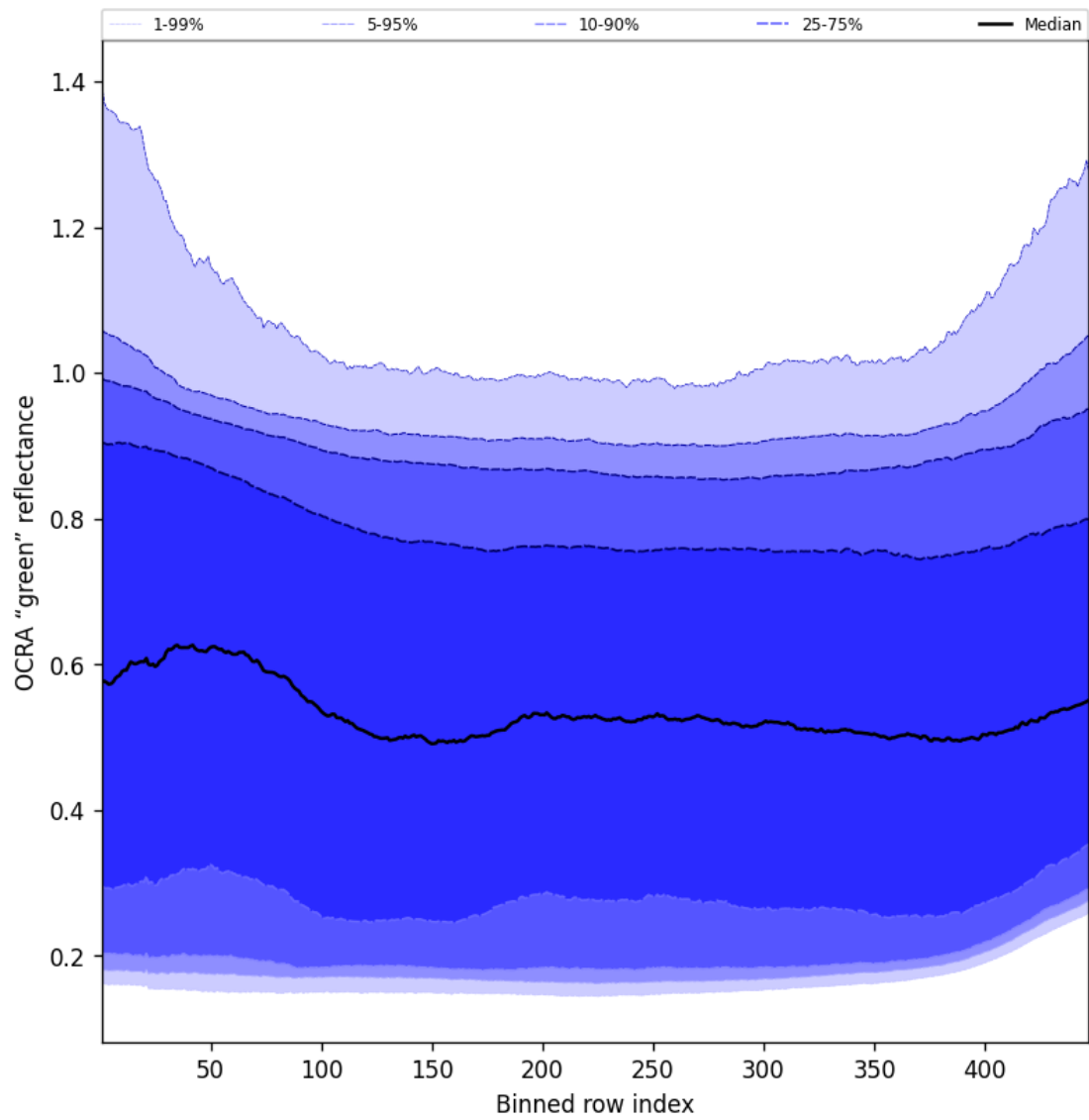
Figure 68: Along track statistics of “OCRA “green” reflectance” for 2024-11-05 to 2024-11-07
