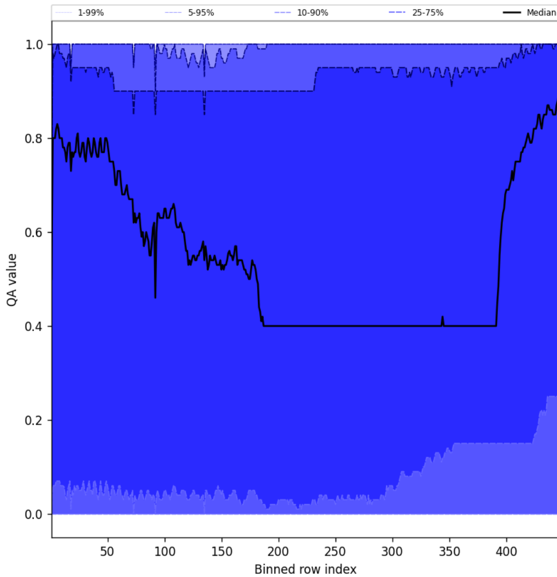
Figure 54: Along track statistics of “QA value” for 2024-11-05 to 2024-11-07
