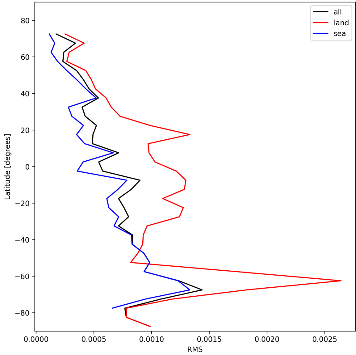
Figure 31: Zonal average of “RMS” for 2024-11-05 to 2024-11-07.
