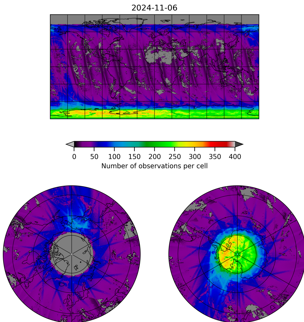
Figure 21: Map of the number of observations for 2024-11-05 to 2024-11-07
