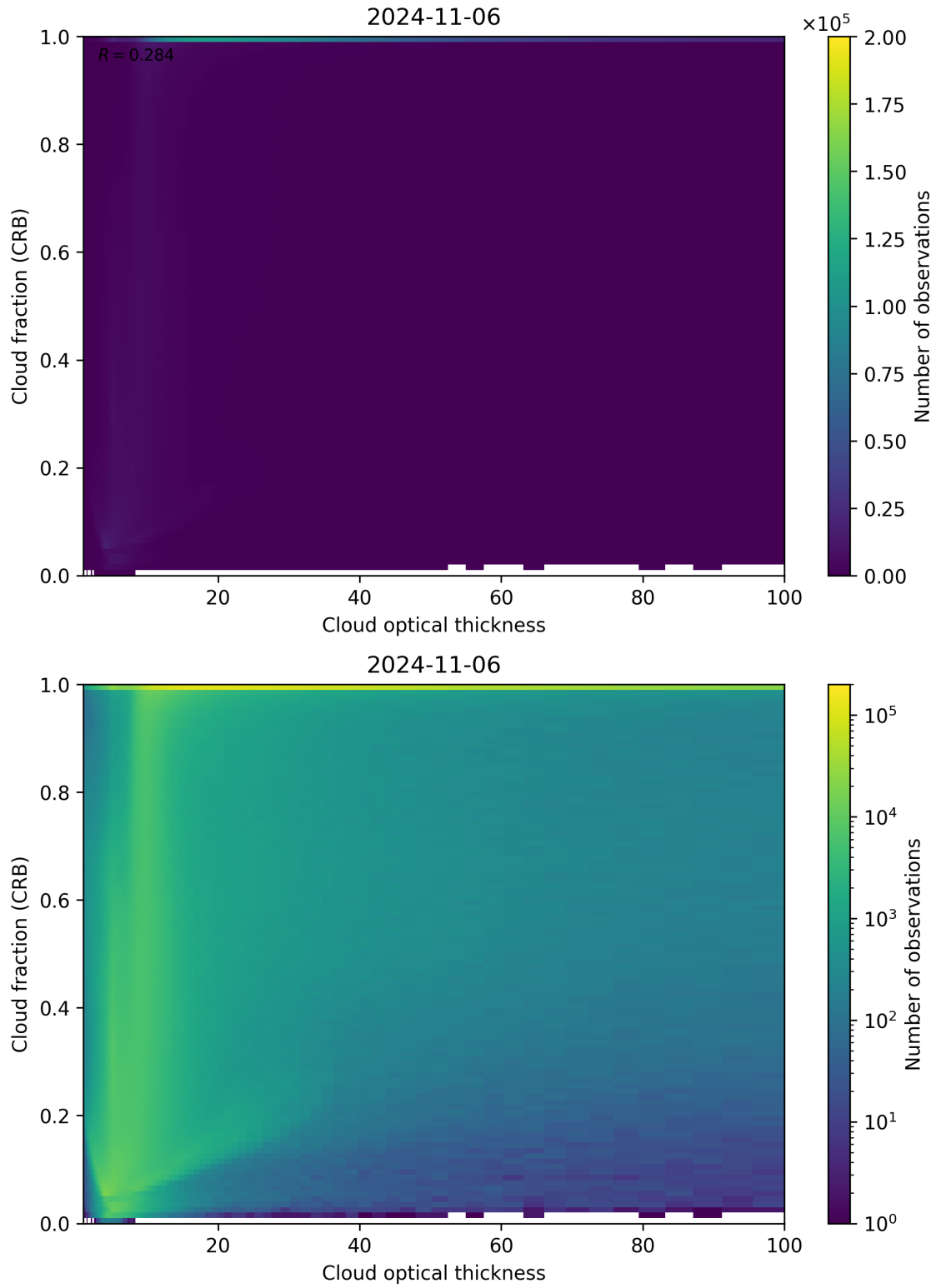
Figure 84: Scatter density plot of “Cloud optical thickness” against “Cloud fraction (CRB)” for 2024-11-05 to 2024-11-07.
