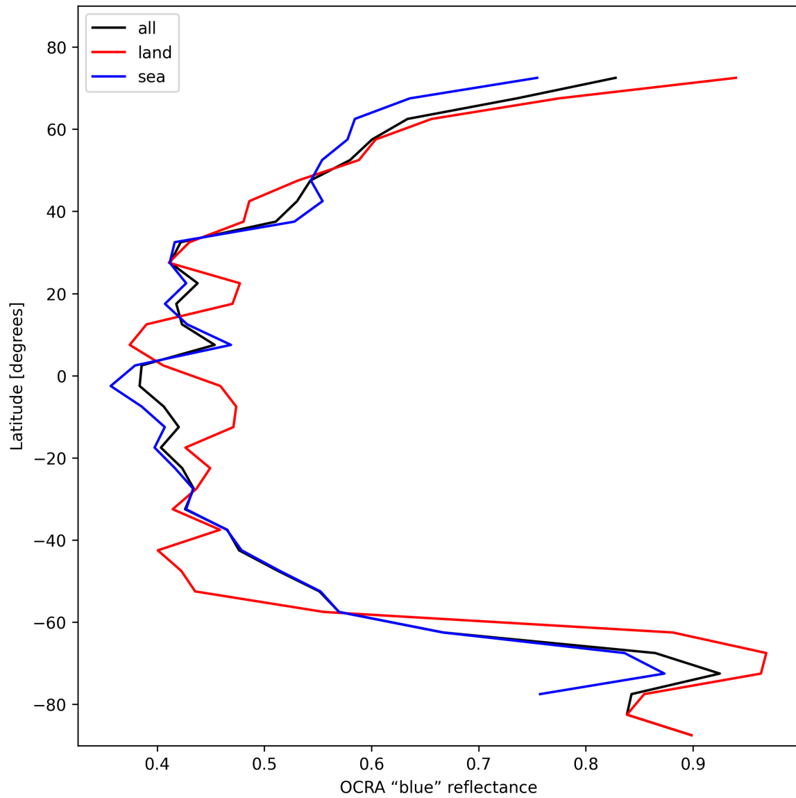
Figure 35: Zonal average of “OCRA “blue” reflectance” for 2024-11-05 to 2024-11-07.
