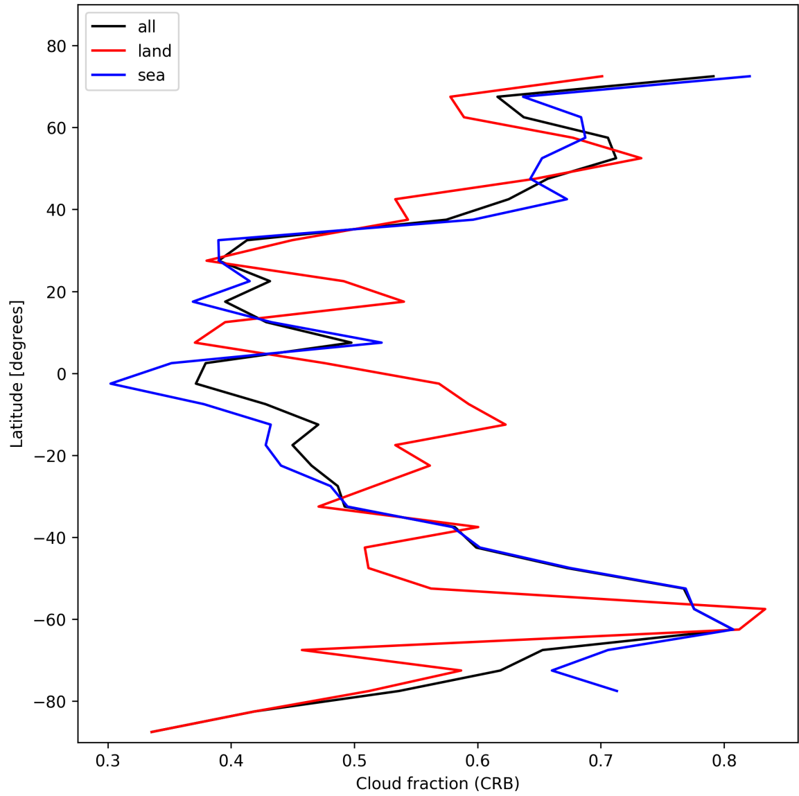
Figure 26: Zonal average of “Cloud fraction (CRB)” for 2024-11-05 to 2024-11-07.
