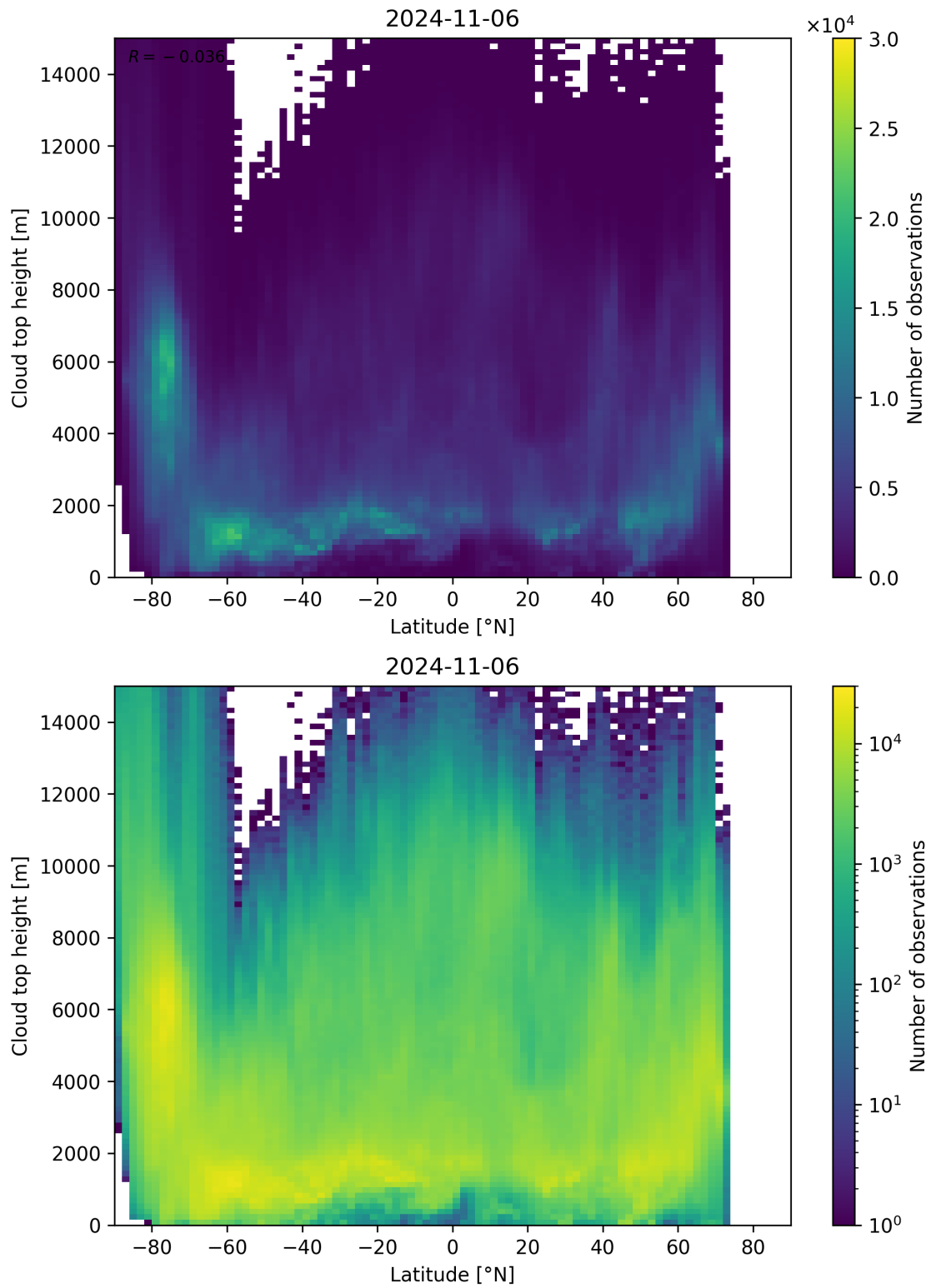
Figure 97: Scatter density plot of “Latitude” against “Cloud top height” for 2024-11-05 to 2024-11-07.
