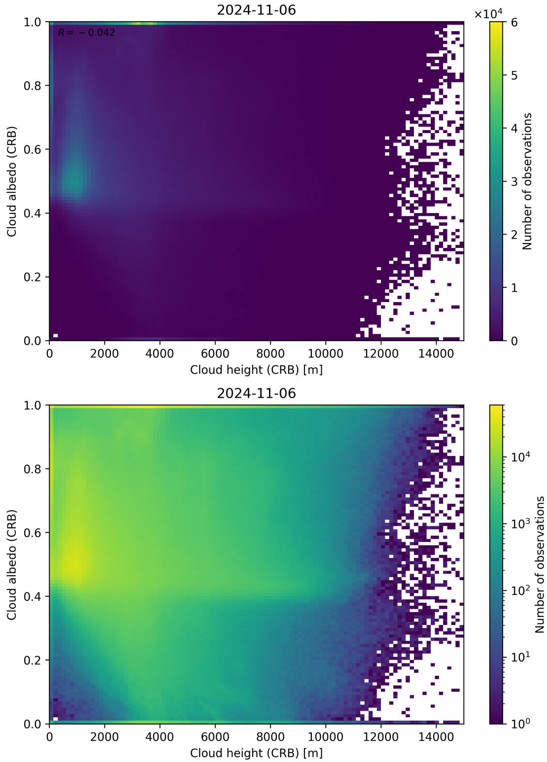
Figure 80: Scatter density plot of “Cloud height (CRB)” against “Cloud albedo (CRB)” for 2024-11-05 to 2024-11-07.
