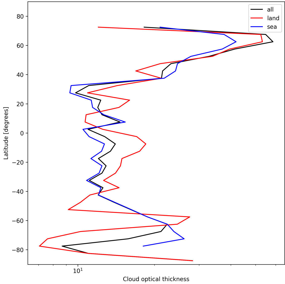
Figure 25: Zonal average of “Cloud optical thickness” for 2024-11-05 to 2024-11-07.
