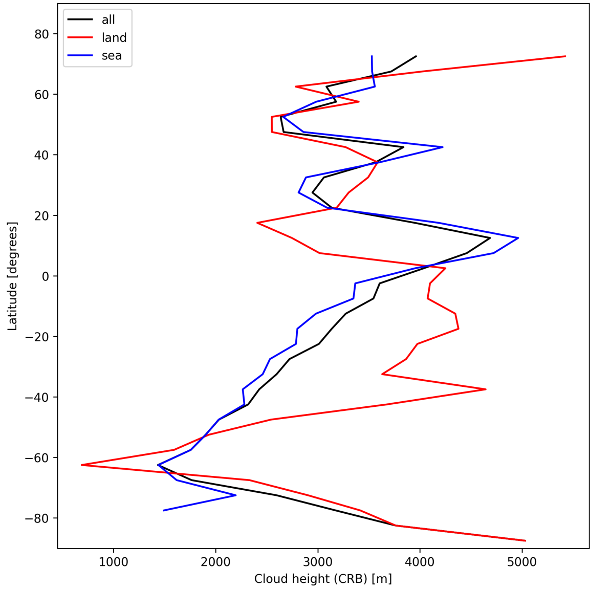
Figure 27: Zonal average of “Cloud height (CRB)” for 2024-11-05 to 2024-11-07.
