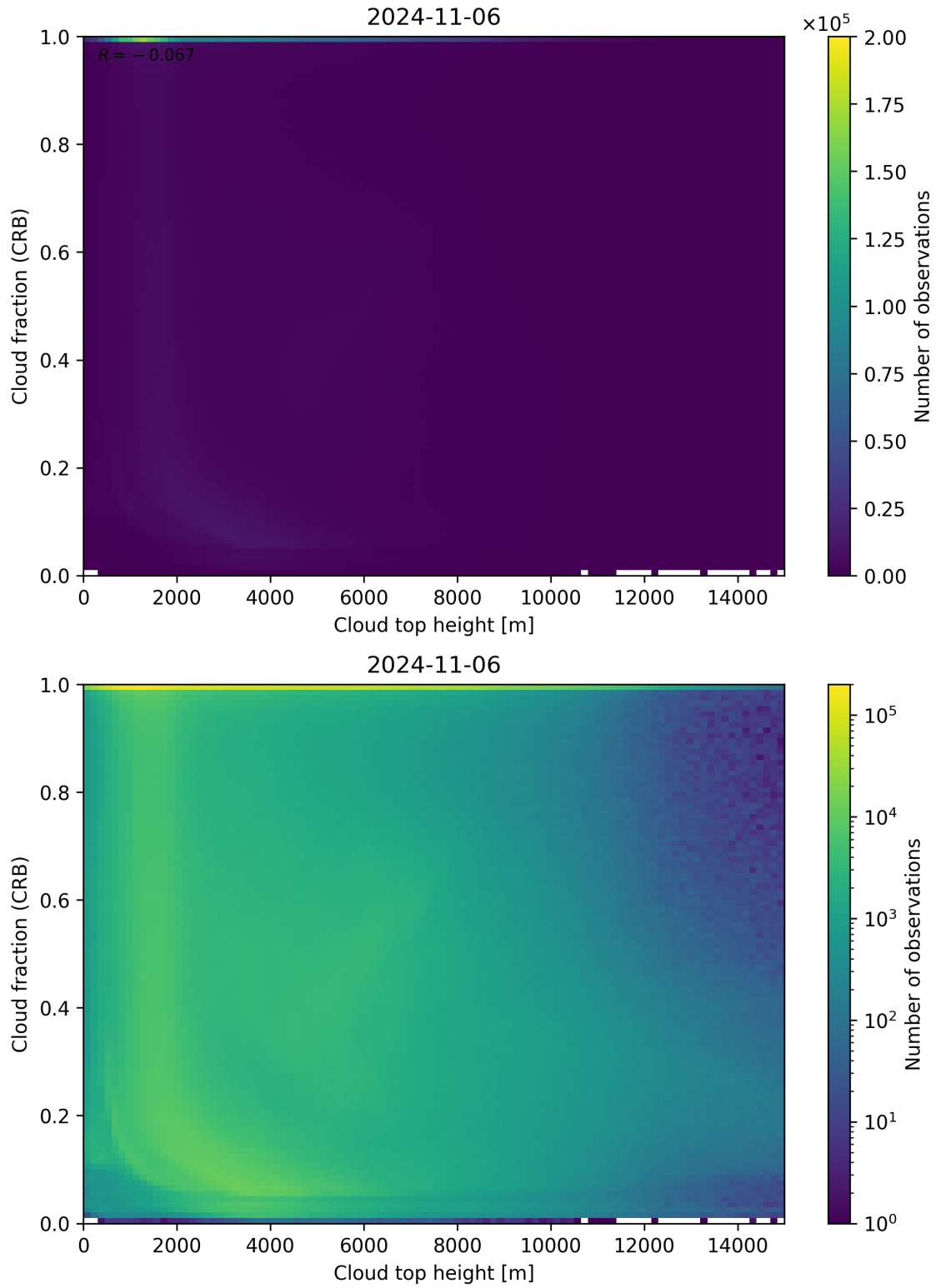
Figure 88: Scatter density plot of “Cloud top height” against “Cloud fraction (CRB)” for 2024-11-05 to 2024-11-07.
