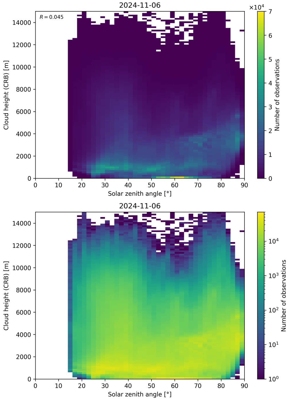
Figure 102: Scatter density plot of “Solar zenith angle” against “Cloud height (CRB)” for 2024-11-05 to 2024-11-07.
