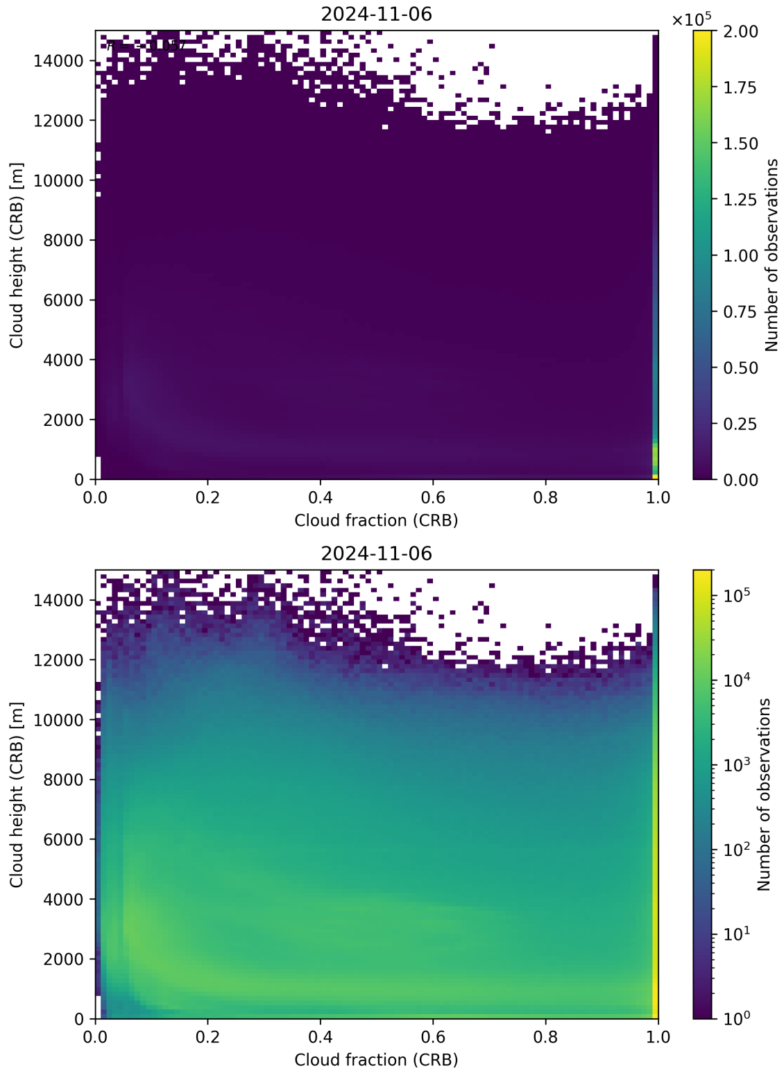
Figure 79: Scatter density plot of “Cloud fraction (CRB)” against “Cloud height (CRB)” for 2024-11-05 to 2024-11-07.
