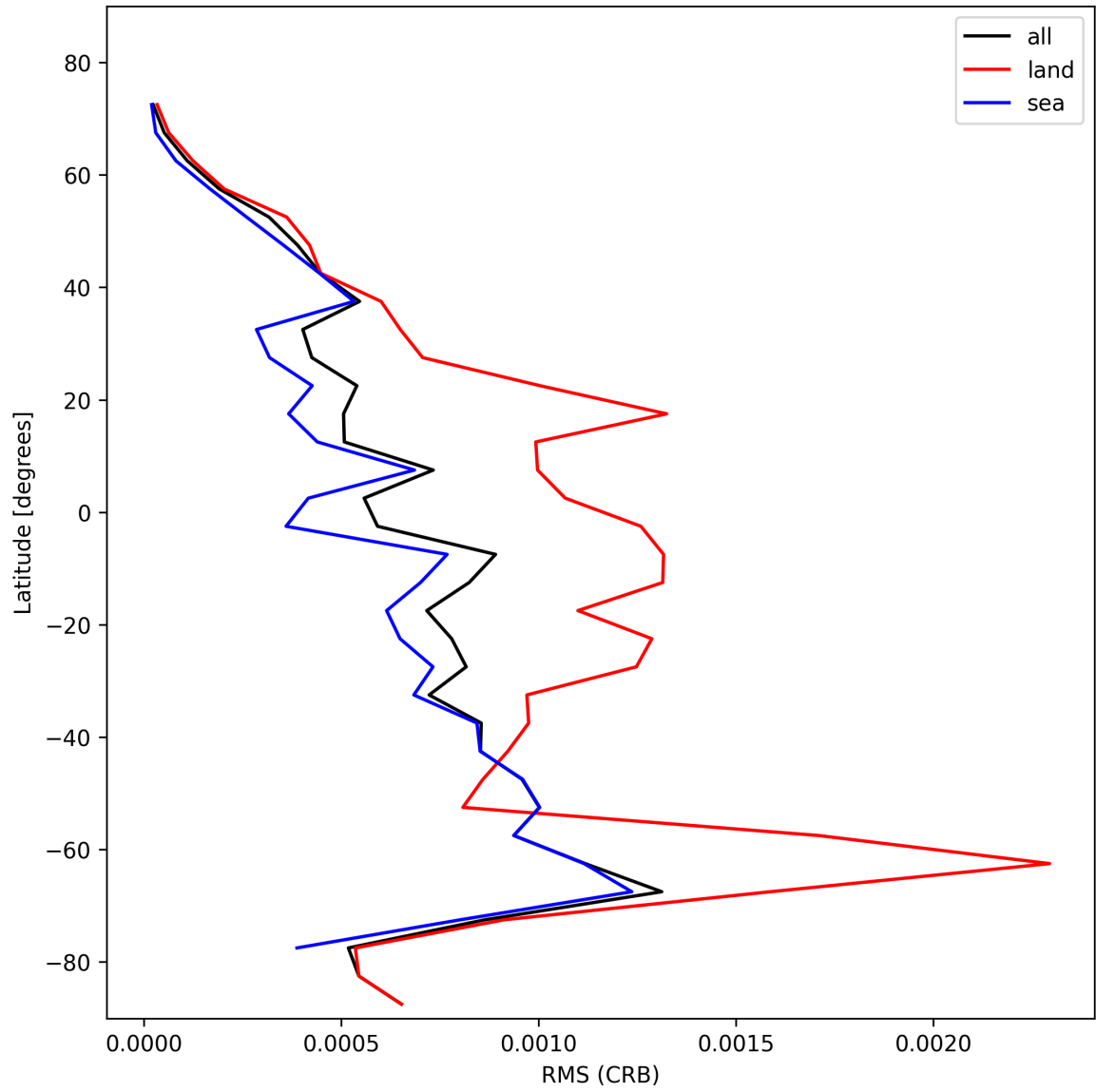
Figure 32: Zonal average of “RMS (CRB)” for 2024-11-05 to 2024-11-07.
