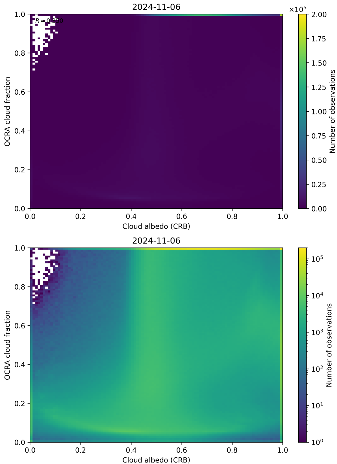
Figure 70: Scatter density plot of “Cloud albedo (CRB)” against “OCRA cloud fraction” for 2024-11-05 to 2024-11-07.
