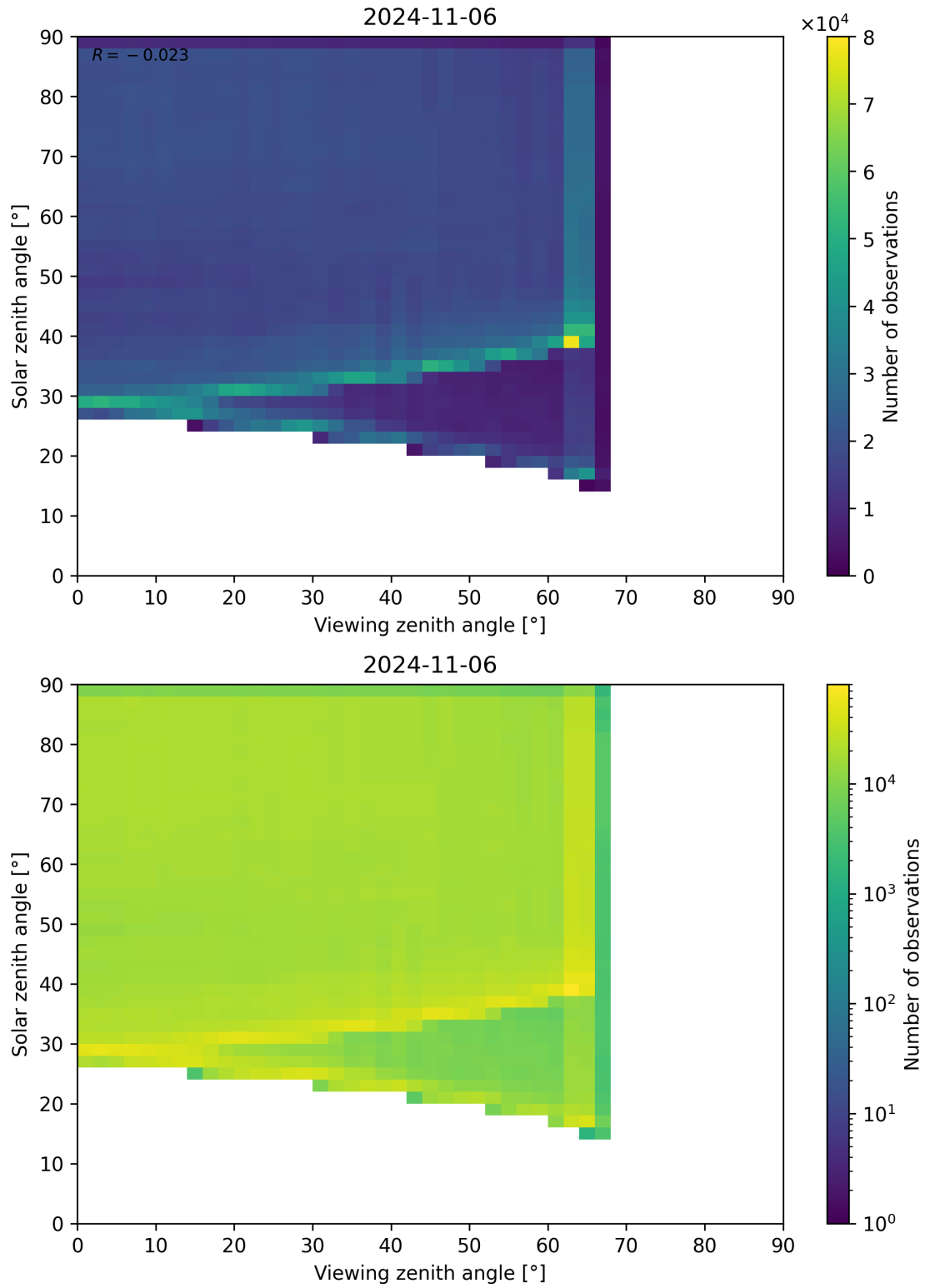
Figure 114: Scatter density plot of “Viewing zenith angle” against “Solar zenith angle” for 2024-11-05 to 2024-11-07.
