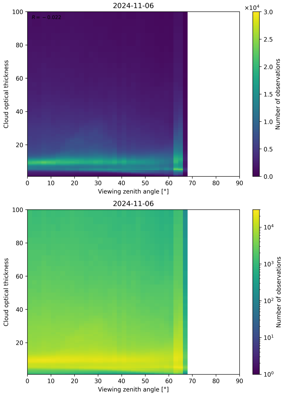
Figure 111: Scatter density plot of “Viewing zenith angle” against “Cloud optical thickness” for 2024-11-05 to 2024-11-07.
