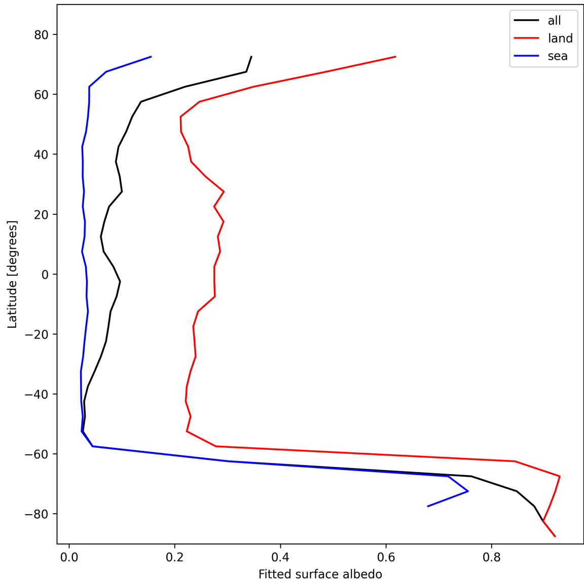
Figure 29: Zonal average of “Fitted surface albedo” for 2024-11-05 to 2024-11-07.
