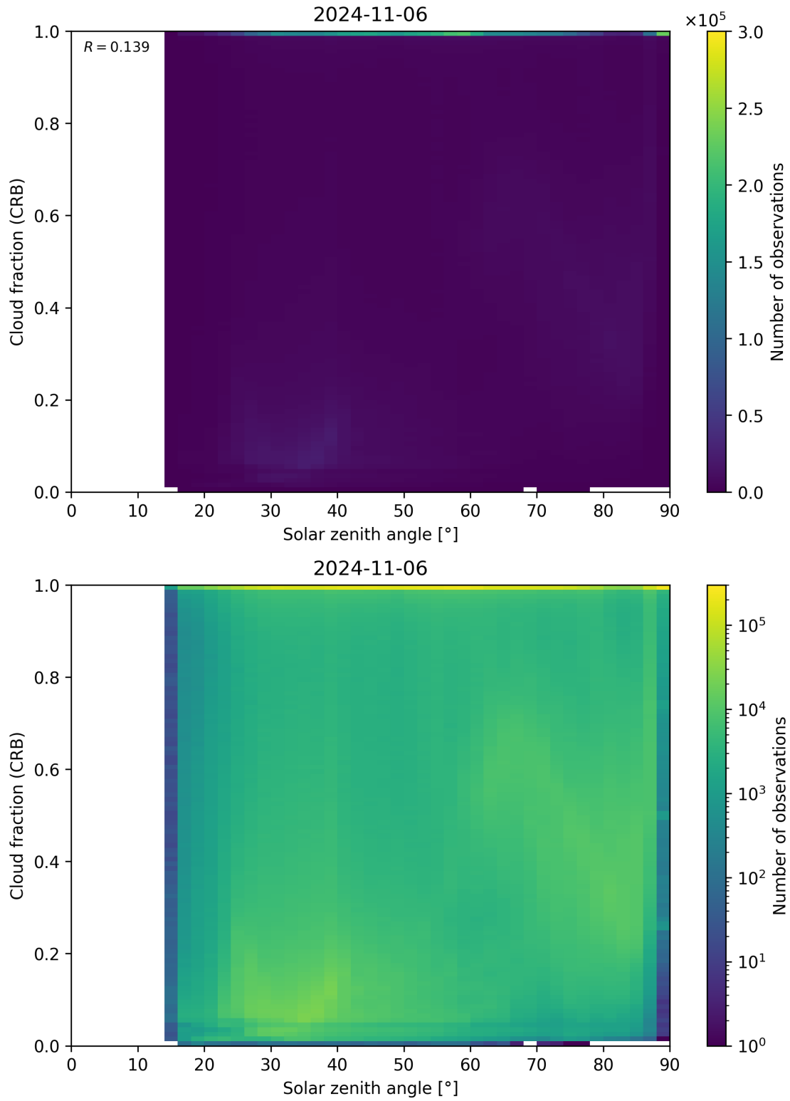
Figure 101: Scatter density plot of “Solar zenith angle” against “Cloud fraction (CRB)” for 2024-11-05 to 2024-11-07.
