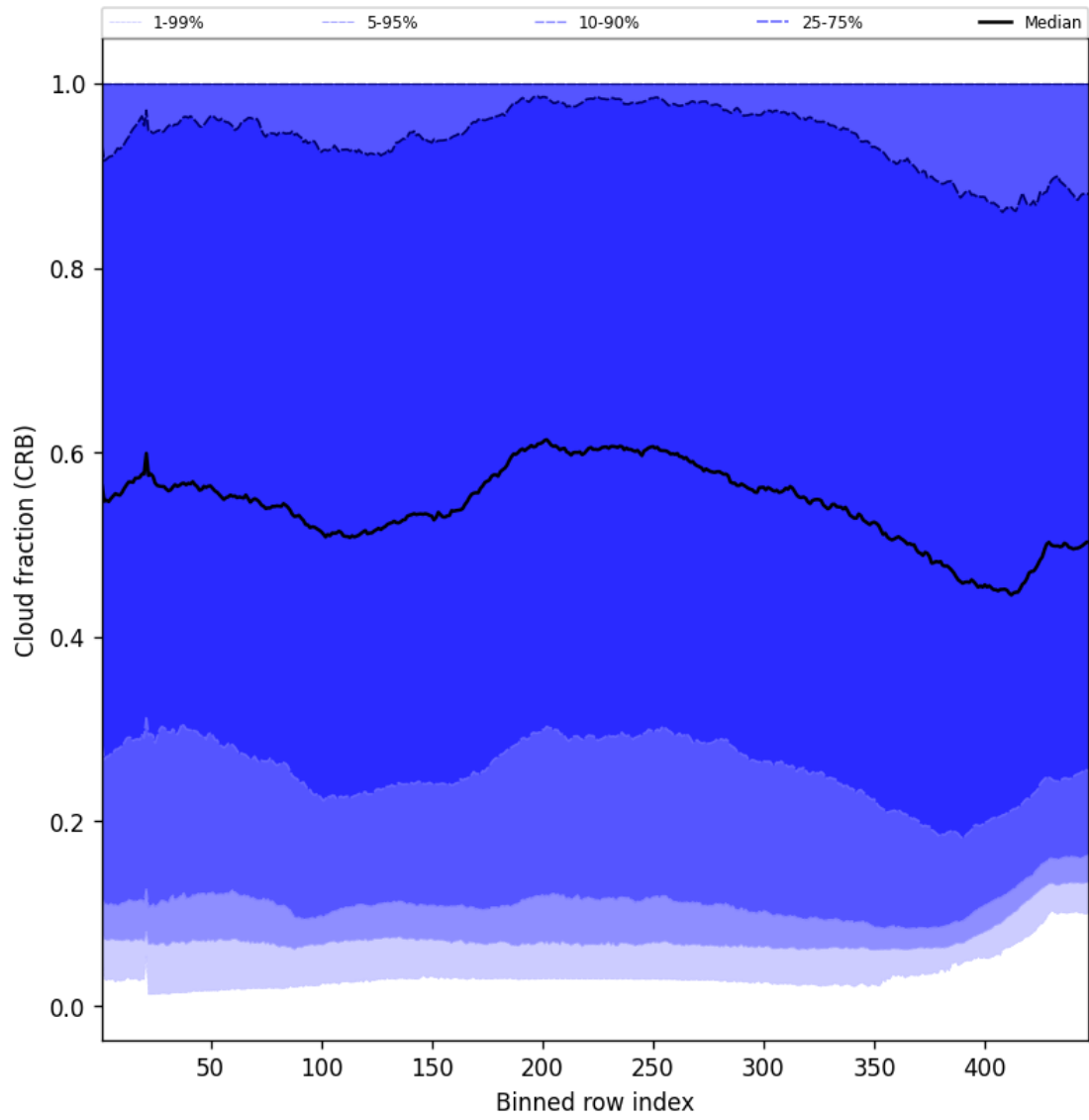
Figure 58: Along track statistics of “Cloud fraction (CRB)” for 2024-11-05 to 2024-11-07
