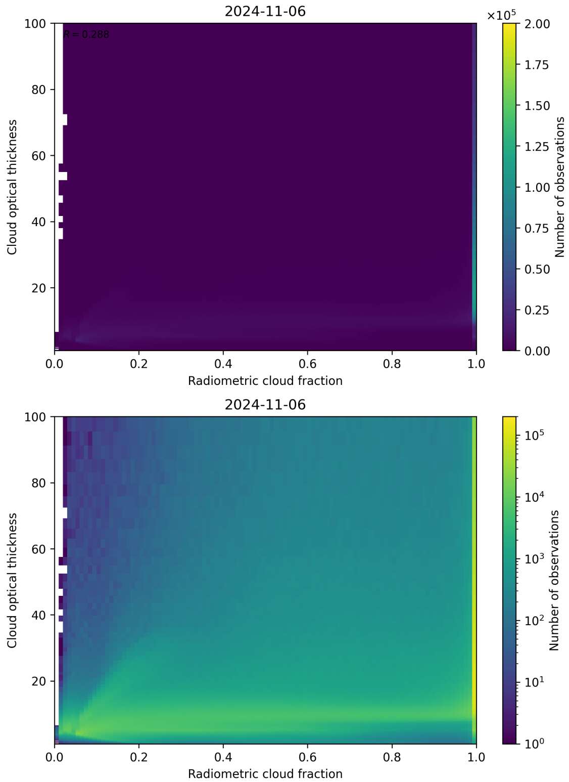
Figure 75: Scatter density plot of “Radiometric cloud fraction” against “Cloud optical thickness” for 2024-11-05 to 2024-11-07.
