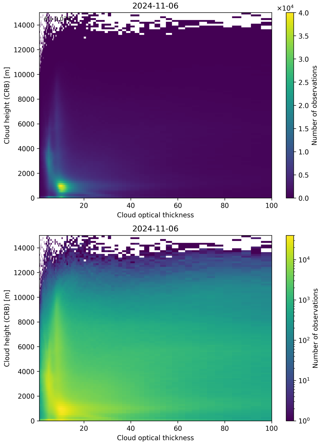
Figure 85: Scatter density plot of “Cloud optical thickness” against “Cloud height (CRB)” for 2024-11-05 to 2024-11-07.
