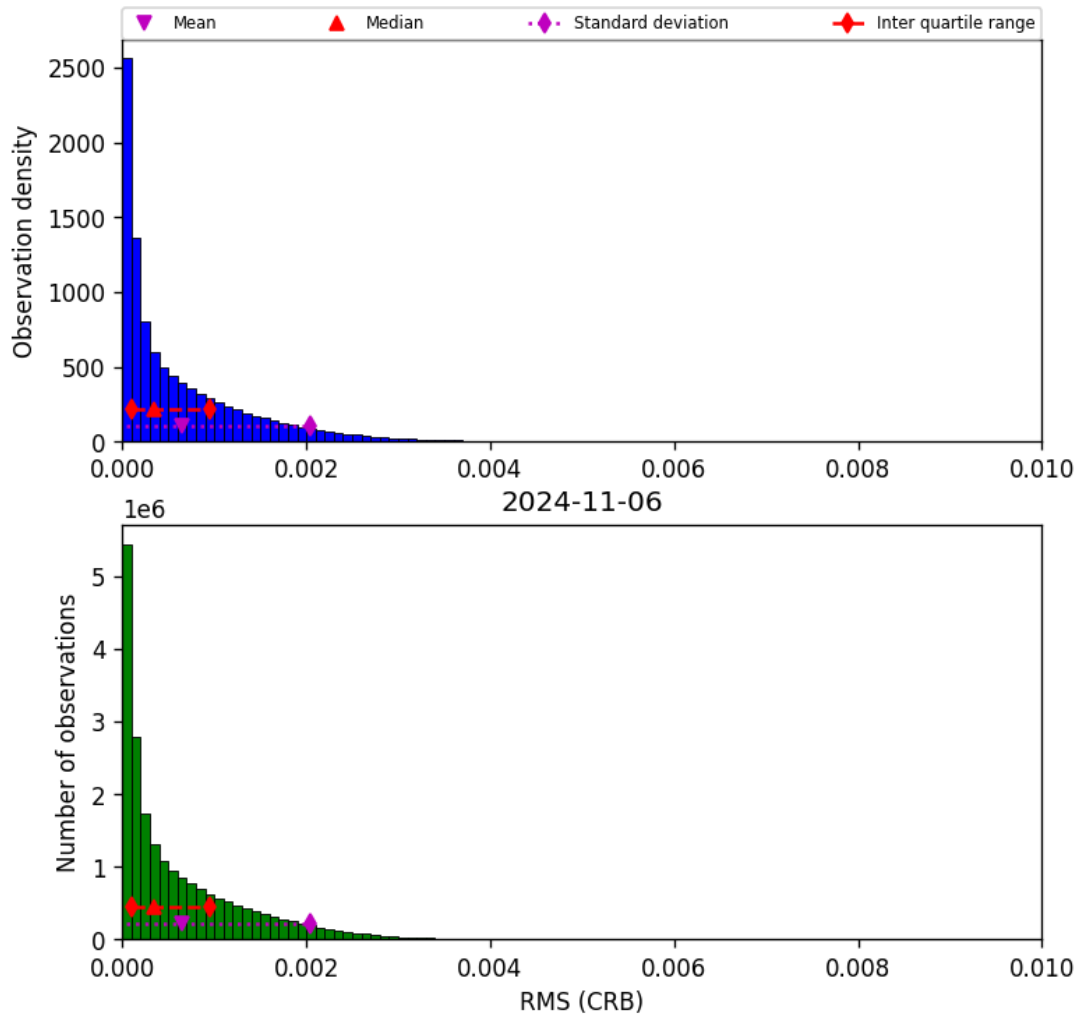
Figure 48: Histogram of “RMS (CRB)” for 2024-11-05 to 2024-11-07
