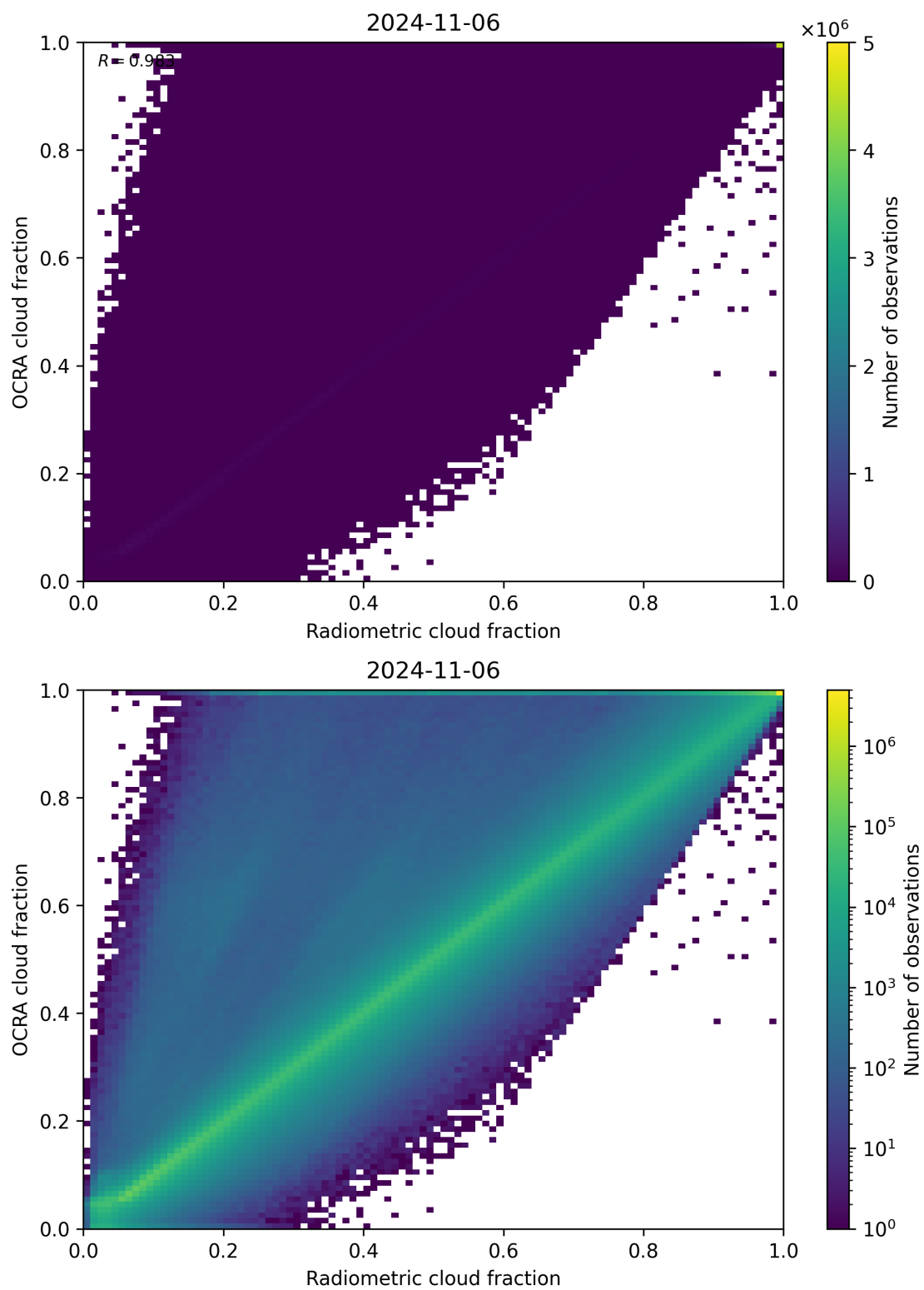
Figure 72: Scatter density plot of “Radiometric cloud fraction” against “OCRA cloud fraction” for 2024-11-05 to 2024-11-07.
