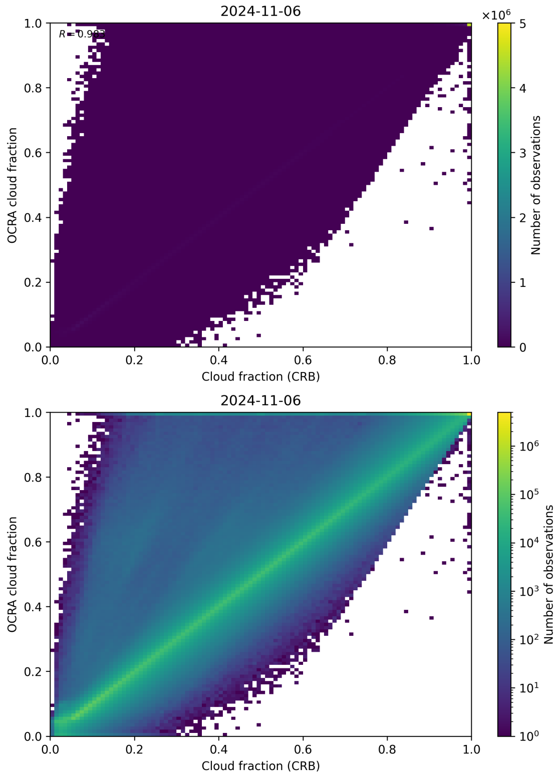
Figure 78: Scatter density plot of “Cloud fraction (CRB)” against “OCRA cloud fraction” for 2024-11-05 to 2024-11-07.
