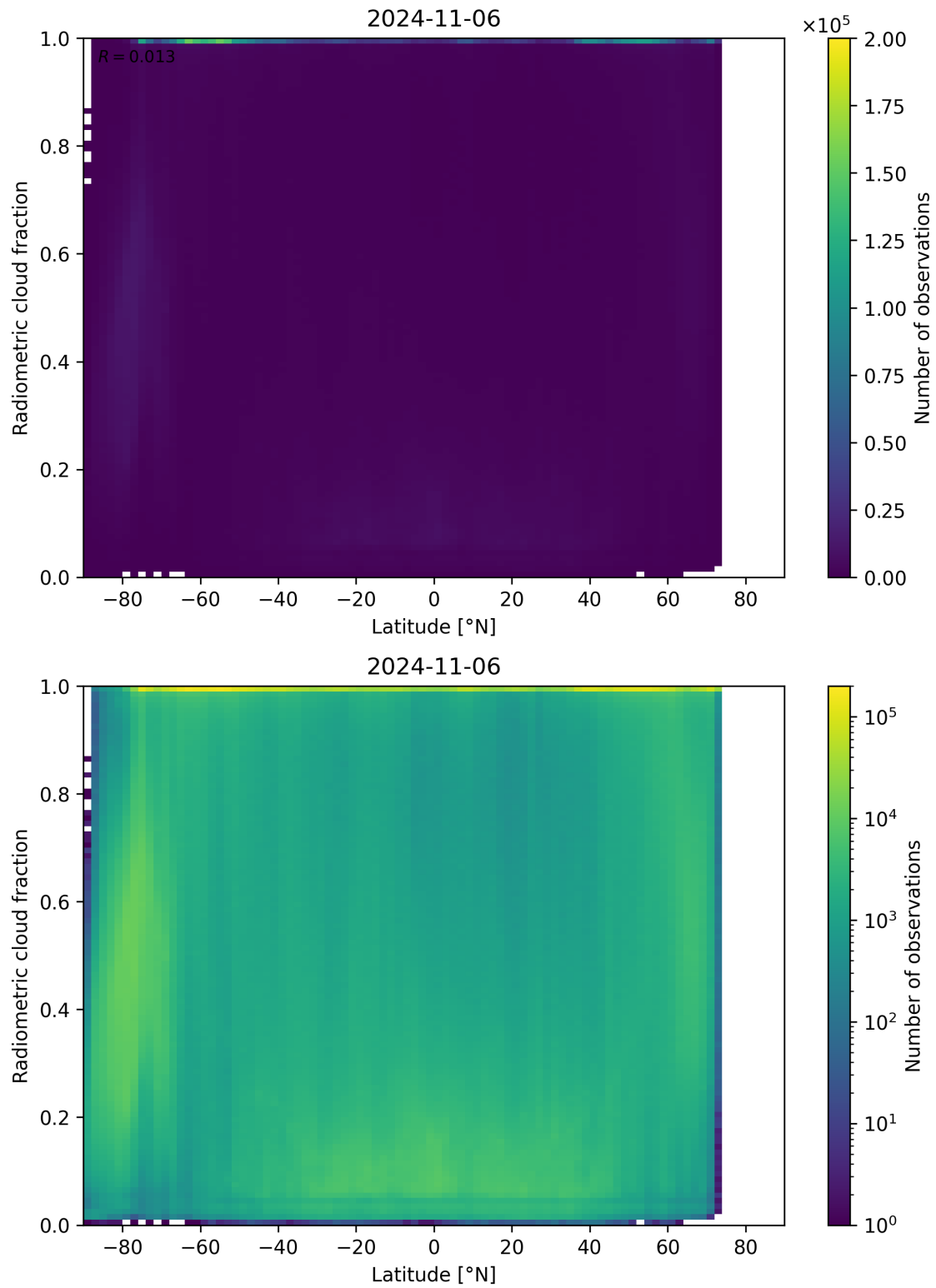
Figure 92: Scatter density plot of “Latitude” against “Radiometric cloud fraction” for 2024-11-05 to 2024-11-07.
