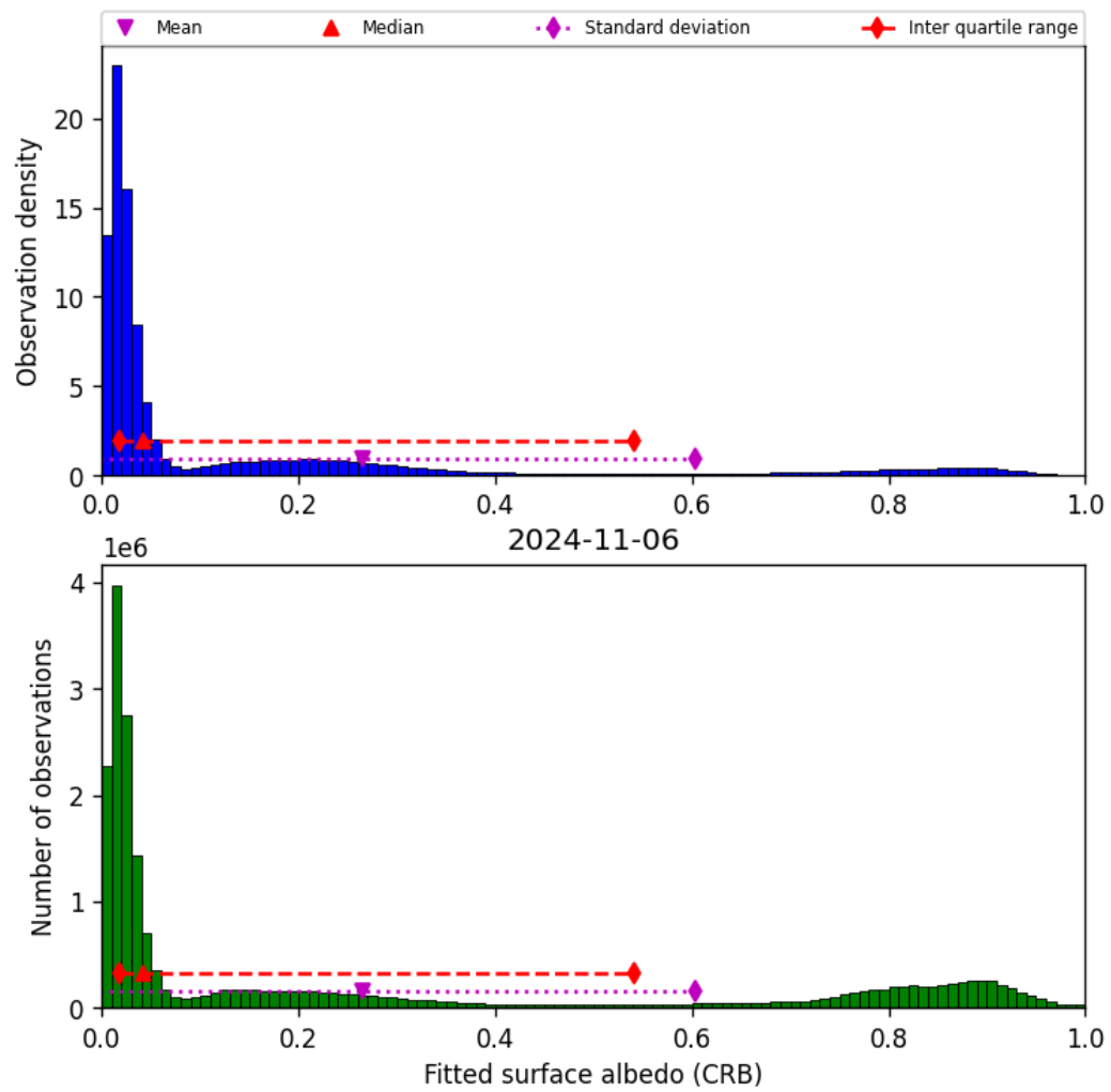
Figure 46: Histogram of “Fitted surface albedo (CRB)” for 2024-11-05 to 2024-11-07
