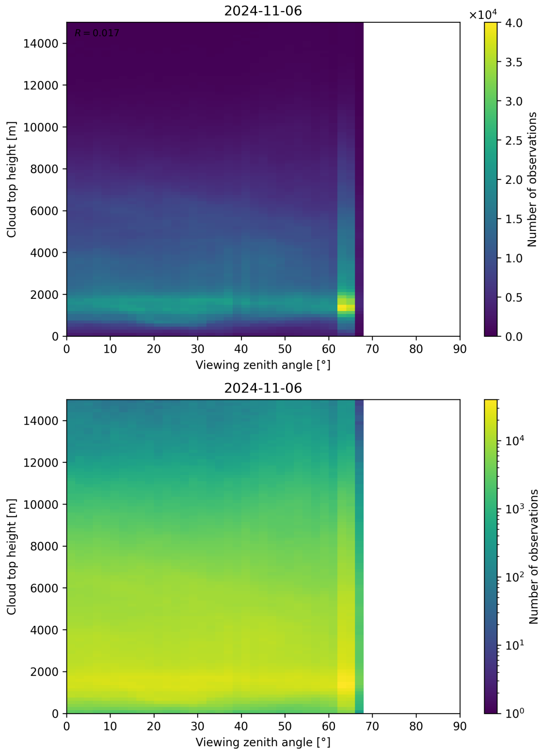
Figure 112: Scatter density plot of “Viewing zenith angle” against “Cloud top height” for 2024-11-05 to 2024-11-07.
