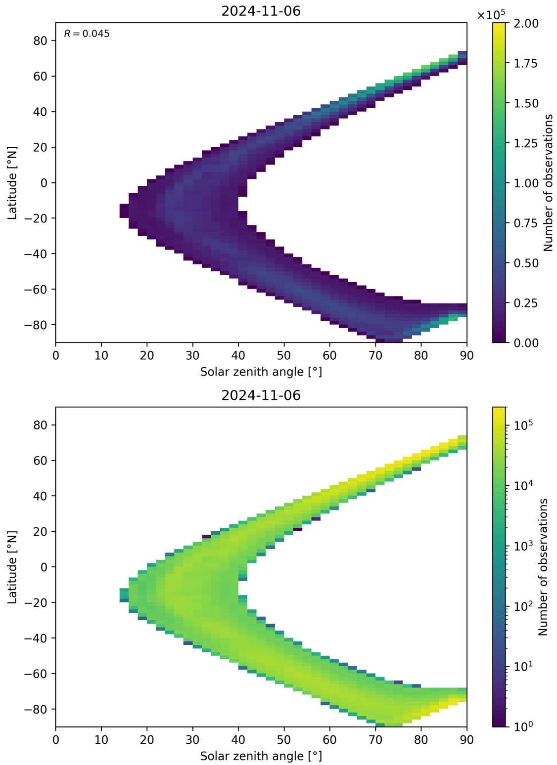
Figure 105: Scatter density plot of “Solar zenith angle” against “Latitude” for 2024-11-05 to 2024-11-07.
