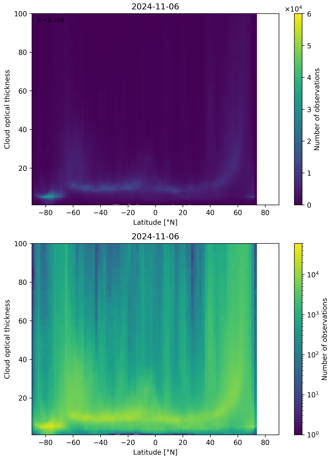
Figure 96: Scatter density plot of “Latitude” against “Cloud optical thickness” for 2024-11-05 to 2024-11-07.
