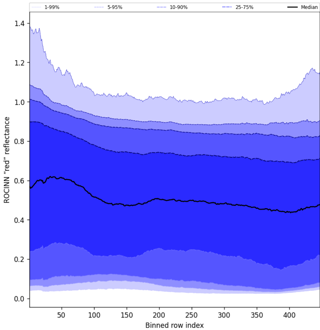
Figure 69: Along track statistics of “ROCINN “red” reflectance” for 2024-11-05 to 2024-11-07
