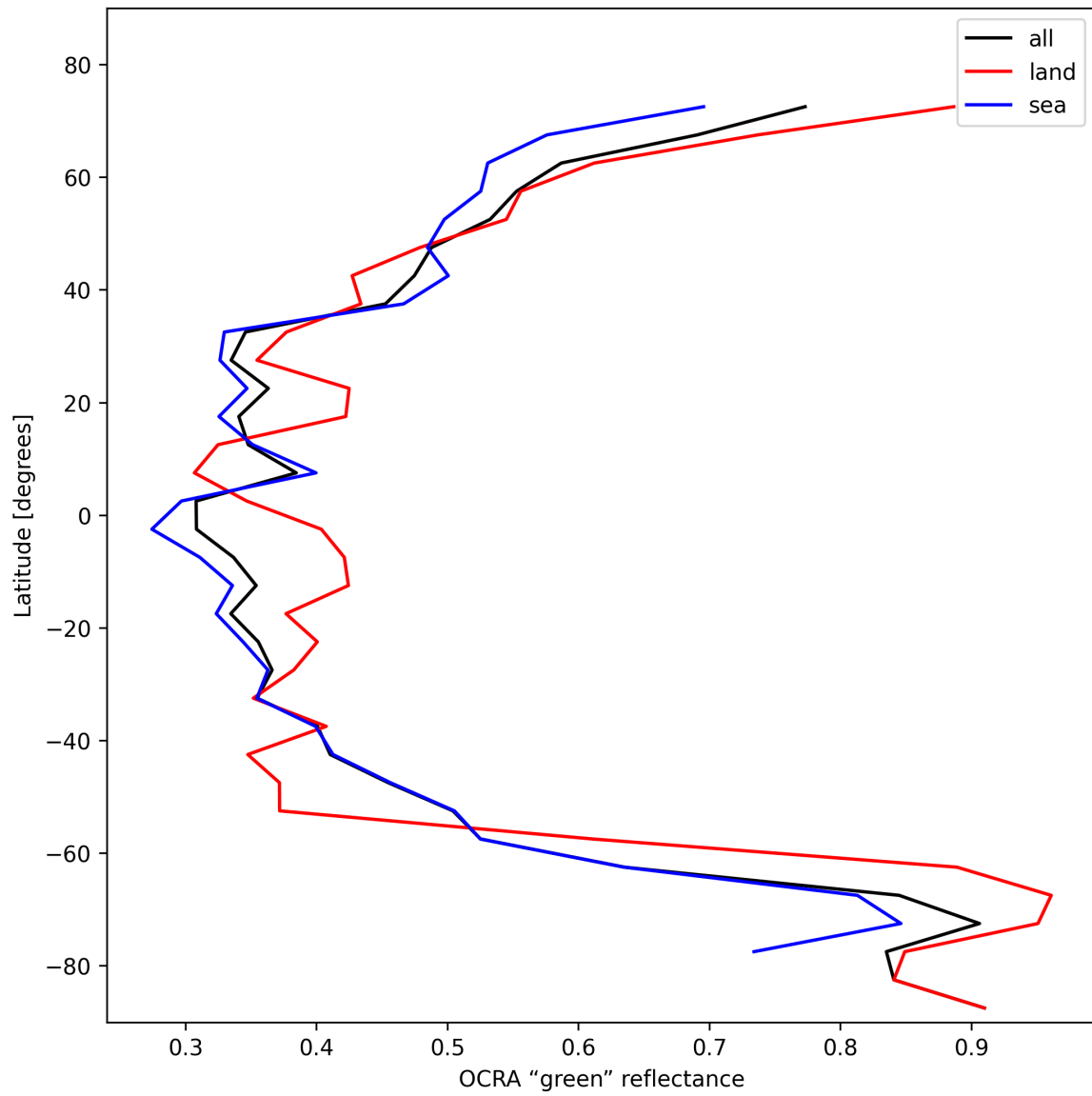
Figure 36: Zonal average of “OCRA “green” reflectance” for 2024-11-05 to 2024-11-07.
