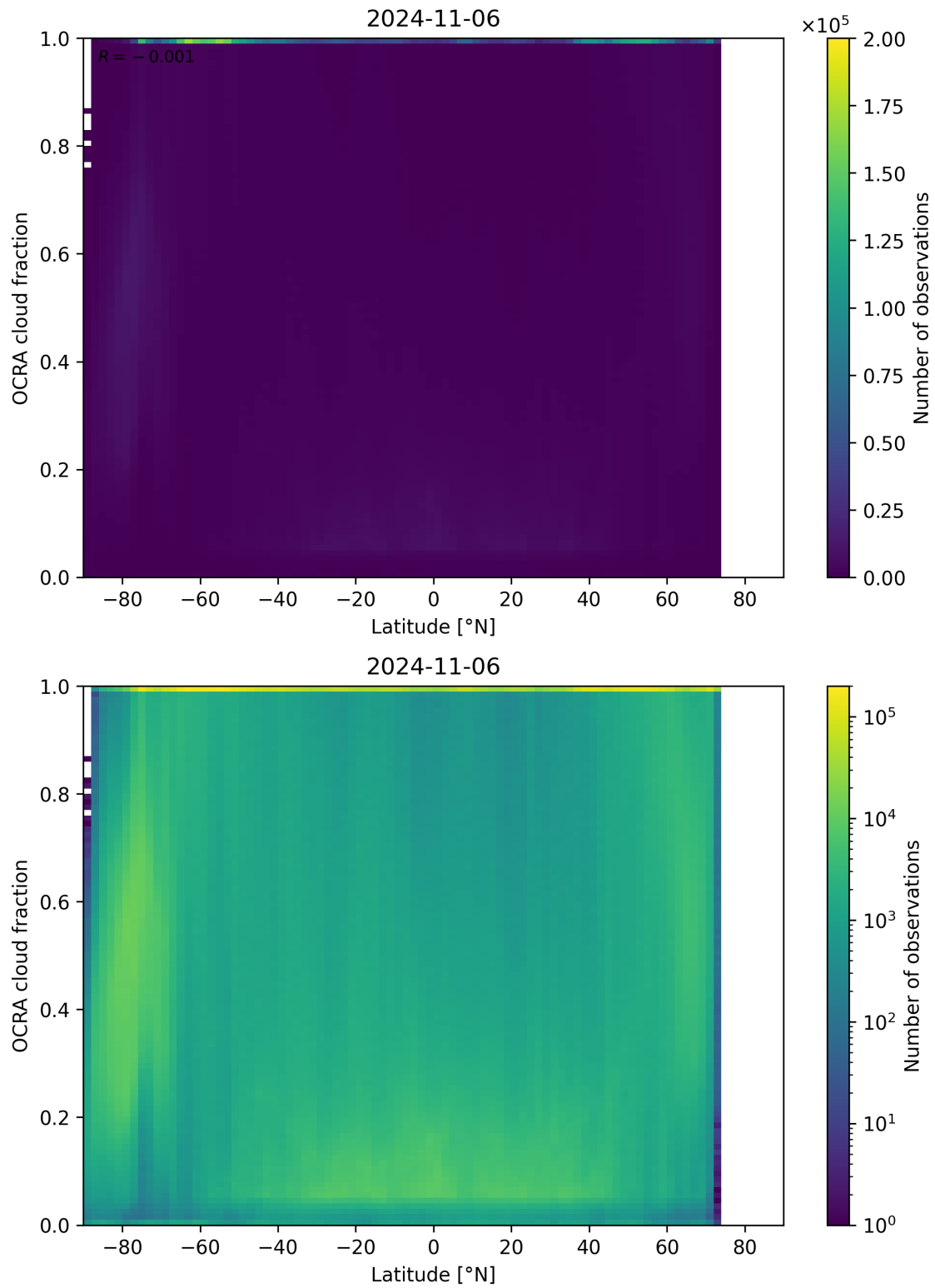
Figure 93: Scatter density plot of “Latitude” against “OCRA cloud fraction” for 2024-11-05 to 2024-11-07.
