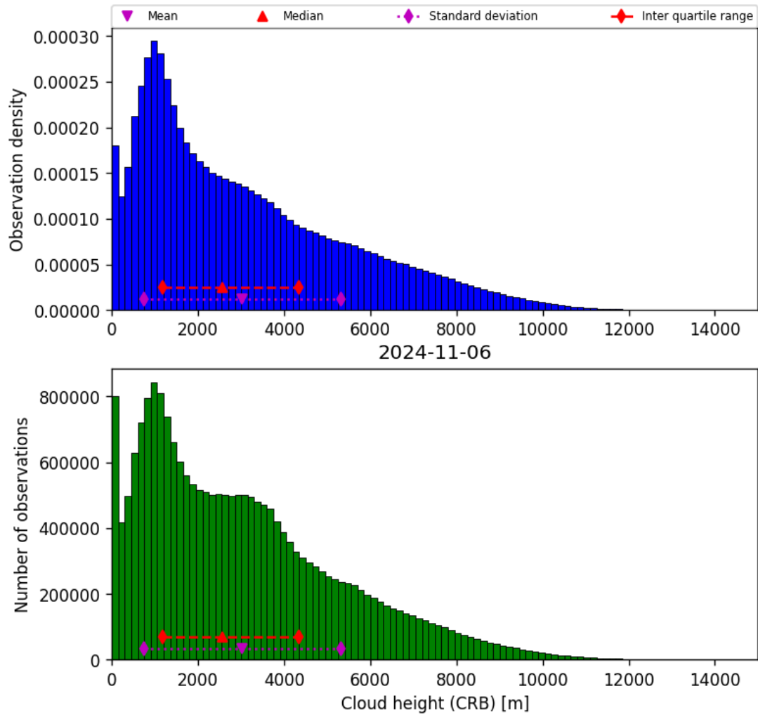
Figure 43: Histogram of “Cloud height (CRB)” for 2024-11-05 to 2024-11-07
