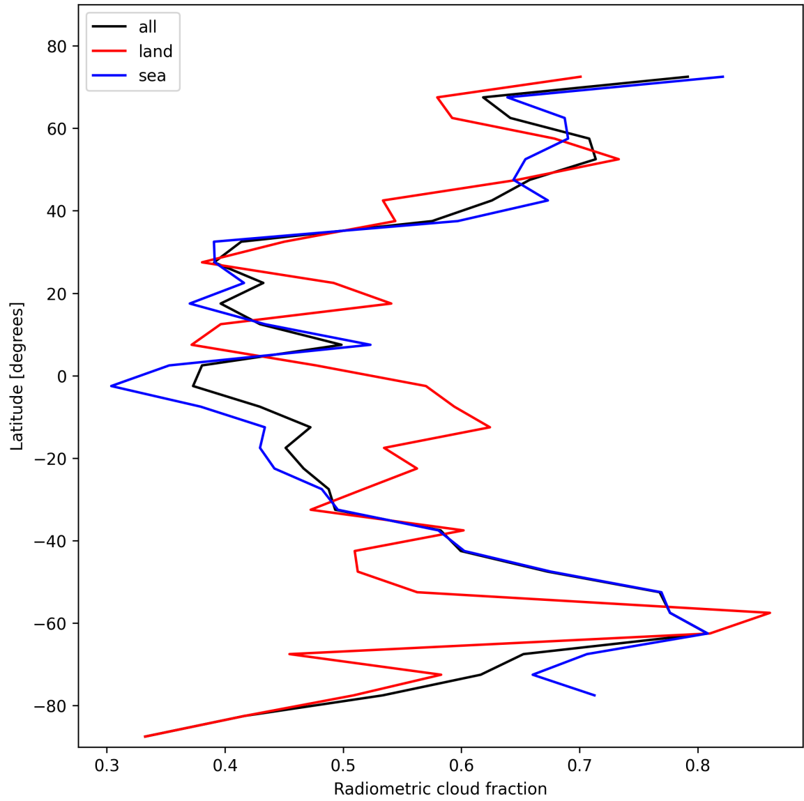
Figure 23: Zonal average of “Radiometric cloud fraction” for 2024-11-05 to 2024-11-07.
