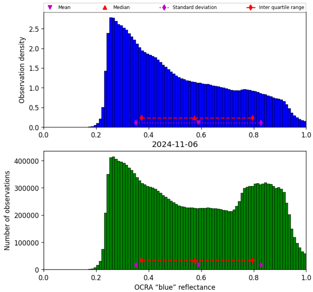
Figure 51: Histogram of “OCRA “blue” reflectance” for 2024-11-05 to 2024-11-07
