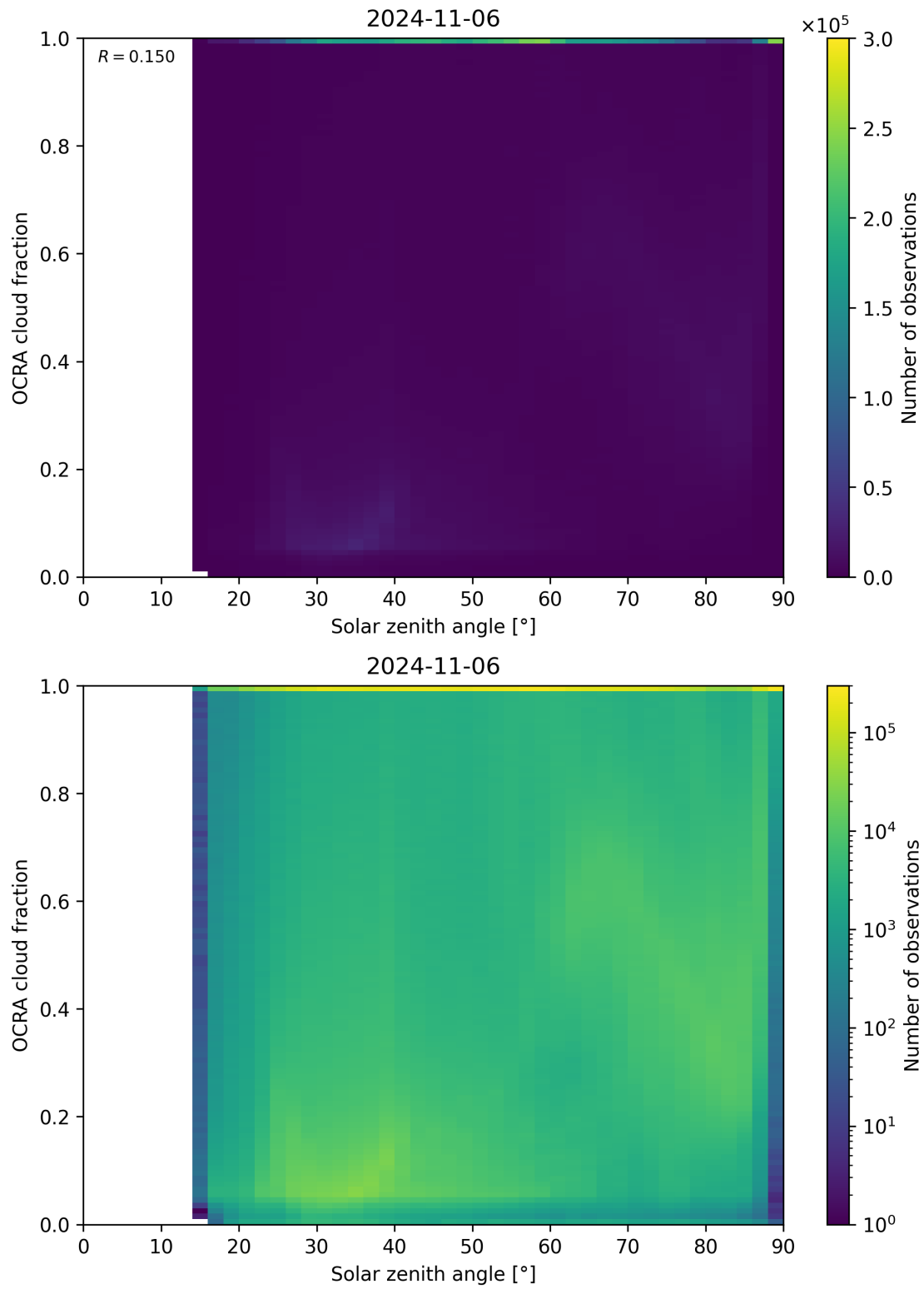
Figure 100: Scatter density plot of “Solar zenith angle” against “OCRA cloud fraction” for 2024-11-05 to 2024-11-07.
