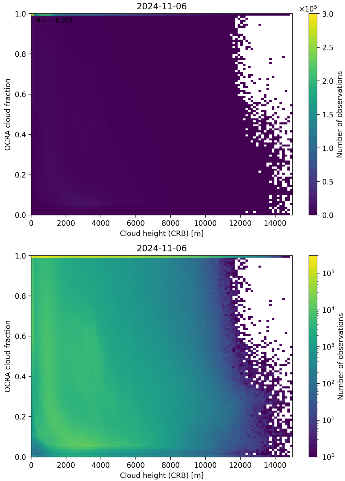
Figure 81: Scatter density plot of “Cloud height (CRB)” against “OCRA cloud fraction” for 2024-11-05 to 2024-11-07.
