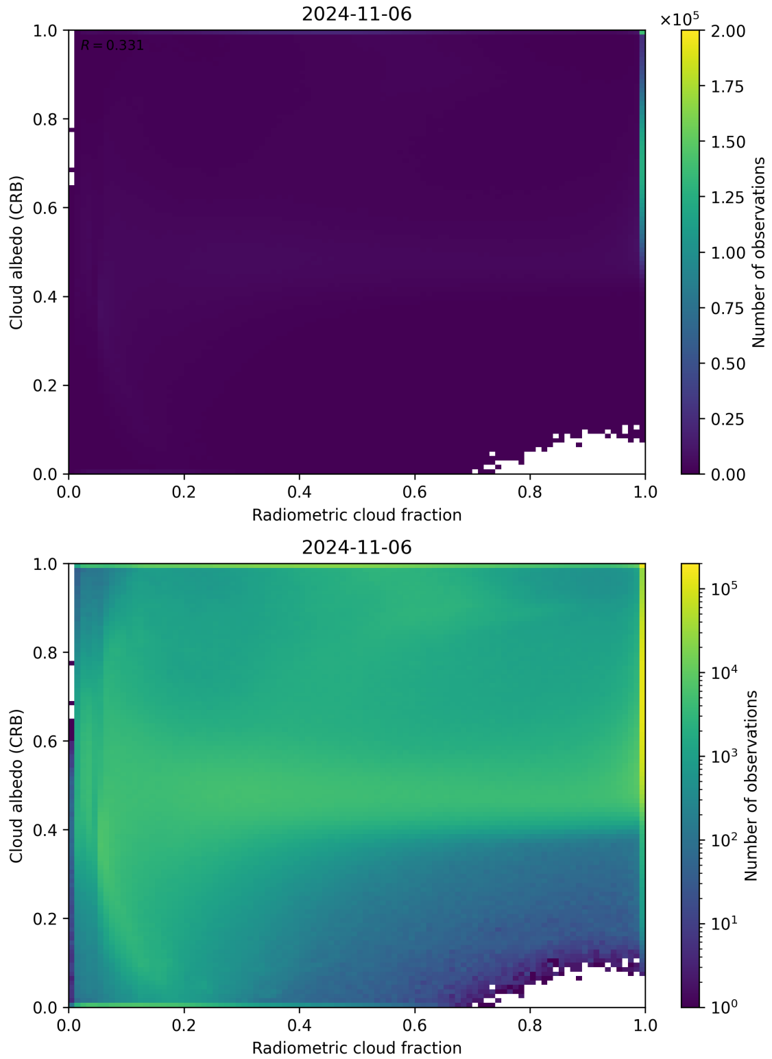
Figure 71: Scatter density plot of “Radiometric cloud fraction” against “Cloud albedo (CRB)” for 2024-11-05 to 2024-11-07.
