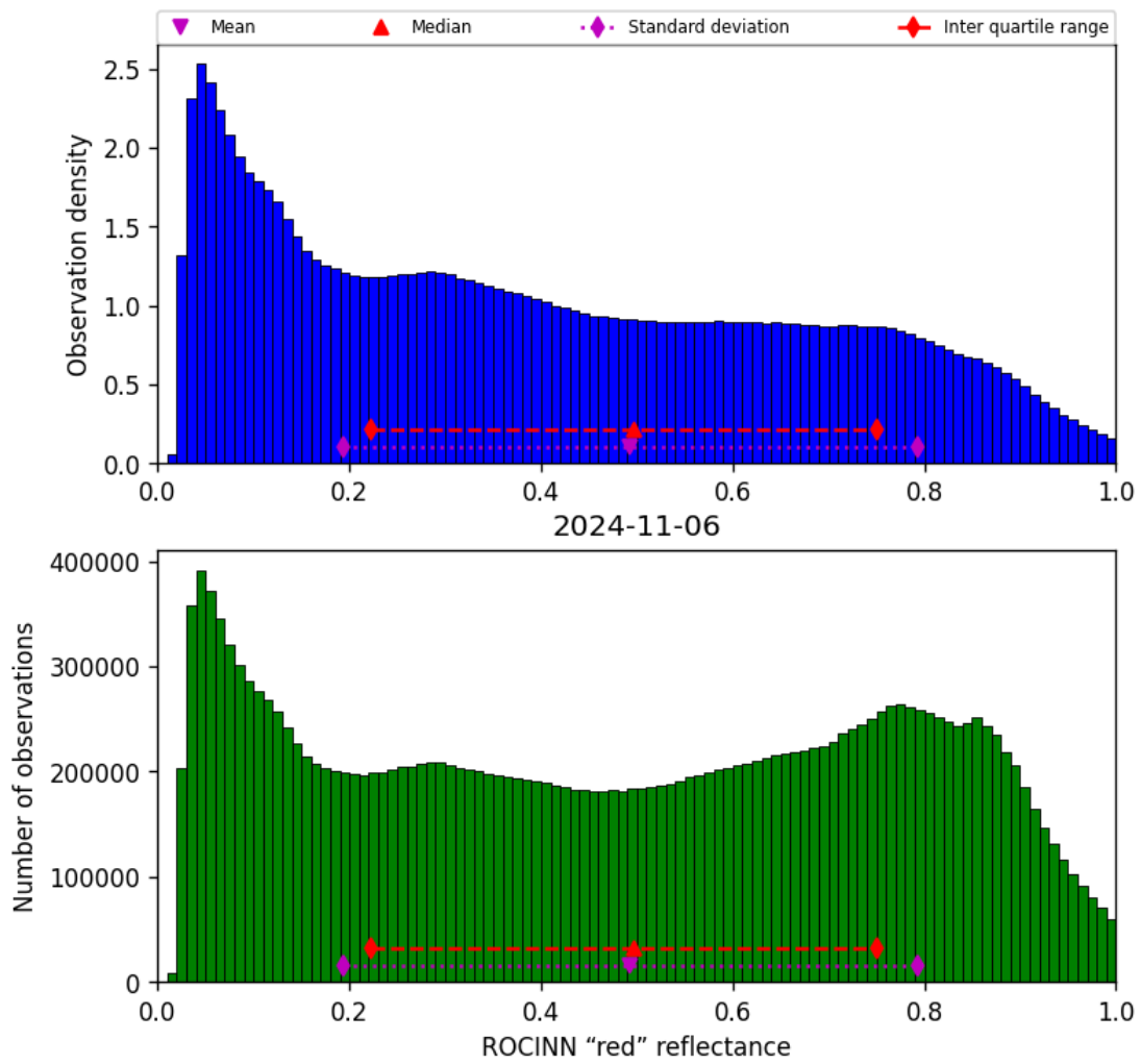
Figure 53: Histogram of “ROCINN “red” reflectance” for 2024-11-05 to 2024-11-07
