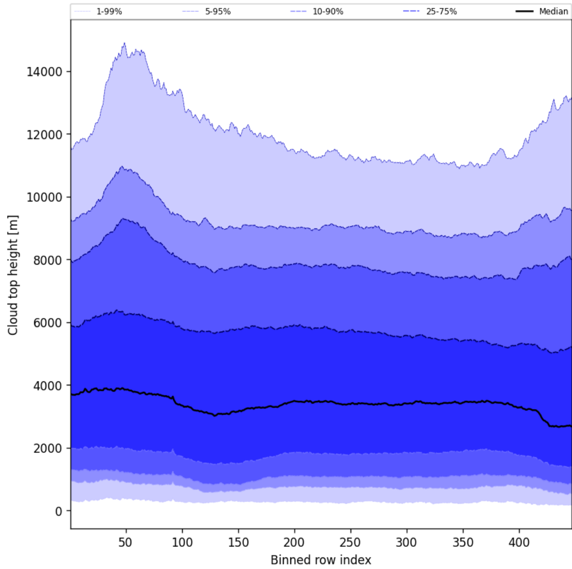
Figure 56: Along track statistics of “Cloud top height” for 2024-11-05 to 2024-11-07
