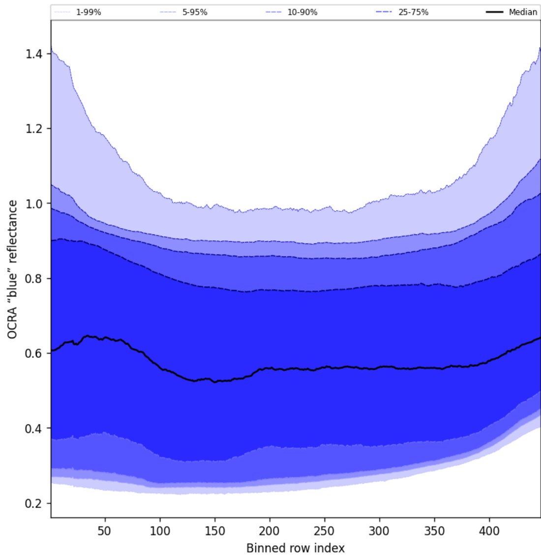
Figure 67: Along track statistics of “OCRA “blue” reflectance” for 2024-11-05 to 2024-11-07
