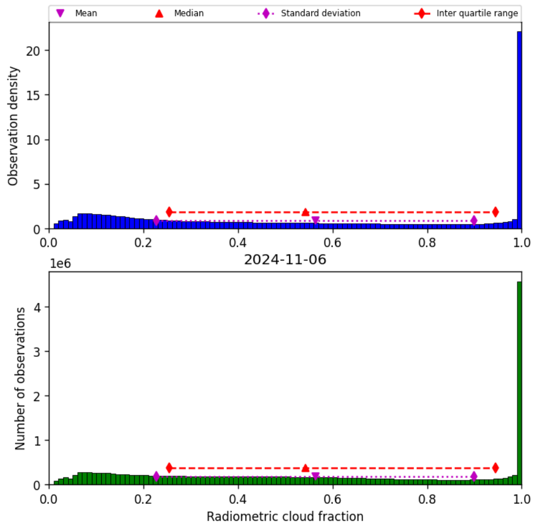
Figure 39: Histogram of “Radiometric cloud fraction” for 2024-11-05 to 2024-11-07
