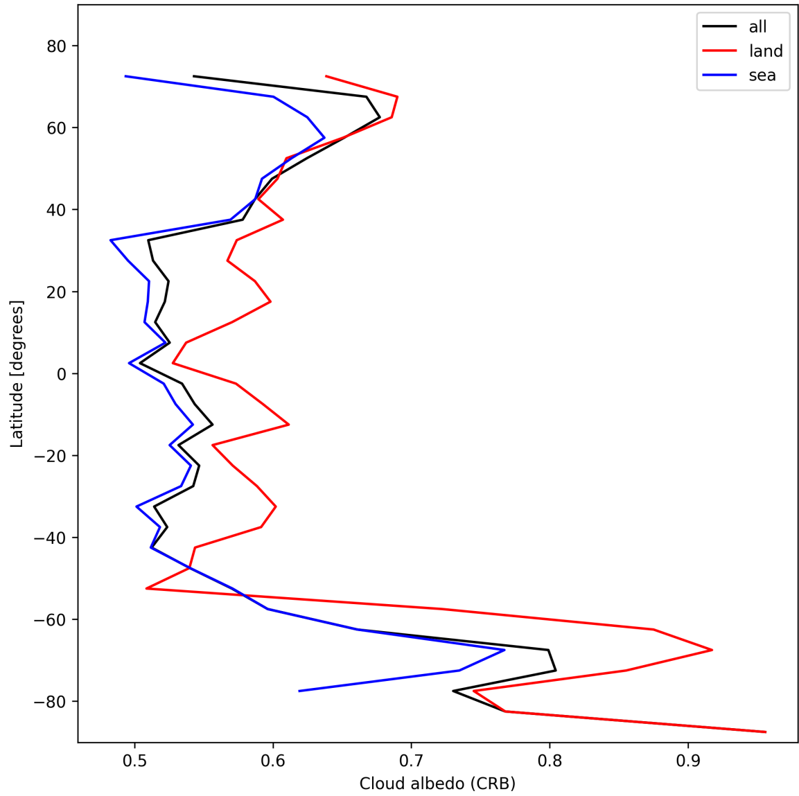
Figure 28: Zonal average of “Cloud albedo (CRB)” for 2024-11-05 to 2024-11-07.
