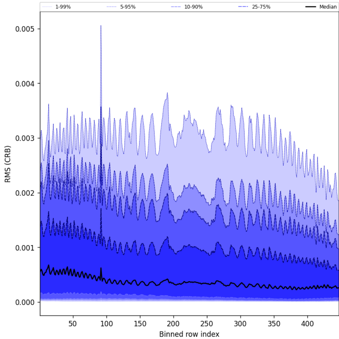
Figure 64: Along track statistics of “RMS (CRB)” for 2024-11-05 to 2024-11-07
