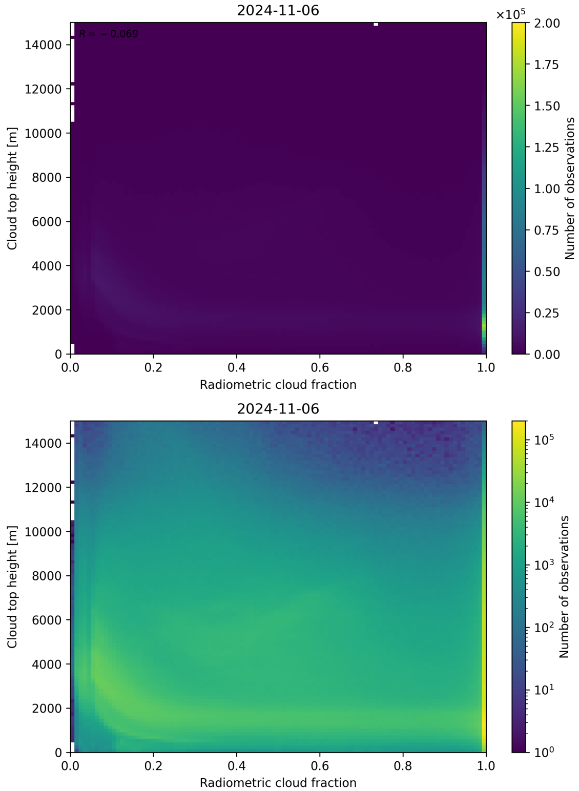
Figure 76: Scatter density plot of “Radiometric cloud fraction” against “Cloud top height” for 2024-11-05 to 2024-11-07.
