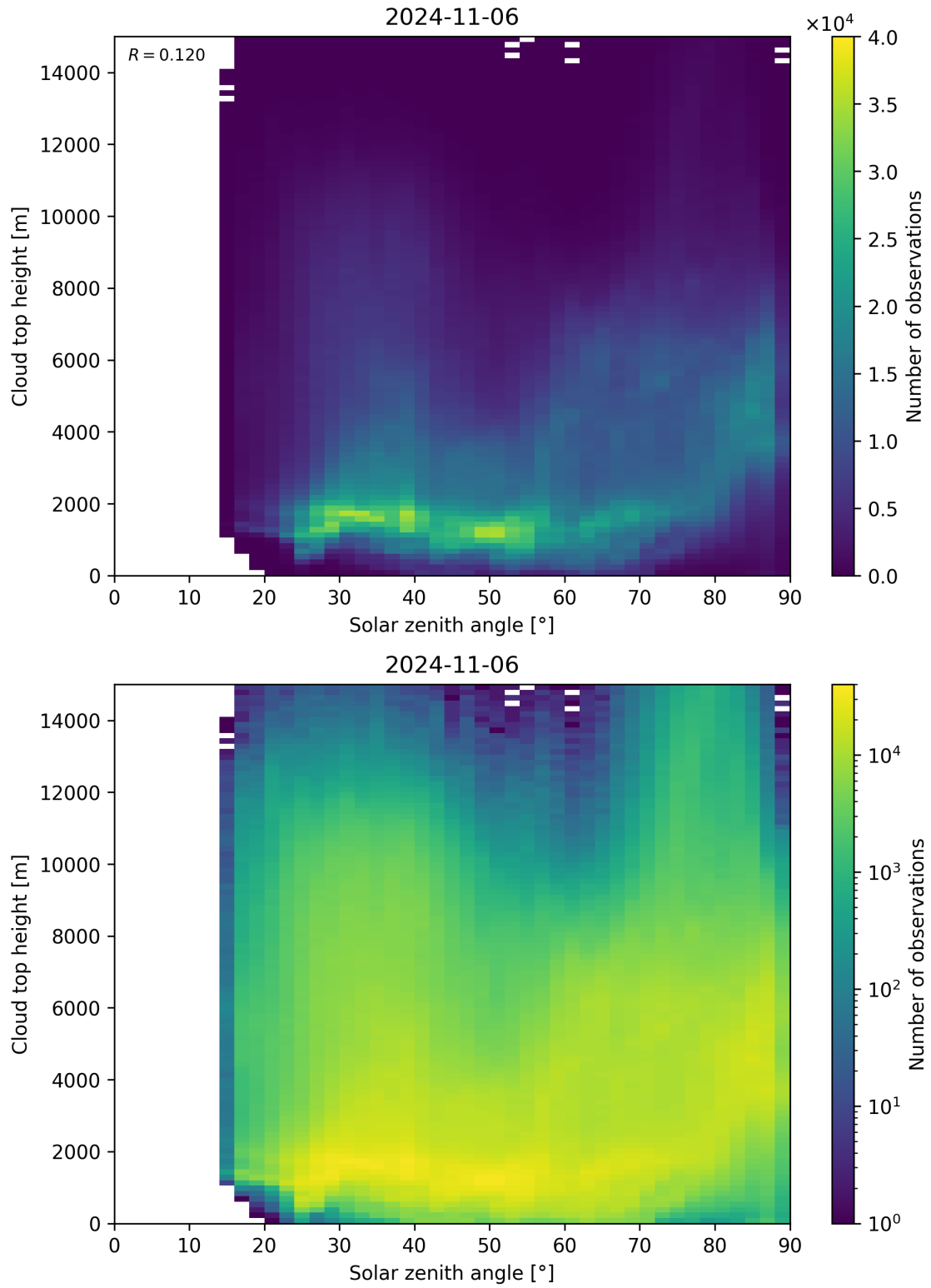
Figure 104: Scatter density plot of “Solar zenith angle” against “Cloud top height” for 2024-11-05 to 2024-11-07.
