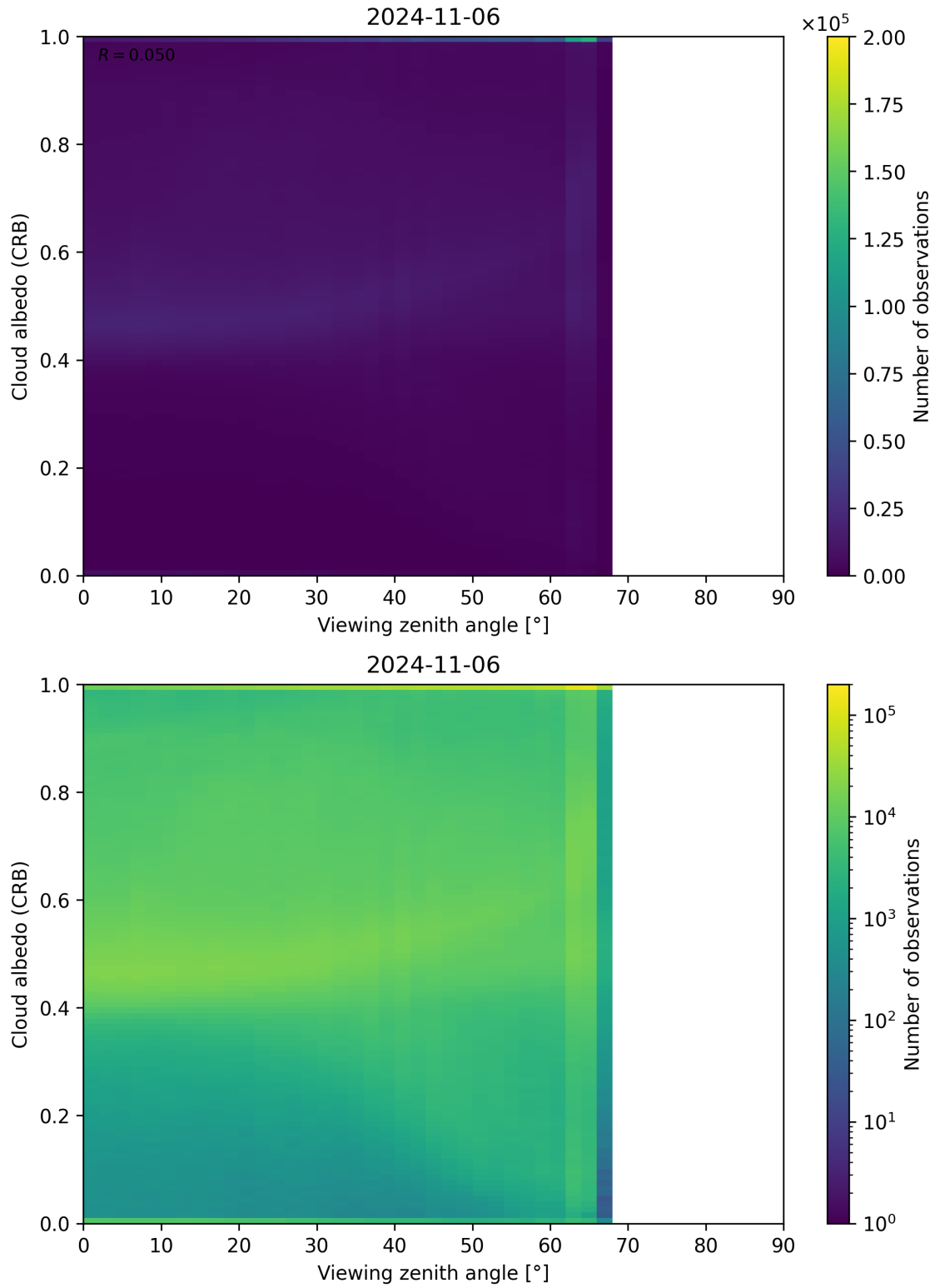
Figure 106: Scatter density plot of “Viewing zenith angle” against “Cloud albedo (CRB)” for 2024-11-05 to 2024-11-07.
