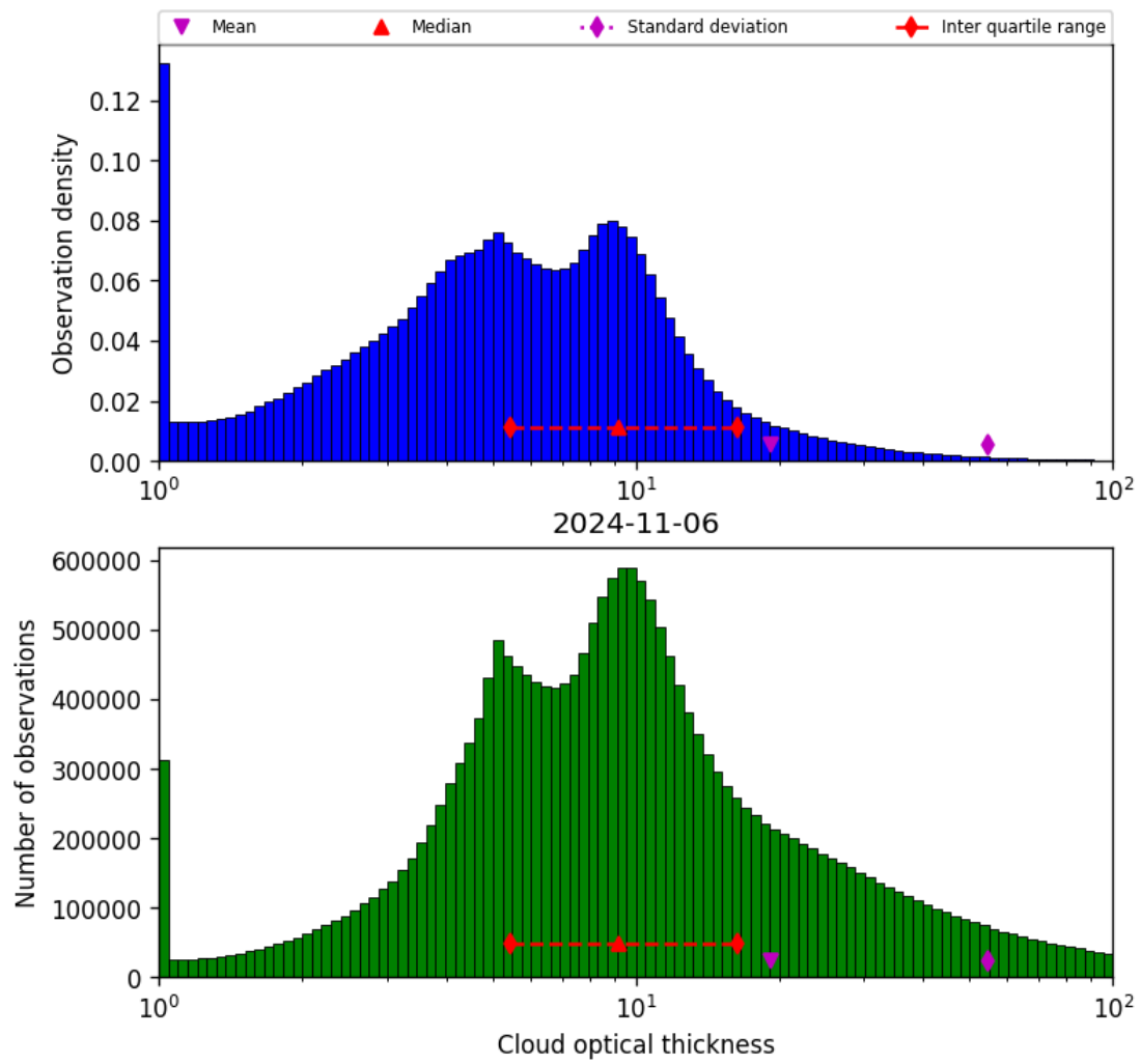
Figure 41: Histogram of “Cloud optical thickness” for 2024-11-05 to 2024-11-07
