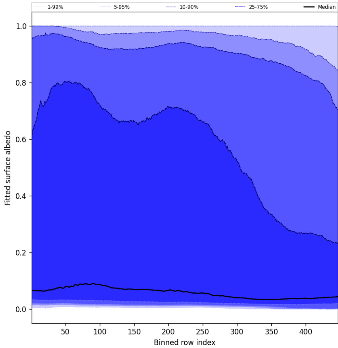
Figure 61: Along track statistics of “Fitted surface albedo” for 2024-11-05 to 2024-11-07
