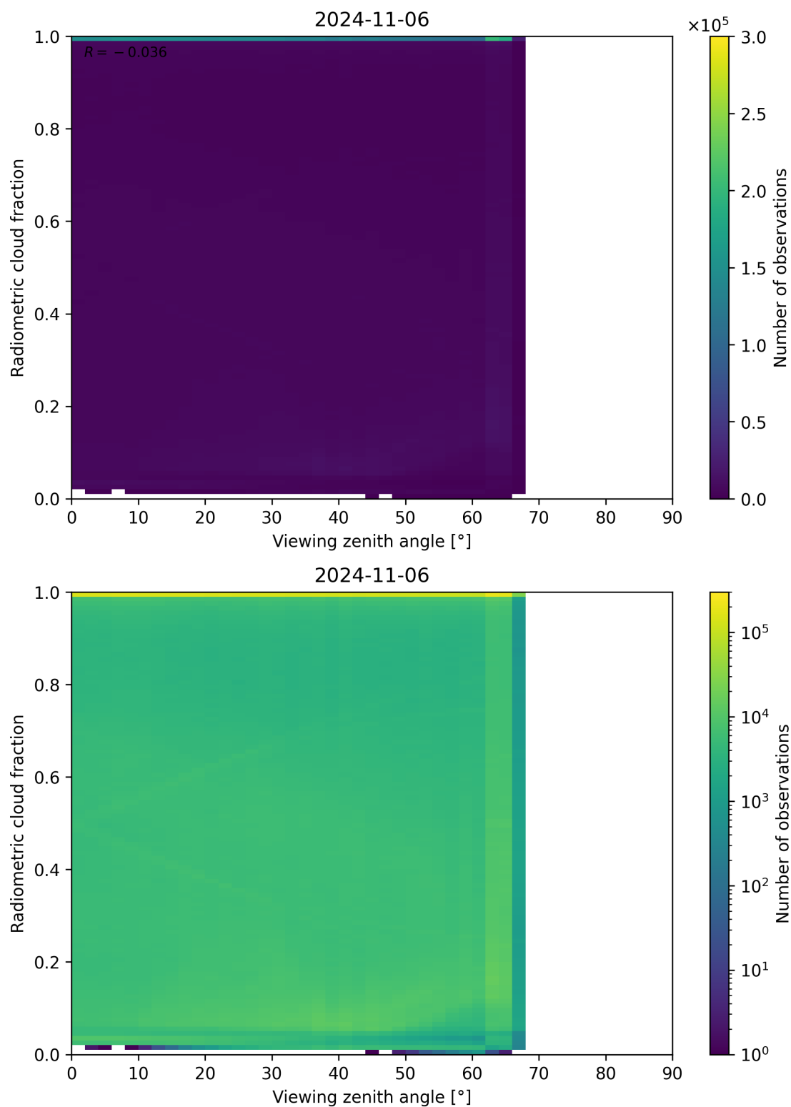
Figure 107: Scatter density plot of “Viewing zenith angle” against “Radiometric cloud fraction” for 2024-11-05 to 2024-11-07.
