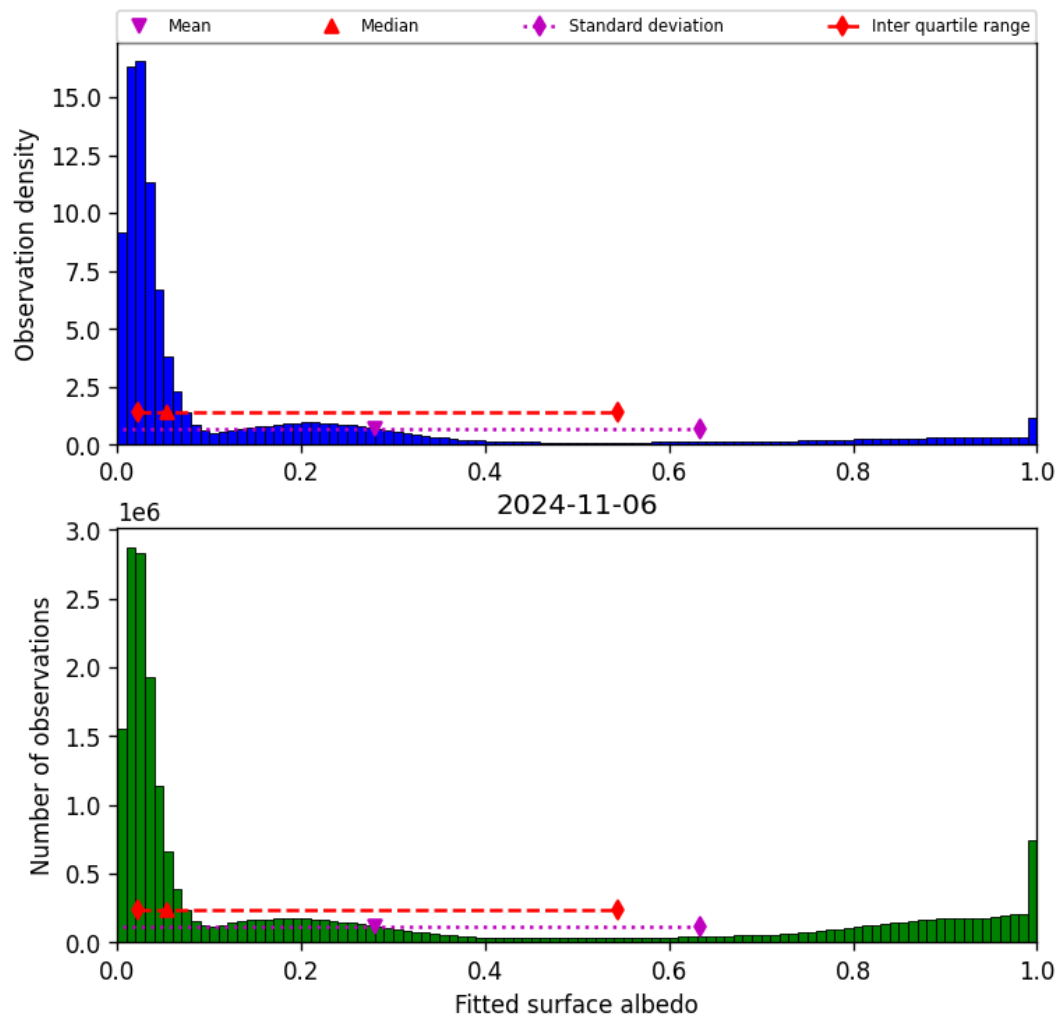
Figure 45: Histogram of “Fitted surface albedo” for 2024-11-05 to 2024-11-07
