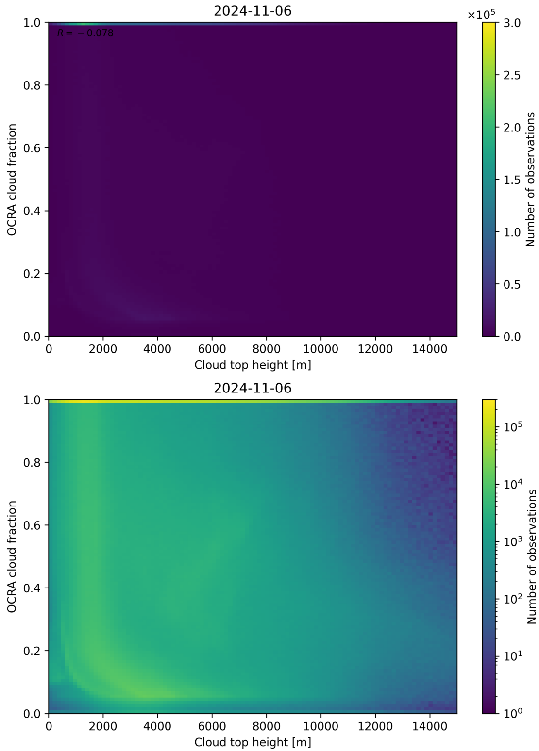
Figure 87: Scatter density plot of “Cloud top height” against “OCRA cloud fraction” for 2024-11-05 to 2024-11-07.
