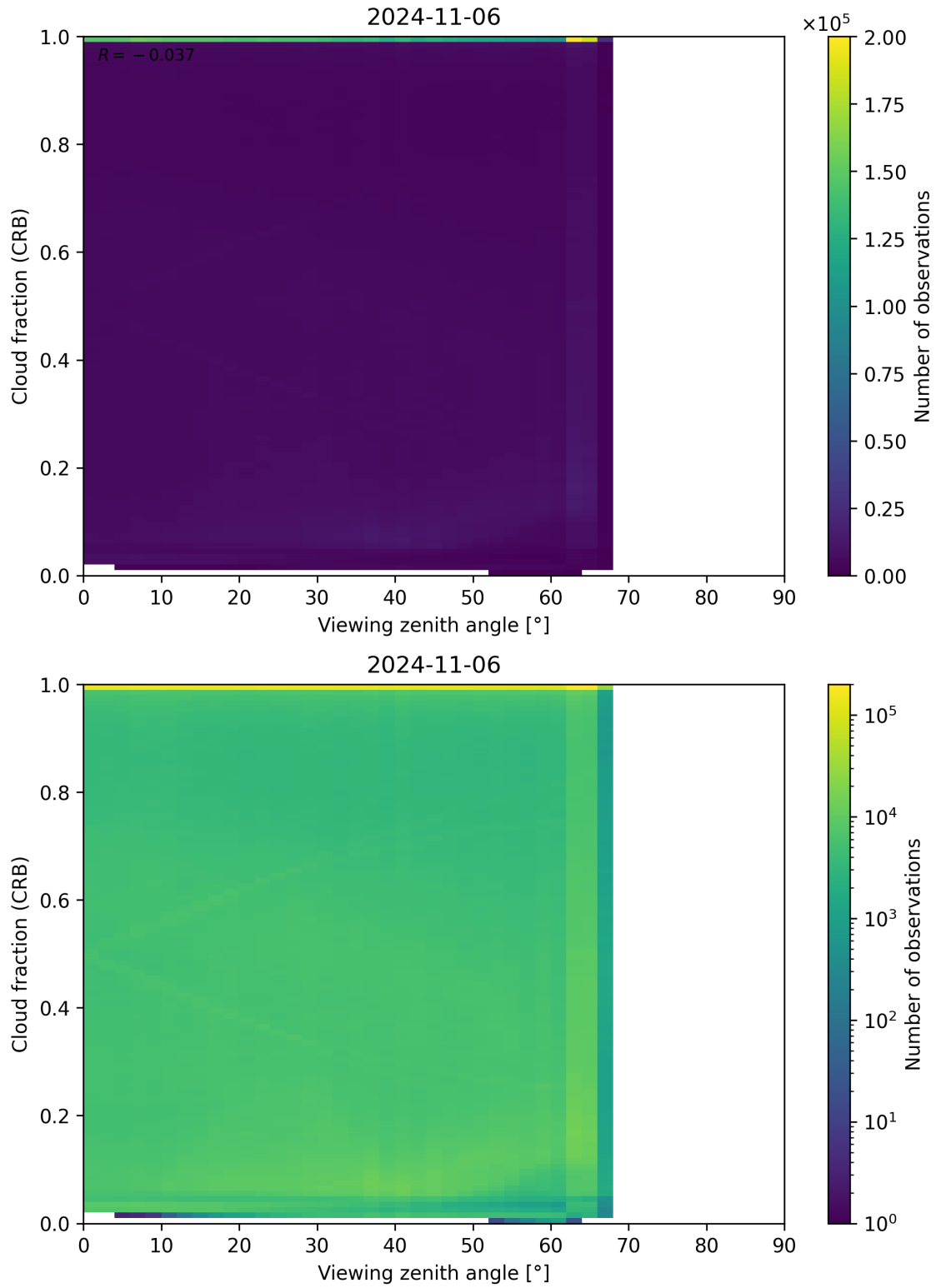
Figure 109: Scatter density plot of “Viewing zenith angle” against “Cloud fraction (CRB)” for 2024-11-05 to 2024-11-07.
