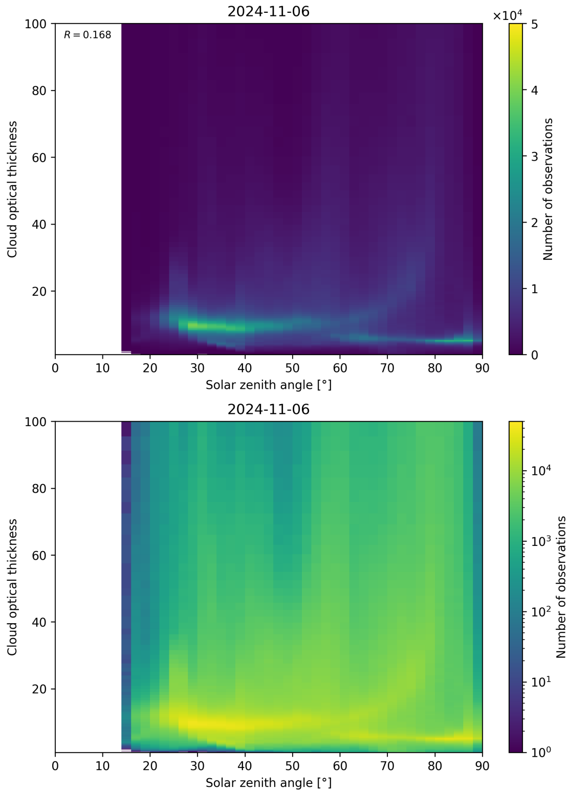
Figure 103: Scatter density plot of “Solar zenith angle” against “Cloud optical thickness” for 2024-11-05 to 2024-11-07.
