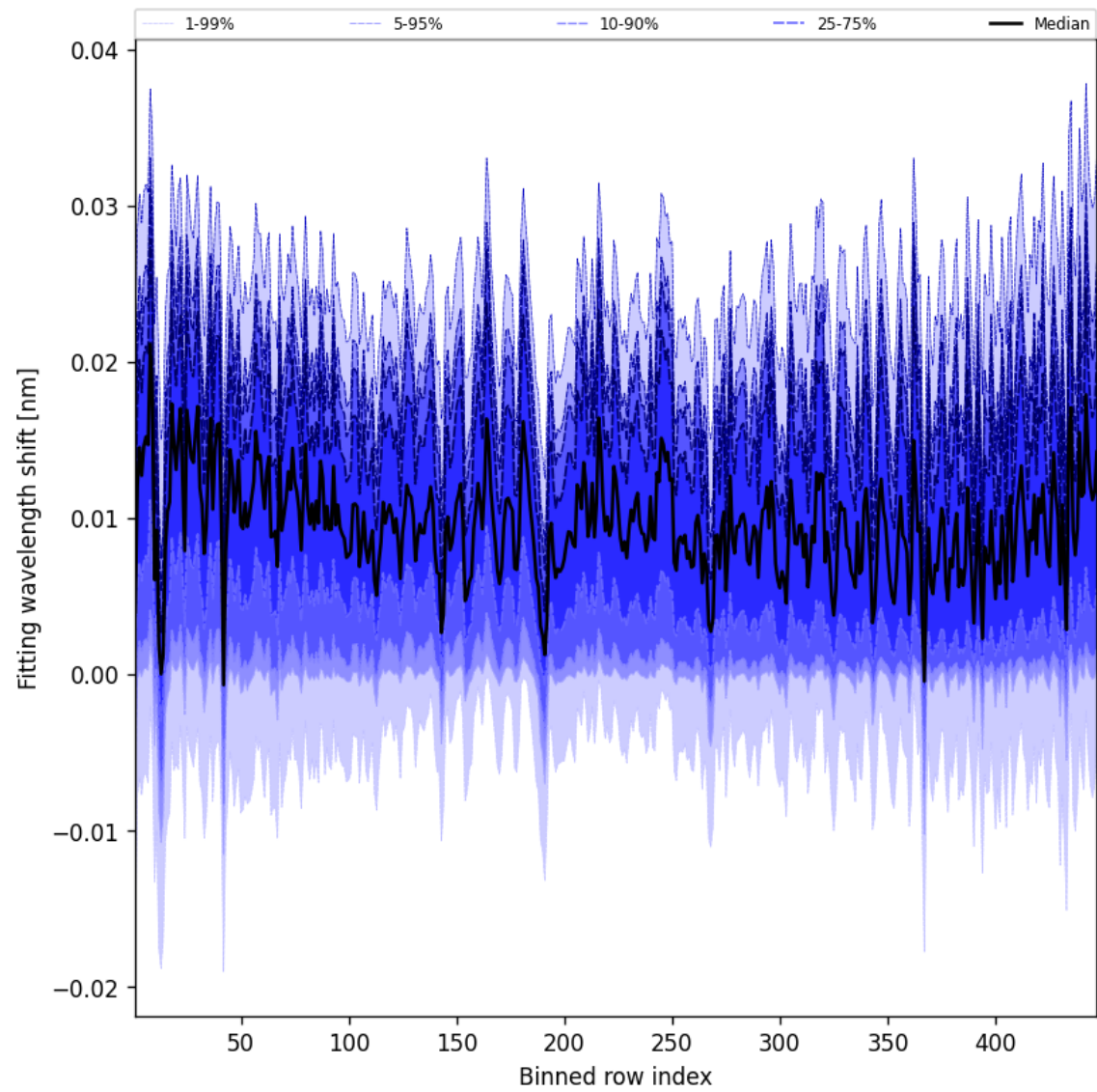
Figure 65: Along track statistics of “Fitting wavelength shift” for 2024-11-05 to 2024-11-07
