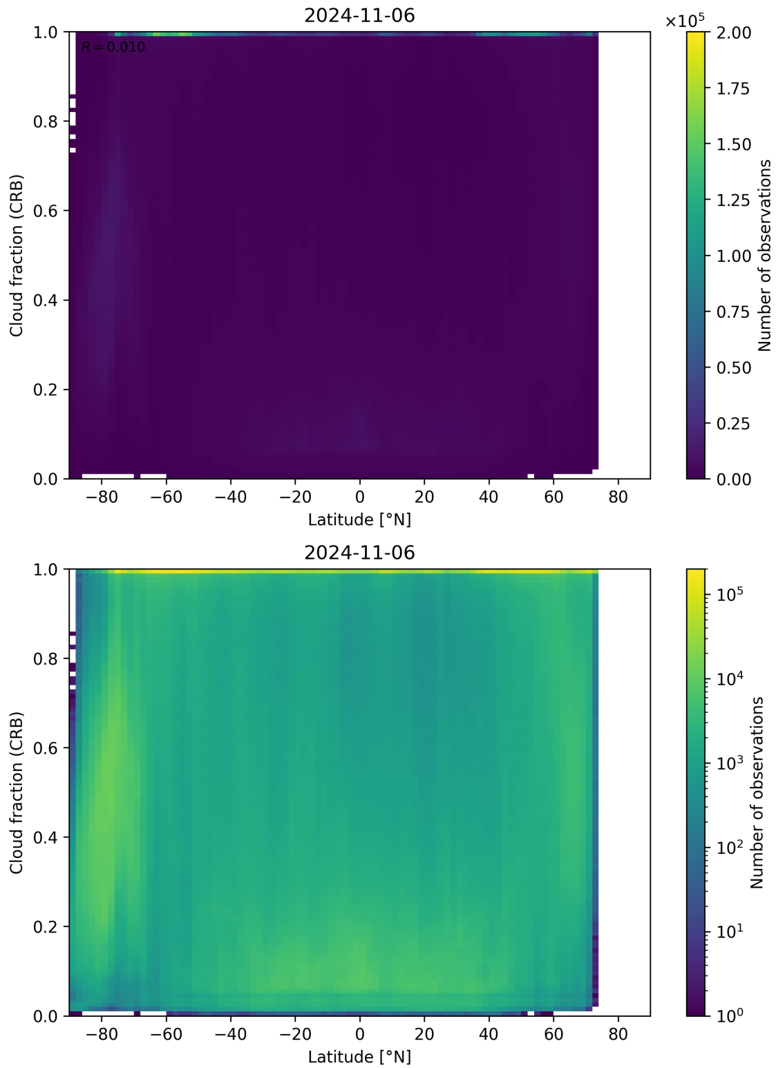
Figure 94: Scatter density plot of “Latitude” against “Cloud fraction (CRB)” for 2024-11-05 to 2024-11-07.
