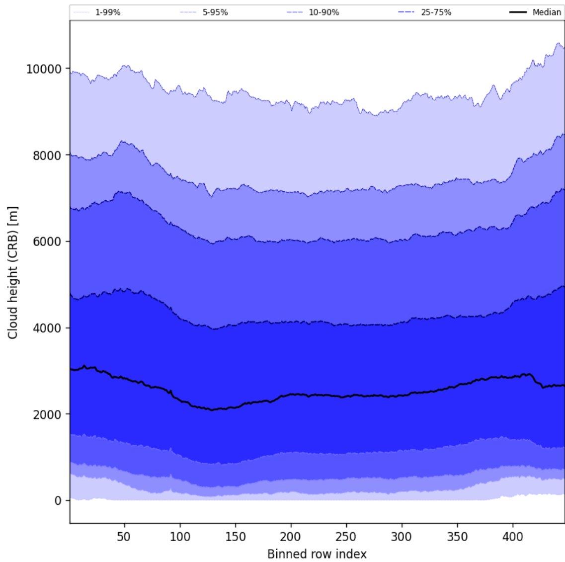
Figure 59: Along track statistics of “Cloud height (CRB)” for 2024-11-05 to 2024-11-07
