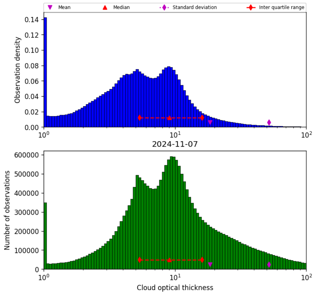
Figure 41: Histogram of “Cloud optical thickness” for 2024-11-06 to 2024-11-08
