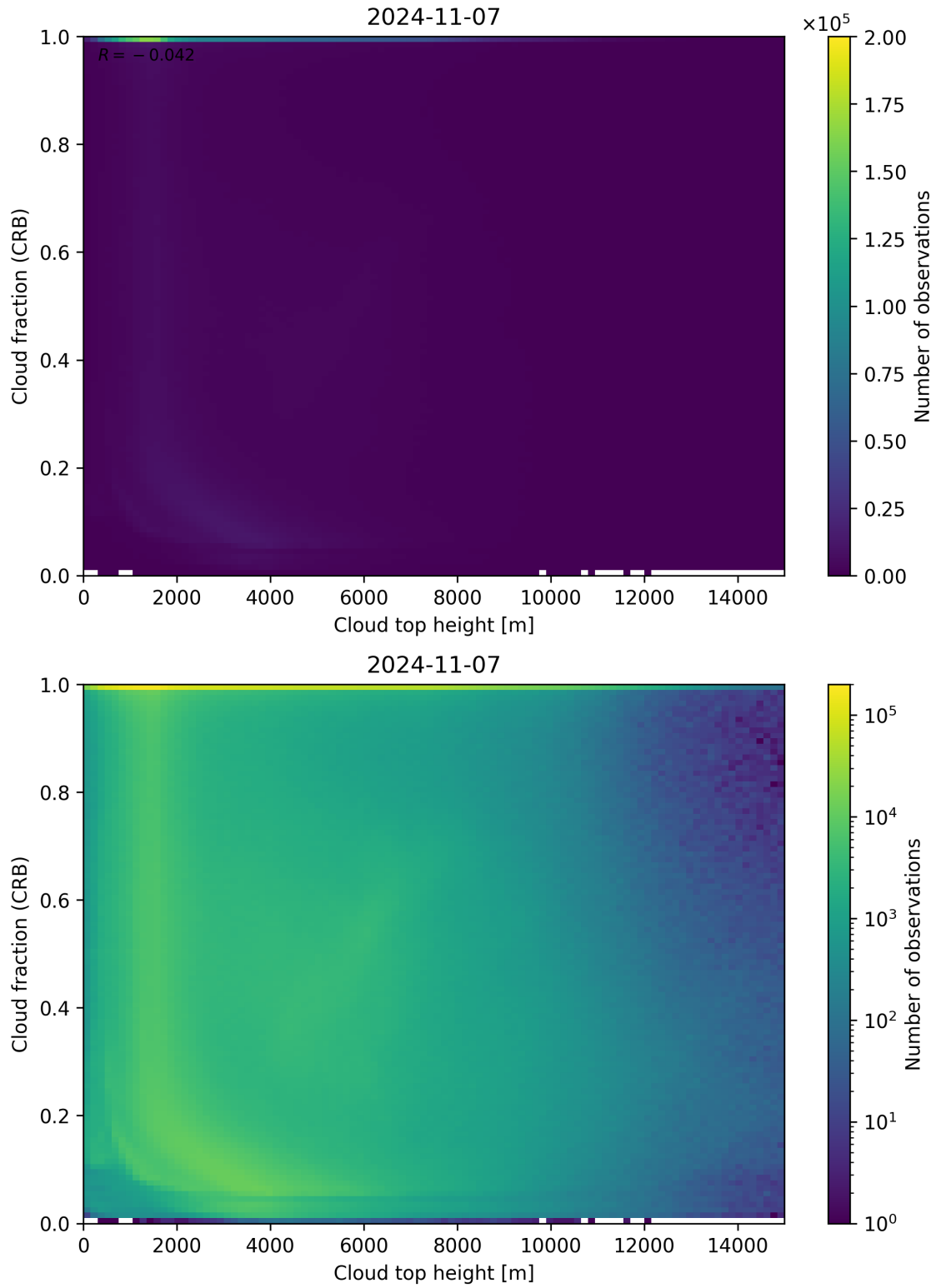
Figure 88: Scatter density plot of “Cloud top height” against “Cloud fraction (CRB)” for 2024-11-06 to 2024-11-08.
