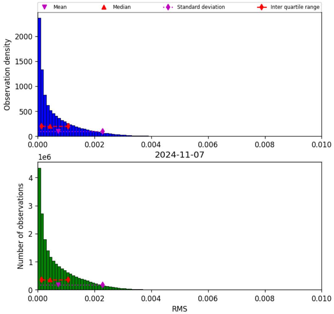
Figure 47: Histogram of “RMS” for 2024-11-06 to 2024-11-08
