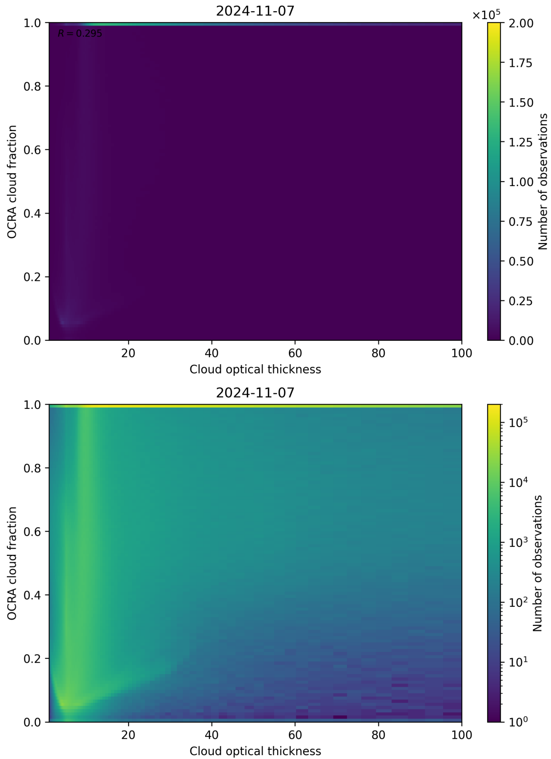
Figure 83: Scatter density plot of “Cloud optical thickness” against “OCRA cloud fraction” for 2024-11-06 to 2024-11-08.
