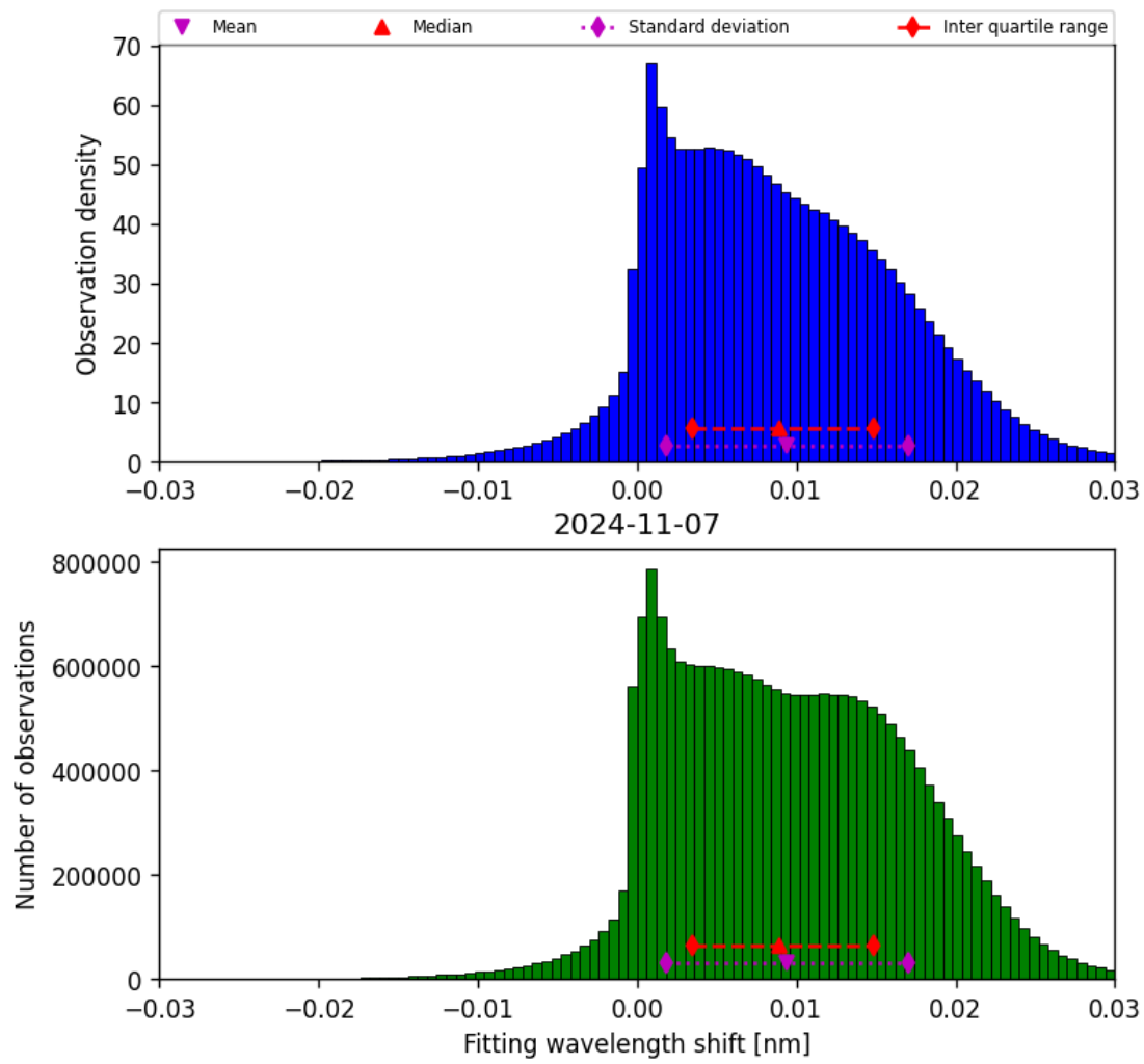
Figure 49: Histogram of “Fitting wavelength shift” for 2024-11-06 to 2024-11-08
