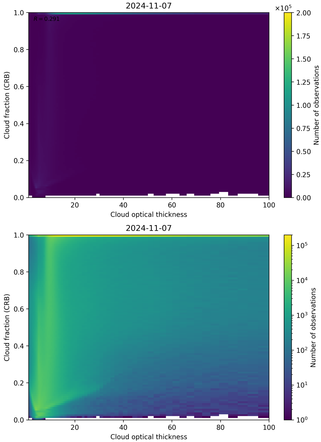
Figure 84: Scatter density plot of “Cloud optical thickness” against “Cloud fraction (CRB)” for 2024-11-06 to 2024-11-08.
