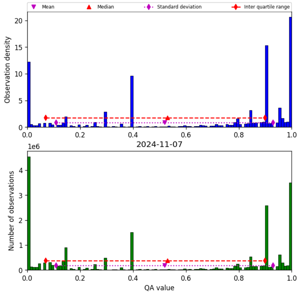
Figure 38: Histogram of “QA value” for 2024-11-06 to 2024-11-08
