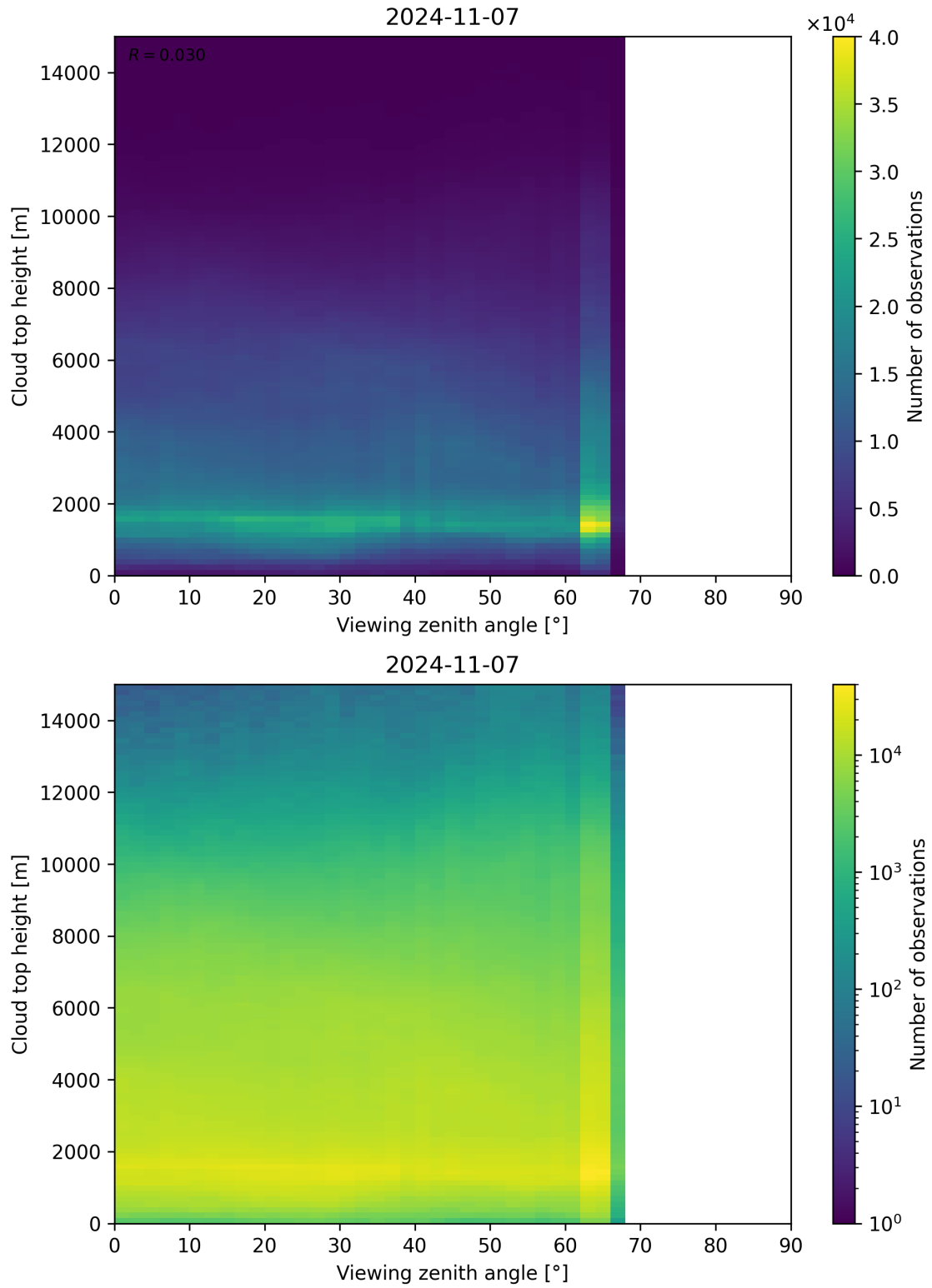
Figure 112: Scatter density plot of “Viewing zenith angle” against “Cloud top height” for 2024-11-06 to 2024-11-08.
