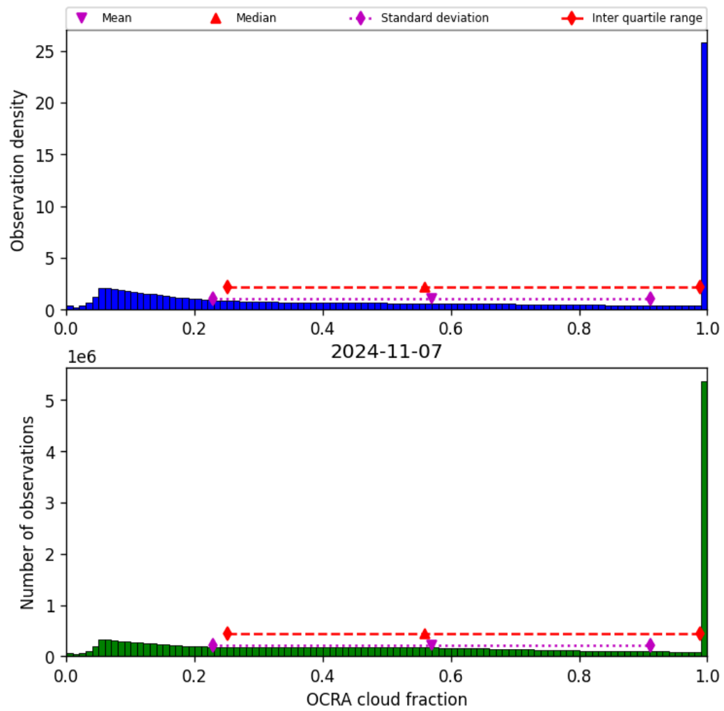
Figure 50: Histogram of “OCRA cloud fraction” for 2024-11-06 to 2024-11-08
