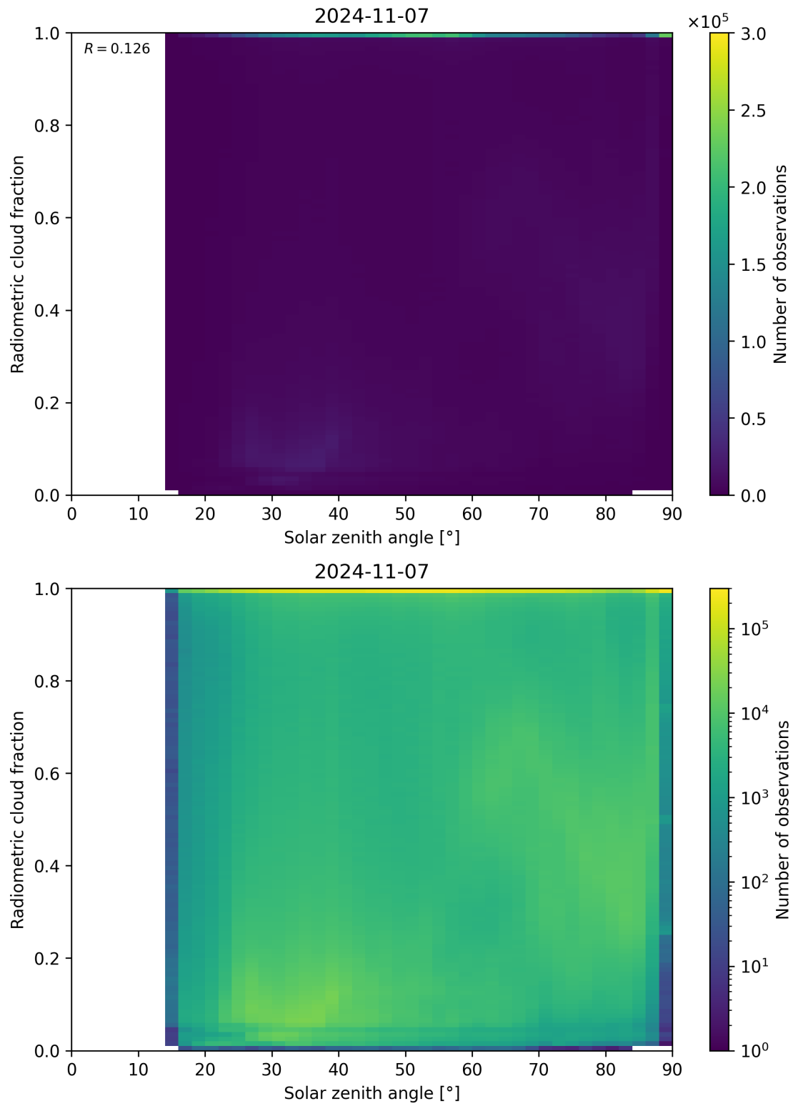
Figure 99: Scatter density plot of “Solar zenith angle” against “Radiometric cloud fraction” for 2024-11-06 to 2024-11-08.
