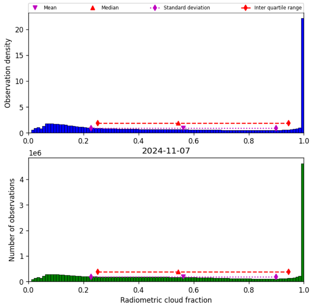
Figure 39: Histogram of “Radiometric cloud fraction” for 2024-11-06 to 2024-11-08
