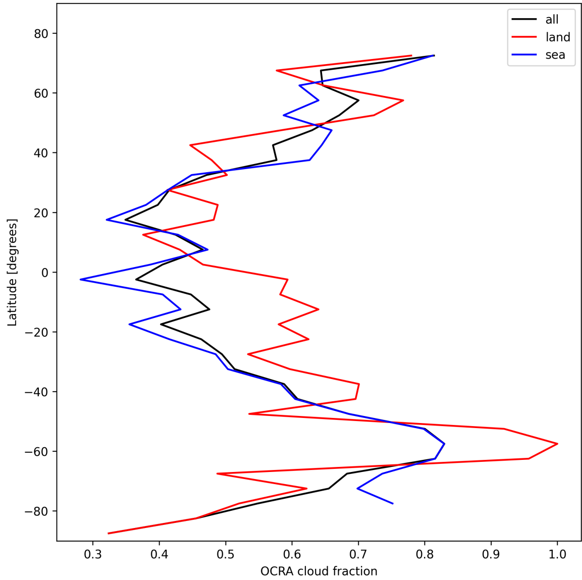
Figure 34: Zonal average of “OCRA cloud fraction” for 2024-11-06 to 2024-11-08.
