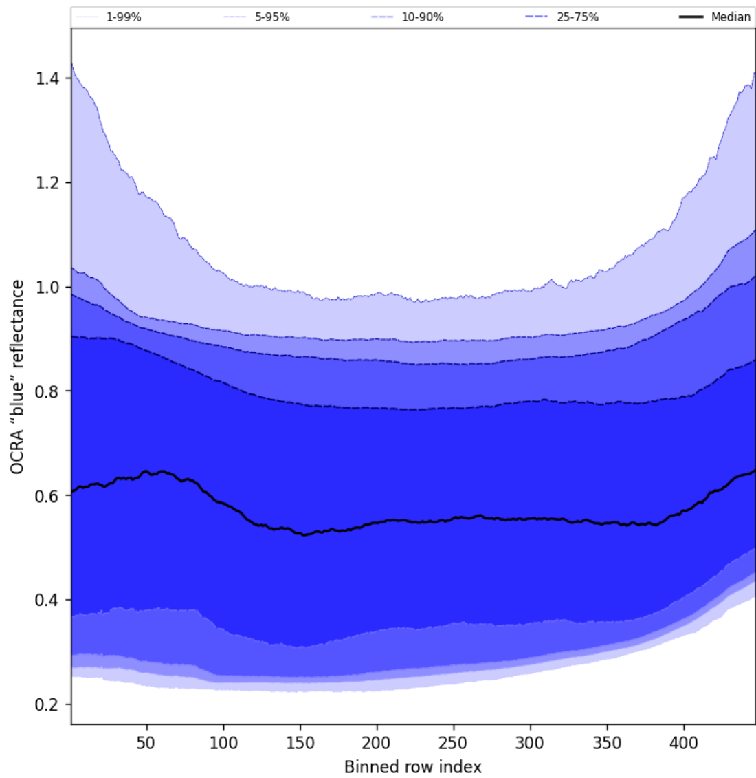
Figure 67: Along track statistics of “OCRA “blue” reflectance” for 2024-11-06 to 2024-11-08
