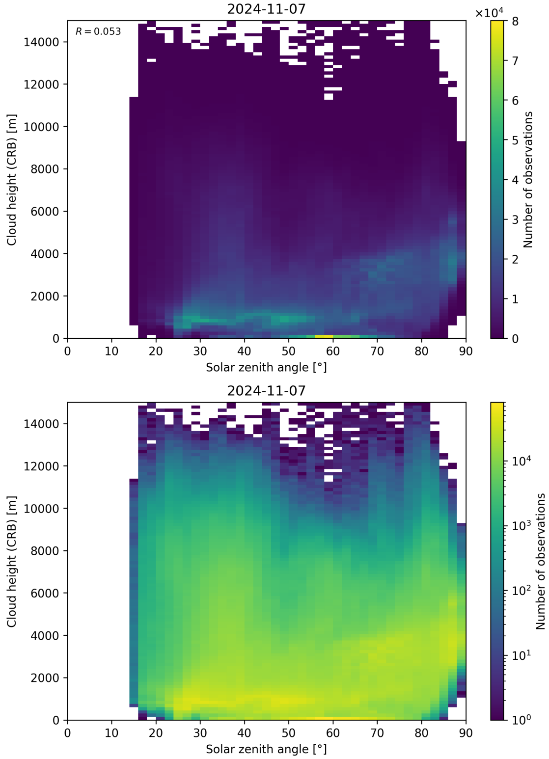
Figure 102: Scatter density plot of “Solar zenith angle” against “Cloud height (CRB)” for 2024-11-06 to 2024-11-08.
