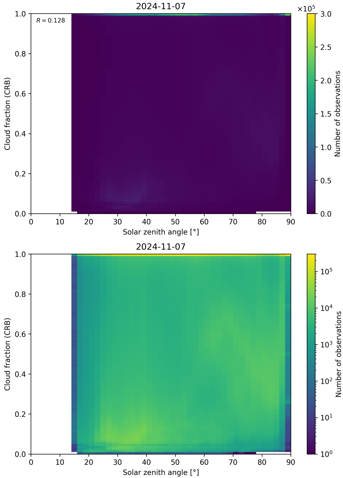
Figure 101: Scatter density plot of “Solar zenith angle” against “Cloud fraction (CRB)” for 2024-11-06 to 2024-11-08.
