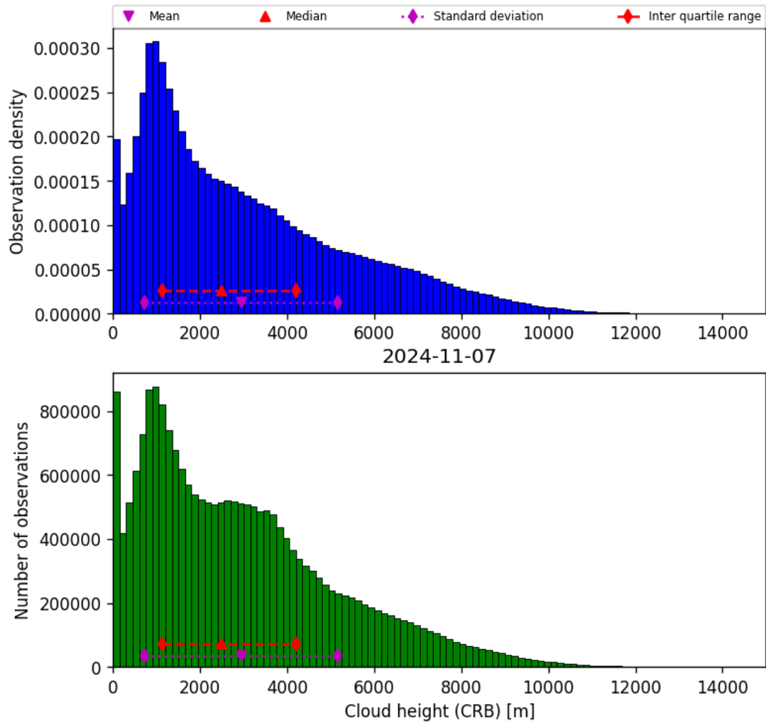
Figure 43: Histogram of “Cloud height (CRB)” for 2024-11-06 to 2024-11-08
