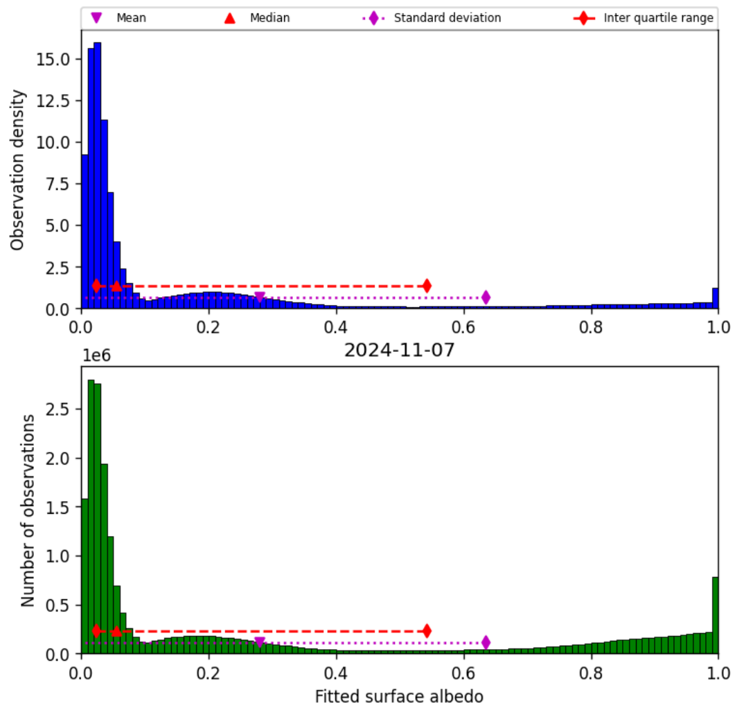
Figure 45: Histogram of “Fitted surface albedo” for 2024-11-06 to 2024-11-08
