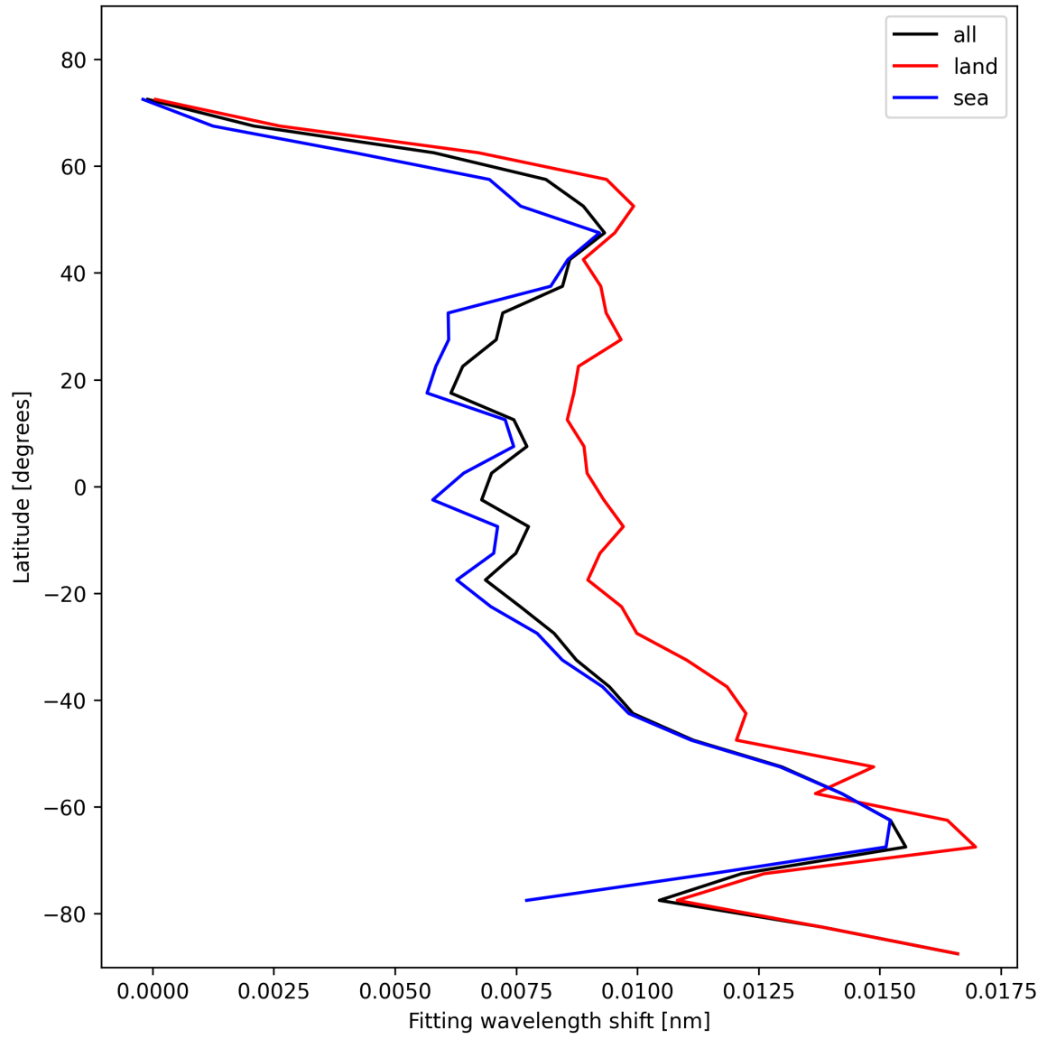
Figure 33: Zonal average of “Fitting wavelength shift” for 2024-11-06 to 2024-11-08.
