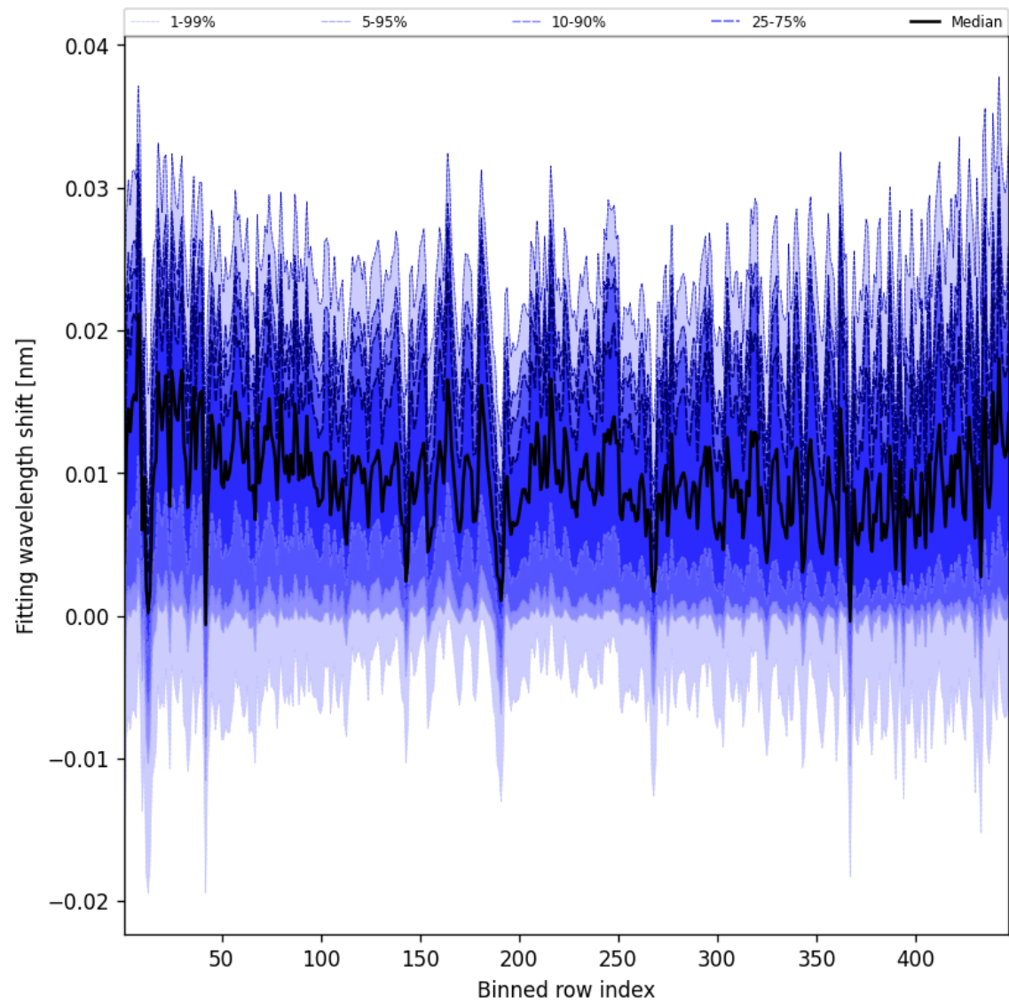
Figure 65: Along track statistics of “Fitting wavelength shift” for 2024-11-06 to 2024-11-08
