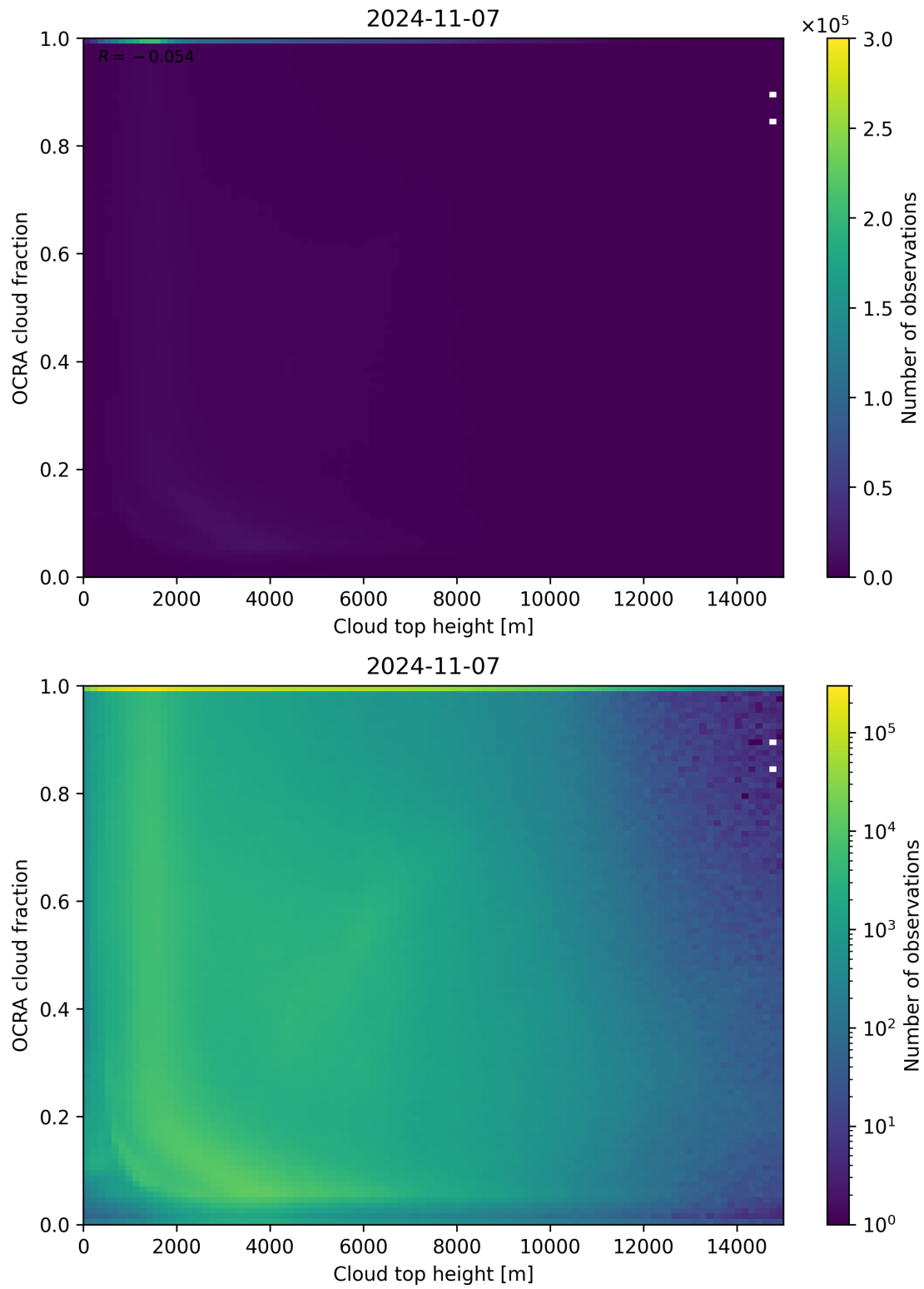
Figure 87: Scatter density plot of “Cloud top height” against “OCRA cloud fraction” for 2024-11-06 to 2024-11-08.
