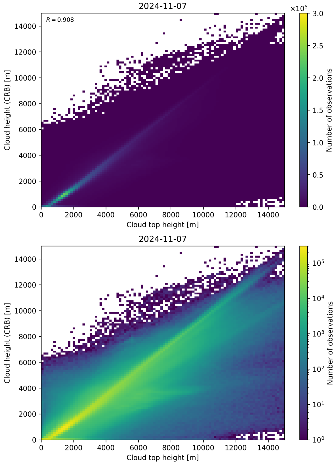
Figure 89: Scatter density plot of “Cloud top height” against “Cloud height (CRB)” for 2024-11-06 to 2024-11-08.
