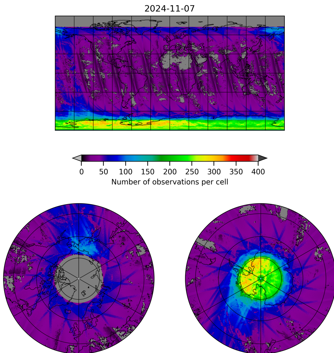
Figure 21: Map of the number of observations for 2024-11-06 to 2024-11-08
