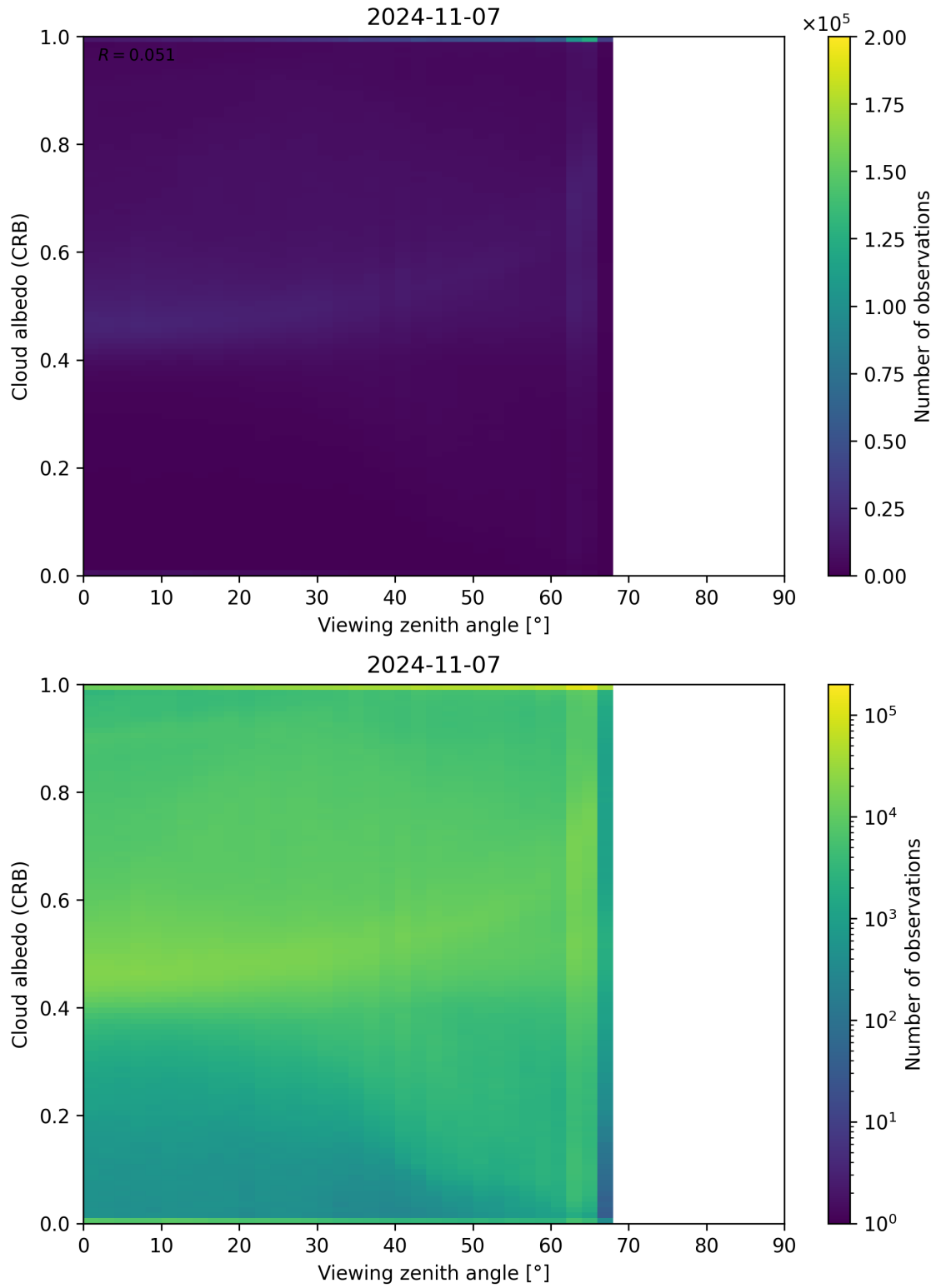
Figure 106: Scatter density plot of “Viewing zenith angle” against “Cloud albedo (CRB)” for 2024-11-06 to 2024-11-08.
