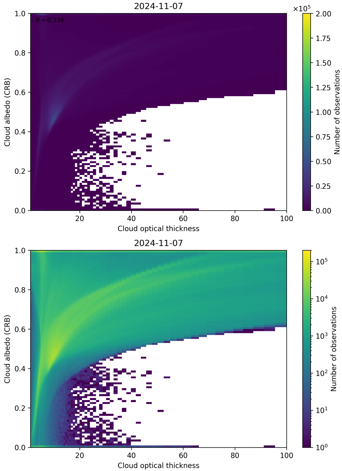
Figure 82: Scatter density plot of “Cloud optical thickness” against “Cloud albedo (CRB)” for 2024-11-06 to 2024-11-08.
