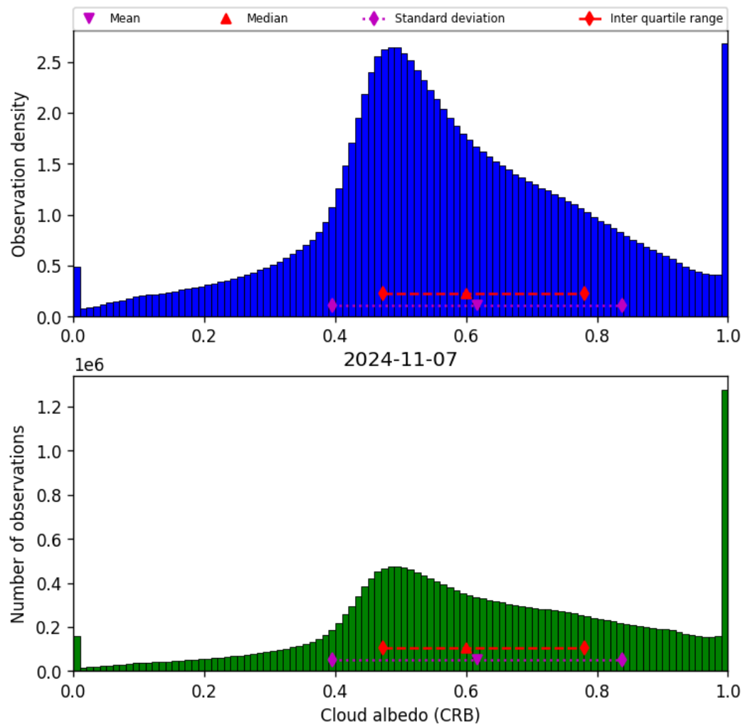
Figure 44: Histogram of “Cloud albedo (CRB)” for 2024-11-06 to 2024-11-08
