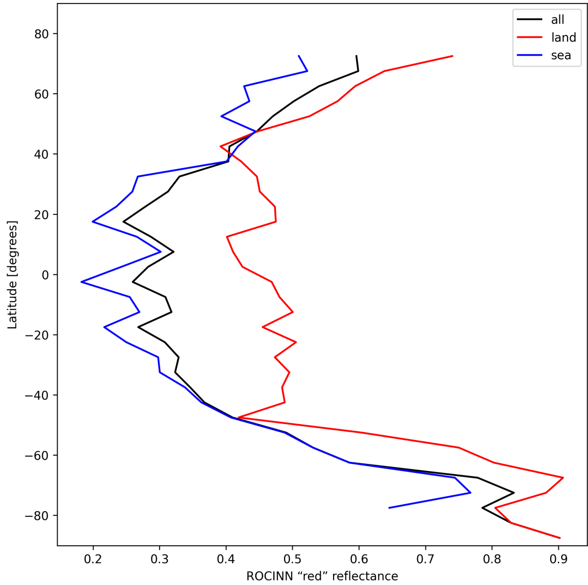
Figure 37: Zonal average of "ROCINN "red" reflectance" for 2024-11-06 to 2024-11-08.
