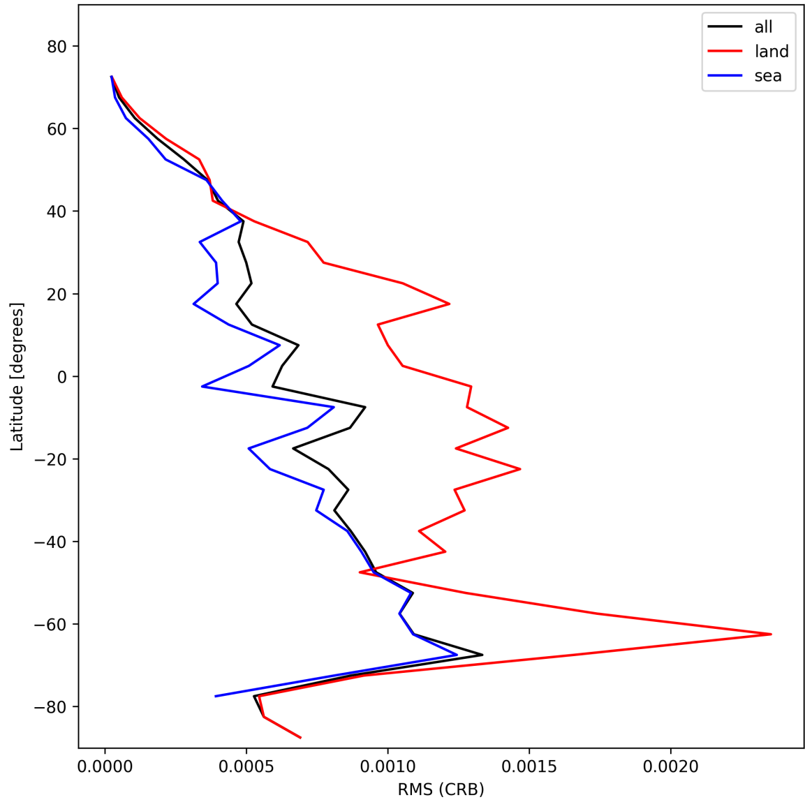
Figure 32: Zonal average of “RMS (CRB)” for 2024-11-06 to 2024-11-08.
