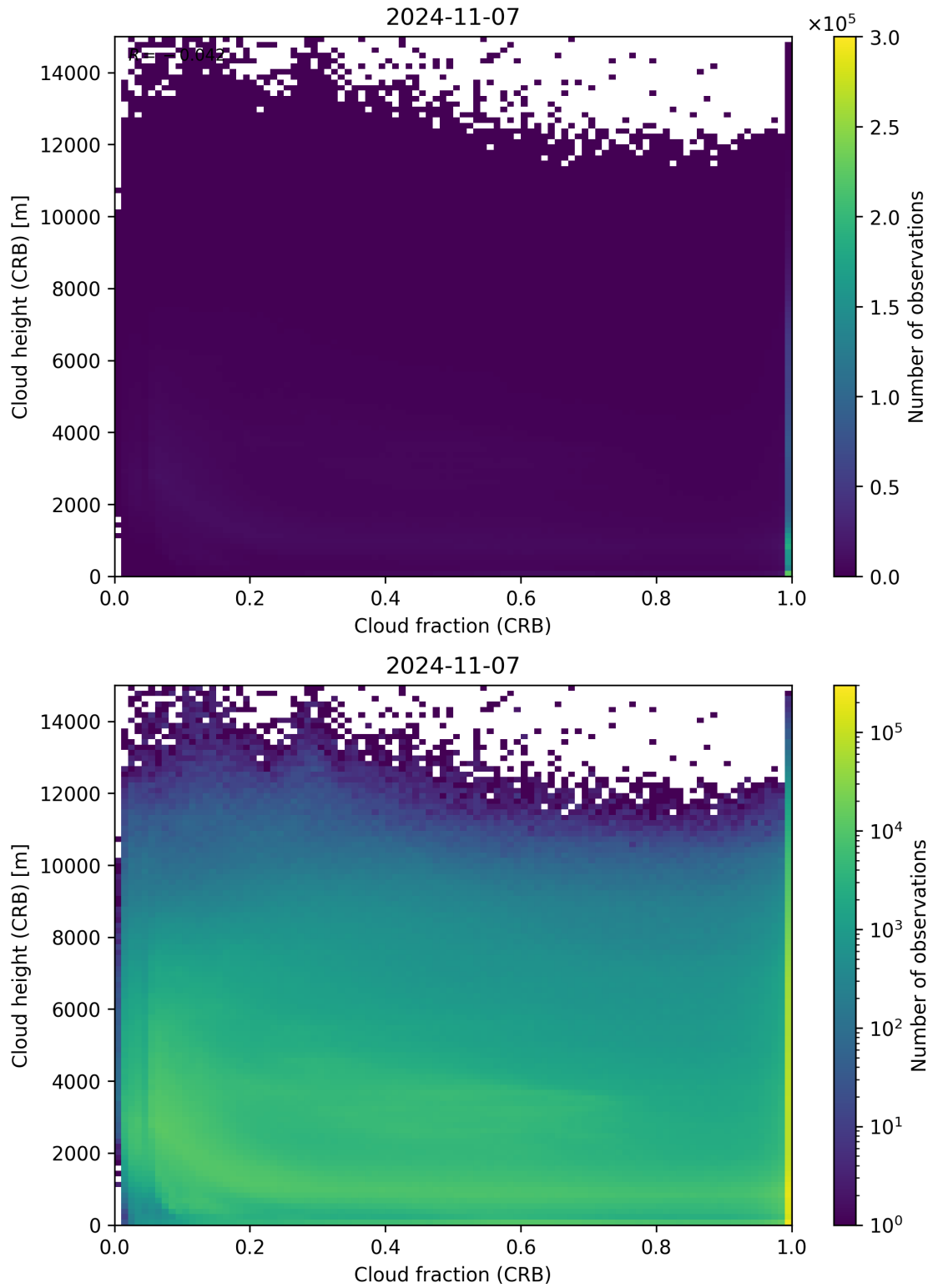
Figure 79: Scatter density plot of “Cloud fraction (CRB)” against “Cloud height (CRB)” for 2024-11-06 to 2024-11-08.
