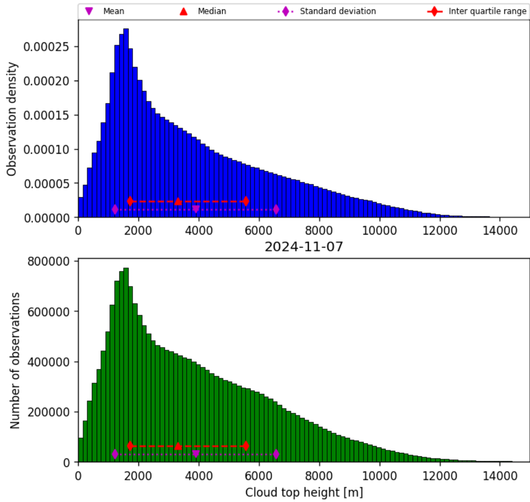
Figure 40: Histogram of “Cloud top height” for 2024-11-06 to 2024-11-08
