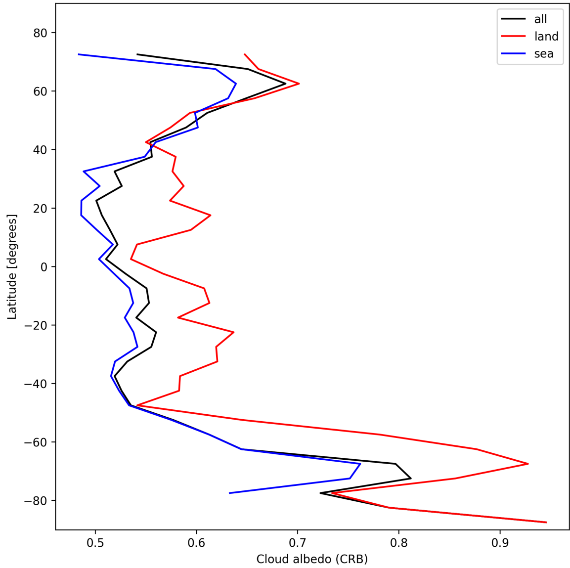
Figure 28: Zonal average of “Cloud albedo (CRB)” for 2024-11-06 to 2024-11-08.
