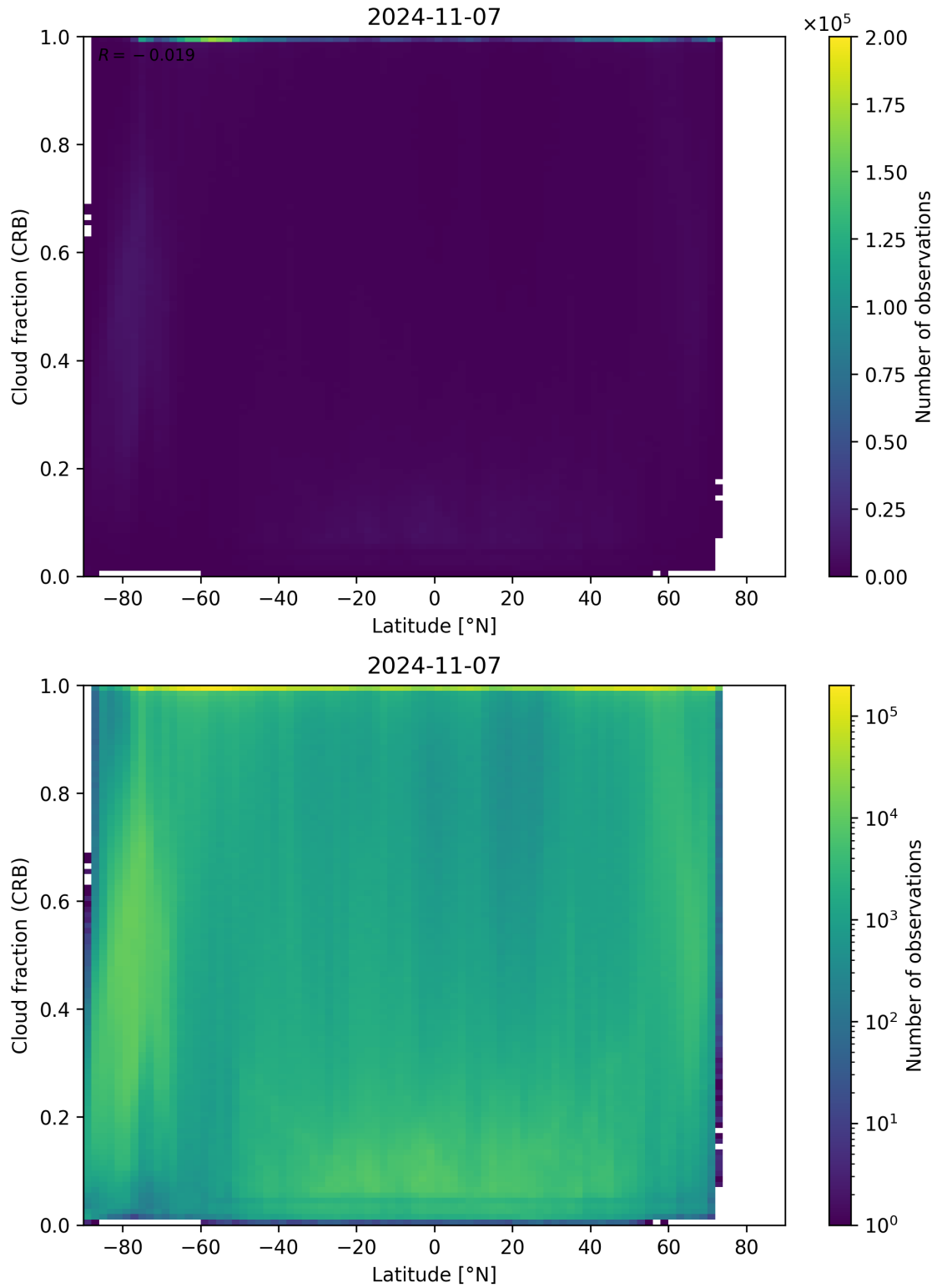
Figure 94: Scatter density plot of “Latitude” against “Cloud fraction (CRB)” for 2024-11-06 to 2024-11-08.
