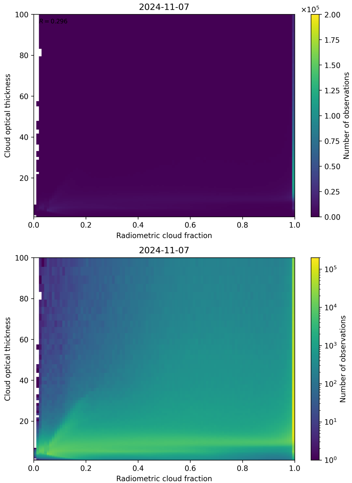
Figure 75: Scatter density plot of “Radiometric cloud fraction” against “Cloud optical thickness” for 2024-11-06 to 2024-11-08.
