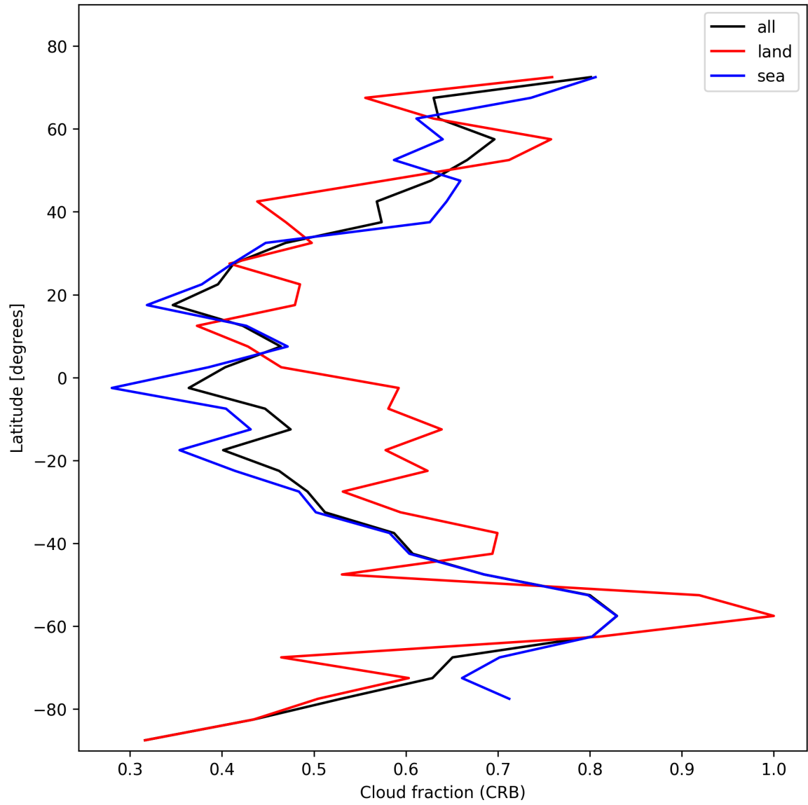
Figure 26: Zonal average of “Cloud fraction (CRB)” for 2024-11-06 to 2024-11-08.
