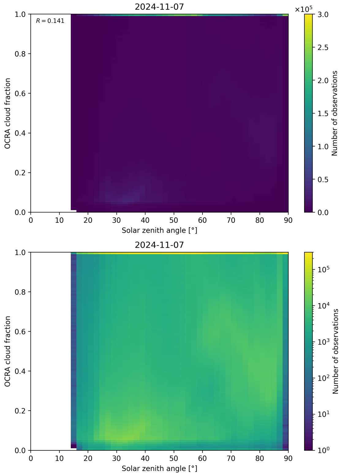
Figure 100: Scatter density plot of “Solar zenith angle” against “OCRA cloud fraction” for 2024-11-06 to 2024-11-08.
