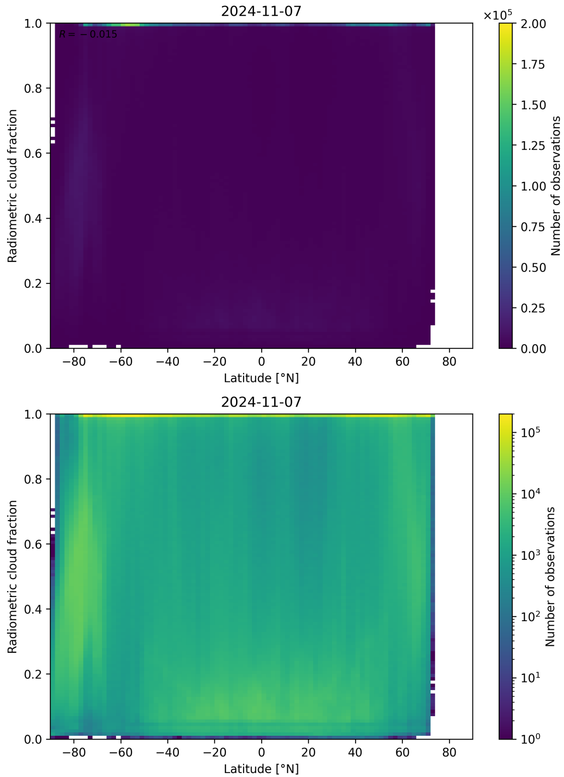
Figure 92: Scatter density plot of “Latitude” against “Radiometric cloud fraction” for 2024-11-06 to 2024-11-08.
