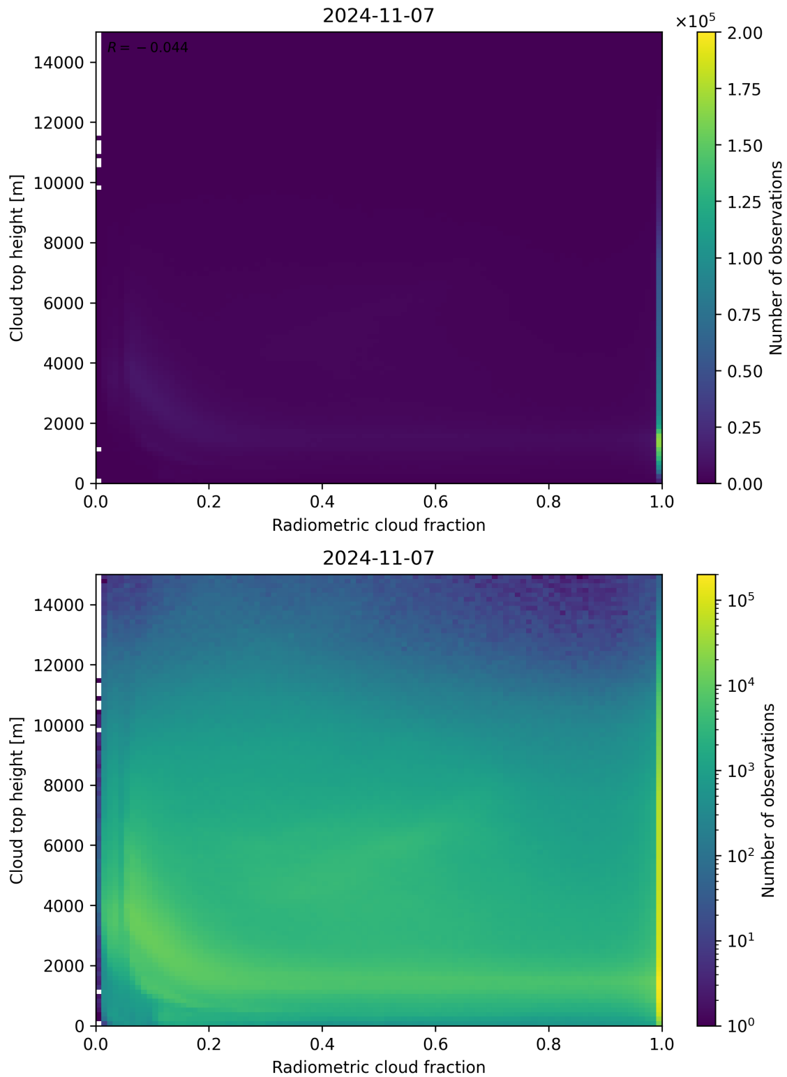
Figure 76: Scatter density plot of “Radiometric cloud fraction” against “Cloud top height” for 2024-11-06 to 2024-11-08.
