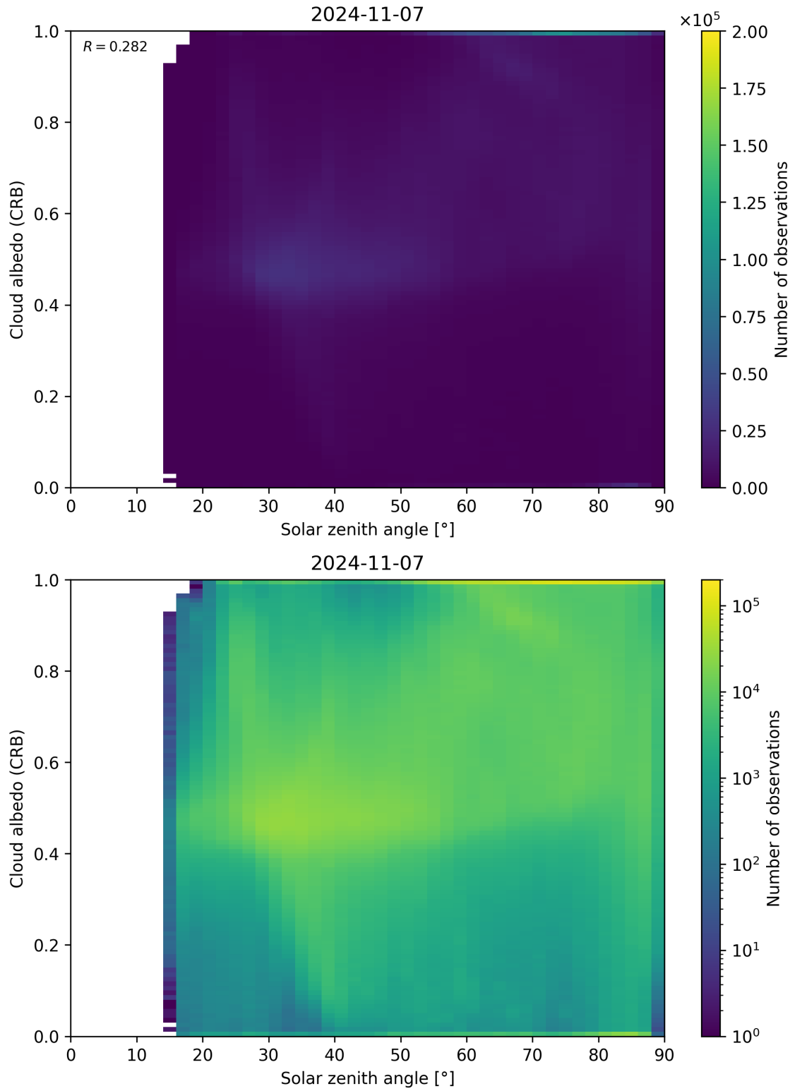
Figure 98: Scatter density plot of “Solar zenith angle” against “Cloud albedo (CRB)” for 2024-11-06 to 2024-11-08.
