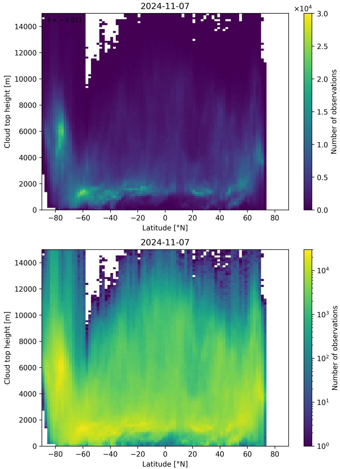
Figure 97: Scatter density plot of “Latitude” against “Cloud top height” for 2024-11-06 to 2024-11-08.
