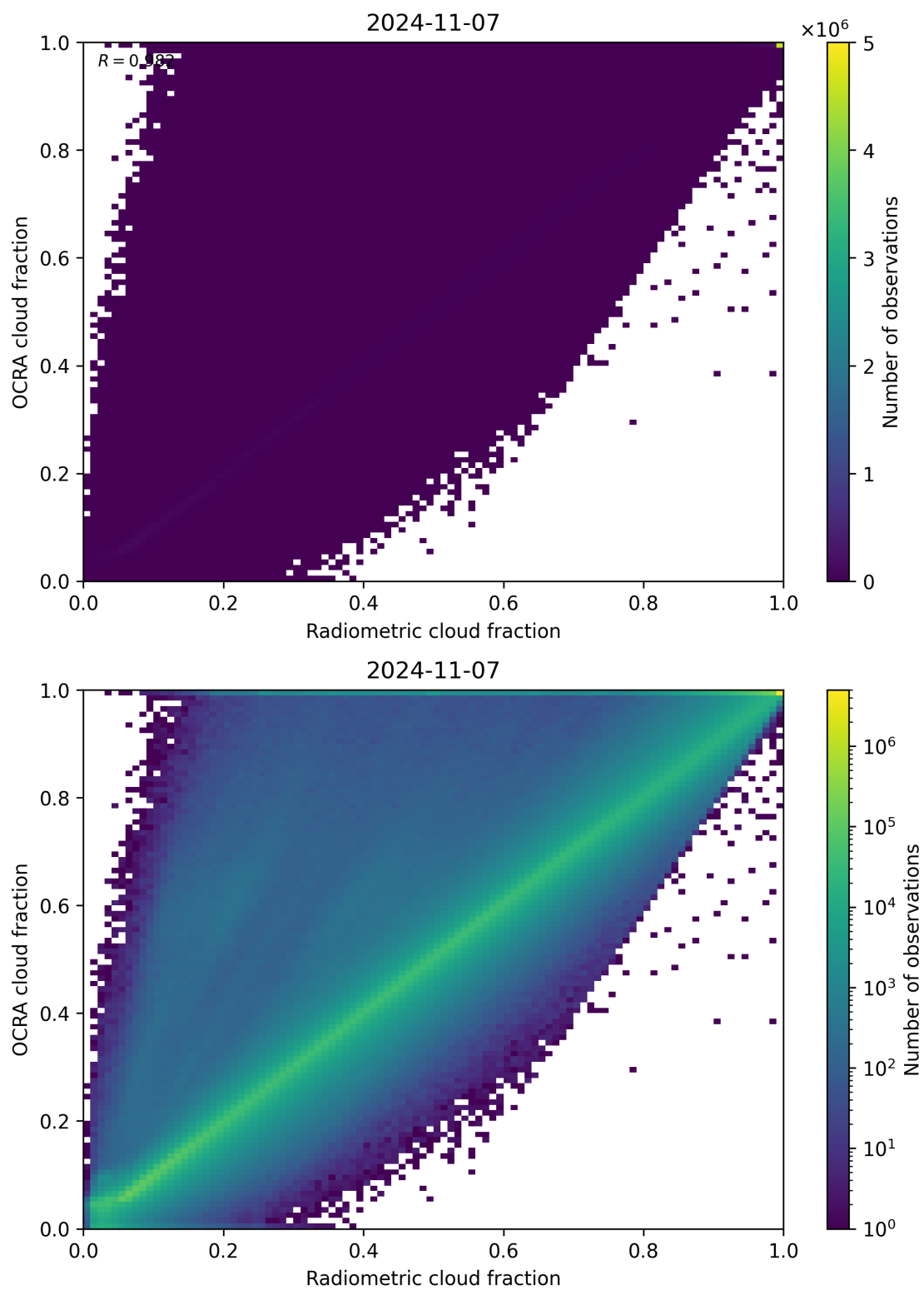
Figure 72: Scatter density plot of “Radiometric cloud fraction” against “OCRA cloud fraction” for 2024-11-06 to 2024-11-08.
