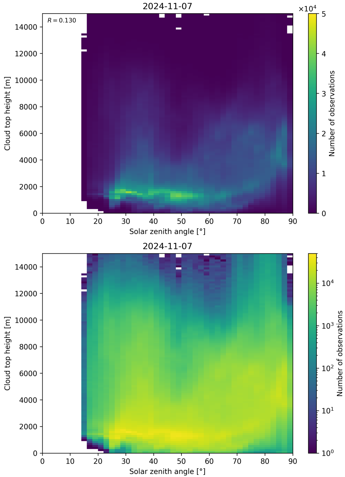
Figure 104: Scatter density plot of “Solar zenith angle” against “Cloud top height” for 2024-11-06 to 2024-11-08.
