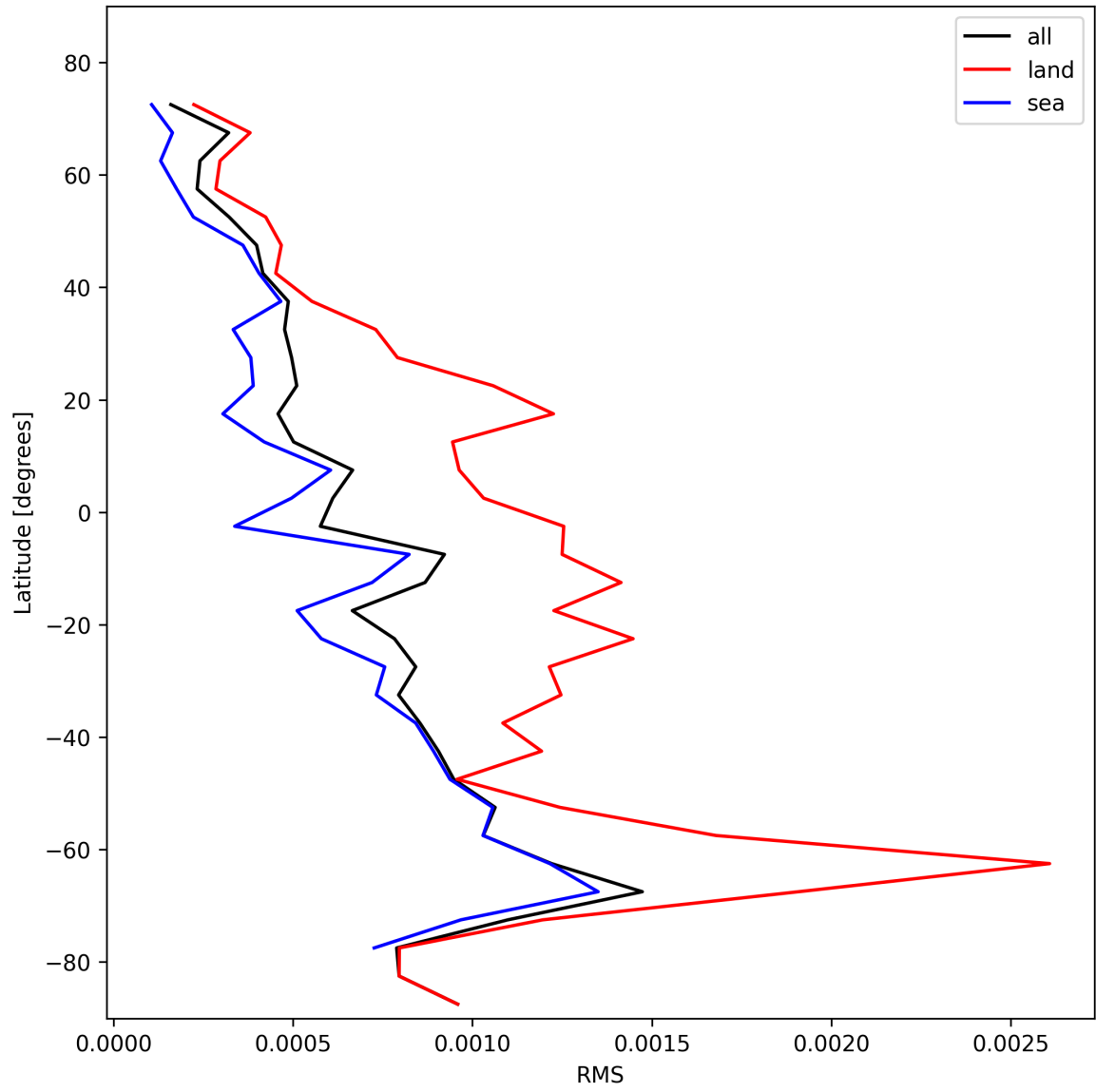
Figure 31: Zonal average of “RMS” for 2024-11-06 to 2024-11-08.
