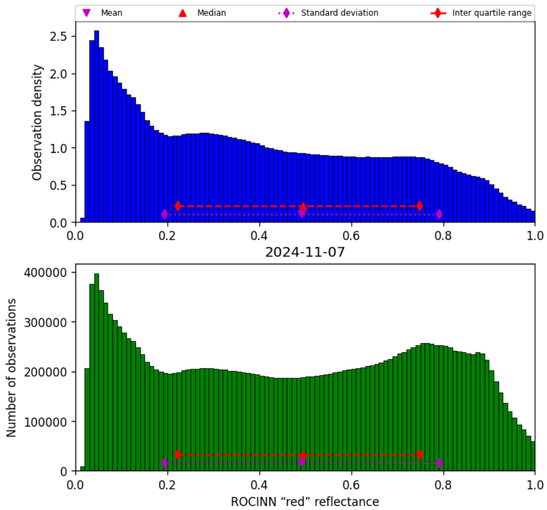
Figure 53: Histogram of “ROCINN “red” reflectance” for 2024-11-06 to 2024-11-08
