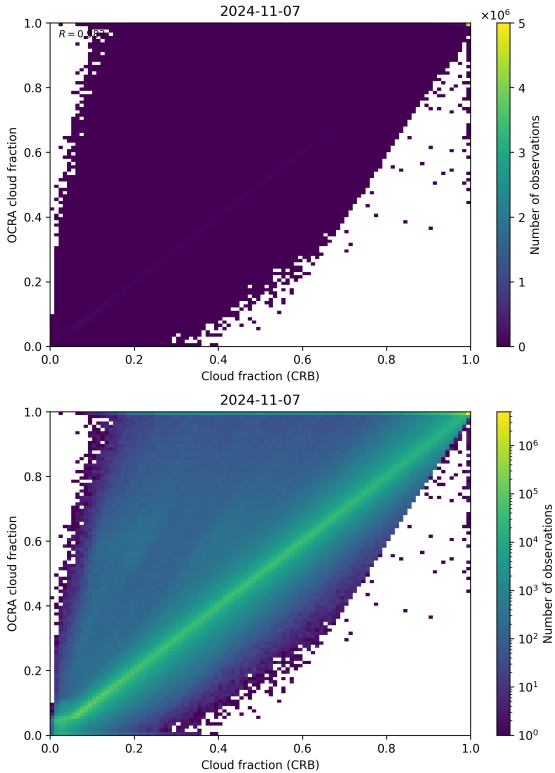
Figure 78: Scatter density plot of “Cloud fraction (CRB)” against “OCRA cloud fraction” for 2024-11-06 to 2024-11-08.
