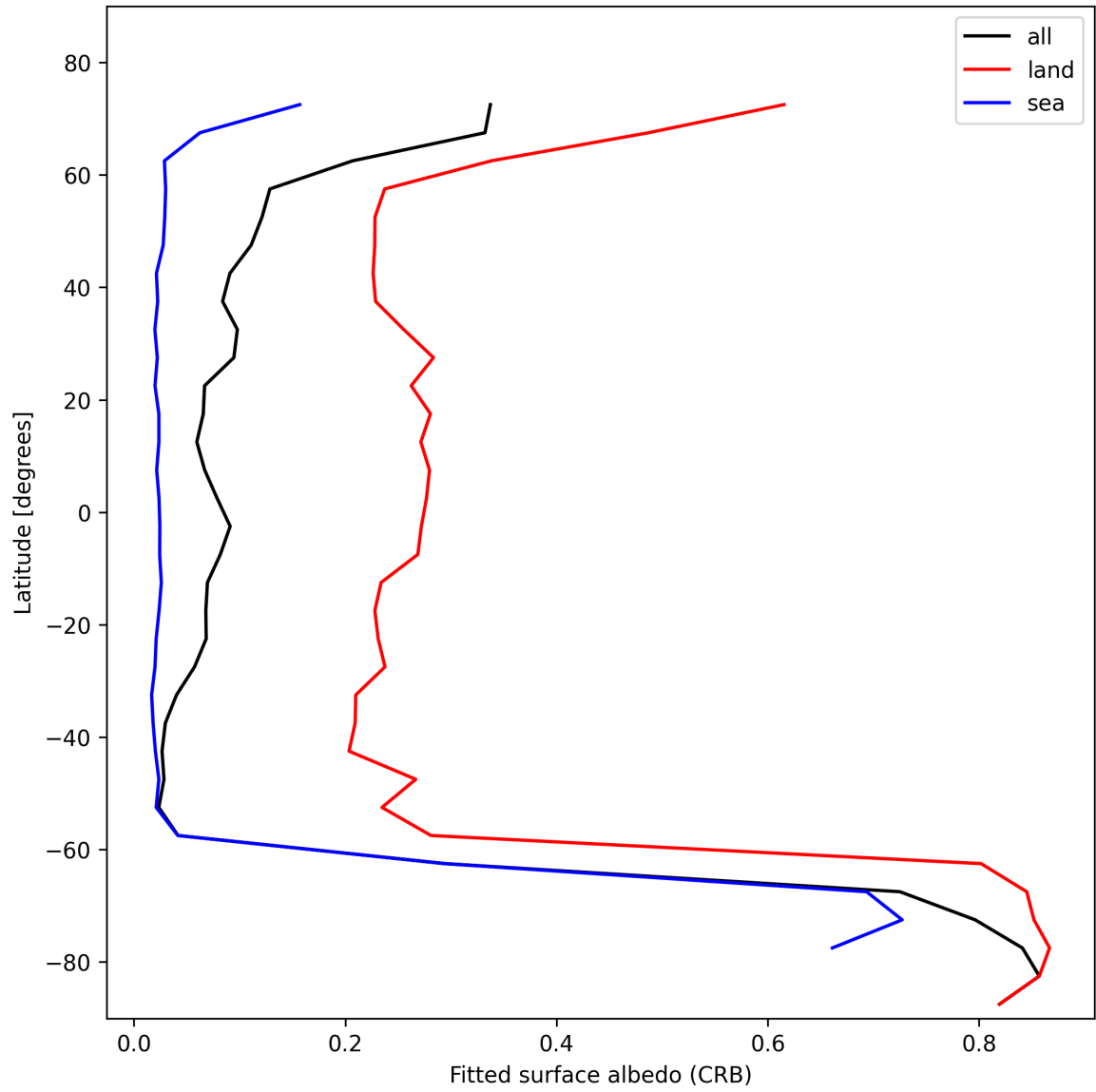
Figure 30: Zonal average of “Fitted surface albedo (CRB)” for 2024-11-06 to 2024-11-08.
