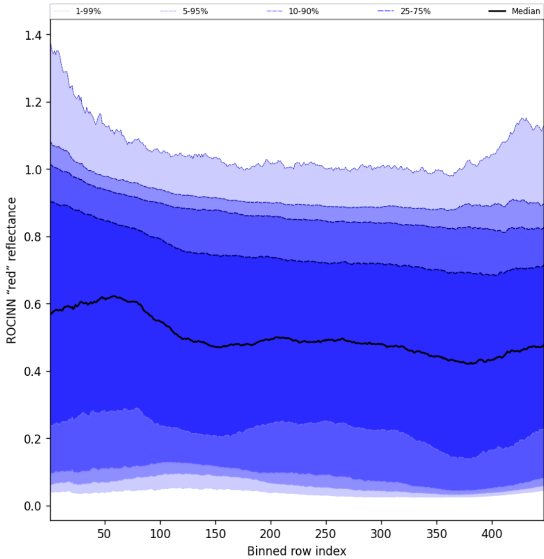
Figure 69: Along track statistics of “ROCINN “red” reflectance” for 2024-11-06 to 2024-11-08
