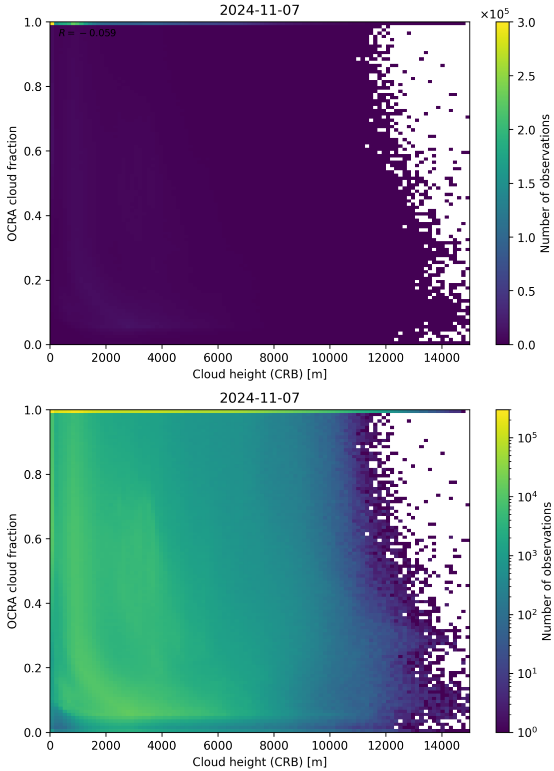
Figure 81: Scatter density plot of “Cloud height (CRB)” against “OCRA cloud fraction” for 2024-11-06 to 2024-11-08.
