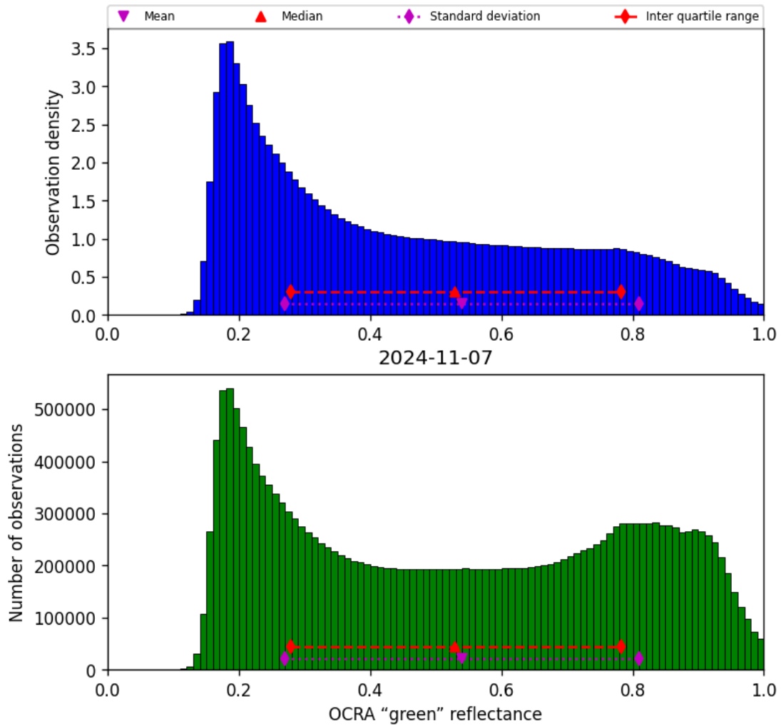
Figure 52: Histogram of “OCRA “green” reflectance” for 2024-11-06 to 2024-11-08
