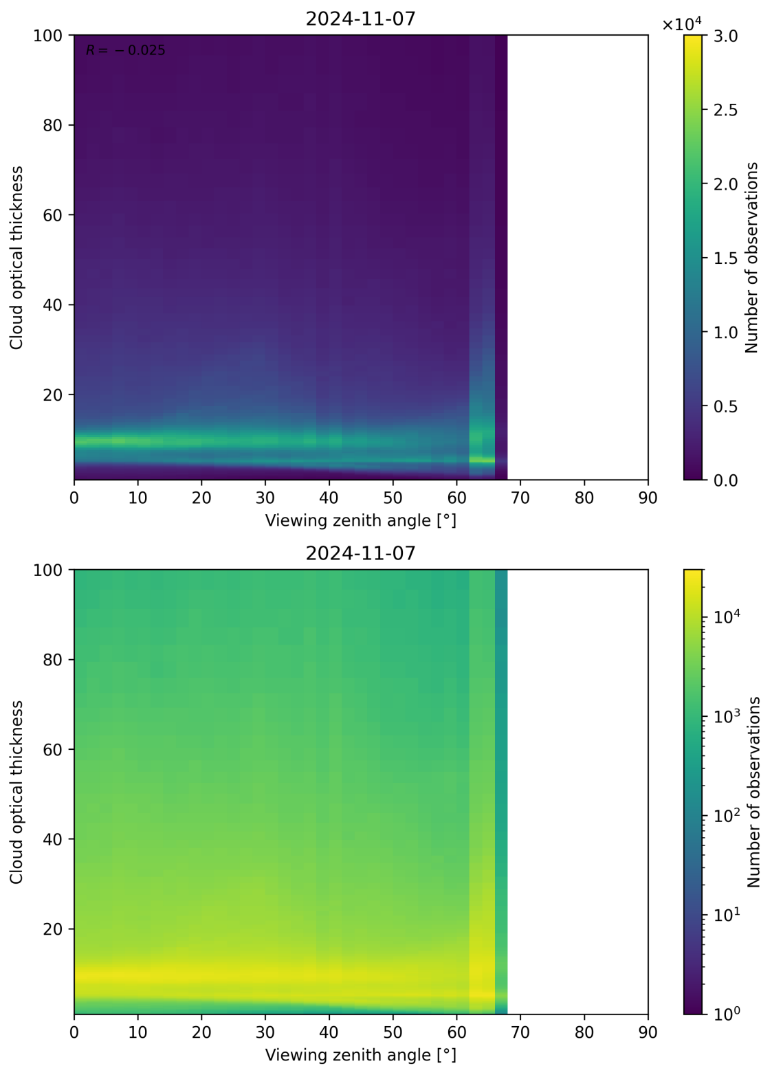
Figure 111: Scatter density plot of “Viewing zenith angle” against “Cloud optical thickness” for 2024-11-06 to 2024-11-08.
