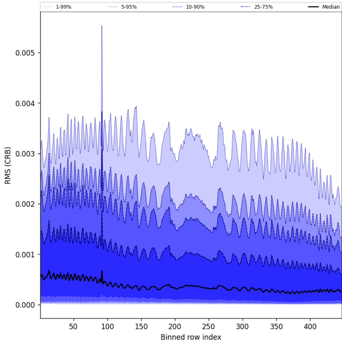
Figure 64: Along track statistics of “RMS (CRB)” for 2024-11-06 to 2024-11-08
