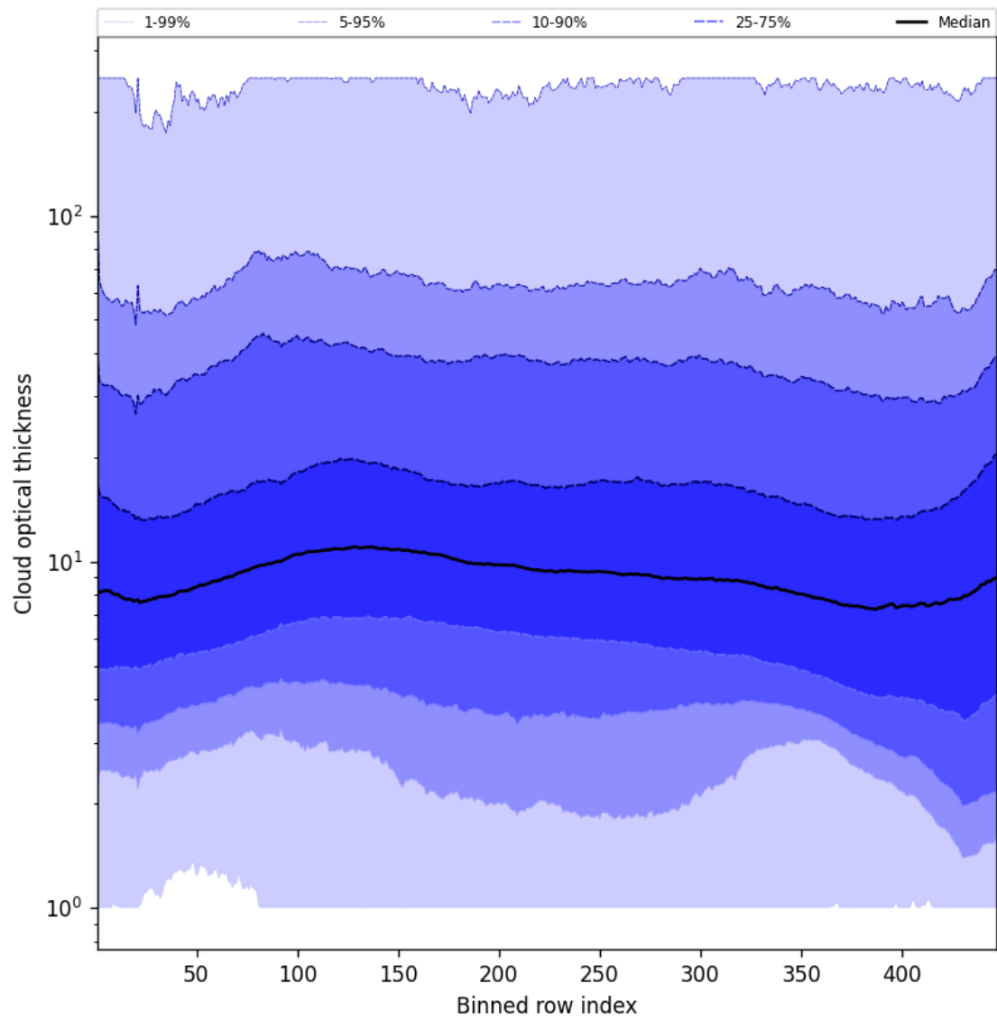
Figure 57: Along track statistics of “Cloud optical thickness” for 2024-11-06 to 2024-11-08
