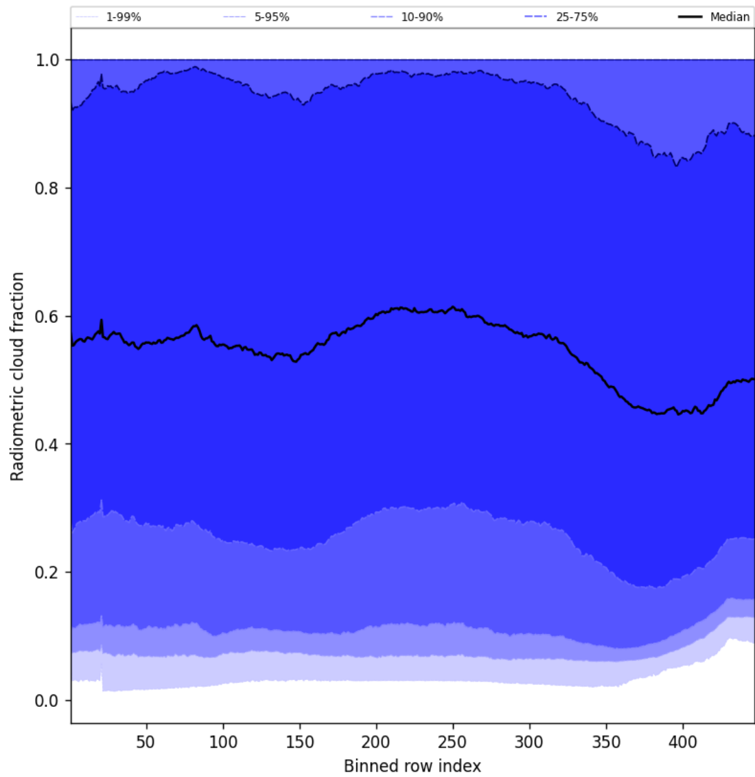
Figure 55: Along track statistics of “Radiometric cloud fraction” for 2024-11-06 to 2024-11-08
