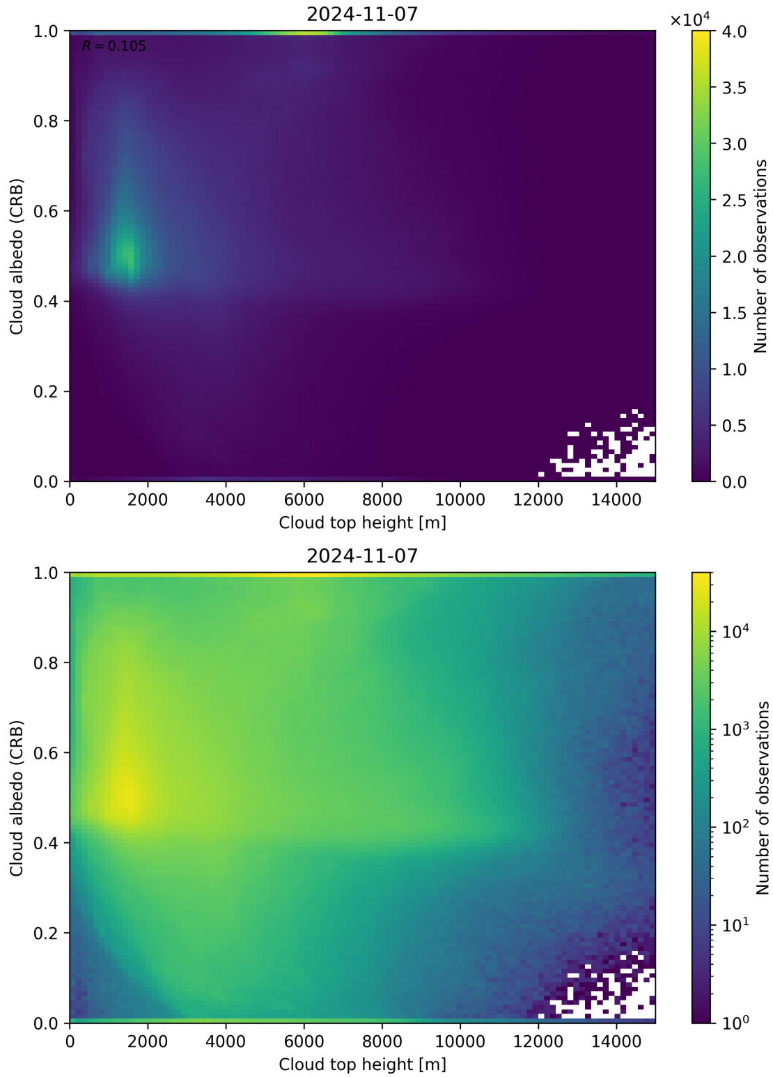
Figure 86: Scatter density plot of “Cloud top height” against “Cloud albedo (CRB)” for 2024-11-06 to 2024-11-08.
