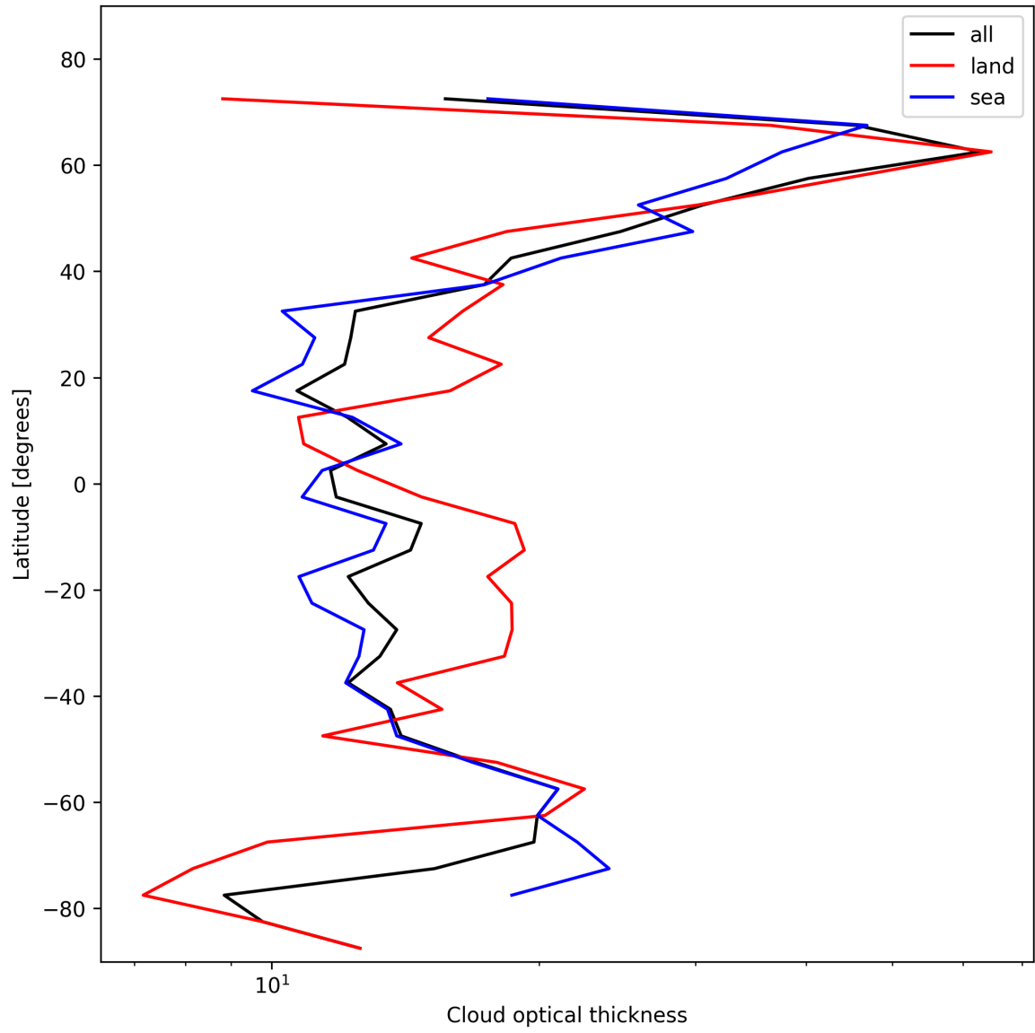
Figure 25: Zonal average of “Cloud optical thickness” for 2024-11-06 to 2024-11-08.
