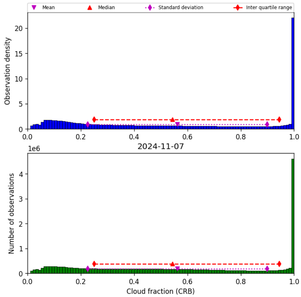
Figure 42: Histogram of “Cloud fraction (CRB)” for 2024-11-06 to 2024-11-08
