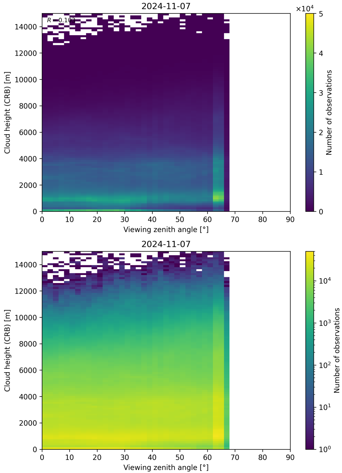
Figure 110: Scatter density plot of “Viewing zenith angle” against “Cloud height (CRB)” for 2024-11-06 to 2024-11-08.
