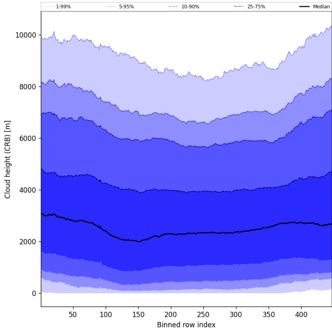
Figure 59: Along track statistics of “Cloud height (CRB)” for 2024-11-06 to 2024-11-08
