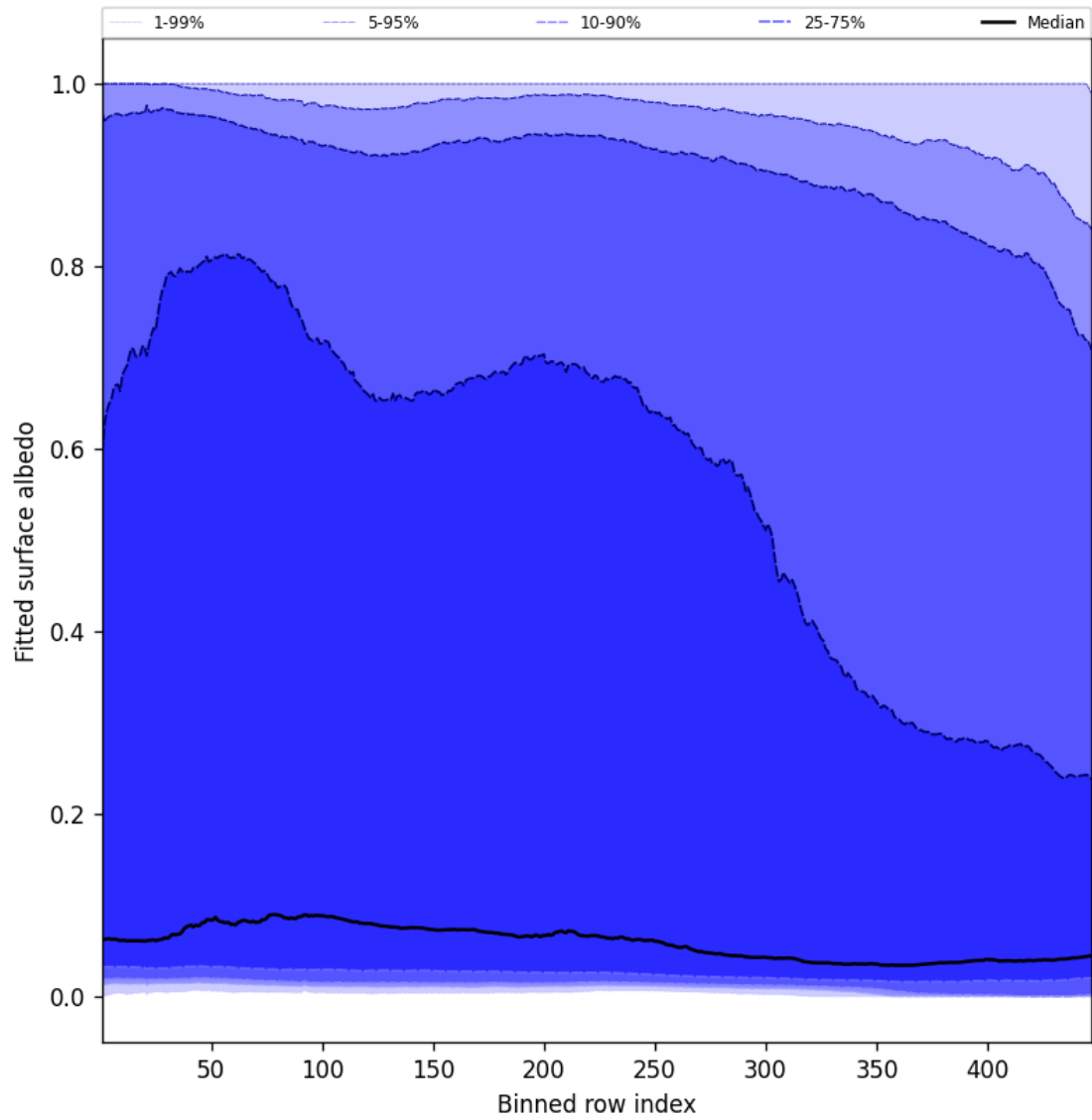
Figure 61: Along track statistics of “Fitted surface albedo” for 2024-11-06 to 2024-11-08
