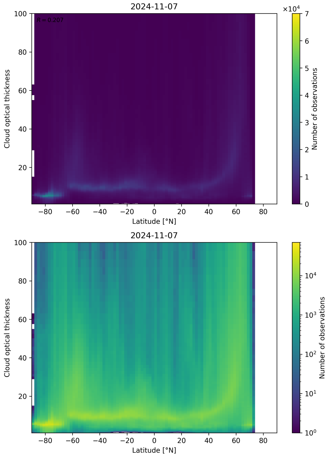
Figure 96: Scatter density plot of “Latitude” against “Cloud optical thickness” for 2024-11-06 to 2024-11-08.
