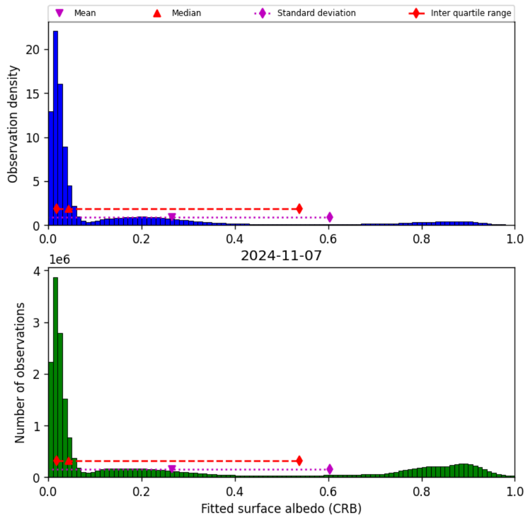
Figure 46: Histogram of “Fitted surface albedo (CRB)” for 2024-11-06 to 2024-11-08
