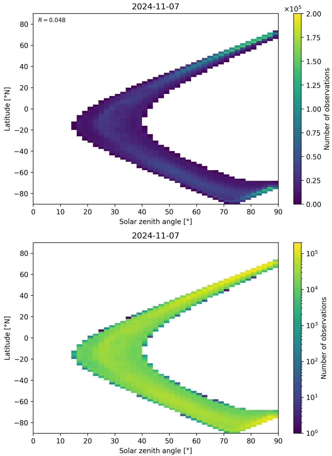
Figure 105: Scatter density plot of “Solar zenith angle” against “Latitude” for 2024-11-06 to 2024-11-08.
