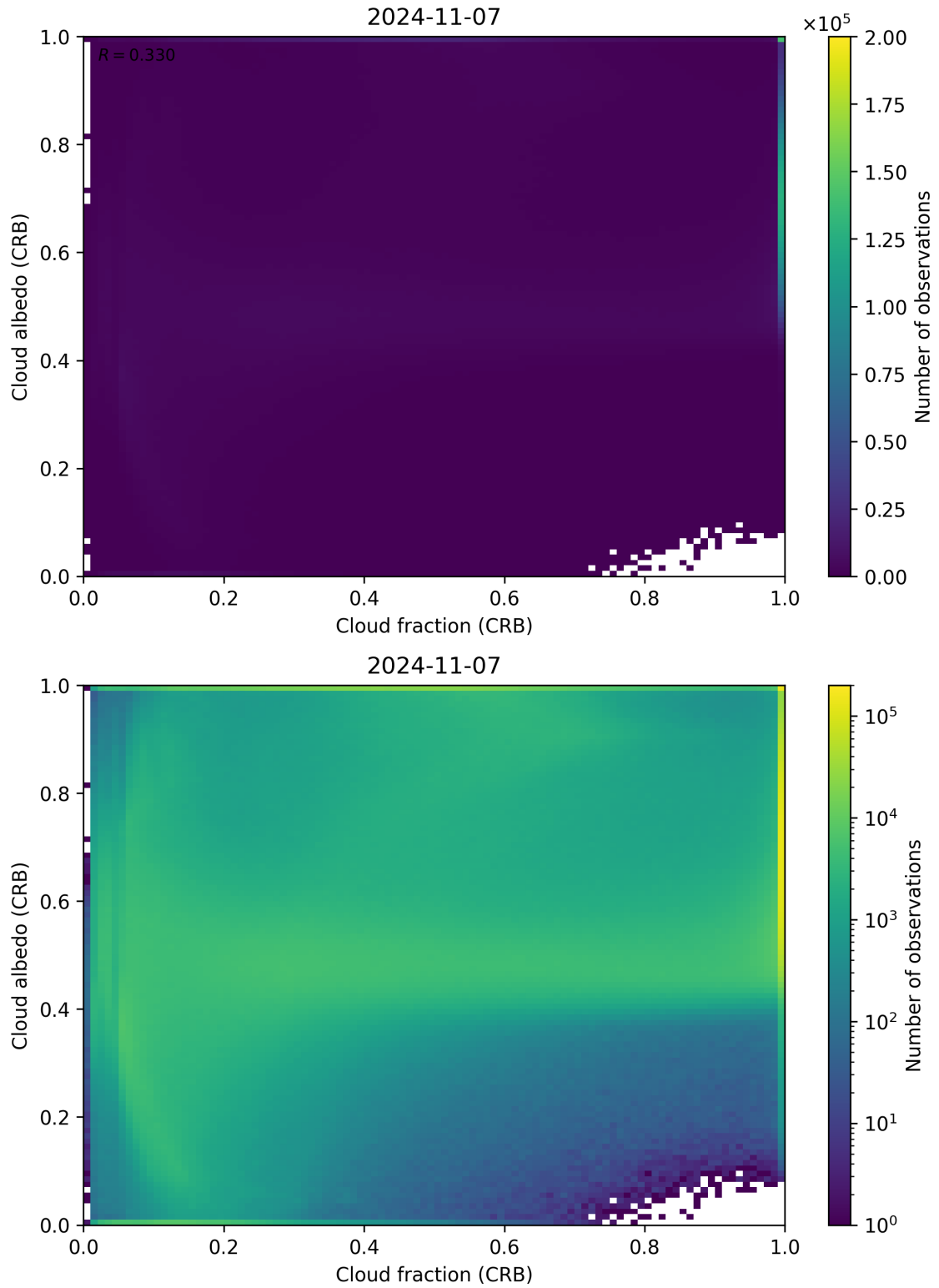
Figure 77: Scatter density plot of “Cloud fraction (CRB)” against “Cloud albedo (CRB)” for 2024-11-06 to 2024-11-08.
