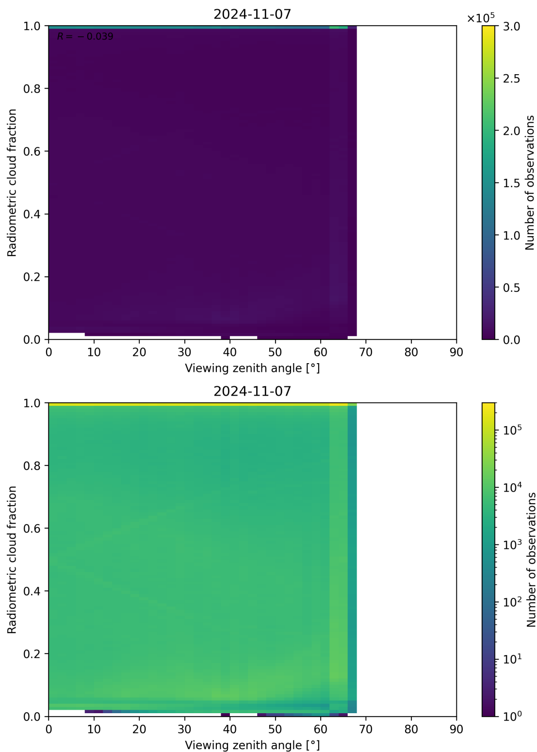
Figure 107: Scatter density plot of “Viewing zenith angle” against “Radiometric cloud fraction” for 2024-11-06 to 2024-11-08.
