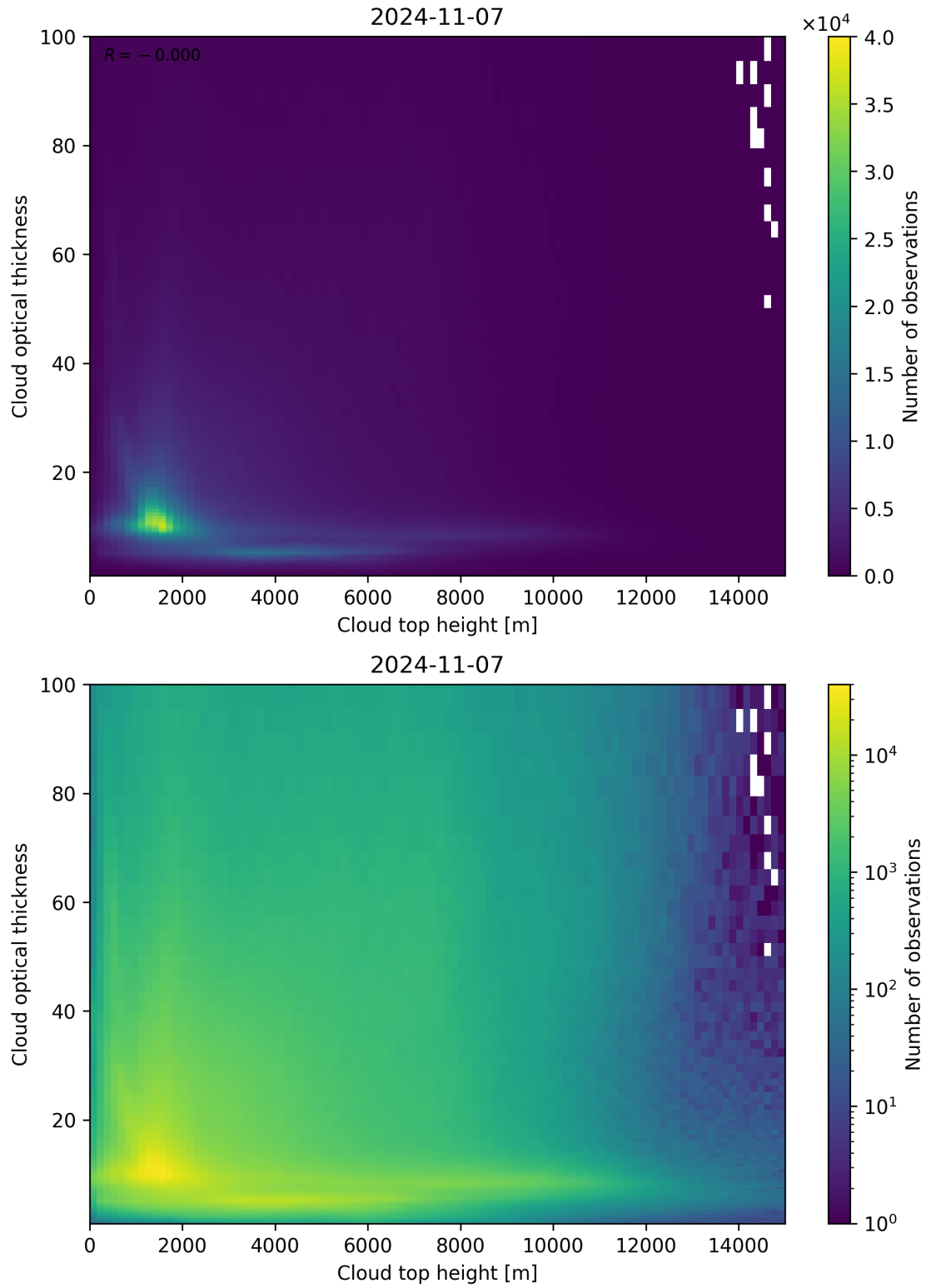
Figure 90: Scatter density plot of “Cloud top height” against “Cloud optical thickness” for 2024-11-06 to 2024-11-08.
