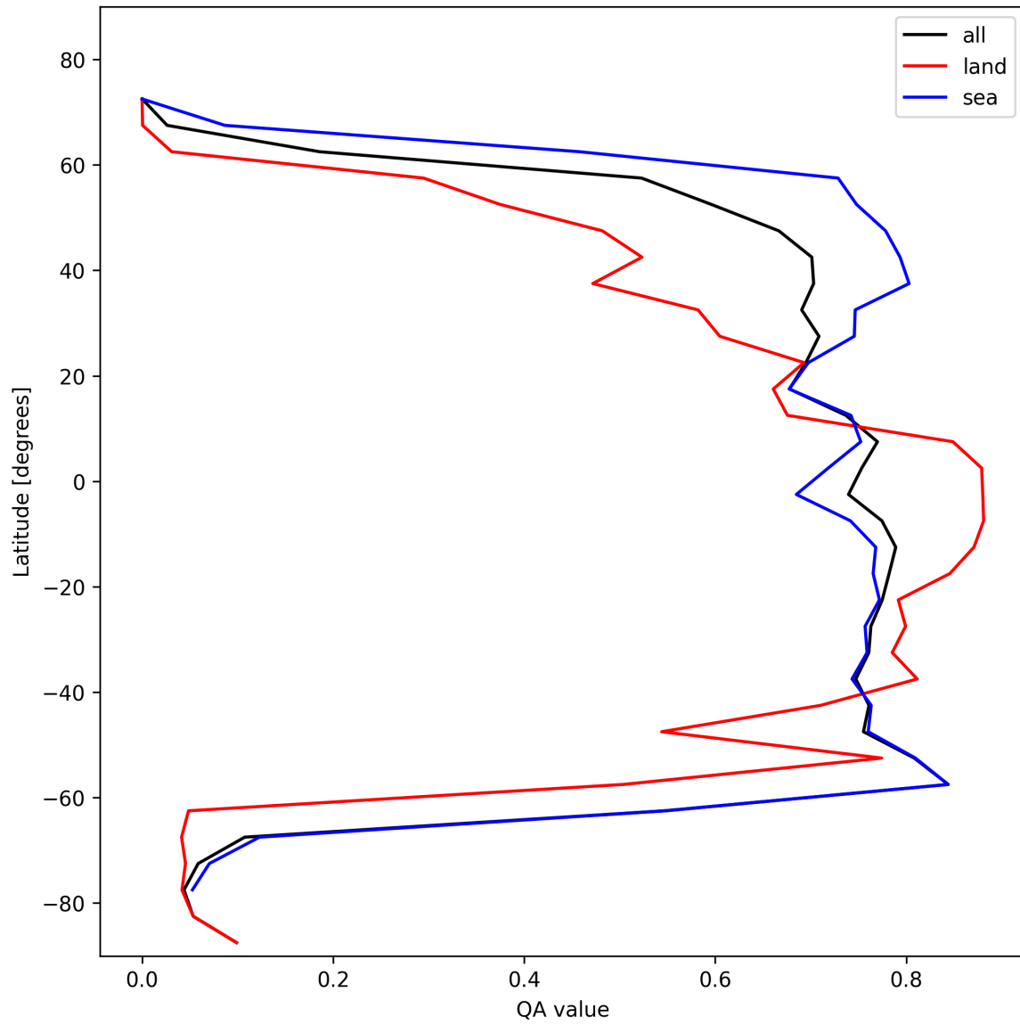
Figure 22: Zonal average of “QA value” for 2024-11-06 to 2024-11-08.
