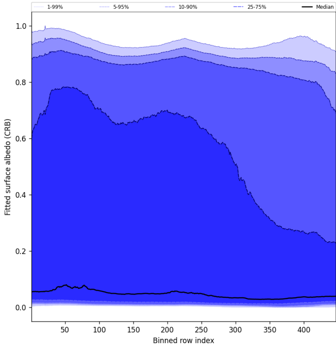
Figure 62: Along track statistics of “Fitted surface albedo (CRB)” for 2024-11-06 to 2024-11-08
