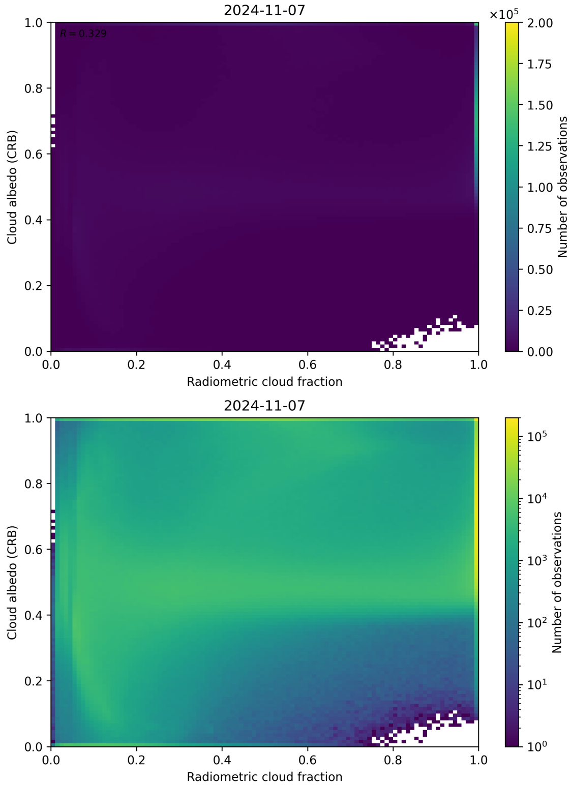
Figure 71: Scatter density plot of “Radiometric cloud fraction” against “Cloud albedo (CRB)” for 2024-11-06 to 2024-11-08.
