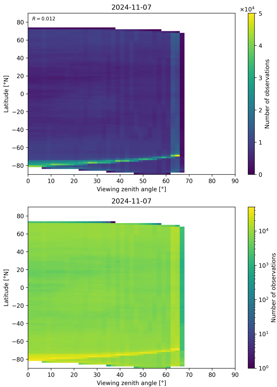
Figure 113: Scatter density plot of “Viewing zenith angle” against “Latitude” for 2024-11-06 to 2024-11-08.
