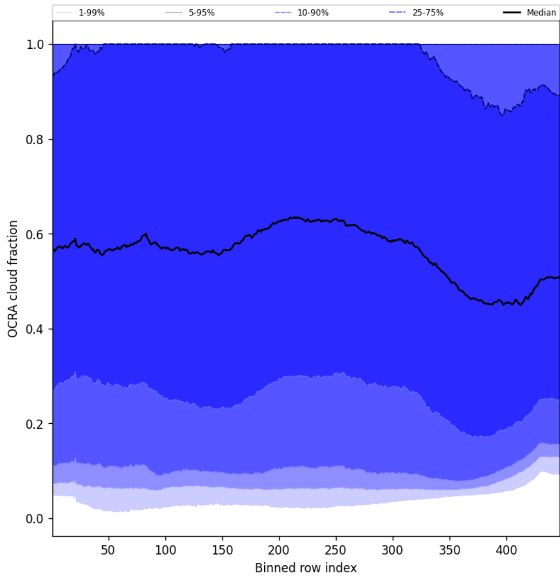
Figure 66: Along track statistics of “OCRA cloud fraction” for 2024-11-06 to 2024-11-08
