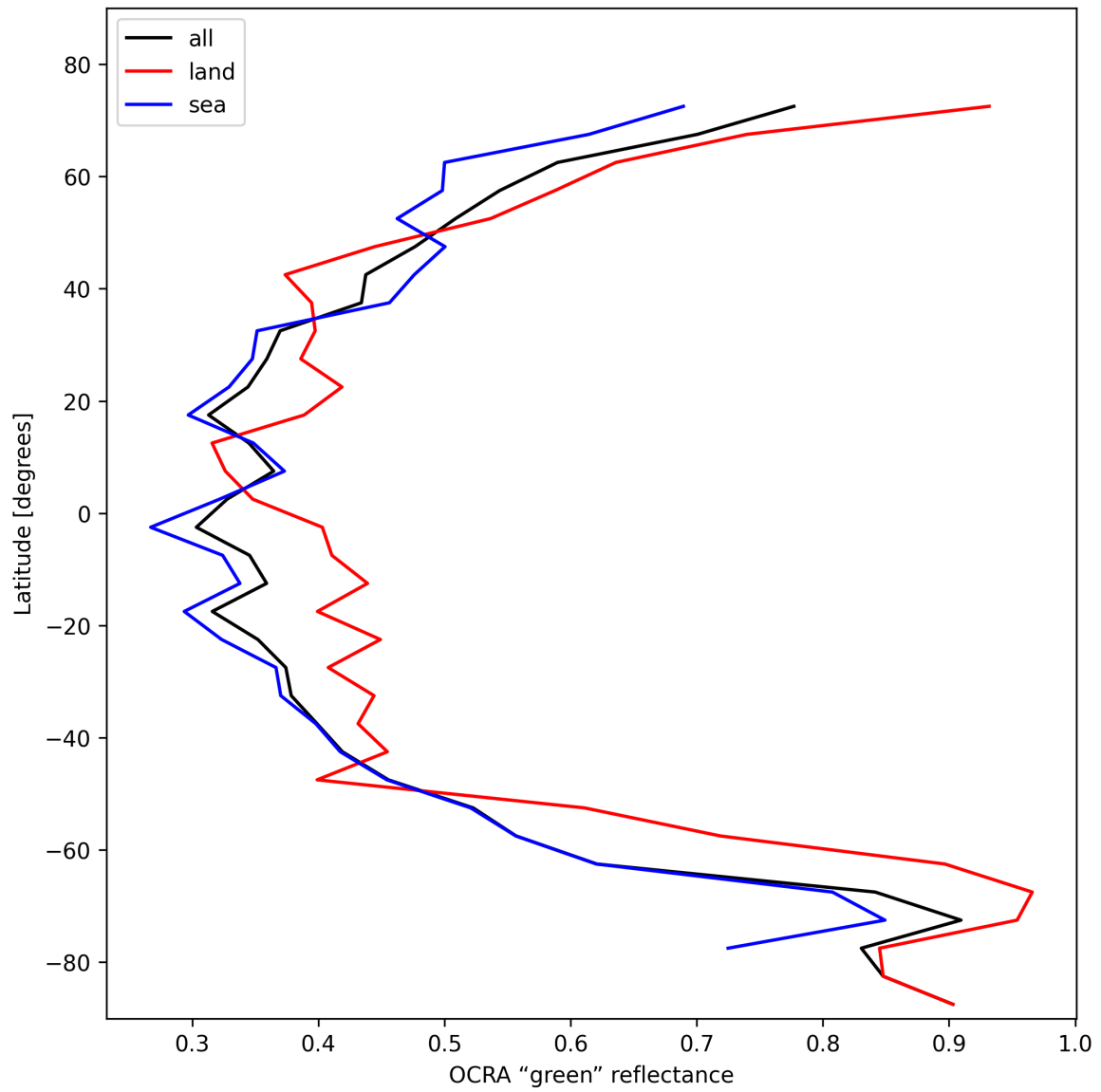
Figure 36: Zonal average of “OCRA “green” reflectance” for 2024-11-06 to 2024-11-08.
