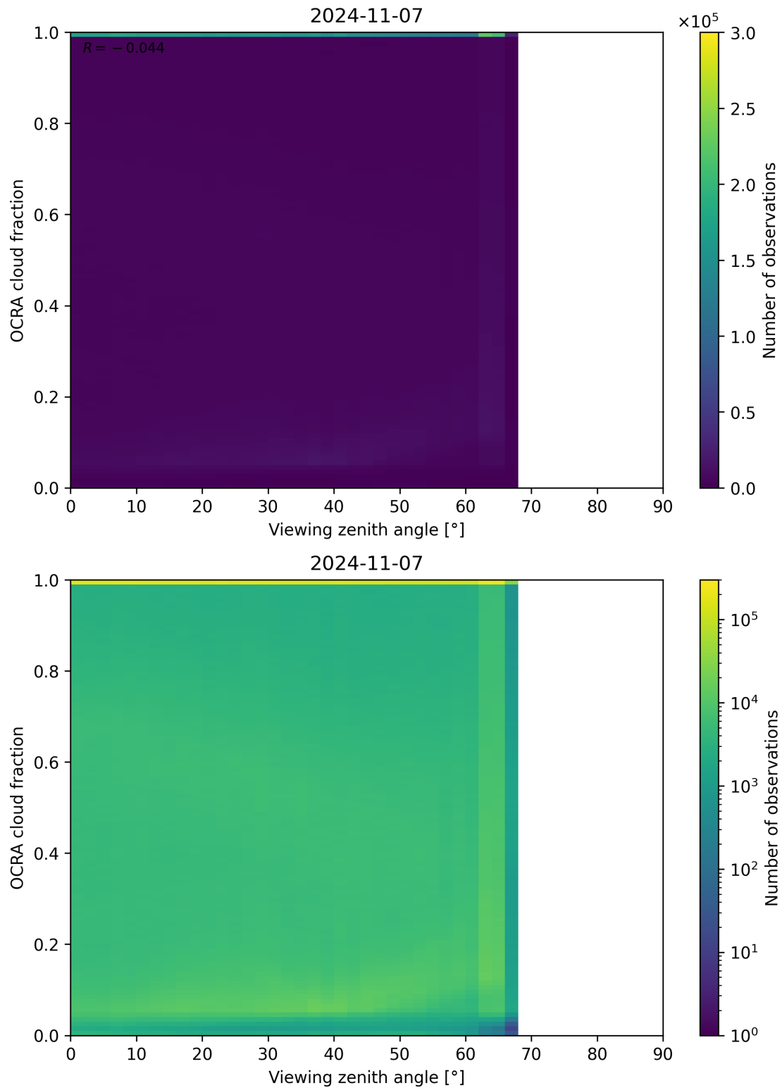
Figure 108: Scatter density plot of “Viewing zenith angle” against “OCRA cloud fraction” for 2024-11-06 to 2024-11-08.
