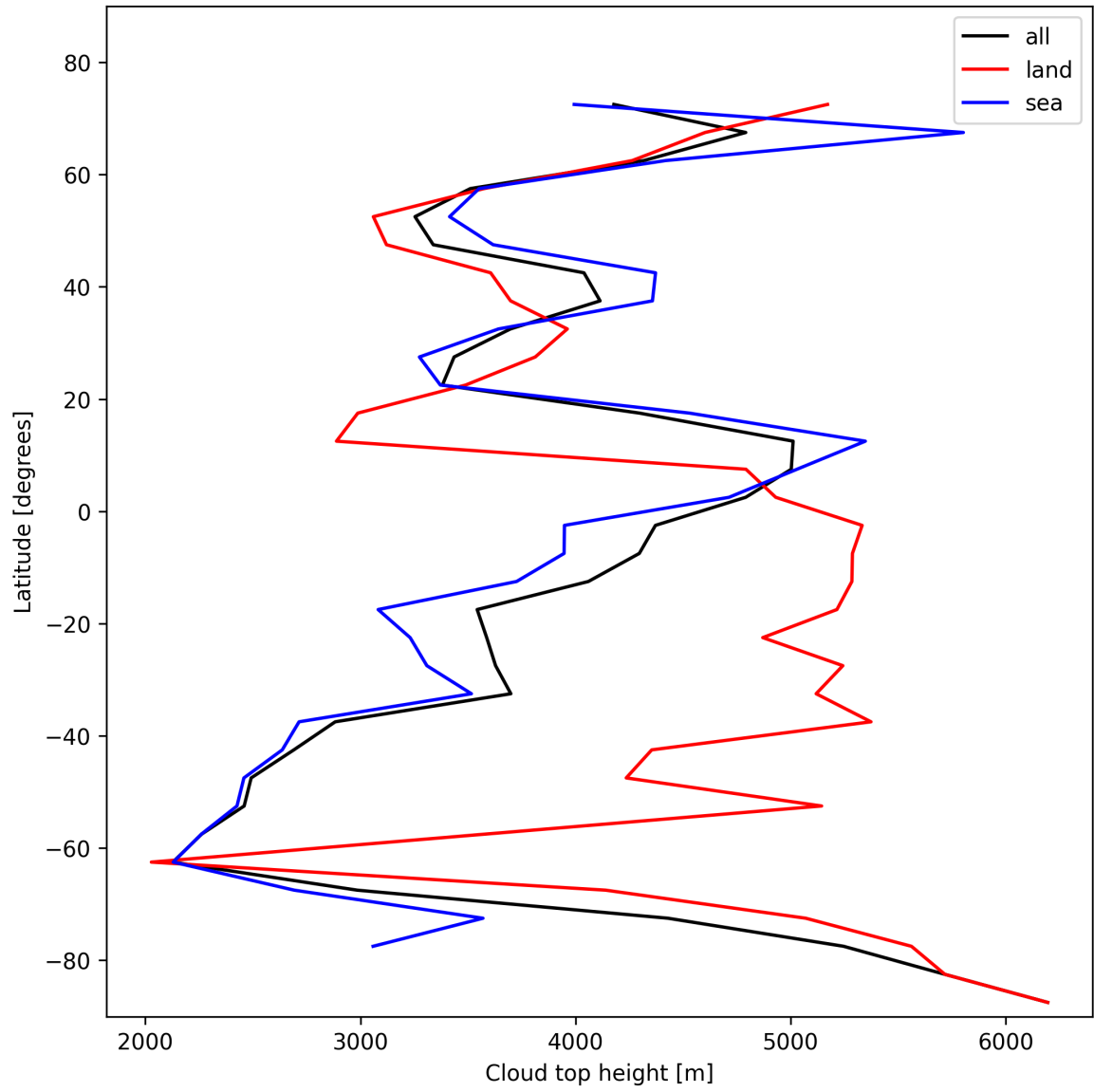
Figure 24: Zonal average of “Cloud top height” for 2024-11-06 to 2024-11-08.
