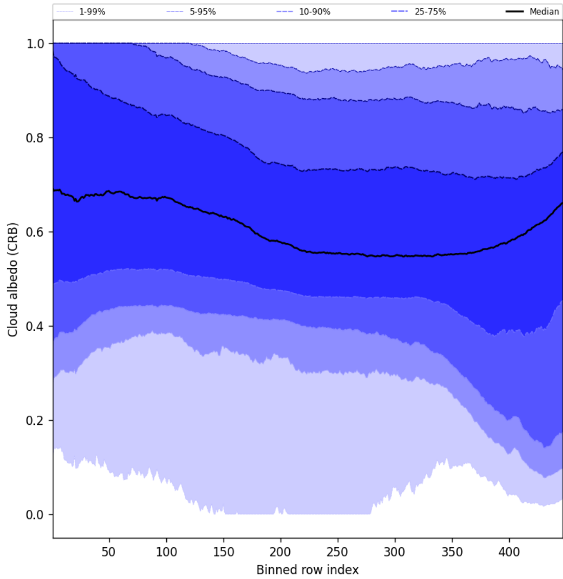
Figure 60: Along track statistics of “Cloud albedo (CRB)” for 2024-11-06 to 2024-11-08
