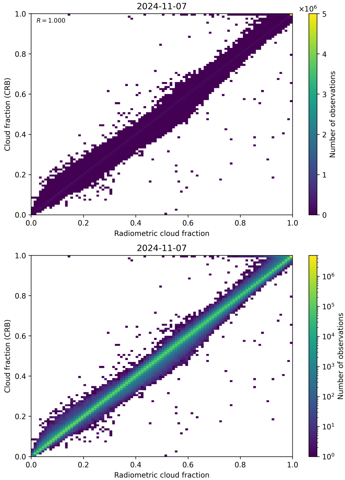
Figure 73: Scatter density plot of “Radiometric cloud fraction” against “Cloud fraction (CRB)” for 2024-11-06 to 2024-11-08.
