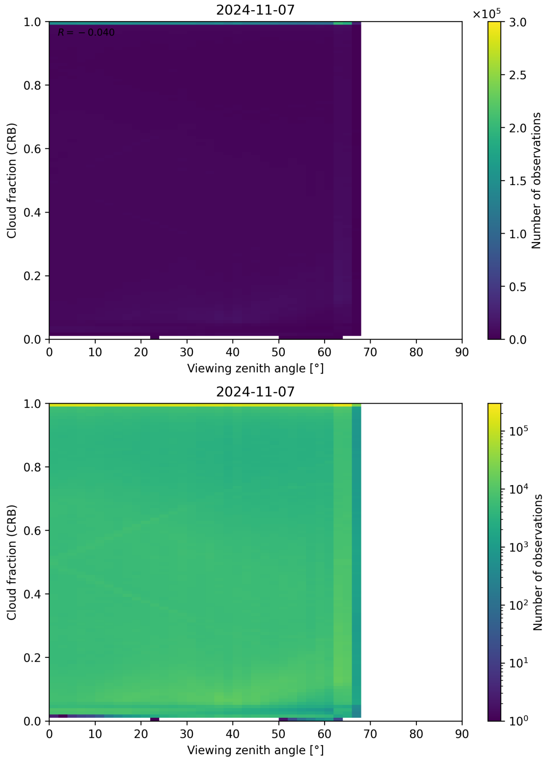
Figure 109: Scatter density plot of “Viewing zenith angle” against “Cloud fraction (CRB)” for 2024-11-06 to 2024-11-08.
