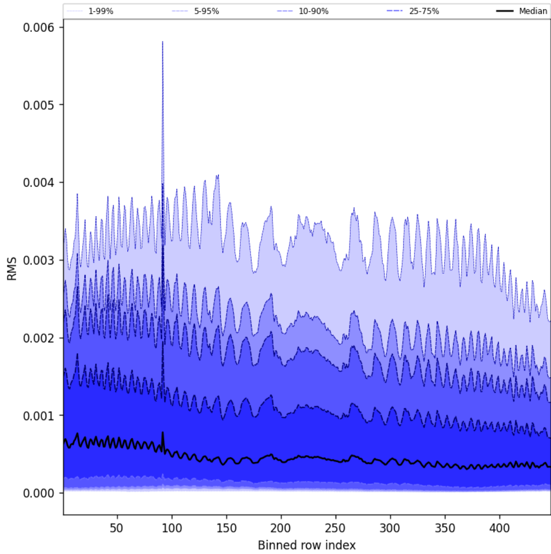
Figure 63: Along track statistics of “RMS” for 2024-11-06 to 2024-11-08
