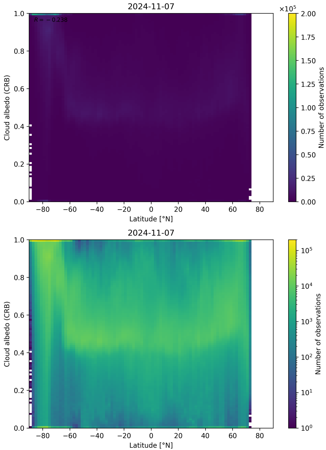
Figure 91: Scatter density plot of “Latitude” against “Cloud albedo (CRB)” for 2024-11-06 to 2024-11-08.
