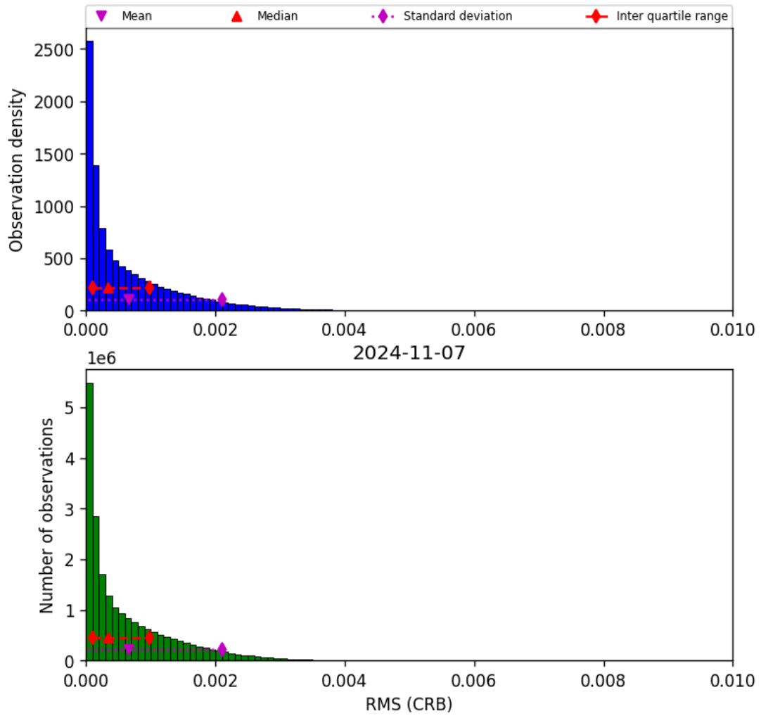
Figure 48: Histogram of “RMS (CRB)” for 2024-11-06 to 2024-11-08
