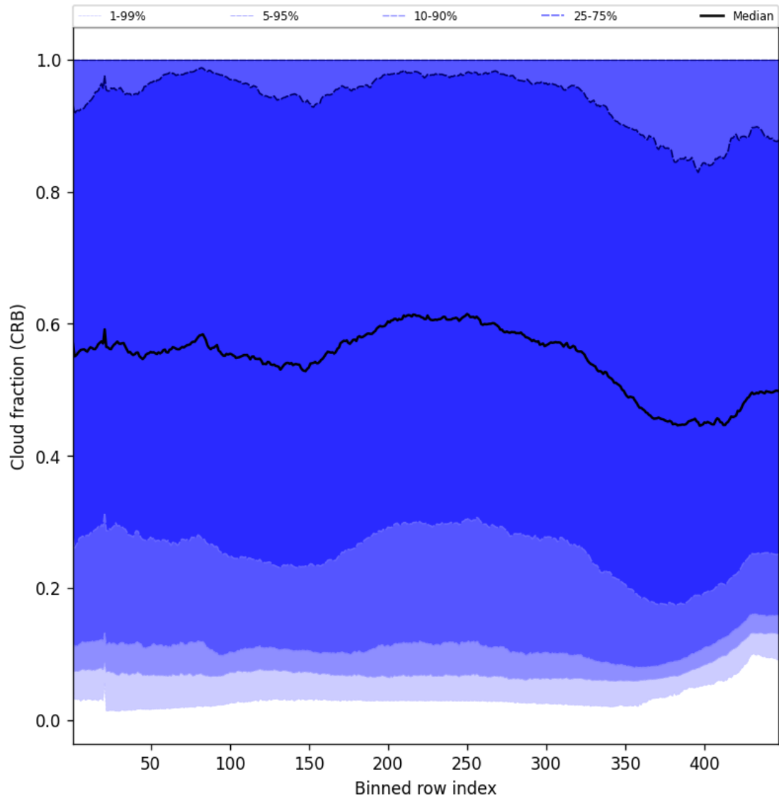
Figure 58: Along track statistics of “Cloud fraction (CRB)” for 2024-11-06 to 2024-11-08
