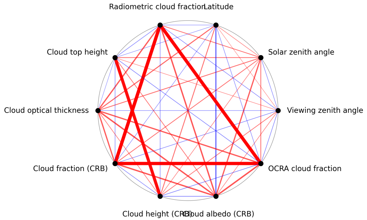
Figure 1: Map of correlation graph for 2024-11-06 to 2024-11-08.
