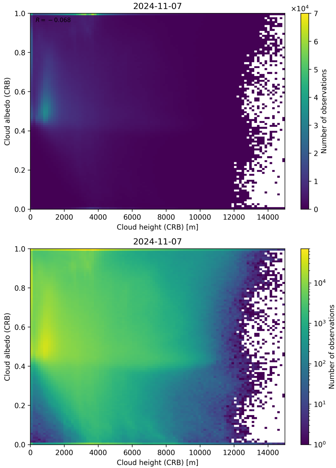
Figure 80: Scatter density plot of “Cloud height (CRB)” against “Cloud albedo (CRB)” for 2024-11-06 to 2024-11-08.
