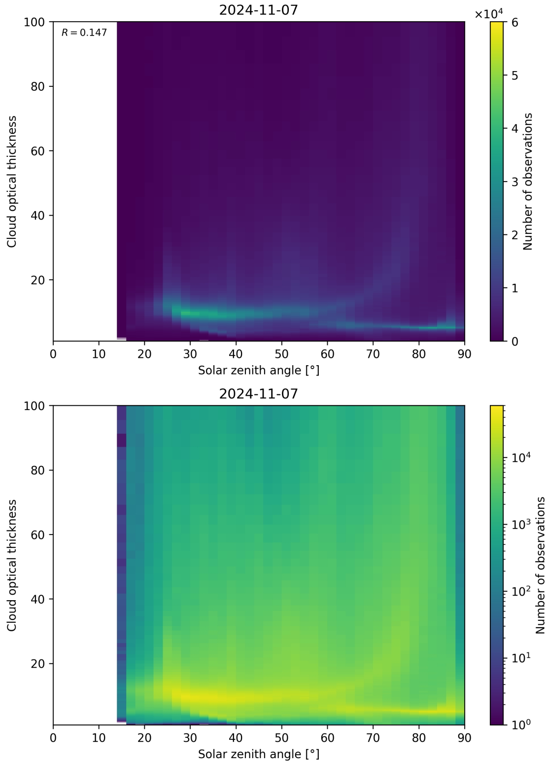
Figure 103: Scatter density plot of “Solar zenith angle” against “Cloud optical thickness” for 2024-11-06 to 2024-11-08.
