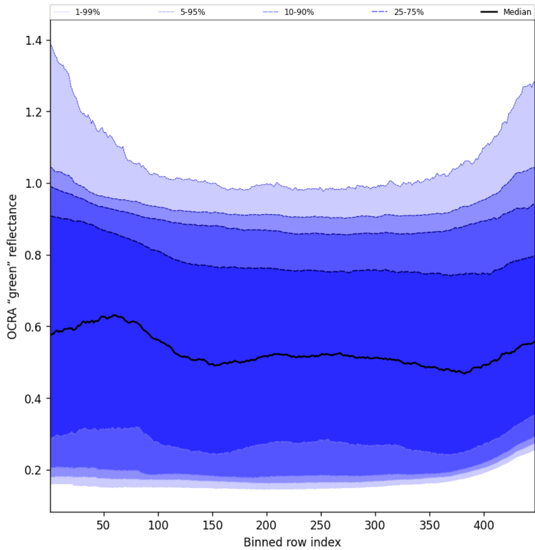
Figure 68: Along track statistics of “OCRA “green” reflectance” for 2024-11-06 to 2024-11-08
