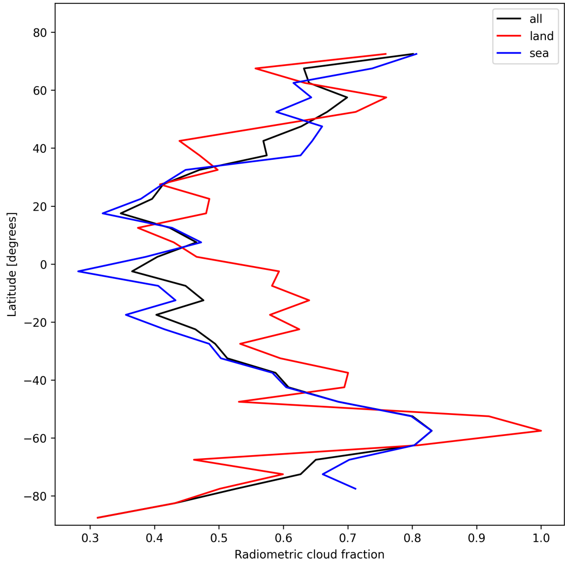
Figure 23: Zonal average of “Radiometric cloud fraction” for 2024-11-06 to 2024-11-08.
