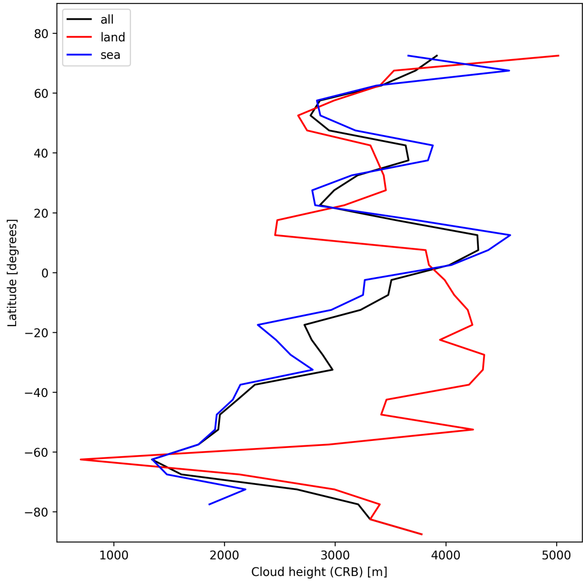
Figure 27: Zonal average of “Cloud height (CRB)” for 2024-11-06 to 2024-11-08.
