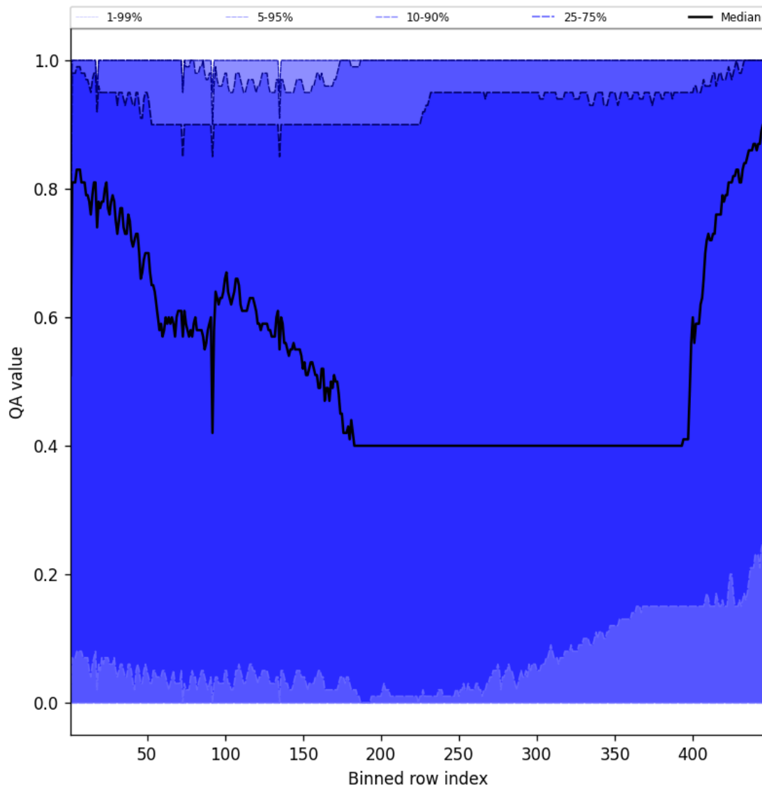
Figure 54: Along track statistics of “QA value” for 2024-11-06 to 2024-11-08
