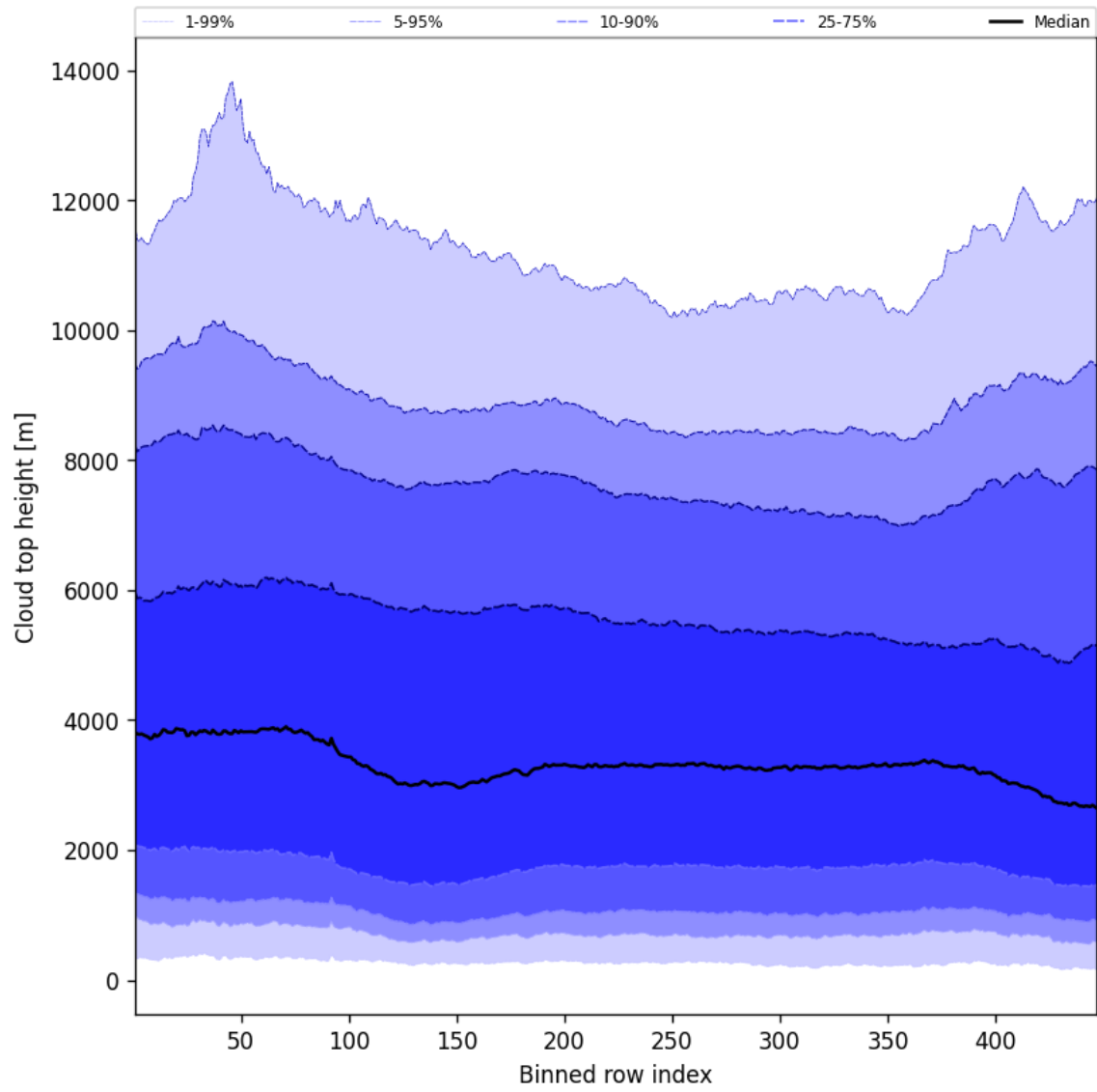
Figure 56: Along track statistics of “Cloud top height” for 2024-11-06 to 2024-11-08
