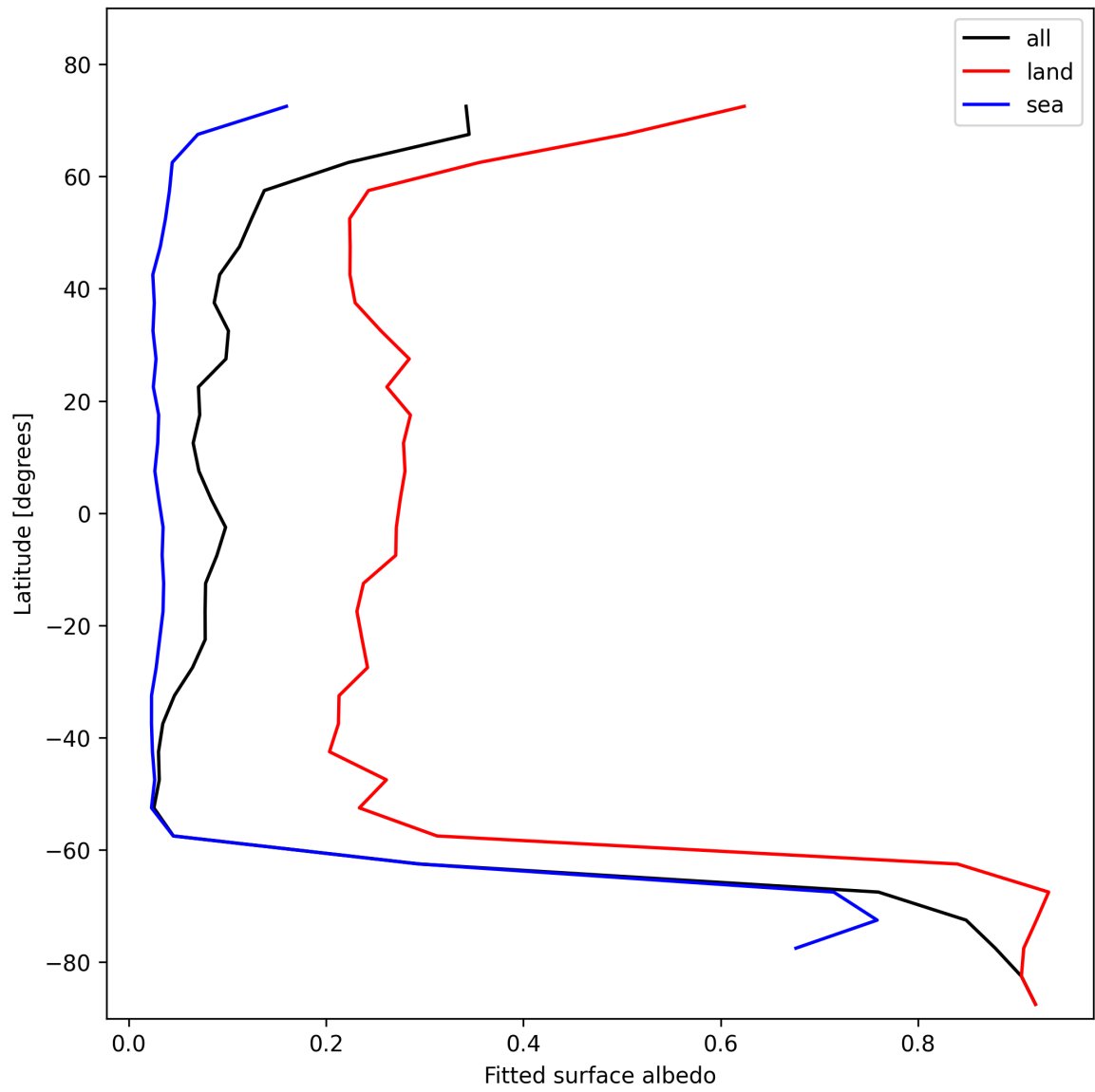
Figure 29: Zonal average of “Fitted surface albedo” for 2024-11-06 to 2024-11-08.
