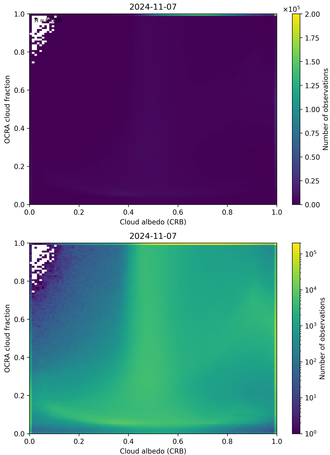
Figure 70: Scatter density plot of “Cloud albedo (CRB)” against “OCRA cloud fraction” for 2024-11-06 to 2024-11-08.
