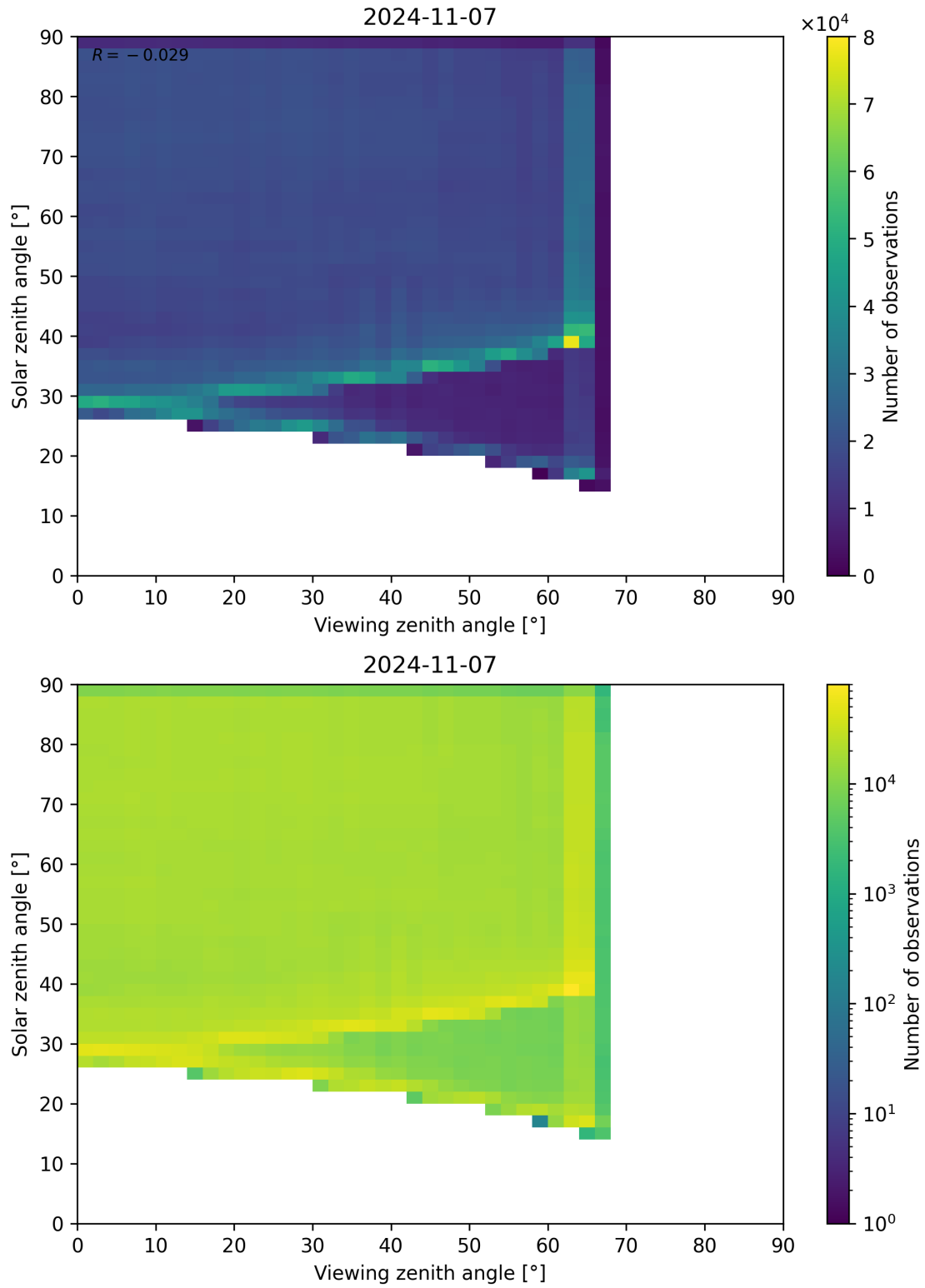
Figure 114: Scatter density plot of “Viewing zenith angle” against “Solar zenith angle” for 2024-11-06 to 2024-11-08.
