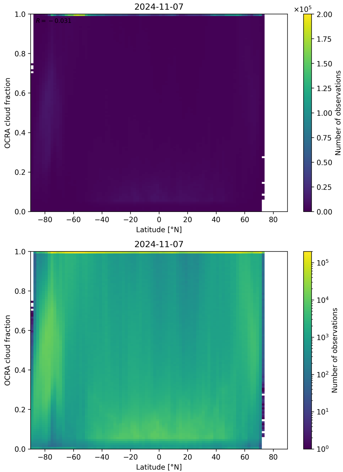
Figure 93: Scatter density plot of “Latitude” against “OCRA cloud fraction” for 2024-11-06 to 2024-11-08.
