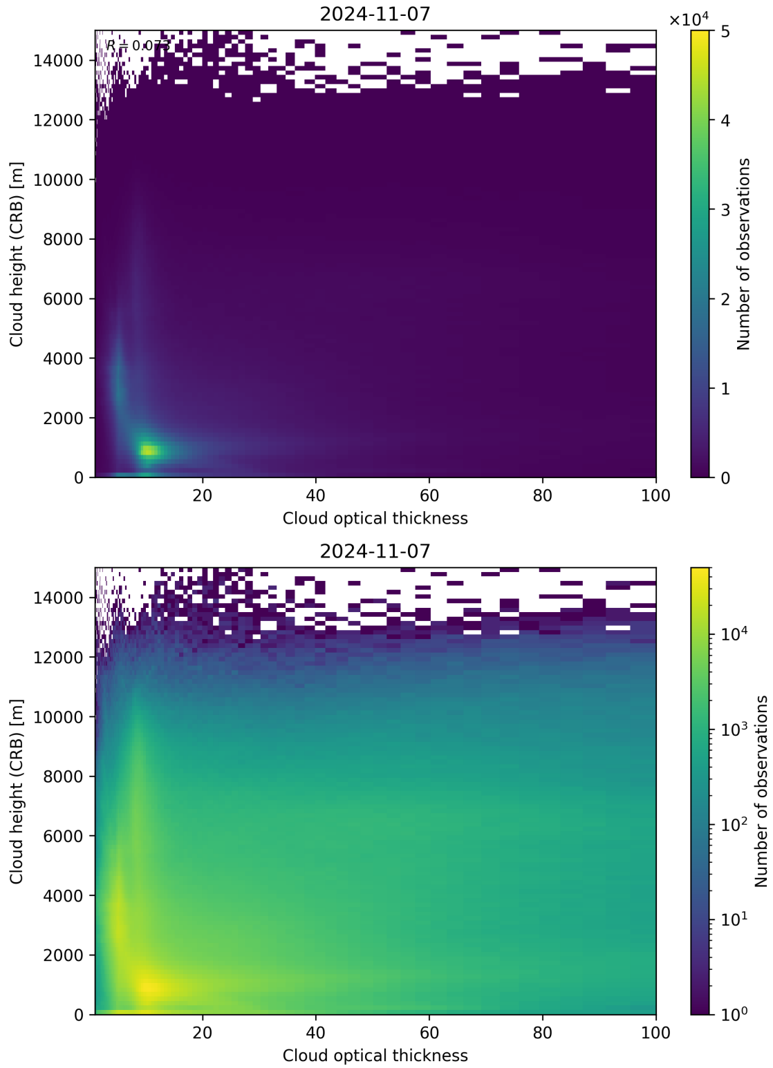
Figure 85: Scatter density plot of “Cloud optical thickness” against “Cloud height (CRB)” for 2024-11-06 to 2024-11-08.
