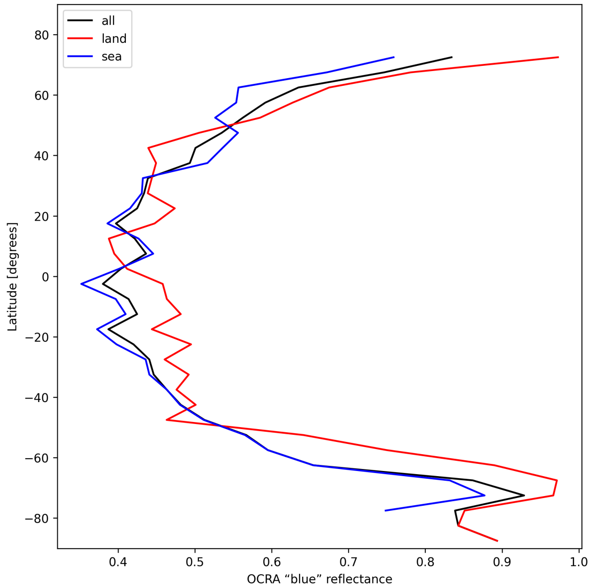
Figure 35: Zonal average of “OCRA “blue” reflectance” for 2024-11-06 to 2024-11-08.
