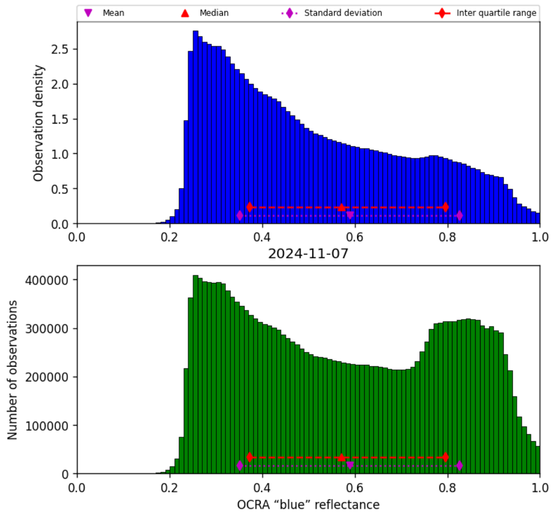
Figure 51: Histogram of “OCRA “blue” reflectance” for 2024-11-06 to 2024-11-08
