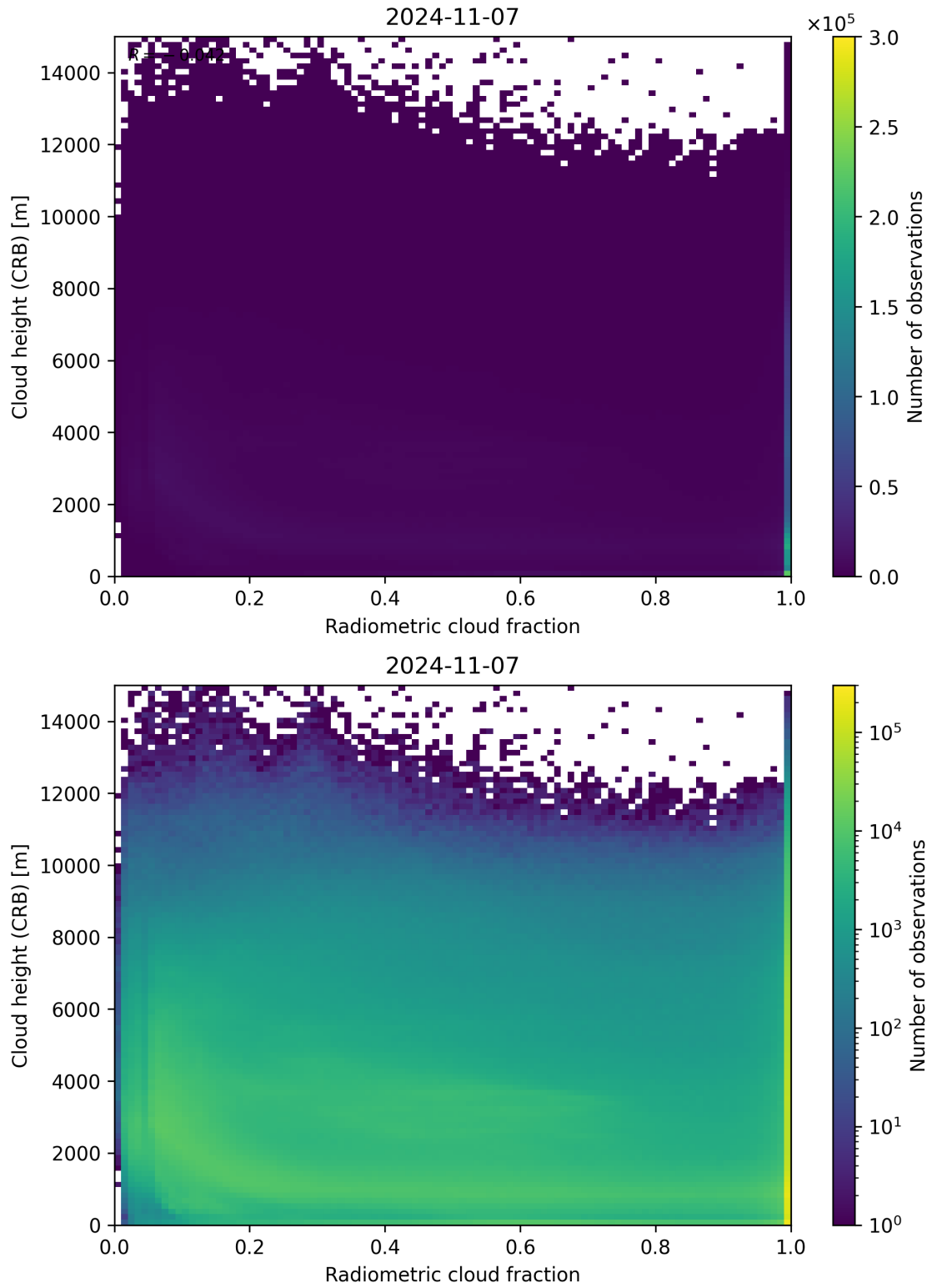
Figure 74: Scatter density plot of “Radiometric cloud fraction” against “Cloud height (CRB)” for 2024-11-06 to 2024-11-08.
