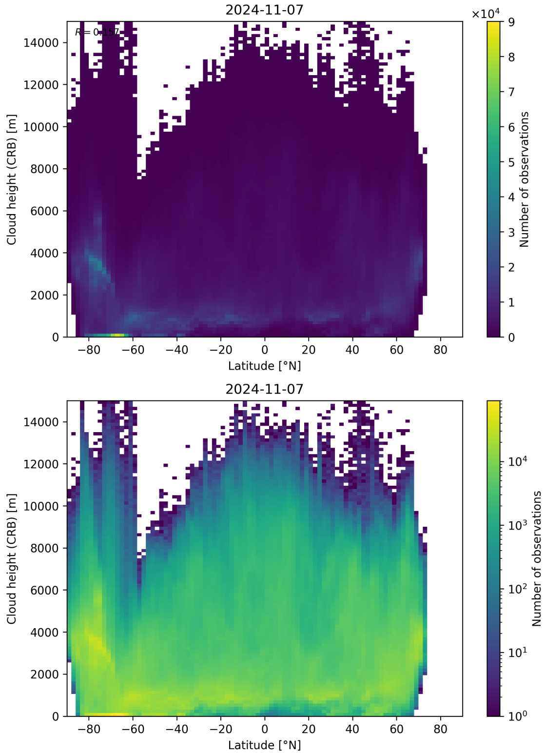
Figure 95: Scatter density plot of “Latitude” against “Cloud height (CRB)” for 2024-11-06 to 2024-11-08.
