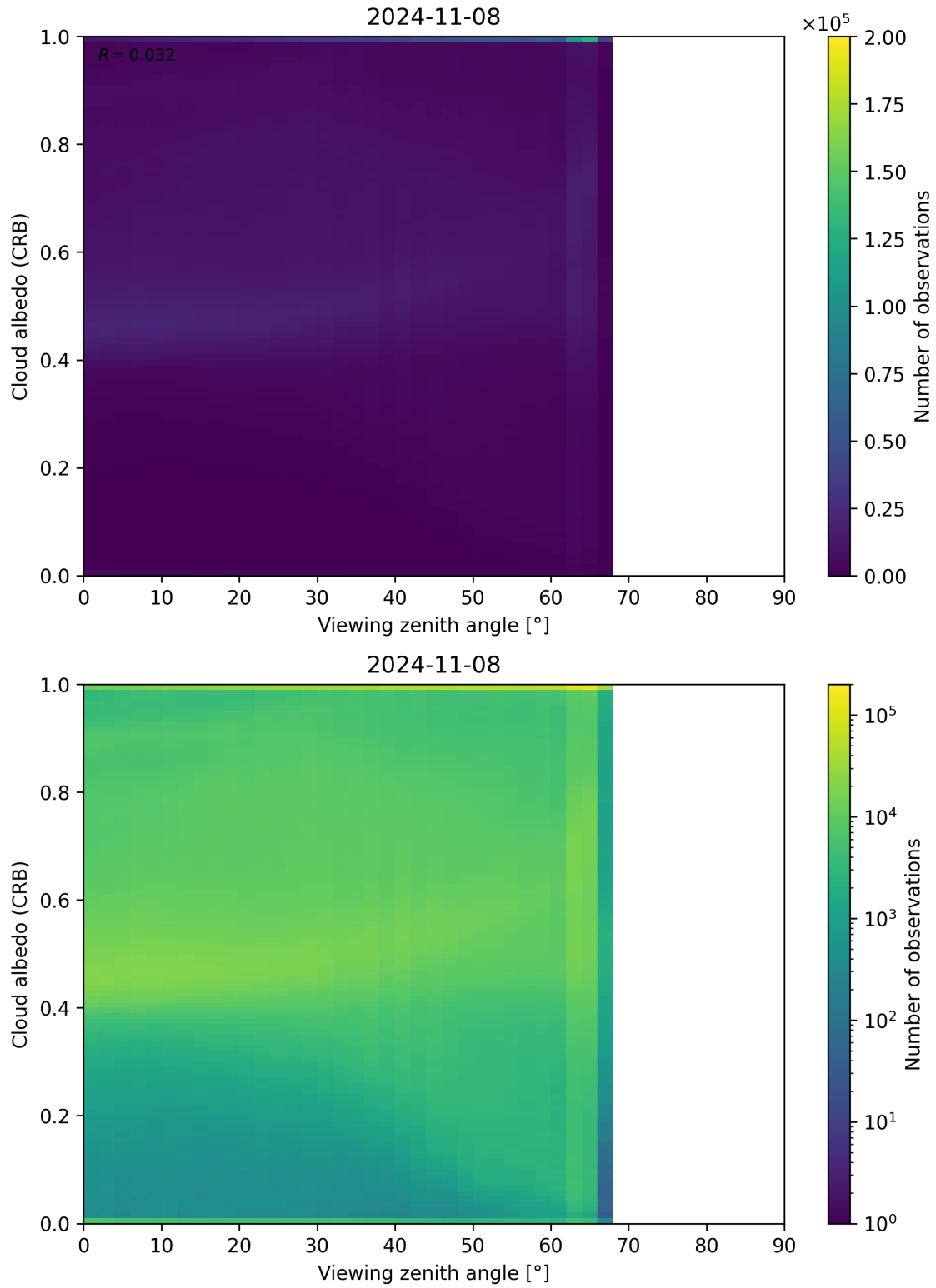
Figure 106: Scatter density plot of “Viewing zenith angle” against “Cloud albedo (CRB)” for 2024-11-07 to 2024-11-09.
