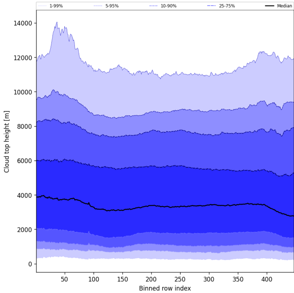
Figure 56: Along track statistics of “Cloud top height” for 2024-11-07 to 2024-11-09
