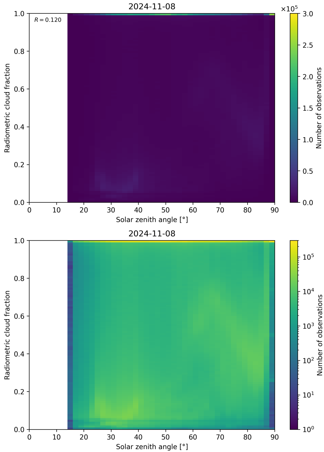
Figure 99: Scatter density plot of “Solar zenith angle” against “Radiometric cloud fraction” for 2024-11-07 to 2024-11-09.
