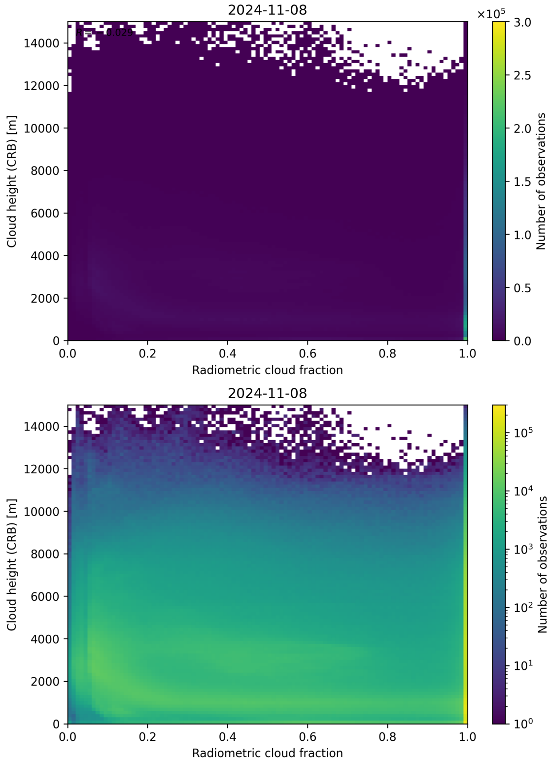
Figure 74: Scatter density plot of “Radiometric cloud fraction” against “Cloud height (CRB)” for 2024-11-07 to 2024-11-09.
