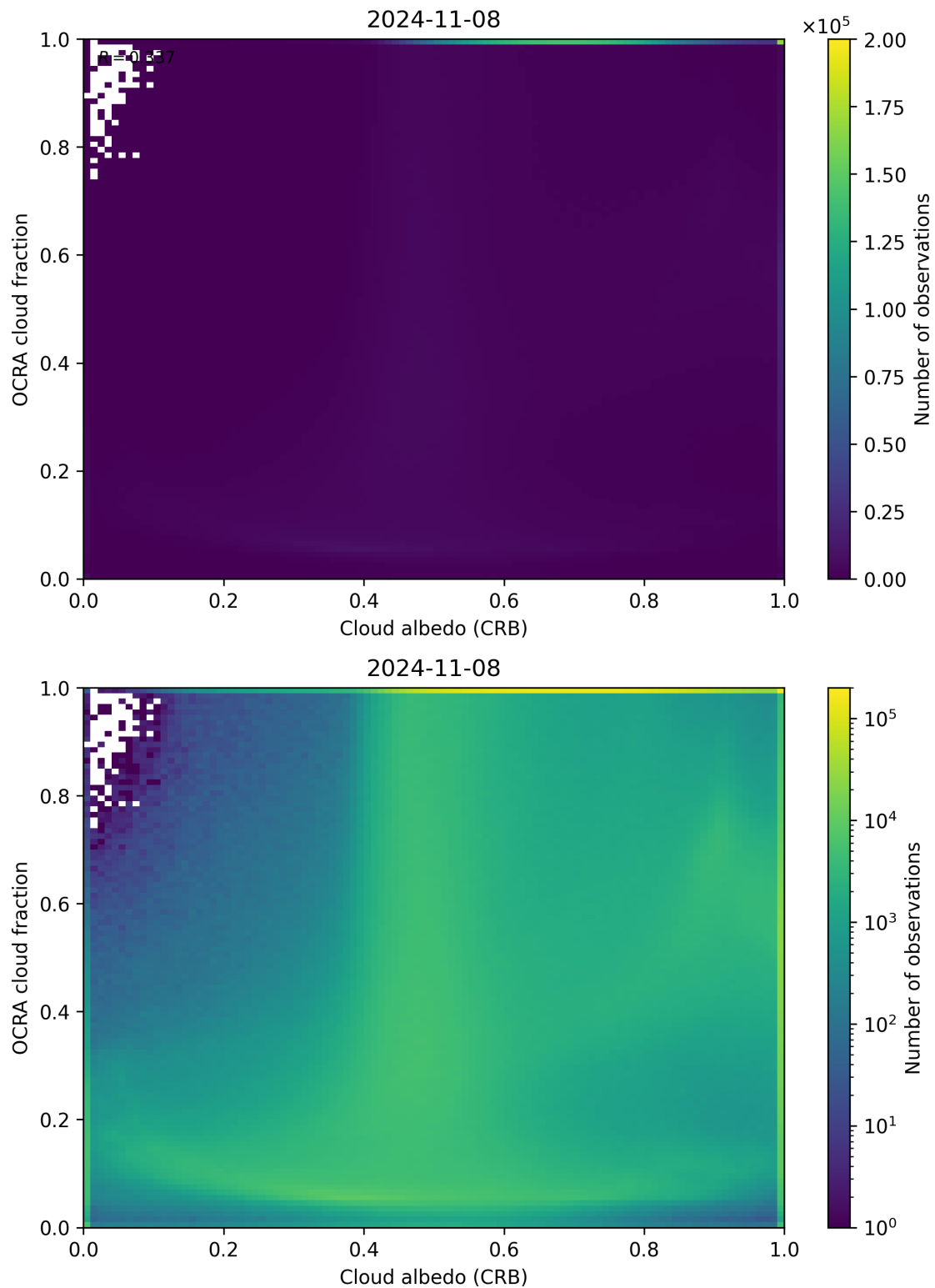
Figure 70: Scatter density plot of “Cloud albedo (CRB)” against “OCRA cloud fraction” for 2024-11-07 to 2024-11-09.
