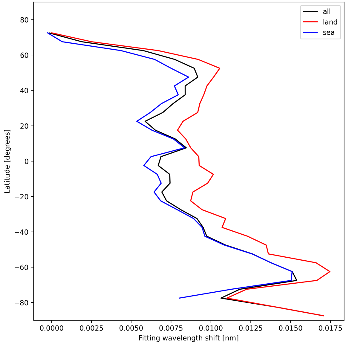
Figure 33: Zonal average of “Fitting wavelength shift” for 2024-11-07 to 2024-11-09.
