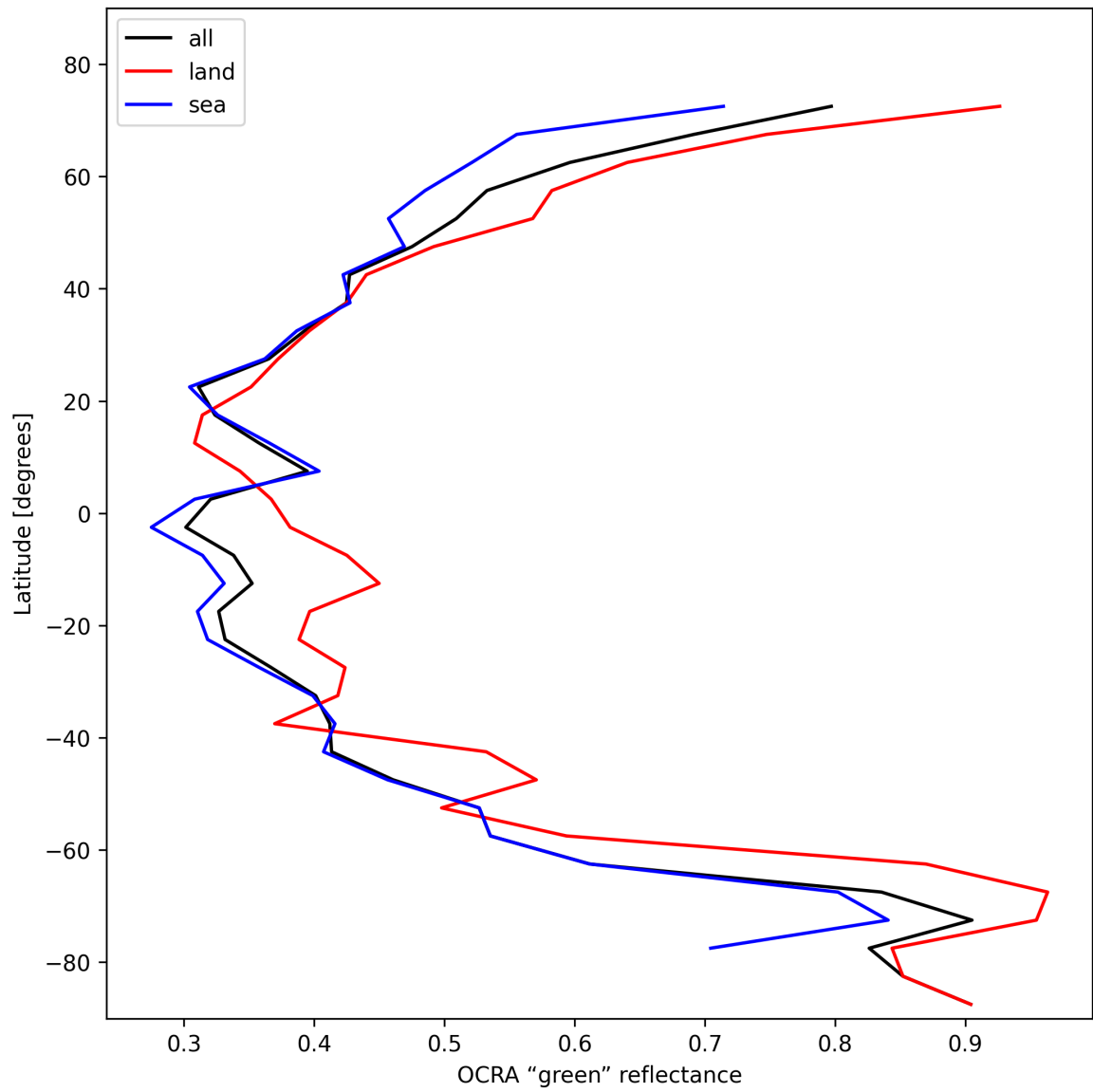
Figure 36: Zonal average of “OCRA “green” reflectance” for 2024-11-07 to 2024-11-09.
