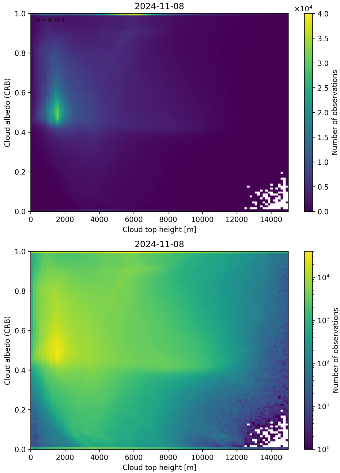
Figure 86: Scatter density plot of “Cloud top height” against “Cloud albedo (CRB)” for 2024-11-07 to 2024-11-09.
