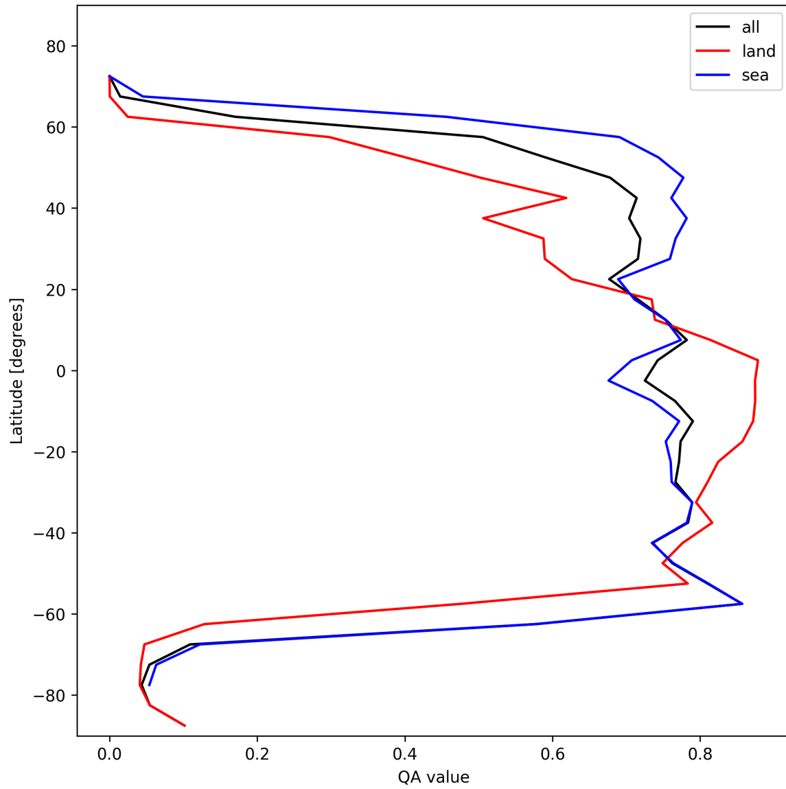
Figure 22: Zonal average of “QA value” for 2024-11-07 to 2024-11-09.
