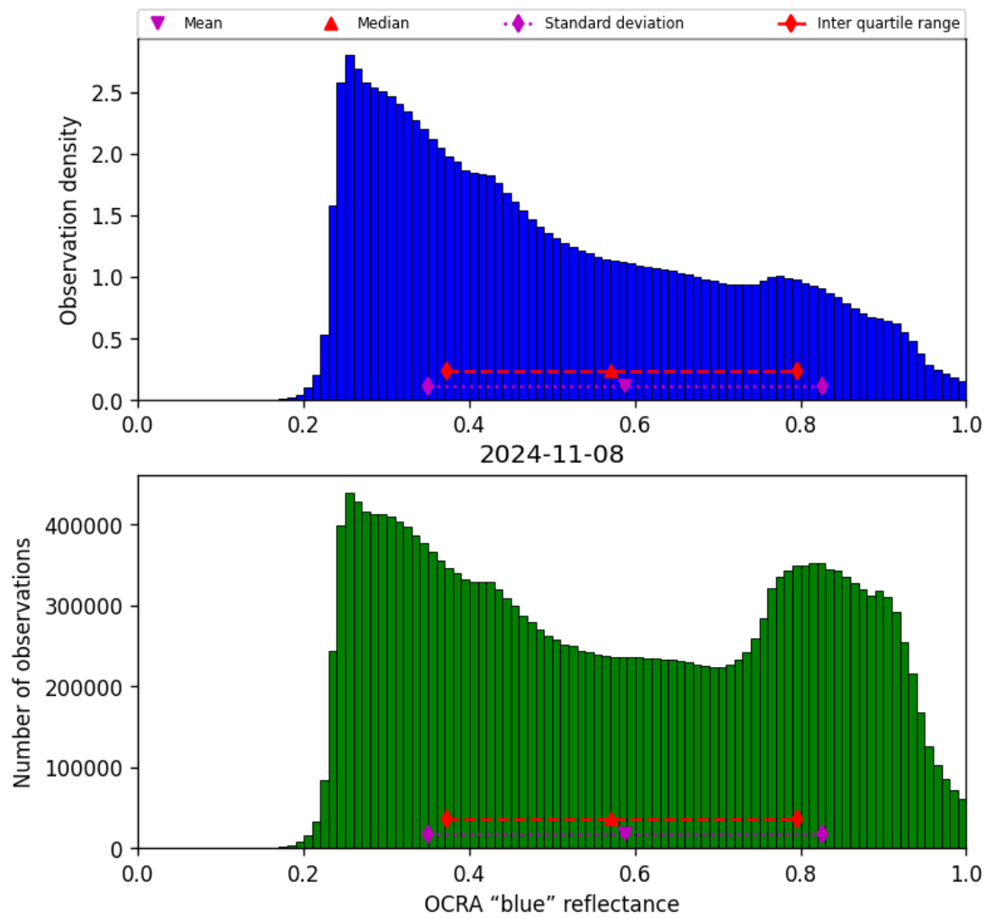
Figure 51: Histogram of “OCRA “blue” reflectance” for 2024-11-07 to 2024-11-09
