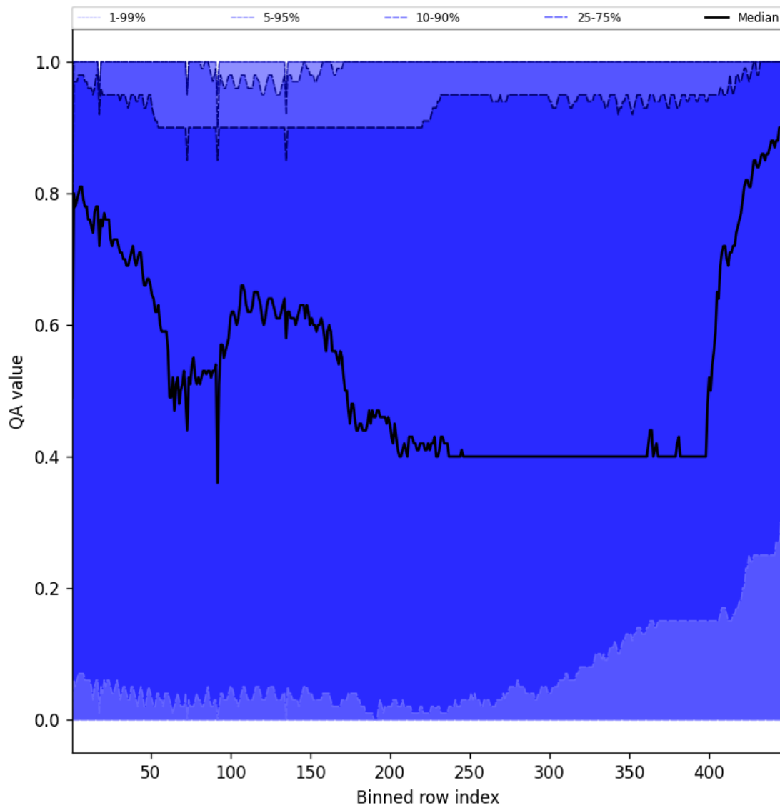
Figure 54: Along track statistics of “QA value” for 2024-11-07 to 2024-11-09
