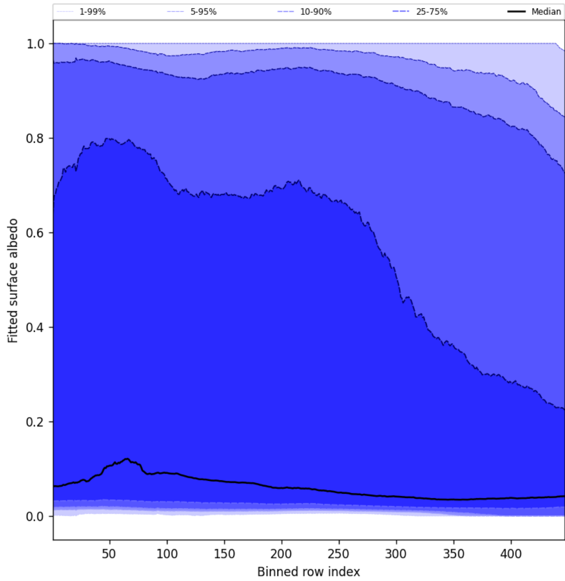
Figure 61: Along track statistics of “Fitted surface albedo” for 2024-11-07 to 2024-11-09
