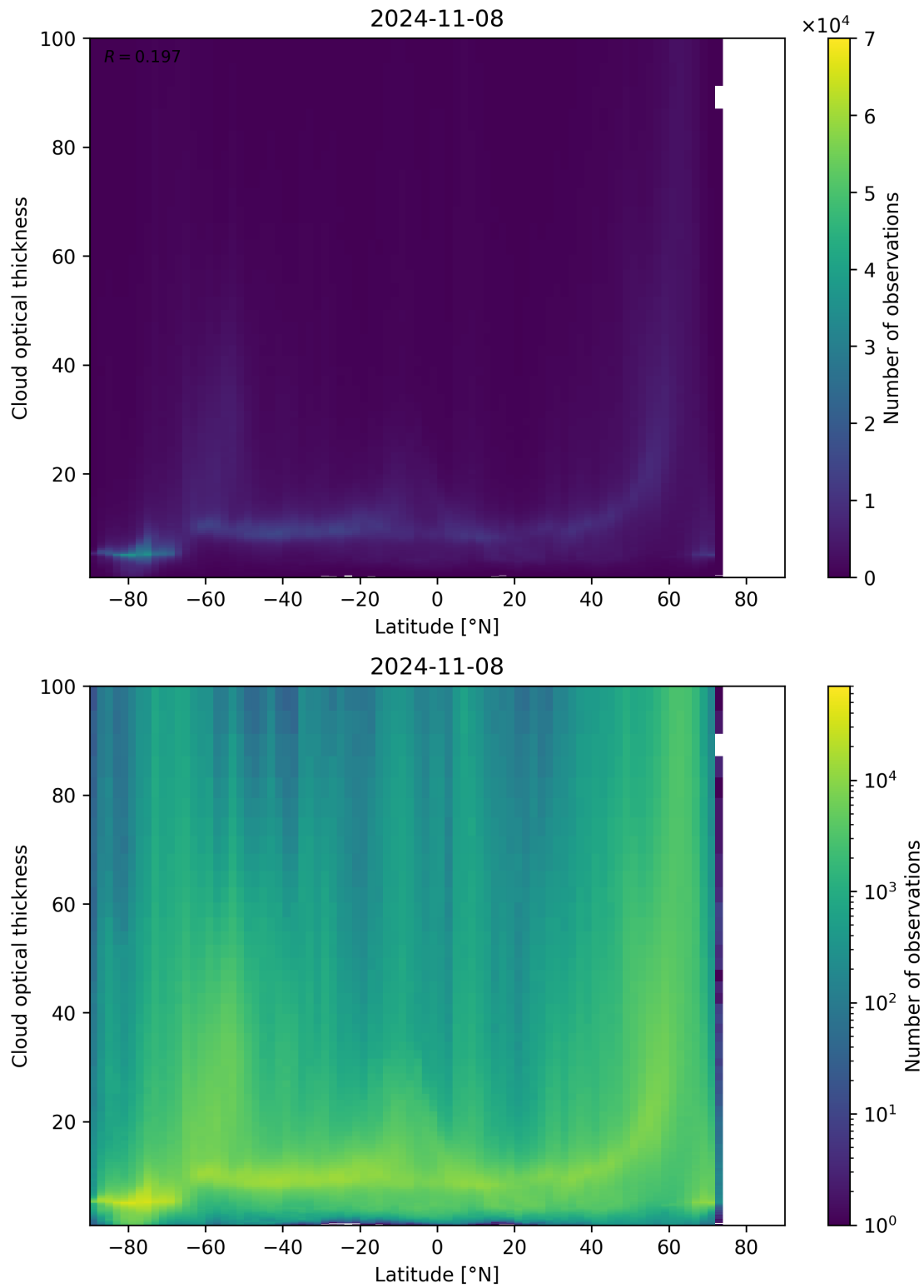
Figure 96: Scatter density plot of “Latitude” against “Cloud optical thickness” for 2024-11-07 to 2024-11-09.
