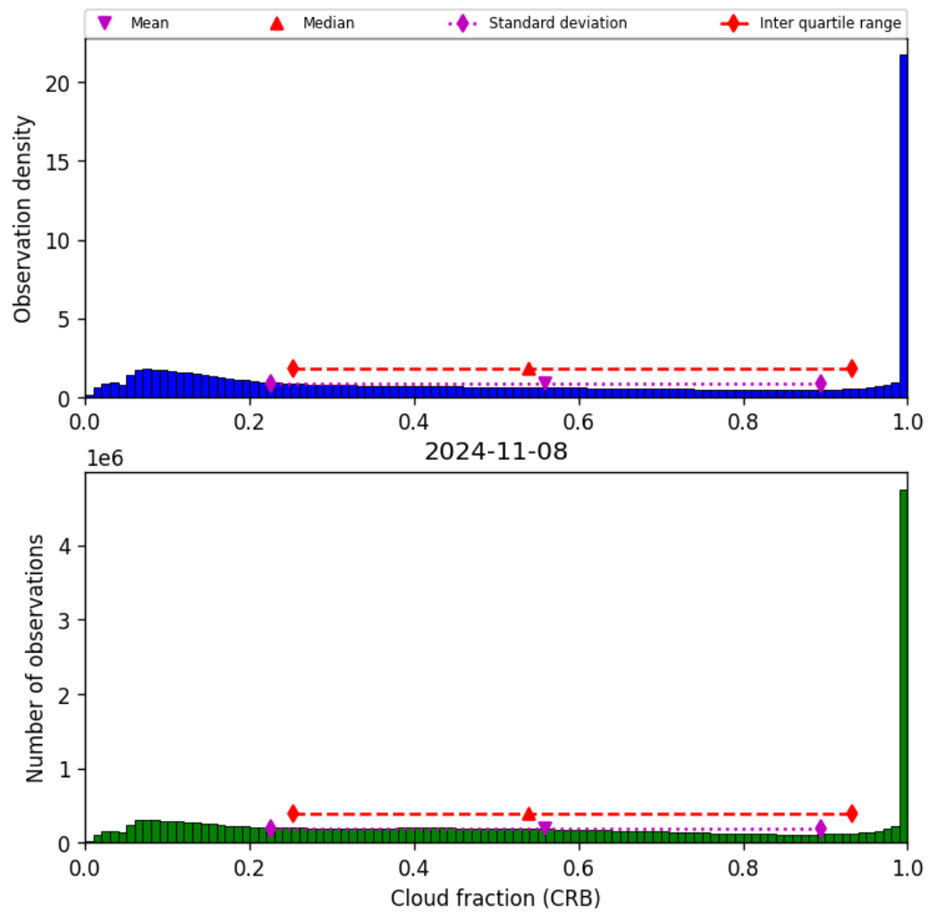
Figure 42: Histogram of “Cloud fraction (CRB)” for 2024-11-07 to 2024-11-09
