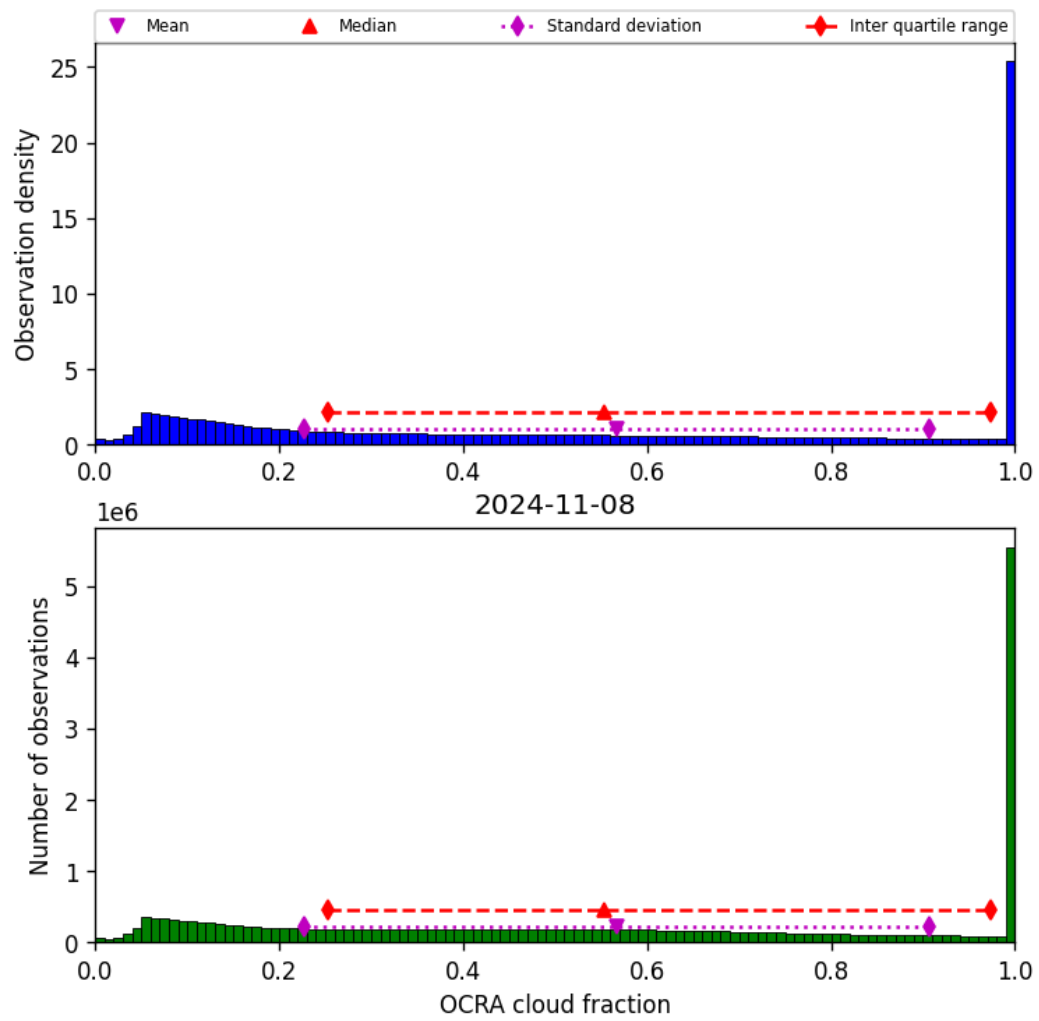
Figure 50: Histogram of “OCRA cloud fraction” for 2024-11-07 to 2024-11-09
