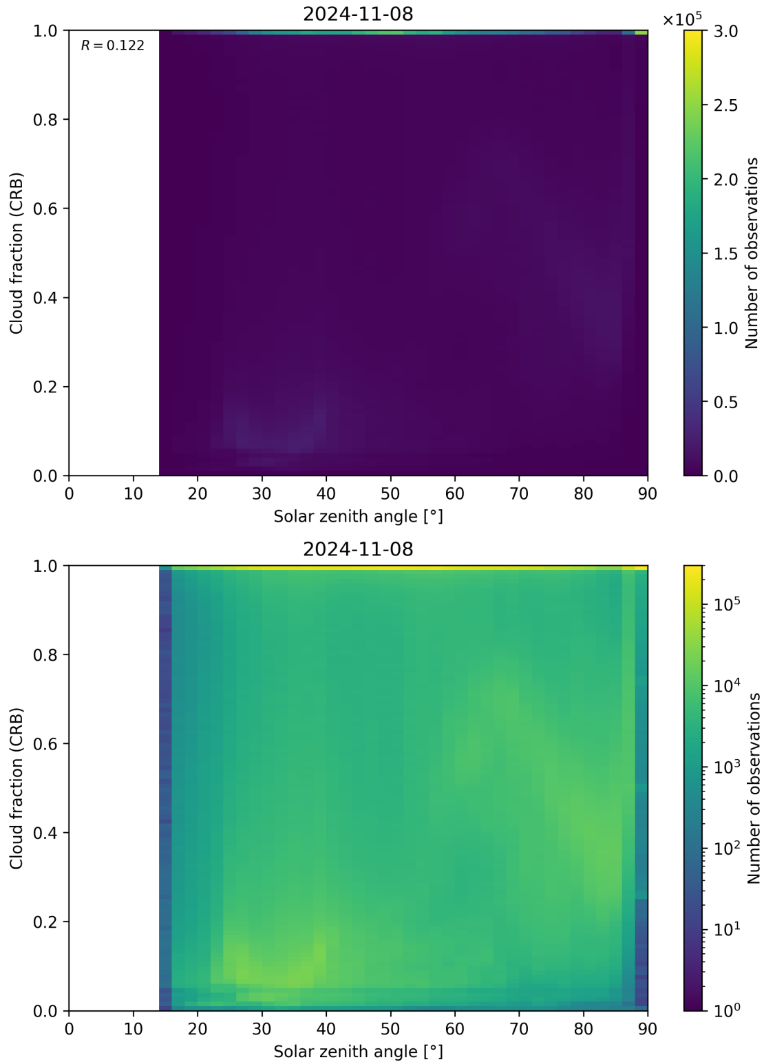
Figure 101: Scatter density plot of “Solar zenith angle” against “Cloud fraction (CRB)” for 2024-11-07 to 2024-11-09.
