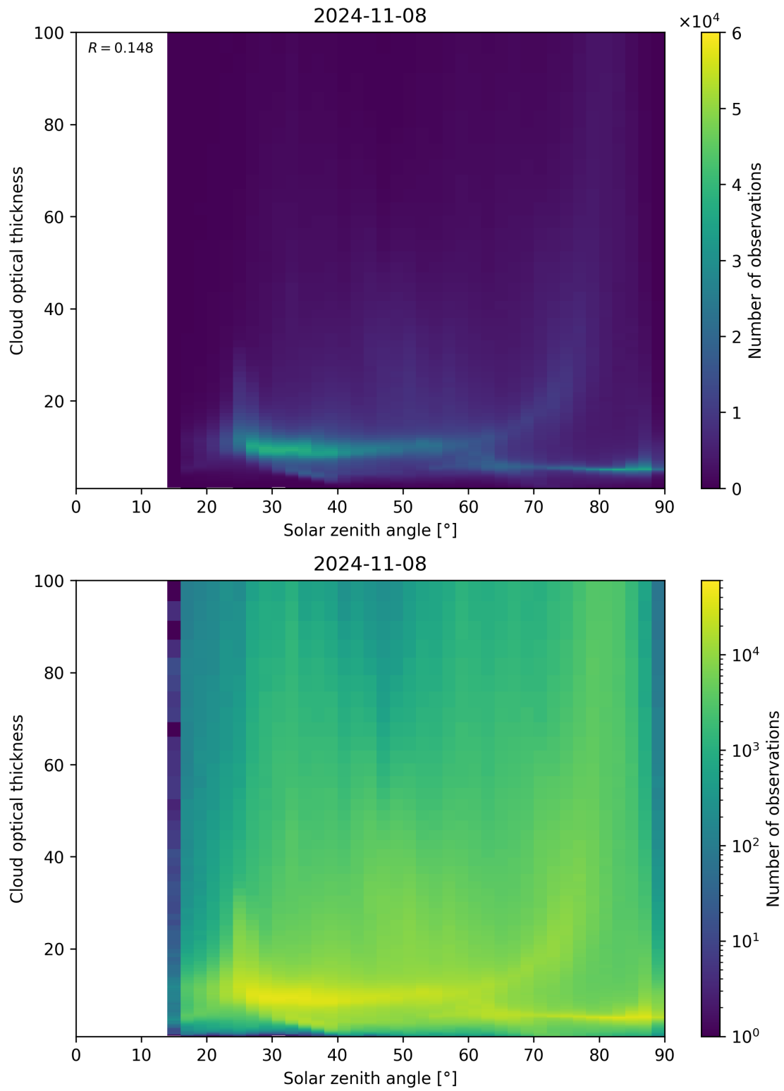
Figure 103: Scatter density plot of “Solar zenith angle” against “Cloud optical thickness” for 2024-11-07 to 2024-11-09.
