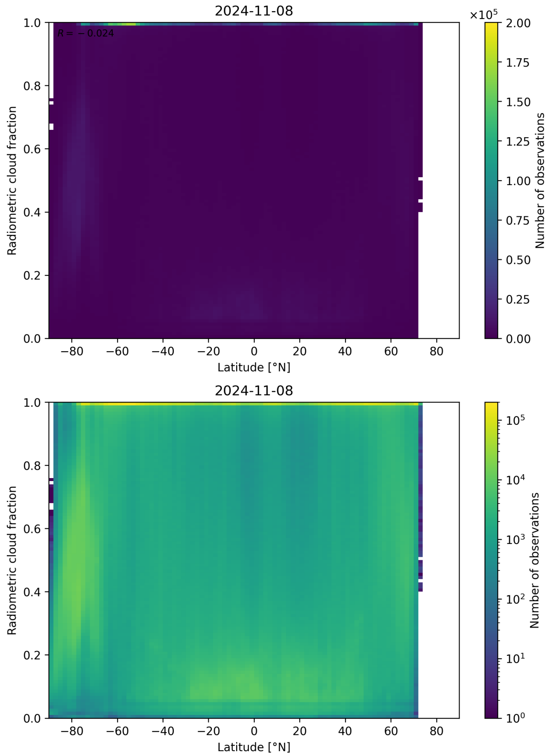
Figure 92: Scatter density plot of “Latitude” against “Radiometric cloud fraction” for 2024-11-07 to 2024-11-09.
