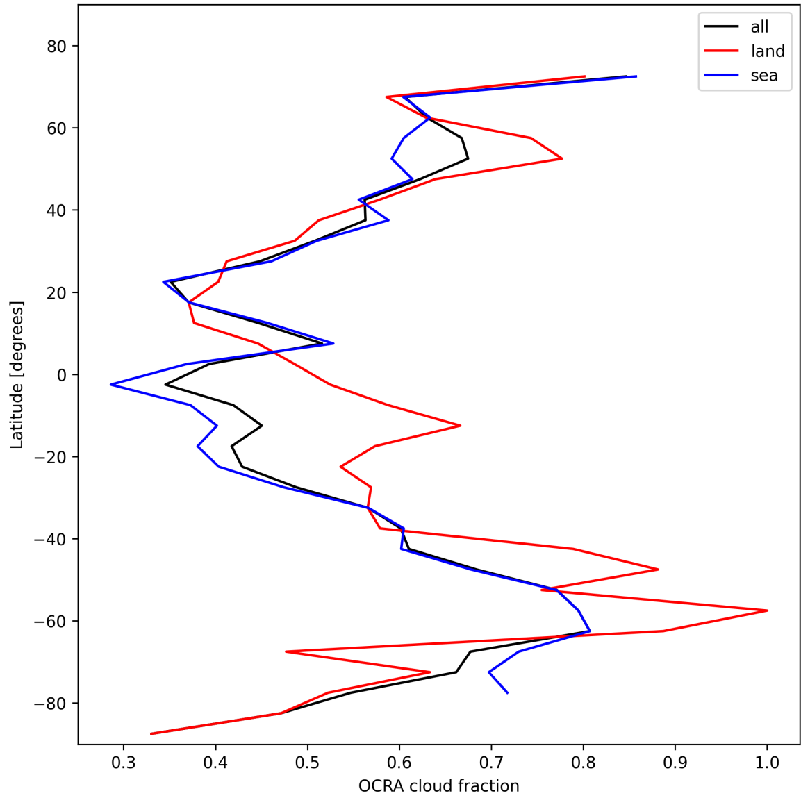
Figure 34: Zonal average of “OCRA cloud fraction” for 2024-11-07 to 2024-11-09.
