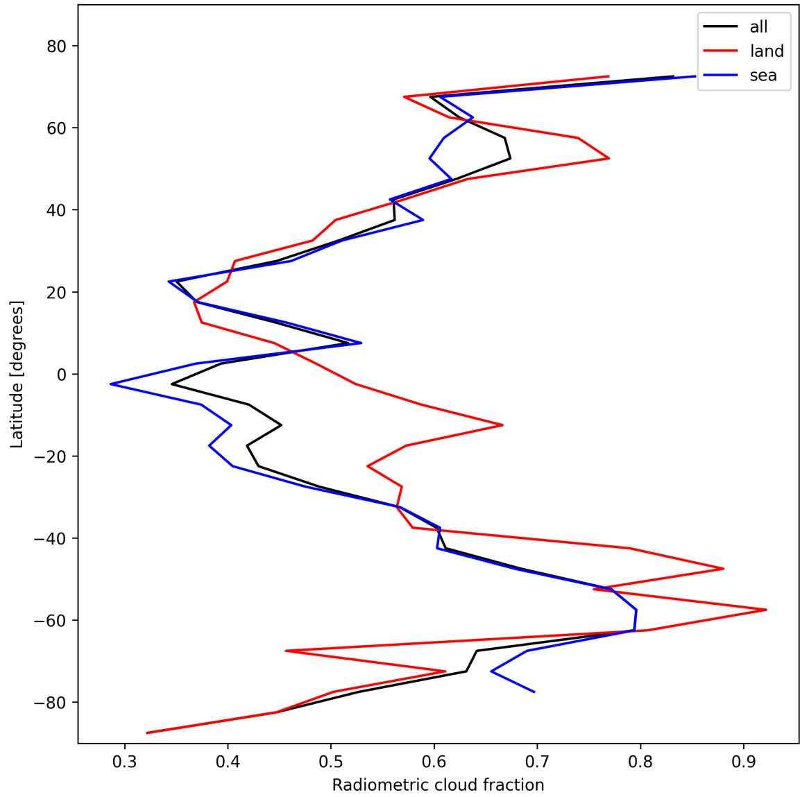
Figure 23: Zonal average of “Radiometric cloud fraction” for 2024-11-07 to 2024-11-09.
