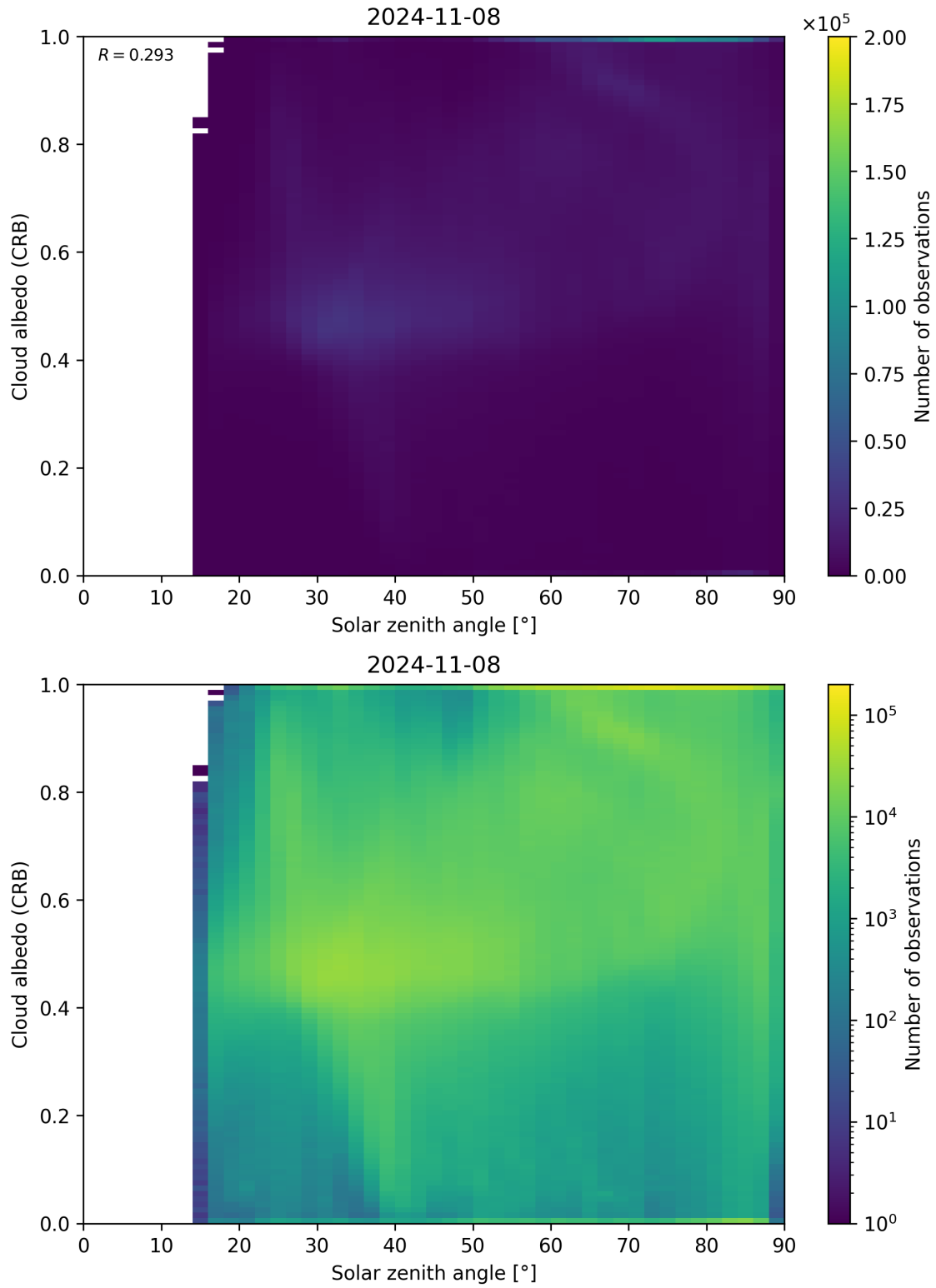
Figure 98: Scatter density plot of “Solar zenith angle” against “Cloud albedo (CRB)” for 2024-11-07 to 2024-11-09.
