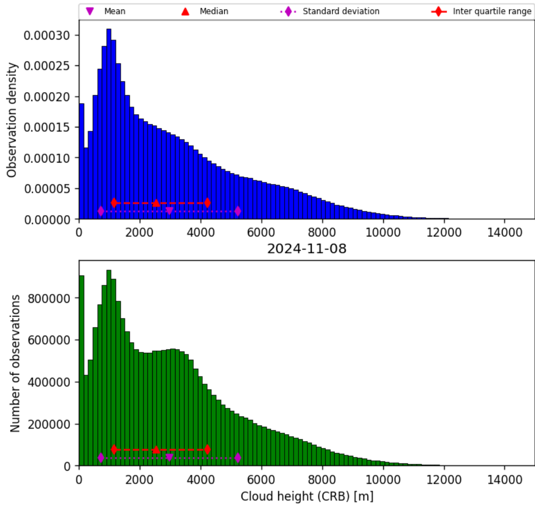
Figure 43: Histogram of “Cloud height (CRB)” for 2024-11-07 to 2024-11-09
