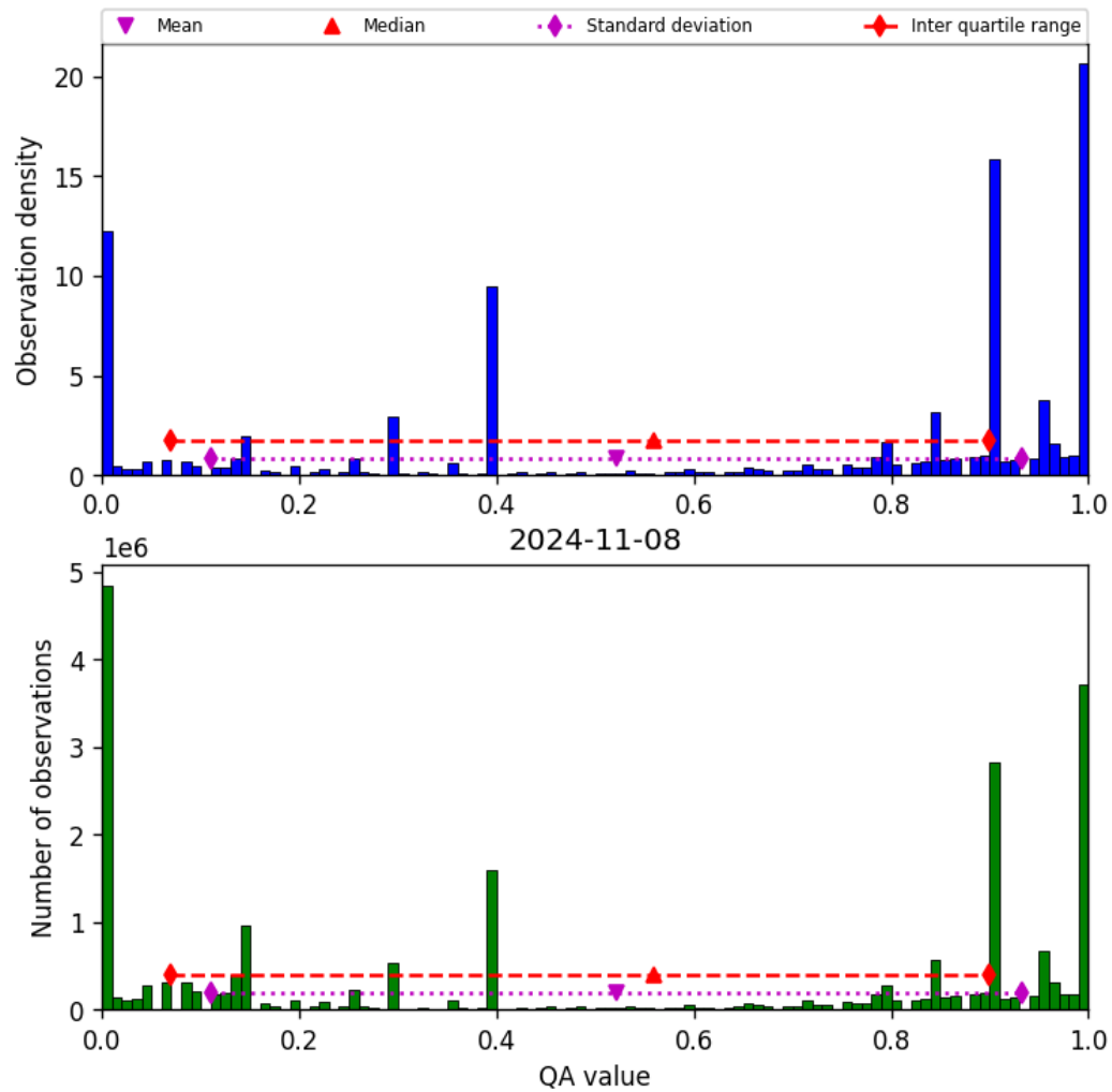
Figure 38: Histogram of “QA value” for 2024-11-07 to 2024-11-09
