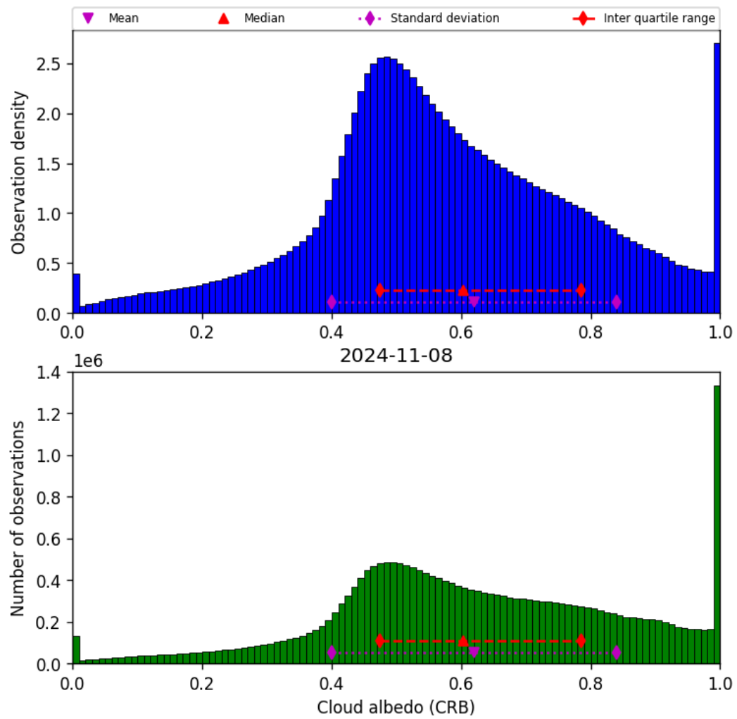
Figure 44: Histogram of “Cloud albedo (CRB)” for 2024-11-07 to 2024-11-09
