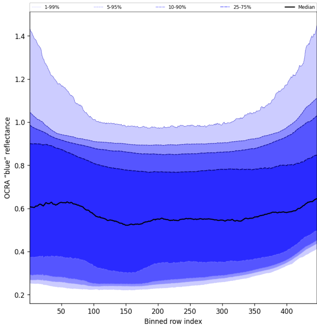
Figure 67: Along track statistics of “OCRA “blue” reflectance” for 2024-11-07 to 2024-11-09
