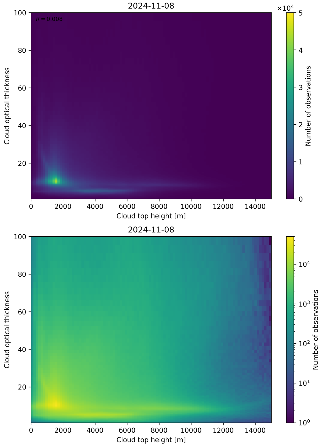
Figure 90: Scatter density plot of “Cloud top height” against “Cloud optical thickness” for 2024-11-07 to 2024-11-09.
