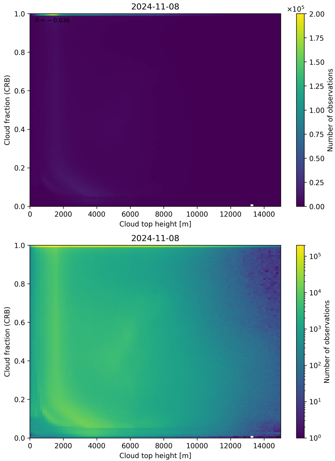
Figure 88: Scatter density plot of “Cloud top height” against “Cloud fraction (CRB)” for 2024-11-07 to 2024-11-09.
