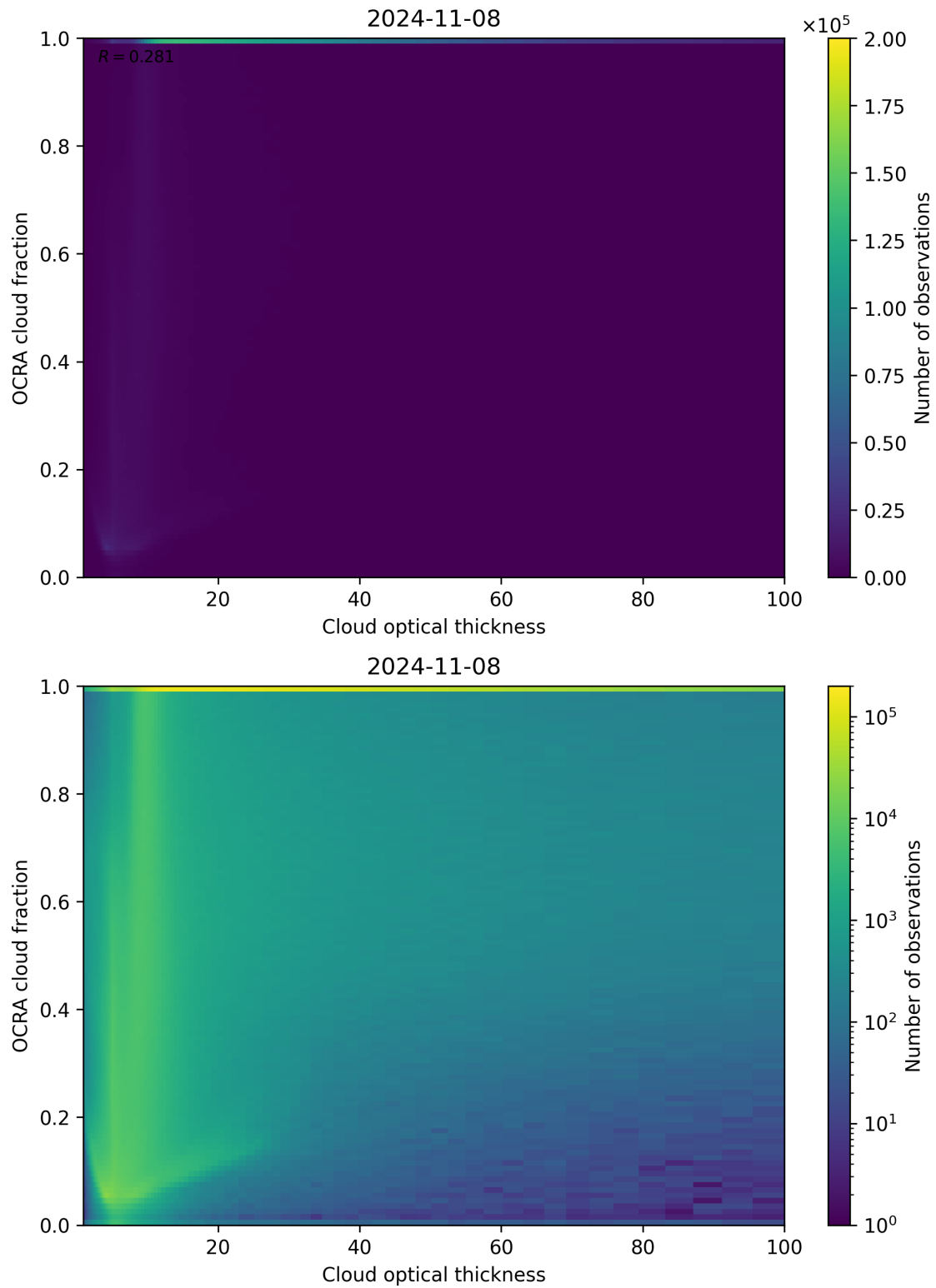
Figure 83: Scatter density plot of “Cloud optical thickness” against “OCRA cloud fraction” for 2024-11-07 to 2024-11-09.
