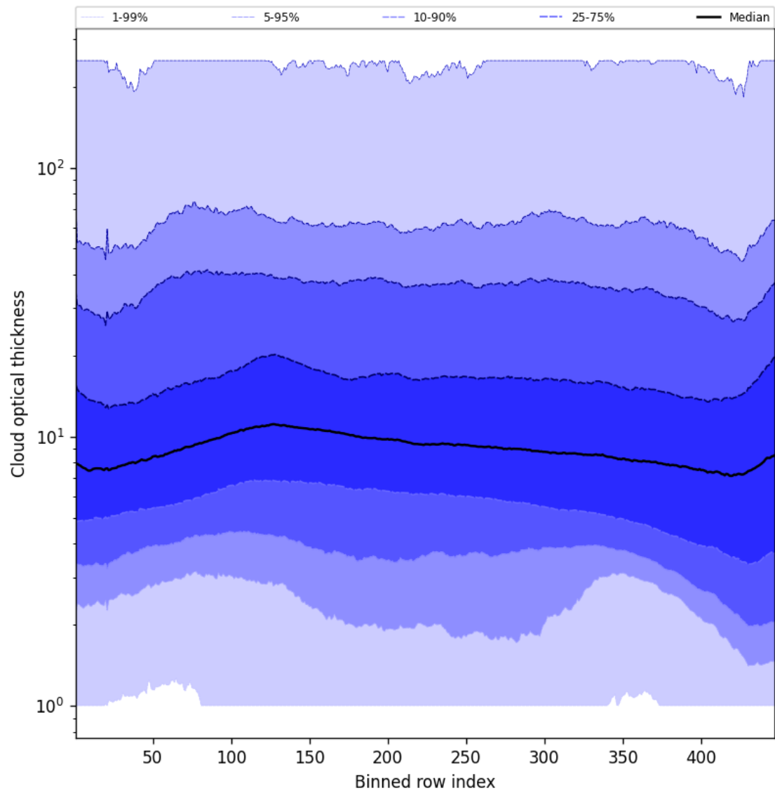
Figure 57: Along track statistics of “Cloud optical thickness” for 2024-11-07 to 2024-11-09
