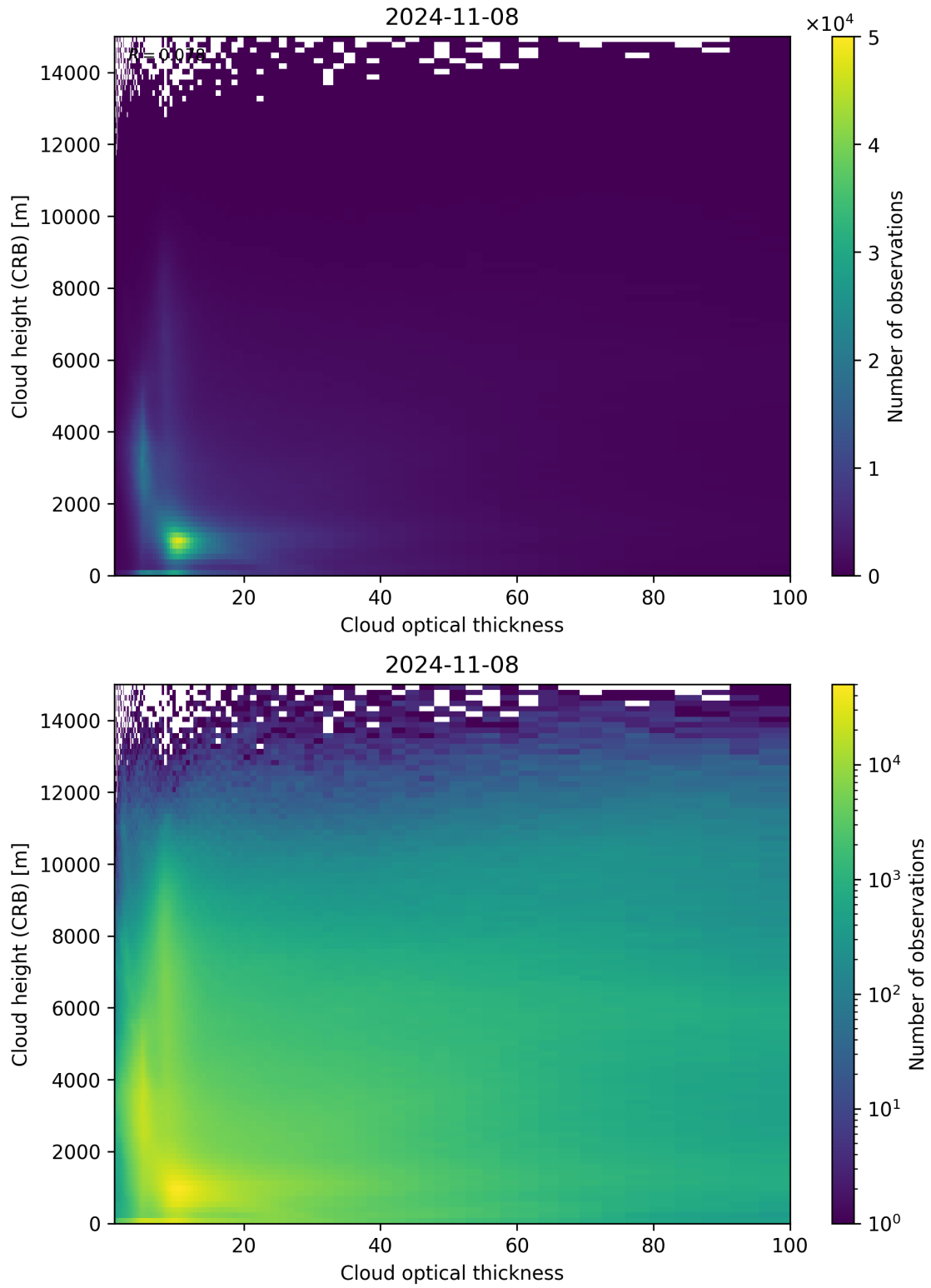
Figure 85: Scatter density plot of “Cloud optical thickness” against “Cloud height (CRB)” for 2024-11-07 to 2024-11-09.
