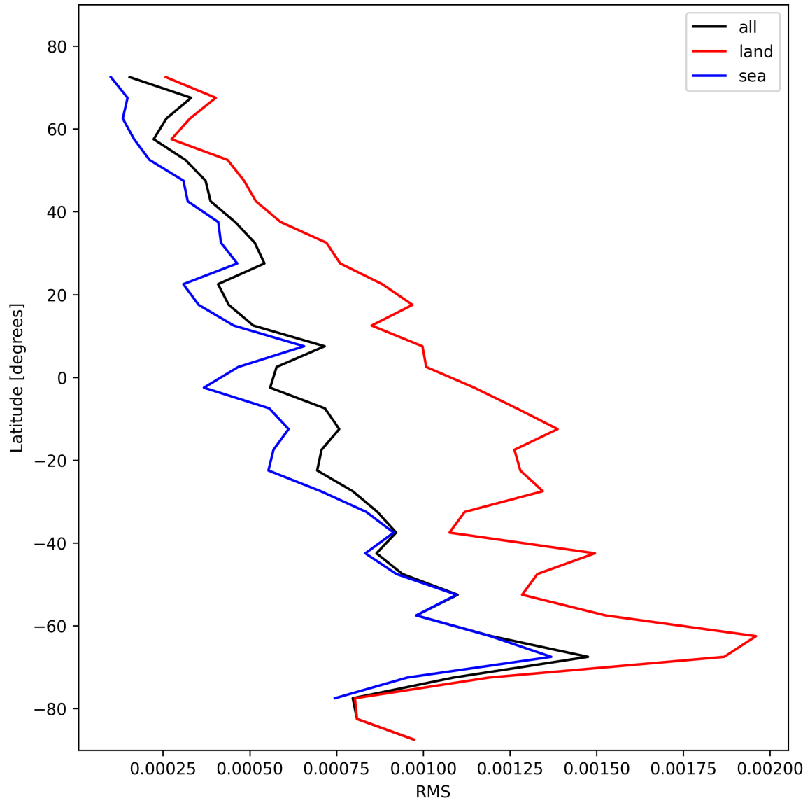
Figure 31: Zonal average of “RMS” for 2024-11-07 to 2024-11-09.
