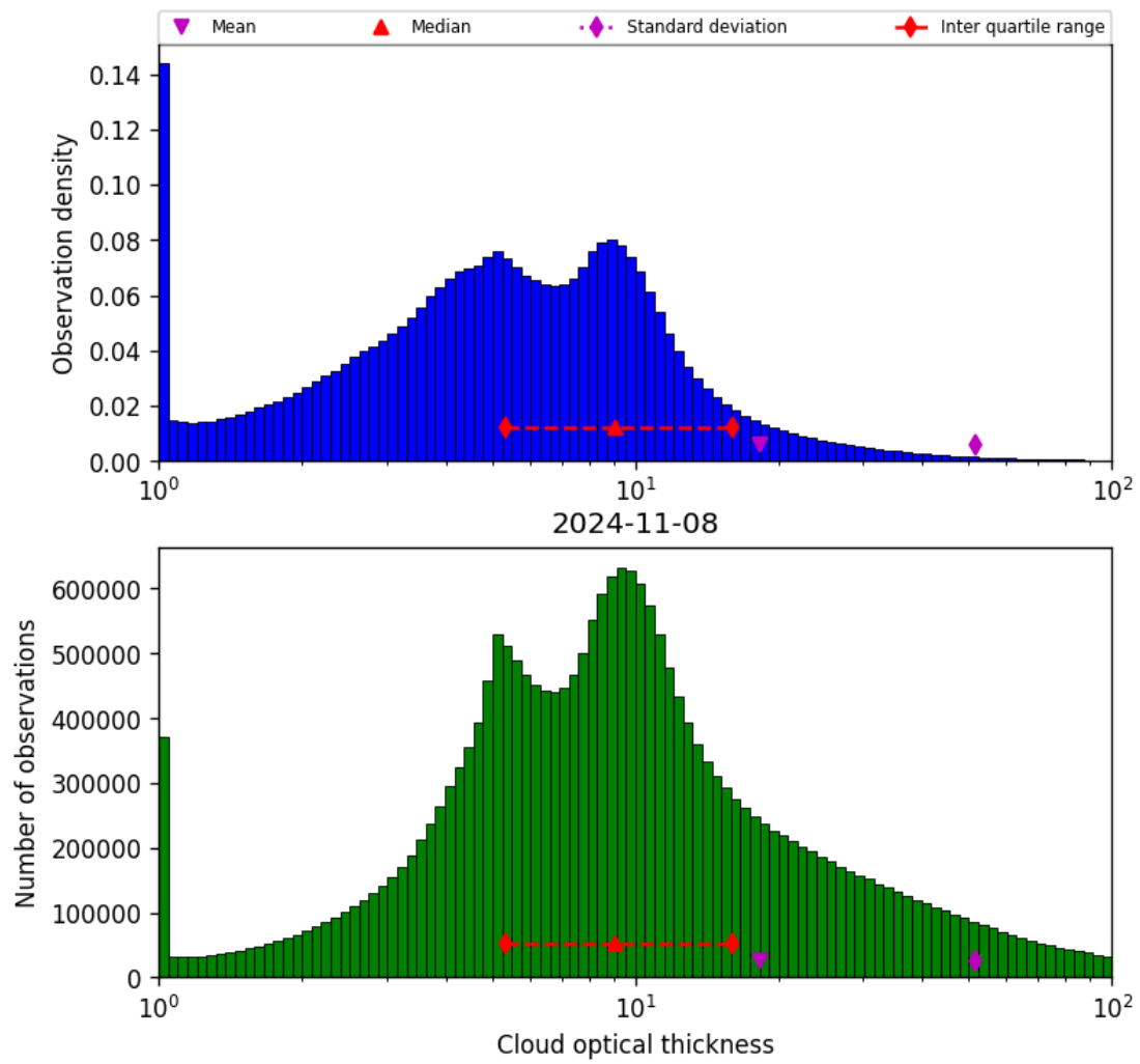
Figure 41: Histogram of “Cloud optical thickness” for 2024-11-07 to 2024-11-09
