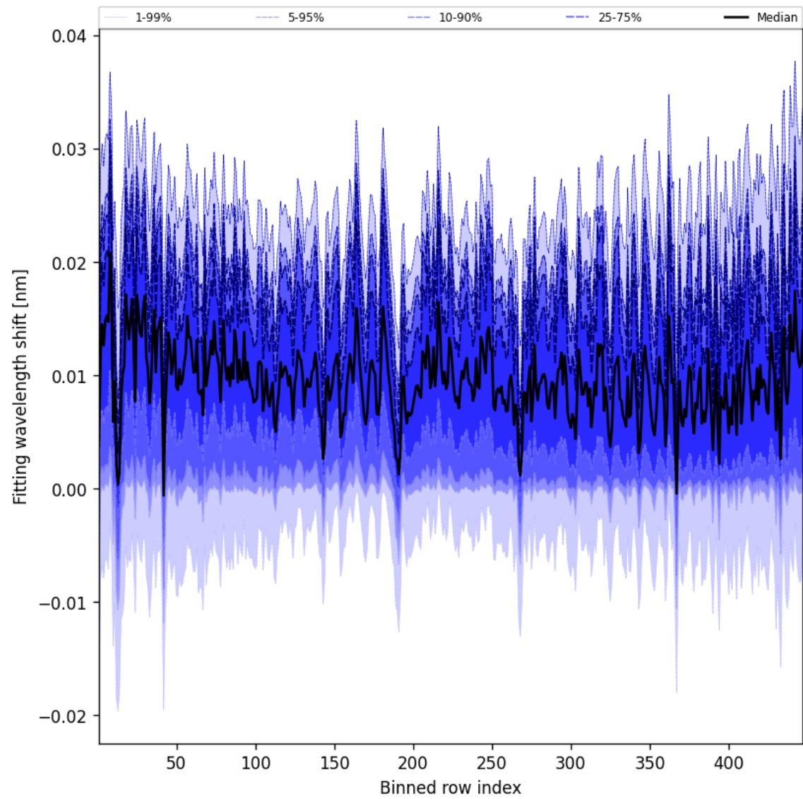
Figure 65: Along track statistics of “Fitting wavelength shift” for 2024-11-07 to 2024-11-09
