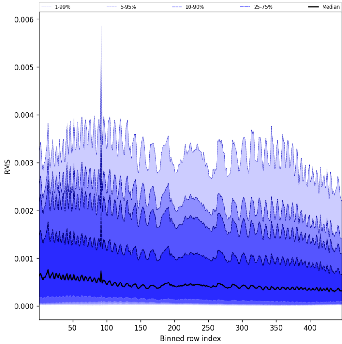
Figure 63: Along track statistics of “RMS” for 2024-11-07 to 2024-11-09
