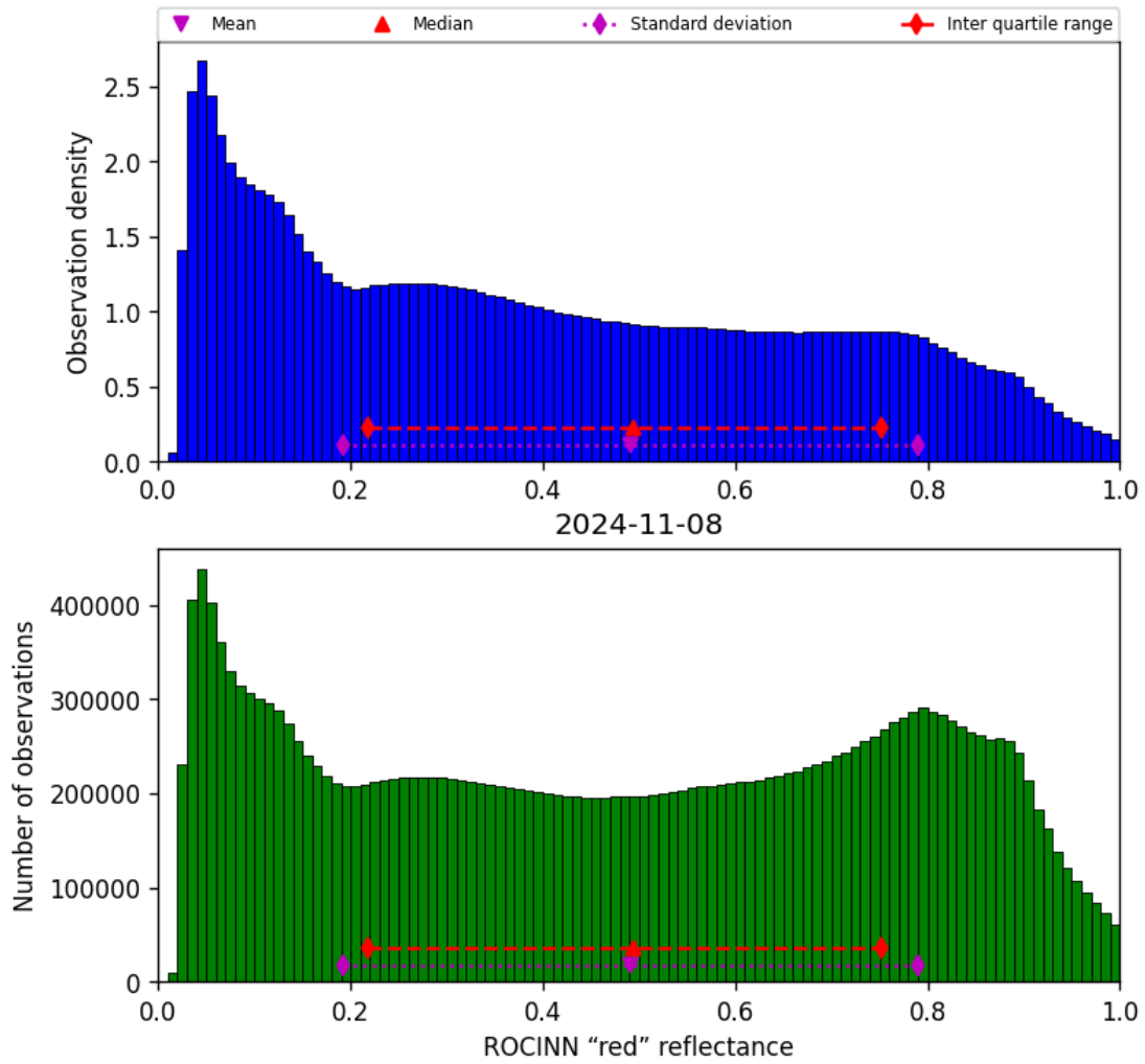
Figure 53: Histogram of “ROCINN “red” reflectance” for 2024-11-07 to 2024-11-09
