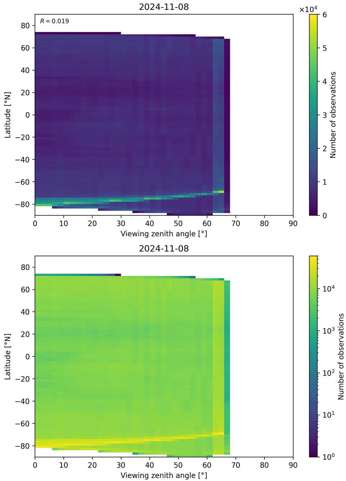
Figure 113: Scatter density plot of “Viewing zenith angle” against “Latitude” for 2024-11-07 to 2024-11-09.
