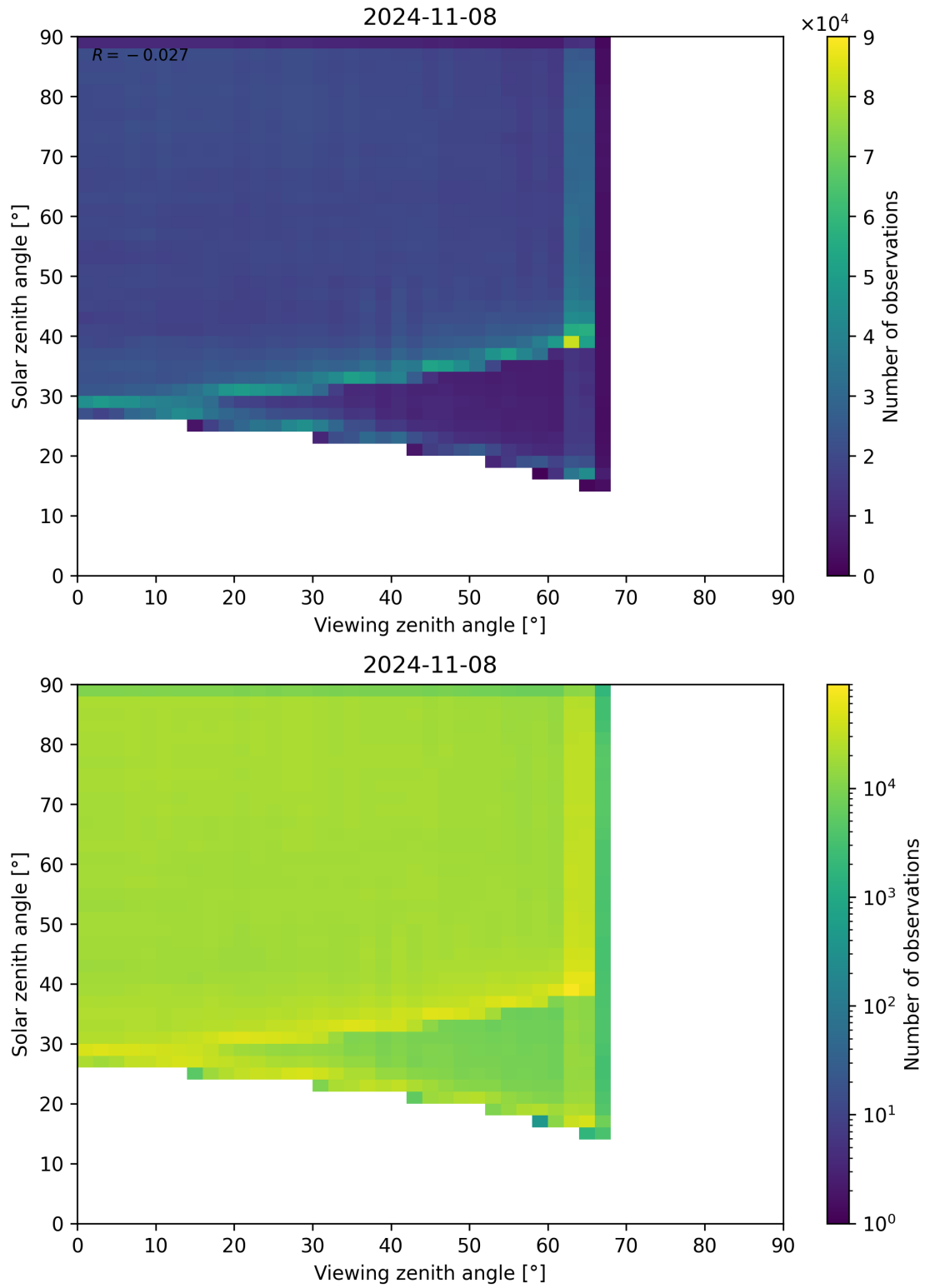
Figure 114: Scatter density plot of “Viewing zenith angle” against “Solar zenith angle” for 2024-11-07 to 2024-11-09.
