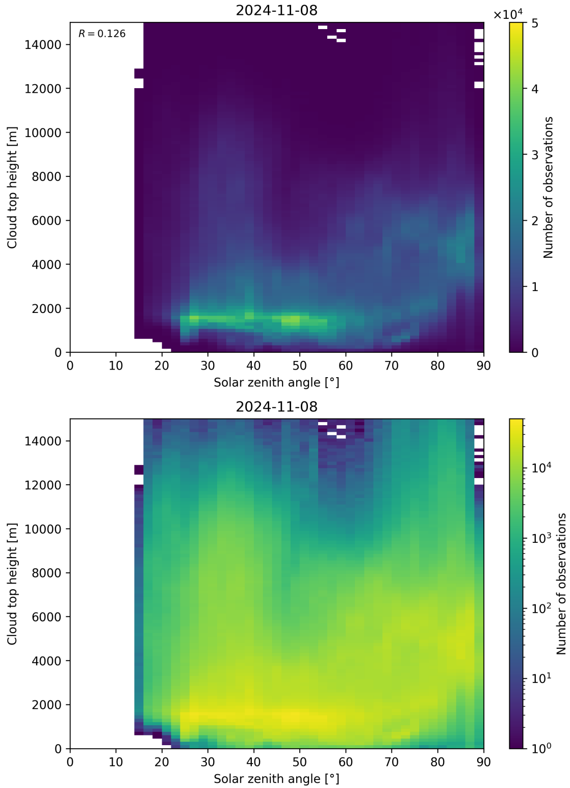
Figure 104: Scatter density plot of “Solar zenith angle” against “Cloud top height” for 2024-11-07 to 2024-11-09.
