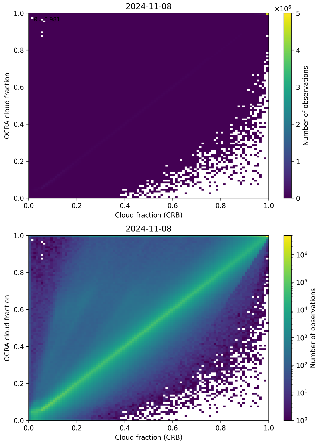
Figure 78: Scatter density plot of “Cloud fraction (CRB)” against “OCRA cloud fraction” for 2024-11-07 to 2024-11-09.
