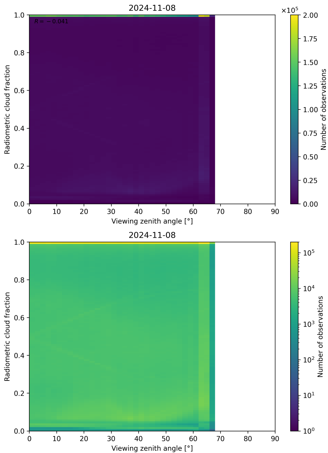
Figure 107: Scatter density plot of “Viewing zenith angle” against “Radiometric cloud fraction” for 2024-11-07 to 2024-11-09.
