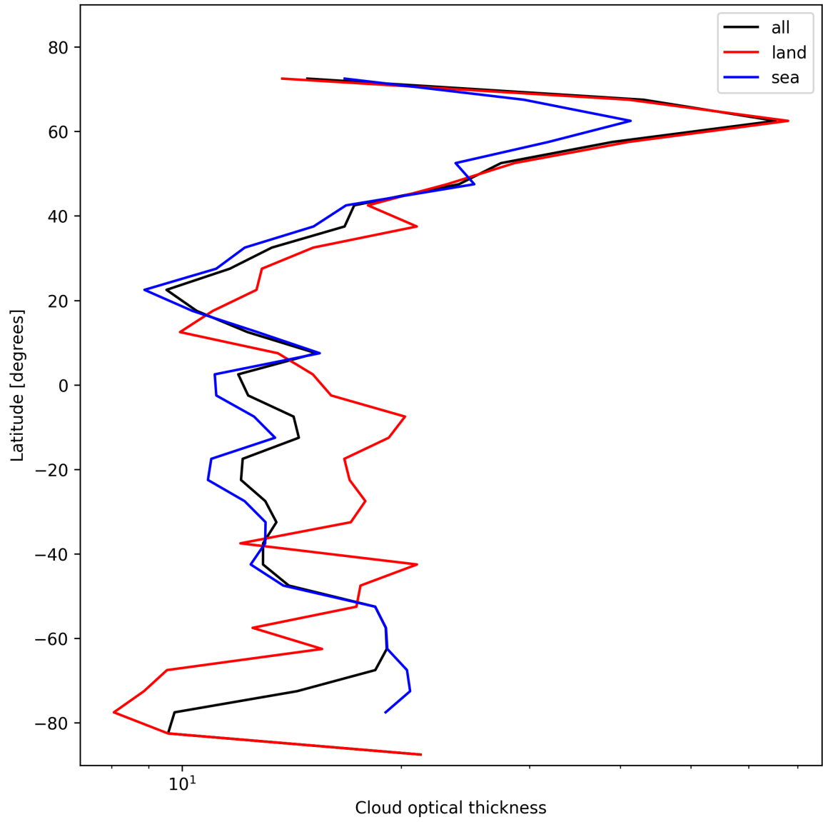
Figure 25: Zonal average of “Cloud optical thickness” for 2024-11-07 to 2024-11-09.
