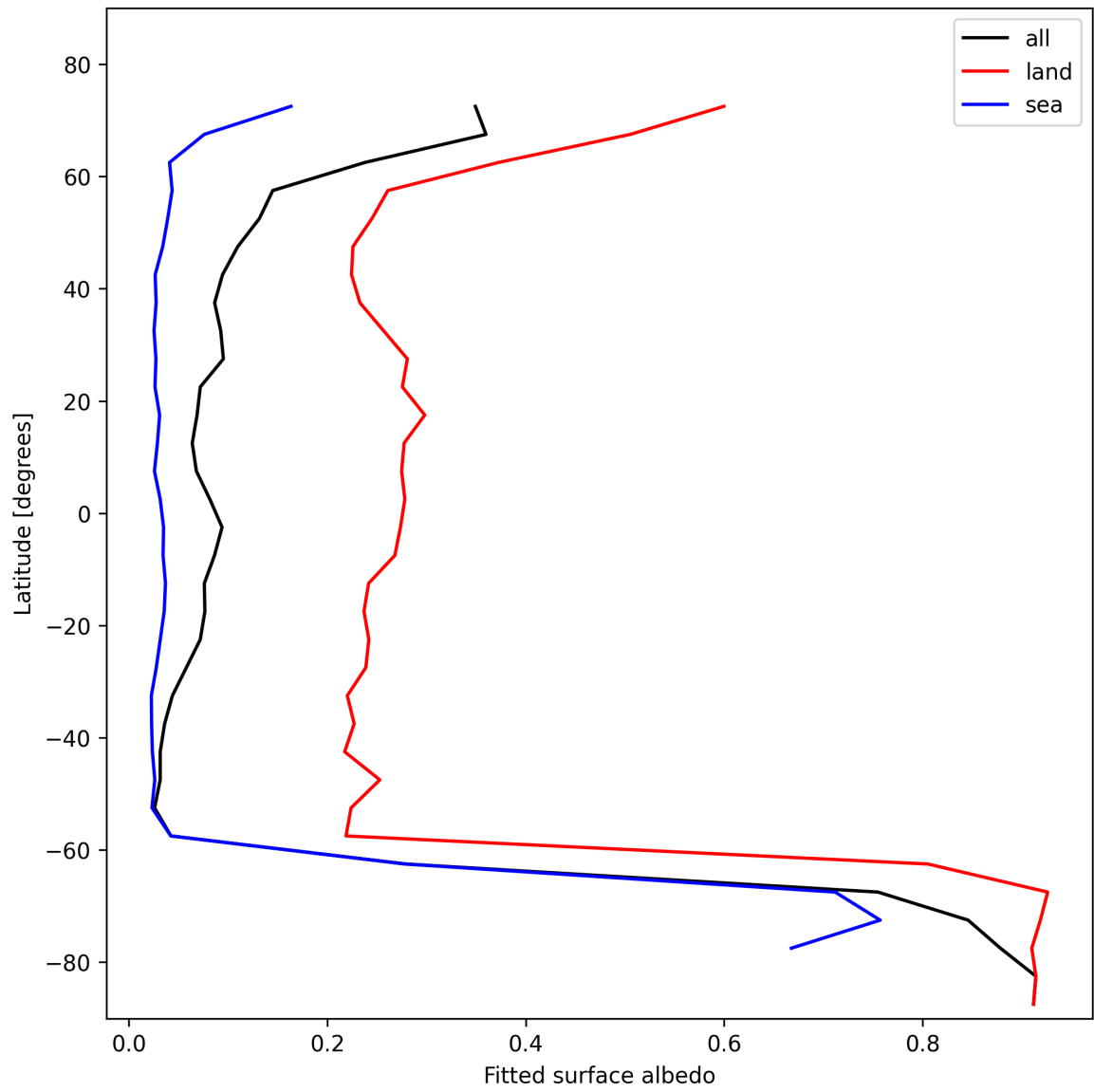
Figure 29: Zonal average of “Fitted surface albedo” for 2024-11-07 to 2024-11-09.
