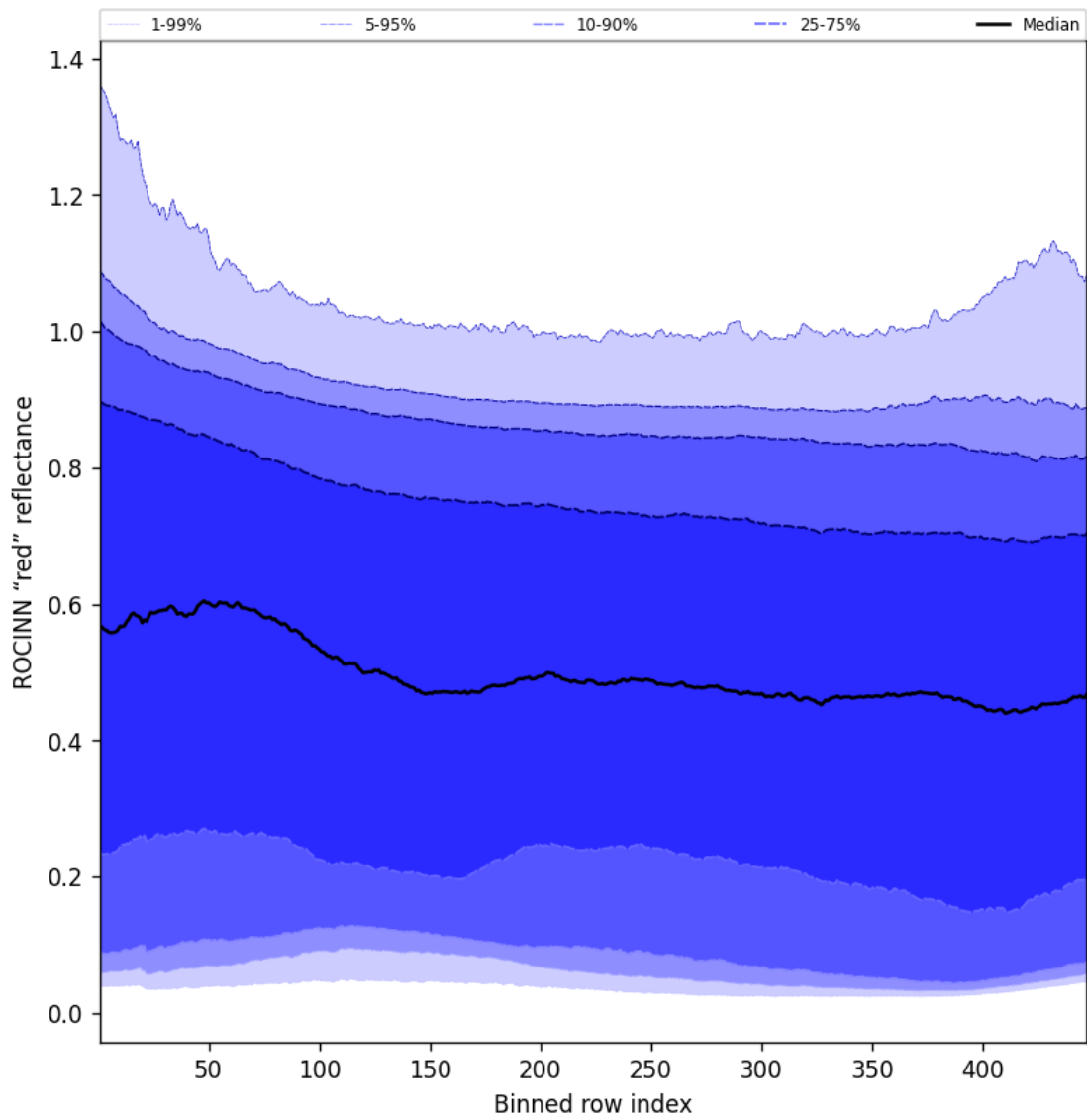
Figure 69: Along track statistics of “ROCINN “red” reflectance” for 2024-11-07 to 2024-11-09
