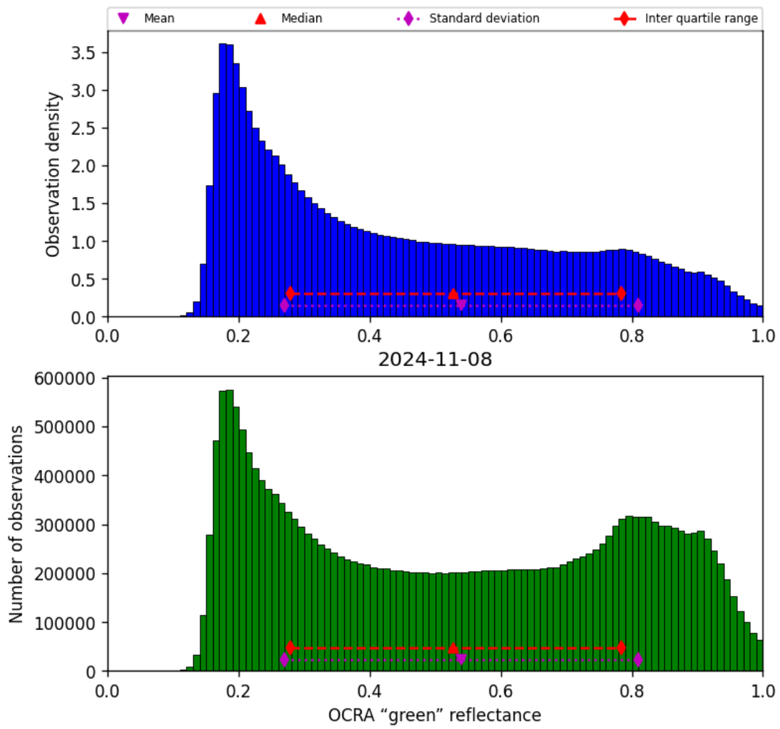
Figure 52: Histogram of “OCRA “green” reflectance” for 2024-11-07 to 2024-11-09
