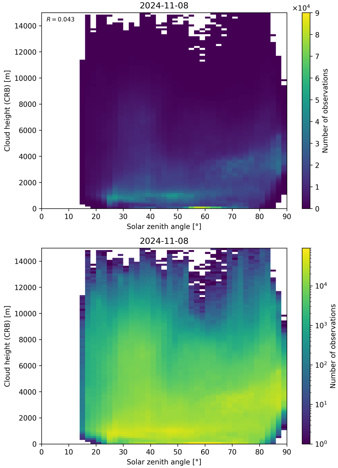
Figure 102: Scatter density plot of “Solar zenith angle” against “Cloud height (CRB)” for 2024-11-07 to 2024-11-09.
