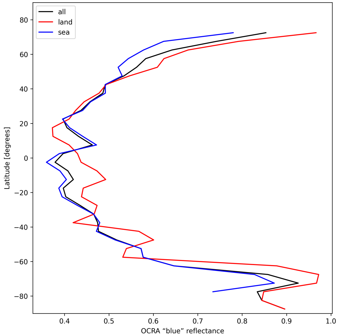
Figure 35: Zonal average of “OCRA “blue” reflectance” for 2024-11-07 to 2024-11-09.
