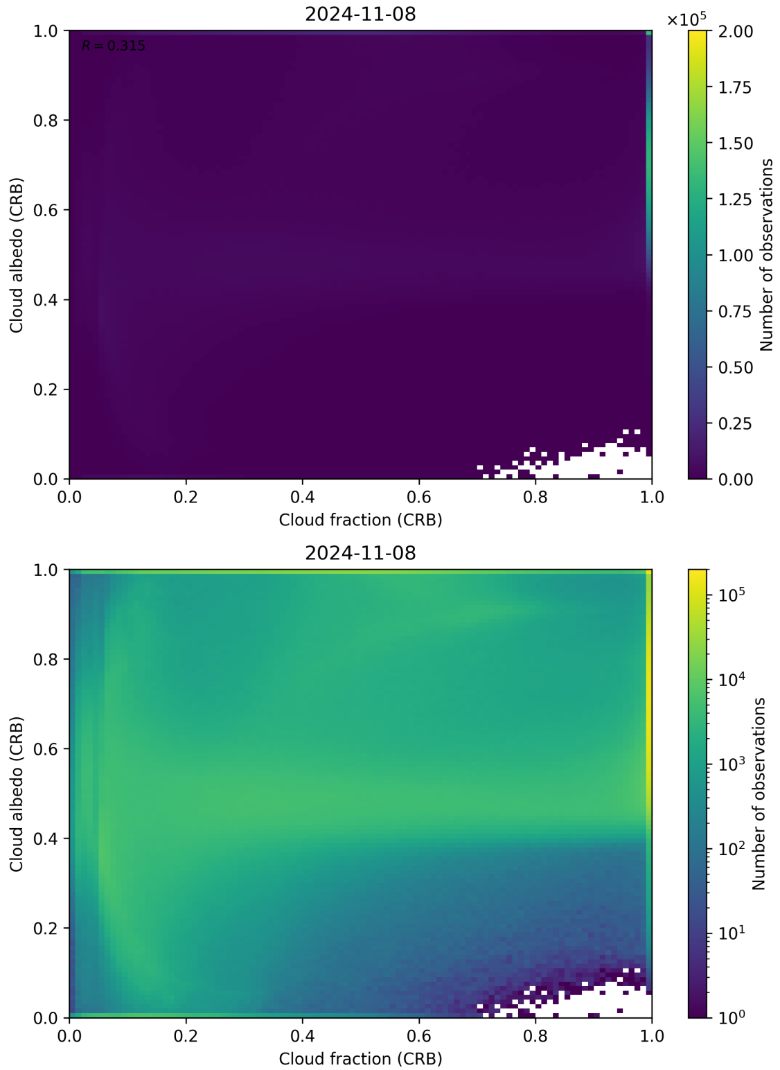
Figure 77: Scatter density plot of “Cloud fraction (CRB)” against “Cloud albedo (CRB)” for 2024-11-07 to 2024-11-09.
