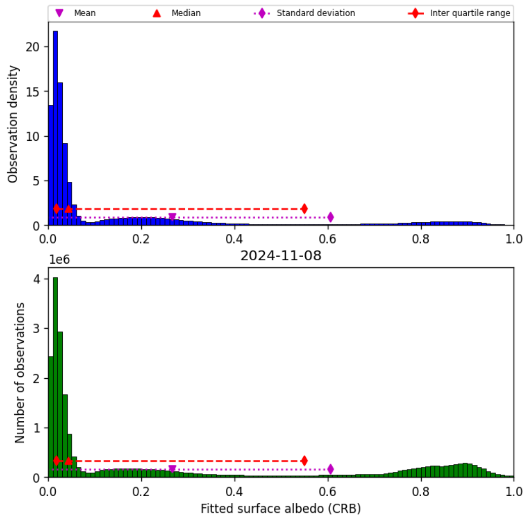
Figure 46: Histogram of “Fitted surface albedo (CRB)” for 2024-11-07 to 2024-11-09
