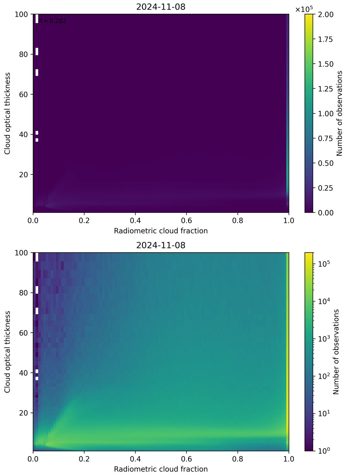
Figure 75: Scatter density plot of “Radiometric cloud fraction” against “Cloud optical thickness” for 2024-11-07 to 2024-11-09.
