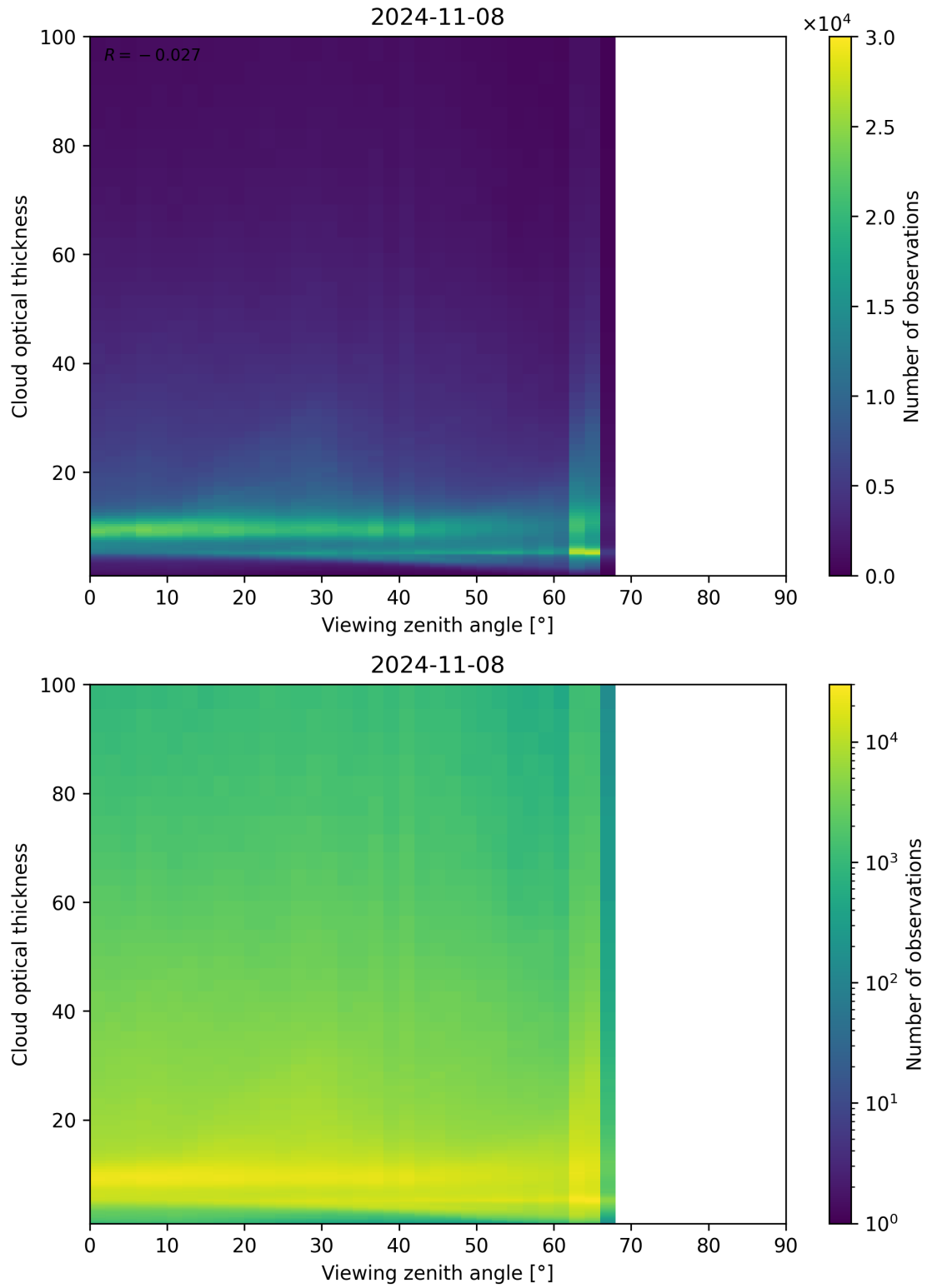
Figure 111: Scatter density plot of “Viewing zenith angle” against “Cloud optical thickness” for 2024-11-07 to 2024-11-09.
