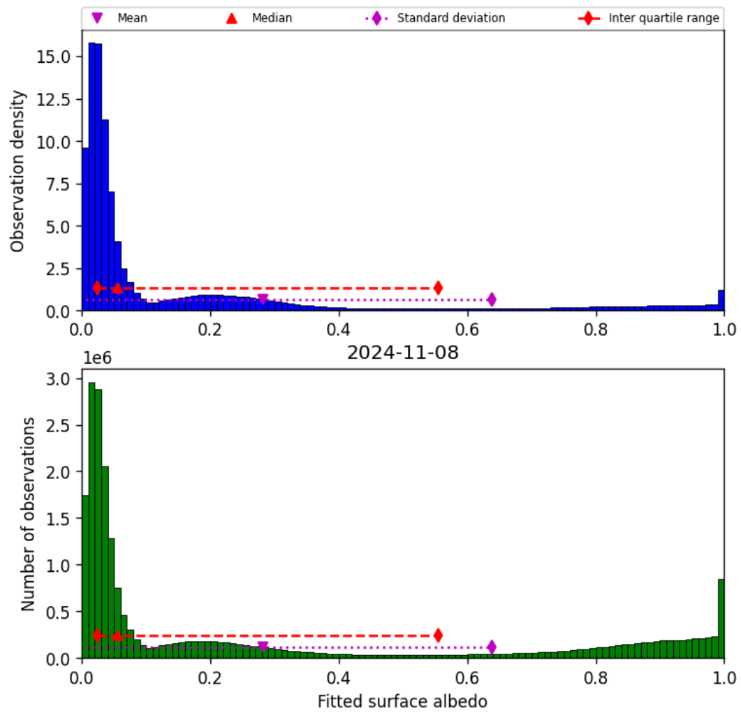
Figure 45: Histogram of “Fitted surface albedo” for 2024-11-07 to 2024-11-09
