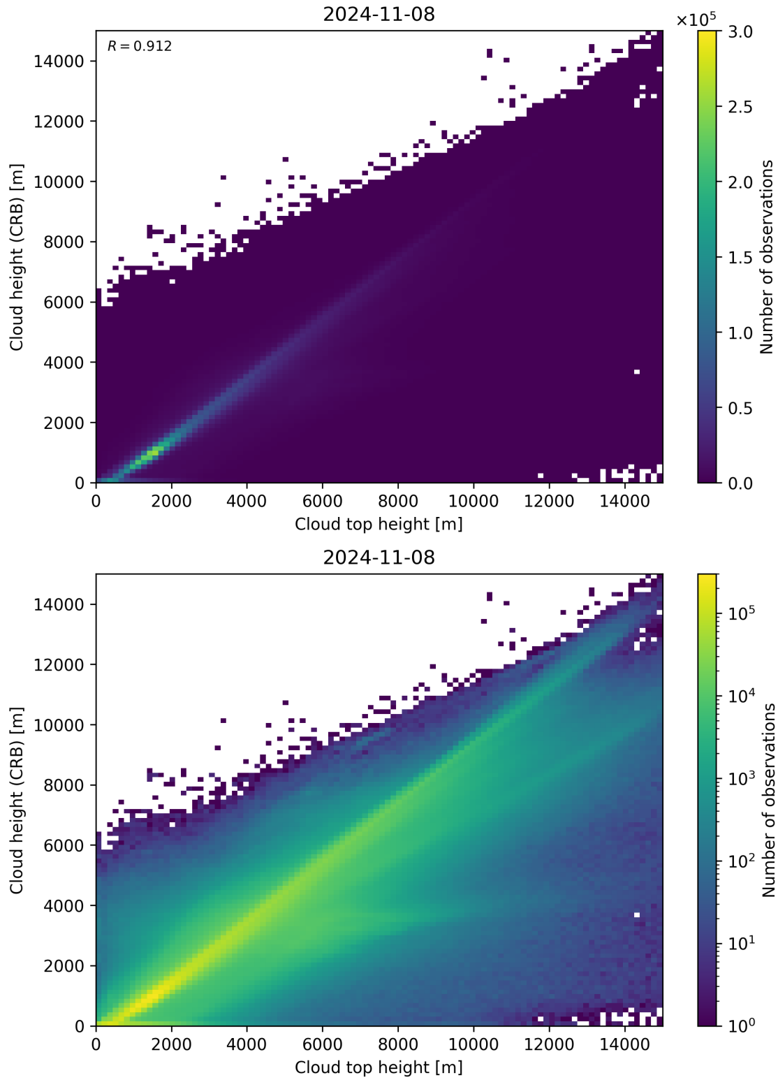
Figure 89: Scatter density plot of “Cloud top height” against “Cloud height (CRB)” for 2024-11-07 to 2024-11-09.
