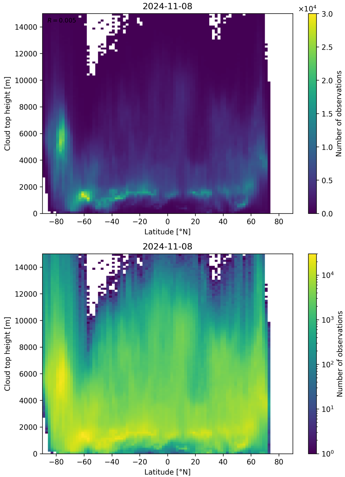
Figure 97: Scatter density plot of “Latitude” against “Cloud top height” for 2024-11-07 to 2024-11-09.
