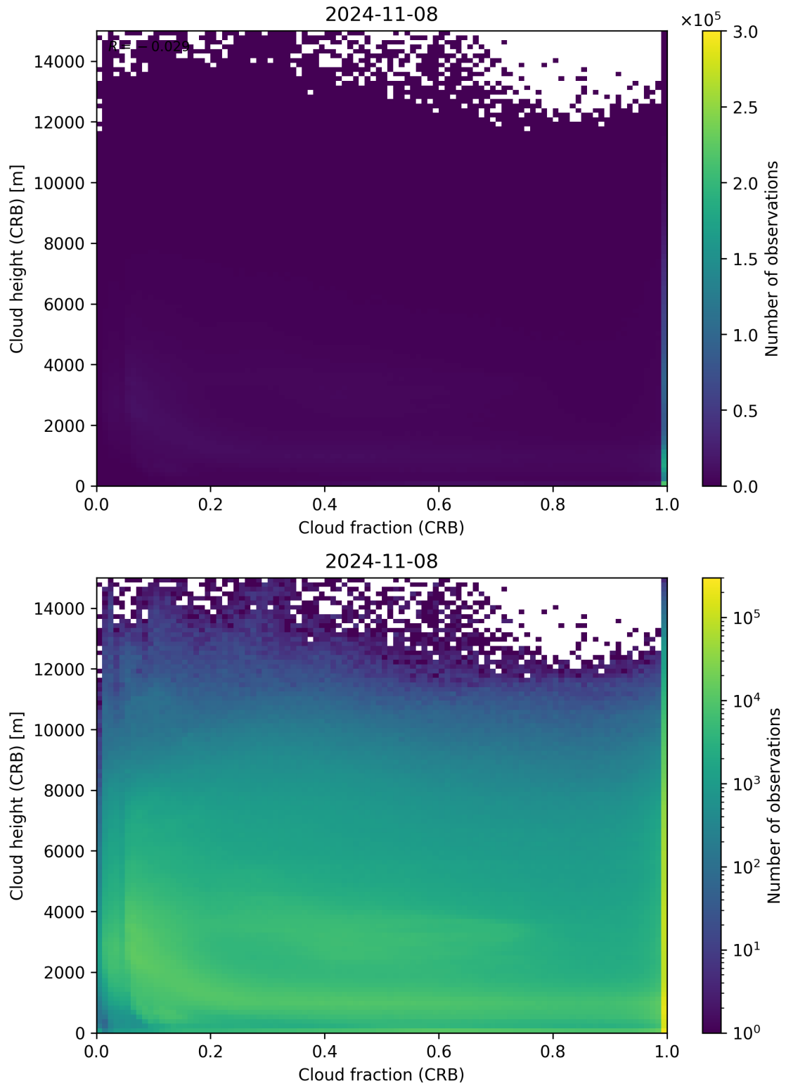
Figure 79: Scatter density plot of “Cloud fraction (CRB)” against “Cloud height (CRB)” for 2024-11-07 to 2024-11-09.
