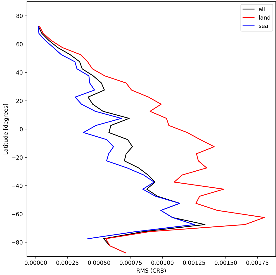
Figure 32: Zonal average of “RMS (CRB)” for 2024-11-07 to 2024-11-09.
