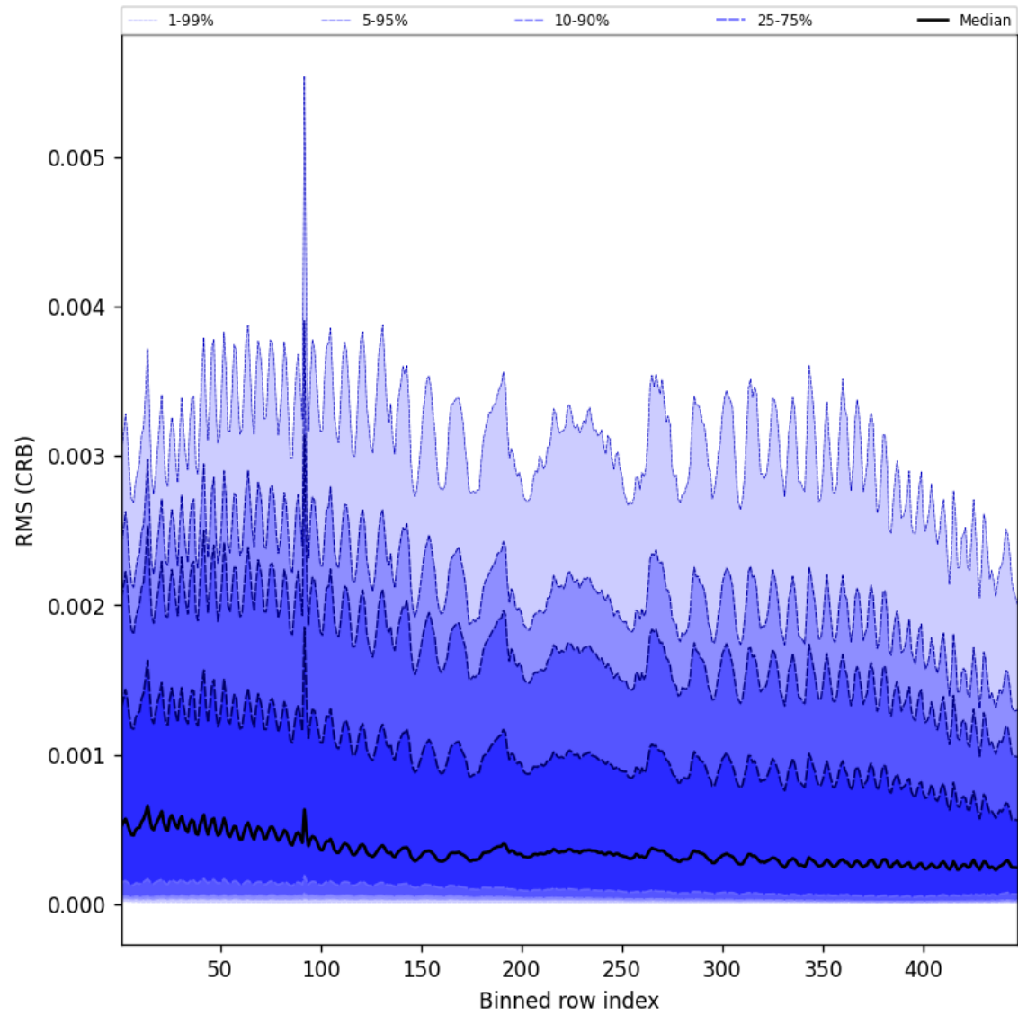
Figure 64: Along track statistics of “RMS (CRB)” for 2024-11-07 to 2024-11-09
