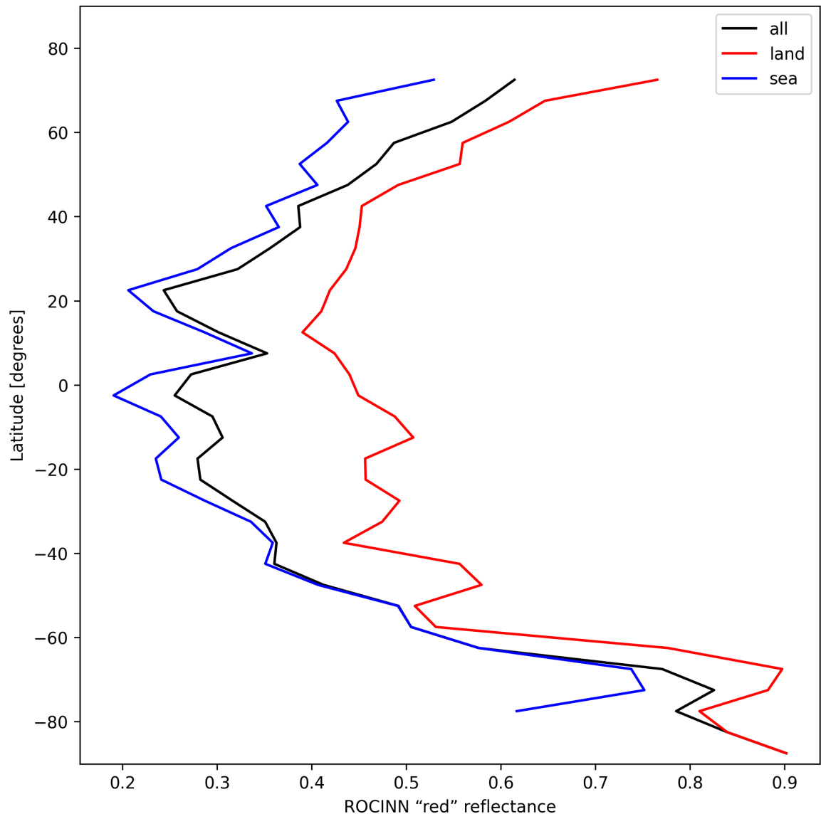
Figure 37: Zonal average of "ROCINN "red" reflectance" for 2024-11-07 to 2024-11-09.
