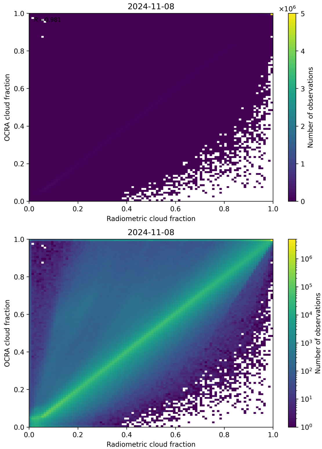
Figure 72: Scatter density plot of “Radiometric cloud fraction” against “OCRA cloud fraction” for 2024-11-07 to 2024-11-09.
