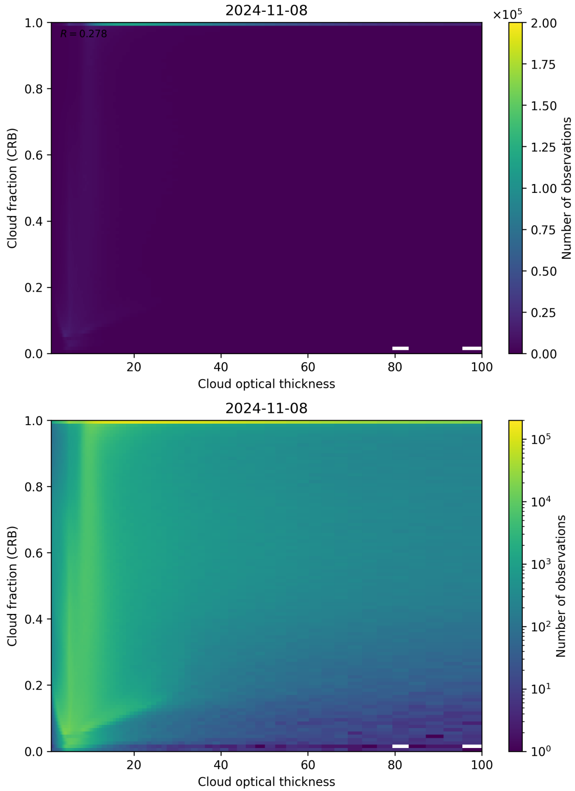
Figure 84: Scatter density plot of “Cloud optical thickness” against “Cloud fraction (CRB)” for 2024-11-07 to 2024-11-09.
