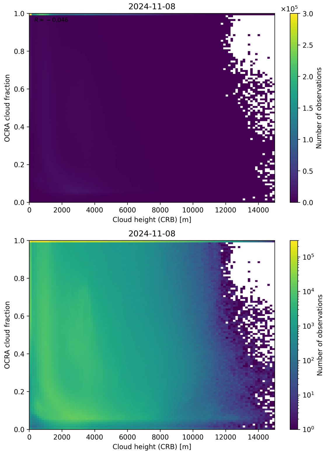
Figure 81: Scatter density plot of “Cloud height (CRB)” against “OCRA cloud fraction” for 2024-11-07 to 2024-11-09.
