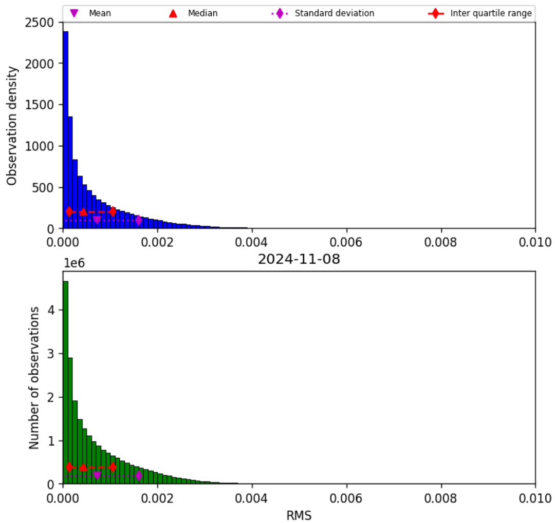
Figure 47: Histogram of “RMS” for 2024-11-07 to 2024-11-09
