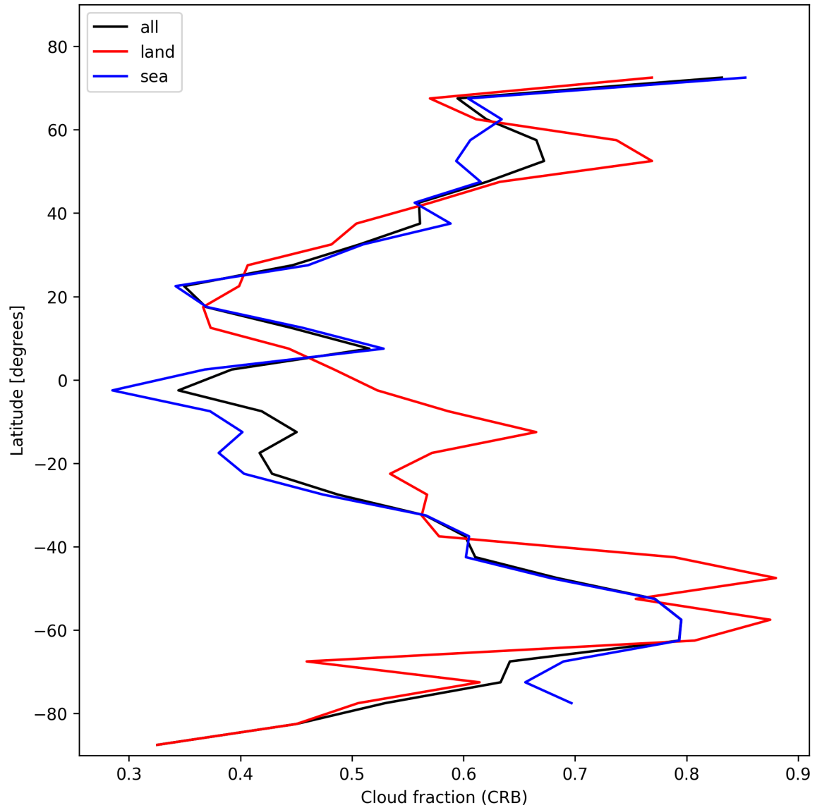
Figure 26: Zonal average of “Cloud fraction (CRB)” for 2024-11-07 to 2024-11-09.
