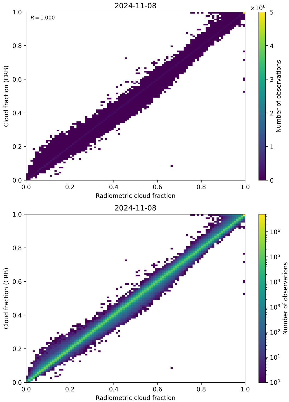
Figure 73: Scatter density plot of “Radiometric cloud fraction” against “Cloud fraction (CRB)” for 2024-11-07 to 2024-11-09.
