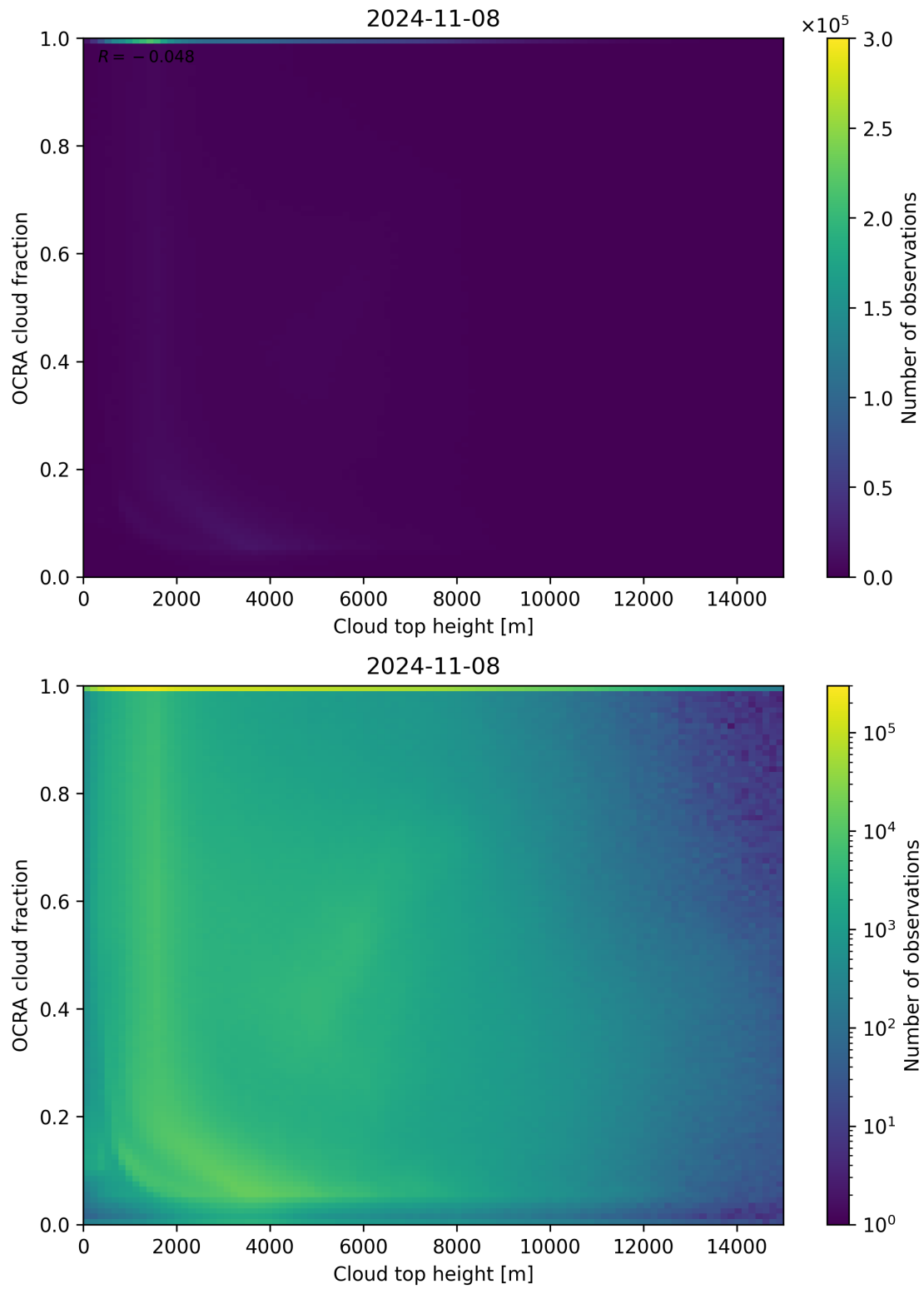
Figure 87: Scatter density plot of “Cloud top height” against “OCRA cloud fraction” for 2024-11-07 to 2024-11-09.
