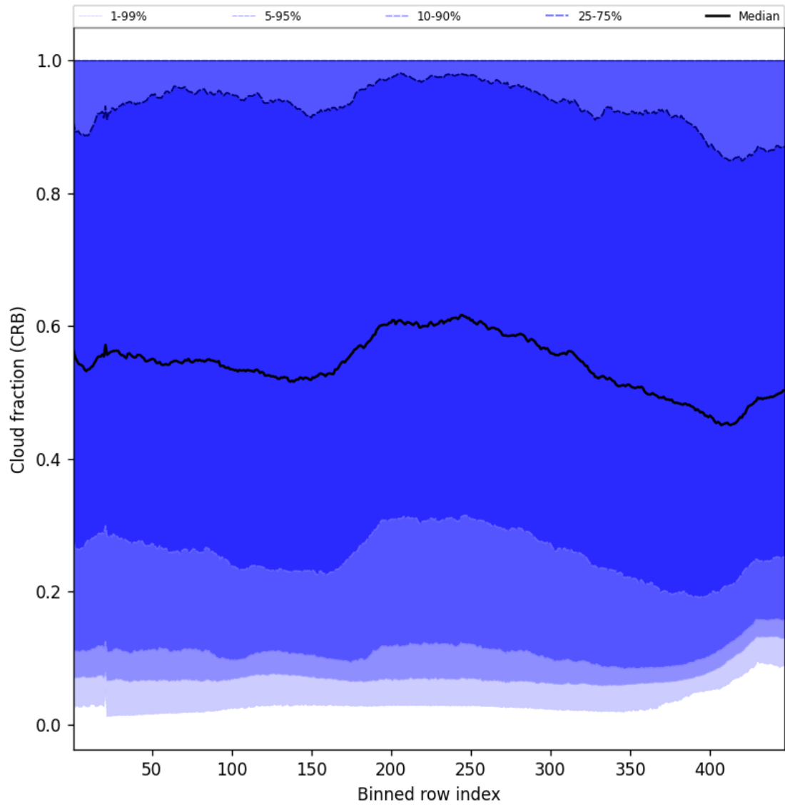
Figure 58: Along track statistics of “Cloud fraction (CRB)” for 2024-11-07 to 2024-11-09
