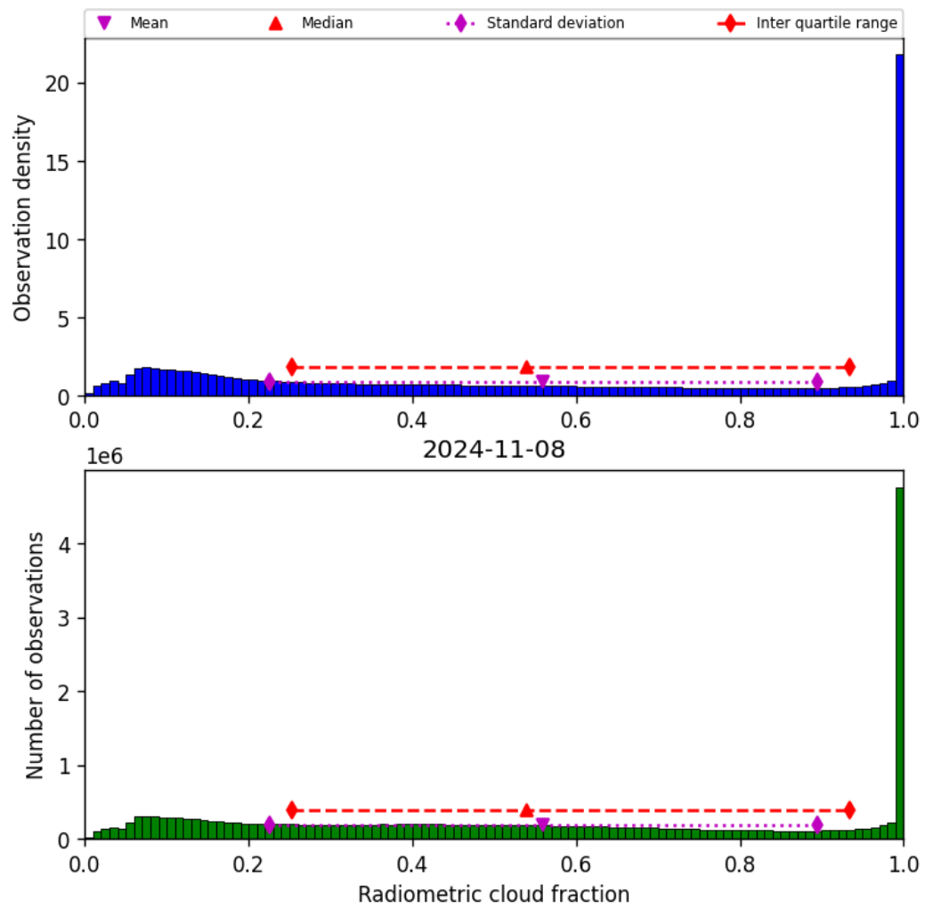
Figure 39: Histogram of “Radiometric cloud fraction” for 2024-11-07 to 2024-11-09
