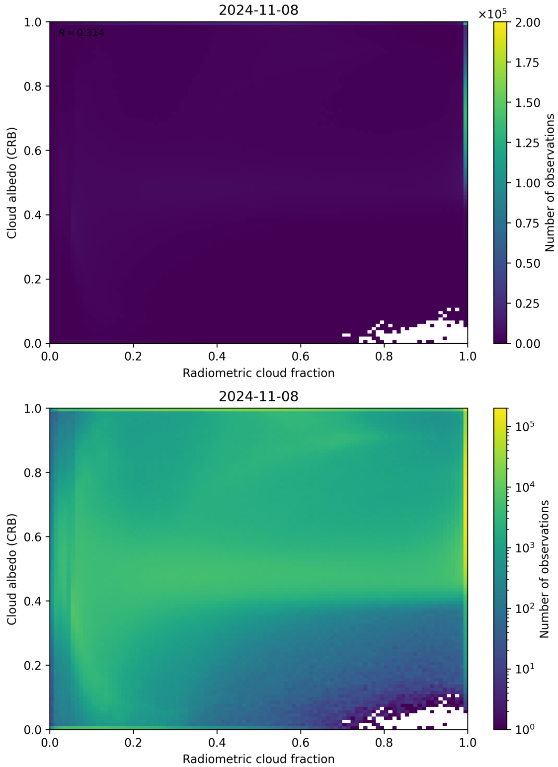
Figure 71: Scatter density plot of “Radiometric cloud fraction” against “Cloud albedo (CRB)” for 2024-11-07 to 2024-11-09.
