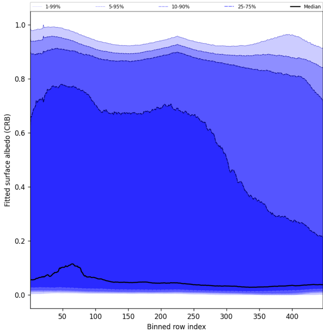
Figure 62: Along track statistics of “Fitted surface albedo (CRB)” for 2024-11-07 to 2024-11-09
