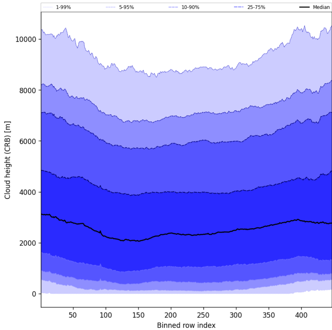
Figure 59: Along track statistics of “Cloud height (CRB)” for 2024-11-07 to 2024-11-09
