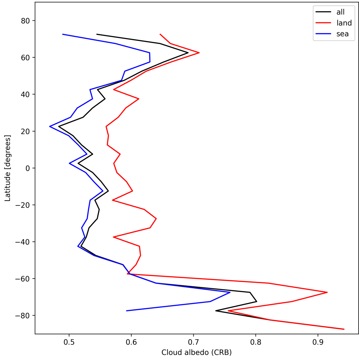
Figure 28: Zonal average of “Cloud albedo (CRB)” for 2024-11-07 to 2024-11-09.
