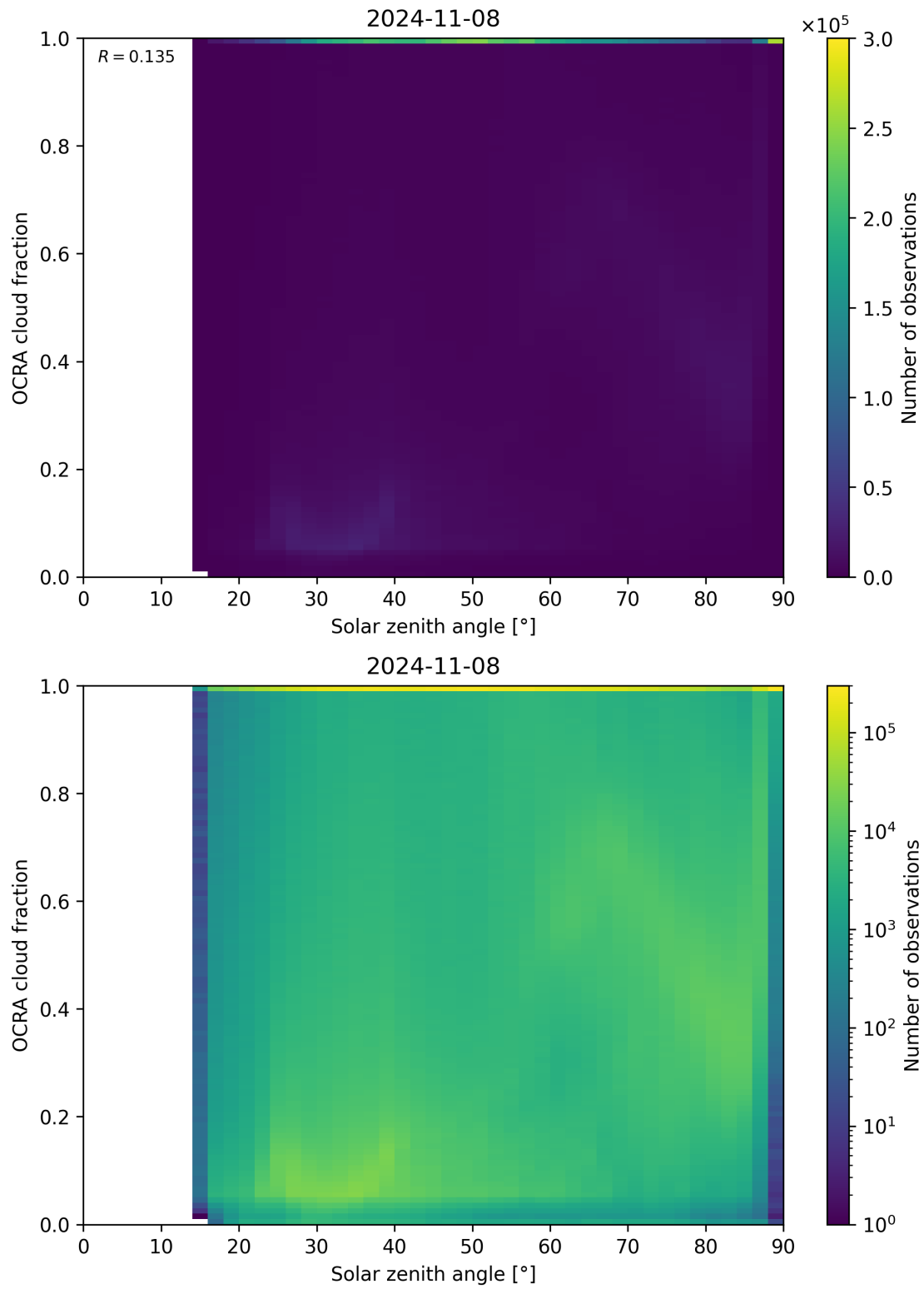
Figure 100: Scatter density plot of “Solar zenith angle” against “OCRA cloud fraction” for 2024-11-07 to 2024-11-09.
