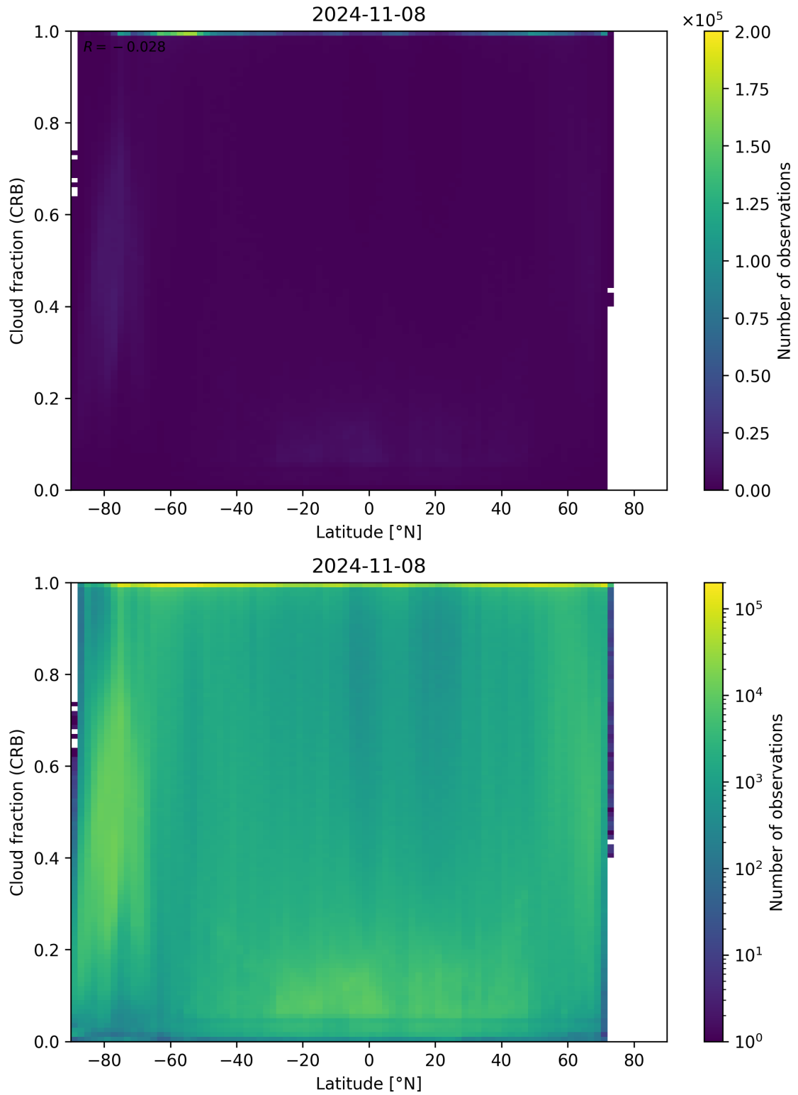
Figure 94: Scatter density plot of “Latitude” against “Cloud fraction (CRB)” for 2024-11-07 to 2024-11-09.
