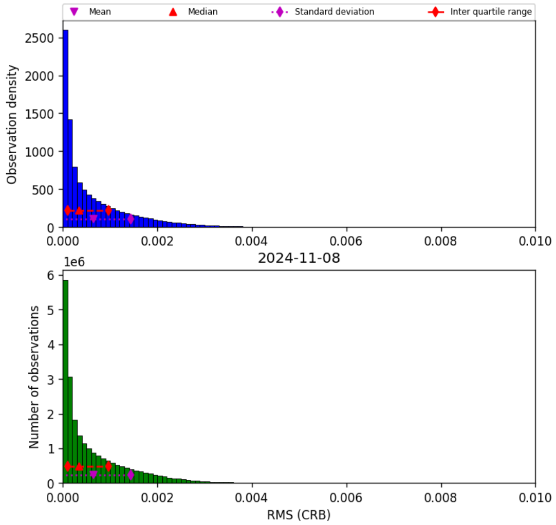
Figure 48: Histogram of “RMS (CRB)” for 2024-11-07 to 2024-11-09
