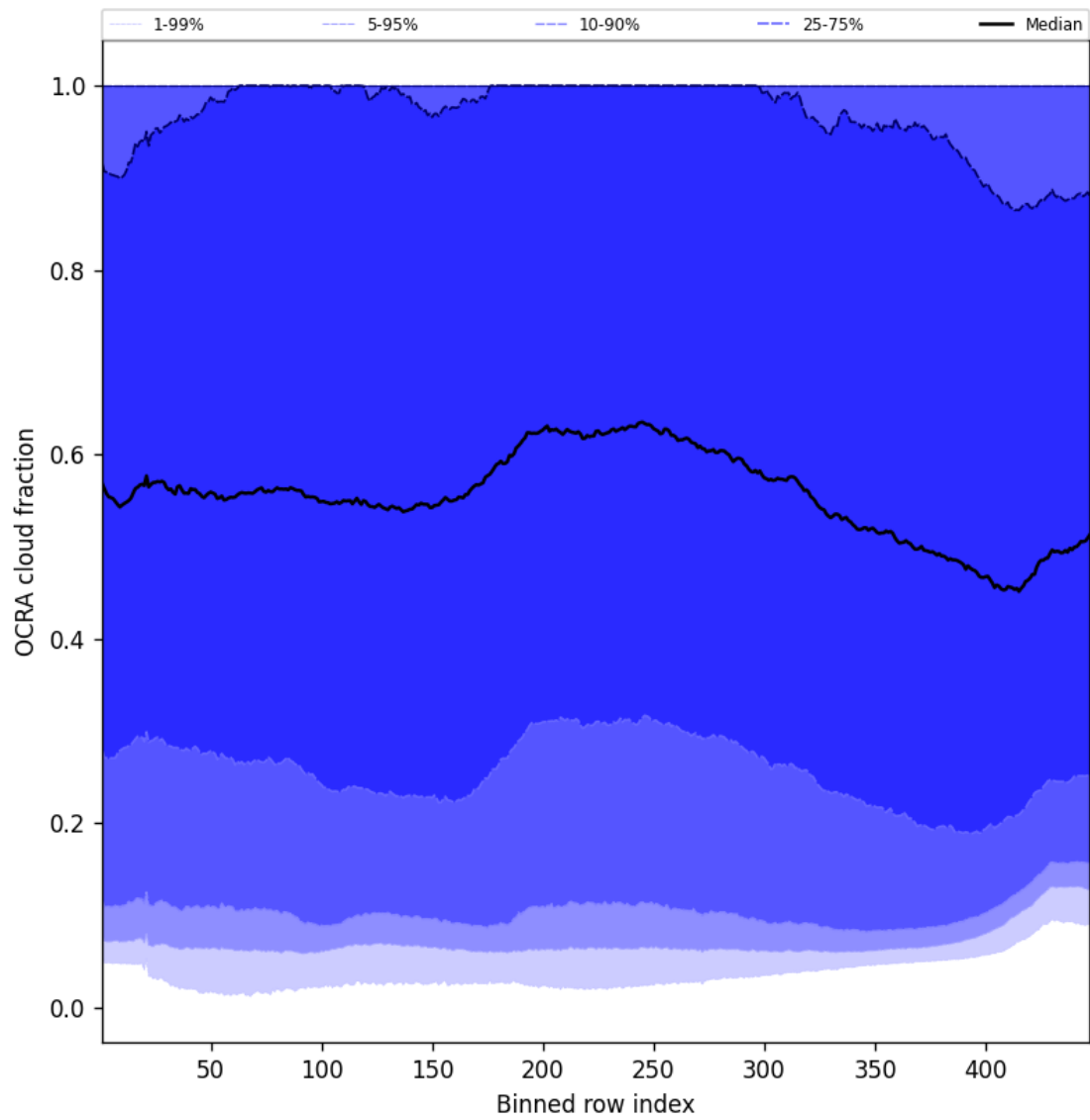
Figure 66: Along track statistics of “OCRA cloud fraction” for 2024-11-07 to 2024-11-09
