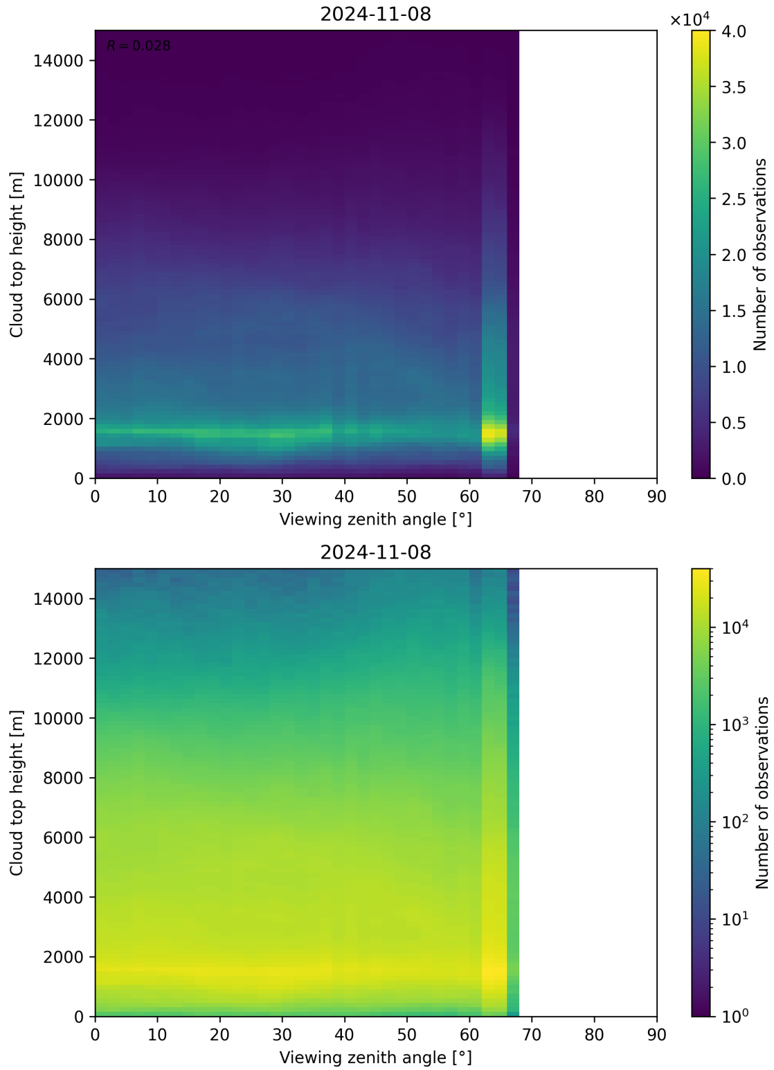
Figure 112: Scatter density plot of “Viewing zenith angle” against “Cloud top height” for 2024-11-07 to 2024-11-09.
