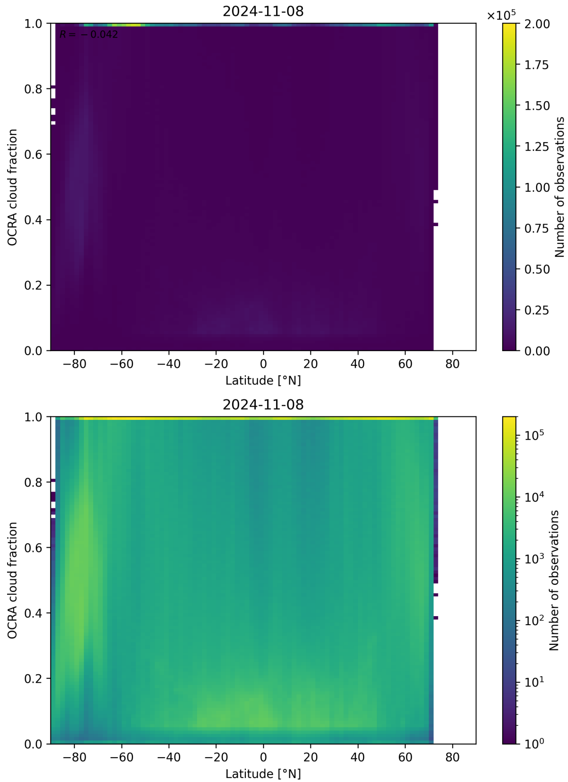
Figure 93: Scatter density plot of “Latitude” against “OCRA cloud fraction” for 2024-11-07 to 2024-11-09.
