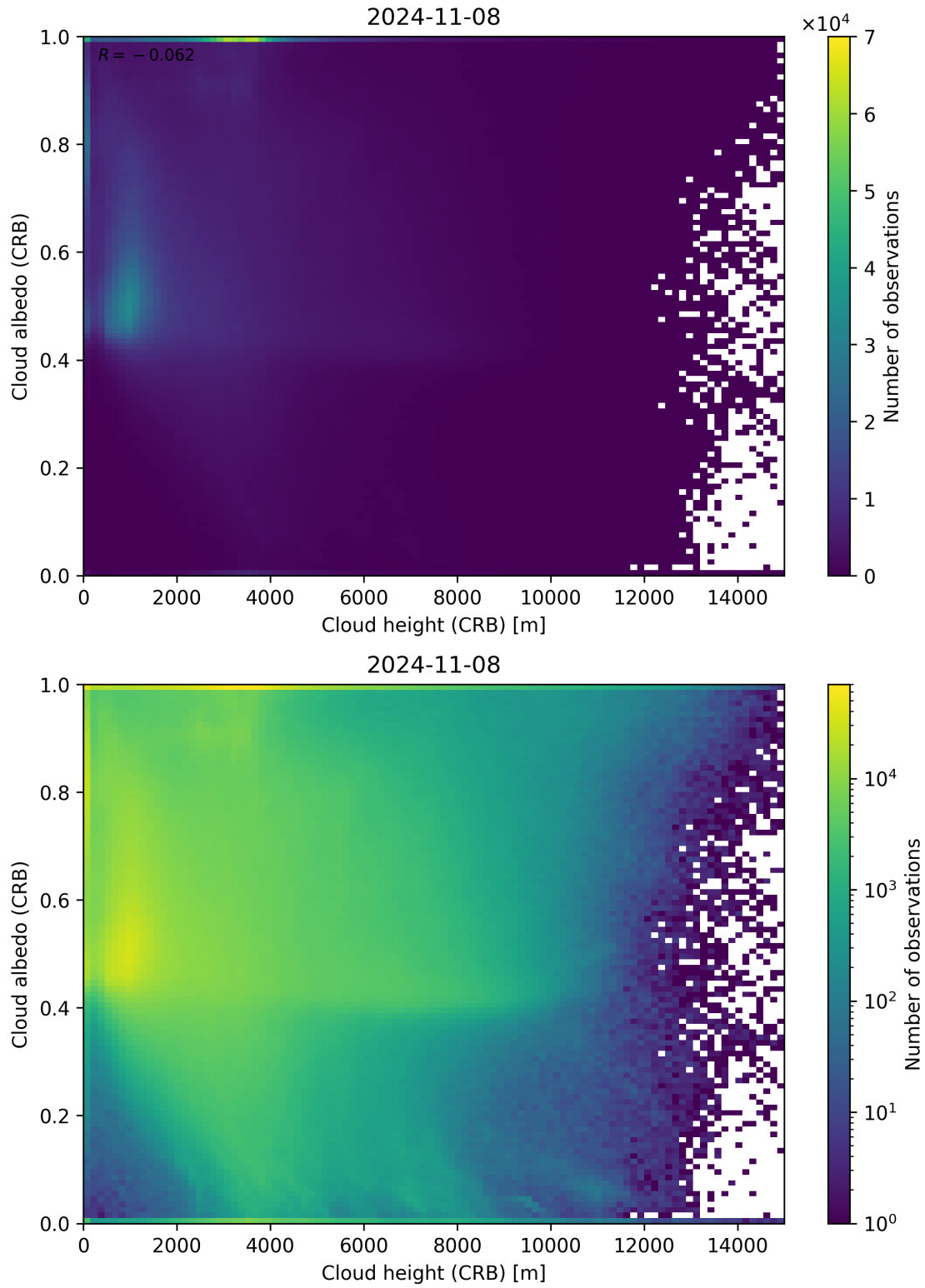
Figure 80: Scatter density plot of “Cloud height (CRB)” against “Cloud albedo (CRB)” for 2024-11-07 to 2024-11-09.
