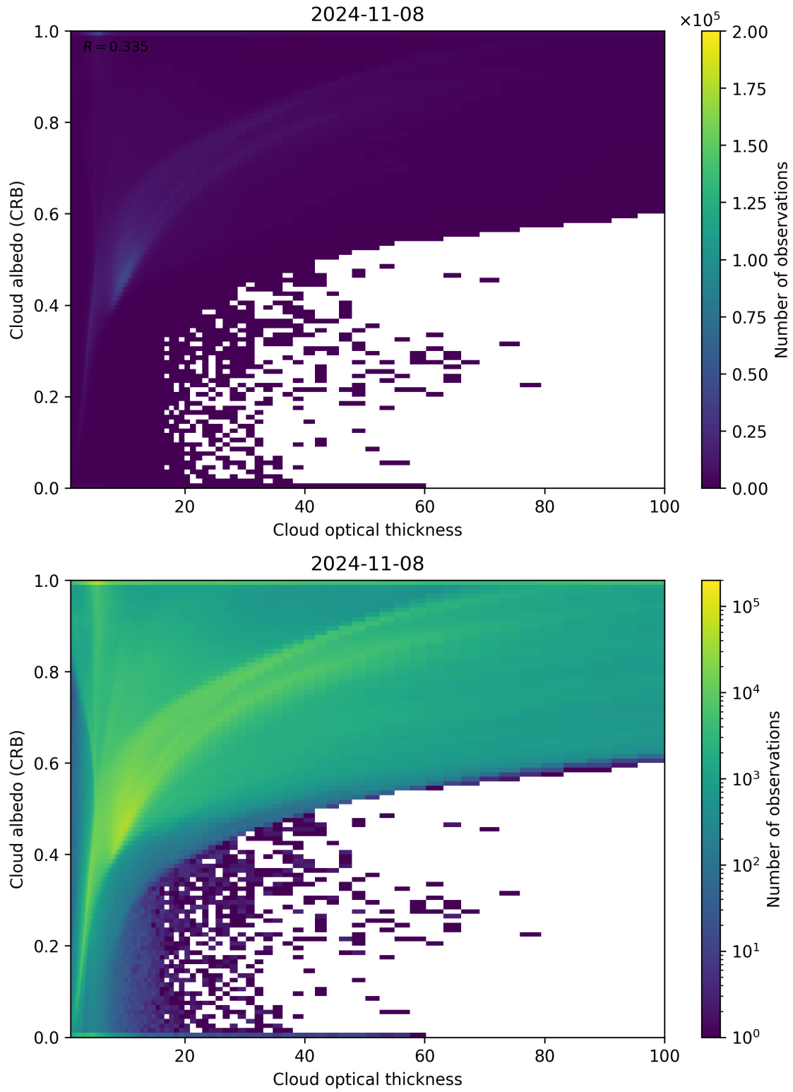
Figure 82: Scatter density plot of “Cloud optical thickness” against “Cloud albedo (CRB)” for 2024-11-07 to 2024-11-09.
