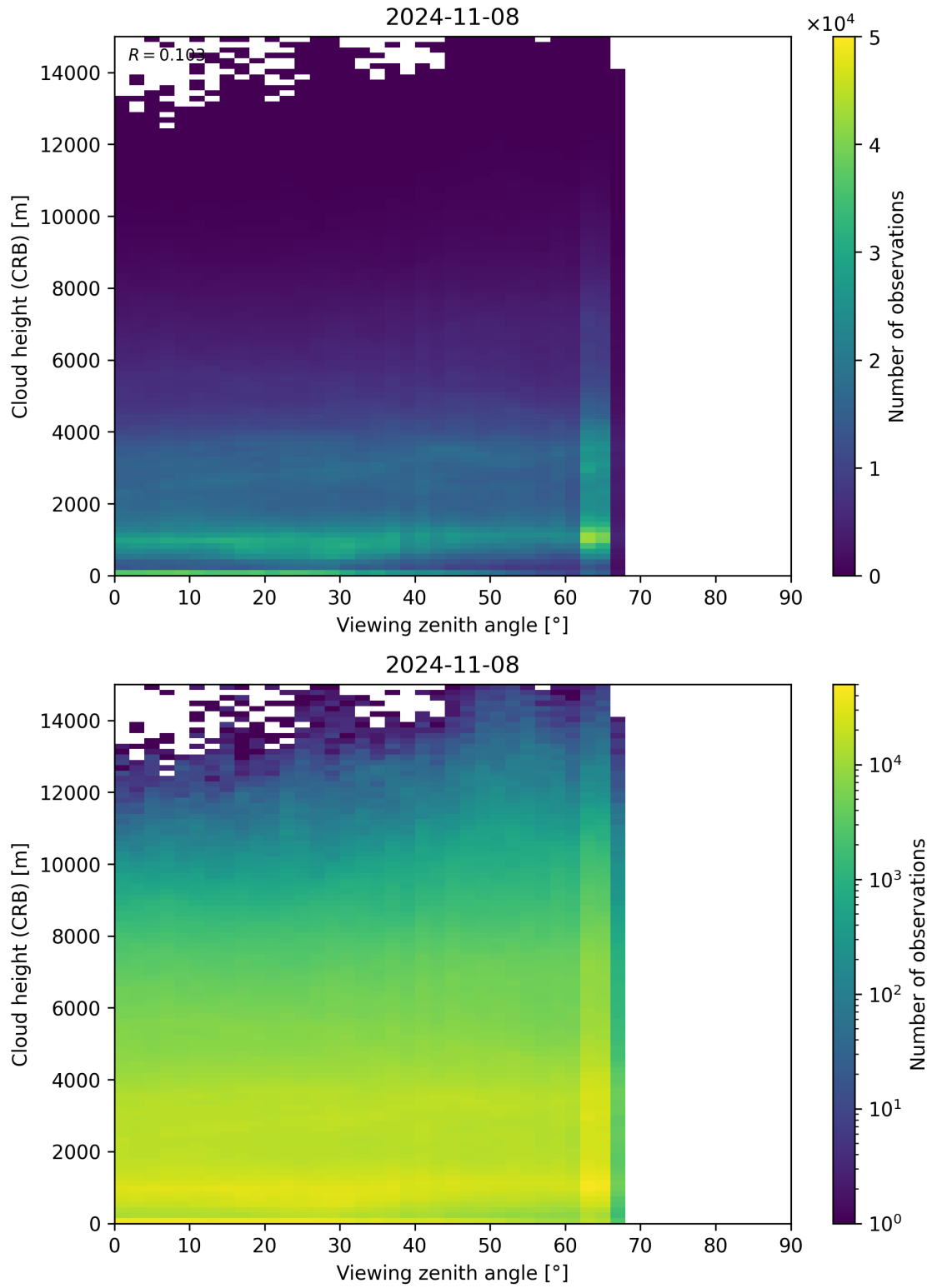
Figure 110: Scatter density plot of “Viewing zenith angle” against “Cloud height (CRB)” for 2024-11-07 to 2024-11-09.
