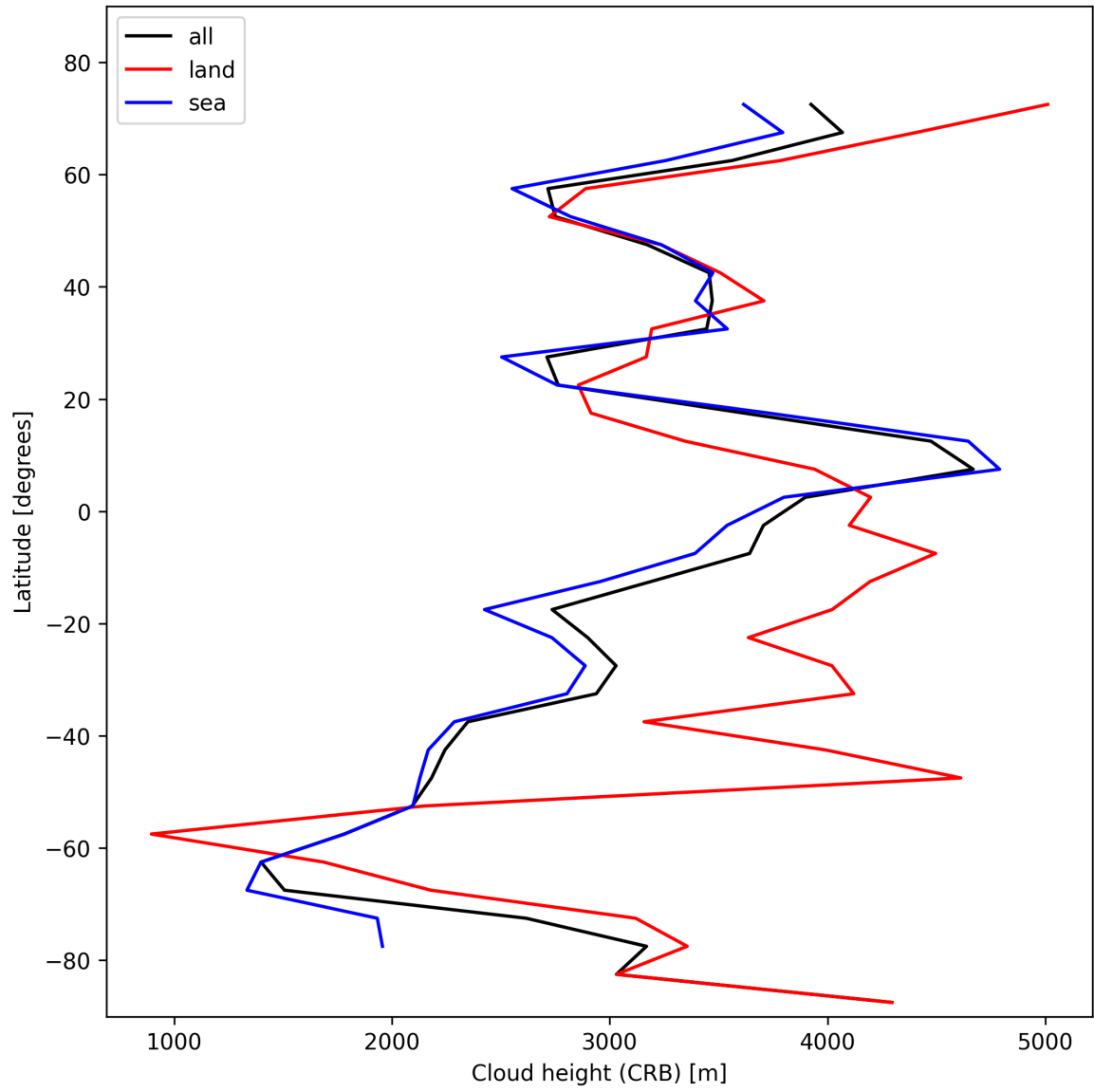
Figure 27: Zonal average of “Cloud height (CRB)” for 2024-11-07 to 2024-11-09.
