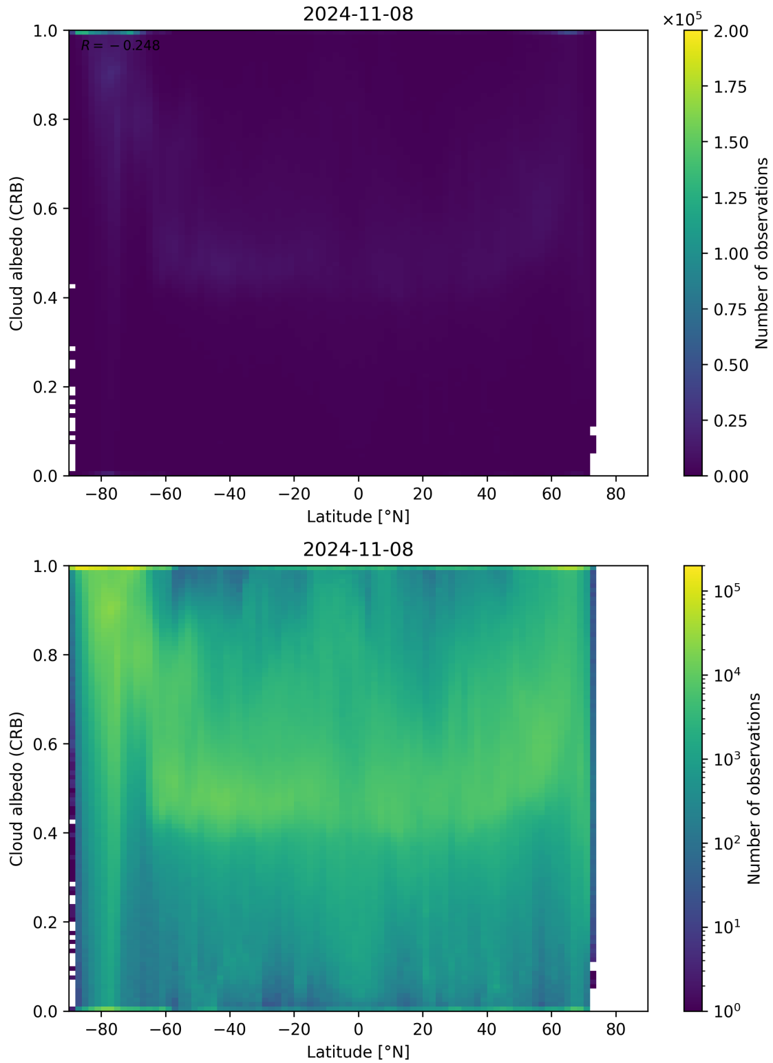
Figure 91: Scatter density plot of “Latitude” against “Cloud albedo (CRB)” for 2024-11-07 to 2024-11-09.
