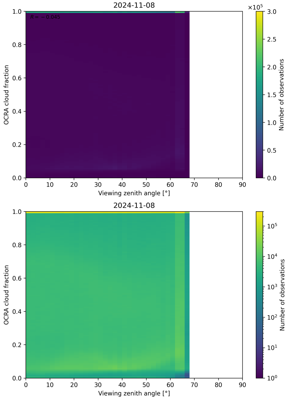
Figure 108: Scatter density plot of “Viewing zenith angle” against “OCRA cloud fraction” for 2024-11-07 to 2024-11-09.
