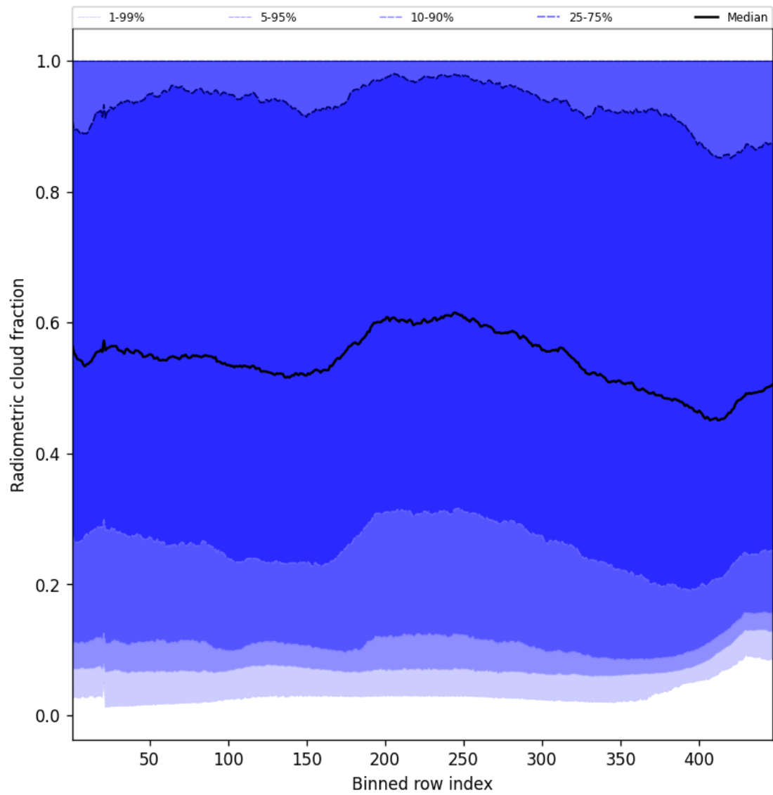
Figure 55: Along track statistics of “Radiometric cloud fraction” for 2024-11-07 to 2024-11-09
