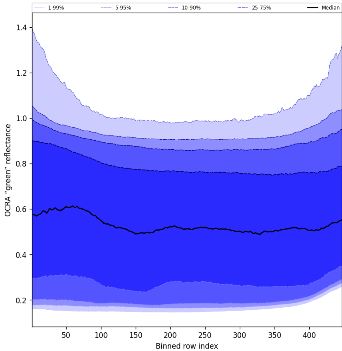
Figure 68: Along track statistics of “OCRA “green” reflectance” for 2024-11-07 to 2024-11-09
