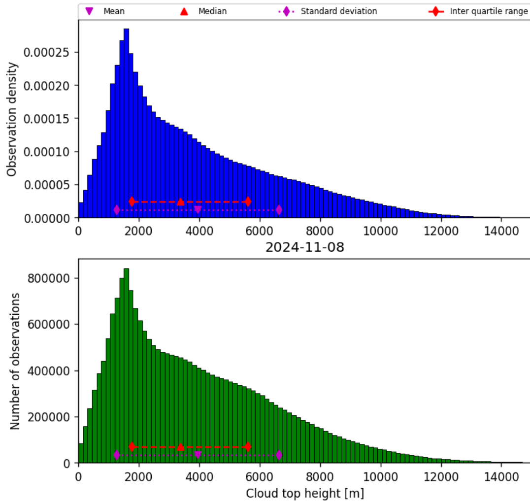
Figure 40: Histogram of “Cloud top height” for 2024-11-07 to 2024-11-09
