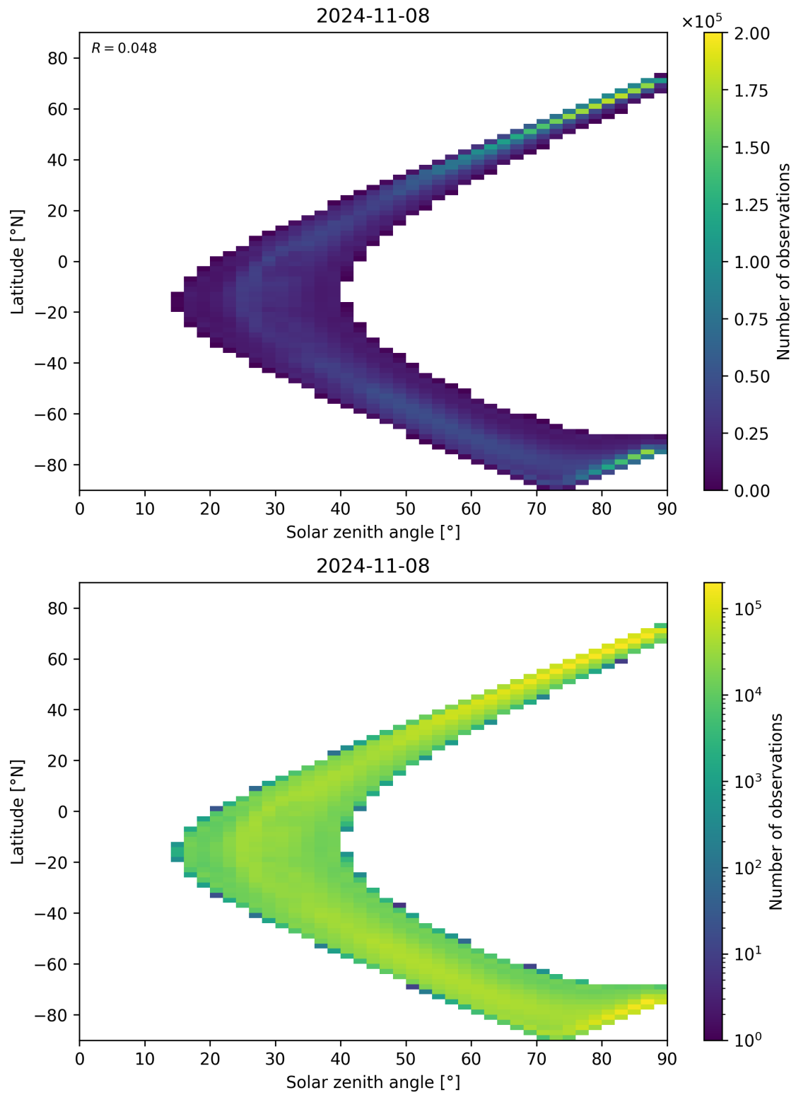
Figure 105: Scatter density plot of “Solar zenith angle” against “Latitude” for 2024-11-07 to 2024-11-09.
