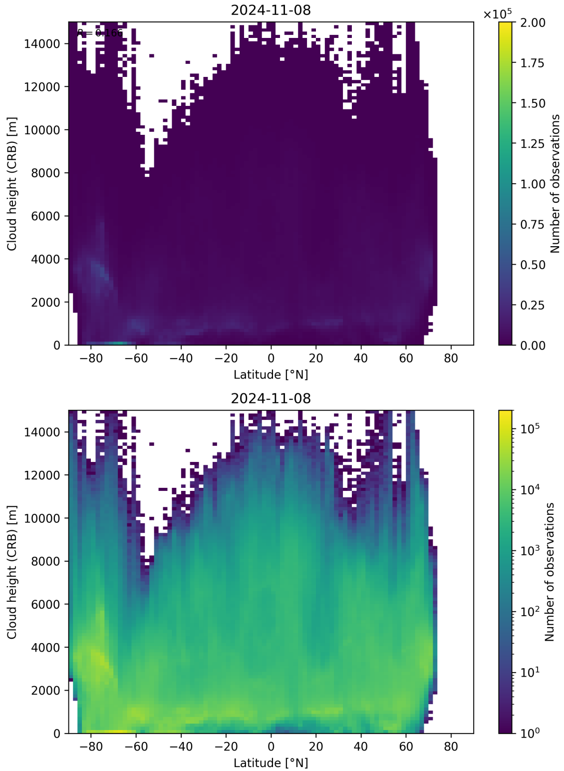
Figure 95: Scatter density plot of “Latitude” against “Cloud height (CRB)” for 2024-11-07 to 2024-11-09.
