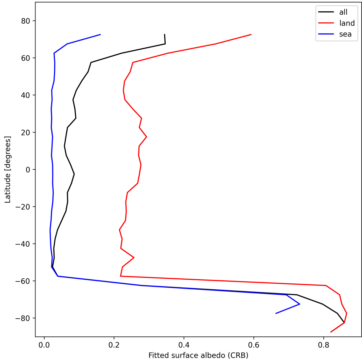
Figure 30: Zonal average of “Fitted surface albedo (CRB)” for 2024-11-07 to 2024-11-09.
