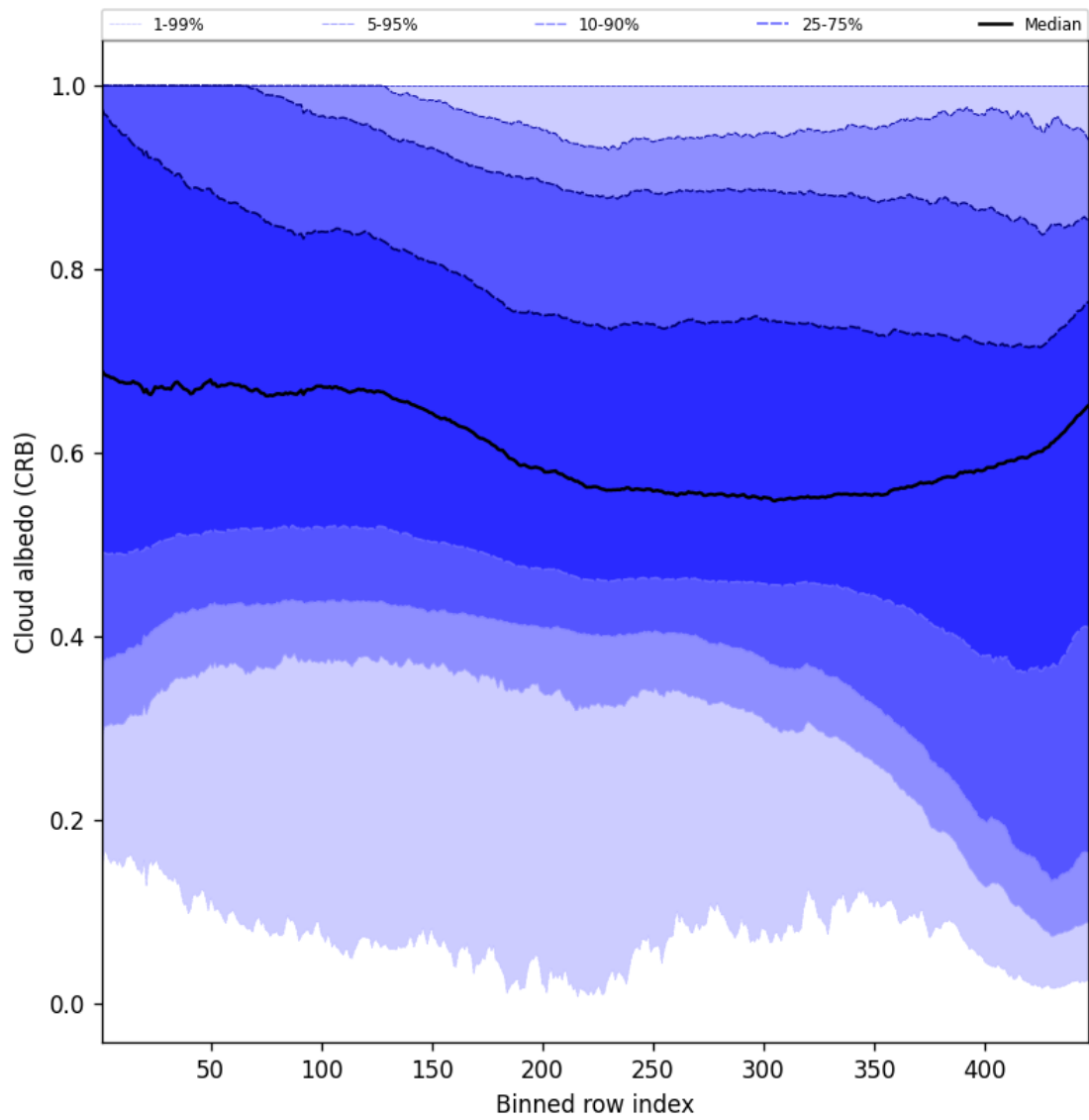
Figure 60: Along track statistics of “Cloud albedo (CRB)” for 2024-11-07 to 2024-11-09
