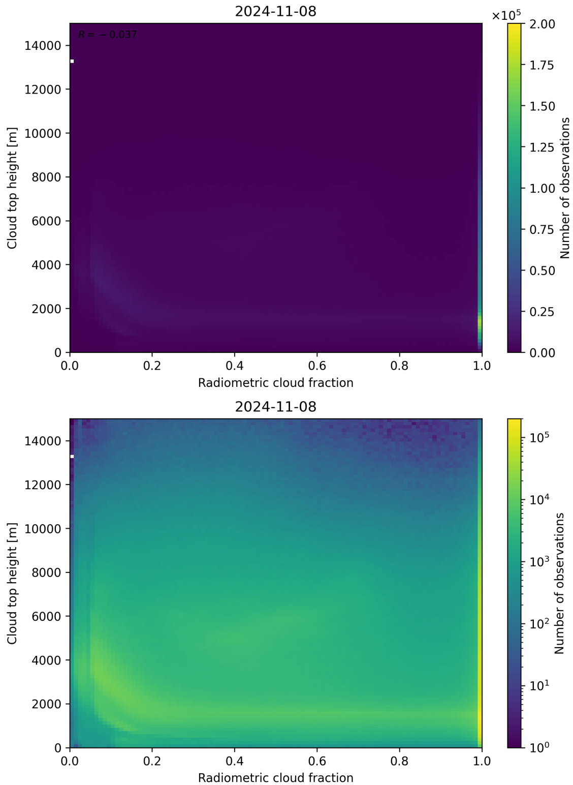
Figure 76: Scatter density plot of “Radiometric cloud fraction” against “Cloud top height” for 2024-11-07 to 2024-11-09.
