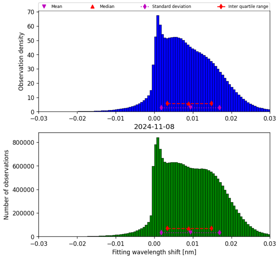
Figure 49: Histogram of “Fitting wavelength shift” for 2024-11-07 to 2024-11-09
