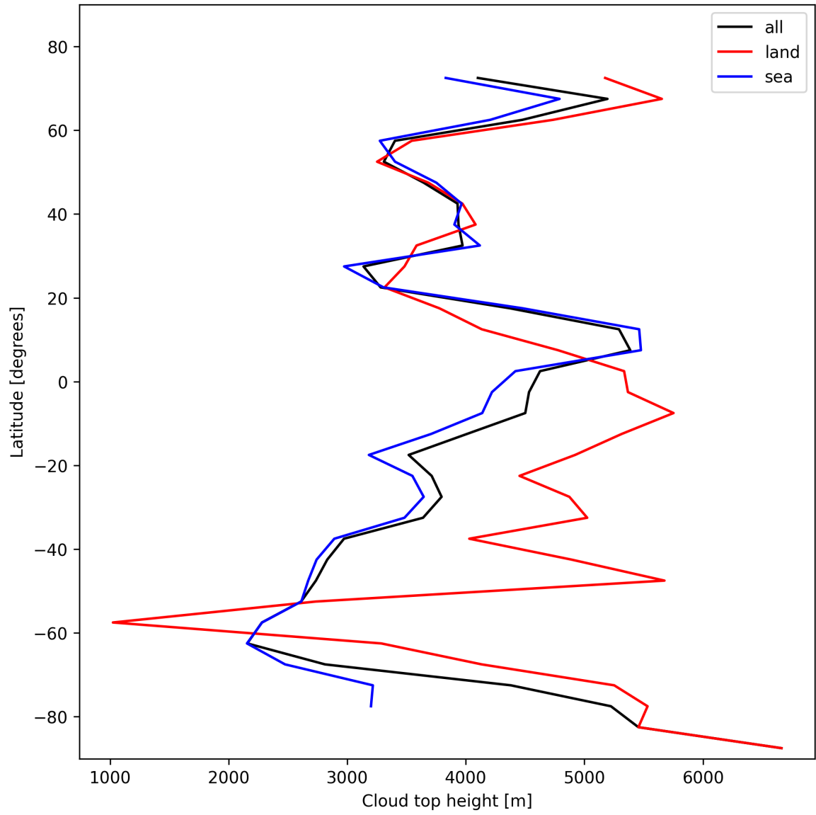
Figure 24: Zonal average of “Cloud top height” for 2024-11-07 to 2024-11-09.
