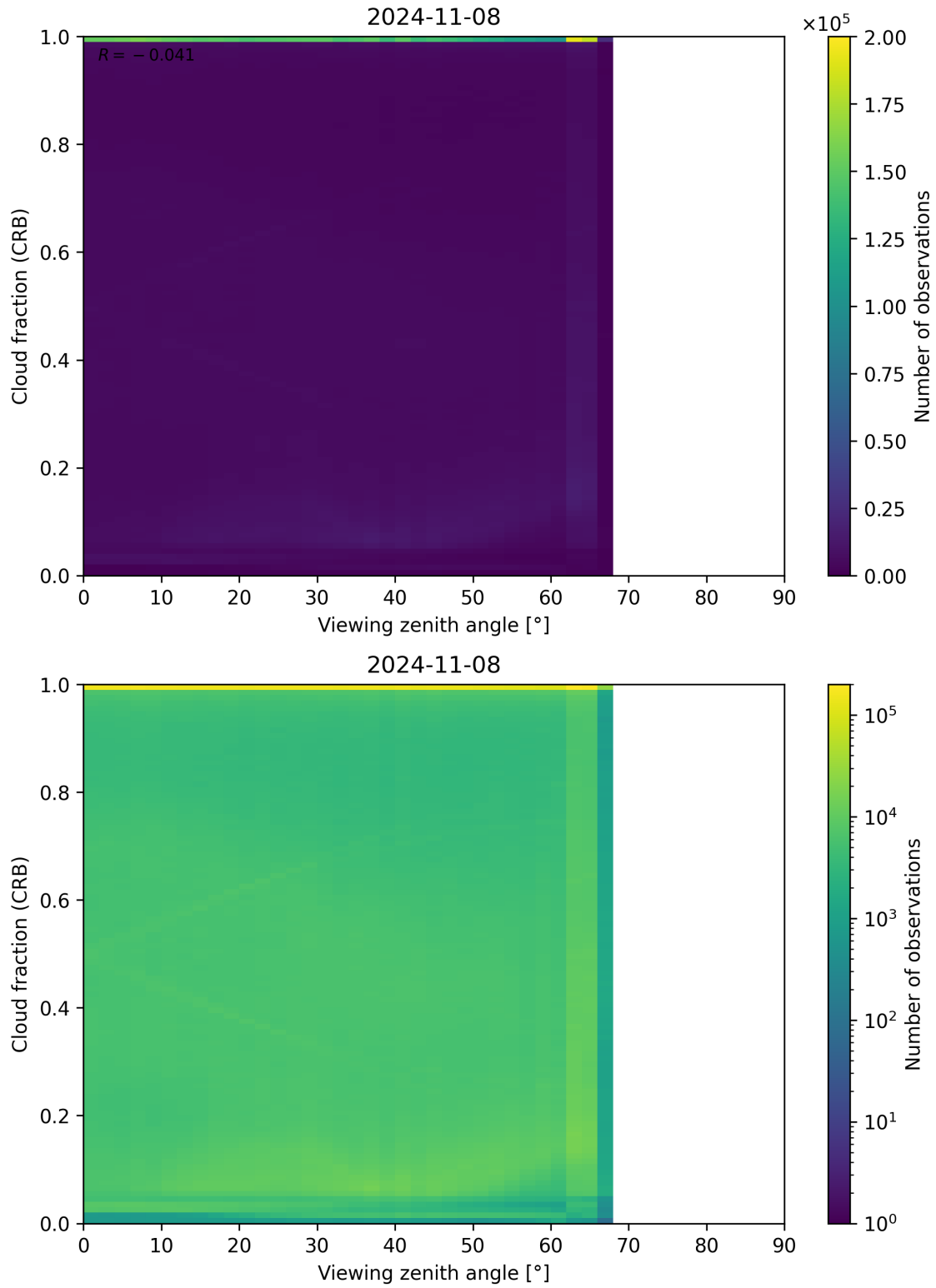
Figure 109: Scatter density plot of “Viewing zenith angle” against “Cloud fraction (CRB)” for 2024-11-07 to 2024-11-09.
