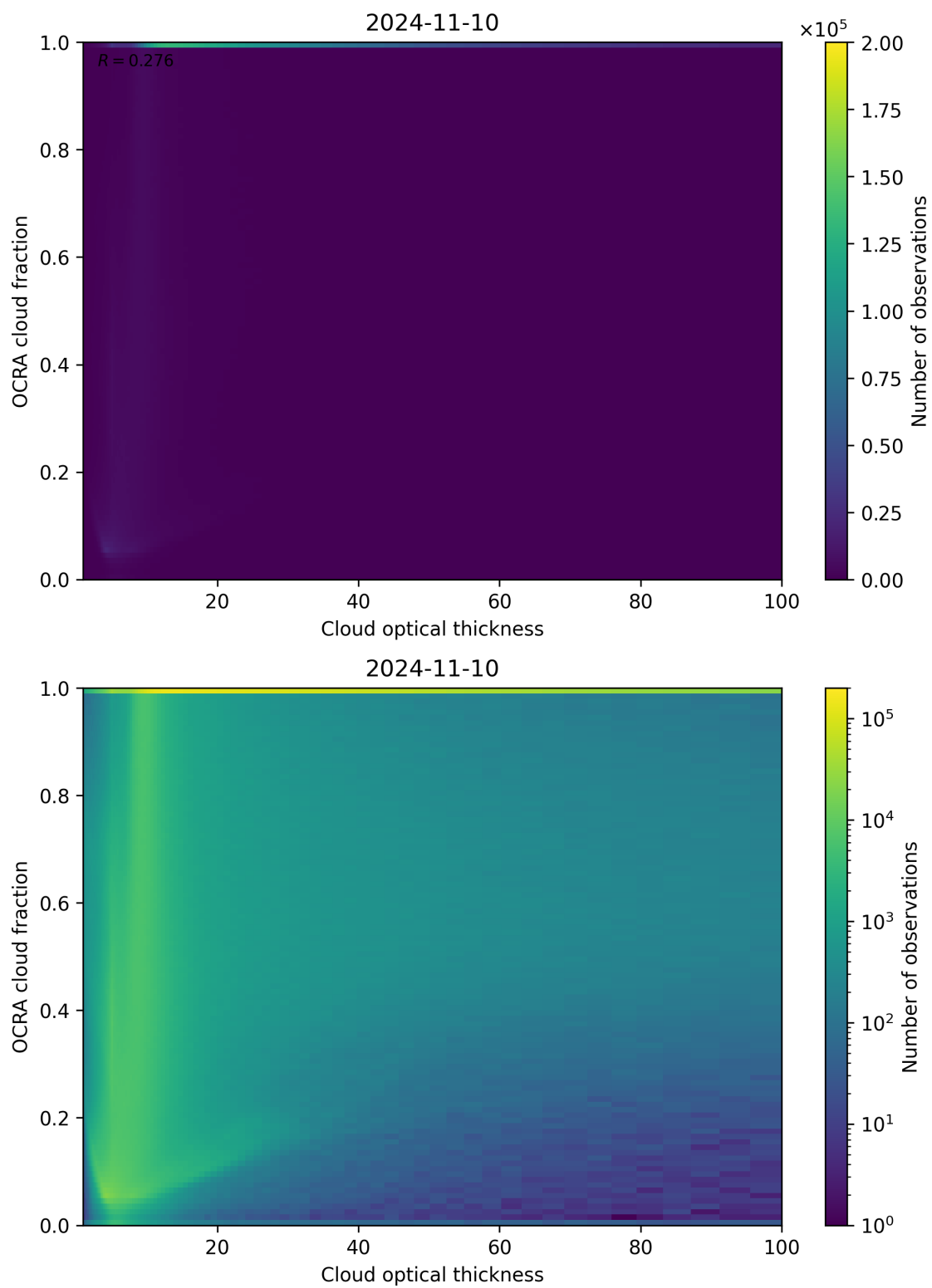
Figure 83: Scatter density plot of “Cloud optical thickness” against “OCRA cloud fraction” for 2024-11-09 to 2024-11-11.
