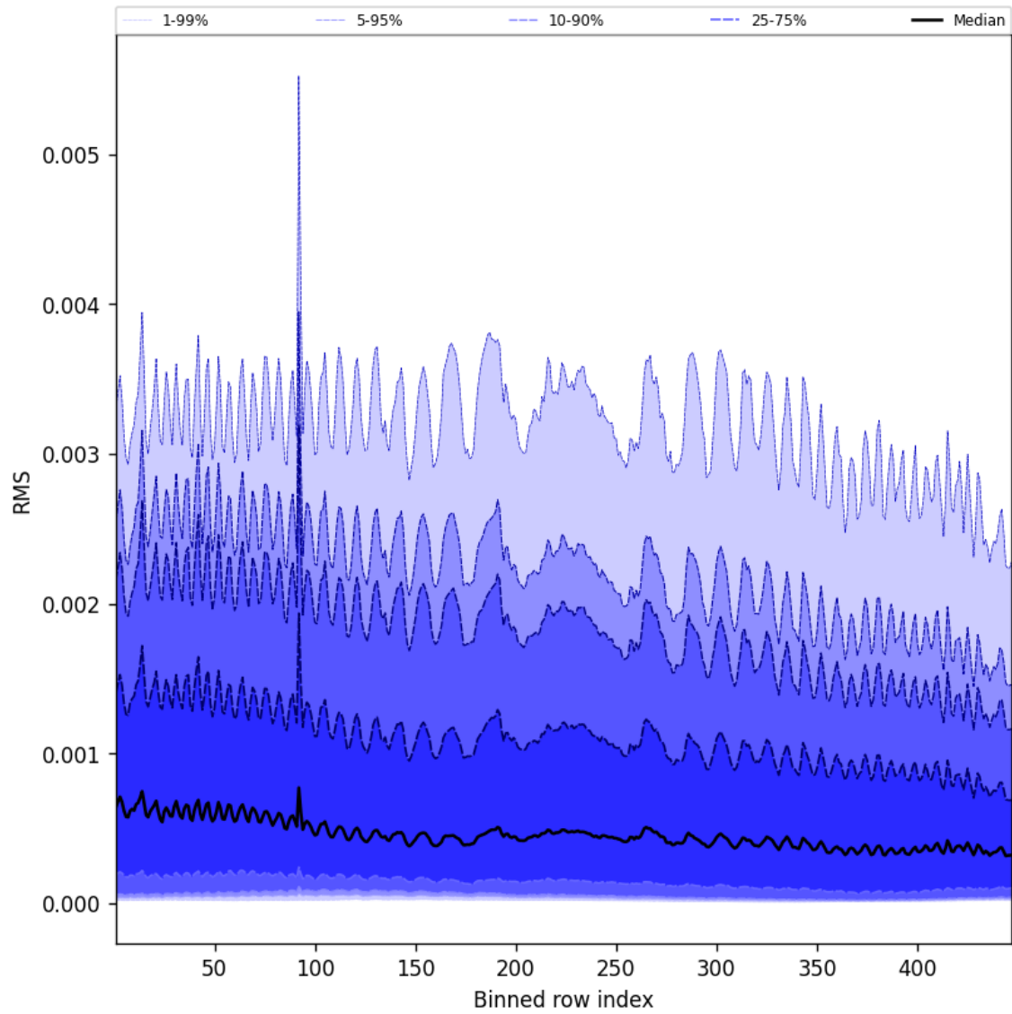
Figure 63: Along track statistics of “RMS” for 2024-11-09 to 2024-11-11
