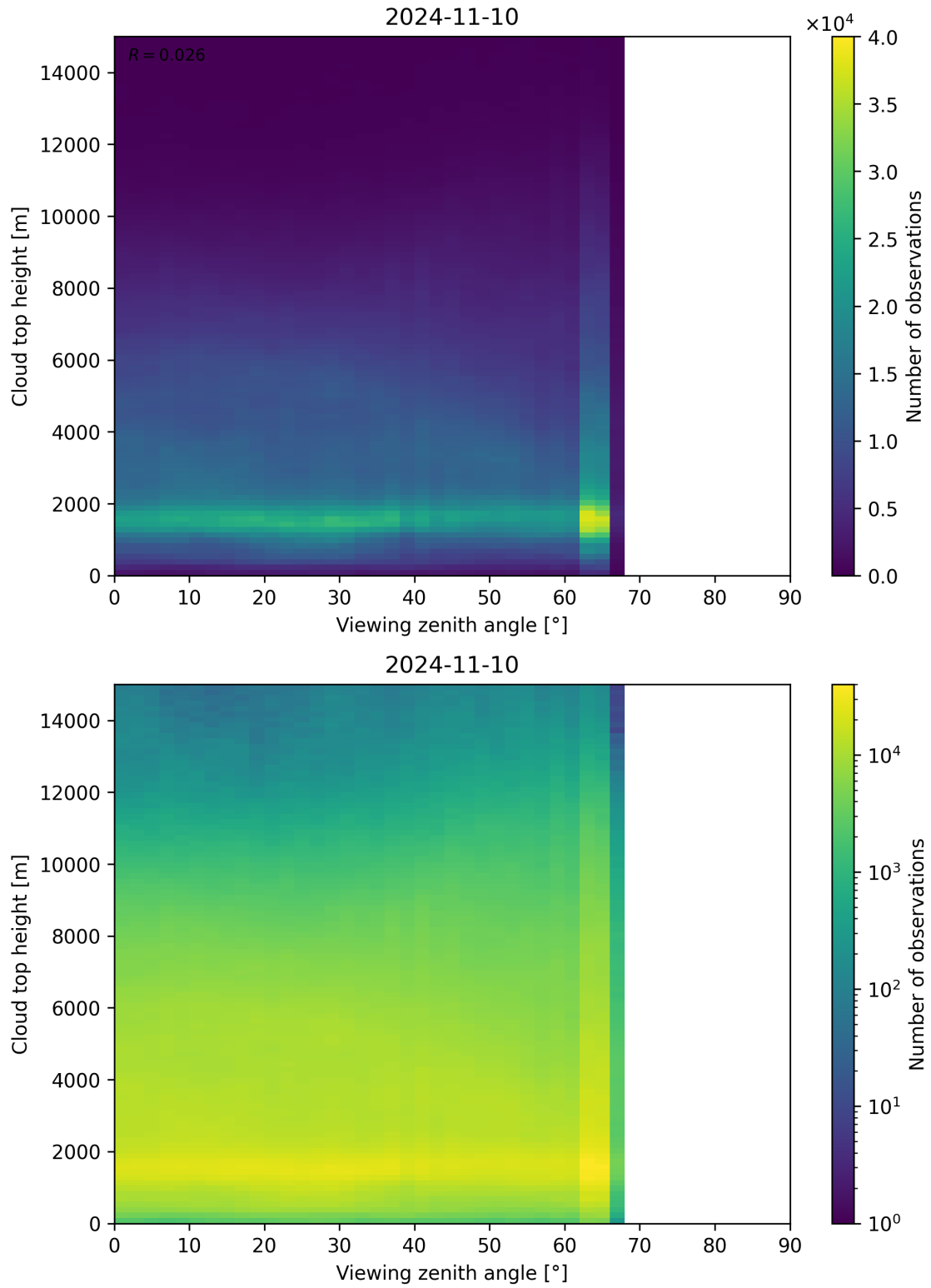
Figure 112: Scatter density plot of “Viewing zenith angle” against “Cloud top height” for 2024-11-09 to 2024-11-11.
