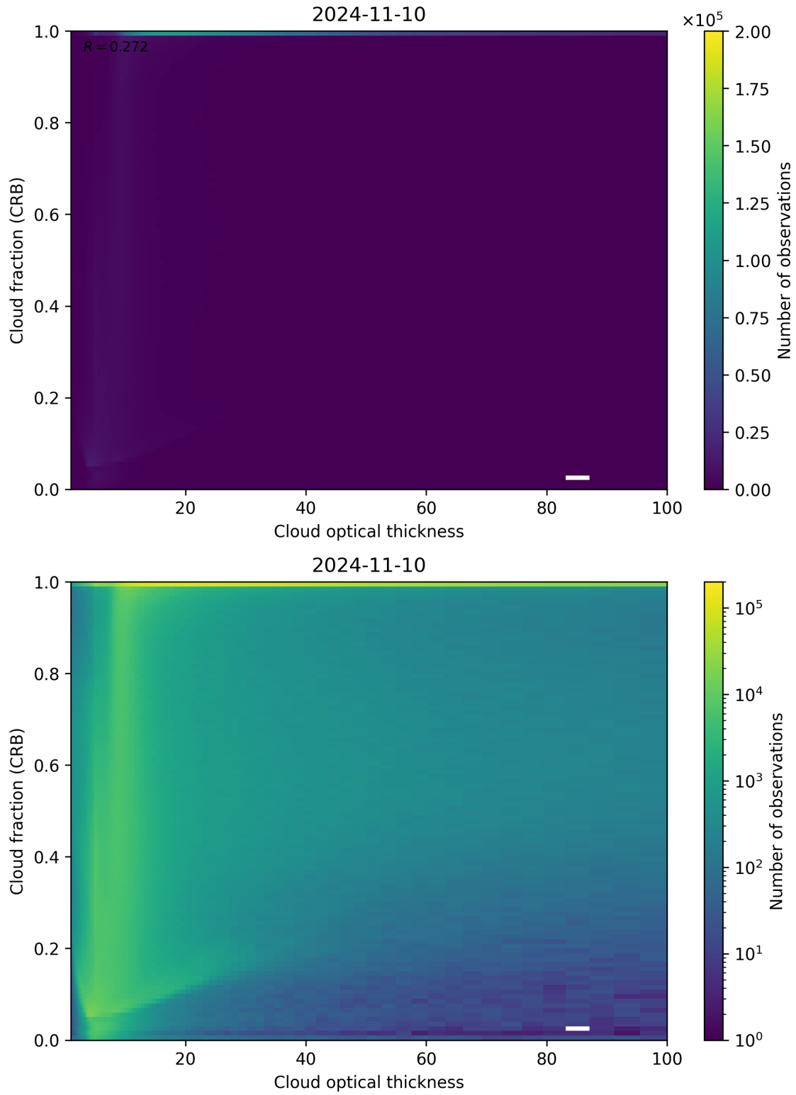
Figure 84: Scatter density plot of “Cloud optical thickness” against “Cloud fraction (CRB)” for 2024-11-09 to 2024-11-11.
