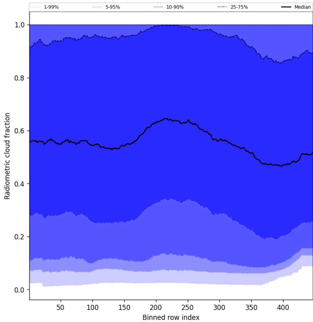
Figure 55: Along track statistics of “Radiometric cloud fraction” for 2024-11-09 to 2024-11-11
