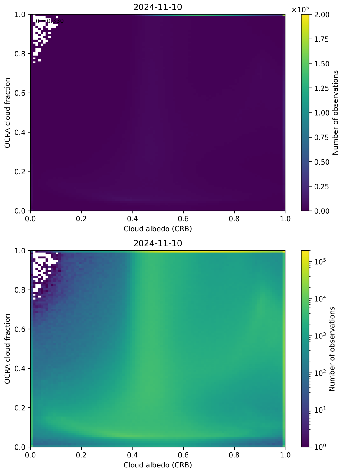
Figure 70: Scatter density plot of “Cloud albedo (CRB)” against “OCRA cloud fraction” for 2024-11-09 to 2024-11-11.
