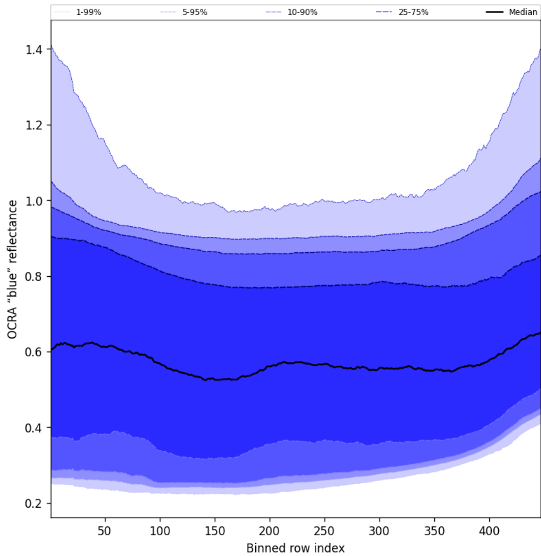
Figure 67: Along track statistics of “OCRA “blue” reflectance” for 2024-11-09 to 2024-11-11
