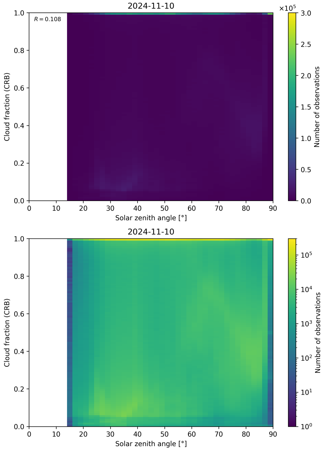
Figure 101: Scatter density plot of “Solar zenith angle” against “Cloud fraction (CRB)” for 2024-11-09 to 2024-11-11.
