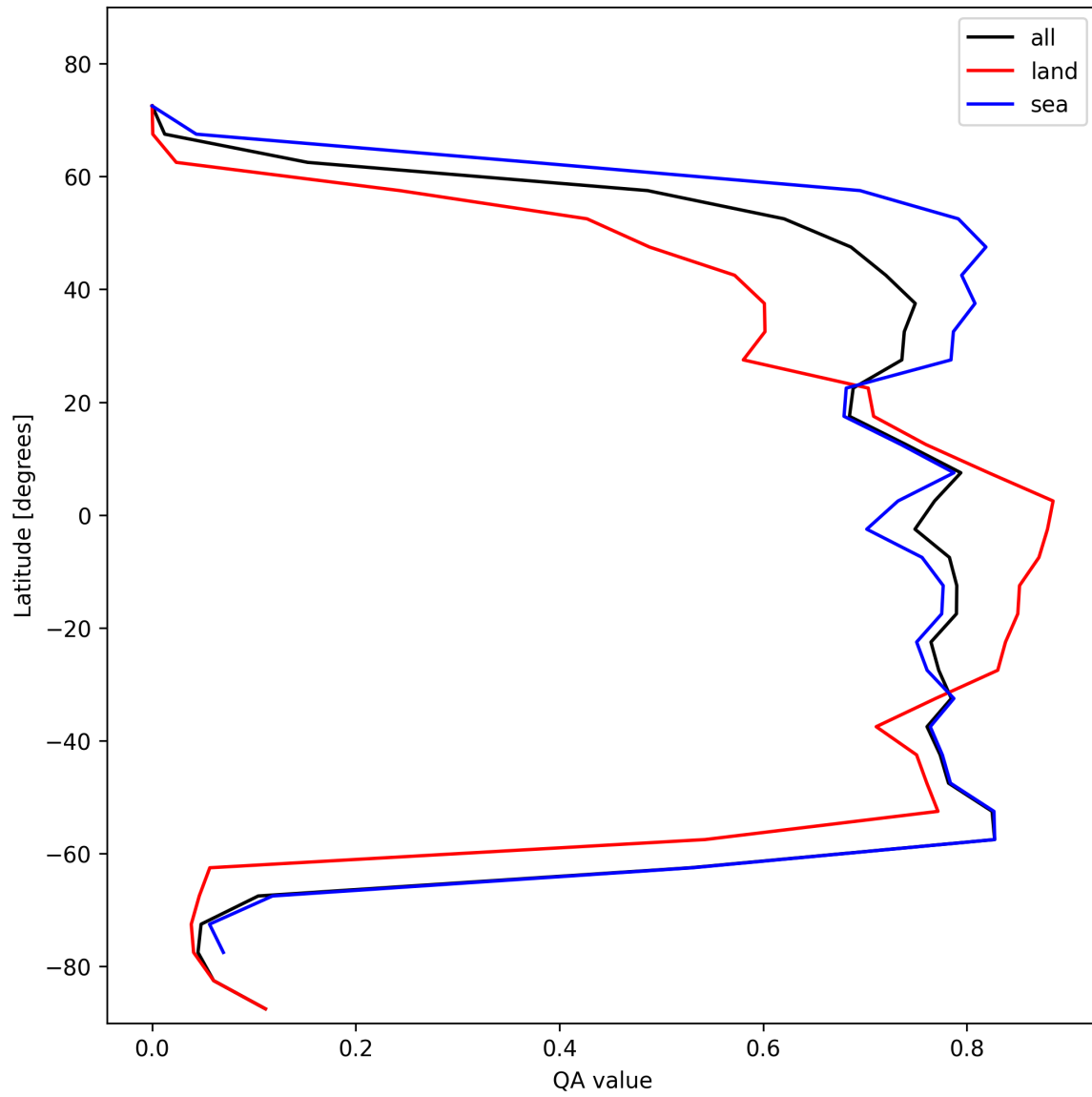
Figure 22: Zonal average of “QA value” for 2024-11-09 to 2024-11-11.
