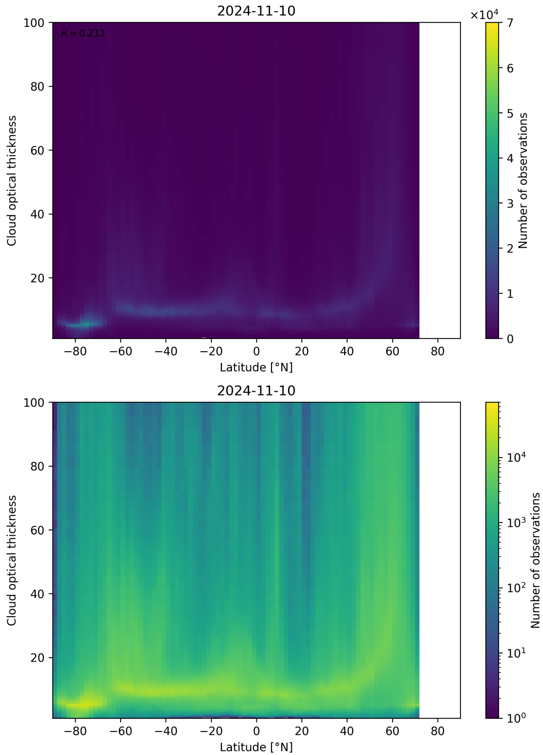
Figure 96: Scatter density plot of “Latitude” against “Cloud optical thickness” for 2024-11-09 to 2024-11-11.
