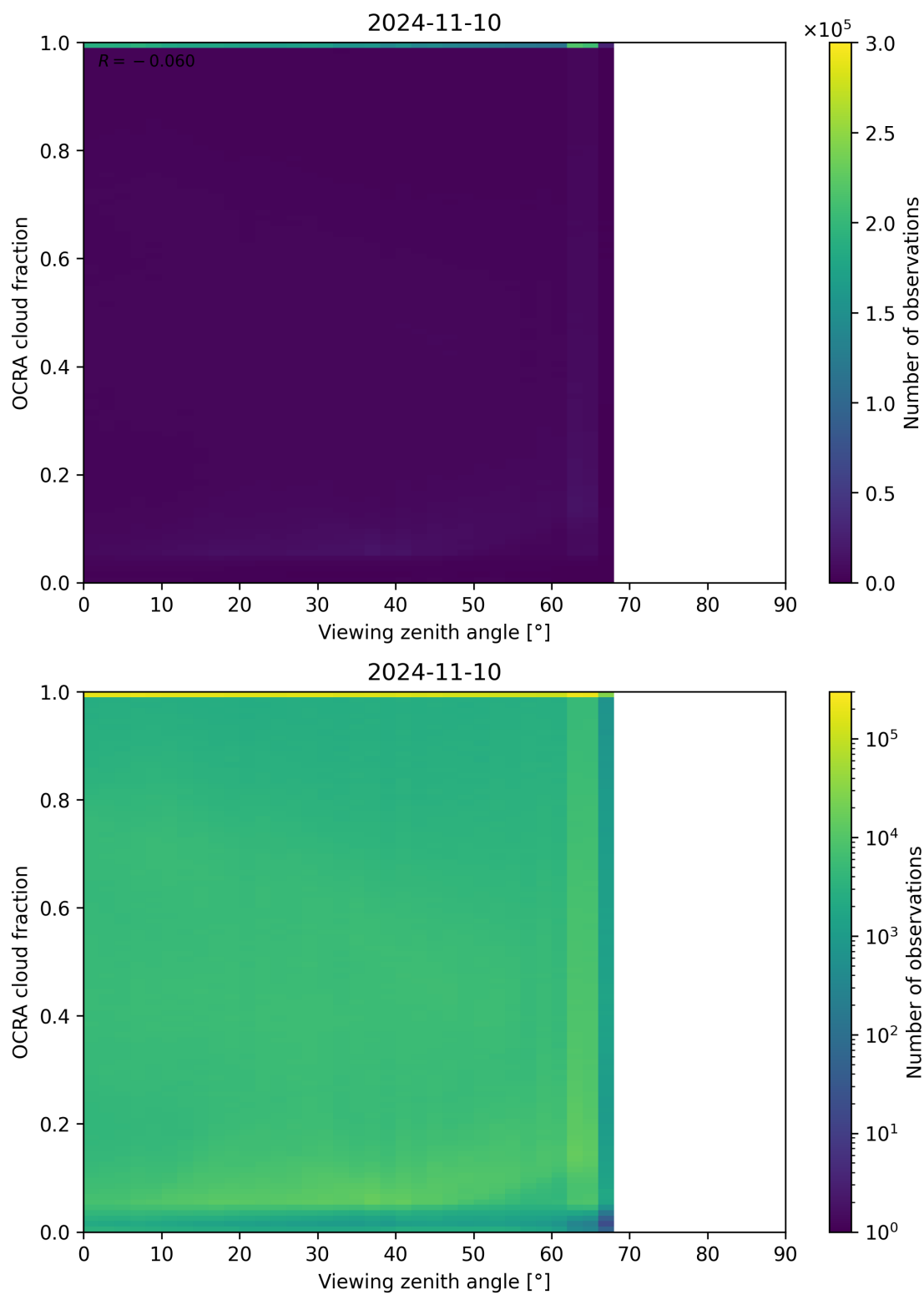
Figure 108: Scatter density plot of “Viewing zenith angle” against “OCRA cloud fraction” for 2024-11-09 to 2024-11-11.
