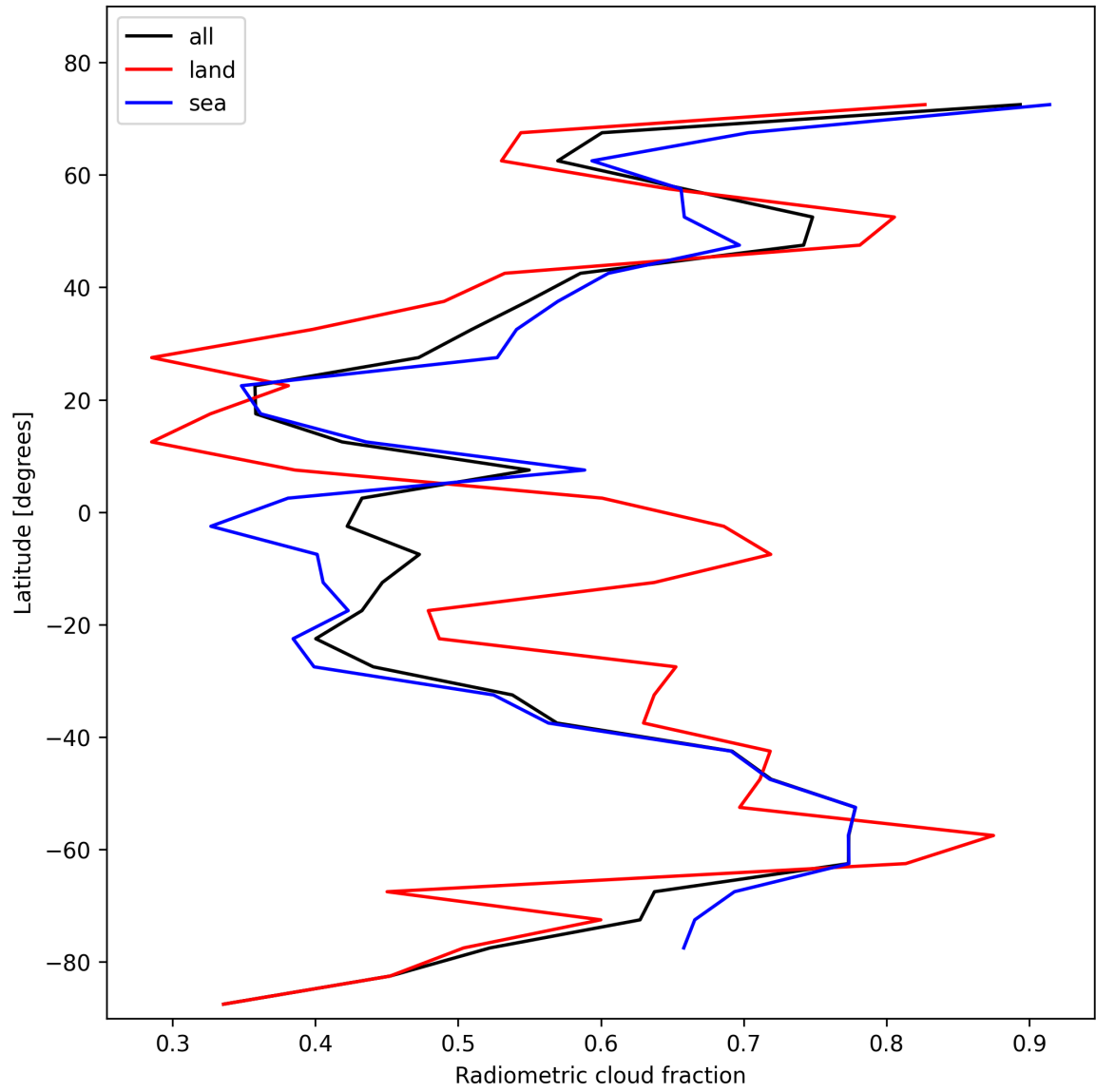
Figure 23: Zonal average of “Radiometric cloud fraction” for 2024-11-09 to 2024-11-11.
