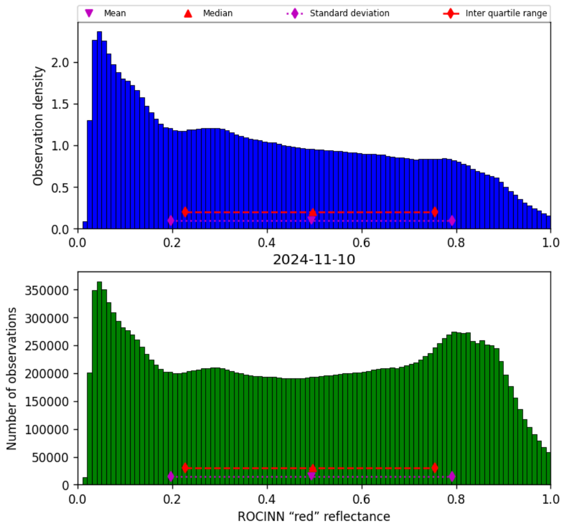
Figure 53: Histogram of “ROCINN “red” reflectance” for 2024-11-09 to 2024-11-11
