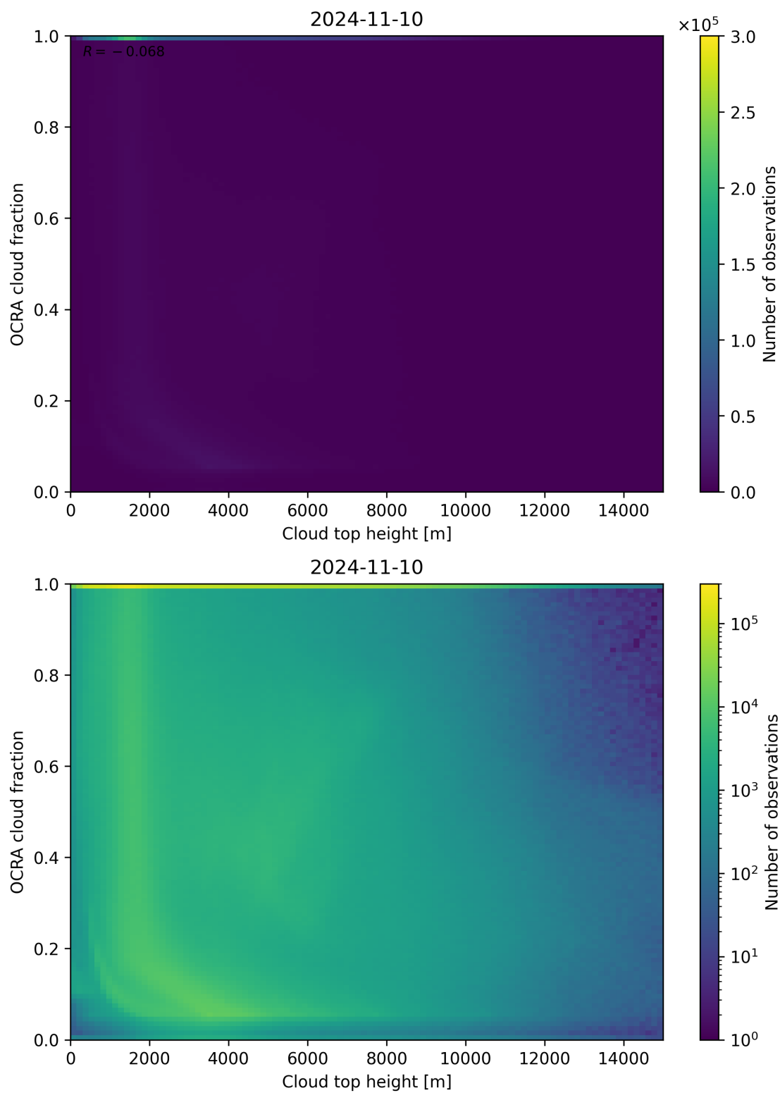
Figure 87: Scatter density plot of “Cloud top height” against “OCRA cloud fraction” for 2024-11-09 to 2024-11-11.
