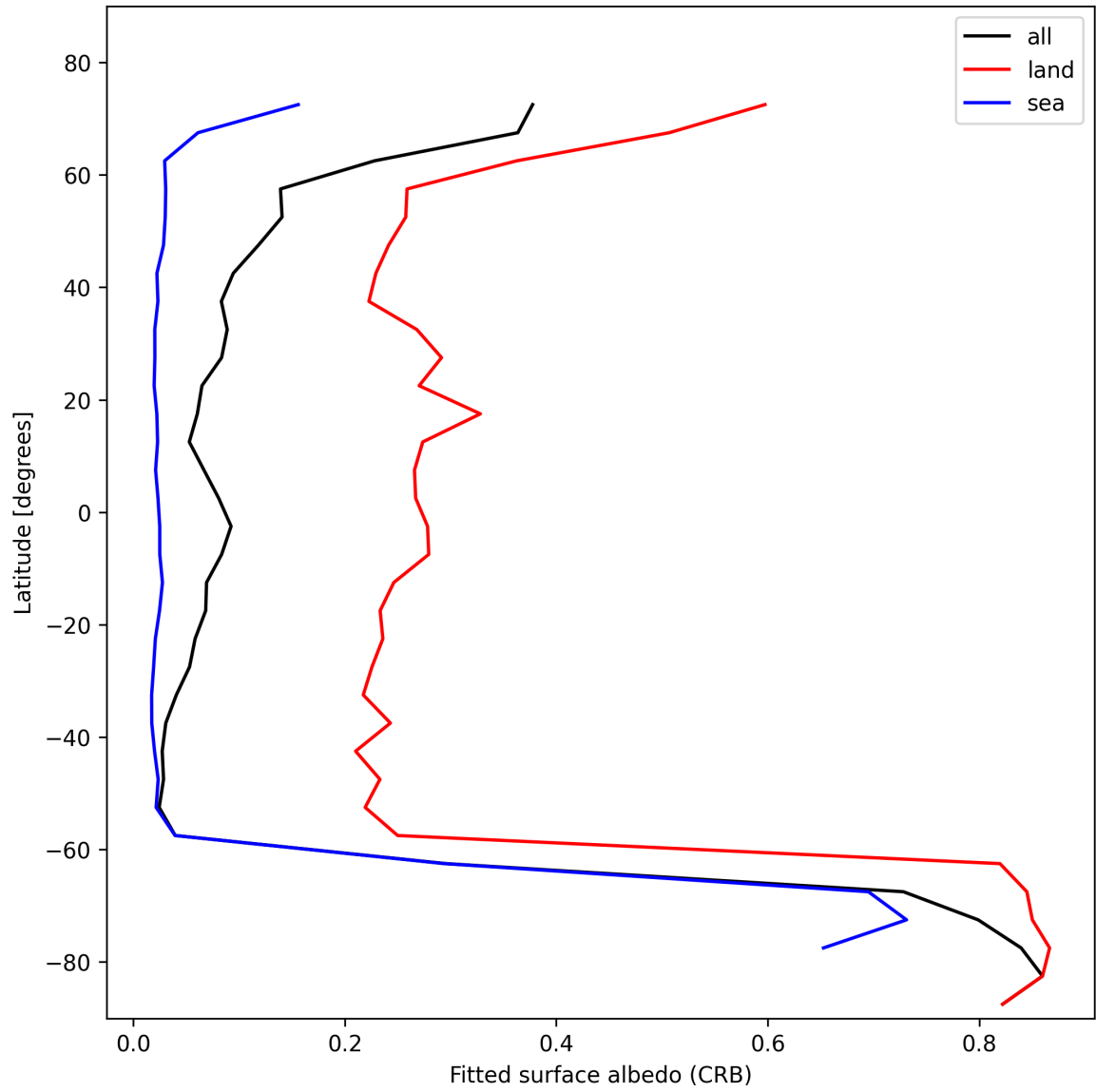
Figure 30: Zonal average of “Fitted surface albedo (CRB)” for 2024-11-09 to 2024-11-11.
