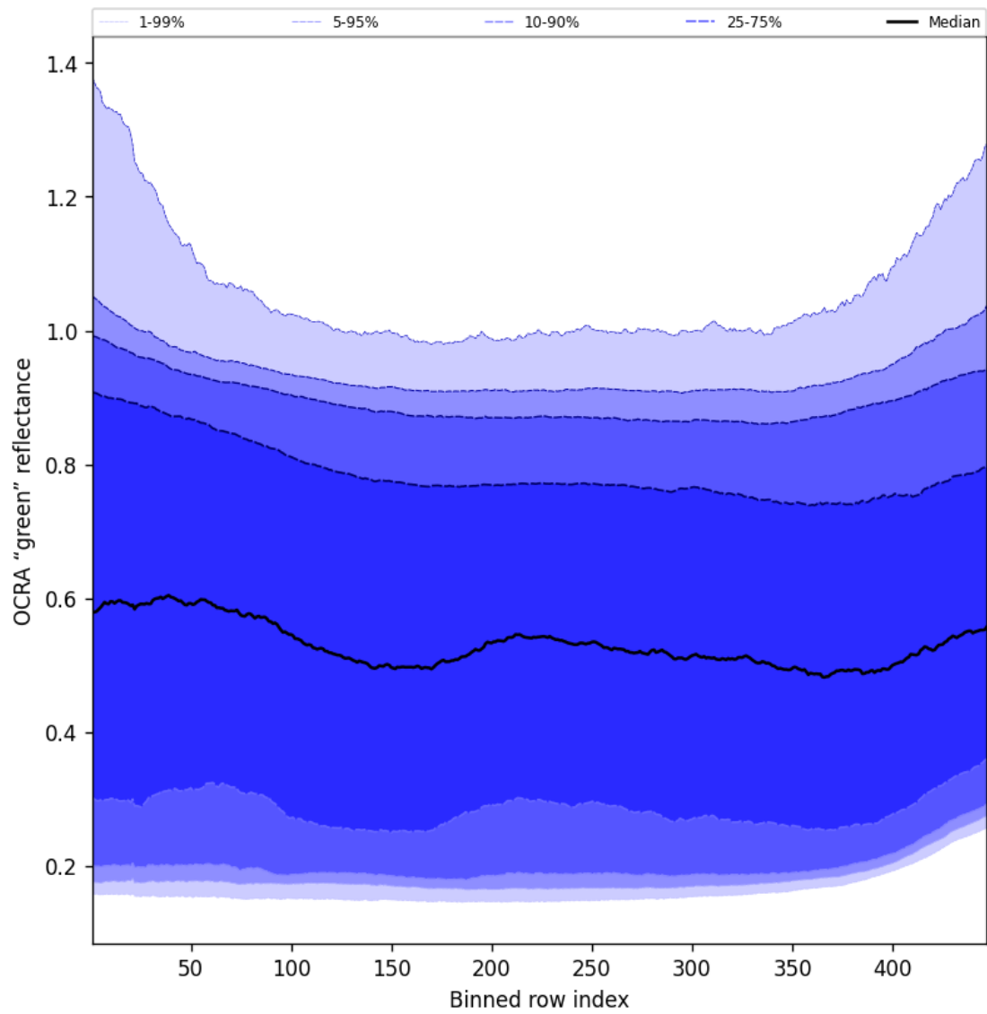
Figure 68: Along track statistics of “OCRA “green” reflectance” for 2024-11-09 to 2024-11-11
