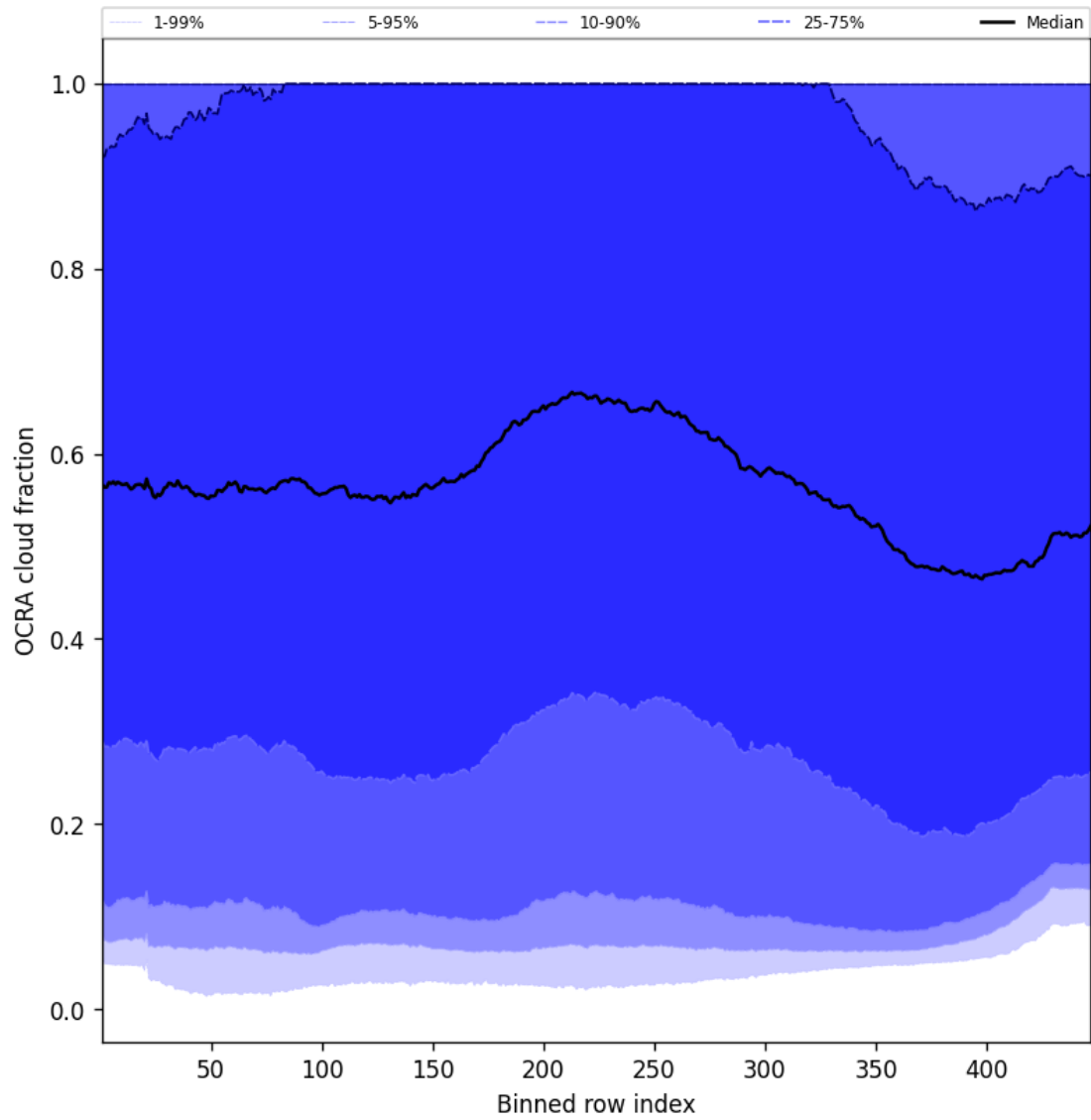
Figure 66: Along track statistics of “OCRA cloud fraction” for 2024-11-09 to 2024-11-11
