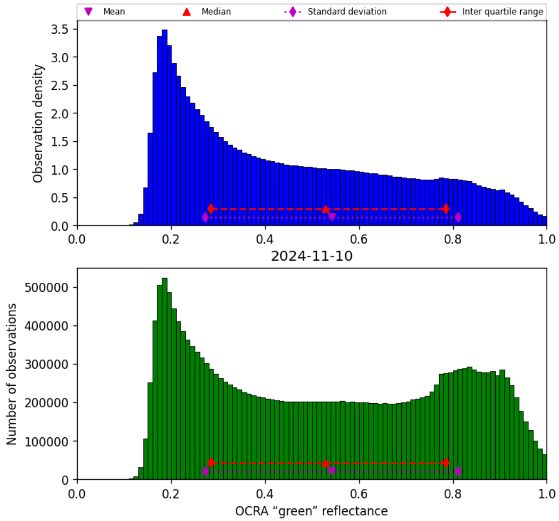
Figure 52: Histogram of “OCRA “green” reflectance” for 2024-11-09 to 2024-11-11
