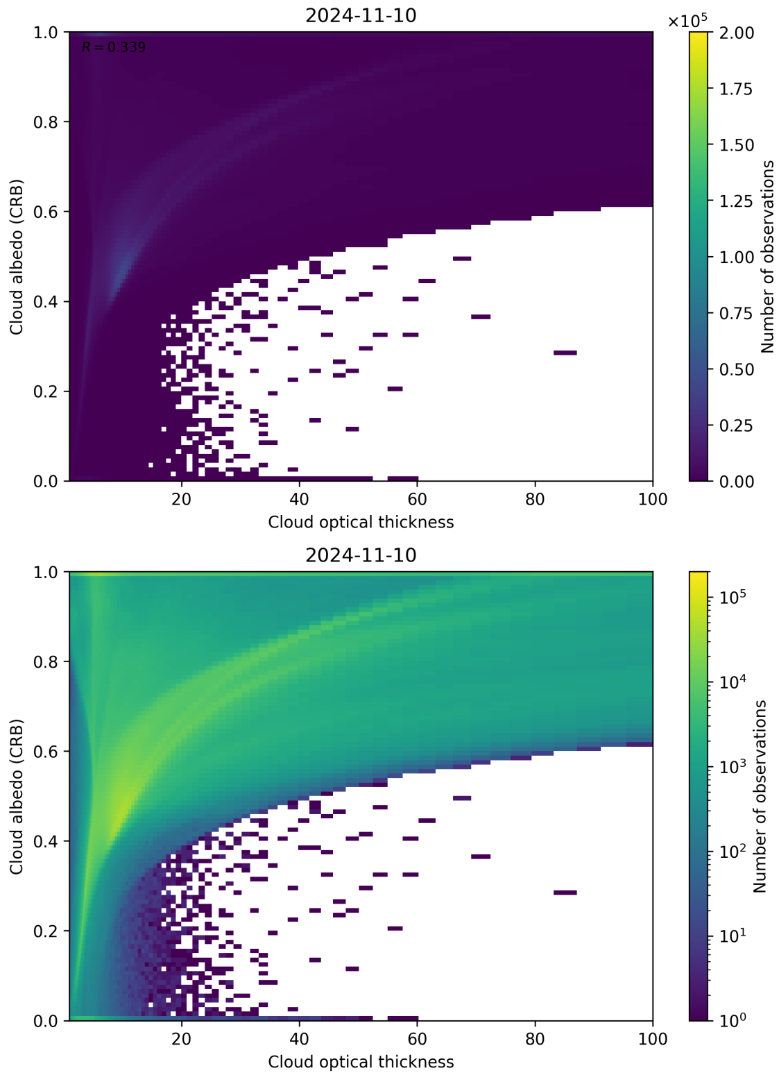
Figure 82: Scatter density plot of “Cloud optical thickness” against “Cloud albedo (CRB)” for 2024-11-09 to 2024-11-11.
