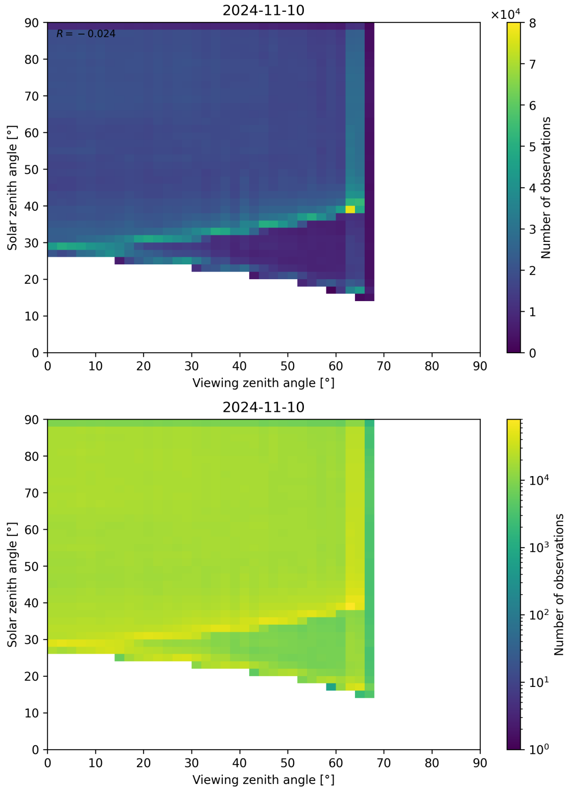
Figure 114: Scatter density plot of “Viewing zenith angle” against “Solar zenith angle” for 2024-11-09 to 2024-11-11.
