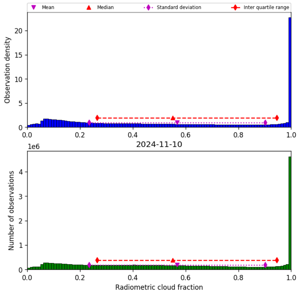
Figure 39: Histogram of “Radiometric cloud fraction” for 2024-11-09 to 2024-11-11
