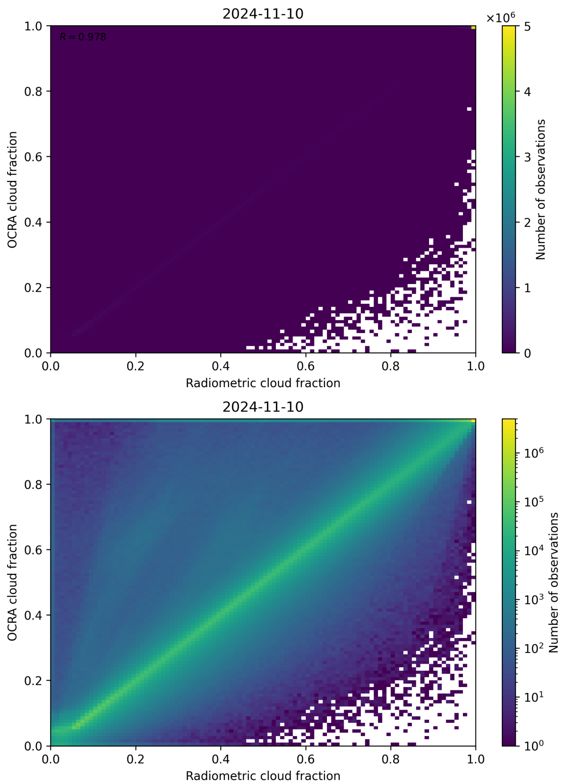
Figure 72: Scatter density plot of “Radiometric cloud fraction” against “OCRA cloud fraction” for 2024-11-09 to 2024-11-11.
