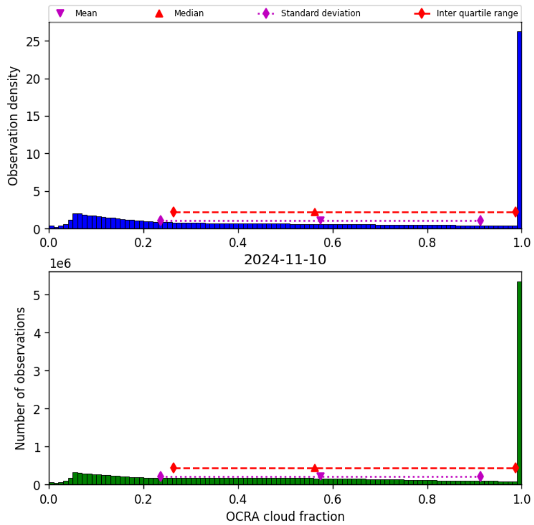
Figure 50: Histogram of “OCRA cloud fraction” for 2024-11-09 to 2024-11-11
