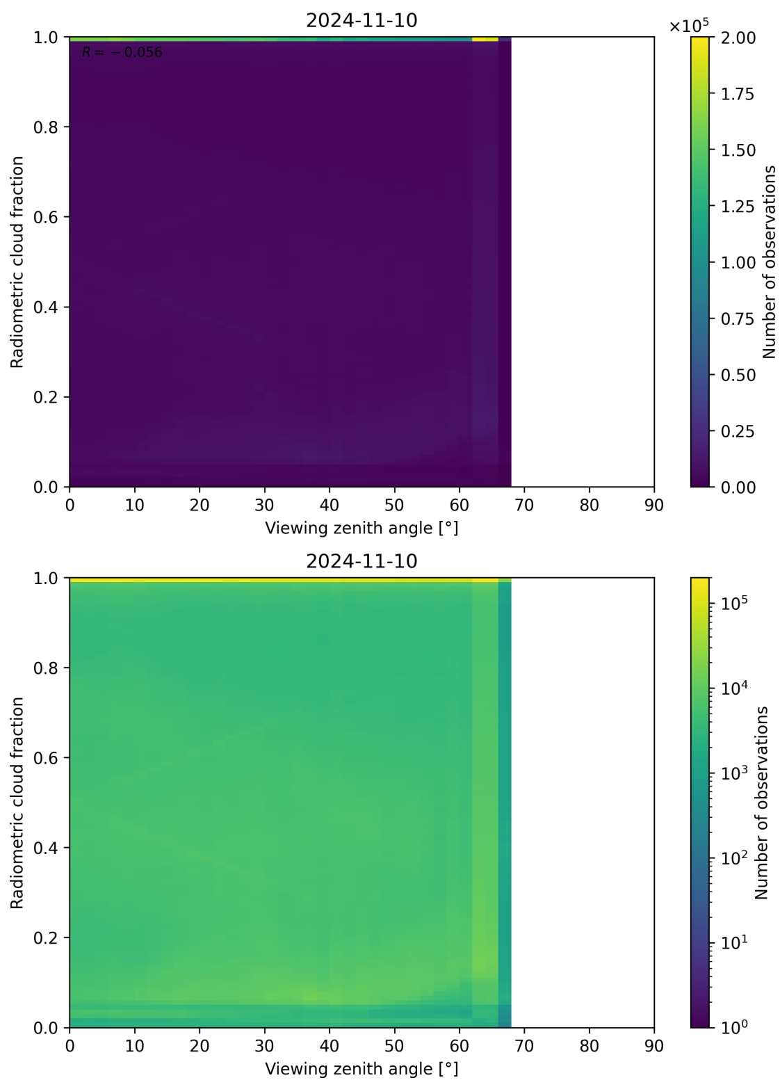
Figure 107: Scatter density plot of “Viewing zenith angle” against “Radiometric cloud fraction” for 2024-11-09 to 2024-11-11.
