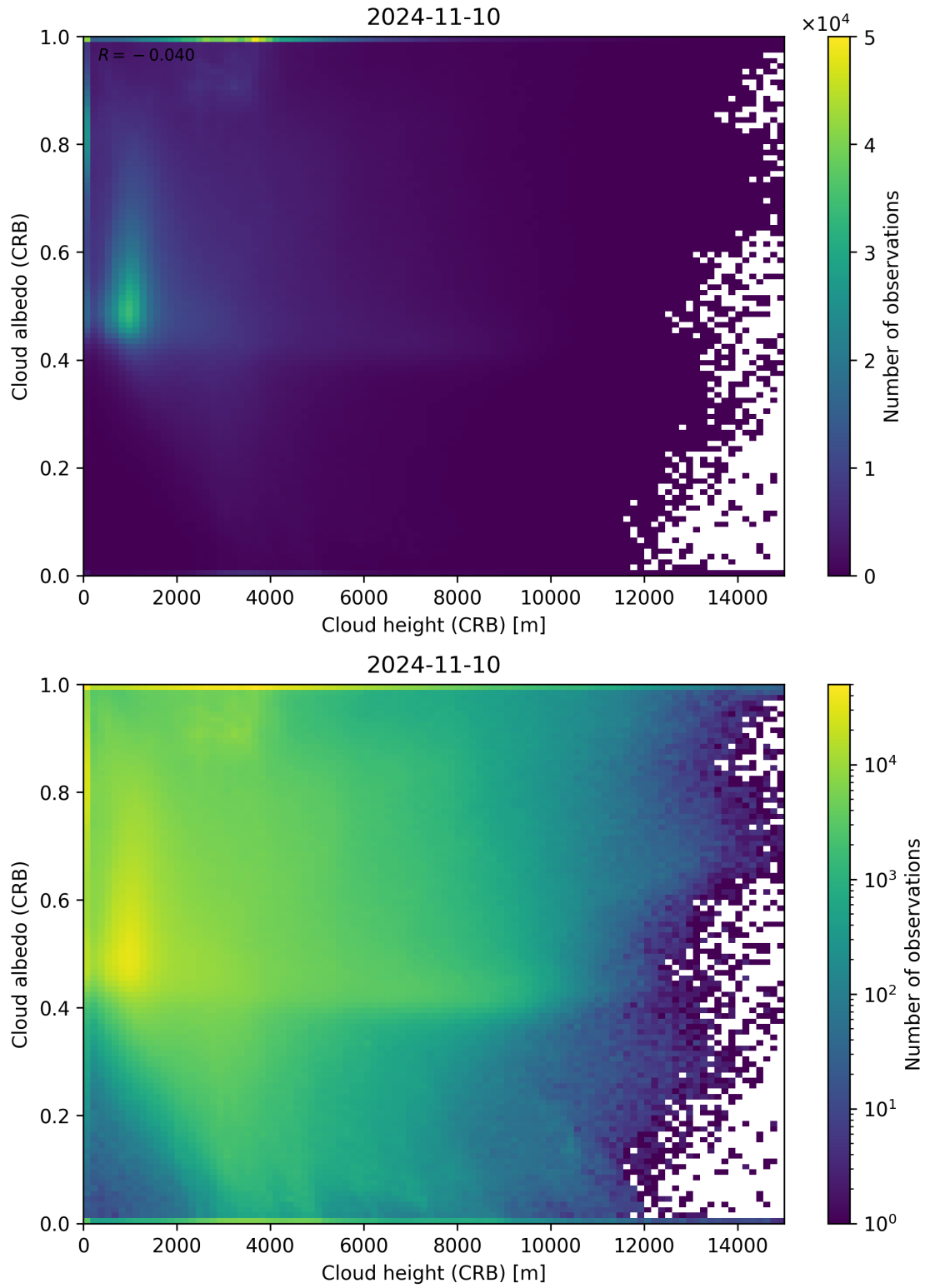
Figure 80: Scatter density plot of “Cloud height (CRB)” against “Cloud albedo (CRB)” for 2024-11-09 to 2024-11-11.
