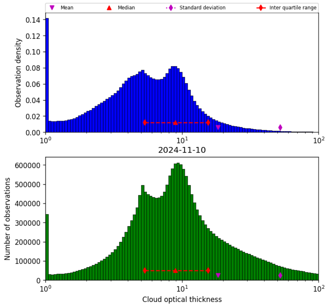
Figure 41: Histogram of “Cloud optical thickness” for 2024-11-09 to 2024-11-11
