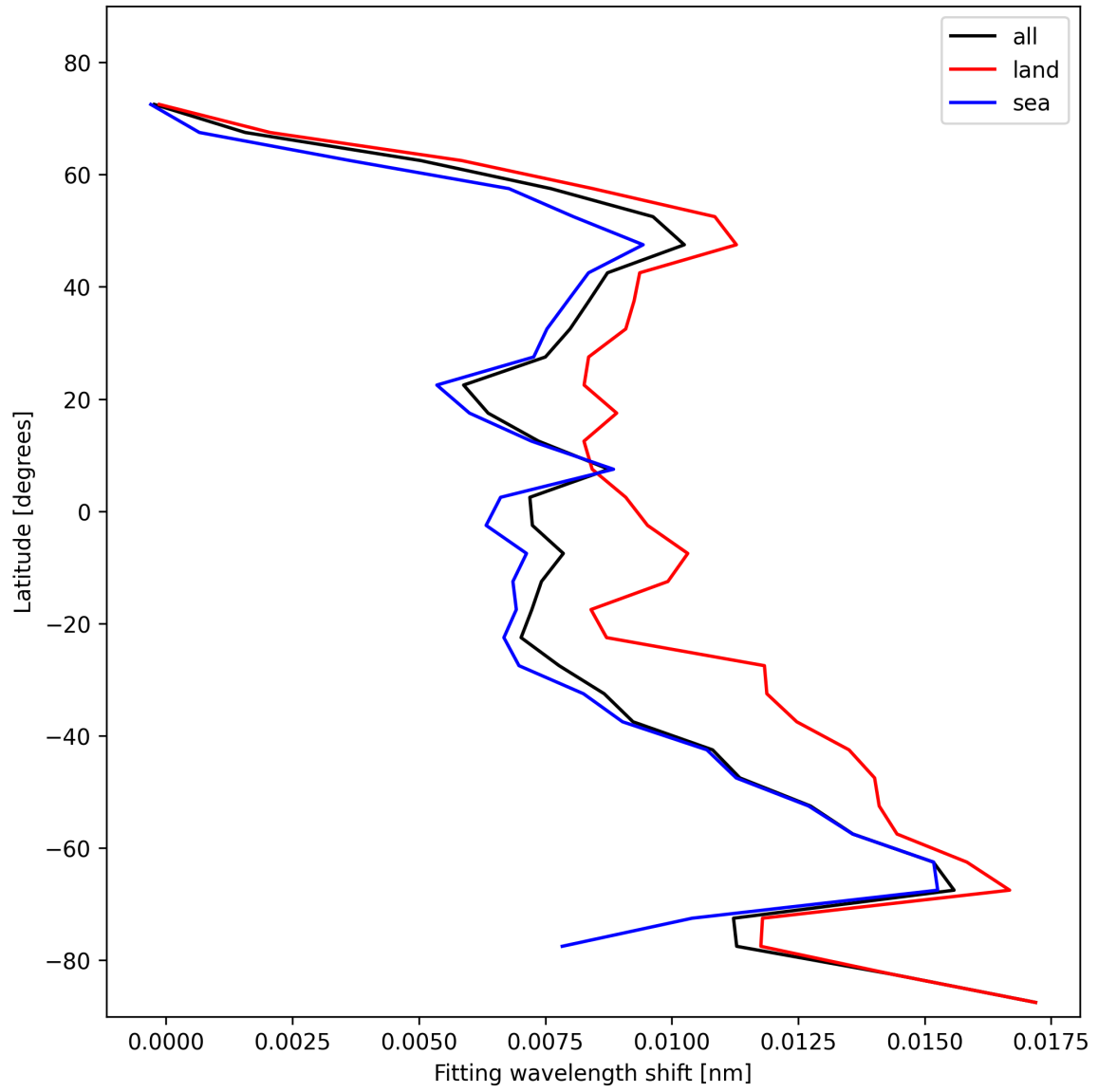
Figure 33: Zonal average of “Fitting wavelength shift” for 2024-11-09 to 2024-11-11.
