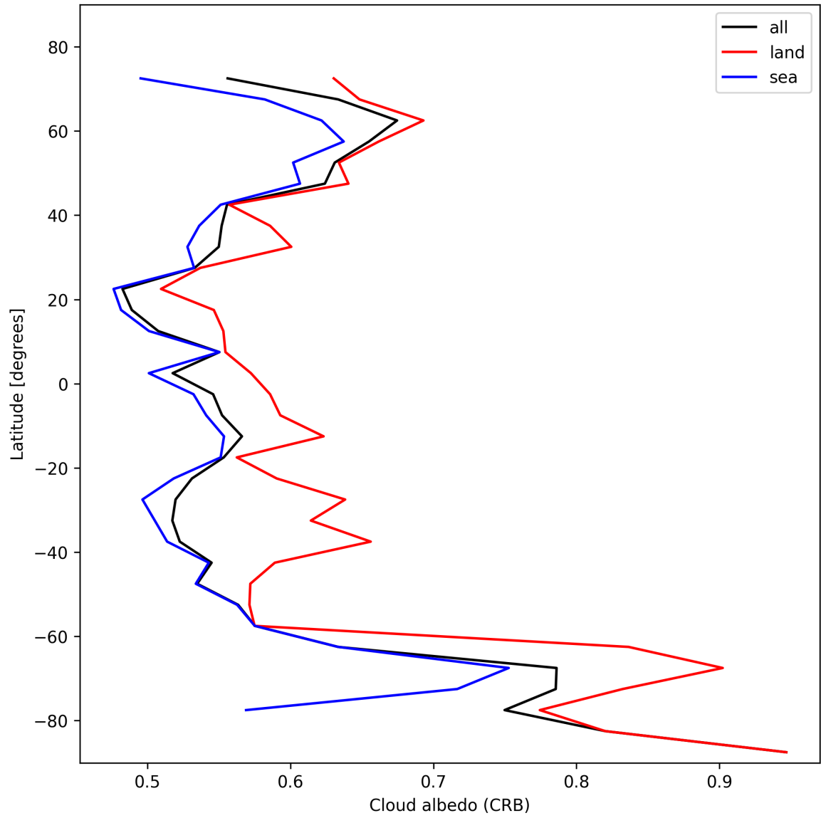
Figure 28: Zonal average of “Cloud albedo (CRB)” for 2024-11-09 to 2024-11-11.
