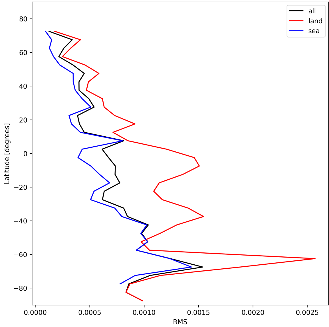
Figure 31: Zonal average of “RMS” for 2024-11-09 to 2024-11-11.
