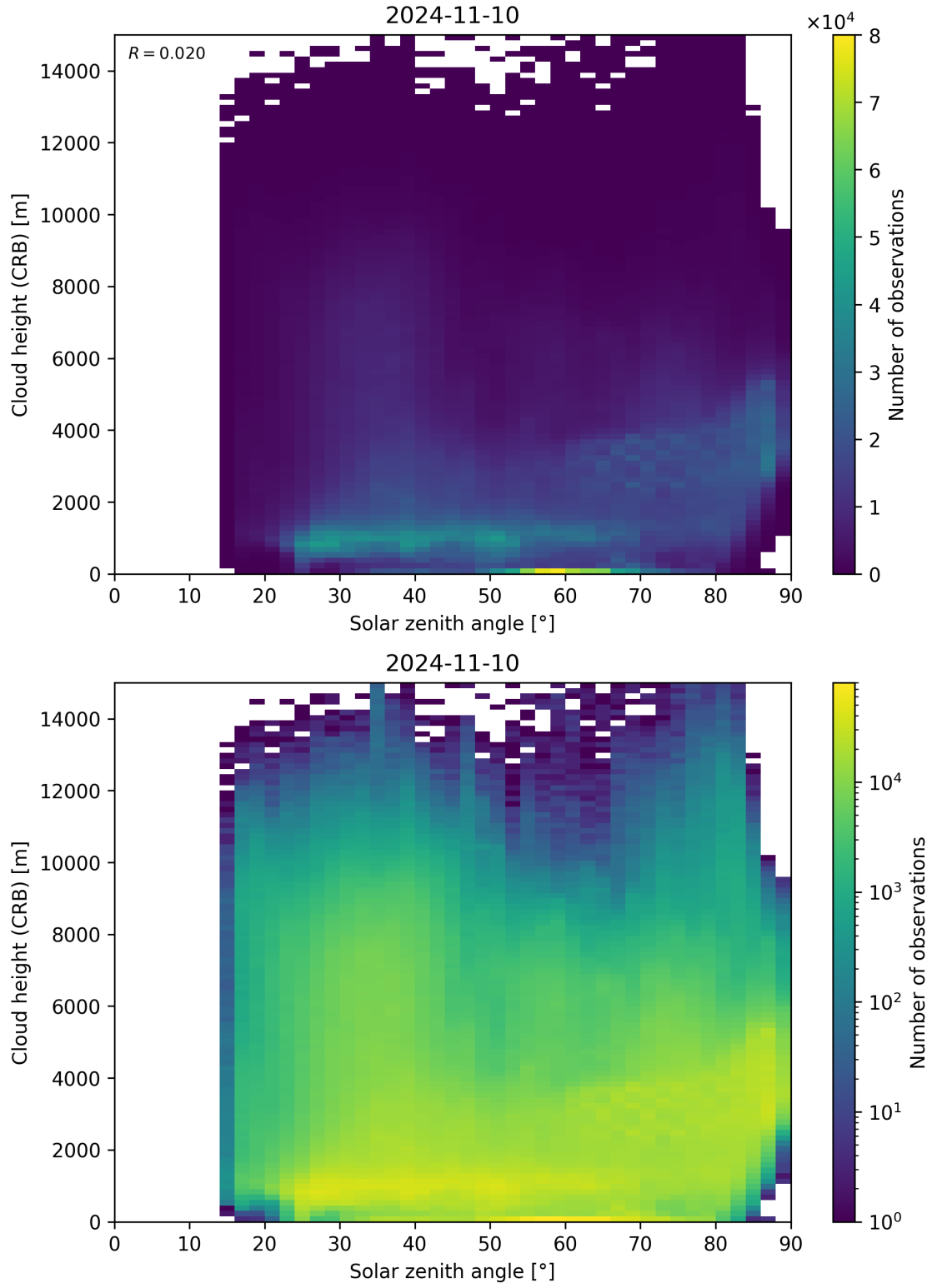
Figure 102: Scatter density plot of “Solar zenith angle” against “Cloud height (CRB)” for 2024-11-09 to 2024-11-11.
