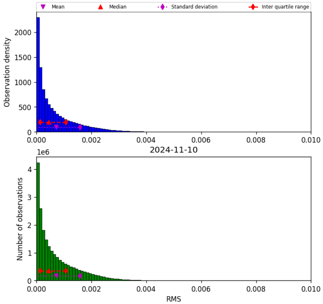
Figure 47: Histogram of “RMS” for 2024-11-09 to 2024-11-11
