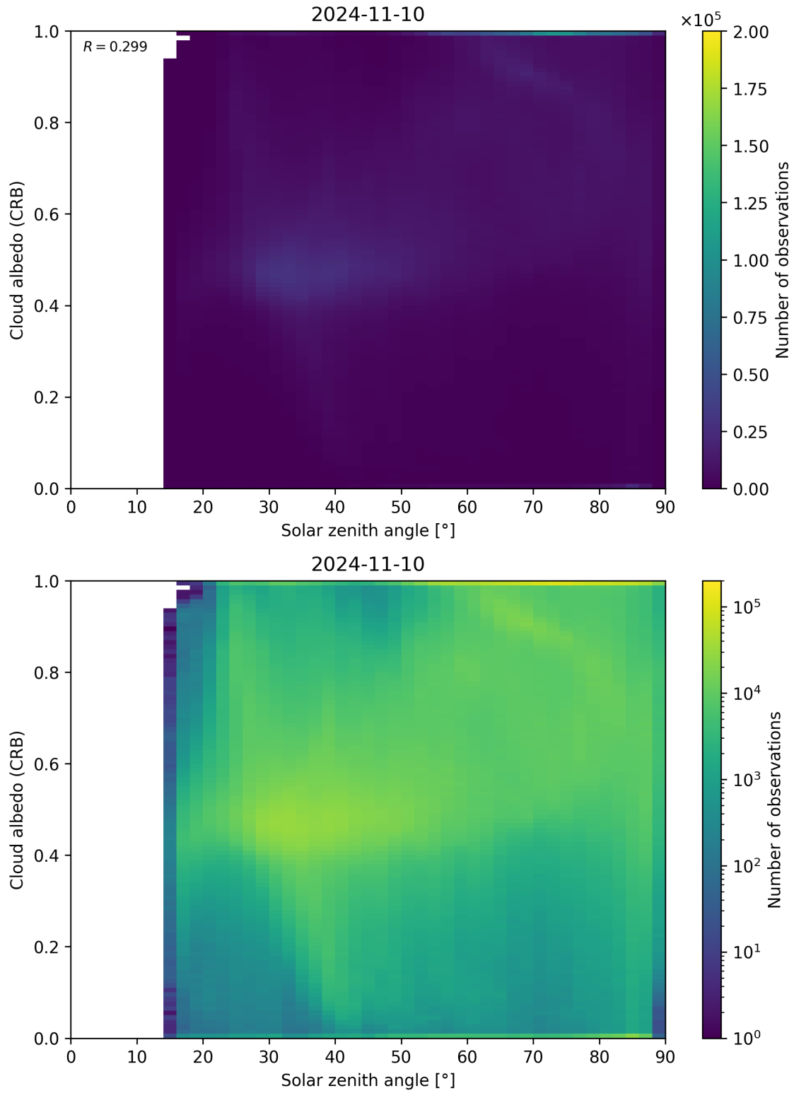
Figure 98: Scatter density plot of “Solar zenith angle” against “Cloud albedo (CRB)” for 2024-11-09 to 2024-11-11.
