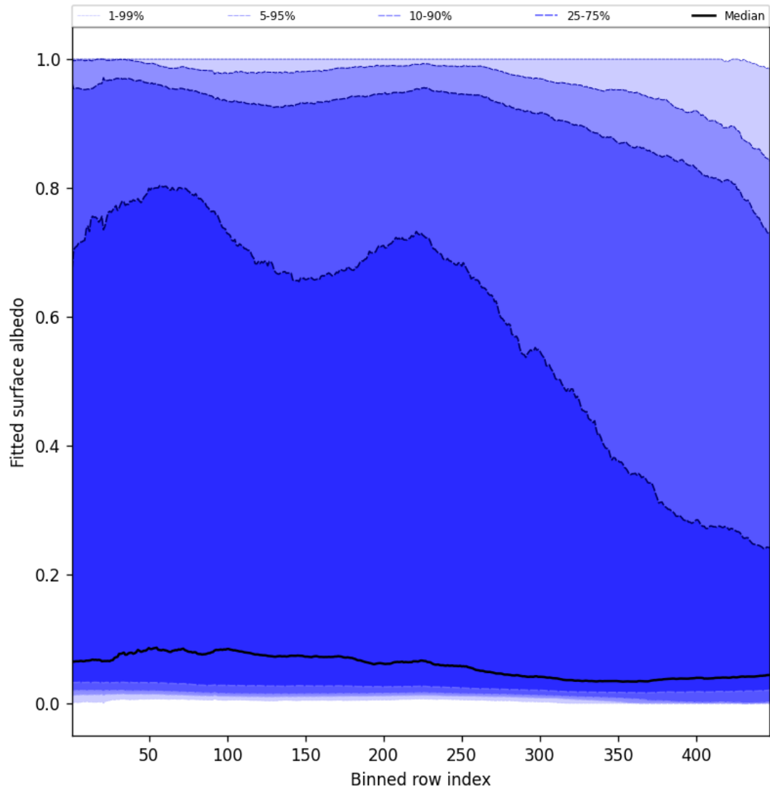
Figure 61: Along track statistics of “Fitted surface albedo” for 2024-11-09 to 2024-11-11
