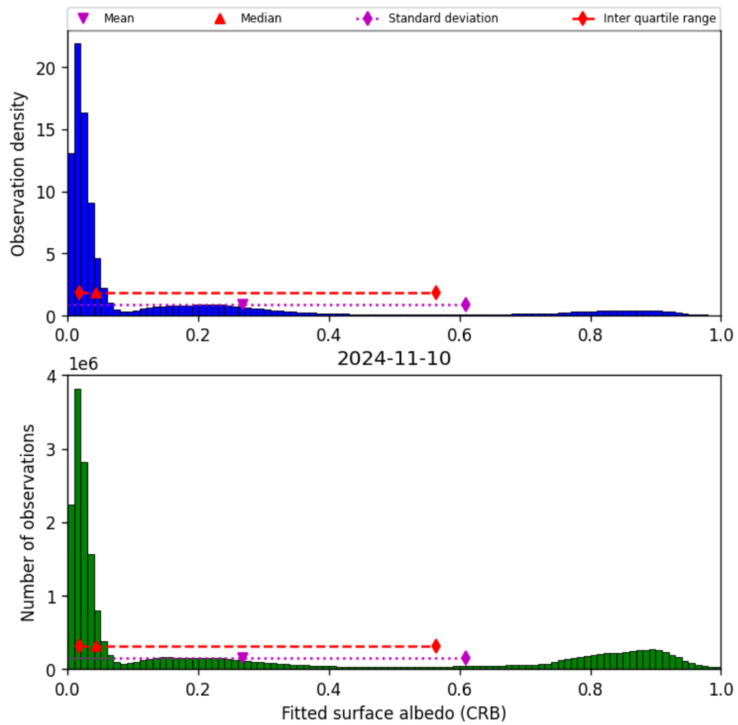
Figure 46: Histogram of “Fitted surface albedo (CRB)” for 2024-11-09 to 2024-11-11
