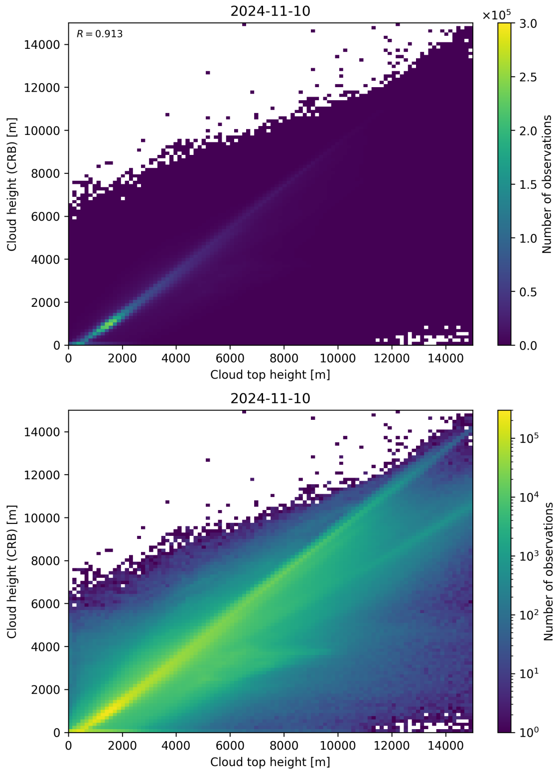
Figure 89: Scatter density plot of “Cloud top height” against “Cloud height (CRB)” for 2024-11-09 to 2024-11-11.
