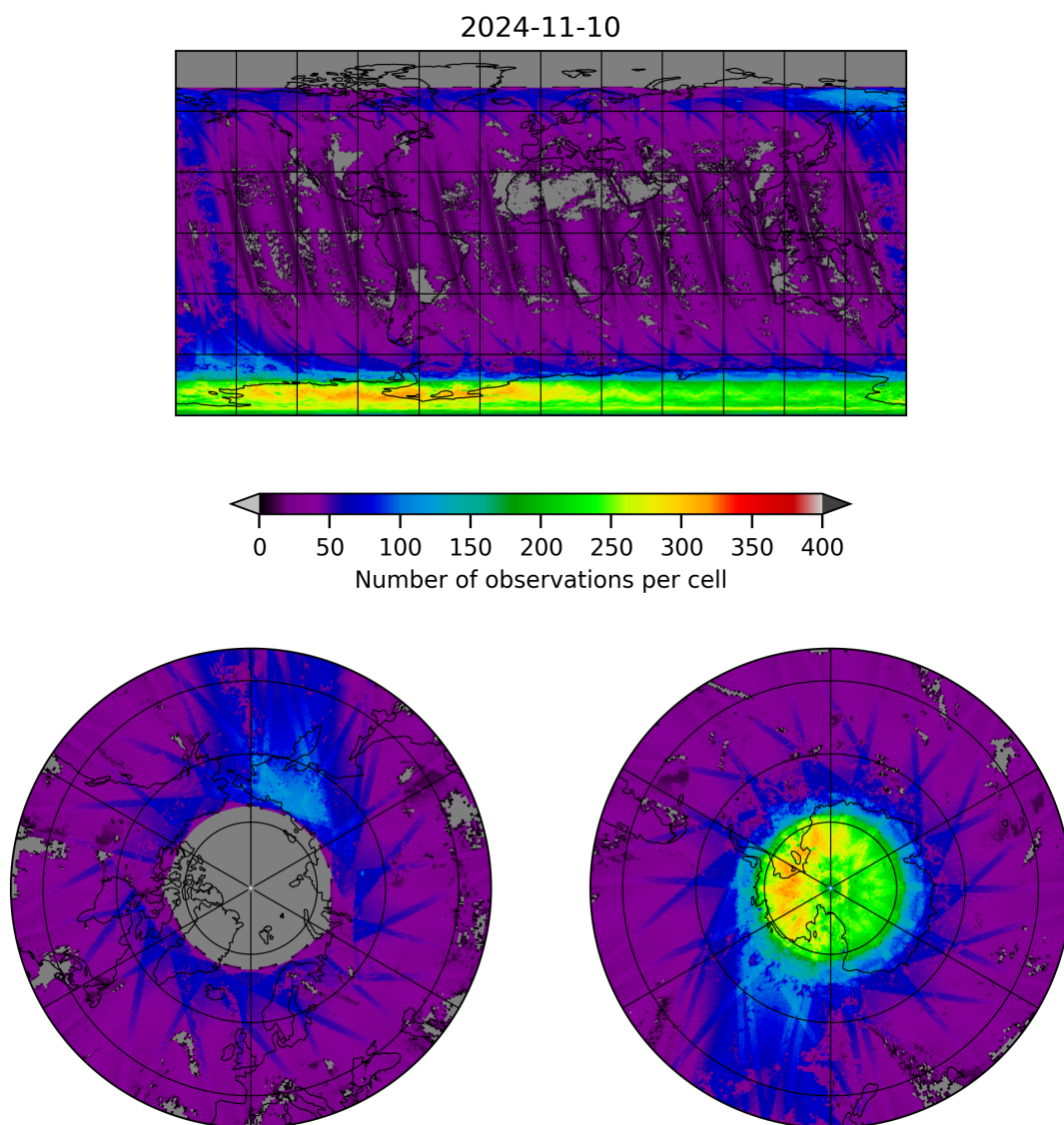
Figure 21: Map of the number of observations for 2024-11-09 to 2024-11-11
