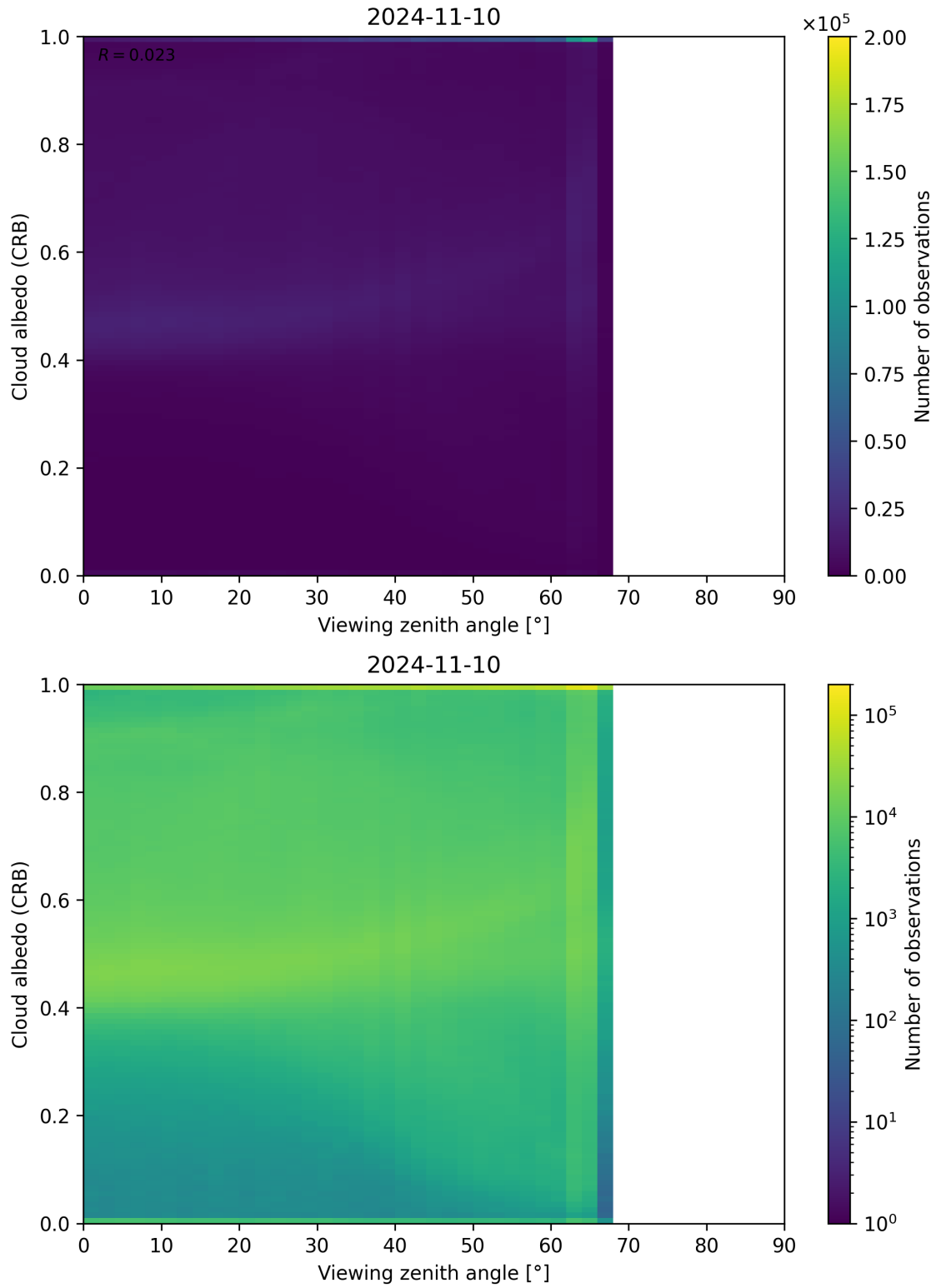
Figure 106: Scatter density plot of “Viewing zenith angle” against “Cloud albedo (CRB)” for 2024-11-09 to 2024-11-11.
