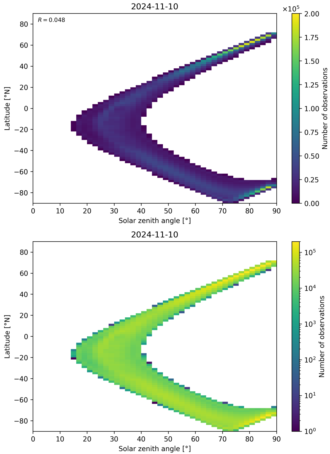
Figure 105: Scatter density plot of “Solar zenith angle” against “Latitude” for 2024-11-09 to 2024-11-11.
