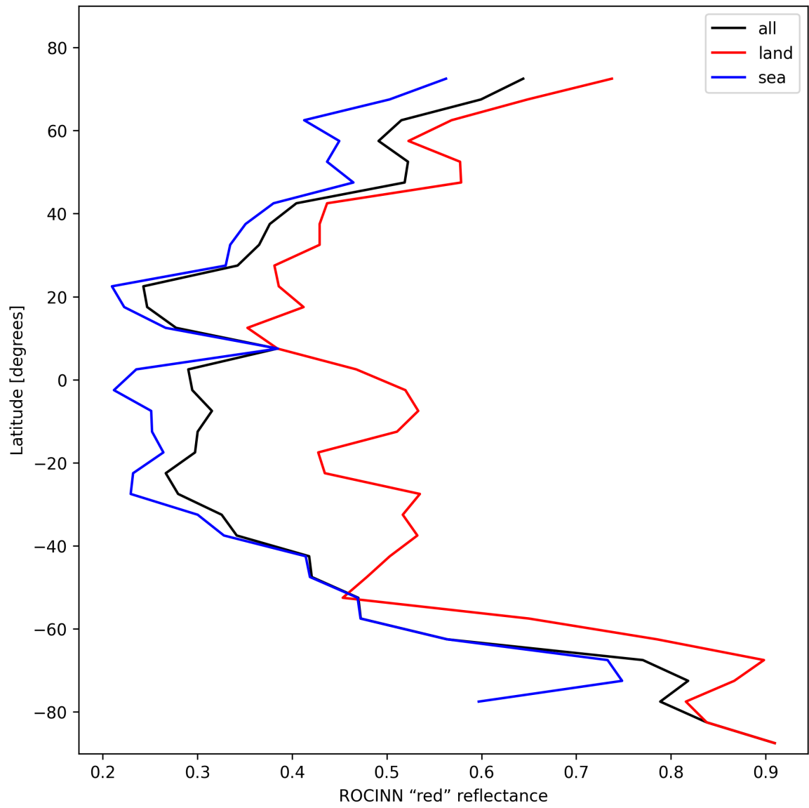
Figure 37: Zonal average of “ROCINN “red” reflectance” for 2024-11-09 to 2024-11-11.
