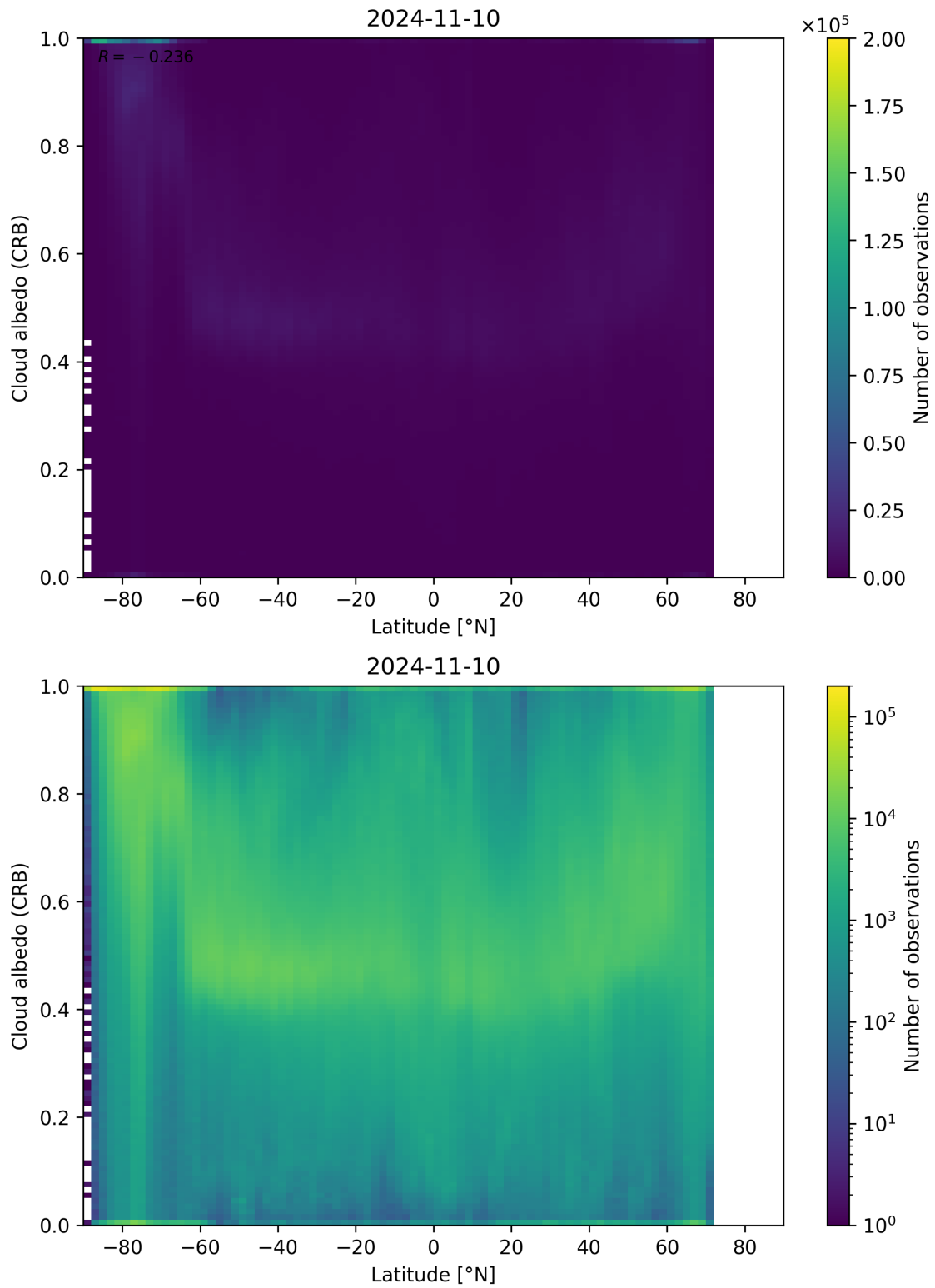
Figure 91: Scatter density plot of “Latitude” against “Cloud albedo (CRB)” for 2024-11-09 to 2024-11-11.
