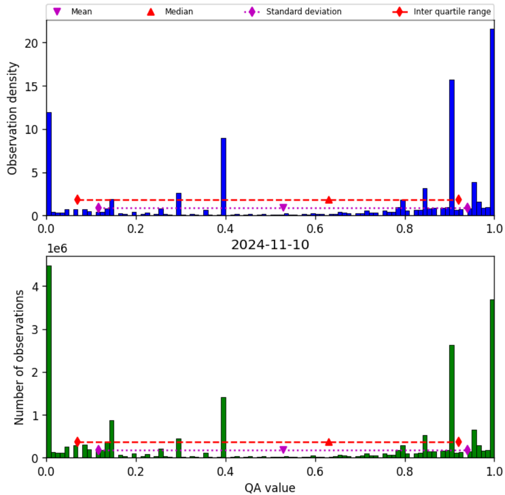
Figure 38: Histogram of “QA value” for 2024-11-09 to 2024-11-11
