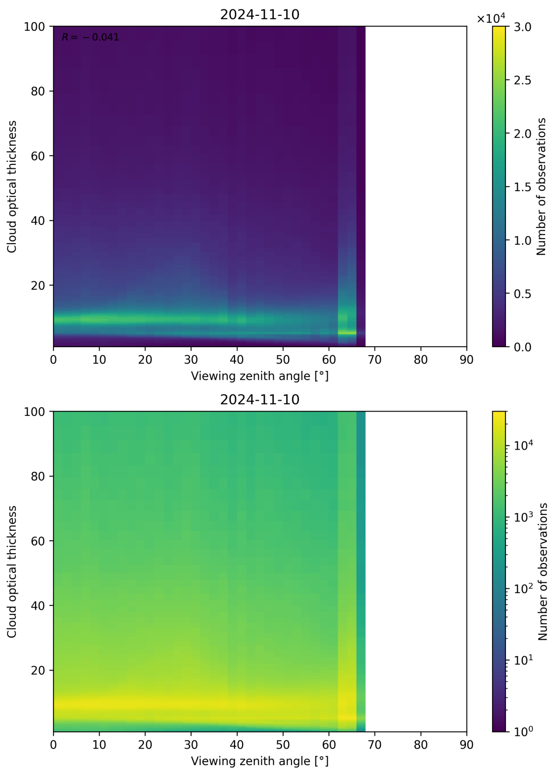
Figure 111: Scatter density plot of “Viewing zenith angle” against “Cloud optical thickness” for 2024-11-09 to 2024-11-11.
