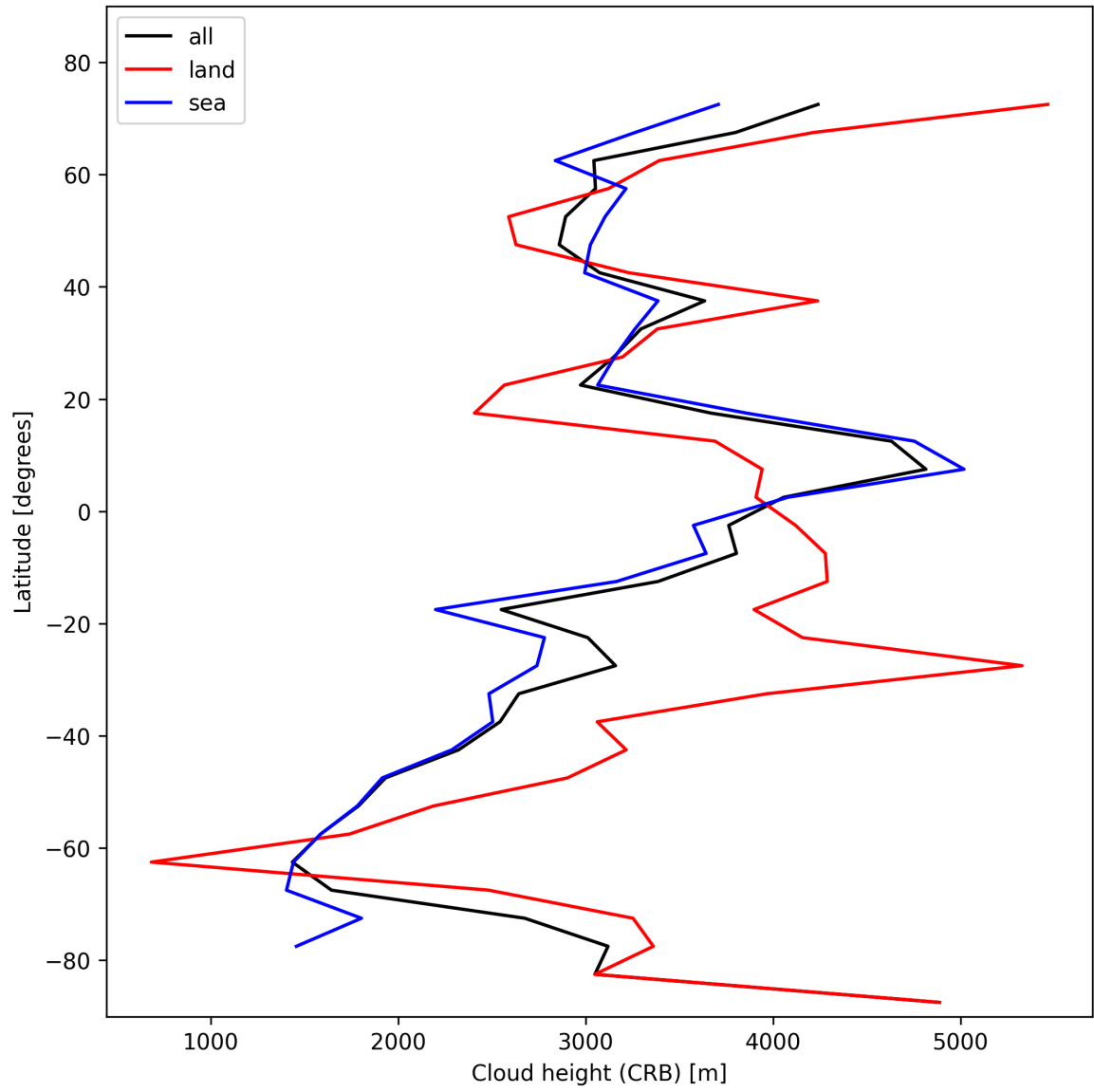
Figure 27: Zonal average of “Cloud height (CRB)” for 2024-11-09 to 2024-11-11.
