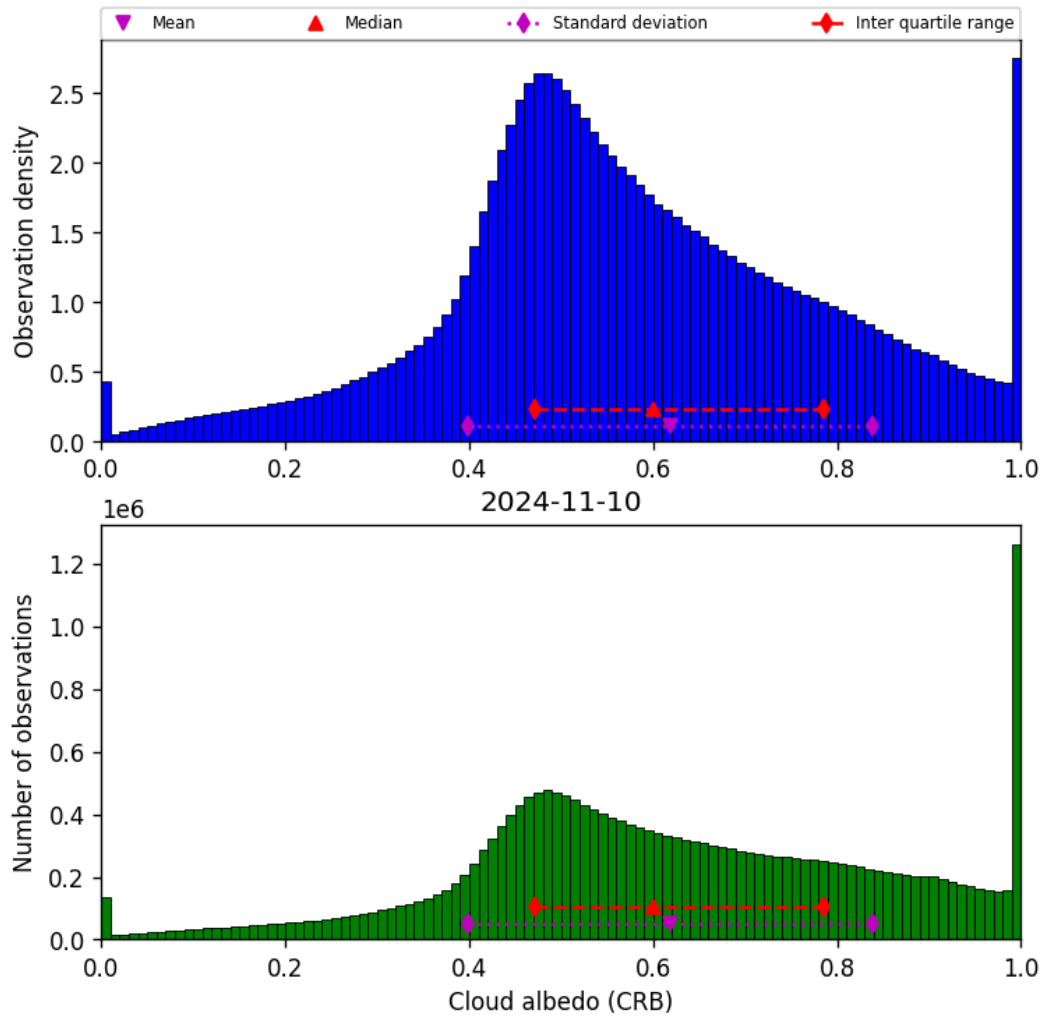
Figure 44: Histogram of “Cloud albedo (CRB)” for 2024-11-09 to 2024-11-11
