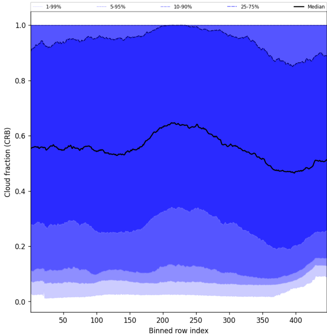
Figure 58: Along track statistics of “Cloud fraction (CRB)” for 2024-11-09 to 2024-11-11
