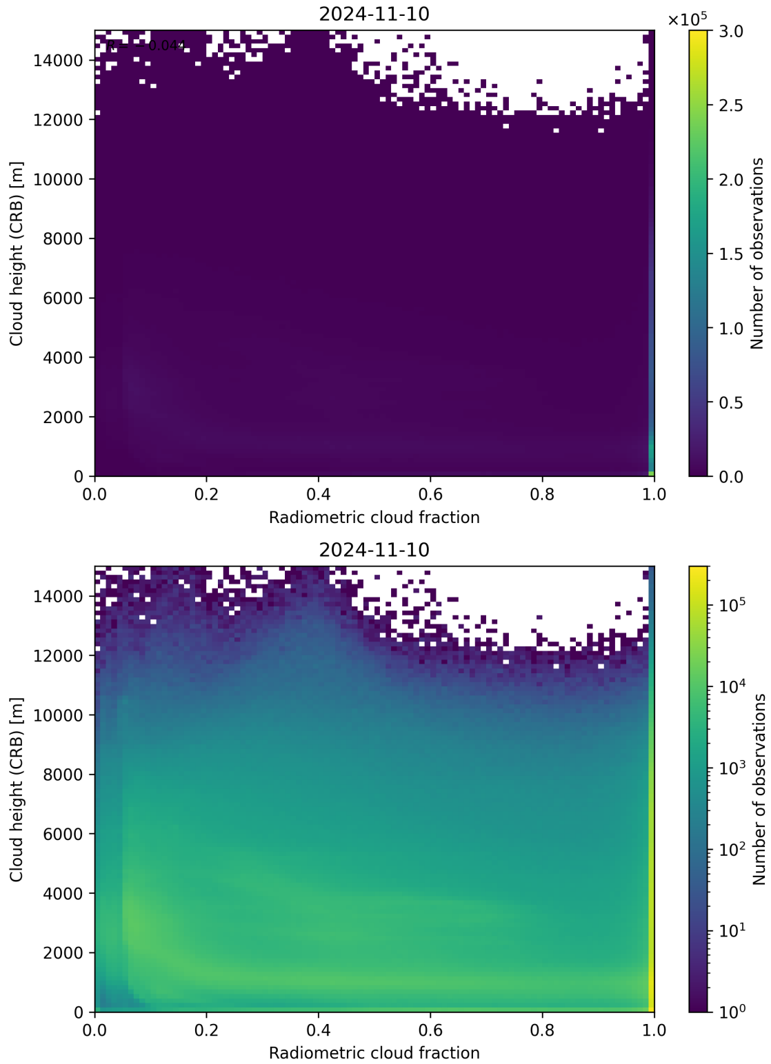
Figure 74: Scatter density plot of “Radiometric cloud fraction” against “Cloud height (CRB)” for 2024-11-09 to 2024-11-11.
