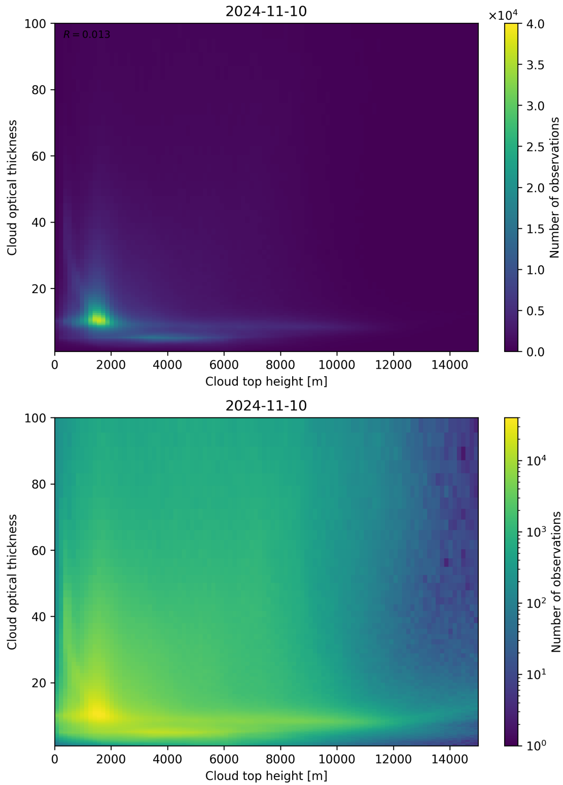
Figure 90: Scatter density plot of “Cloud top height” against “Cloud optical thickness” for 2024-11-09 to 2024-11-11.
