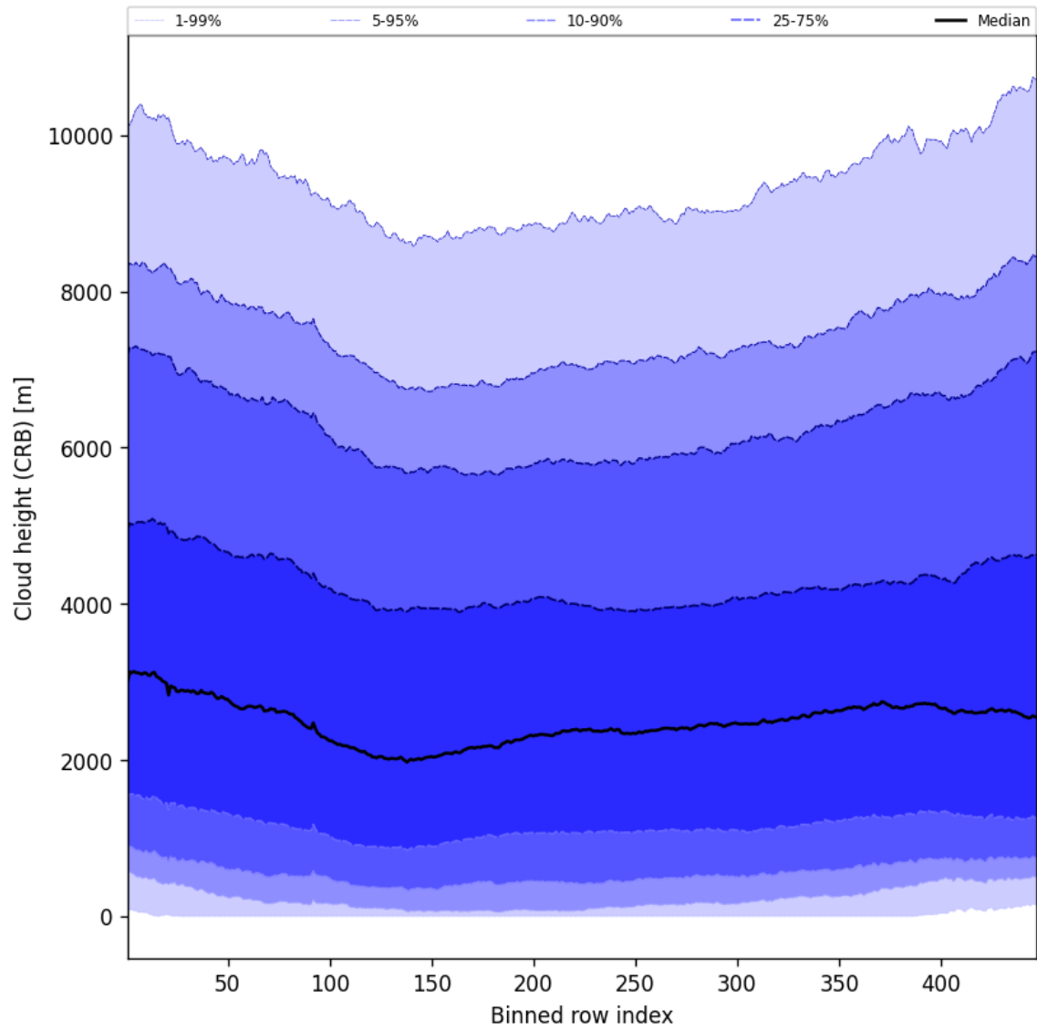
Figure 59: Along track statistics of “Cloud height (CRB)” for 2024-11-09 to 2024-11-11
