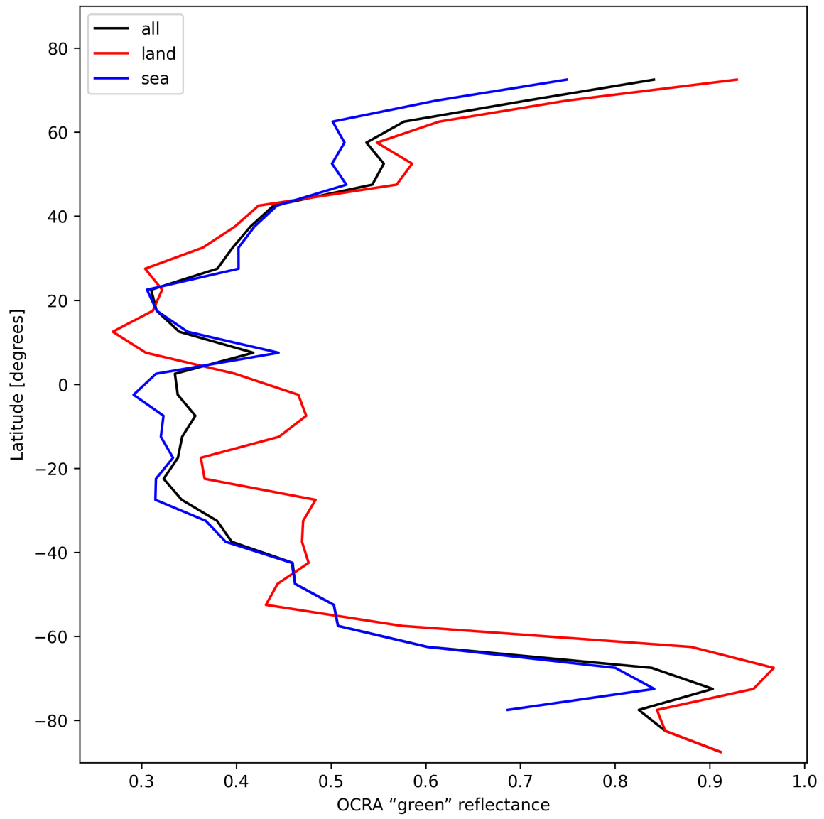
Figure 36: Zonal average of “OCRA “green” reflectance” for 2024-11-09 to 2024-11-11.
