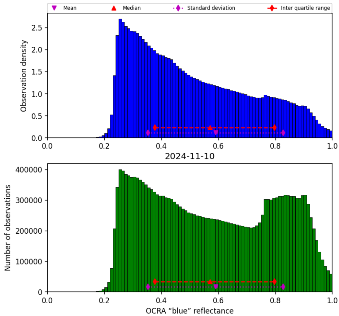
Figure 51: Histogram of “OCRA “blue” reflectance” for 2024-11-09 to 2024-11-11
