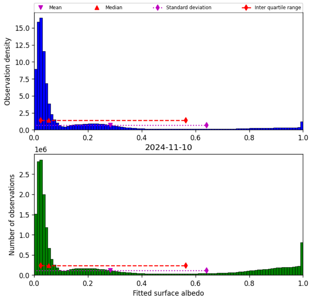
Figure 45: Histogram of “Fitted surface albedo” for 2024-11-09 to 2024-11-11
