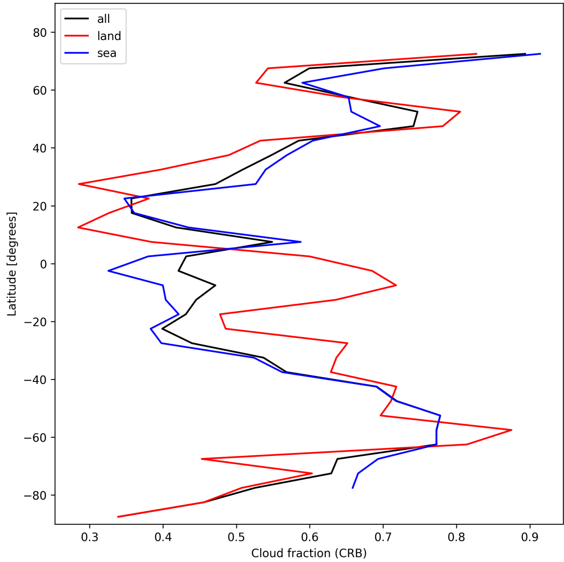
Figure 26: Zonal average of “Cloud fraction (CRB)” for 2024-11-09 to 2024-11-11.
