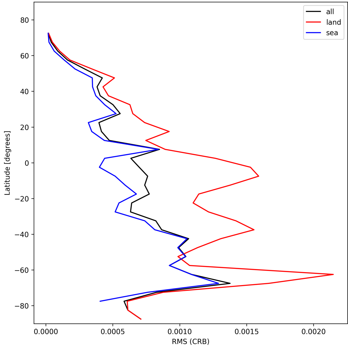
Figure 32: Zonal average of “RMS (CRB)” for 2024-11-09 to 2024-11-11.
