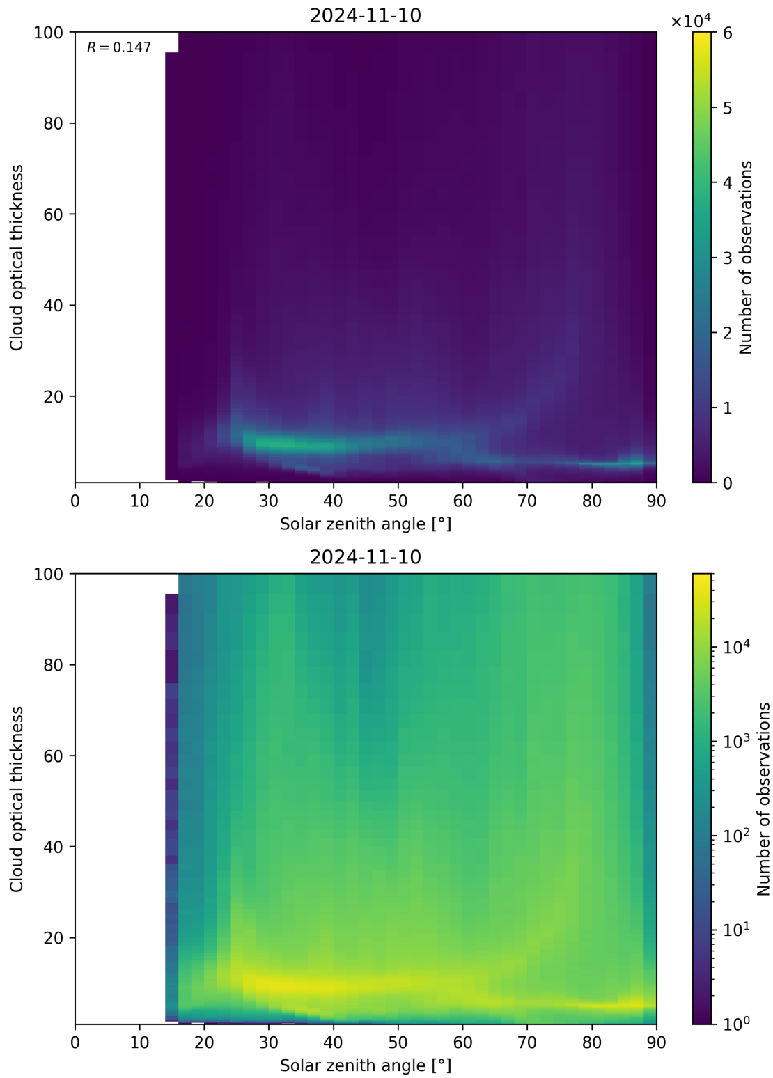
Figure 103: Scatter density plot of “Solar zenith angle” against “Cloud optical thickness” for 2024-11-09 to 2024-11-11.
