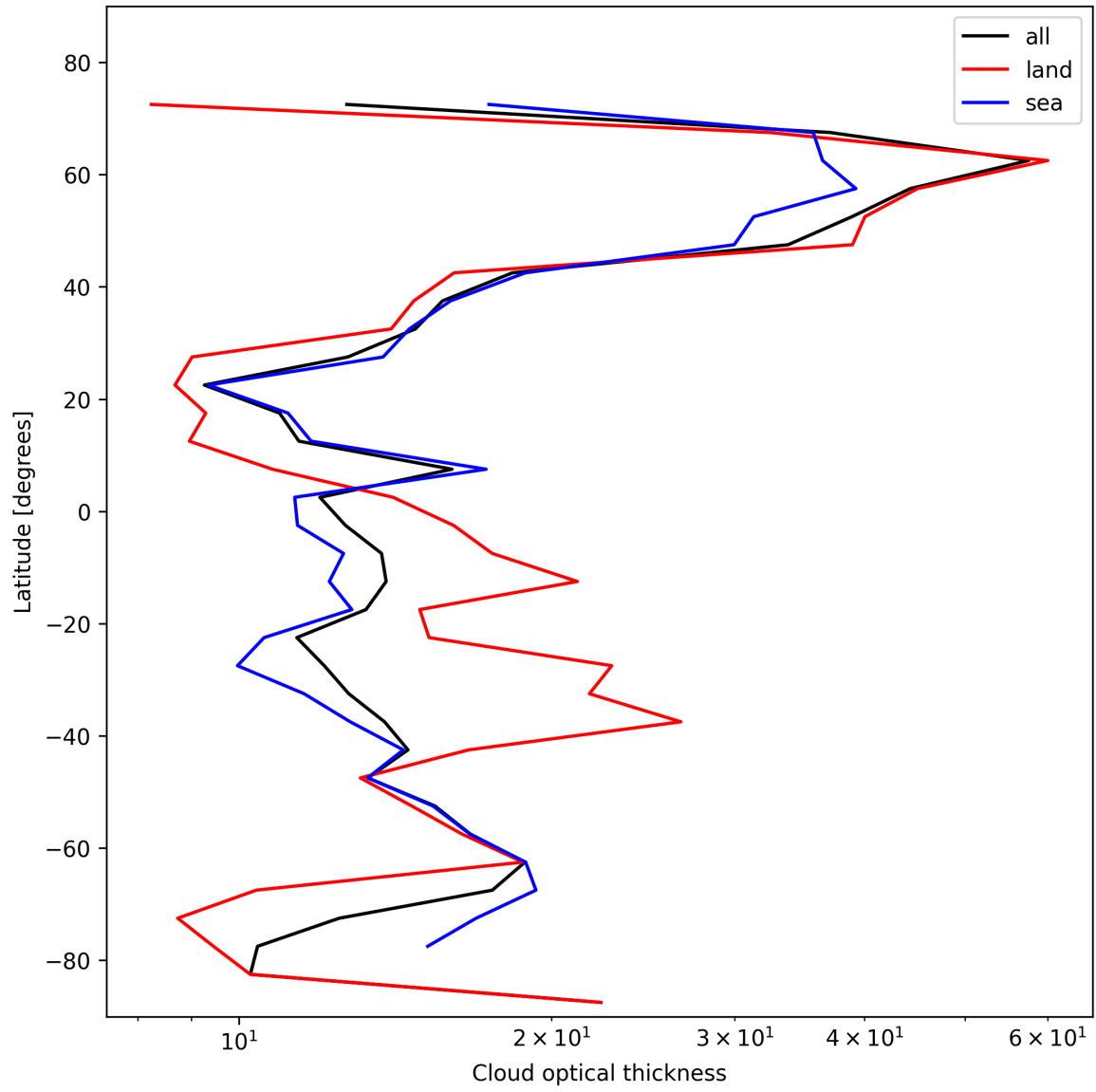
Figure 25: Zonal average of “Cloud optical thickness” for 2024-11-09 to 2024-11-11.
