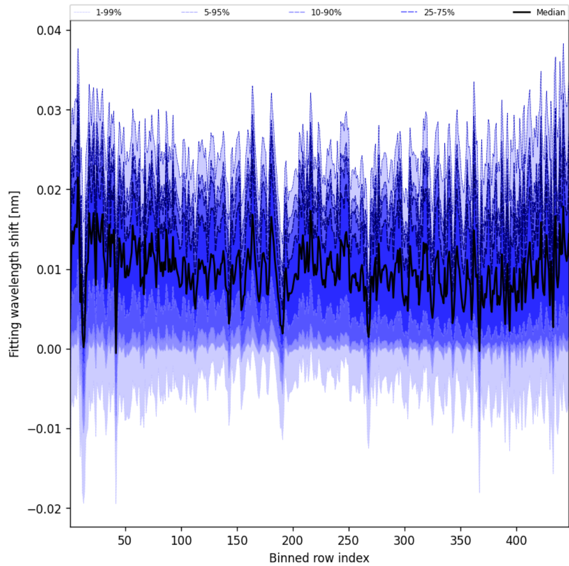
Figure 65: Along track statistics of “Fitting wavelength shift” for 2024-11-09 to 2024-11-11
