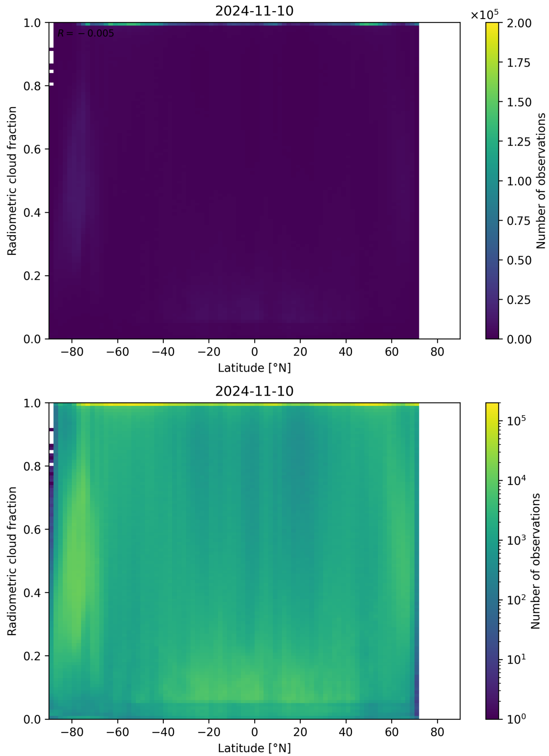
Figure 92: Scatter density plot of “Latitude” against “Radiometric cloud fraction” for 2024-11-09 to 2024-11-11.
