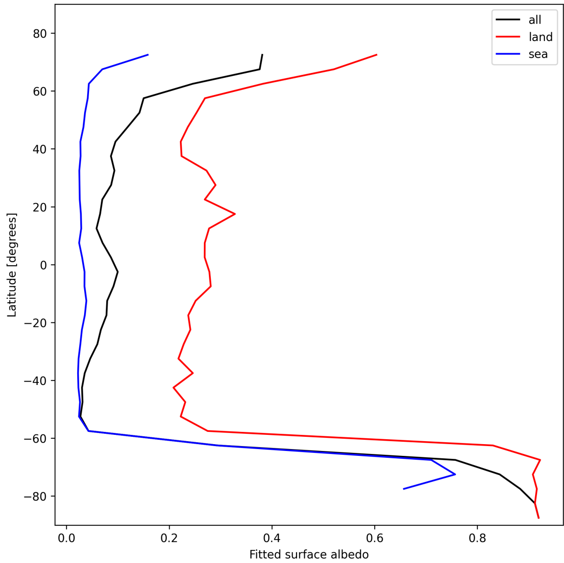
Figure 29: Zonal average of “Fitted surface albedo” for 2024-11-09 to 2024-11-11.
