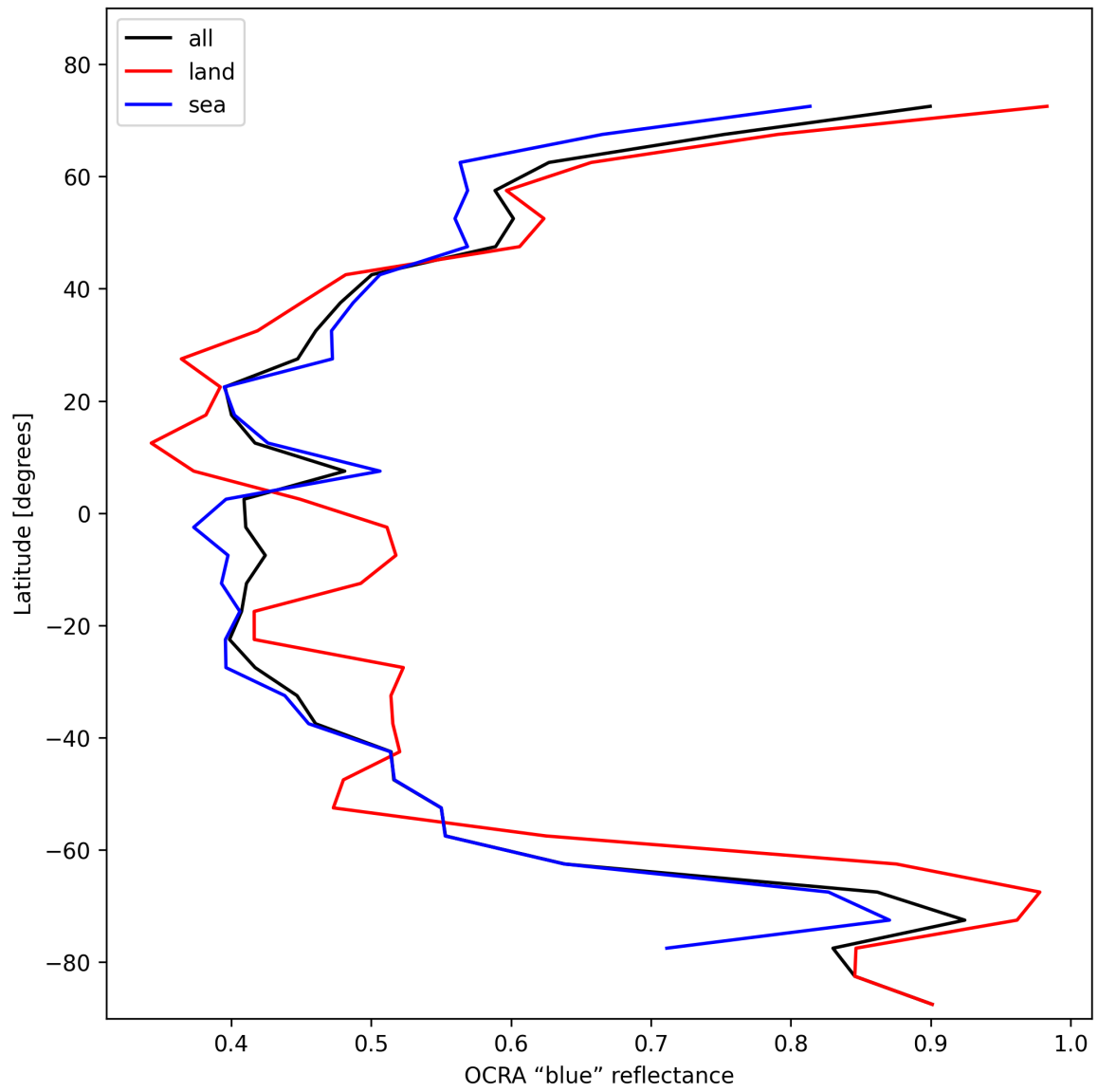
Figure 35: Zonal average of “OCRA “blue” reflectance” for 2024-11-09 to 2024-11-11.
