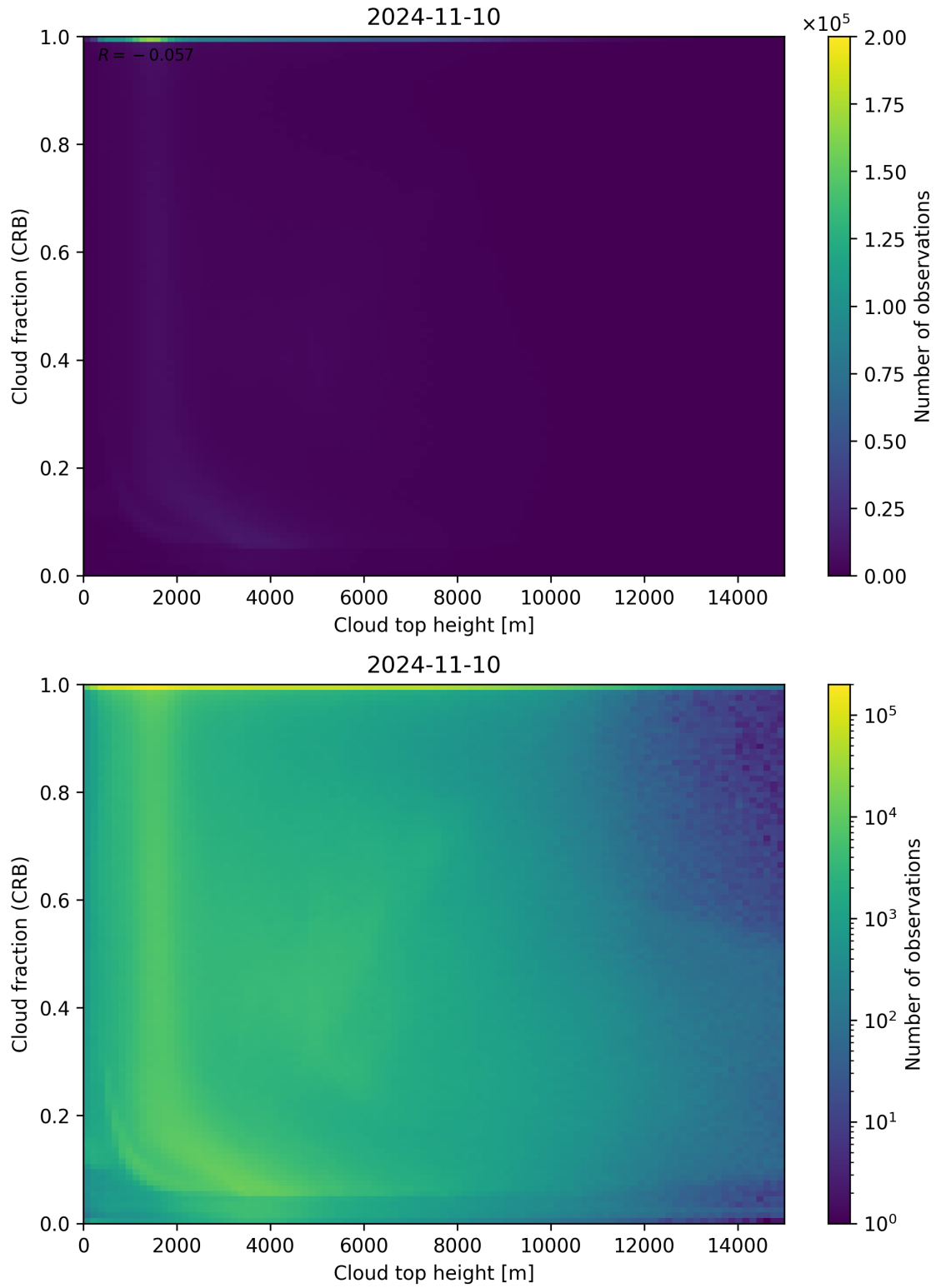
Figure 88: Scatter density plot of “Cloud top height” against “Cloud fraction (CRB)” for 2024-11-09 to 2024-11-11.
