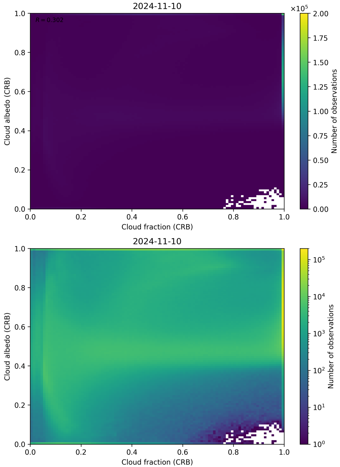
Figure 77: Scatter density plot of “Cloud fraction (CRB)” against “Cloud albedo (CRB)” for 2024-11-09 to 2024-11-11.
