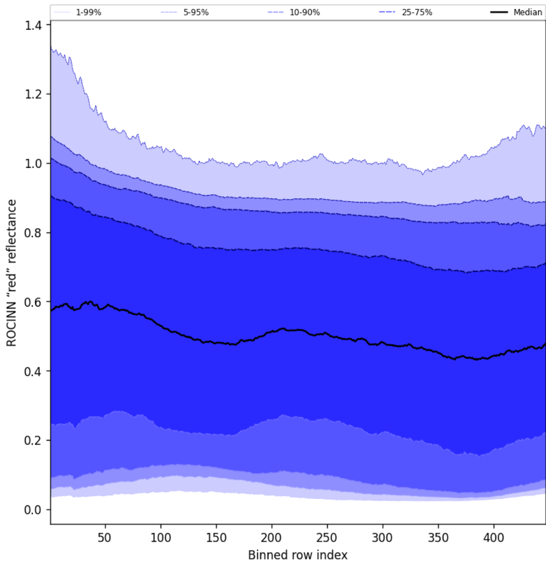
Figure 69: Along track statistics of “ROCINN “red” reflectance” for 2024-11-09 to 2024-11-11
