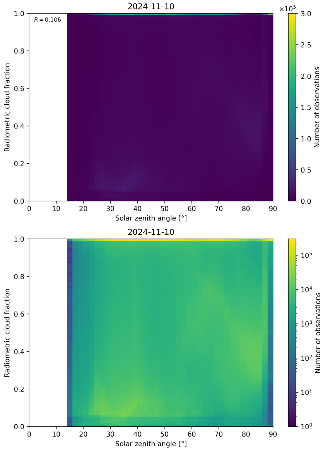
Figure 99: Scatter density plot of “Solar zenith angle” against “Radiometric cloud fraction” for 2024-11-09 to 2024-11-11.
