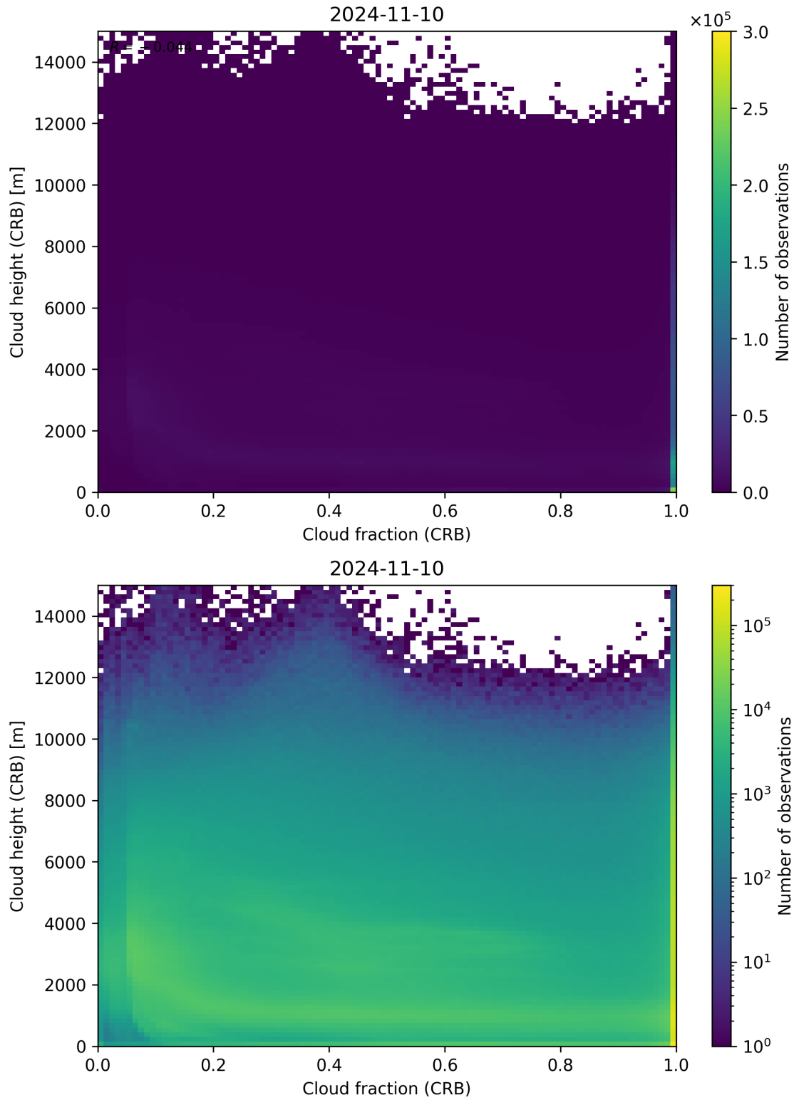
Figure 79: Scatter density plot of “Cloud fraction (CRB)” against “Cloud height (CRB)” for 2024-11-09 to 2024-11-11.
