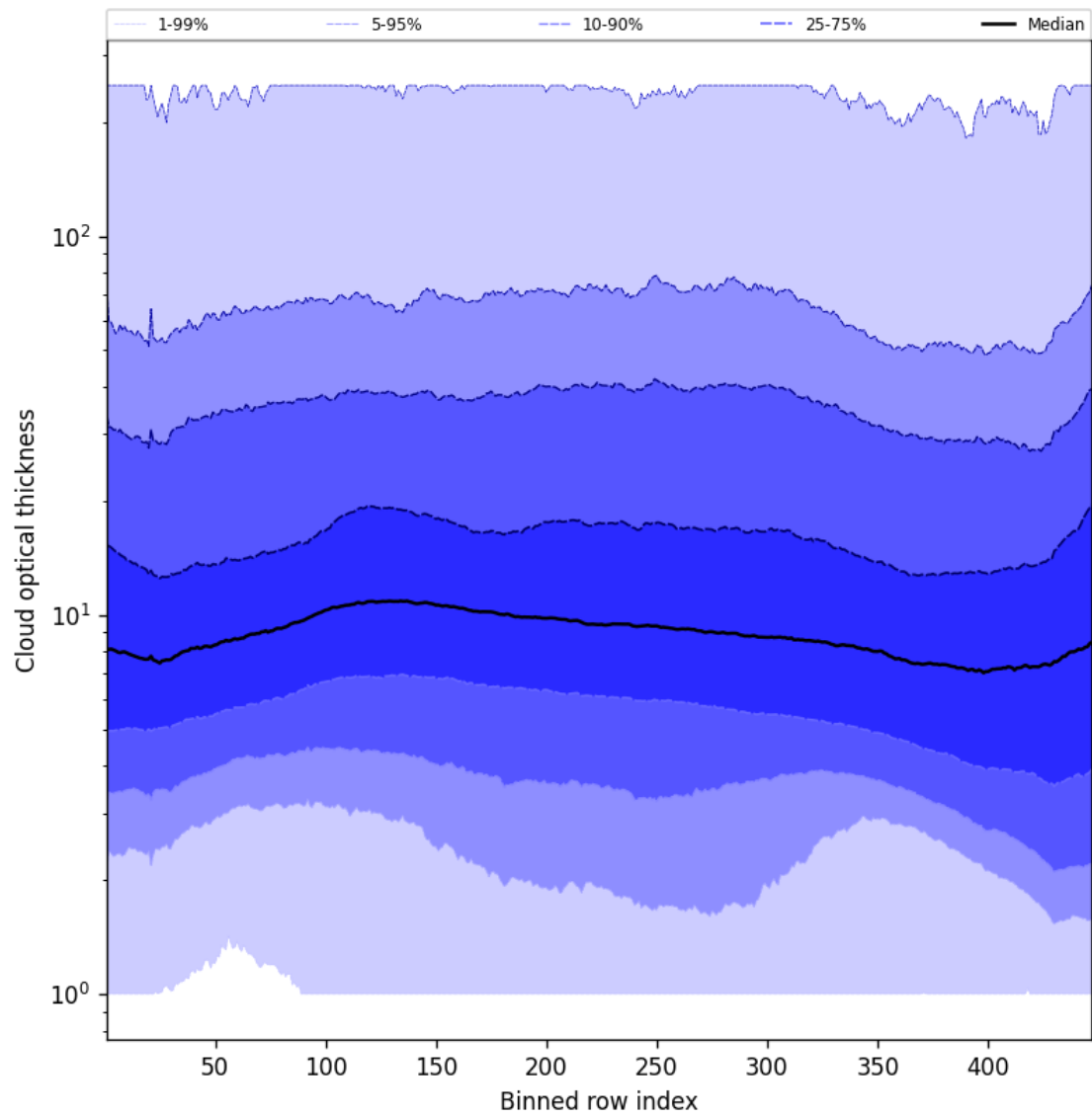
Figure 57: Along track statistics of “Cloud optical thickness” for 2024-11-09 to 2024-11-11
