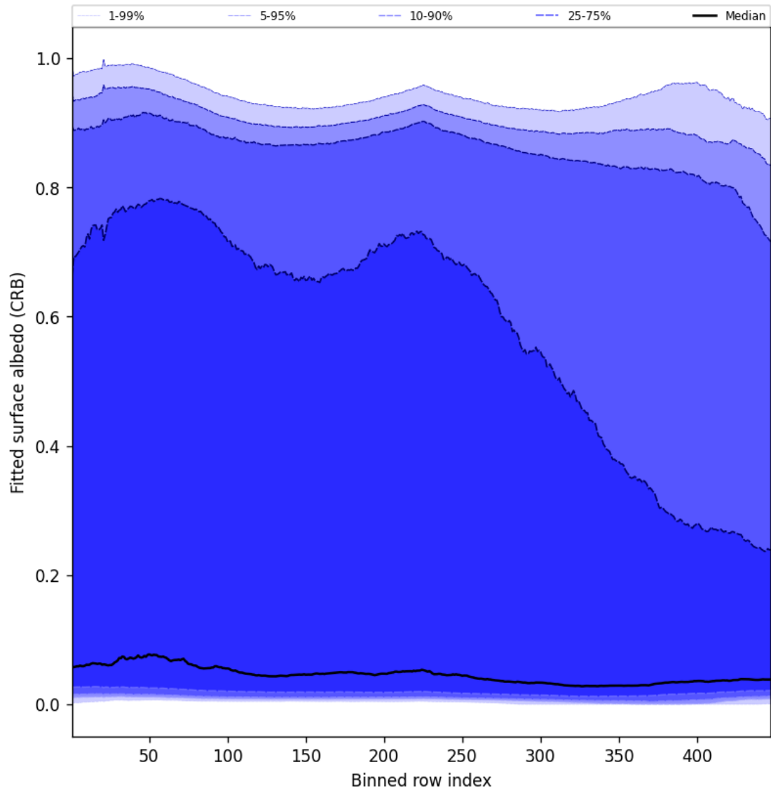
Figure 62: Along track statistics of “Fitted surface albedo (CRB)” for 2024-11-09 to 2024-11-11
