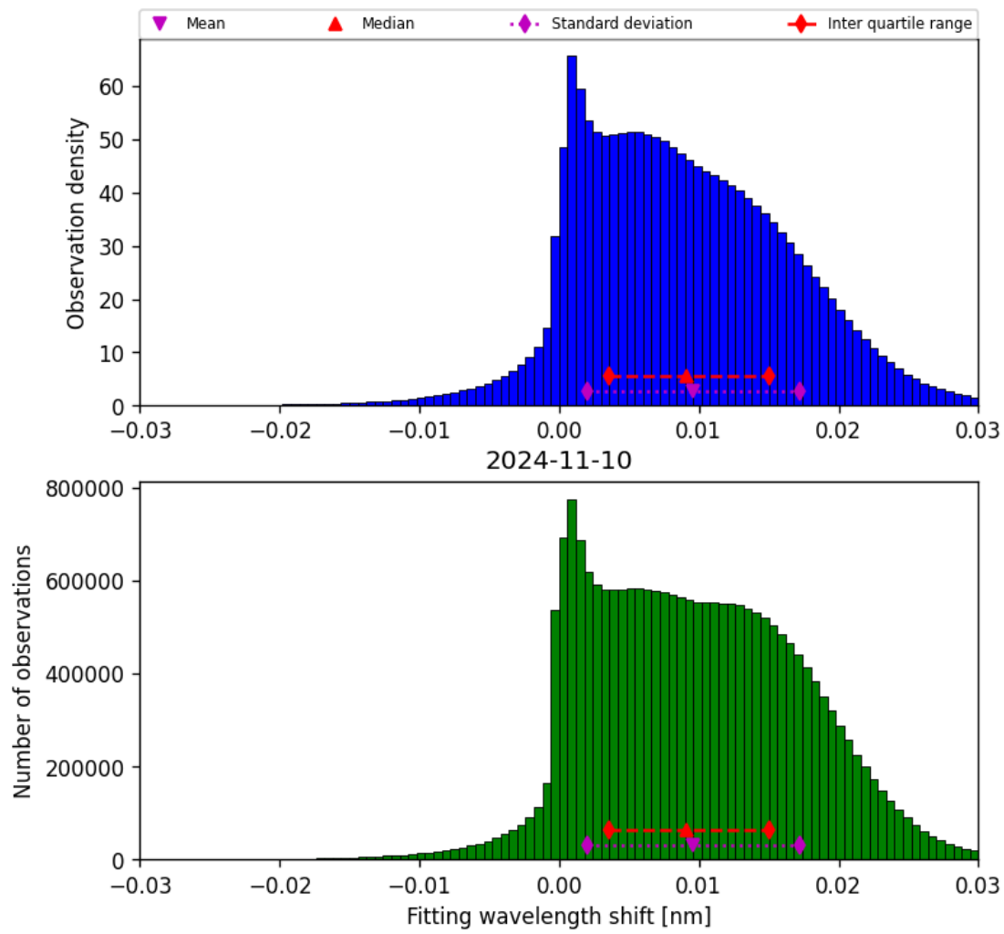
Figure 49: Histogram of “Fitting wavelength shift” for 2024-11-09 to 2024-11-11
