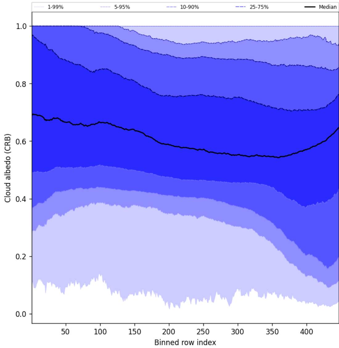
Figure 60: Along track statistics of “Cloud albedo (CRB)” for 2024-11-09 to 2024-11-11
