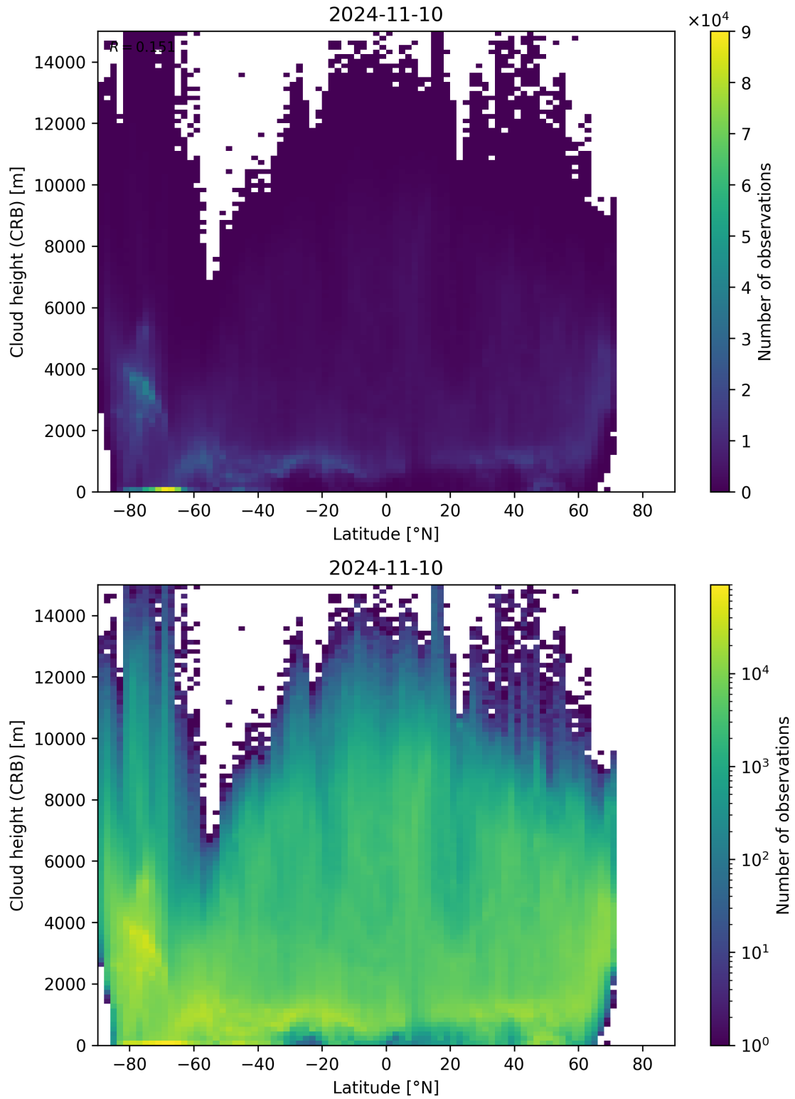
Figure 95: Scatter density plot of “Latitude” against “Cloud height (CRB)” for 2024-11-09 to 2024-11-11.
