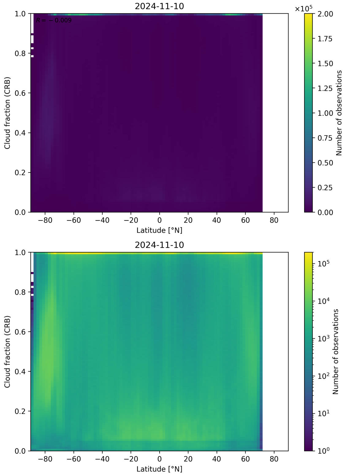
Figure 94: Scatter density plot of “Latitude” against “Cloud fraction (CRB)” for 2024-11-09 to 2024-11-11.
