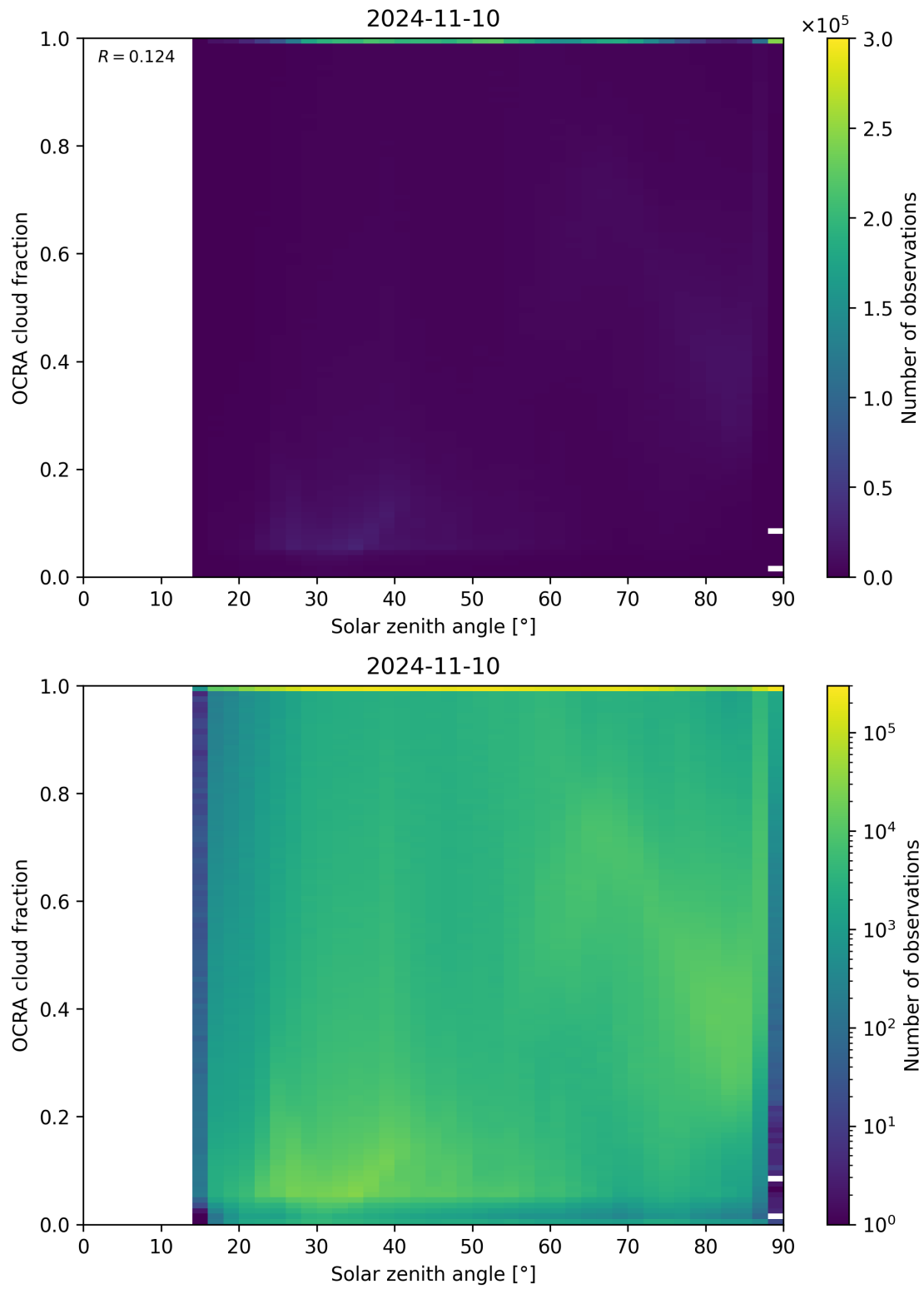
Figure 100: Scatter density plot of “Solar zenith angle” against “OCRA cloud fraction” for 2024-11-09 to 2024-11-11.
