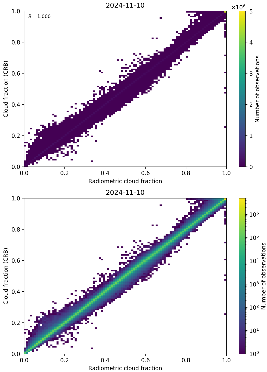
Figure 73: Scatter density plot of “Radiometric cloud fraction” against “Cloud fraction (CRB)” for 2024-11-09 to 2024-11-11.
