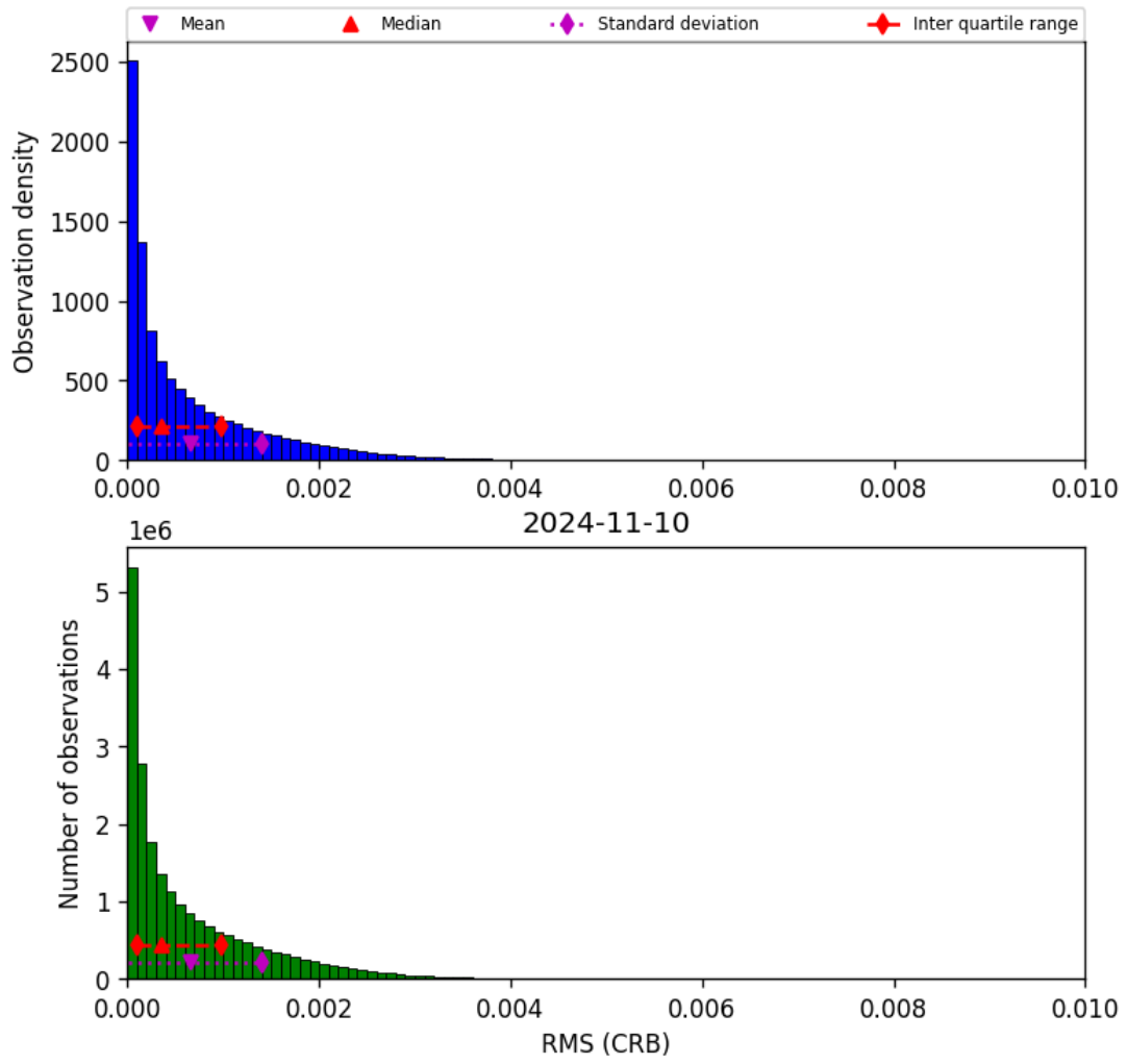
Figure 48: Histogram of “RMS (CRB)” for 2024-11-09 to 2024-11-11
