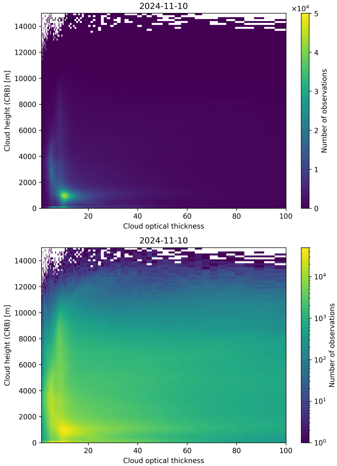
Figure 85: Scatter density plot of “Cloud optical thickness” against “Cloud height (CRB)” for 2024-11-09 to 2024-11-11.
