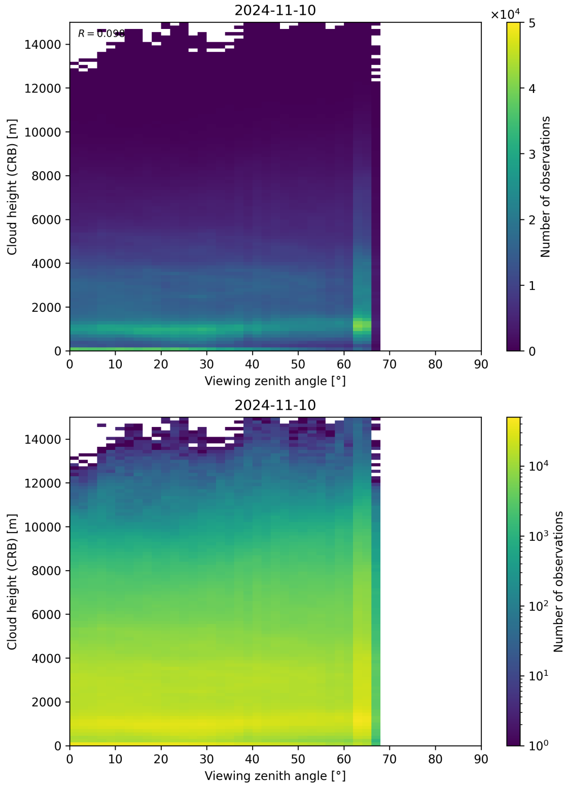
Figure 110: Scatter density plot of “Viewing zenith angle” against “Cloud height (CRB)” for 2024-11-09 to 2024-11-11.
