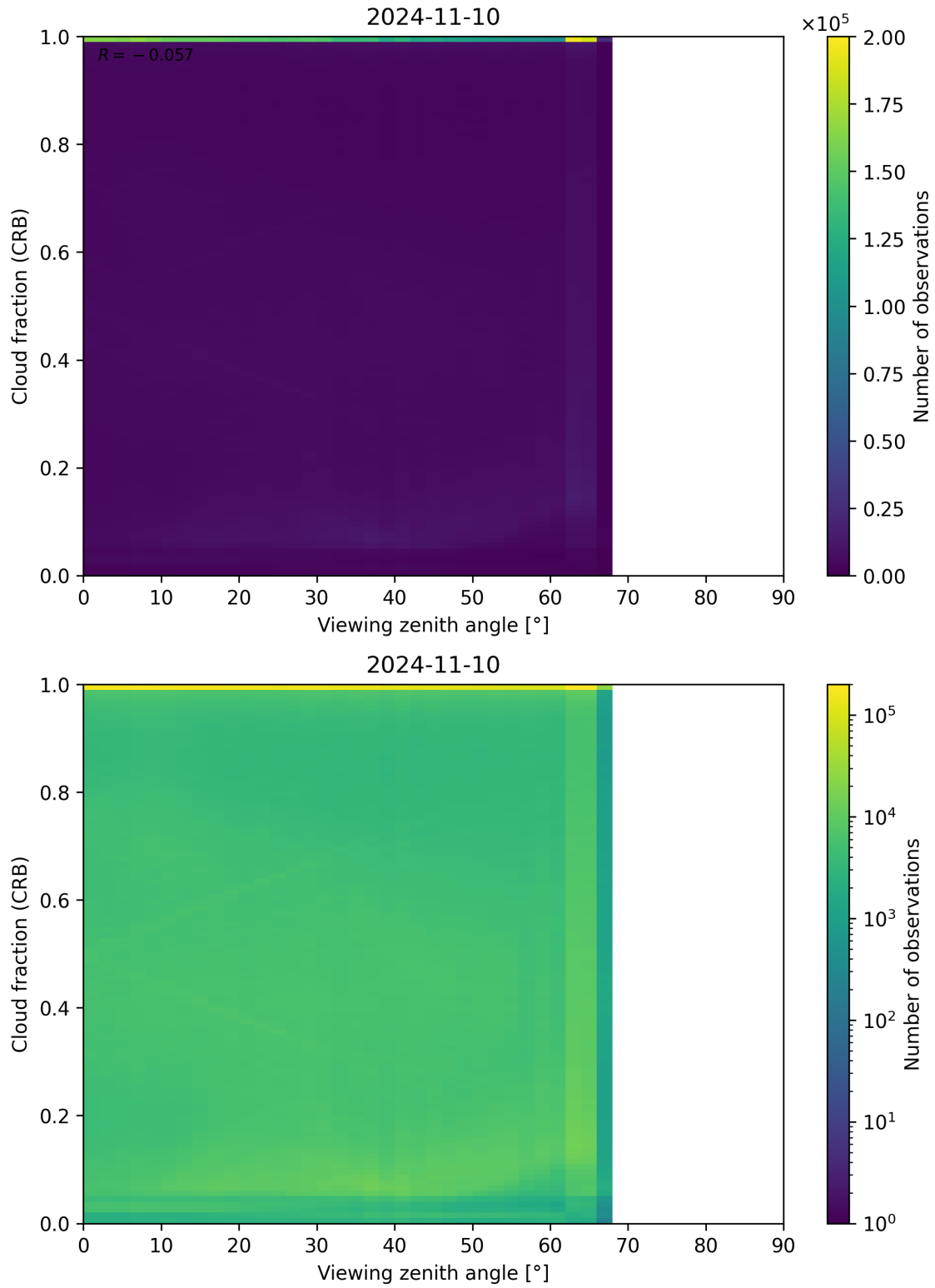
Figure 109: Scatter density plot of “Viewing zenith angle” against “Cloud fraction (CRB)” for 2024-11-09 to 2024-11-11.
