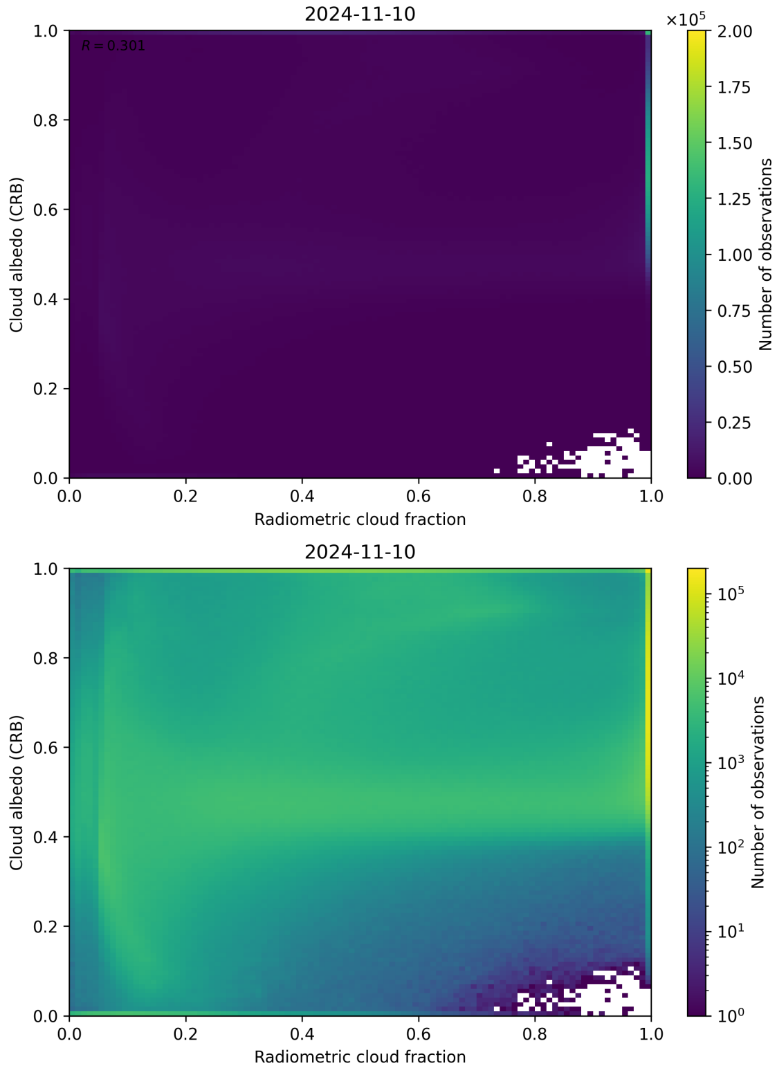
Figure 71: Scatter density plot of “Radiometric cloud fraction” against “Cloud albedo (CRB)” for 2024-11-09 to 2024-11-11.
