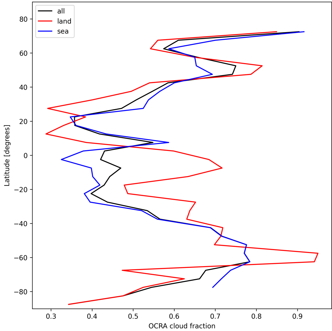
Figure 34: Zonal average of “OCRA cloud fraction” for 2024-11-09 to 2024-11-11.
