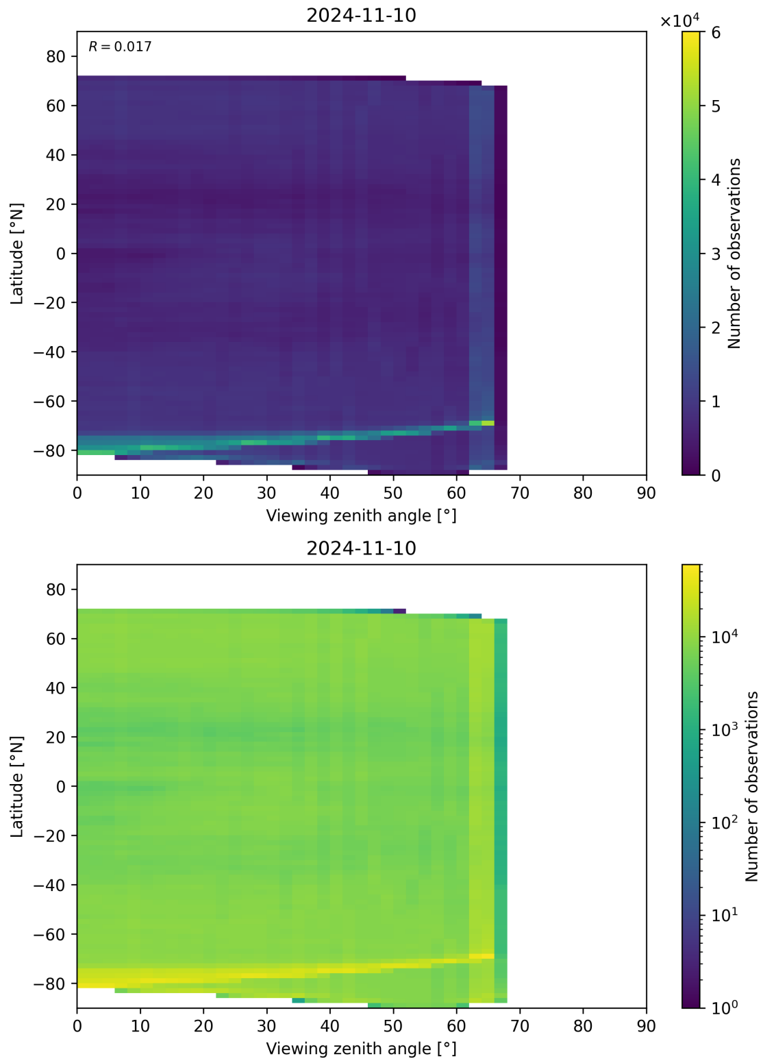
Figure 113: Scatter density plot of “Viewing zenith angle” against “Latitude” for 2024-11-09 to 2024-11-11.
