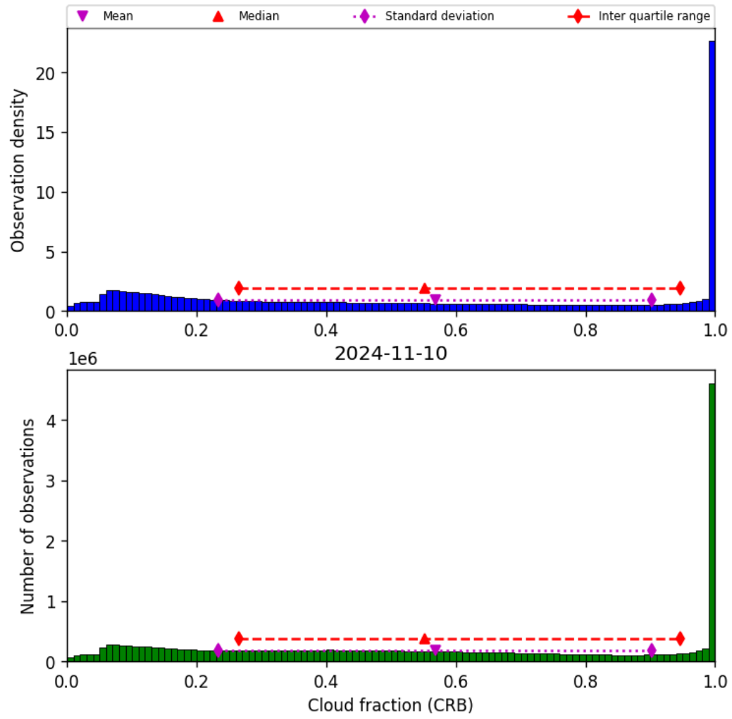
Figure 42: Histogram of “Cloud fraction (CRB)” for 2024-11-09 to 2024-11-11
