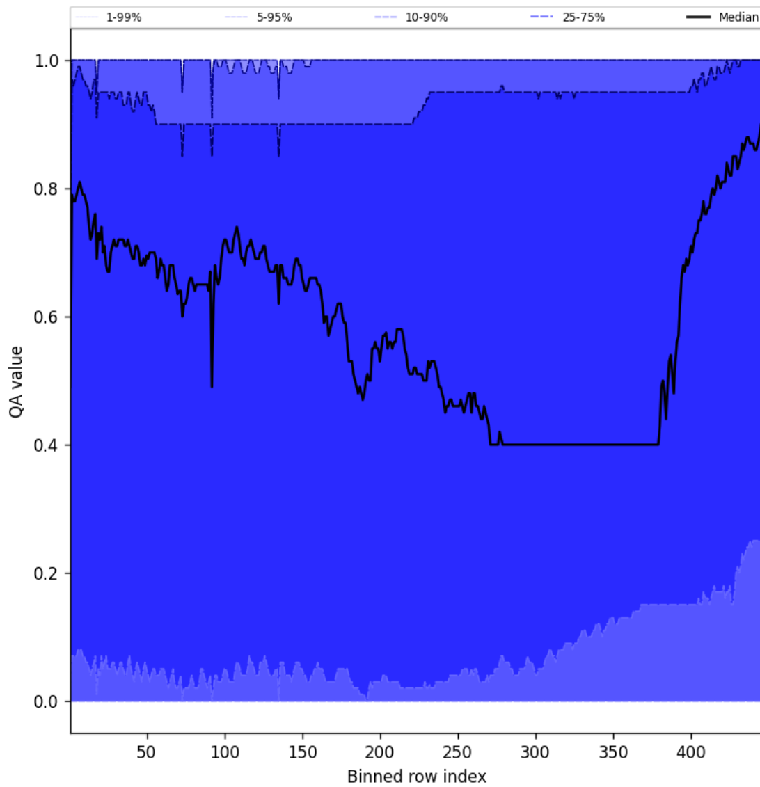
Figure 54: Along track statistics of “QA value” for 2024-11-09 to 2024-11-11
