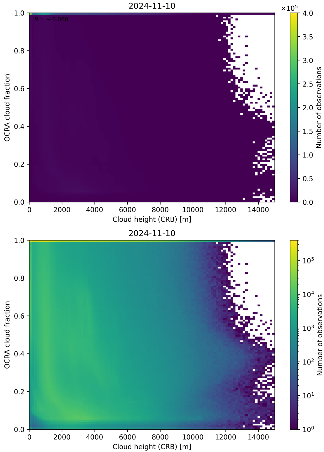
Figure 81: Scatter density plot of “Cloud height (CRB)” against “OCRA cloud fraction” for 2024-11-09 to 2024-11-11.
