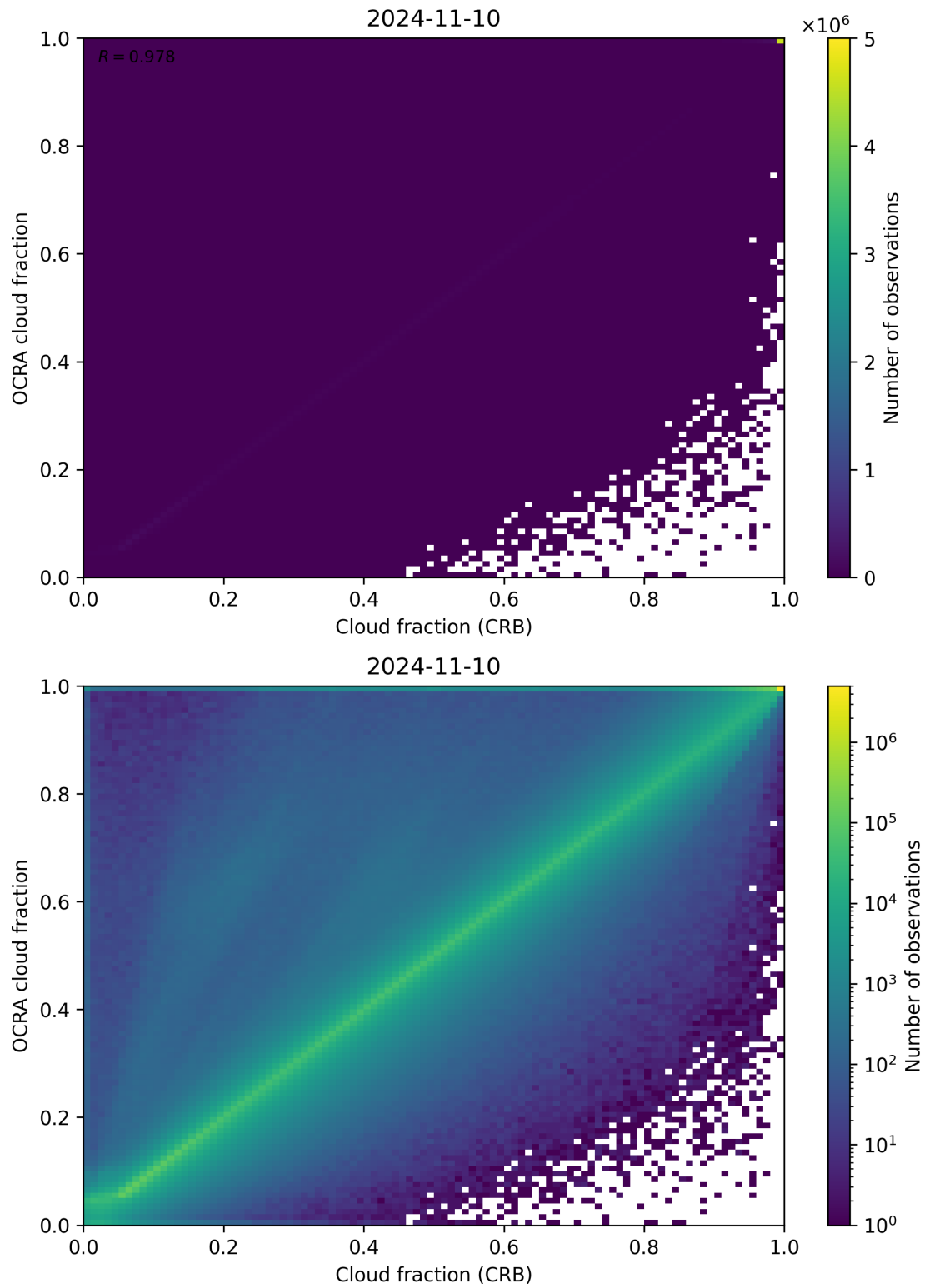
Figure 78: Scatter density plot of “Cloud fraction (CRB)” against “OCRA cloud fraction” for 2024-11-09 to 2024-11-11.
