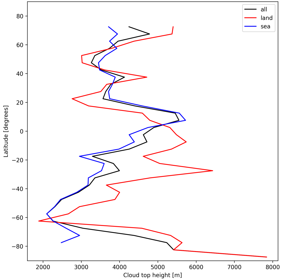
Figure 24: Zonal average of “Cloud top height” for 2024-11-09 to 2024-11-11.
