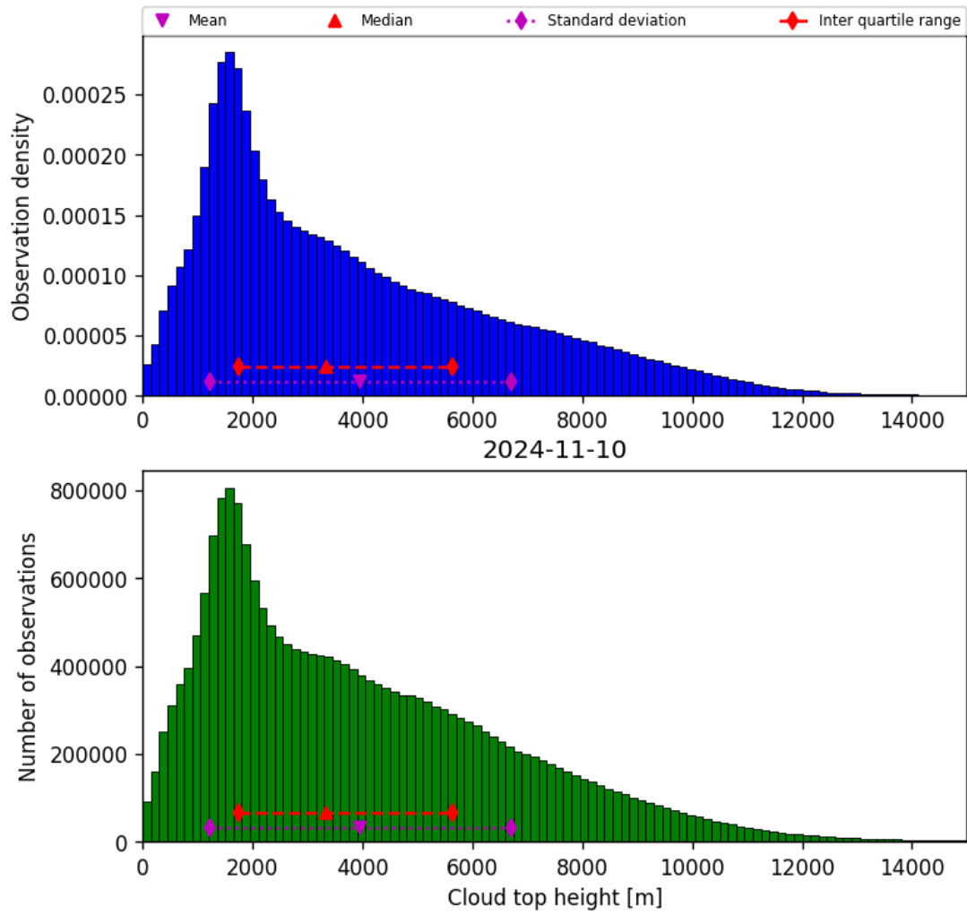
Figure 40: Histogram of “Cloud top height” for 2024-11-09 to 2024-11-11
