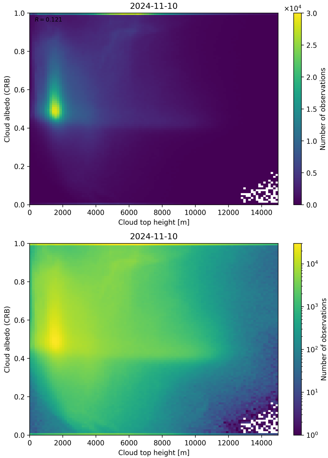
Figure 86: Scatter density plot of “Cloud top height” against “Cloud albedo (CRB)” for 2024-11-09 to 2024-11-11.
