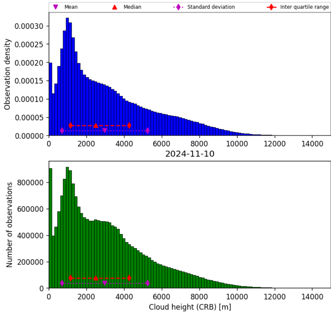
Figure 43: Histogram of “Cloud height (CRB)” for 2024-11-09 to 2024-11-11
