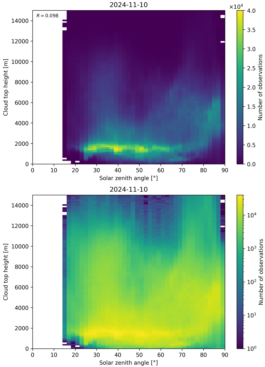
Figure 104: Scatter density plot of “Solar zenith angle” against “Cloud top height” for 2024-11-09 to 2024-11-11.
