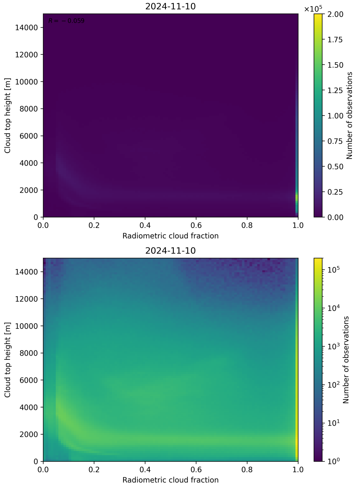
Figure 76: Scatter density plot of “Radiometric cloud fraction” against “Cloud top height” for 2024-11-09 to 2024-11-11.
