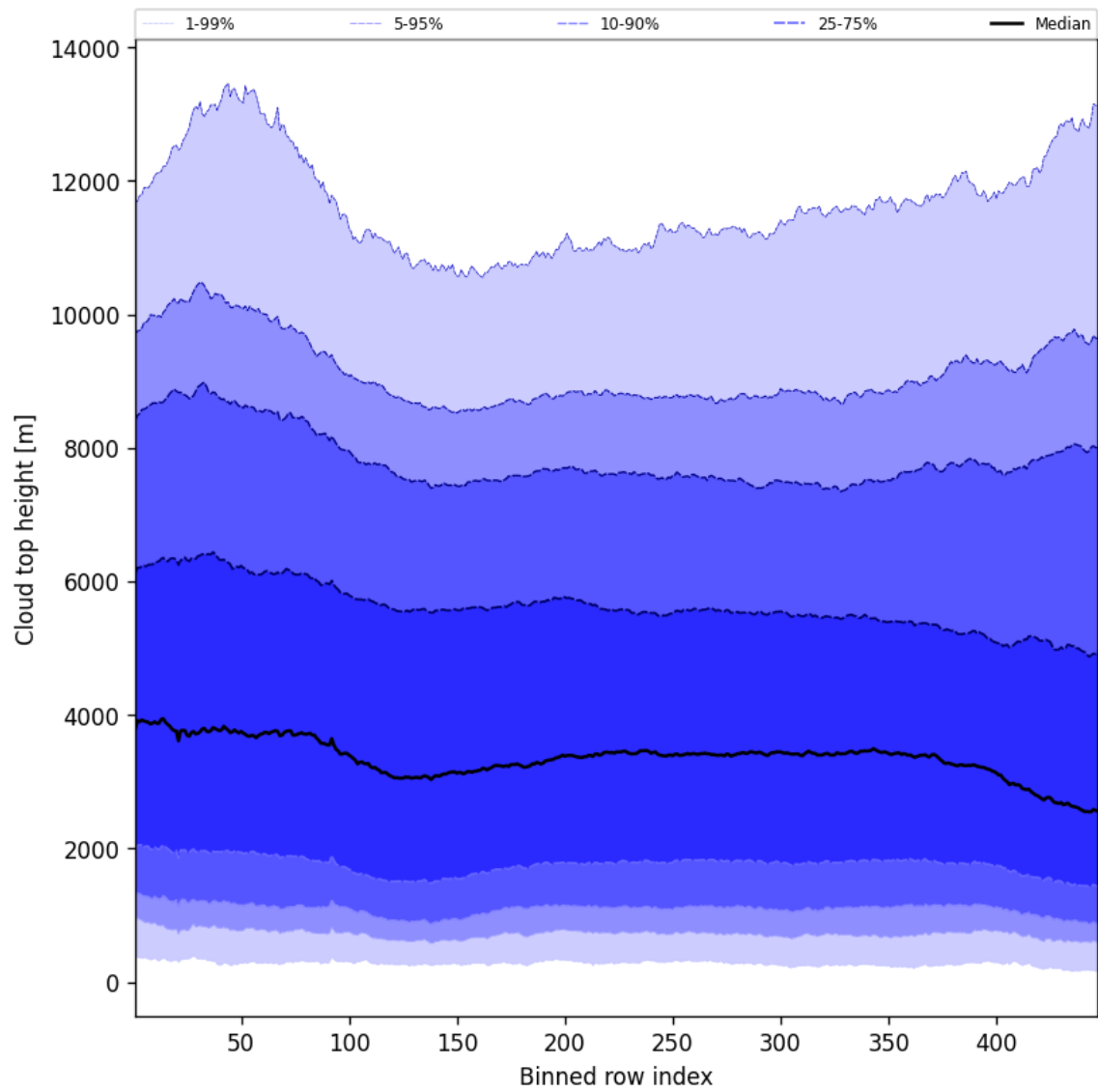
Figure 56: Along track statistics of “Cloud top height” for 2024-11-09 to 2024-11-11
