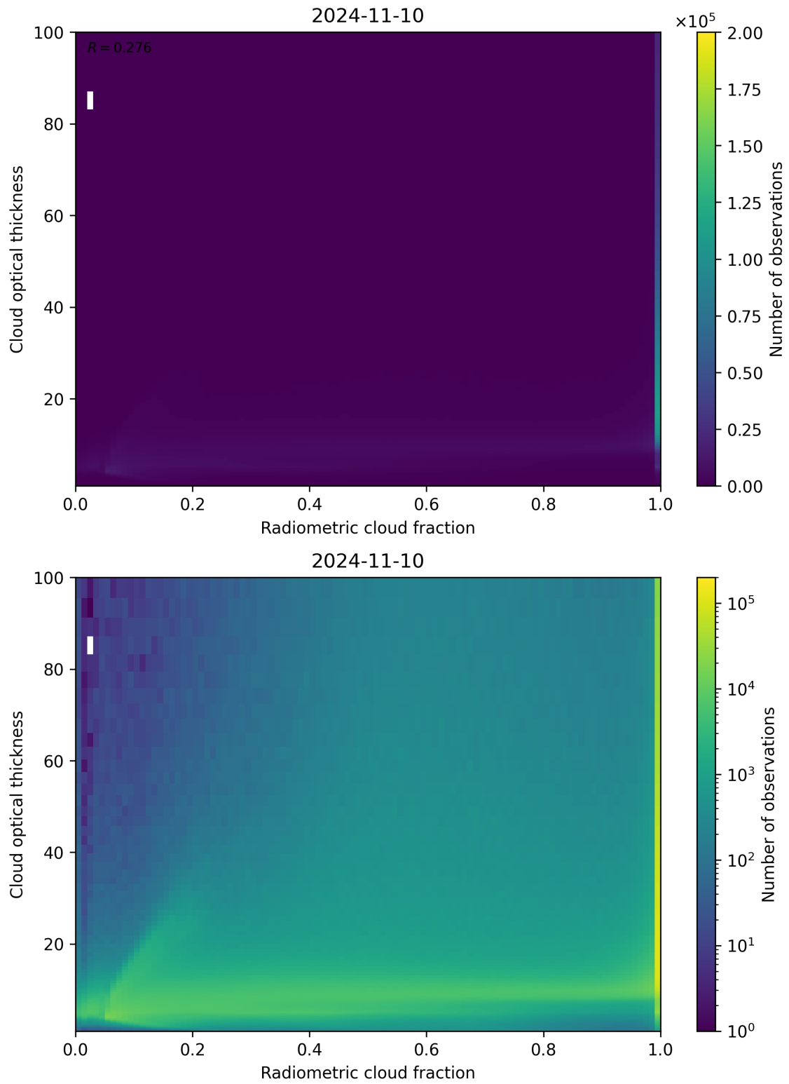
Figure 75: Scatter density plot of “Radiometric cloud fraction” against “Cloud optical thickness” for 2024-11-09 to 2024-11-11.
