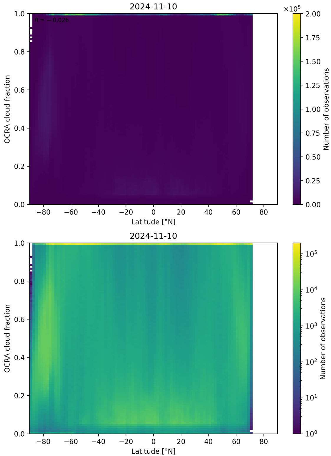
Figure 93: Scatter density plot of “Latitude” against “OCRA cloud fraction” for 2024-11-09 to 2024-11-11.
