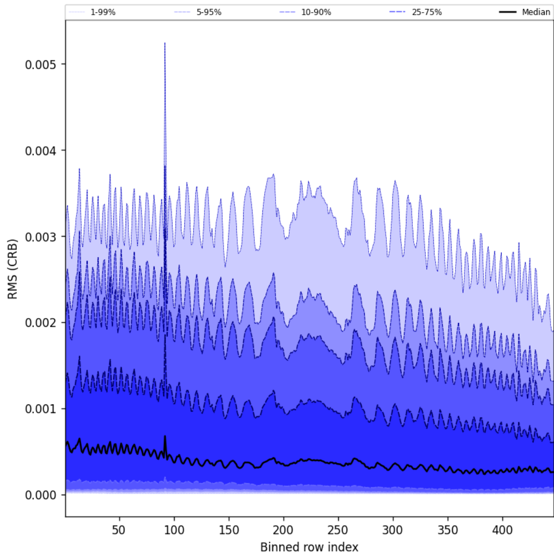
Figure 64: Along track statistics of “RMS (CRB)” for 2024-11-09 to 2024-11-11
