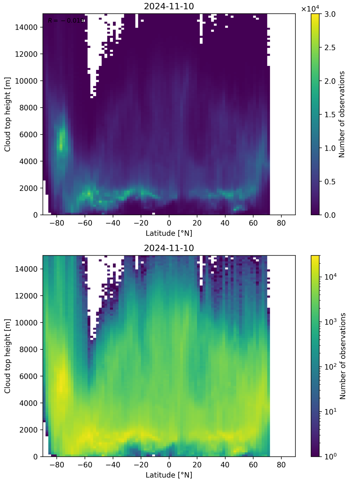
Figure 97: Scatter density plot of “Latitude” against “Cloud top height” for 2024-11-09 to 2024-11-11.
