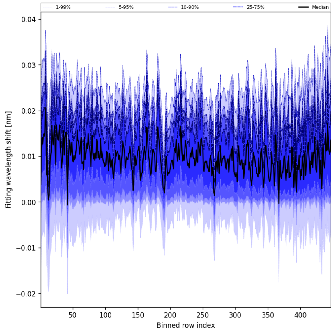
Figure 65: Along track statistics of “Fitting wavelength shift” for 2024-11-12 to 2024-11-14
