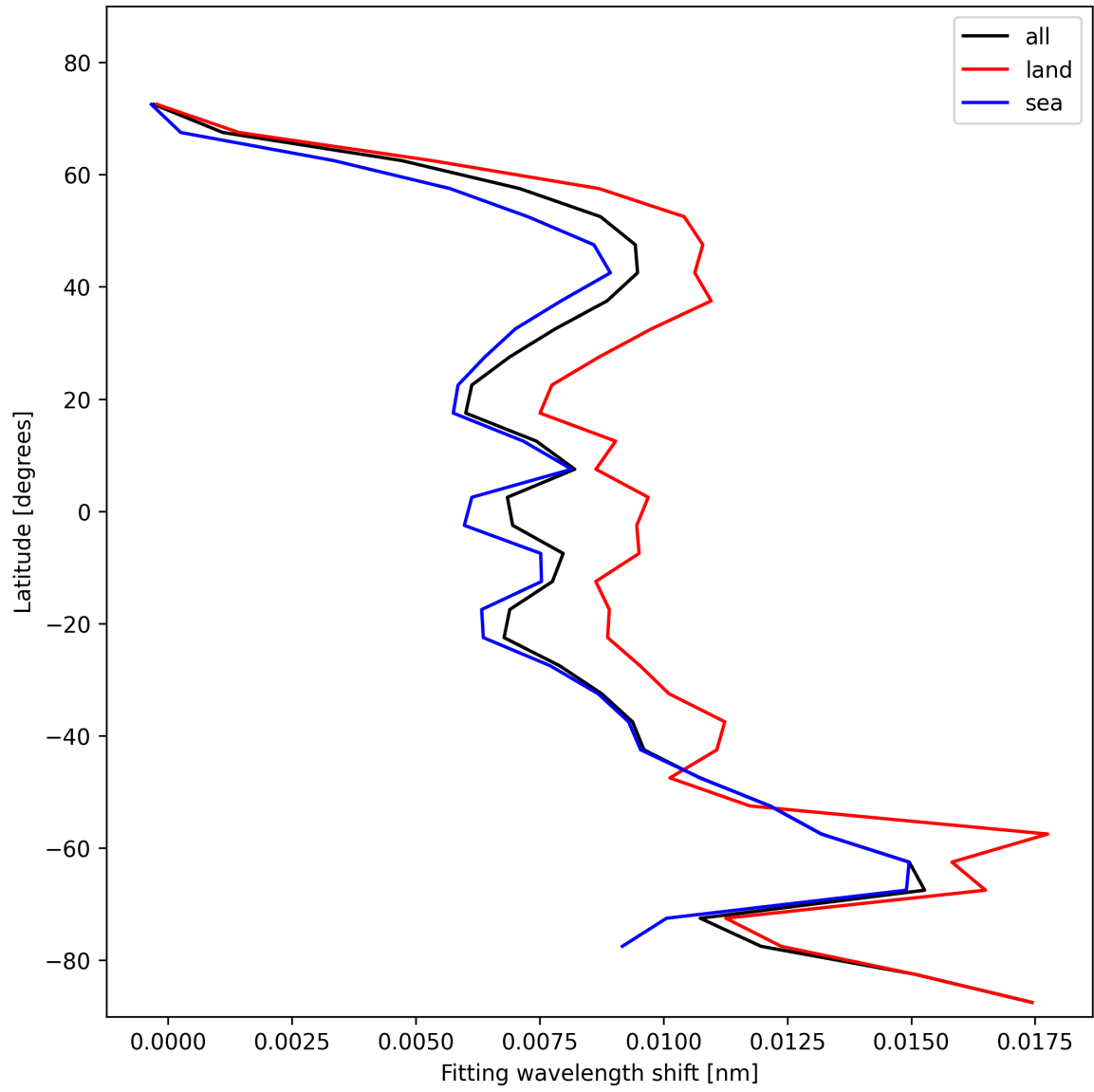
Figure 33: Zonal average of “Fitting wavelength shift” for 2024-11-12 to 2024-11-14.
