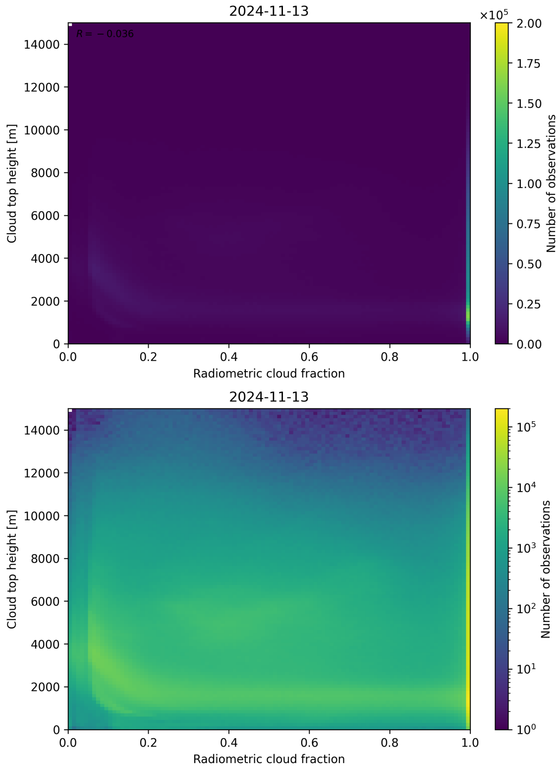
Figure 76: Scatter density plot of “Radiometric cloud fraction” against “Cloud top height” for 2024-11-12 to 2024-11-14.
