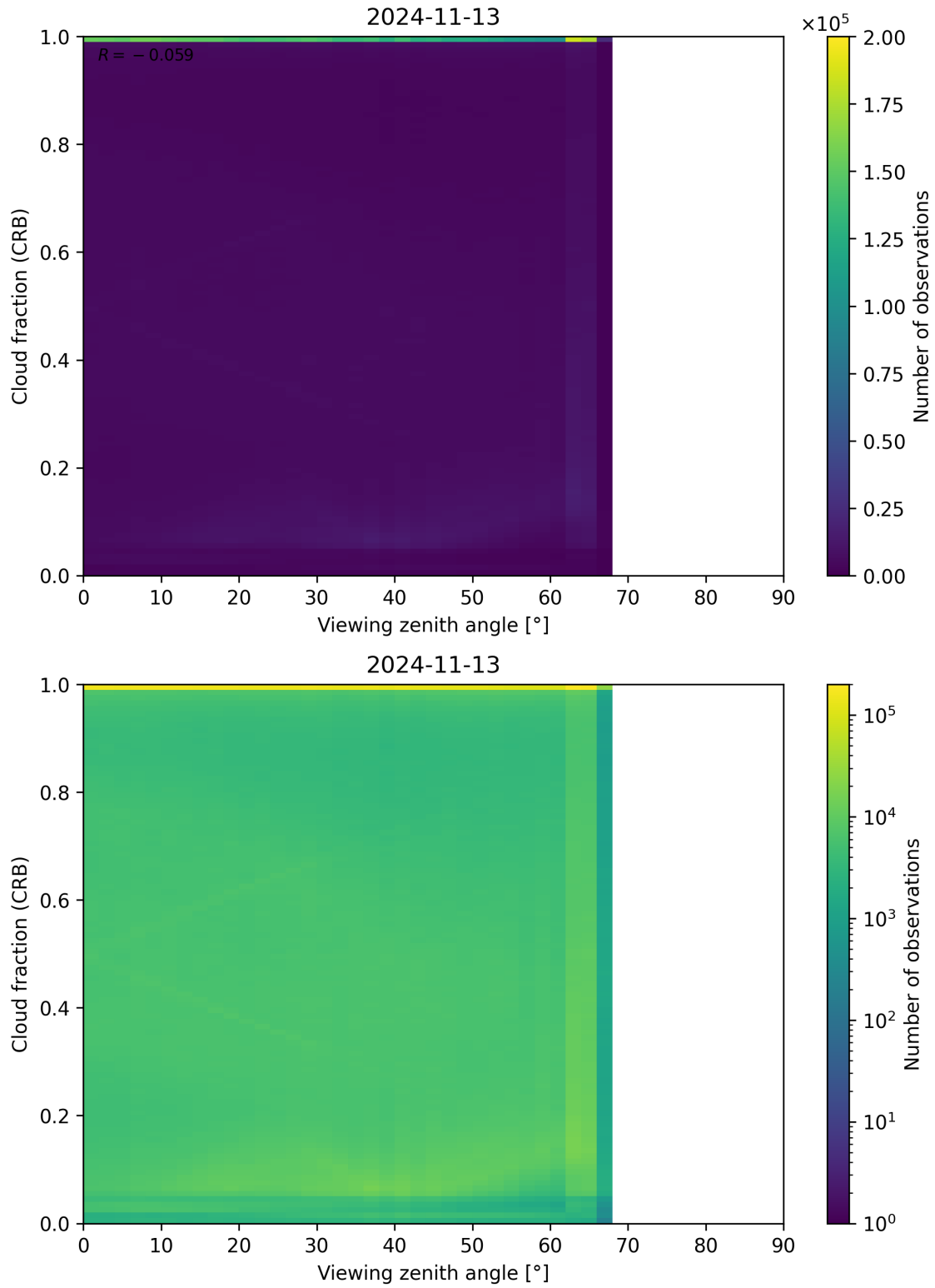
Figure 109: Scatter density plot of “Viewing zenith angle” against “Cloud fraction (CRB)” for 2024-11-12 to 2024-11-14.
