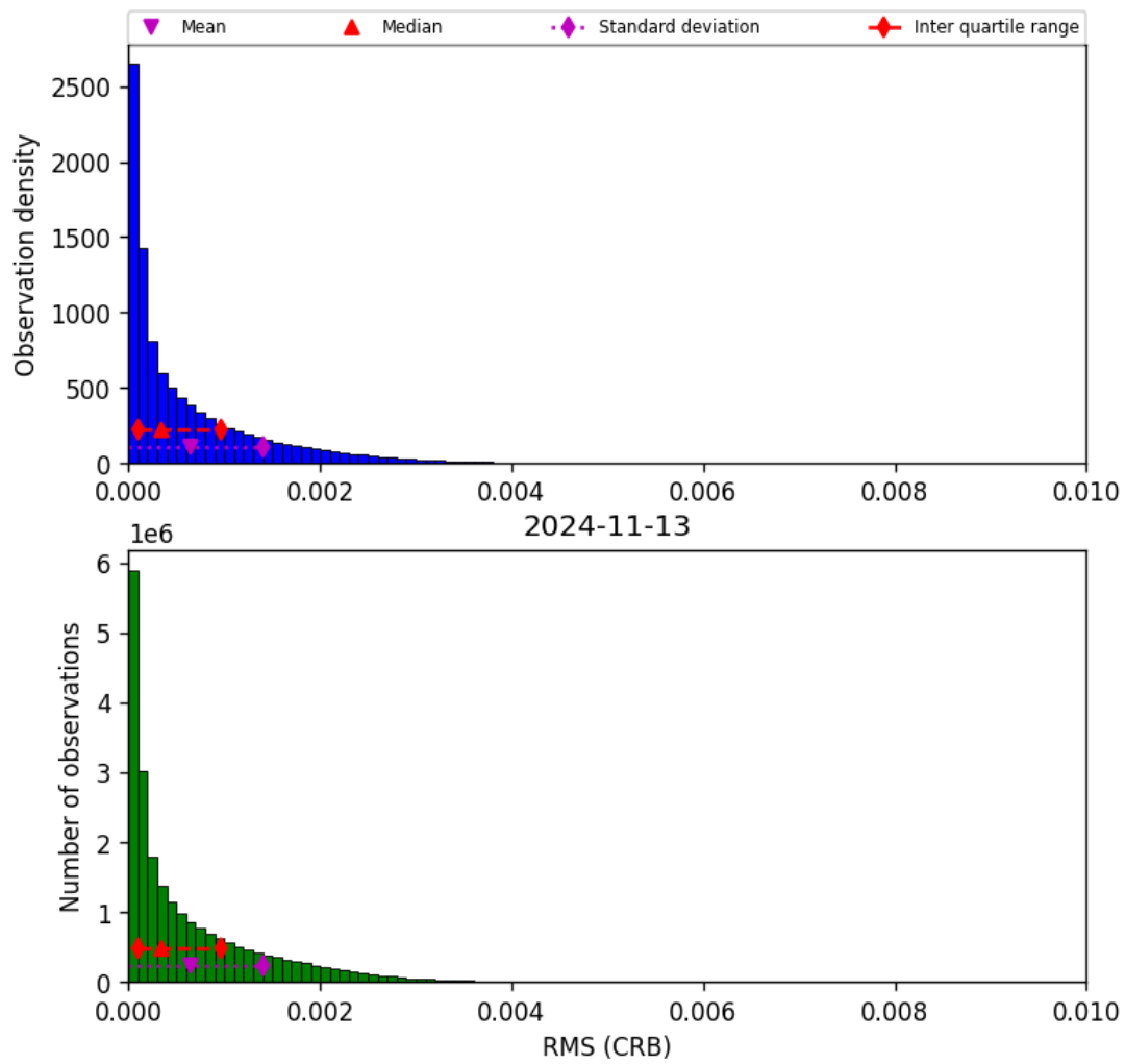
Figure 48: Histogram of “RMS (CRB)” for 2024-11-12 to 2024-11-14
