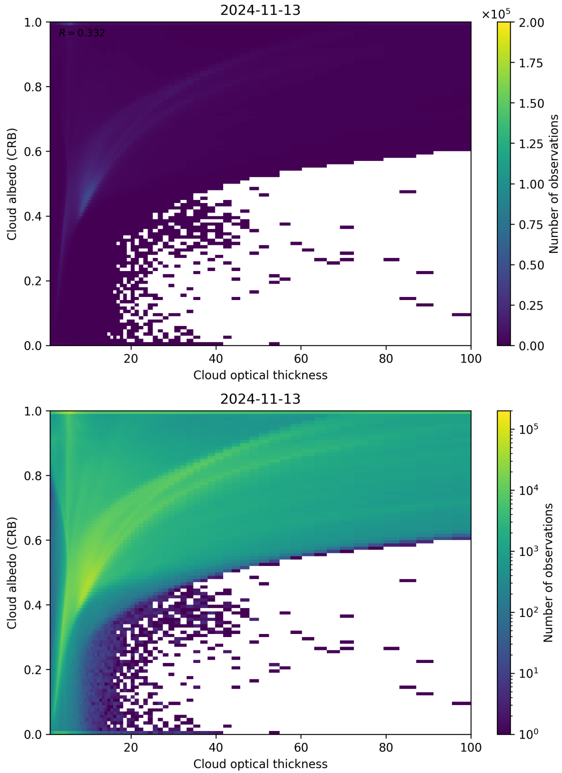
Figure 82: Scatter density plot of “Cloud optical thickness” against “Cloud albedo (CRB)” for 2024-11-12 to 2024-11-14.
