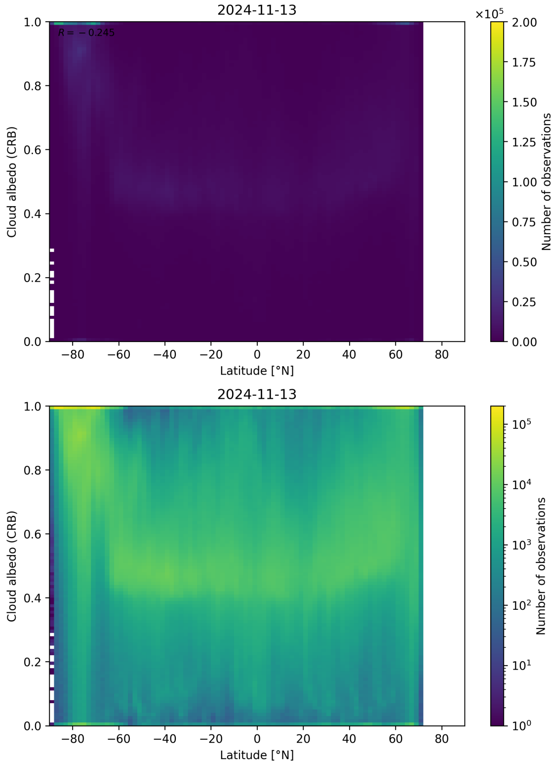
Figure 91: Scatter density plot of “Latitude” against “Cloud albedo (CRB)” for 2024-11-12 to 2024-11-14.
