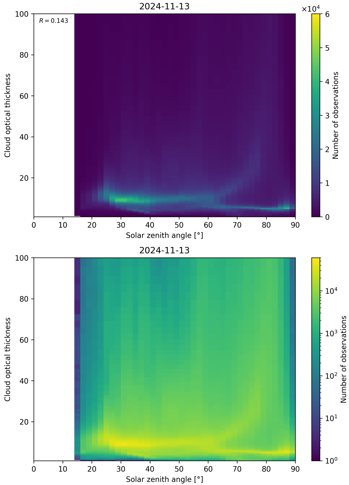
Figure 103: Scatter density plot of “Solar zenith angle” against “Cloud optical thickness” for 2024-11-12 to 2024-11-14.
