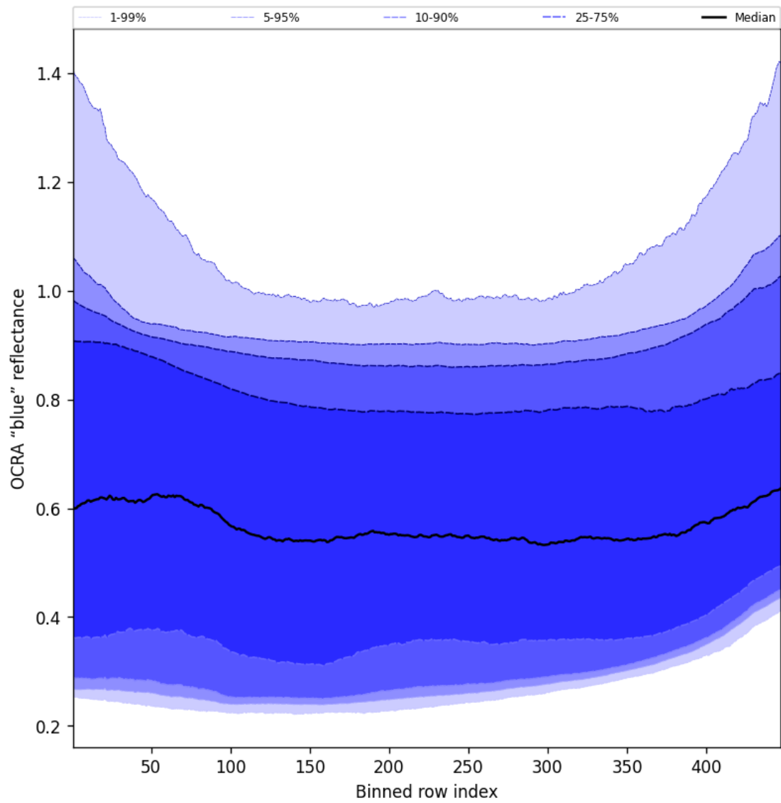
Figure 67: Along track statistics of “OCRA “blue” reflectance” for 2024-11-12 to 2024-11-14
