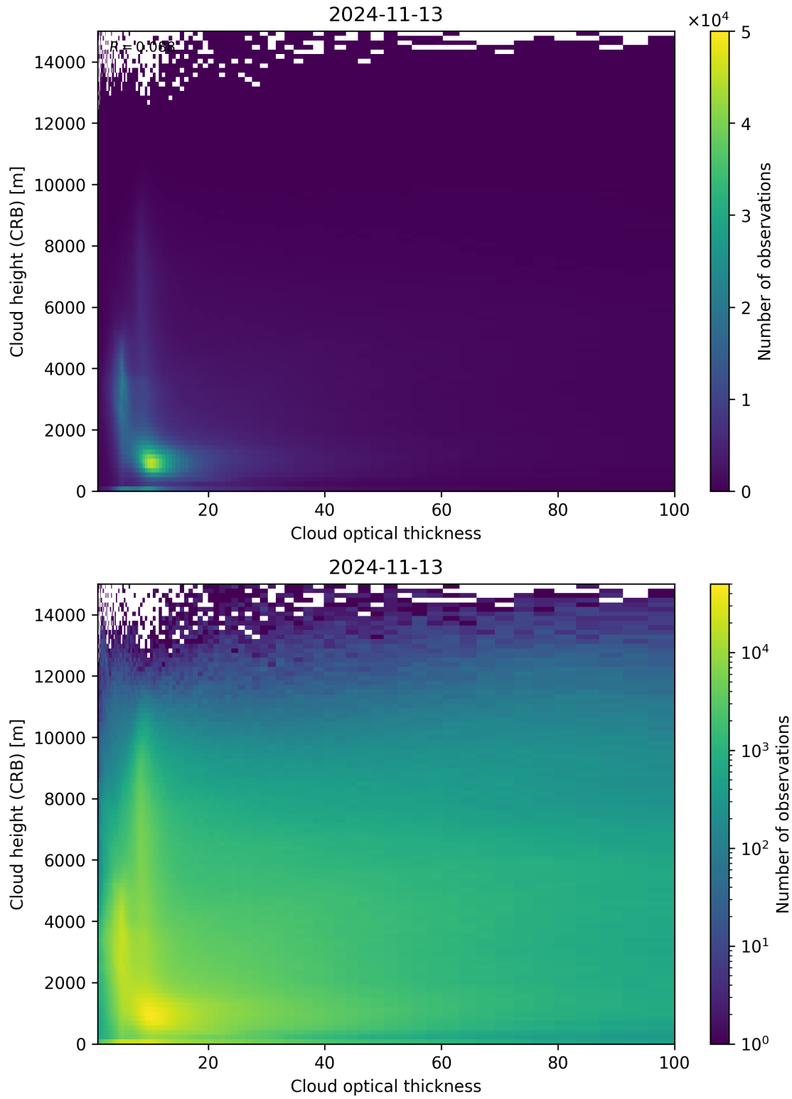
Figure 85: Scatter density plot of “Cloud optical thickness” against “Cloud height (CRB)” for 2024-11-12 to 2024-11-14.
