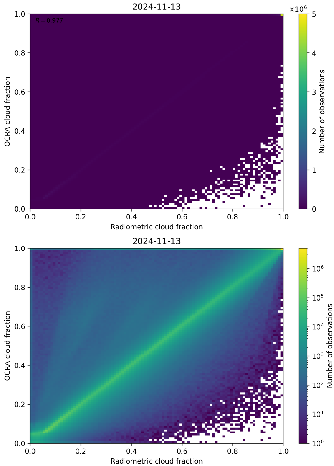
Figure 72: Scatter density plot of “Radiometric cloud fraction” against “OCRA cloud fraction” for 2024-11-12 to 2024-11-14.
