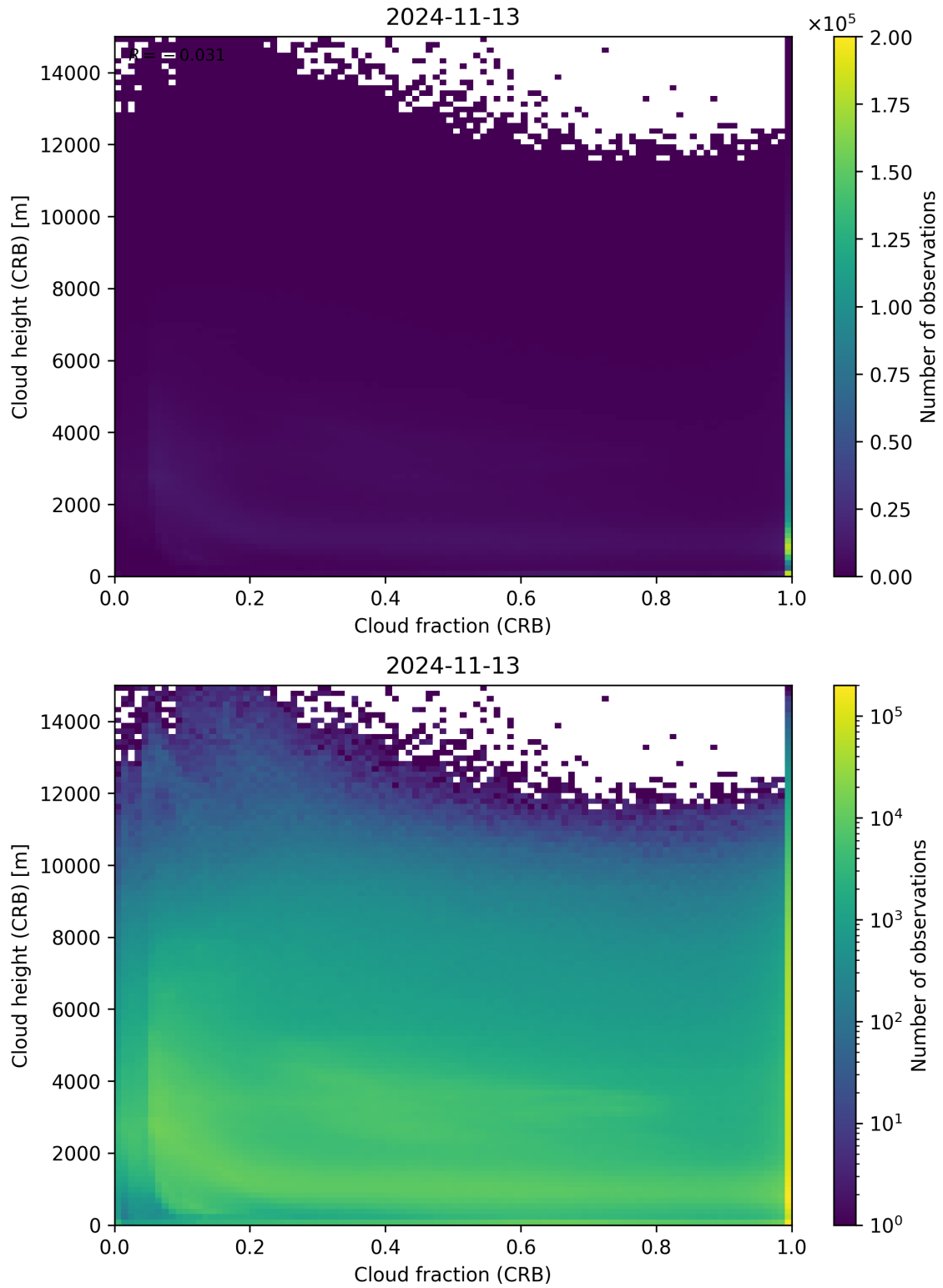
Figure 79: Scatter density plot of “Cloud fraction (CRB)” against “Cloud height (CRB)” for 2024-11-12 to 2024-11-14.
