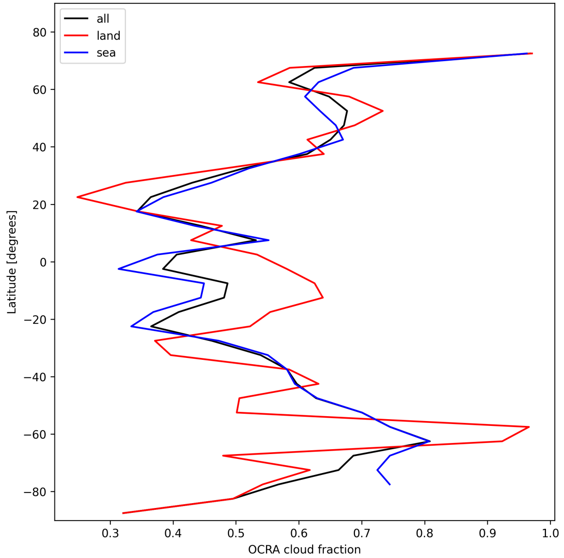
Figure 34: Zonal average of “OCRA cloud fraction” for 2024-11-12 to 2024-11-14.
