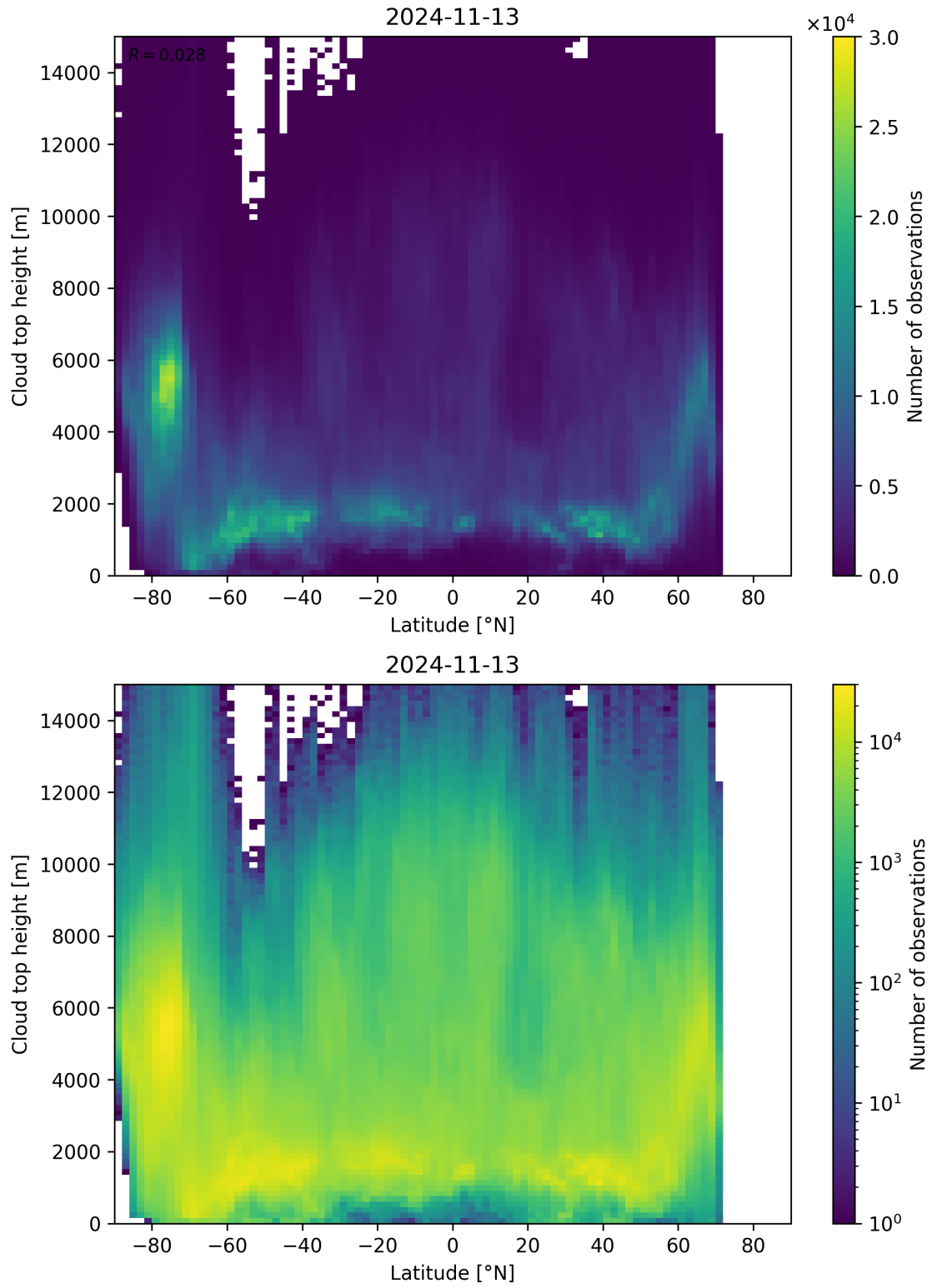
Figure 97: Scatter density plot of “Latitude” against “Cloud top height” for 2024-11-12 to 2024-11-14.
