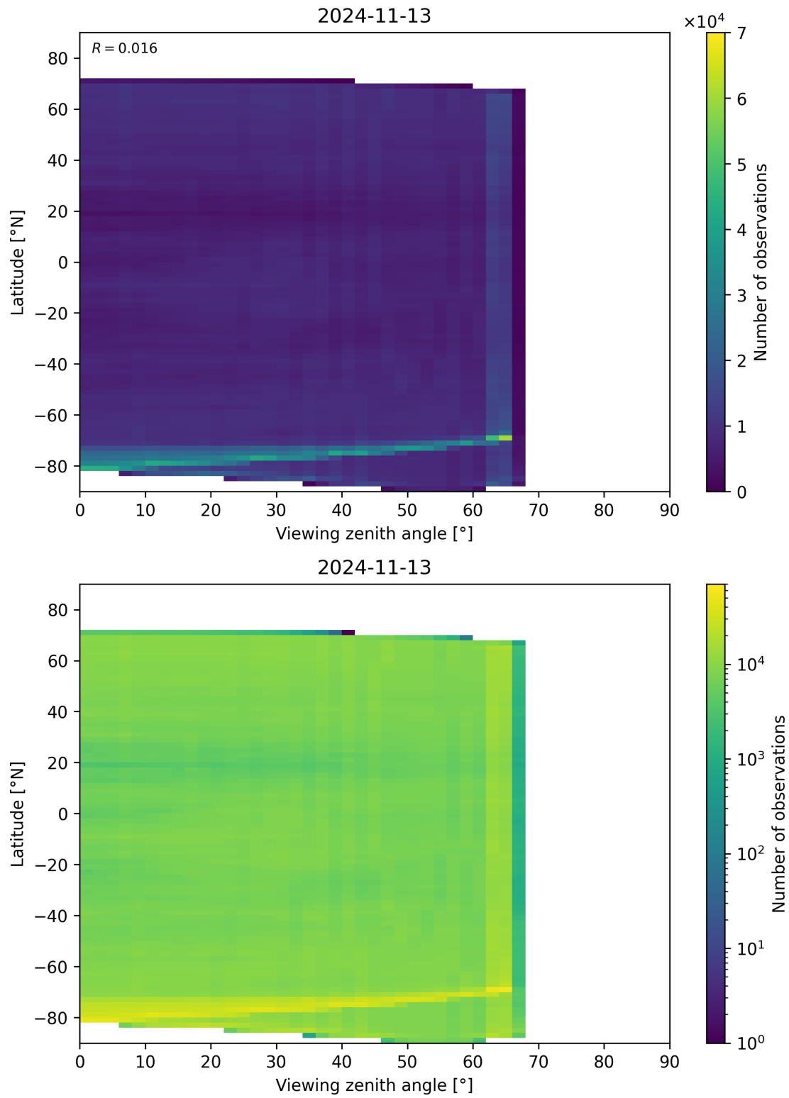
Figure 113: Scatter density plot of “Viewing zenith angle” against “Latitude” for 2024-11-12 to 2024-11-14.
