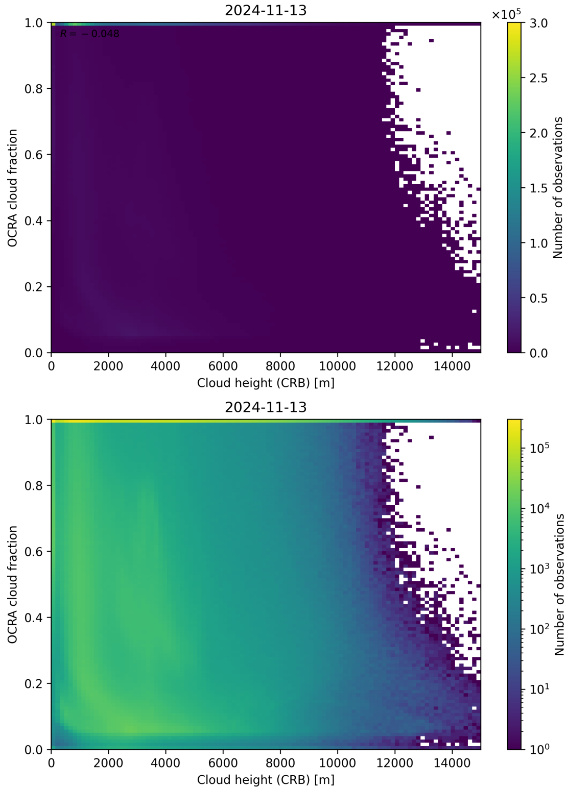
Figure 81: Scatter density plot of “Cloud height (CRB)” against “OCRA cloud fraction” for 2024-11-12 to 2024-11-14.
