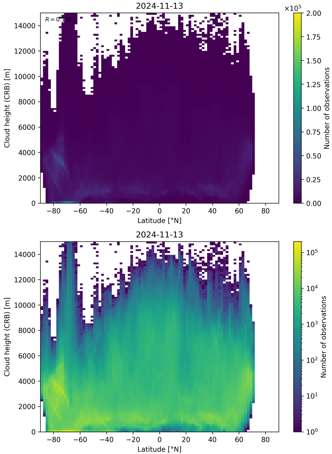
Figure 95: Scatter density plot of “Latitude” against “Cloud height (CRB)” for 2024-11-12 to 2024-11-14.
