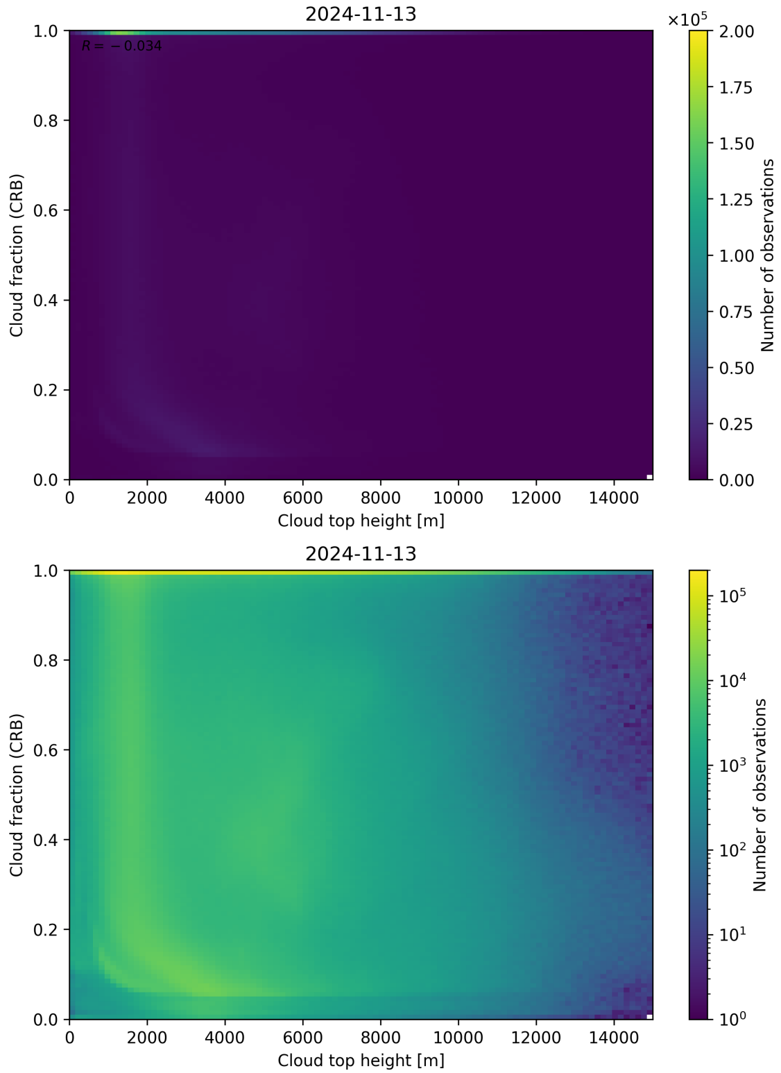
Figure 88: Scatter density plot of “Cloud top height” against “Cloud fraction (CRB)” for 2024-11-12 to 2024-11-14.
