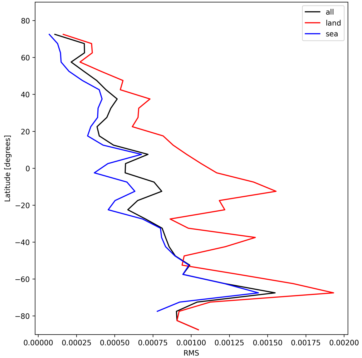
Figure 31: Zonal average of “RMS” for 2024-11-12 to 2024-11-14.
