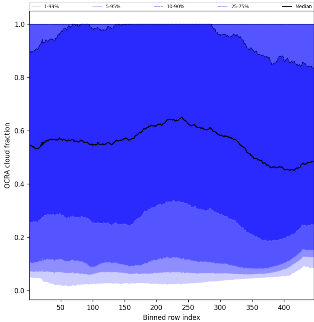
Figure 66: Along track statistics of “OCRA cloud fraction” for 2024-11-12 to 2024-11-14
