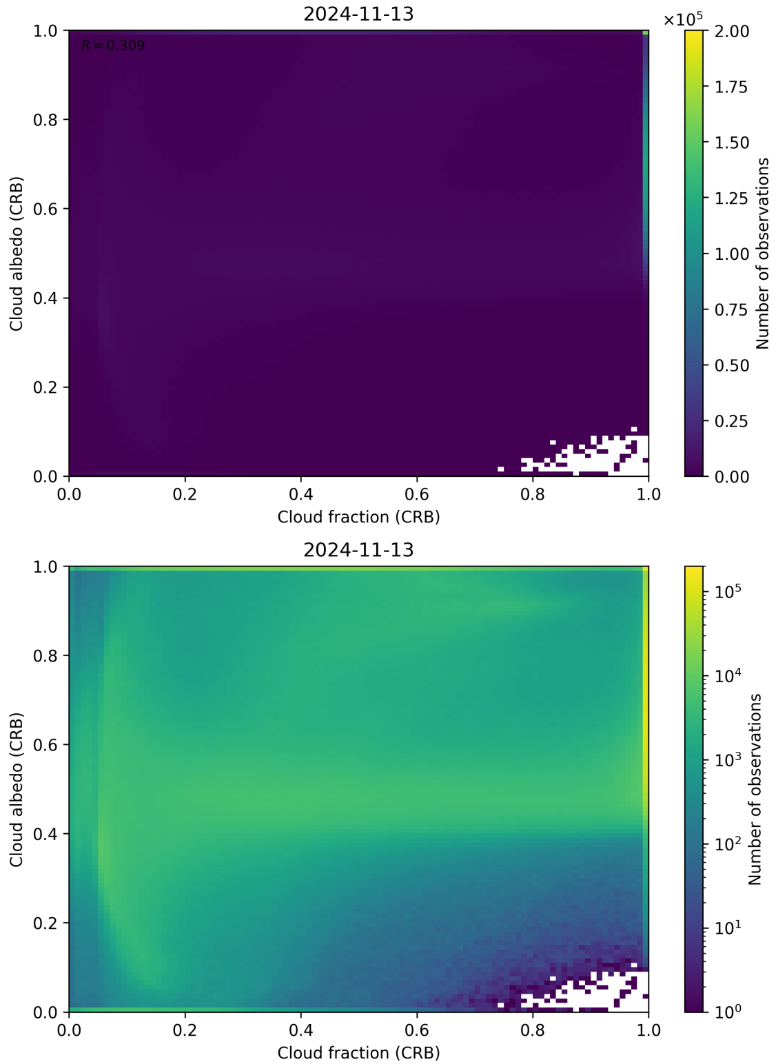
Figure 77: Scatter density plot of “Cloud fraction (CRB)” against “Cloud albedo (CRB)” for 2024-11-12 to 2024-11-14.
