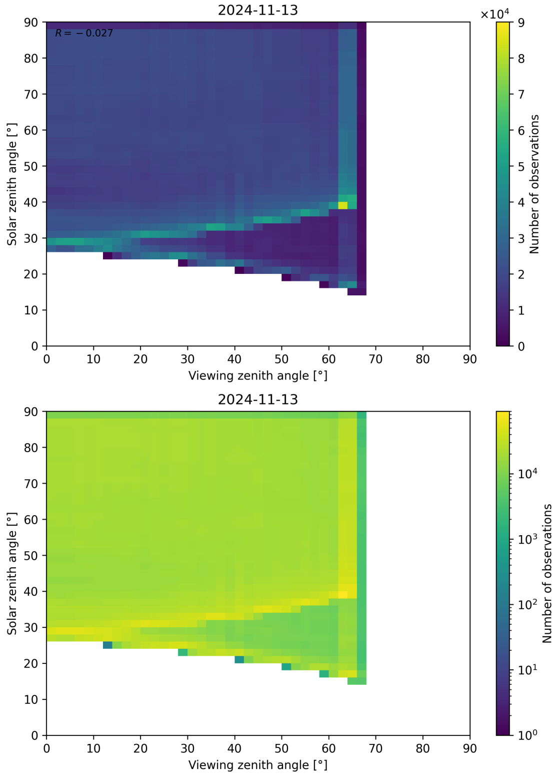
Figure 114: Scatter density plot of “Viewing zenith angle” against “Solar zenith angle” for 2024-11-12 to 2024-11-14.
