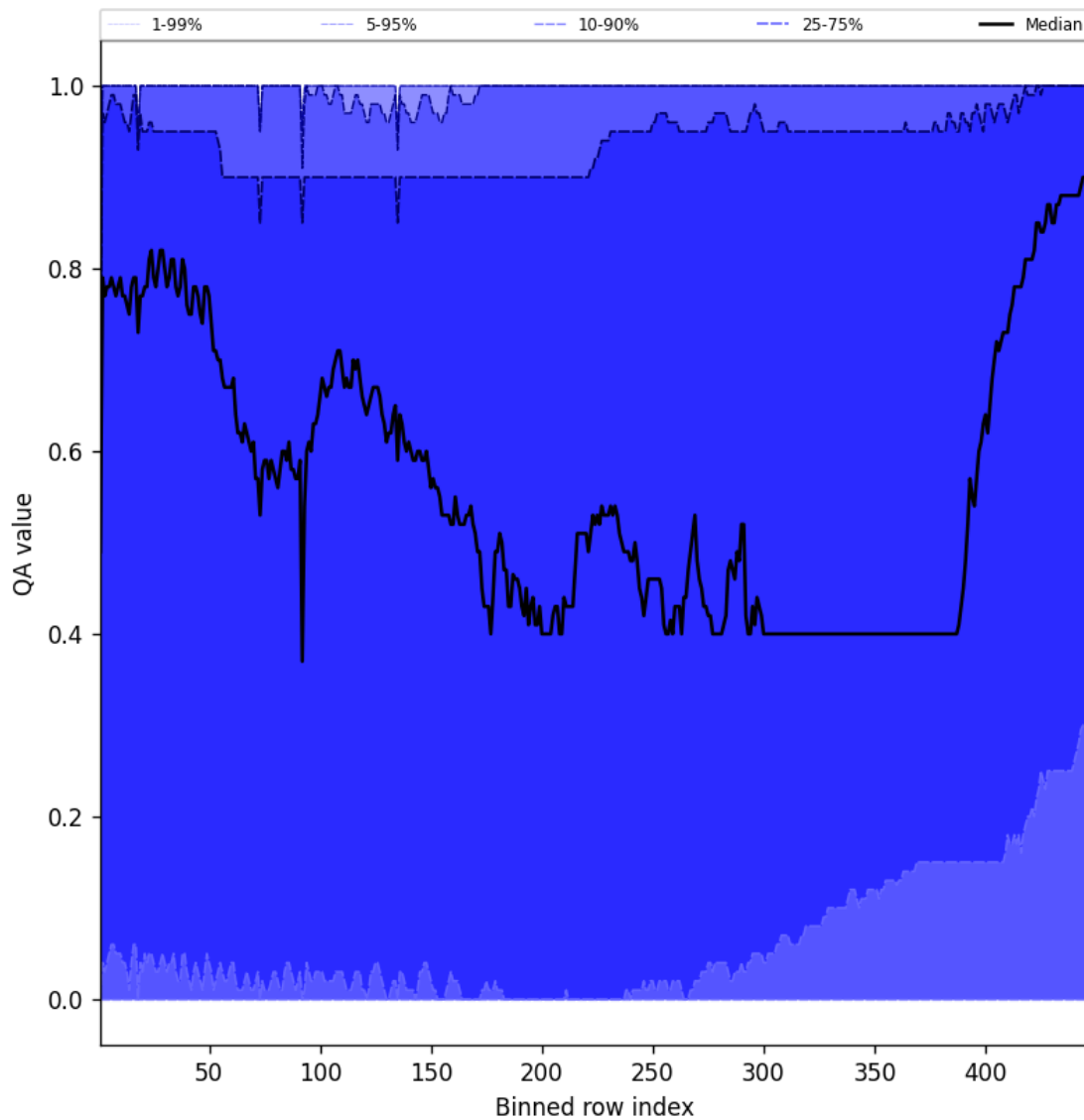
Figure 54: Along track statistics of “QA value” for 2024-11-12 to 2024-11-14
