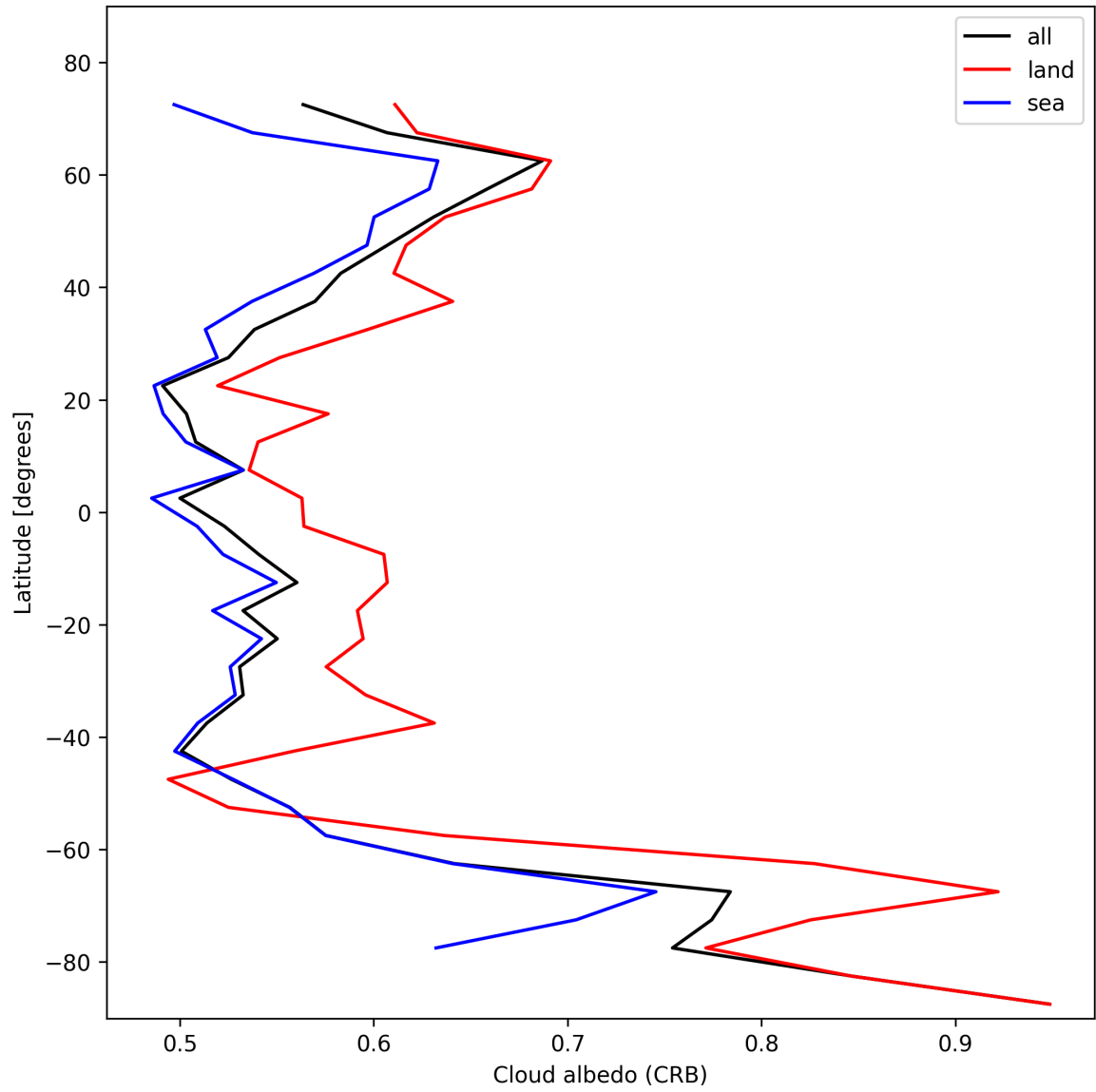
Figure 28: Zonal average of “Cloud albedo (CRB)” for 2024-11-12 to 2024-11-14.
