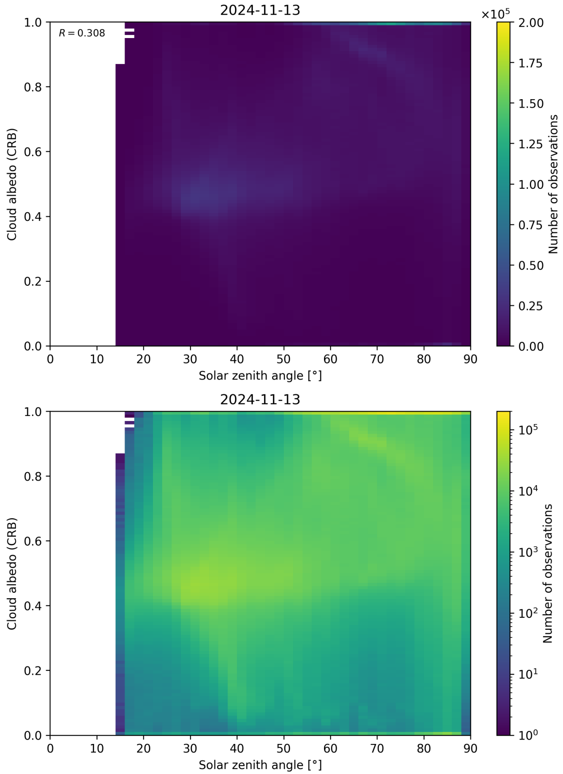
Figure 98: Scatter density plot of “Solar zenith angle” against “Cloud albedo (CRB)” for 2024-11-12 to 2024-11-14.
