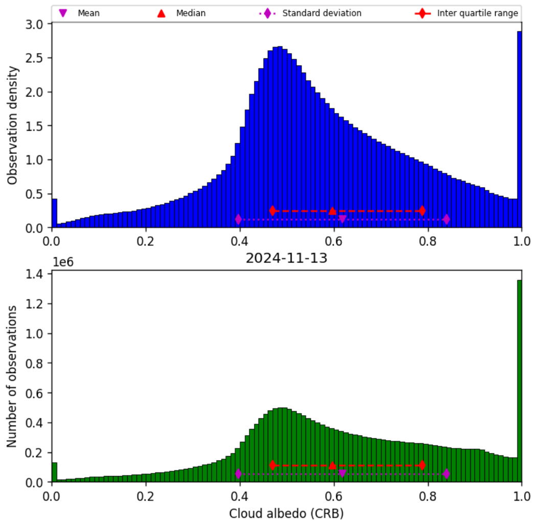
Figure 44: Histogram of “Cloud albedo (CRB)” for 2024-11-12 to 2024-11-14
