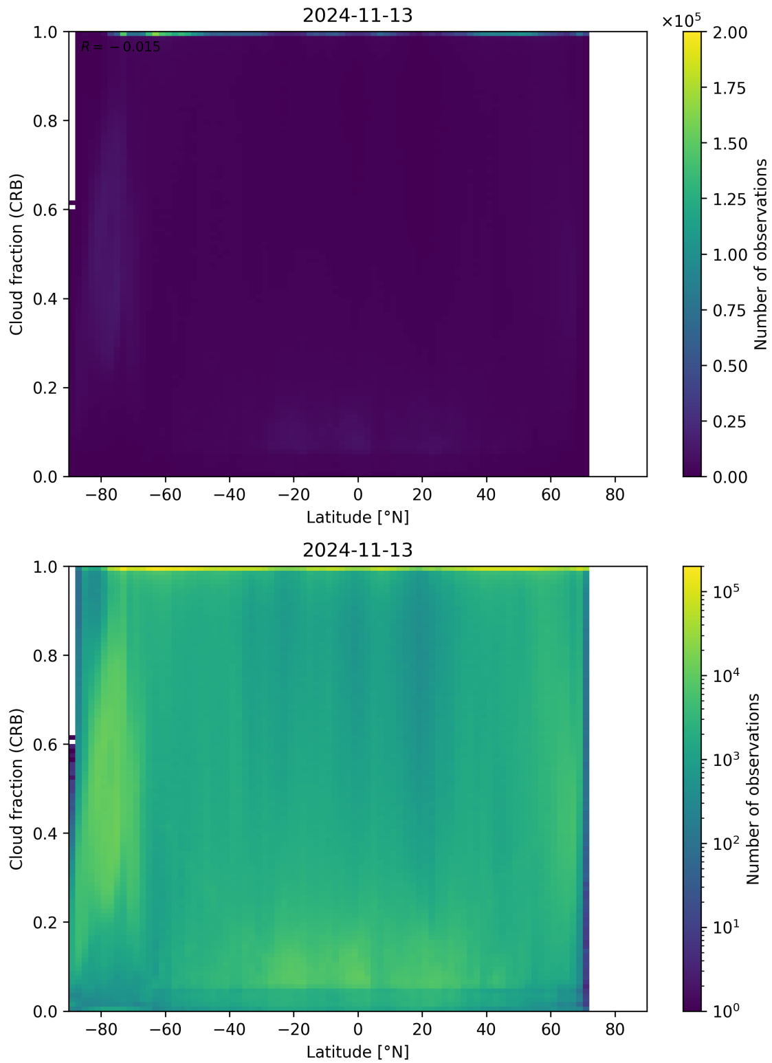
Figure 94: Scatter density plot of “Latitude” against “Cloud fraction (CRB)” for 2024-11-12 to 2024-11-14.
