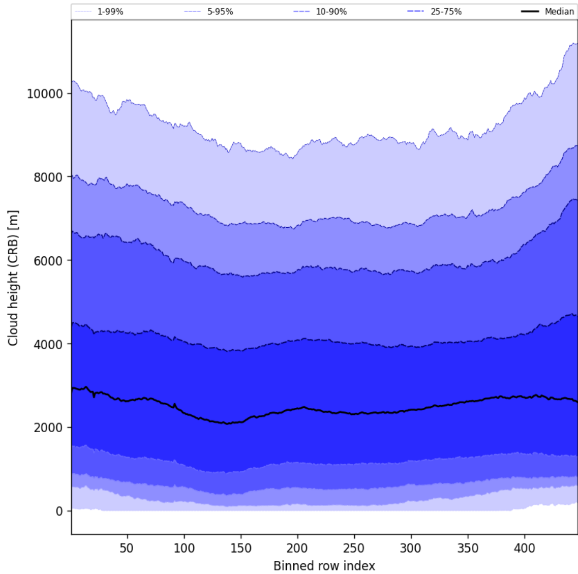
Figure 59: Along track statistics of “Cloud height (CRB)” for 2024-11-12 to 2024-11-14
