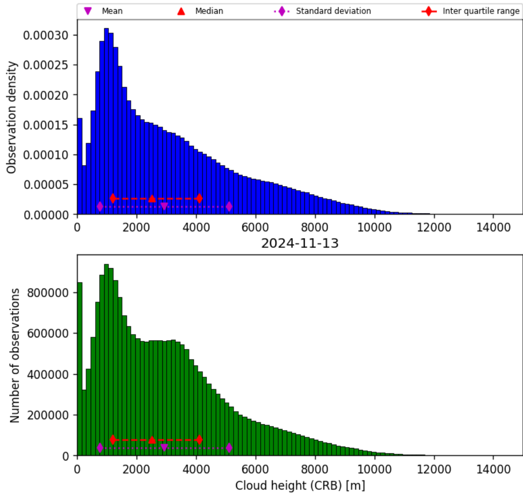
Figure 43: Histogram of “Cloud height (CRB)” for 2024-11-12 to 2024-11-14
