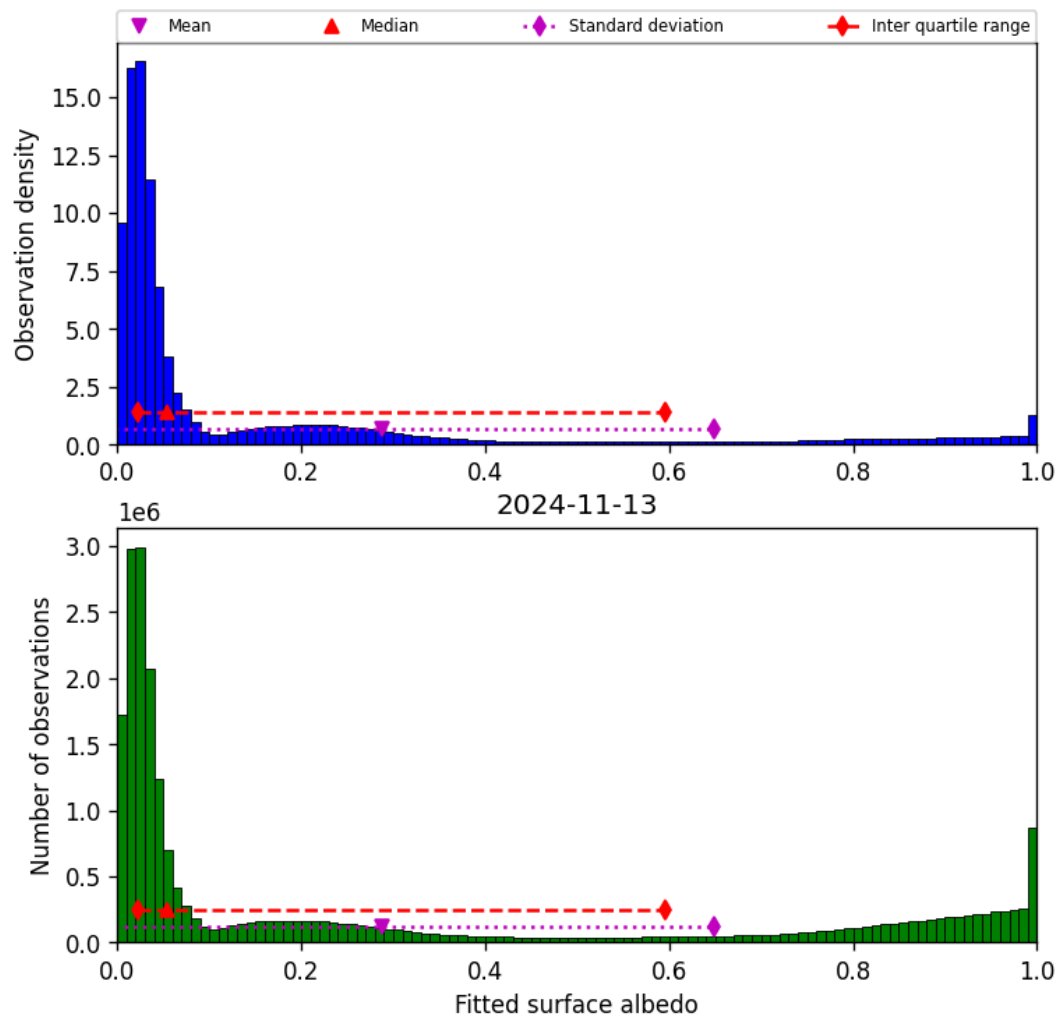
Figure 45: Histogram of “Fitted surface albedo” for 2024-11-12 to 2024-11-14
