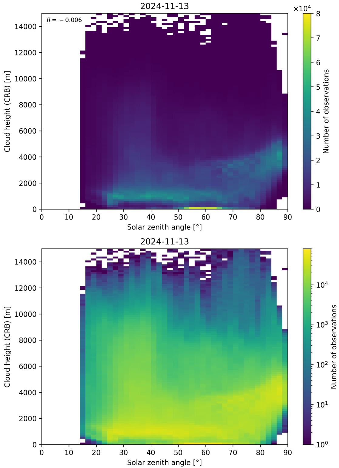
Figure 102: Scatter density plot of “Solar zenith angle” against “Cloud height (CRB)” for 2024-11-12 to 2024-11-14.
