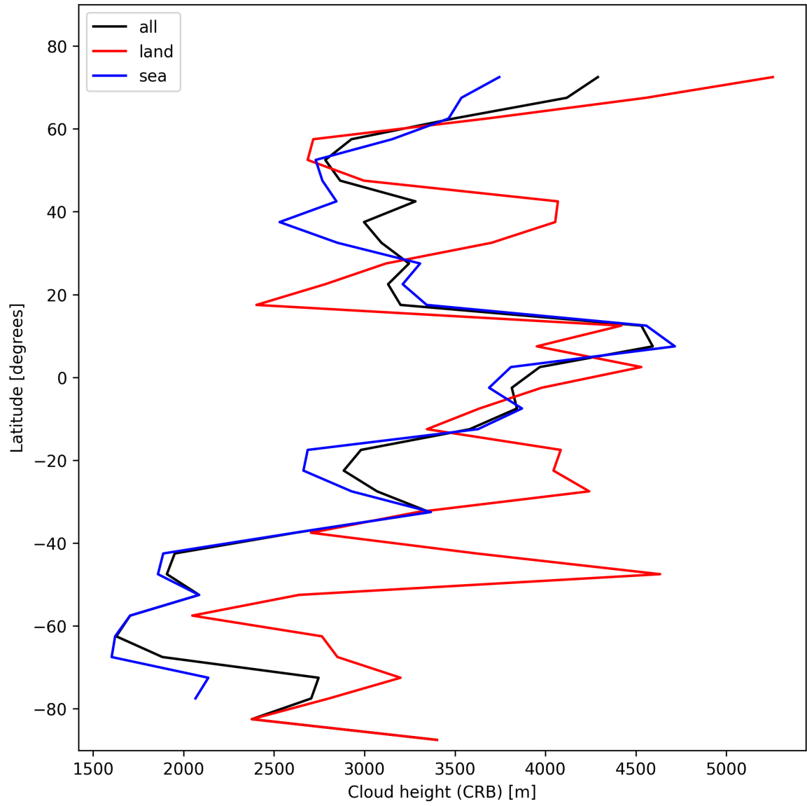
Figure 27: Zonal average of “Cloud height (CRB)” for 2024-11-12 to 2024-11-14.
