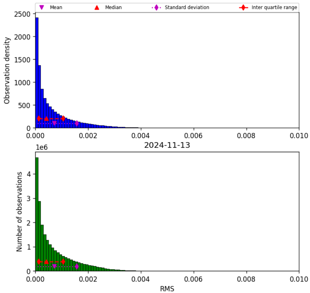
Figure 47: Histogram of “RMS” for 2024-11-12 to 2024-11-14
