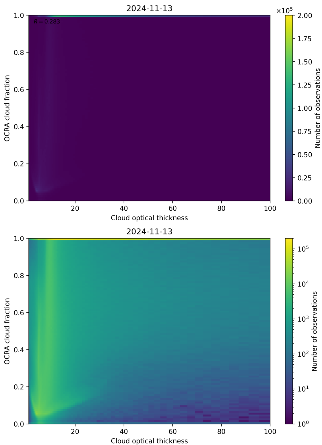
Figure 83: Scatter density plot of “Cloud optical thickness” against “OCRA cloud fraction” for 2024-11-12 to 2024-11-14.
