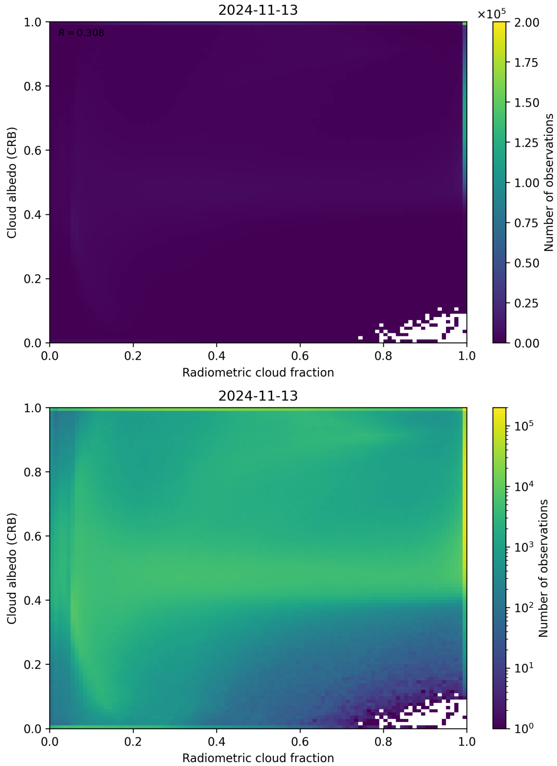
Figure 71: Scatter density plot of “Radiometric cloud fraction” against “Cloud albedo (CRB)” for 2024-11-12 to 2024-11-14.
