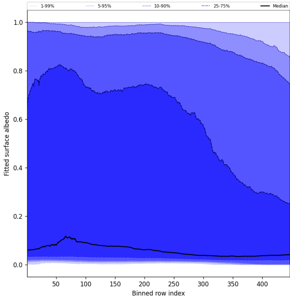
Figure 61: Along track statistics of “Fitted surface albedo” for 2024-11-12 to 2024-11-14
