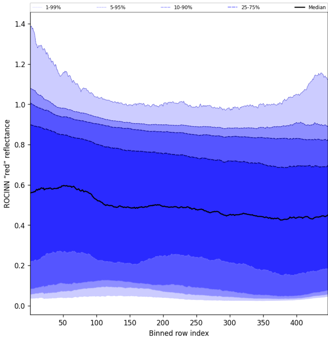
Figure 69: Along track statistics of "ROCINN "red" reflectance" for 2024-11-12 to 2024-11-14
