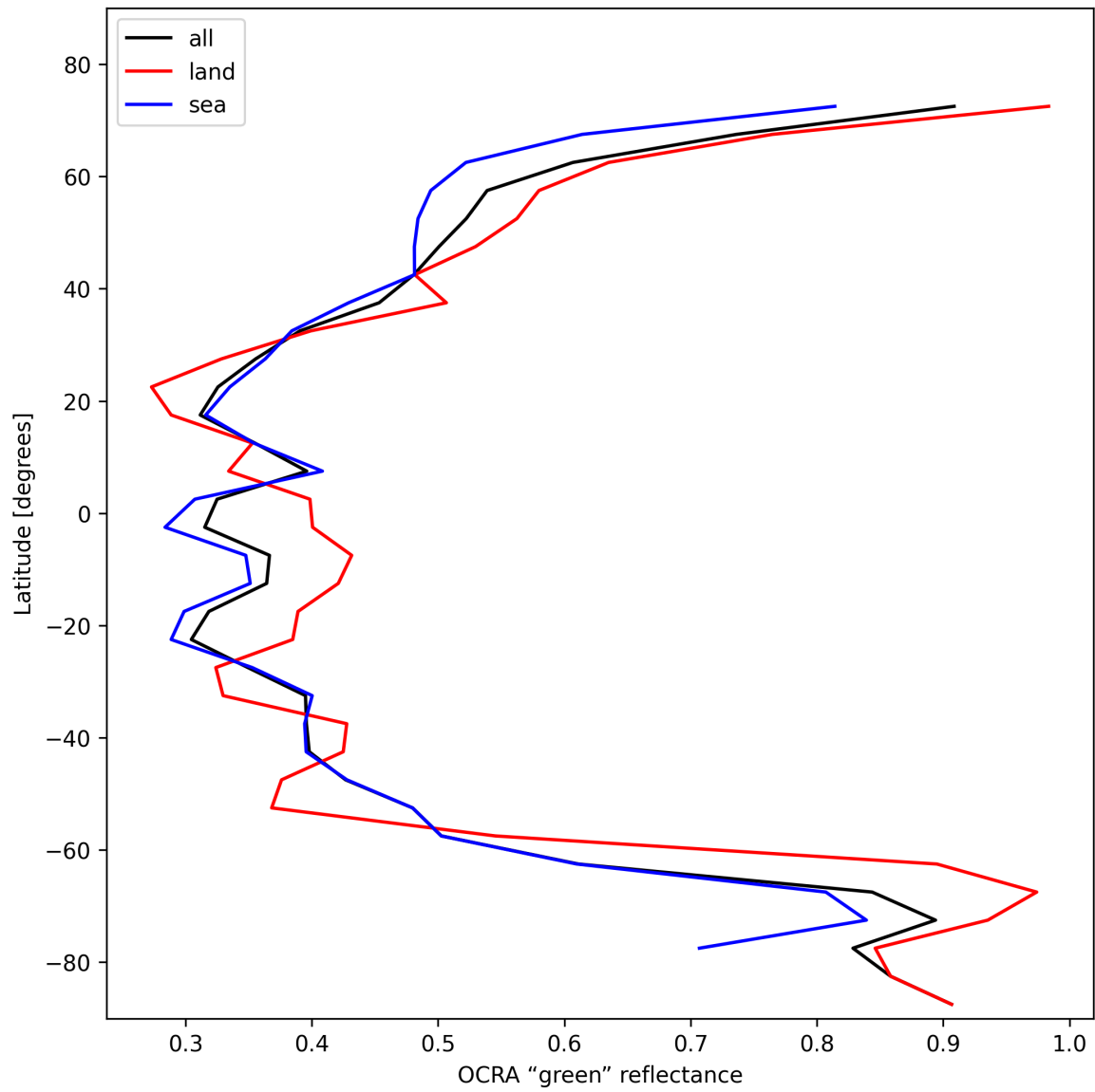
Figure 36: Zonal average of “OCRA “green” reflectance” for 2024-11-12 to 2024-11-14.
