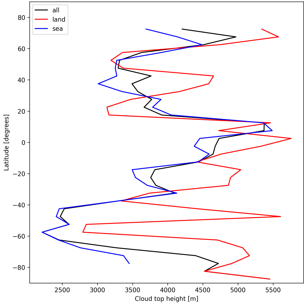
Figure 24: Zonal average of “Cloud top height” for 2024-11-12 to 2024-11-14.
