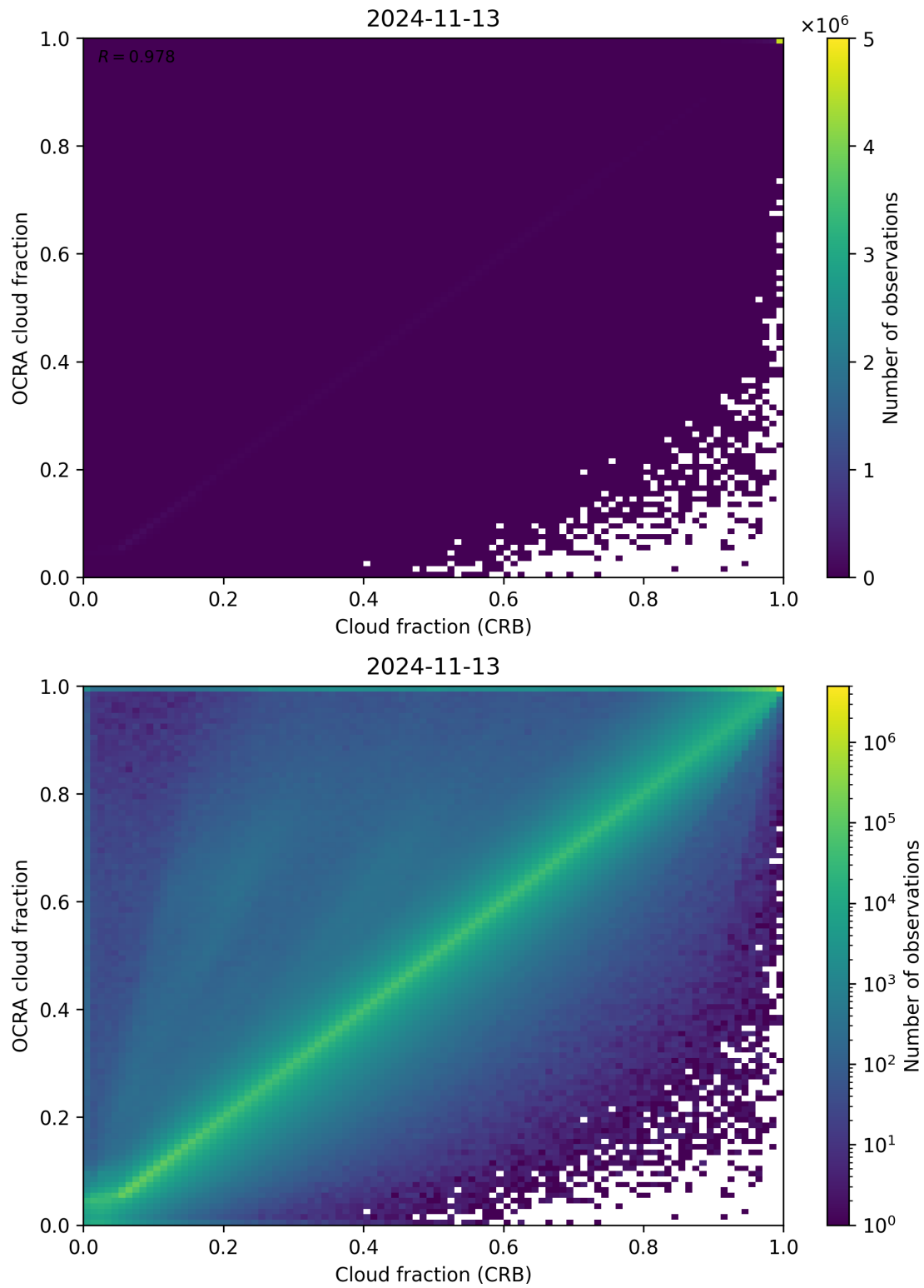
Figure 78: Scatter density plot of “Cloud fraction (CRB)” against “OCRA cloud fraction” for 2024-11-12 to 2024-11-14.
