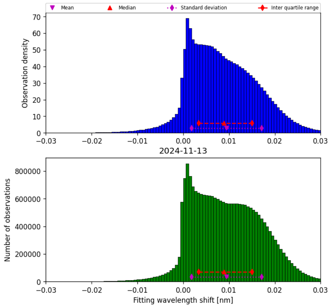
Figure 49: Histogram of “Fitting wavelength shift” for 2024-11-12 to 2024-11-14
