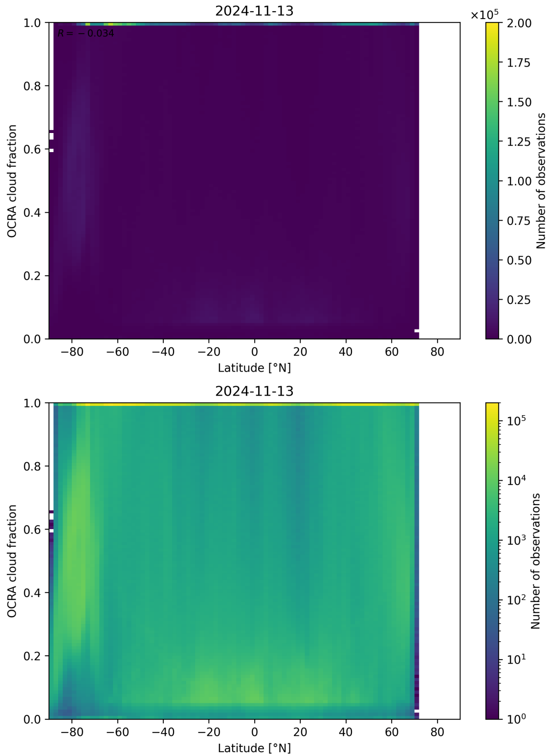
Figure 93: Scatter density plot of “Latitude” against “OCRA cloud fraction” for 2024-11-12 to 2024-11-14.
