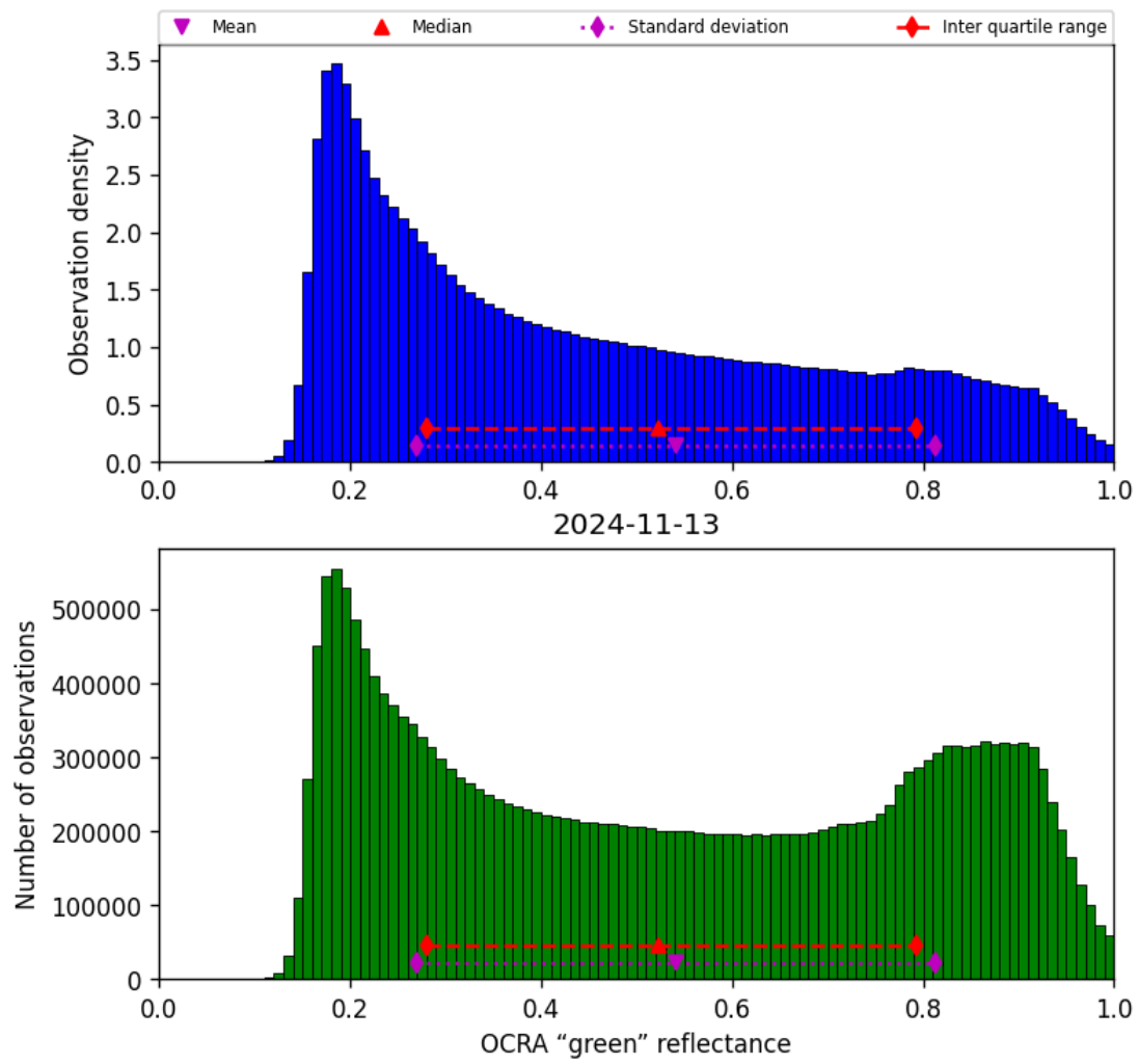
Figure 52: Histogram of “OCRA “green” reflectance” for 2024-11-12 to 2024-11-14
