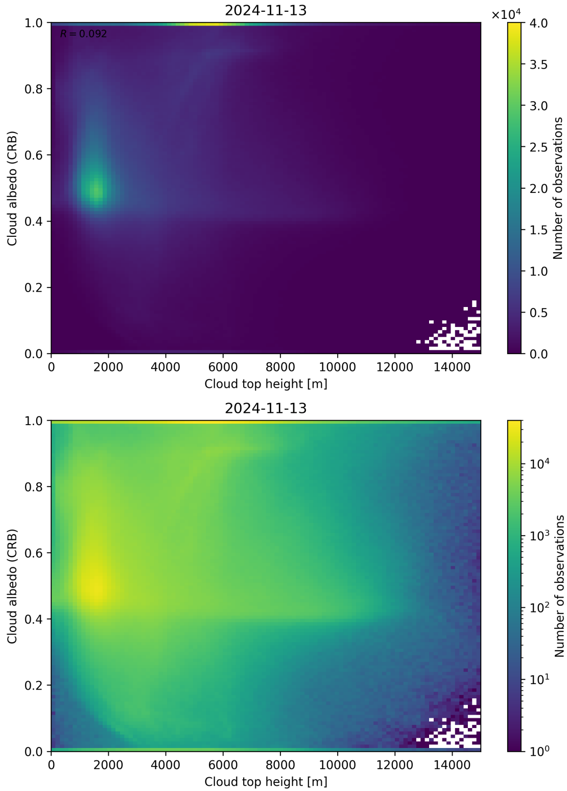
Figure 86: Scatter density plot of “Cloud top height” against “Cloud albedo (CRB)” for 2024-11-12 to 2024-11-14.
