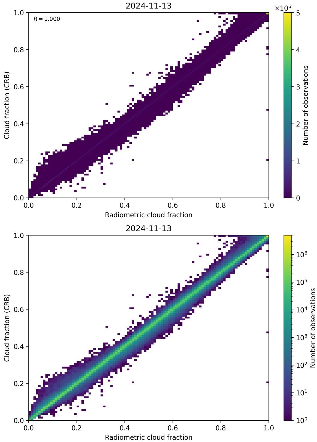
Figure 73: Scatter density plot of “Radiometric cloud fraction” against “Cloud fraction (CRB)” for 2024-11-12 to 2024-11-14.
