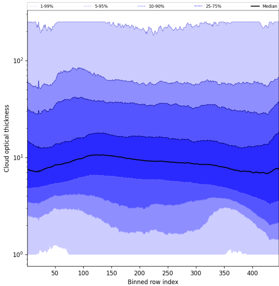
Figure 57: Along track statistics of “Cloud optical thickness” for 2024-11-12 to 2024-11-14
