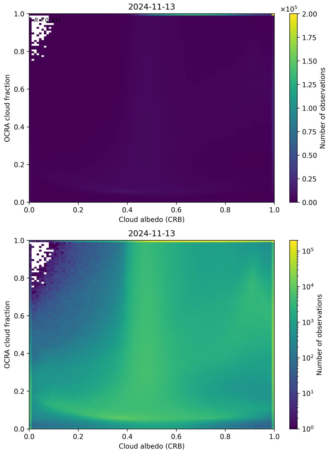
Figure 70: Scatter density plot of “Cloud albedo (CRB)” against “OCRA cloud fraction” for 2024-11-12 to 2024-11-14.
