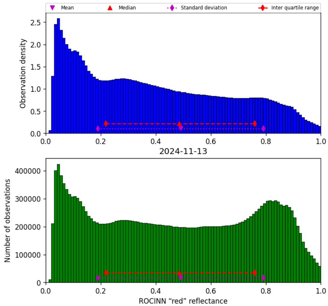
Figure 53: Histogram of “ROCINN “red” reflectance” for 2024-11-12 to 2024-11-14
