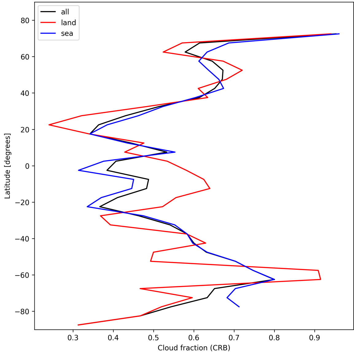
Figure 26: Zonal average of “Cloud fraction (CRB)” for 2024-11-12 to 2024-11-14.
