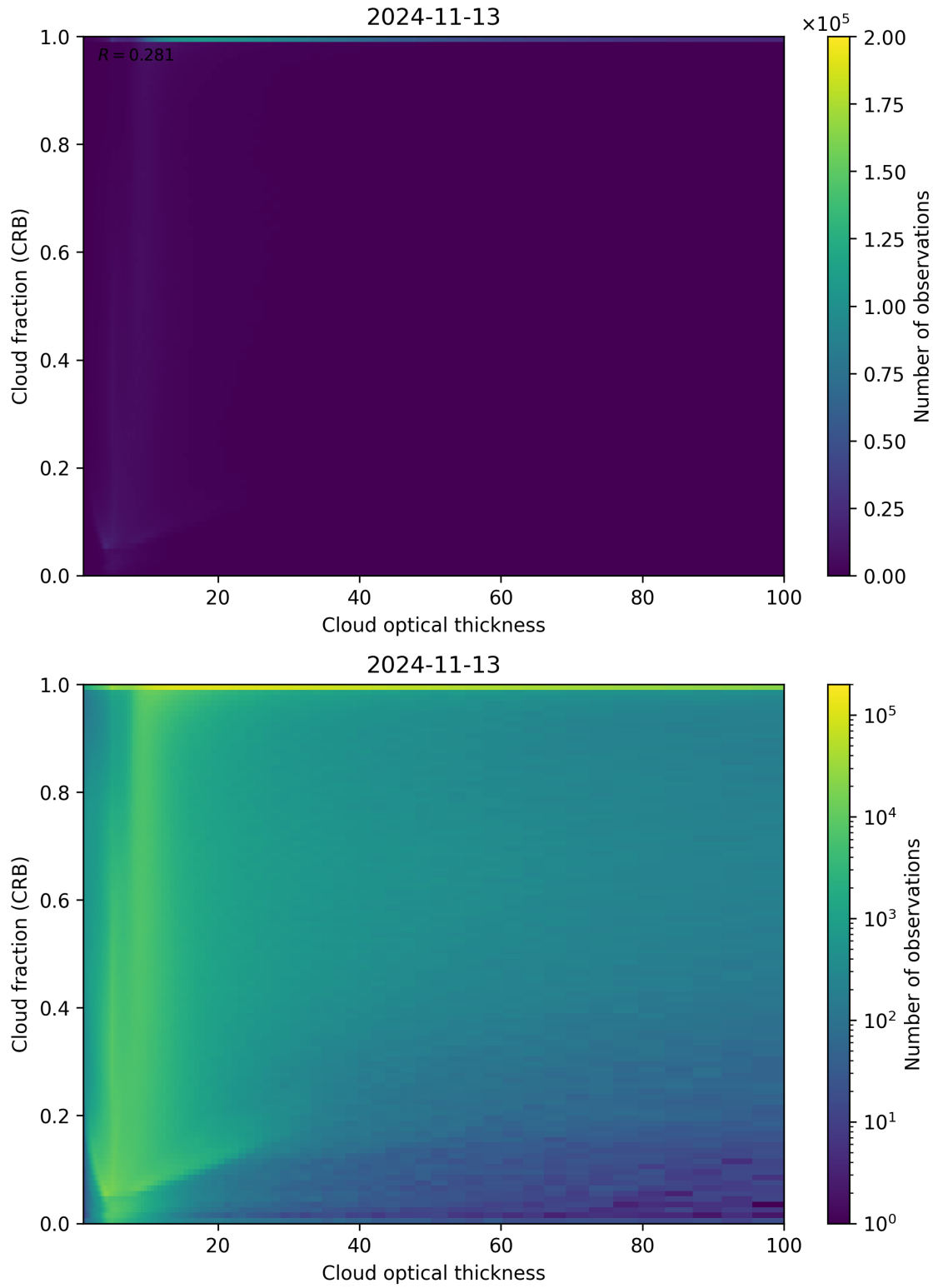
Figure 84: Scatter density plot of “Cloud optical thickness” against “Cloud fraction (CRB)” for 2024-11-12 to 2024-11-14.
