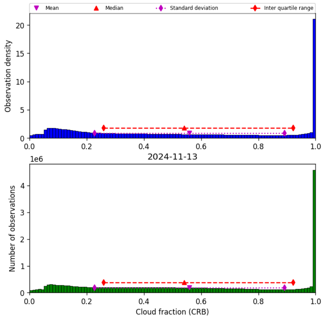
Figure 42: Histogram of “Cloud fraction (CRB)” for 2024-11-12 to 2024-11-14
