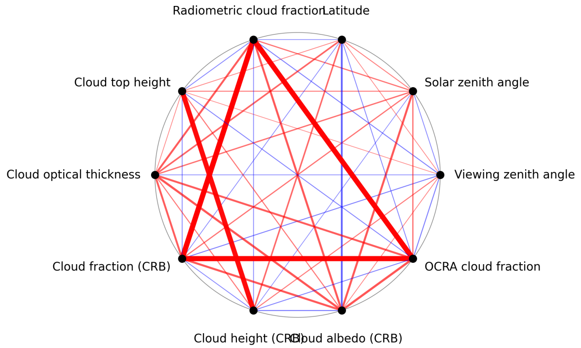
Figure 1: Map of correlation graph for 2024-11-12 to 2024-11-14.
