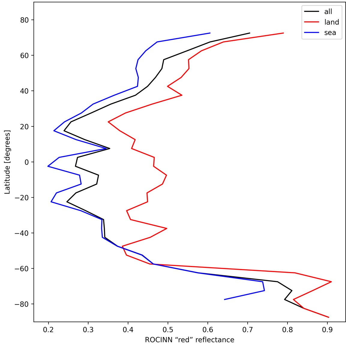
Figure 37: Zonal average of “ROCINN “red” reflectance” for 2024-11-12 to 2024-11-14.
