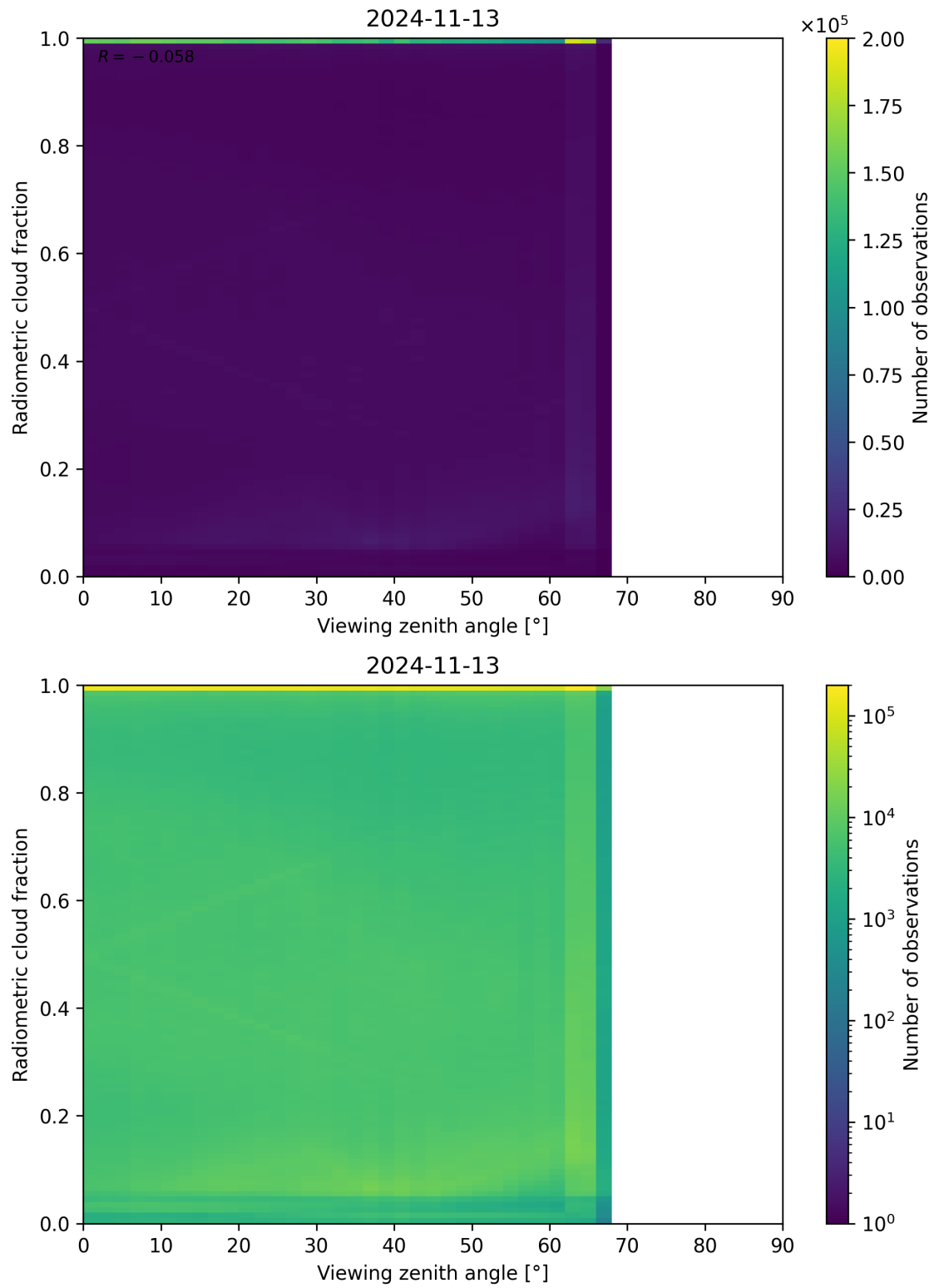
Figure 107: Scatter density plot of “Viewing zenith angle” against “Radiometric cloud fraction” for 2024-11-12 to 2024-11-14.
