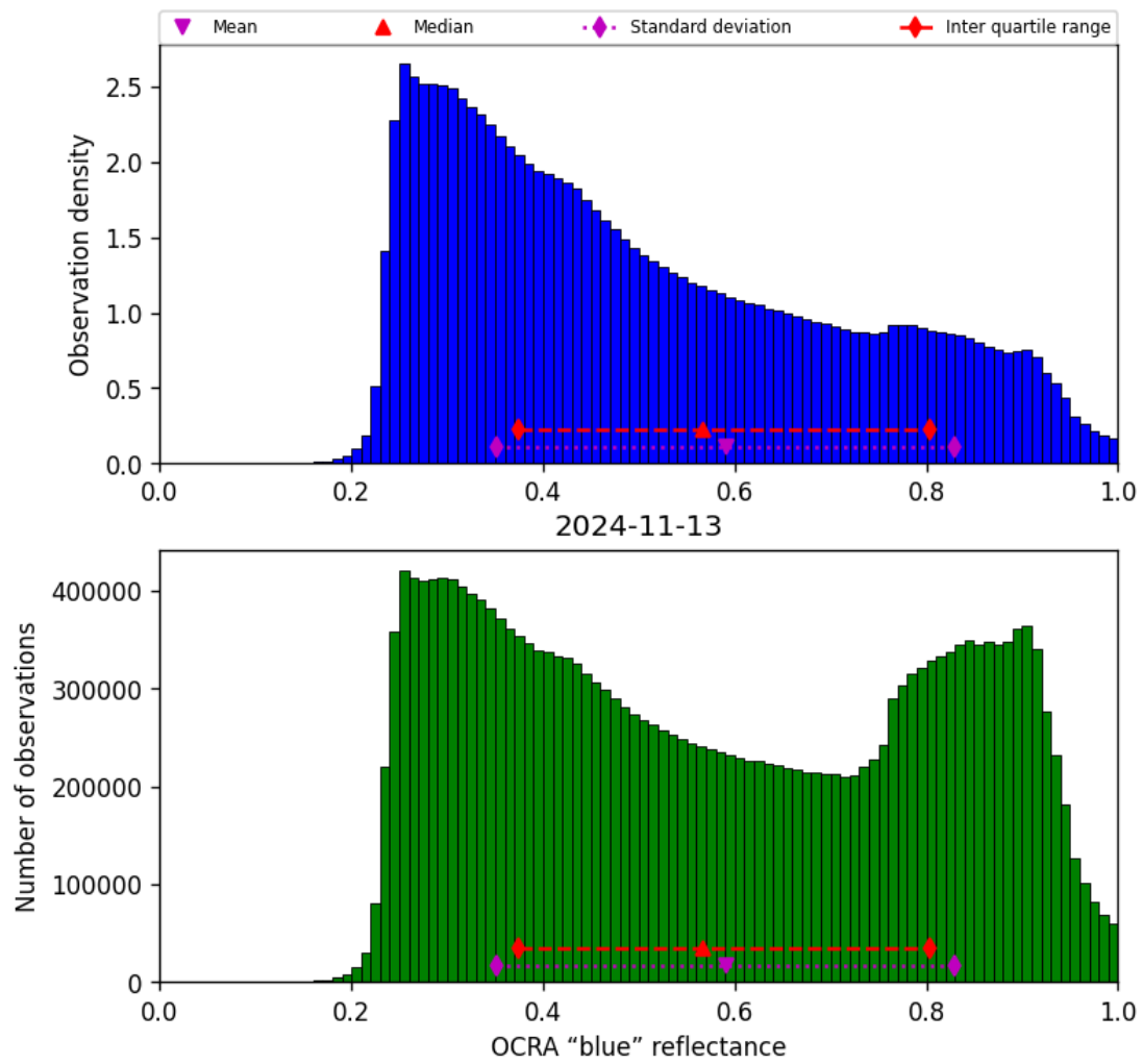
Figure 51: Histogram of “OCRA “blue” reflectance” for 2024-11-12 to 2024-11-14
