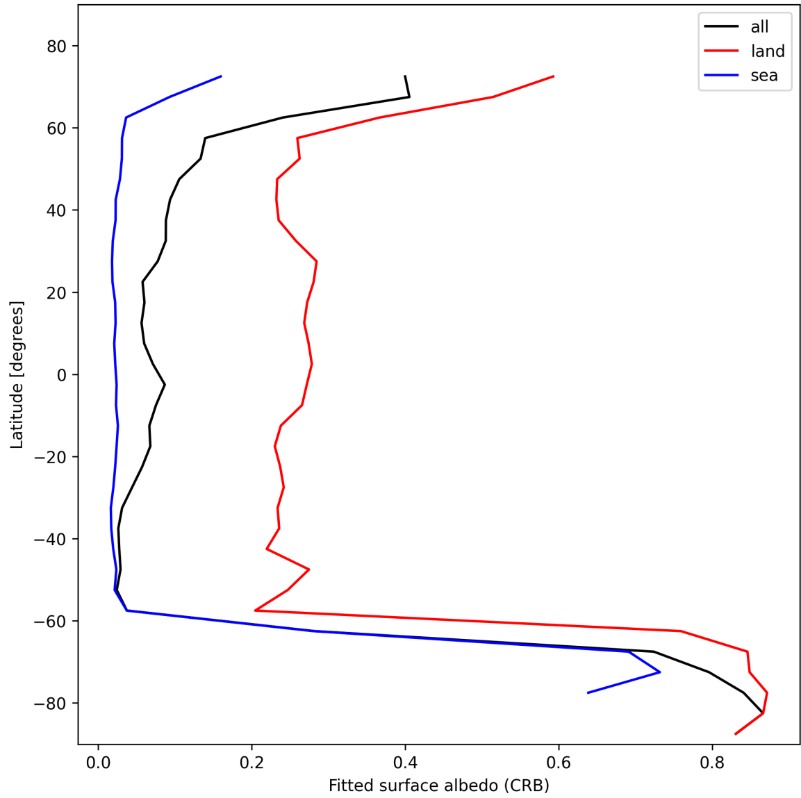
Figure 30: Zonal average of “Fitted surface albedo (CRB)” for 2024-11-12 to 2024-11-14.
