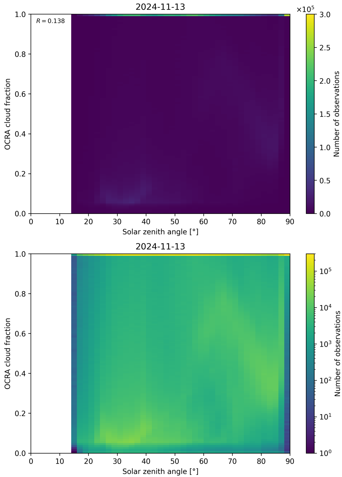
Figure 100: Scatter density plot of “Solar zenith angle” against “OCRA cloud fraction” for 2024-11-12 to 2024-11-14.
