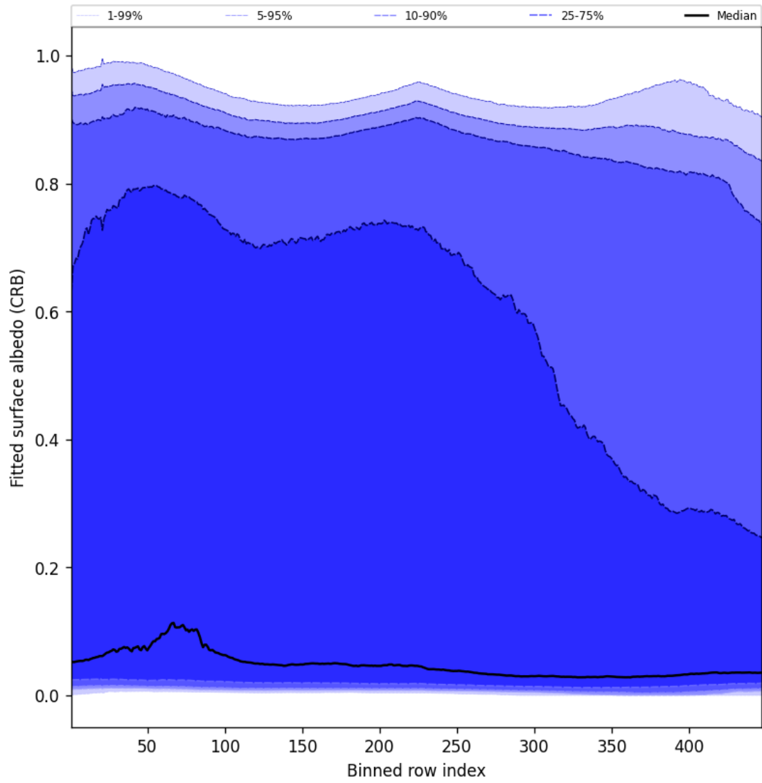
Figure 62: Along track statistics of “Fitted surface albedo (CRB)” for 2024-11-12 to 2024-11-14
