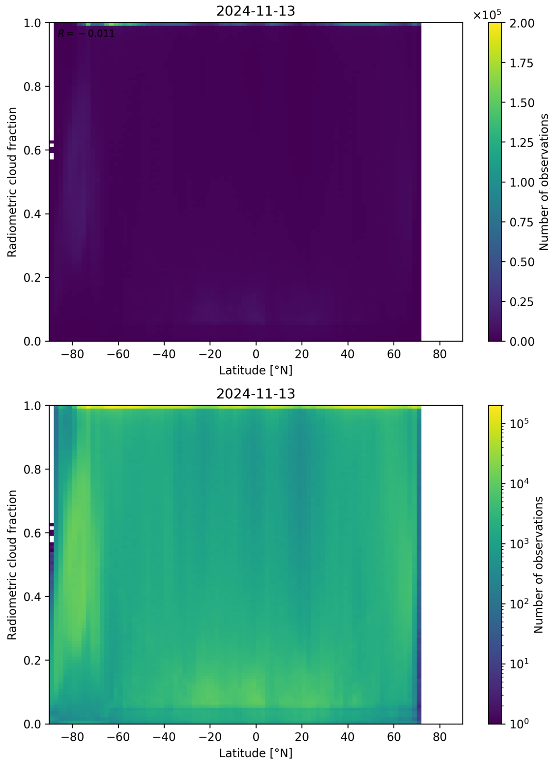
Figure 92: Scatter density plot of “Latitude” against “Radiometric cloud fraction” for 2024-11-12 to 2024-11-14.
