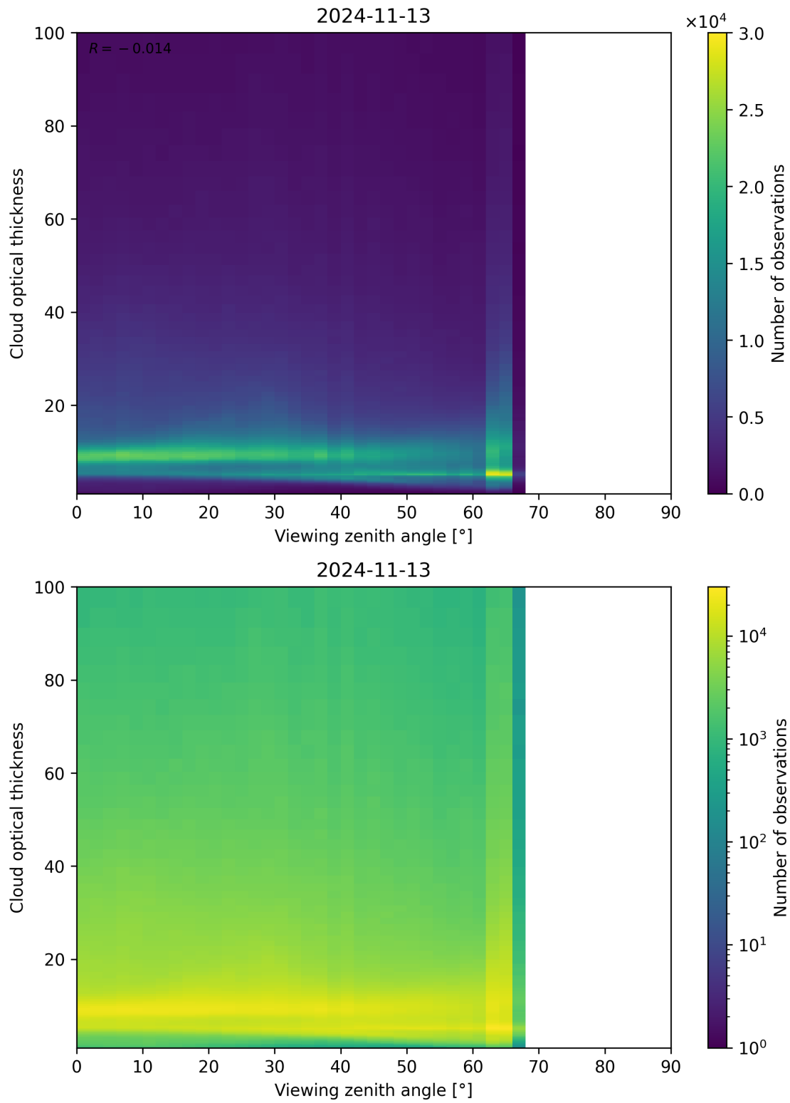
Figure 111: Scatter density plot of “Viewing zenith angle” against “Cloud optical thickness” for 2024-11-12 to 2024-11-14.
