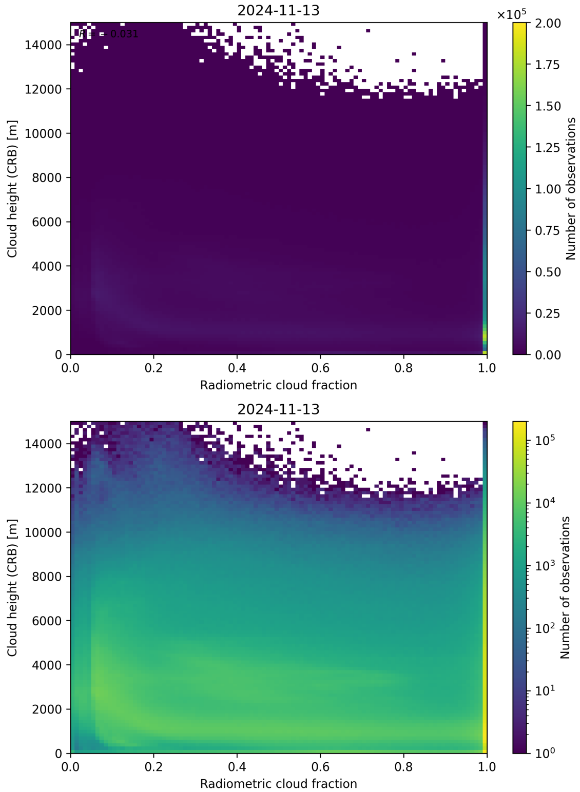
Figure 74: Scatter density plot of “Radiometric cloud fraction” against “Cloud height (CRB)” for 2024-11-12 to 2024-11-14.
