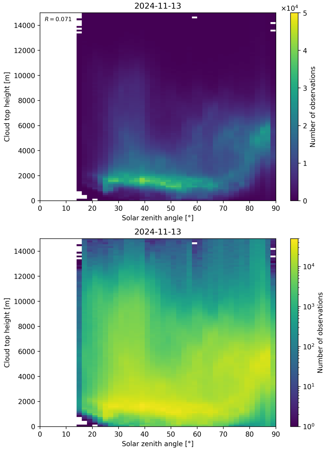
Figure 104: Scatter density plot of “Solar zenith angle” against “Cloud top height” for 2024-11-12 to 2024-11-14.
