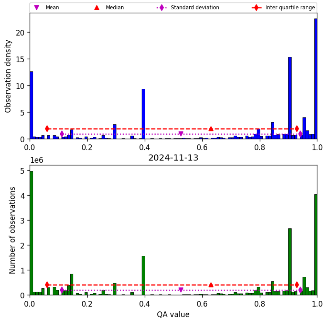
Figure 38: Histogram of “QA value” for 2024-11-12 to 2024-11-14
