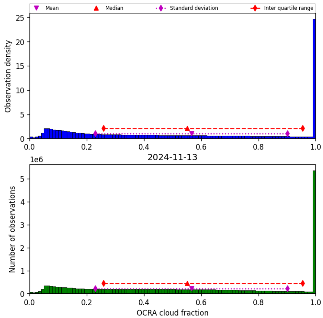
Figure 50: Histogram of “OCRA cloud fraction” for 2024-11-12 to 2024-11-14
