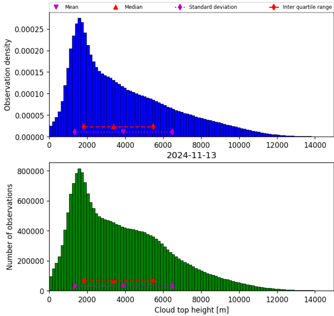
Figure 40: Histogram of “Cloud top height” for 2024-11-12 to 2024-11-14
