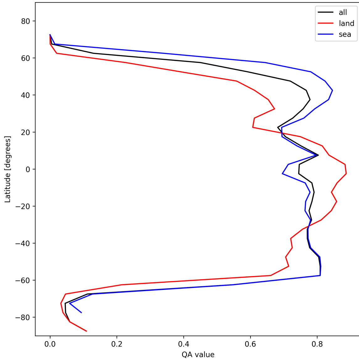
Figure 22: Zonal average of “QA value” for 2024-11-12 to 2024-11-14.
