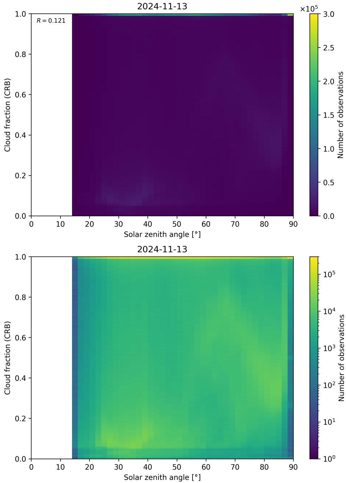
Figure 101: Scatter density plot of “Solar zenith angle” against “Cloud fraction (CRB)” for 2024-11-12 to 2024-11-14.
