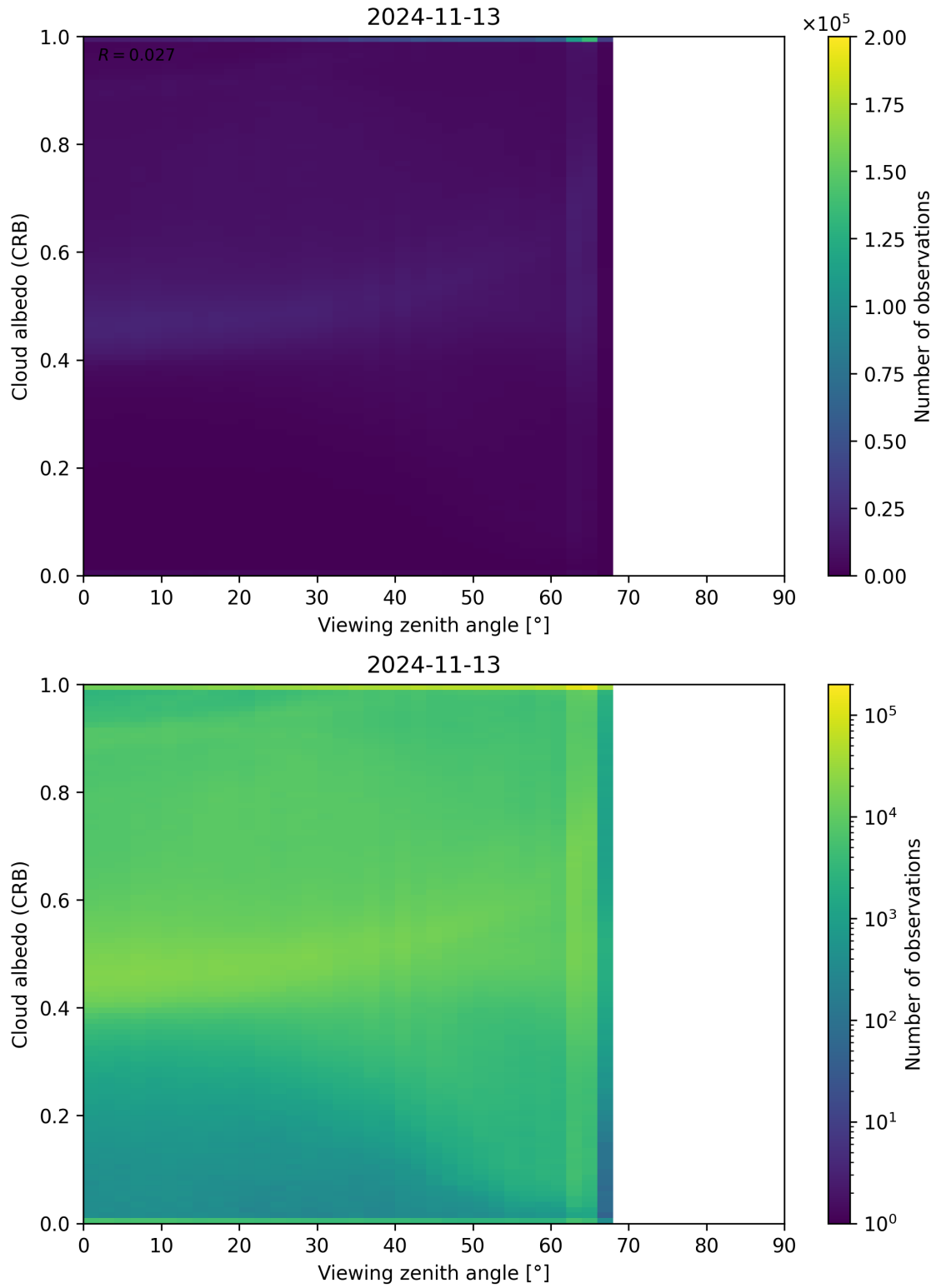
Figure 106: Scatter density plot of “Viewing zenith angle” against “Cloud albedo (CRB)” for 2024-11-12 to 2024-11-14.
