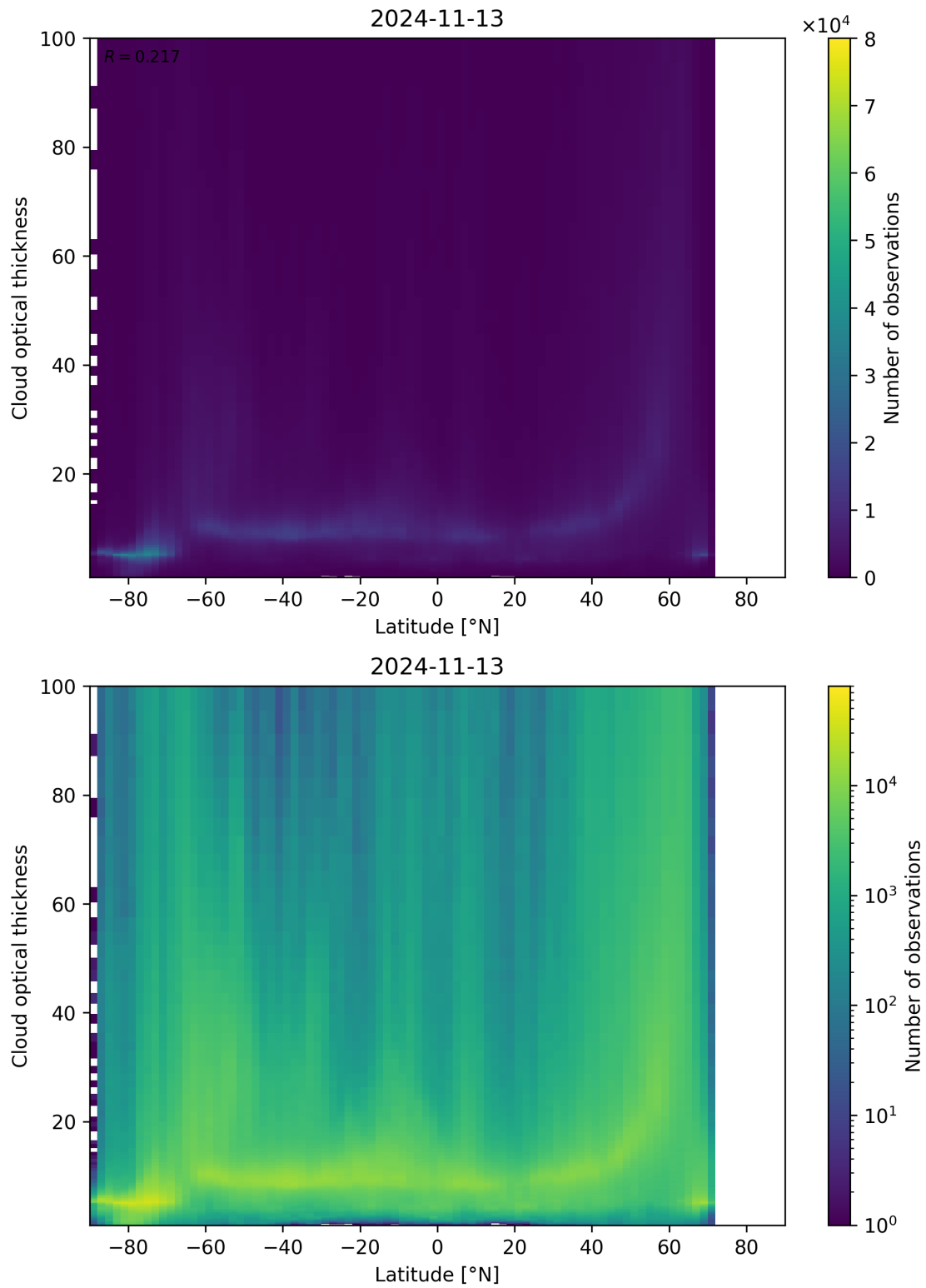
Figure 96: Scatter density plot of “Latitude” against “Cloud optical thickness” for 2024-11-12 to 2024-11-14.
