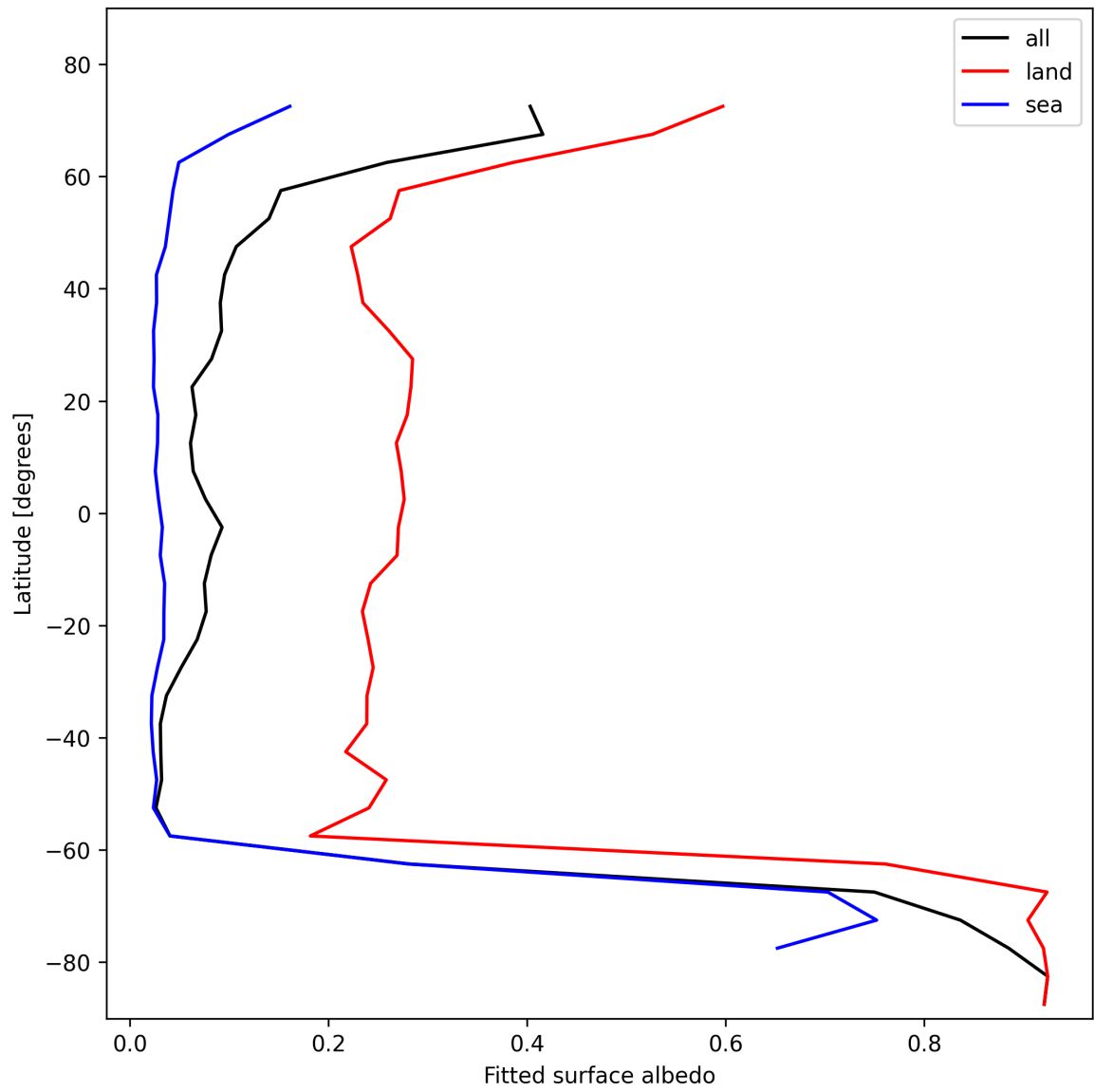
Figure 29: Zonal average of “Fitted surface albedo” for 2024-11-12 to 2024-11-14.
