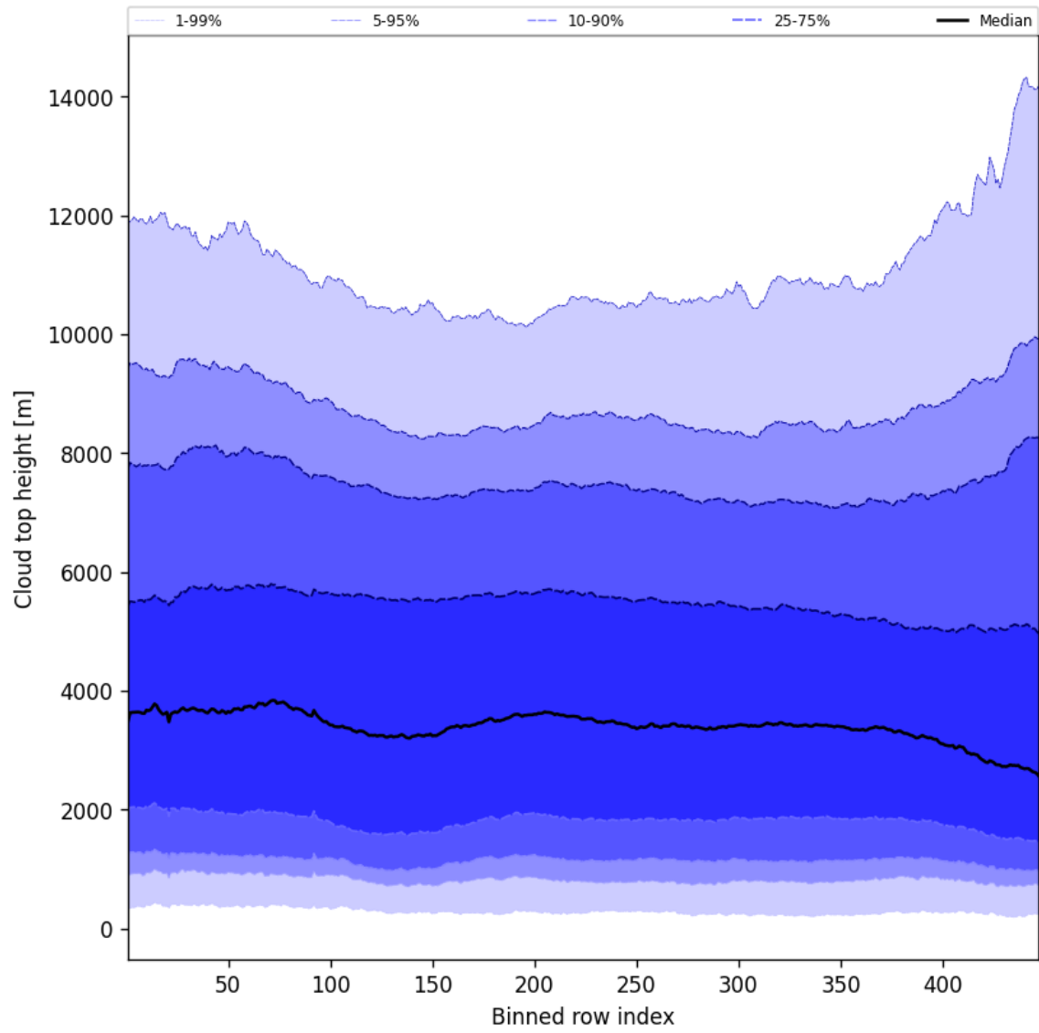
Figure 56: Along track statistics of “Cloud top height” for 2024-11-12 to 2024-11-14
