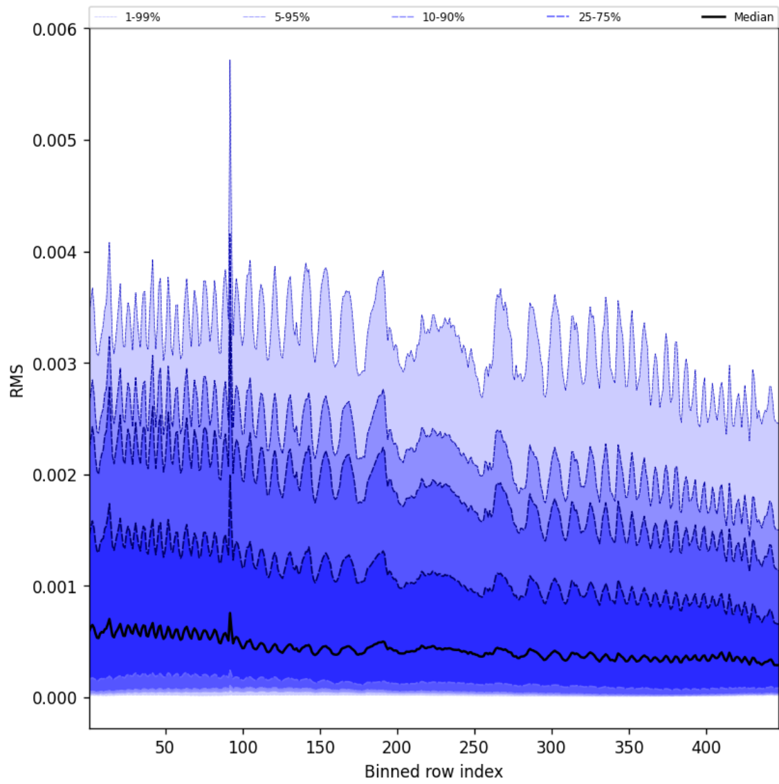
Figure 63: Along track statistics of “RMS” for 2024-11-12 to 2024-11-14
