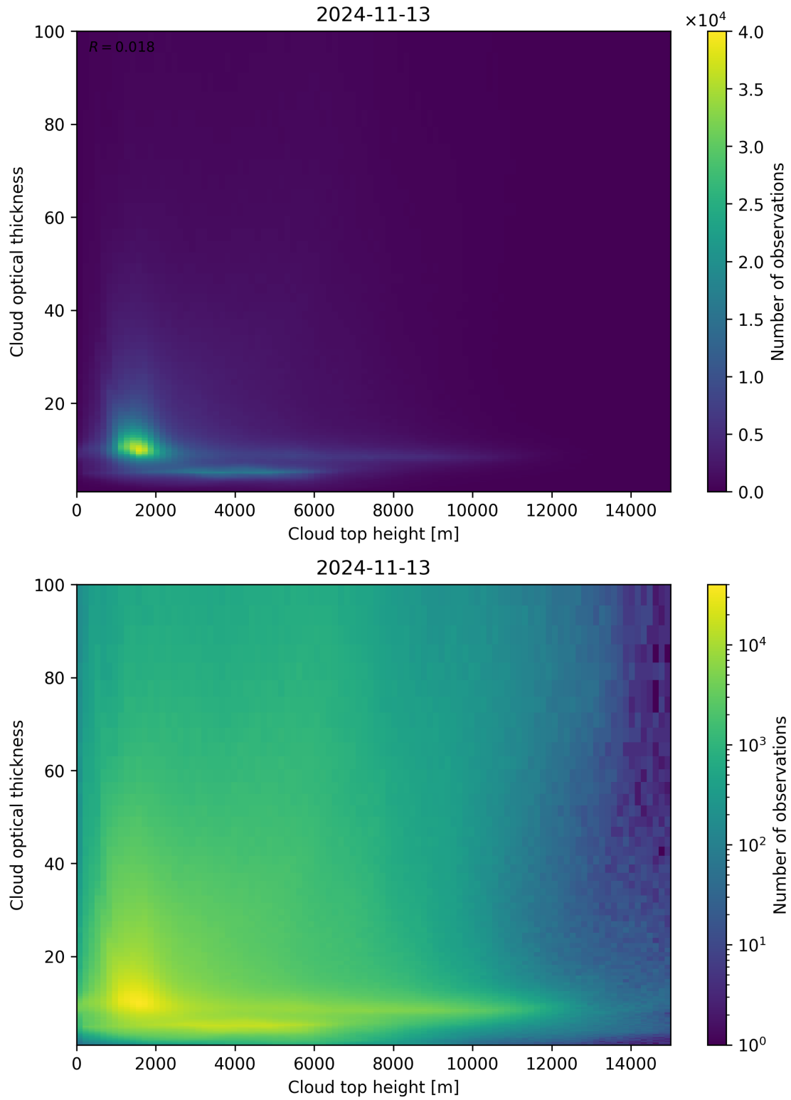
Figure 90: Scatter density plot of “Cloud top height” against “Cloud optical thickness” for 2024-11-12 to 2024-11-14.
