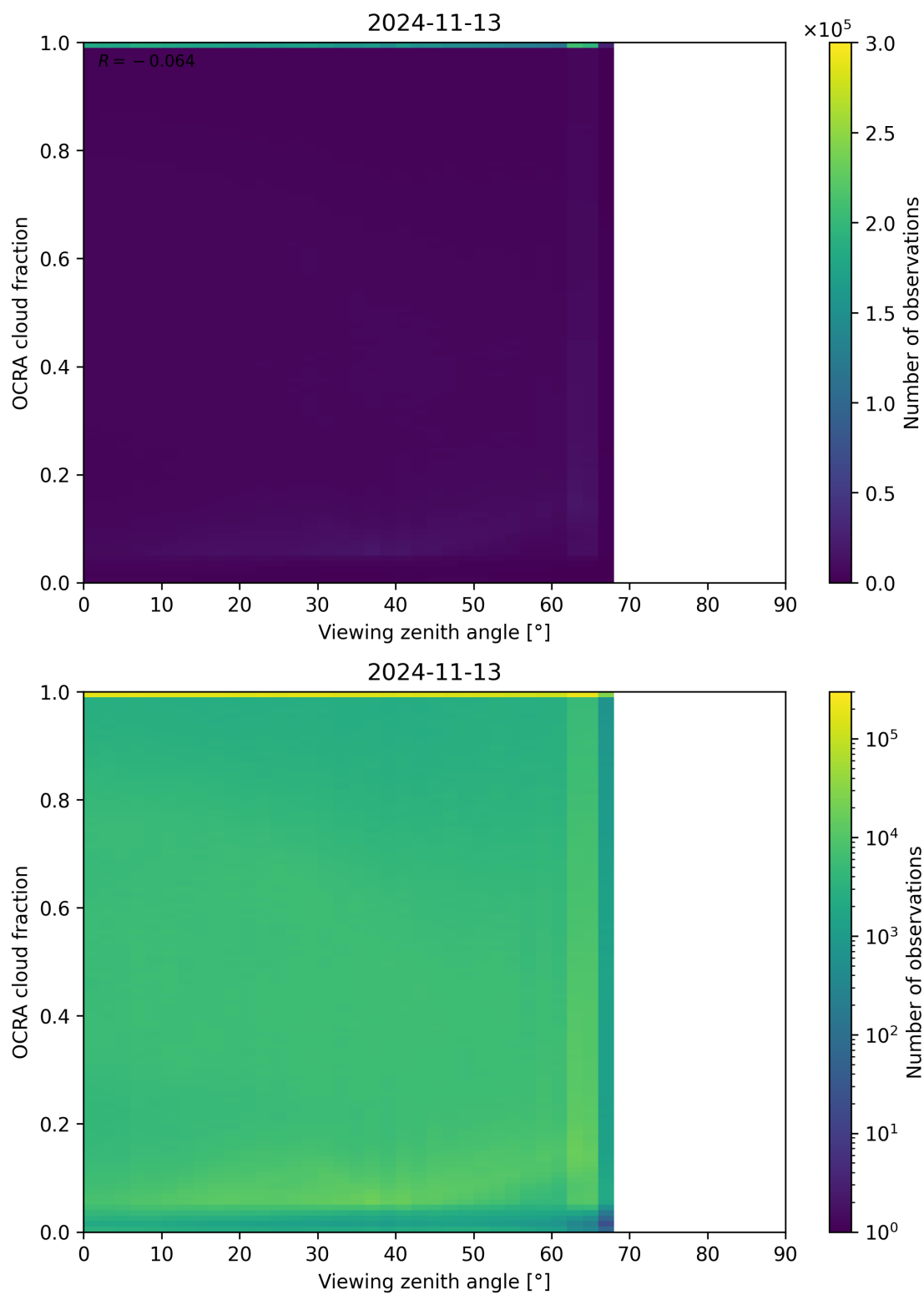
Figure 108: Scatter density plot of “Viewing zenith angle” against “OCRA cloud fraction” for 2024-11-12 to 2024-11-14.
