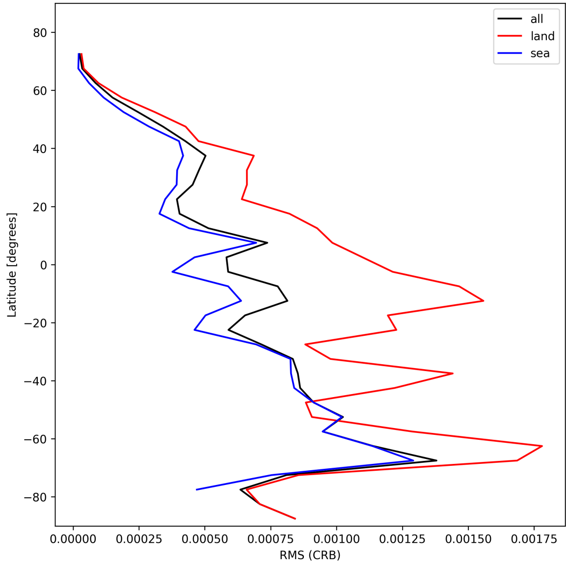
Figure 32: Zonal average of “RMS (CRB)” for 2024-11-12 to 2024-11-14.
