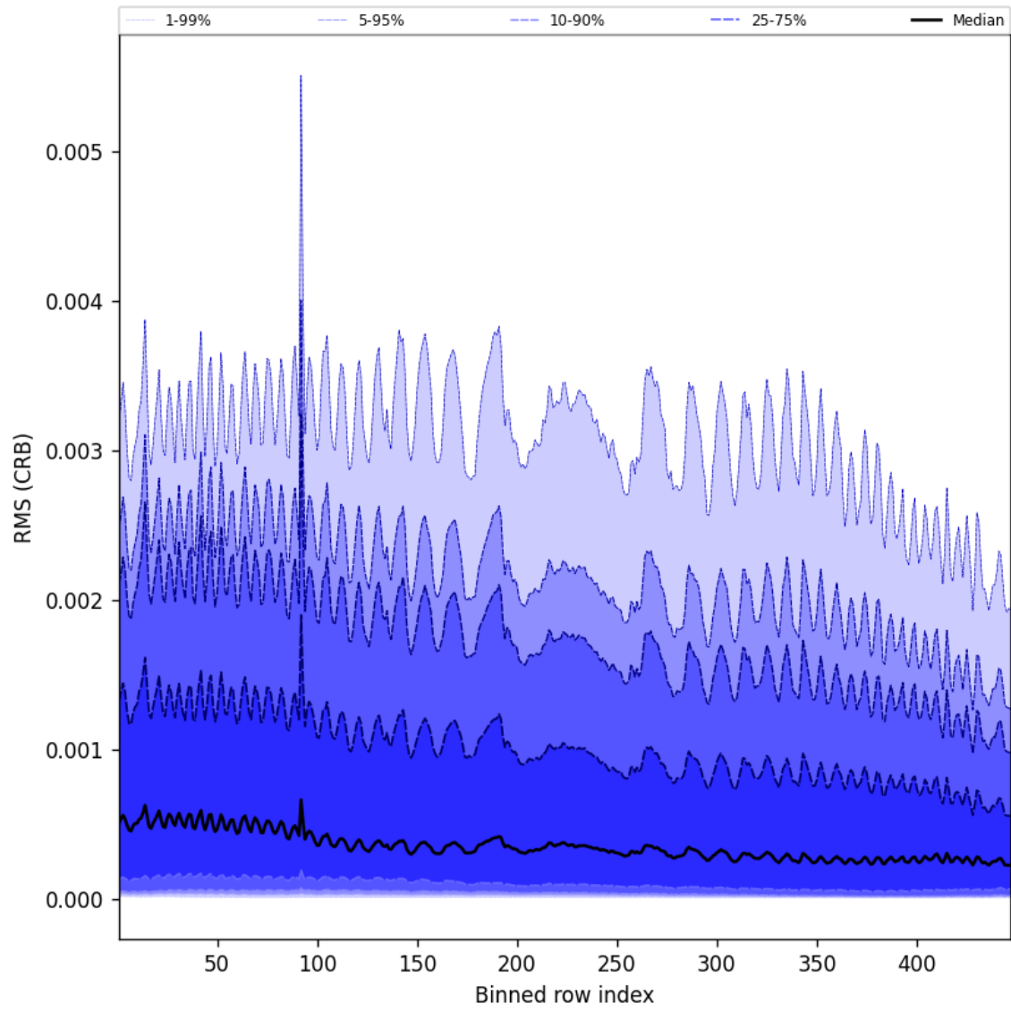
Figure 64: Along track statistics of “RMS (CRB)” for 2024-11-12 to 2024-11-14
