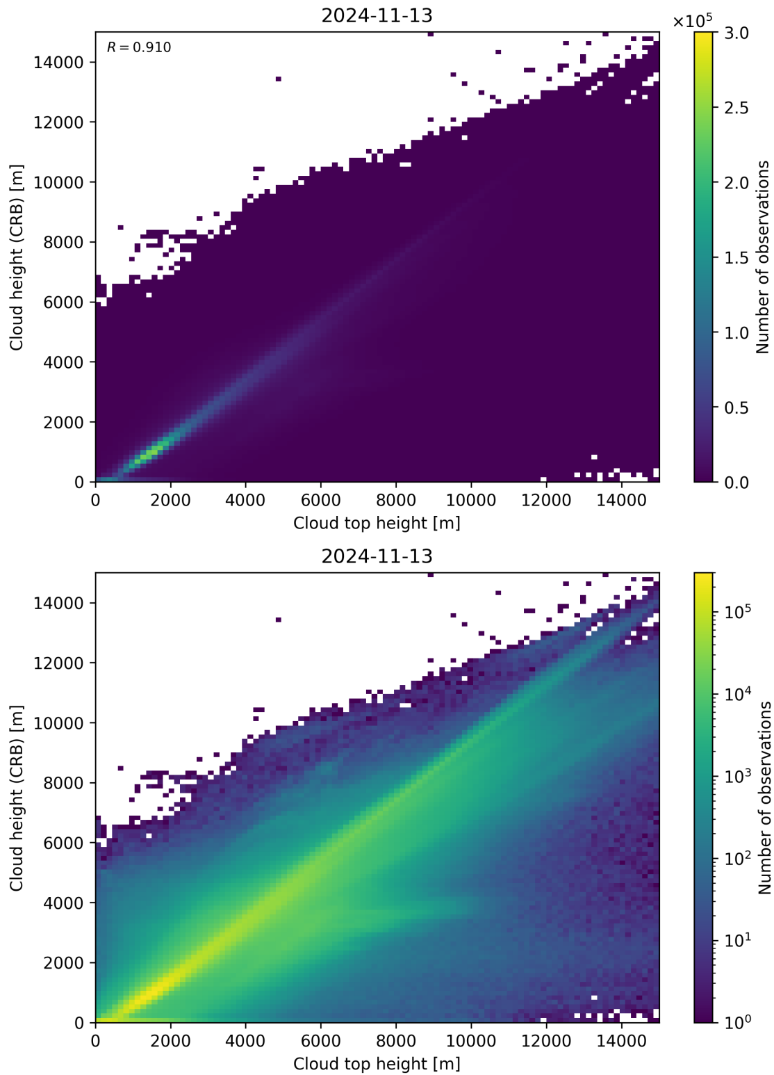
Figure 89: Scatter density plot of “Cloud top height” against “Cloud height (CRB)” for 2024-11-12 to 2024-11-14.
