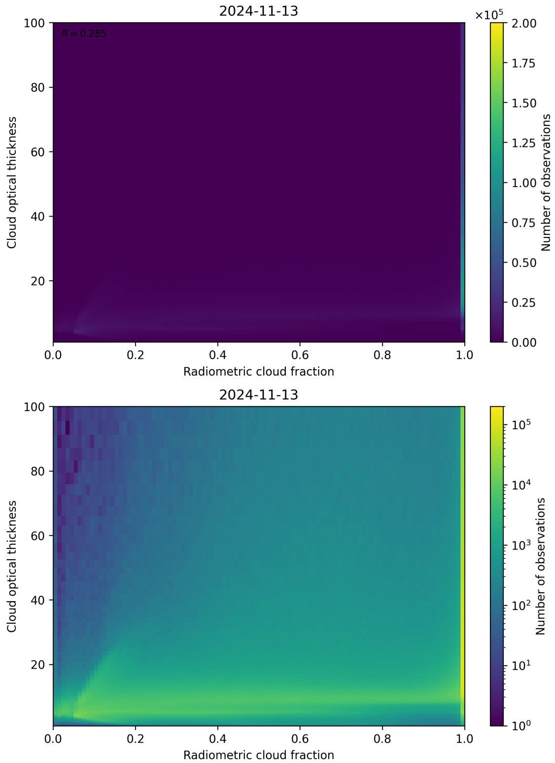
Figure 75: Scatter density plot of “Radiometric cloud fraction” against “Cloud optical thickness” for 2024-11-12 to 2024-11-14.
