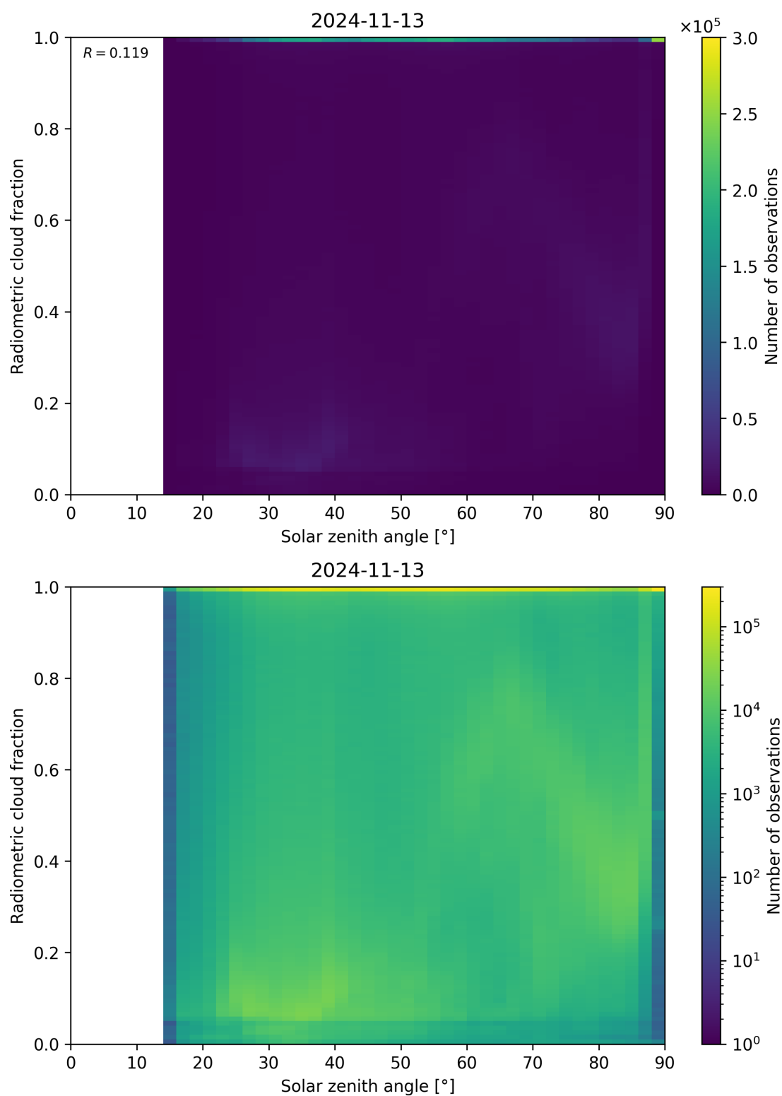
Figure 99: Scatter density plot of “Solar zenith angle” against “Radiometric cloud fraction” for 2024-11-12 to 2024-11-14.
