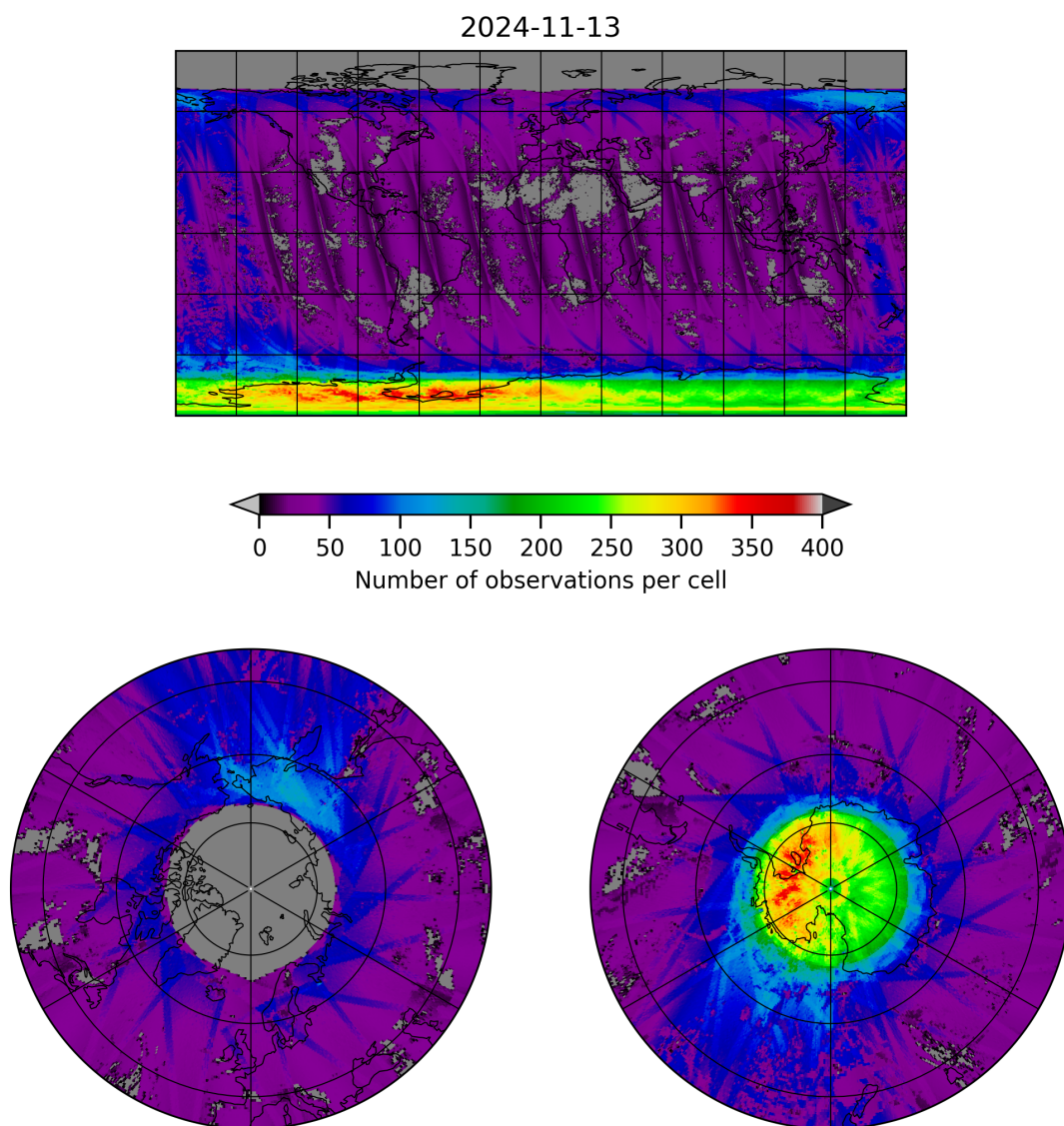
Figure 21: Map of the number of observations for 2024-11-12 to 2024-11-14
