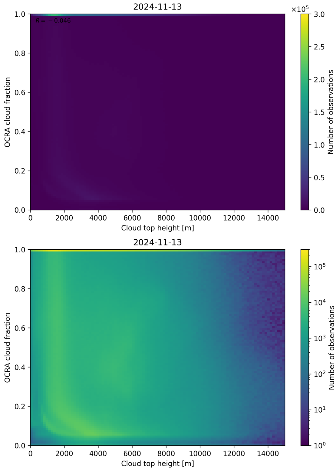
Figure 87: Scatter density plot of “Cloud top height” against “OCRA cloud fraction” for 2024-11-12 to 2024-11-14.
