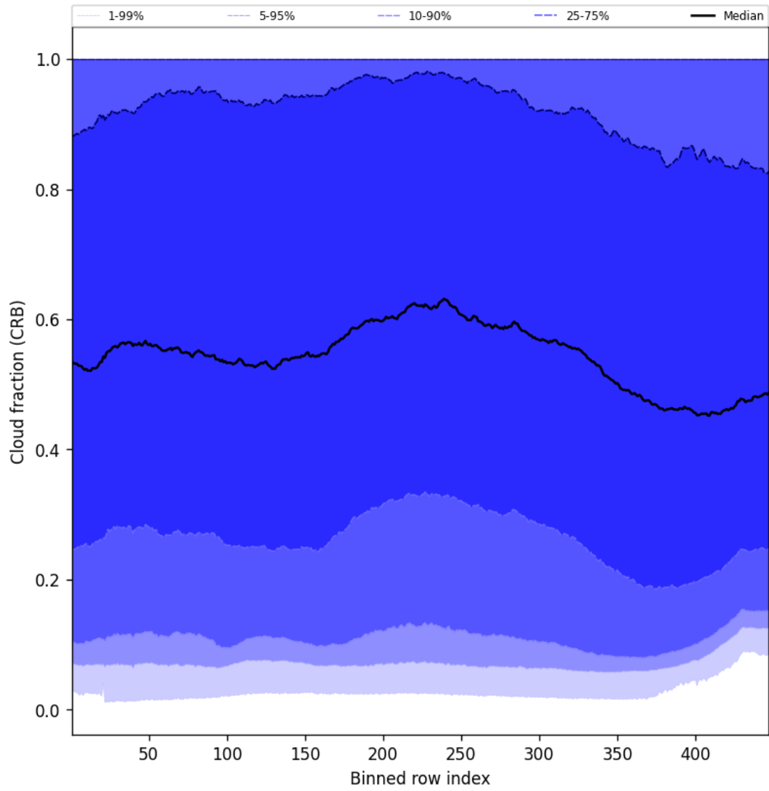
Figure 58: Along track statistics of “Cloud fraction (CRB)” for 2024-11-12 to 2024-11-14
