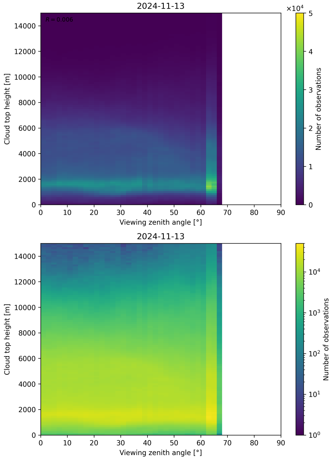
Figure 112: Scatter density plot of “Viewing zenith angle” against “Cloud top height” for 2024-11-12 to 2024-11-14.
