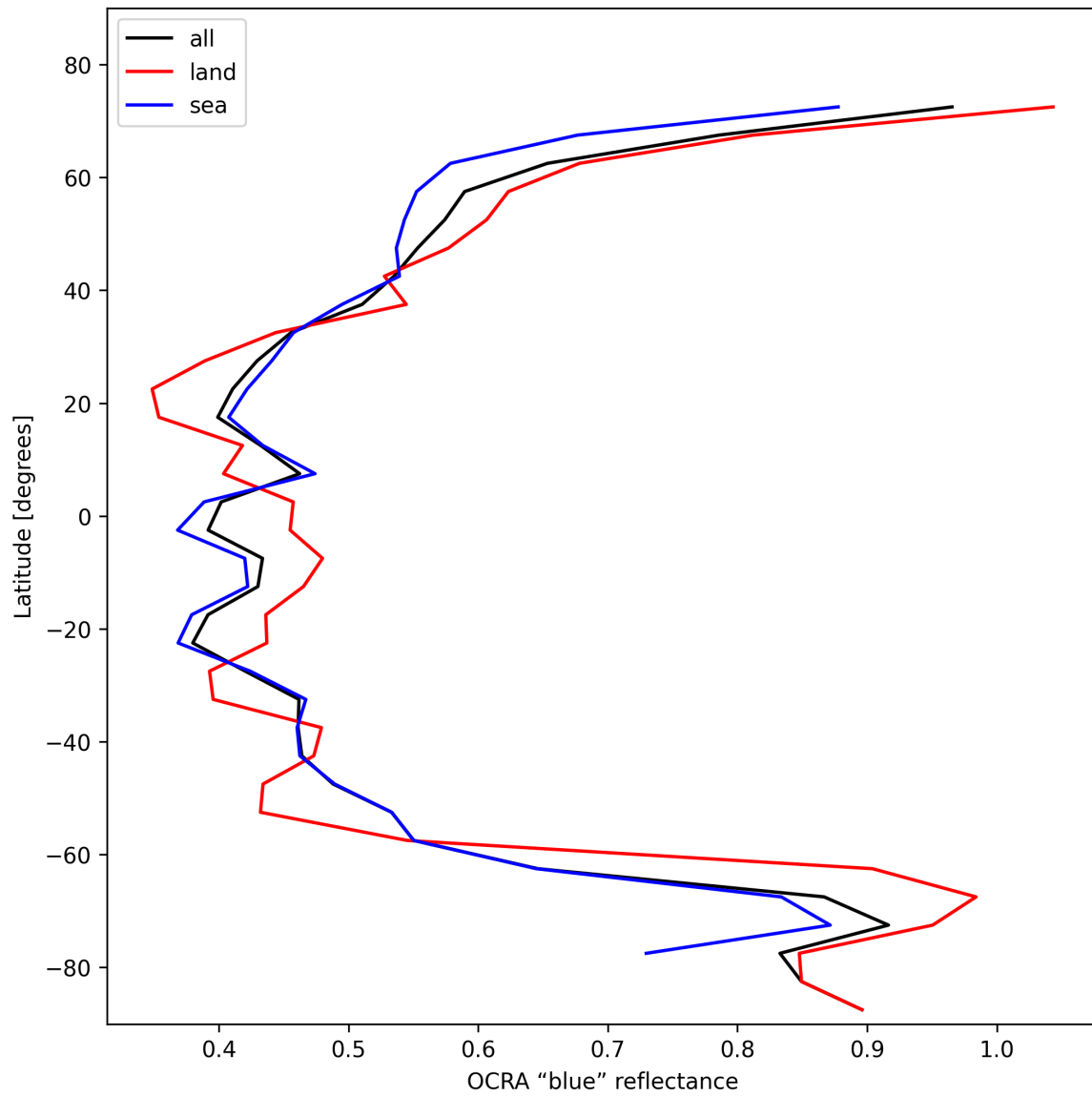
Figure 35: Zonal average of "OCRA "blue" reflectance" for 2024-11-12 to 2024-11-14.
