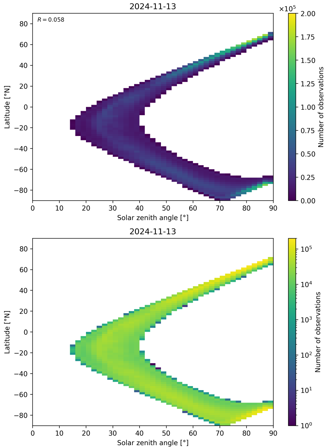
Figure 105: Scatter density plot of “Solar zenith angle” against “Latitude” for 2024-11-12 to 2024-11-14.
