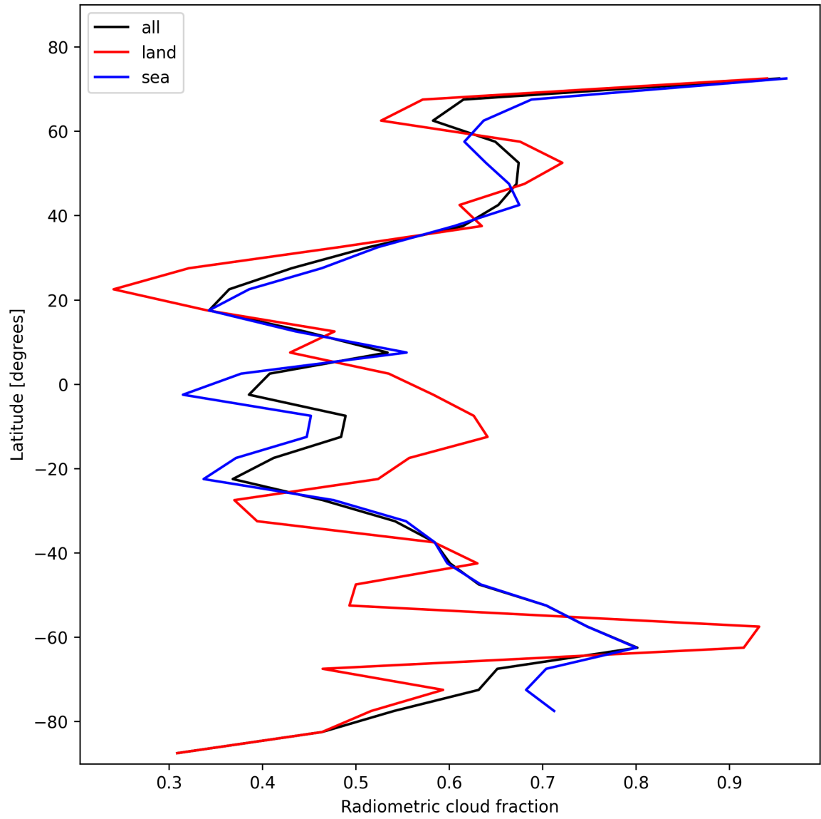
Figure 23: Zonal average of “Radiometric cloud fraction” for 2024-11-12 to 2024-11-14.
