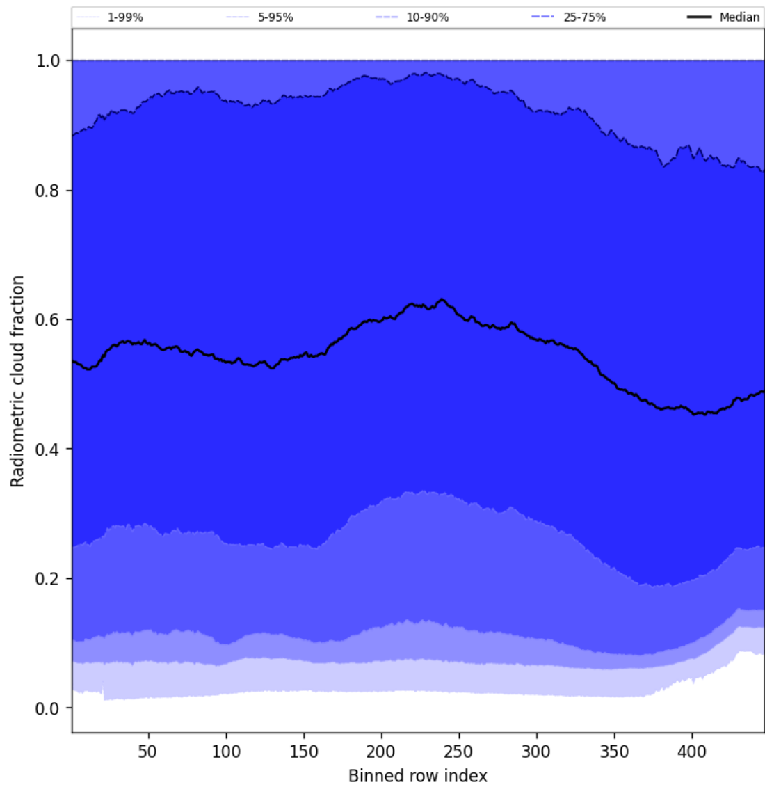
Figure 55: Along track statistics of “Radiometric cloud fraction” for 2024-11-12 to 2024-11-14
