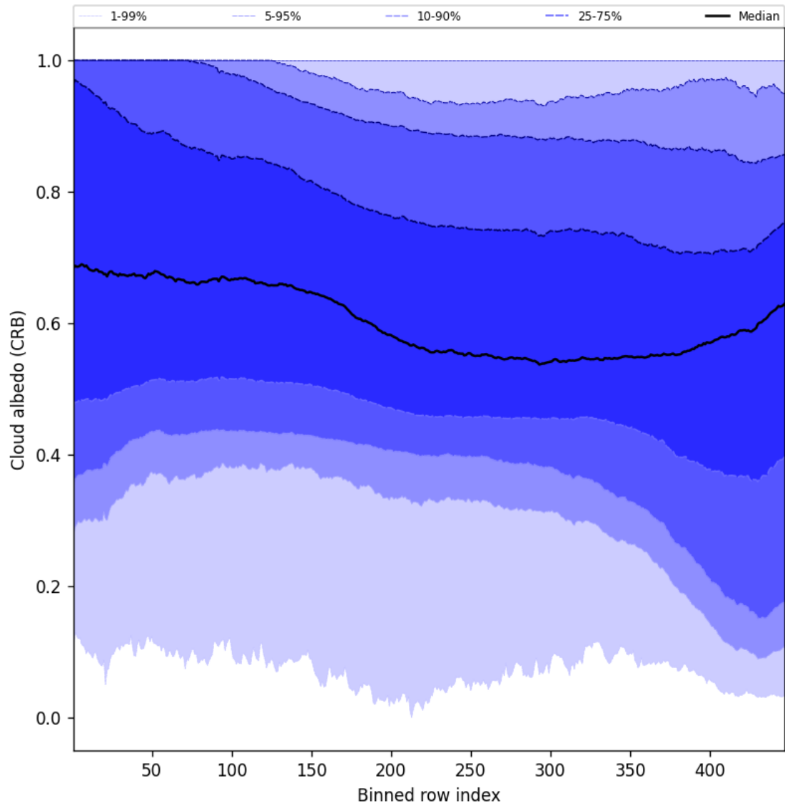
Figure 60: Along track statistics of “Cloud albedo (CRB)” for 2024-11-12 to 2024-11-14
