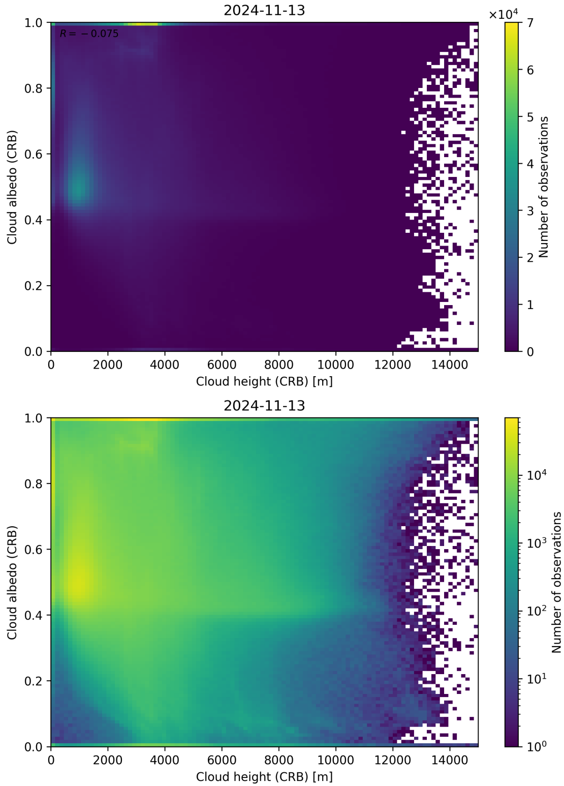
Figure 80: Scatter density plot of “Cloud height (CRB)” against “Cloud albedo (CRB)” for 2024-11-12 to 2024-11-14.
