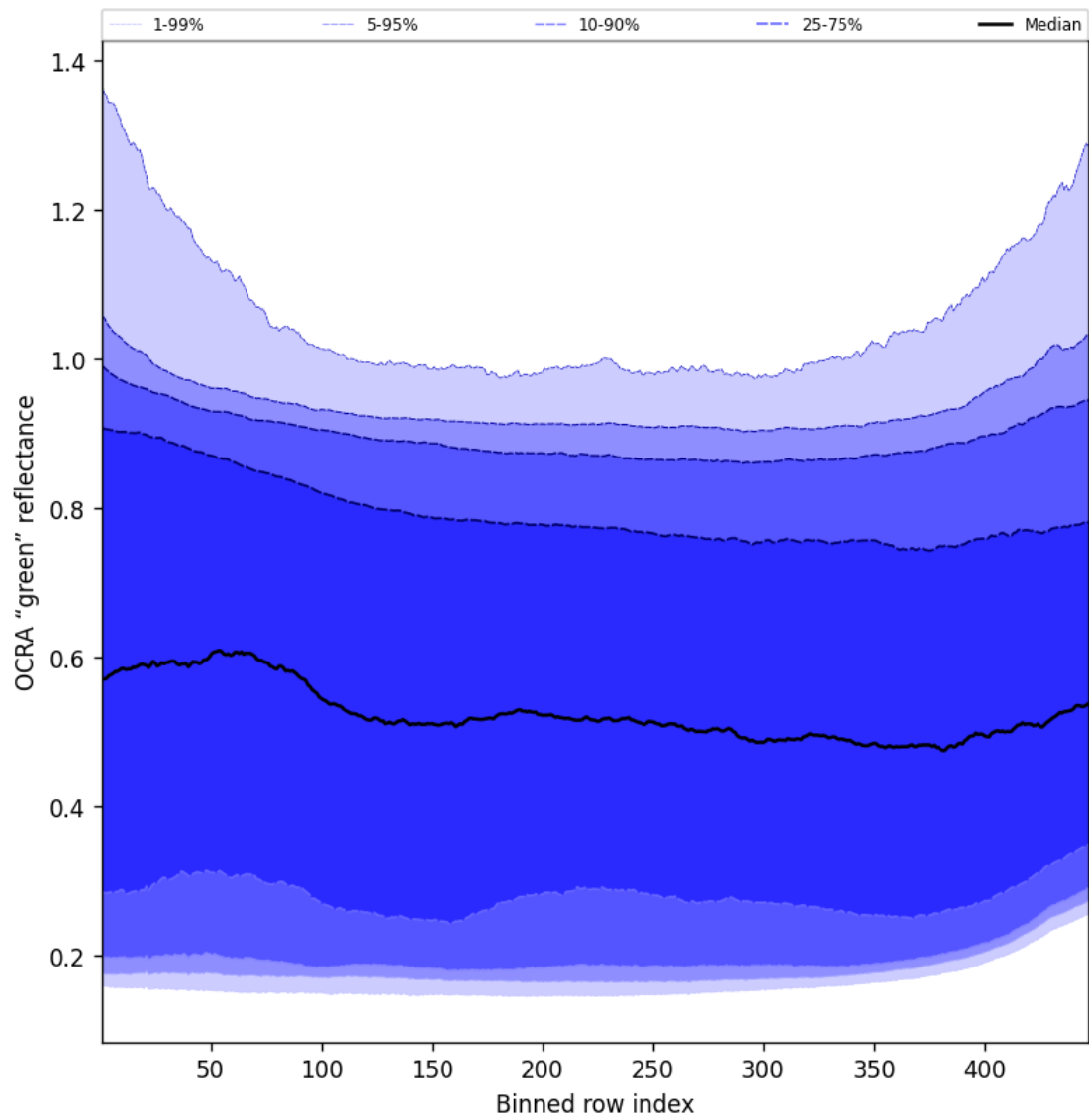
Figure 68: Along track statistics of “OCRA “green” reflectance” for 2024-11-12 to 2024-11-14
