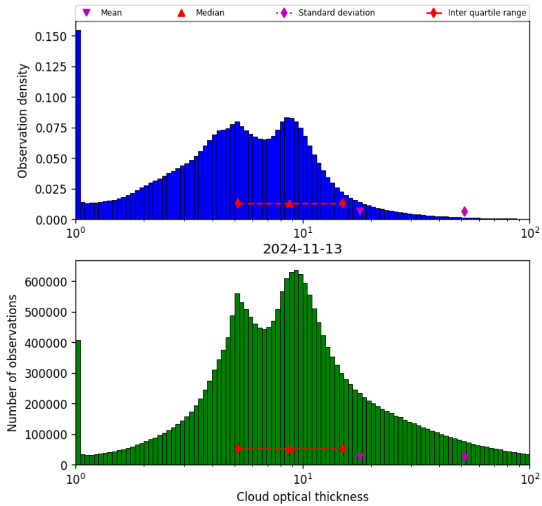
Figure 41: Histogram of “Cloud optical thickness” for 2024-11-12 to 2024-11-14
