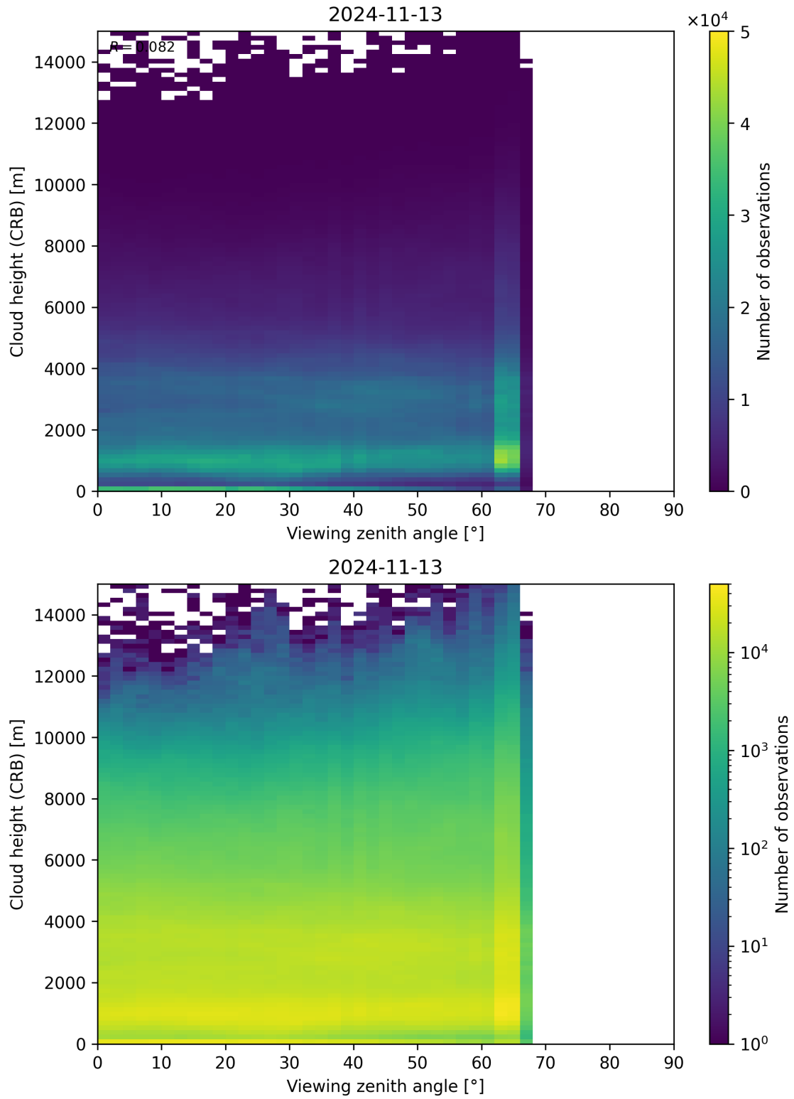
Figure 110: Scatter density plot of “Viewing zenith angle” against “Cloud height (CRB)” for 2024-11-12 to 2024-11-14.
