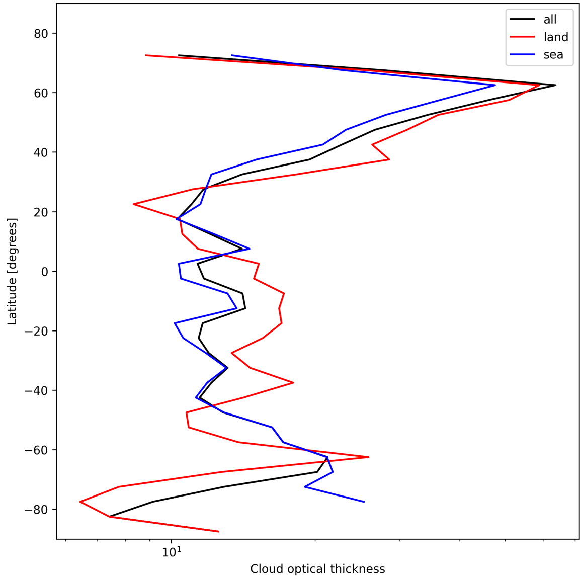
Figure 25: Zonal average of “Cloud optical thickness” for 2024-11-12 to 2024-11-14.
