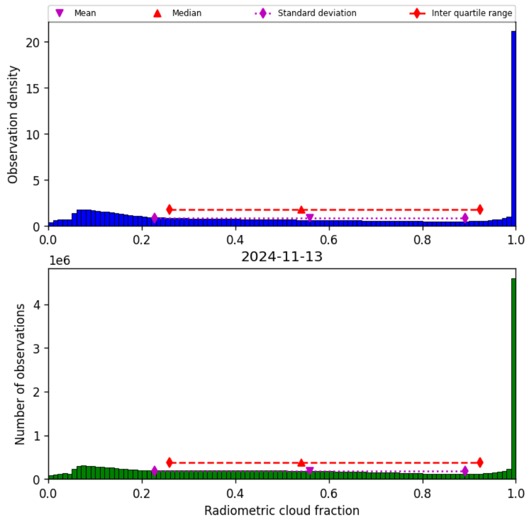
Figure 39: Histogram of “Radiometric cloud fraction” for 2024-11-12 to 2024-11-14
