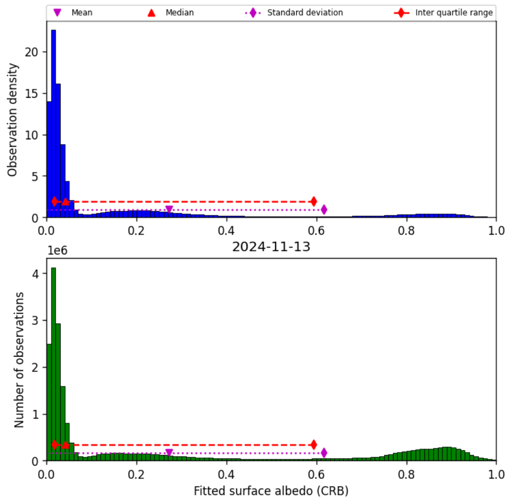
Figure 46: Histogram of “Fitted surface albedo (CRB)” for 2024-11-12 to 2024-11-14
