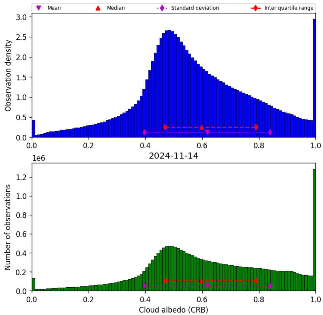
Figure 44: Histogram of “Cloud albedo (CRB)” for 2024-11-14 to 2024-11-15
