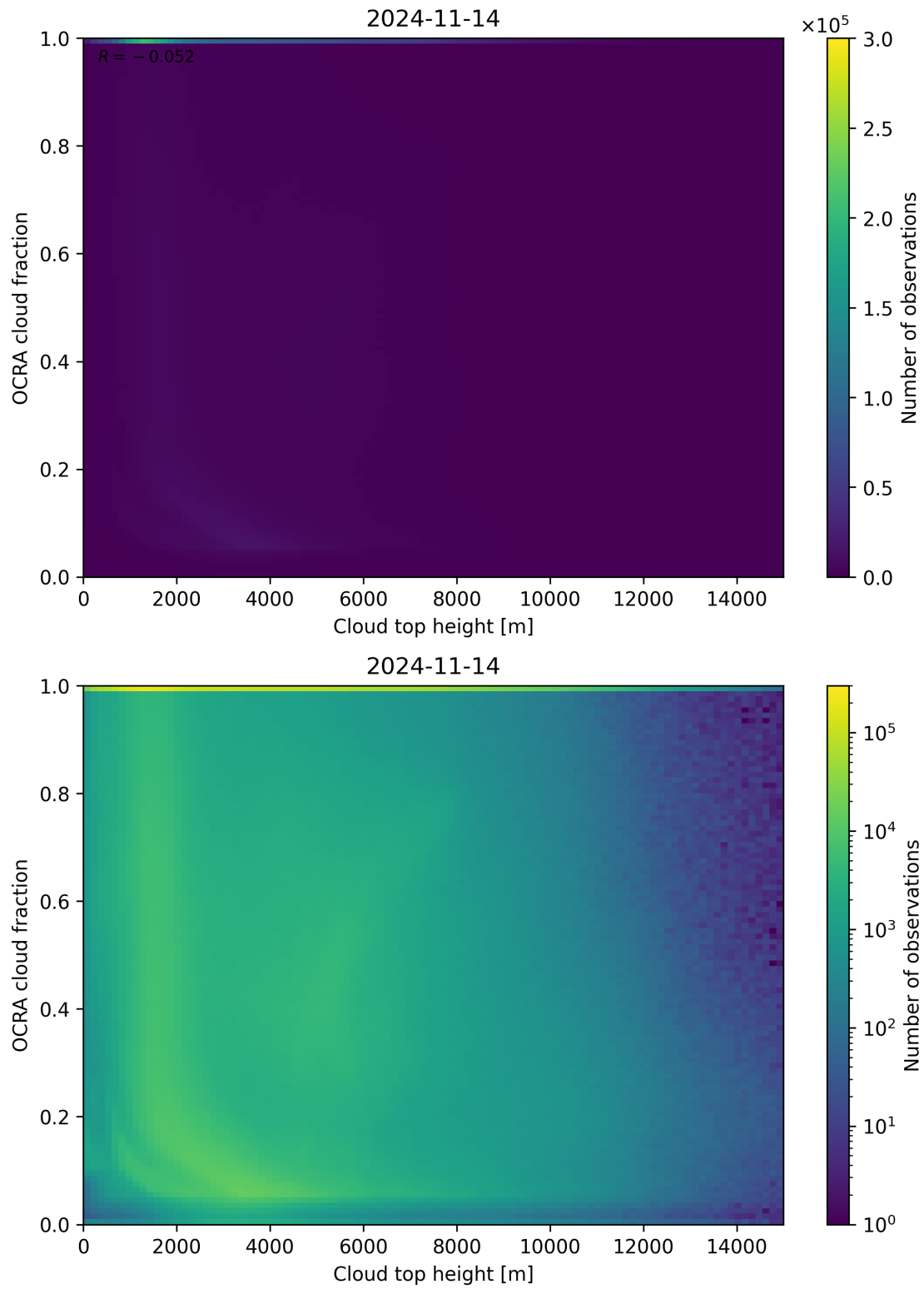
Figure 87: Scatter density plot of “Cloud top height” against “OCRA cloud fraction” for 2024-11-14 to 2024-11-15.
