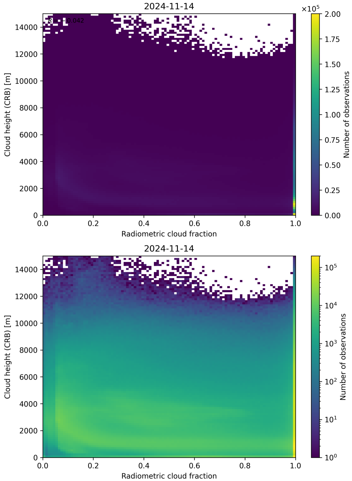
Figure 74: Scatter density plot of “Radiometric cloud fraction” against “Cloud height (CRB)” for 2024-11-14 to 2024-11-15.
