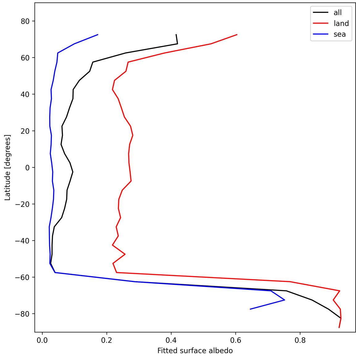
Figure 29: Zonal average of “Fitted surface albedo” for 2024-11-14 to 2024-11-15.
