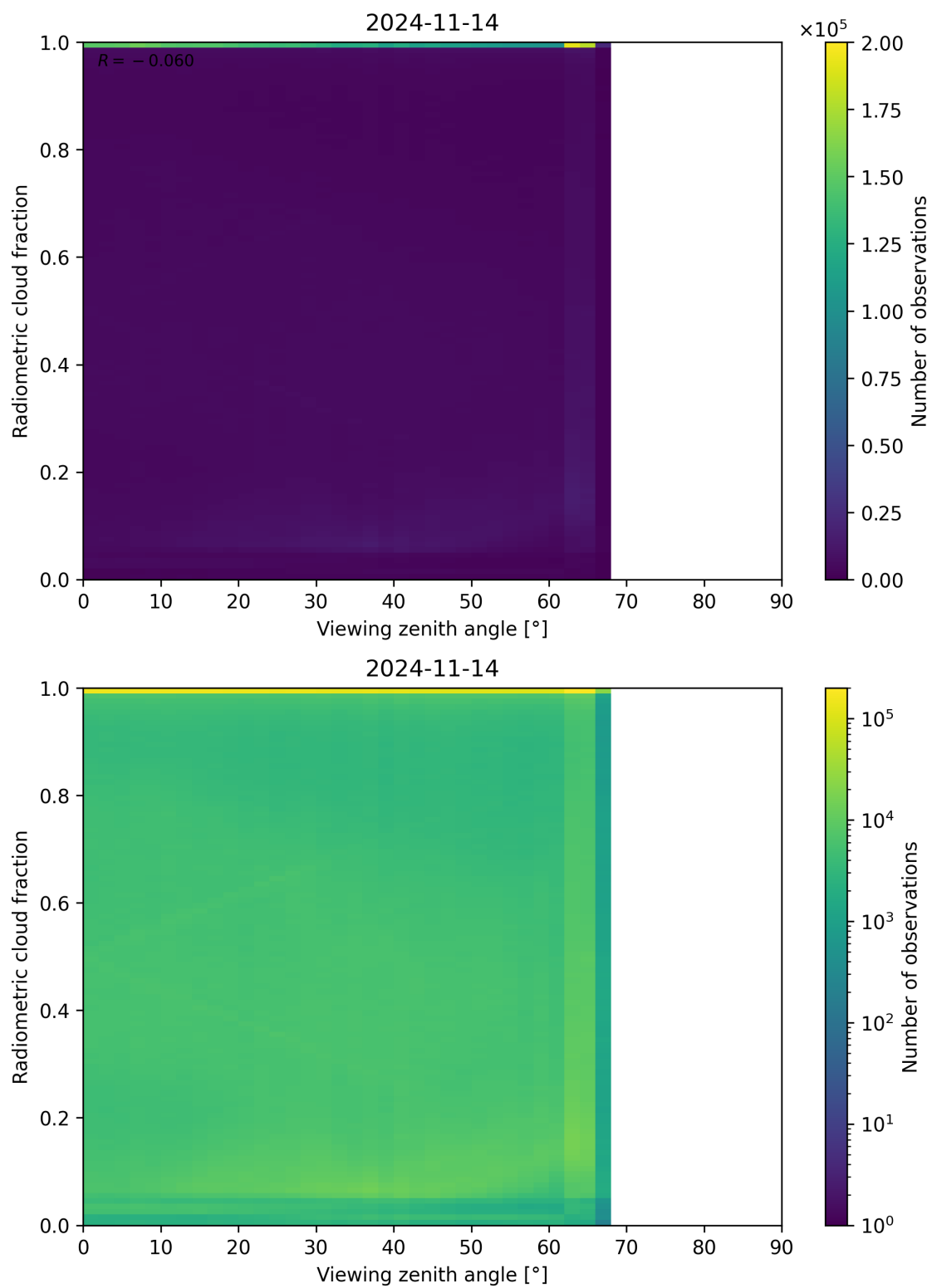
Figure 107: Scatter density plot of “Viewing zenith angle” against “Radiometric cloud fraction” for 2024-11-14 to 2024-11-15.
