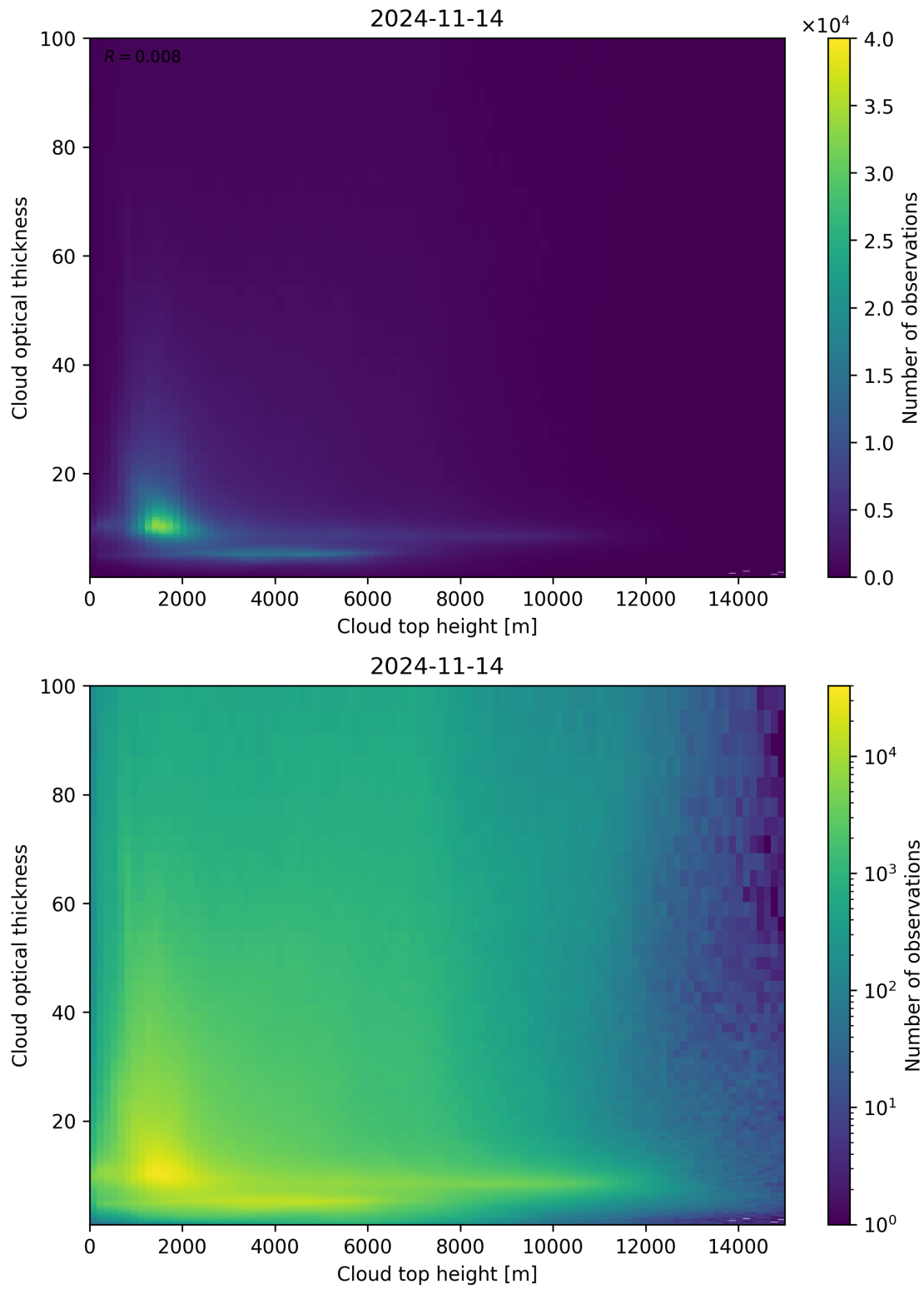
Figure 90: Scatter density plot of “Cloud top height” against “Cloud optical thickness” for 2024-11-14 to 2024-11-15.
