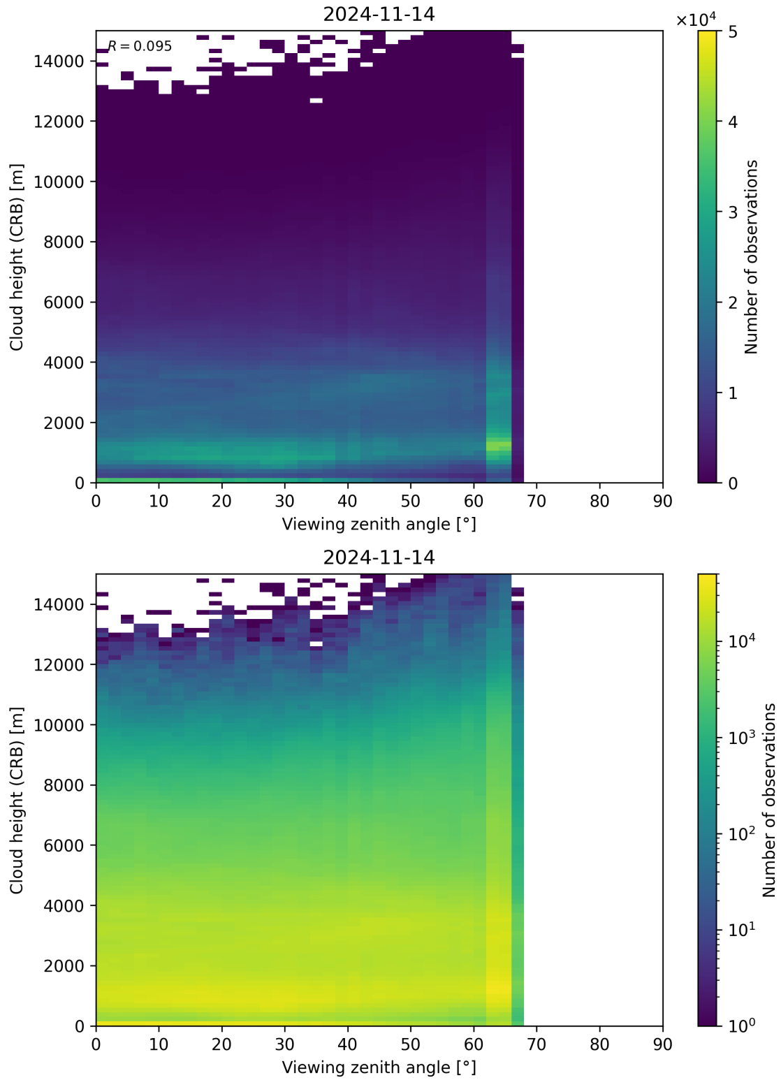
Figure 110: Scatter density plot of “Viewing zenith angle” against “Cloud height (CRB)” for 2024-11-14 to 2024-11-15.
