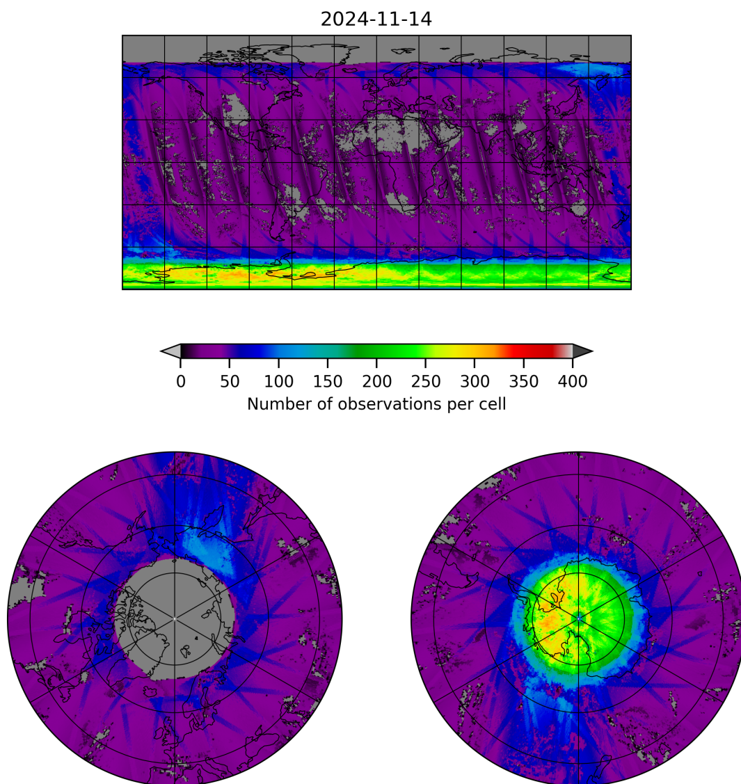
Figure 21: Map of the number of observations for 2024-11-14 to 2024-11-15
