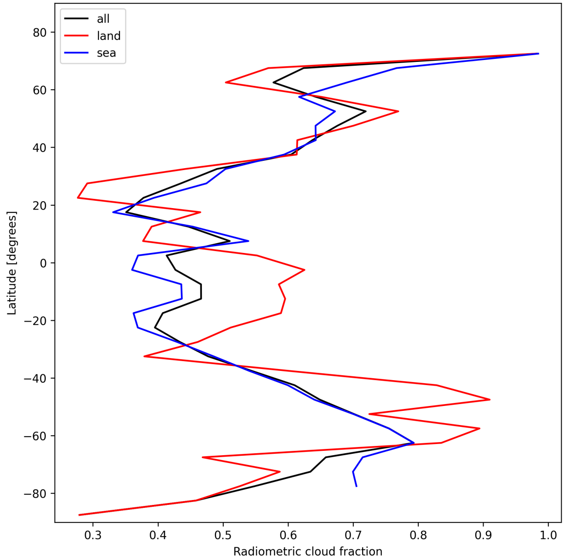
Figure 23: Zonal average of “Radiometric cloud fraction” for 2024-11-14 to 2024-11-15.
