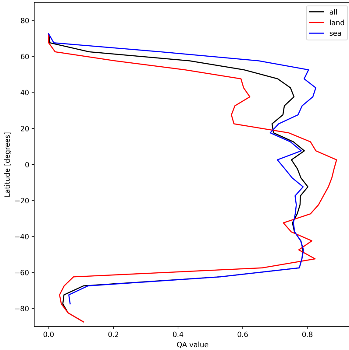
Figure 22: Zonal average of “QA value” for 2024-11-14 to 2024-11-15.
