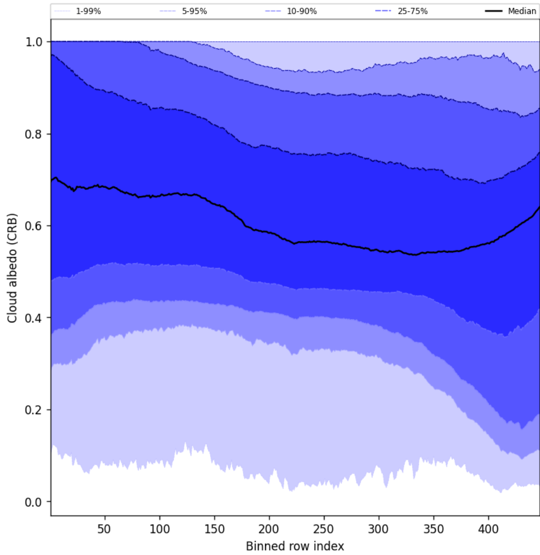
Figure 60: Along track statistics of “Cloud albedo (CRB)” for 2024-11-14 to 2024-11-15
