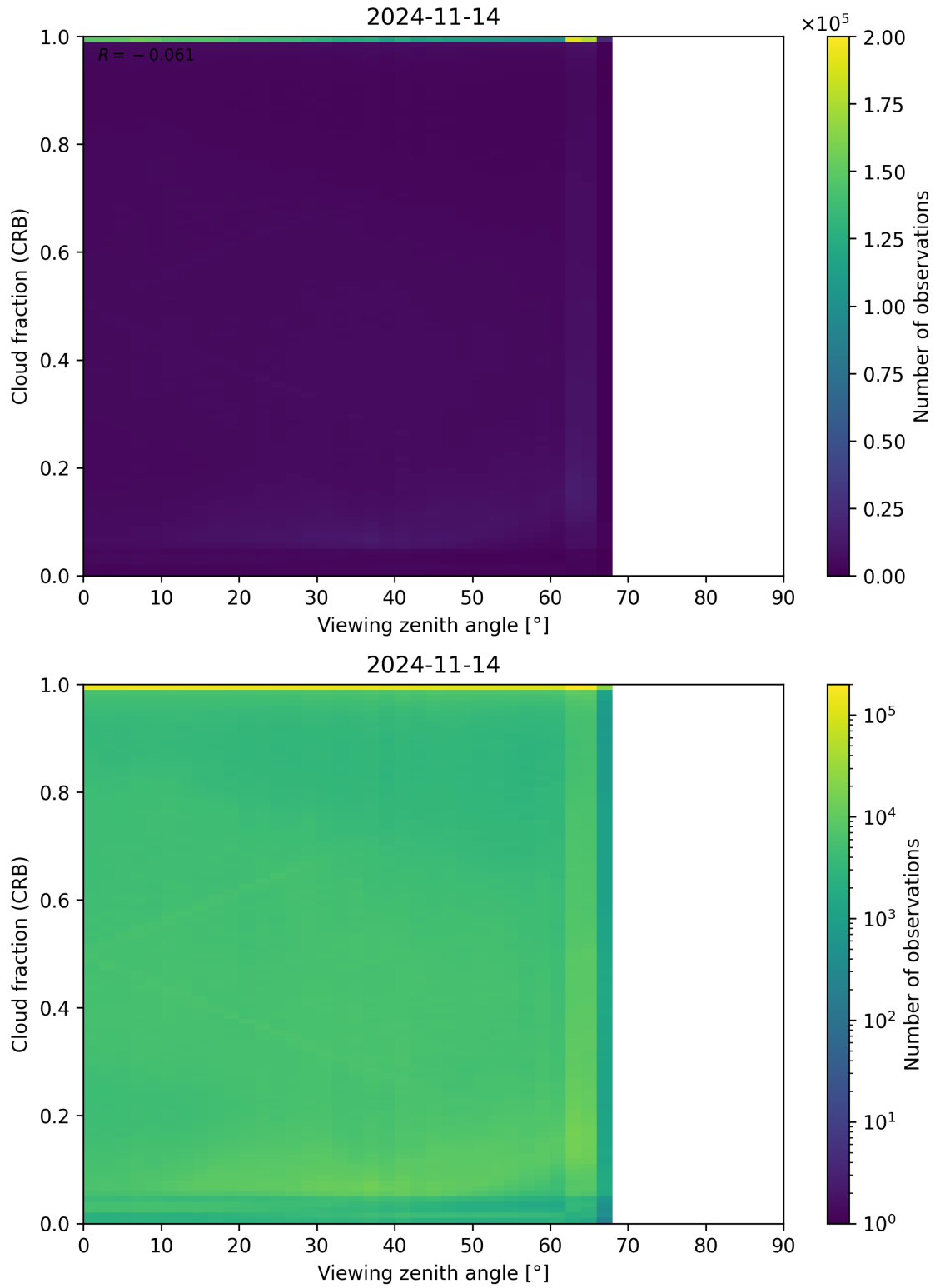
Figure 109: Scatter density plot of “Viewing zenith angle” against “Cloud fraction (CRB)” for 2024-11-14 to 2024-11-15.
