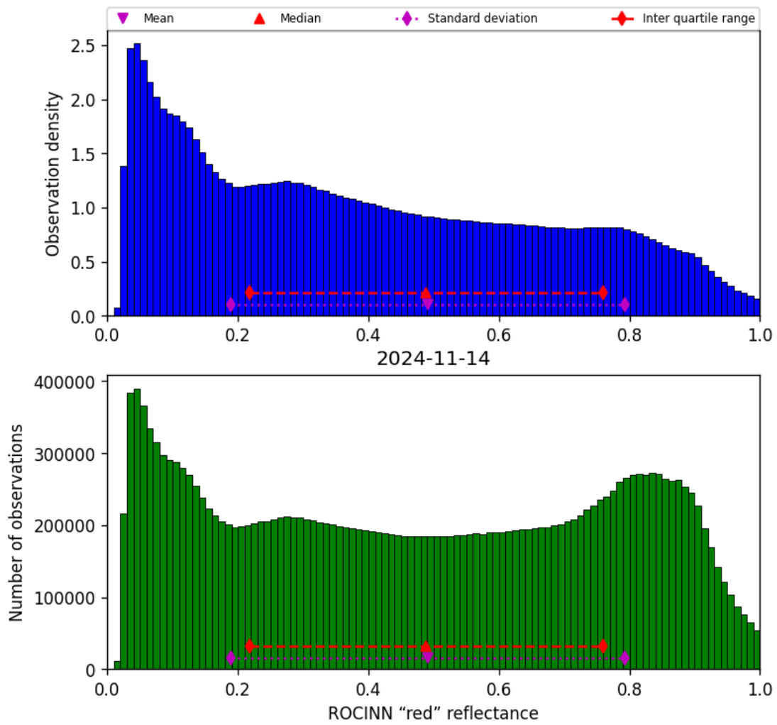
Figure 53: Histogram of “ROCINN “red” reflectance” for 2024-11-14 to 2024-11-15
