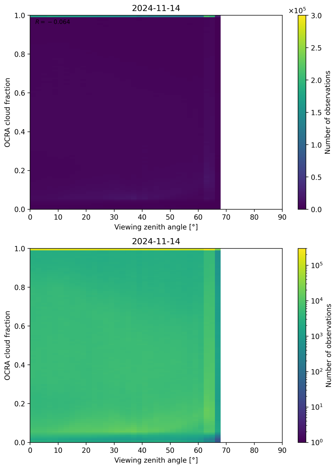
Figure 108: Scatter density plot of “Viewing zenith angle” against “OCRA cloud fraction” for 2024-11-14 to 2024-11-15.
