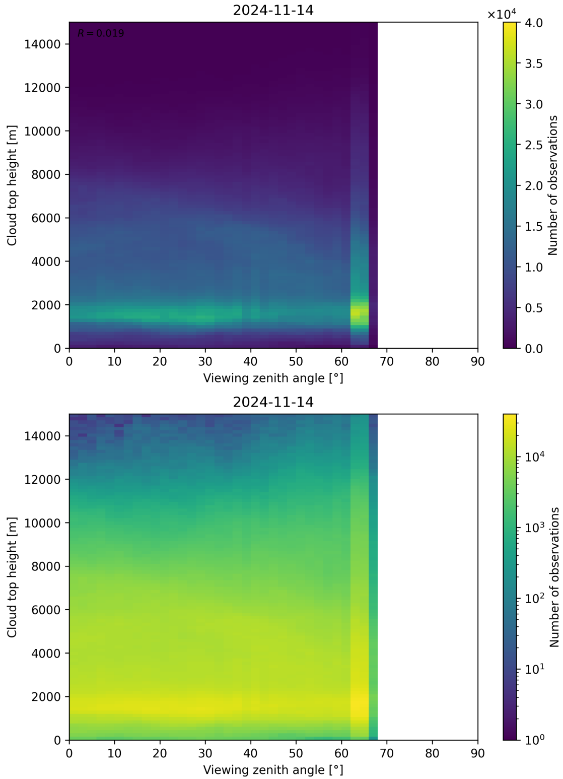
Figure 112: Scatter density plot of “Viewing zenith angle” against “Cloud top height” for 2024-11-14 to 2024-11-15.
