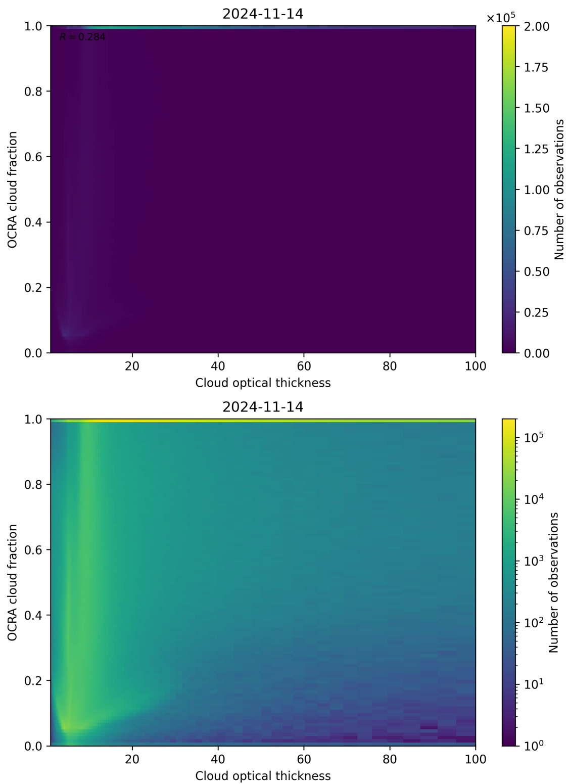
Figure 83: Scatter density plot of “Cloud optical thickness” against “OCRA cloud fraction” for 2024-11-14 to 2024-11-15.
