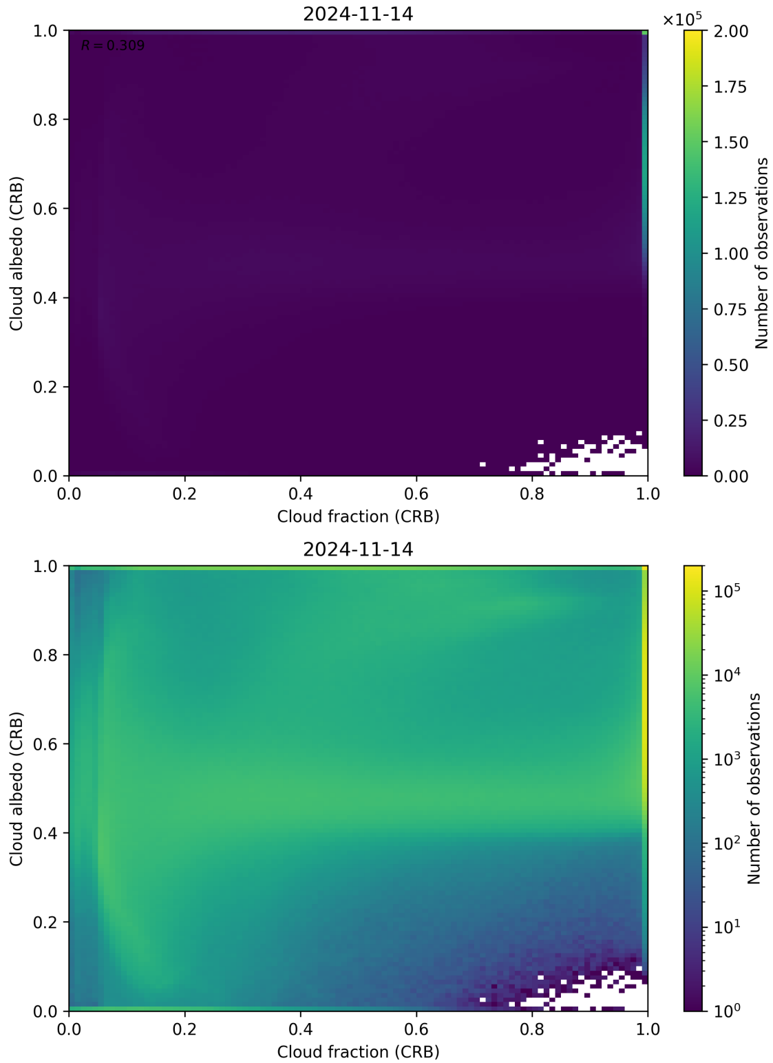
Figure 77: Scatter density plot of “Cloud fraction (CRB)” against “Cloud albedo (CRB)” for 2024-11-14 to 2024-11-15.
