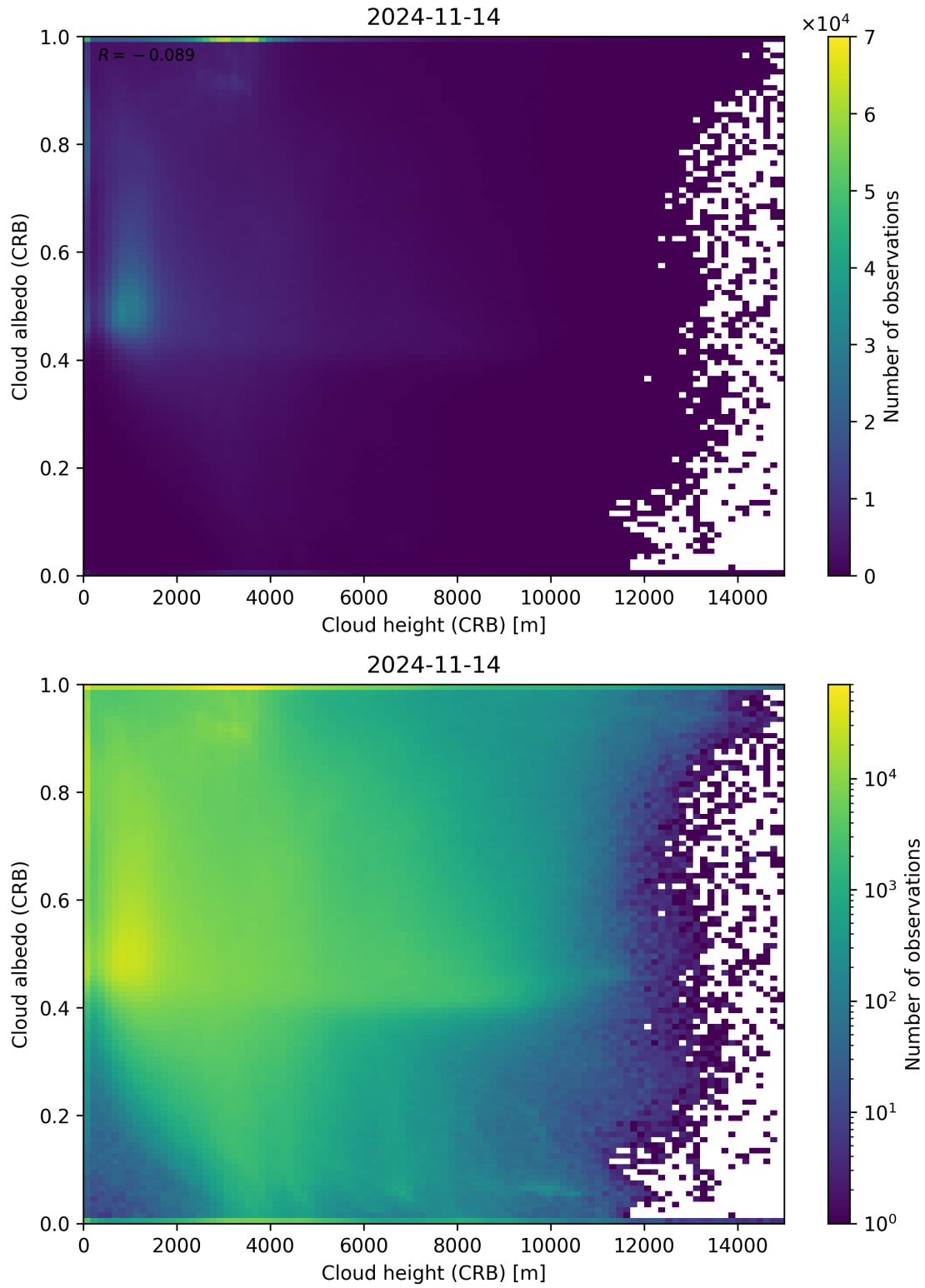
Figure 80: Scatter density plot of “Cloud height (CRB)” against “Cloud albedo (CRB)” for 2024-11-14 to 2024-11-15.
