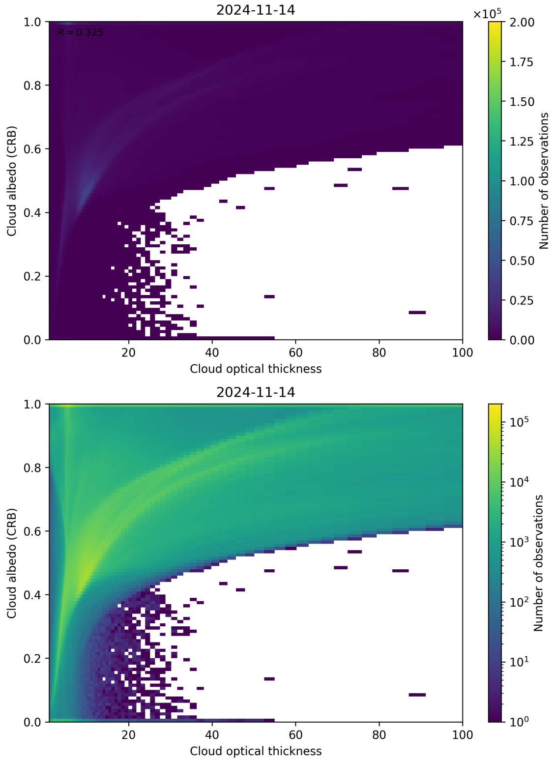
Figure 82: Scatter density plot of “Cloud optical thickness” against “Cloud albedo (CRB)” for 2024-11-14 to 2024-11-15.
