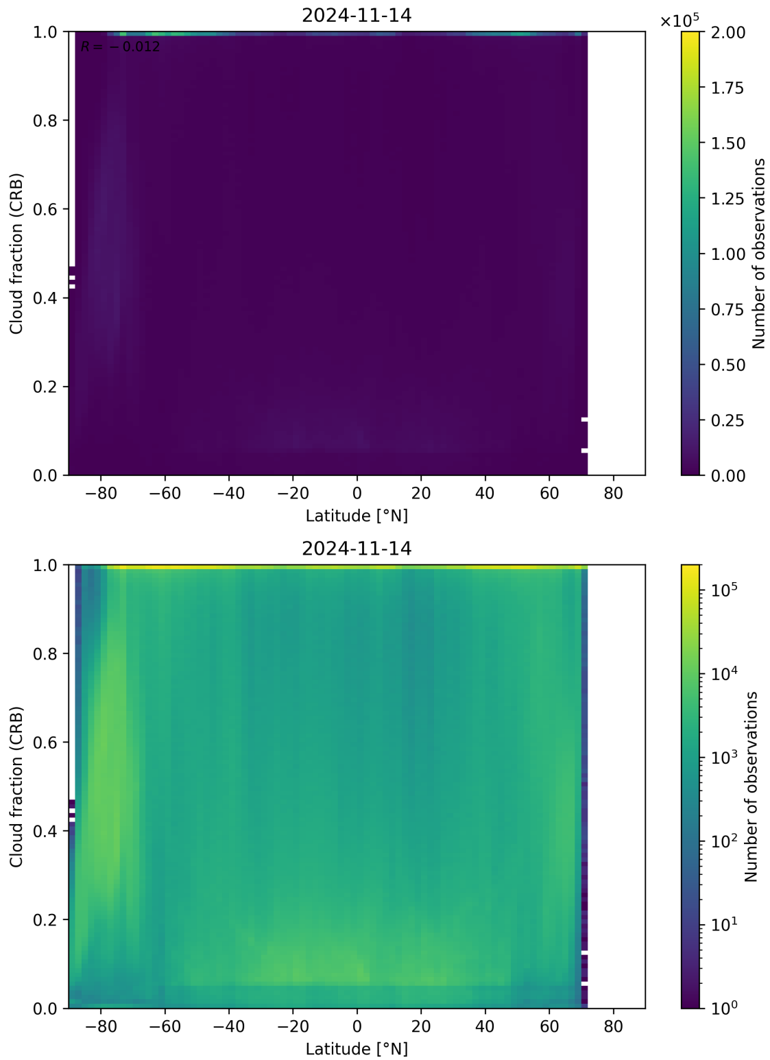
Figure 94: Scatter density plot of “Latitude” against “Cloud fraction (CRB)” for 2024-11-14 to 2024-11-15.
