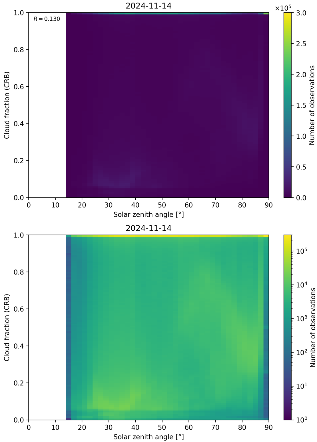
Figure 101: Scatter density plot of “Solar zenith angle” against “Cloud fraction (CRB)” for 2024-11-14 to 2024-11-15.
