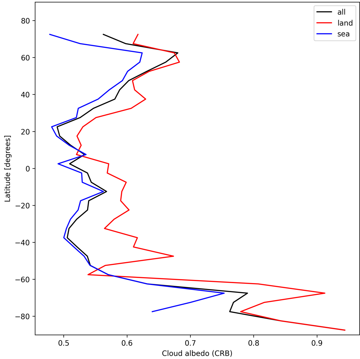
Figure 28: Zonal average of “Cloud albedo (CRB)” for 2024-11-14 to 2024-11-15.
