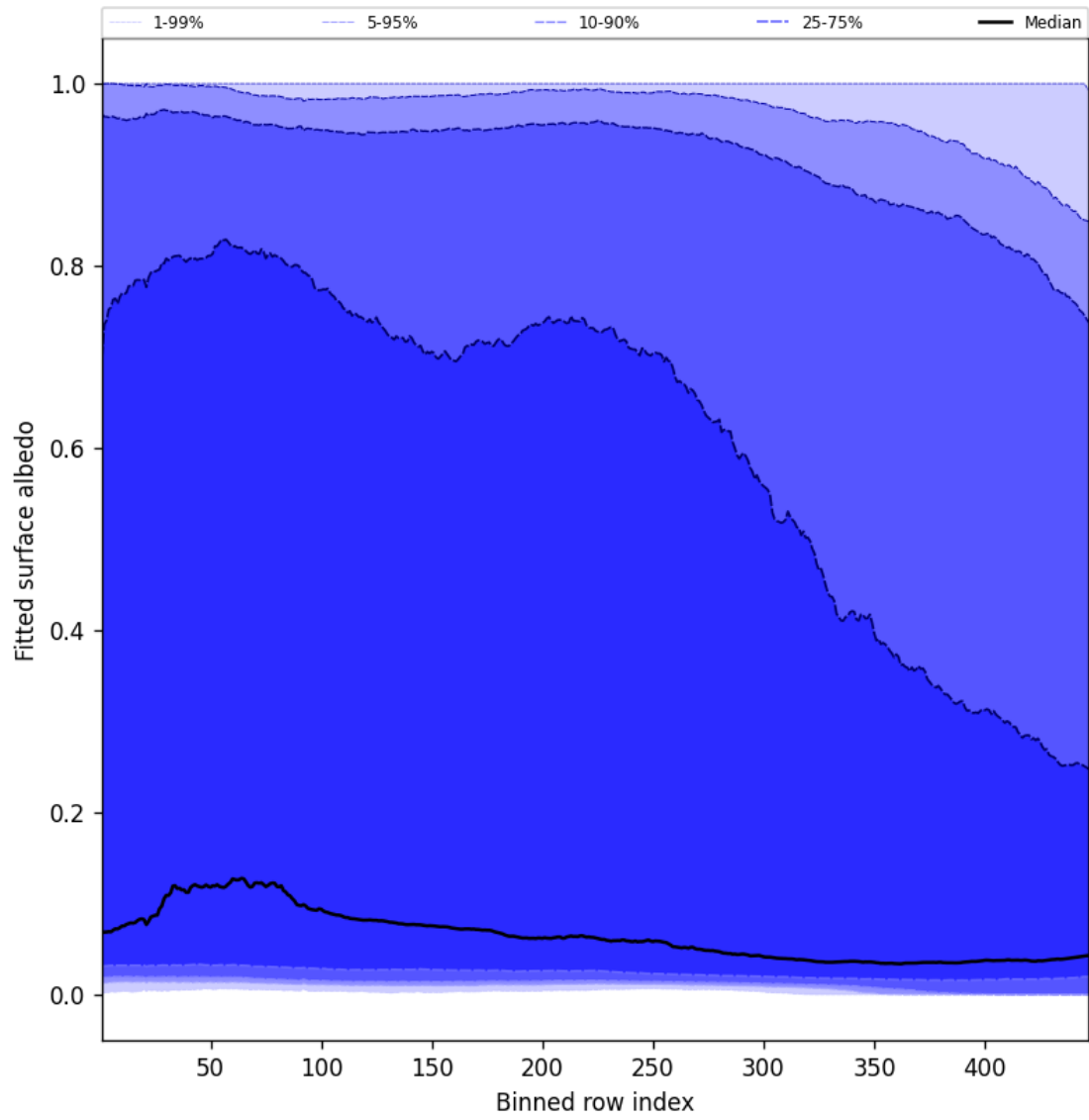
Figure 61: Along track statistics of “Fitted surface albedo” for 2024-11-14 to 2024-11-15
