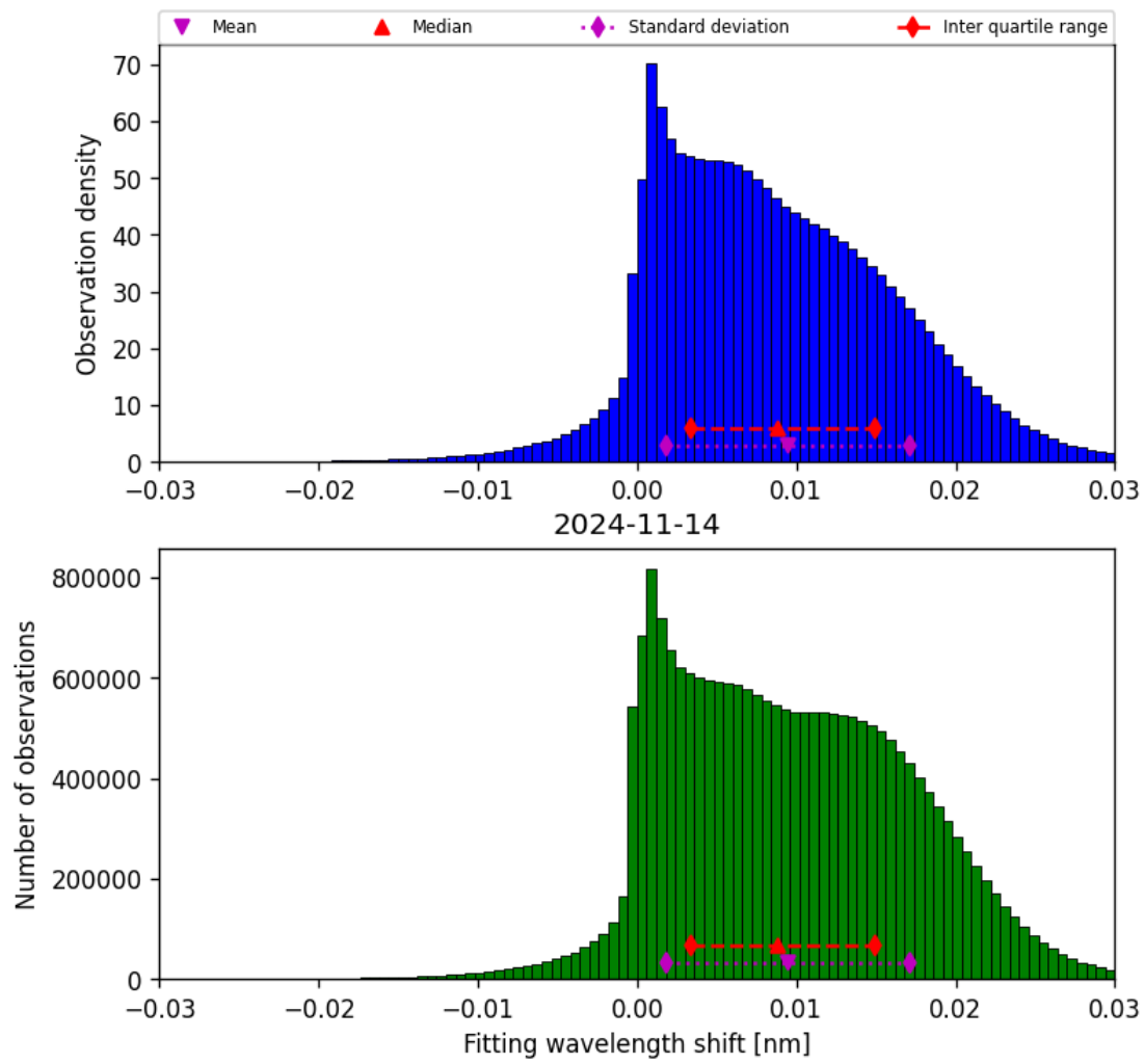
Figure 49: Histogram of “Fitting wavelength shift” for 2024-11-14 to 2024-11-15
