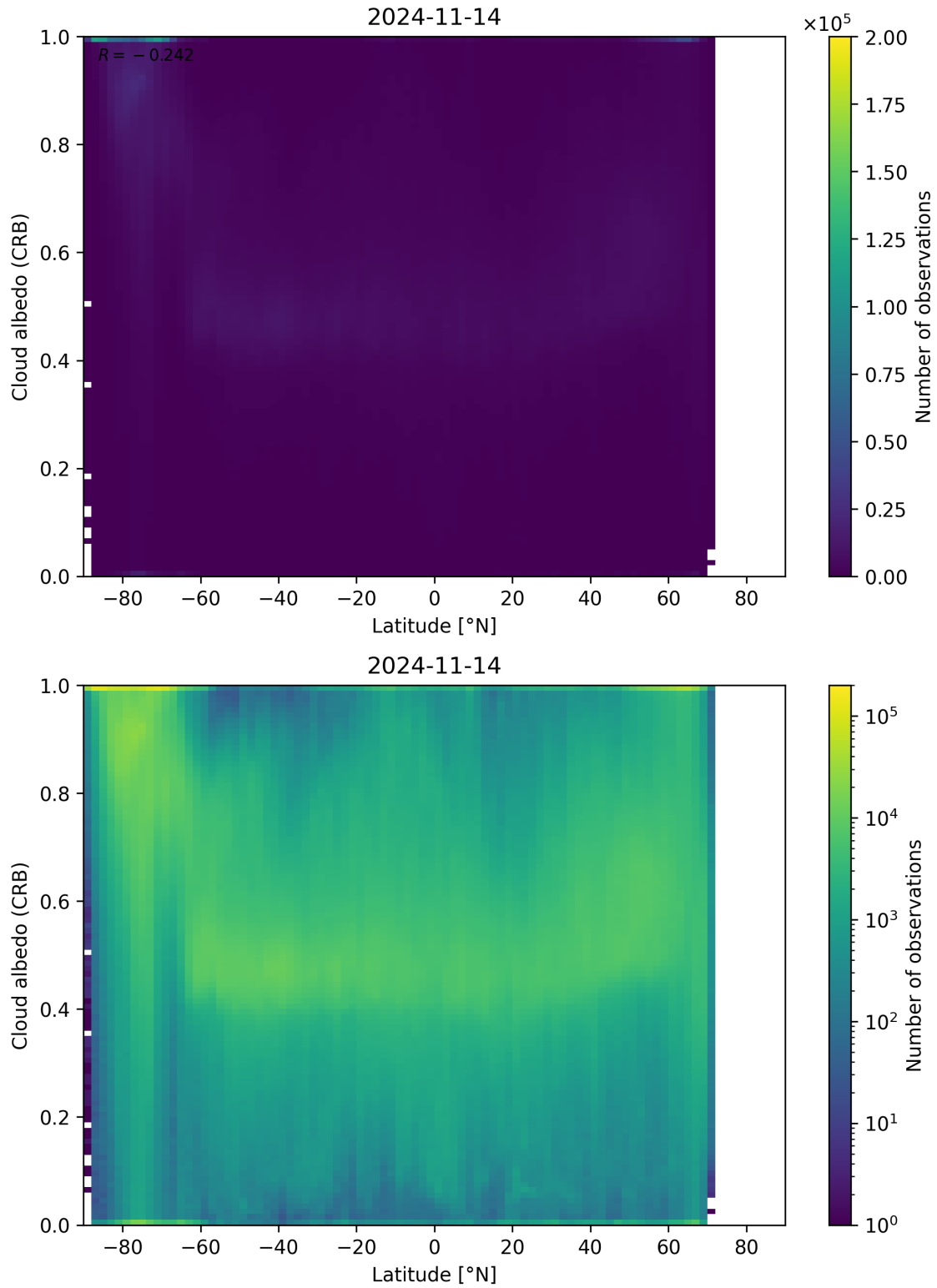
Figure 91: Scatter density plot of “Latitude” against “Cloud albedo (CRB)” for 2024-11-14 to 2024-11-15.
