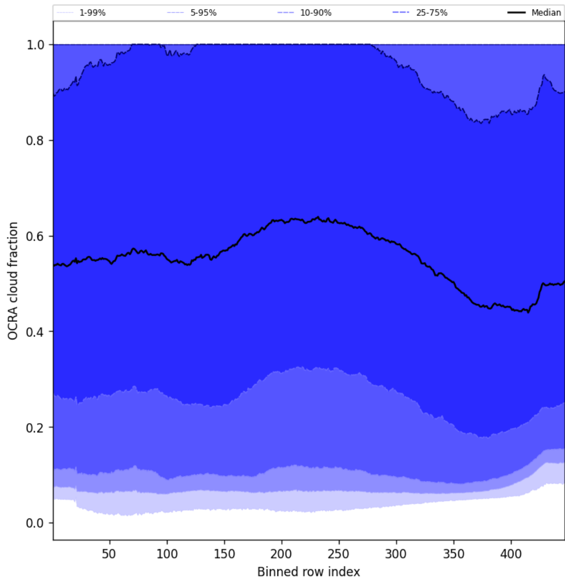
Figure 66: Along track statistics of “OCRA cloud fraction” for 2024-11-14 to 2024-11-15
