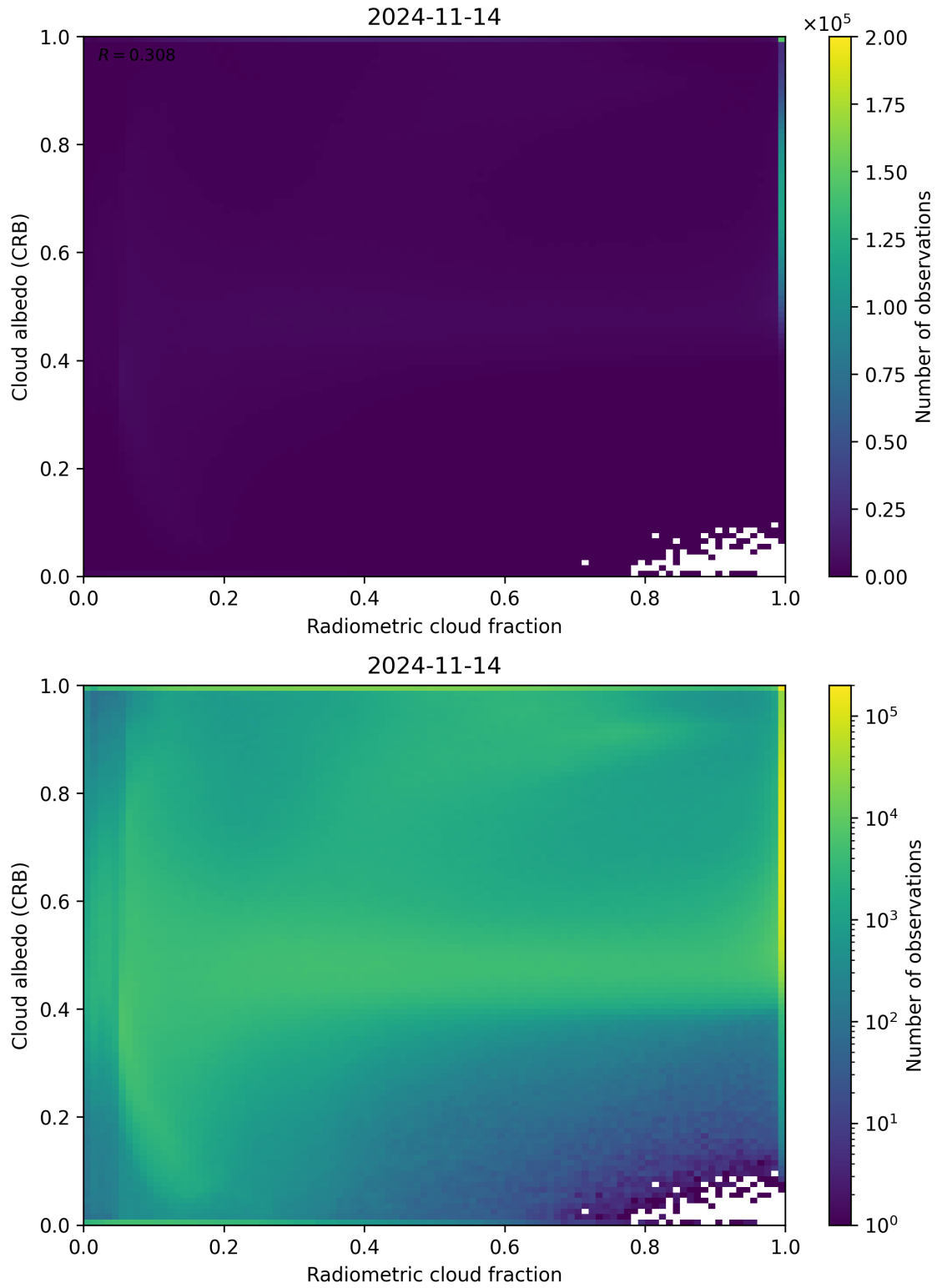
Figure 71: Scatter density plot of “Radiometric cloud fraction” against “Cloud albedo (CRB)” for 2024-11-14 to 2024-11-15.
