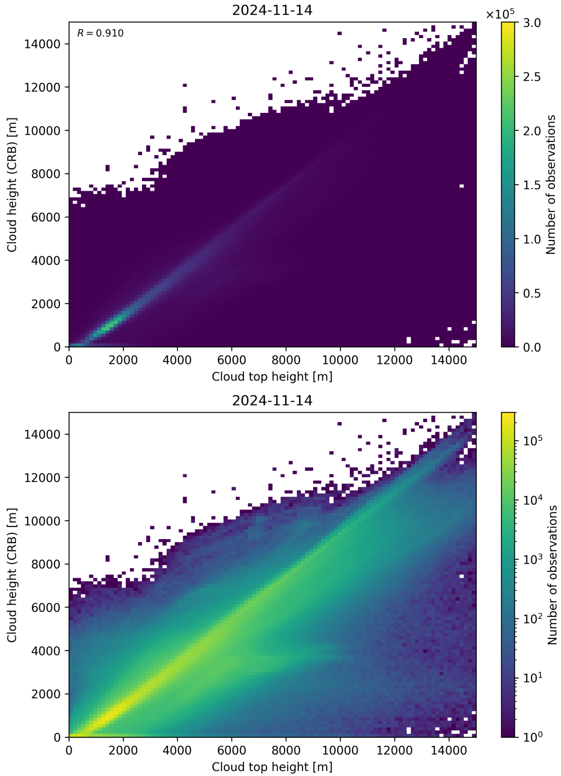
Figure 89: Scatter density plot of “Cloud top height” against “Cloud height (CRB)” for 2024-11-14 to 2024-11-15.
