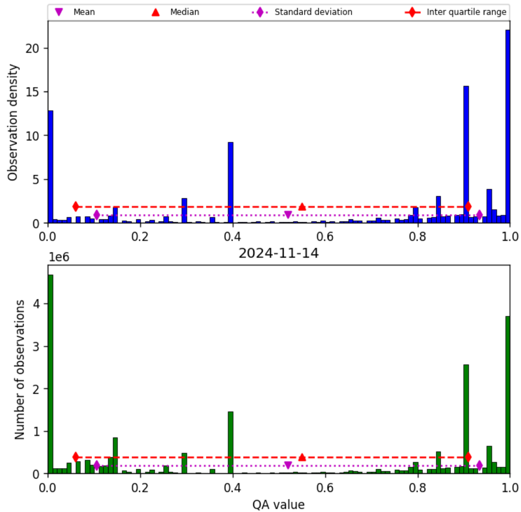
Figure 38: Histogram of “QA value” for 2024-11-14 to 2024-11-15
