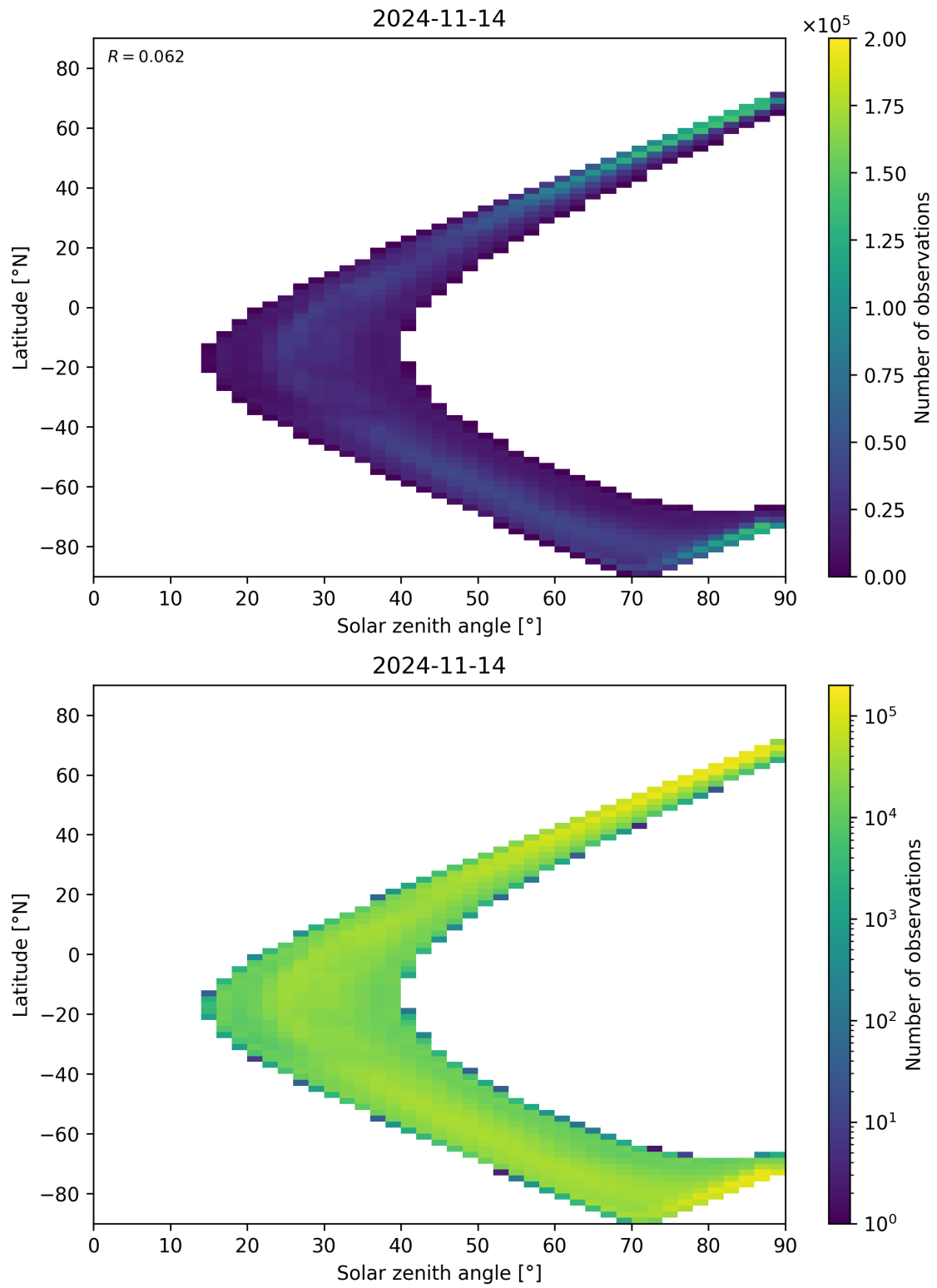
Figure 105: Scatter density plot of “Solar zenith angle” against “Latitude” for 2024-11-14 to 2024-11-15.
