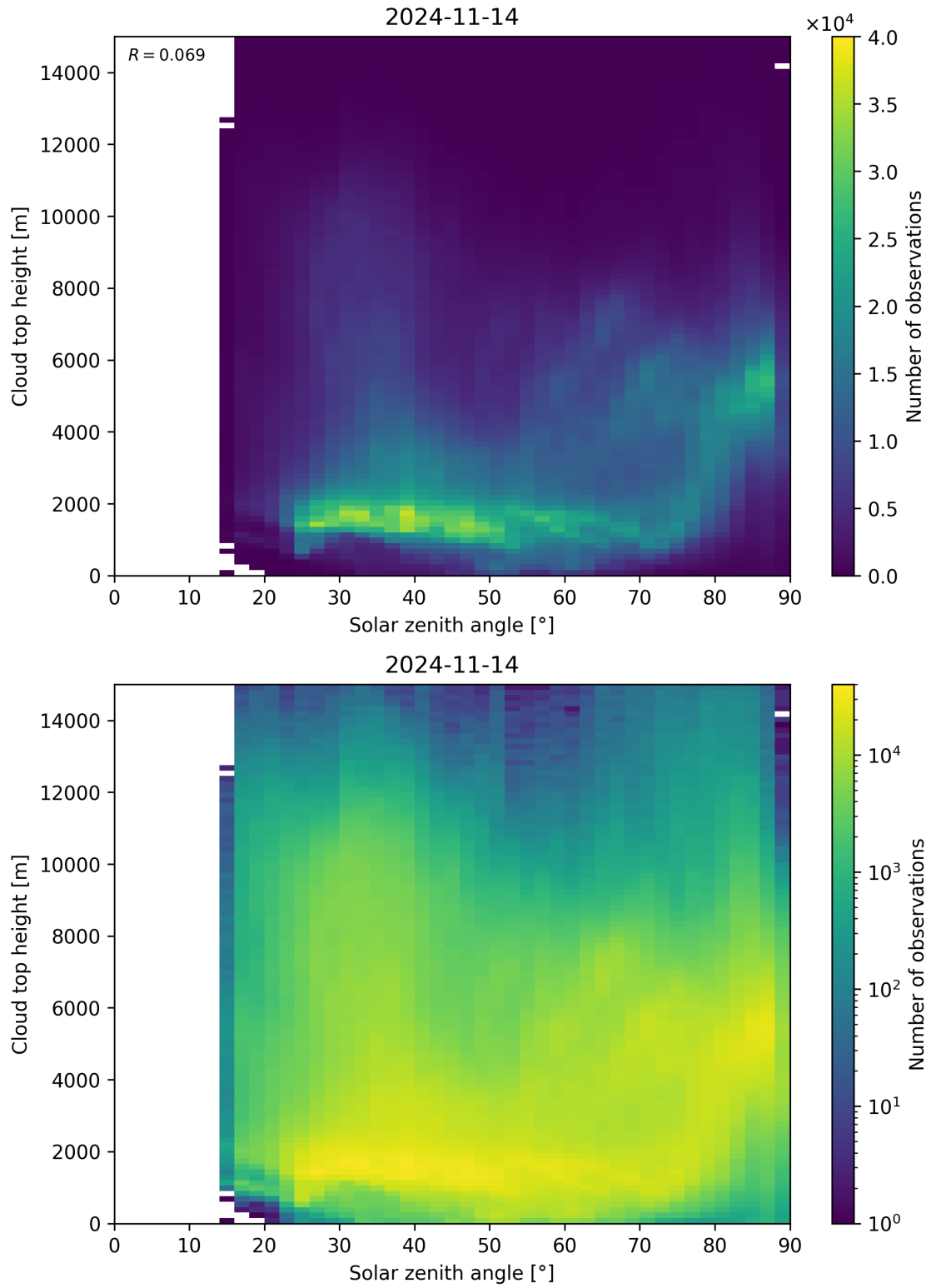
Figure 104: Scatter density plot of “Solar zenith angle” against “Cloud top height” for 2024-11-14 to 2024-11-15.
