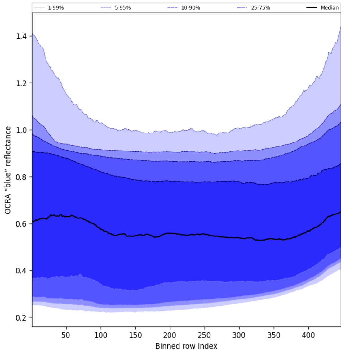
Figure 67: Along track statistics of “OCRA “blue” reflectance” for 2024-11-14 to 2024-11-15
