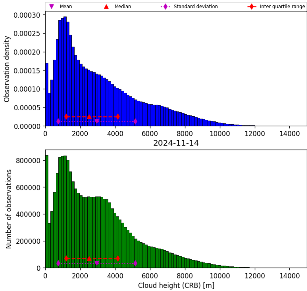
Figure 43: Histogram of “Cloud height (CRB)” for 2024-11-14 to 2024-11-15
