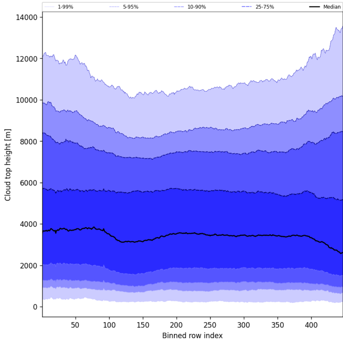
Figure 56: Along track statistics of “Cloud top height” for 2024-11-14 to 2024-11-15
