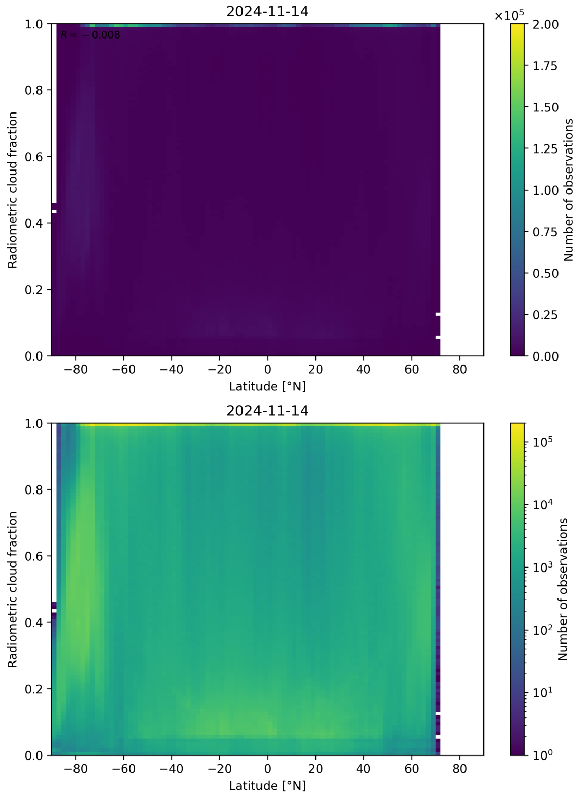
Figure 92: Scatter density plot of “Latitude” against “Radiometric cloud fraction” for 2024-11-14 to 2024-11-15.
