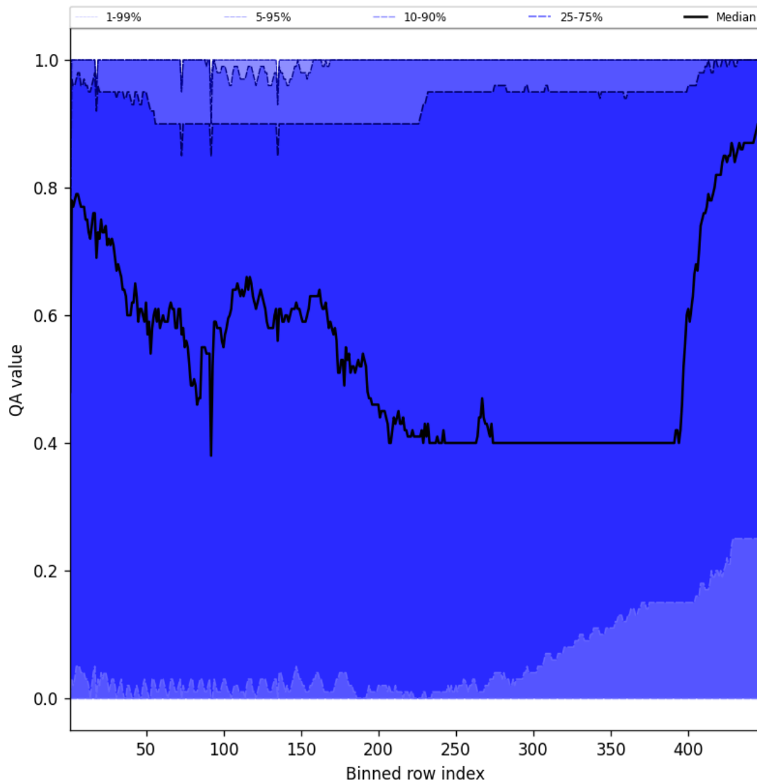
Figure 54: Along track statistics of “QA value” for 2024-11-14 to 2024-11-15
