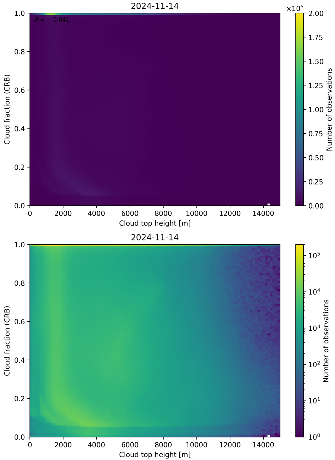
Figure 88: Scatter density plot of “Cloud top height” against “Cloud fraction (CRB)” for 2024-11-14 to 2024-11-15.
