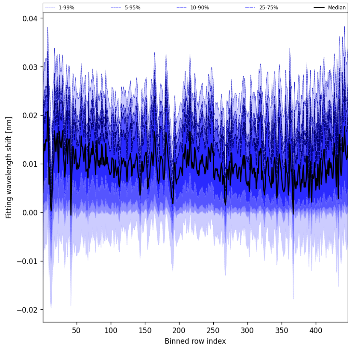
Figure 65: Along track statistics of “Fitting wavelength shift” for 2024-11-14 to 2024-11-15
