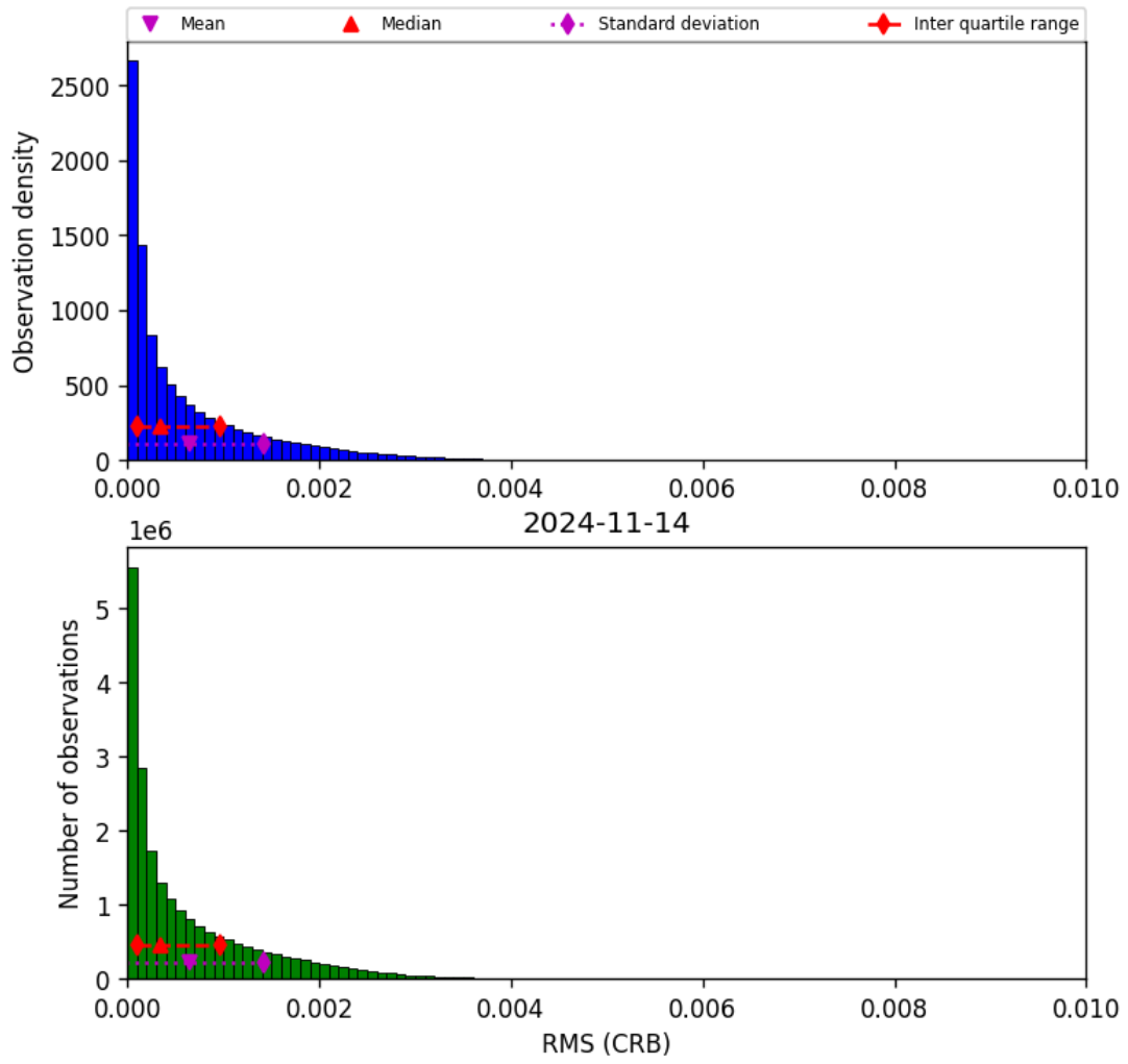
Figure 48: Histogram of "RMS (CRB)" for 2024-11-14 to 2024-11-15
