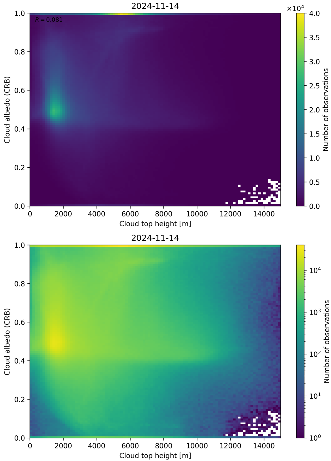
Figure 86: Scatter density plot of “Cloud top height” against “Cloud albedo (CRB)” for 2024-11-14 to 2024-11-15.
