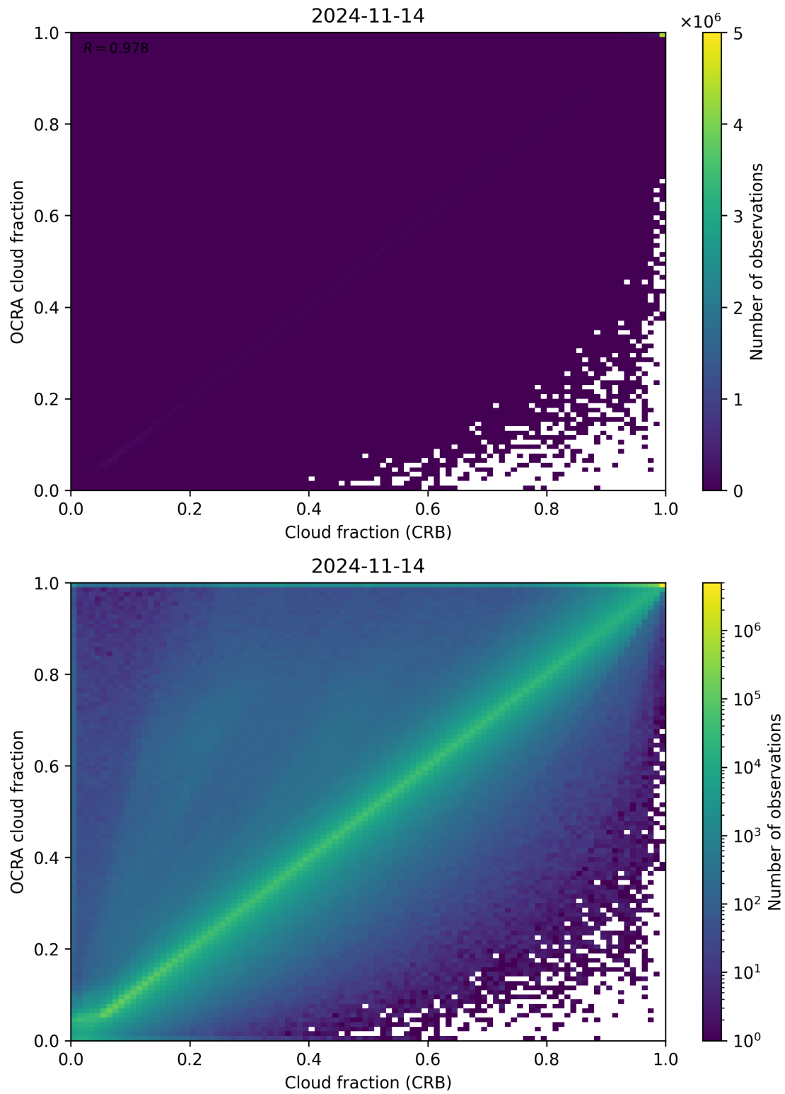
Figure 78: Scatter density plot of “Cloud fraction (CRB)” against “OCRA cloud fraction” for 2024-11-14 to 2024-11-15.
