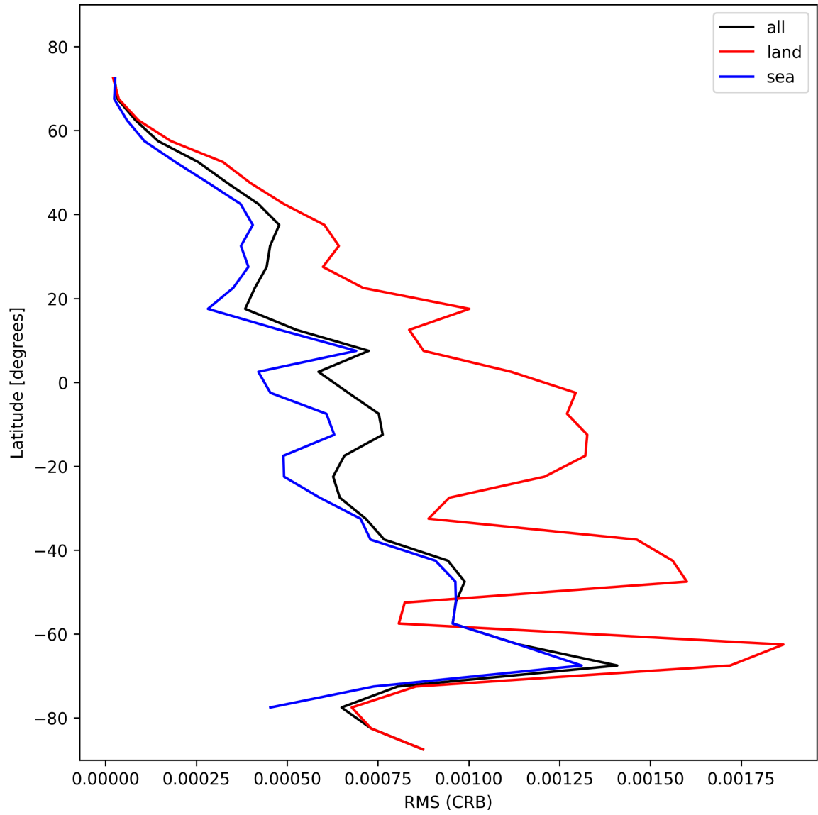
Figure 32: Zonal average of “RMS (CRB)” for 2024-11-14 to 2024-11-15.
