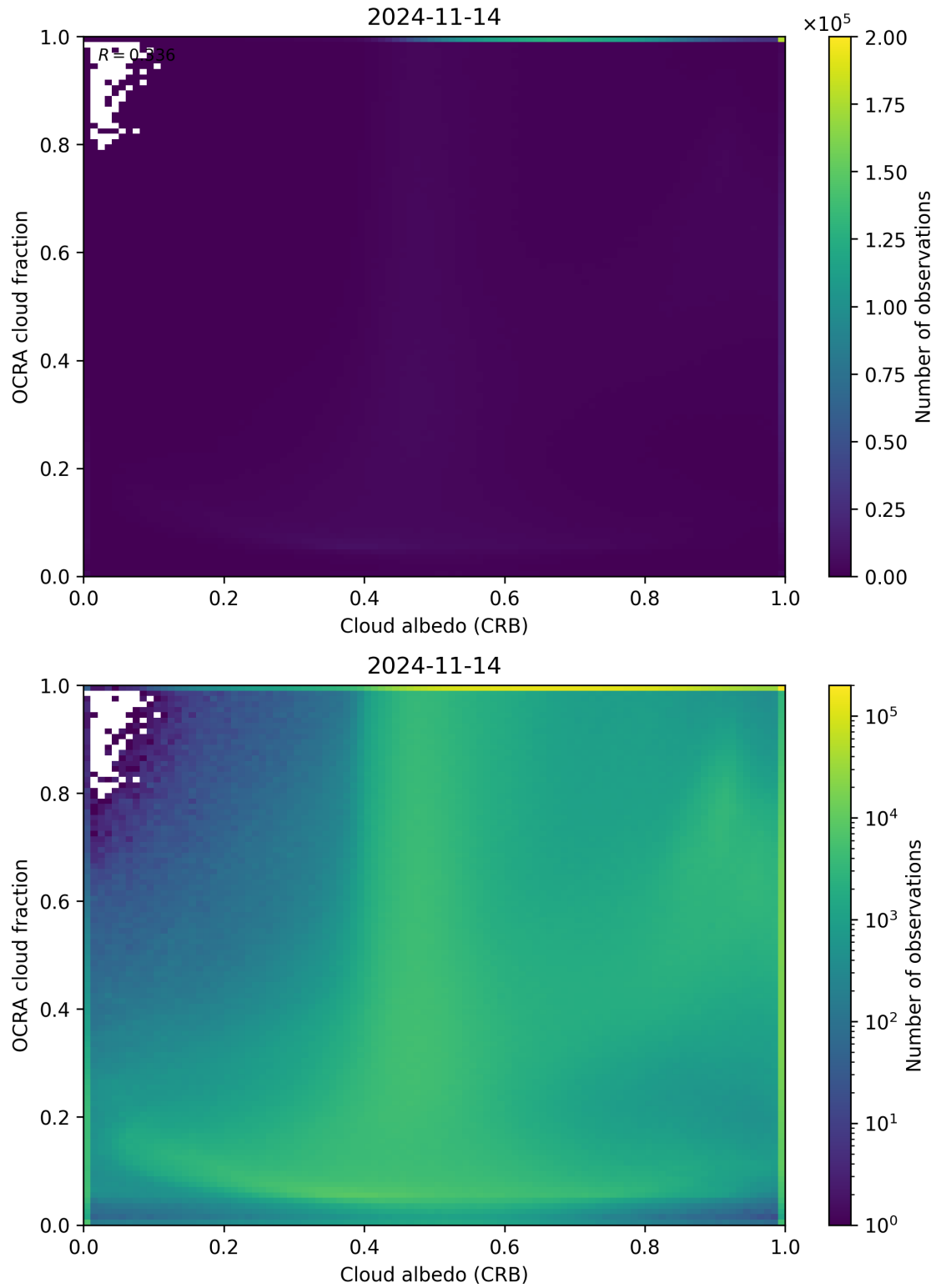
Figure 70: Scatter density plot of “Cloud albedo (CRB)” against “OCRA cloud fraction” for 2024-11-14 to 2024-11-15.
