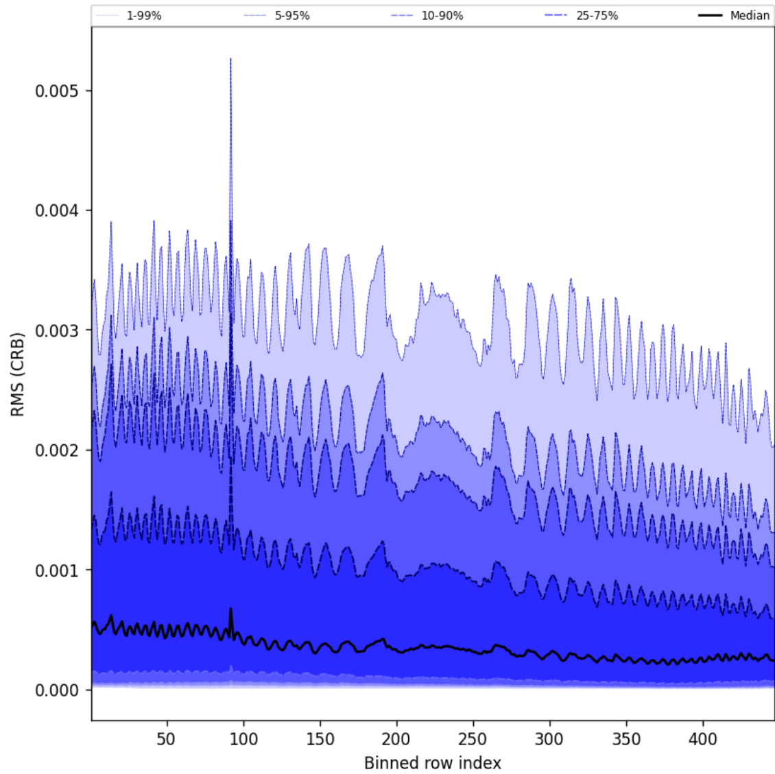
Figure 64: Along track statistics of “RMS (CRB)” for 2024-11-14 to 2024-11-15
