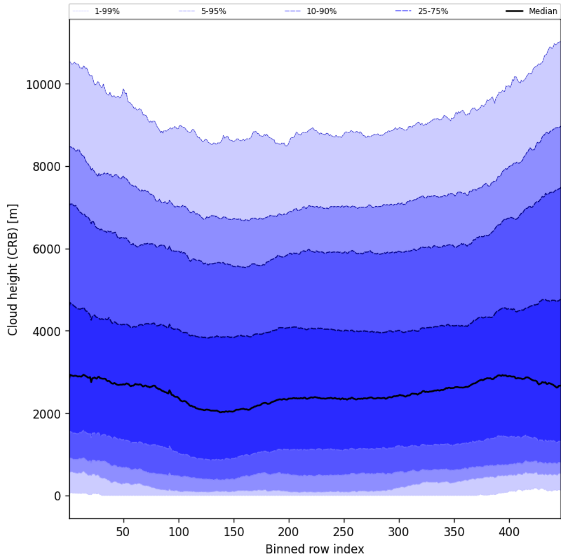
Figure 59: Along track statistics of “Cloud height (CRB)” for 2024-11-14 to 2024-11-15
