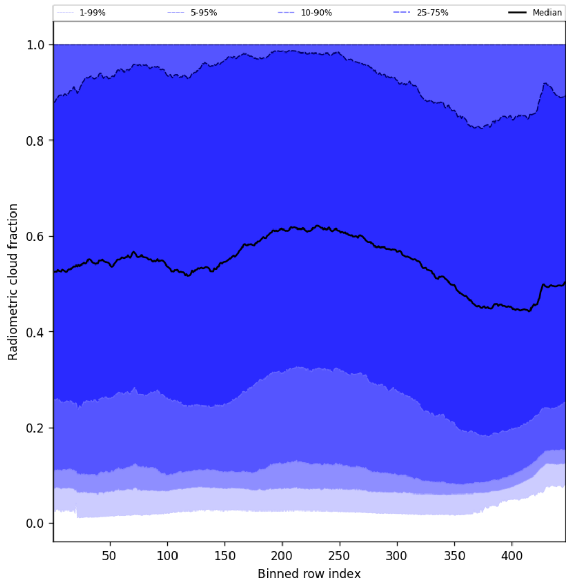
Figure 55: Along track statistics of “Radiometric cloud fraction” for 2024-11-14 to 2024-11-15
