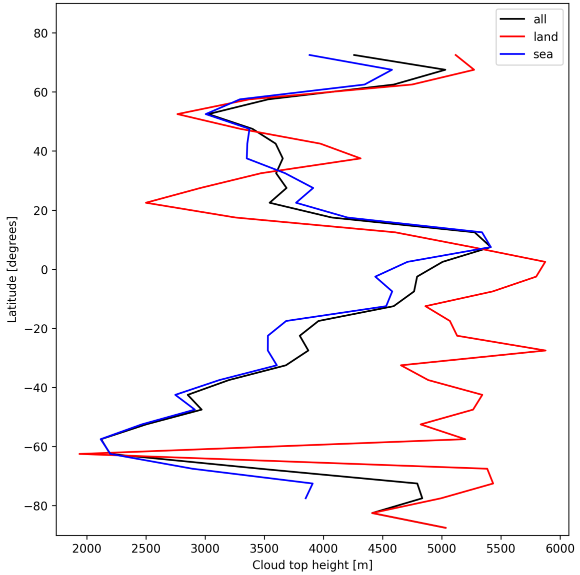
Figure 24: Zonal average of “Cloud top height” for 2024-11-14 to 2024-11-15.
