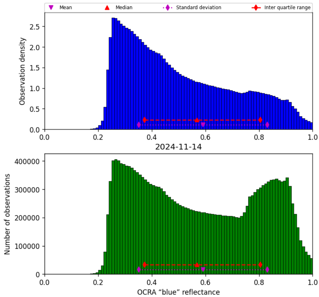
Figure 51: Histogram of “OCRA “blue” reflectance” for 2024-11-14 to 2024-11-15
