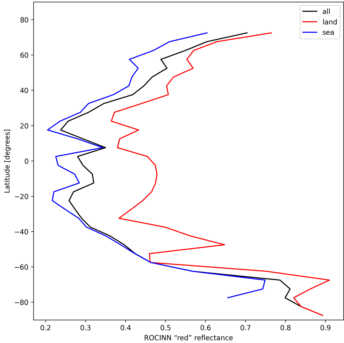
Figure 37: Zonal average of “ROCINN “red” reflectance” for 2024-11-14 to 2024-11-15.
