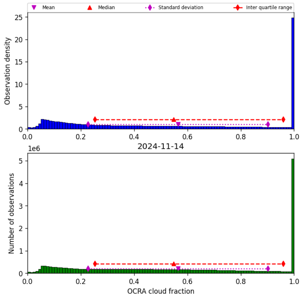
Figure 50: Histogram of “OCRA cloud fraction” for 2024-11-14 to 2024-11-15
