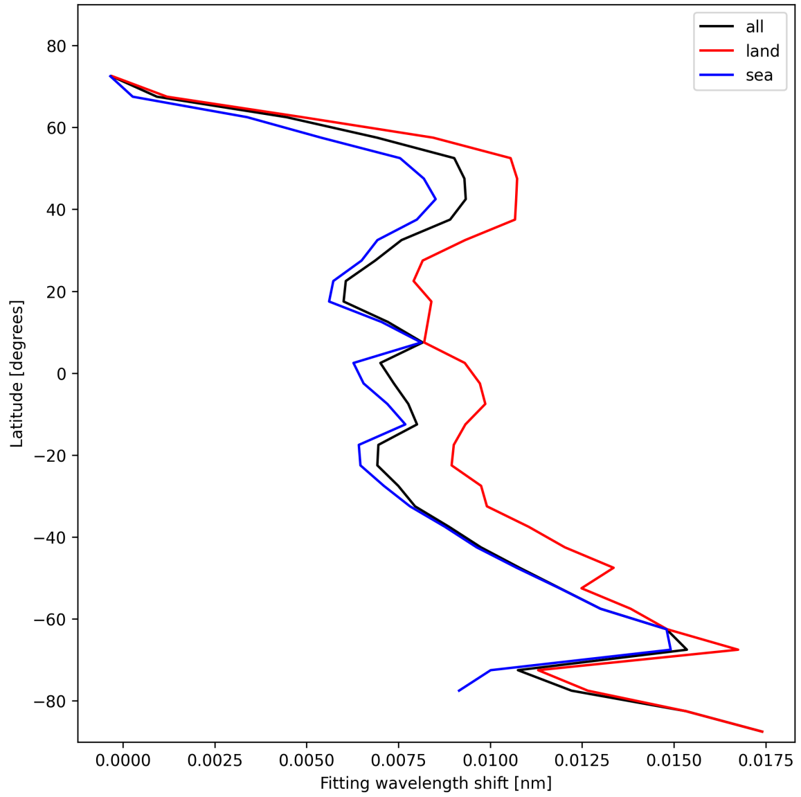
Figure 33: Zonal average of “Fitting wavelength shift” for 2024-11-14 to 2024-11-15.
