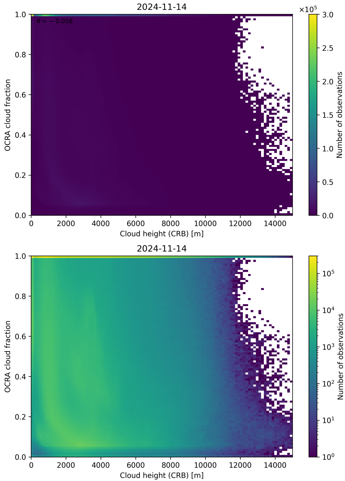
Figure 81: Scatter density plot of “Cloud height (CRB)” against “OCRA cloud fraction” for 2024-11-14 to 2024-11-15.
