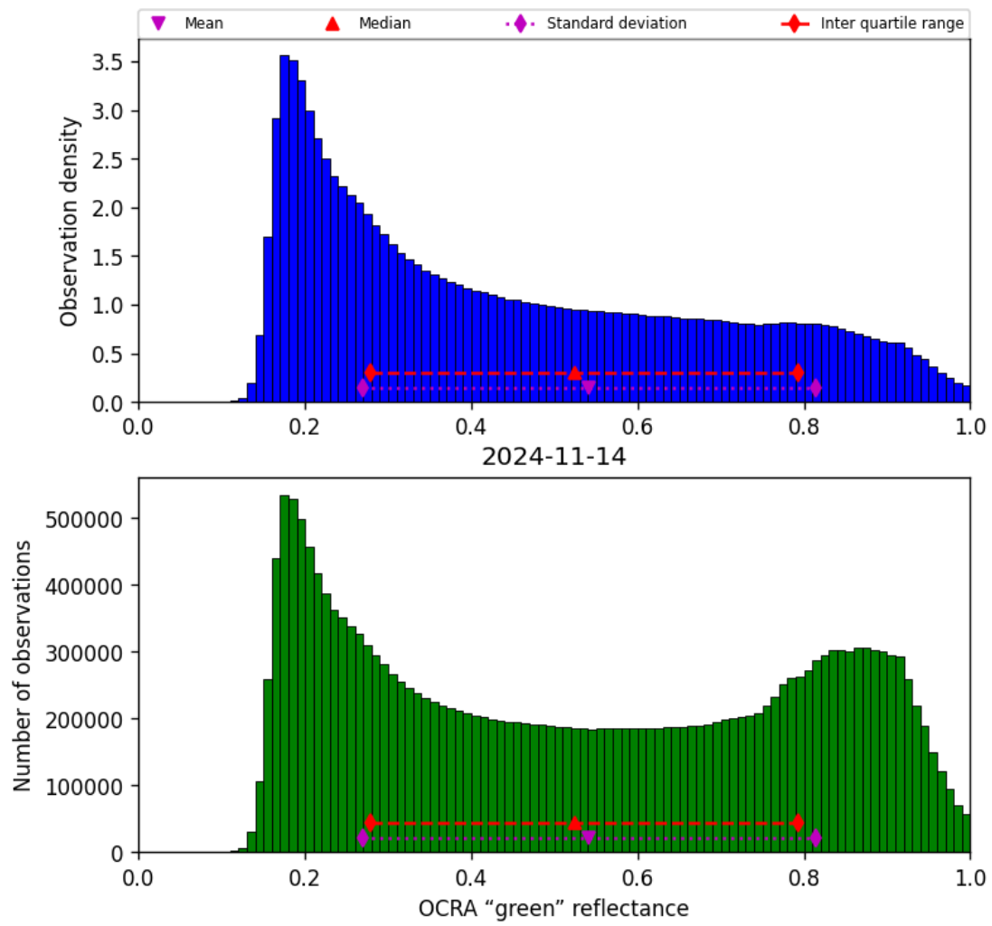
Figure 52: Histogram of “OCRA “green” reflectance” for 2024-11-14 to 2024-11-15
