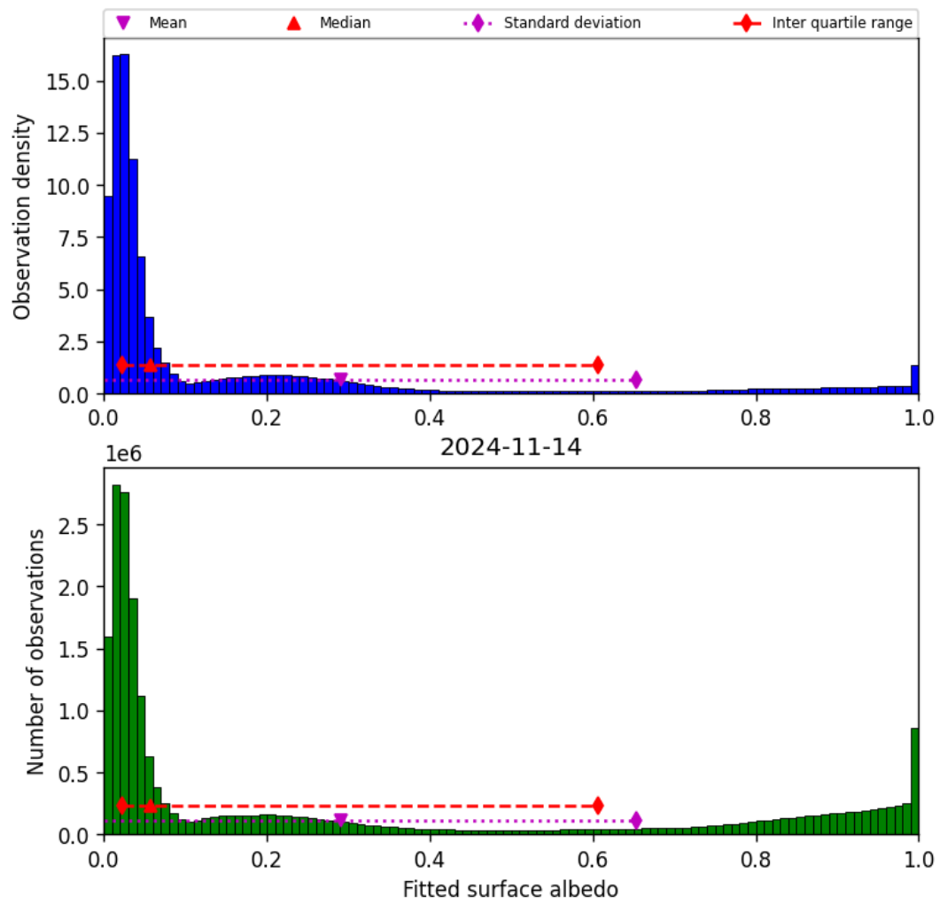
Figure 45: Histogram of “Fitted surface albedo” for 2024-11-14 to 2024-11-15
