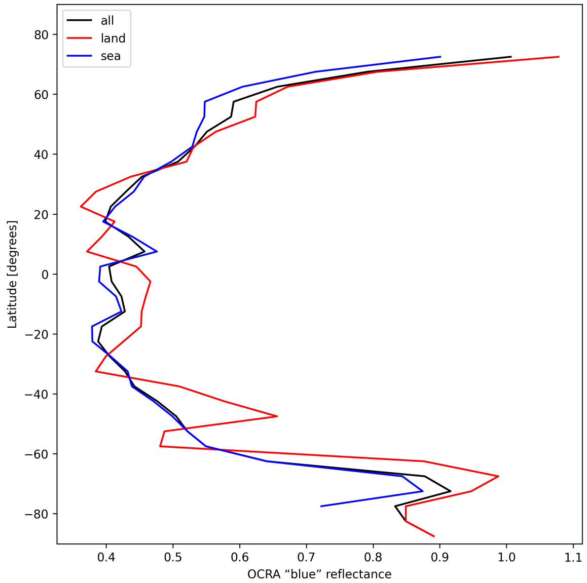
Figure 35: Zonal average of "OCRA "blue" reflectance" for 2024-11-14 to 2024-11-15.
