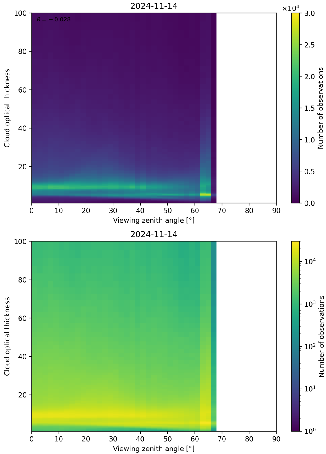
Figure 111: Scatter density plot of “Viewing zenith angle” against “Cloud optical thickness” for 2024-11-14 to 2024-11-15.
