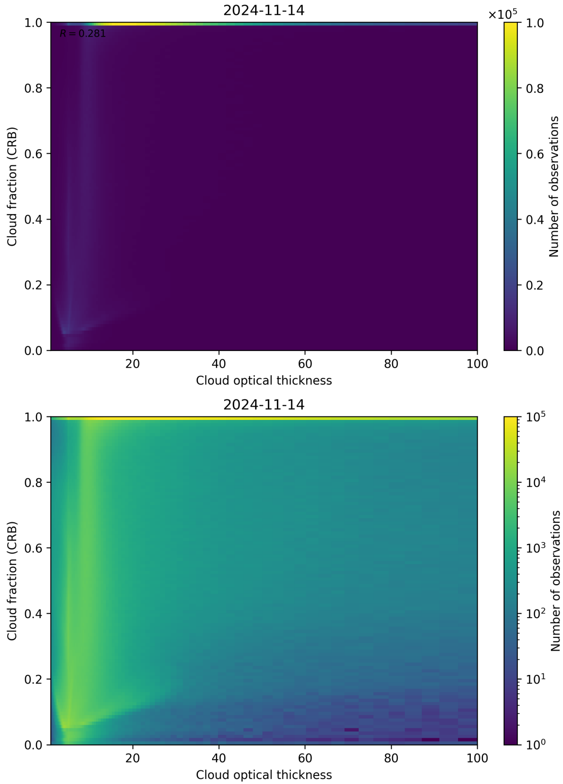
Figure 84: Scatter density plot of “Cloud optical thickness” against “Cloud fraction (CRB)” for 2024-11-14 to 2024-11-15.
