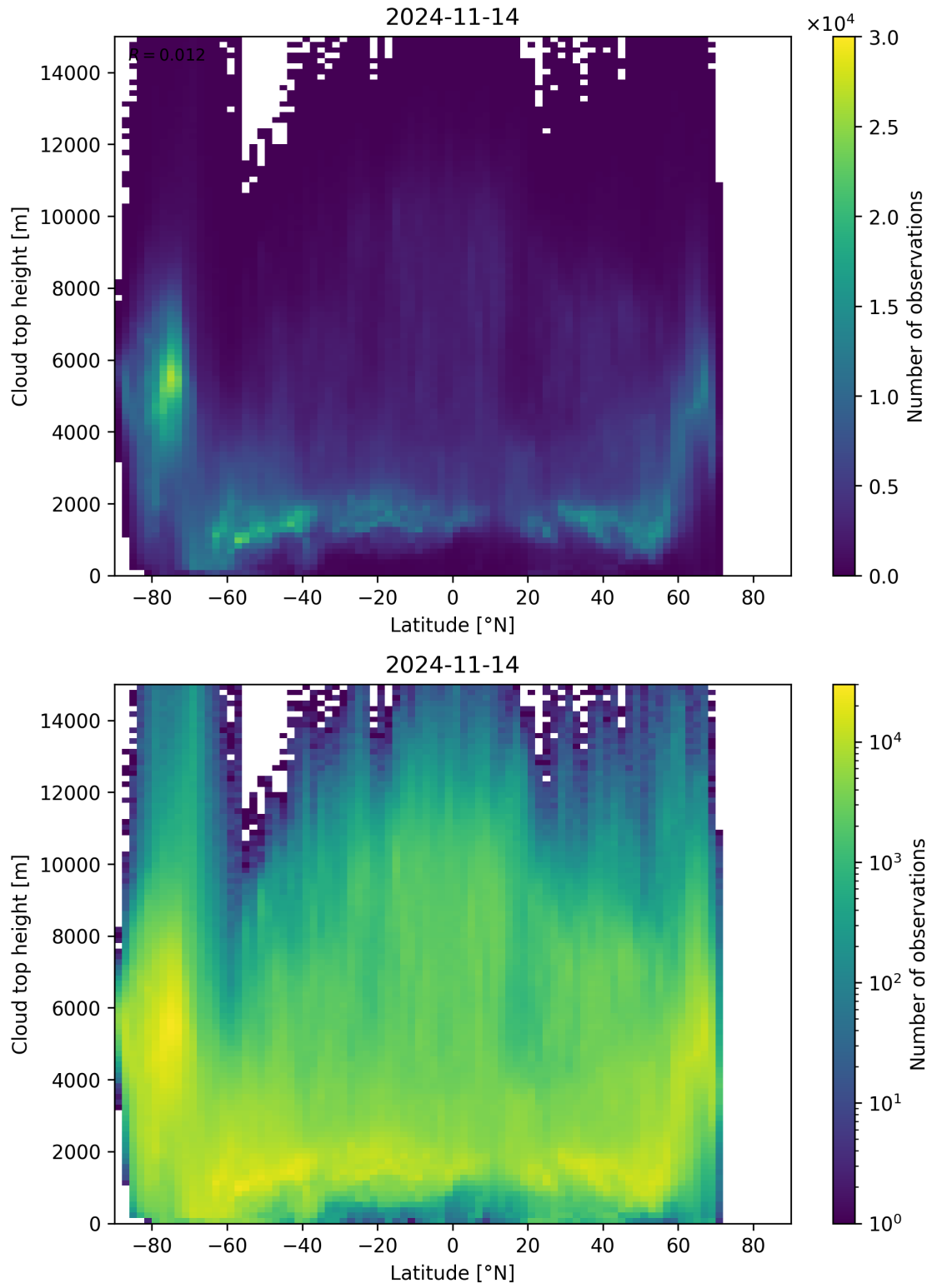
Figure 97: Scatter density plot of “Latitude” against “Cloud top height” for 2024-11-14 to 2024-11-15.
