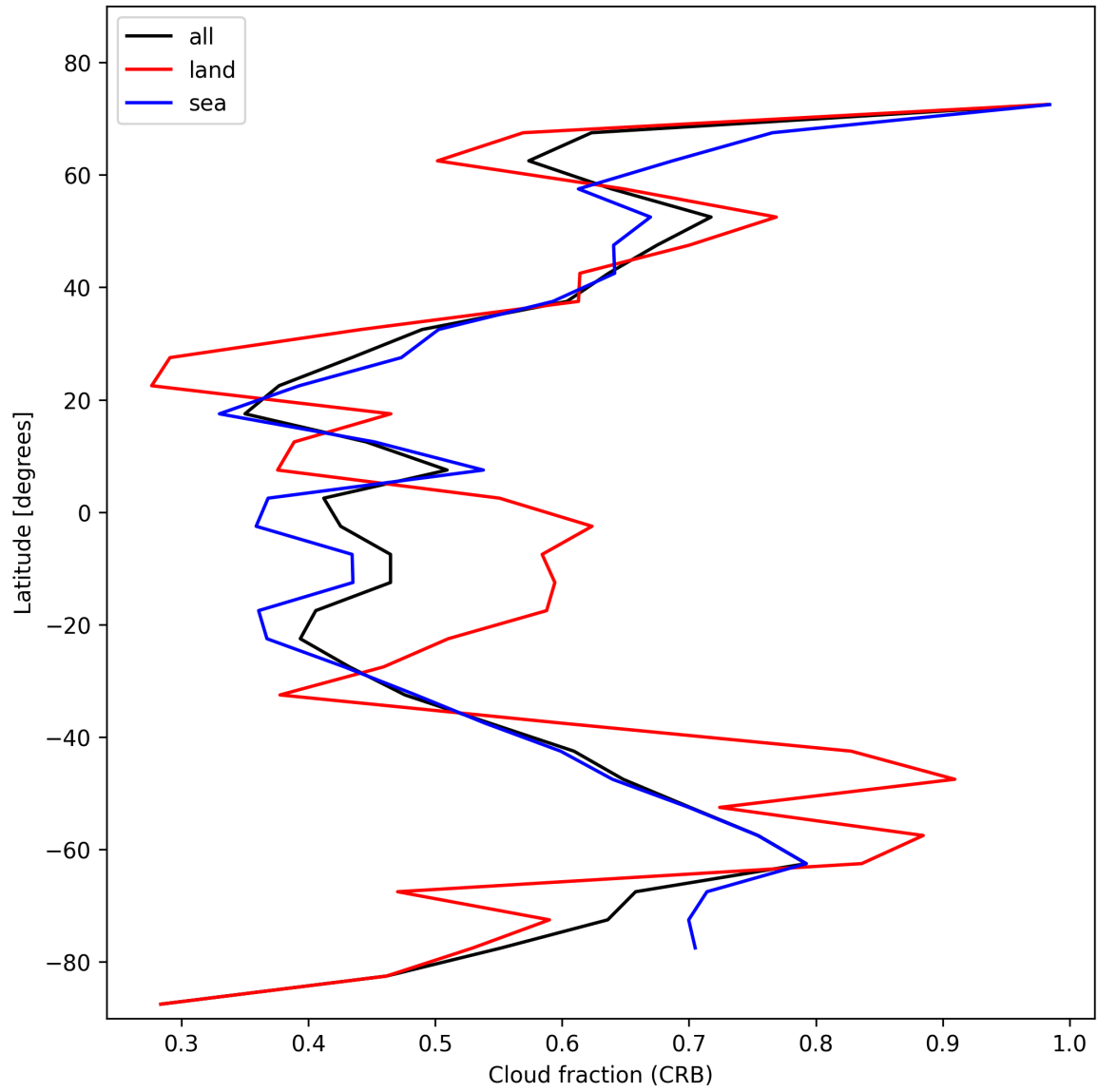
Figure 26: Zonal average of “Cloud fraction (CRB)” for 2024-11-14 to 2024-11-15.
