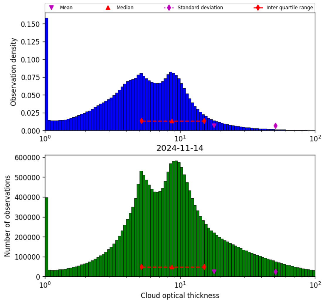
Figure 41: Histogram of “Cloud optical thickness” for 2024-11-14 to 2024-11-15
