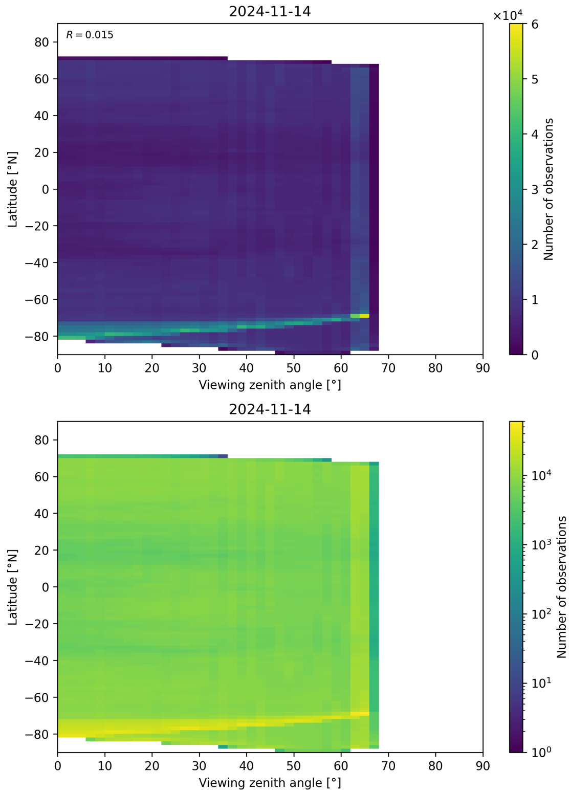
Figure 113: Scatter density plot of “Viewing zenith angle” against “Latitude” for 2024-11-14 to 2024-11-15.
