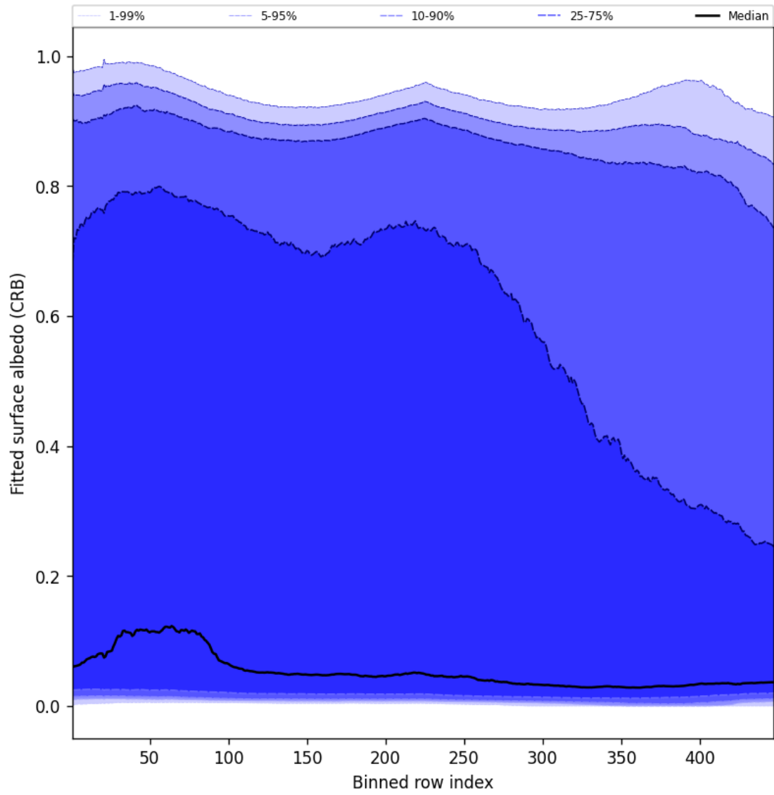
Figure 62: Along track statistics of “Fitted surface albedo (CRB)” for 2024-11-14 to 2024-11-15
