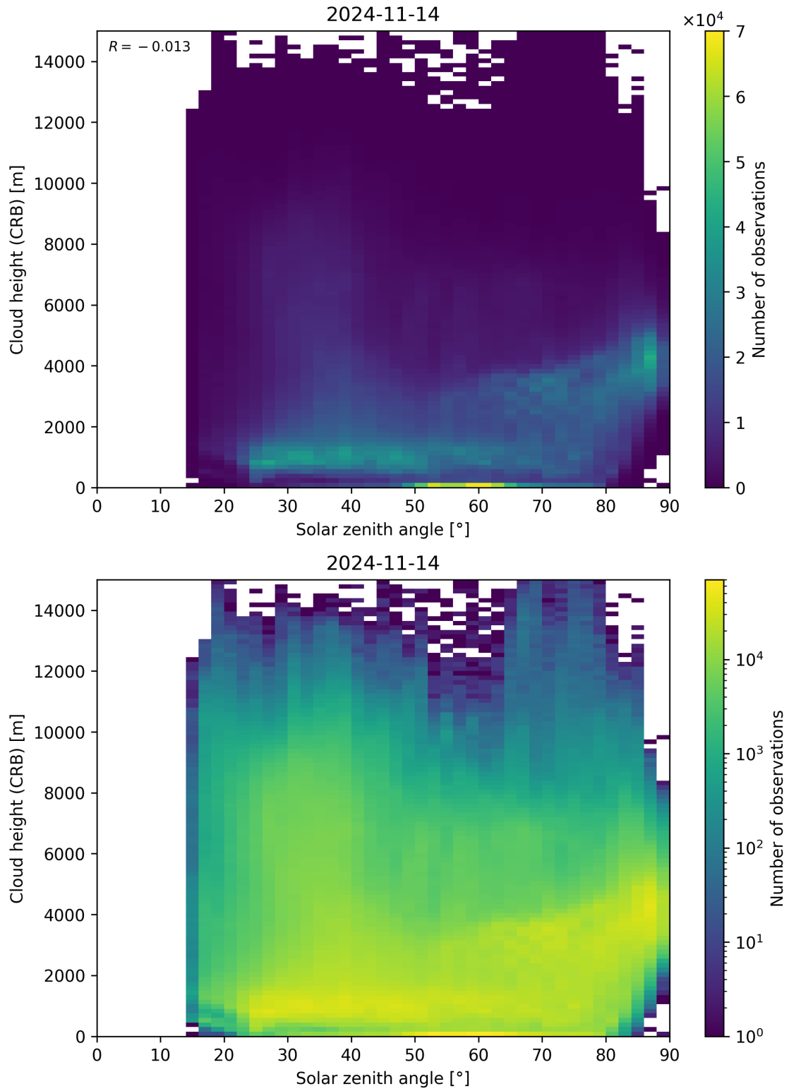
Figure 102: Scatter density plot of “Solar zenith angle” against “Cloud height (CRB)” for 2024-11-14 to 2024-11-15.
