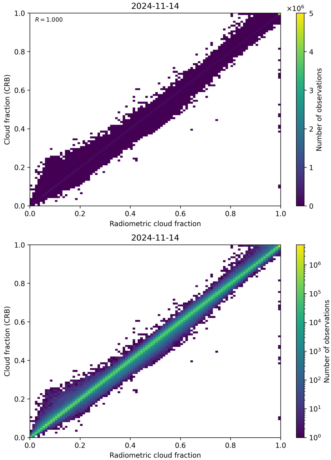
Figure 73: Scatter density plot of “Radiometric cloud fraction” against “Cloud fraction (CRB)” for 2024-11-14 to 2024-11-15.
