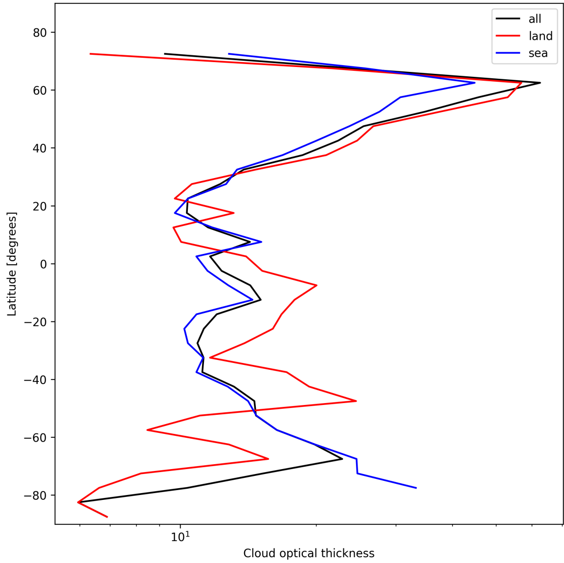
Figure 25: Zonal average of “Cloud optical thickness” for 2024-11-14 to 2024-11-15.
