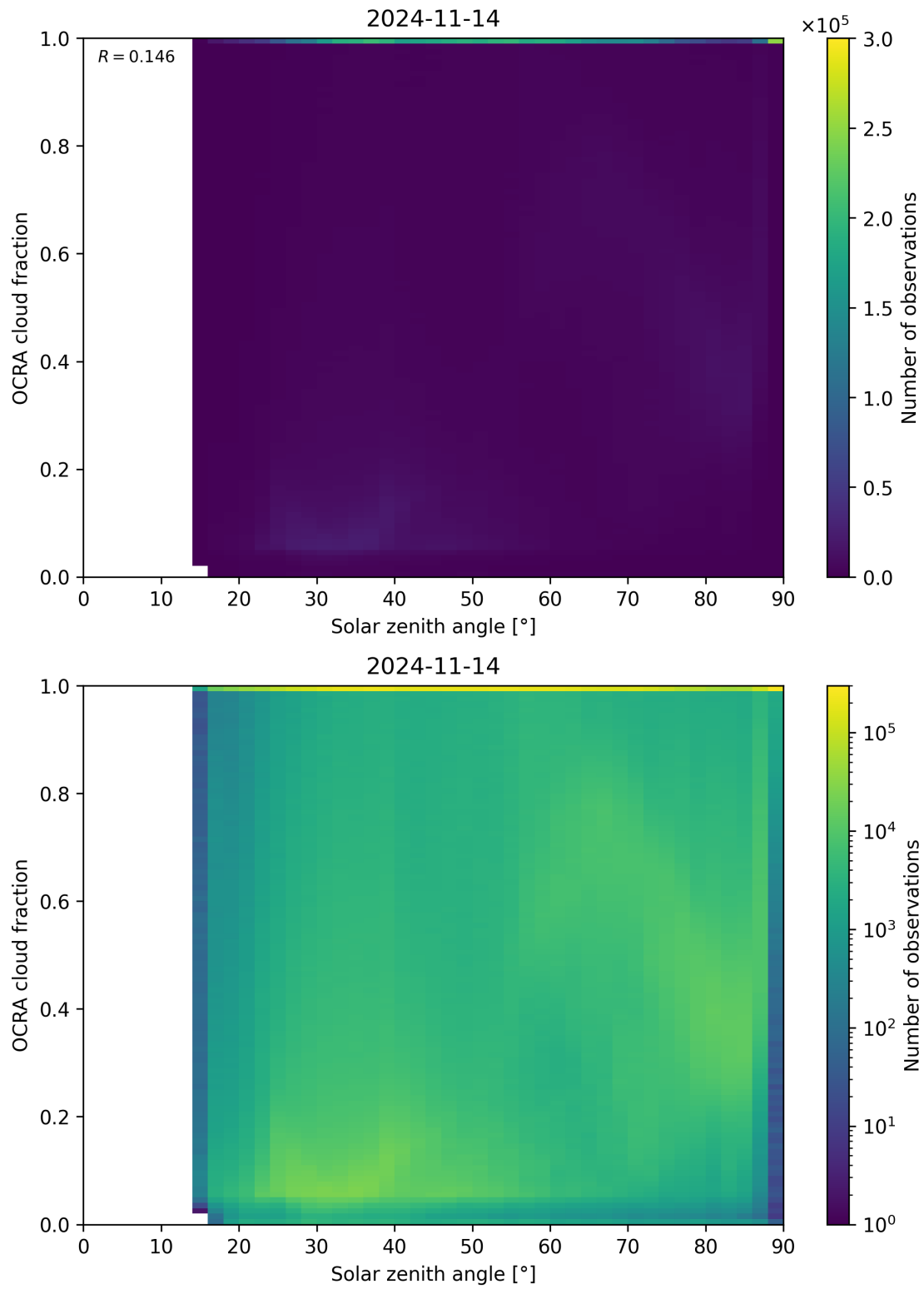
Figure 100: Scatter density plot of “Solar zenith angle” against “OCRA cloud fraction” for 2024-11-14 to 2024-11-15.
