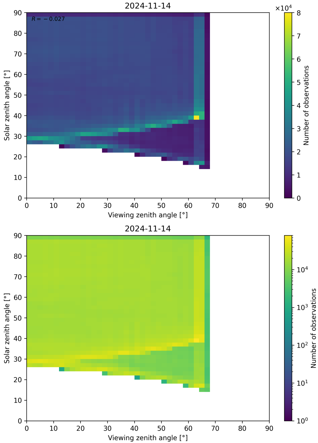
Figure 114: Scatter density plot of “Viewing zenith angle” against “Solar zenith angle” for 2024-11-14 to 2024-11-15.
