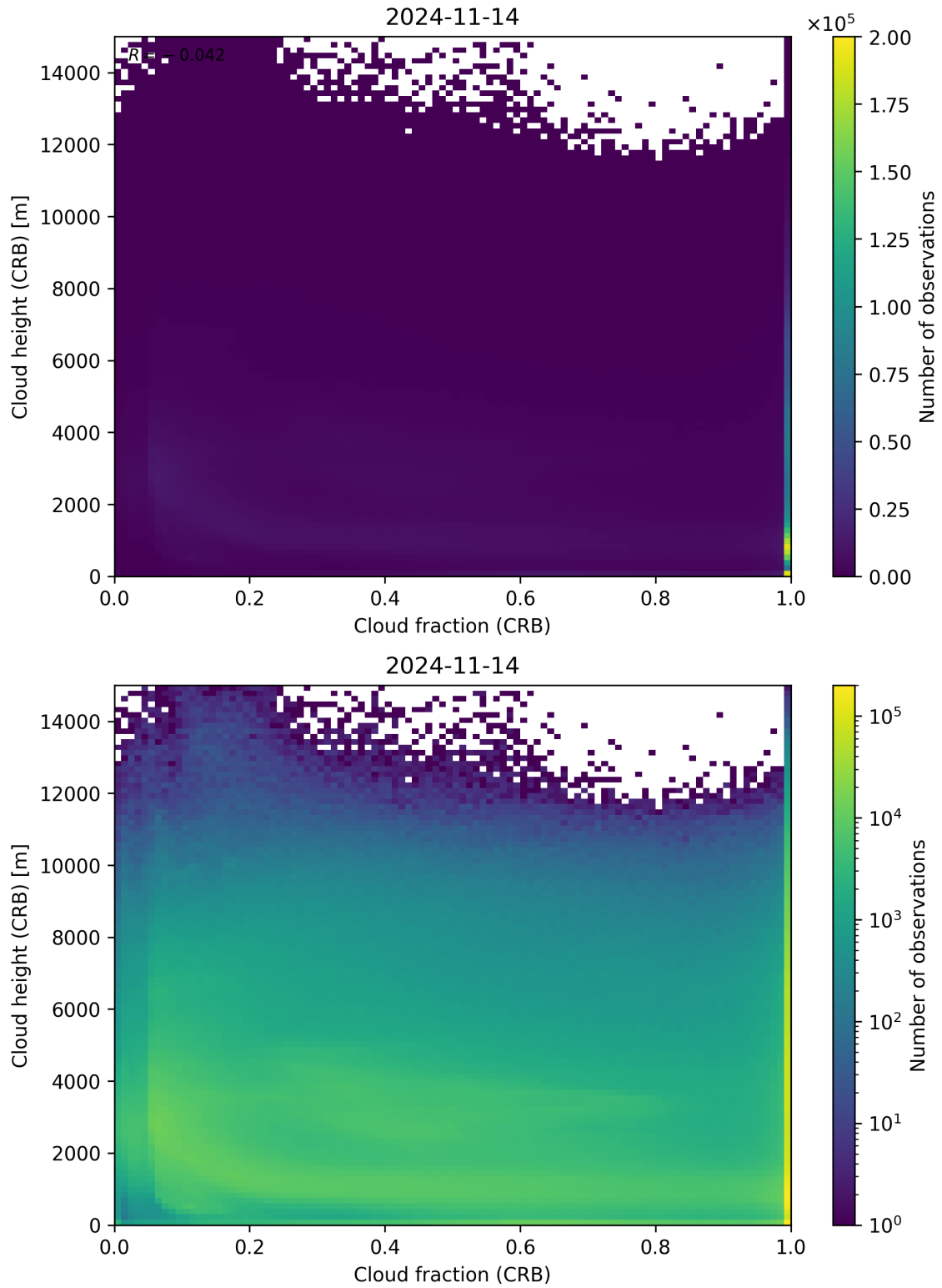
Figure 79: Scatter density plot of “Cloud fraction (CRB)” against “Cloud height (CRB)” for 2024-11-14 to 2024-11-15.
