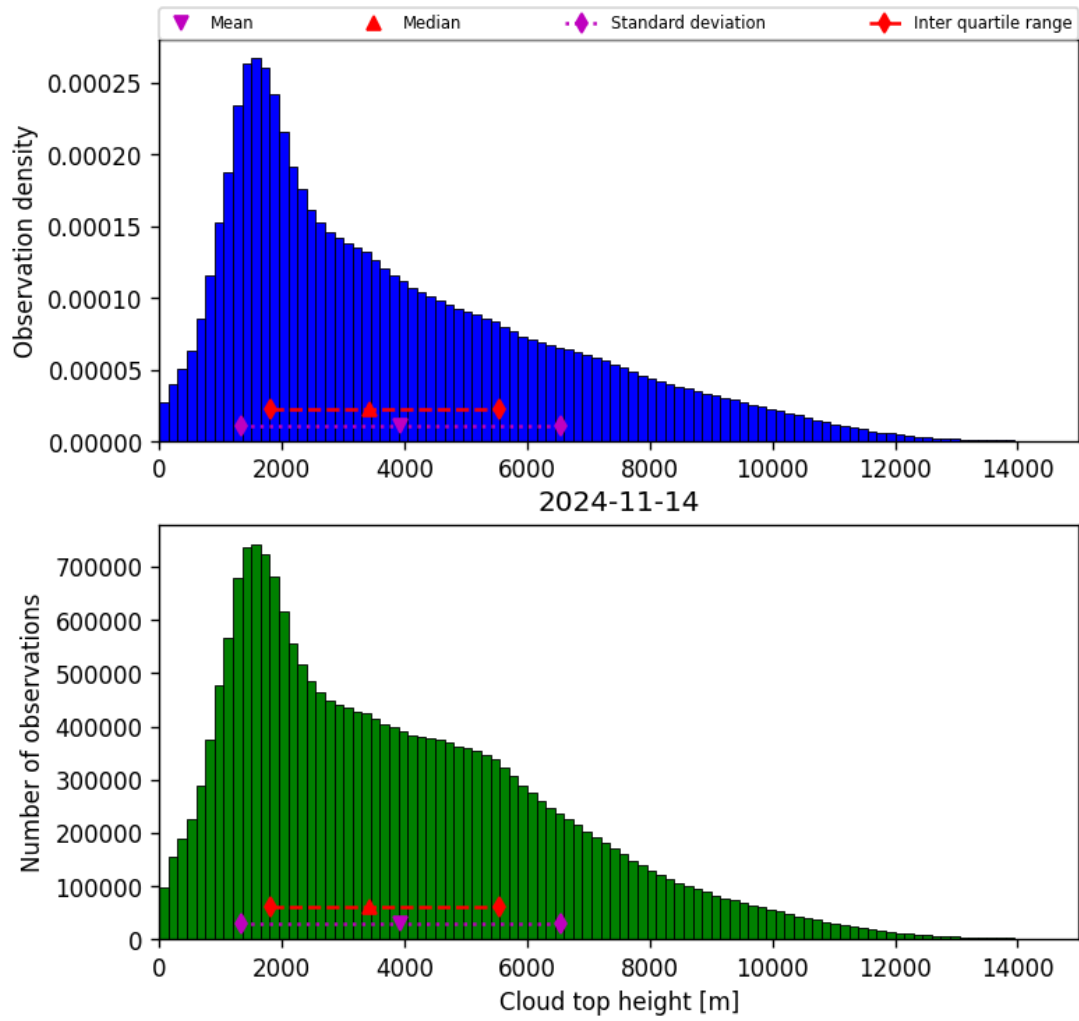
Figure 40: Histogram of “Cloud top height” for 2024-11-14 to 2024-11-15
