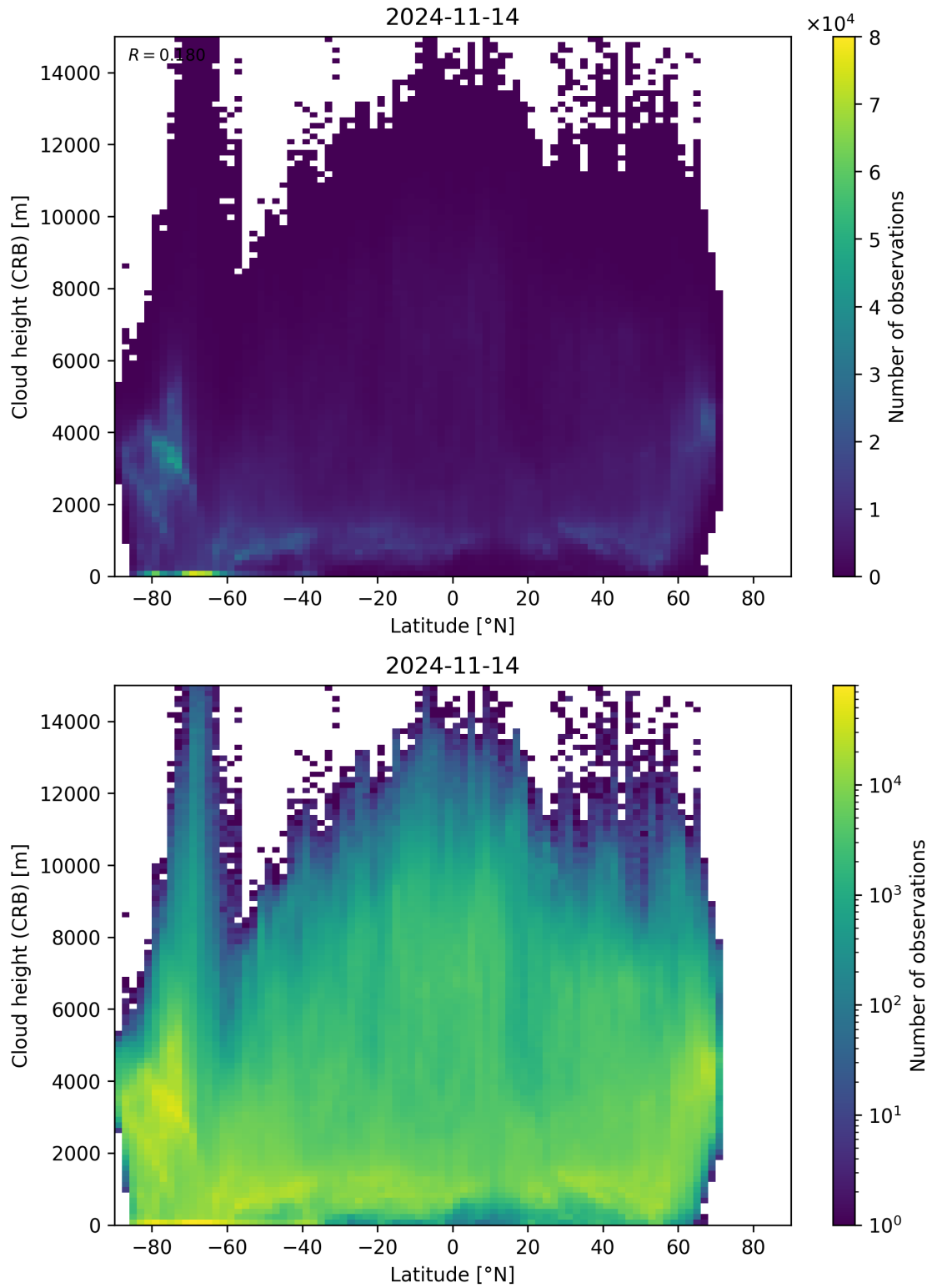
Figure 95: Scatter density plot of “Latitude” against “Cloud height (CRB)” for 2024-11-14 to 2024-11-15.
