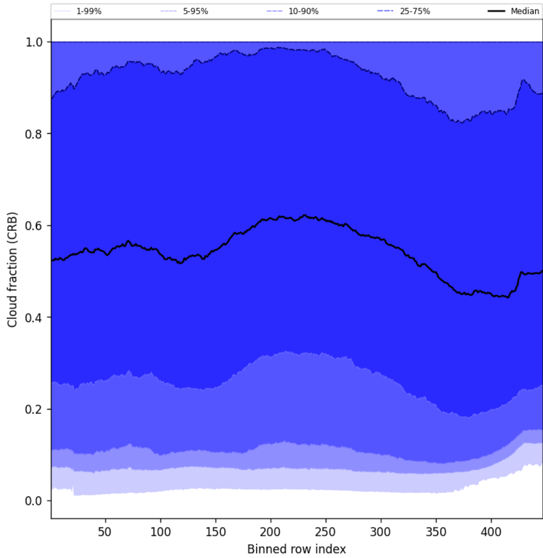
Figure 58: Along track statistics of “Cloud fraction (CRB)” for 2024-11-14 to 2024-11-15
