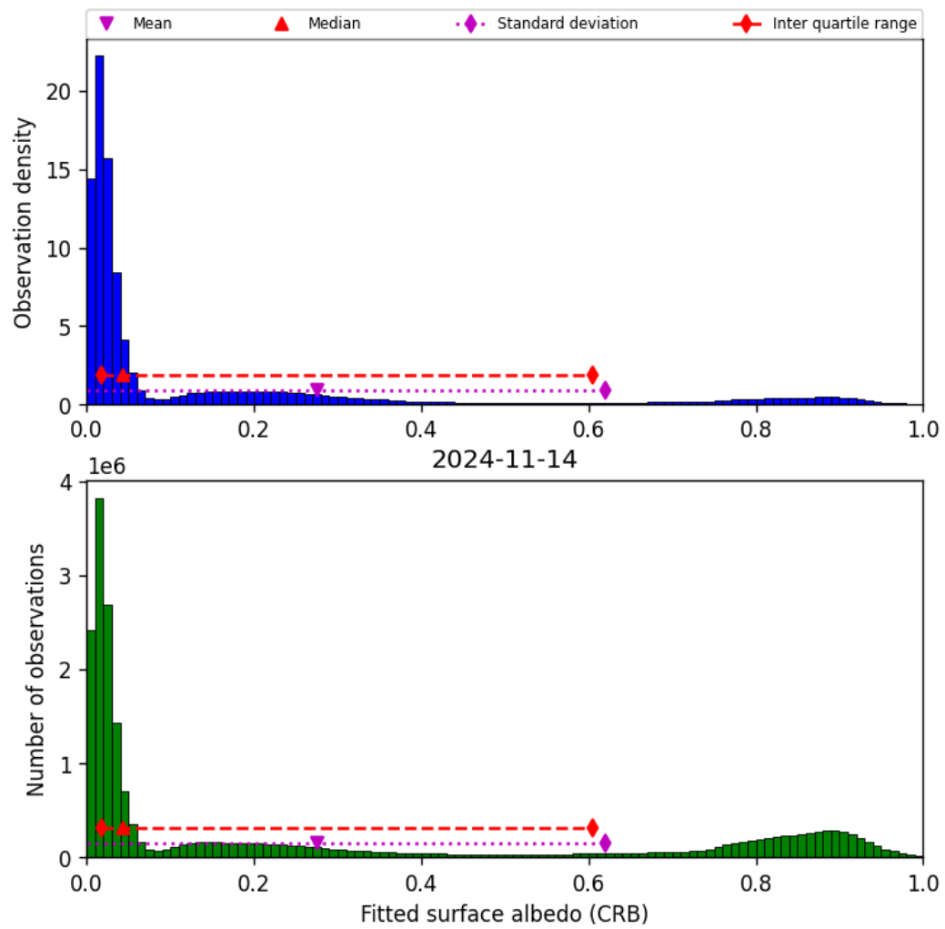
Figure 46: Histogram of “Fitted surface albedo (CRB)” for 2024-11-14 to 2024-11-15
