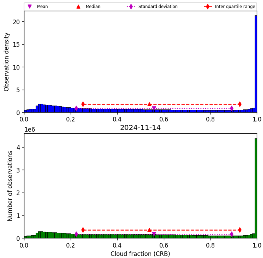
Figure 42: Histogram of “Cloud fraction (CRB)” for 2024-11-14 to 2024-11-15
