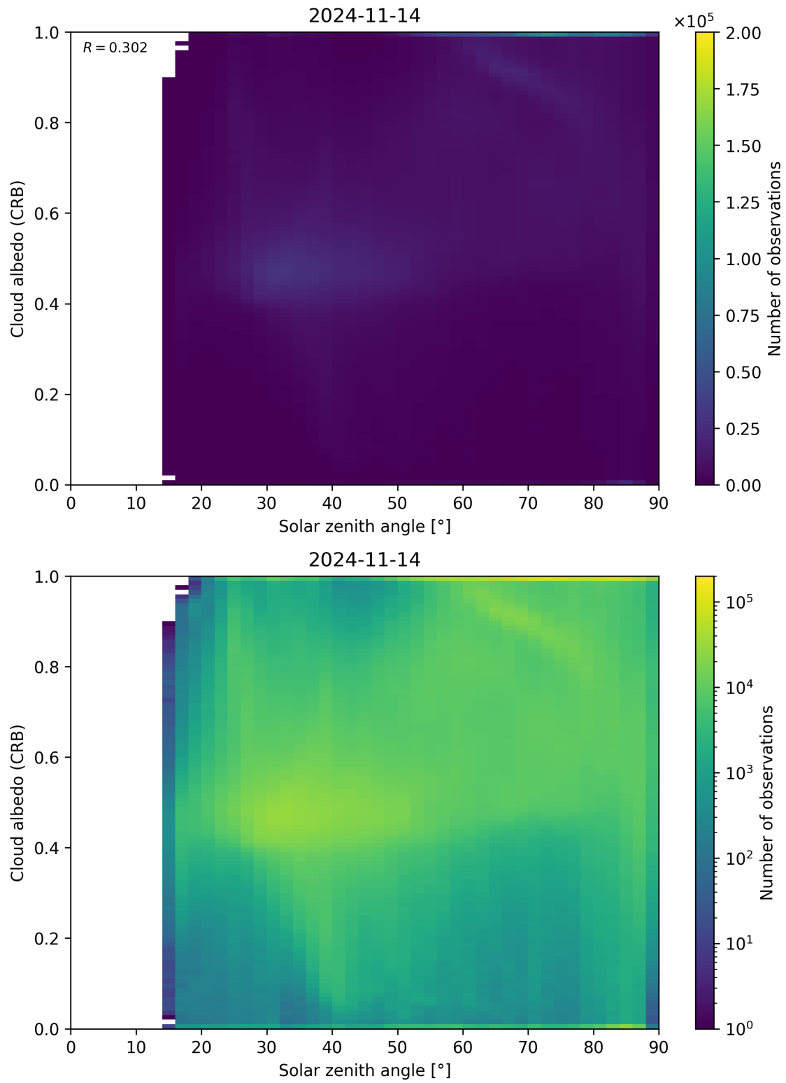
Figure 98: Scatter density plot of “Solar zenith angle” against “Cloud albedo (CRB)” for 2024-11-14 to 2024-11-15.
