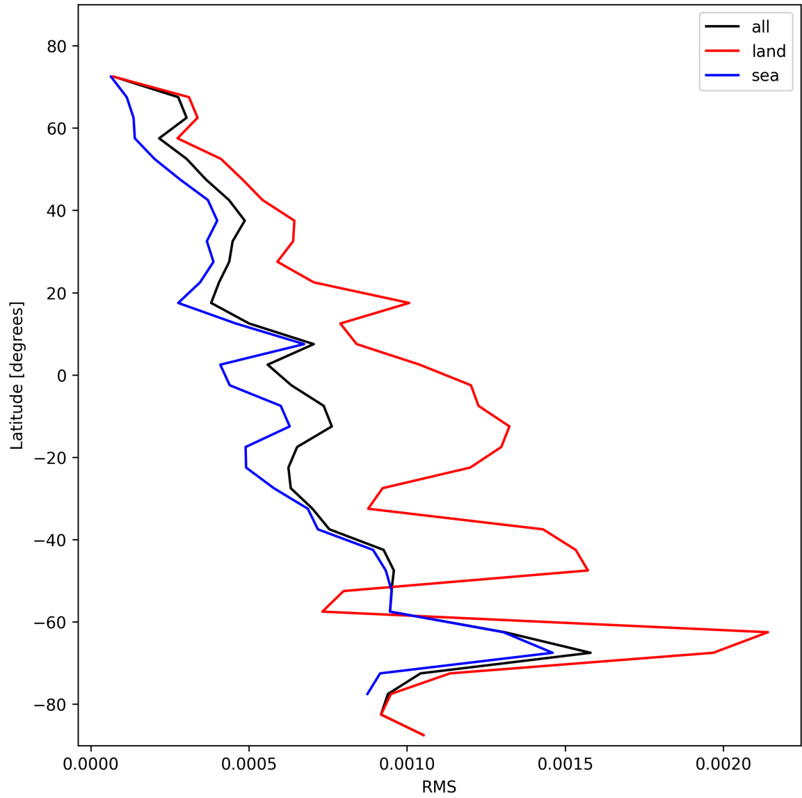
Figure 31: Zonal average of “RMS” for 2024-11-14 to 2024-11-15.
