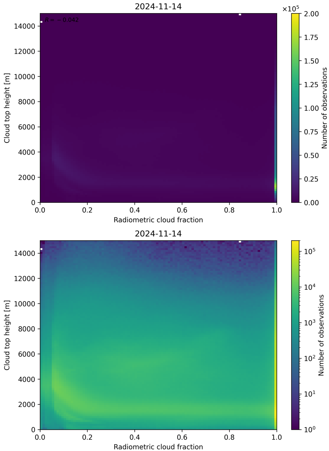
Figure 76: Scatter density plot of “Radiometric cloud fraction” against “Cloud top height” for 2024-11-14 to 2024-11-15.
