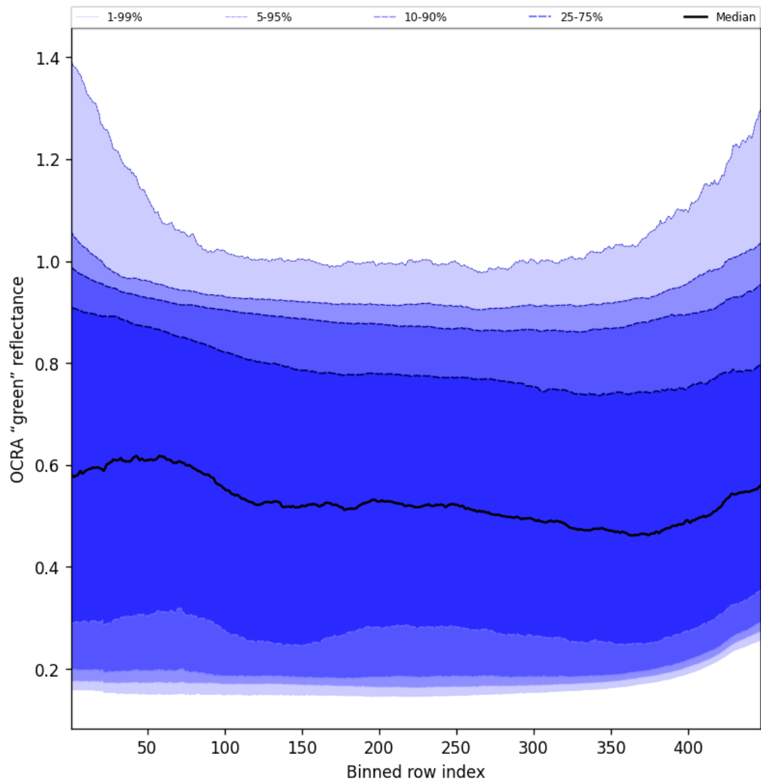
Figure 68: Along track statistics of “OCRA “green” reflectance” for 2024-11-14 to 2024-11-15
