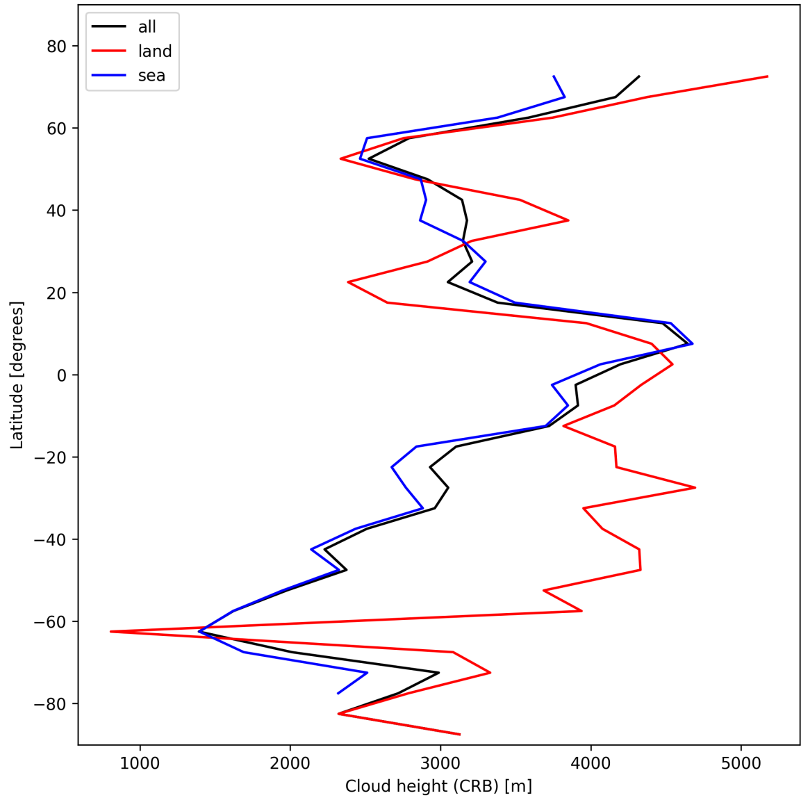
Figure 27: Zonal average of “Cloud height (CRB)” for 2024-11-14 to 2024-11-15.
