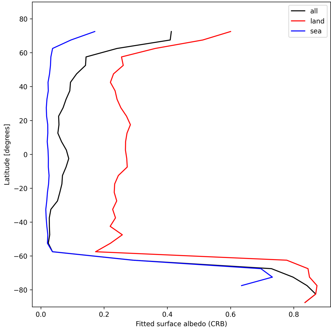
Figure 30: Zonal average of “Fitted surface albedo (CRB)” for 2024-11-14 to 2024-11-15.
