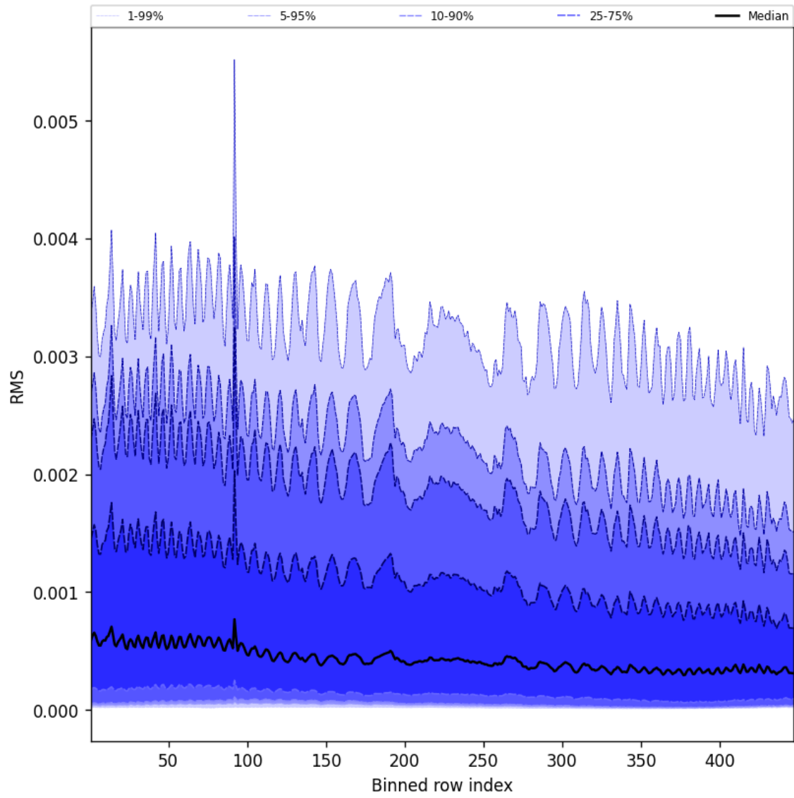
Figure 63: Along track statistics of “RMS” for 2024-11-14 to 2024-11-15
