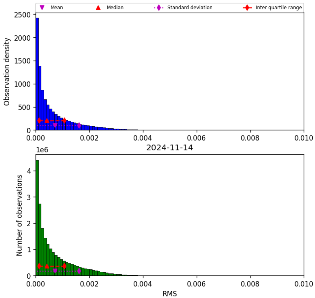
Figure 47: Histogram of “RMS” for 2024-11-14 to 2024-11-15
