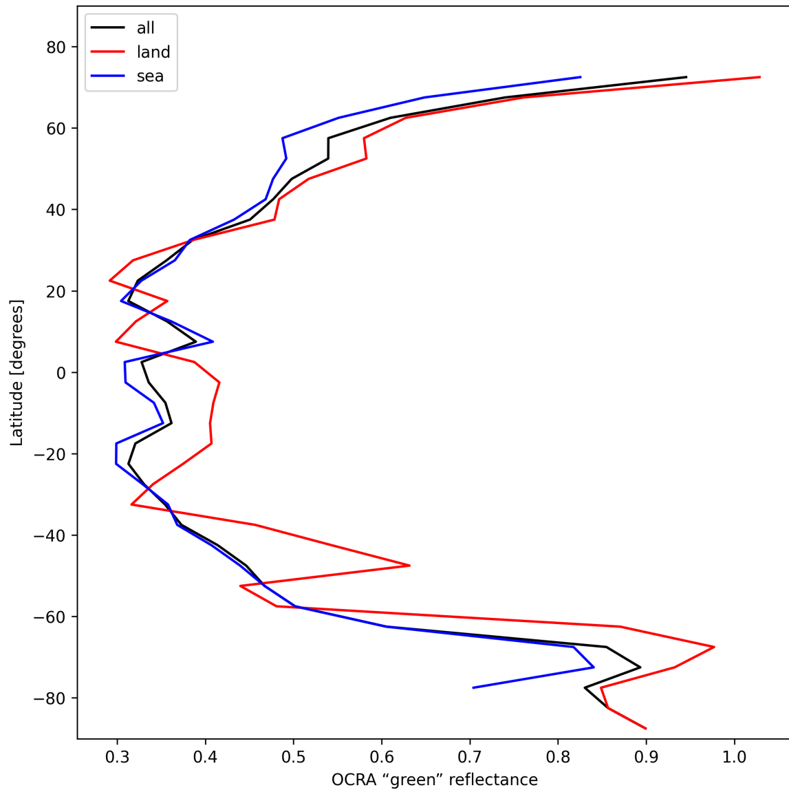
Figure 36: Zonal average of “OCRA “green” reflectance” for 2024-11-14 to 2024-11-15.
