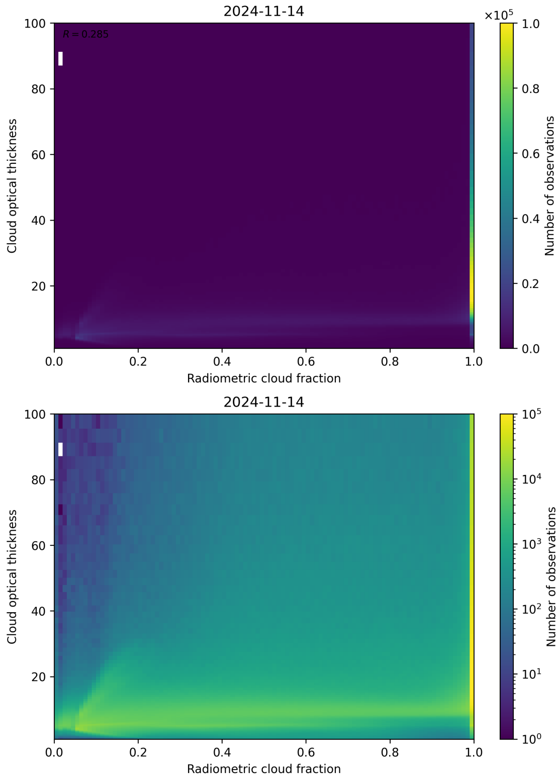
Figure 75: Scatter density plot of “Radiometric cloud fraction” against “Cloud optical thickness” for 2024-11-14 to 2024-11-15.
