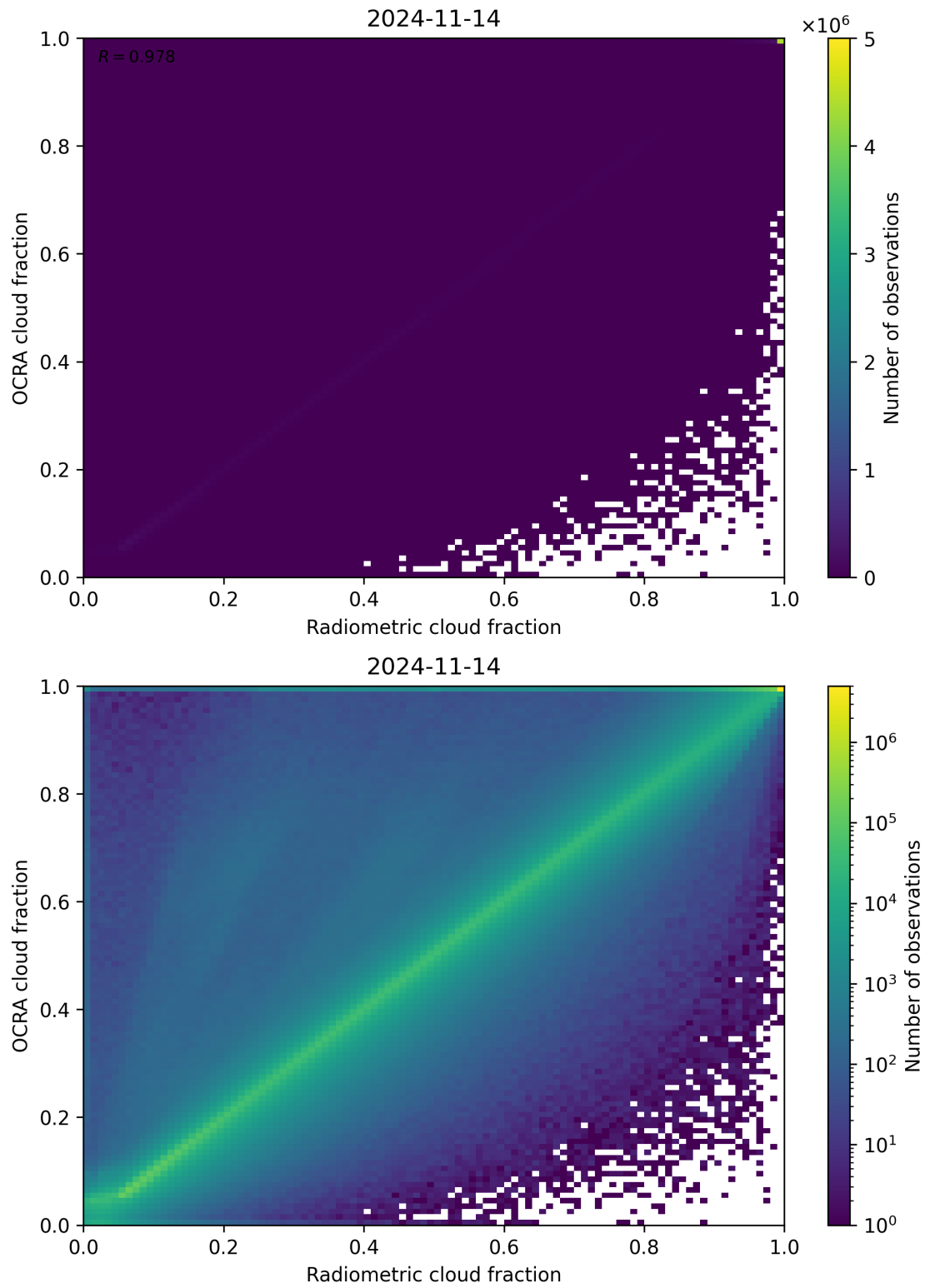
Figure 72: Scatter density plot of “Radiometric cloud fraction” against “OCRA cloud fraction” for 2024-11-14 to 2024-11-15.
