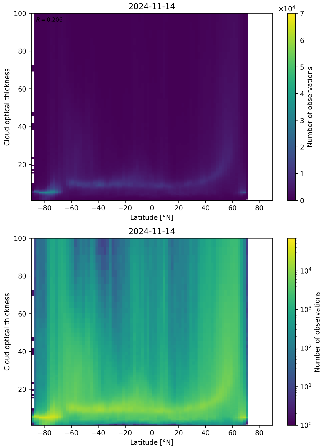
Figure 96: Scatter density plot of “Latitude” against “Cloud optical thickness” for 2024-11-14 to 2024-11-15.
