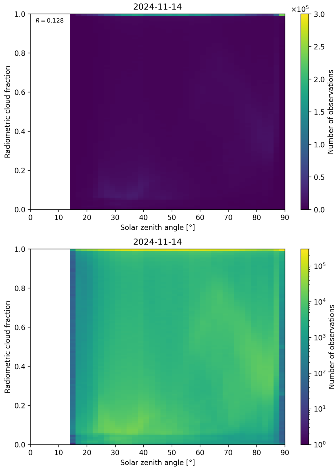
Figure 99: Scatter density plot of “Solar zenith angle” against “Radiometric cloud fraction” for 2024-11-14 to 2024-11-15.
