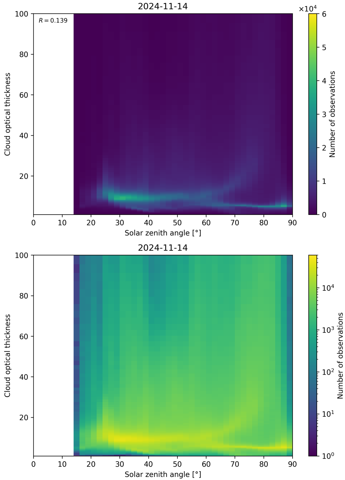
Figure 103: Scatter density plot of “Solar zenith angle” against “Cloud optical thickness” for 2024-11-14 to 2024-11-15.
