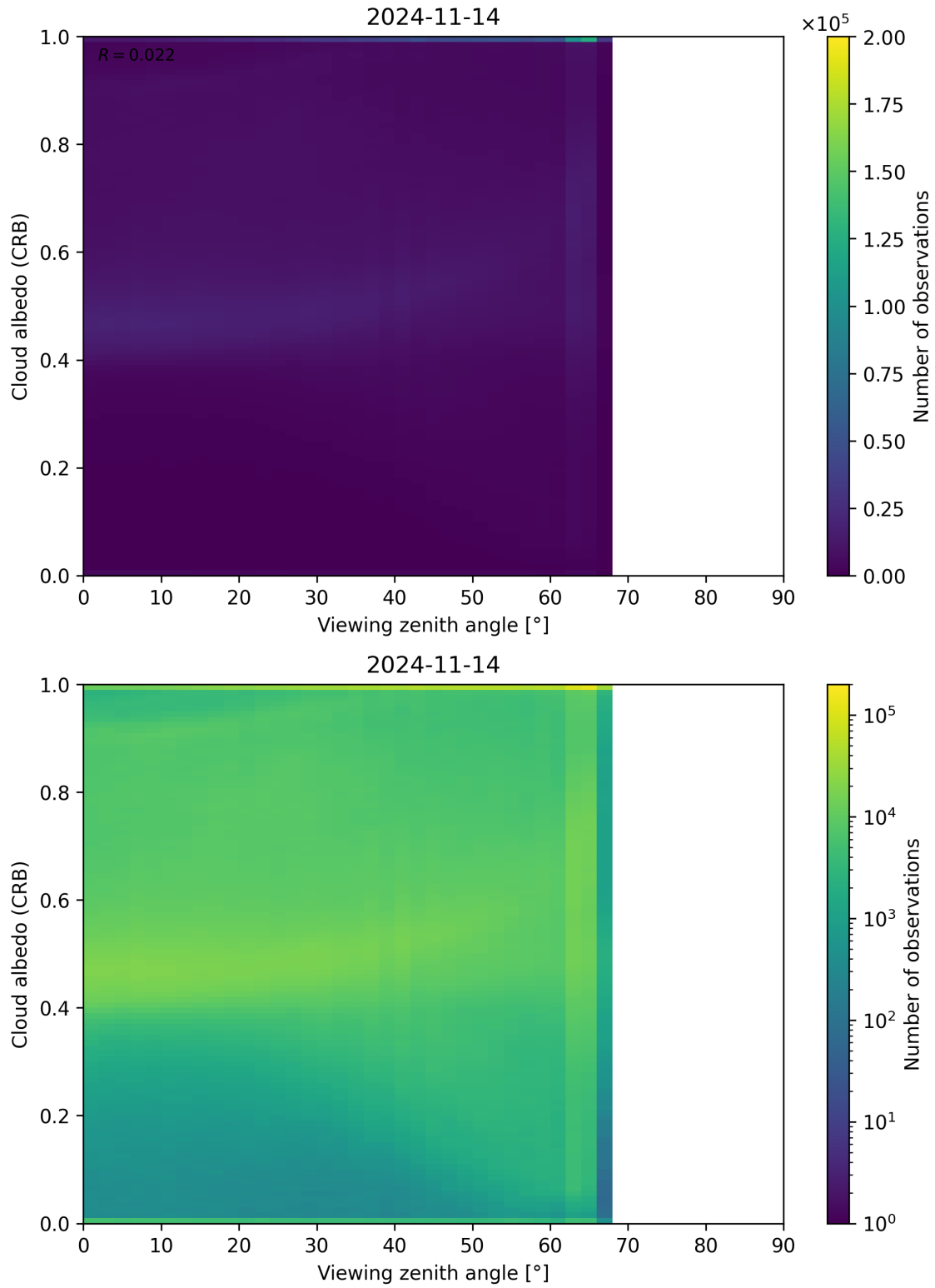
Figure 106: Scatter density plot of “Viewing zenith angle” against “Cloud albedo (CRB)” for 2024-11-14 to 2024-11-15.
