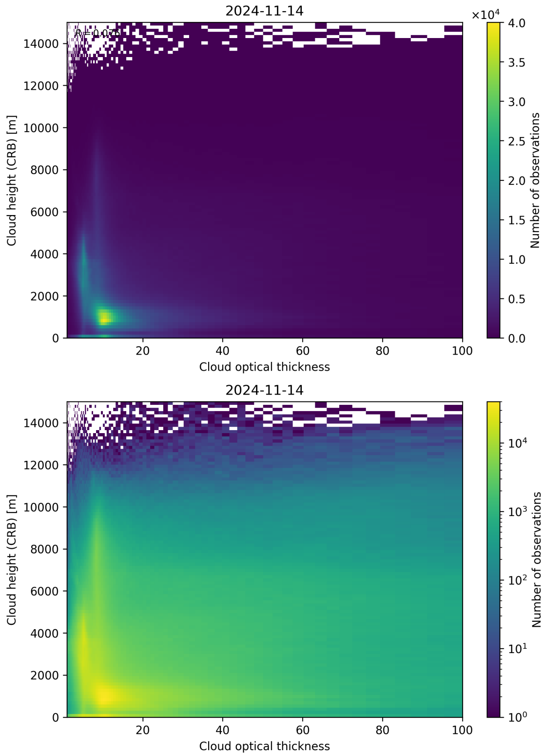
Figure 85: Scatter density plot of “Cloud optical thickness” against “Cloud height (CRB)” for 2024-11-14 to 2024-11-15.
