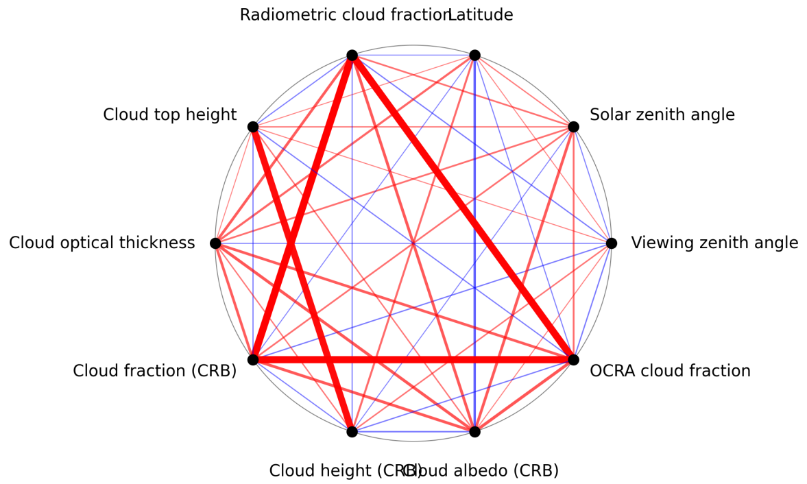
Figure 1: Map of correlation graph for 2024-11-14 to 2024-11-15.
