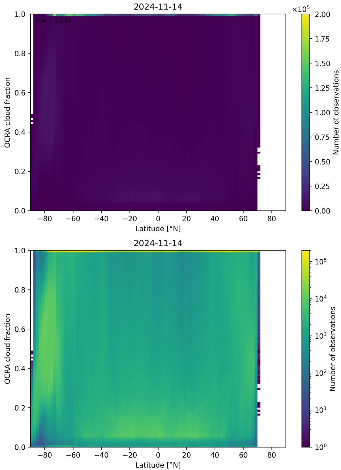
Figure 93: Scatter density plot of “Latitude” against “OCRA cloud fraction” for 2024-11-14 to 2024-11-15.
