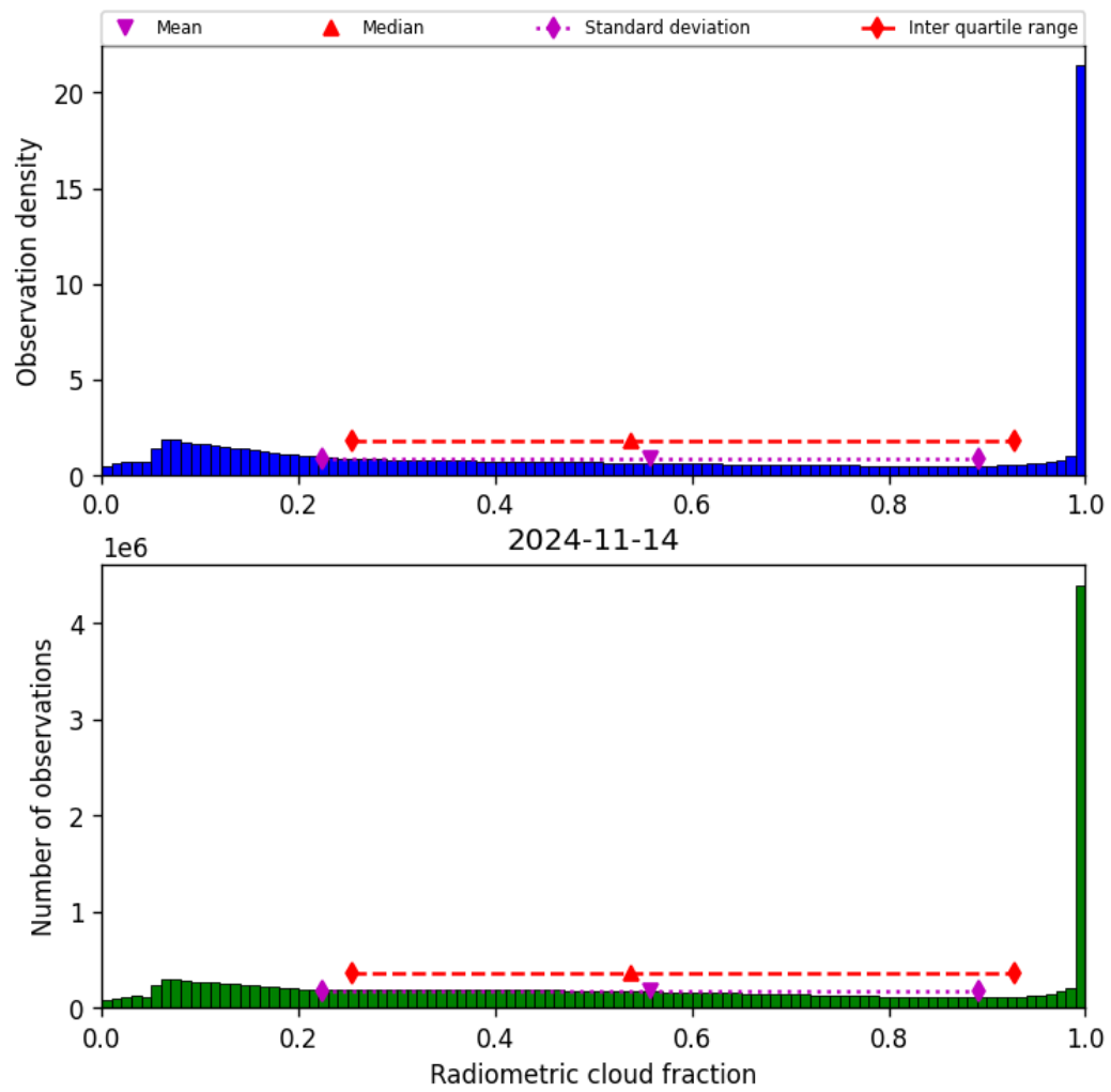
Figure 39: Histogram of “Radiometric cloud fraction” for 2024-11-14 to 2024-11-15
