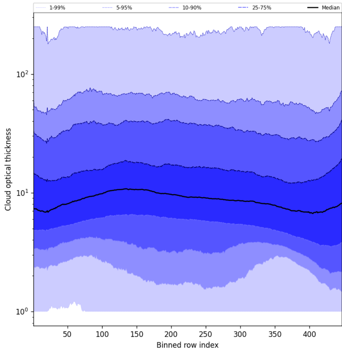
Figure 57: Along track statistics of “Cloud optical thickness” for 2024-11-14 to 2024-11-15
