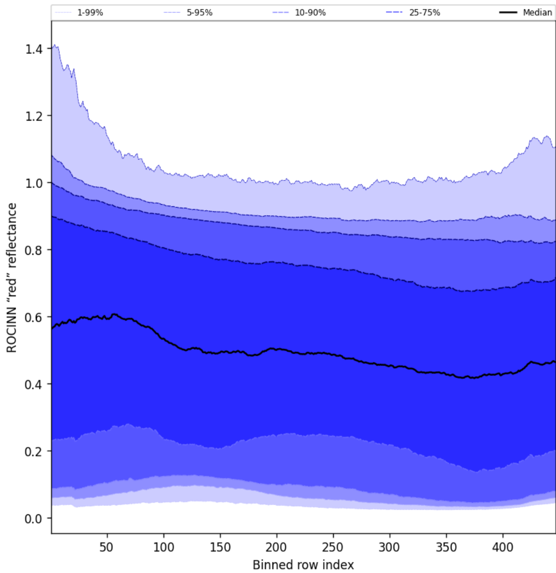
Figure 69: Along track statistics of “ROCINN “red” reflectance” for 2024-11-14 to 2024-11-15
