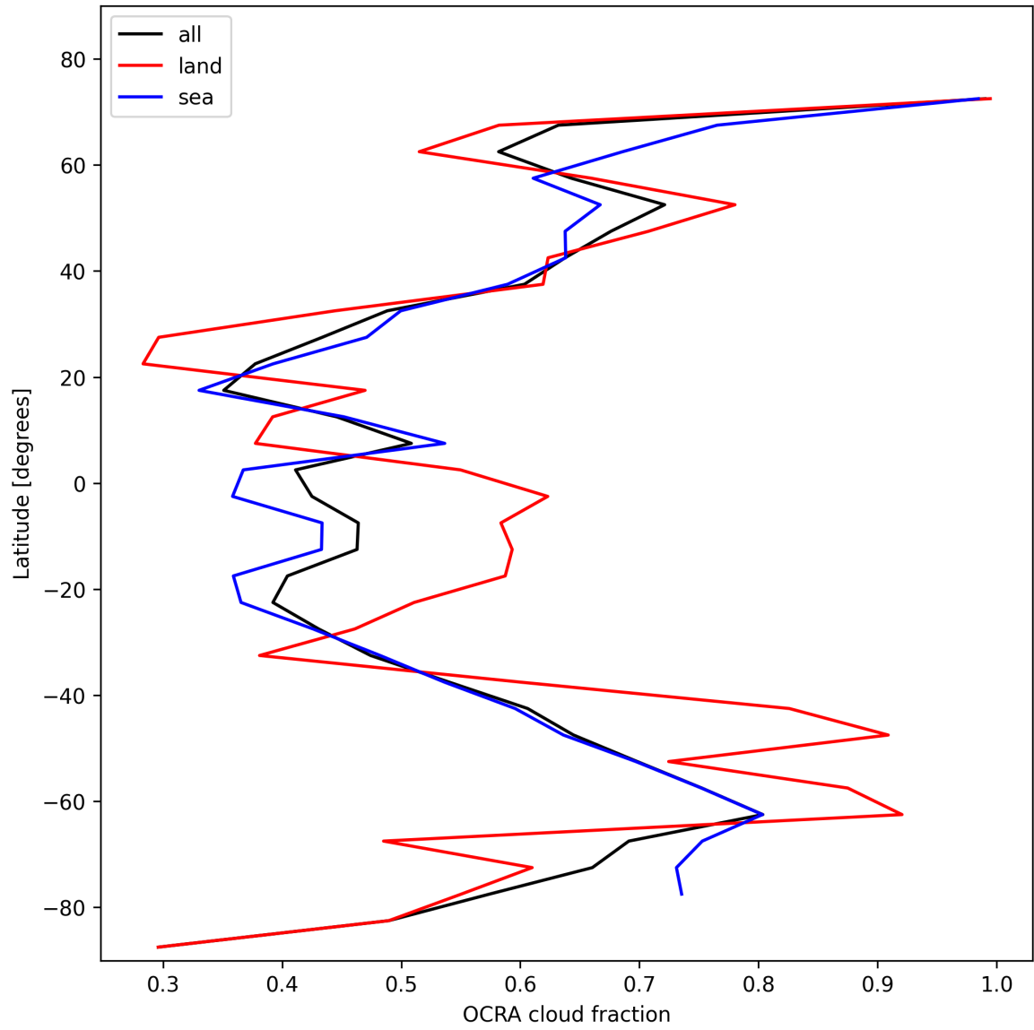
Figure 34: Zonal average of “OCRA cloud fraction” for 2024-11-14 to 2024-11-15.
