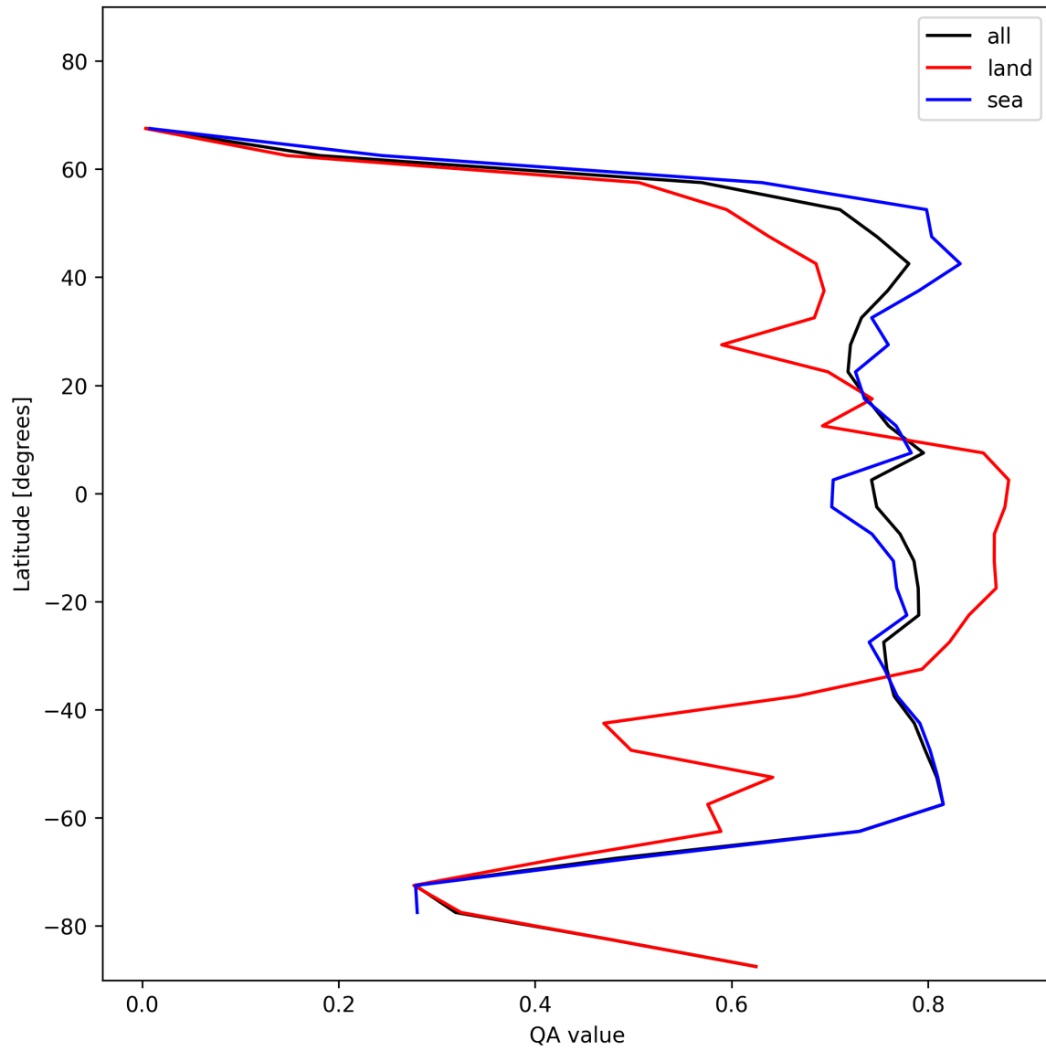
Figure 22: Zonal average of “QA value” for 2024-11-17 to 2024-11-19.
