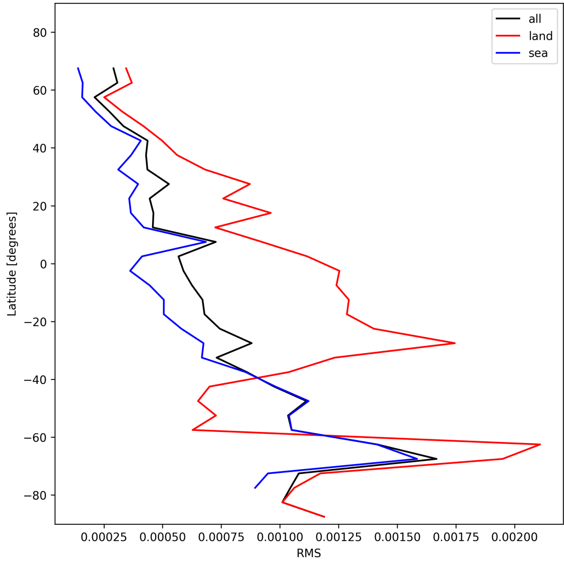
Figure 31: Zonal average of “RMS” for 2024-11-17 to 2024-11-19.
