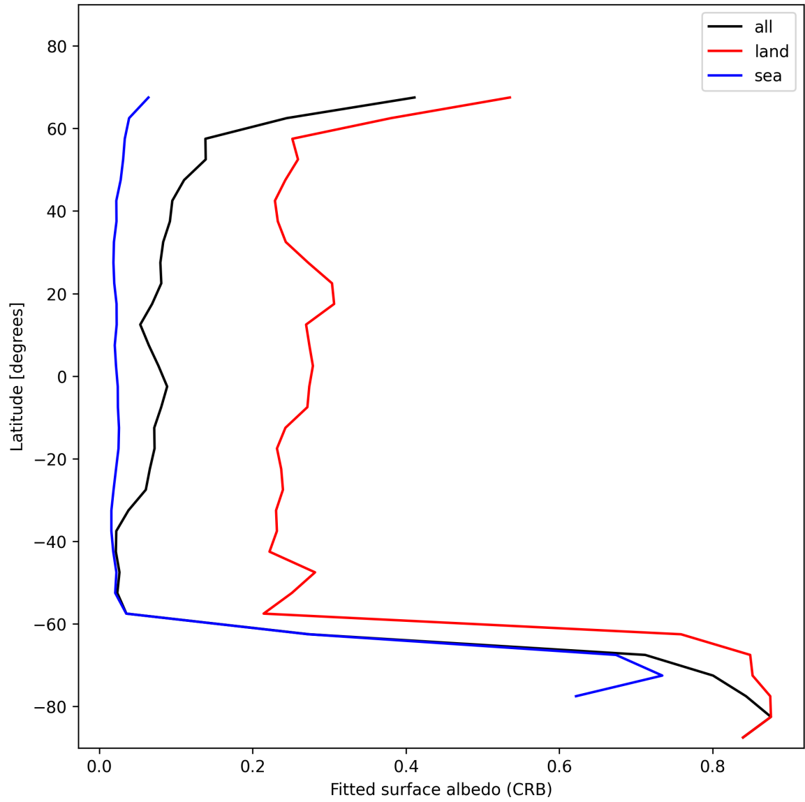
Figure 30: Zonal average of “Fitted surface albedo (CRB)” for 2024-11-17 to 2024-11-19.
