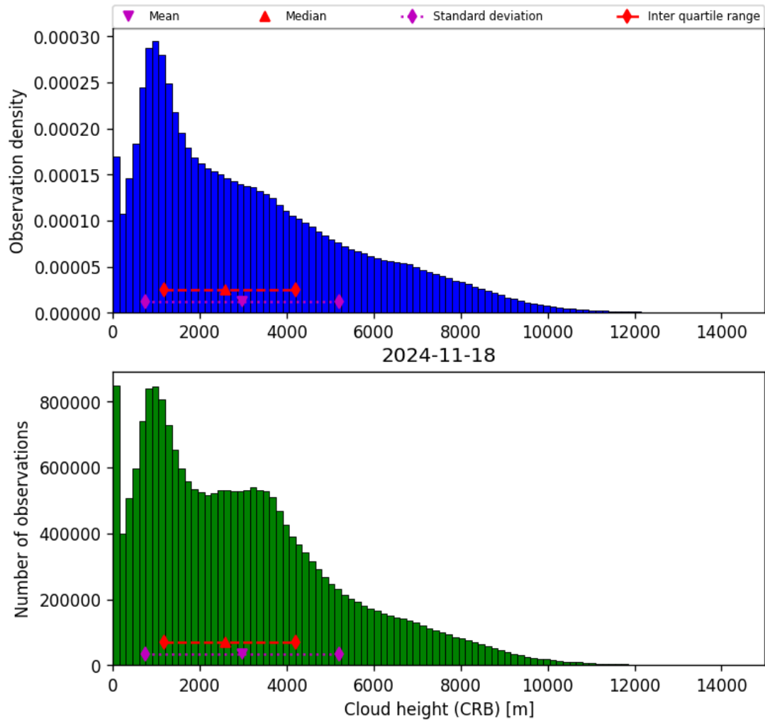
Figure 43: Histogram of “Cloud height (CRB)” for 2024-11-17 to 2024-11-19
