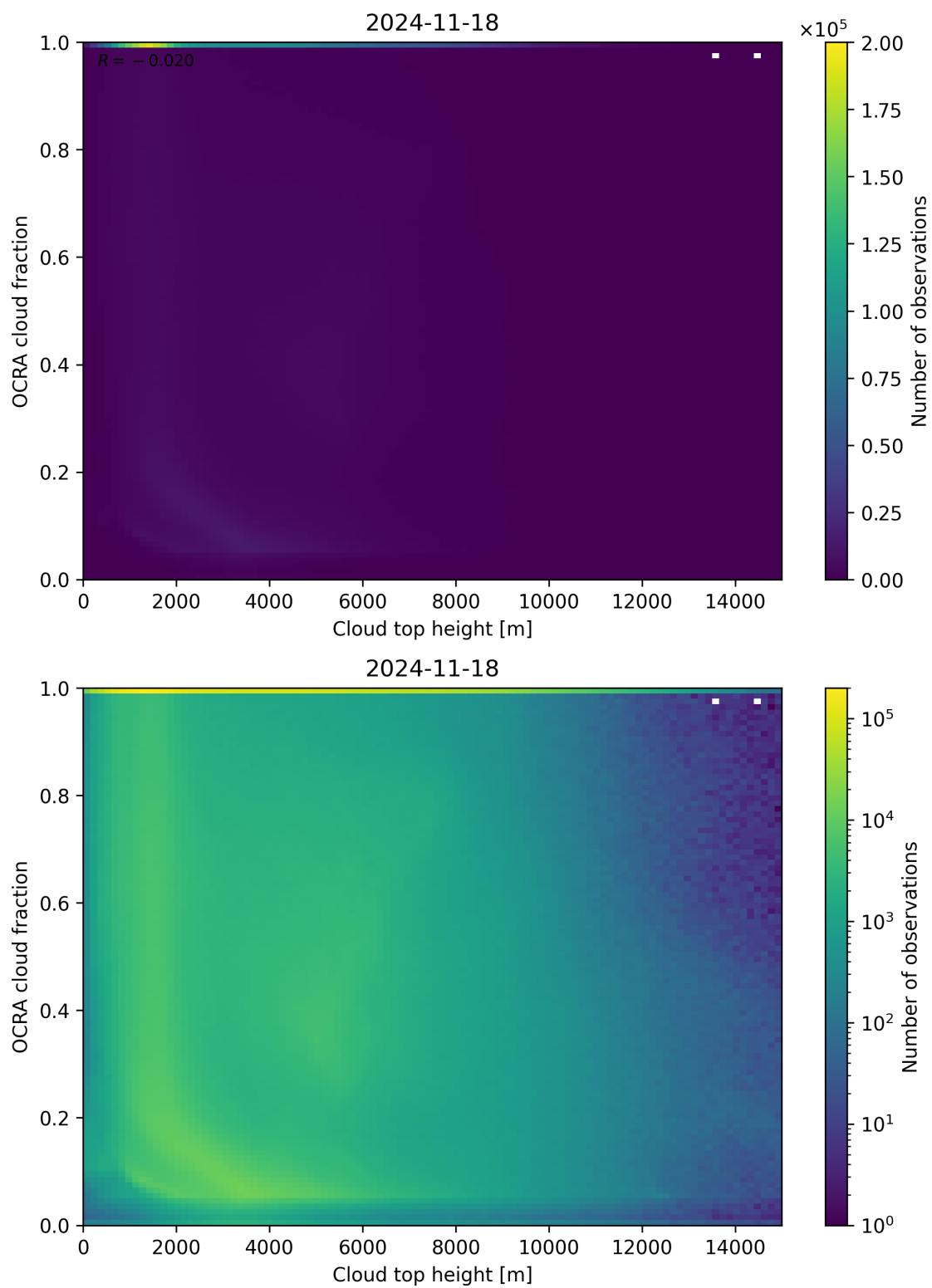
Figure 87: Scatter density plot of “Cloud top height” against “OCRA cloud fraction” for 2024-11-17 to 2024-11-19.
