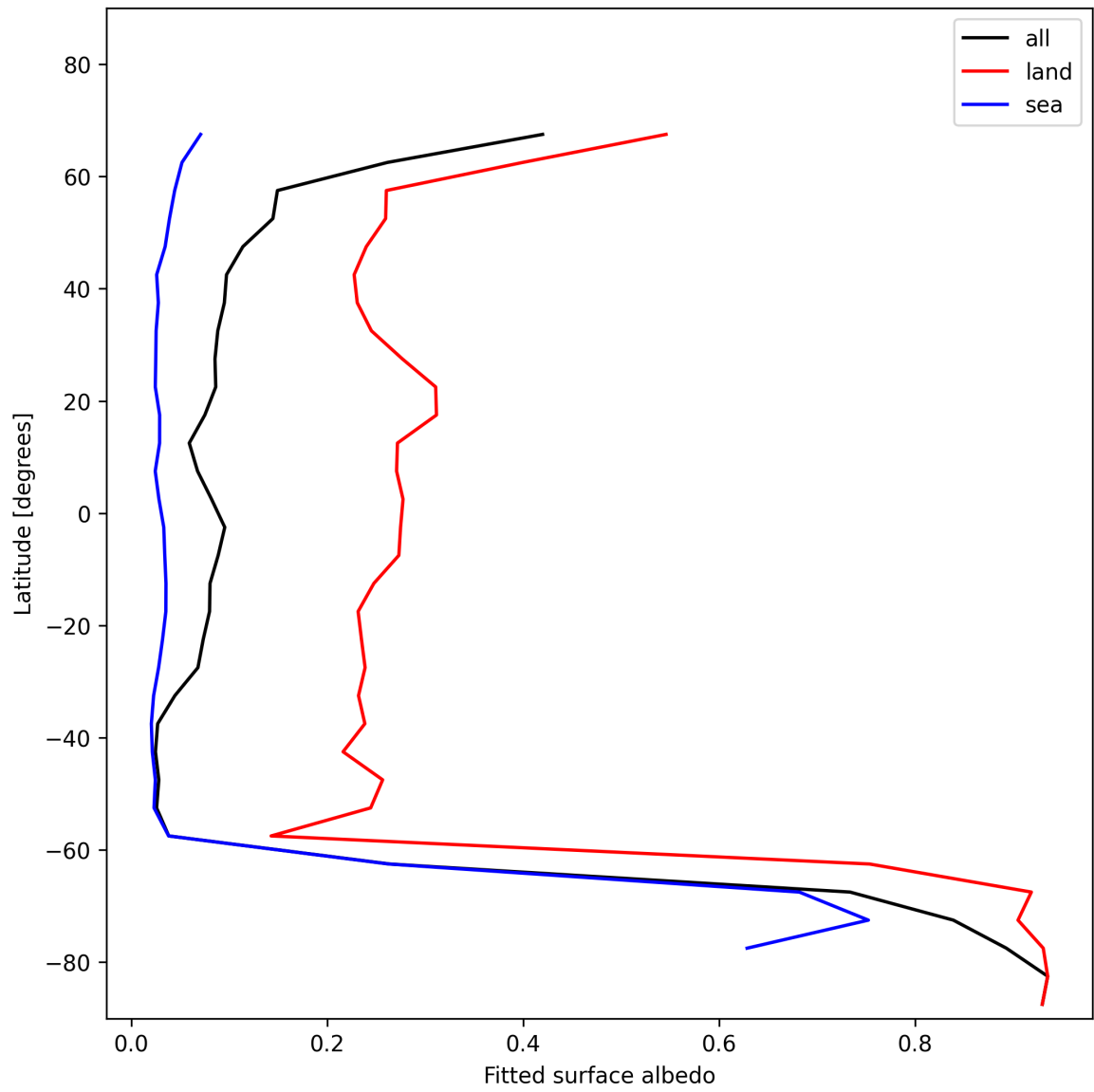
Figure 29: Zonal average of “Fitted surface albedo” for 2024-11-17 to 2024-11-19.
