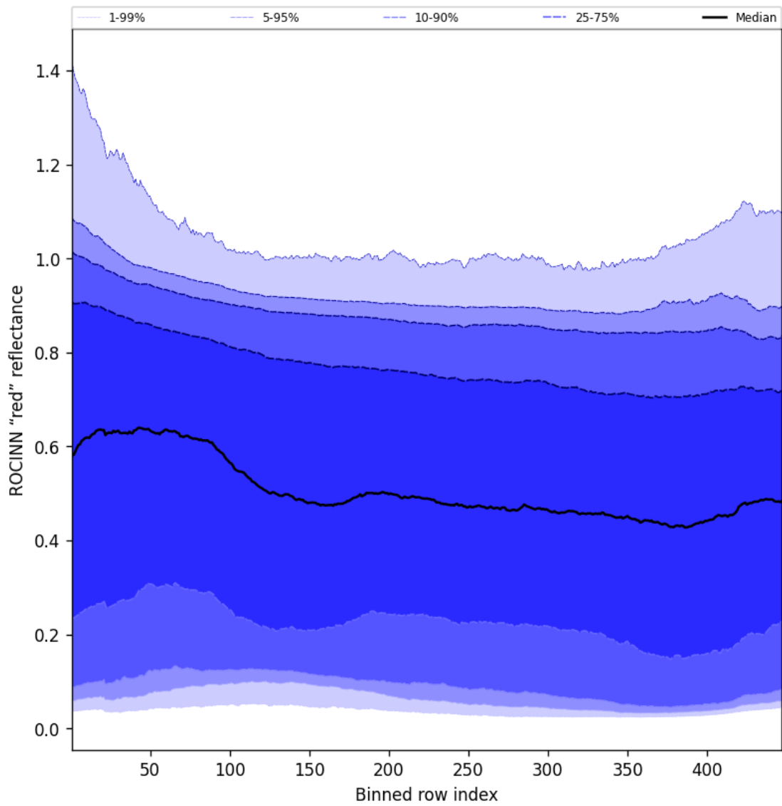
Figure 69: Along track statistics of “ROCINN “red” reflectance” for 2024-11-17 to 2024-11-19
