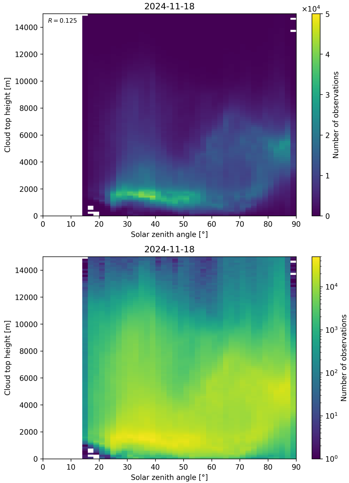
Figure 104: Scatter density plot of “Solar zenith angle” against “Cloud top height” for 2024-11-17 to 2024-11-19.
