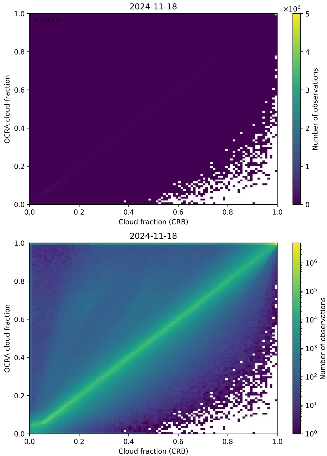
Figure 78: Scatter density plot of “Cloud fraction (CRB)” against “OCRA cloud fraction” for 2024-11-17 to 2024-11-19.
