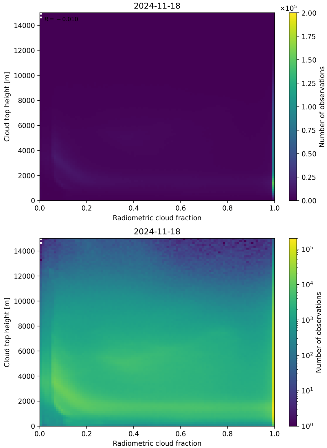
Figure 76: Scatter density plot of “Radiometric cloud fraction” against “Cloud top height” for 2024-11-17 to 2024-11-19.
