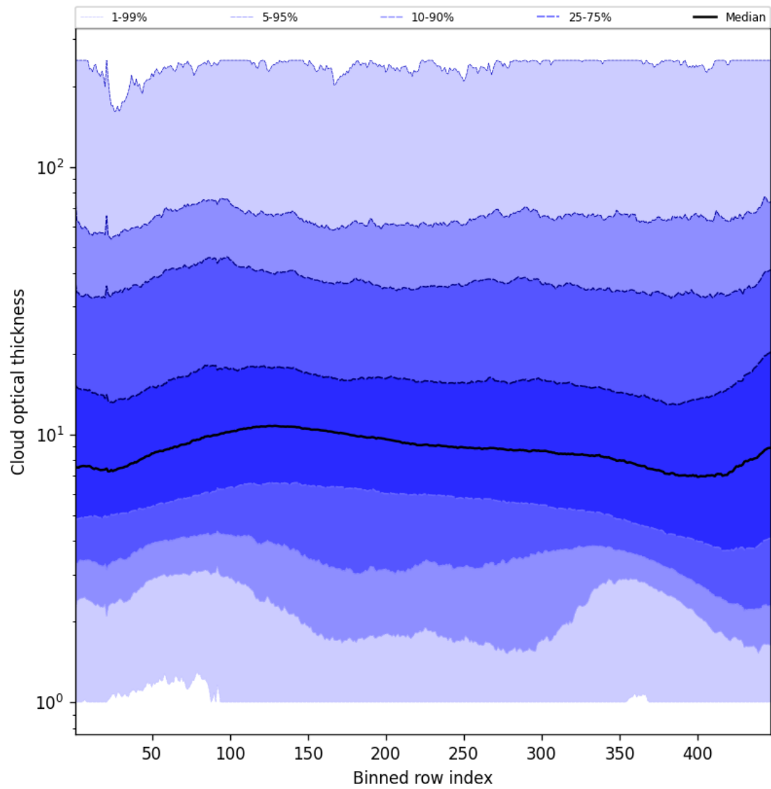
Figure 57: Along track statistics of “Cloud optical thickness” for 2024-11-17 to 2024-11-19
