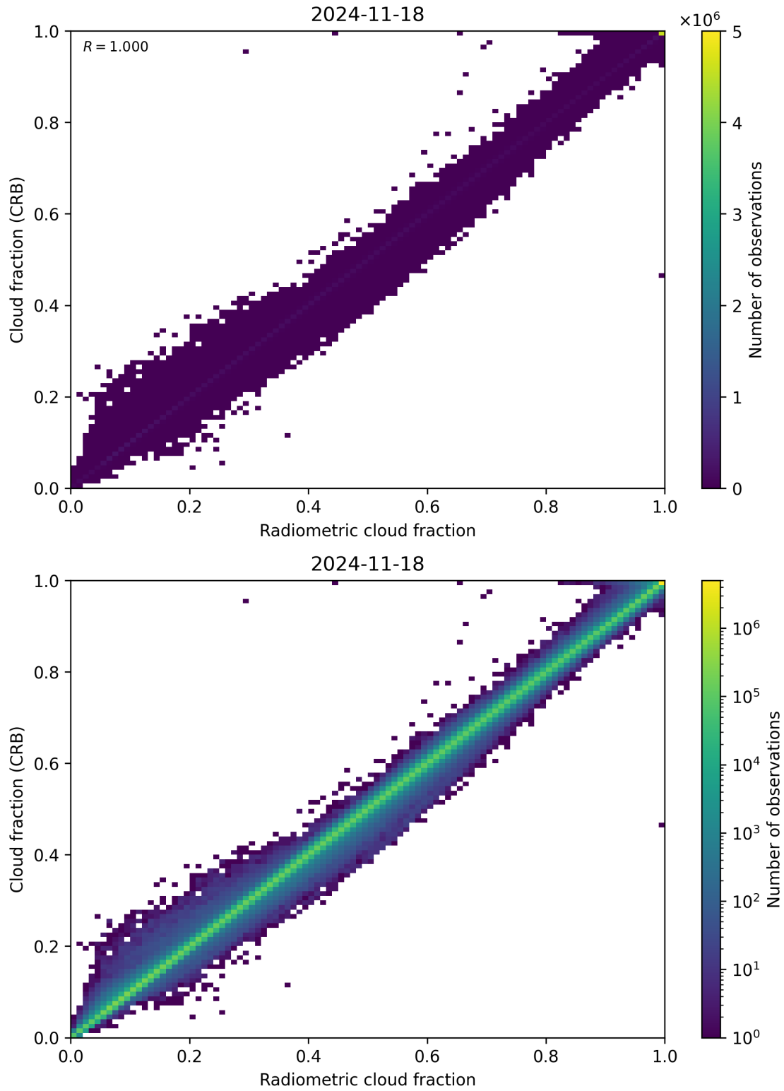
Figure 73: Scatter density plot of “Radiometric cloud fraction” against “Cloud fraction (CRB)” for 2024-11-17 to 2024-11-19.
