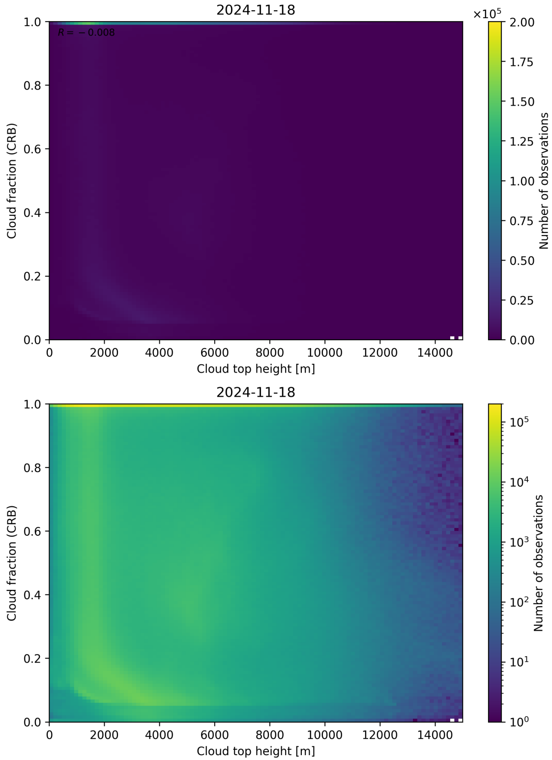
Figure 88: Scatter density plot of “Cloud top height” against “Cloud fraction (CRB)” for 2024-11-17 to 2024-11-19.
