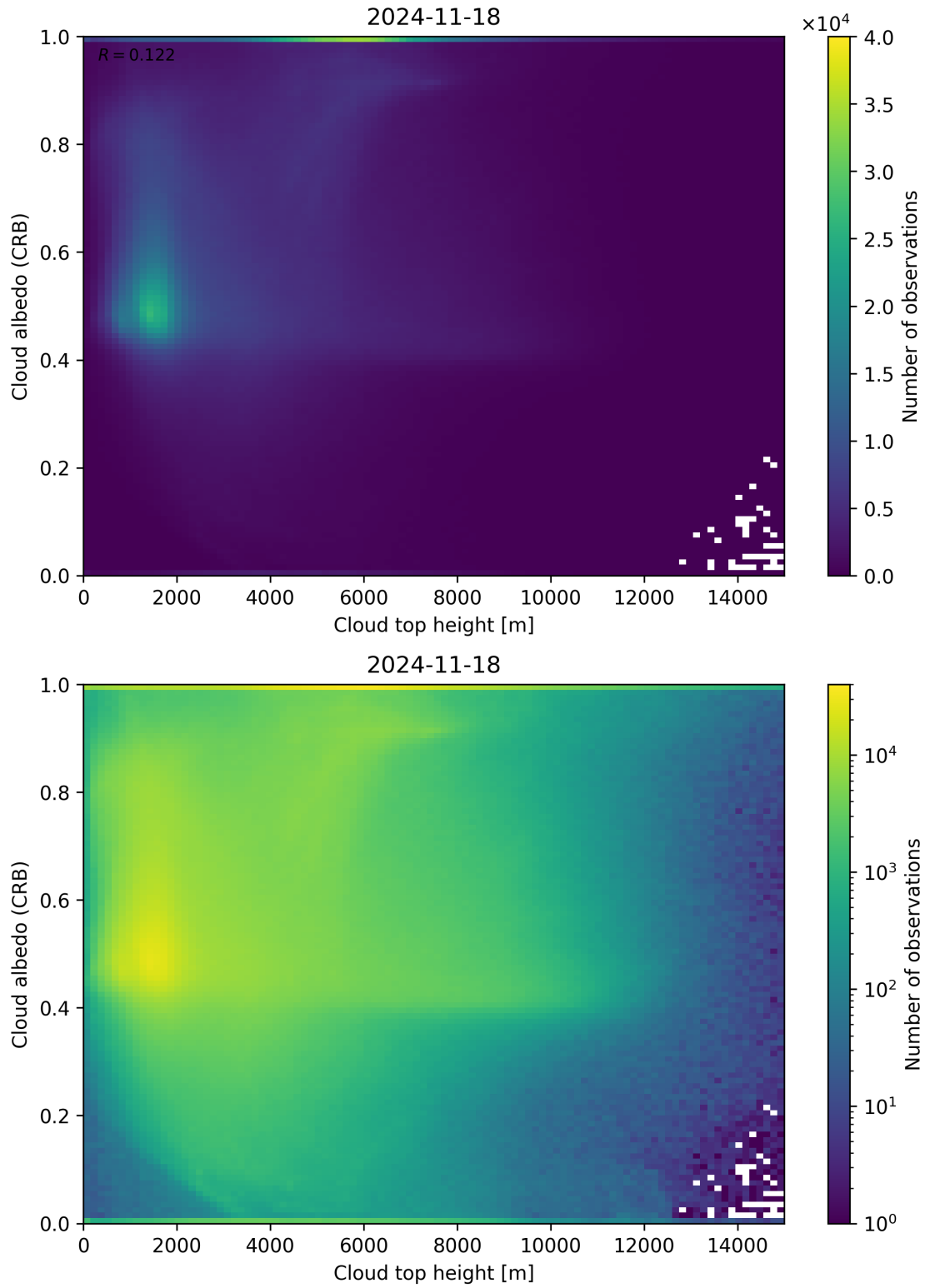
Figure 86: Scatter density plot of “Cloud top height” against “Cloud albedo (CRB)” for 2024-11-17 to 2024-11-19.
