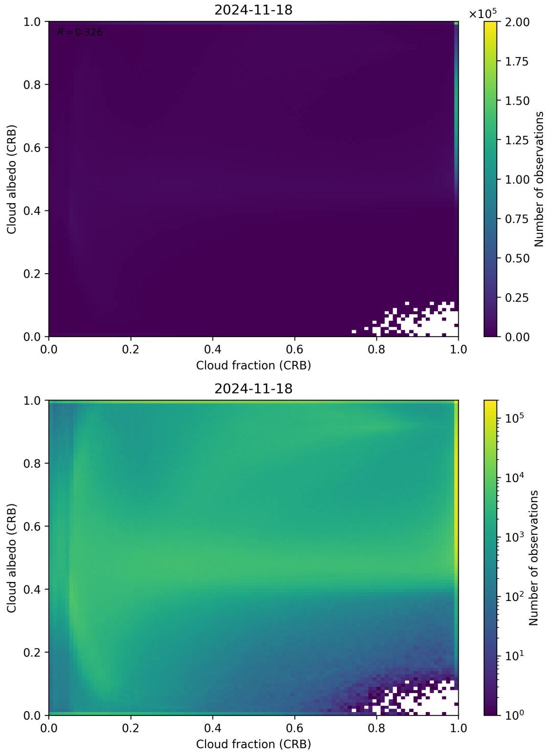
Figure 77: Scatter density plot of “Cloud fraction (CRB)” against “Cloud albedo (CRB)” for 2024-11-17 to 2024-11-19.
