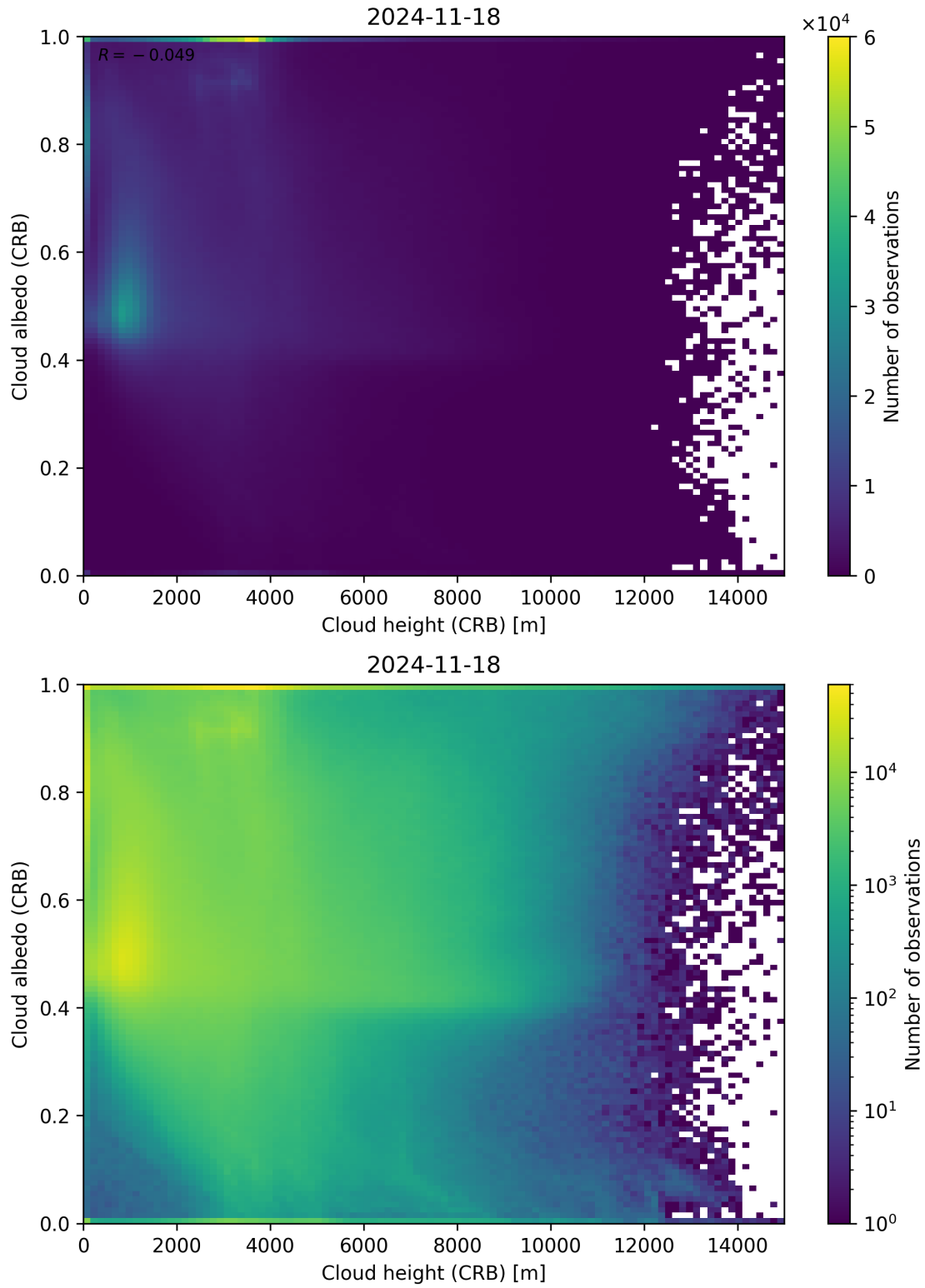
Figure 80: Scatter density plot of “Cloud height (CRB)” against “Cloud albedo (CRB)” for 2024-11-17 to 2024-11-19.
