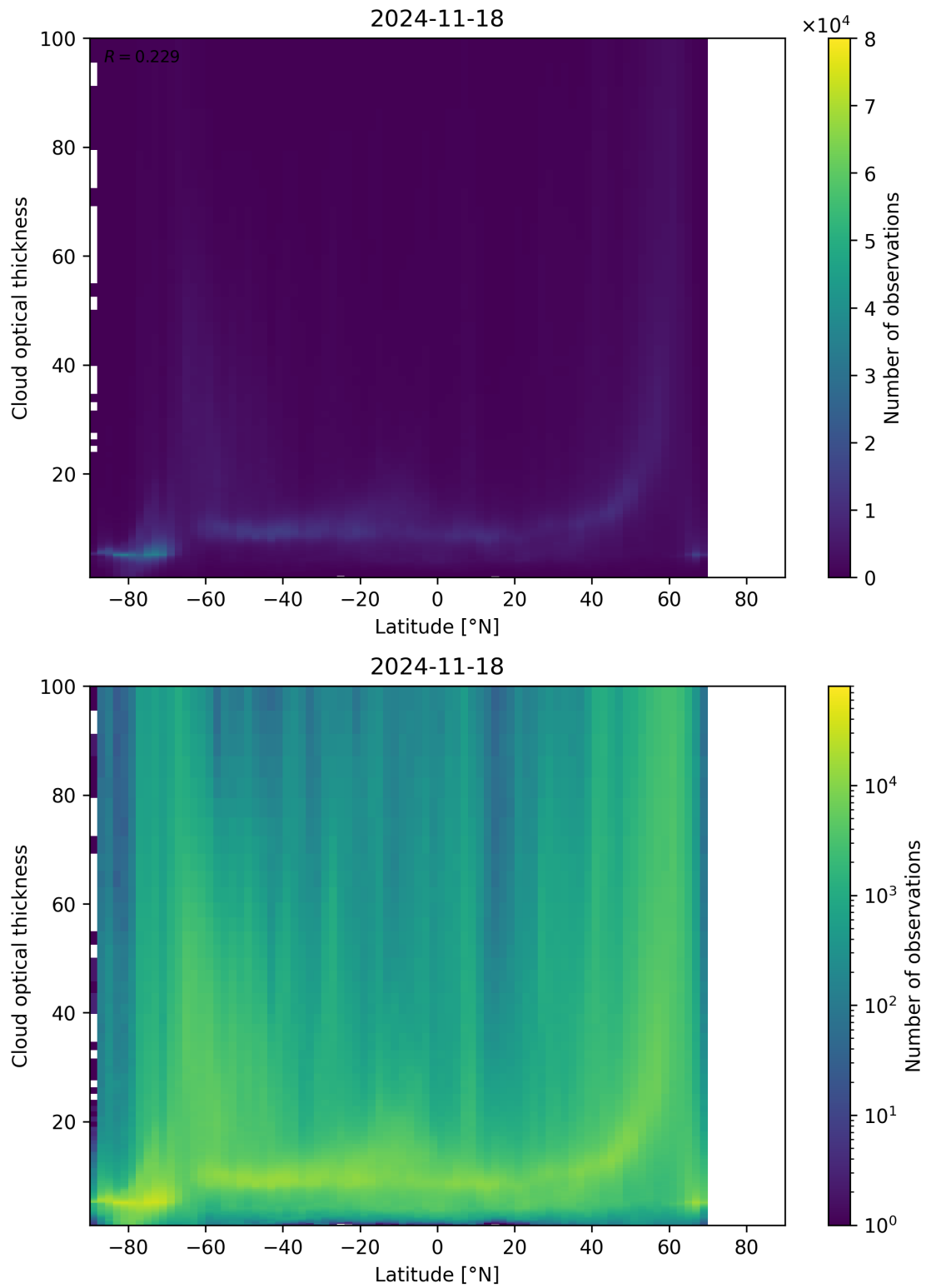
Figure 96: Scatter density plot of “Latitude” against “Cloud optical thickness” for 2024-11-17 to 2024-11-19.
