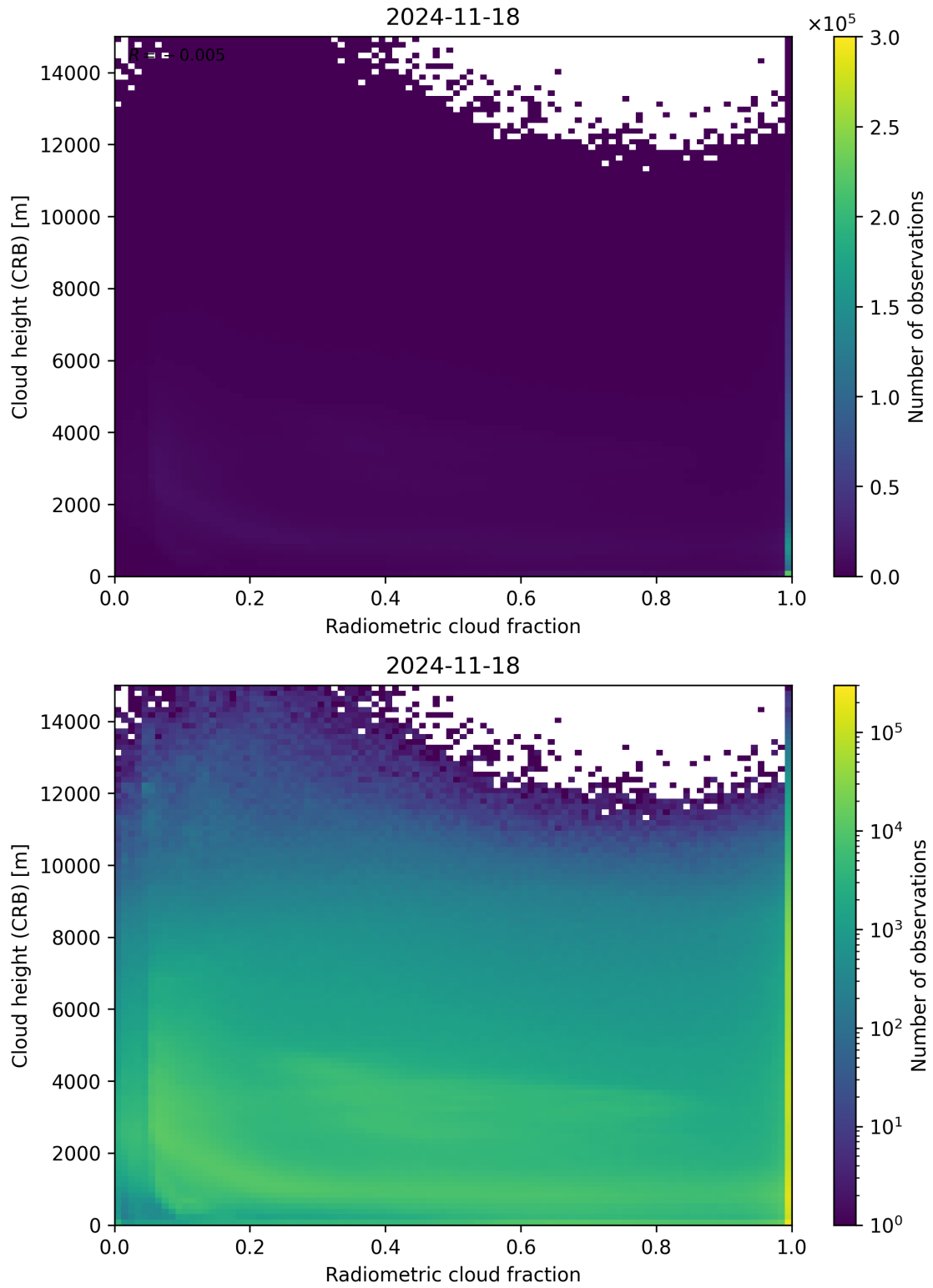
Figure 74: Scatter density plot of “Radiometric cloud fraction” against “Cloud height (CRB)” for 2024-11-17 to 2024-11-19.
