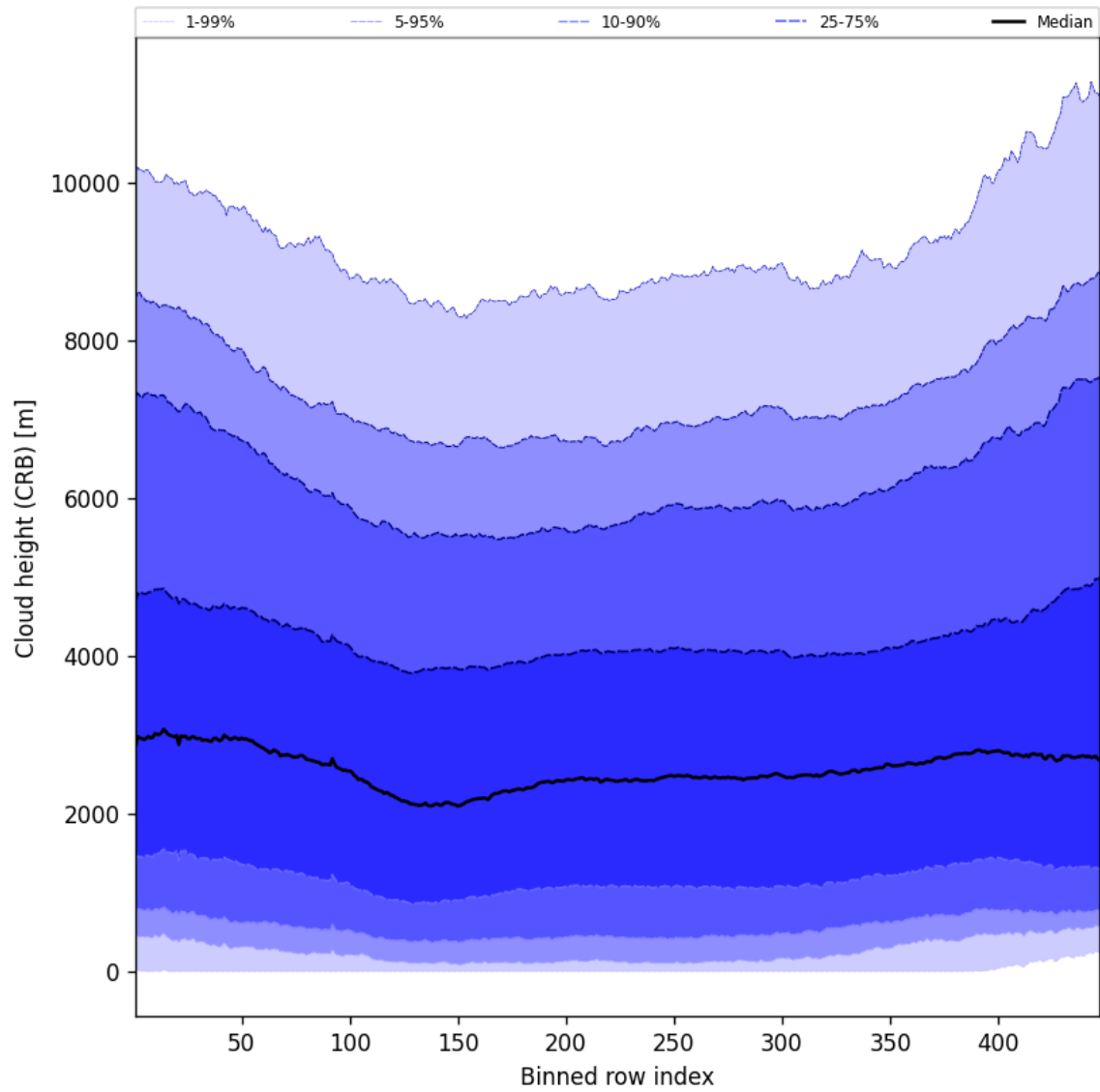
Figure 59: Along track statistics of “Cloud height (CRB)” for 2024-11-17 to 2024-11-19
