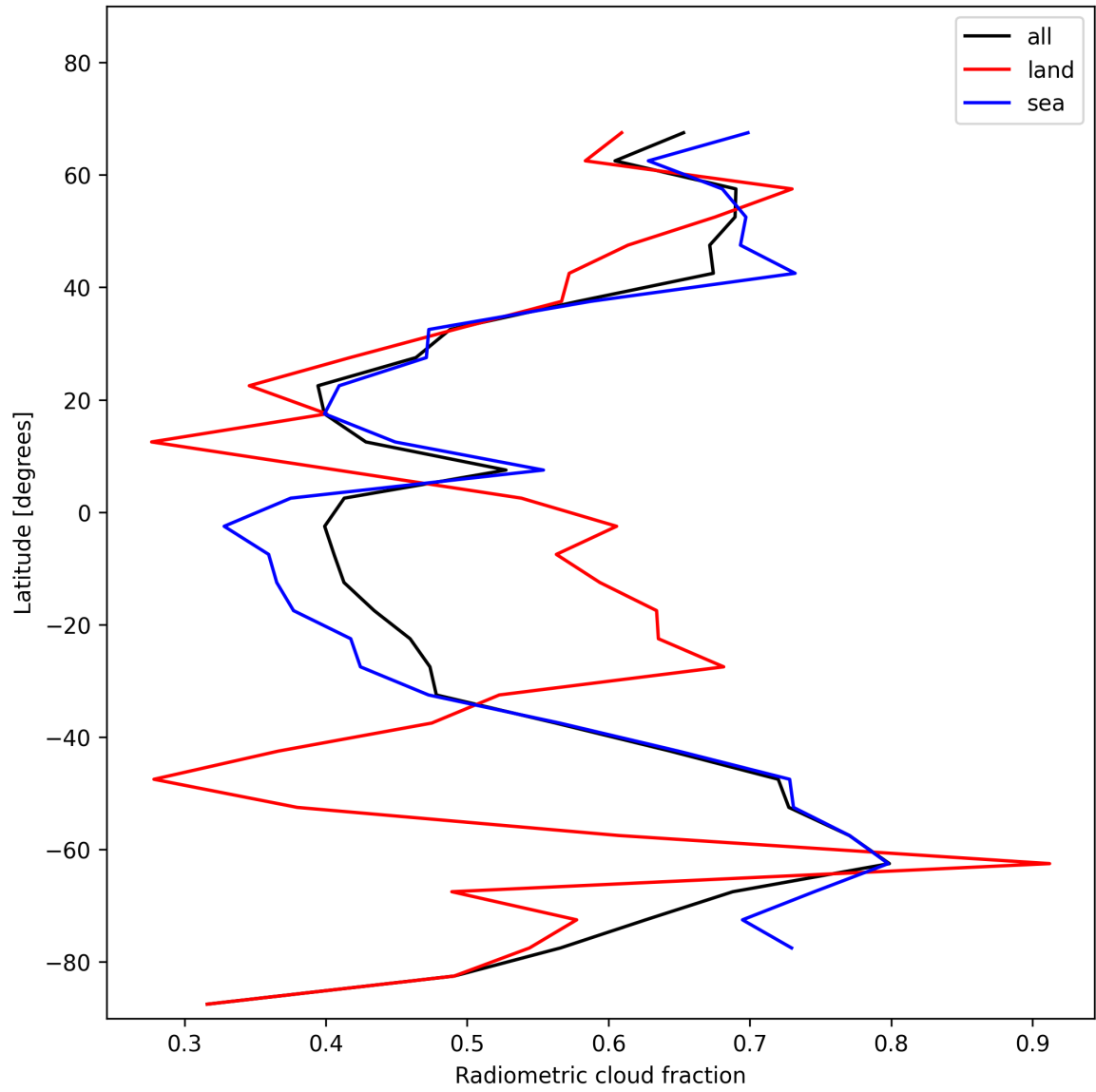
Figure 23: Zonal average of “Radiometric cloud fraction” for 2024-11-17 to 2024-11-19.
