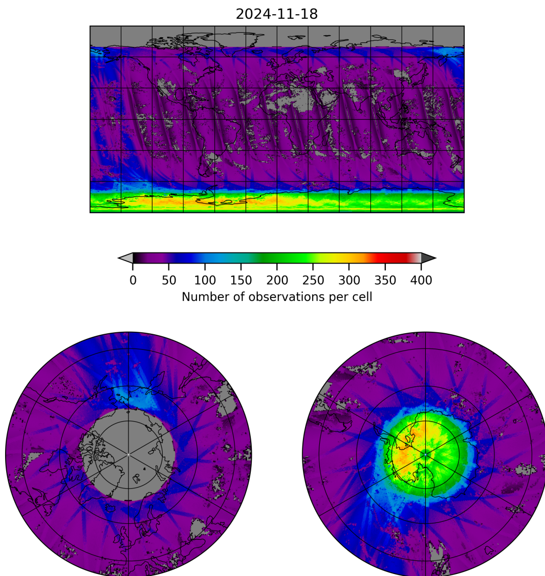
Figure 21: Map of the number of observations for 2024-11-17 to 2024-11-19
