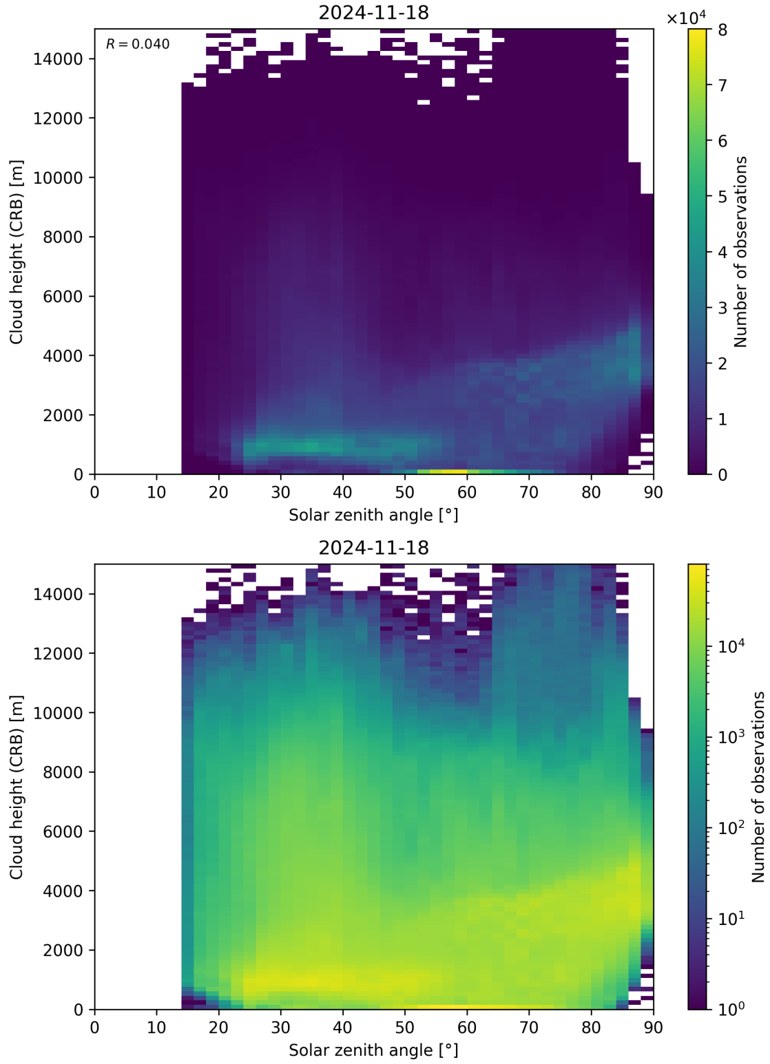
Figure 102: Scatter density plot of “Solar zenith angle” against “Cloud height (CRB)” for 2024-11-17 to 2024-11-19.
