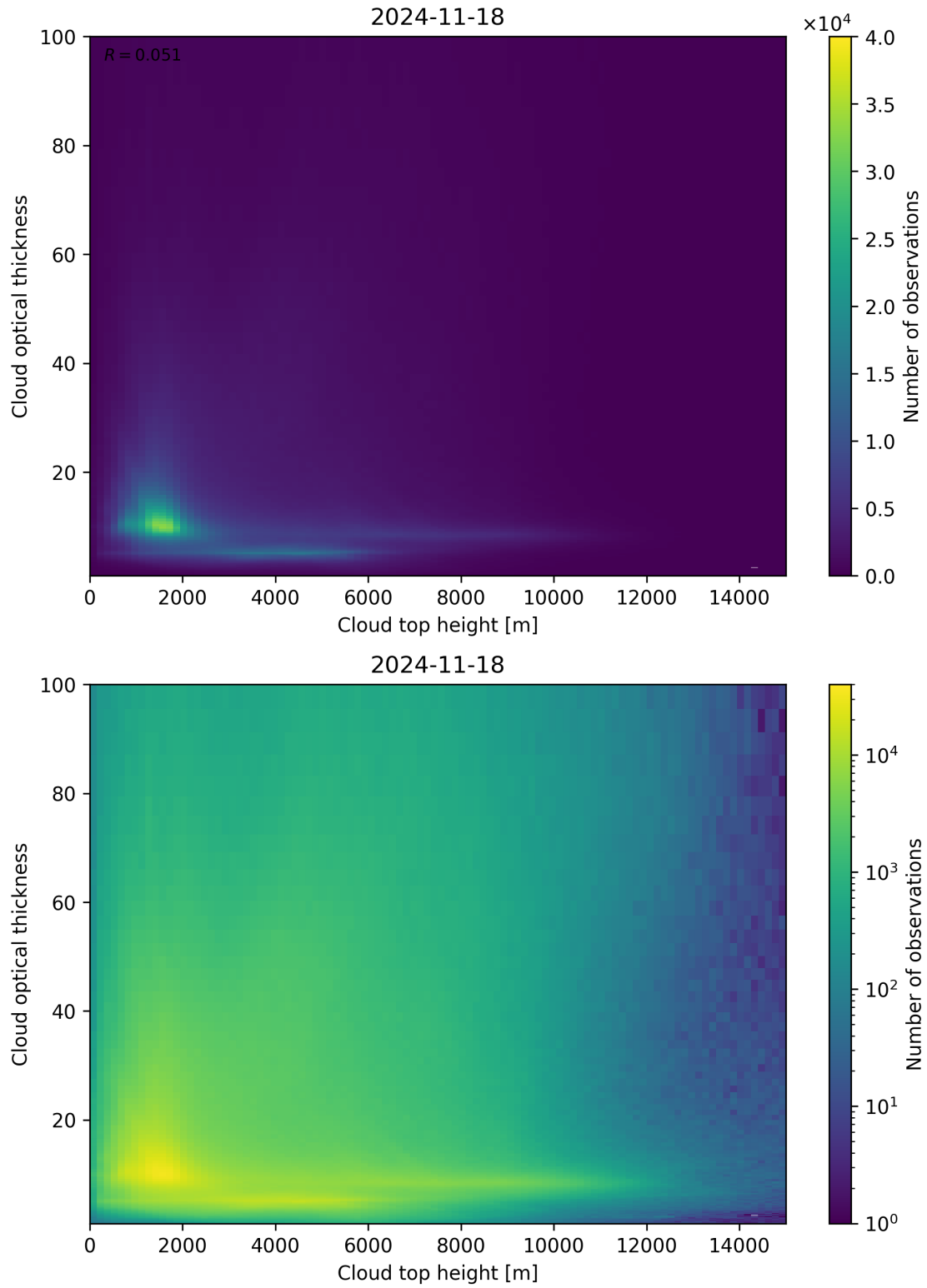
Figure 90: Scatter density plot of “Cloud top height” against “Cloud optical thickness” for 2024-11-17 to 2024-11-19.
