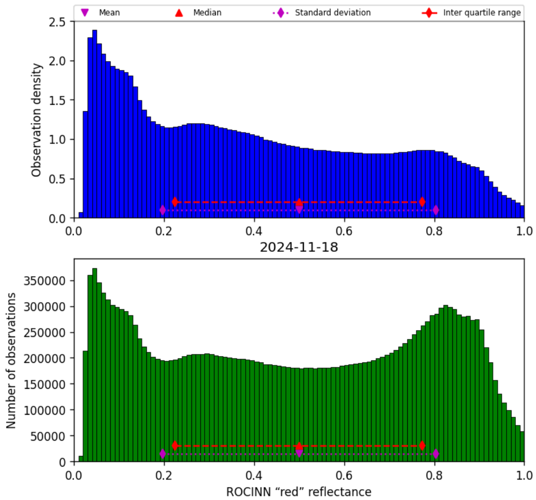
Figure 53: Histogram of “ROCINN “red” reflectance” for 2024-11-17 to 2024-11-19
