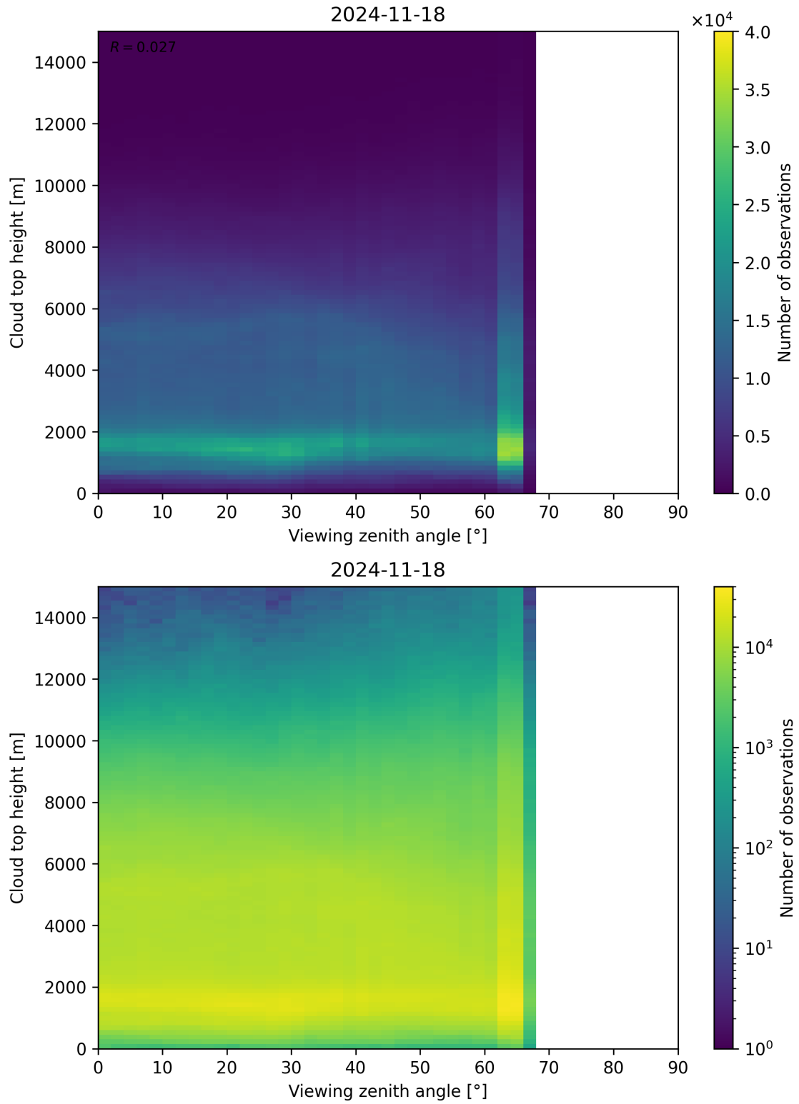
Figure 112: Scatter density plot of “Viewing zenith angle” against “Cloud top height” for 2024-11-17 to 2024-11-19.
