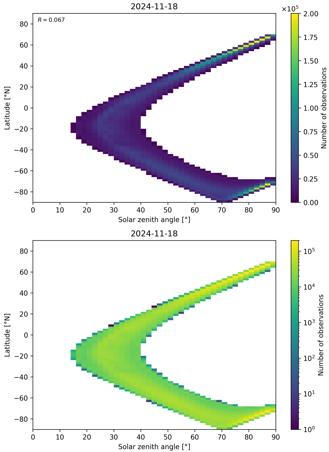
Figure 105: Scatter density plot of “Solar zenith angle” against “Latitude” for 2024-11-17 to 2024-11-19.
