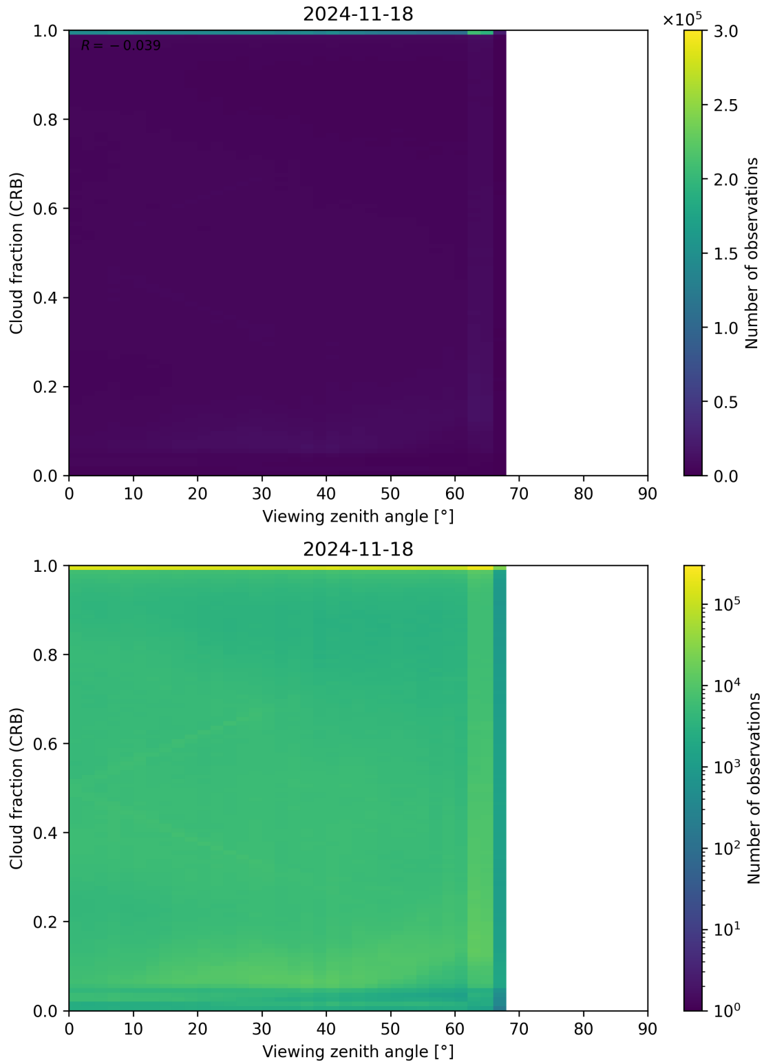
Figure 109: Scatter density plot of “Viewing zenith angle” against “Cloud fraction (CRB)” for 2024-11-17 to 2024-11-19.
