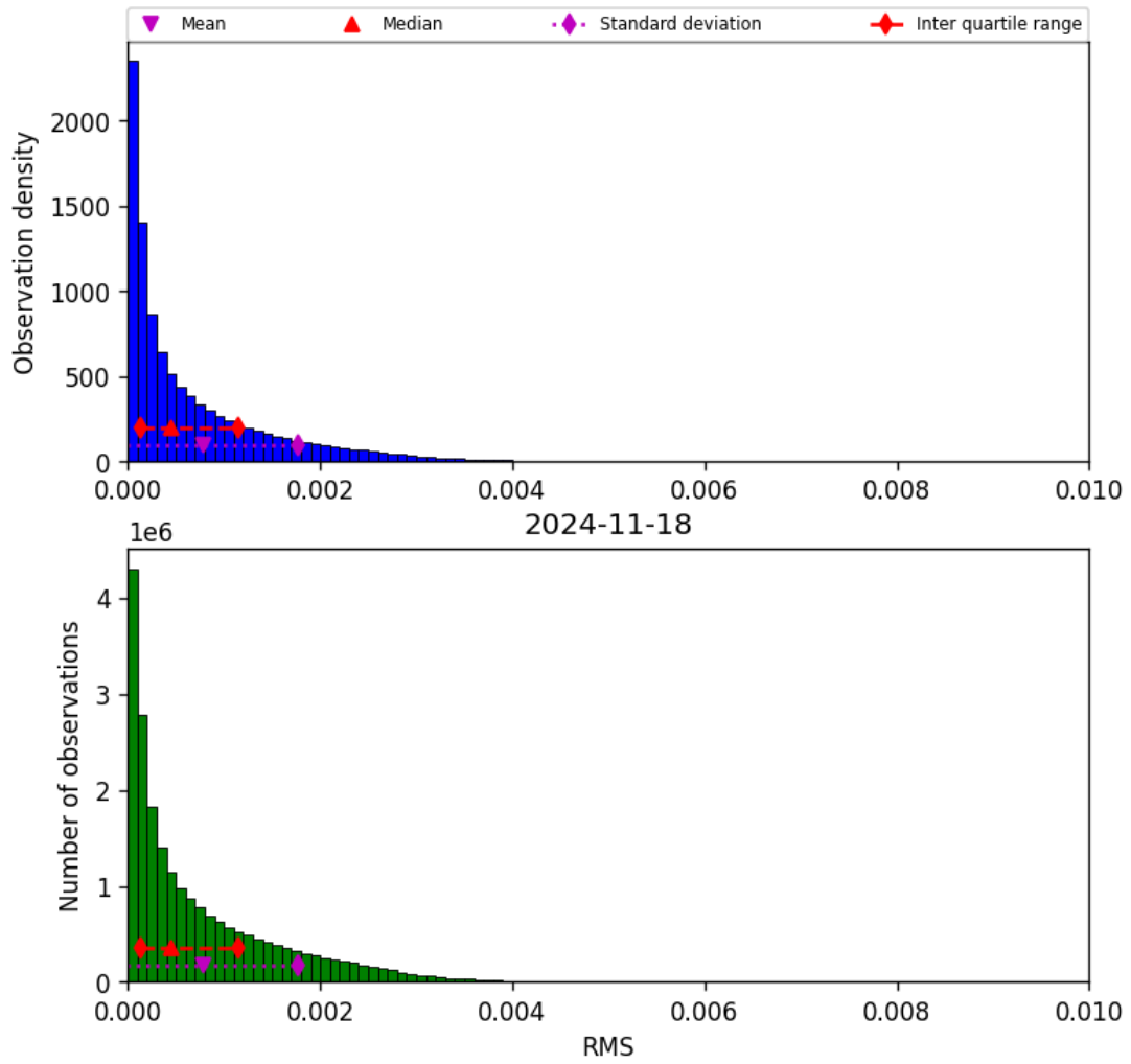
Figure 47: Histogram of “RMS” for 2024-11-17 to 2024-11-19
