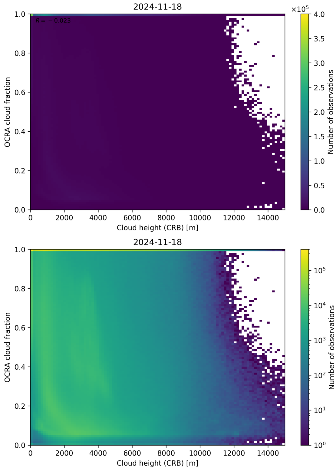
Figure 81: Scatter density plot of “Cloud height (CRB)” against “OCRA cloud fraction” for 2024-11-17 to 2024-11-19.
