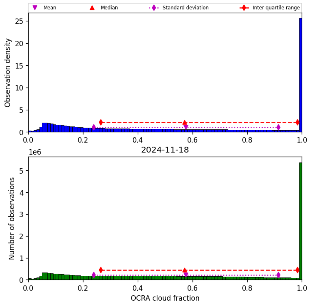
Figure 50: Histogram of “OCRA cloud fraction” for 2024-11-17 to 2024-11-19
