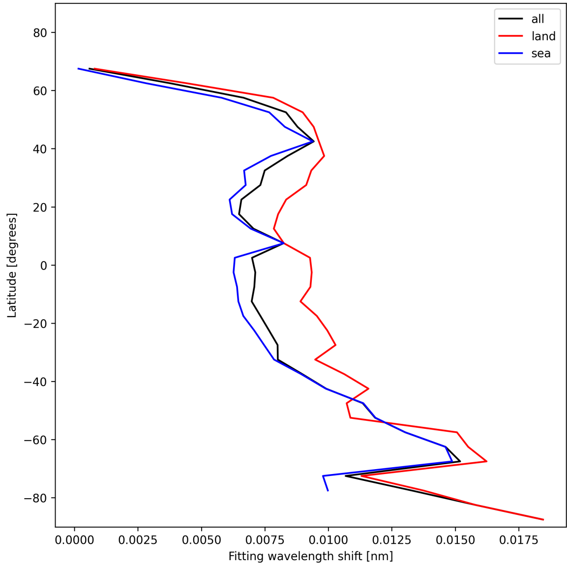
Figure 33: Zonal average of “Fitting wavelength shift” for 2024-11-17 to 2024-11-19.
