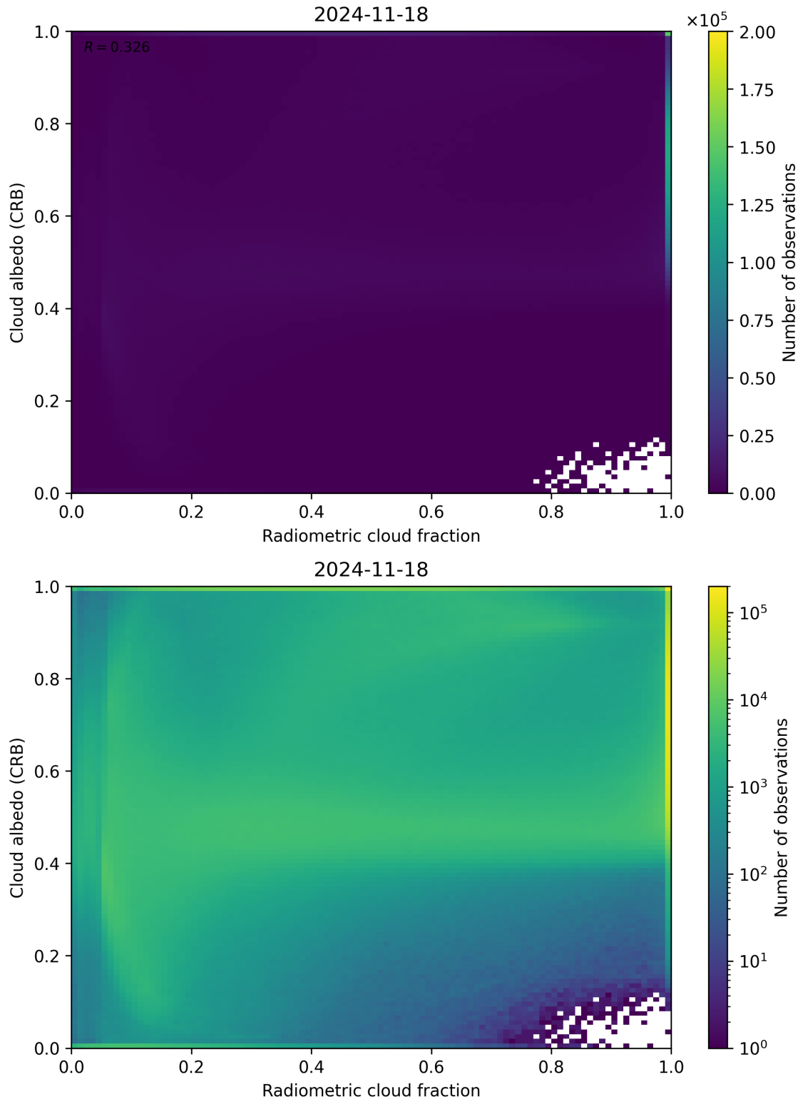
Figure 71: Scatter density plot of “Radiometric cloud fraction” against “Cloud albedo (CRB)” for 2024-11-17 to 2024-11-19.
