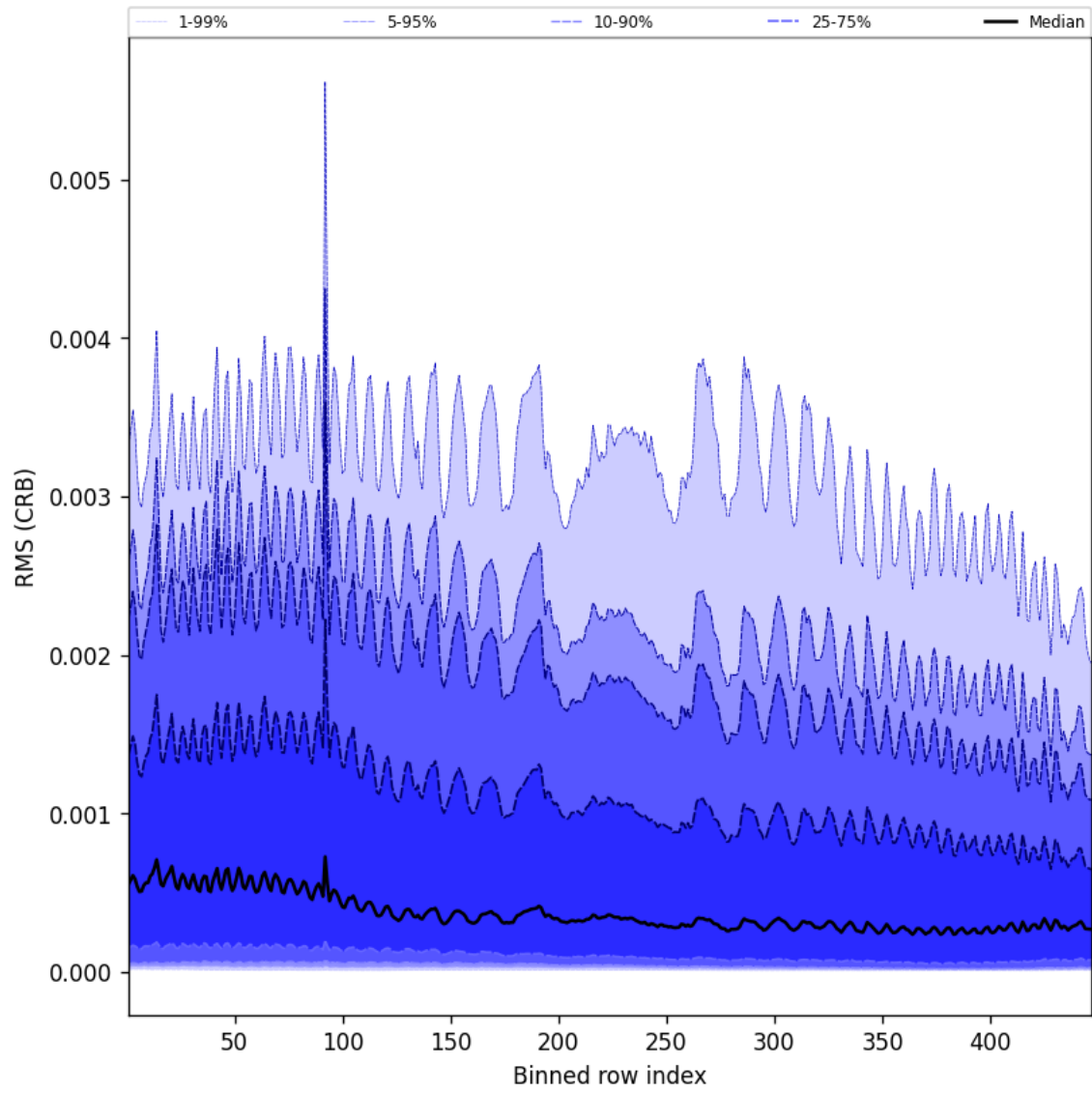
Figure 64: Along track statistics of “RMS (CRB)” for 2024-11-17 to 2024-11-19
