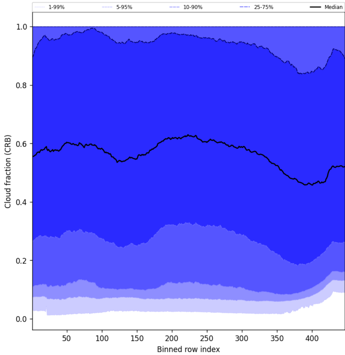
Figure 58: Along track statistics of “Cloud fraction (CRB)” for 2024-11-17 to 2024-11-19
