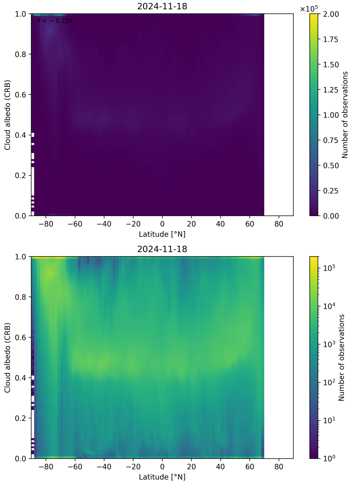
Figure 91: Scatter density plot of “Latitude” against “Cloud albedo (CRB)” for 2024-11-17 to 2024-11-19.
