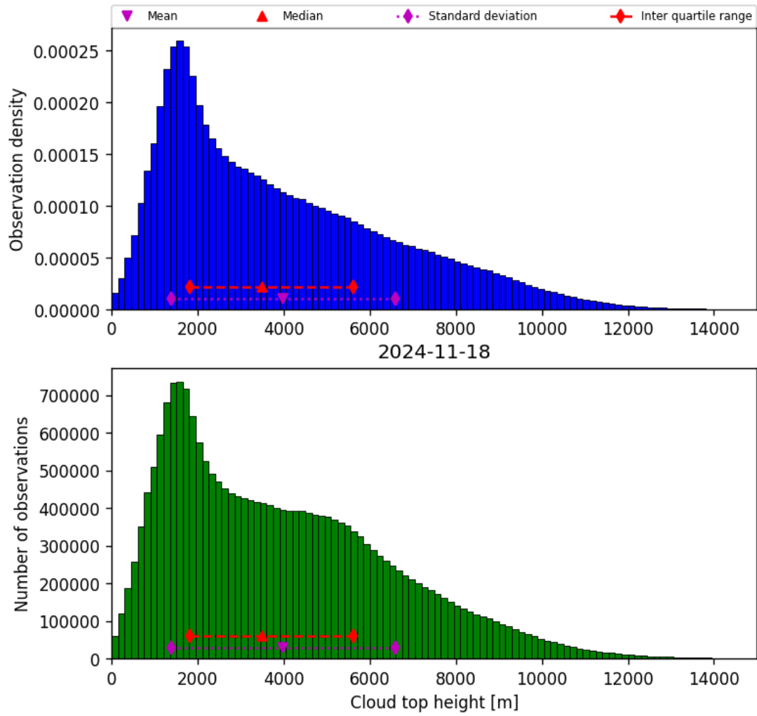
Figure 40: Histogram of “Cloud top height” for 2024-11-17 to 2024-11-19
