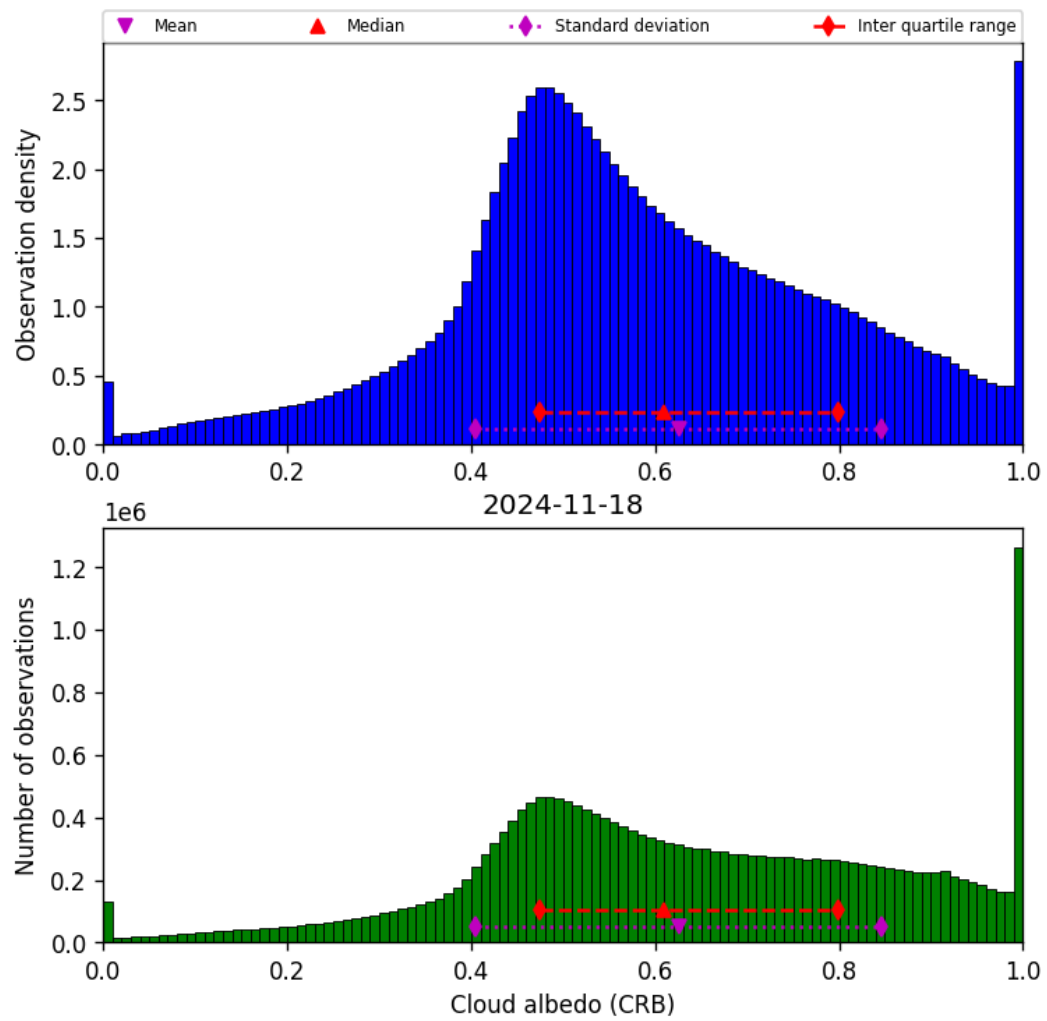
Figure 44: Histogram of “Cloud albedo (CRB)” for 2024-11-17 to 2024-11-19
