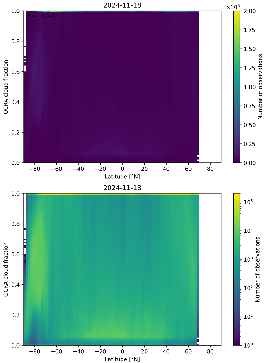
Figure 93: Scatter density plot of “Latitude” against “OCRA cloud fraction” for 2024-11-17 to 2024-11-19.
