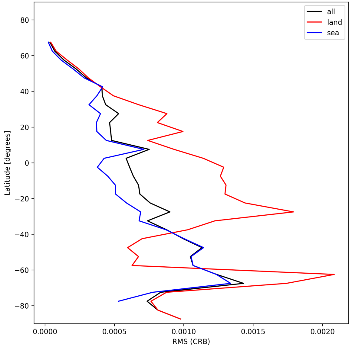
Figure 32: Zonal average of “RMS (CRB)” for 2024-11-17 to 2024-11-19.
