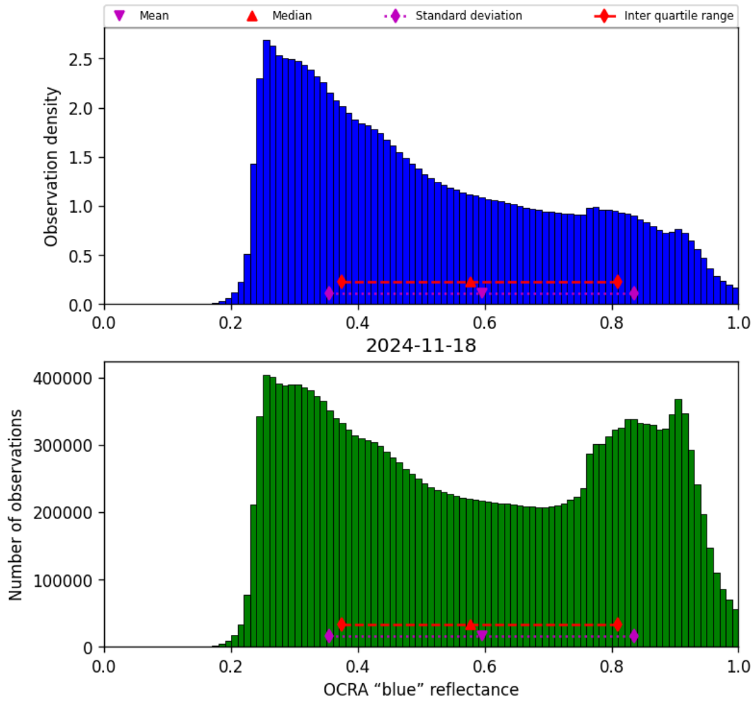
Figure 51: Histogram of "OCRA "blue" reflectance" for 2024-11-17 to 2024-11-19
