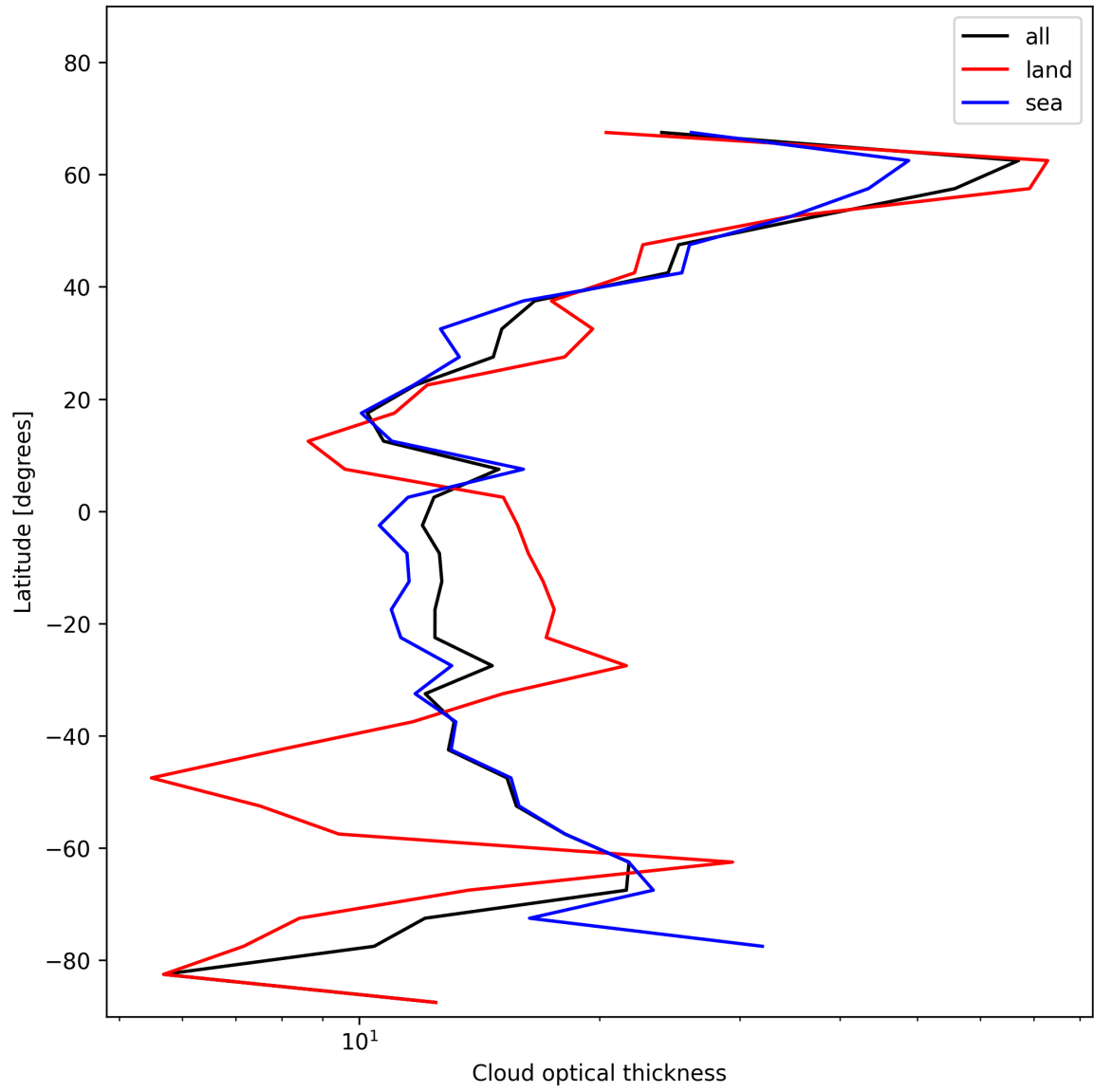
Figure 25: Zonal average of “Cloud optical thickness” for 2024-11-17 to 2024-11-19.
