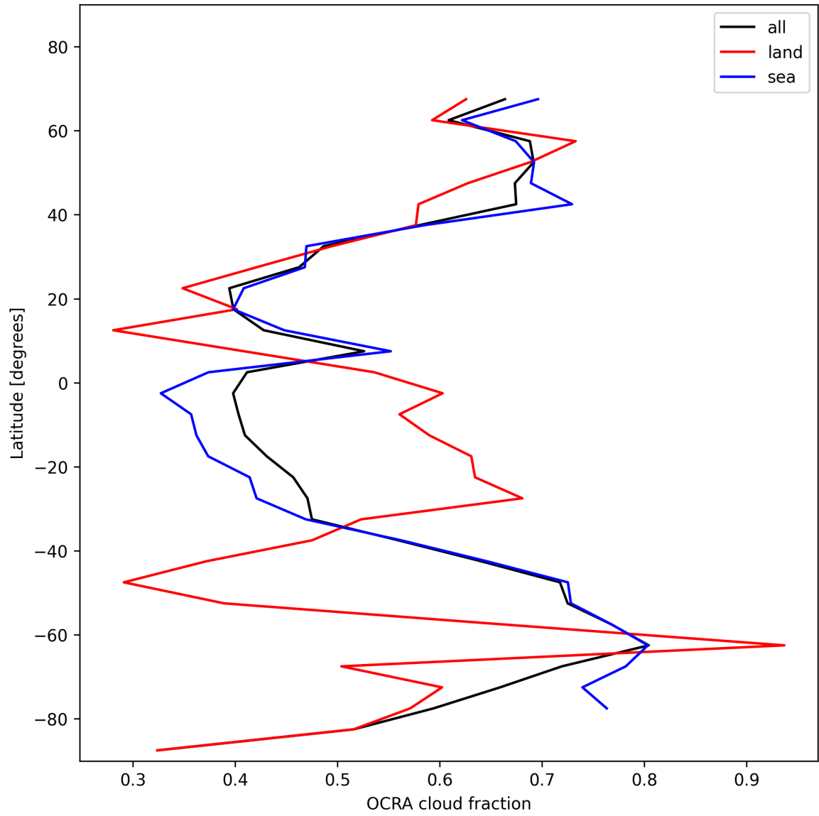
Figure 34: Zonal average of “OCRA cloud fraction” for 2024-11-17 to 2024-11-19.
