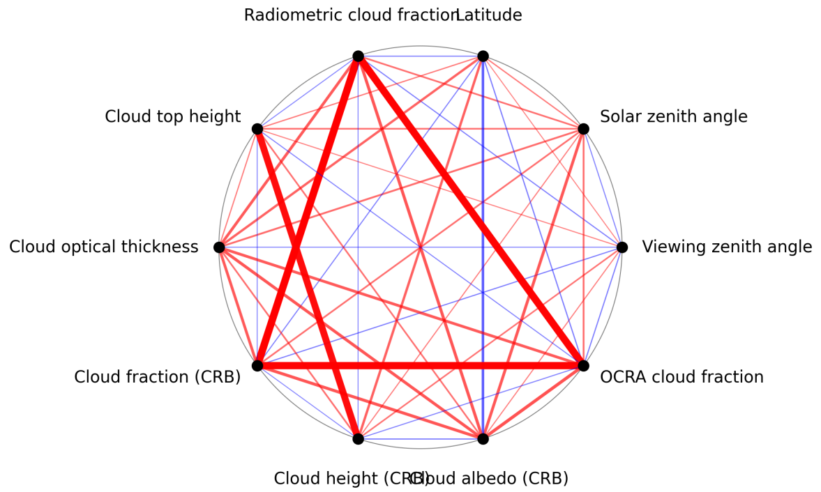
Figure 1: Map of correlation graph for 2024-11-17 to 2024-11-19.
