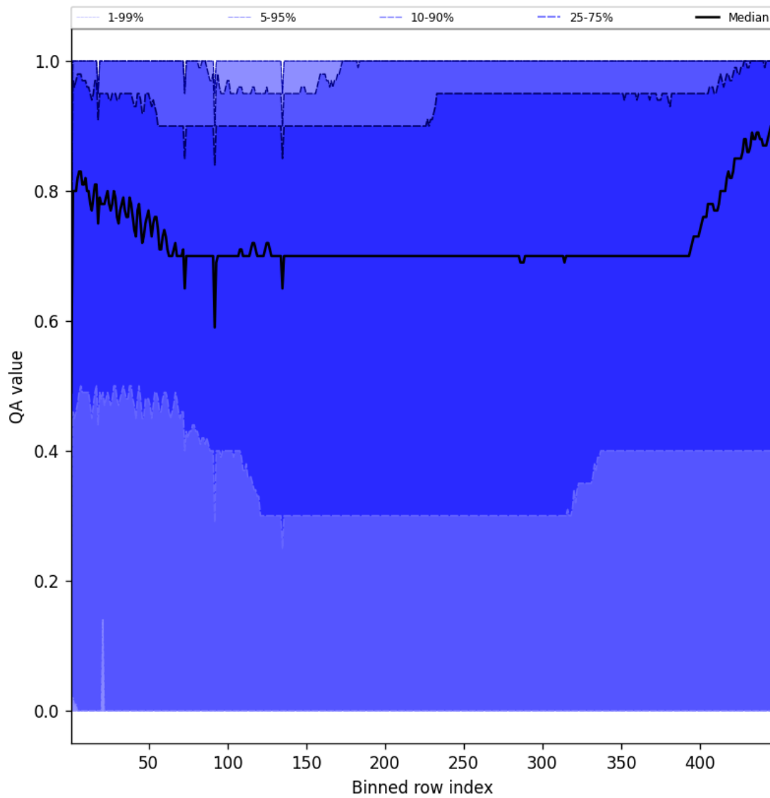
Figure 54: Along track statistics of “QA value” for 2024-11-17 to 2024-11-19
