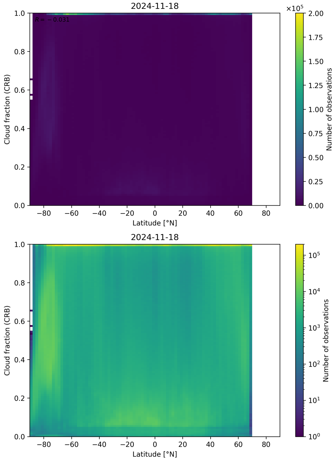
Figure 94: Scatter density plot of “Latitude” against “Cloud fraction (CRB)” for 2024-11-17 to 2024-11-19.
