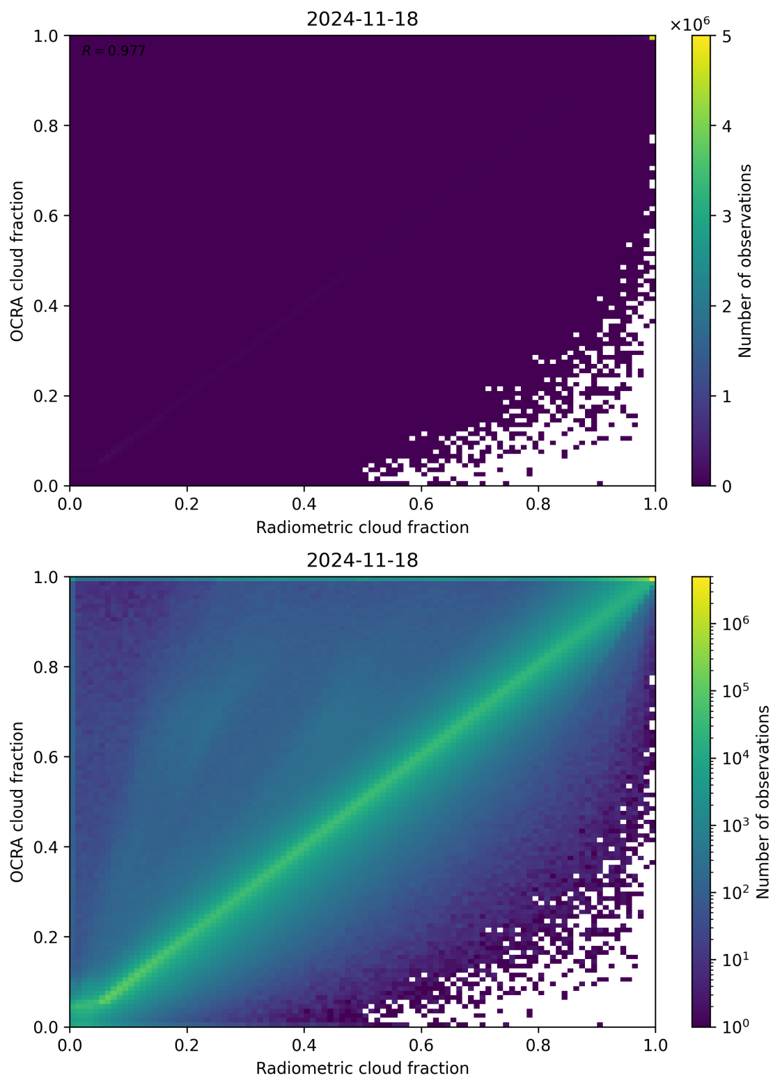
Figure 72: Scatter density plot of “Radiometric cloud fraction” against “OCRA cloud fraction” for 2024-11-17 to 2024-11-19.
