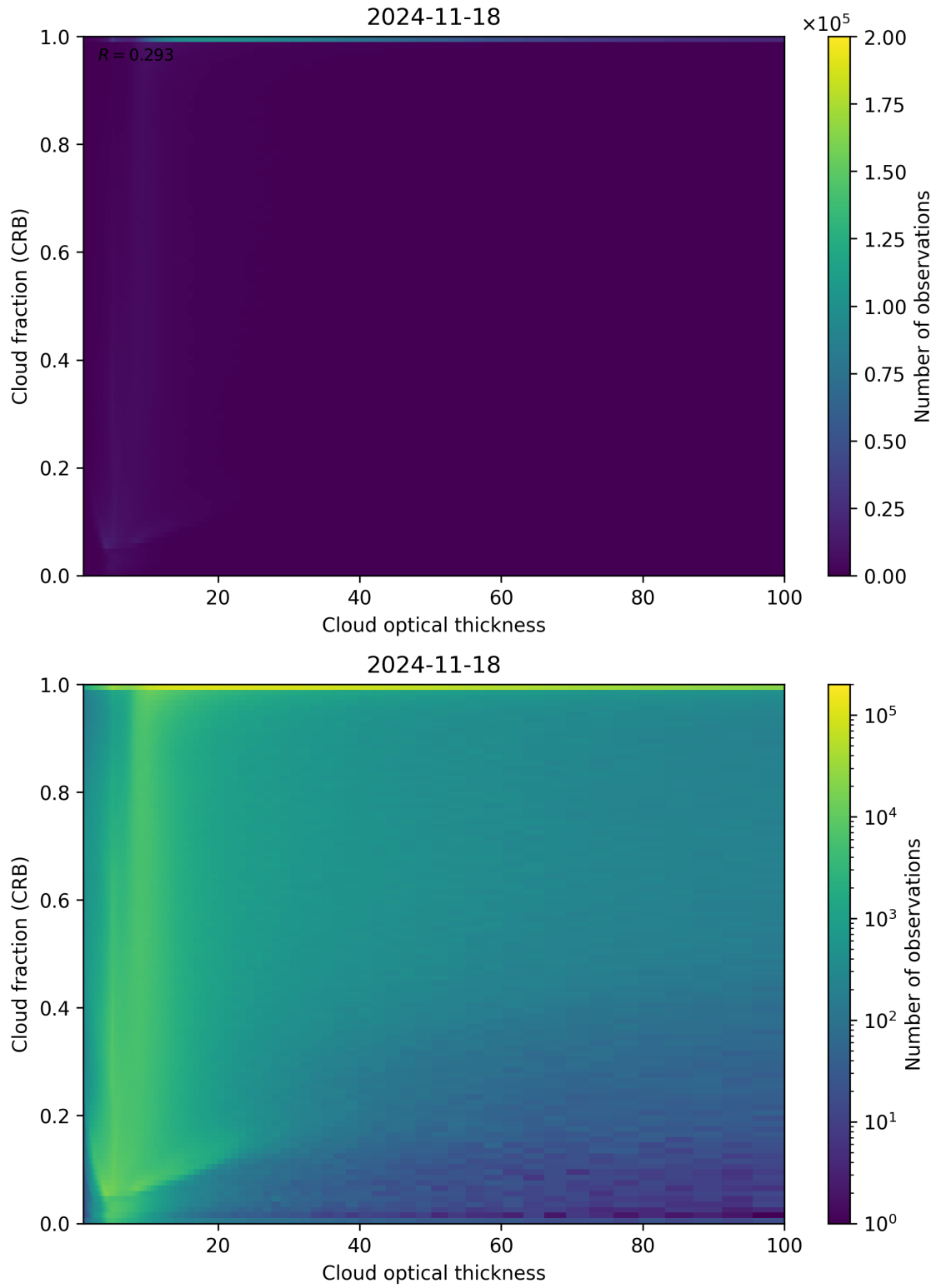
Figure 84: Scatter density plot of “Cloud optical thickness” against “Cloud fraction (CRB)” for 2024-11-17 to 2024-11-19.
