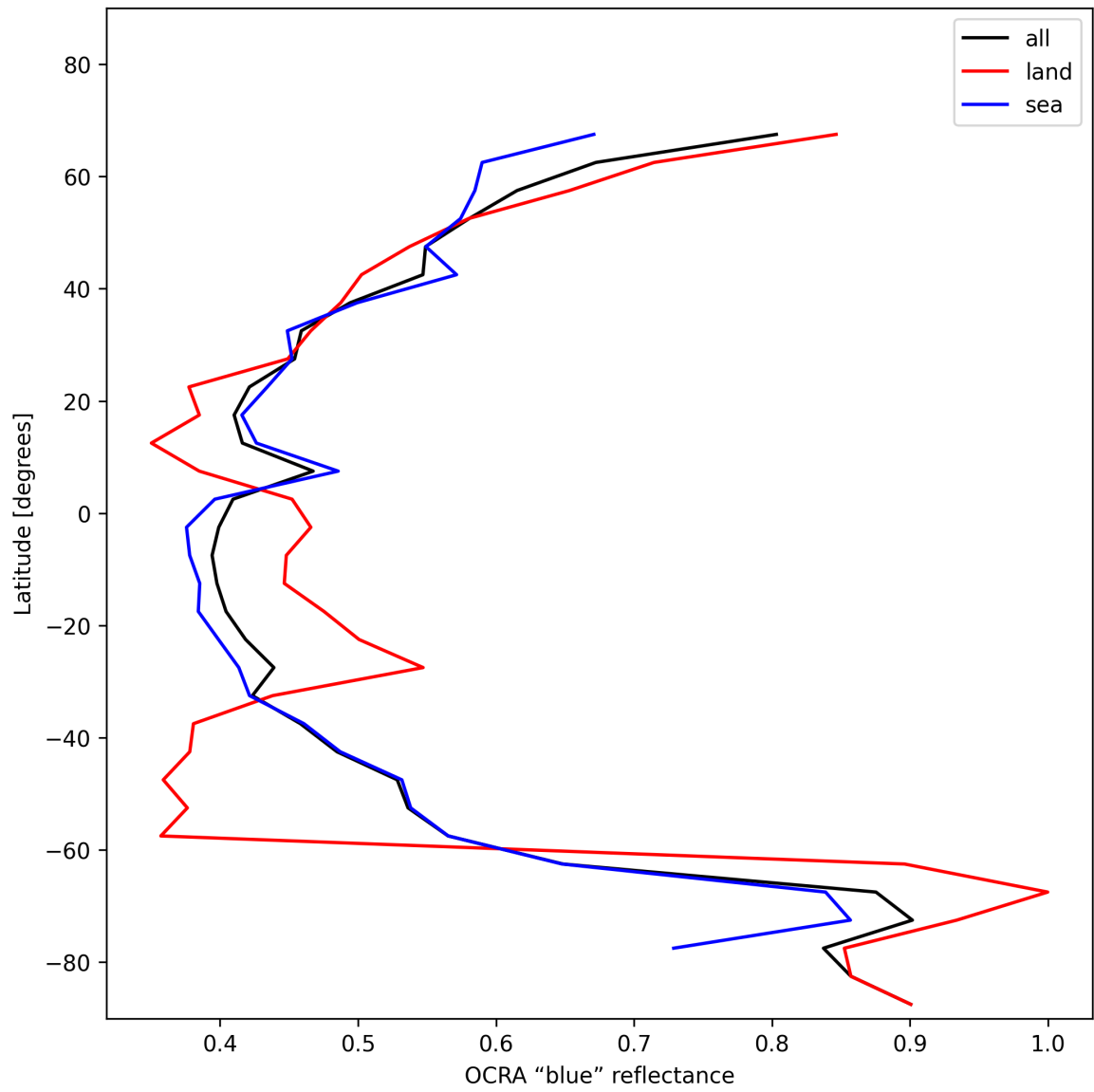
Figure 35: Zonal average of "OCRA "blue" reflectance" for 2024-11-17 to 2024-11-19.
