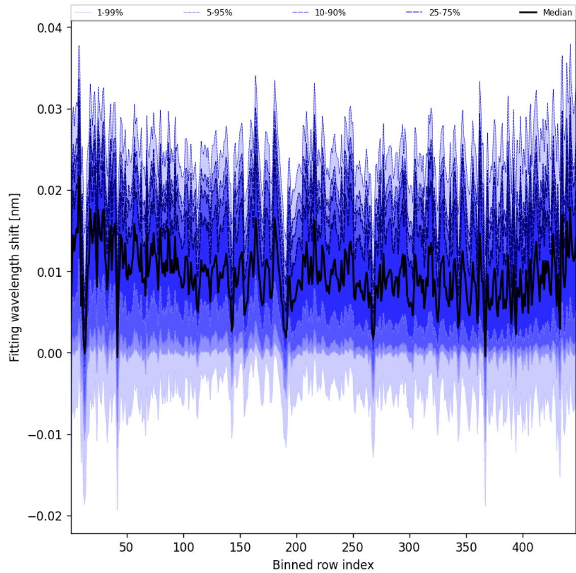
Figure 65: Along track statistics of “Fitting wavelength shift” for 2024-11-17 to 2024-11-19
