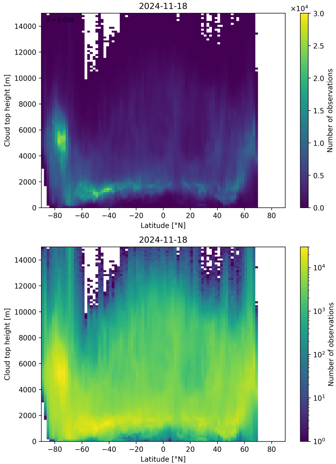
Figure 97: Scatter density plot of “Latitude” against “Cloud top height” for 2024-11-17 to 2024-11-19.
