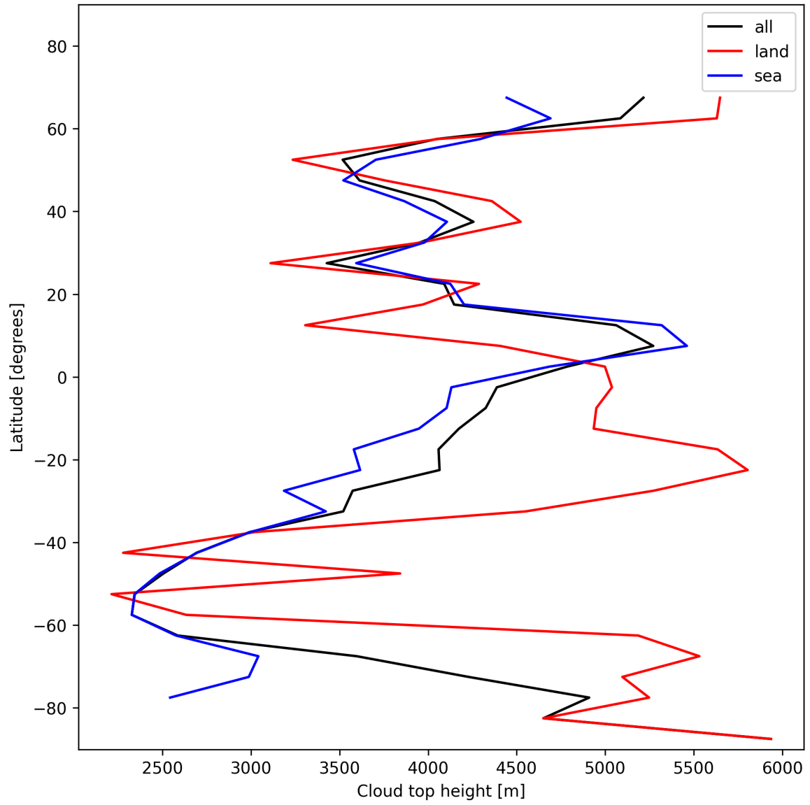
Figure 24: Zonal average of “Cloud top height” for 2024-11-17 to 2024-11-19.
