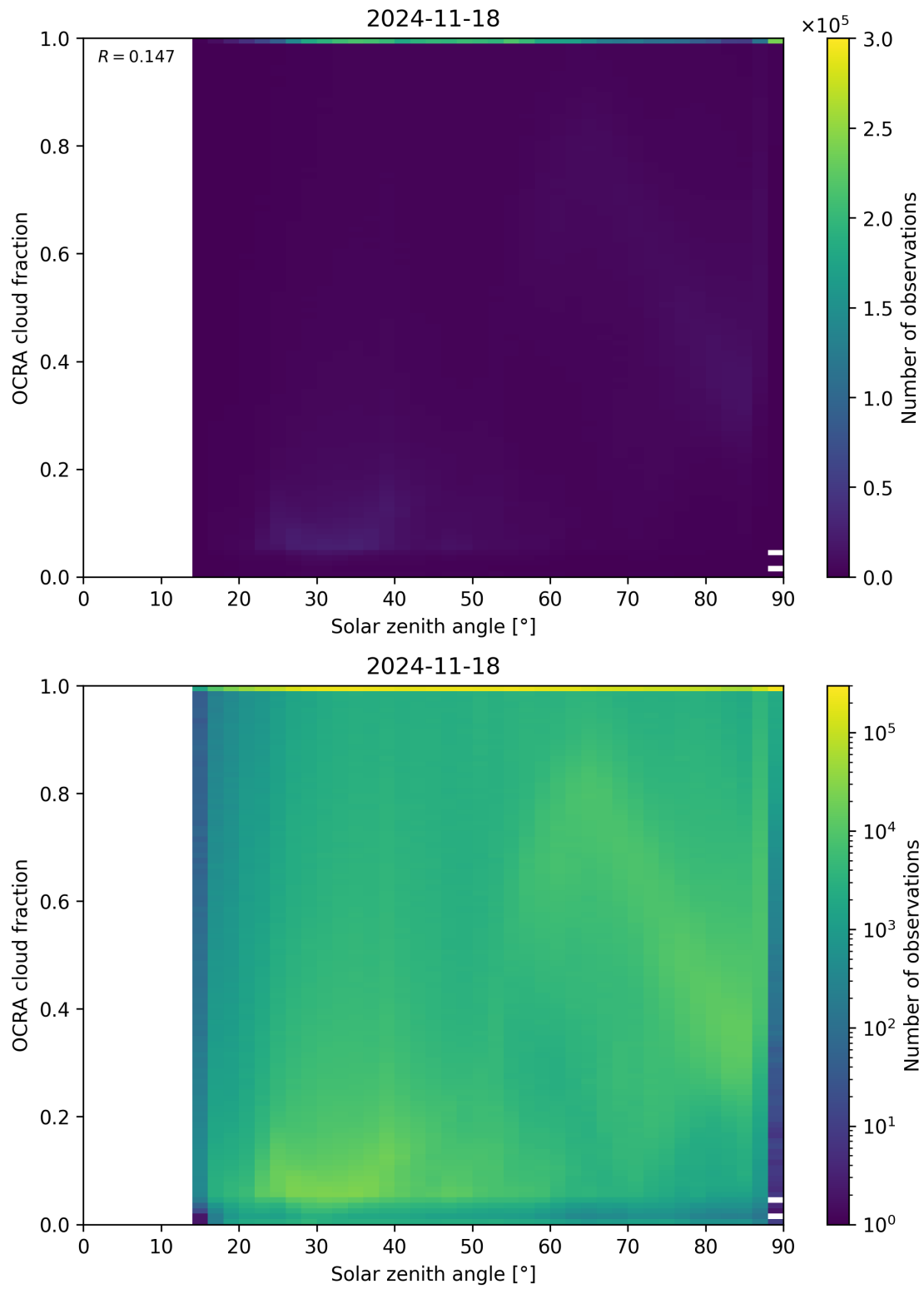
Figure 100: Scatter density plot of “Solar zenith angle” against “OCRA cloud fraction” for 2024-11-17 to 2024-11-19.
