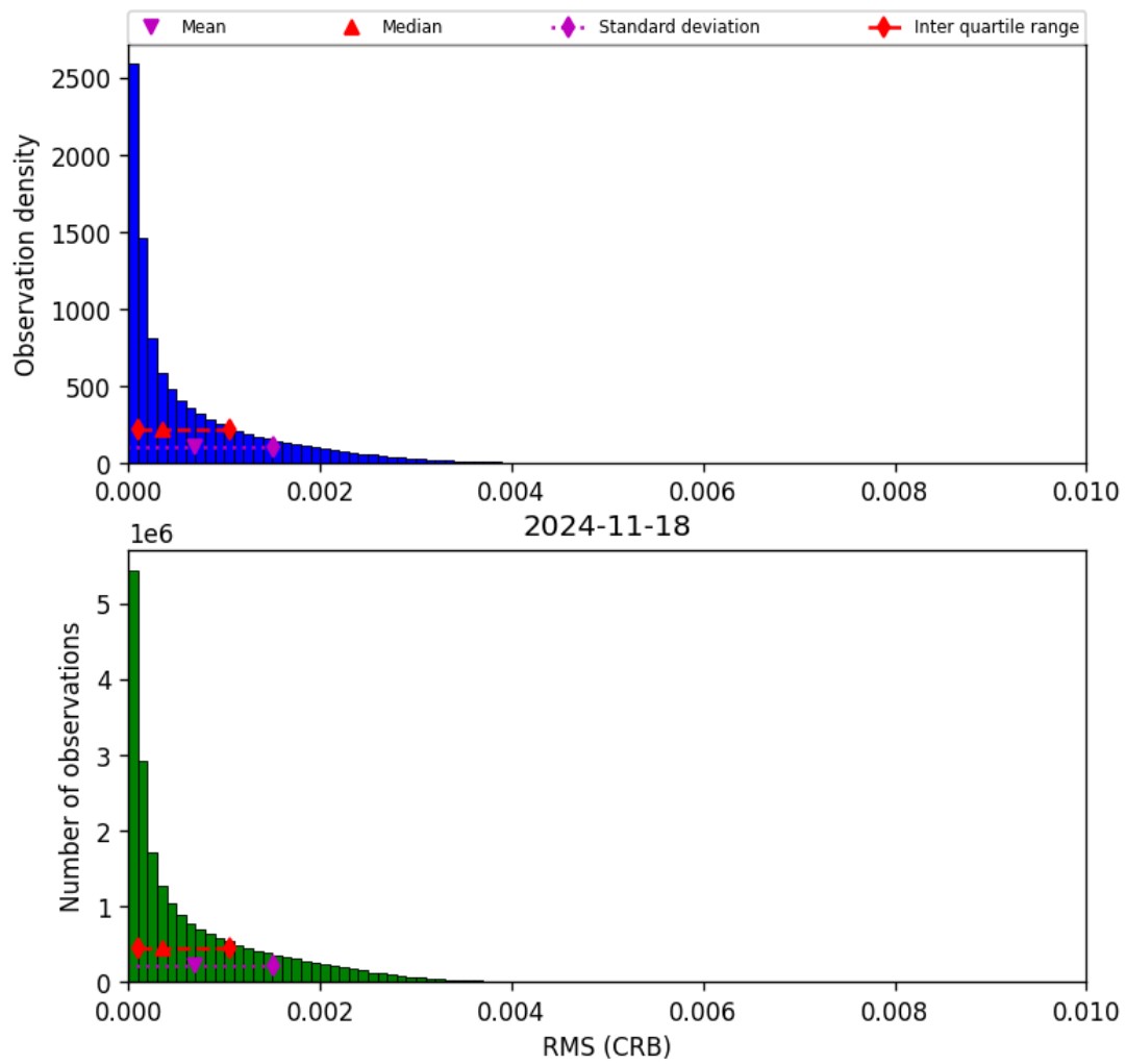
Figure 48: Histogram of “RMS (CRB)” for 2024-11-17 to 2024-11-19
