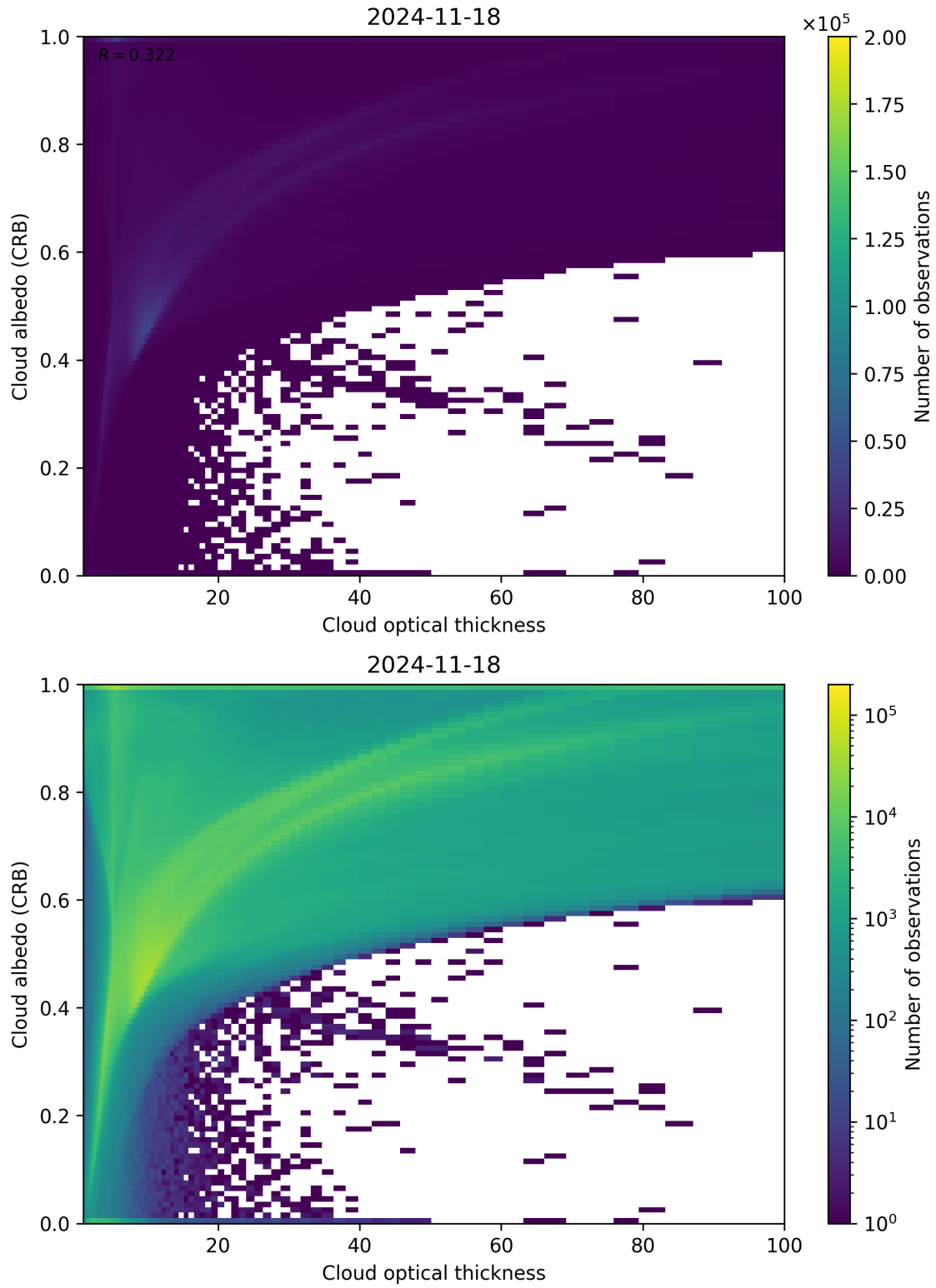
Figure 82: Scatter density plot of “Cloud optical thickness” against “Cloud albedo (CRB)” for 2024-11-17 to 2024-11-19.
