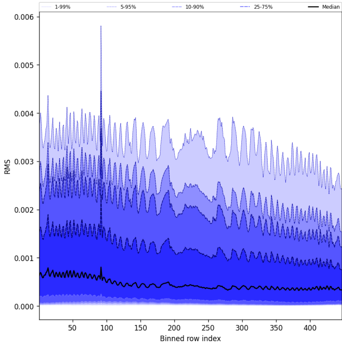
Figure 63: Along track statistics of “RMS” for 2024-11-17 to 2024-11-19
