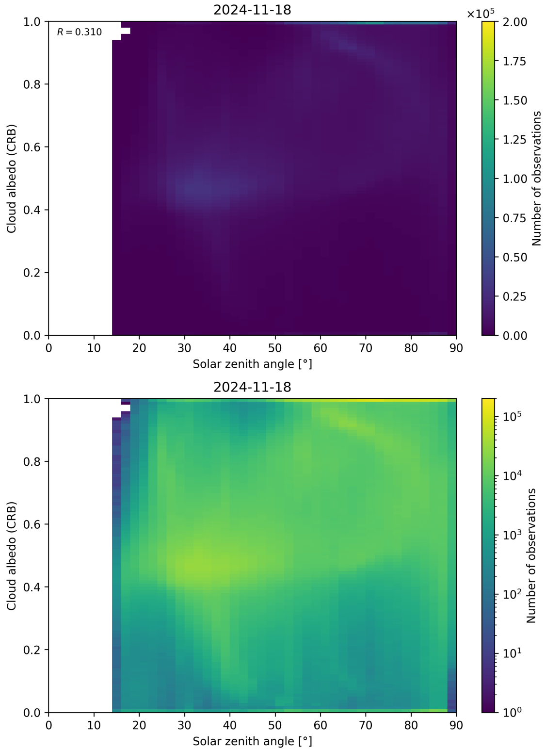
Figure 98: Scatter density plot of “Solar zenith angle” against “Cloud albedo (CRB)” for 2024-11-17 to 2024-11-19.
