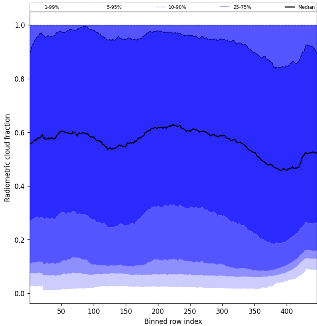
Figure 55: Along track statistics of “Radiometric cloud fraction” for 2024-11-17 to 2024-11-19
