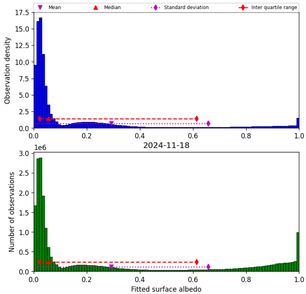
Figure 45: Histogram of “Fitted surface albedo” for 2024-11-17 to 2024-11-19
