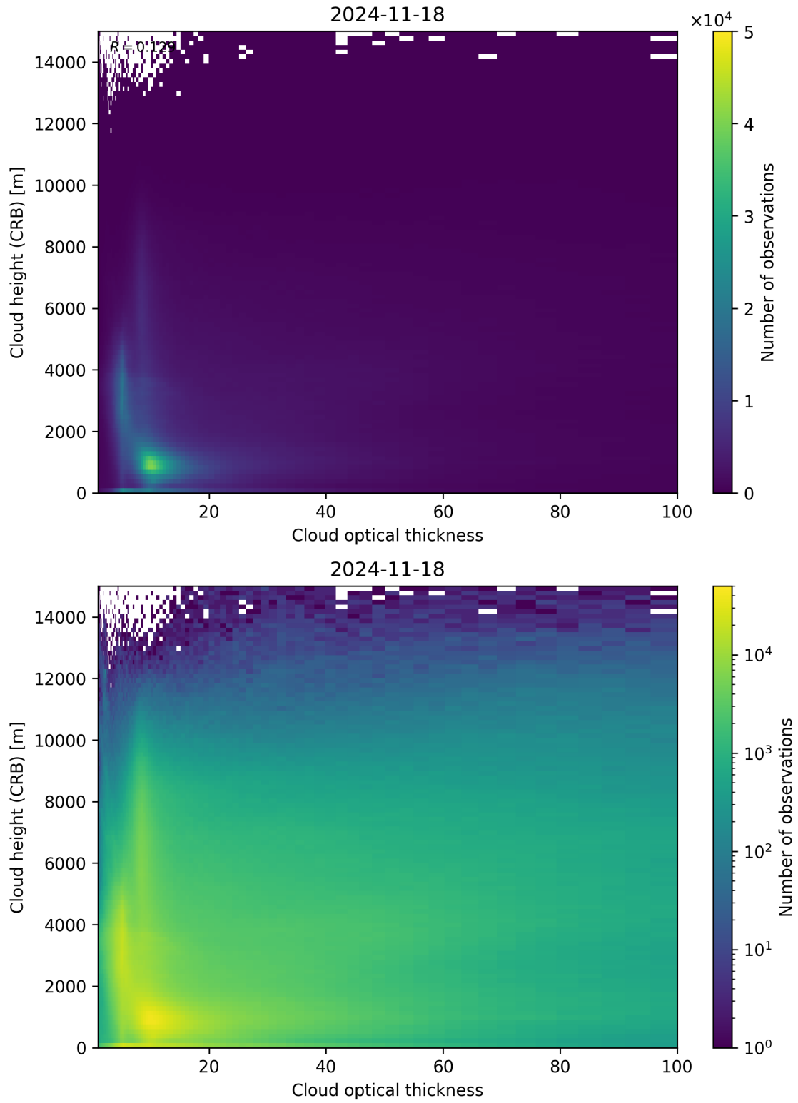
Figure 85: Scatter density plot of “Cloud optical thickness” against “Cloud height (CRB)” for 2024-11-17 to 2024-11-19.
