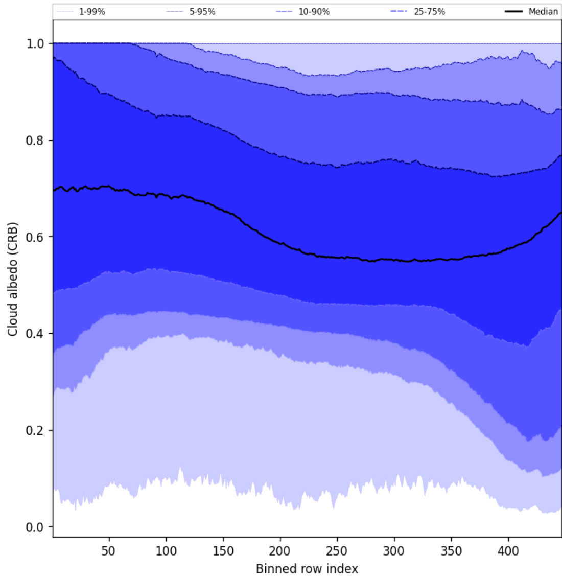
Figure 60: Along track statistics of “Cloud albedo (CRB)” for 2024-11-17 to 2024-11-19
