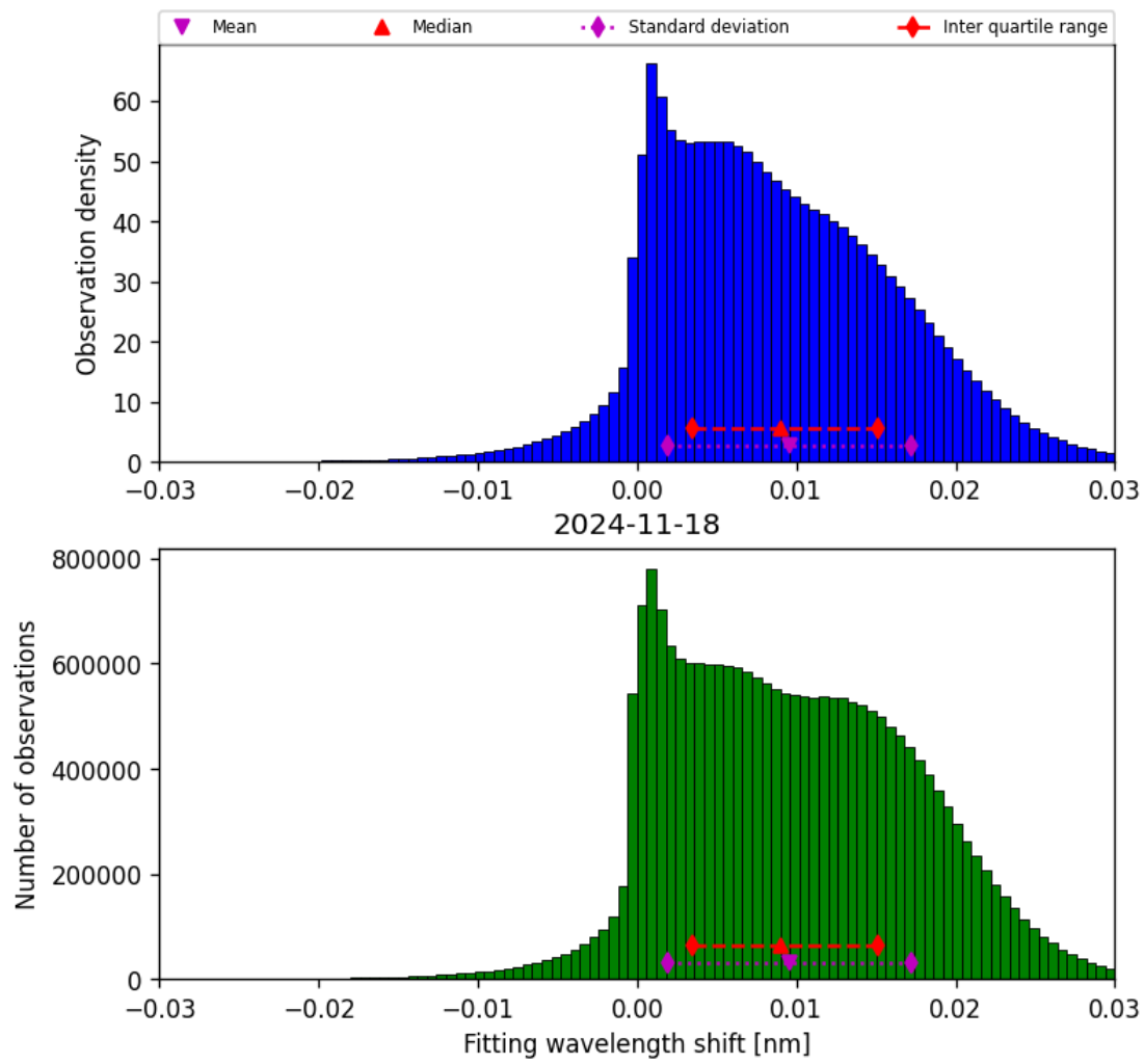
Figure 49: Histogram of “Fitting wavelength shift” for 2024-11-17 to 2024-11-19
