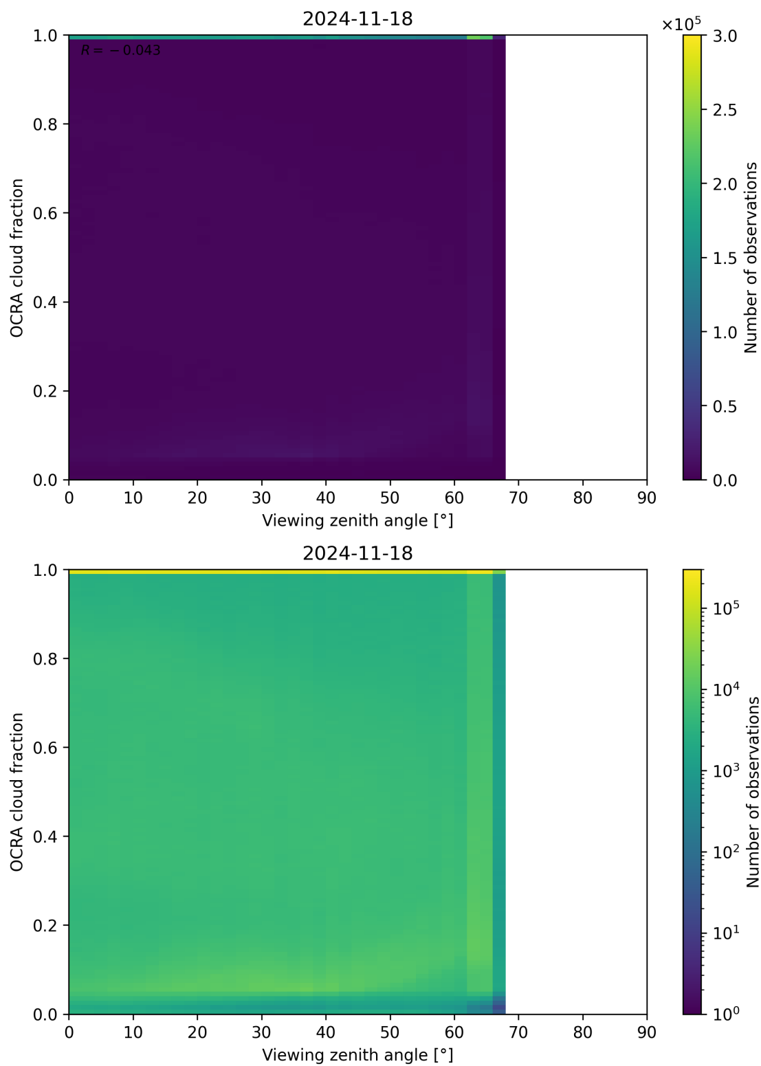
Figure 108: Scatter density plot of “Viewing zenith angle” against “OCRA cloud fraction” for 2024-11-17 to 2024-11-19.
