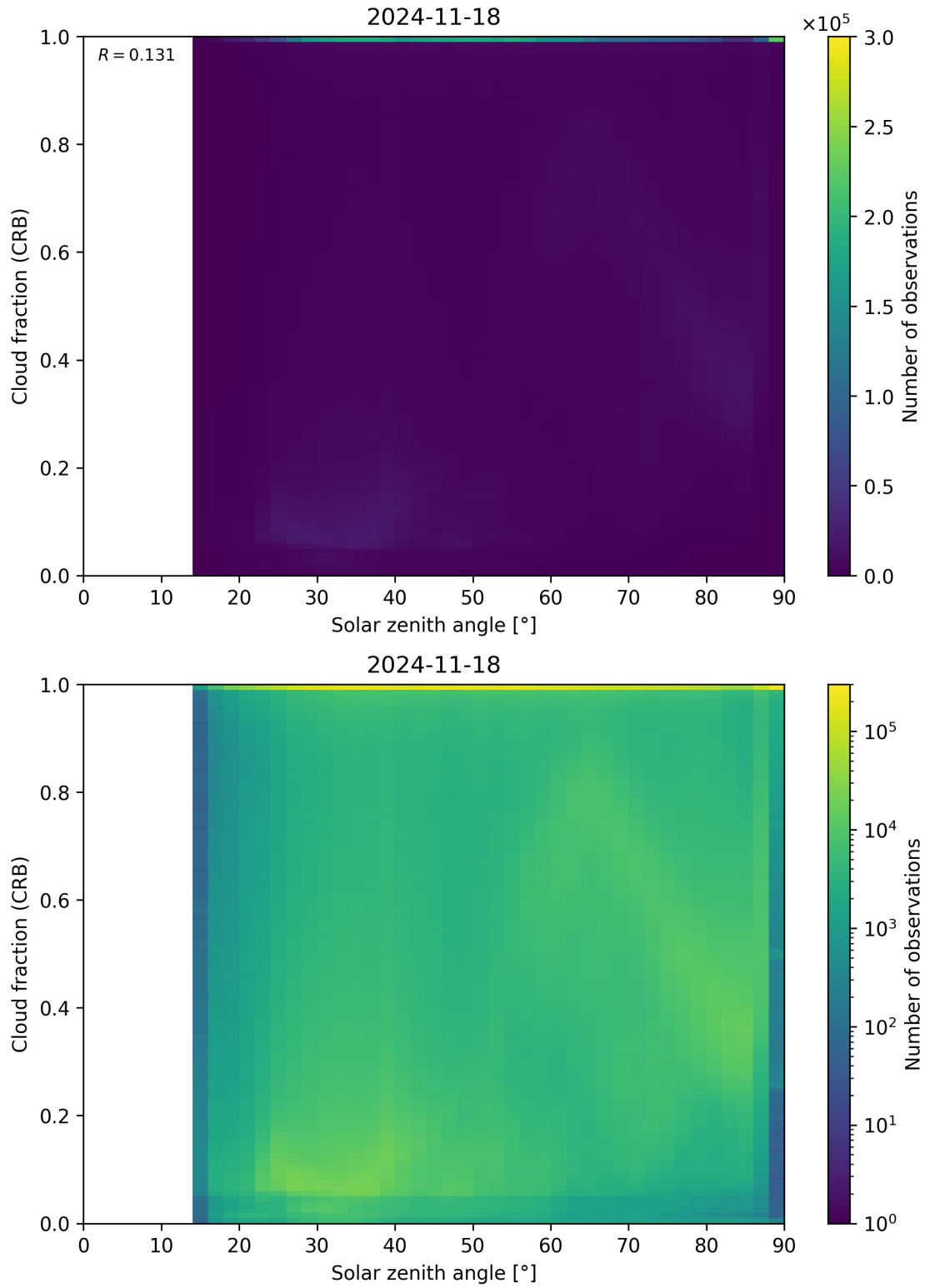
Figure 101: Scatter density plot of “Solar zenith angle” against “Cloud fraction (CRB)” for 2024-11-17 to 2024-11-19.
