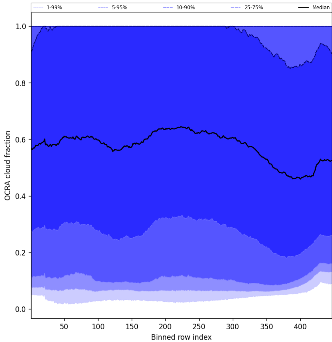
Figure 66: Along track statistics of “OCRA cloud fraction” for 2024-11-17 to 2024-11-19
