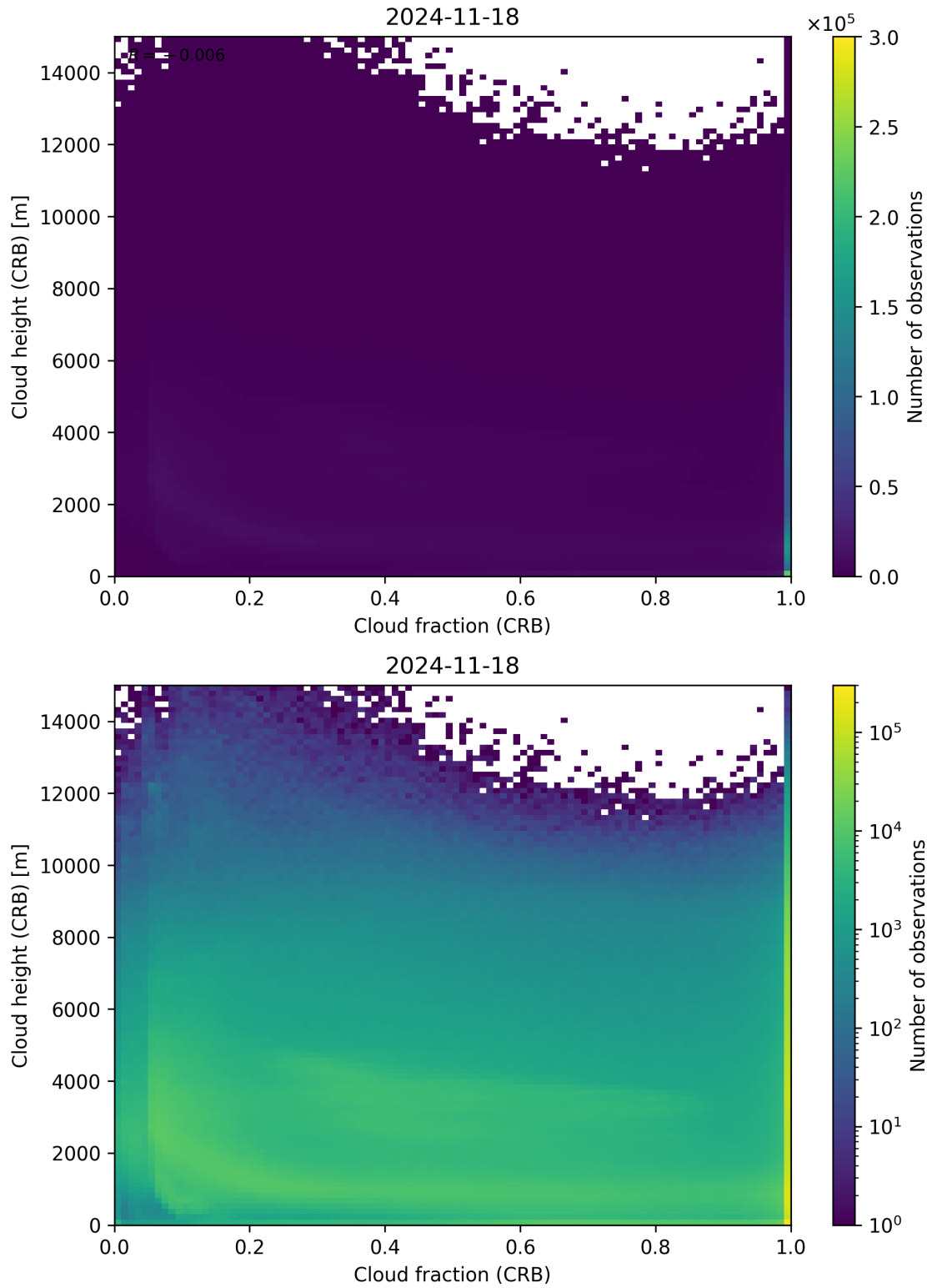
Figure 79: Scatter density plot of “Cloud fraction (CRB)” against “Cloud height (CRB)” for 2024-11-17 to 2024-11-19.
