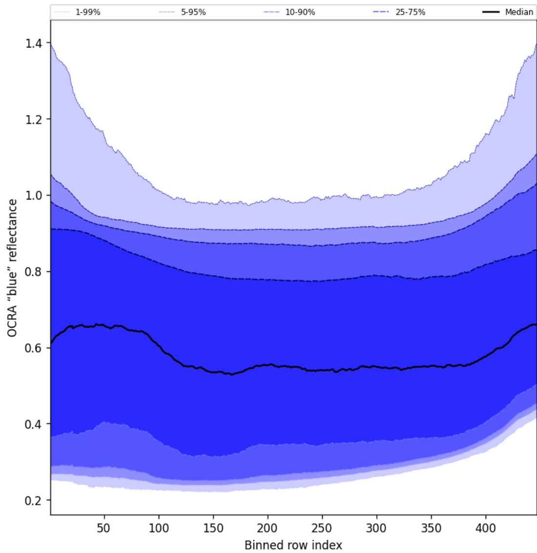
Figure 67: Along track statistics of “OCRA “blue” reflectance” for 2024-11-17 to 2024-11-19
