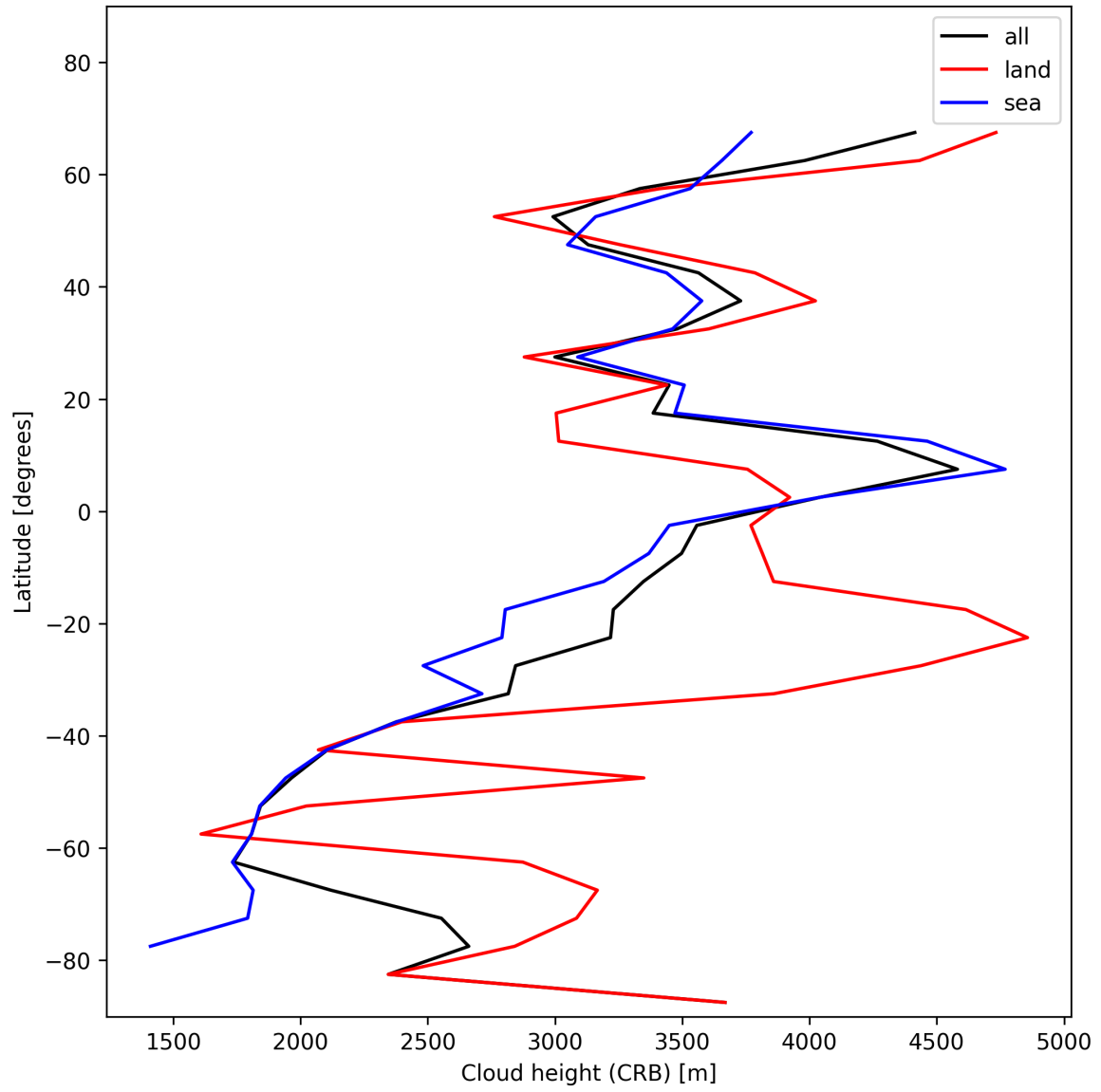
Figure 27: Zonal average of “Cloud height (CRB)” for 2024-11-17 to 2024-11-19.
