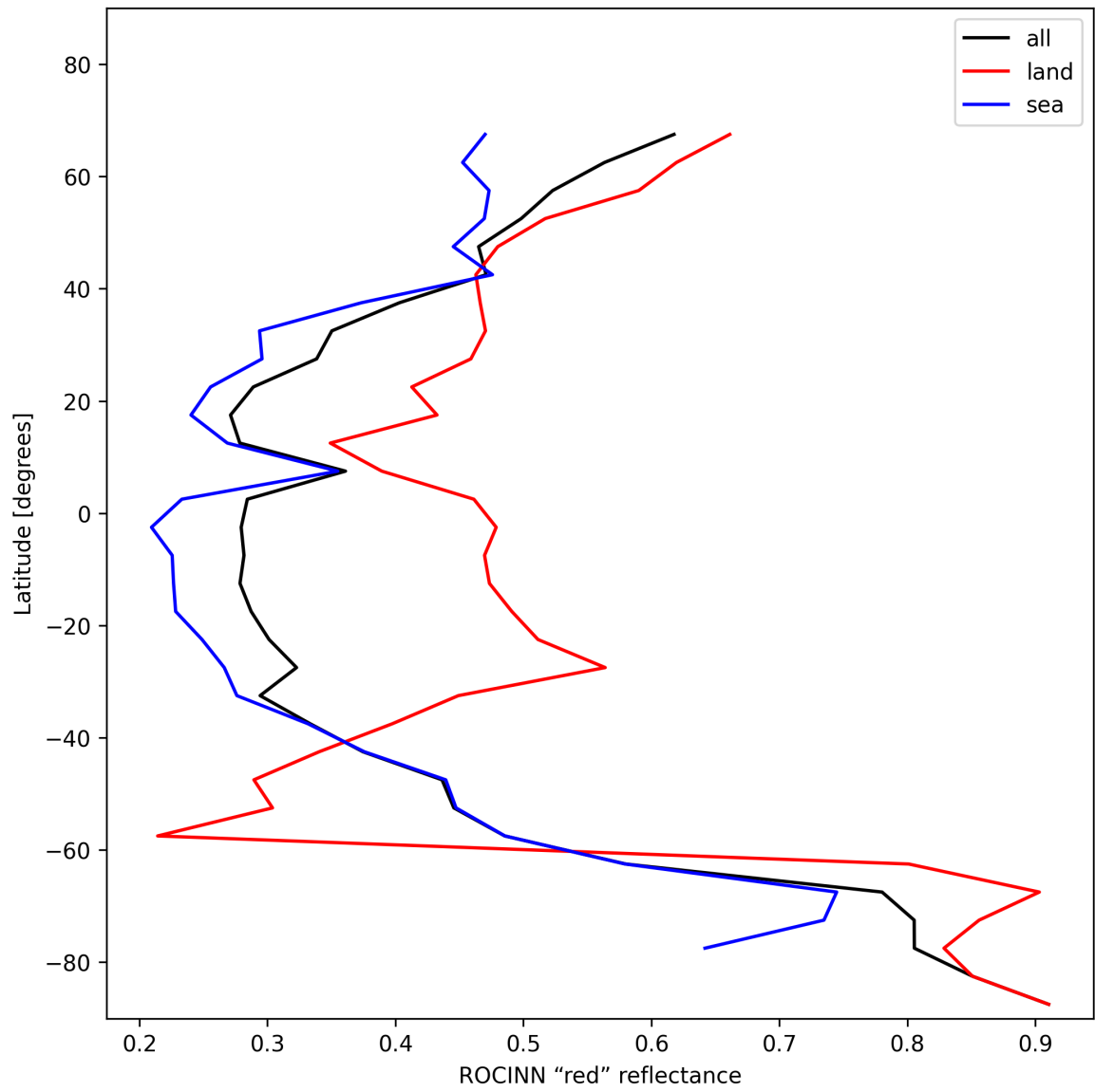
Figure 37: Zonal average of “ROCINN “red” reflectance” for 2024-11-17 to 2024-11-19.
