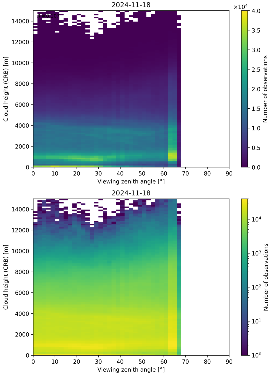
Figure 110: Scatter density plot of “Viewing zenith angle” against “Cloud height (CRB)” for 2024-11-17 to 2024-11-19.
