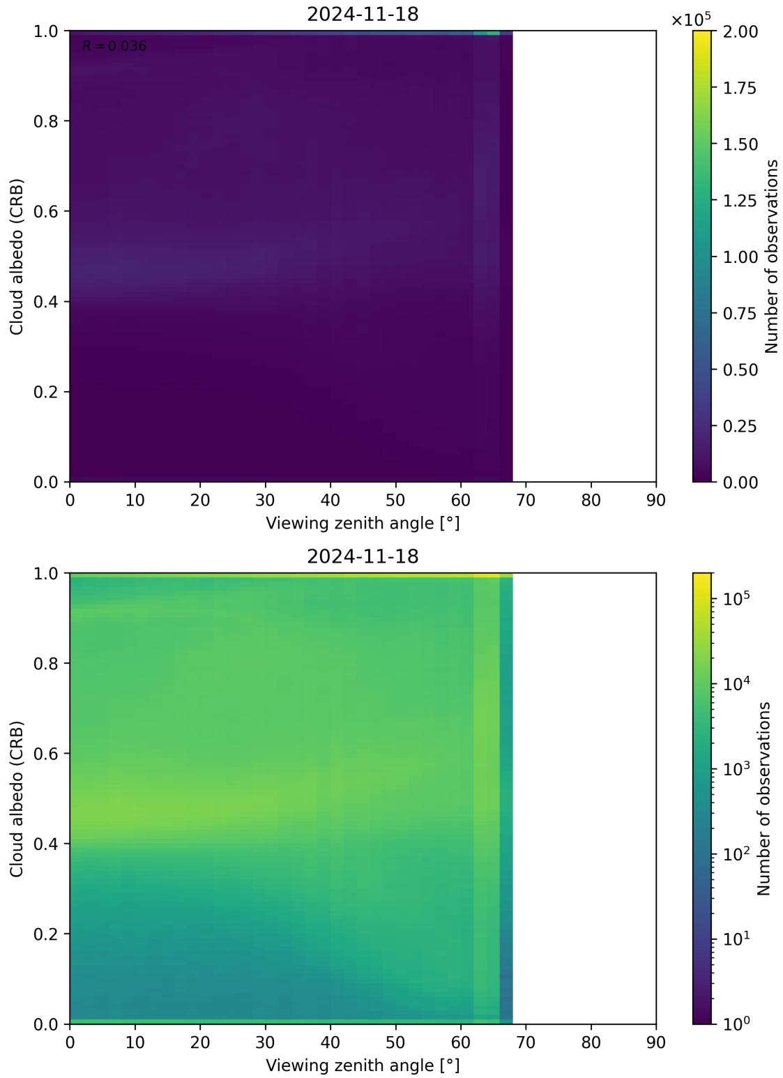
Figure 106: Scatter density plot of “Viewing zenith angle” against “Cloud albedo (CRB)” for 2024-11-17 to 2024-11-19.
