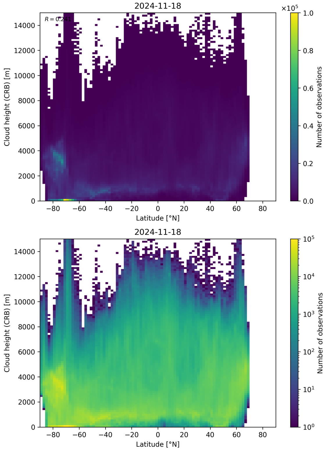
Figure 95: Scatter density plot of “Latitude” against “Cloud height (CRB)” for 2024-11-17 to 2024-11-19.
