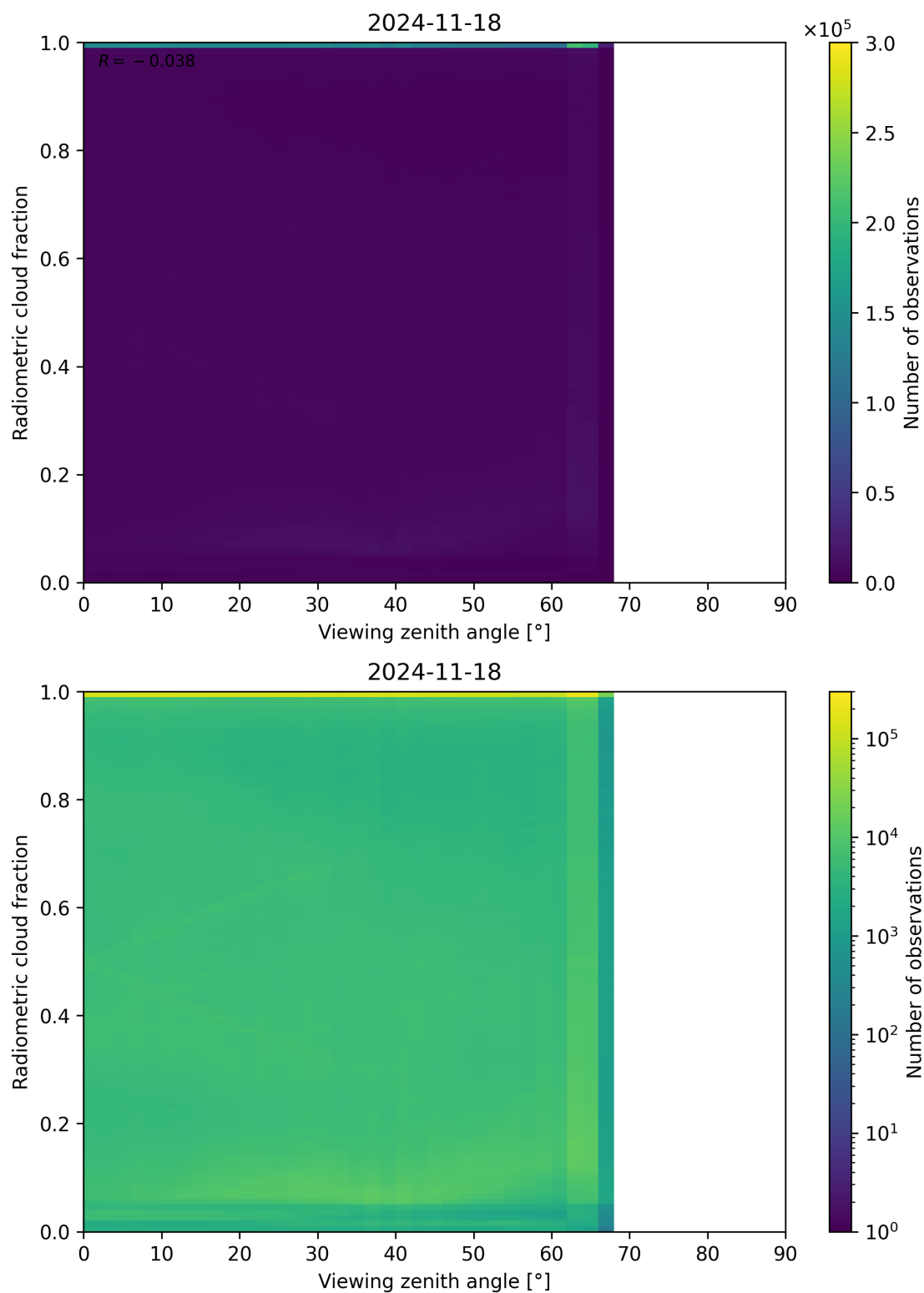
Figure 107: Scatter density plot of “Viewing zenith angle” against “Radiometric cloud fraction” for 2024-11-17 to 2024-11-19.
