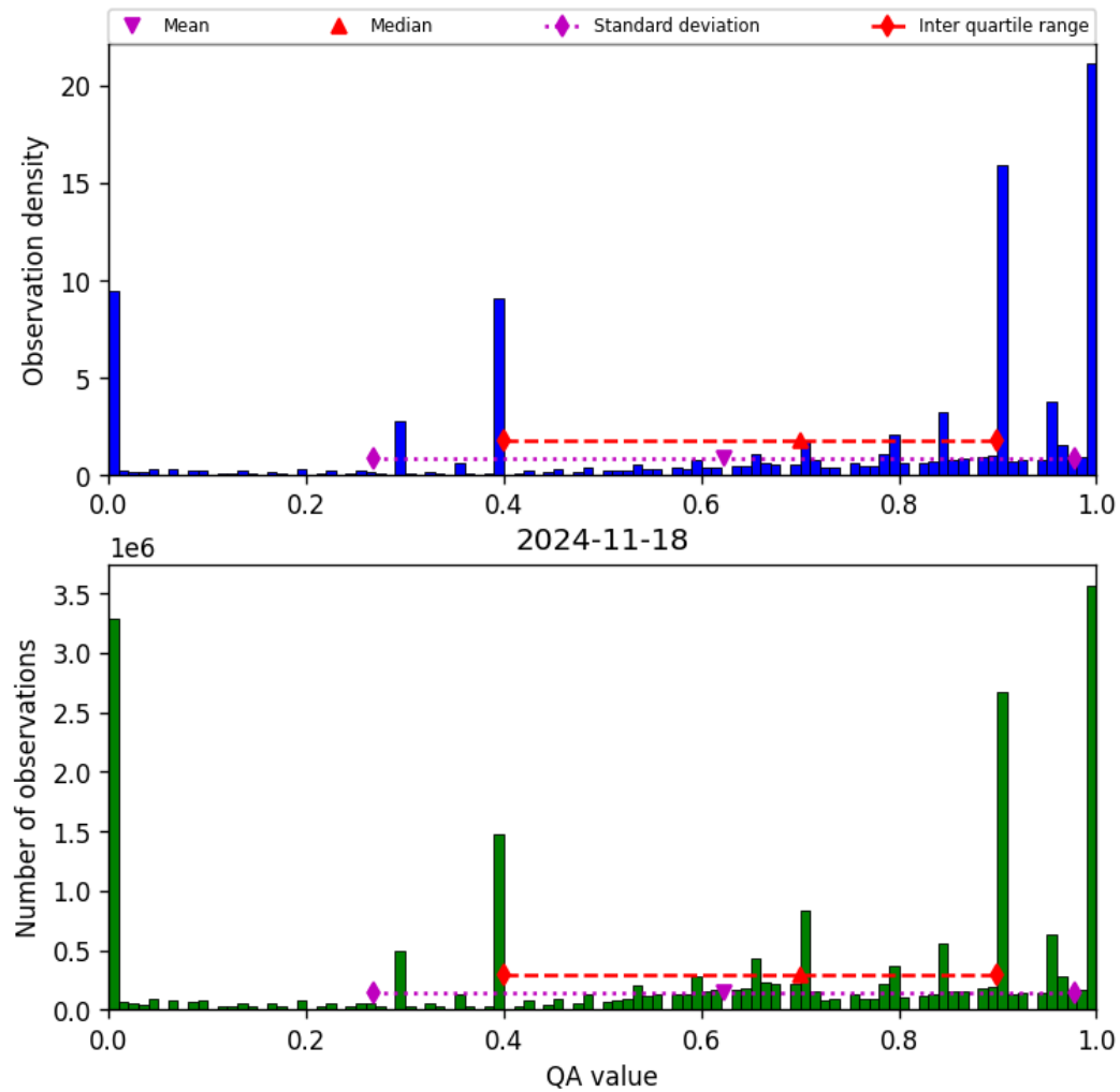
Figure 38: Histogram of “QA value” for 2024-11-17 to 2024-11-19
