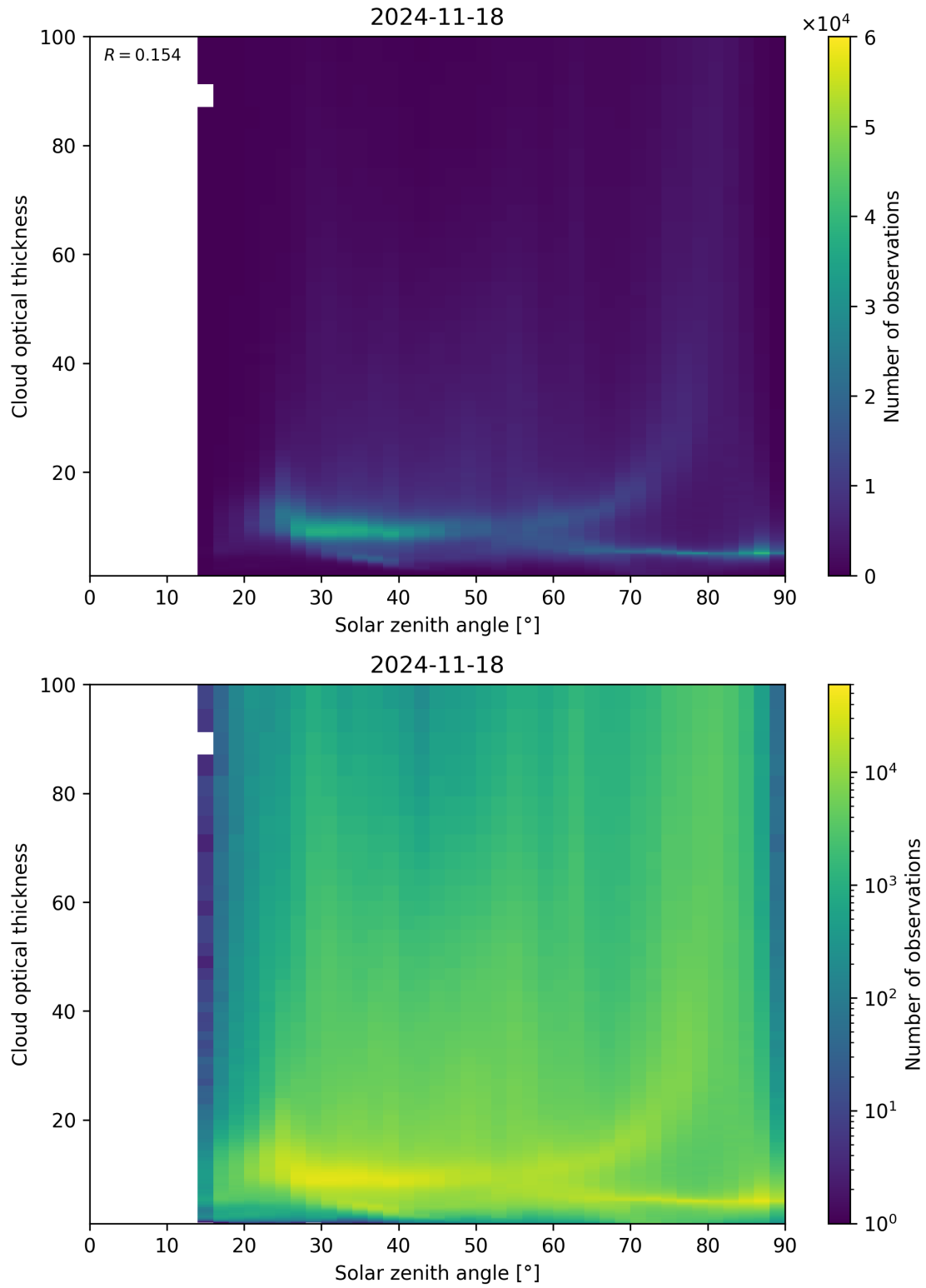
Figure 103: Scatter density plot of “Solar zenith angle” against “Cloud optical thickness” for 2024-11-17 to 2024-11-19.
