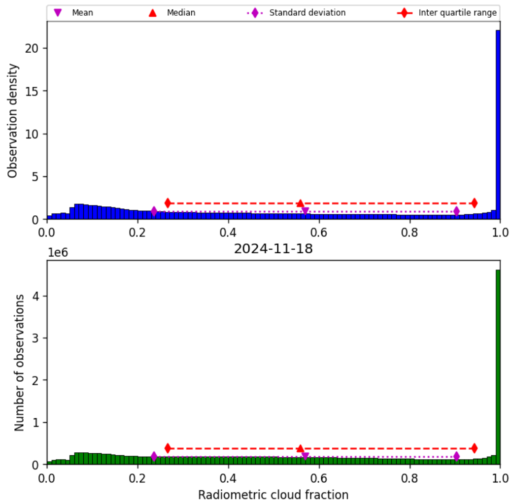
Figure 39: Histogram of “Radiometric cloud fraction” for 2024-11-17 to 2024-11-19
