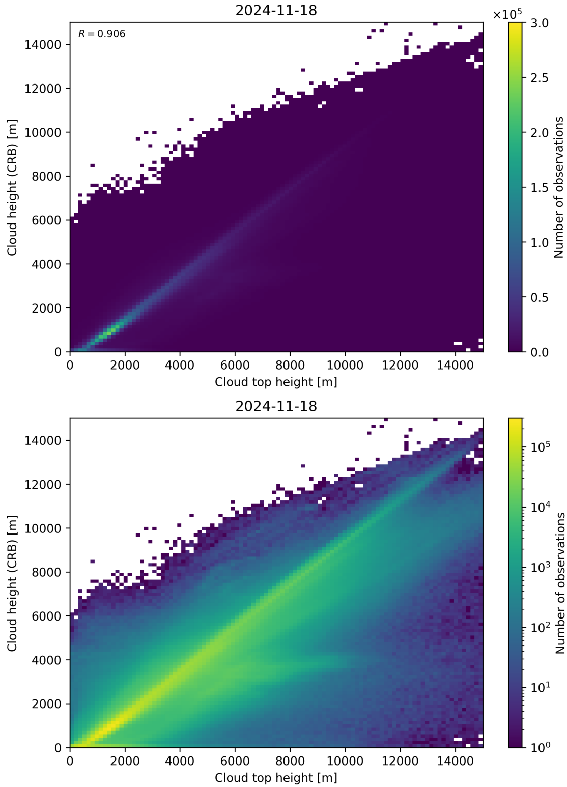
Figure 89: Scatter density plot of “Cloud top height” against “Cloud height (CRB)” for 2024-11-17 to 2024-11-19.
