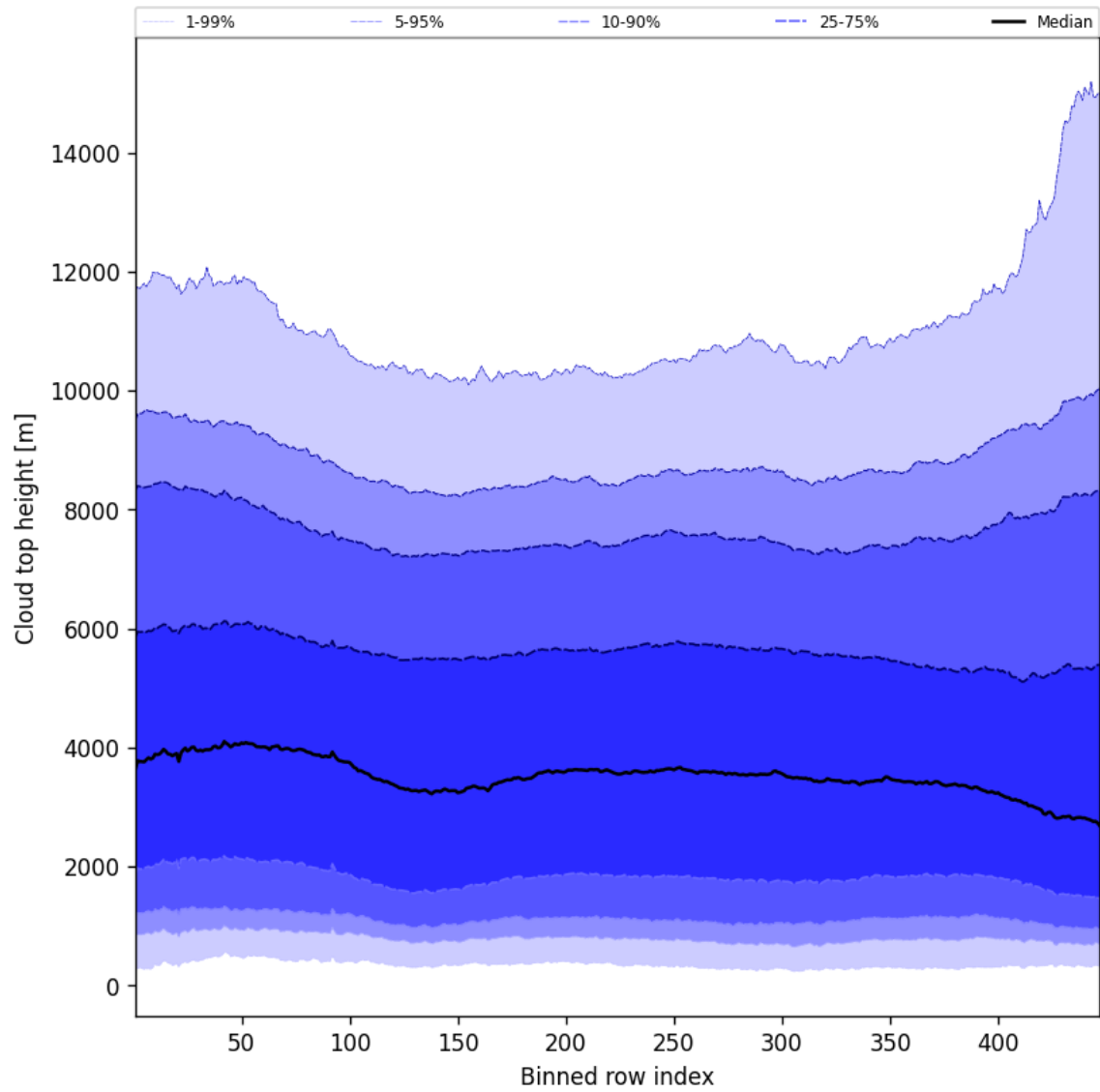
Figure 56: Along track statistics of “Cloud top height” for 2024-11-17 to 2024-11-19
