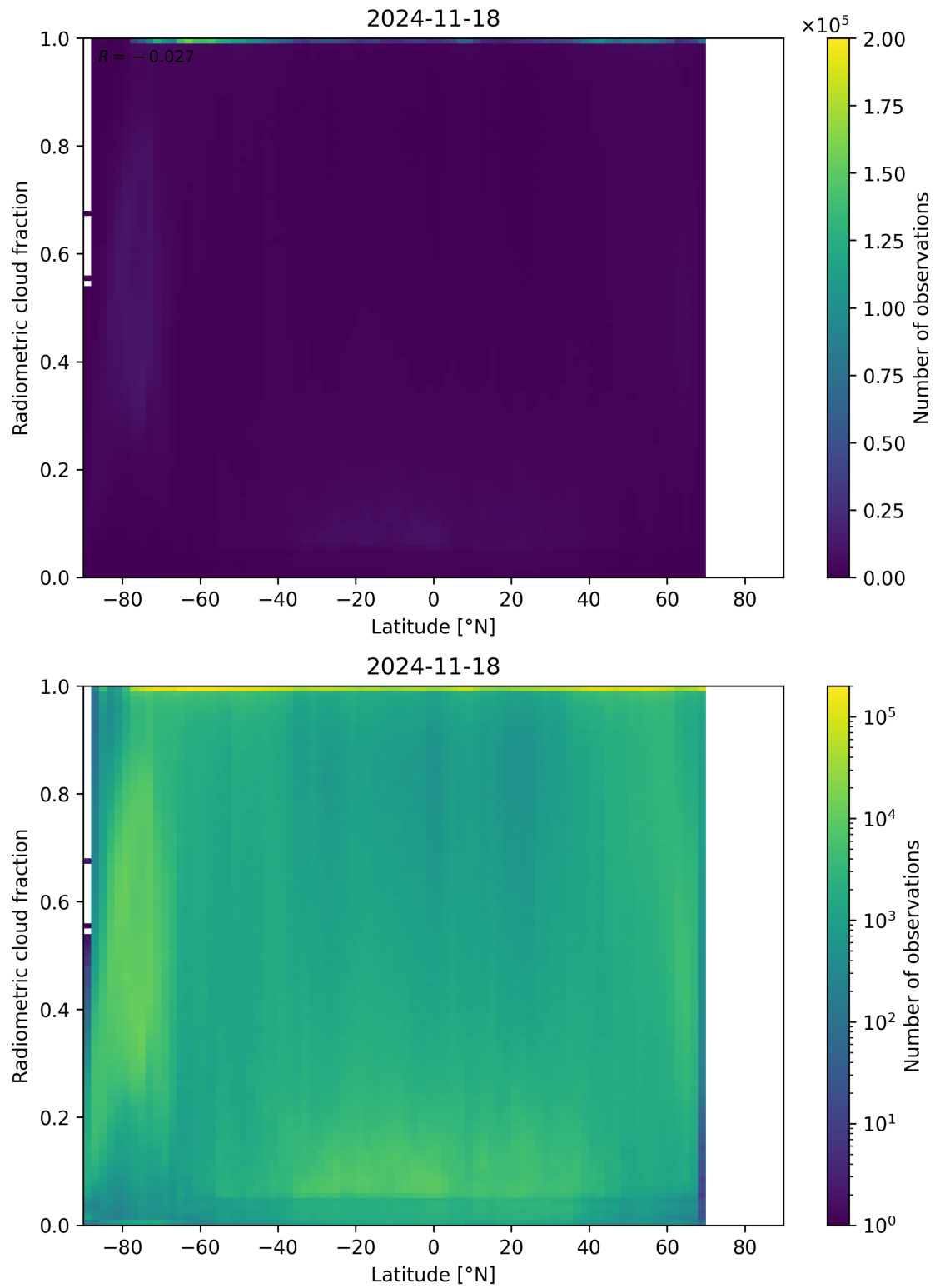
Figure 92: Scatter density plot of “Latitude” against “Radiometric cloud fraction” for 2024-11-17 to 2024-11-19.
