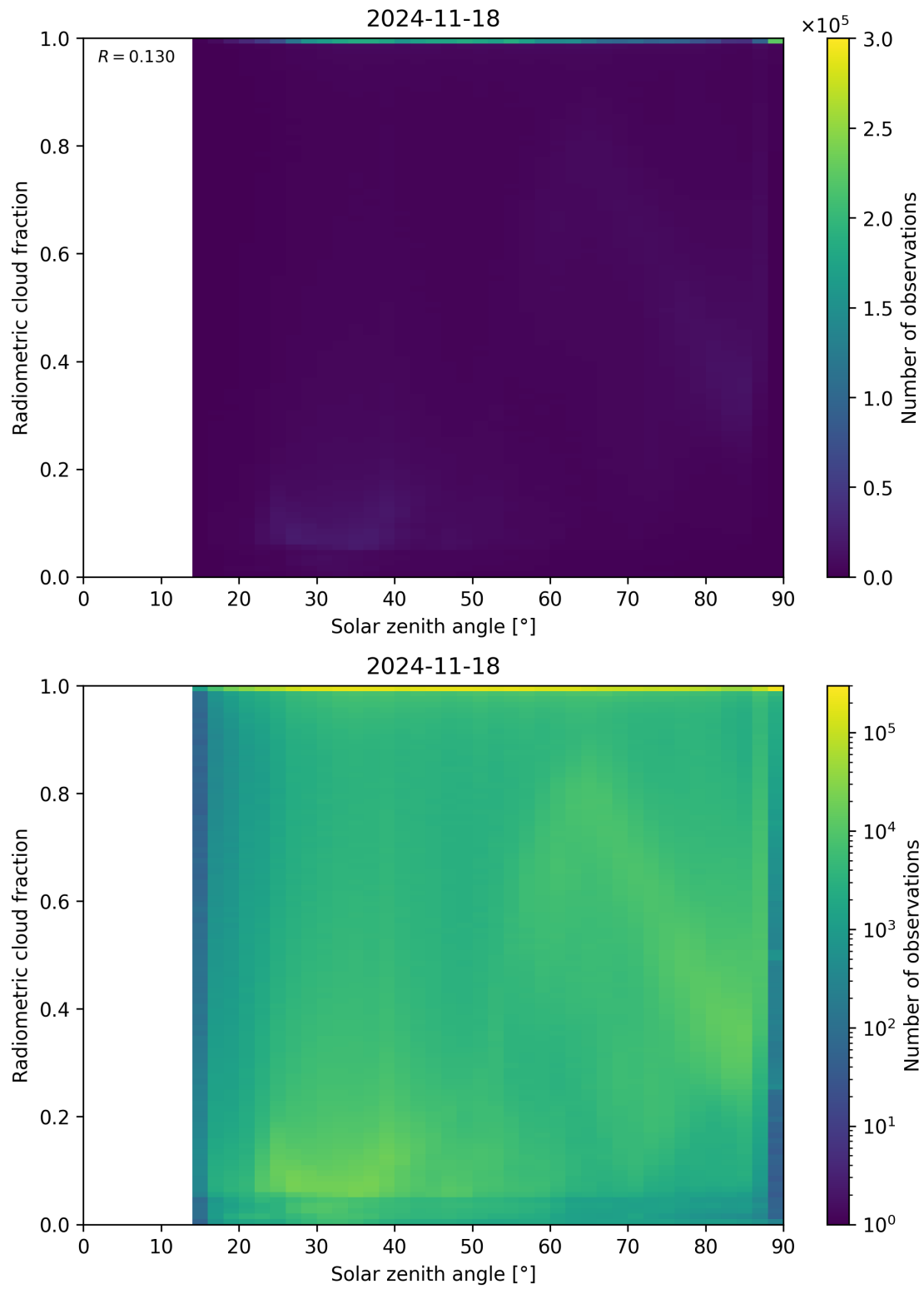
Figure 99: Scatter density plot of “Solar zenith angle” against “Radiometric cloud fraction” for 2024-11-17 to 2024-11-19.
