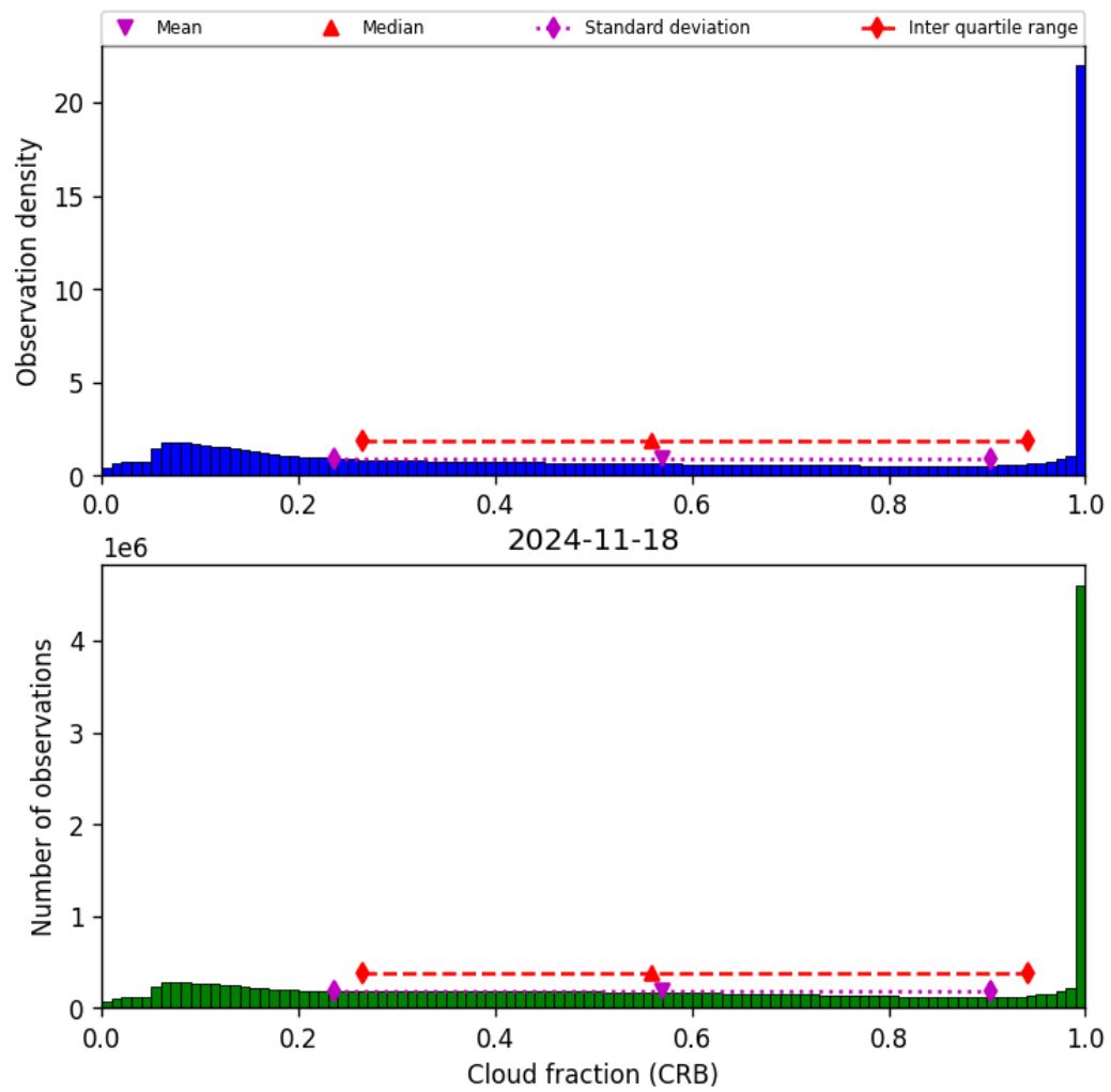
Figure 42: Histogram of “Cloud fraction (CRB)” for 2024-11-17 to 2024-11-19
