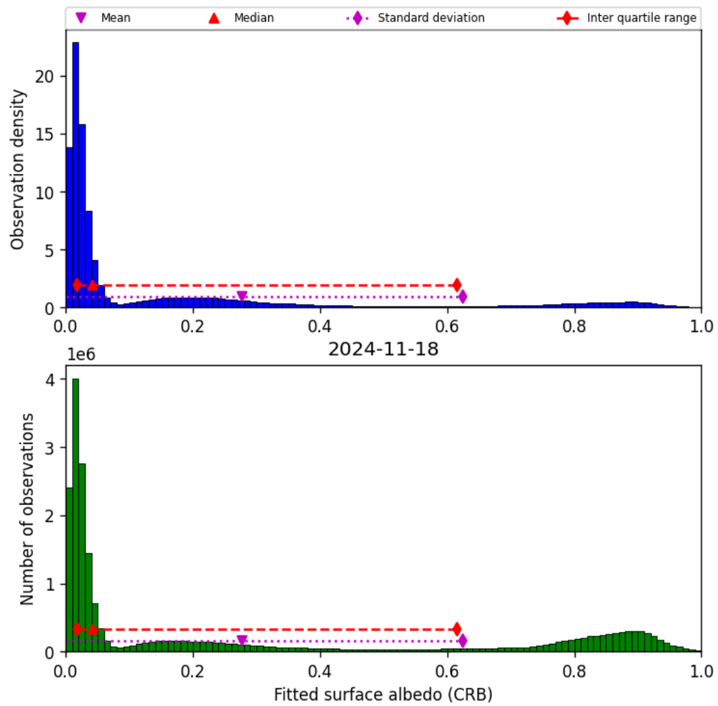
Figure 46: Histogram of “Fitted surface albedo (CRB)” for 2024-11-17 to 2024-11-19
