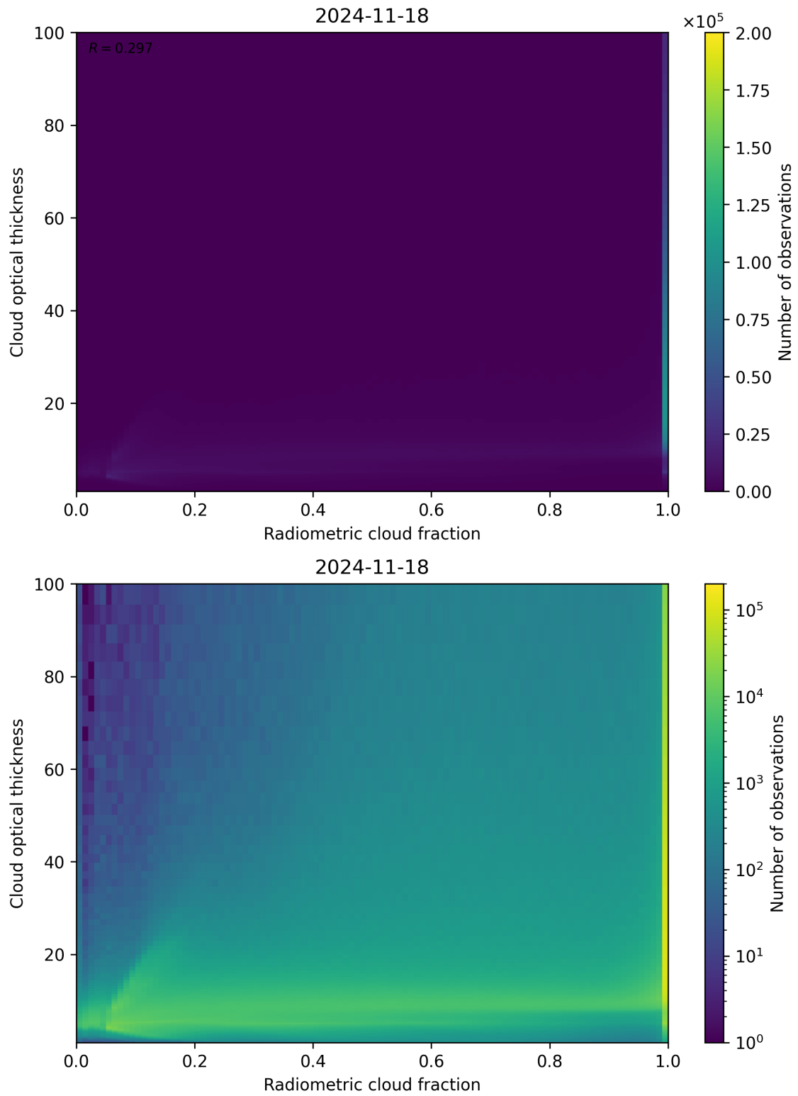
Figure 75: Scatter density plot of “Radiometric cloud fraction” against “Cloud optical thickness” for 2024-11-17 to 2024-11-19.
