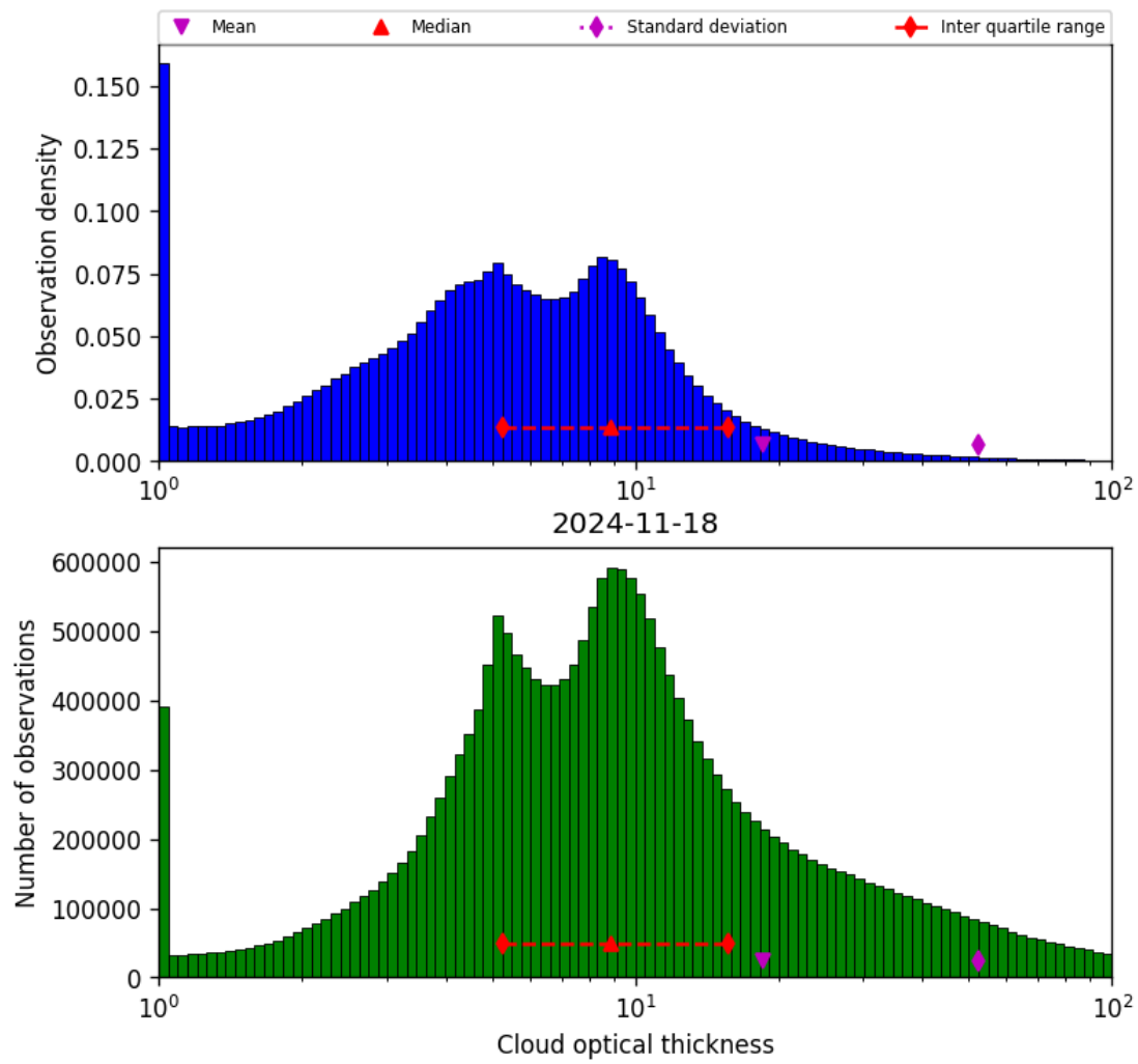
Figure 41: Histogram of “Cloud optical thickness” for 2024-11-17 to 2024-11-19
