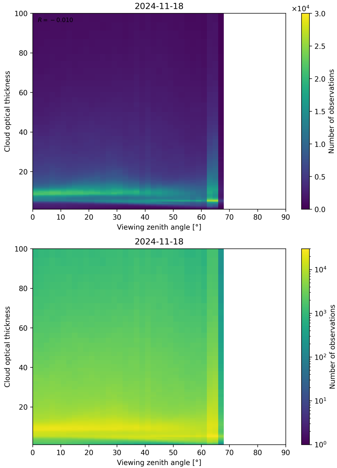
Figure 111: Scatter density plot of “Viewing zenith angle” against “Cloud optical thickness” for 2024-11-17 to 2024-11-19.
