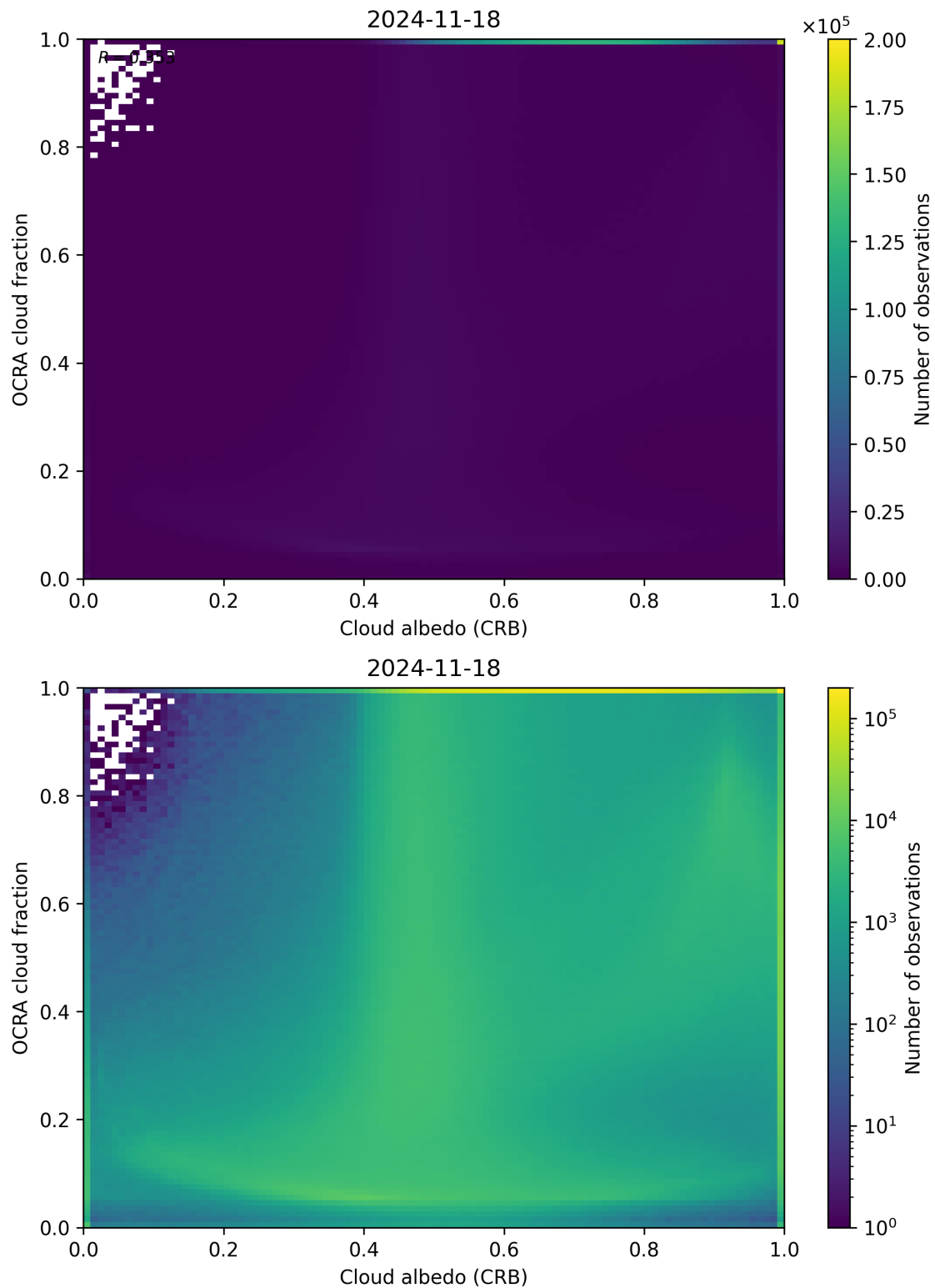
Figure 70: Scatter density plot of “Cloud albedo (CRB)” against “OCRA cloud fraction” for 2024-11-17 to 2024-11-19.
