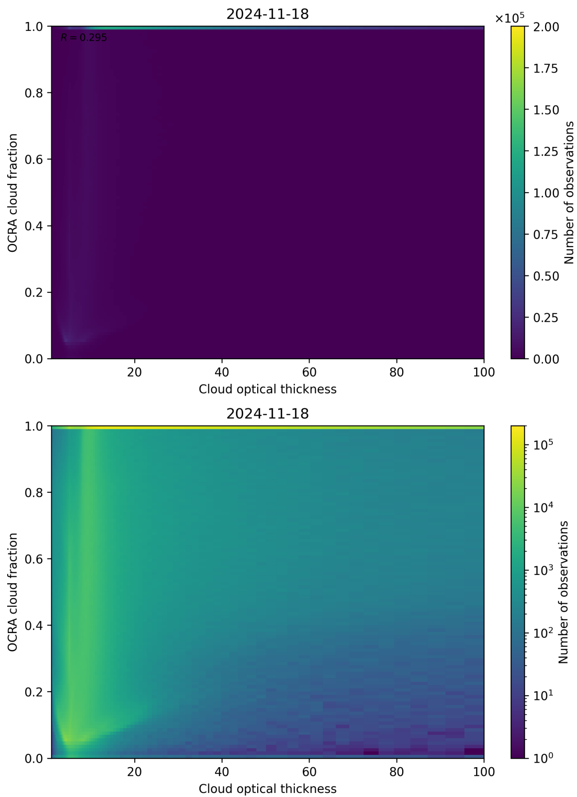
Figure 83: Scatter density plot of “Cloud optical thickness” against “OCRA cloud fraction” for 2024-11-17 to 2024-11-19.
