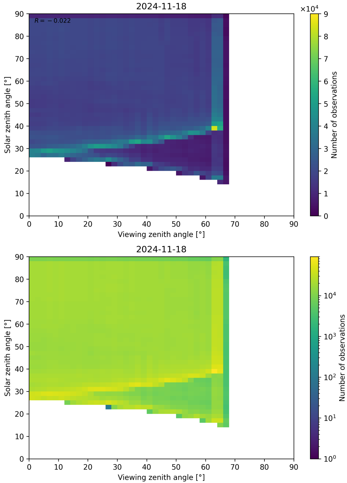
Figure 114: Scatter density plot of “Viewing zenith angle” against “Solar zenith angle” for 2024-11-17 to 2024-11-19.
