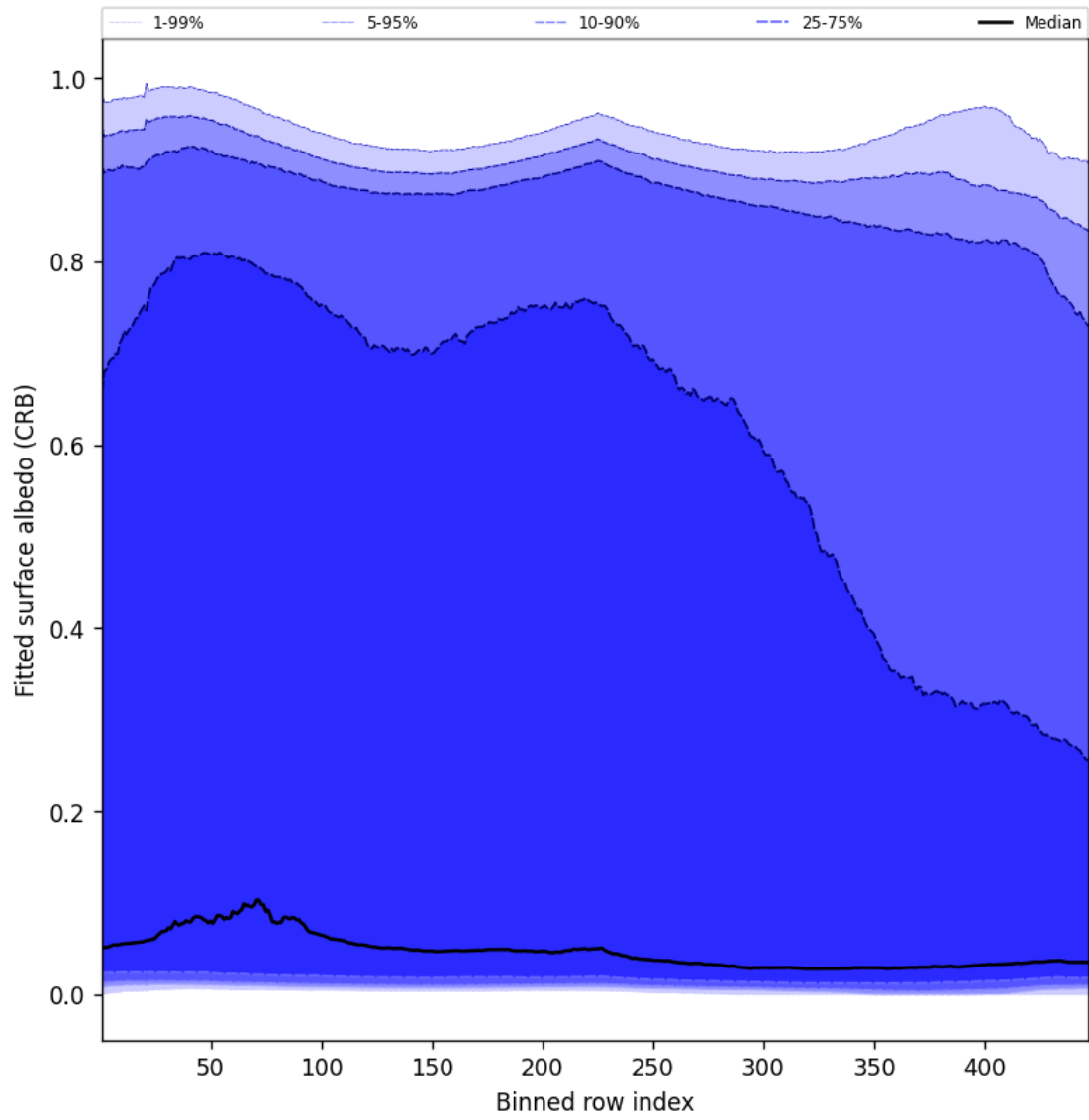
Figure 62: Along track statistics of “Fitted surface albedo (CRB)” for 2024-11-17 to 2024-11-19
