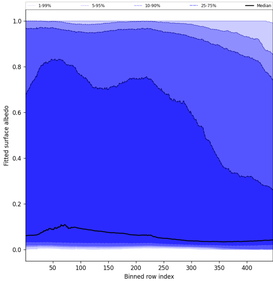
Figure 61: Along track statistics of “Fitted surface albedo” for 2024-11-17 to 2024-11-19
