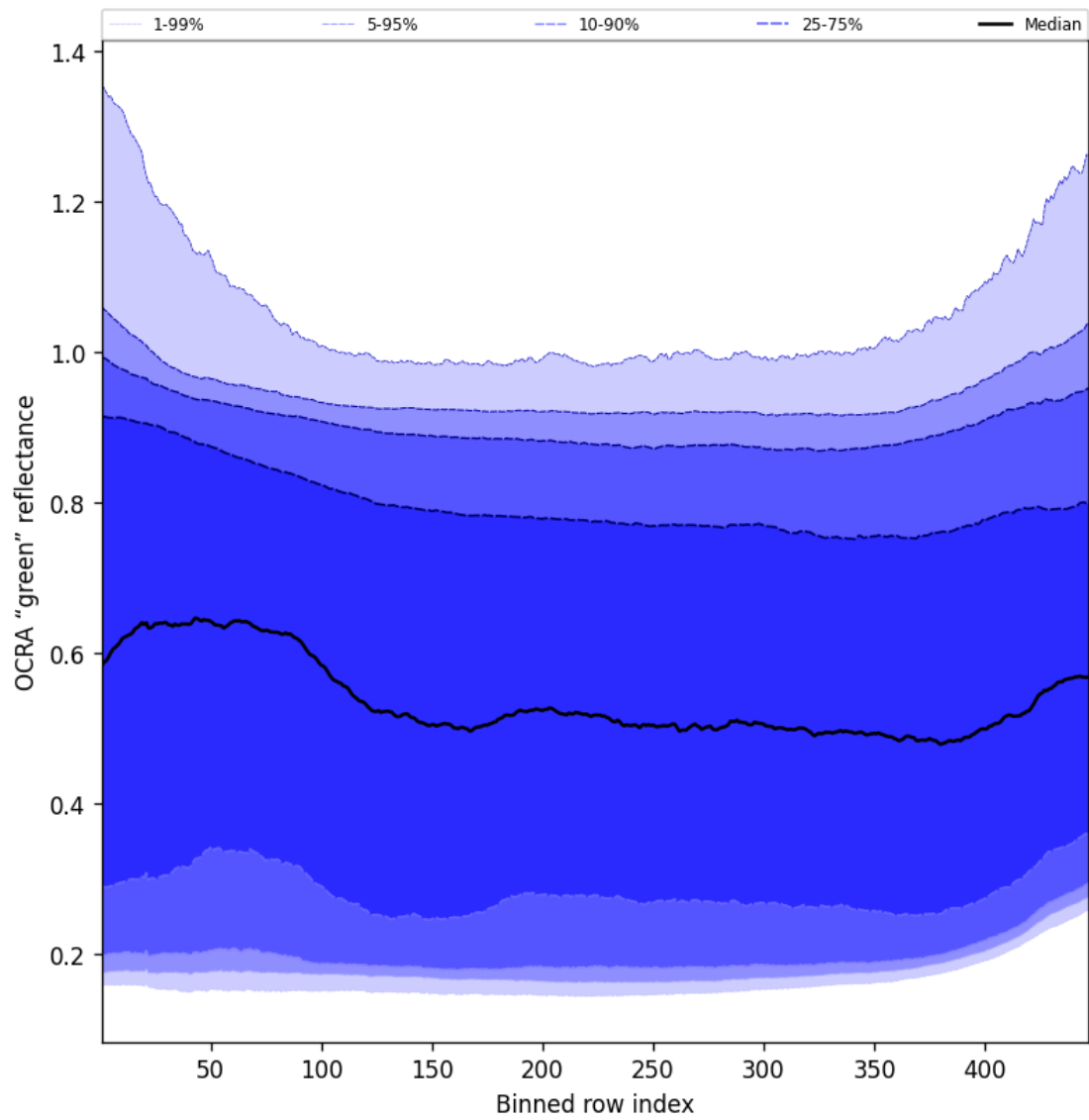
Figure 68: Along track statistics of "OCRA "green" reflectance" for 2024-11-17 to 2024-11-19
