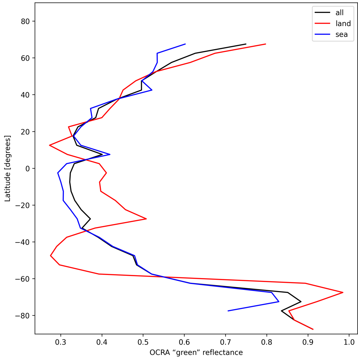
Figure 36: Zonal average of "OCRA "green" reflectance" for 2024-11-17 to 2024-11-19.
