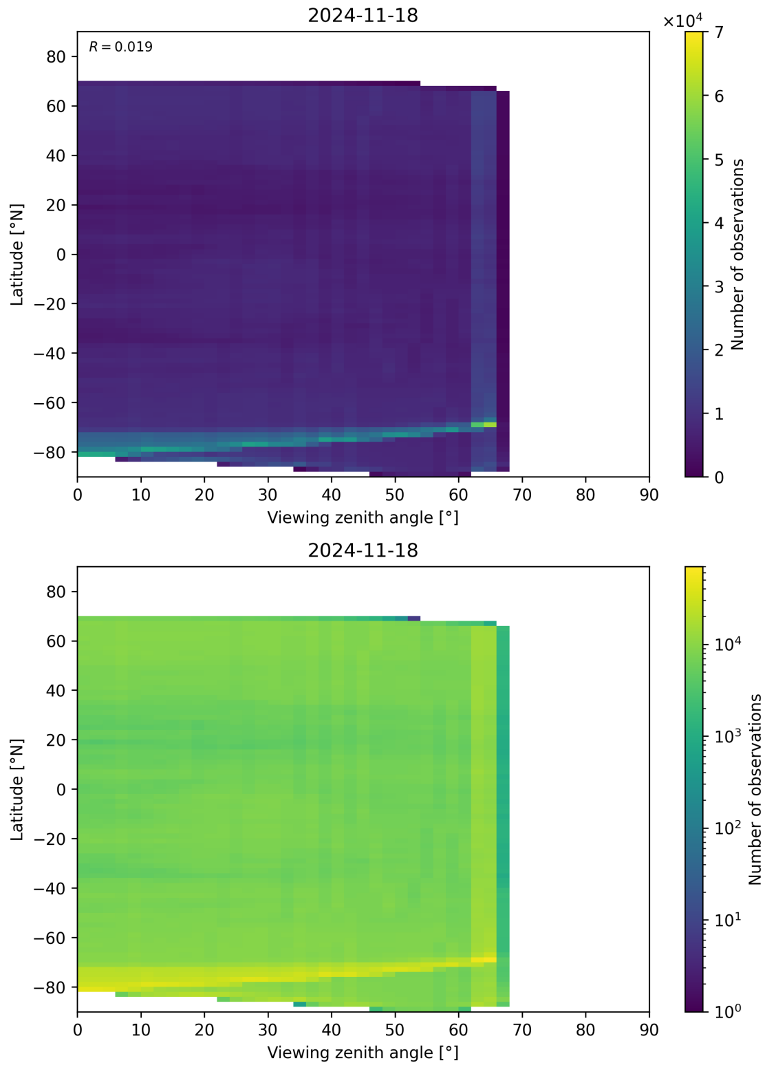
Figure 113: Scatter density plot of “Viewing zenith angle” against “Latitude” for 2024-11-17 to 2024-11-19.
