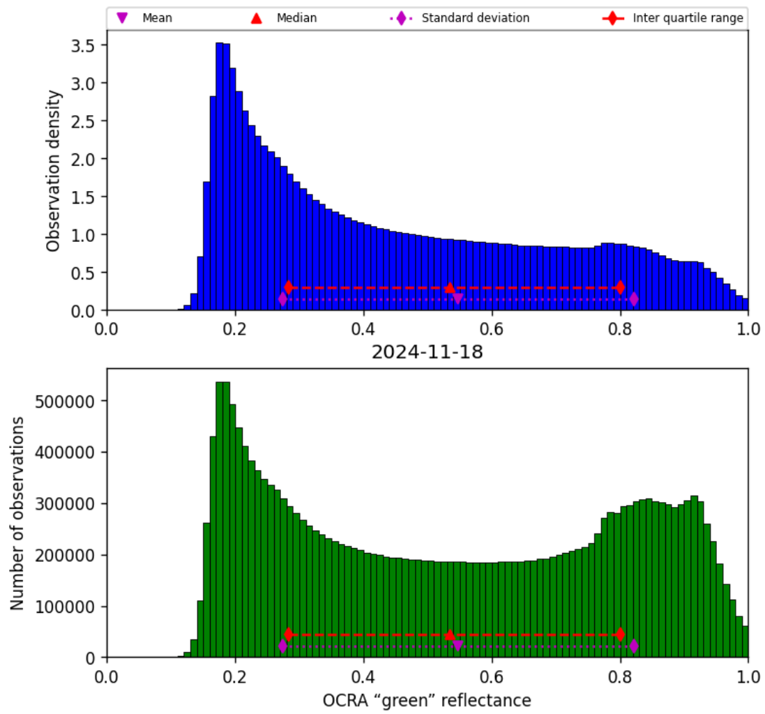
Figure 52: Histogram of “OCRA “green” reflectance” for 2024-11-17 to 2024-11-19
