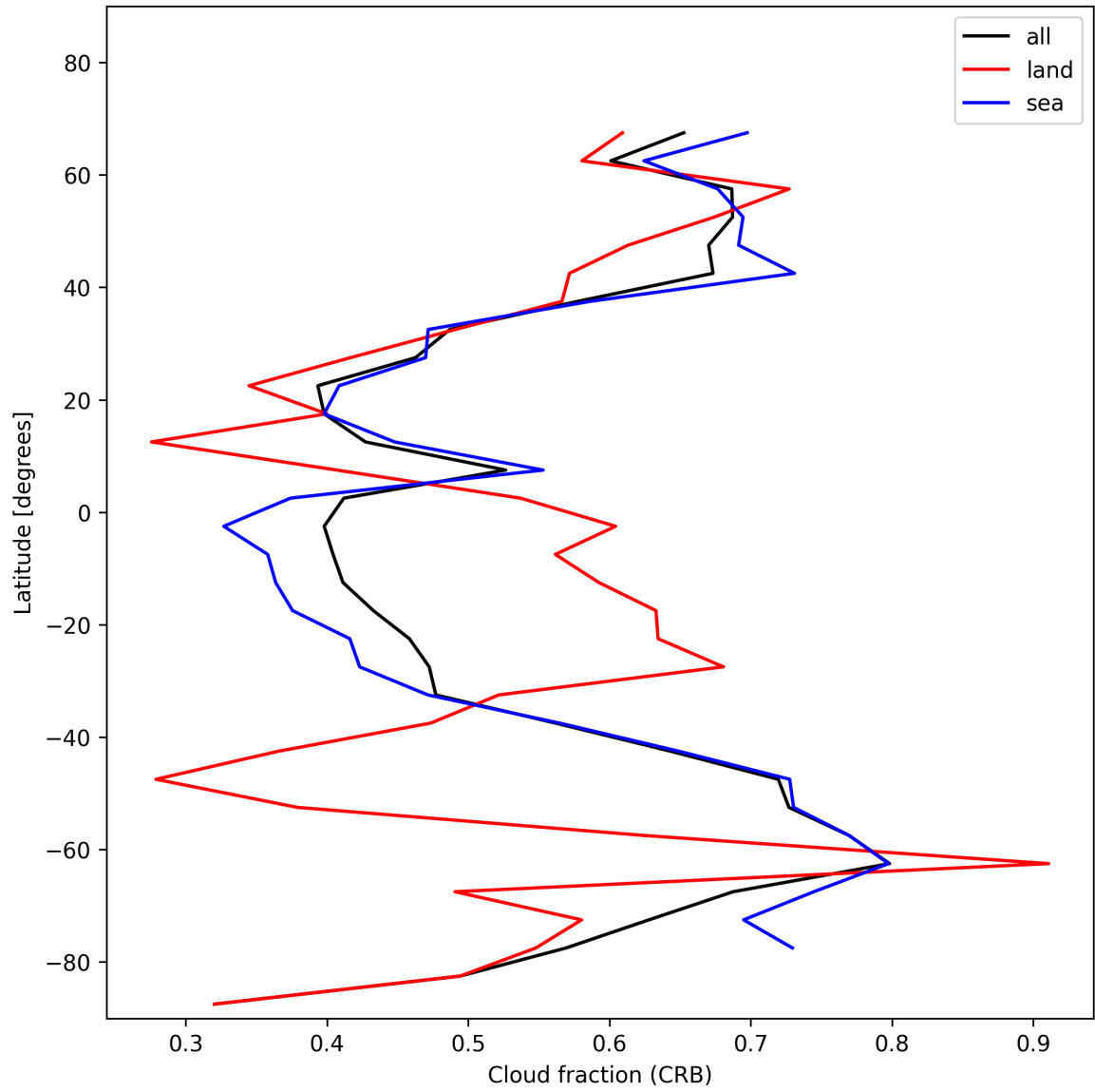
Figure 26: Zonal average of “Cloud fraction (CRB)” for 2024-11-17 to 2024-11-19.
