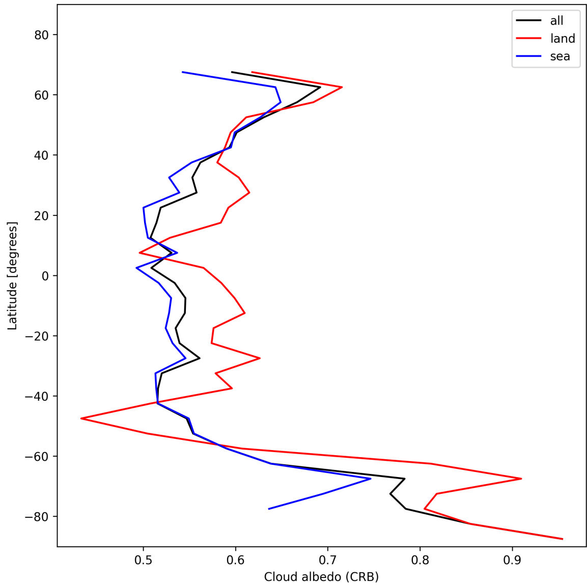
Figure 28: Zonal average of “Cloud albedo (CRB)” for 2024-11-17 to 2024-11-19.
