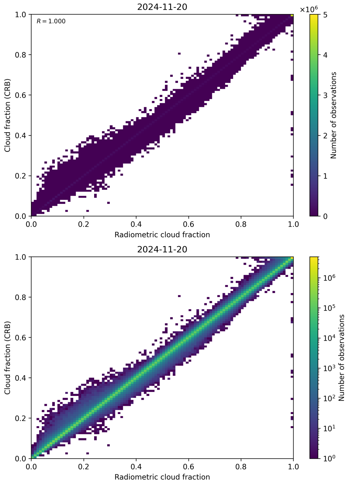
Figure 73: Scatter density plot of “Radiometric cloud fraction” against “Cloud fraction (CRB)” for 2024-11-20 to 2024-11-21.
