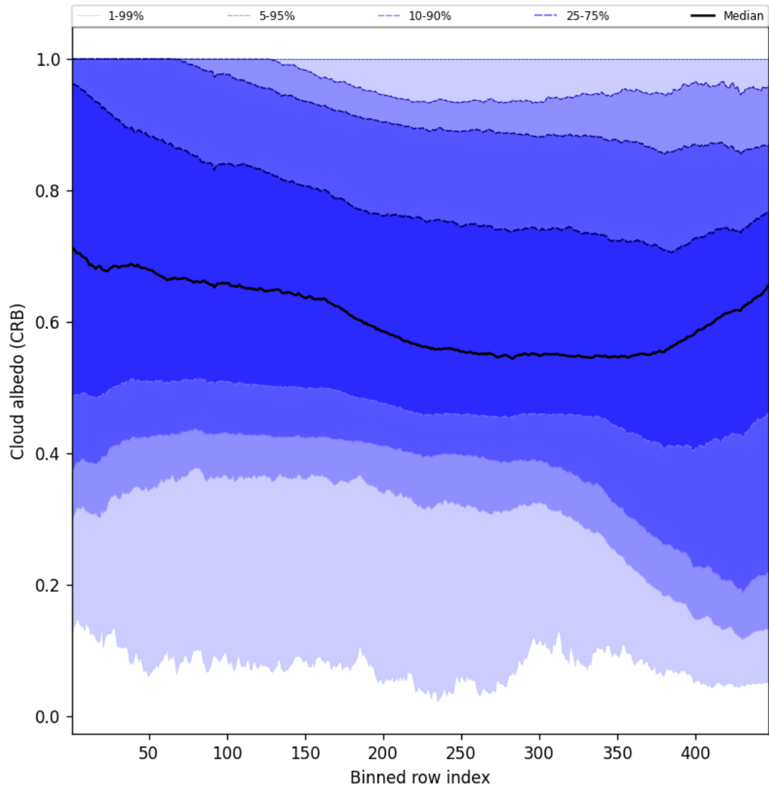
Figure 60: Along track statistics of “Cloud albedo (CRB)” for 2024-11-20 to 2024-11-21
