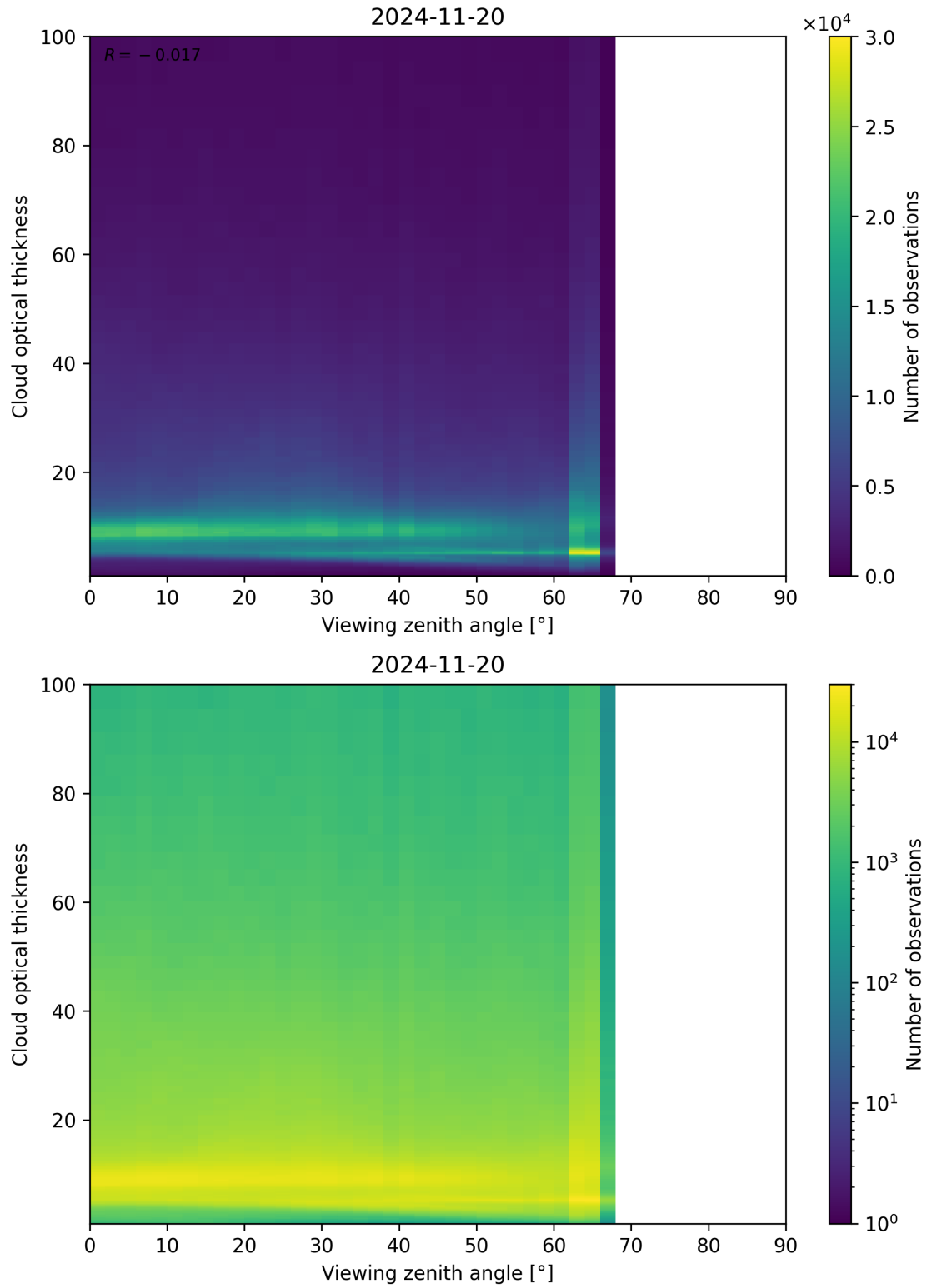
Figure 111: Scatter density plot of “Viewing zenith angle” against “Cloud optical thickness” for 2024-11-20 to 2024-11-21.
