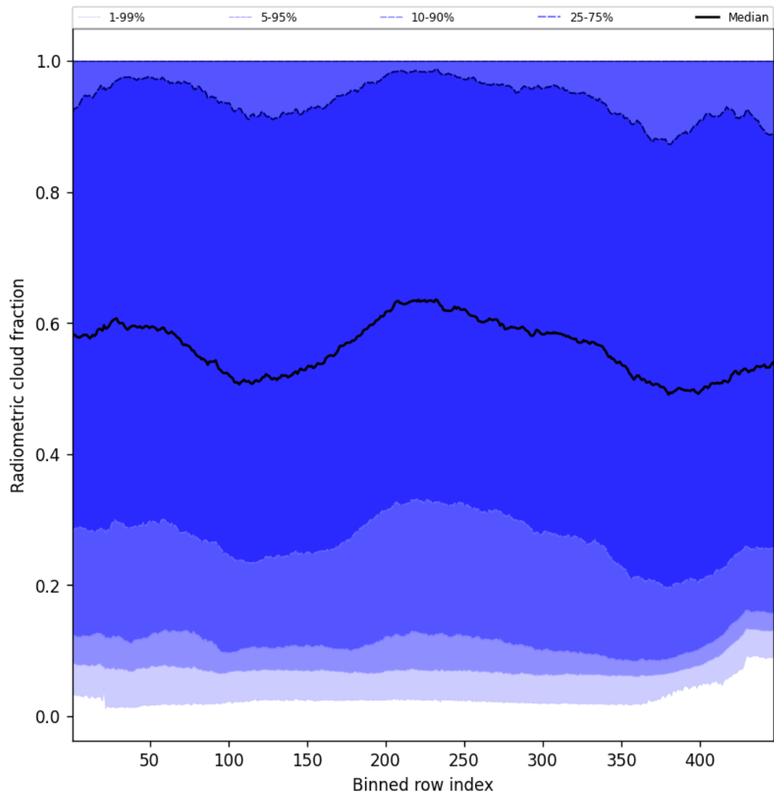
Figure 55: Along track statistics of “Radiometric cloud fraction” for 2024-11-20 to 2024-11-21
