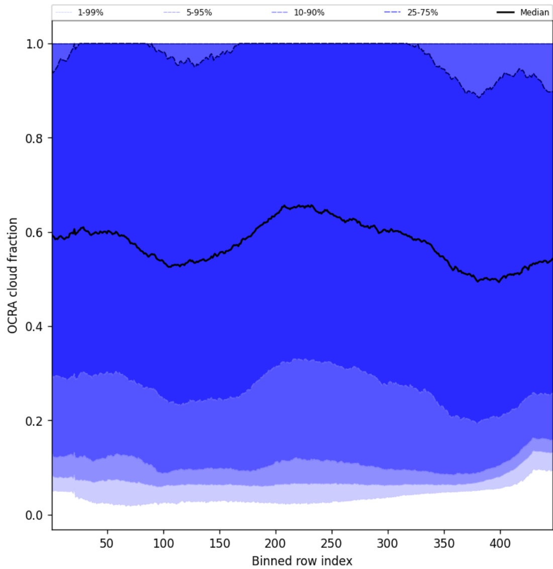
Figure 66: Along track statistics of “OCRA cloud fraction” for 2024-11-20 to 2024-11-21
