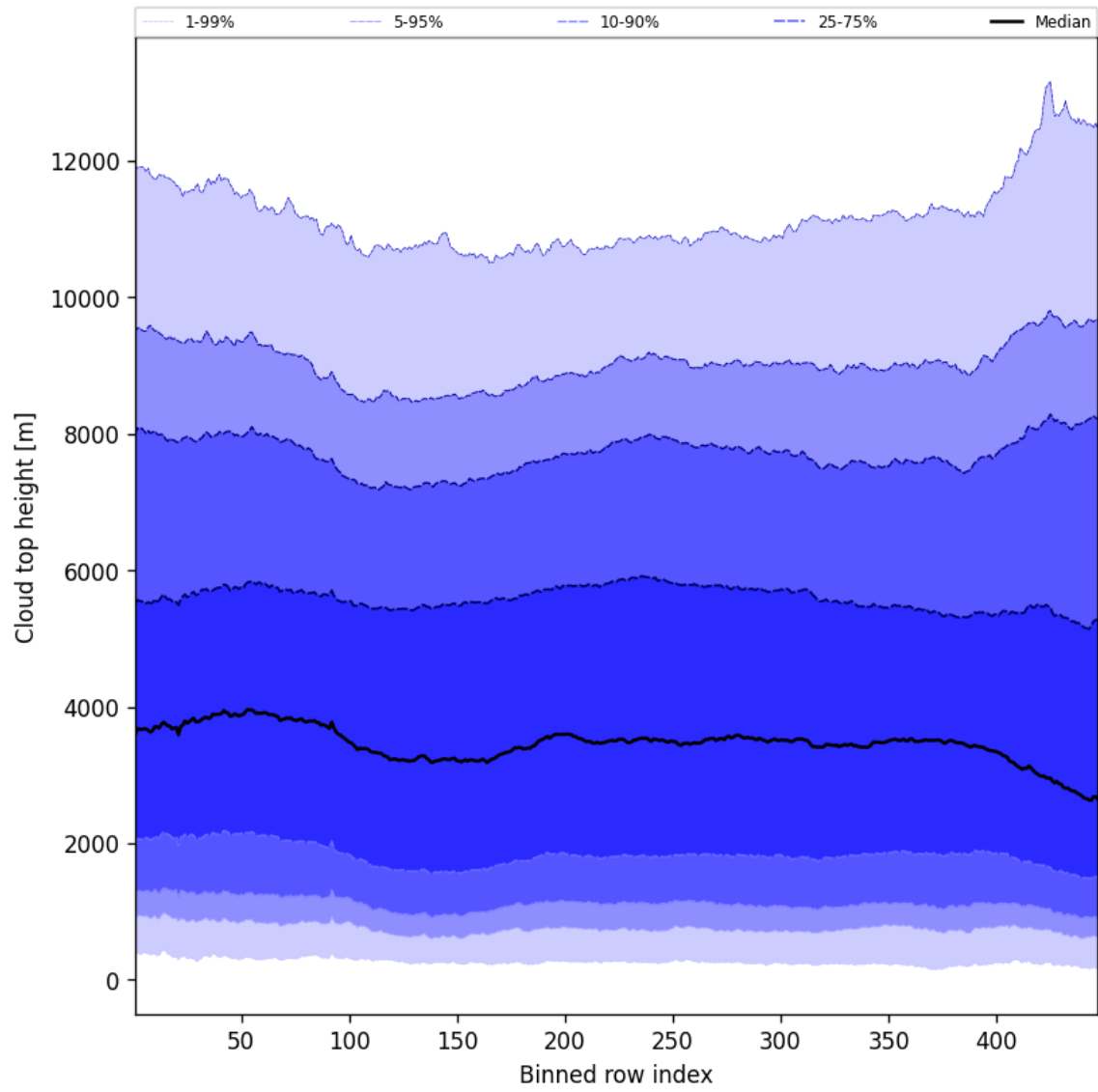
Figure 56: Along track statistics of “Cloud top height” for 2024-11-20 to 2024-11-21
