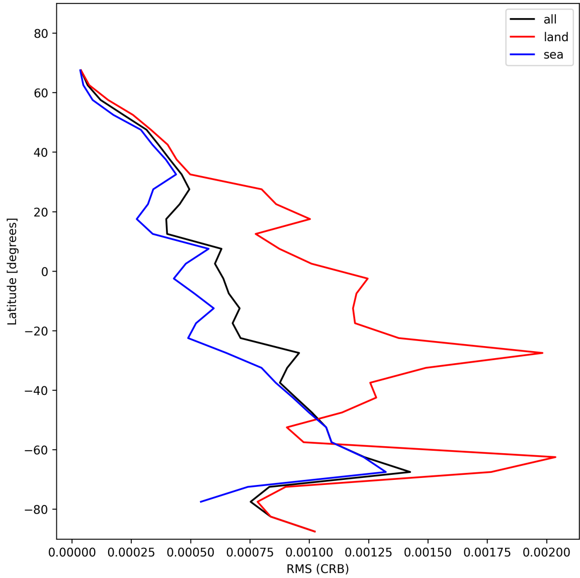
Figure 32: Zonal average of “RMS (CRB)” for 2024-11-20 to 2024-11-21.
