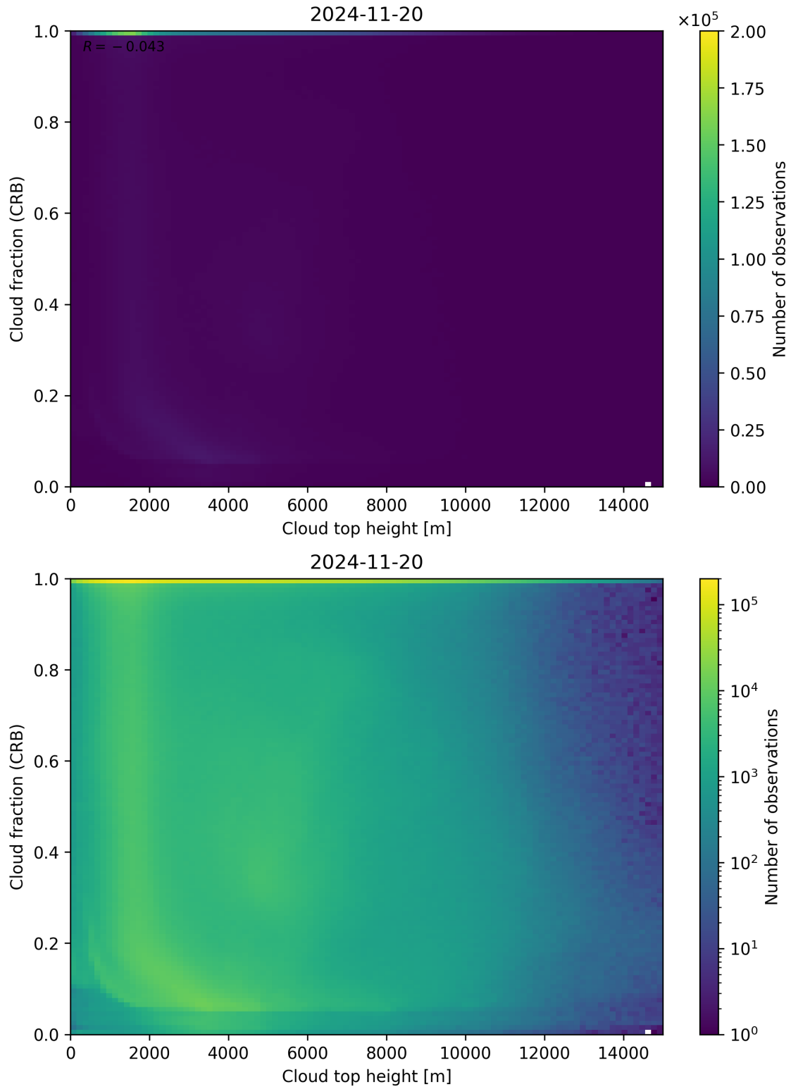
Figure 88: Scatter density plot of “Cloud top height” against “Cloud fraction (CRB)” for 2024-11-20 to 2024-11-21.
