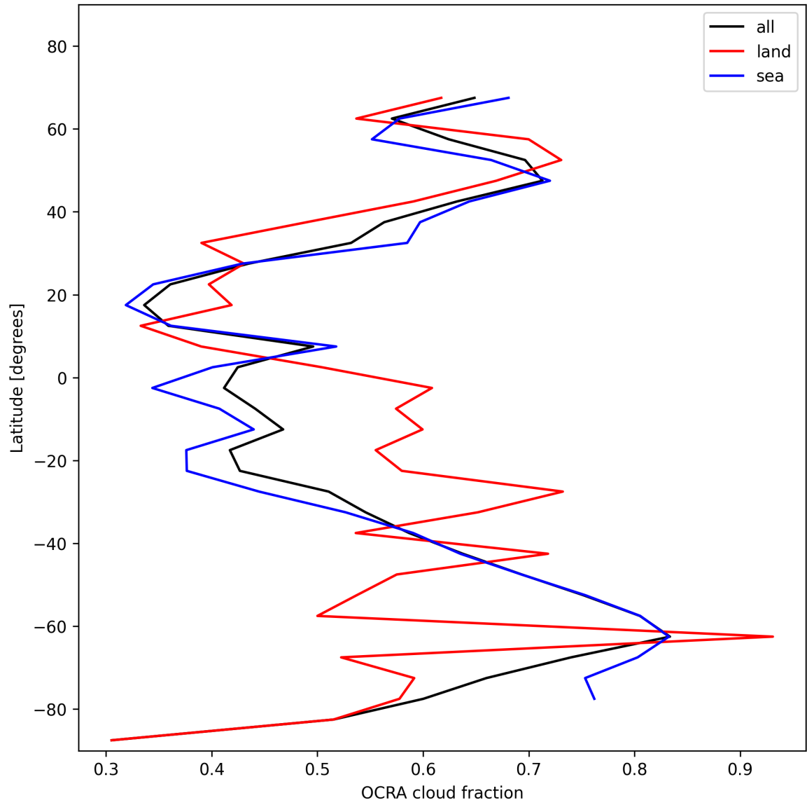
Figure 34: Zonal average of “OCRA cloud fraction” for 2024-11-20 to 2024-11-21.
