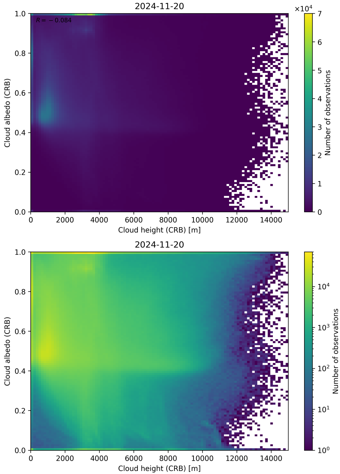
Figure 80: Scatter density plot of “Cloud height (CRB)” against “Cloud albedo (CRB)” for 2024-11-20 to 2024-11-21.
