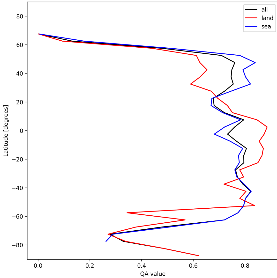
Figure 22: Zonal average of “QA value” for 2024-11-20 to 2024-11-21.
