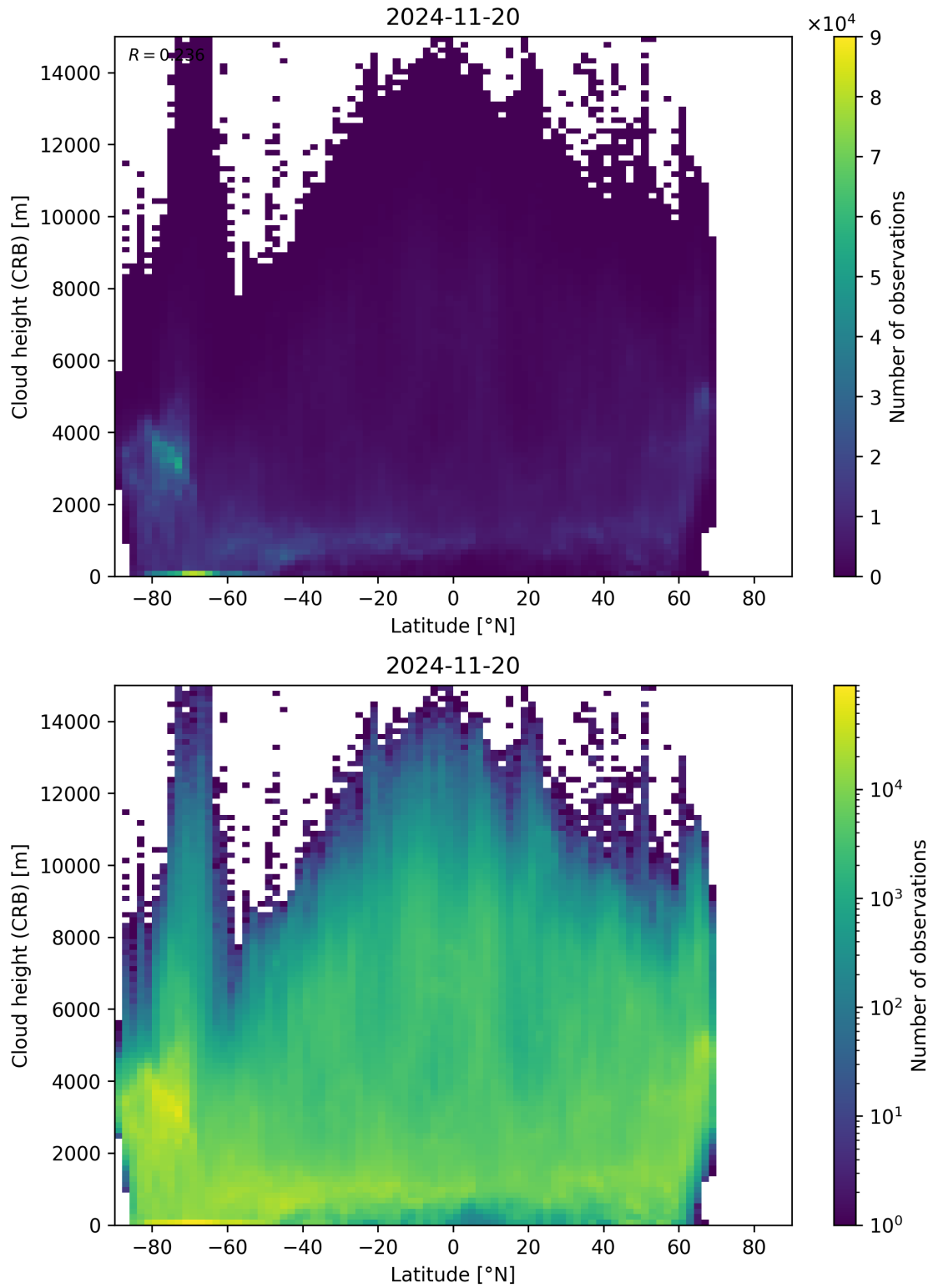
Figure 95: Scatter density plot of “Latitude” against “Cloud height (CRB)” for 2024-11-20 to 2024-11-21.
