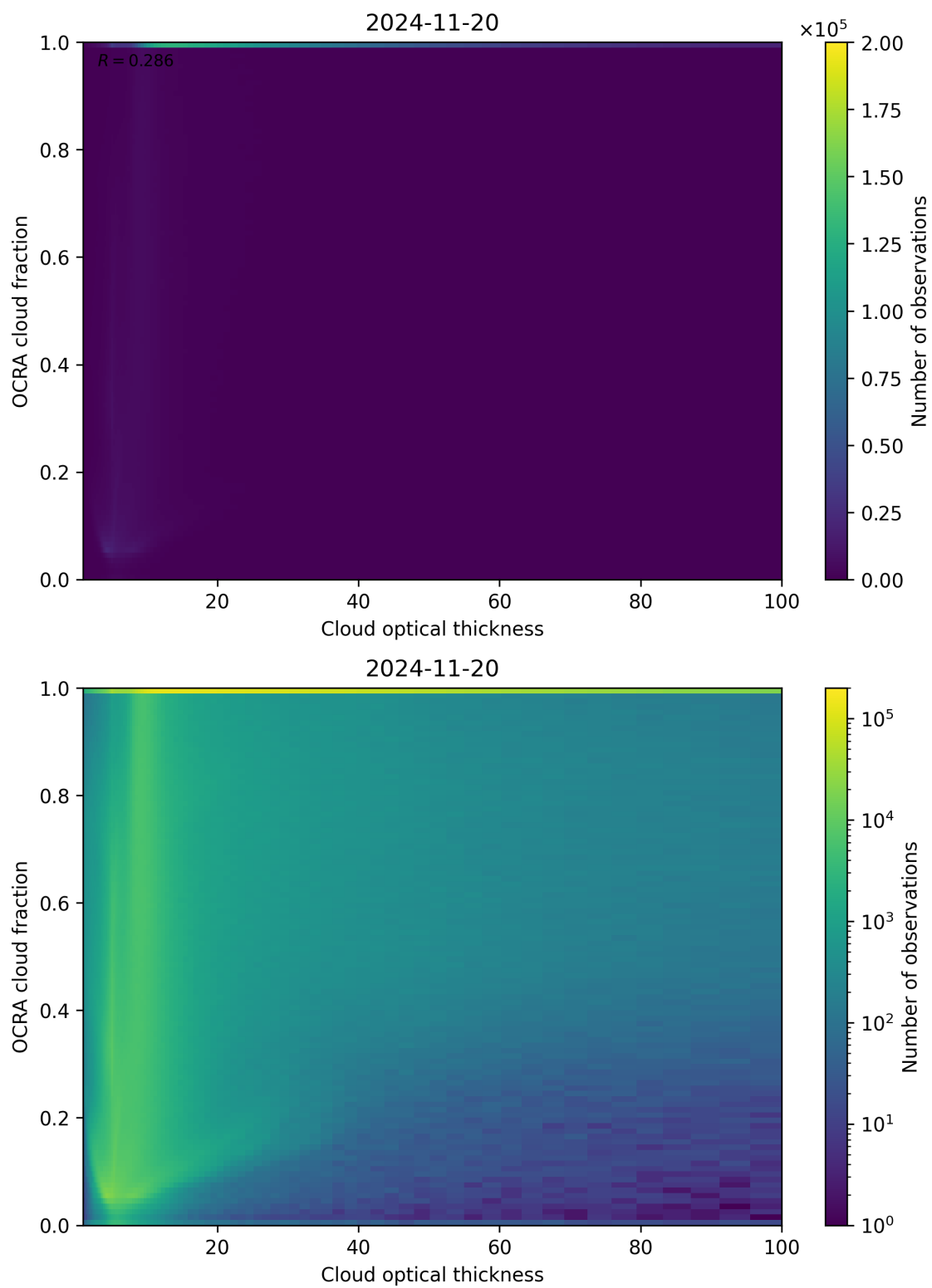
Figure 83: Scatter density plot of “Cloud optical thickness” against “OCRA cloud fraction” for 2024-11-20 to 2024-11-21.
