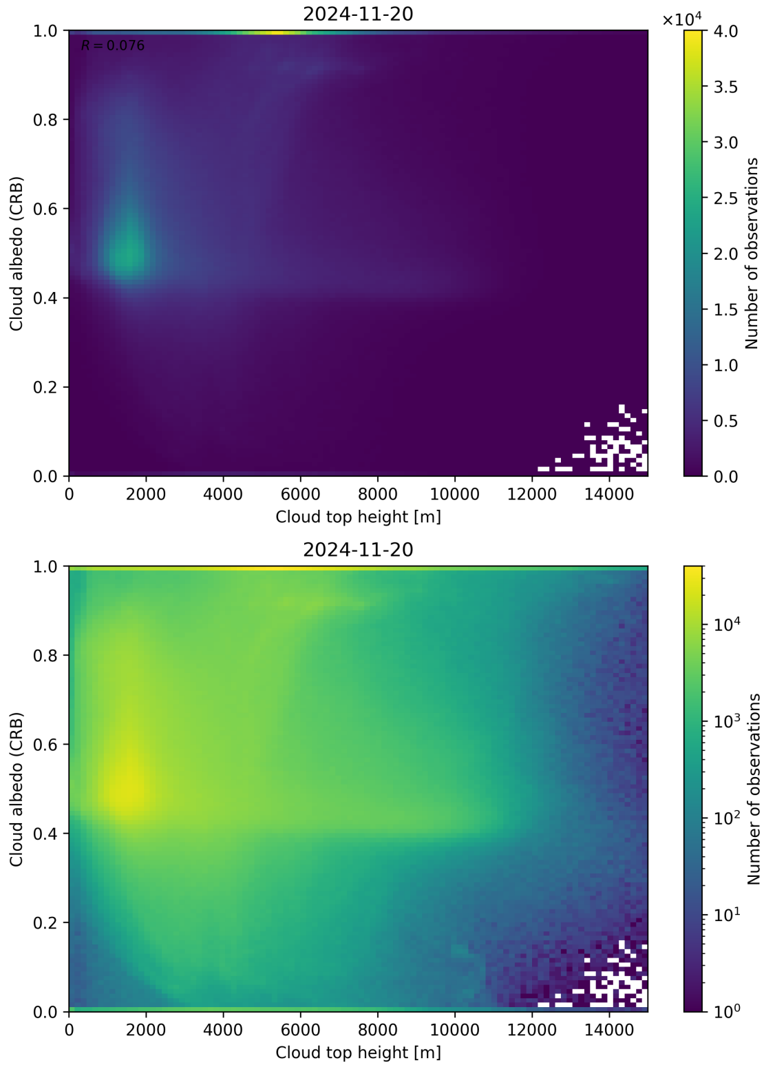
Figure 86: Scatter density plot of “Cloud top height” against “Cloud albedo (CRB)” for 2024-11-20 to 2024-11-21.
