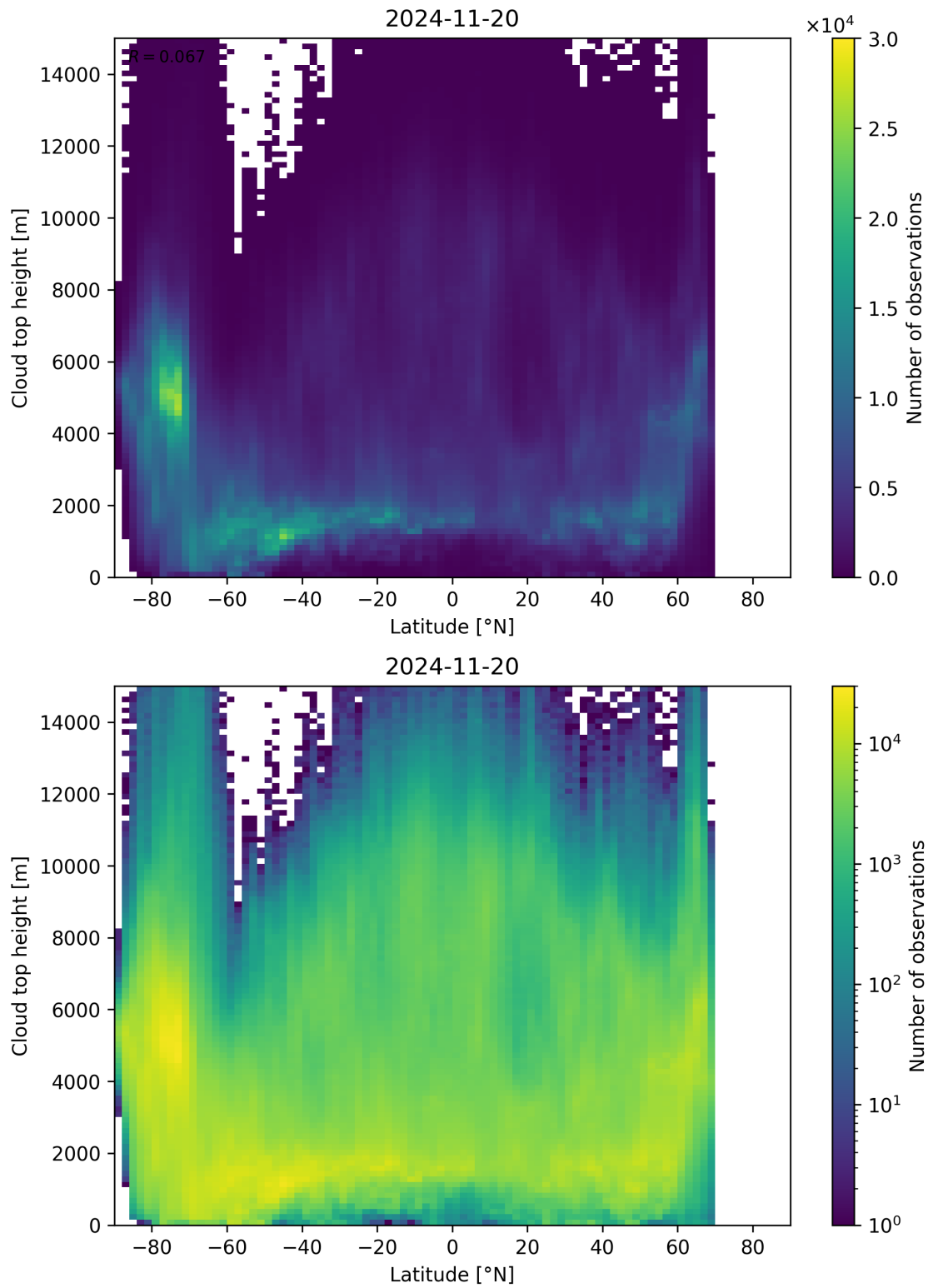
Figure 97: Scatter density plot of “Latitude” against “Cloud top height” for 2024-11-20 to 2024-11-21.
