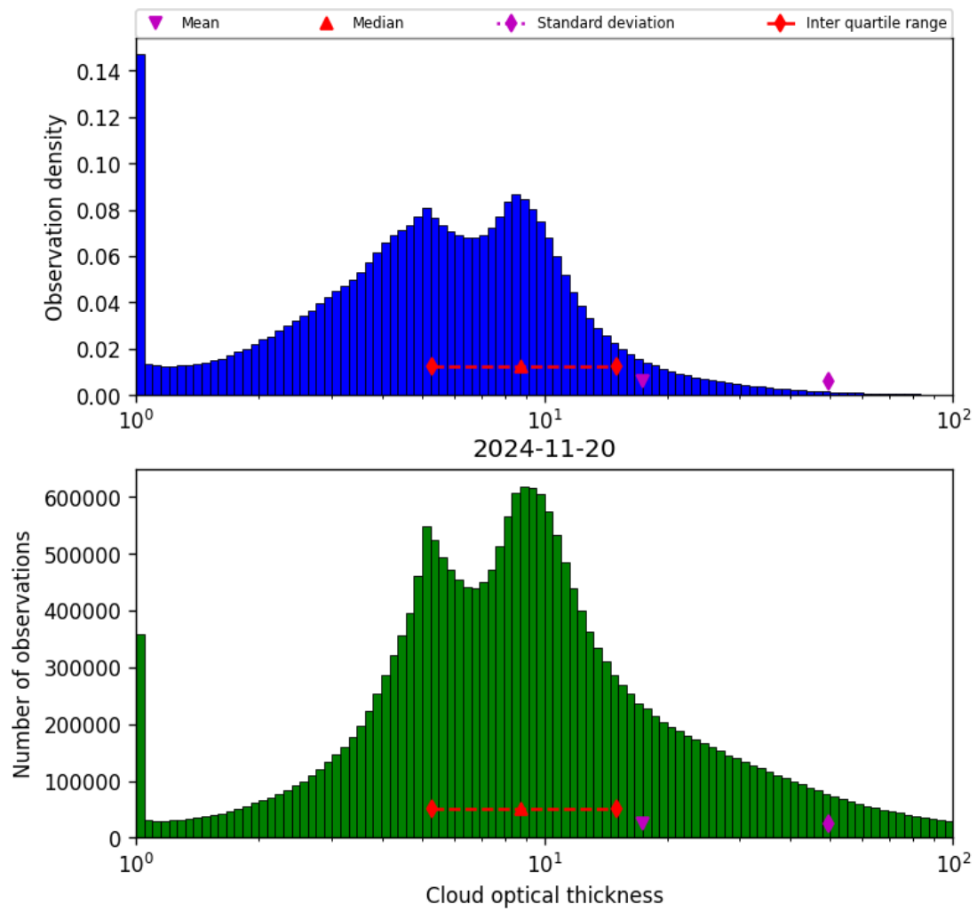
Figure 41: Histogram of “Cloud optical thickness” for 2024-11-20 to 2024-11-21
