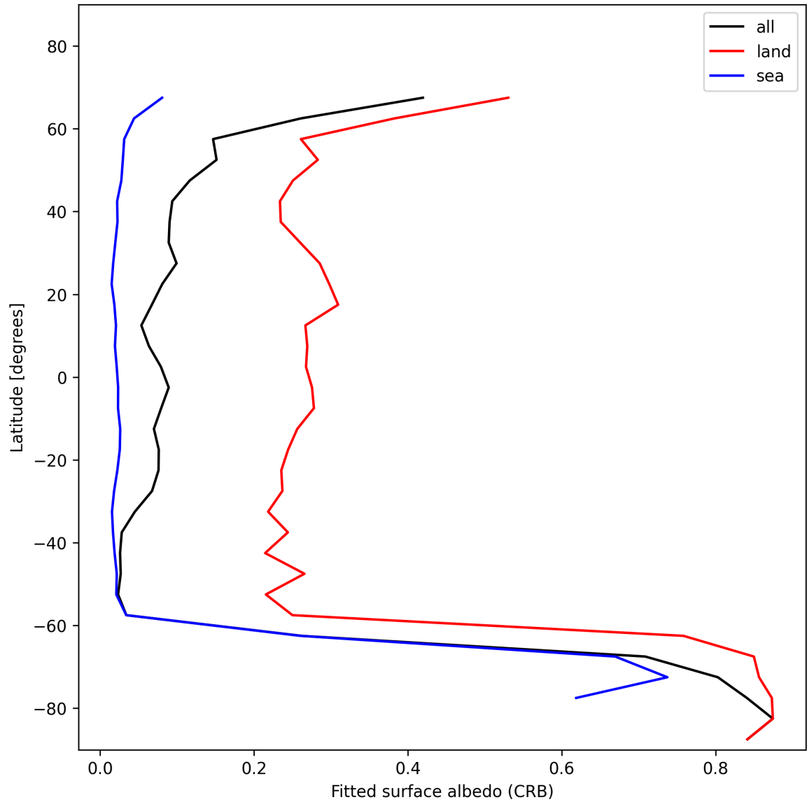
Figure 30: Zonal average of “Fitted surface albedo (CRB)” for 2024-11-20 to 2024-11-21.
