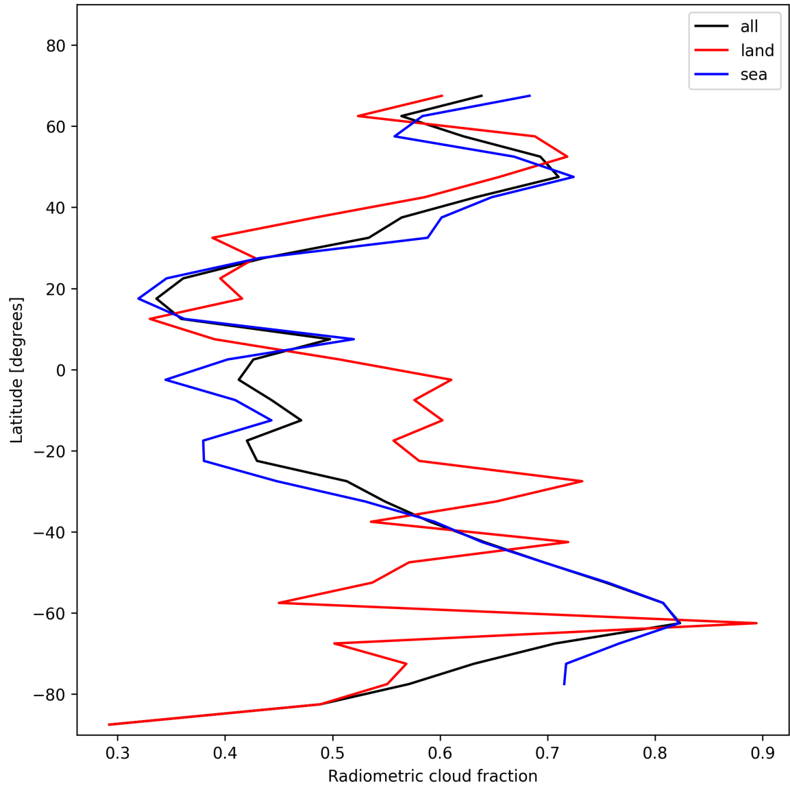
Figure 23: Zonal average of “Radiometric cloud fraction” for 2024-11-20 to 2024-11-21.
