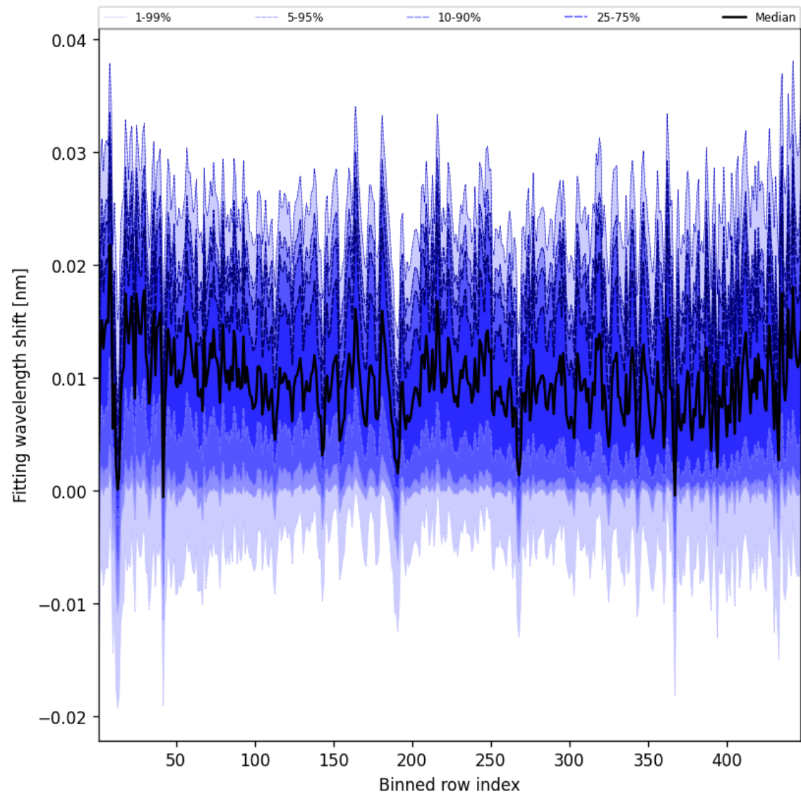
Figure 65: Along track statistics of “Fitting wavelength shift” for 2024-11-20 to 2024-11-21
