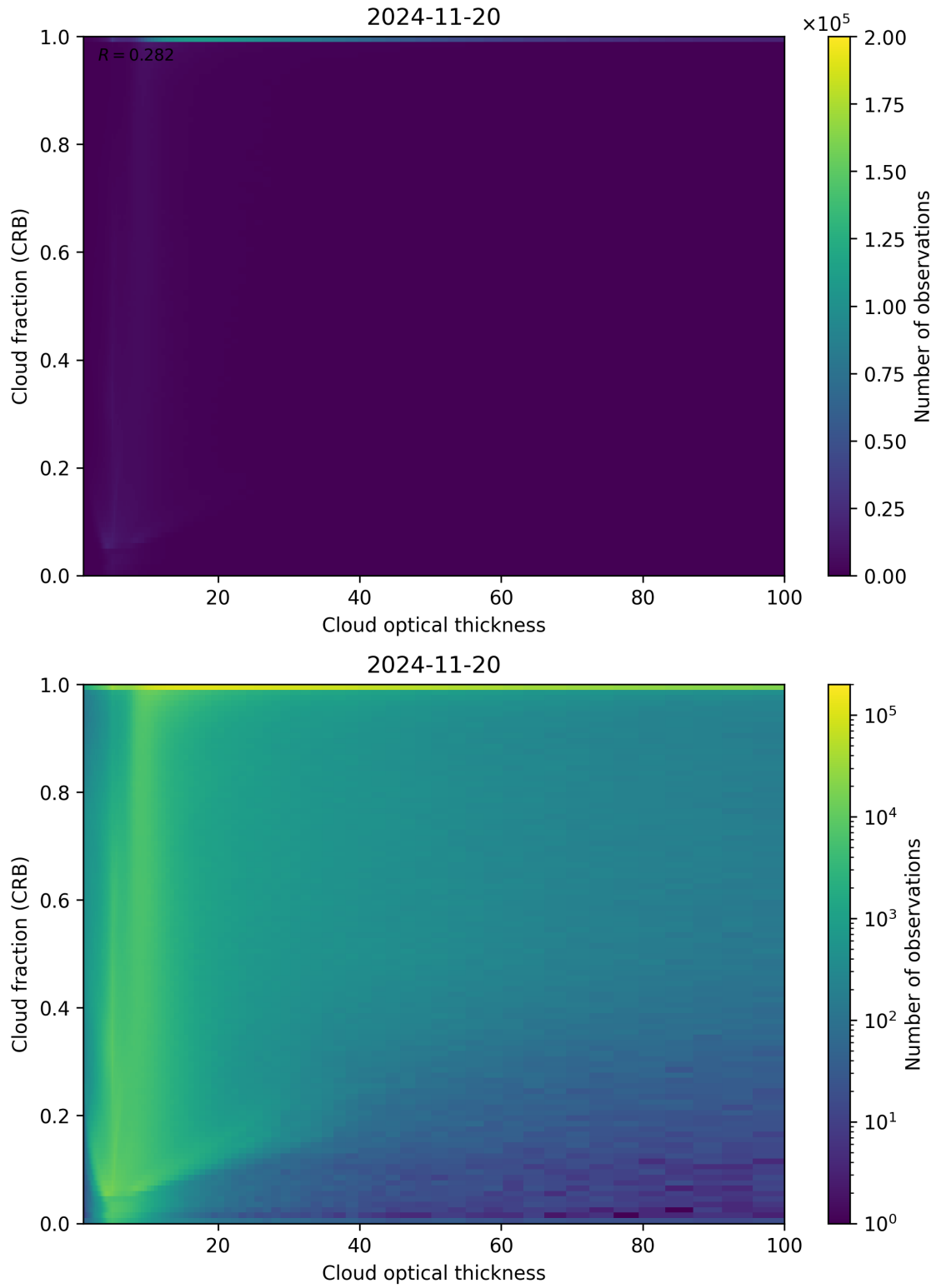
Figure 84: Scatter density plot of “Cloud optical thickness” against “Cloud fraction (CRB)” for 2024-11-20 to 2024-11-21.
