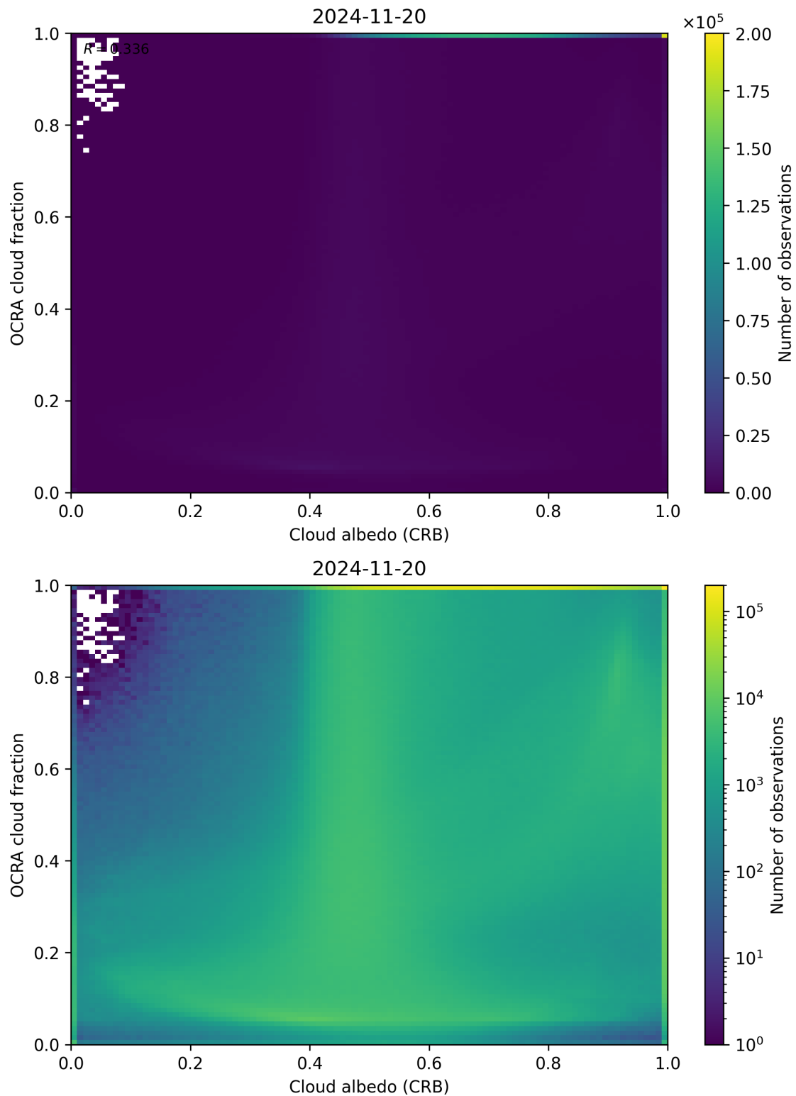
Figure 70: Scatter density plot of “Cloud albedo (CRB)” against “OCRA cloud fraction” for 2024-11-20 to 2024-11-21.
