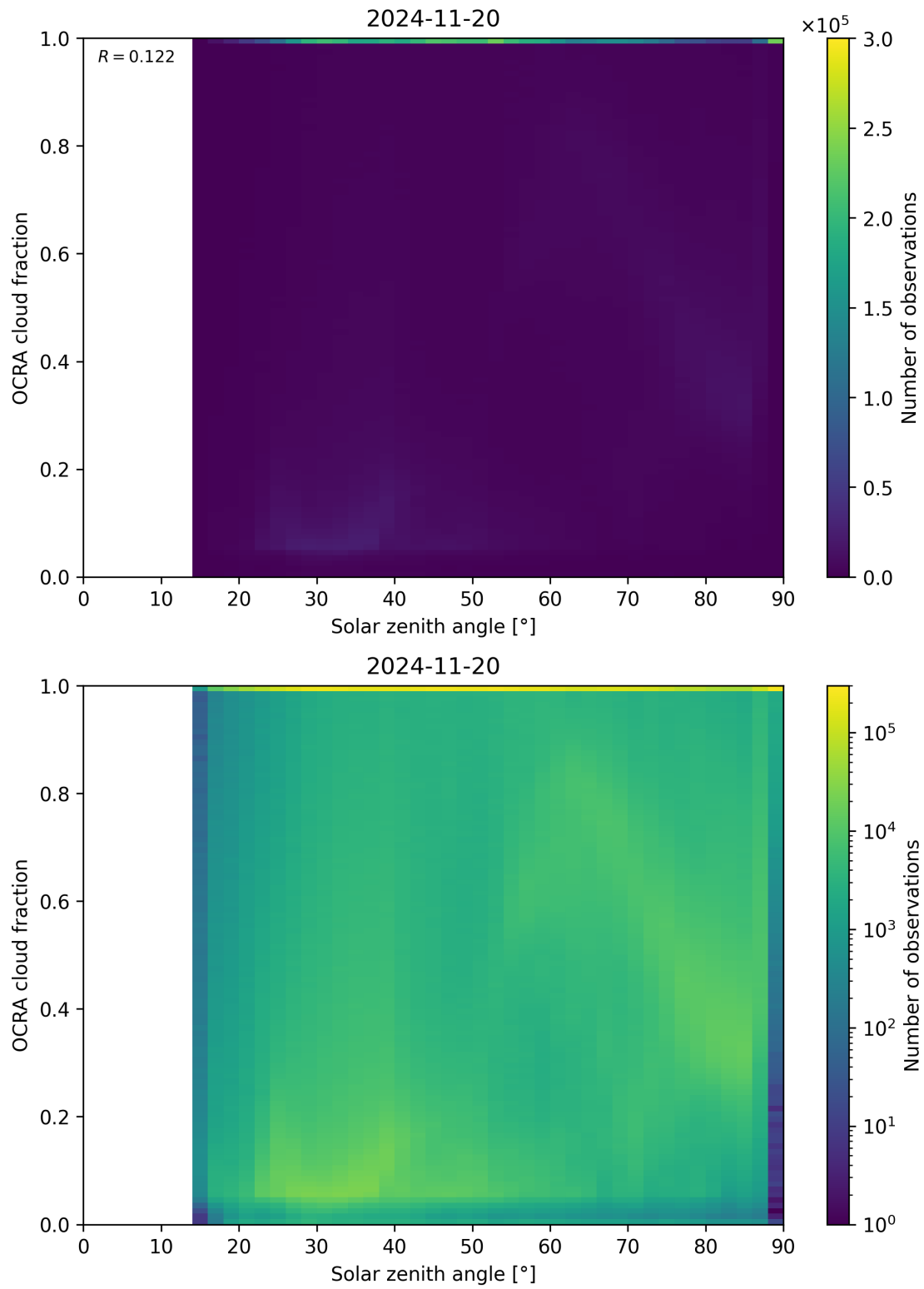
Figure 100: Scatter density plot of “Solar zenith angle” against “OCRA cloud fraction” for 2024-11-20 to 2024-11-21.
