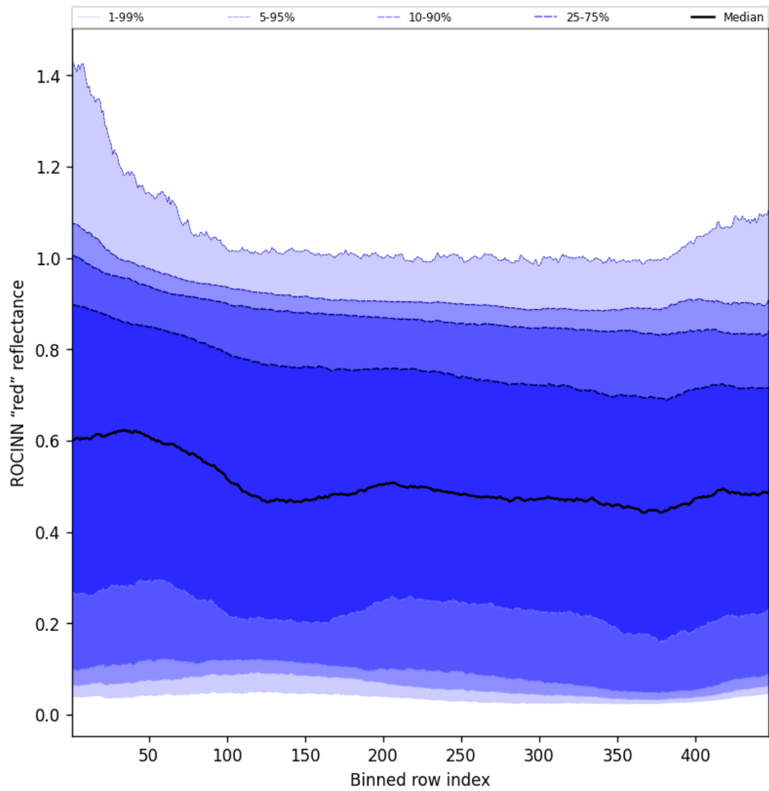
Figure 69: Along track statistics of "ROCINN "red" reflectance" for 2024-11-20 to 2024-11-21
