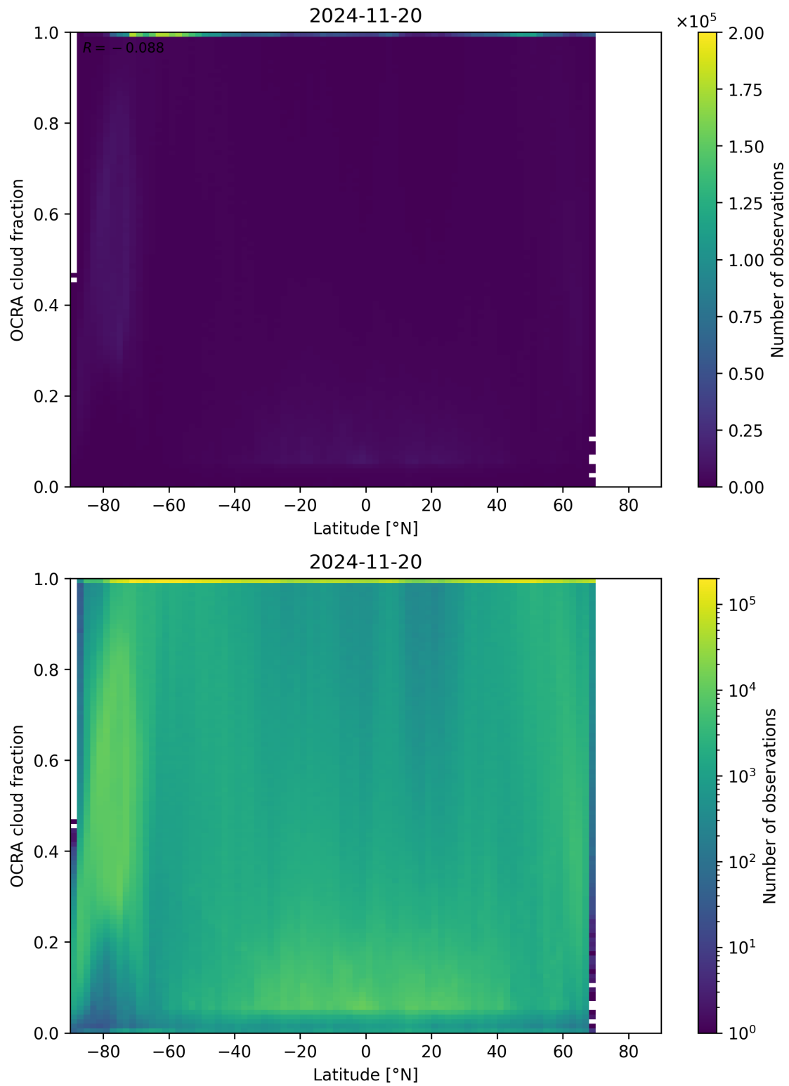
Figure 93: Scatter density plot of “Latitude” against “OCRA cloud fraction” for 2024-11-20 to 2024-11-21.
