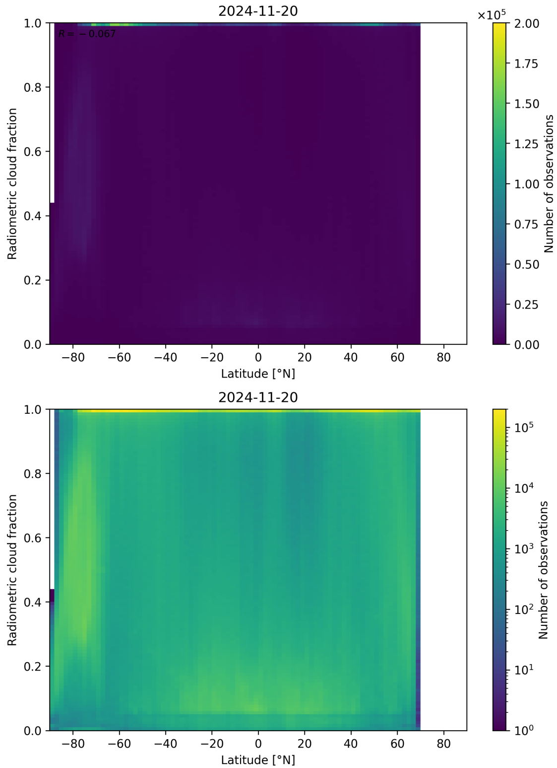
Figure 92: Scatter density plot of “Latitude” against “Radiometric cloud fraction” for 2024-11-20 to 2024-11-21.
