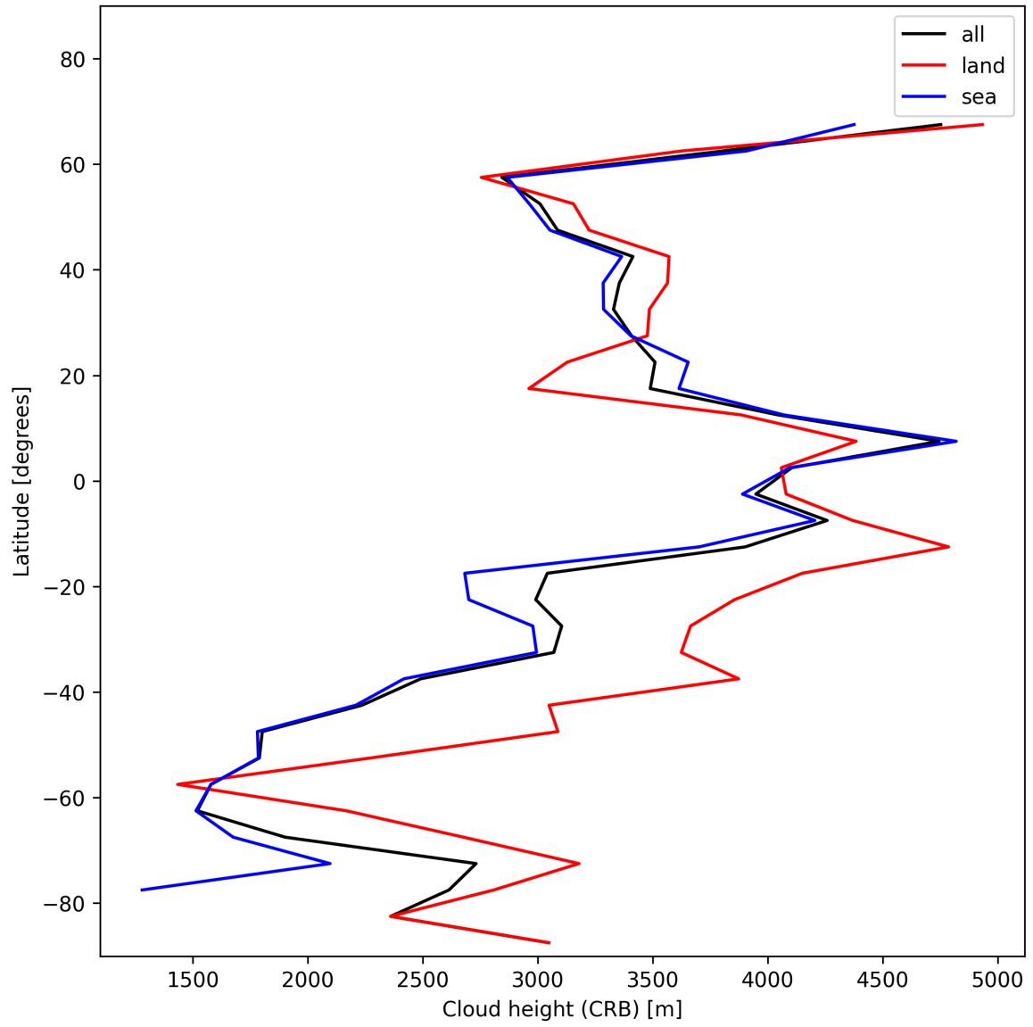
Figure 27: Zonal average of “Cloud height (CRB)” for 2024-11-20 to 2024-11-21.
