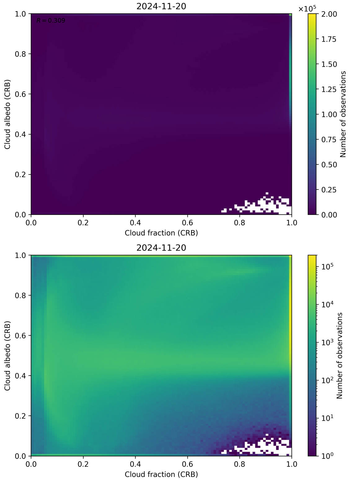
Figure 77: Scatter density plot of “Cloud fraction (CRB)” against “Cloud albedo (CRB)” for 2024-11-20 to 2024-11-21.
