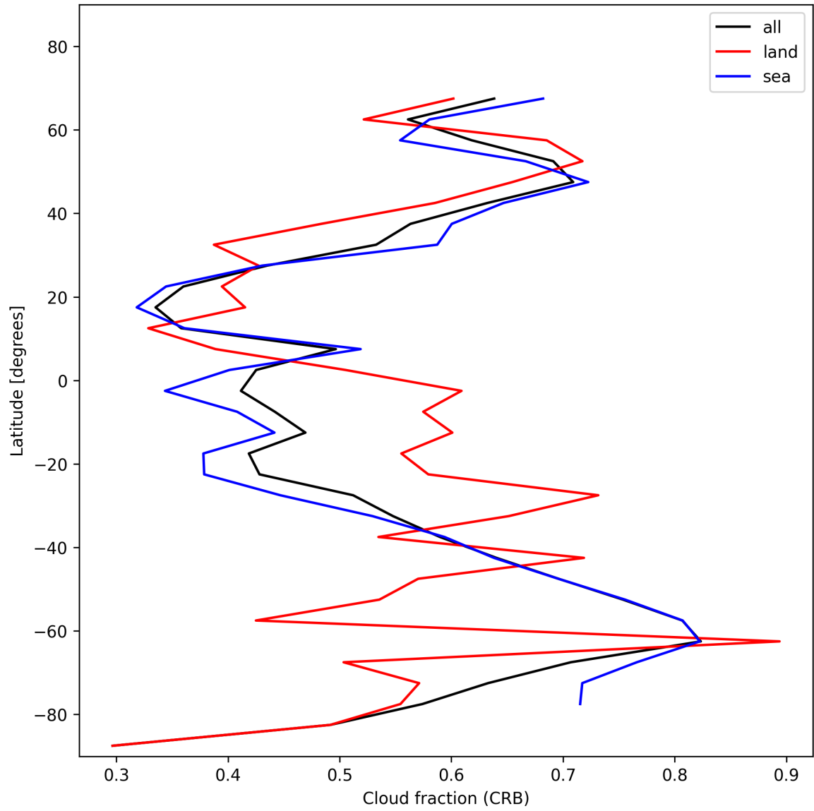
Figure 26: Zonal average of “Cloud fraction (CRB)” for 2024-11-20 to 2024-11-21.
