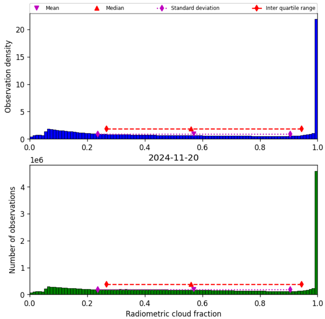
Figure 39: Histogram of “Radiometric cloud fraction” for 2024-11-20 to 2024-11-21
