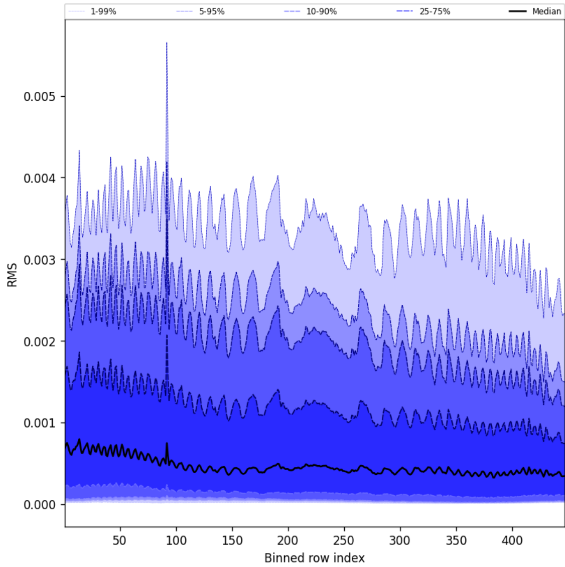
Figure 63: Along track statistics of “RMS” for 2024-11-20 to 2024-11-21
