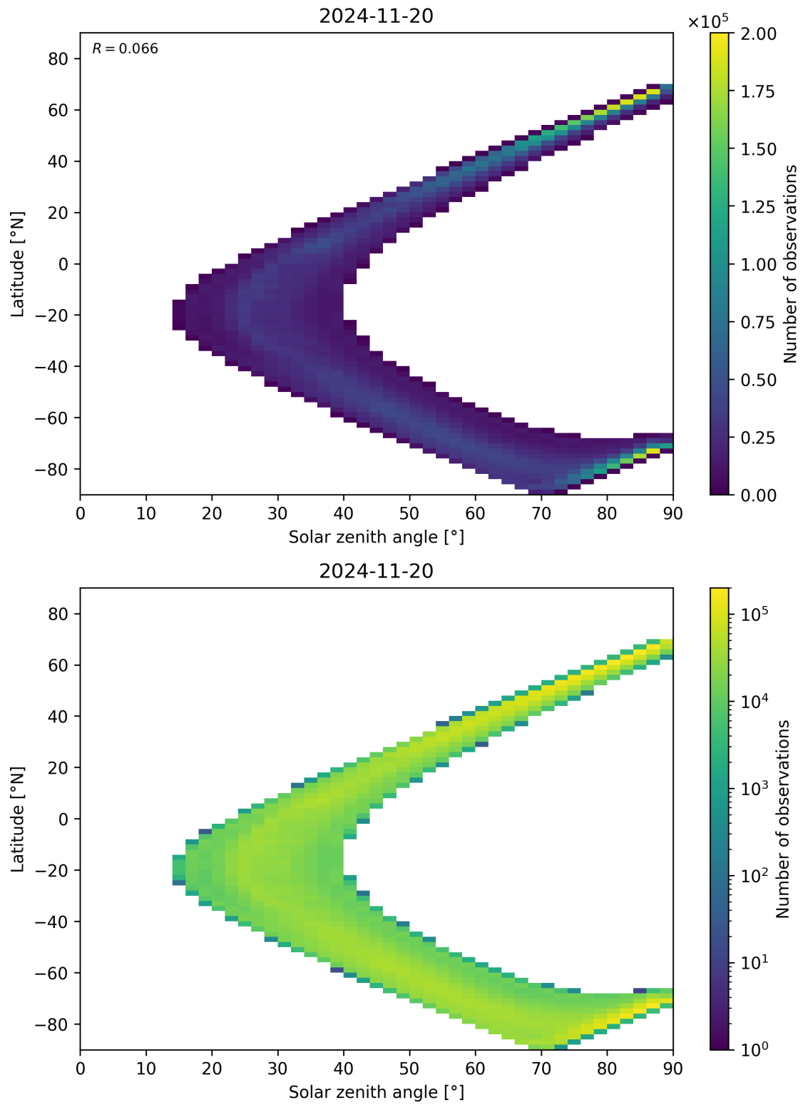
Figure 105: Scatter density plot of “Solar zenith angle” against “Latitude” for 2024-11-20 to 2024-11-21.
