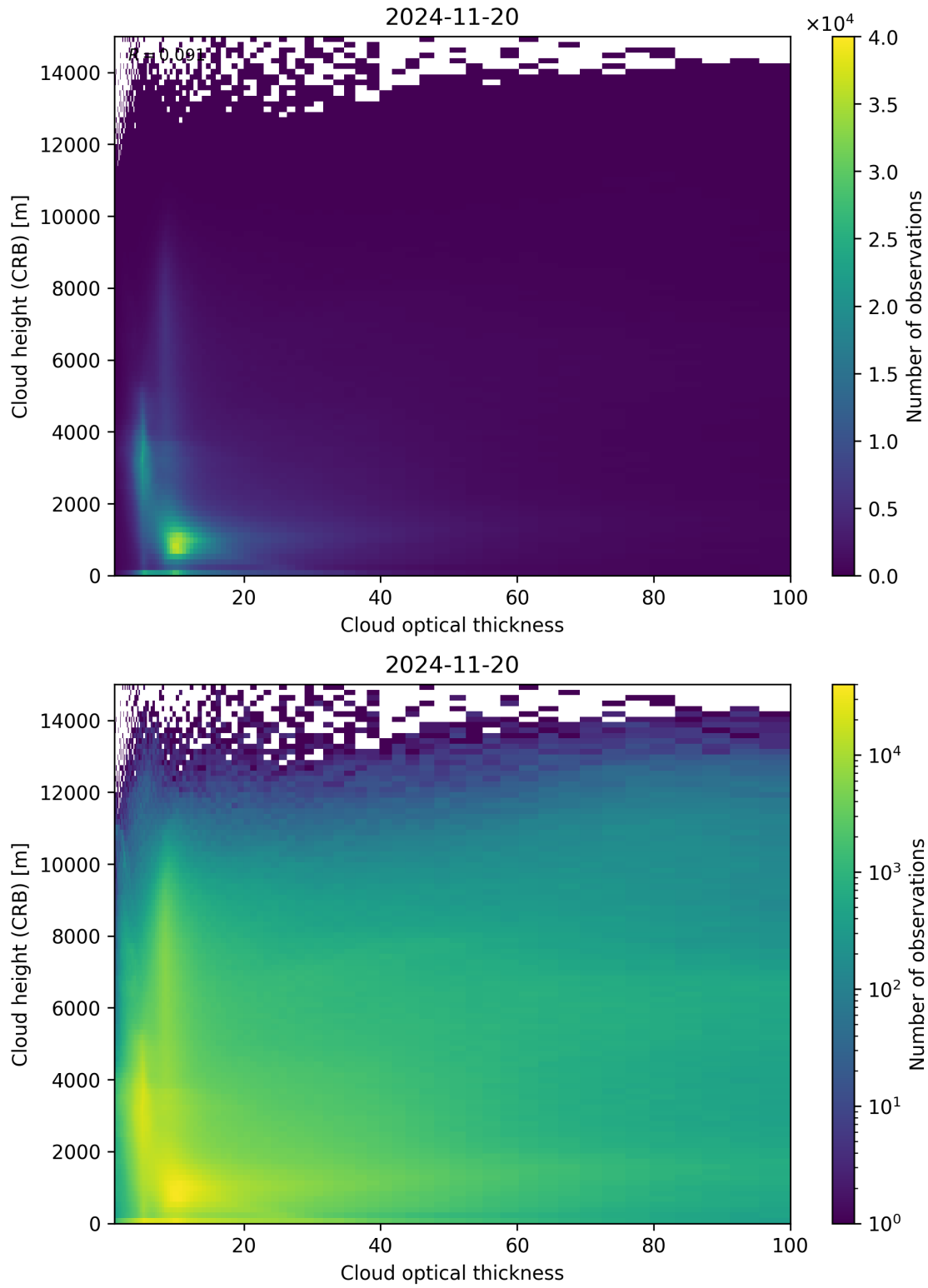
Figure 85: Scatter density plot of “Cloud optical thickness” against “Cloud height (CRB)” for 2024-11-20 to 2024-11-21.
