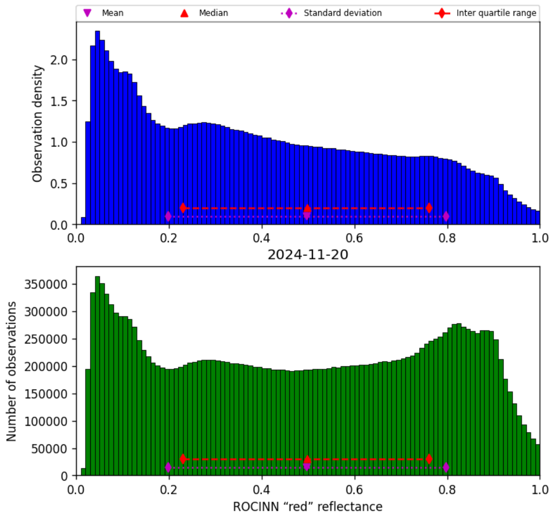
Figure 53: Histogram of “ROCINN “red” reflectance” for 2024-11-20 to 2024-11-21
