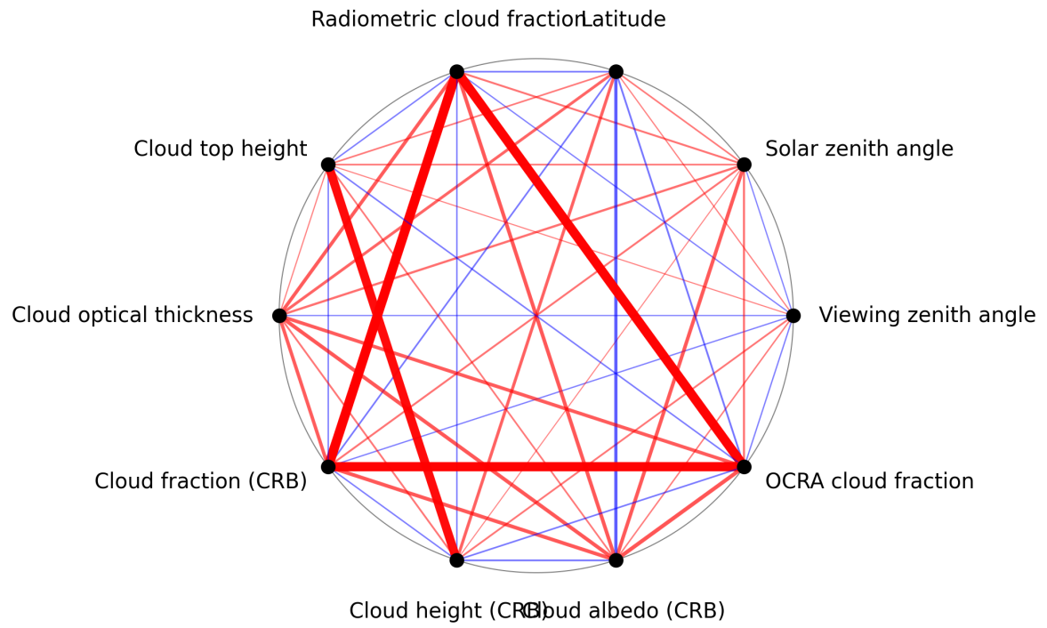
Figure 1: Map of correlation graph for 2024-11-20 to 2024-11-21.
