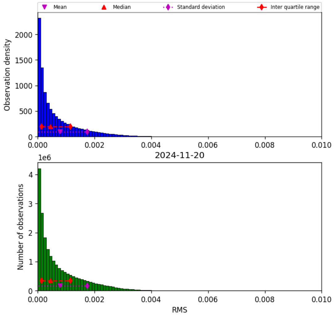
Figure 47: Histogram of “RMS” for 2024-11-20 to 2024-11-21
