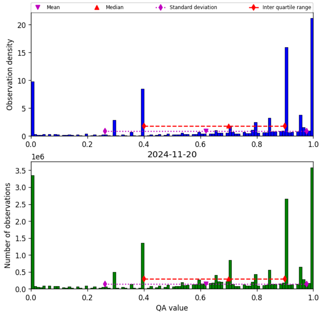
Figure 38: Histogram of “QA value” for 2024-11-20 to 2024-11-21
