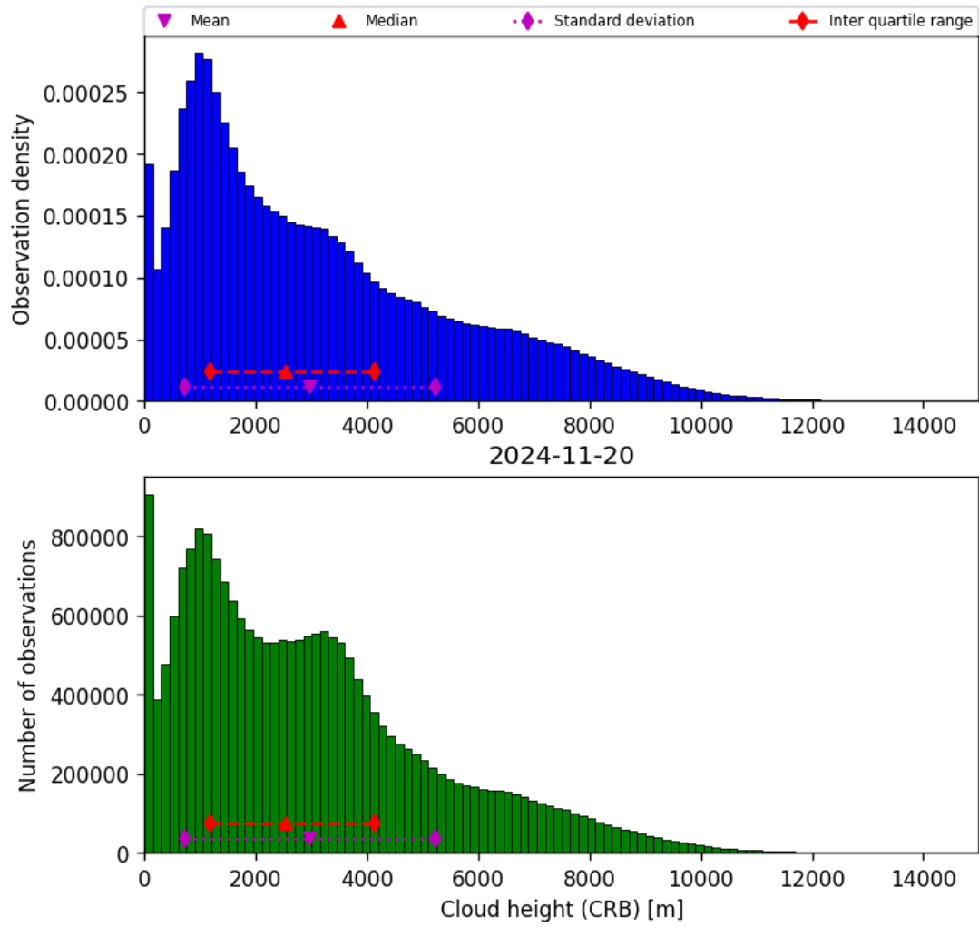
Figure 43: Histogram of “Cloud height (CRB)” for 2024-11-20 to 2024-11-21
