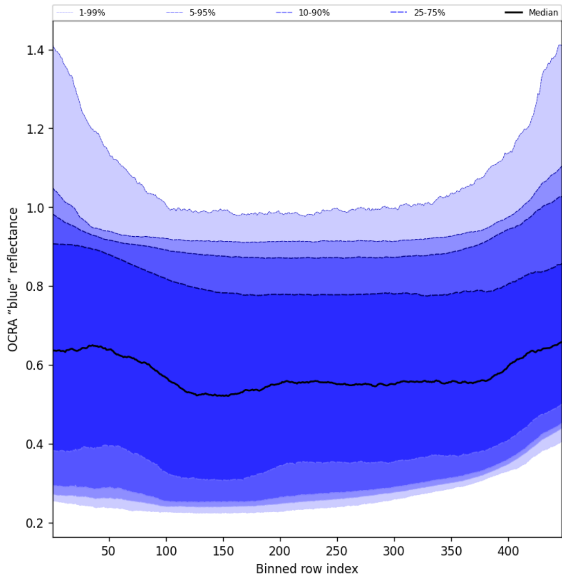
Figure 67: Along track statistics of “OCRA “blue” reflectance” for 2024-11-20 to 2024-11-21
