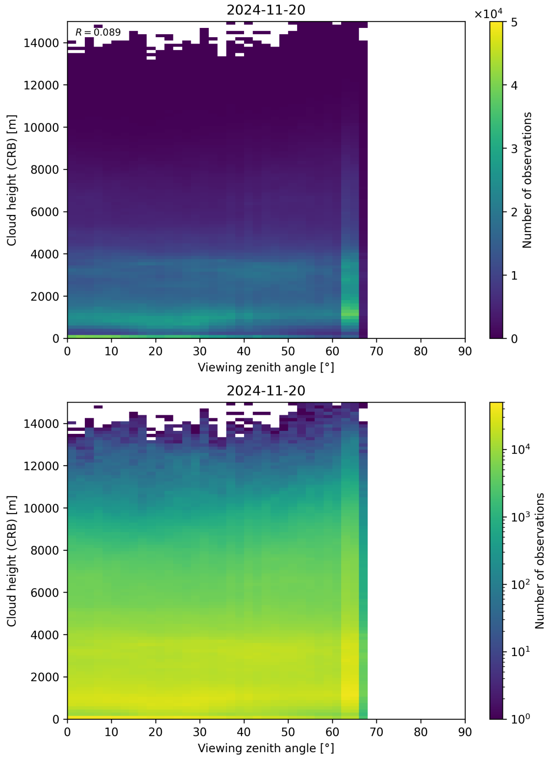
Figure 110: Scatter density plot of “Viewing zenith angle” against “Cloud height (CRB)” for 2024-11-20 to 2024-11-21.
