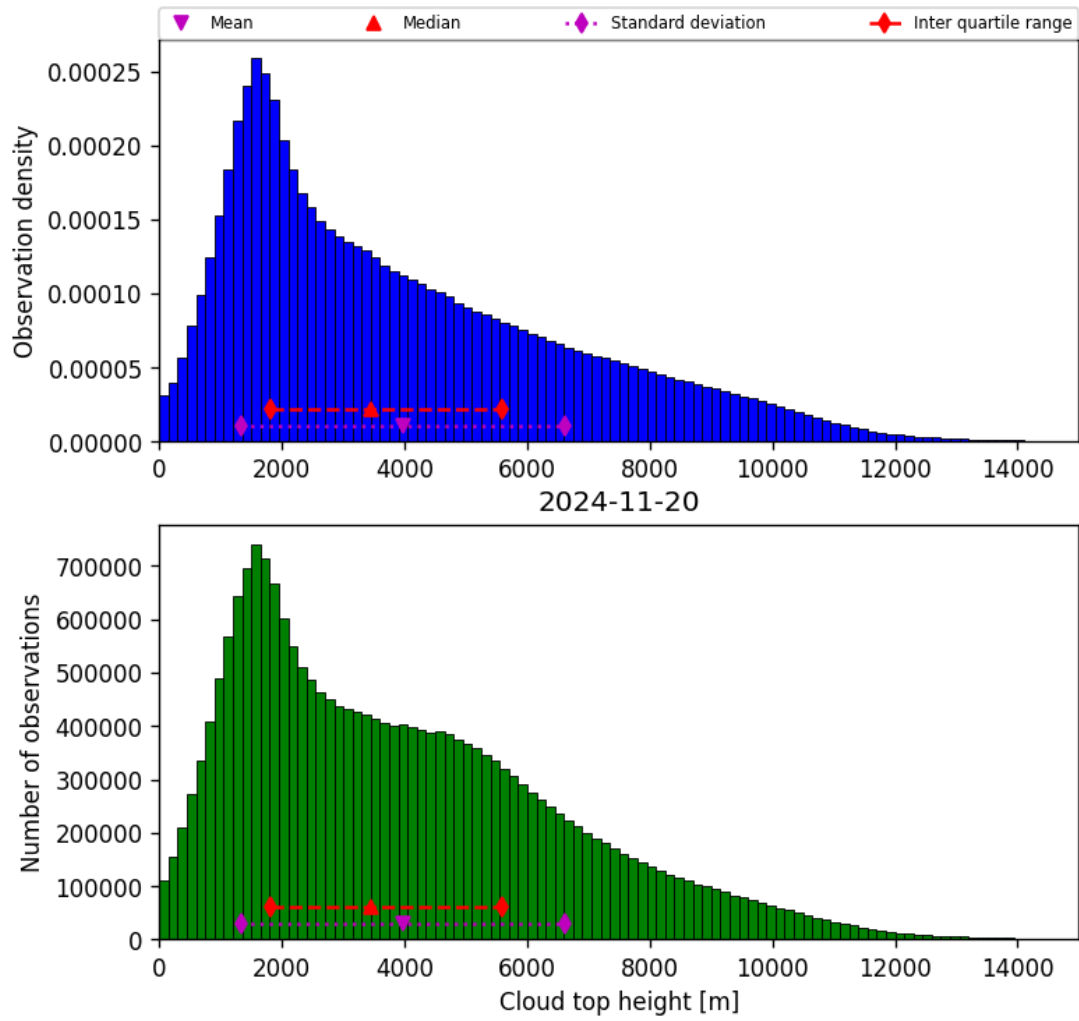
Figure 40: Histogram of “Cloud top height” for 2024-11-20 to 2024-11-21
