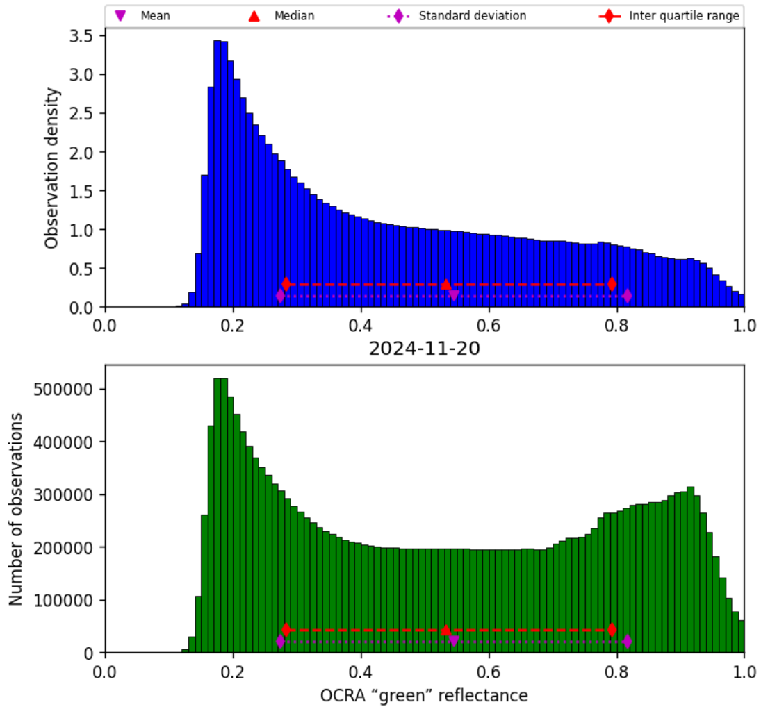
Figure 52: Histogram of “OCRA “green” reflectance” for 2024-11-20 to 2024-11-21
