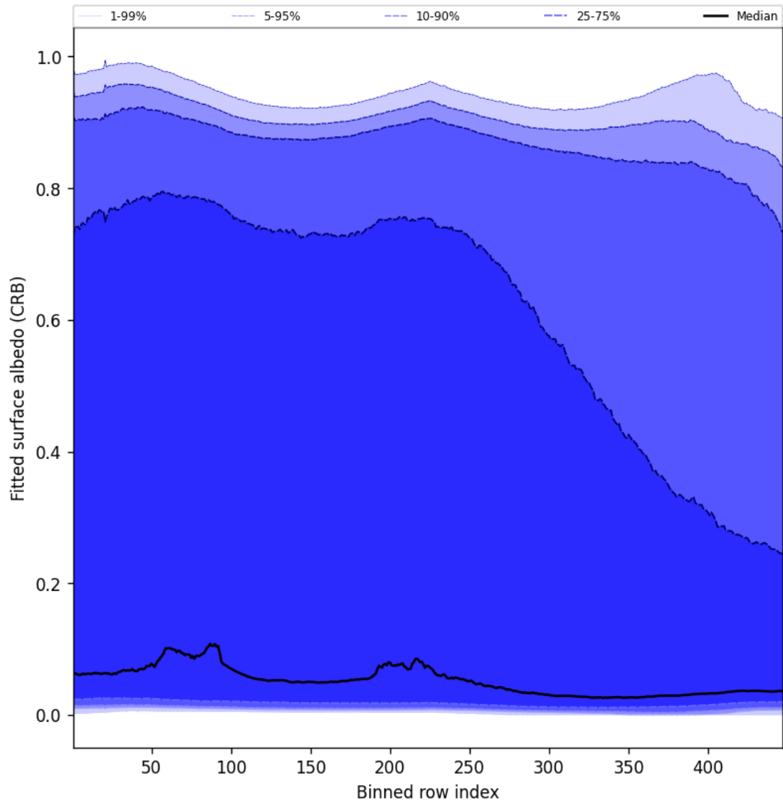
Figure 62: Along track statistics of “Fitted surface albedo (CRB)” for 2024-11-20 to 2024-11-21
