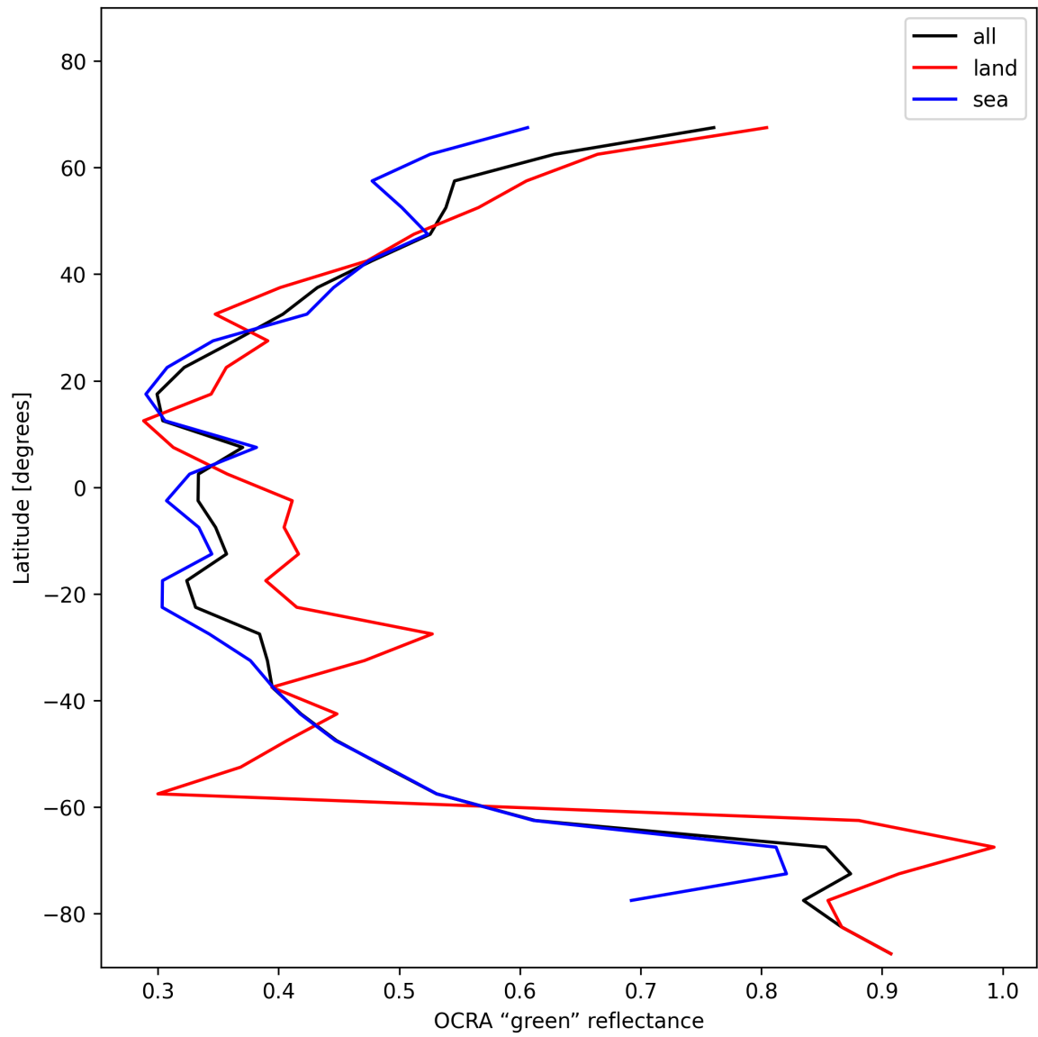
Figure 36: Zonal average of “OCRA “green” reflectance” for 2024-11-20 to 2024-11-21.
