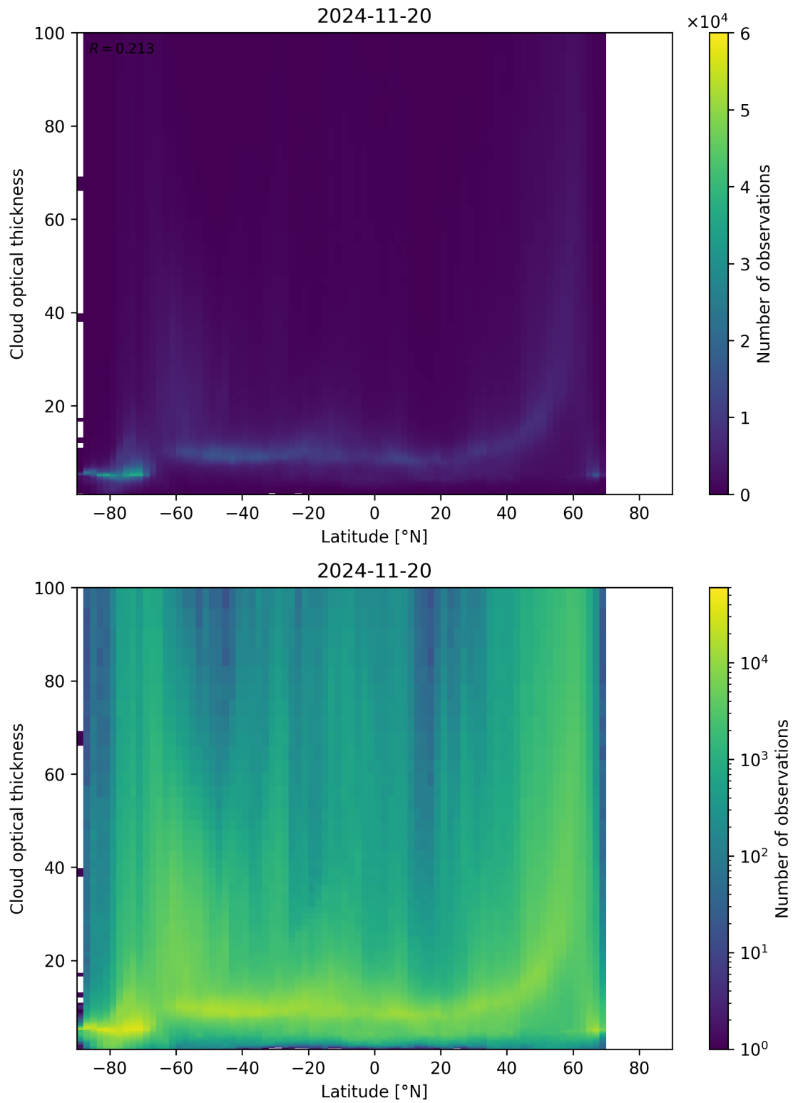
Figure 96: Scatter density plot of “Latitude” against “Cloud optical thickness” for 2024-11-20 to 2024-11-21.
