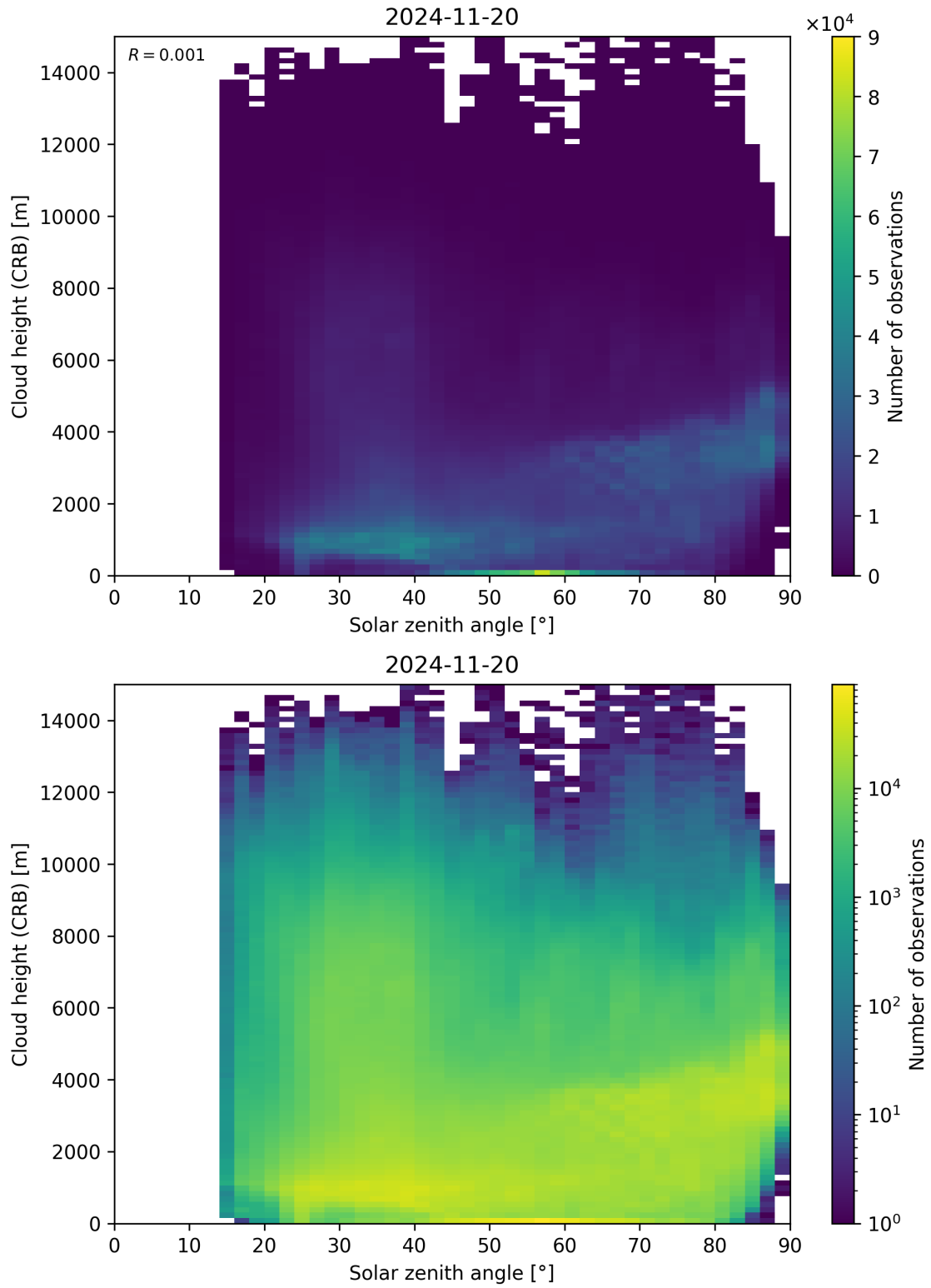
Figure 102: Scatter density plot of “Solar zenith angle” against “Cloud height (CRB)” for 2024-11-20 to 2024-11-21.
