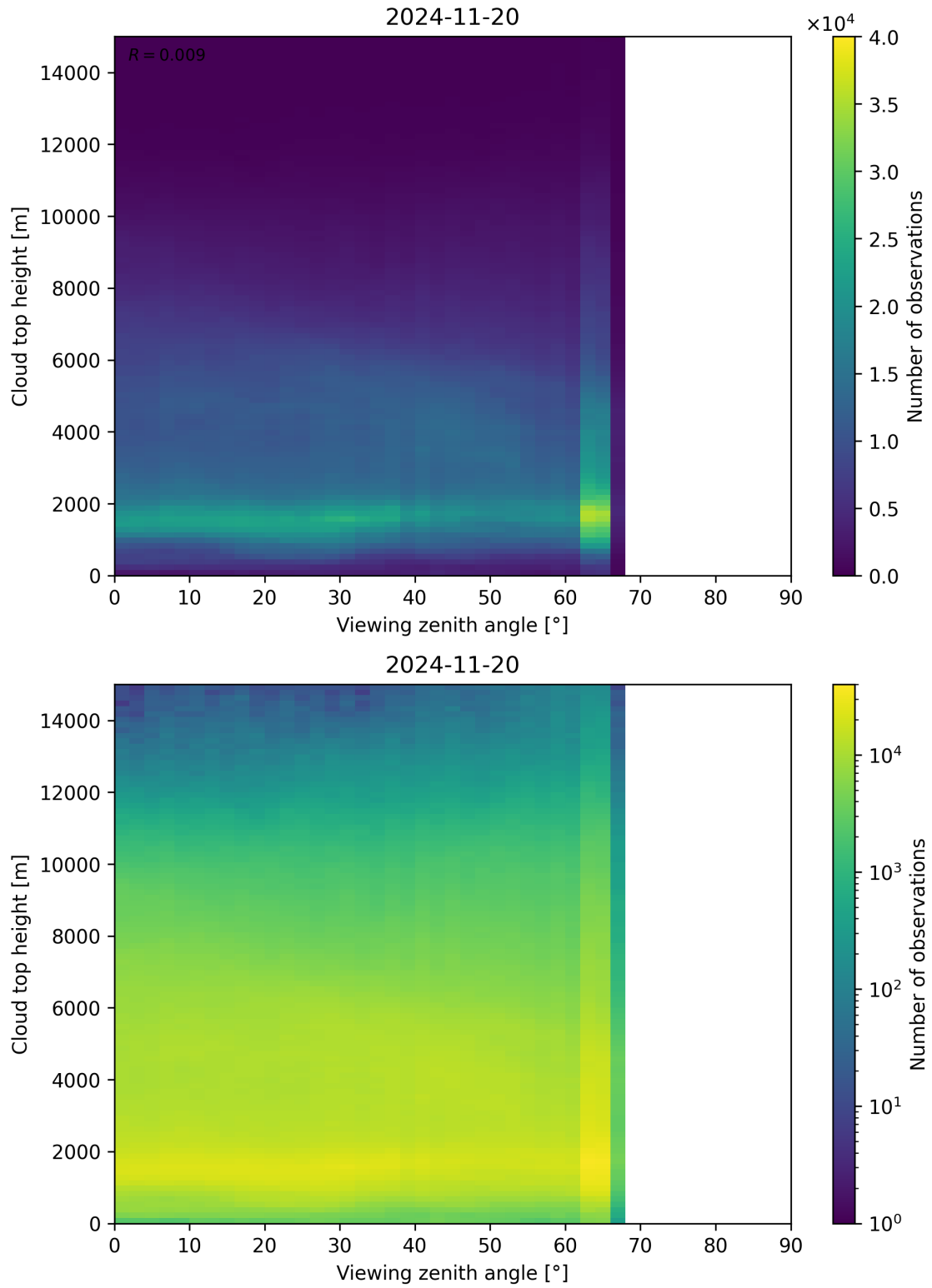
Figure 112: Scatter density plot of “Viewing zenith angle” against “Cloud top height” for 2024-11-20 to 2024-11-21.
