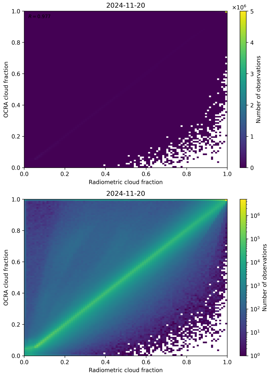
Figure 72: Scatter density plot of “Radiometric cloud fraction” against “OCRA cloud fraction” for 2024-11-20 to 2024-11-21.
