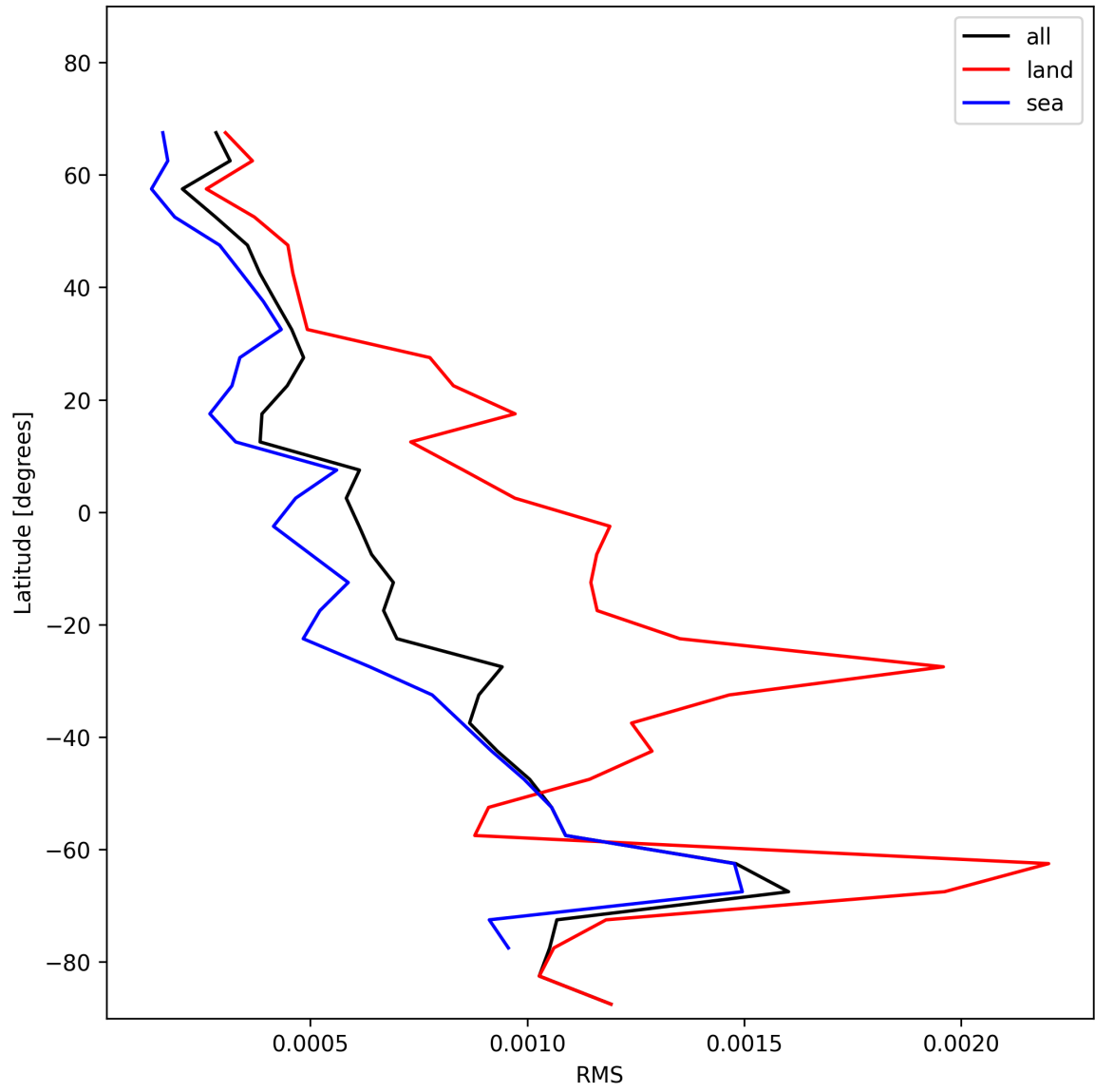
Figure 31: Zonal average of “RMS” for 2024-11-20 to 2024-11-21.
