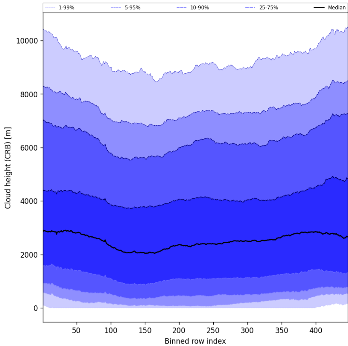
Figure 59: Along track statistics of “Cloud height (CRB)” for 2024-11-20 to 2024-11-21
