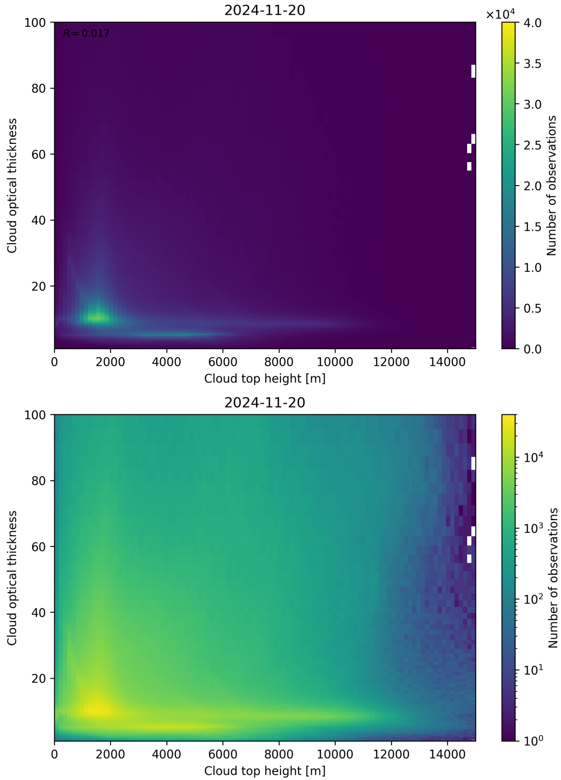
Figure 90: Scatter density plot of “Cloud top height” against “Cloud optical thickness” for 2024-11-20 to 2024-11-21.
