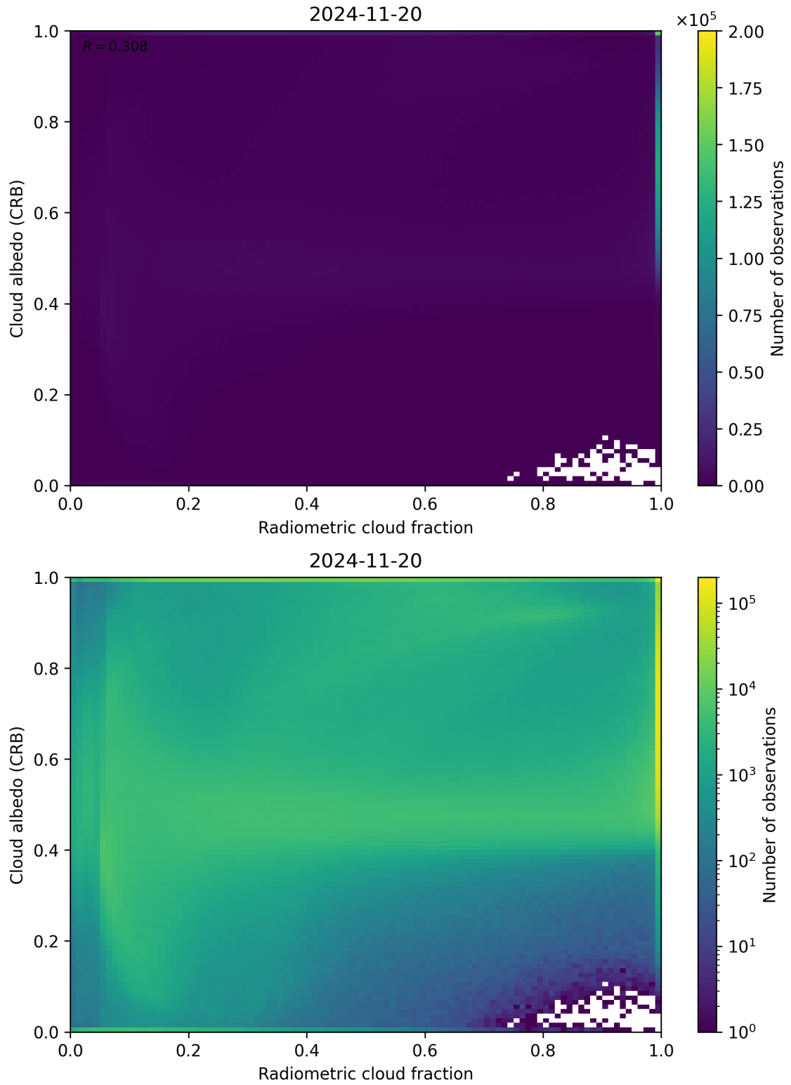
Figure 71: Scatter density plot of “Radiometric cloud fraction” against “Cloud albedo (CRB)” for 2024-11-20 to 2024-11-21.
