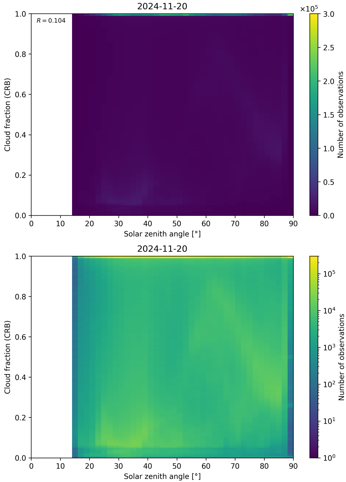
Figure 101: Scatter density plot of “Solar zenith angle” against “Cloud fraction (CRB)” for 2024-11-20 to 2024-11-21.
