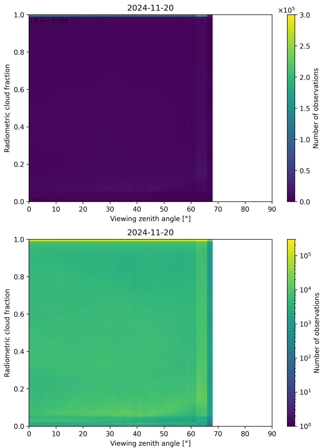
Figure 107: Scatter density plot of “Viewing zenith angle” against “Radiometric cloud fraction” for 2024-11-20 to 2024-11-21.
