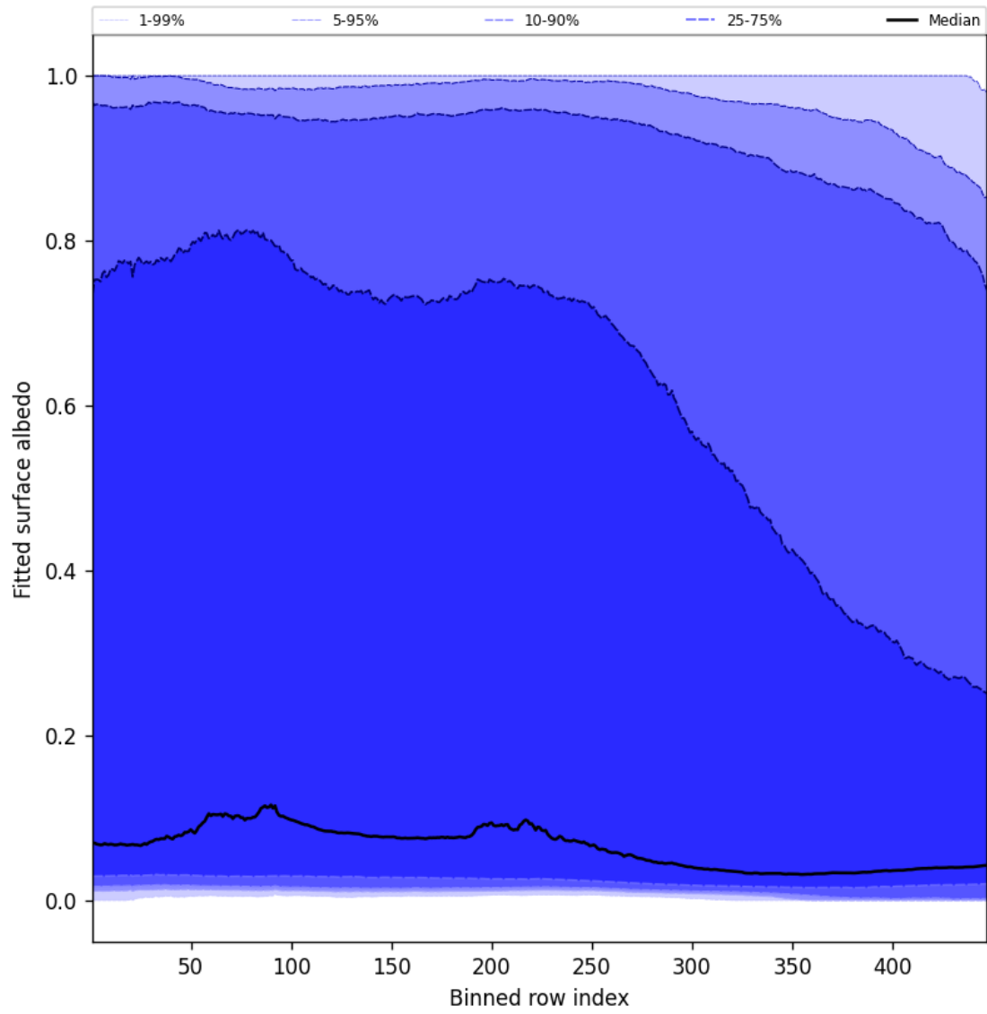
Figure 61: Along track statistics of “Fitted surface albedo” for 2024-11-20 to 2024-11-21
