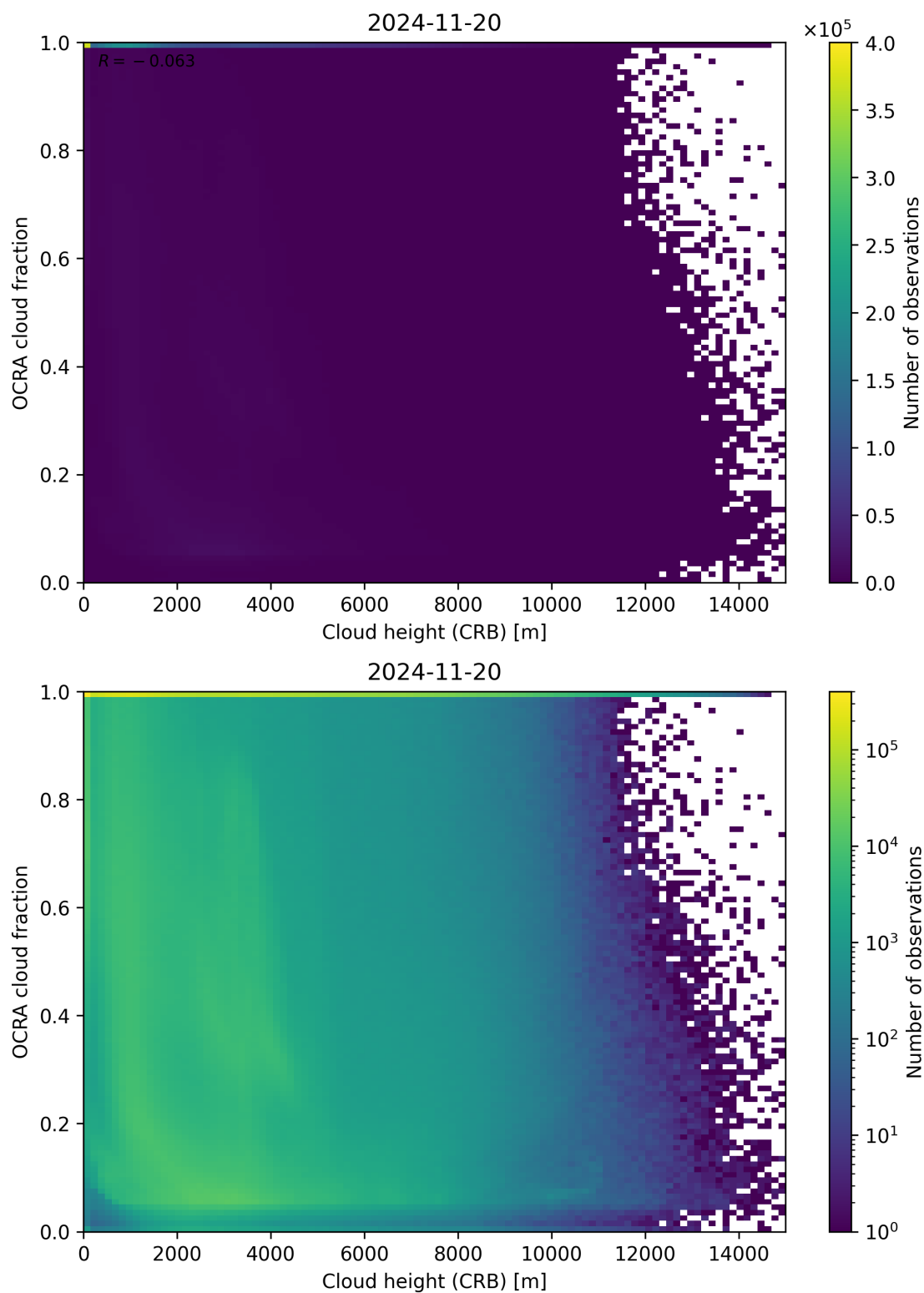
Figure 81: Scatter density plot of “Cloud height (CRB)” against “OCRA cloud fraction” for 2024-11-20 to 2024-11-21.
