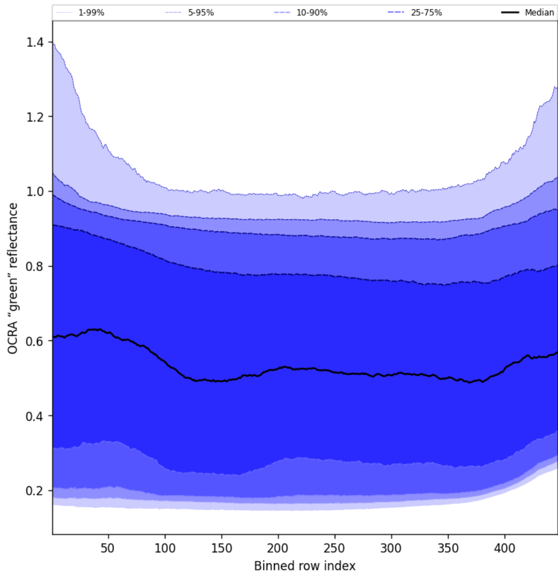
Figure 68: Along track statistics of “OCRA “green” reflectance” for 2024-11-20 to 2024-11-21
