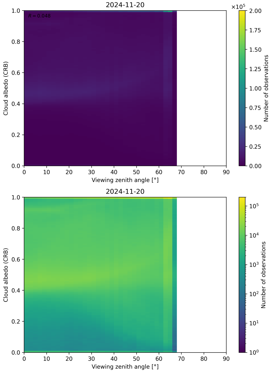
Figure 106: Scatter density plot of “Viewing zenith angle” against “Cloud albedo (CRB)” for 2024-11-20 to 2024-11-21.
