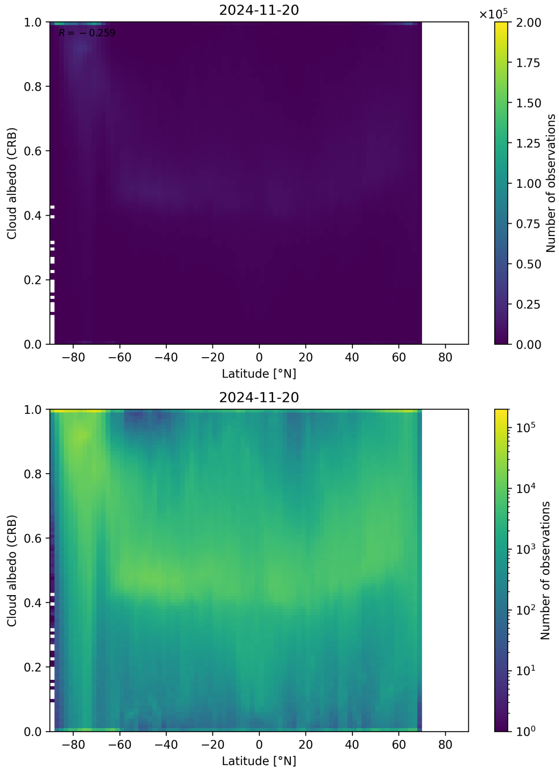
Figure 91: Scatter density plot of “Latitude” against “Cloud albedo (CRB)” for 2024-11-20 to 2024-11-21.
