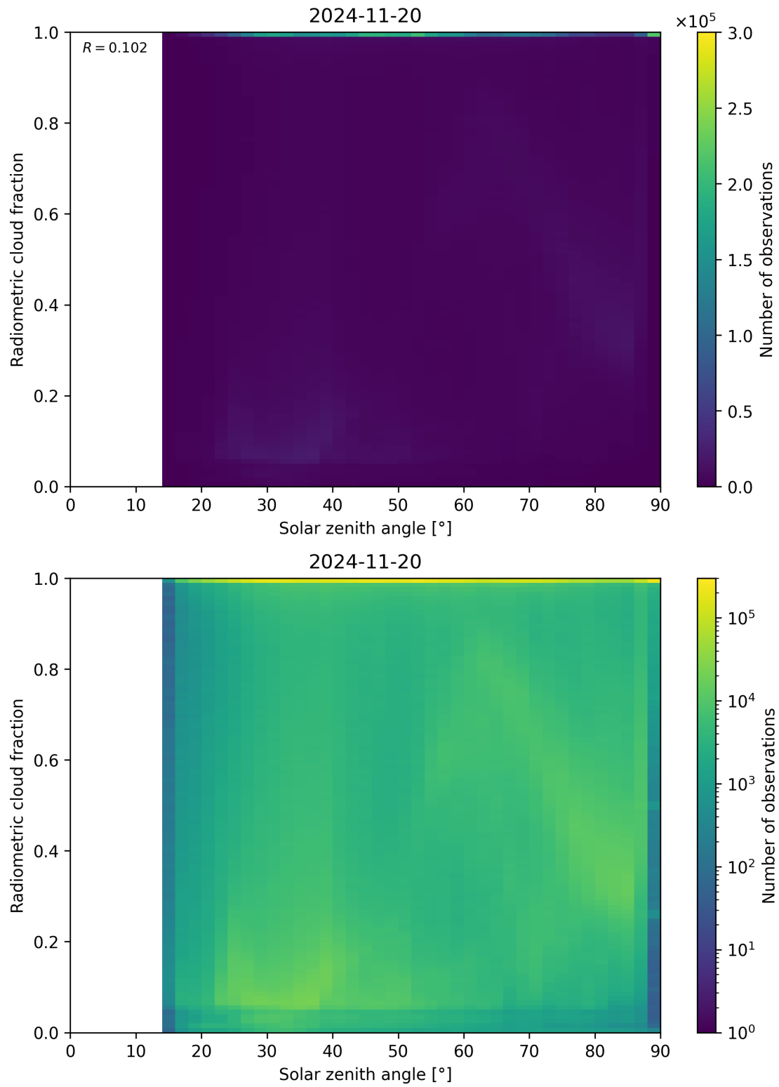
Figure 99: Scatter density plot of “Solar zenith angle” against “Radiometric cloud fraction” for 2024-11-20 to 2024-11-21.
