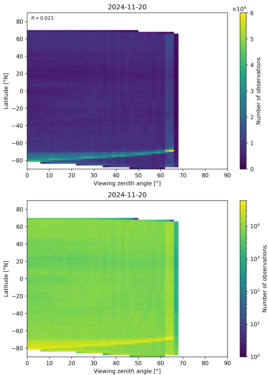
Figure 113: Scatter density plot of “Viewing zenith angle” against “Latitude” for 2024-11-20 to 2024-11-21.
