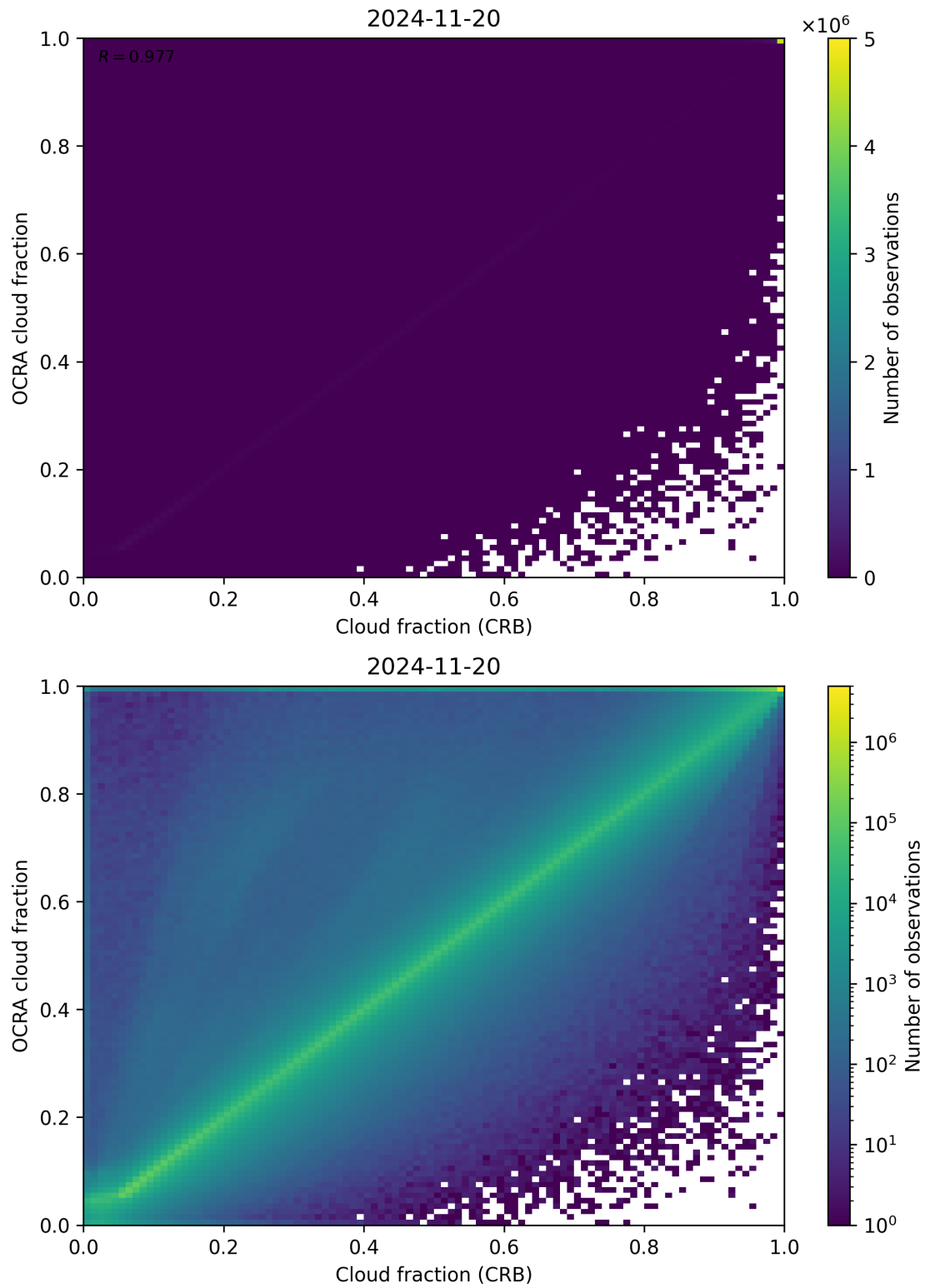
Figure 78: Scatter density plot of “Cloud fraction (CRB)” against “OCRA cloud fraction” for 2024-11-20 to 2024-11-21.
