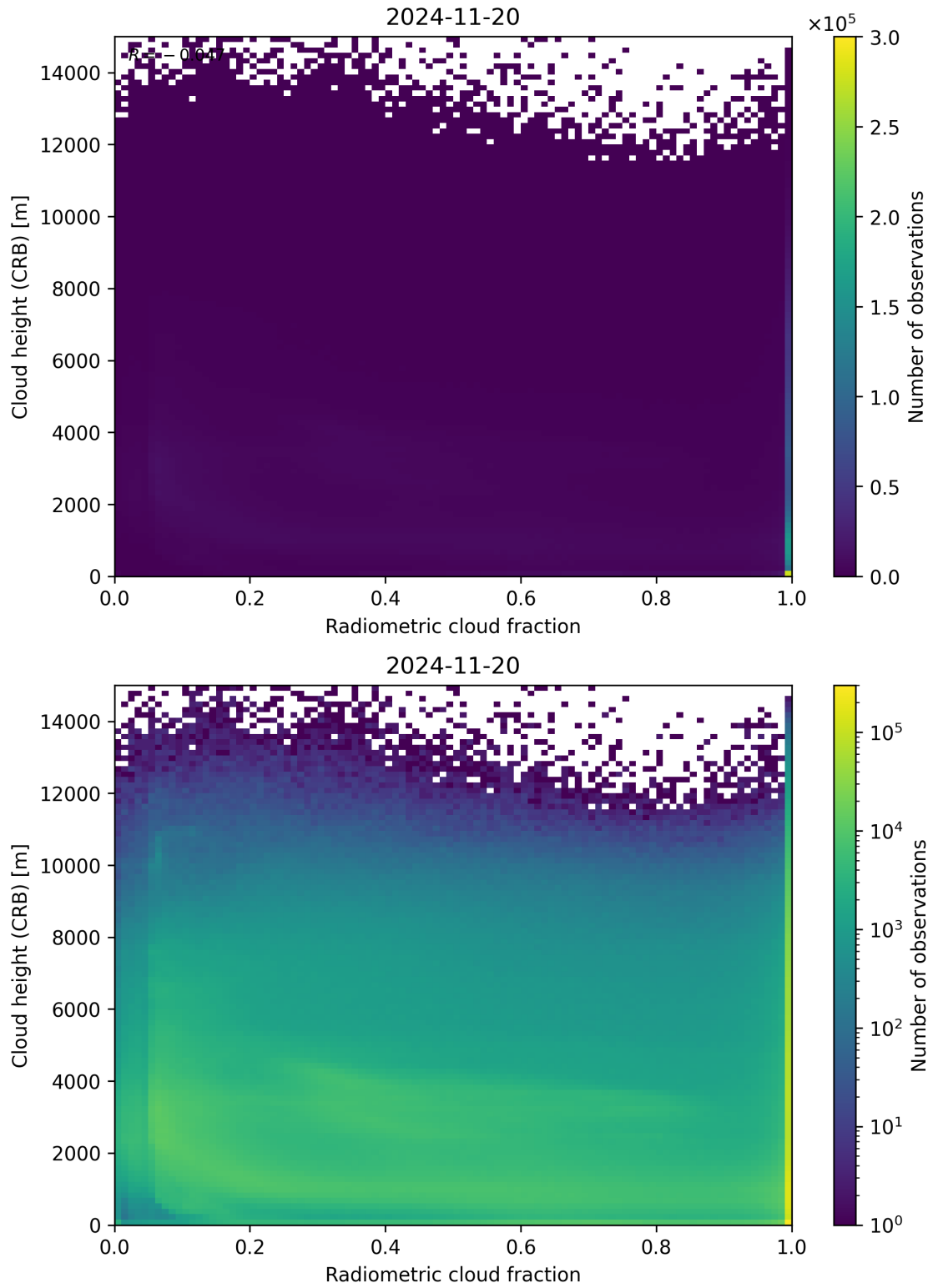
Figure 74: Scatter density plot of “Radiometric cloud fraction” against “Cloud height (CRB)” for 2024-11-20 to 2024-11-21.
