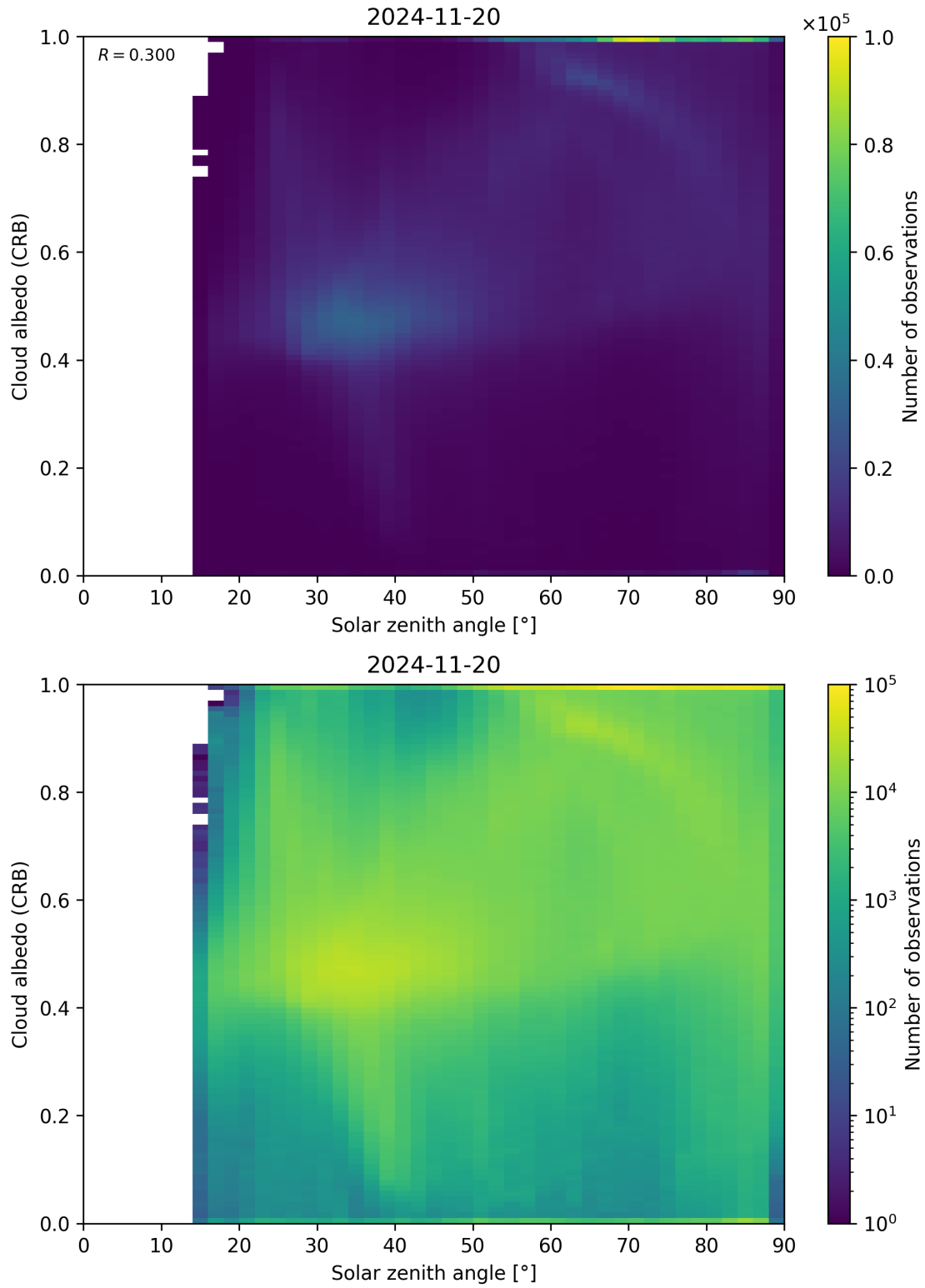
Figure 98: Scatter density plot of “Solar zenith angle” against “Cloud albedo (CRB)” for 2024-11-20 to 2024-11-21.
