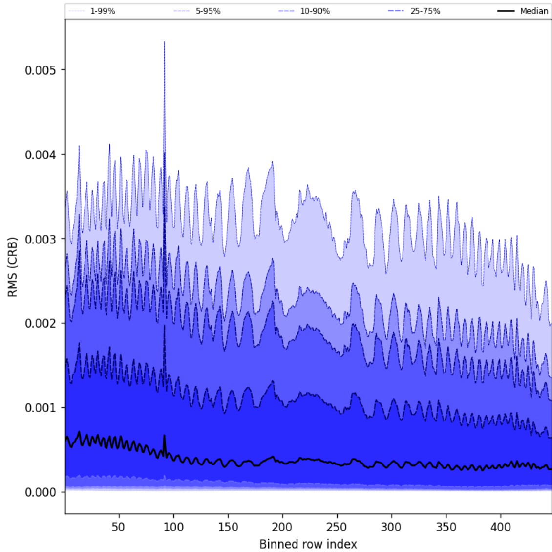
Figure 64: Along track statistics of “RMS (CRB)” for 2024-11-20 to 2024-11-21
