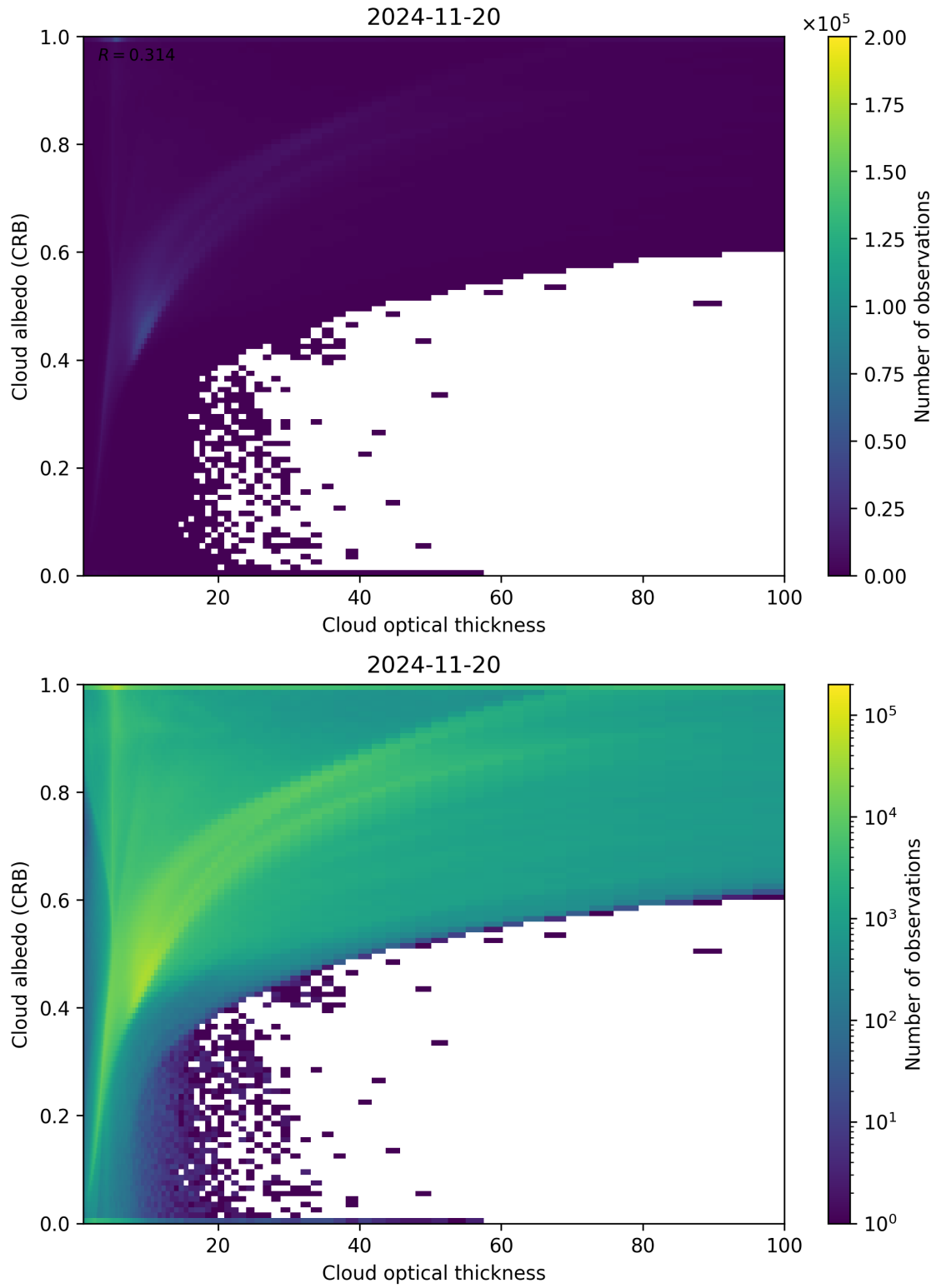
Figure 82: Scatter density plot of “Cloud optical thickness” against “Cloud albedo (CRB)” for 2024-11-20 to 2024-11-21.
