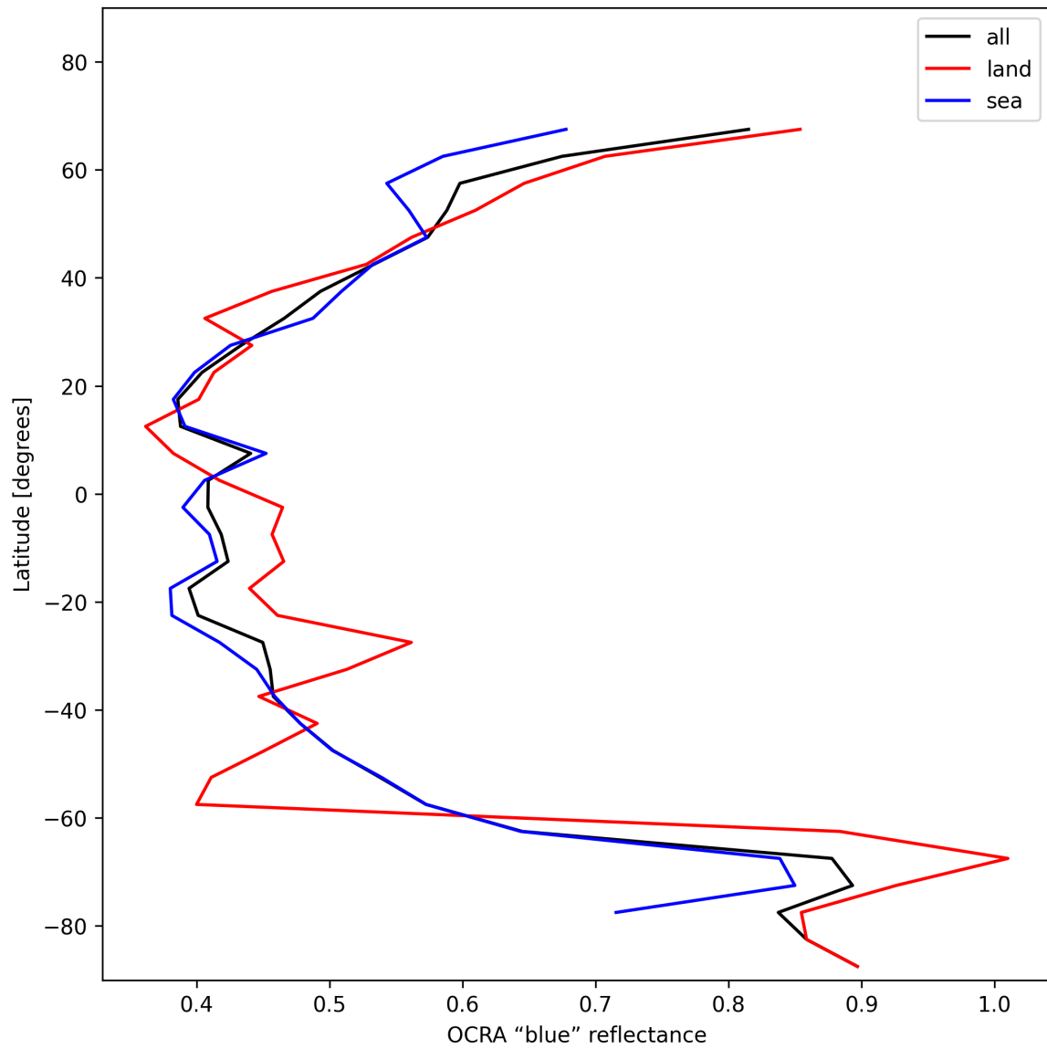
Figure 35: Zonal average of “OCRA “blue” reflectance” for 2024-11-20 to 2024-11-21.
