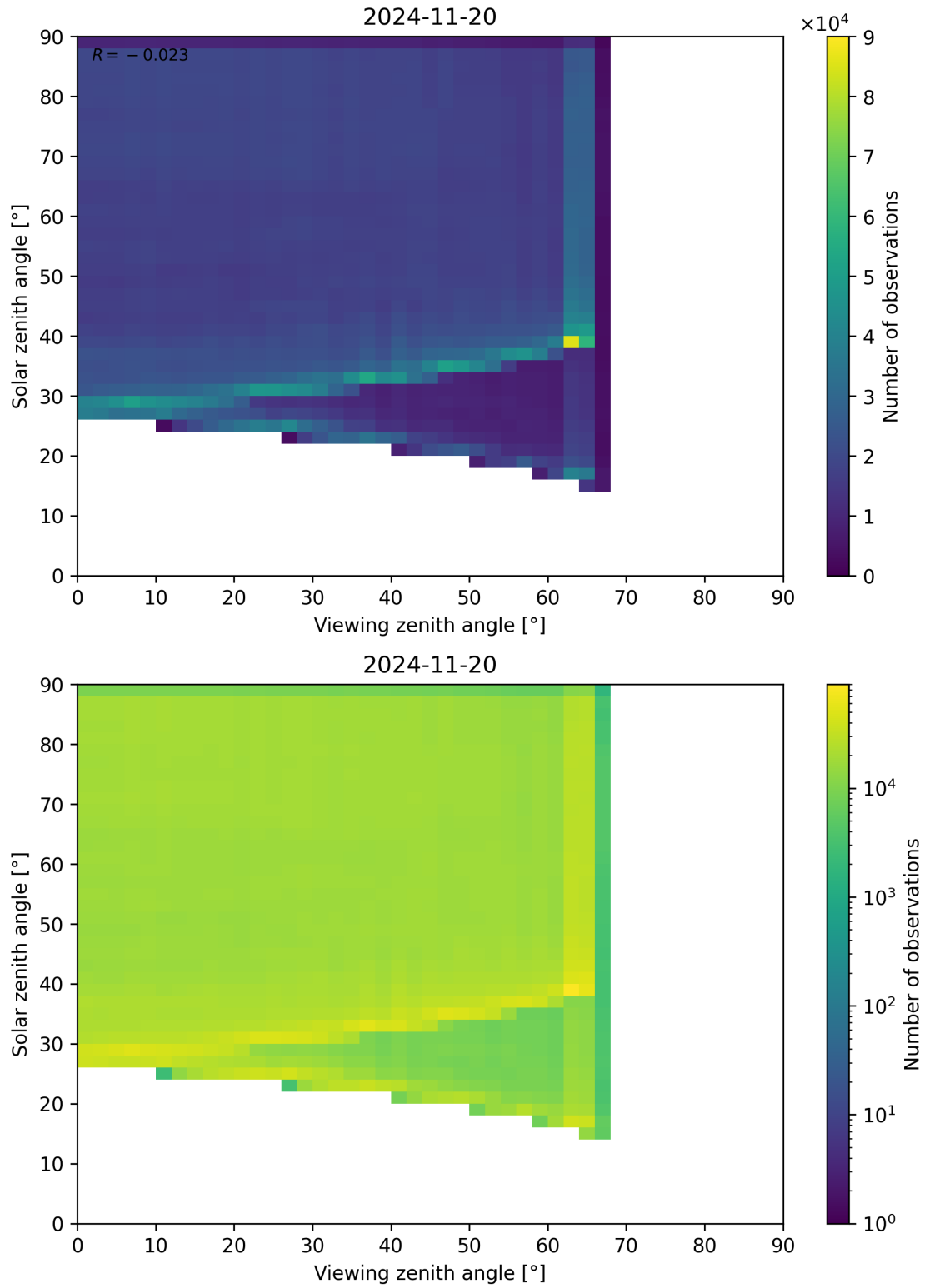
Figure 114: Scatter density plot of “Viewing zenith angle” against “Solar zenith angle” for 2024-11-20 to 2024-11-21.
