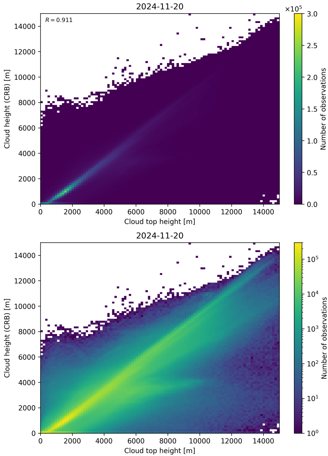
Figure 89: Scatter density plot of “Cloud top height” against “Cloud height (CRB)” for 2024-11-20 to 2024-11-21.
