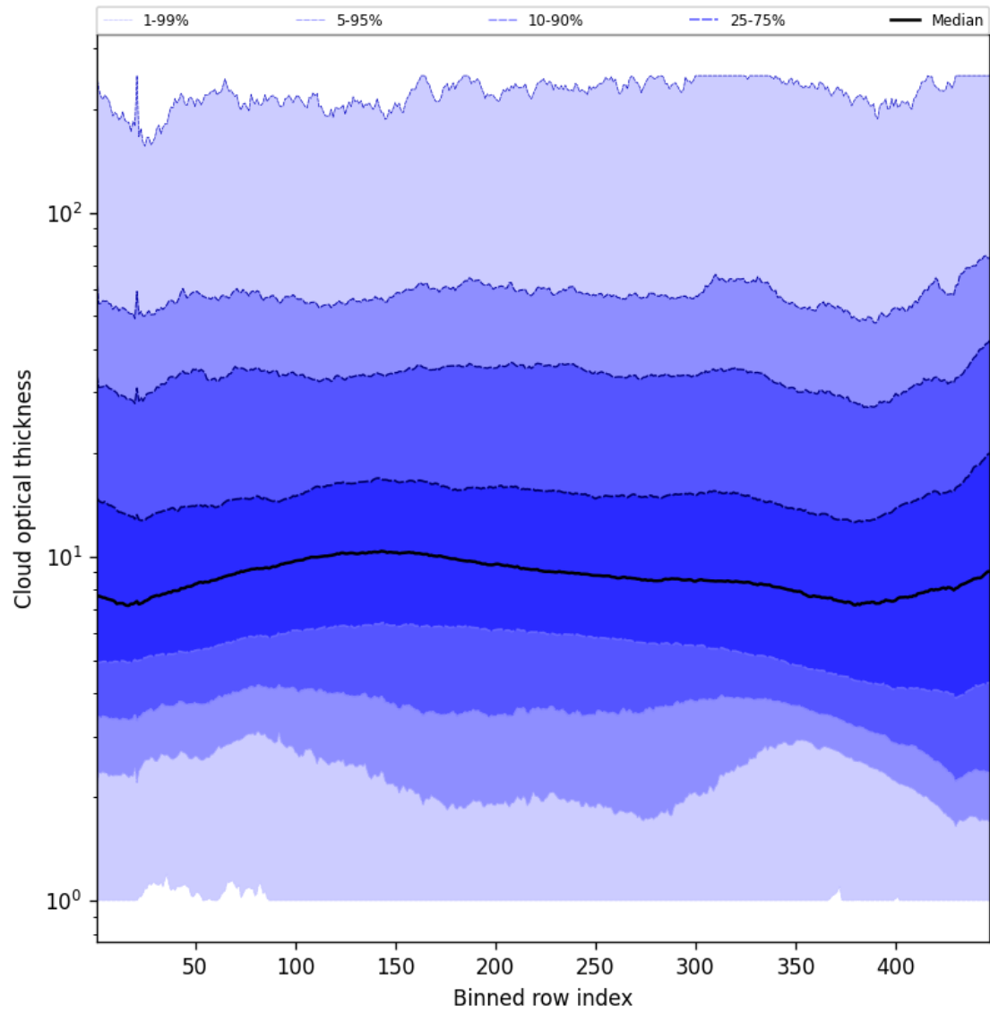
Figure 57: Along track statistics of “Cloud optical thickness” for 2024-11-20 to 2024-11-21
