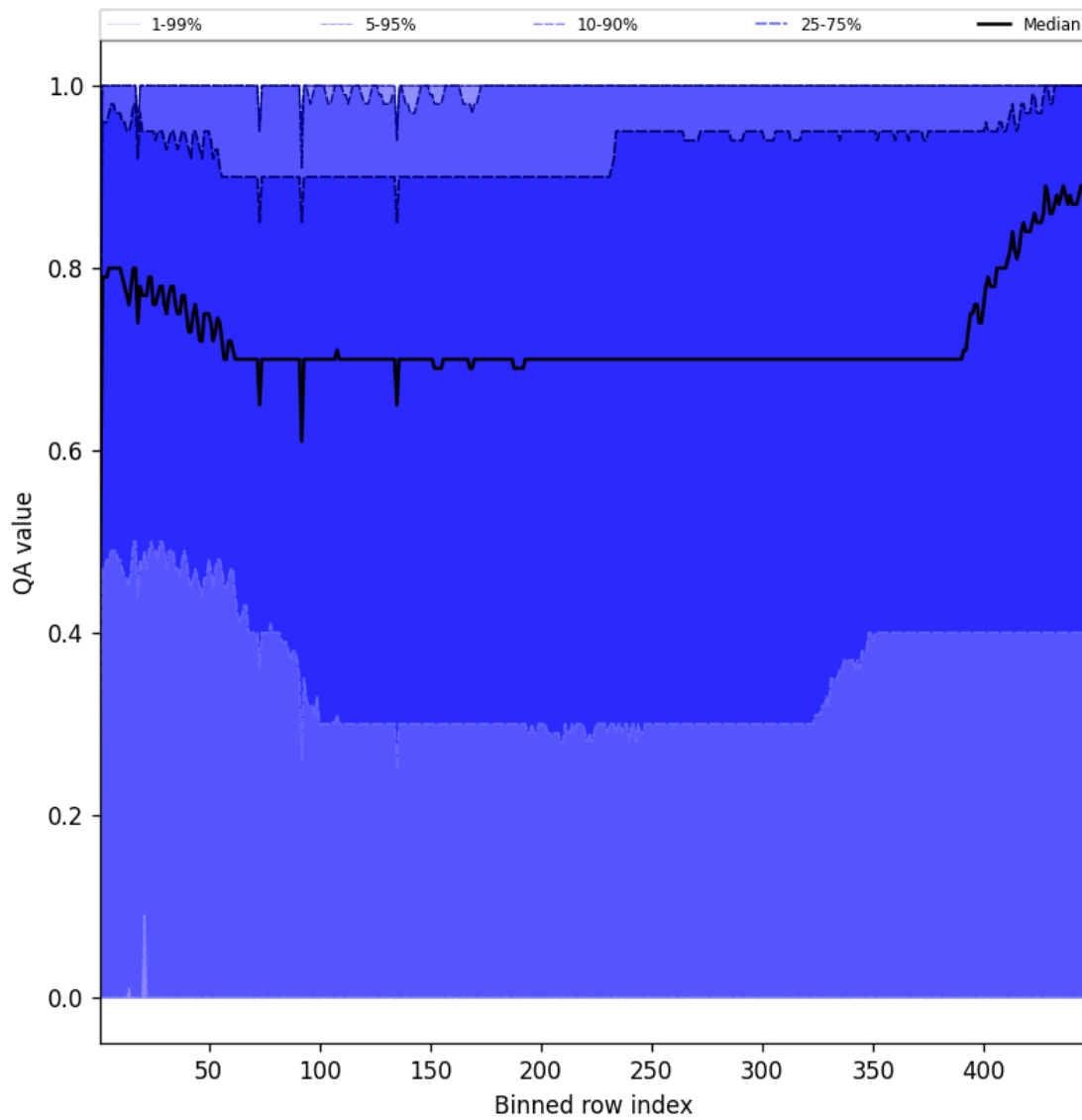
Figure 54: Along track statistics of “QA value” for 2024-11-20 to 2024-11-21
