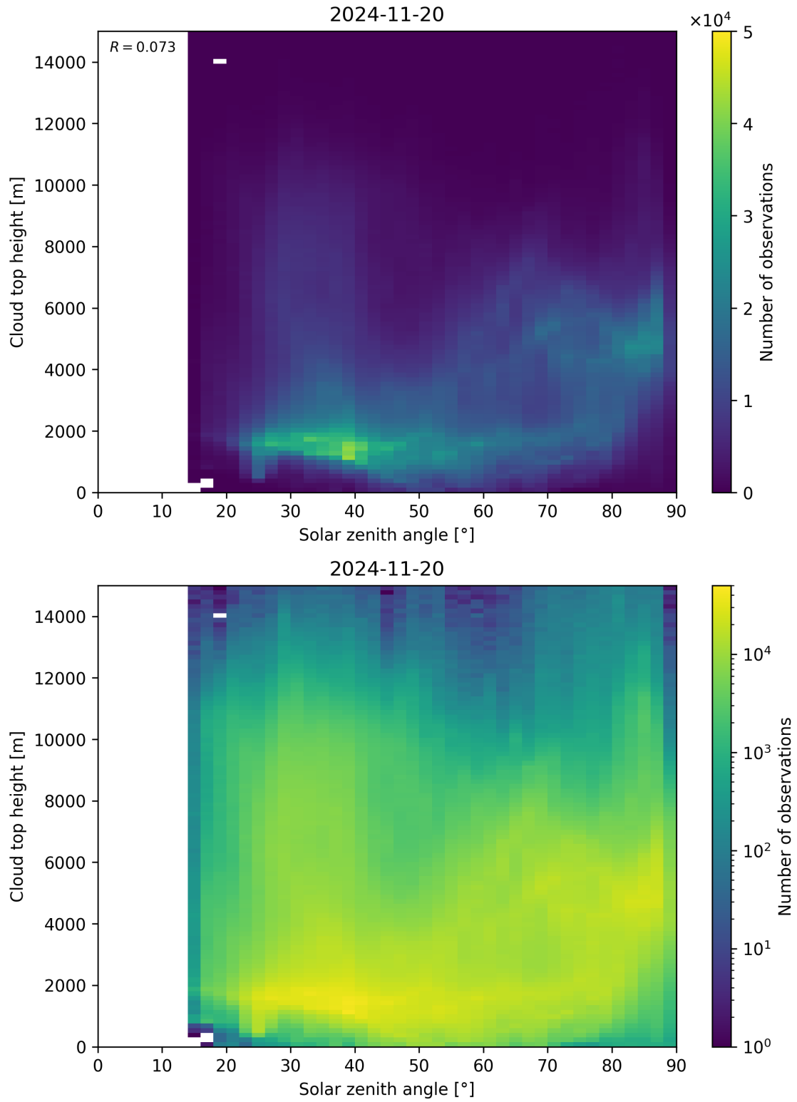
Figure 104: Scatter density plot of “Solar zenith angle” against “Cloud top height” for 2024-11-20 to 2024-11-21.
