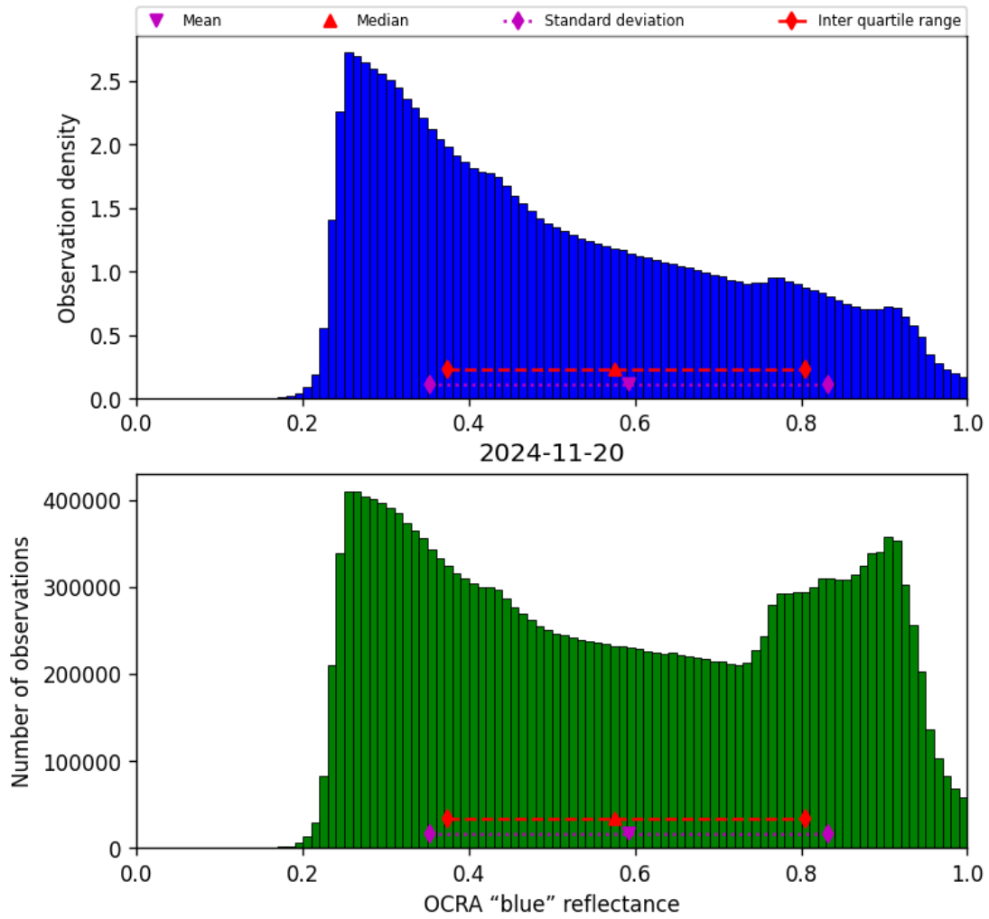
Figure 51: Histogram of “OCRA “blue” reflectance” for 2024-11-20 to 2024-11-21
