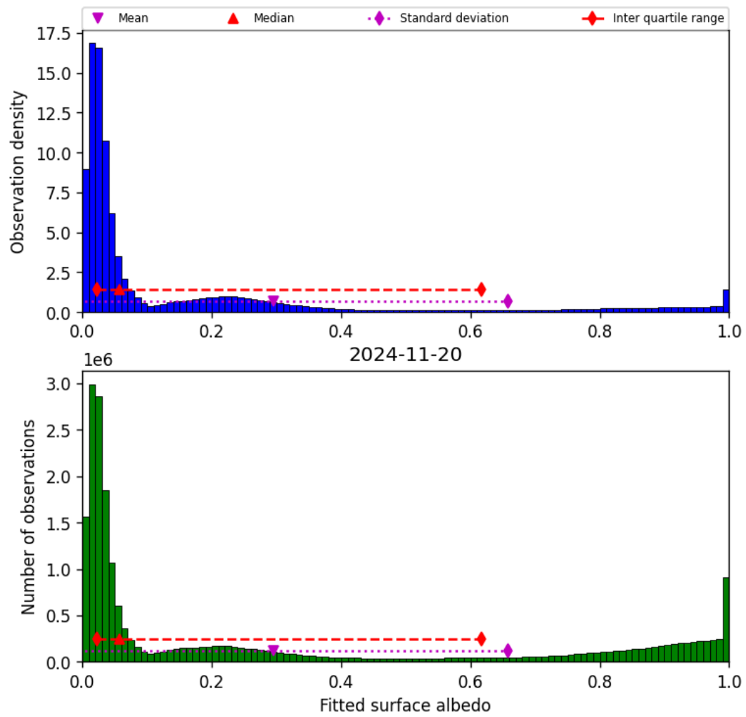
Figure 45: Histogram of “Fitted surface albedo” for 2024-11-20 to 2024-11-21
