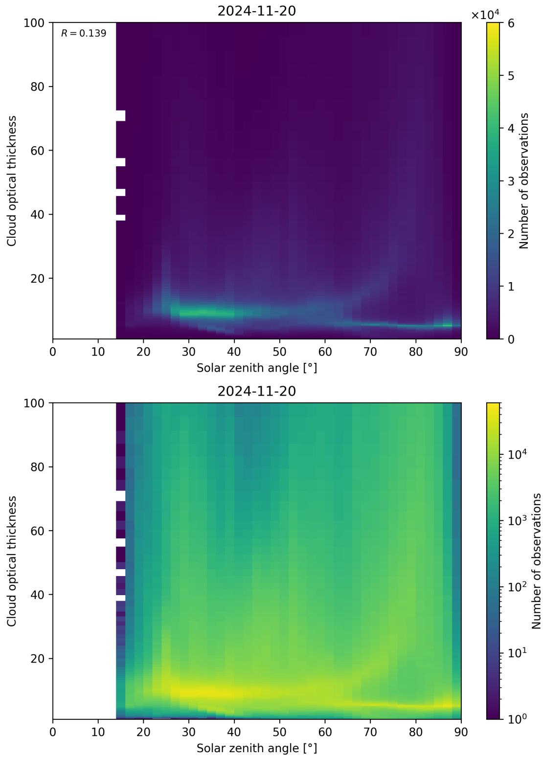
Figure 103: Scatter density plot of “Solar zenith angle” against “Cloud optical thickness” for 2024-11-20 to 2024-11-21.
