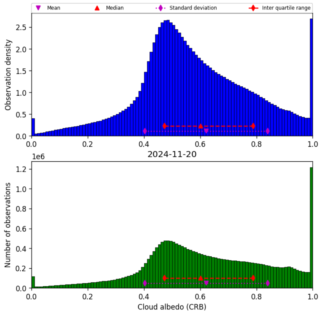
Figure 44: Histogram of “Cloud albedo (CRB)” for 2024-11-20 to 2024-11-21
