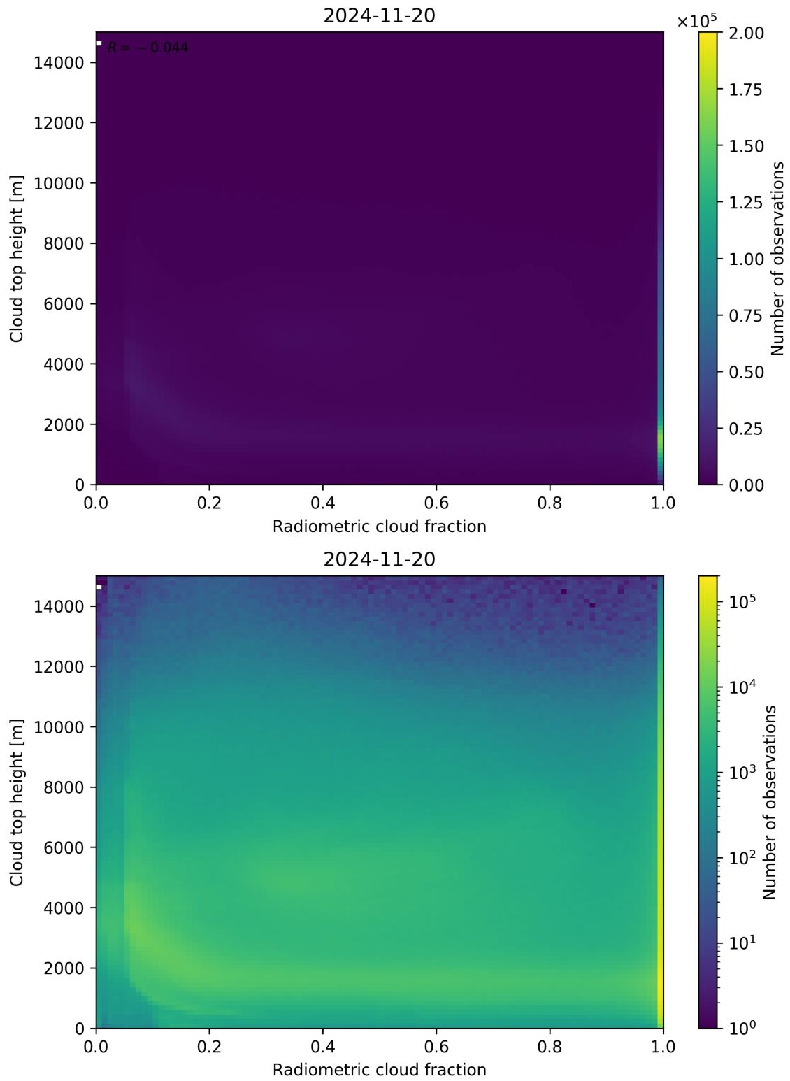
Figure 76: Scatter density plot of “Radiometric cloud fraction” against “Cloud top height” for 2024-11-20 to 2024-11-21.
