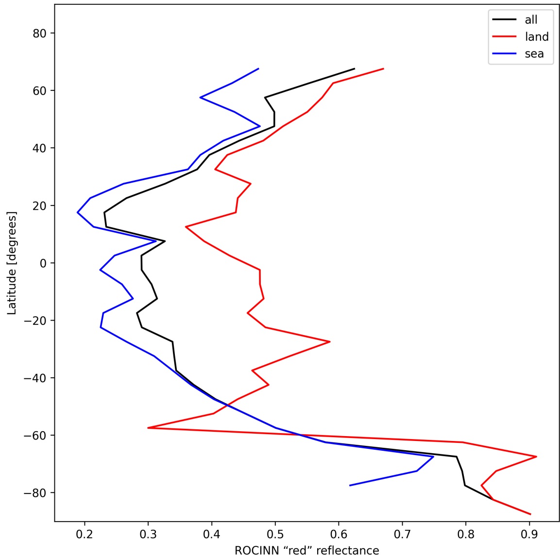
Figure 37: Zonal average of “ROCINN “red” reflectance” for 2024-11-20 to 2024-11-21.
