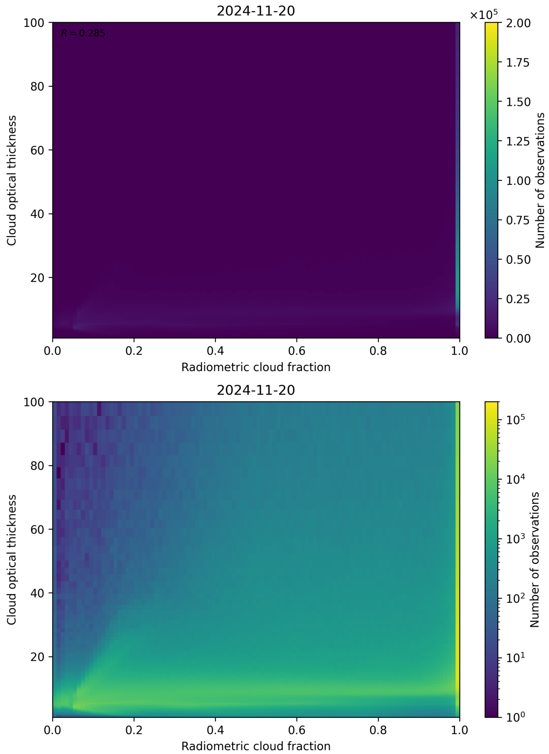
Figure 75: Scatter density plot of “Radiometric cloud fraction” against “Cloud optical thickness” for 2024-11-20 to 2024-11-21.
