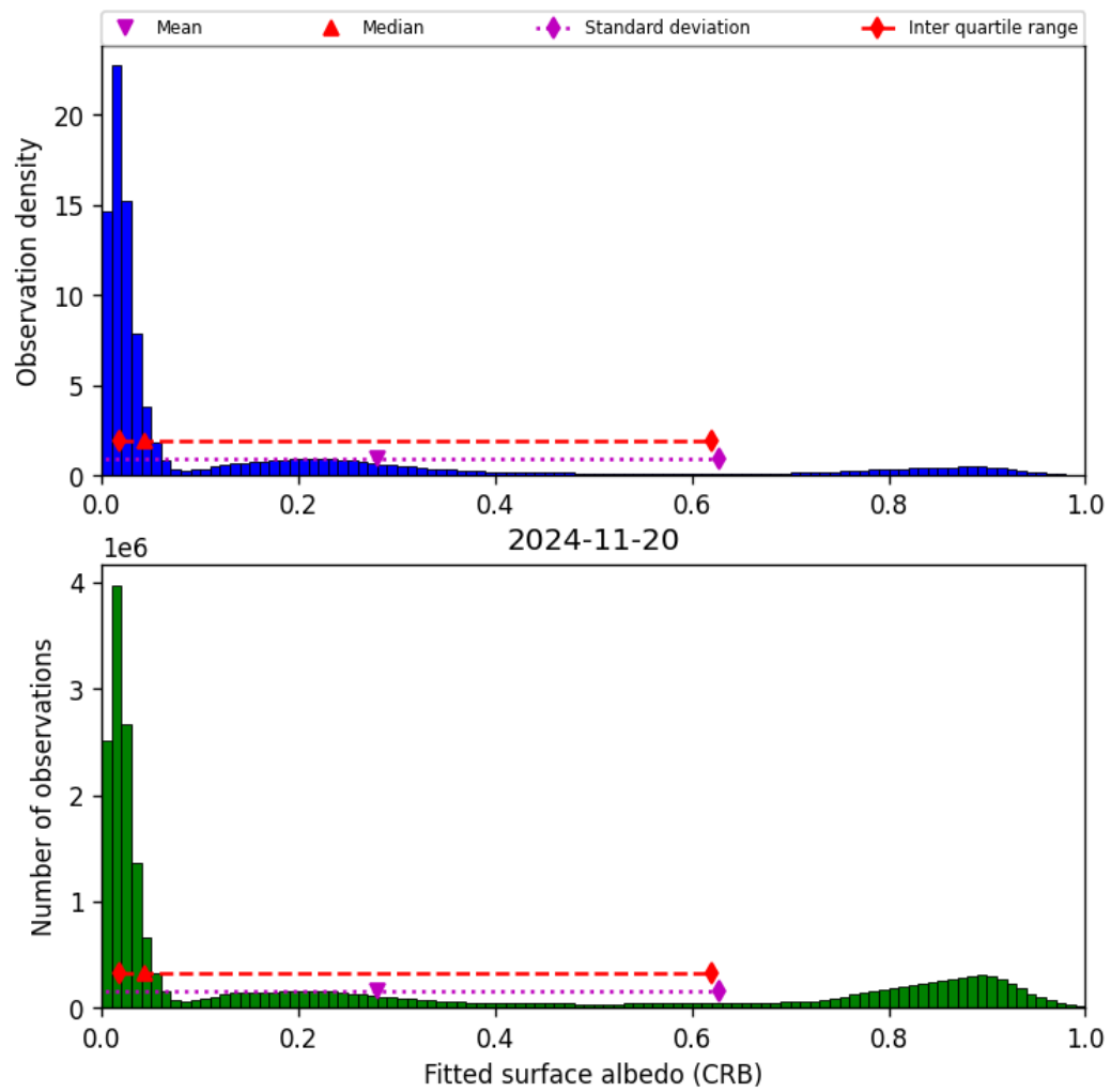
Figure 46: Histogram of “Fitted surface albedo (CRB)” for 2024-11-20 to 2024-11-21
