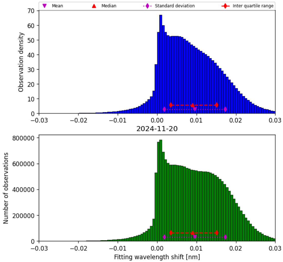
Figure 49: Histogram of “Fitting wavelength shift” for 2024-11-20 to 2024-11-21
