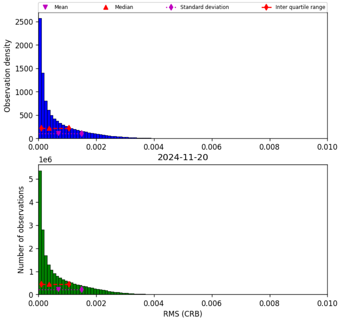
Figure 48: Histogram of “RMS (CRB)” for 2024-11-20 to 2024-11-21
