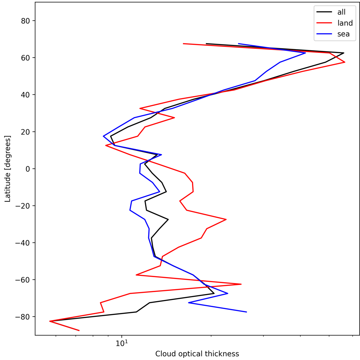
Figure 25: Zonal average of “Cloud optical thickness” for 2024-11-20 to 2024-11-21.
