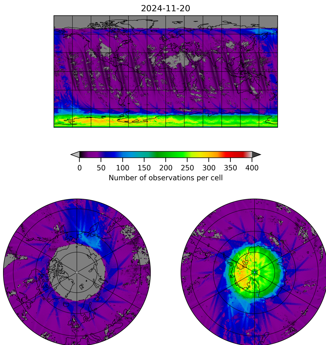
Figure 21: Map of the number of observations for 2024-11-20 to 2024-11-21
