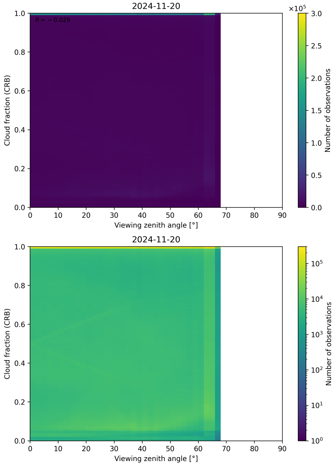
Figure 109: Scatter density plot of “Viewing zenith angle” against “Cloud fraction (CRB)” for 2024-11-20 to 2024-11-21.
