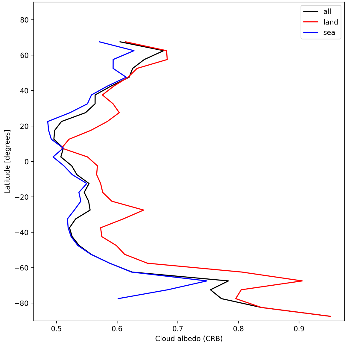
Figure 28: Zonal average of “Cloud albedo (CRB)” for 2024-11-20 to 2024-11-21.
