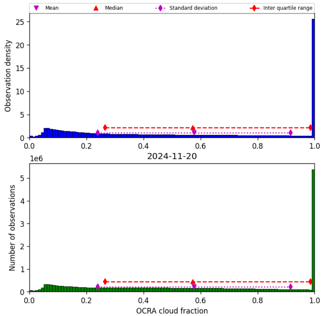
Figure 50: Histogram of “OCRA cloud fraction” for 2024-11-20 to 2024-11-21
