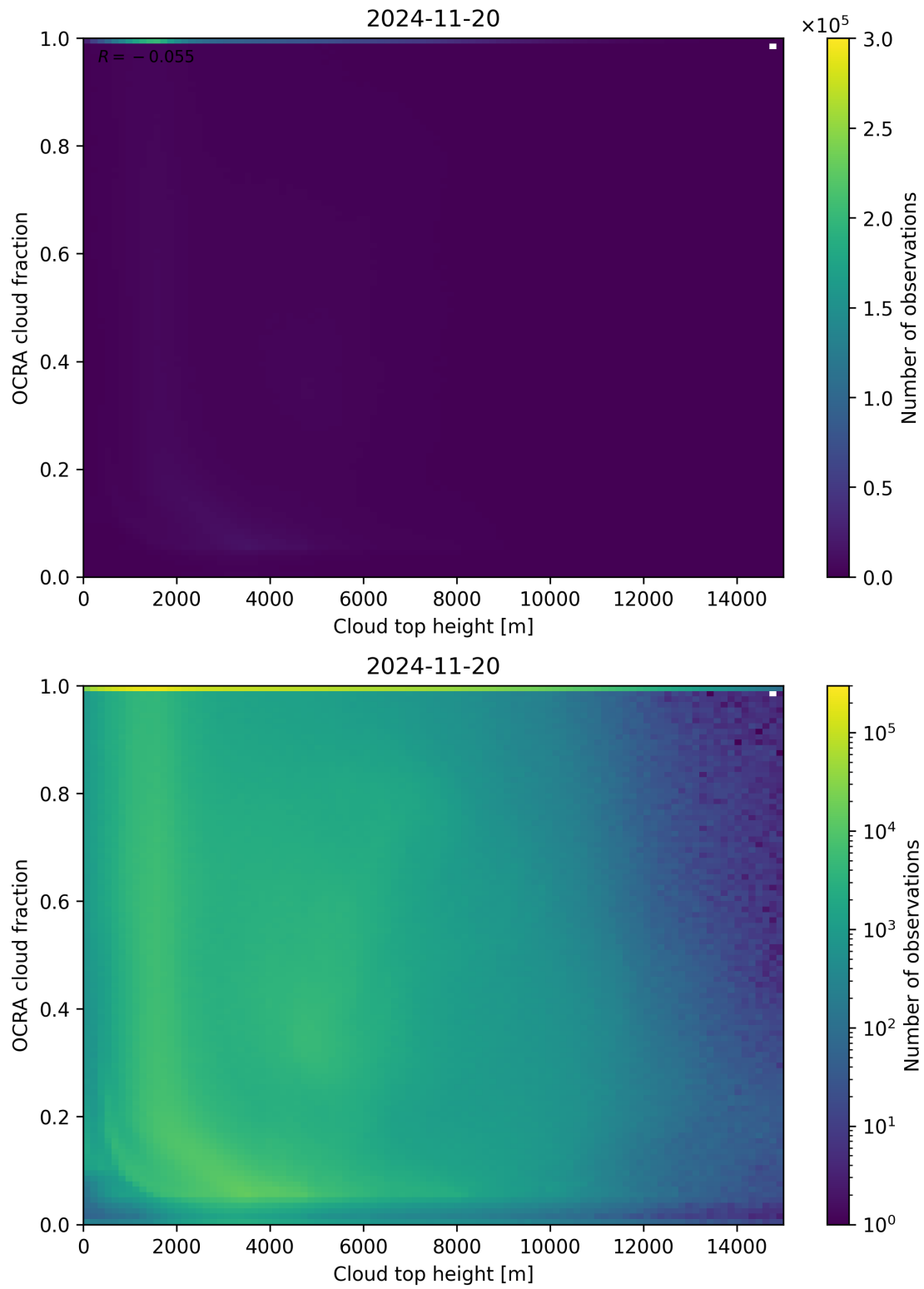
Figure 87: Scatter density plot of “Cloud top height” against “OCRA cloud fraction” for 2024-11-20 to 2024-11-21.
