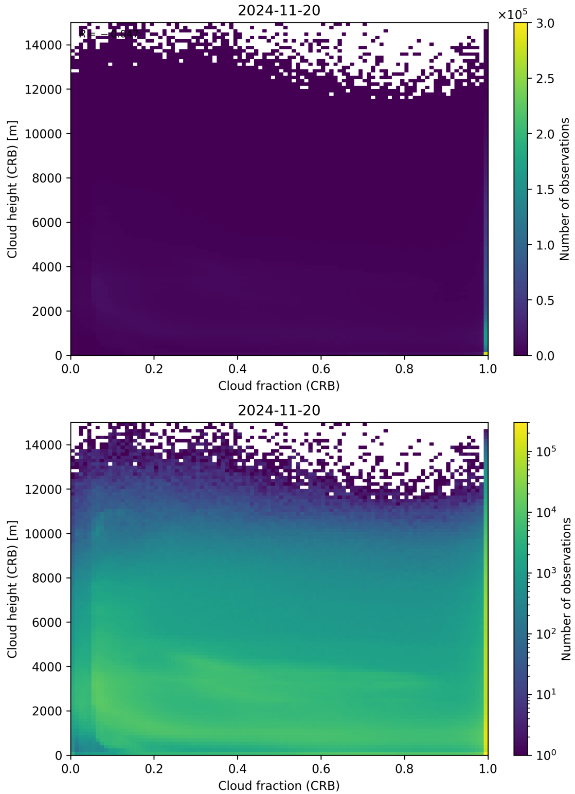
Figure 79: Scatter density plot of “Cloud fraction (CRB)” against “Cloud height (CRB)” for 2024-11-20 to 2024-11-21.
