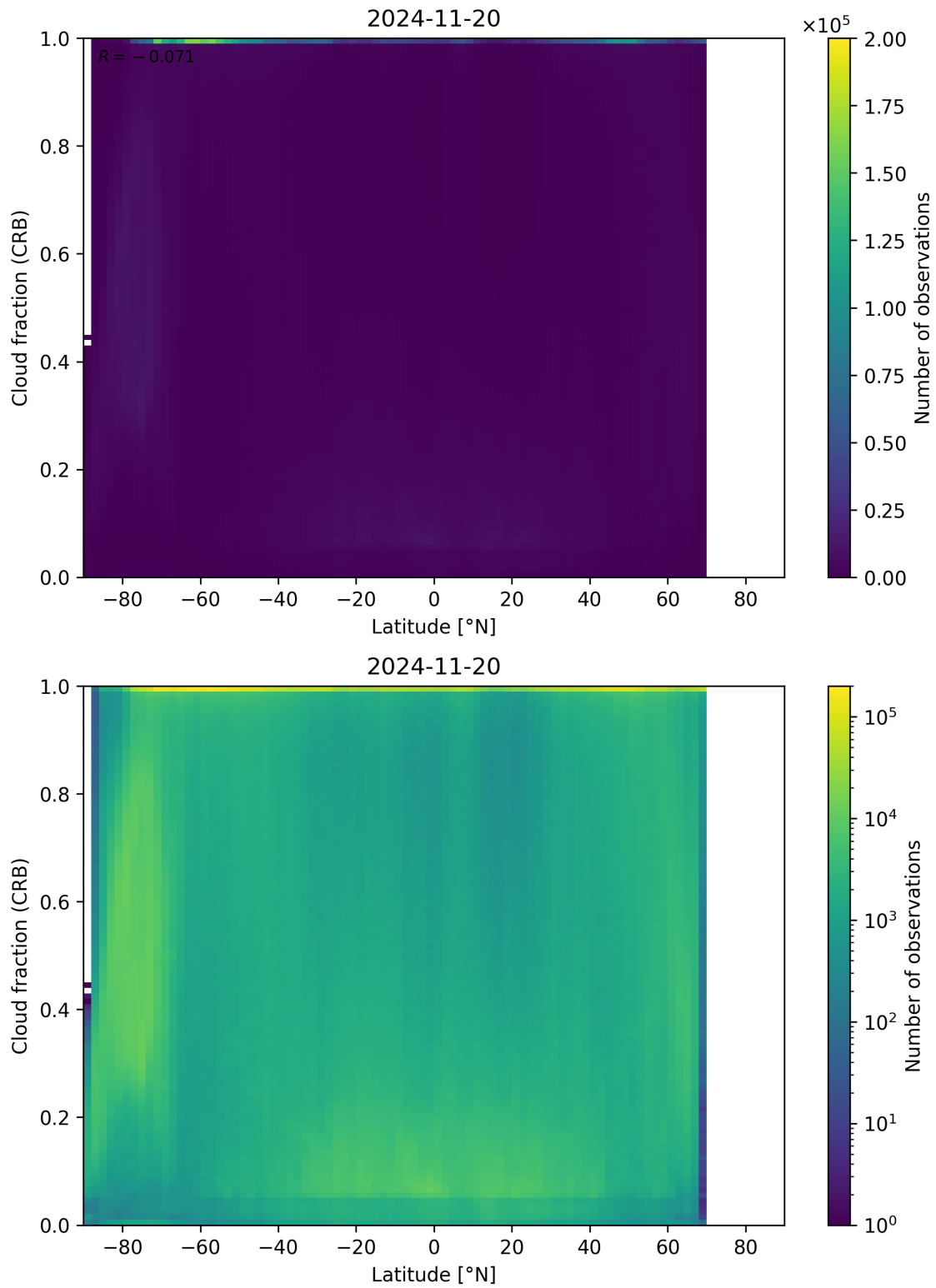
Figure 94: Scatter density plot of “Latitude” against “Cloud fraction (CRB)” for 2024-11-20 to 2024-11-21.
