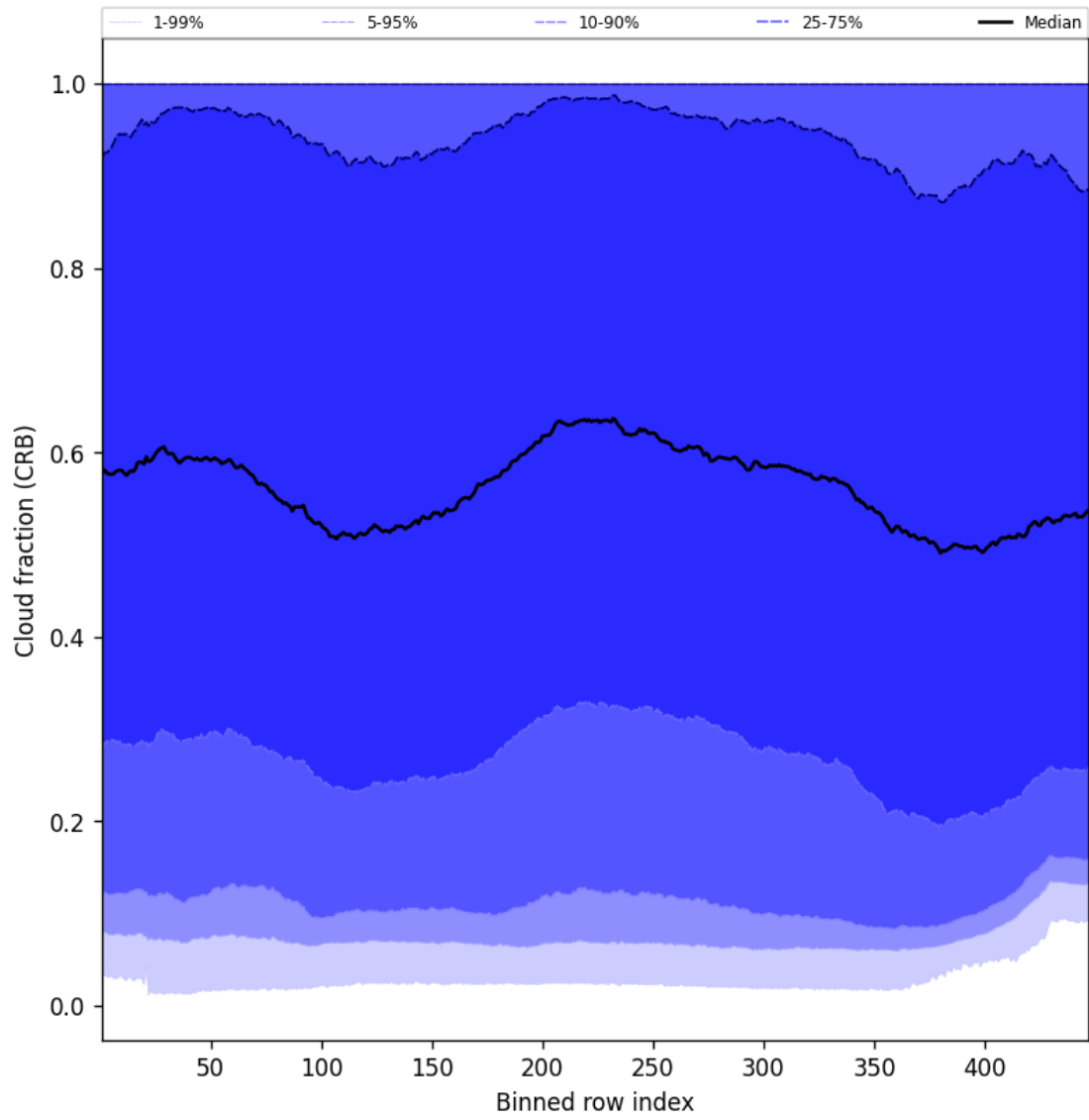
Figure 58: Along track statistics of “Cloud fraction (CRB)” for 2024-11-20 to 2024-11-21
