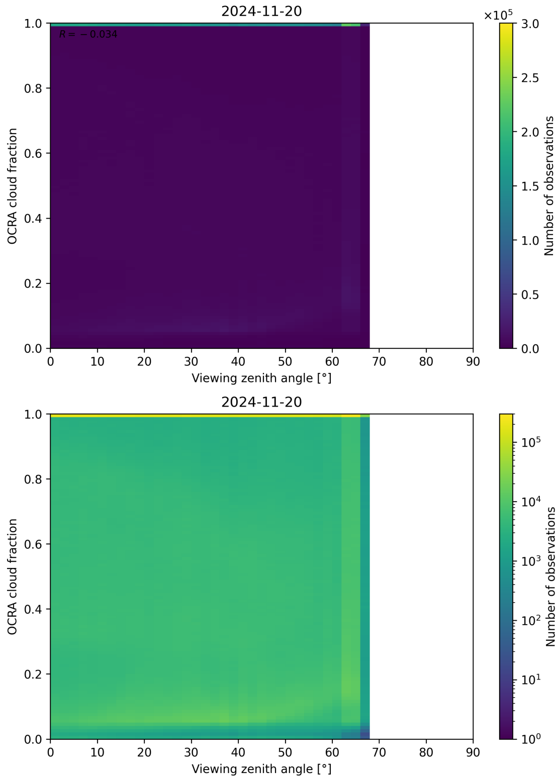
Figure 108: Scatter density plot of “Viewing zenith angle” against “OCRA cloud fraction” for 2024-11-20 to 2024-11-21.
