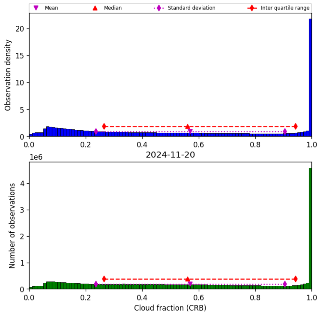
Figure 42: Histogram of “Cloud fraction (CRB)” for 2024-11-20 to 2024-11-21
