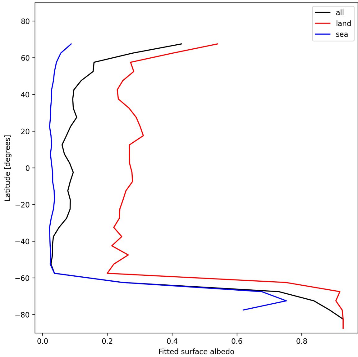
Figure 29: Zonal average of “Fitted surface albedo” for 2024-11-20 to 2024-11-21.
