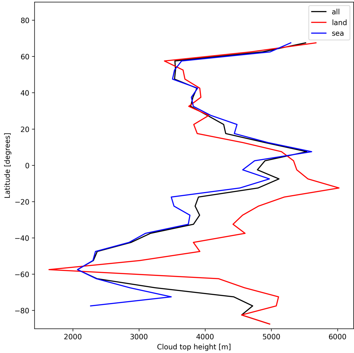
Figure 24: Zonal average of “Cloud top height” for 2024-11-20 to 2024-11-21.
