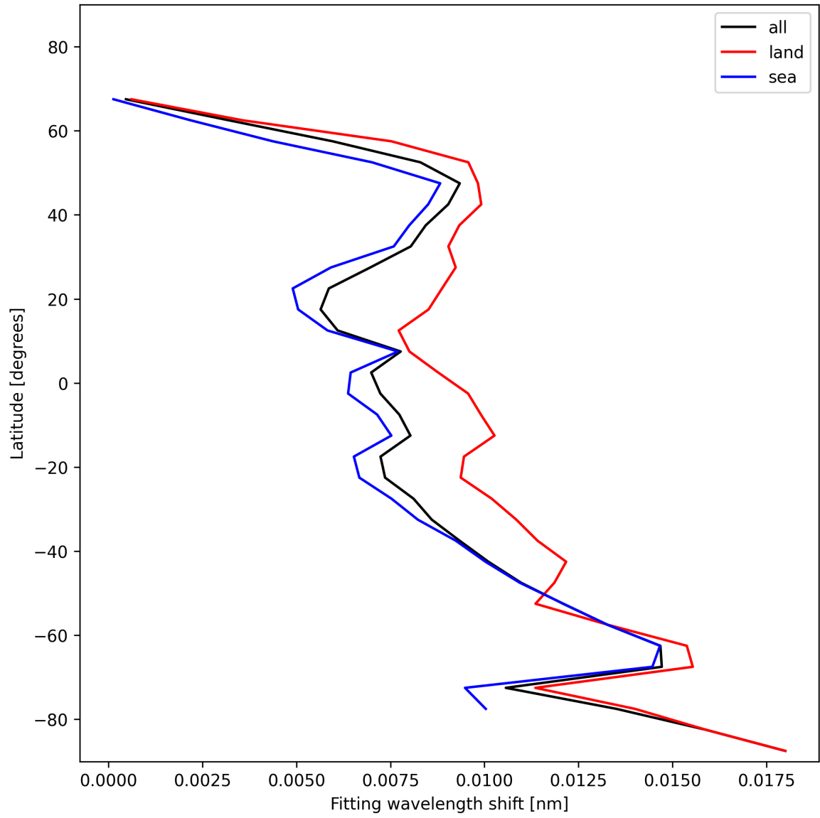
Figure 33: Zonal average of “Fitting wavelength shift” for 2024-11-20 to 2024-11-21.
