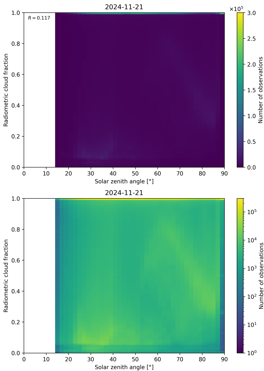
Figure 99: Scatter density plot of “Solar zenith angle” against “Radiometric cloud fraction” for 2024-11-20 to 2024-11-22.
