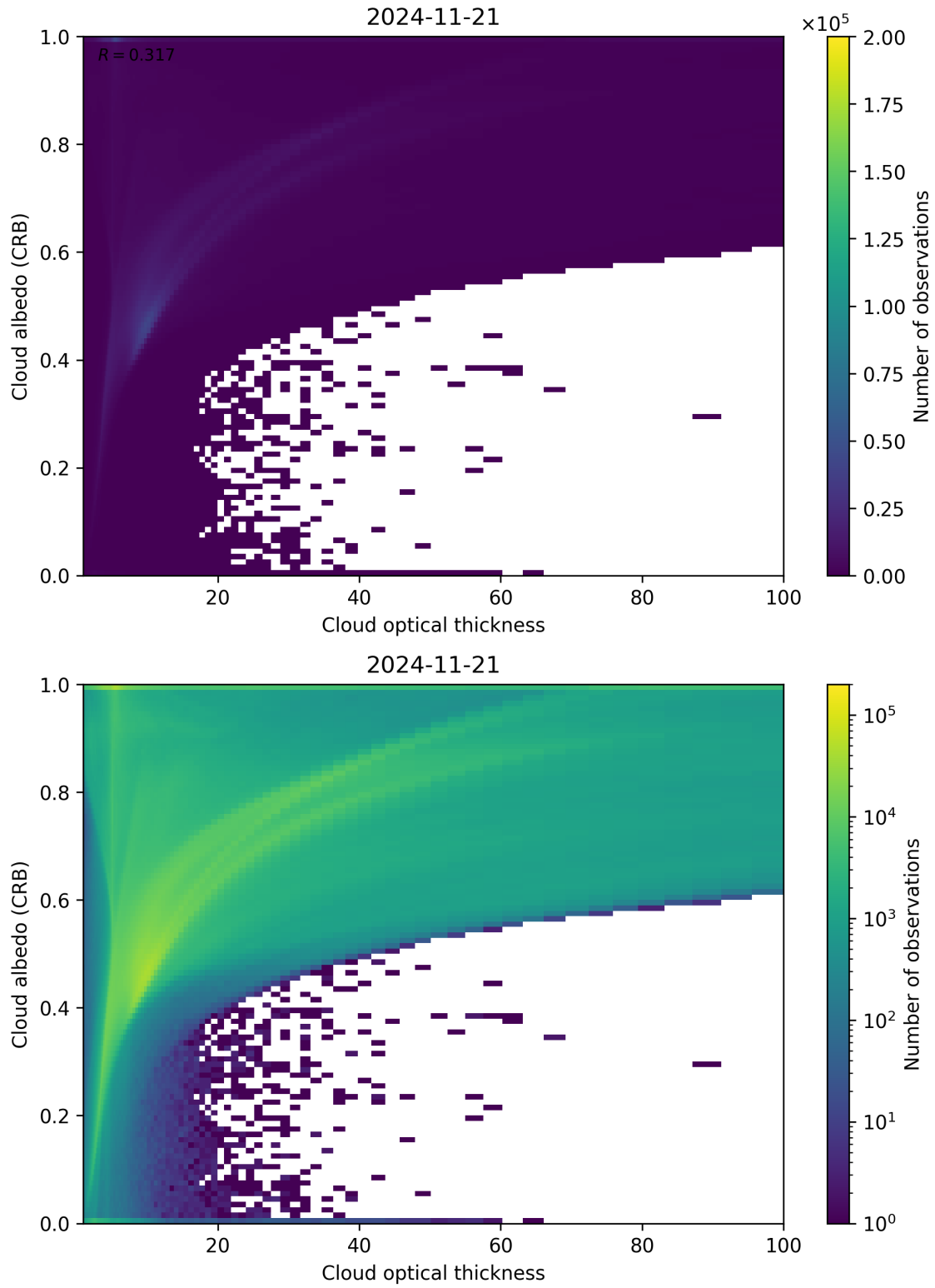
Figure 82: Scatter density plot of “Cloud optical thickness” against “Cloud albedo (CRB)” for 2024-11-20 to 2024-11-22.
