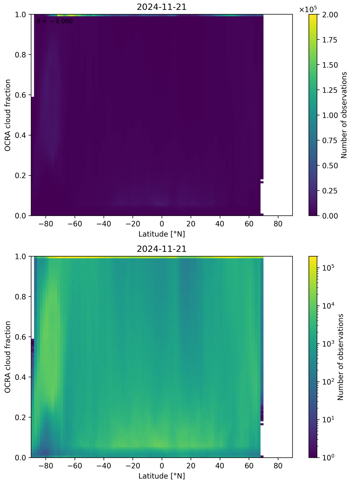
Figure 93: Scatter density plot of “Latitude” against “OCRA cloud fraction” for 2024-11-20 to 2024-11-22.
