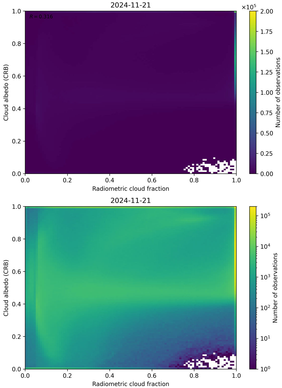
Figure 71: Scatter density plot of “Radiometric cloud fraction” against “Cloud albedo (CRB)” for 2024-11-20 to 2024-11-22.
