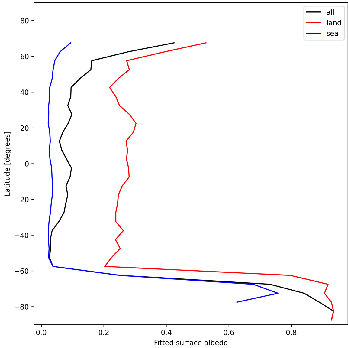
Figure 29: Zonal average of “Fitted surface albedo” for 2024-11-20 to 2024-11-22.
