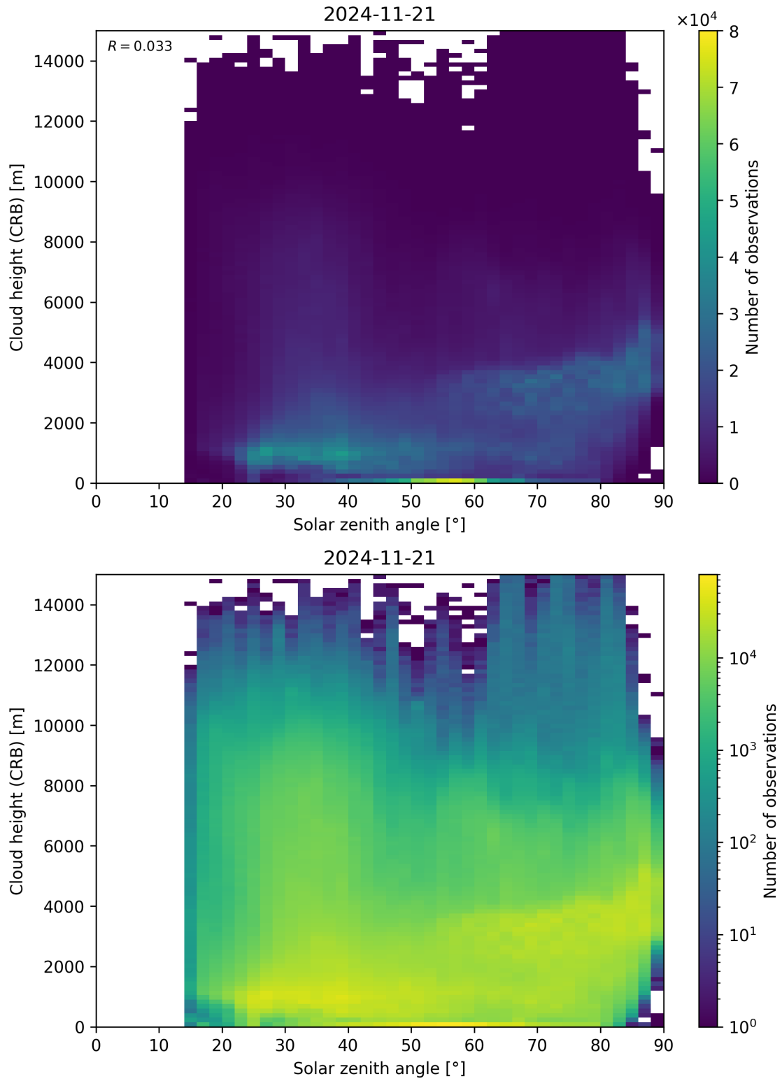
Figure 102: Scatter density plot of “Solar zenith angle” against “Cloud height (CRB)” for 2024-11-20 to 2024-11-22.
