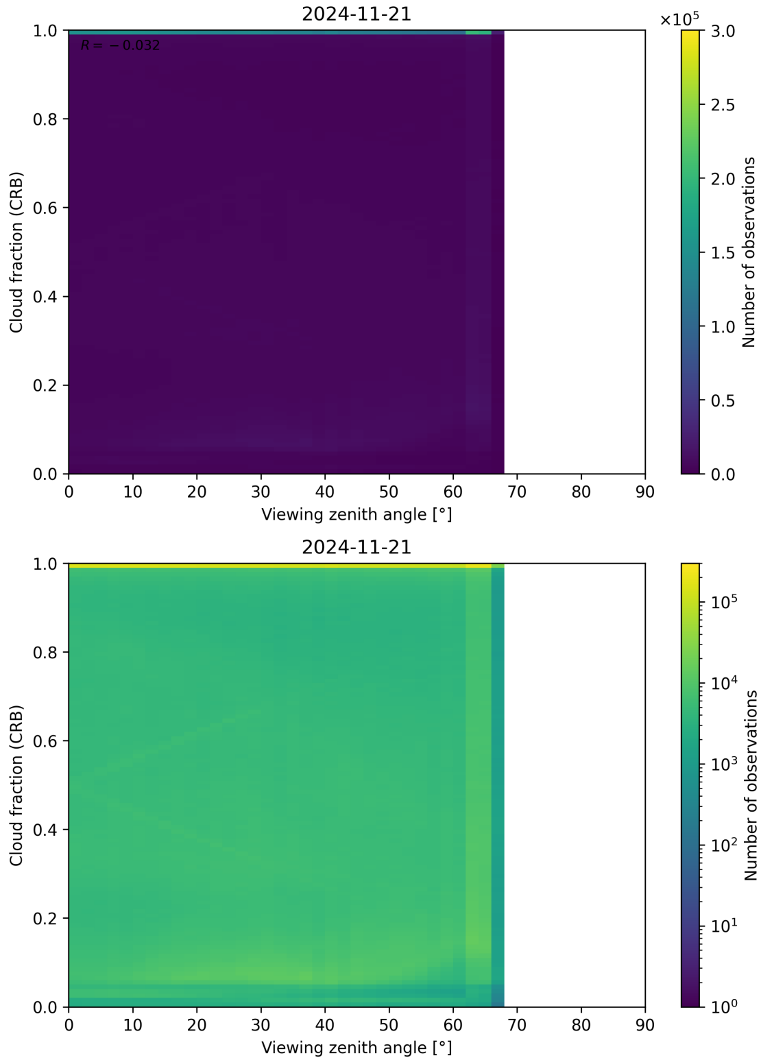
Figure 109: Scatter density plot of “Viewing zenith angle” against “Cloud fraction (CRB)” for 2024-11-20 to 2024-11-22.
