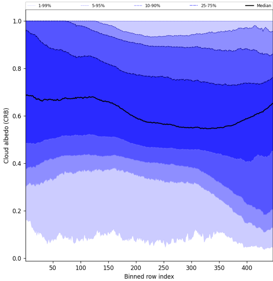
Figure 60: Along track statistics of “Cloud albedo (CRB)” for 2024-11-20 to 2024-11-22
