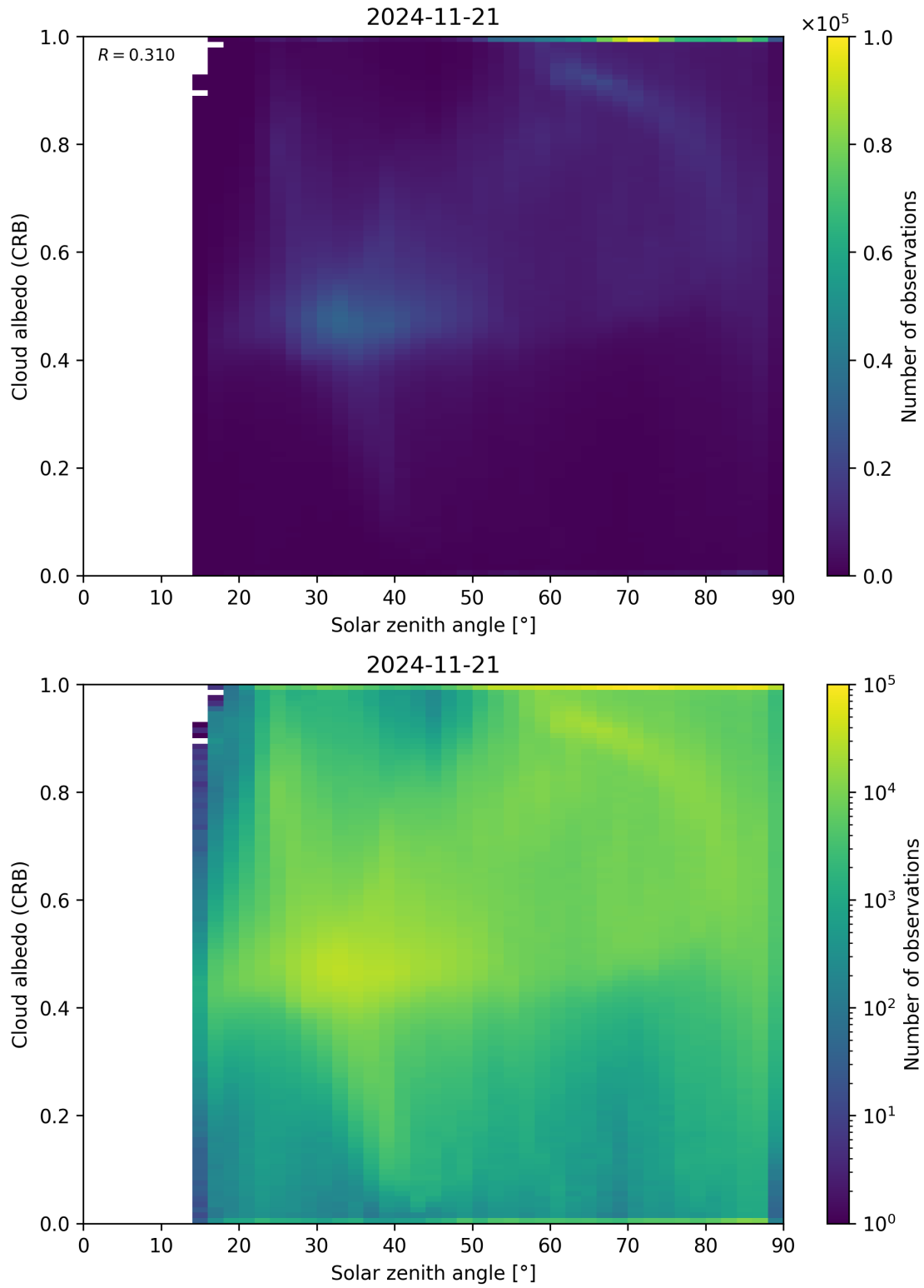
Figure 98: Scatter density plot of “Solar zenith angle” against “Cloud albedo (CRB)” for 2024-11-20 to 2024-11-22.
