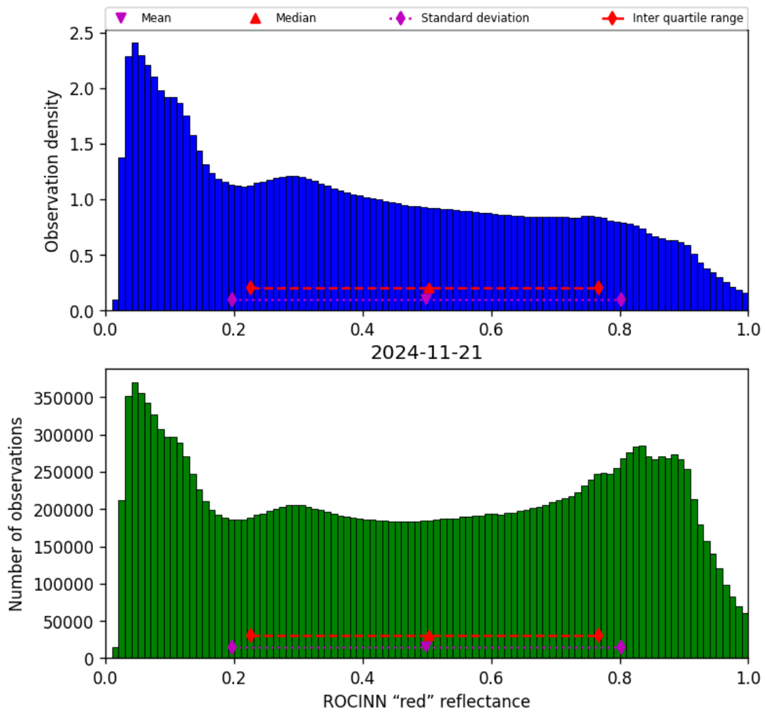
Figure 53: Histogram of “ROCINN “red” reflectance” for 2024-11-20 to 2024-11-22
