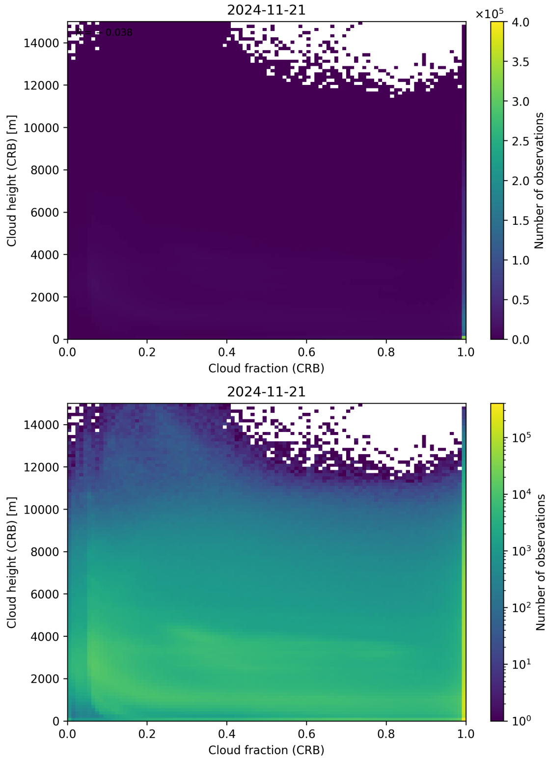
Figure 79: Scatter density plot of “Cloud fraction (CRB)” against “Cloud height (CRB)” for 2024-11-20 to 2024-11-22.
