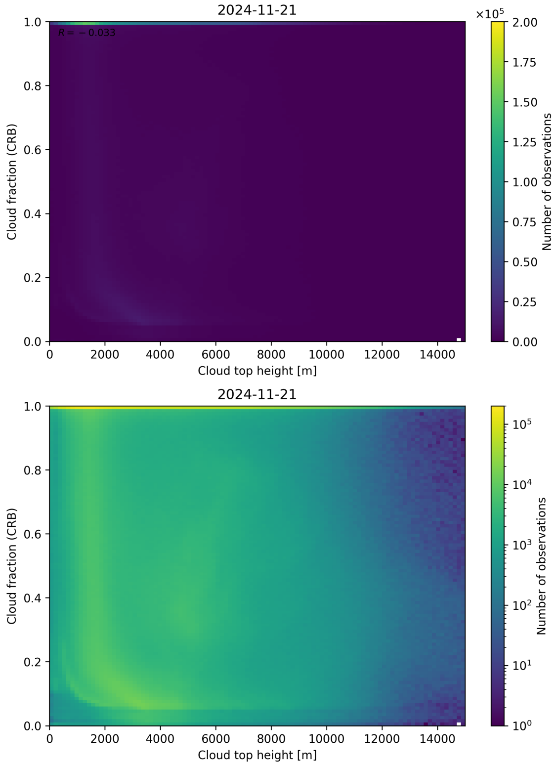
Figure 88: Scatter density plot of “Cloud top height” against “Cloud fraction (CRB)” for 2024-11-20 to 2024-11-22.
