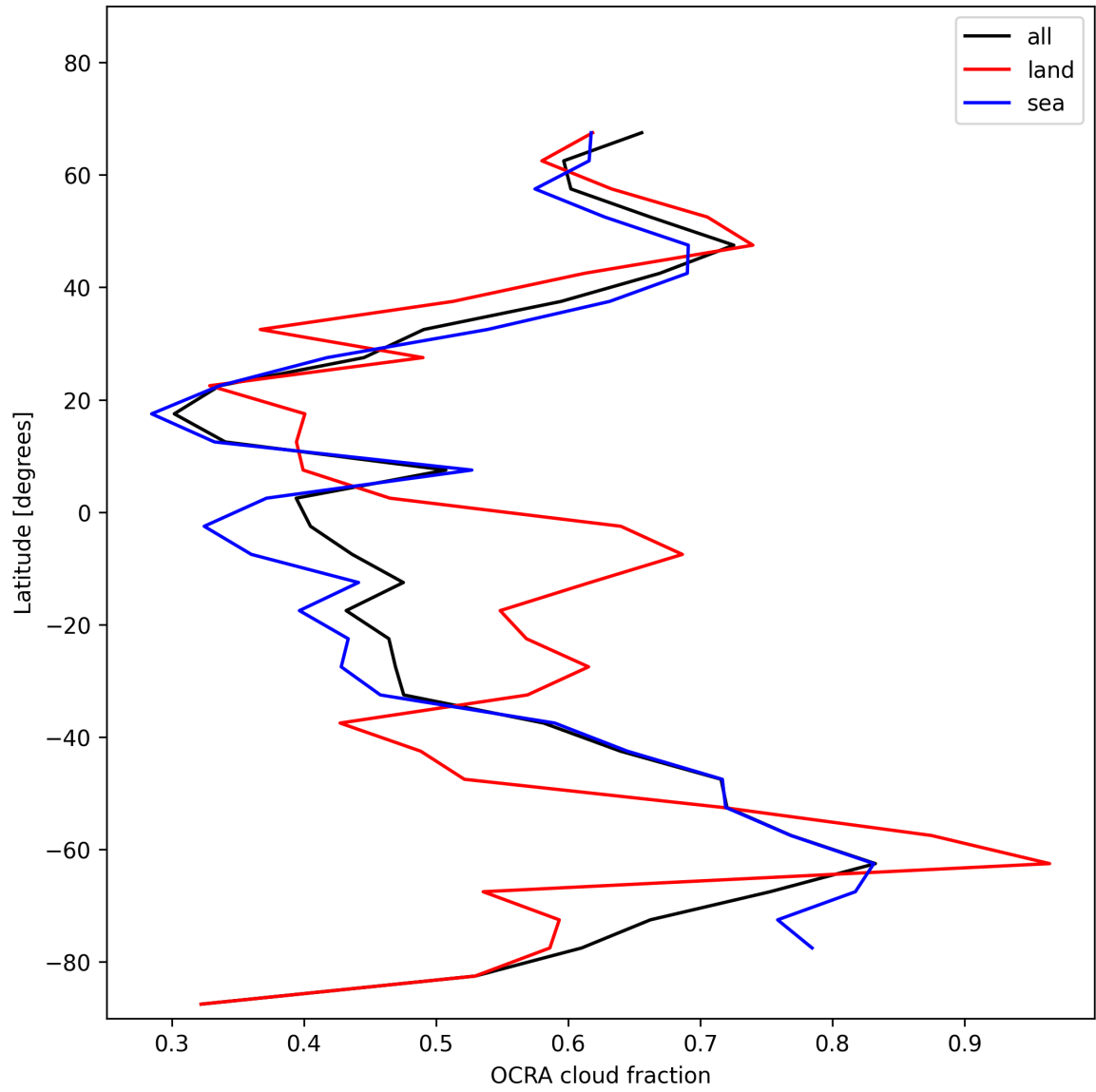
Figure 34: Zonal average of “OCRA cloud fraction” for 2024-11-20 to 2024-11-22.
