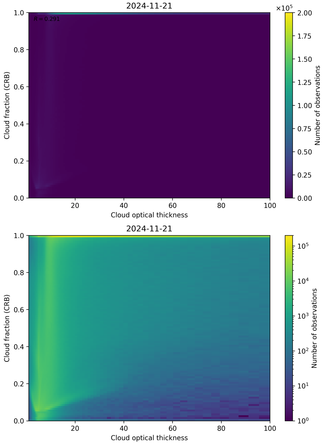
Figure 84: Scatter density plot of “Cloud optical thickness” against “Cloud fraction (CRB)” for 2024-11-20 to 2024-11-22.
