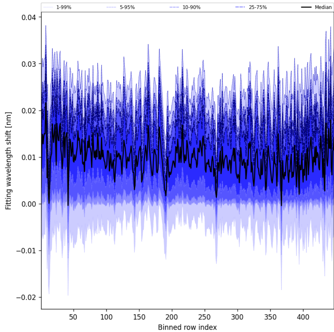
Figure 65: Along track statistics of “Fitting wavelength shift” for 2024-11-20 to 2024-11-22
