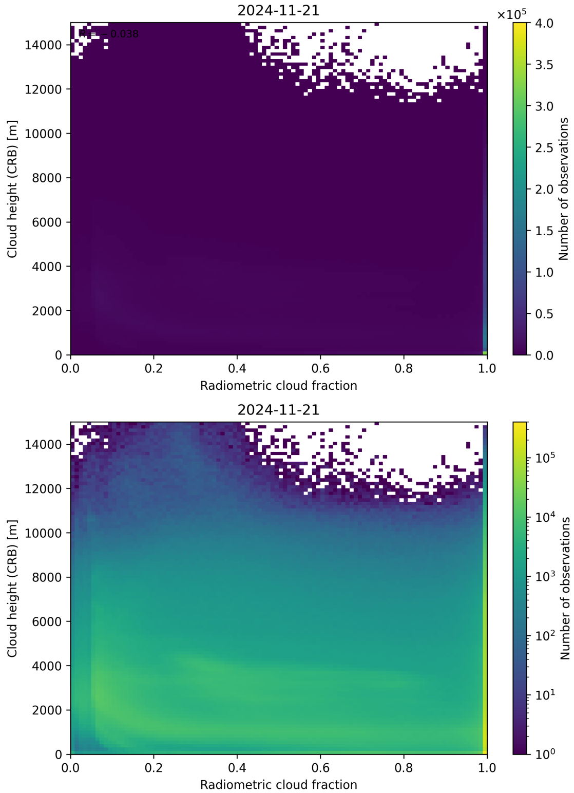
Figure 74: Scatter density plot of “Radiometric cloud fraction” against “Cloud height (CRB)” for 2024-11-20 to 2024-11-22.
