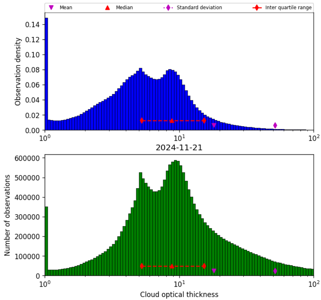
Figure 41: Histogram of “Cloud optical thickness” for 2024-11-20 to 2024-11-22
