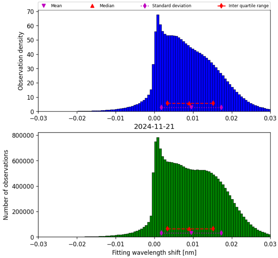
Figure 49: Histogram of “Fitting wavelength shift” for 2024-11-20 to 2024-11-22
