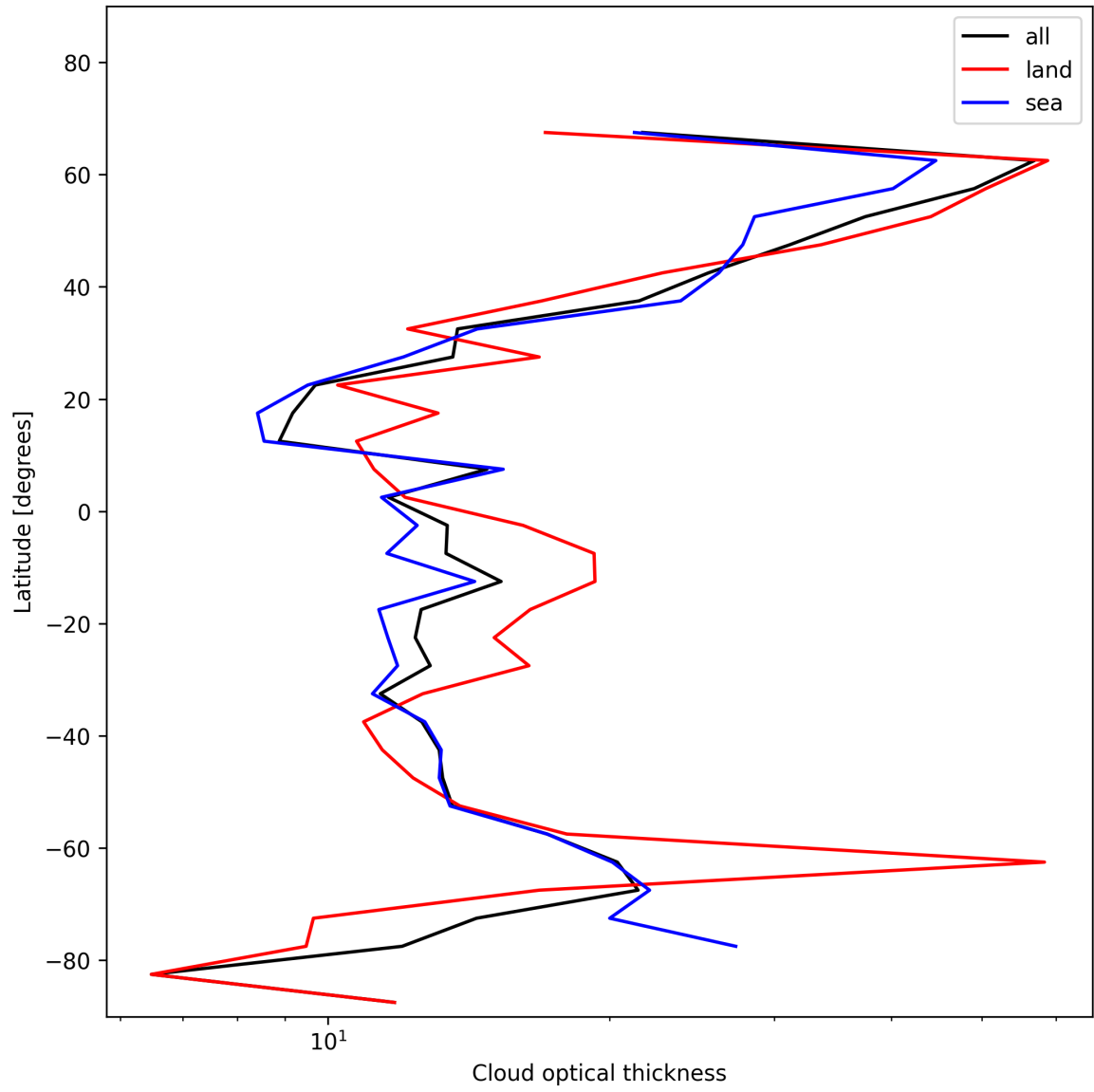
Figure 25: Zonal average of “Cloud optical thickness” for 2024-11-20 to 2024-11-22.
