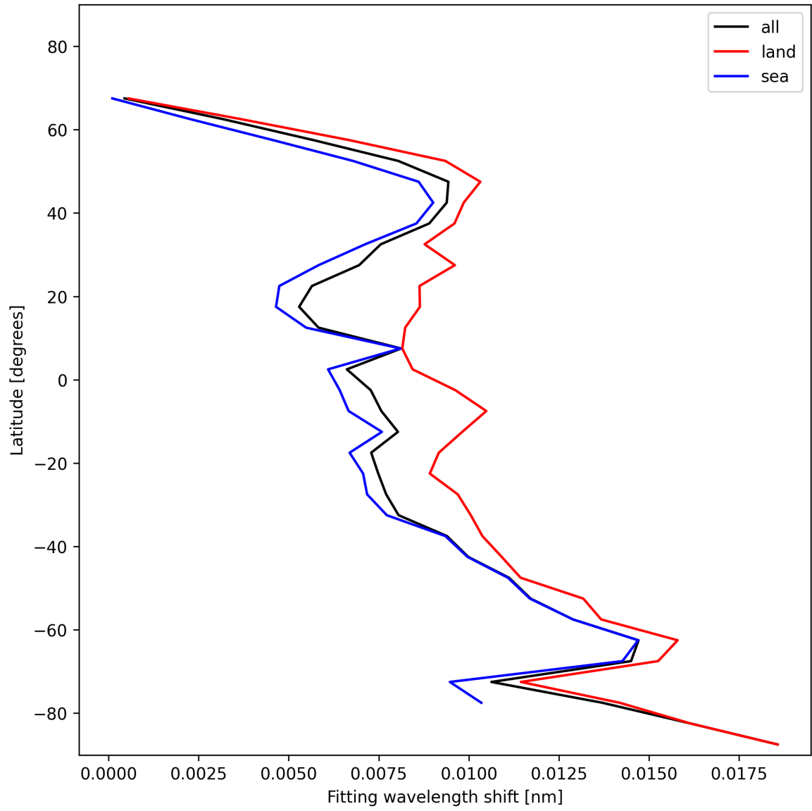
Figure 33: Zonal average of “Fitting wavelength shift” for 2024-11-20 to 2024-11-22.
