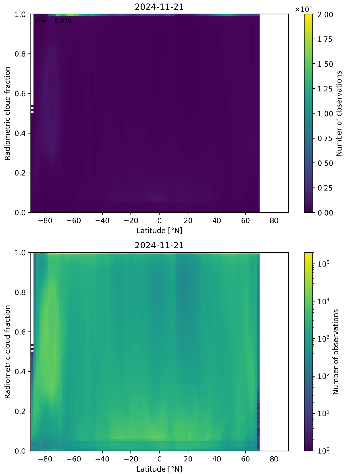
Figure 92: Scatter density plot of “Latitude” against “Radiometric cloud fraction” for 2024-11-20 to 2024-11-22.
