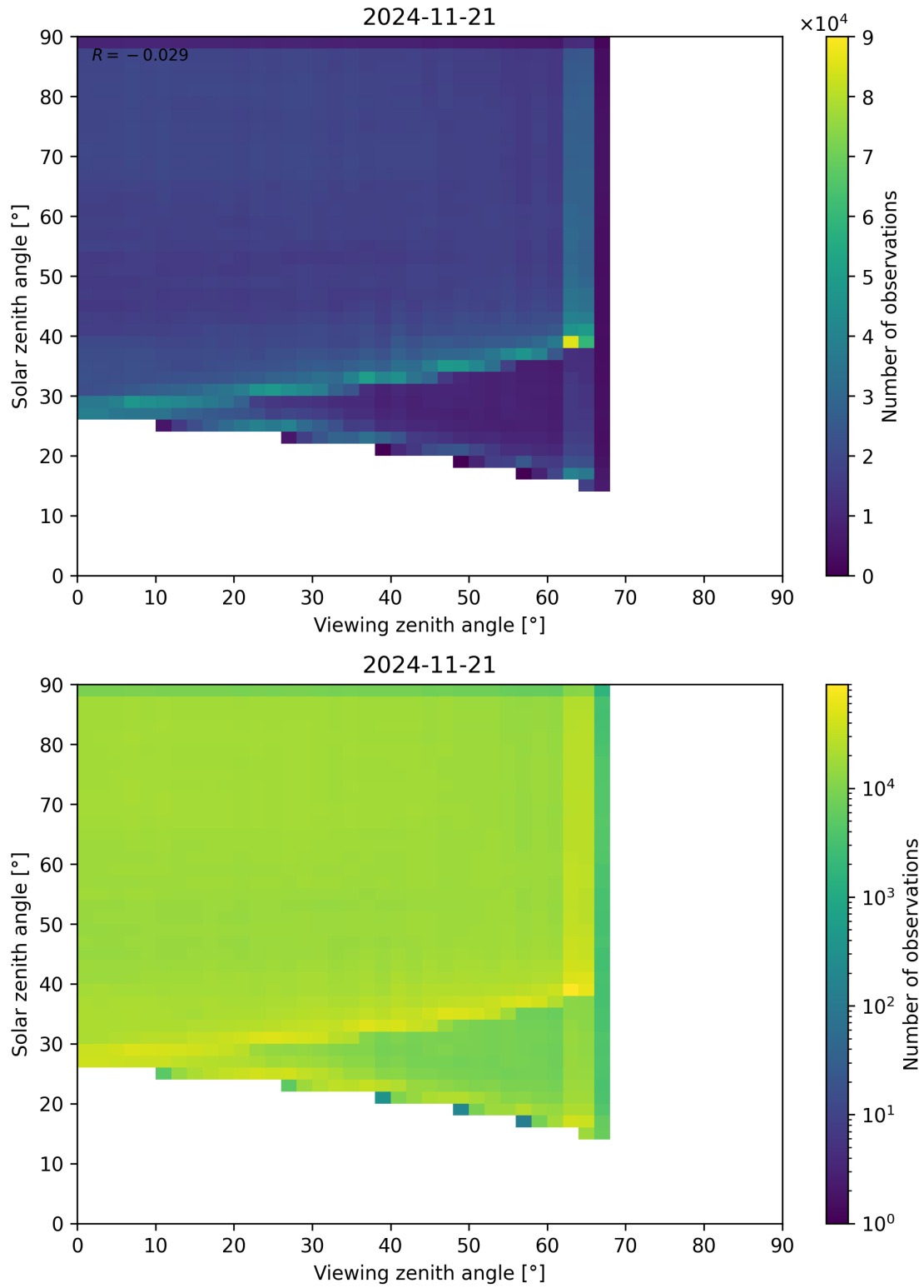
Figure 114: Scatter density plot of “Viewing zenith angle” against “Solar zenith angle” for 2024-11-20 to 2024-11-22.
