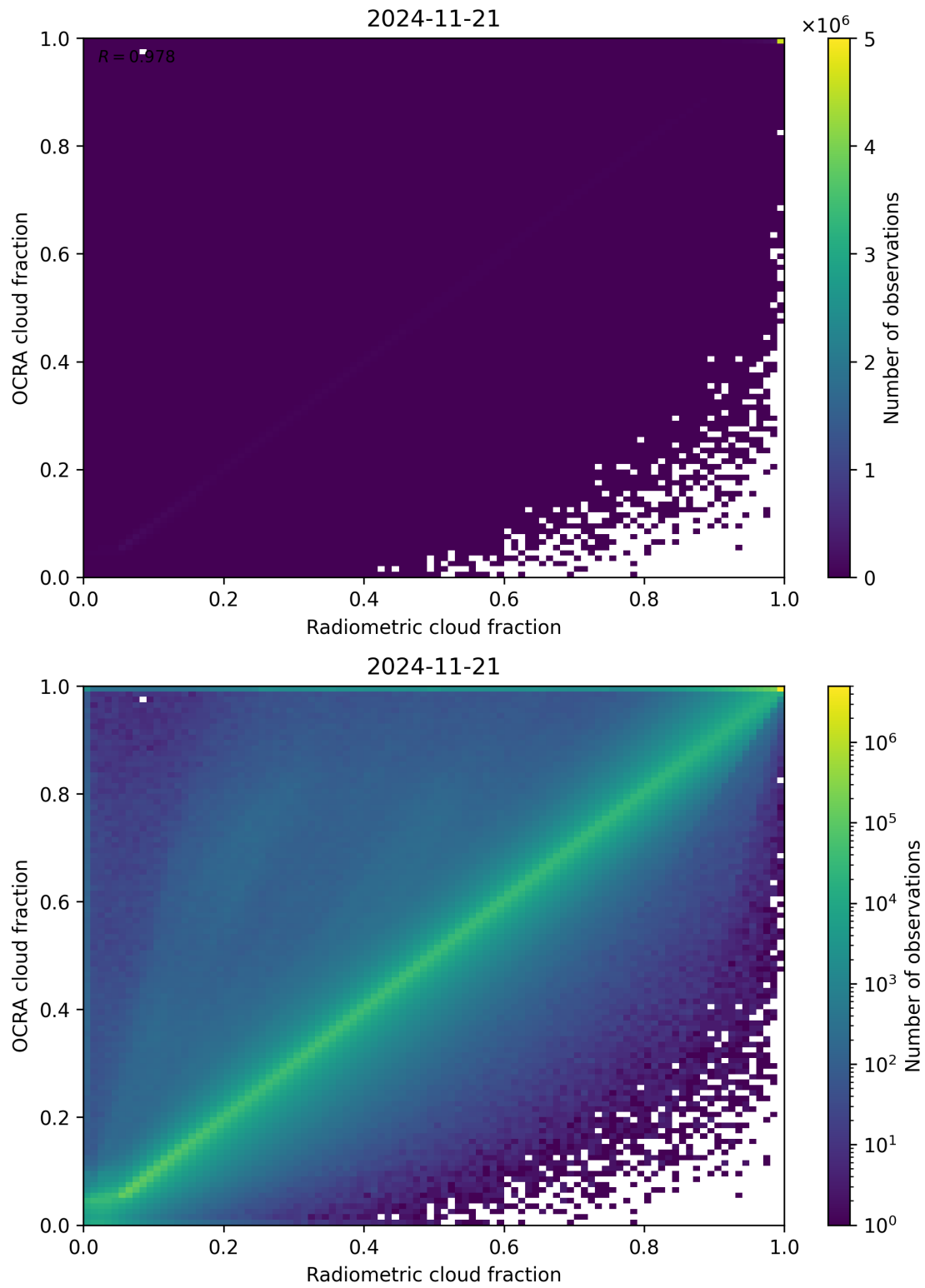
Figure 72: Scatter density plot of “Radiometric cloud fraction” against “OCRA cloud fraction” for 2024-11-20 to 2024-11-22.
