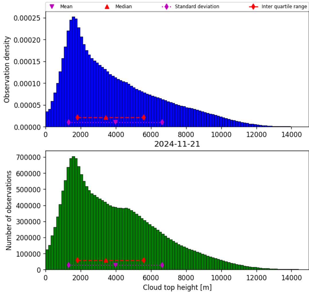
Figure 40: Histogram of “Cloud top height” for 2024-11-20 to 2024-11-22
