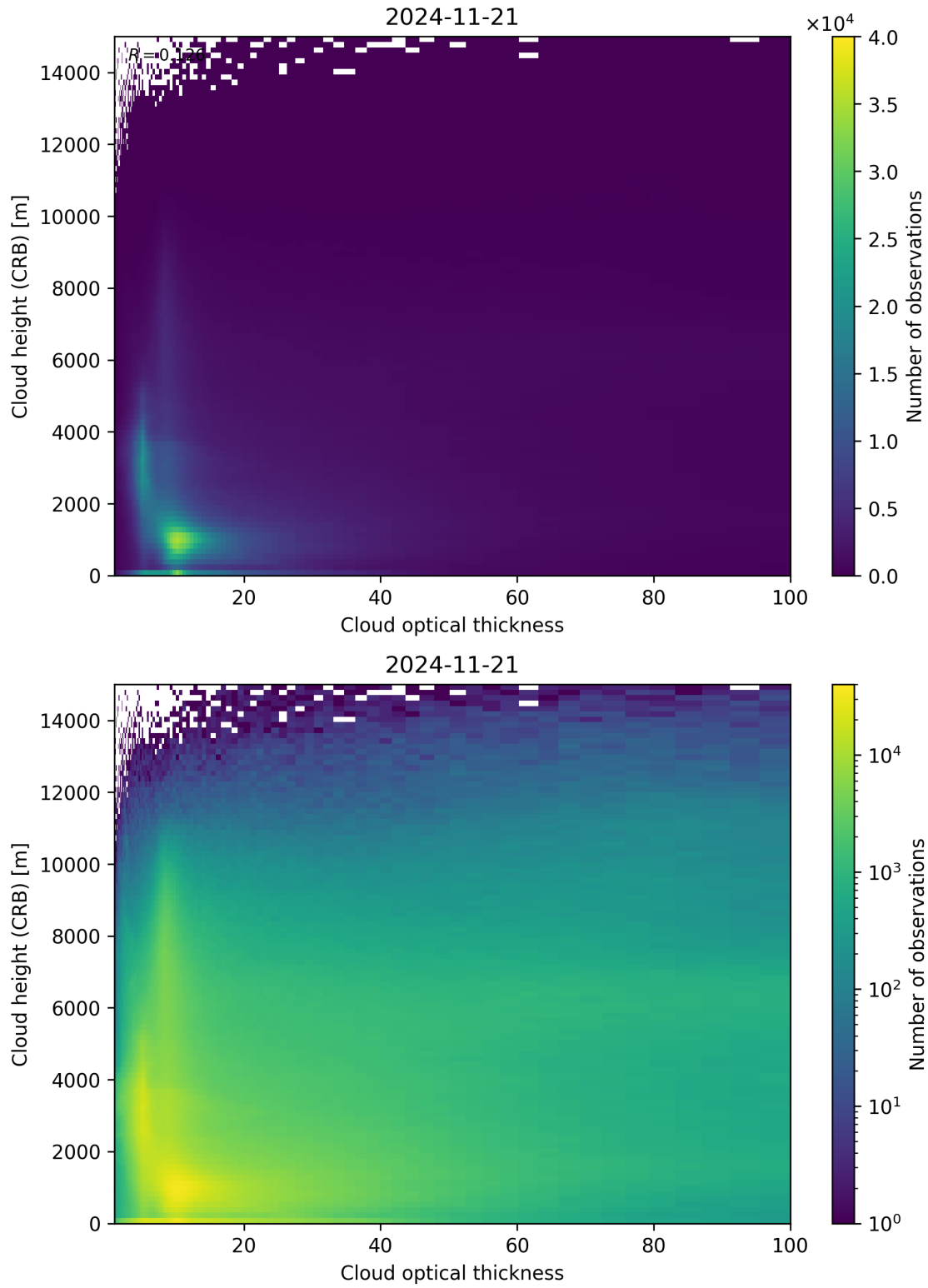
Figure 85: Scatter density plot of “Cloud optical thickness” against “Cloud height (CRB)” for 2024-11-20 to 2024-11-22.
