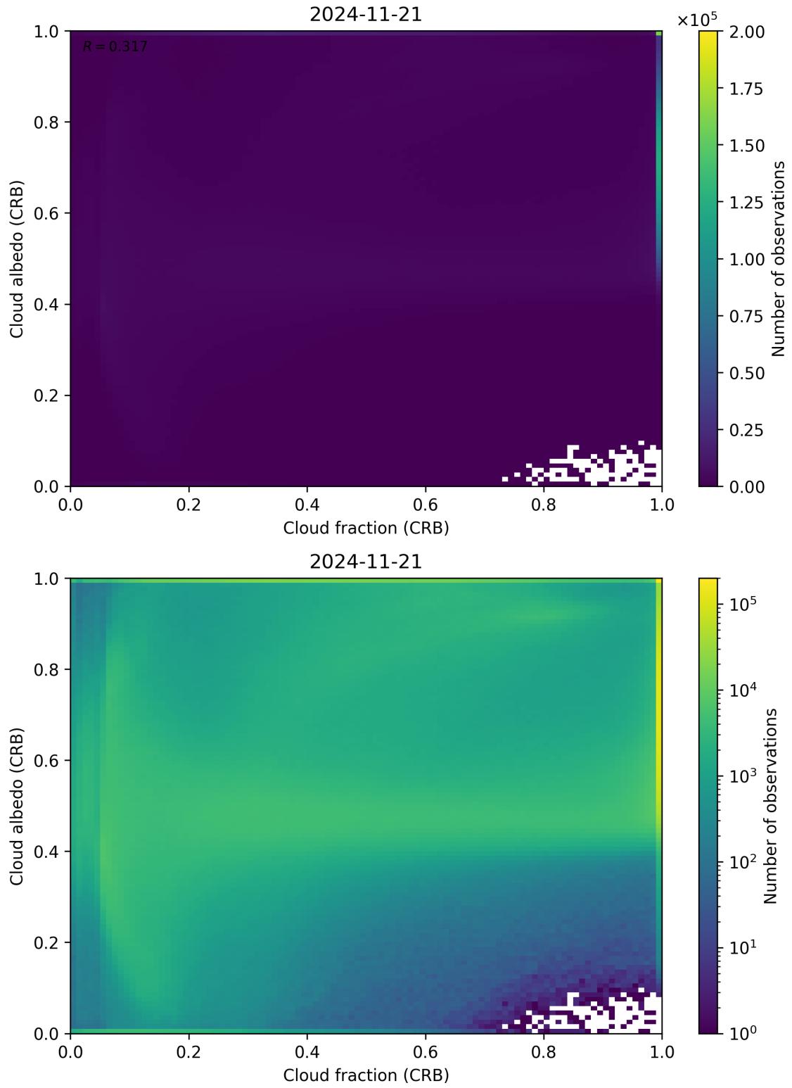
Figure 77: Scatter density plot of “Cloud fraction (CRB)” against “Cloud albedo (CRB)” for 2024-11-20 to 2024-11-22.
