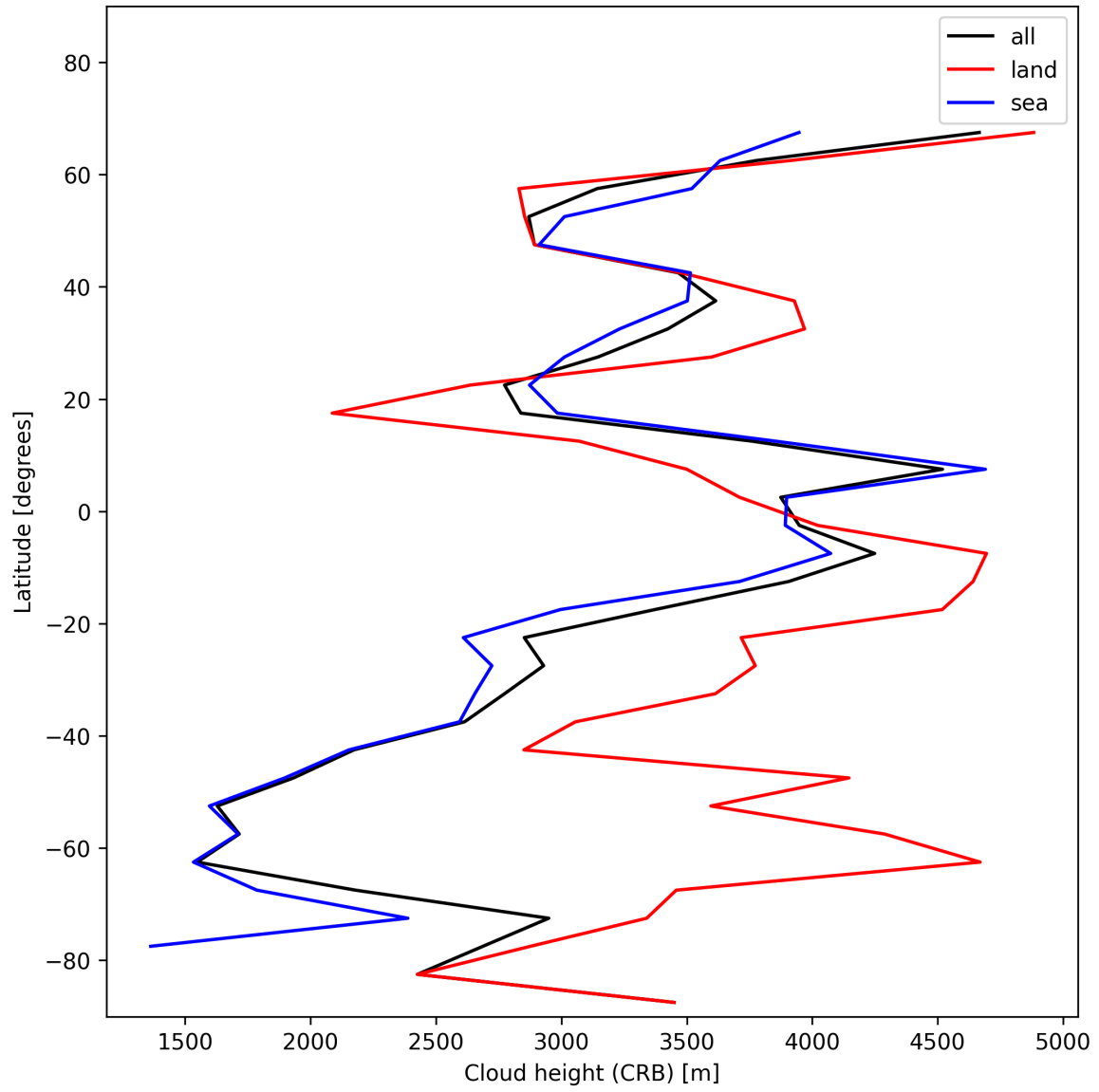
Figure 27: Zonal average of “Cloud height (CRB)” for 2024-11-20 to 2024-11-22.
