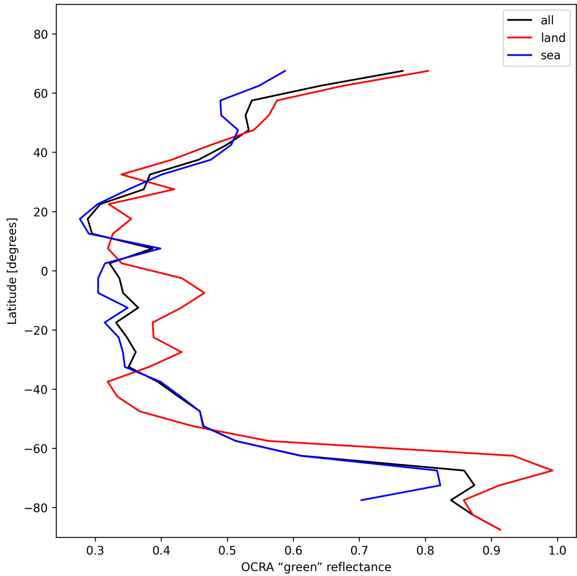
Figure 36: Zonal average of “OCRA “green” reflectance” for 2024-11-20 to 2024-11-22.
