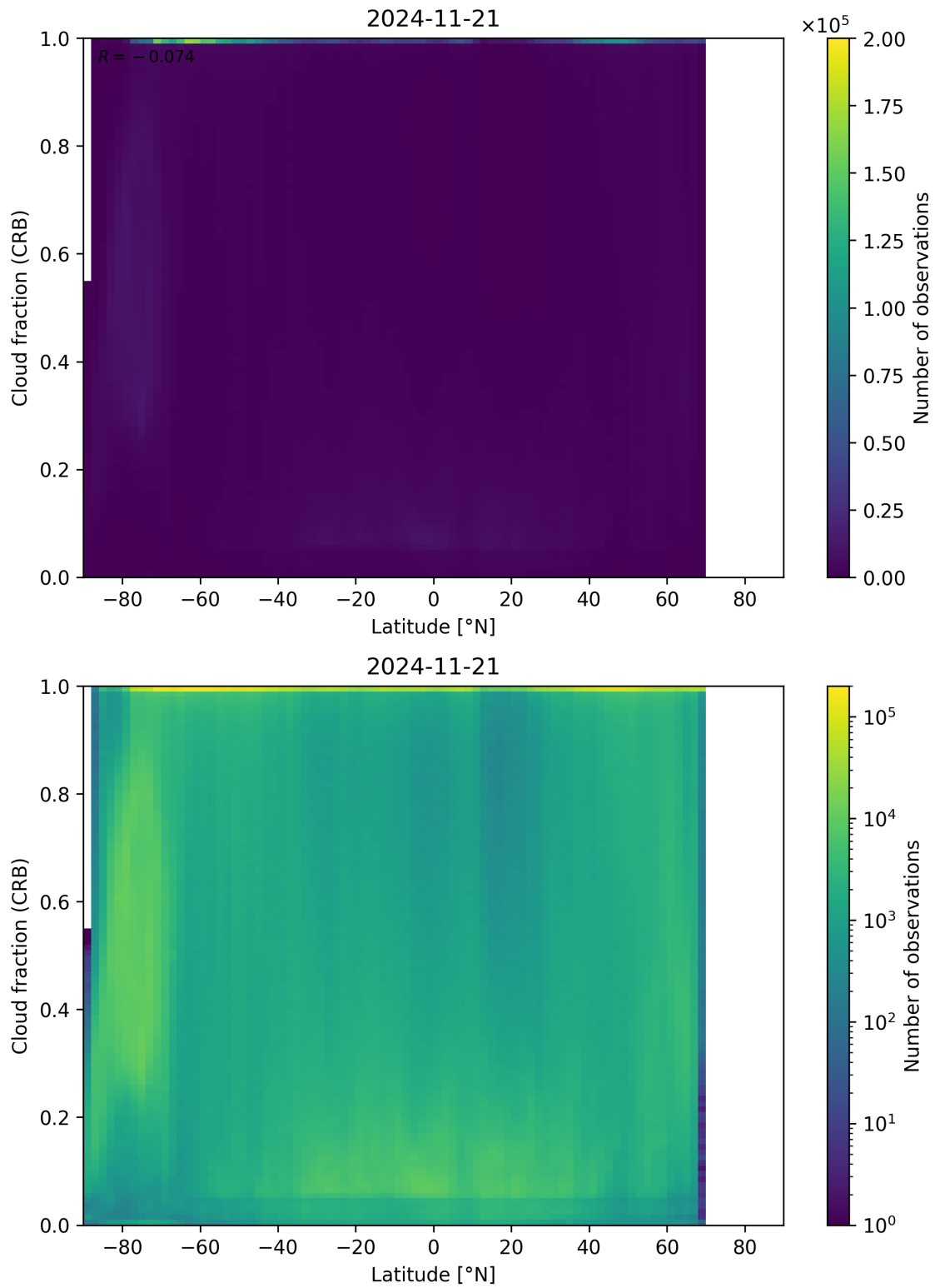
Figure 94: Scatter density plot of “Latitude” against “Cloud fraction (CRB)” for 2024-11-20 to 2024-11-22.
