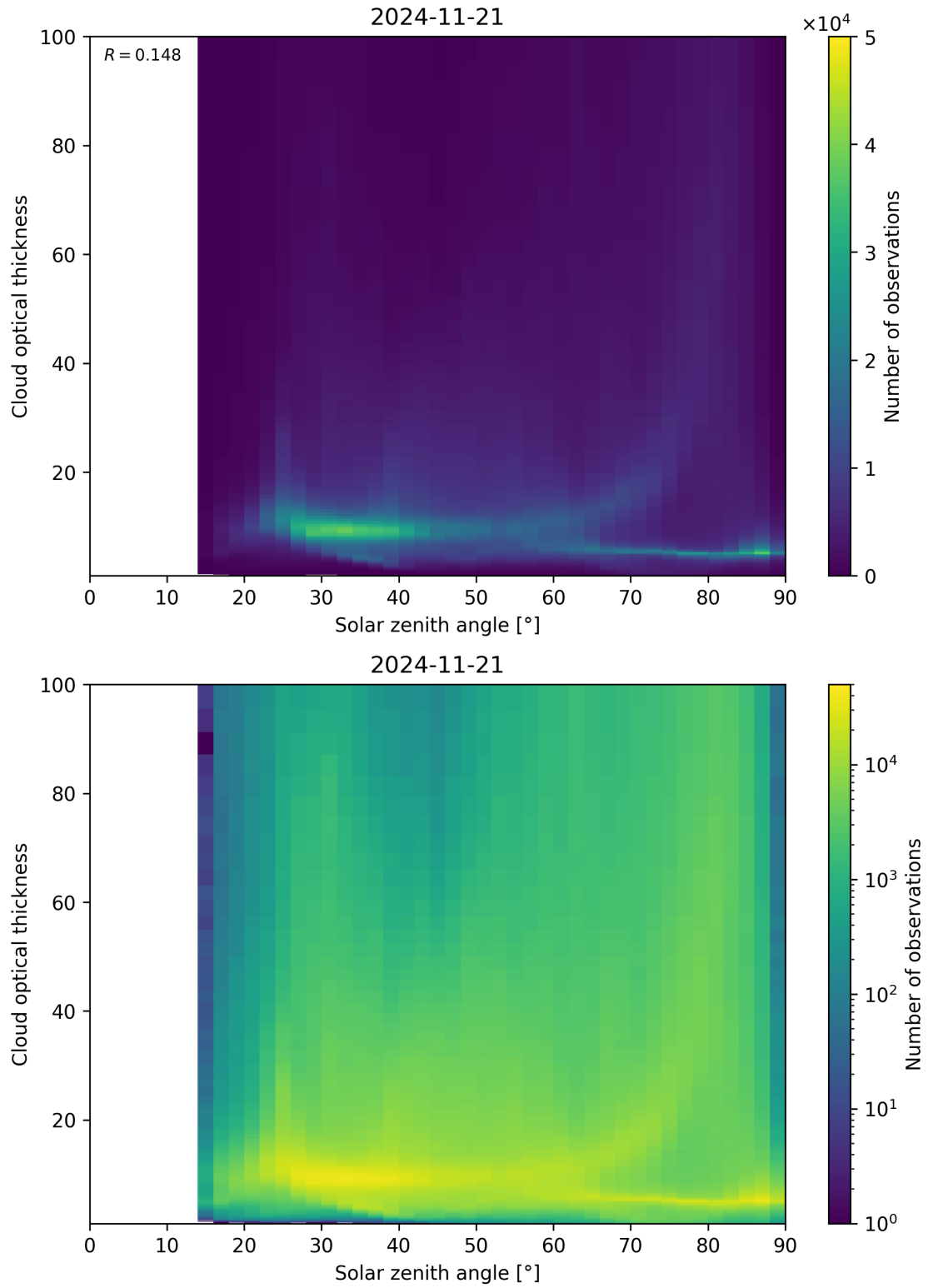
Figure 103: Scatter density plot of “Solar zenith angle” against “Cloud optical thickness” for 2024-11-20 to 2024-11-22.
