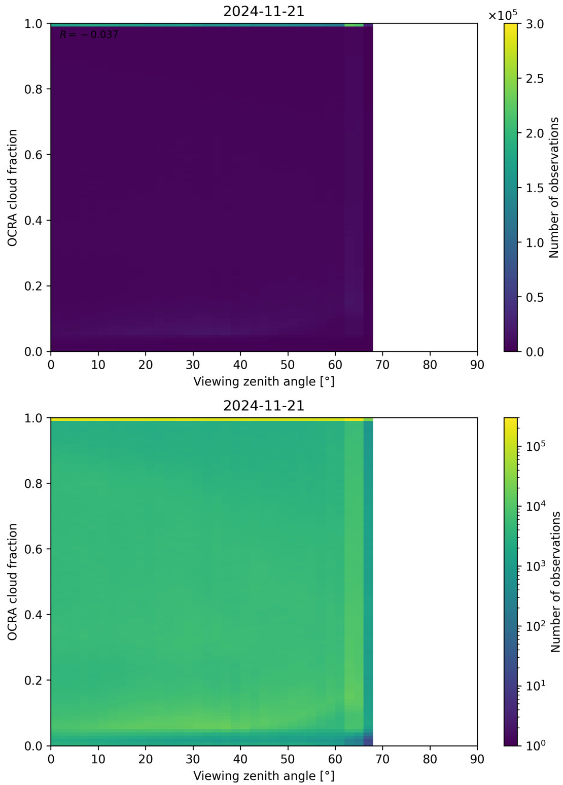
Figure 108: Scatter density plot of “Viewing zenith angle” against “OCRA cloud fraction” for 2024-11-20 to 2024-11-22.
