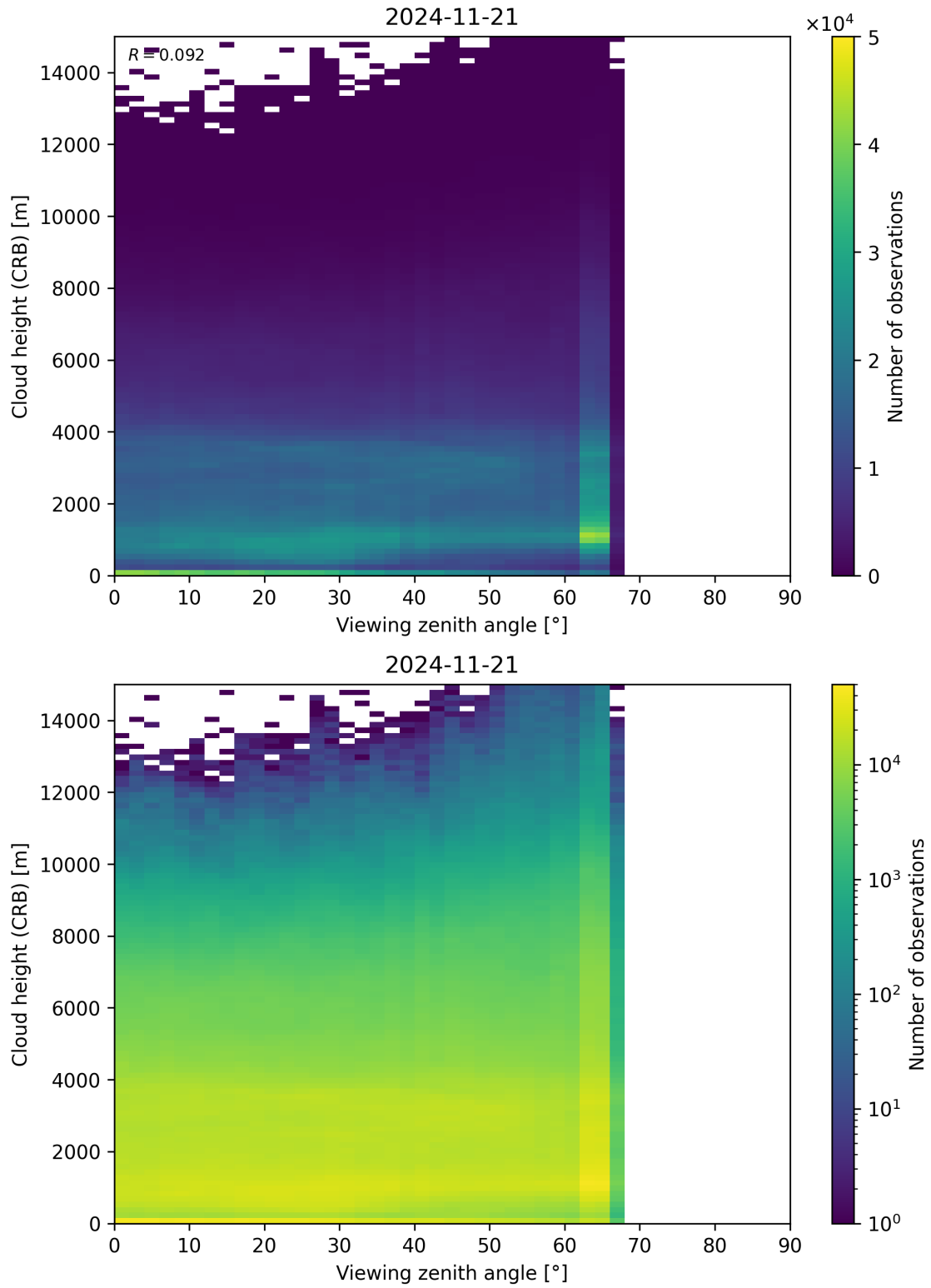
Figure 110: Scatter density plot of “Viewing zenith angle” against “Cloud height (CRB)” for 2024-11-20 to 2024-11-22.
