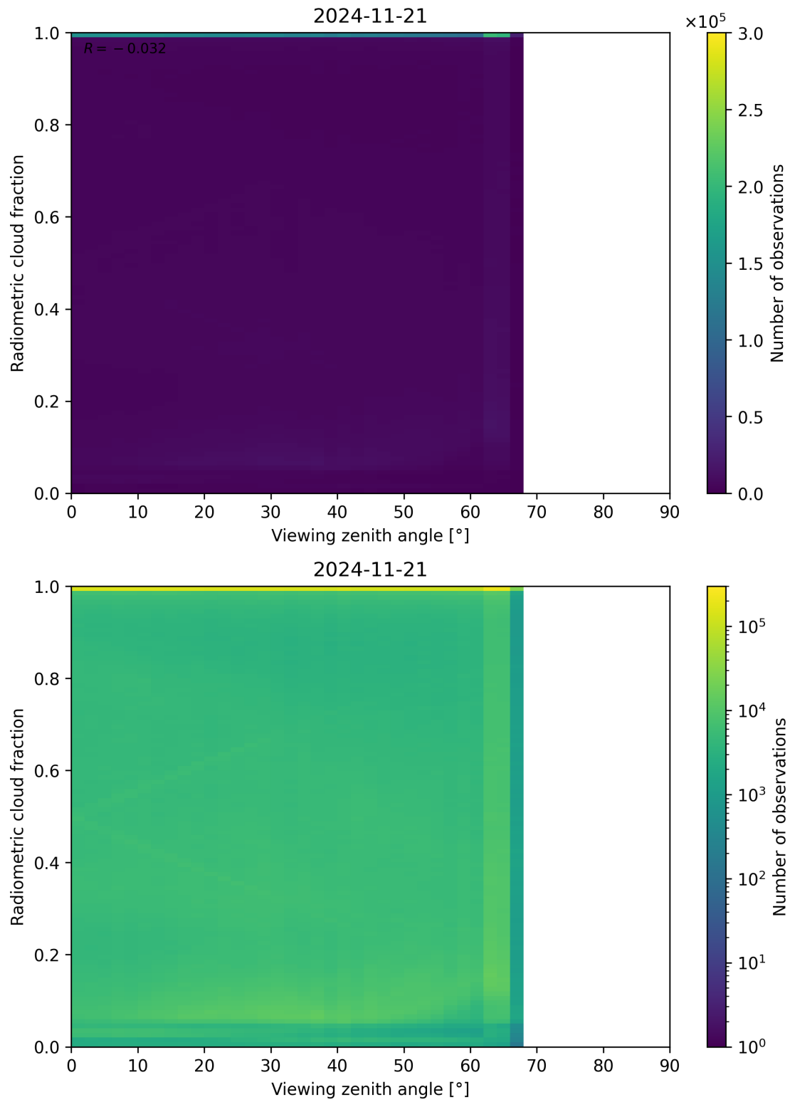
Figure 107: Scatter density plot of “Viewing zenith angle” against “Radiometric cloud fraction” for 2024-11-20 to 2024-11-22.
