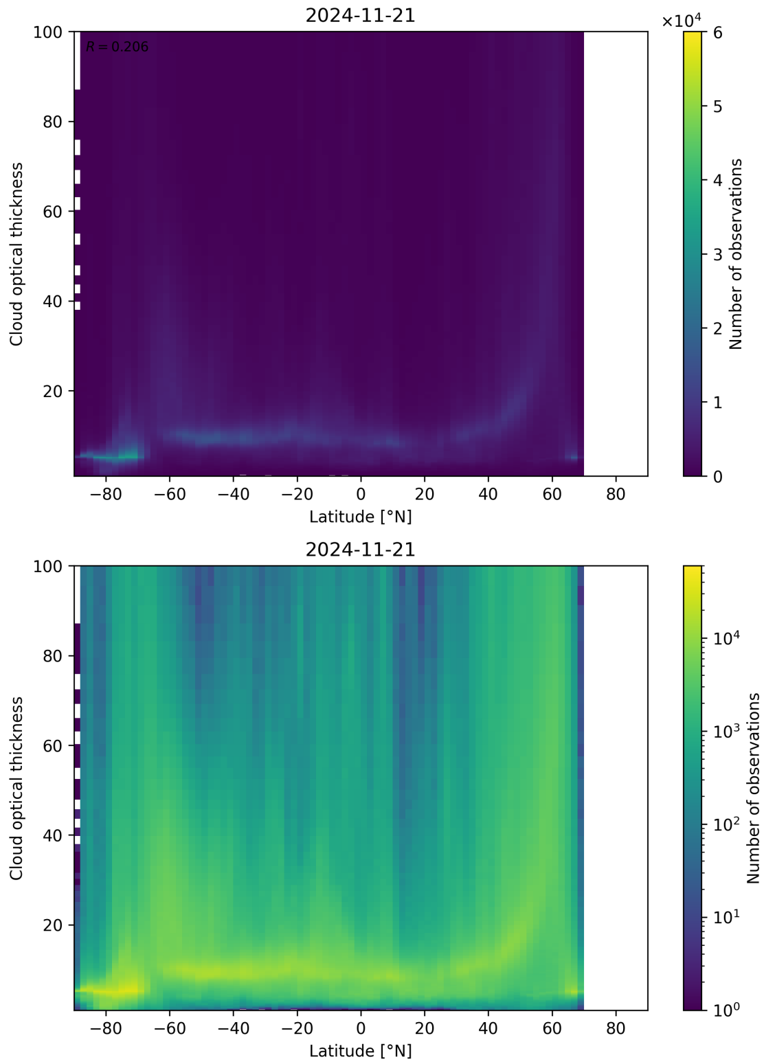
Figure 96: Scatter density plot of “Latitude” against “Cloud optical thickness” for 2024-11-20 to 2024-11-22.
