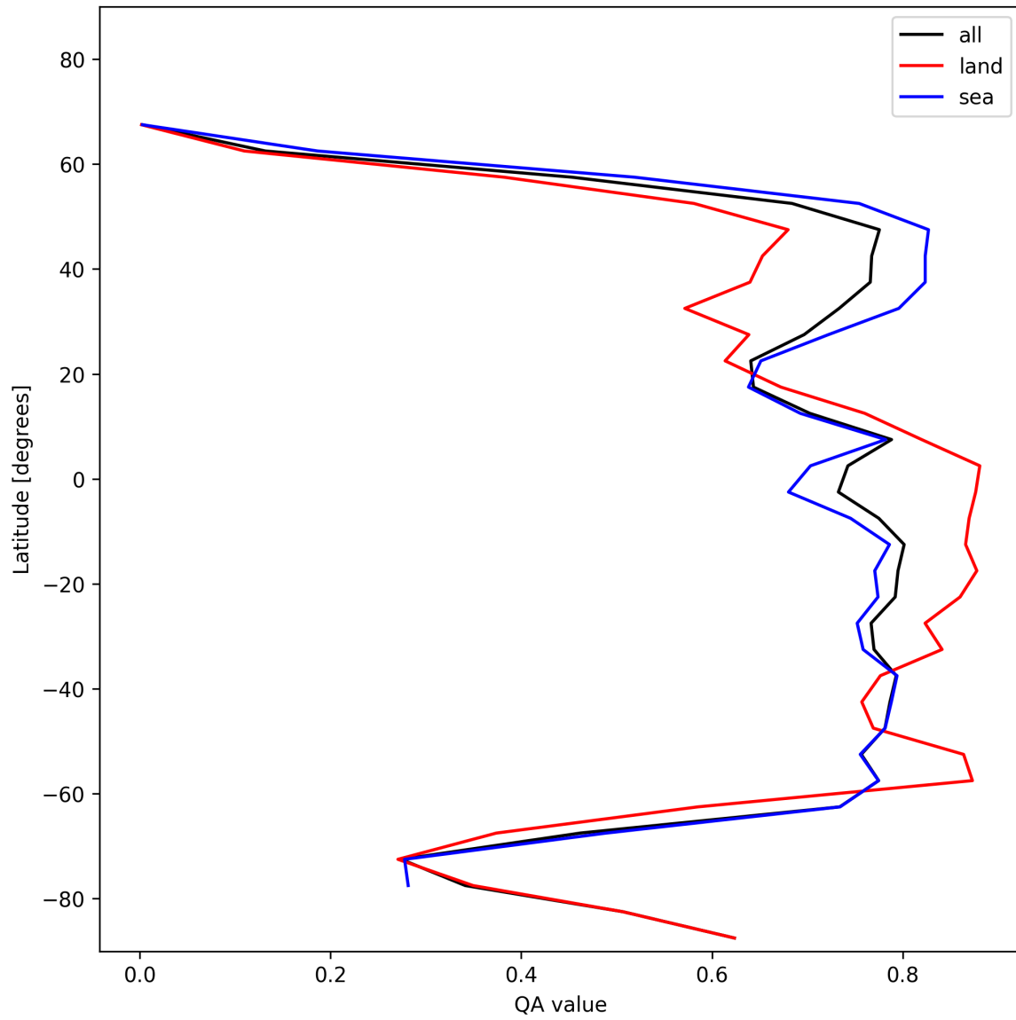
Figure 22: Zonal average of “QA value” for 2024-11-20 to 2024-11-22.
