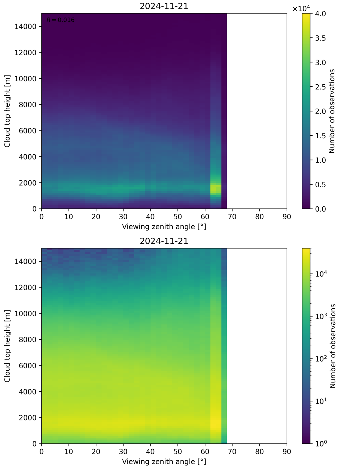
Figure 112: Scatter density plot of “Viewing zenith angle” against “Cloud top height” for 2024-11-20 to 2024-11-22.
