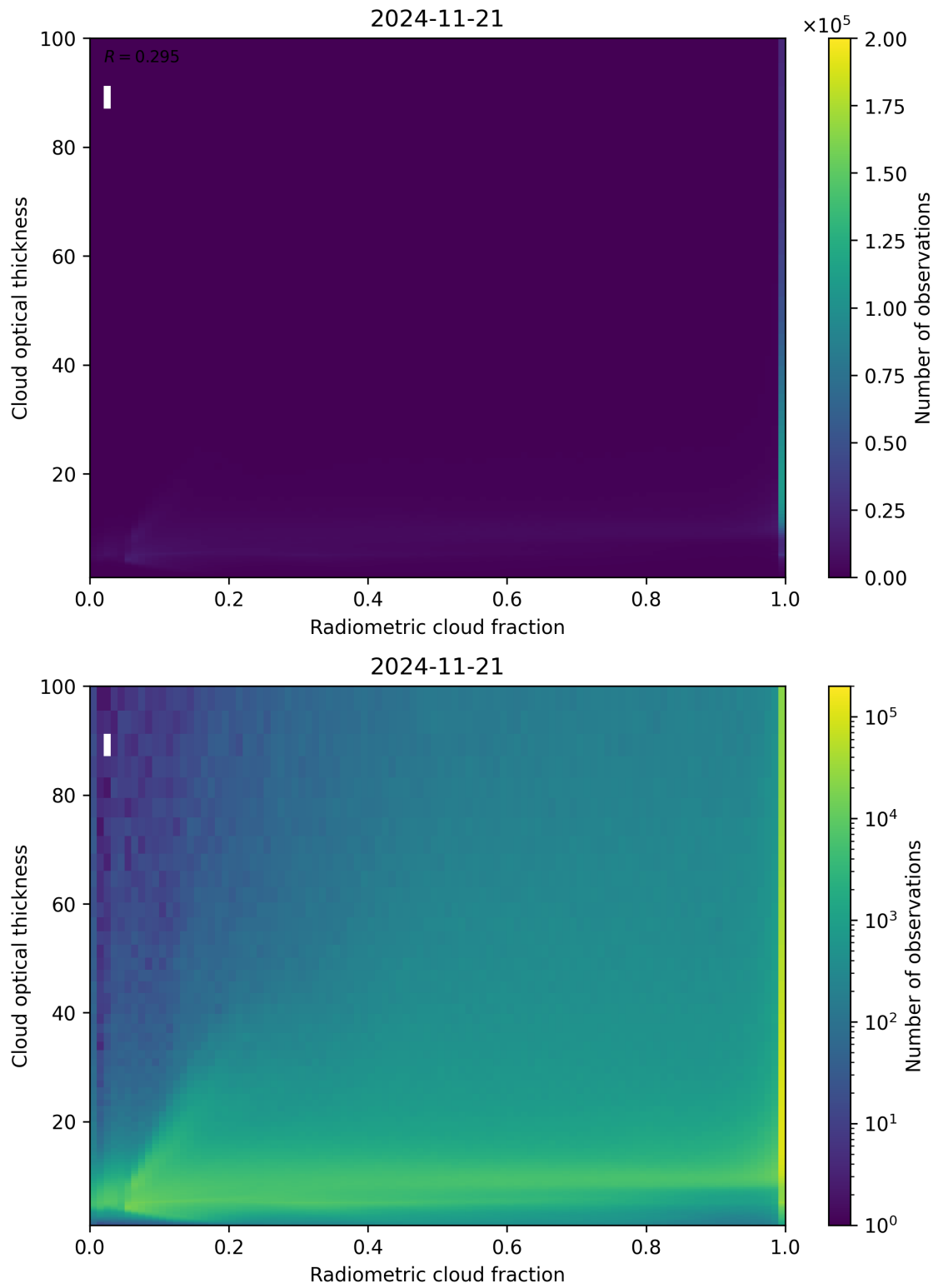
Figure 75: Scatter density plot of “Radiometric cloud fraction” against “Cloud optical thickness” for 2024-11-20 to 2024-11-22.
