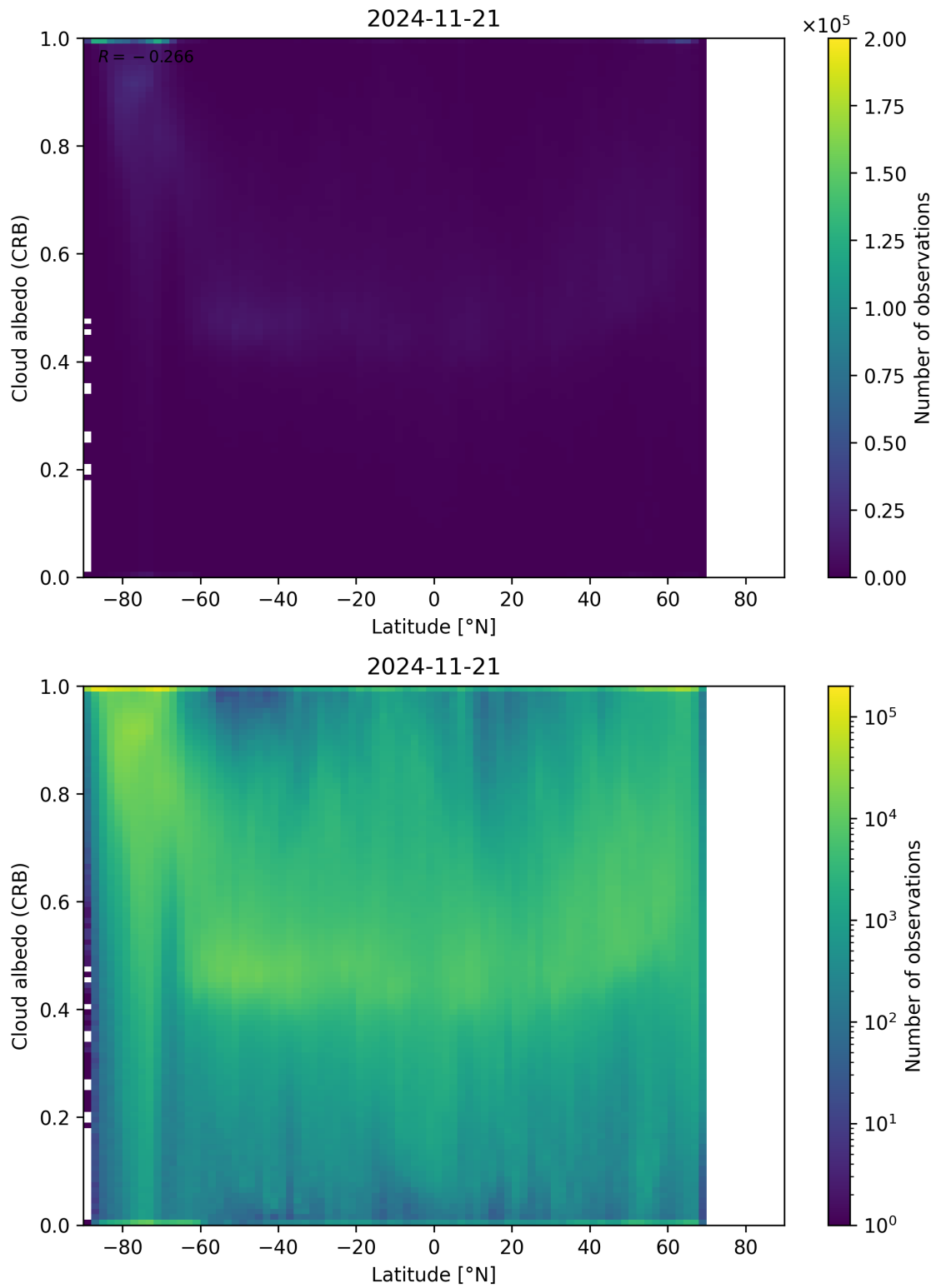
Figure 91: Scatter density plot of “Latitude” against “Cloud albedo (CRB)” for 2024-11-20 to 2024-11-22.
