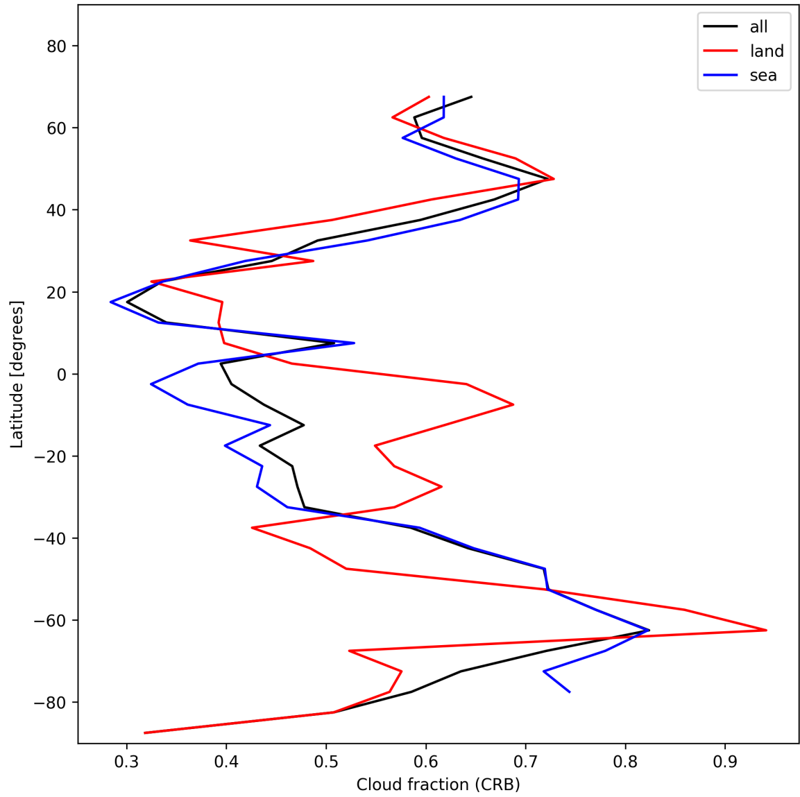
Figure 26: Zonal average of “Cloud fraction (CRB)” for 2024-11-20 to 2024-11-22.
