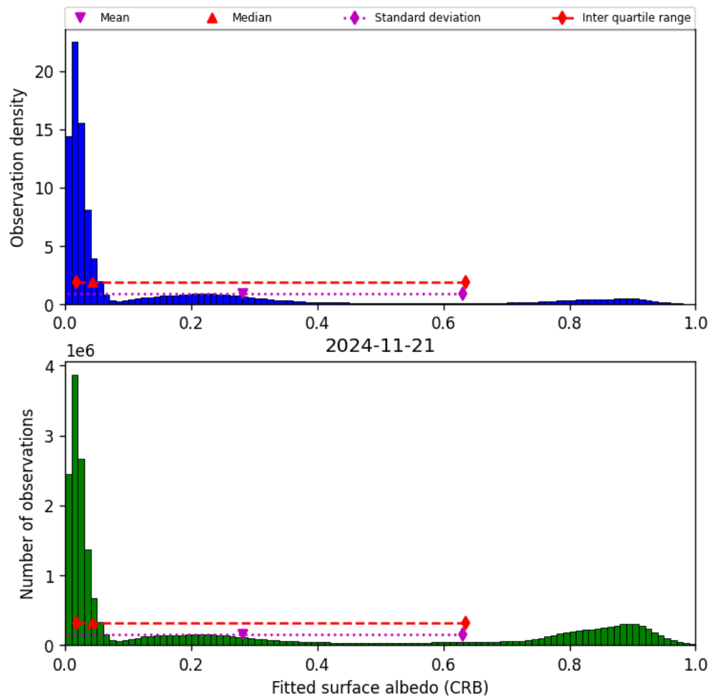
Figure 46: Histogram of “Fitted surface albedo (CRB)” for 2024-11-20 to 2024-11-22
