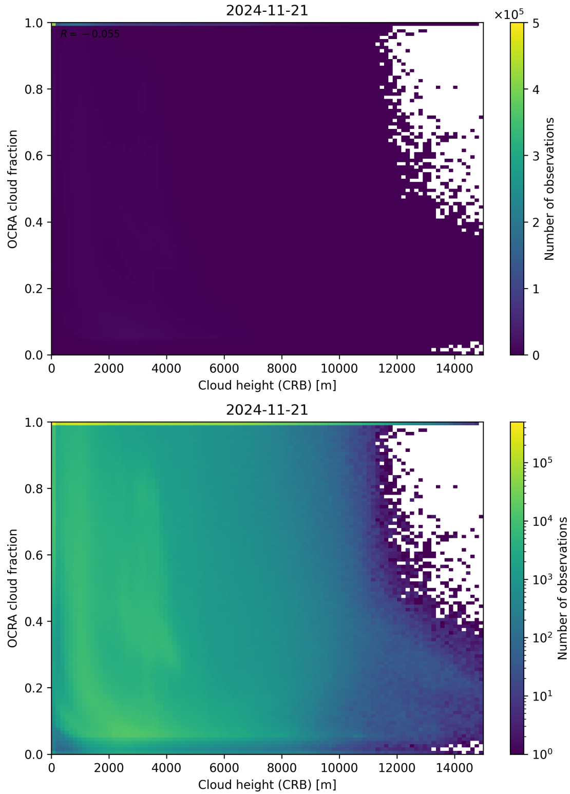
Figure 81: Scatter density plot of “Cloud height (CRB)” against “OCRA cloud fraction” for 2024-11-20 to 2024-11-22.
