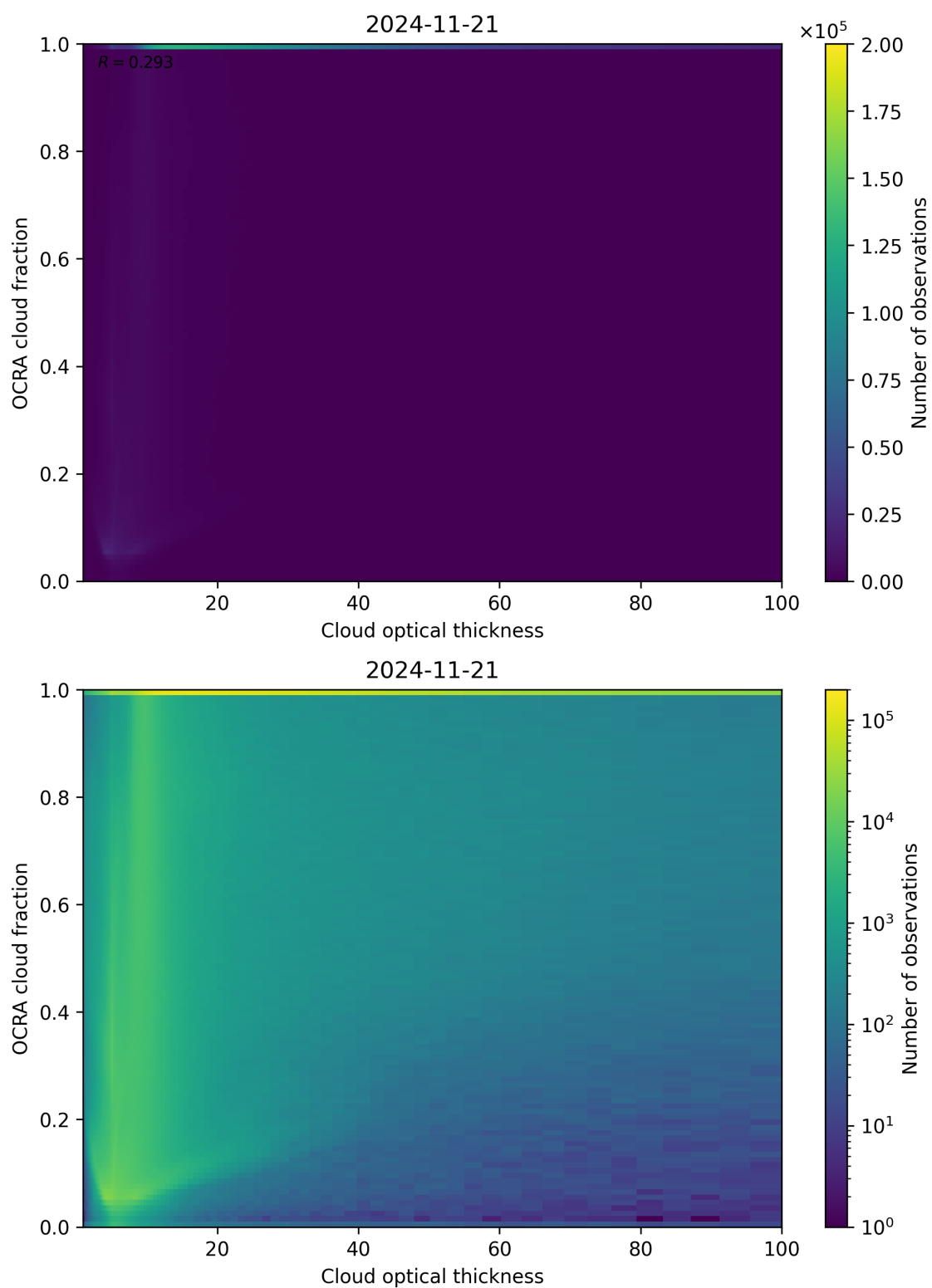
Figure 83: Scatter density plot of “Cloud optical thickness” against “OCRA cloud fraction” for 2024-11-20 to 2024-11-22.
