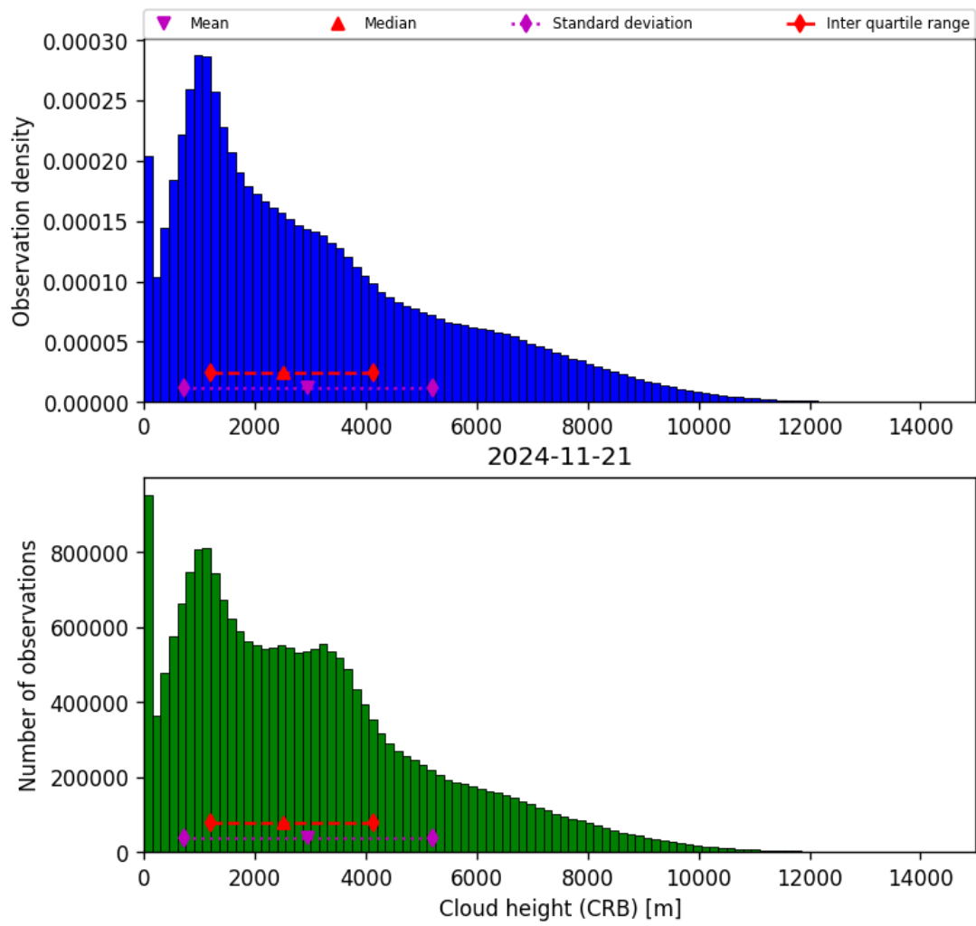
Figure 43: Histogram of “Cloud height (CRB)” for 2024-11-20 to 2024-11-22
