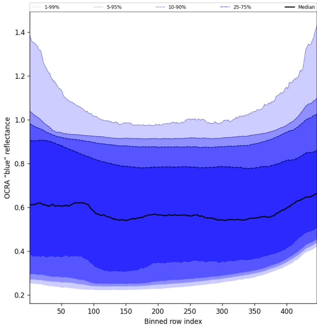
Figure 67: Along track statistics of "OCRA "blue" reflectance" for 2024-11-20 to 2024-11-22
