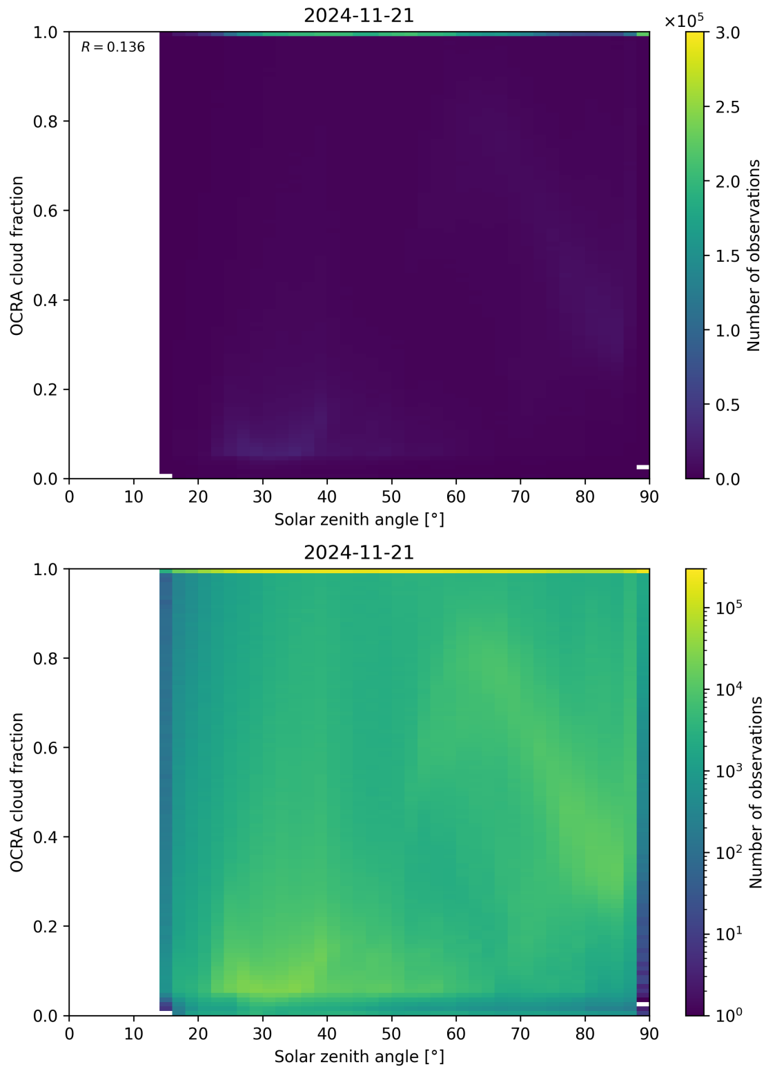
Figure 100: Scatter density plot of “Solar zenith angle” against “OCRA cloud fraction” for 2024-11-20 to 2024-11-22.
