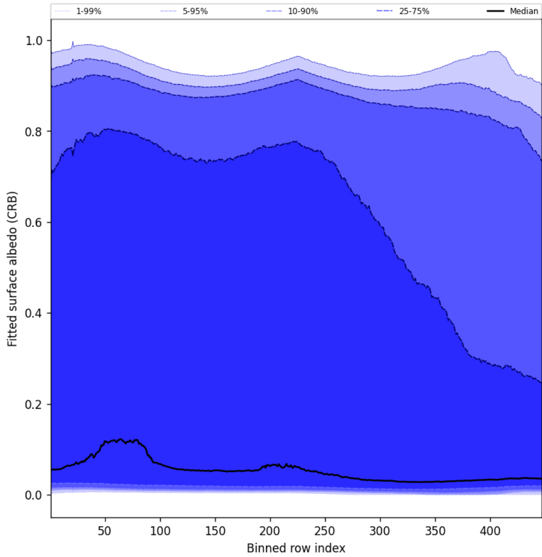
Figure 62: Along track statistics of “Fitted surface albedo (CRB)” for 2024-11-20 to 2024-11-22
