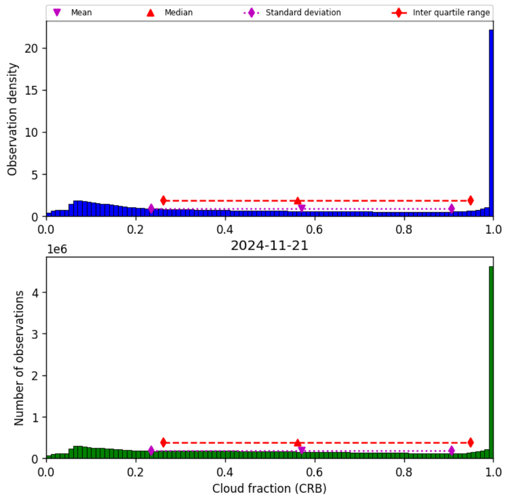
Figure 42: Histogram of “Cloud fraction (CRB)” for 2024-11-20 to 2024-11-22
