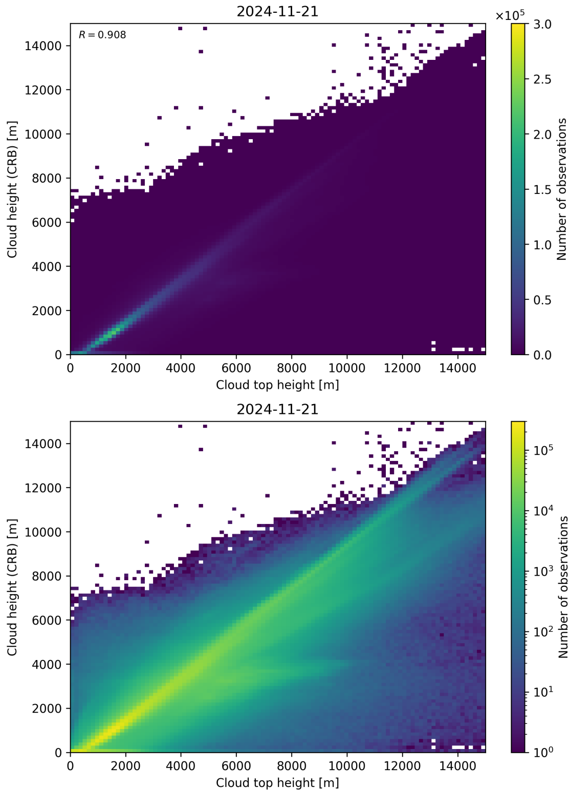
Figure 89: Scatter density plot of “Cloud top height” against “Cloud height (CRB)” for 2024-11-20 to 2024-11-22.
