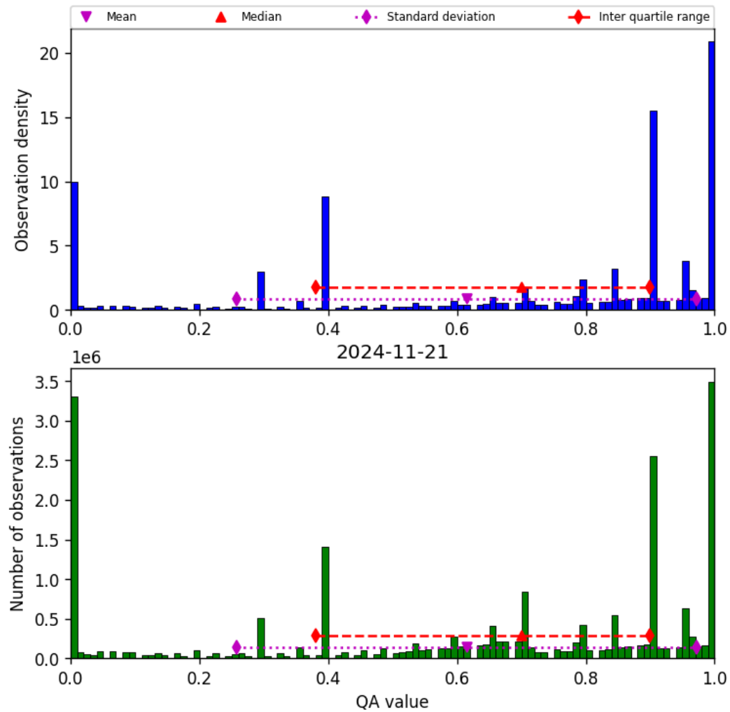
Figure 38: Histogram of “QA value” for 2024-11-20 to 2024-11-22
