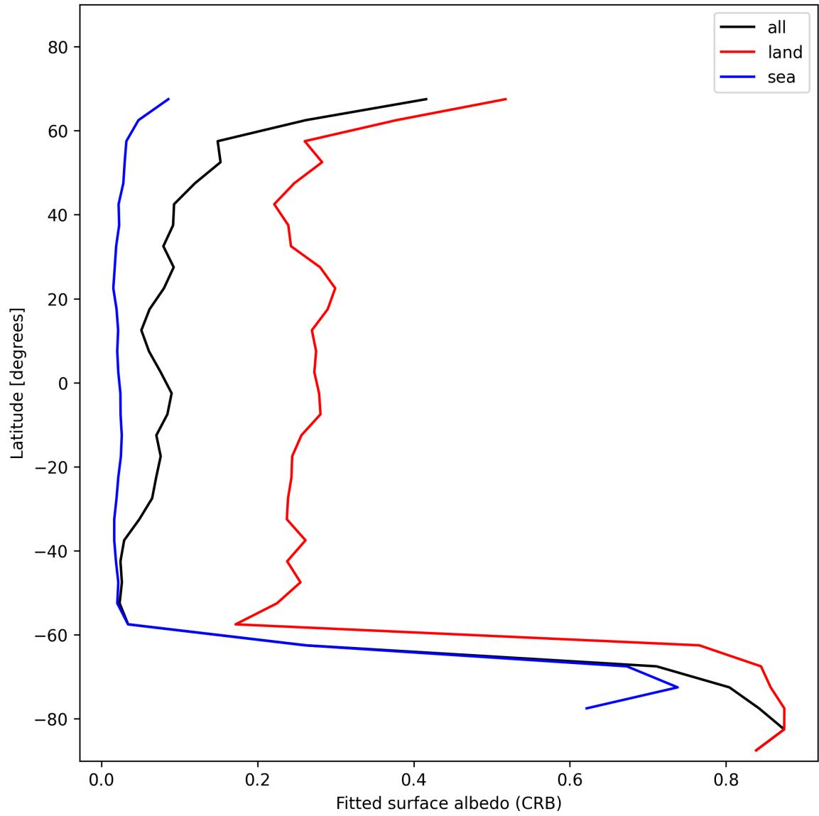
Figure 30: Zonal average of “Fitted surface albedo (CRB)” for 2024-11-20 to 2024-11-22.
