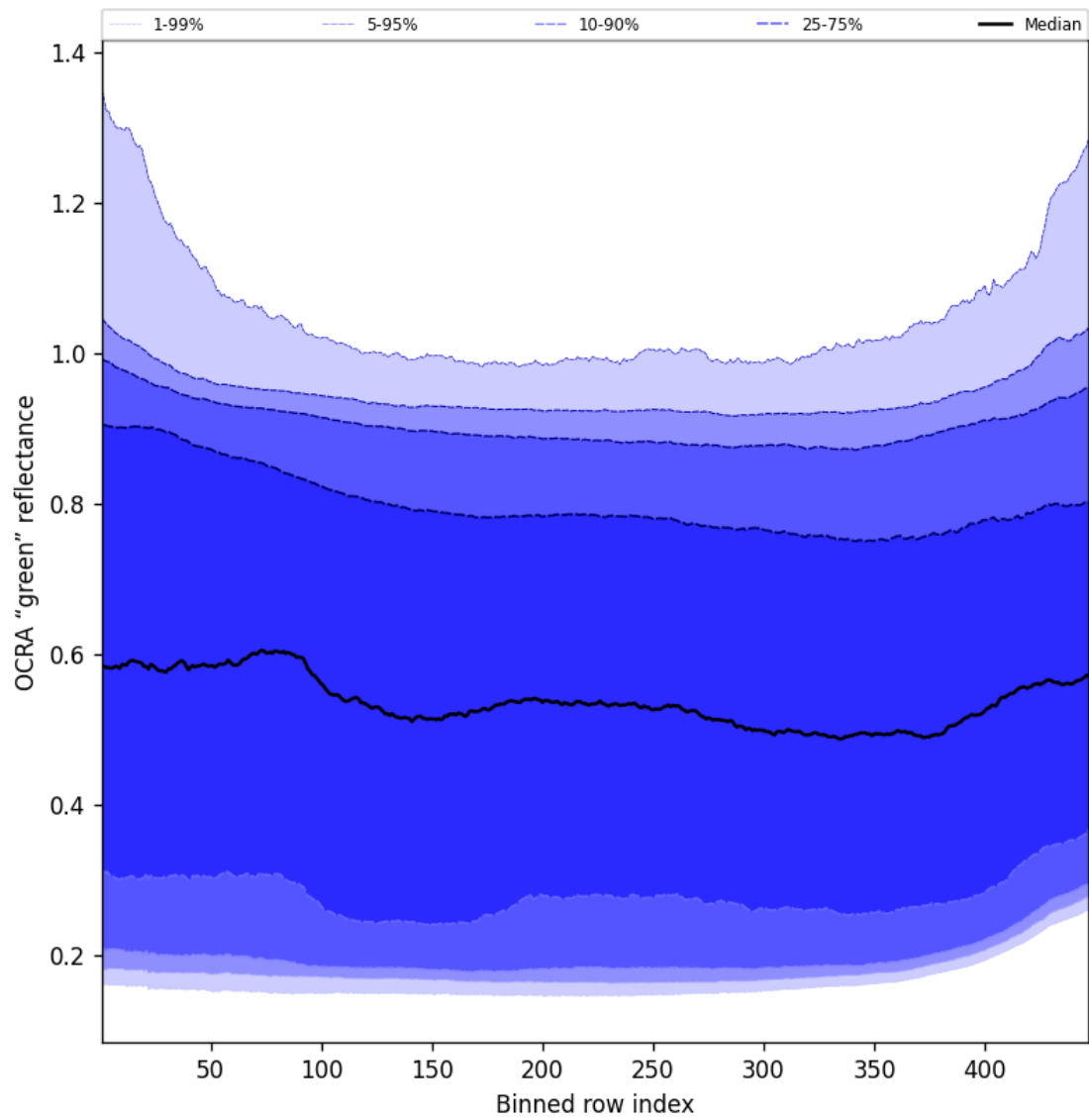
Figure 68: Along track statistics of “OCRA “green” reflectance” for 2024-11-20 to 2024-11-22
