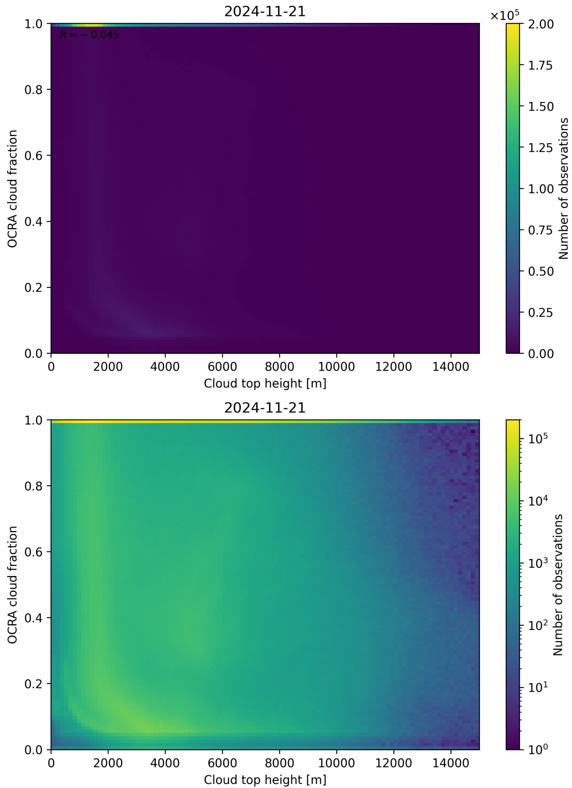
Figure 87: Scatter density plot of “Cloud top height” against “OCRA cloud fraction” for 2024-11-20 to 2024-11-22.
