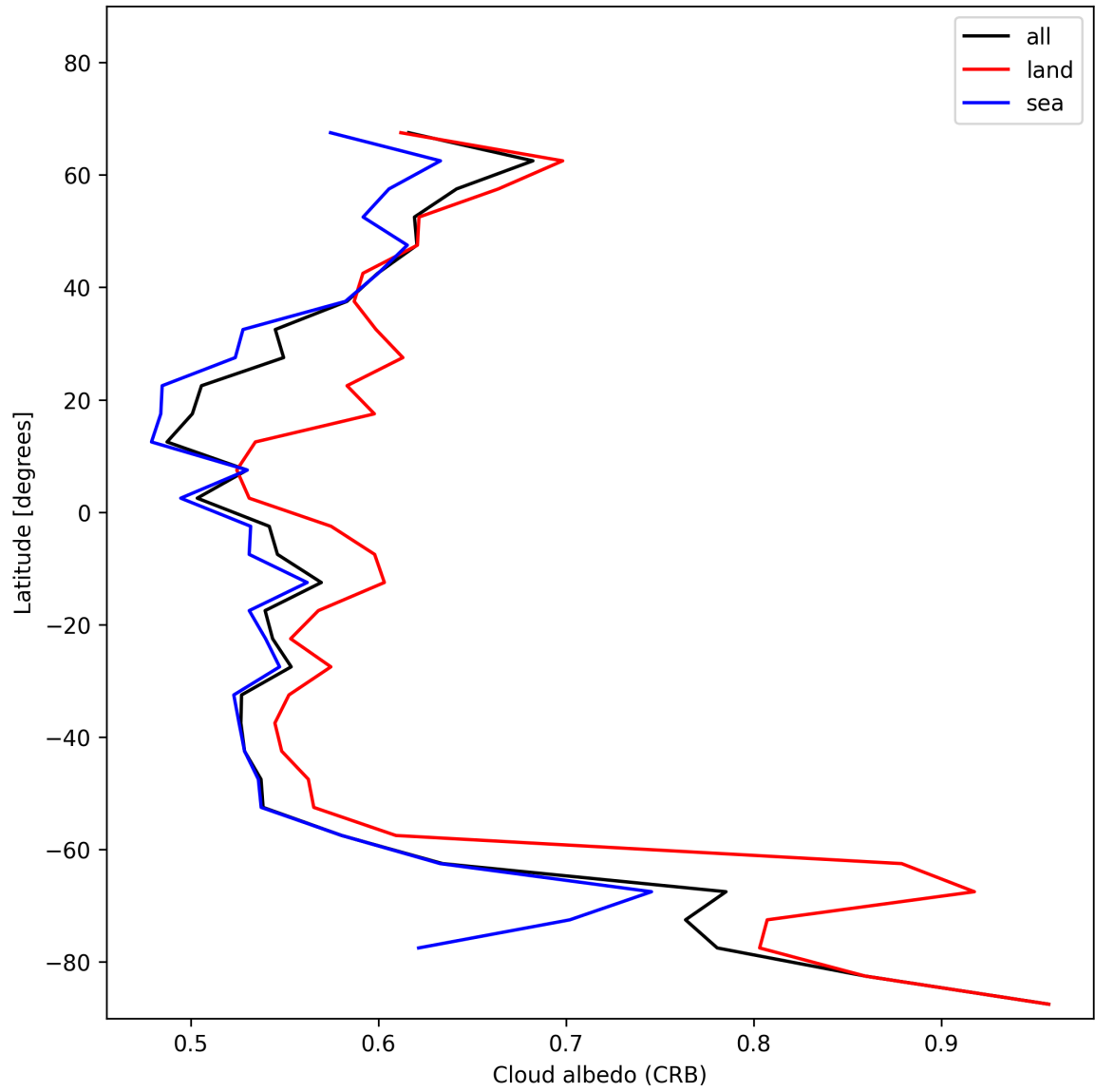
Figure 28: Zonal average of “Cloud albedo (CRB)” for 2024-11-20 to 2024-11-22.
