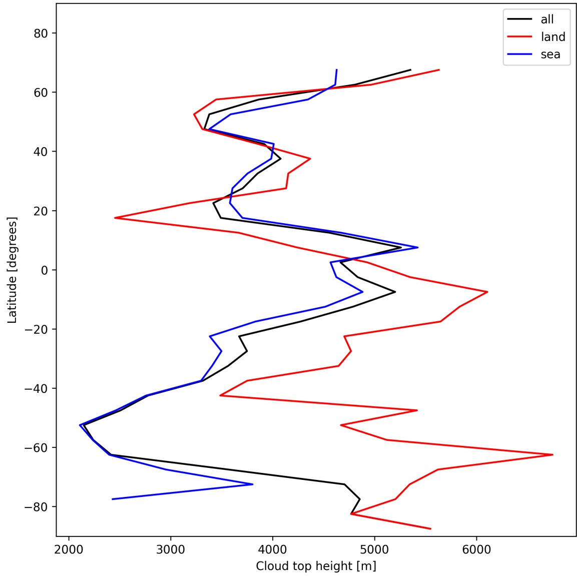
Figure 24: Zonal average of “Cloud top height” for 2024-11-20 to 2024-11-22.
