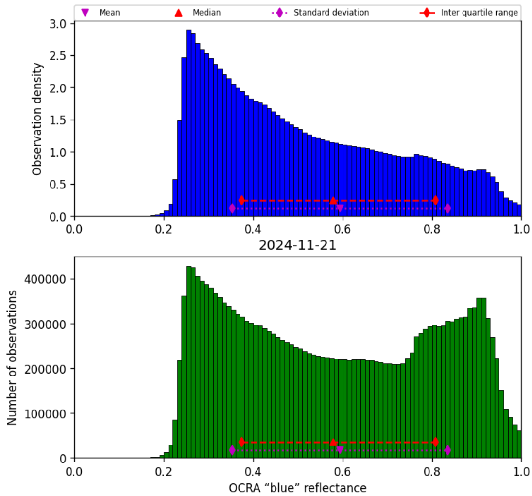
Figure 51: Histogram of “OCRA “blue” reflectance” for 2024-11-20 to 2024-11-22
