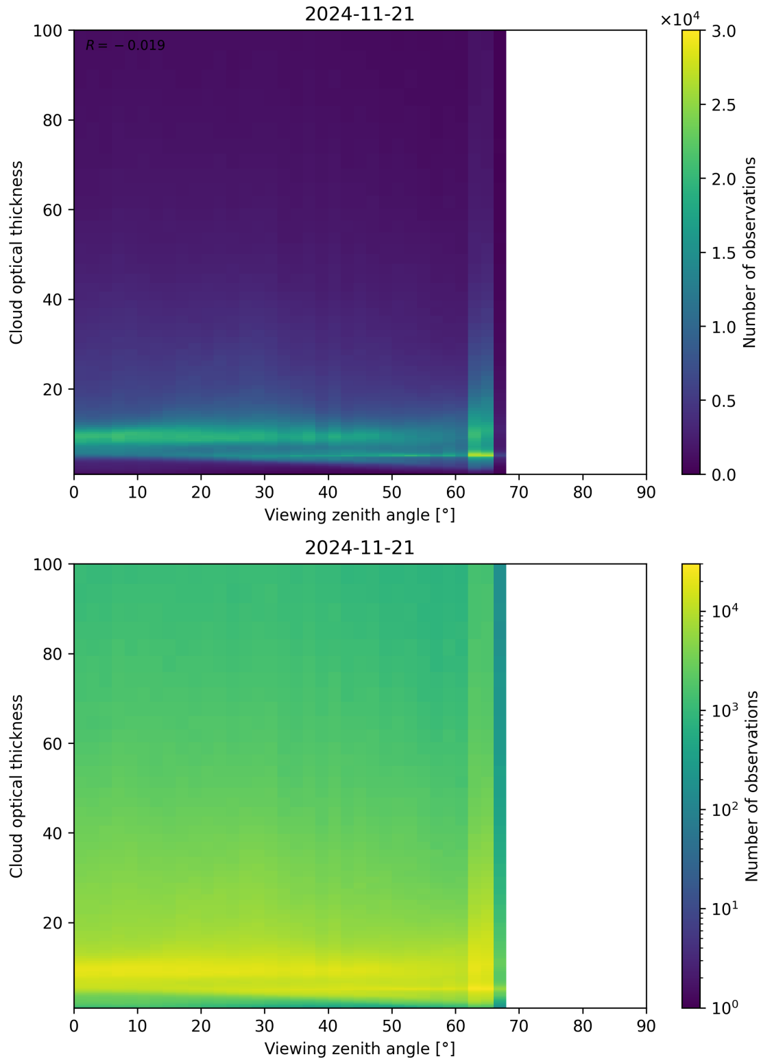
Figure 111: Scatter density plot of “Viewing zenith angle” against “Cloud optical thickness” for 2024-11-20 to 2024-11-22.
