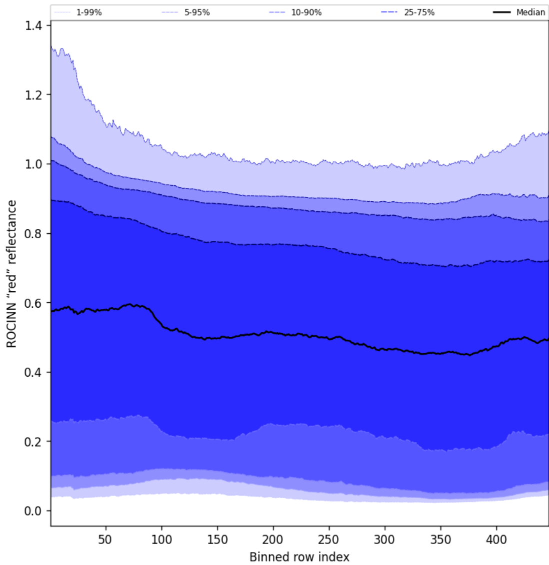
Figure 69: Along track statistics of “ROCINN “red” reflectance” for 2024-11-20 to 2024-11-22
