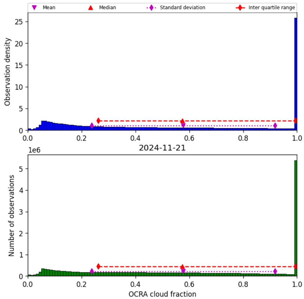
Figure 50: Histogram of “OCRA cloud fraction” for 2024-11-20 to 2024-11-22
