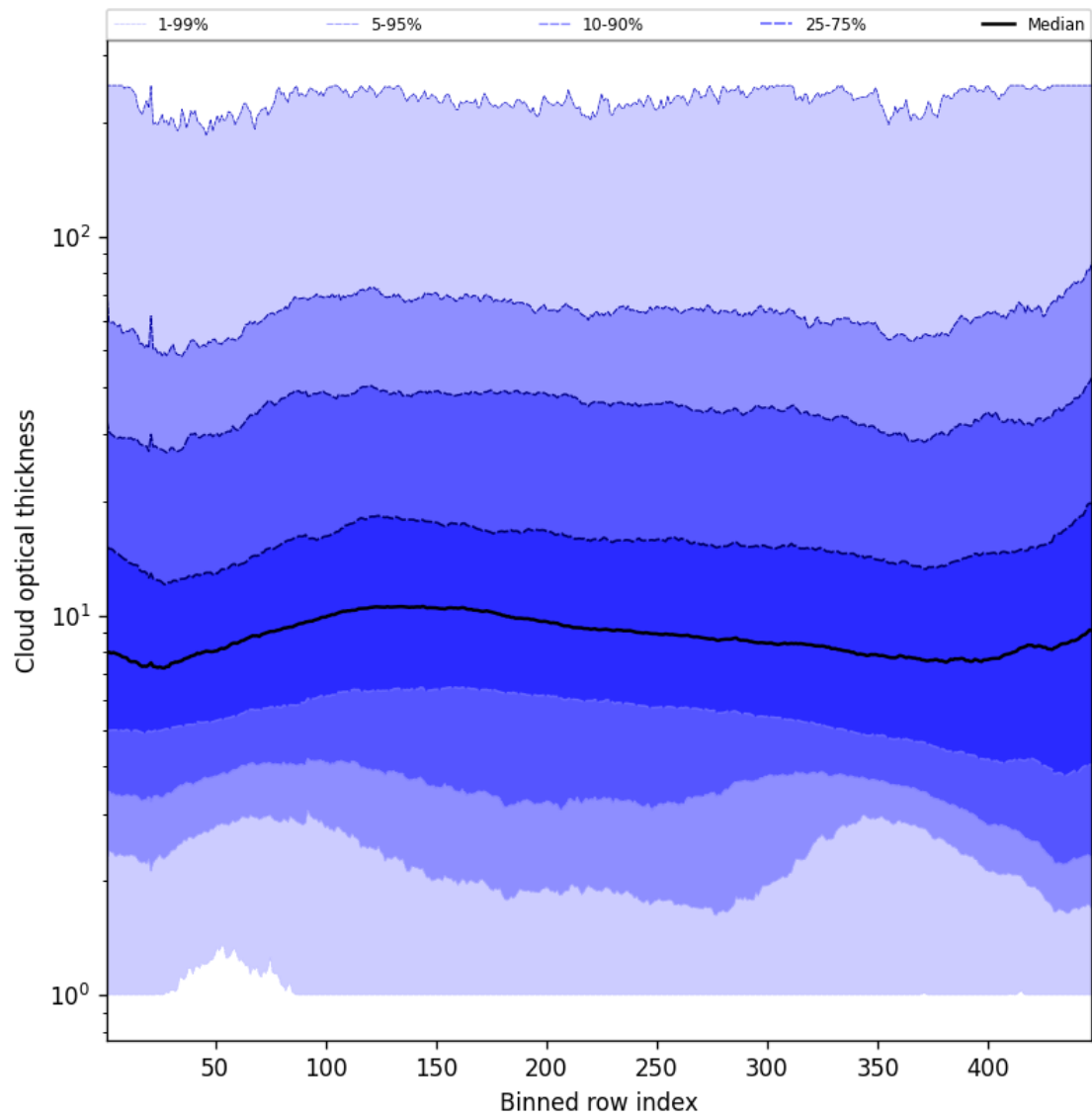
Figure 57: Along track statistics of “Cloud optical thickness” for 2024-11-20 to 2024-11-22
