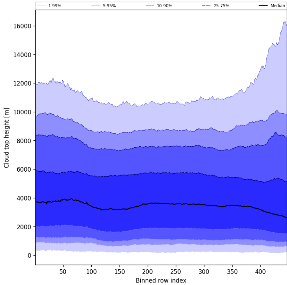
Figure 56: Along track statistics of “Cloud top height” for 2024-11-20 to 2024-11-22
