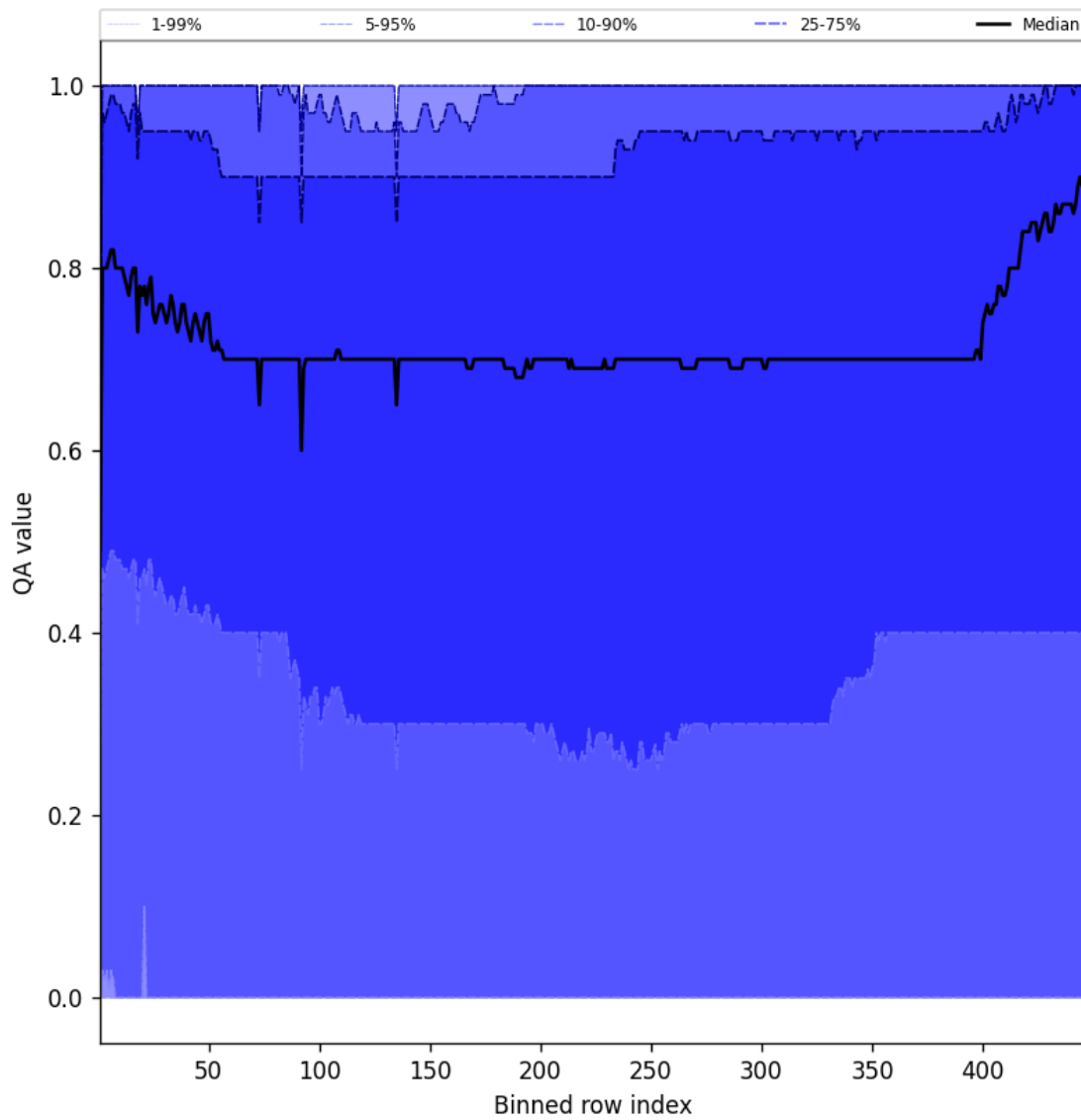
Figure 54: Along track statistics of “QA value” for 2024-11-20 to 2024-11-22
