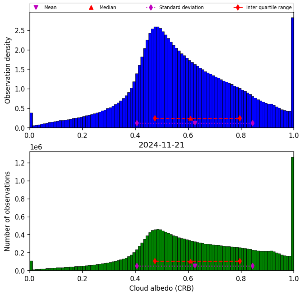
Figure 44: Histogram of “Cloud albedo (CRB)” for 2024-11-20 to 2024-11-22
