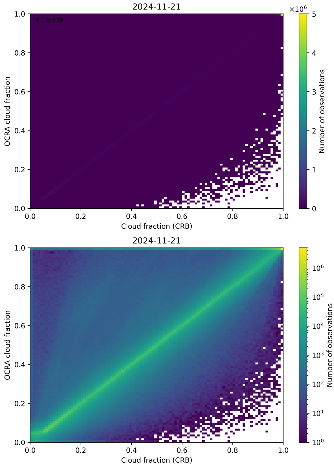
Figure 78: Scatter density plot of “Cloud fraction (CRB)” against “OCRA cloud fraction” for 2024-11-20 to 2024-11-22.
