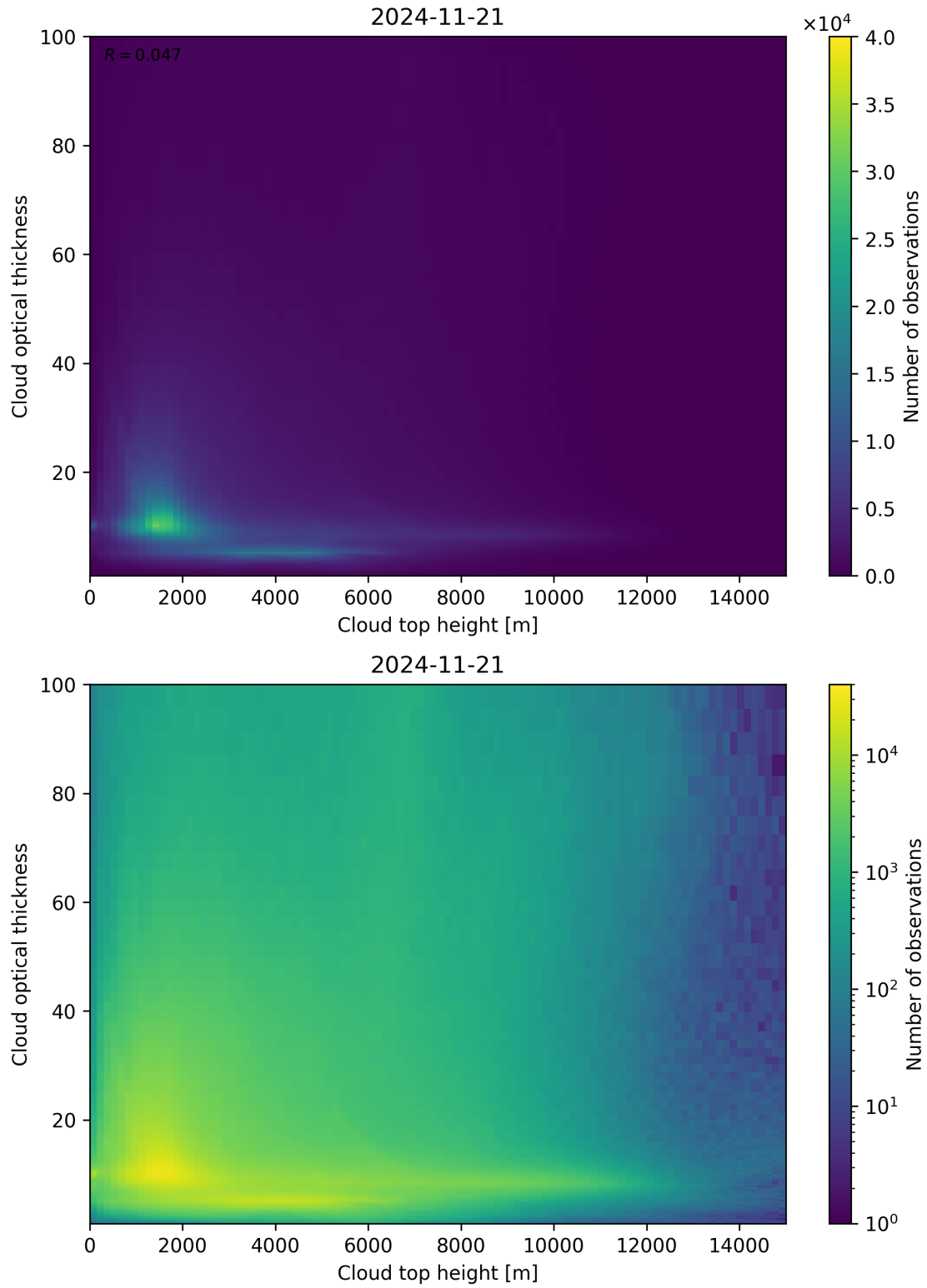
Figure 90: Scatter density plot of “Cloud top height” against “Cloud optical thickness” for 2024-11-20 to 2024-11-22.
