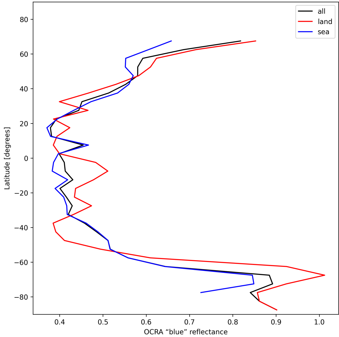
Figure 35: Zonal average of “OCRA “blue” reflectance” for 2024-11-20 to 2024-11-22.
