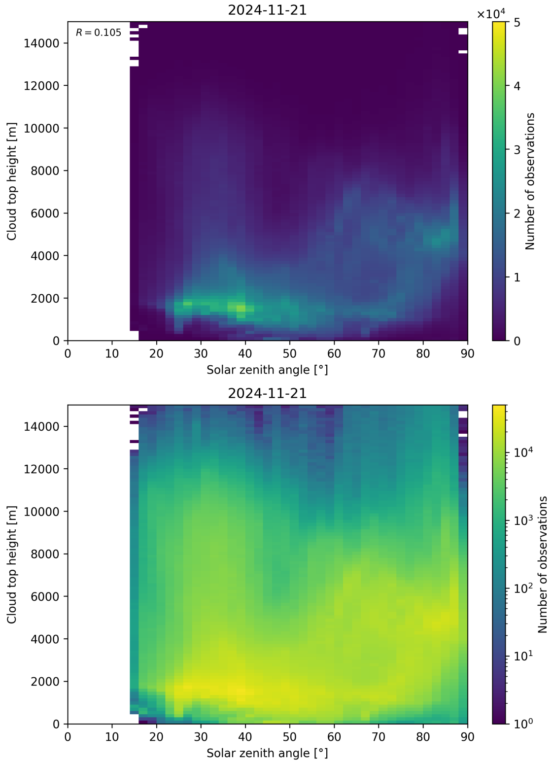
Figure 104: Scatter density plot of “Solar zenith angle” against “Cloud top height” for 2024-11-20 to 2024-11-22.
