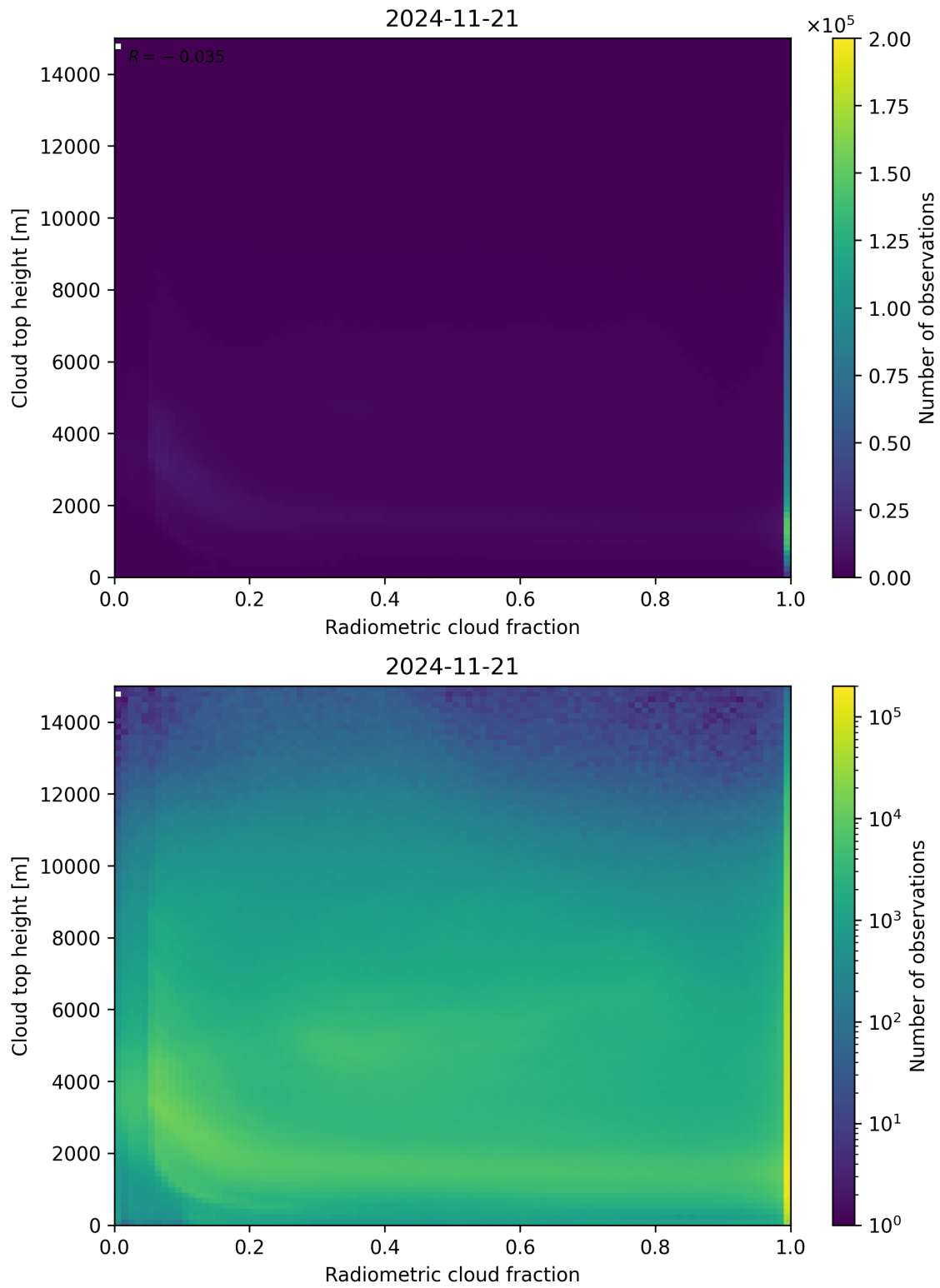
Figure 76: Scatter density plot of “Radiometric cloud fraction” against “Cloud top height” for 2024-11-20 to 2024-11-22.
