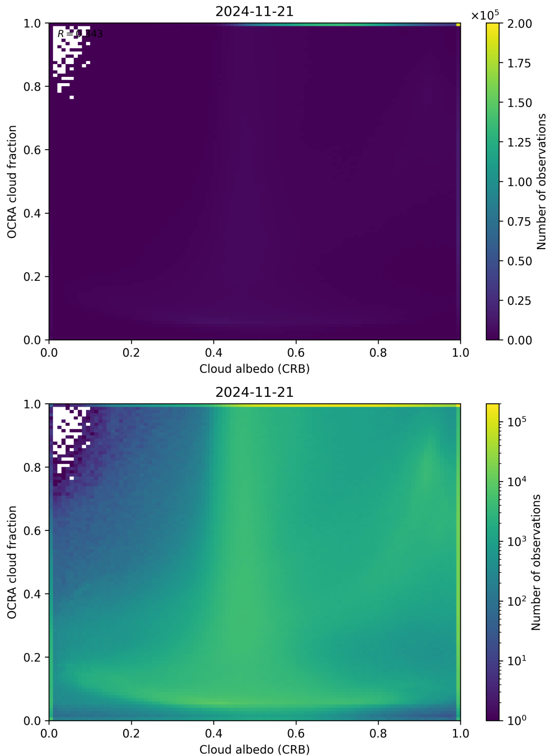
Figure 70: Scatter density plot of “Cloud albedo (CRB)” against “OCRA cloud fraction” for 2024-11-20 to 2024-11-22.
