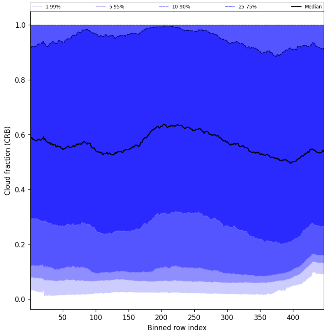
Figure 58: Along track statistics of “Cloud fraction (CRB)” for 2024-11-20 to 2024-11-22
