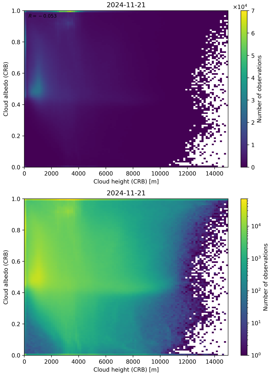
Figure 80: Scatter density plot of “Cloud height (CRB)” against “Cloud albedo (CRB)” for 2024-11-20 to 2024-11-22.
