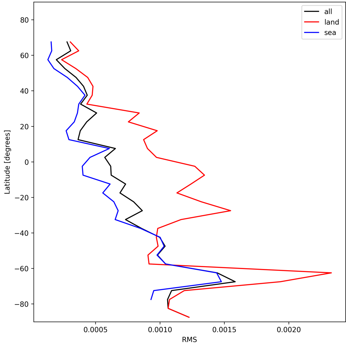
Figure 31: Zonal average of “RMS” for 2024-11-20 to 2024-11-22.
