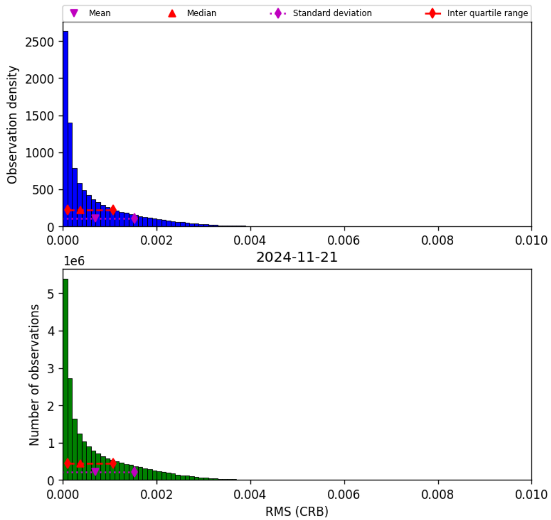
Figure 48: Histogram of “RMS (CRB)” for 2024-11-20 to 2024-11-22
