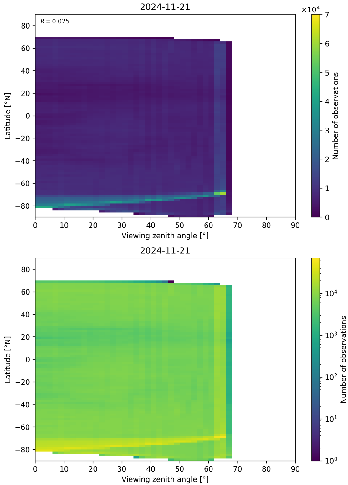
Figure 113: Scatter density plot of “Viewing zenith angle” against “Latitude” for 2024-11-20 to 2024-11-22.
