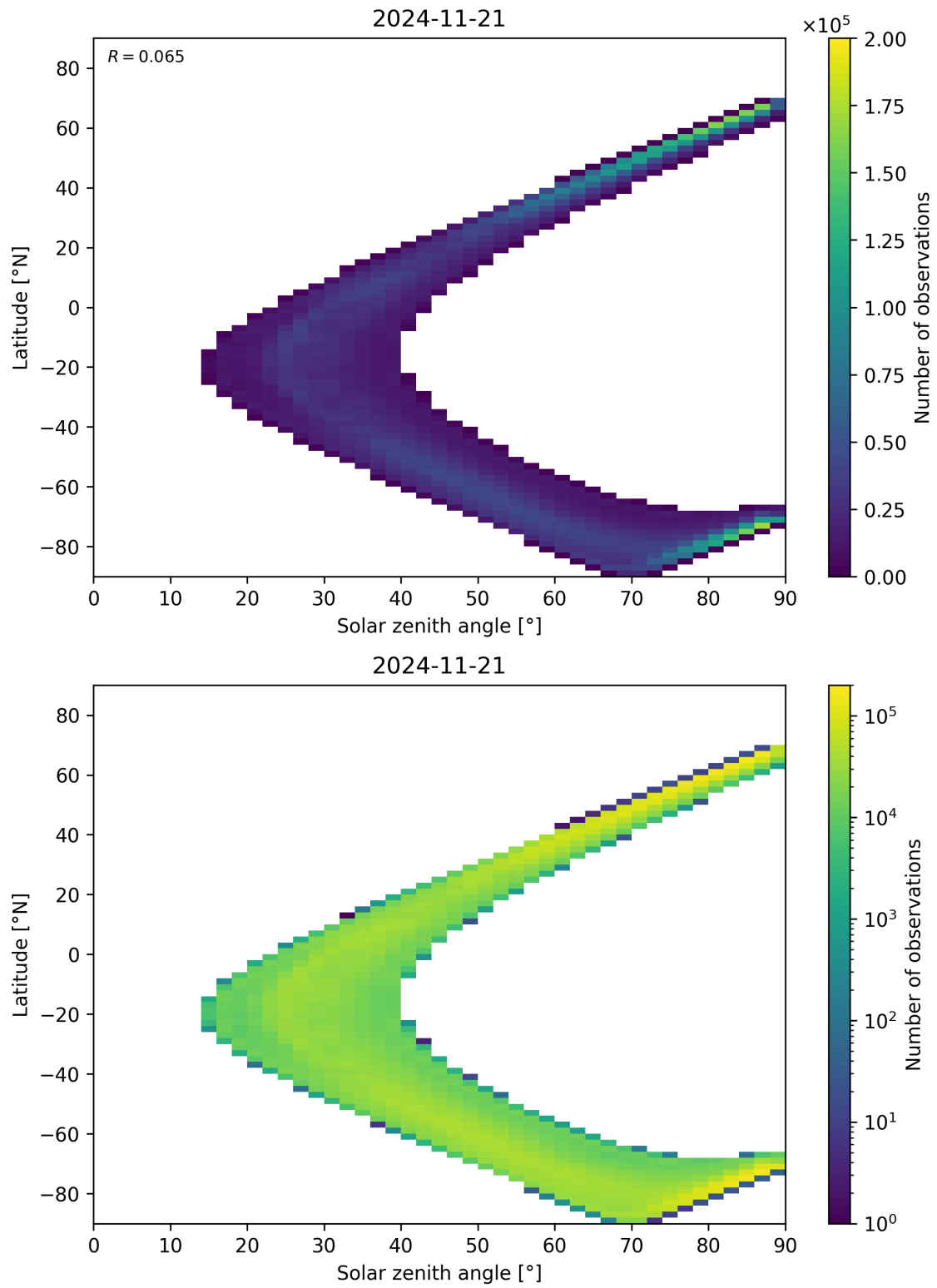
Figure 105: Scatter density plot of “Solar zenith angle” against “Latitude” for 2024-11-20 to 2024-11-22.
