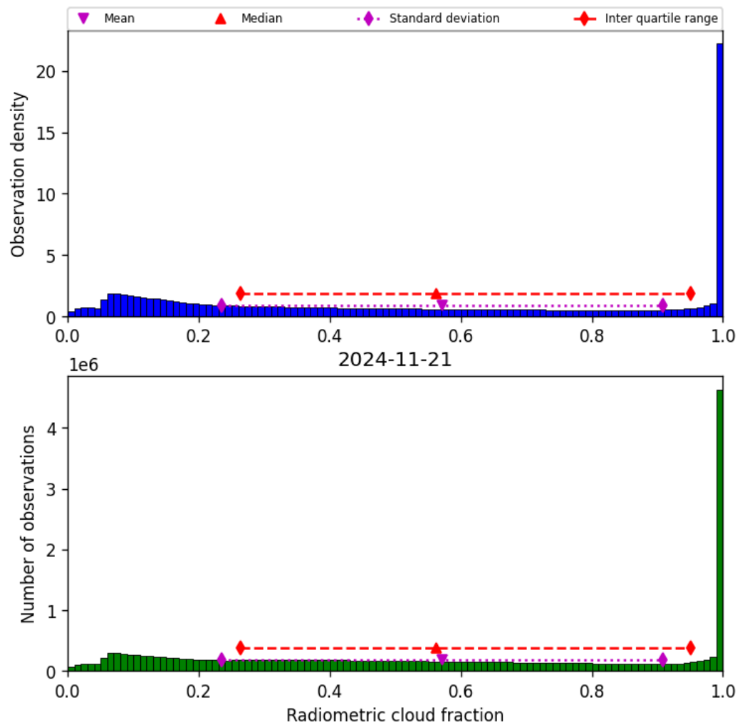
Figure 39: Histogram of “Radiometric cloud fraction” for 2024-11-20 to 2024-11-22
