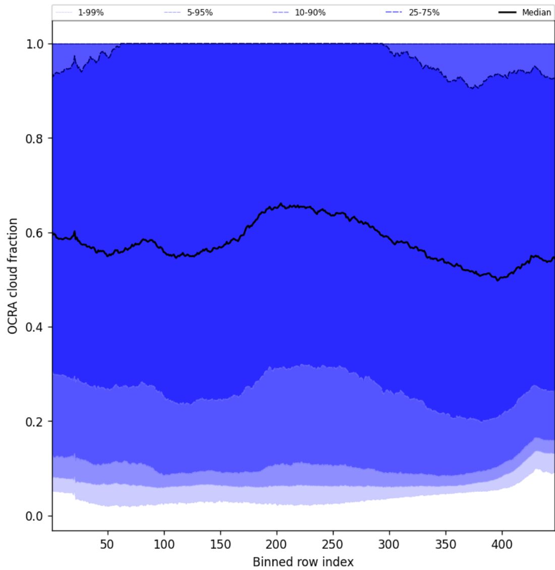
Figure 66: Along track statistics of “OCRA cloud fraction” for 2024-11-20 to 2024-11-22
