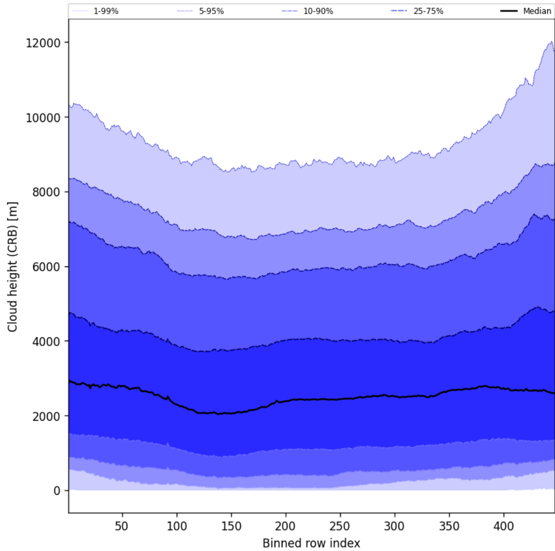
Figure 59: Along track statistics of “Cloud height (CRB)” for 2024-11-20 to 2024-11-22
