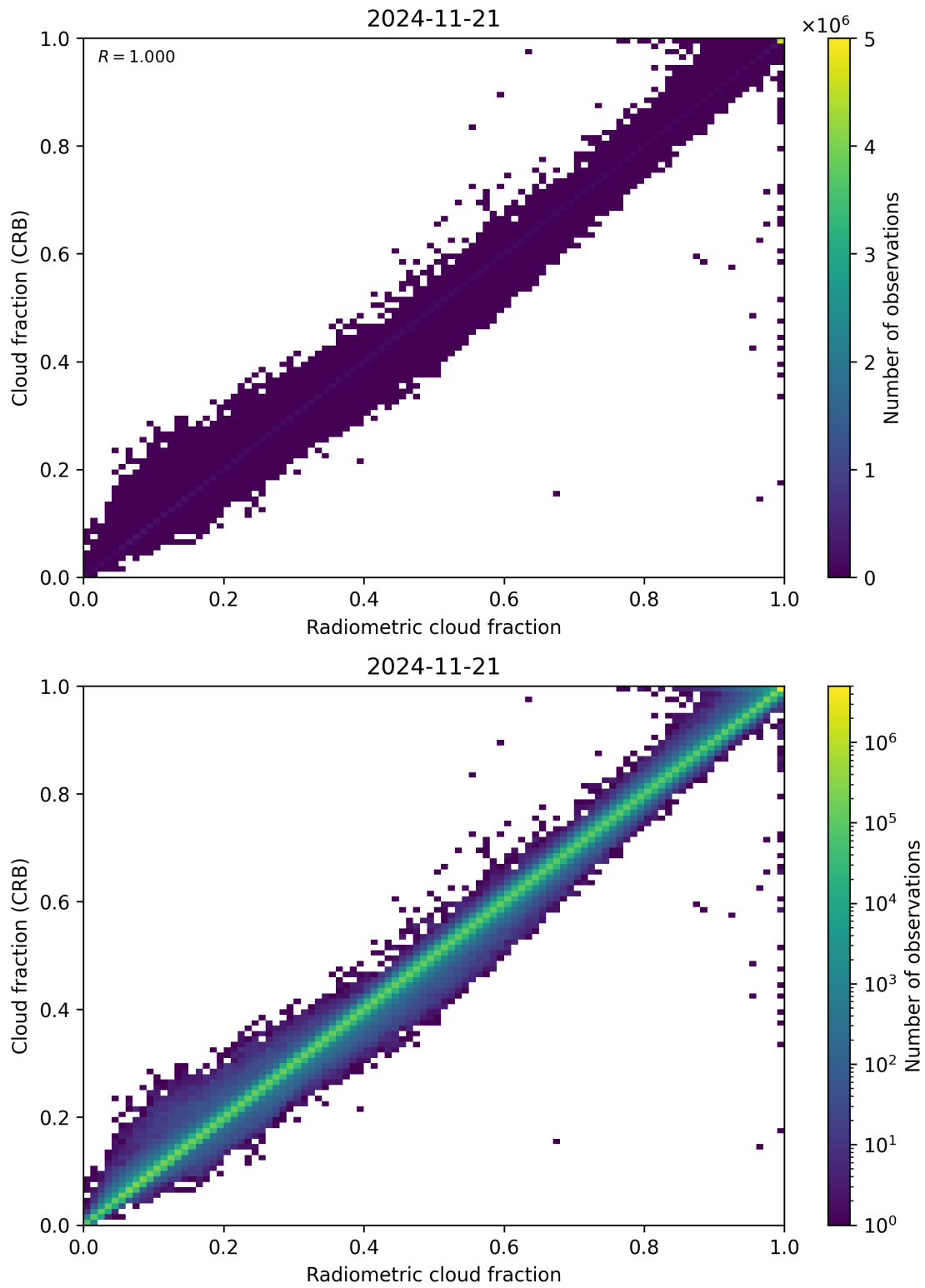
Figure 73: Scatter density plot of “Radiometric cloud fraction” against “Cloud fraction (CRB)” for 2024-11-20 to 2024-11-22.
