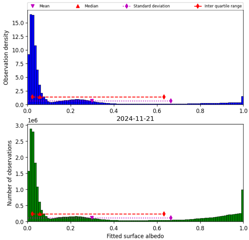
Figure 45: Histogram of “Fitted surface albedo” for 2024-11-20 to 2024-11-22
