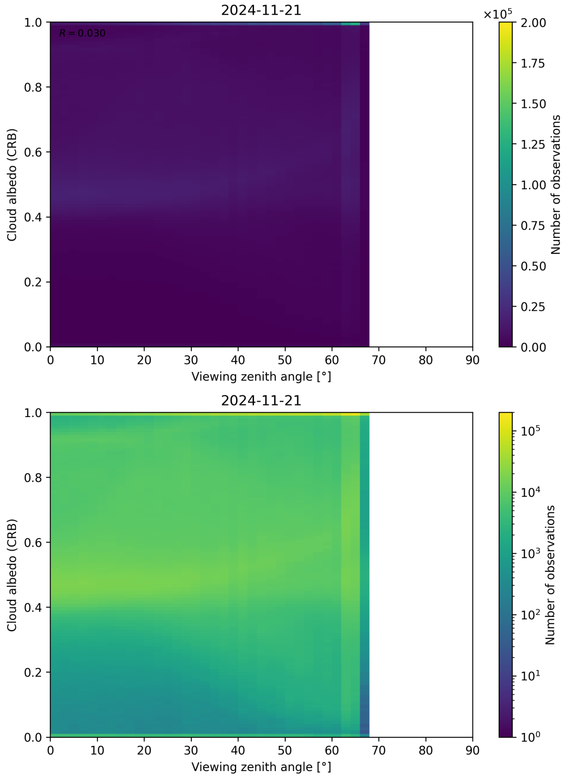
Figure 106: Scatter density plot of “Viewing zenith angle” against “Cloud albedo (CRB)” for 2024-11-20 to 2024-11-22.
