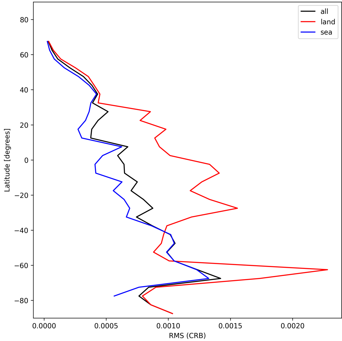
Figure 32: Zonal average of “RMS (CRB)” for 2024-11-20 to 2024-11-22.
