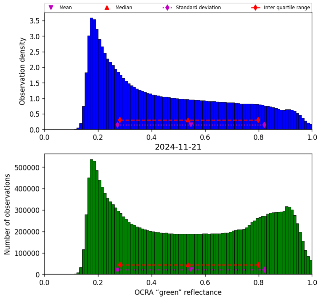
Figure 52: Histogram of “OCRA “green” reflectance” for 2024-11-20 to 2024-11-22
