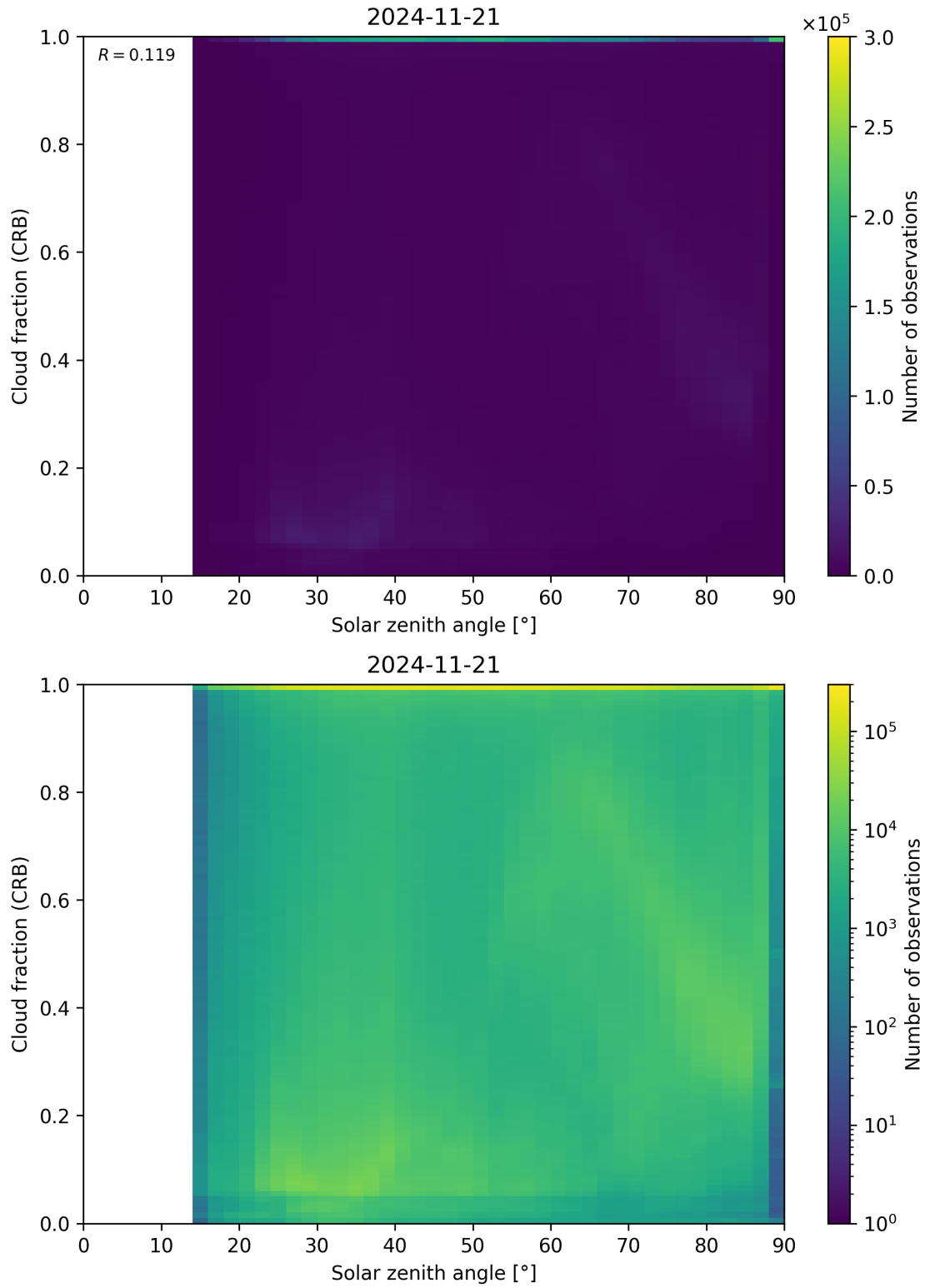
Figure 101: Scatter density plot of “Solar zenith angle” against “Cloud fraction (CRB)” for 2024-11-20 to 2024-11-22.
