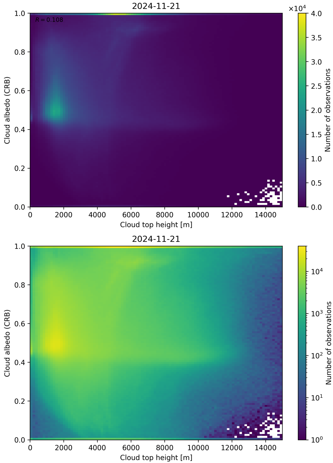
Figure 86: Scatter density plot of “Cloud top height” against “Cloud albedo (CRB)” for 2024-11-20 to 2024-11-22.
