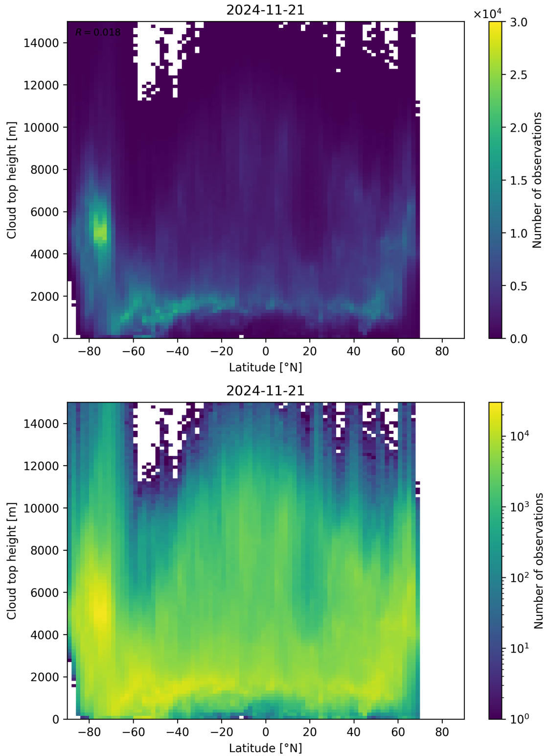
Figure 97: Scatter density plot of “Latitude” against “Cloud top height” for 2024-11-20 to 2024-11-22.
