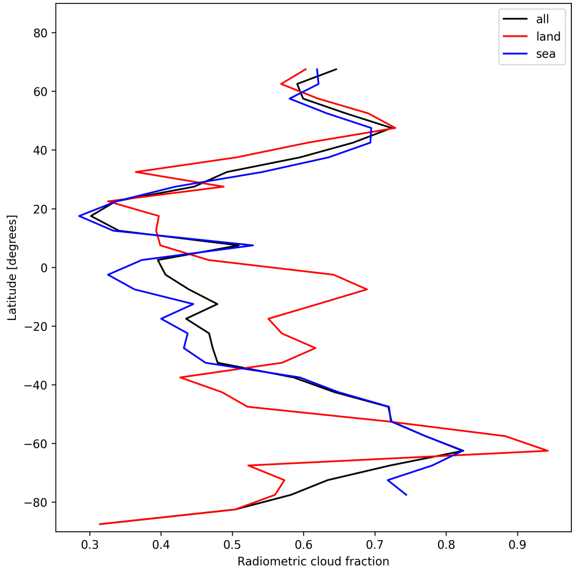
Figure 23: Zonal average of “Radiometric cloud fraction” for 2024-11-20 to 2024-11-22.
