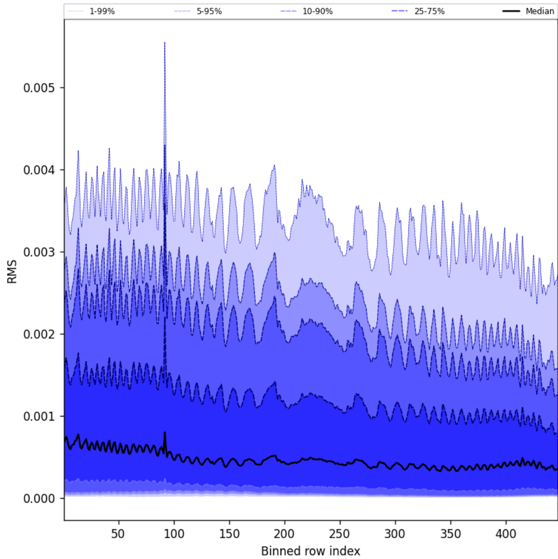
Figure 63: Along track statistics of “RMS” for 2024-11-20 to 2024-11-22
