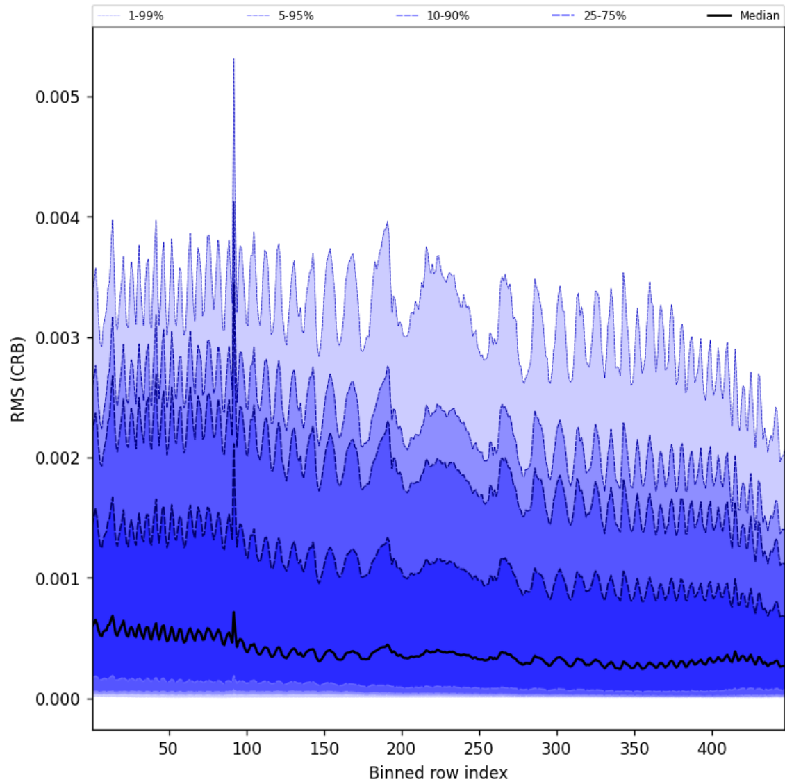
Figure 64: Along track statistics of “RMS (CRB)” for 2024-11-20 to 2024-11-22
