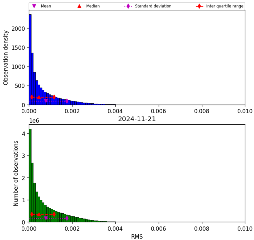
Figure 47: Histogram of “RMS” for 2024-11-20 to 2024-11-22
