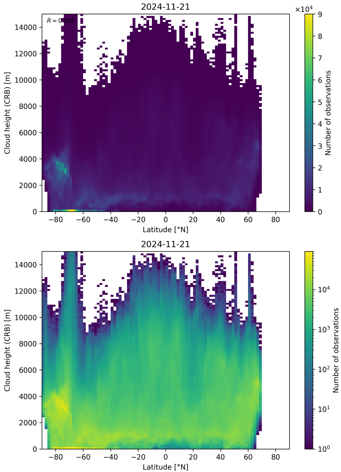
Figure 95: Scatter density plot of “Latitude” against “Cloud height (CRB)” for 2024-11-20 to 2024-11-22.
