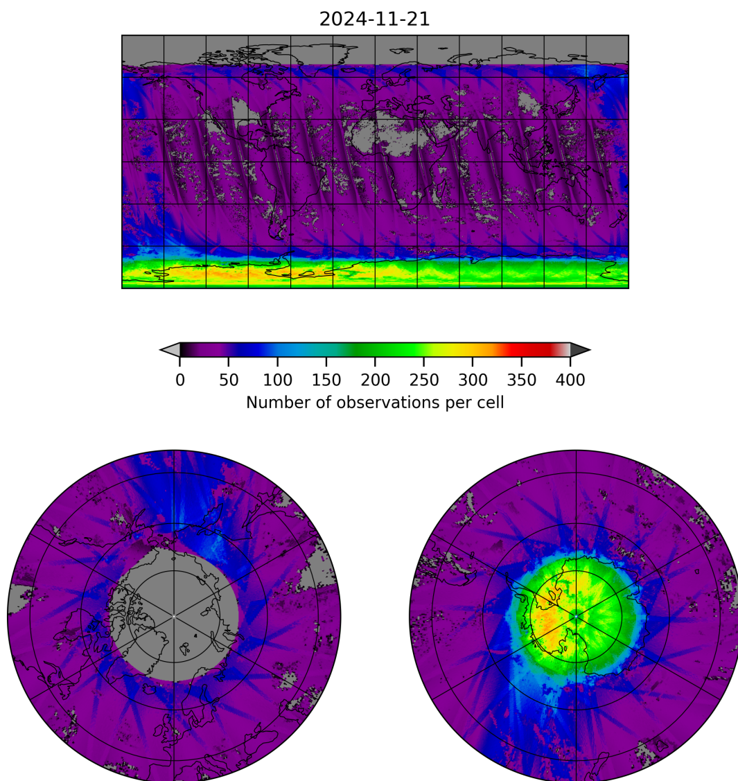
Figure 21: Map of the number of observations for 2024-11-20 to 2024-11-22
