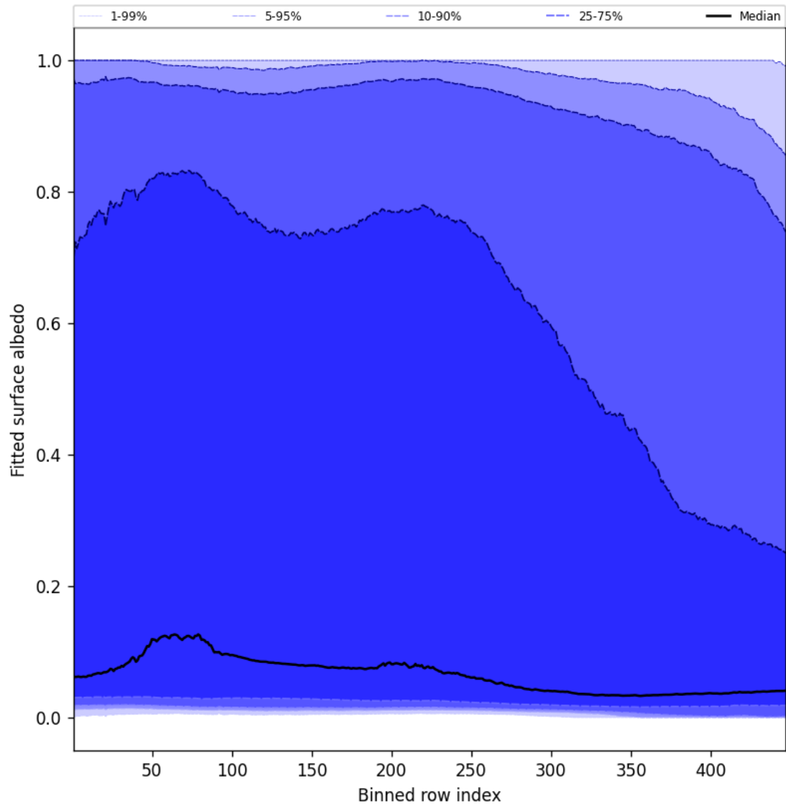
Figure 61: Along track statistics of “Fitted surface albedo” for 2024-11-20 to 2024-11-22
