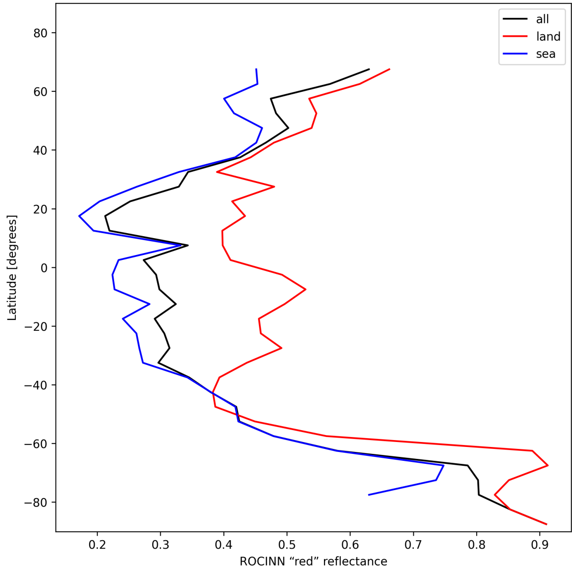
Figure 37: Zonal average of “ROCINN “red” reflectance” for 2024-11-20 to 2024-11-22.
