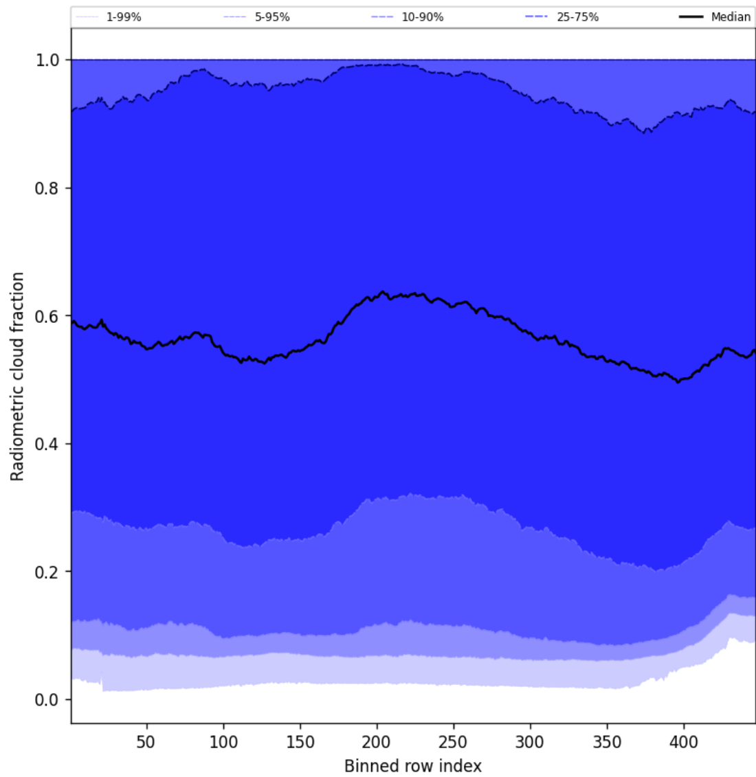
Figure 55: Along track statistics of “Radiometric cloud fraction” for 2024-11-20 to 2024-11-22
