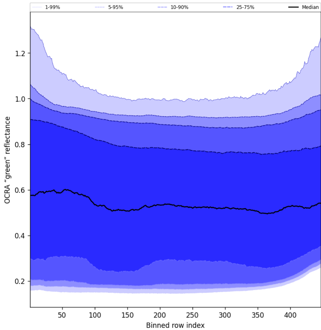
Figure 68: Along track statistics of "OCRA "green" reflectance" for 2024-11-21 to 2024-11-23
