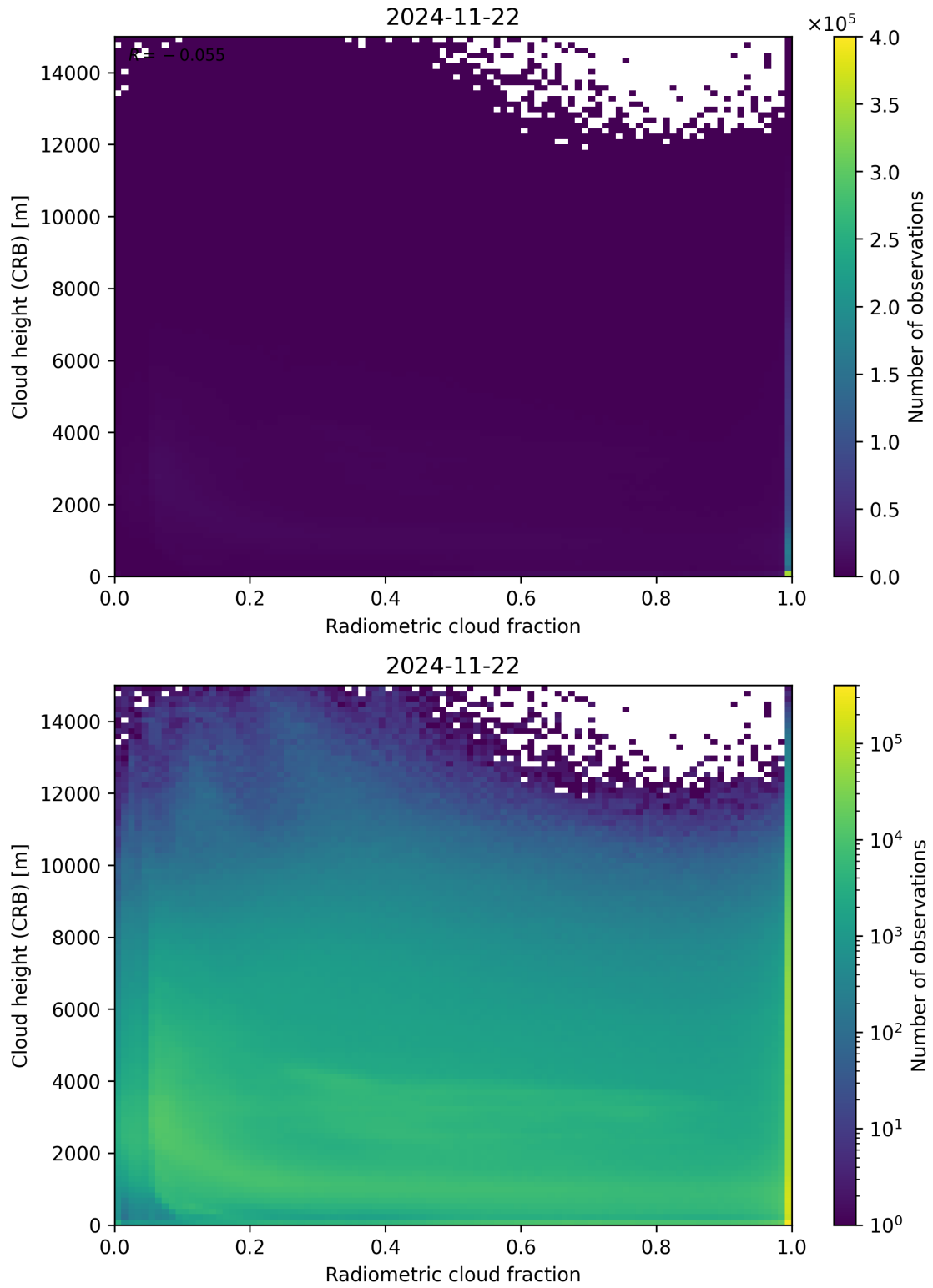
Figure 74: Scatter density plot of “Radiometric cloud fraction” against “Cloud height (CRB)” for 2024-11-21 to 2024-11-23.
