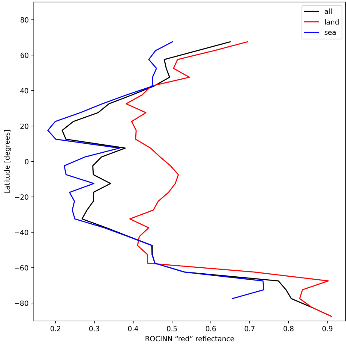
Figure 37: Zonal average of “ROCINN “red” reflectance” for 2024-11-21 to 2024-11-23.
