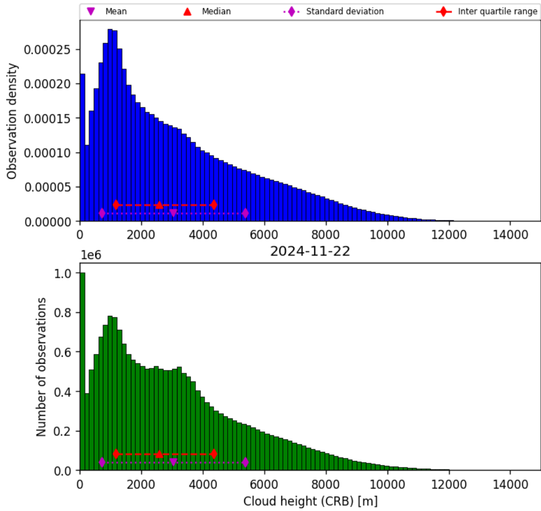
Figure 43: Histogram of “Cloud height (CRB)” for 2024-11-21 to 2024-11-23
