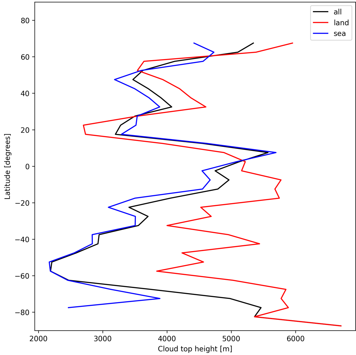
Figure 24: Zonal average of “Cloud top height” for 2024-11-21 to 2024-11-23.
