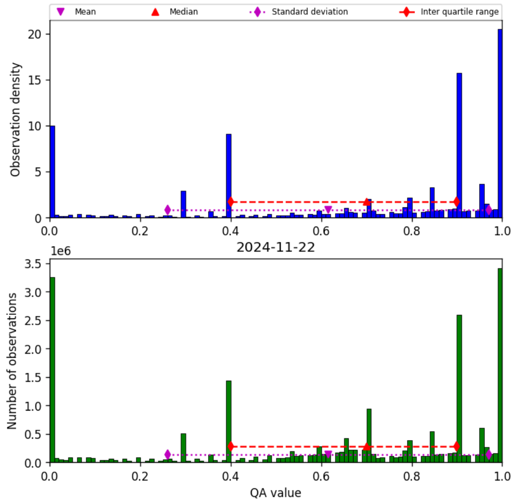
Figure 38: Histogram of “QA value” for 2024-11-21 to 2024-11-23
