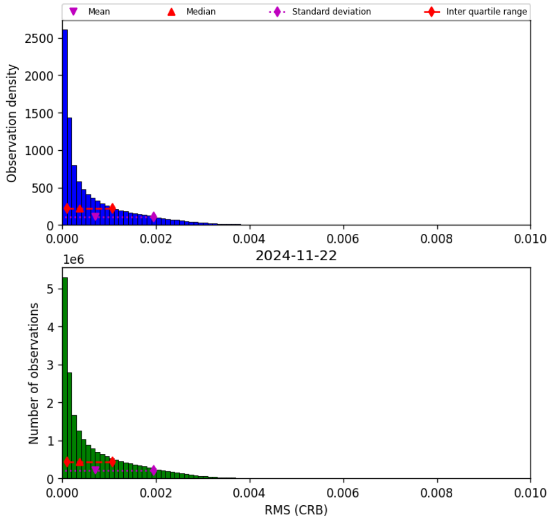
Figure 48: Histogram of “RMS (CRB)” for 2024-11-21 to 2024-11-23
