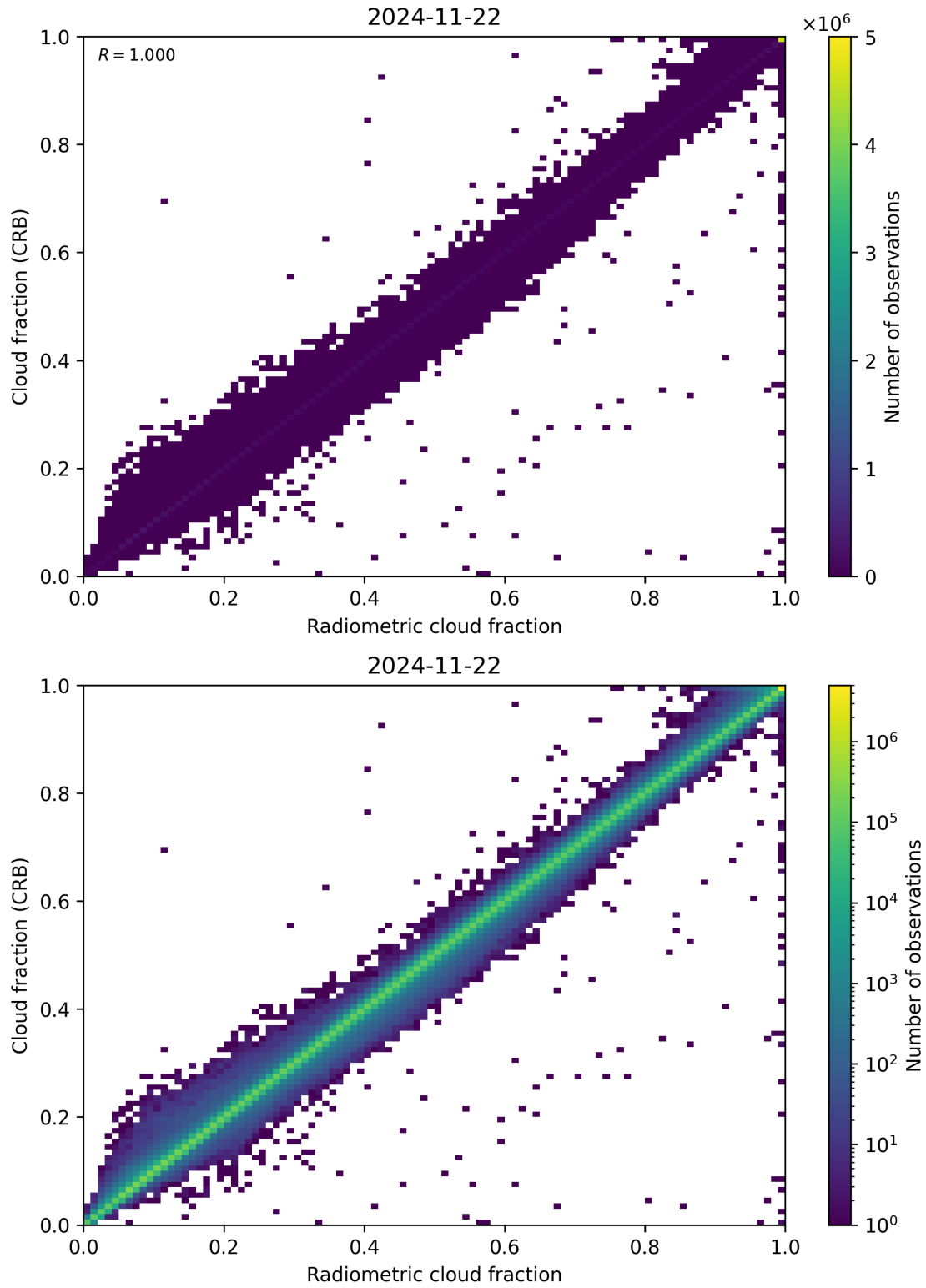
Figure 73: Scatter density plot of “Radiometric cloud fraction” against “Cloud fraction (CRB)” for 2024-11-21 to 2024-11-23.
