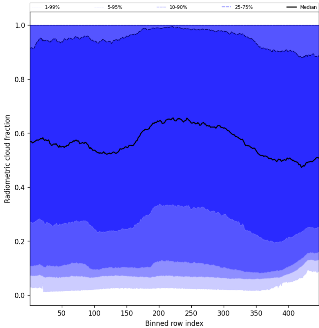
Figure 55: Along track statistics of “Radiometric cloud fraction” for 2024-11-21 to 2024-11-23
