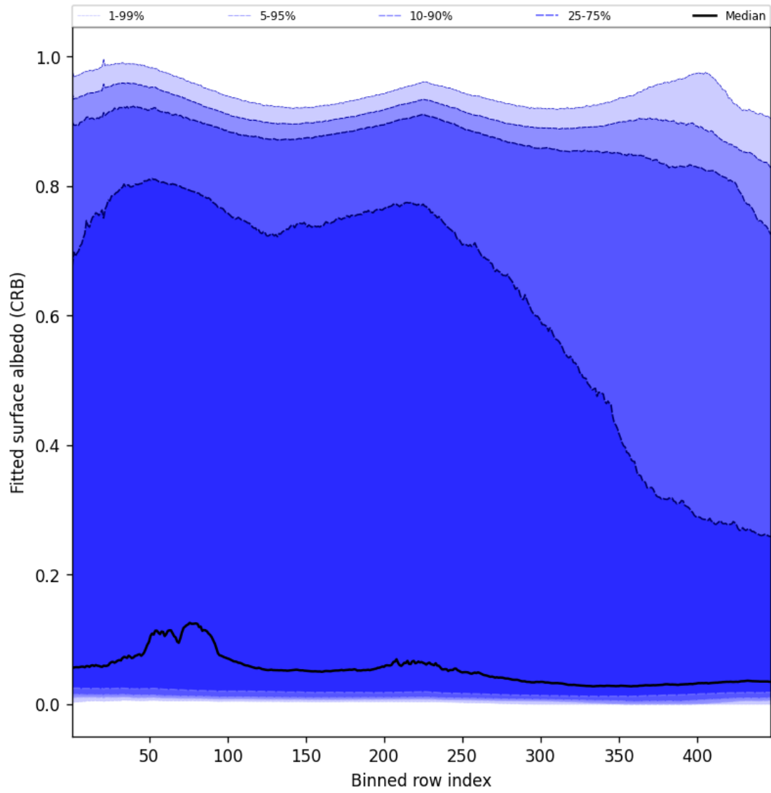
Figure 62: Along track statistics of “Fitted surface albedo (CRB)” for 2024-11-21 to 2024-11-23
