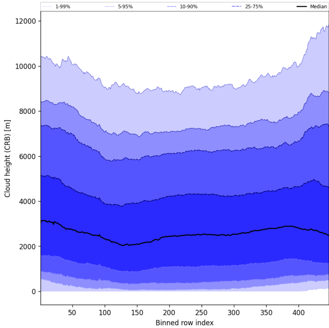
Figure 59: Along track statistics of “Cloud height (CRB)” for 2024-11-21 to 2024-11-23
