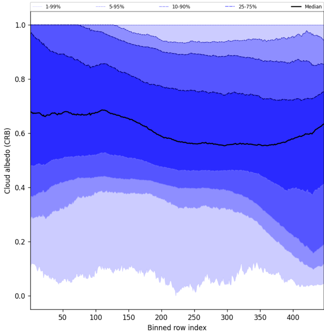
Figure 60: Along track statistics of “Cloud albedo (CRB)” for 2024-11-21 to 2024-11-23
