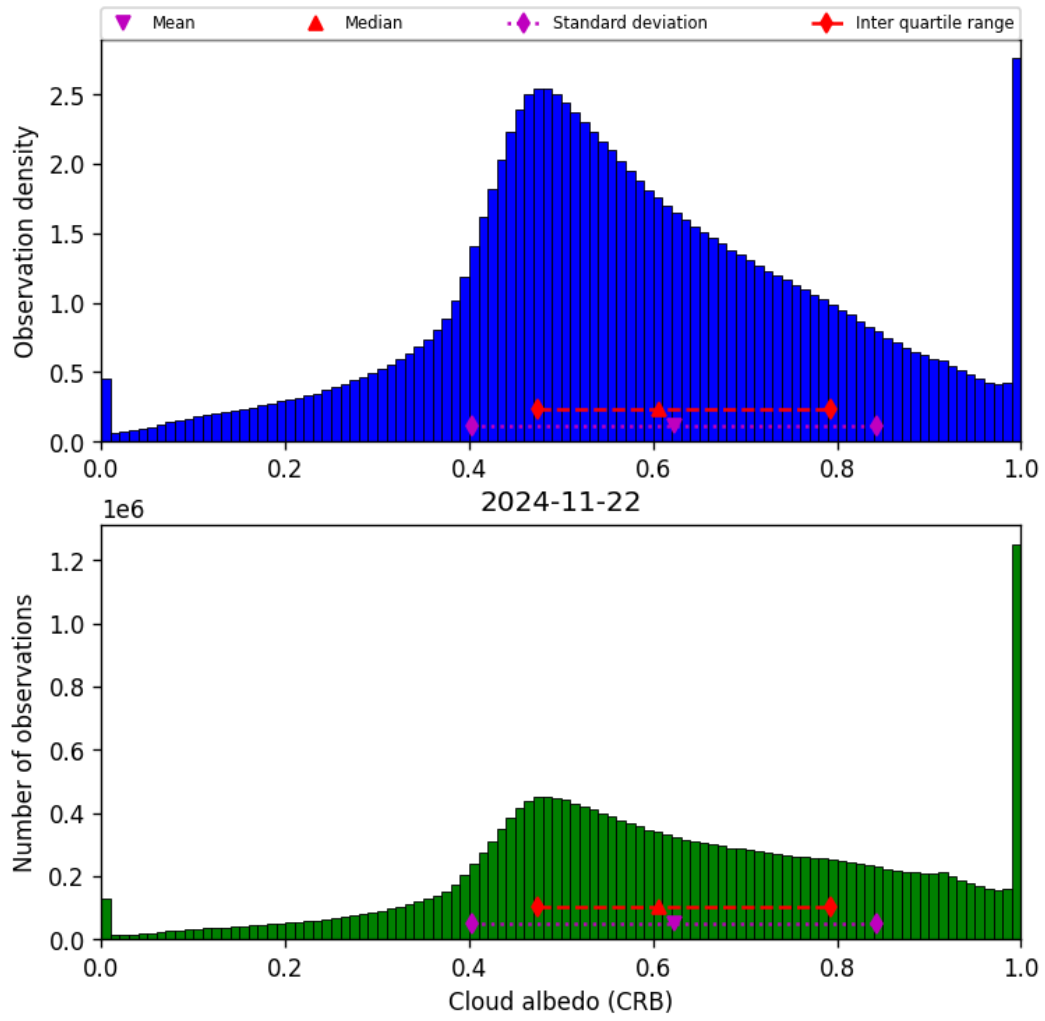
Figure 44: Histogram of “Cloud albedo (CRB)” for 2024-11-21 to 2024-11-23
