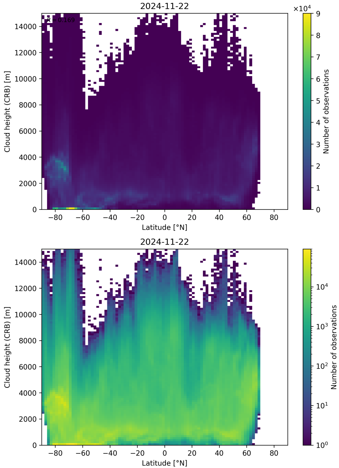
Figure 95: Scatter density plot of “Latitude” against “Cloud height (CRB)” for 2024-11-21 to 2024-11-23.
