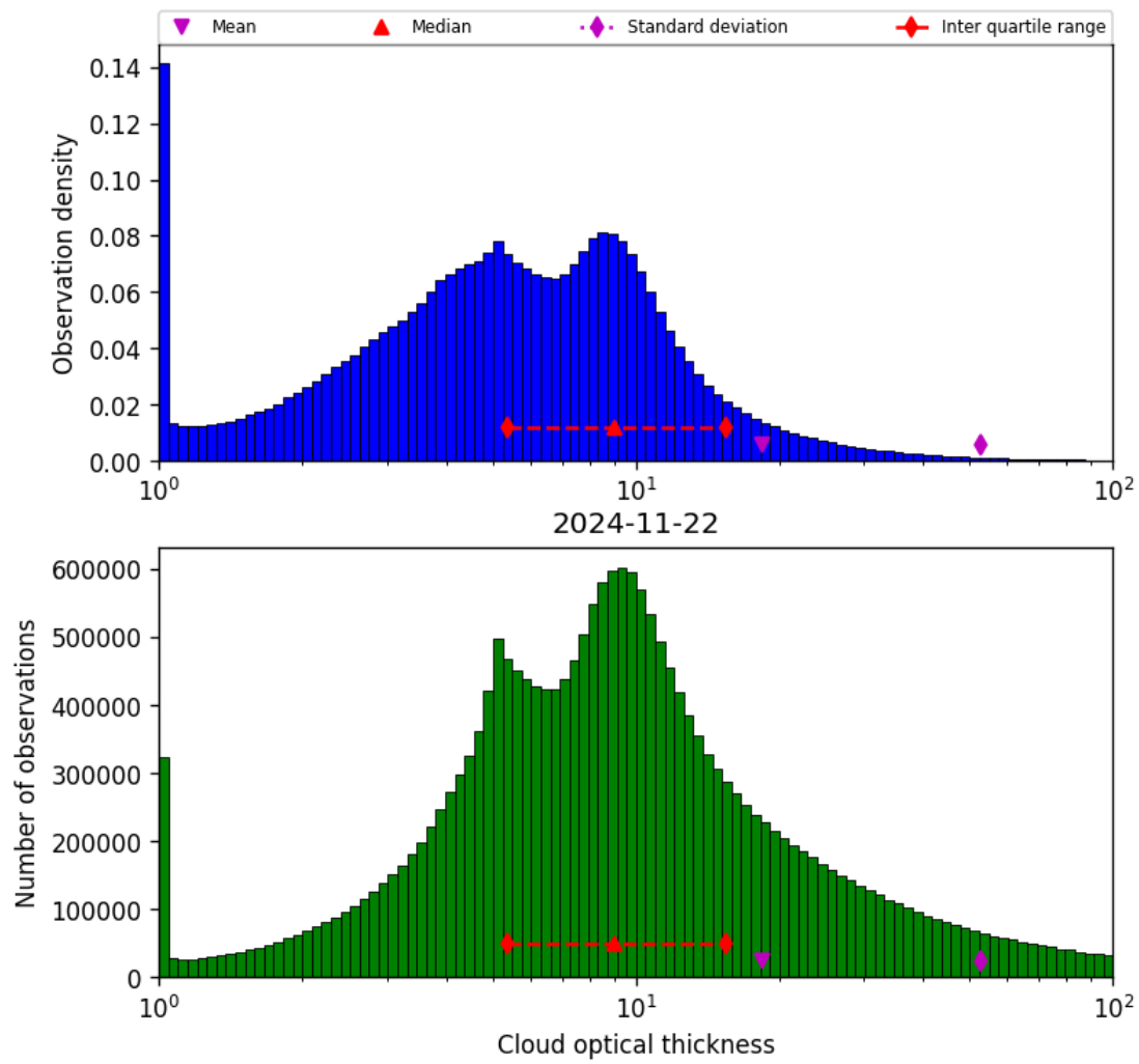
Figure 41: Histogram of “Cloud optical thickness” for 2024-11-21 to 2024-11-23
