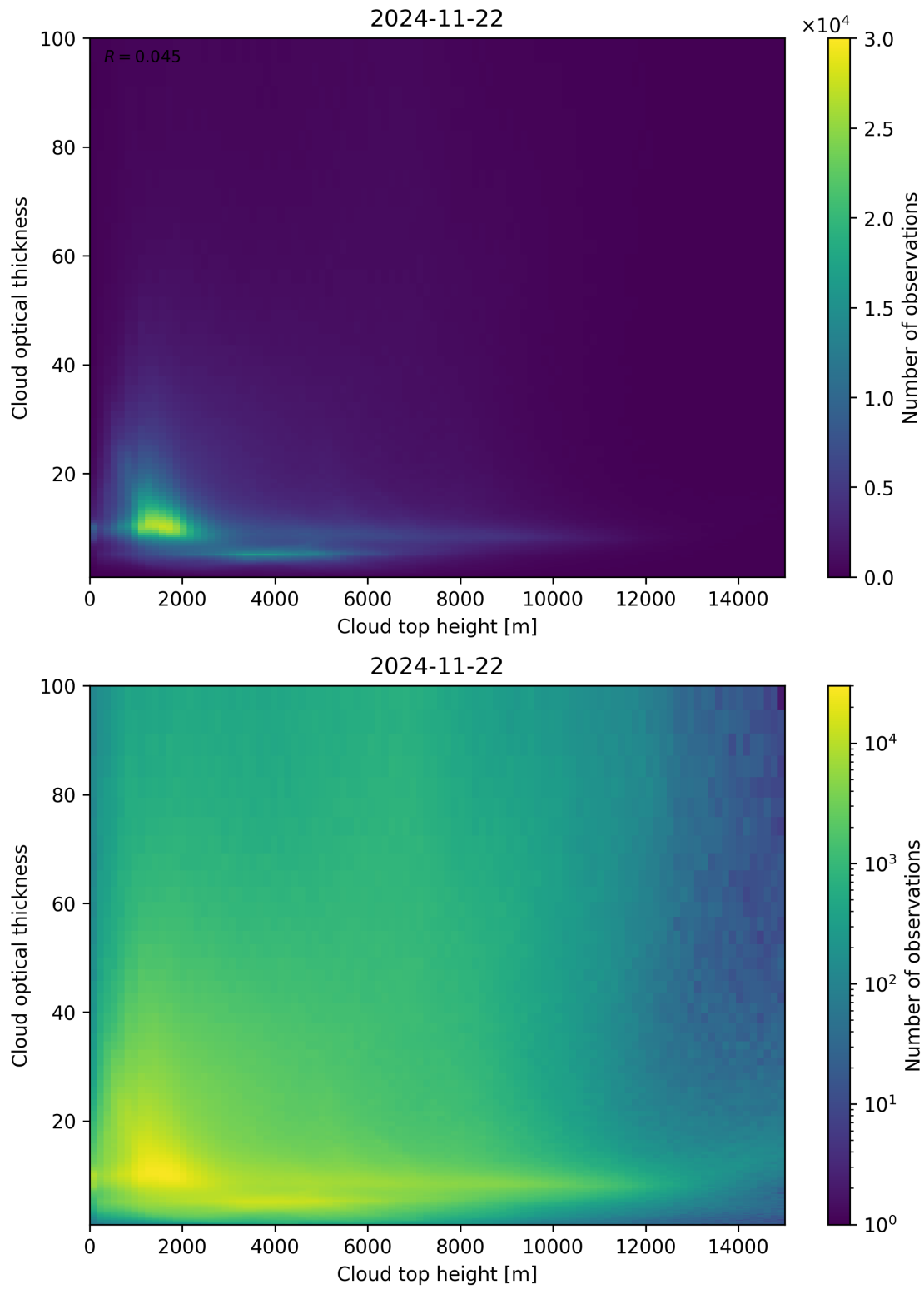
Figure 90: Scatter density plot of “Cloud top height” against “Cloud optical thickness” for 2024-11-21 to 2024-11-23.
