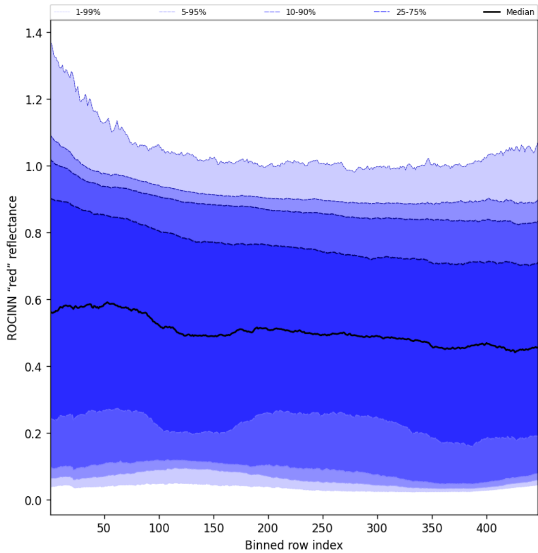
Figure 69: Along track statistics of “ROCINN “red” reflectance” for 2024-11-21 to 2024-11-23
