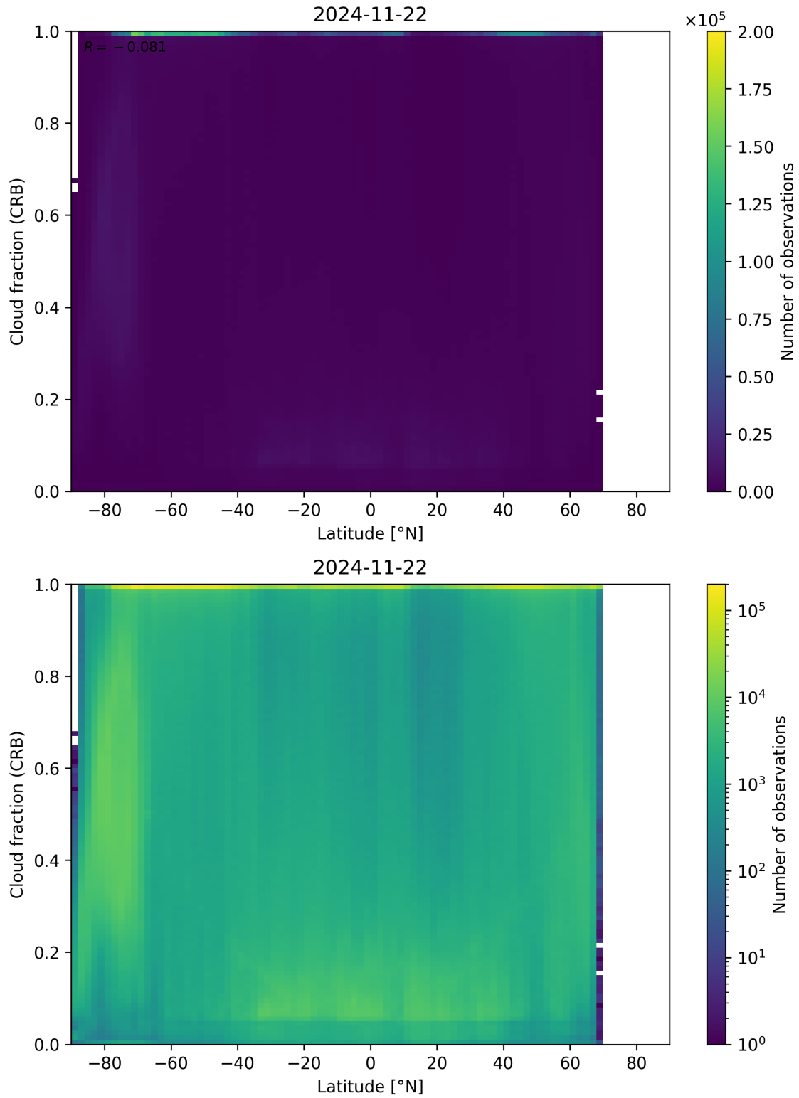
Figure 94: Scatter density plot of “Latitude” against “Cloud fraction (CRB)” for 2024-11-21 to 2024-11-23.
