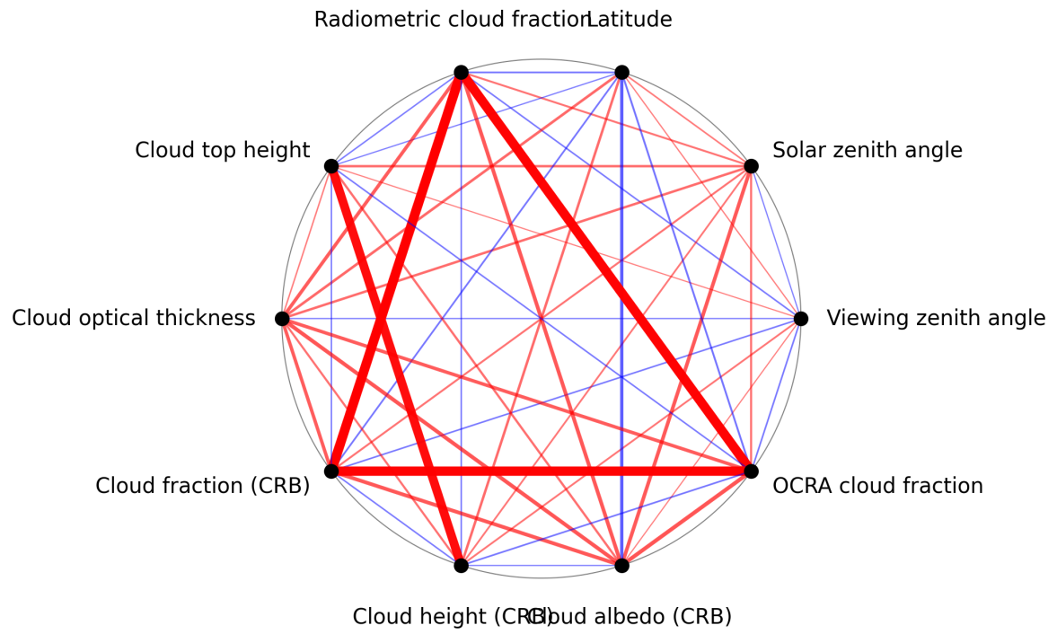
Figure 1: Map of correlation graph for 2024-11-21 to 2024-11-23.
