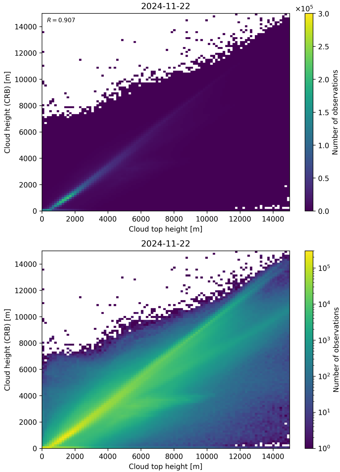
Figure 89: Scatter density plot of “Cloud top height” against “Cloud height (CRB)” for 2024-11-21 to 2024-11-23.
