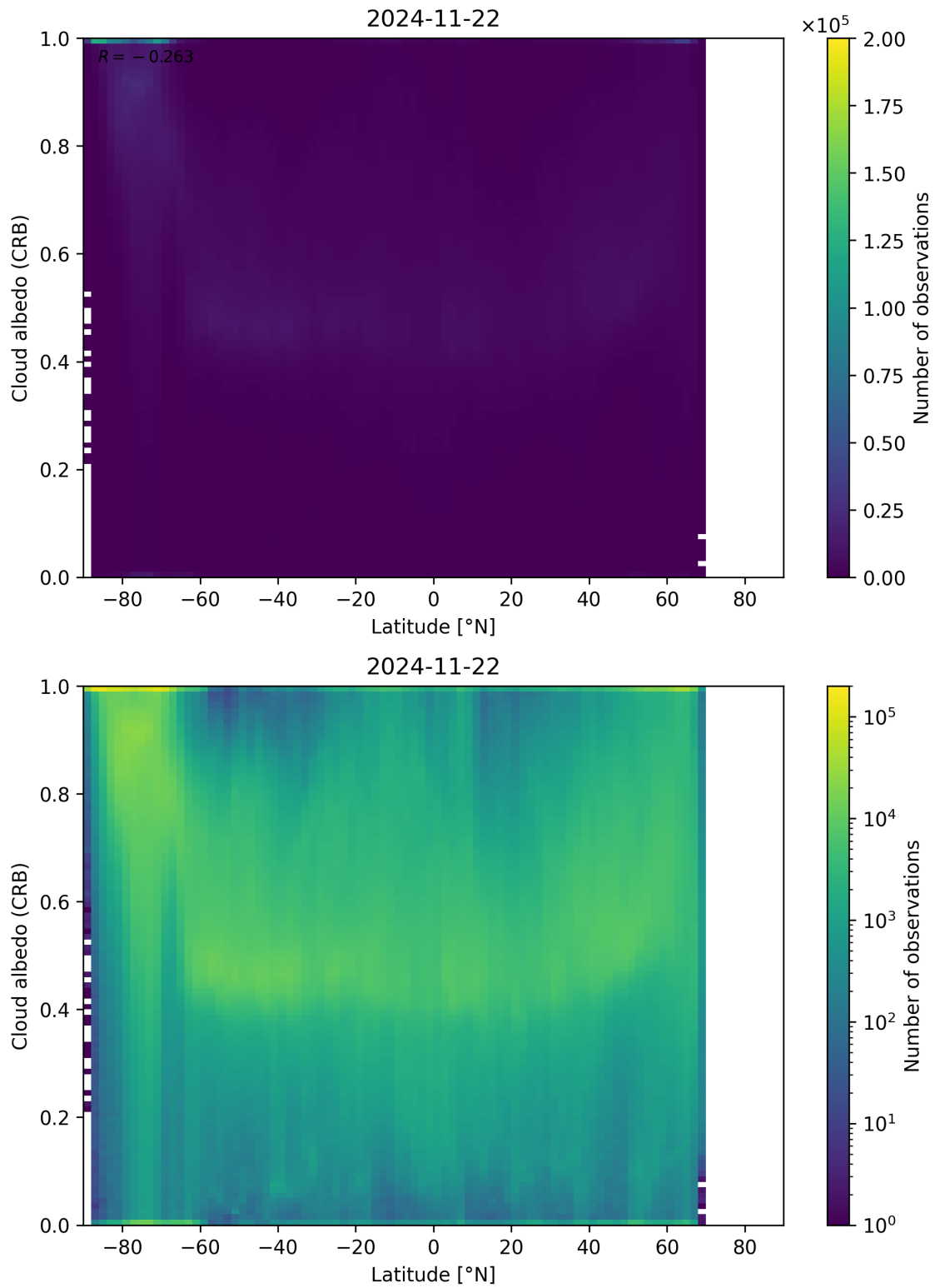
Figure 91: Scatter density plot of “Latitude” against “Cloud albedo (CRB)” for 2024-11-21 to 2024-11-23.
