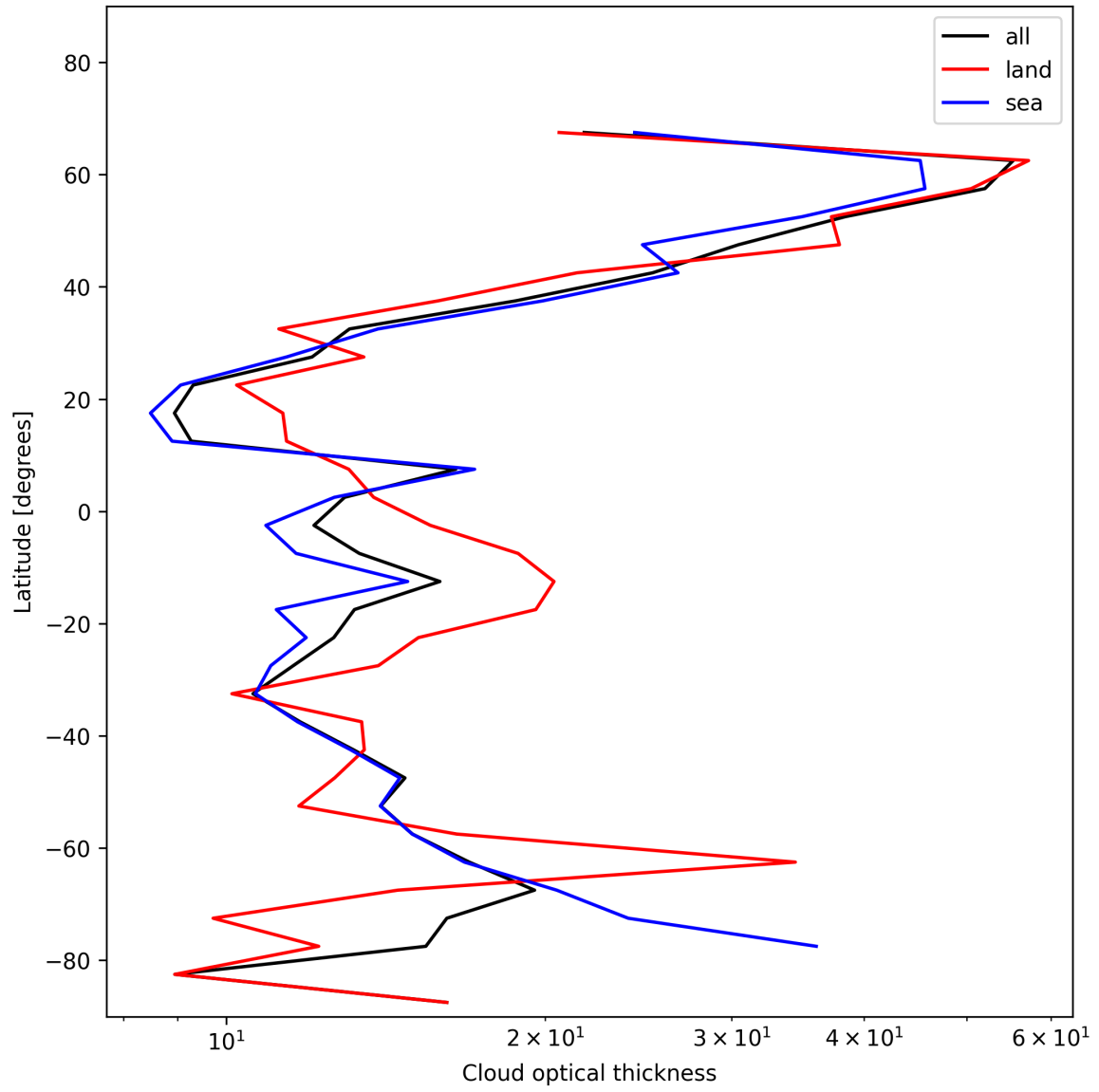
Figure 25: Zonal average of “Cloud optical thickness” for 2024-11-21 to 2024-11-23.
