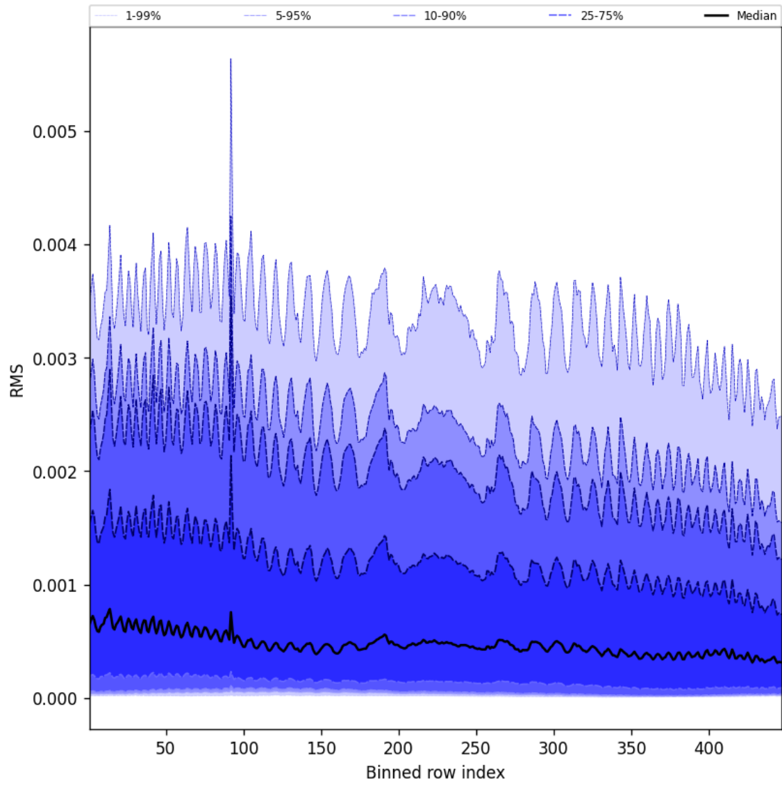
Figure 63: Along track statistics of “RMS” for 2024-11-21 to 2024-11-23
