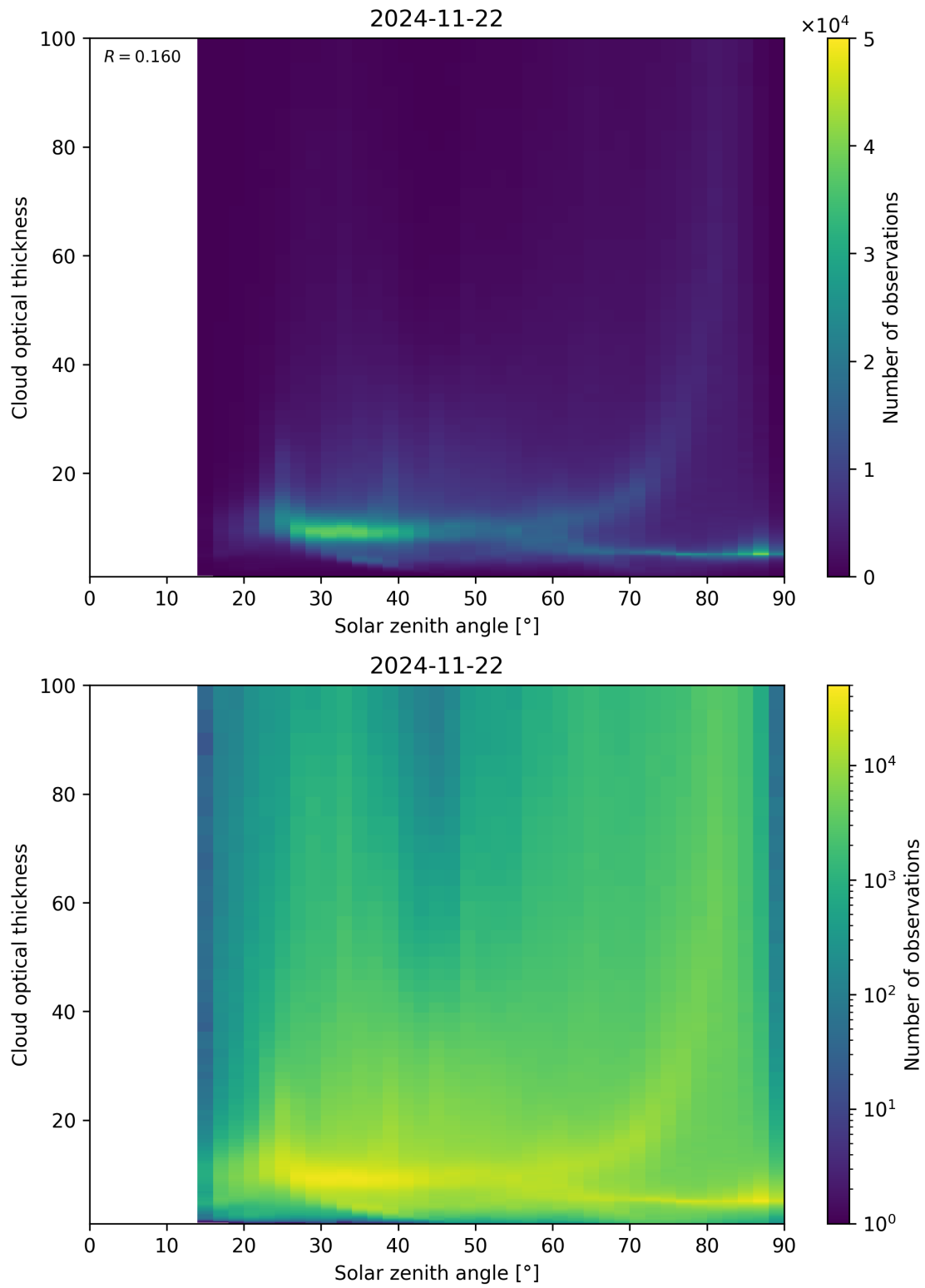
Figure 103: Scatter density plot of “Solar zenith angle” against “Cloud optical thickness” for 2024-11-21 to 2024-11-23.
