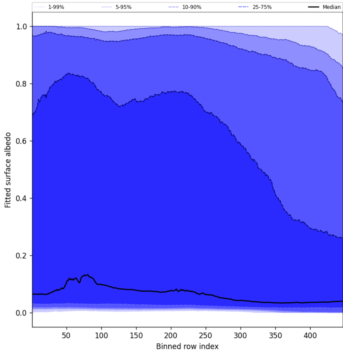
Figure 61: Along track statistics of “Fitted surface albedo” for 2024-11-21 to 2024-11-23
