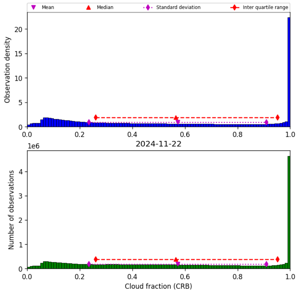
Figure 42: Histogram of “Cloud fraction (CRB)” for 2024-11-21 to 2024-11-23
