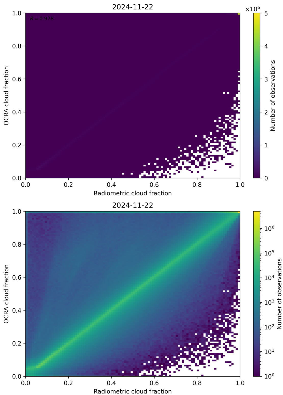
Figure 72: Scatter density plot of “Radiometric cloud fraction” against “OCRA cloud fraction” for 2024-11-21 to 2024-11-23.
