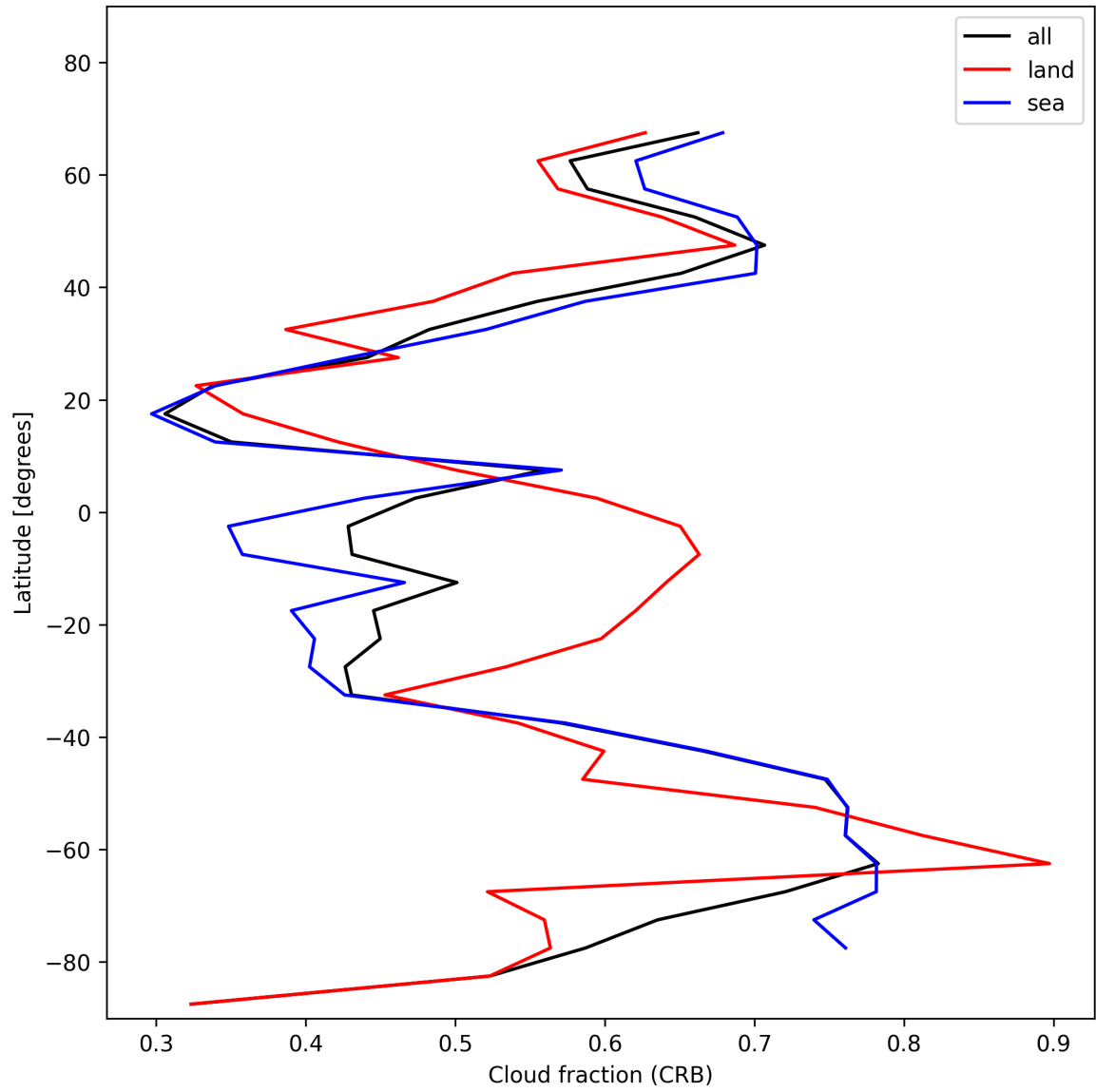
Figure 26: Zonal average of “Cloud fraction (CRB)” for 2024-11-21 to 2024-11-23.
