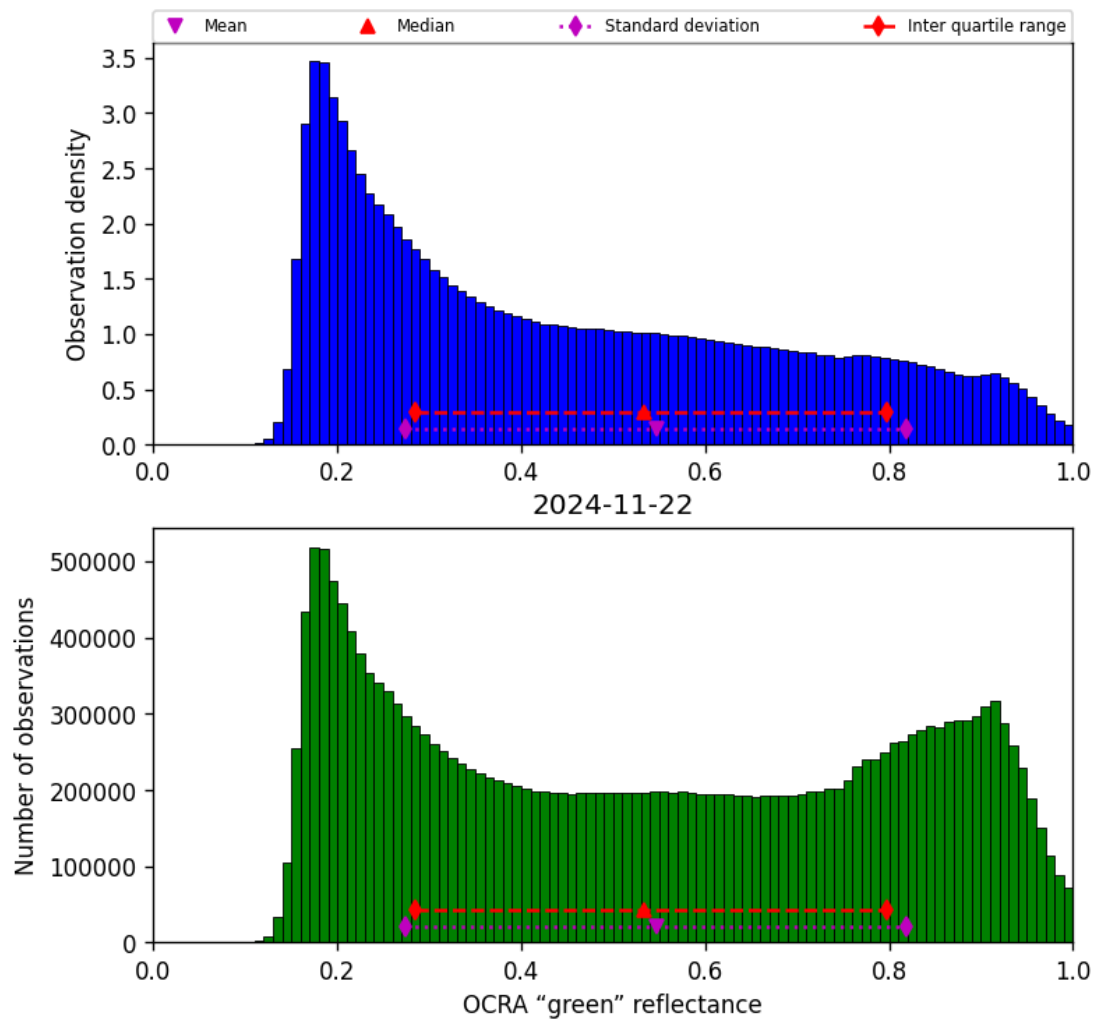
Figure 52: Histogram of “OCRA “green” reflectance” for 2024-11-21 to 2024-11-23
