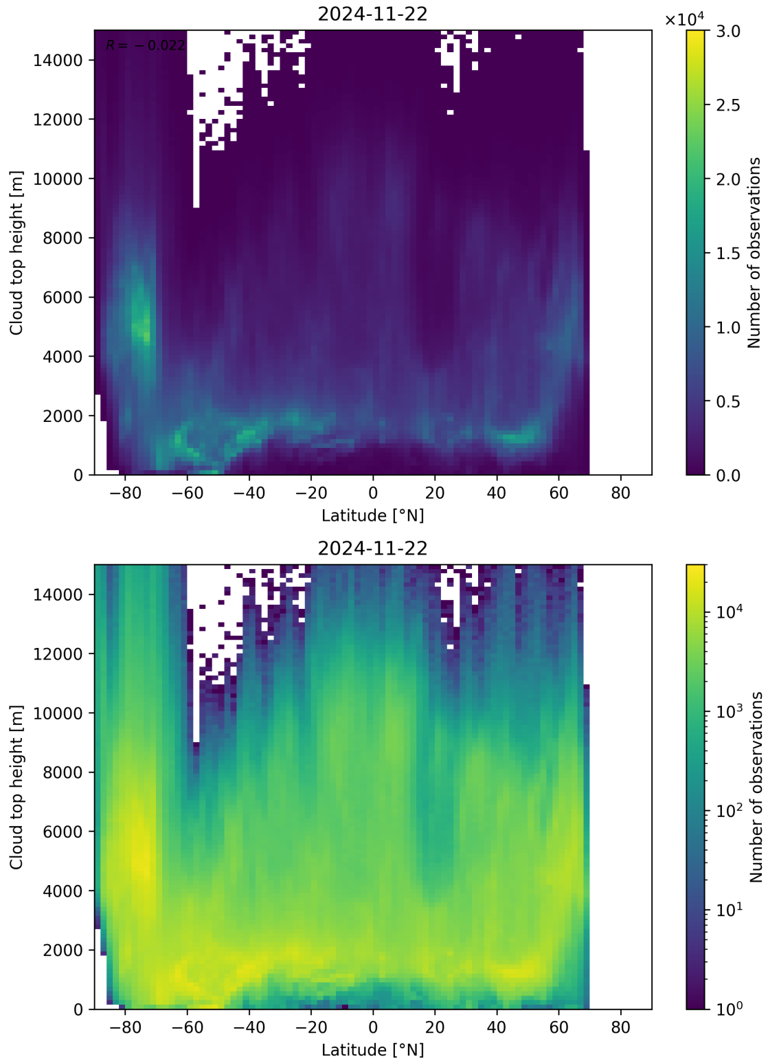
Figure 97: Scatter density plot of “Latitude” against “Cloud top height” for 2024-11-21 to 2024-11-23.
