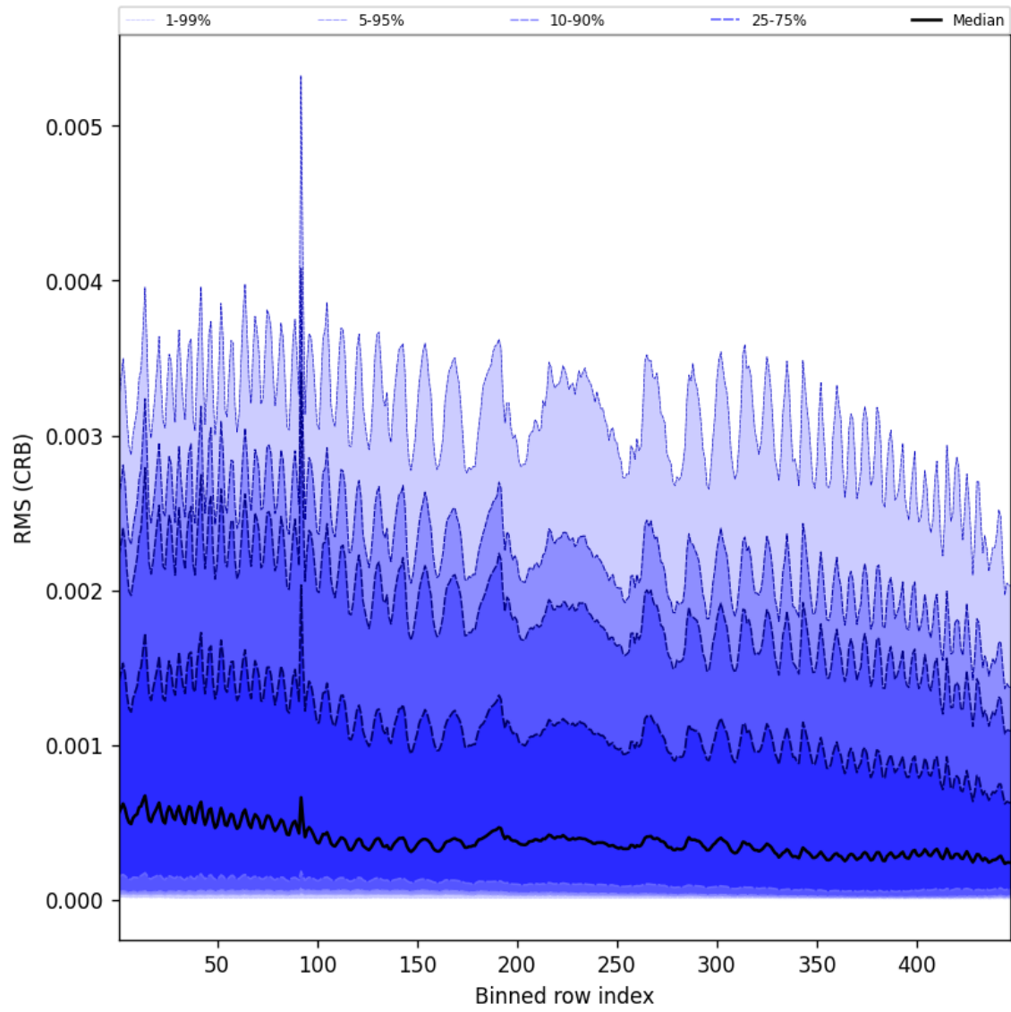
Figure 64: Along track statistics of “RMS (CRB)” for 2024-11-21 to 2024-11-23
