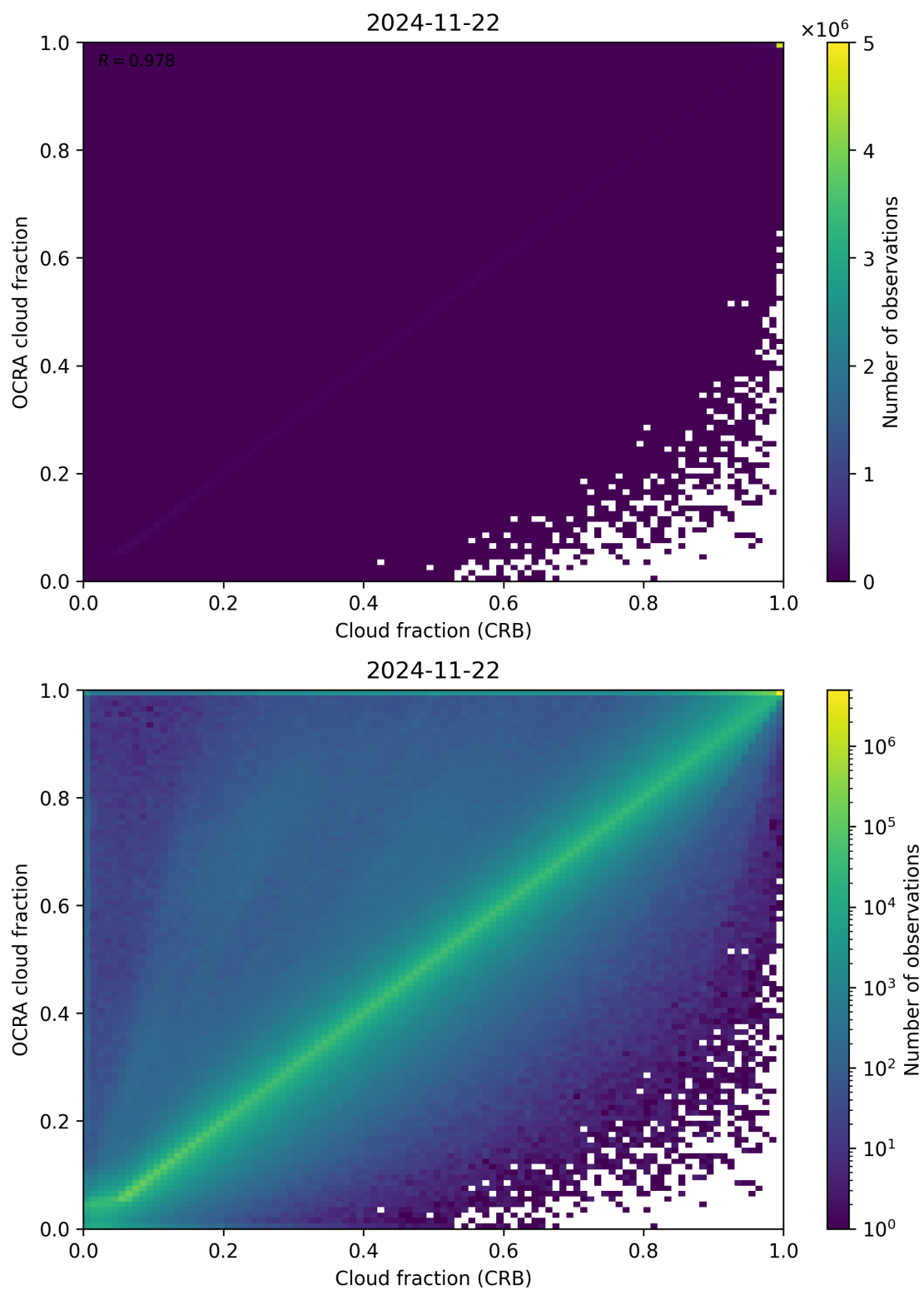
Figure 78: Scatter density plot of “Cloud fraction (CRB)” against “OCRA cloud fraction” for 2024-11-21 to 2024-11-23.
