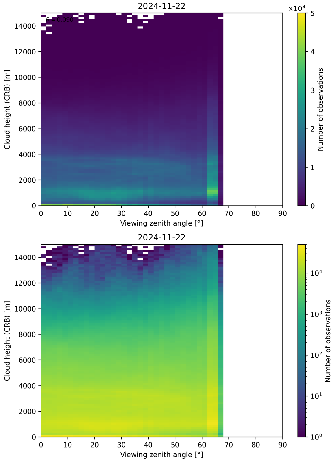
Figure 110: Scatter density plot of “Viewing zenith angle” against “Cloud height (CRB)” for 2024-11-21 to 2024-11-23.
