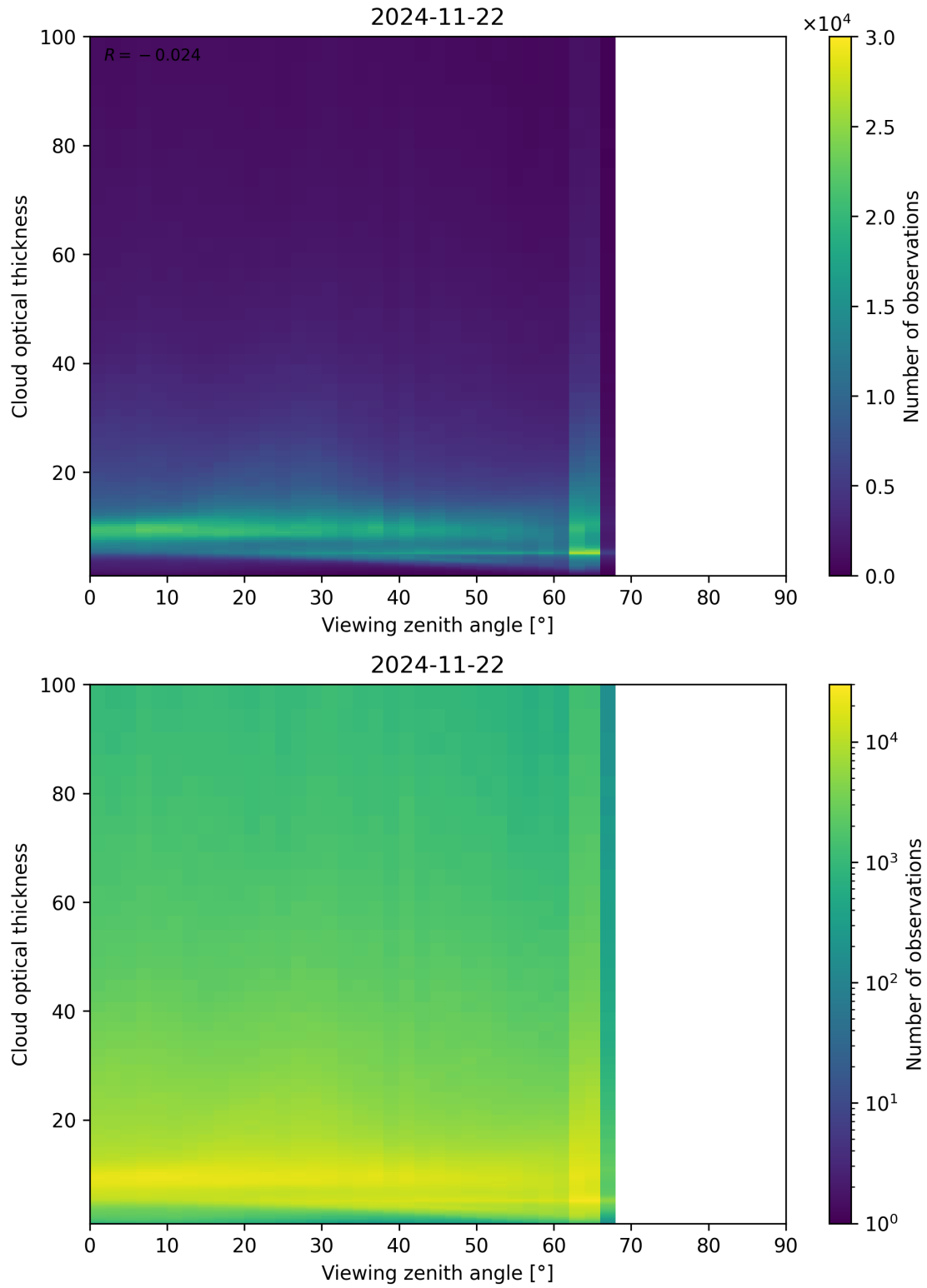
Figure 111: Scatter density plot of “Viewing zenith angle” against “Cloud optical thickness” for 2024-11-21 to 2024-11-23.
