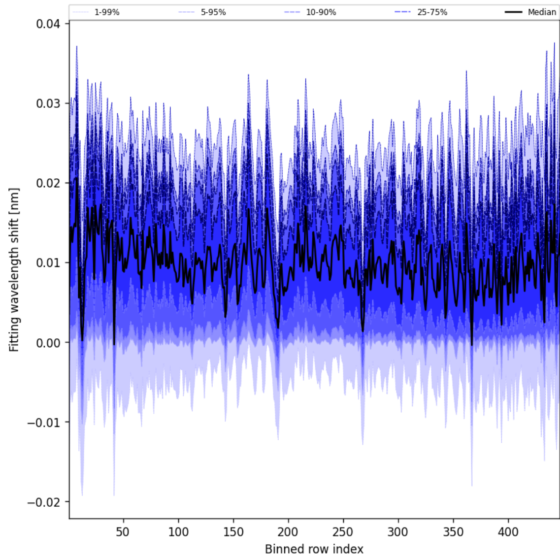
Figure 65: Along track statistics of “Fitting wavelength shift” for 2024-11-21 to 2024-11-23
