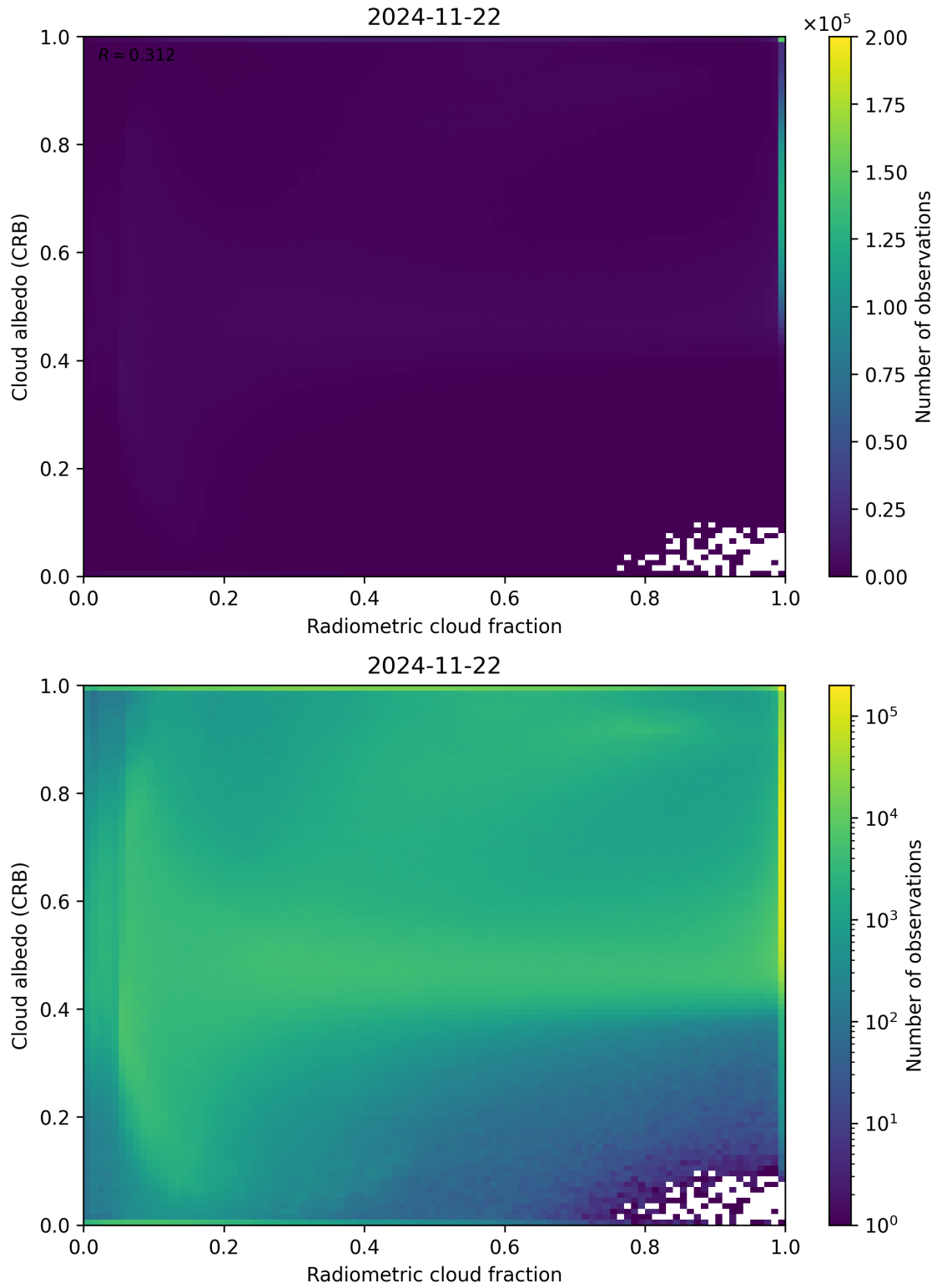
Figure 71: Scatter density plot of “Radiometric cloud fraction” against “Cloud albedo (CRB)” for 2024-11-21 to 2024-11-23.
