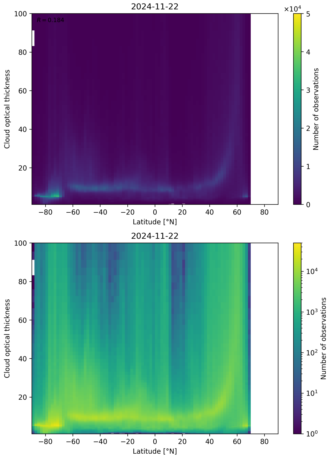
Figure 96: Scatter density plot of “Latitude” against “Cloud optical thickness” for 2024-11-21 to 2024-11-23.
