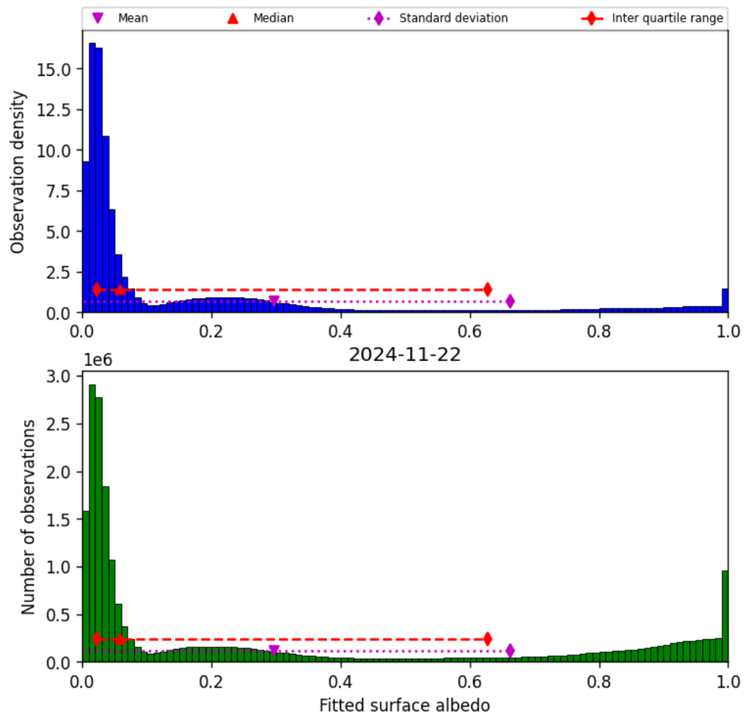
Figure 45: Histogram of “Fitted surface albedo” for 2024-11-21 to 2024-11-23
