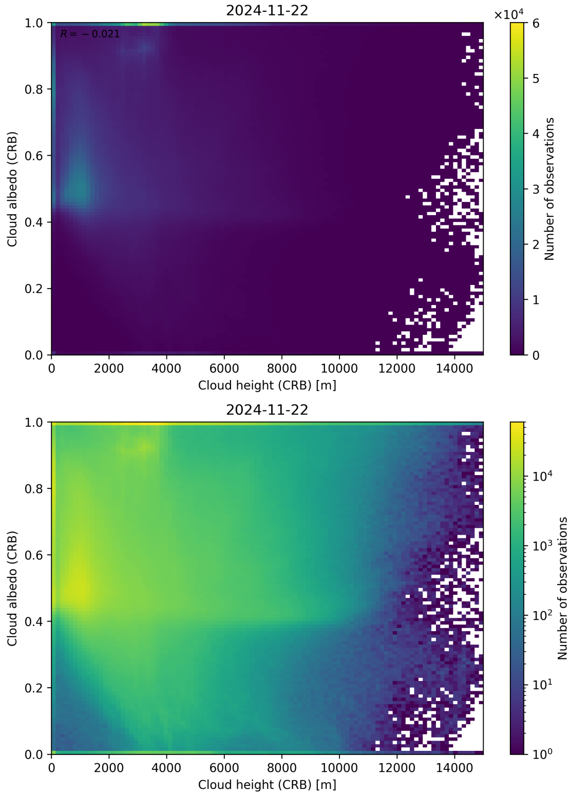
Figure 80: Scatter density plot of “Cloud height (CRB)” against “Cloud albedo (CRB)” for 2024-11-21 to 2024-11-23.
