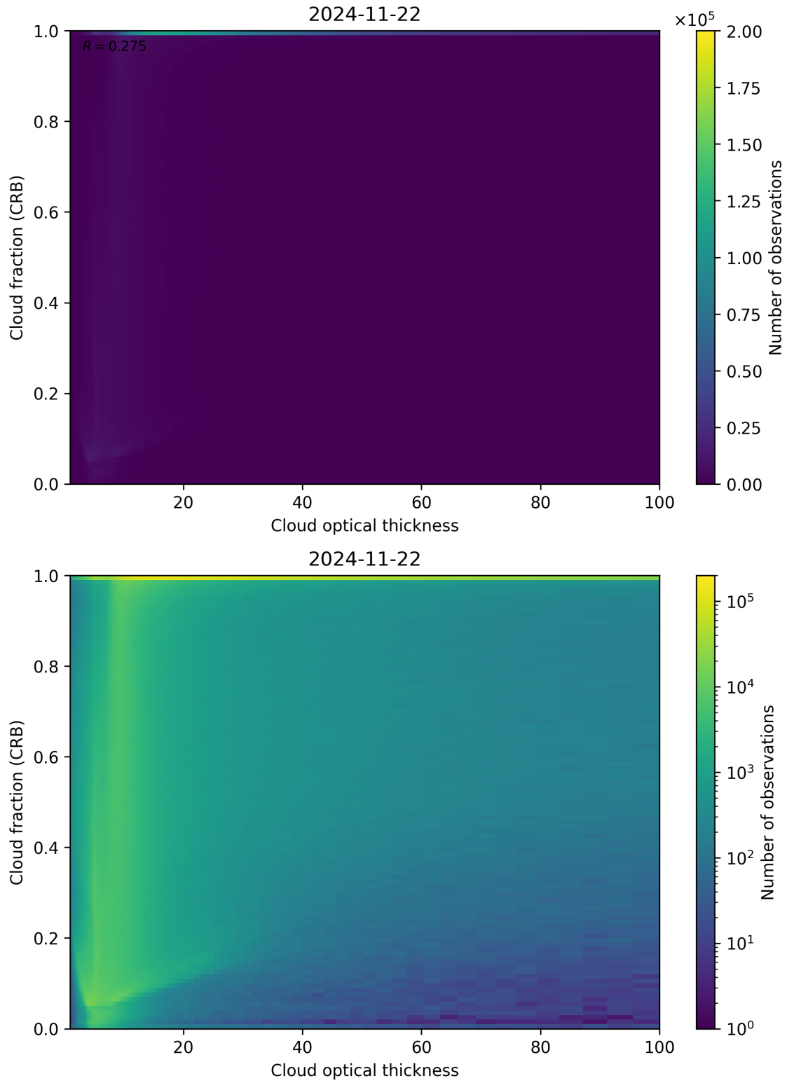
Figure 84: Scatter density plot of “Cloud optical thickness” against “Cloud fraction (CRB)” for 2024-11-21 to 2024-11-23.
