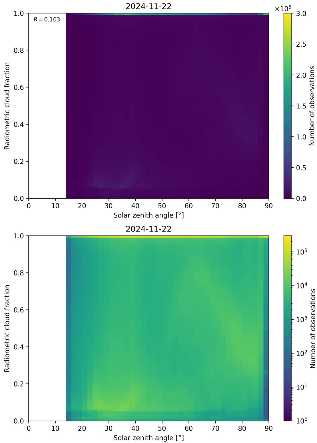
Figure 99: Scatter density plot of “Solar zenith angle” against “Radiometric cloud fraction” for 2024-11-21 to 2024-11-23.
