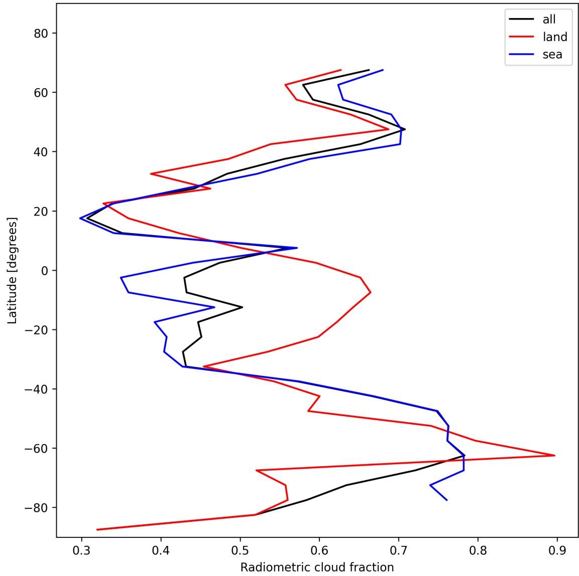
Figure 23: Zonal average of “Radiometric cloud fraction” for 2024-11-21 to 2024-11-23.
