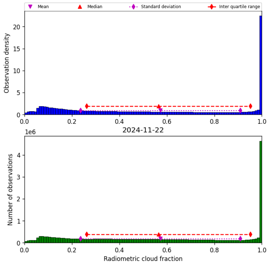
Figure 39: Histogram of “Radiometric cloud fraction” for 2024-11-21 to 2024-11-23
