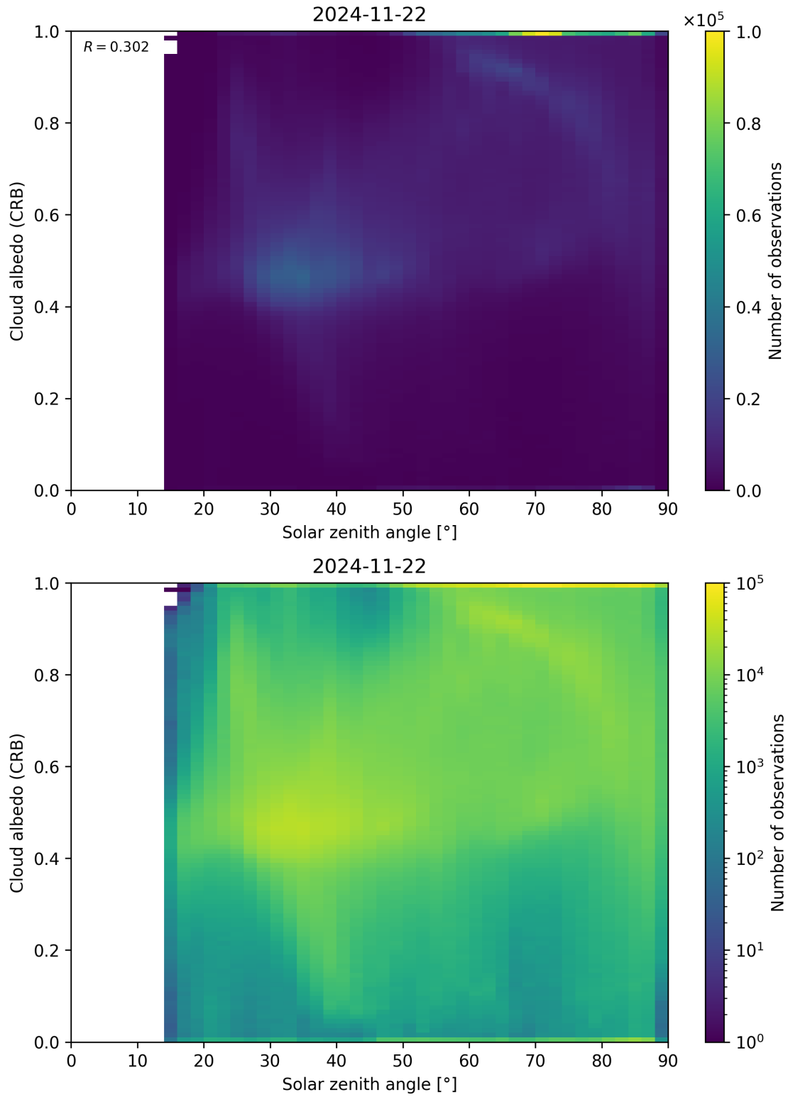
Figure 98: Scatter density plot of “Solar zenith angle” against “Cloud albedo (CRB)” for 2024-11-21 to 2024-11-23.
