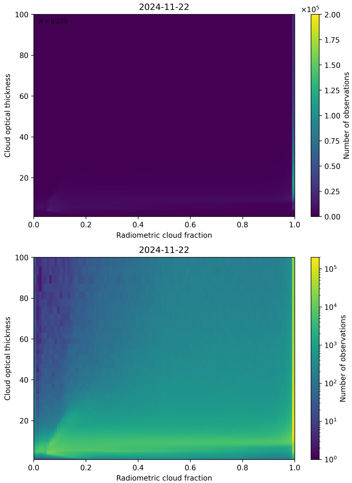
Figure 75: Scatter density plot of “Radiometric cloud fraction” against “Cloud optical thickness” for 2024-11-21 to 2024-11-23.
