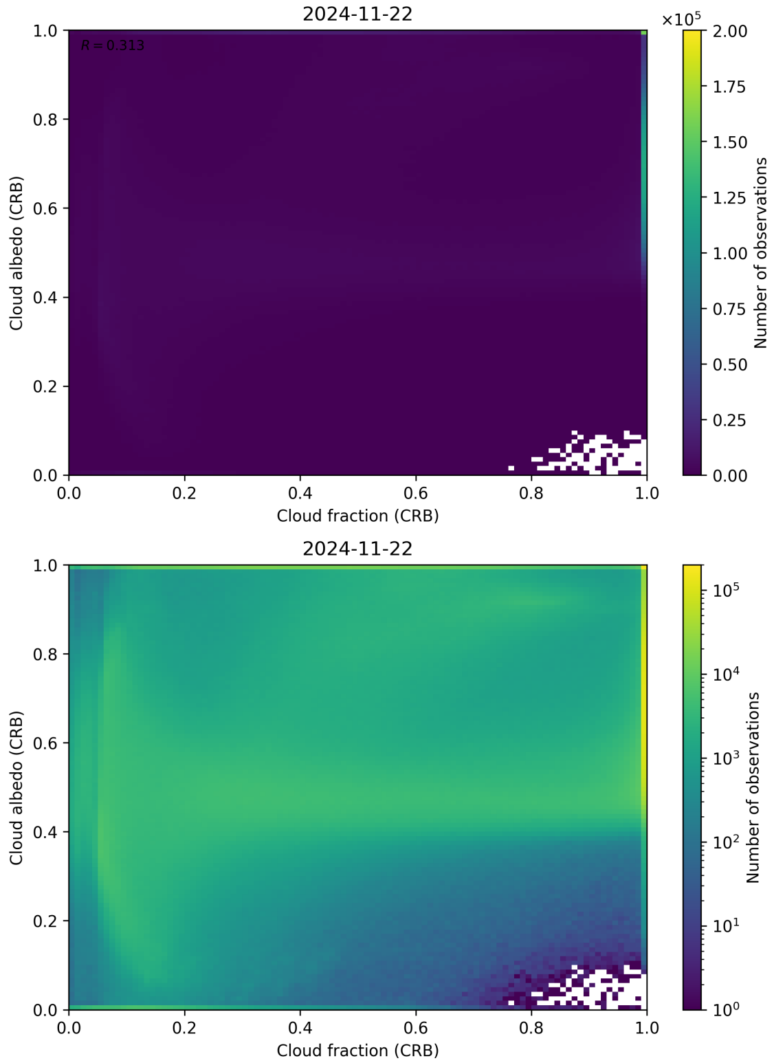
Figure 77: Scatter density plot of “Cloud fraction (CRB)” against “Cloud albedo (CRB)” for 2024-11-21 to 2024-11-23.
