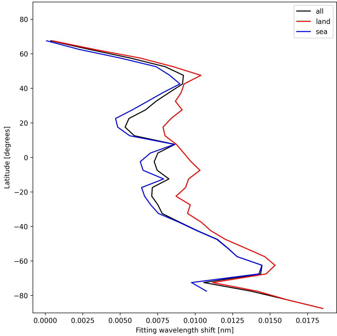
Figure 33: Zonal average of “Fitting wavelength shift” for 2024-11-21 to 2024-11-23.
