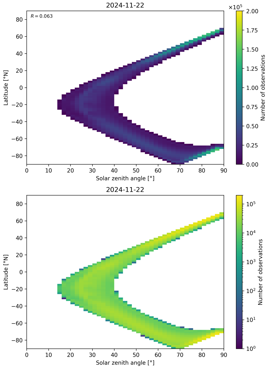
Figure 105: Scatter density plot of “Solar zenith angle” against “Latitude” for 2024-11-21 to 2024-11-23.
