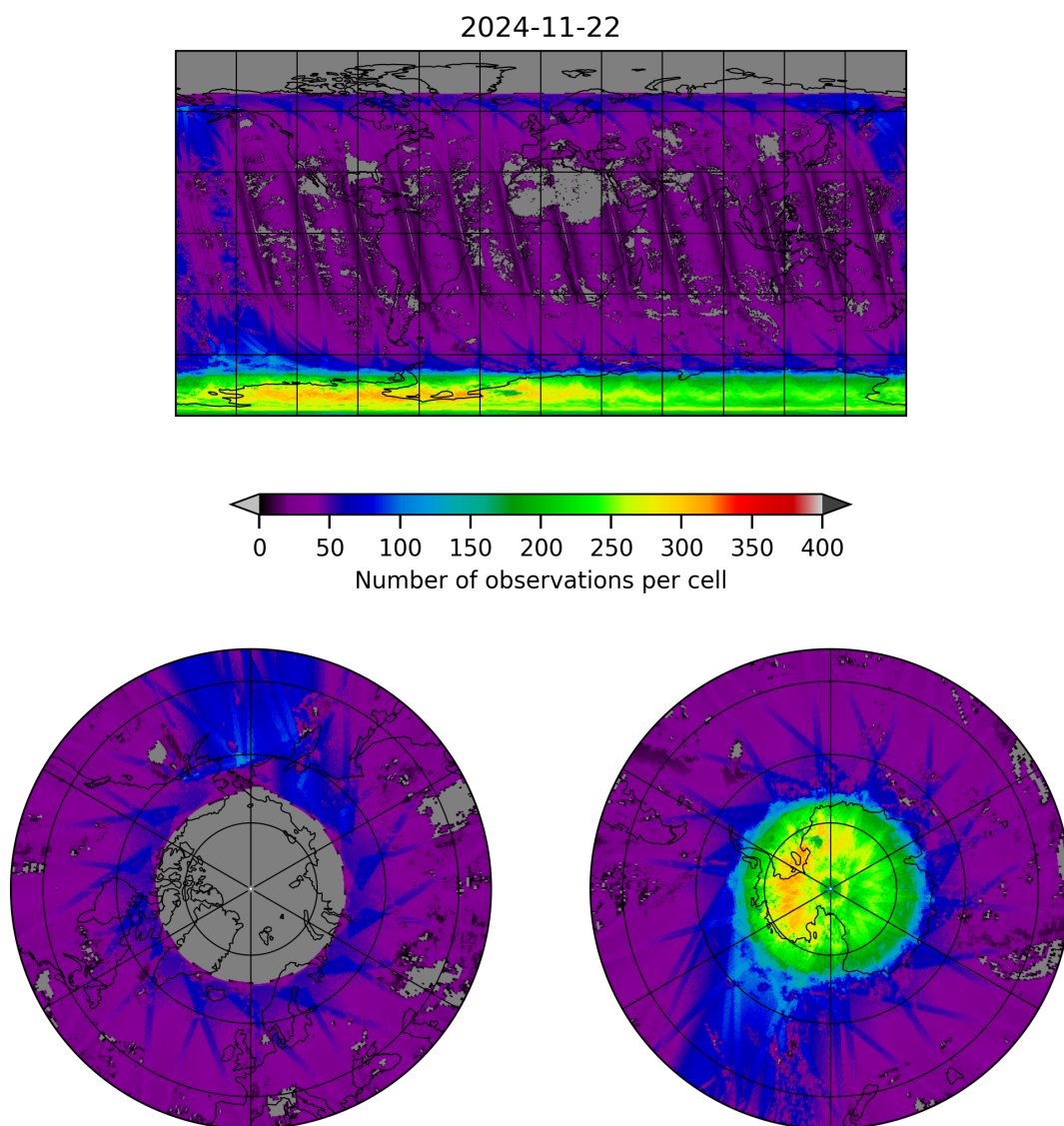
Figure 21: Map of the number of observations for 2024-11-21 to 2024-11-23
