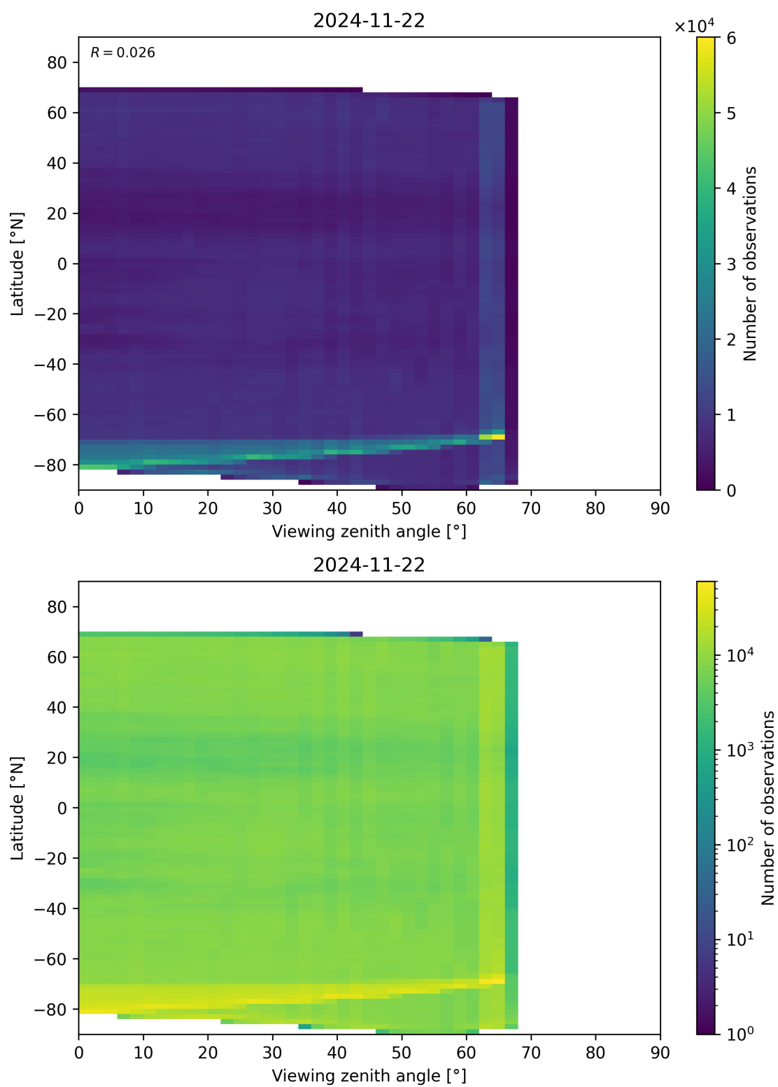
Figure 113: Scatter density plot of “Viewing zenith angle” against “Latitude” for 2024-11-21 to 2024-11-23.
