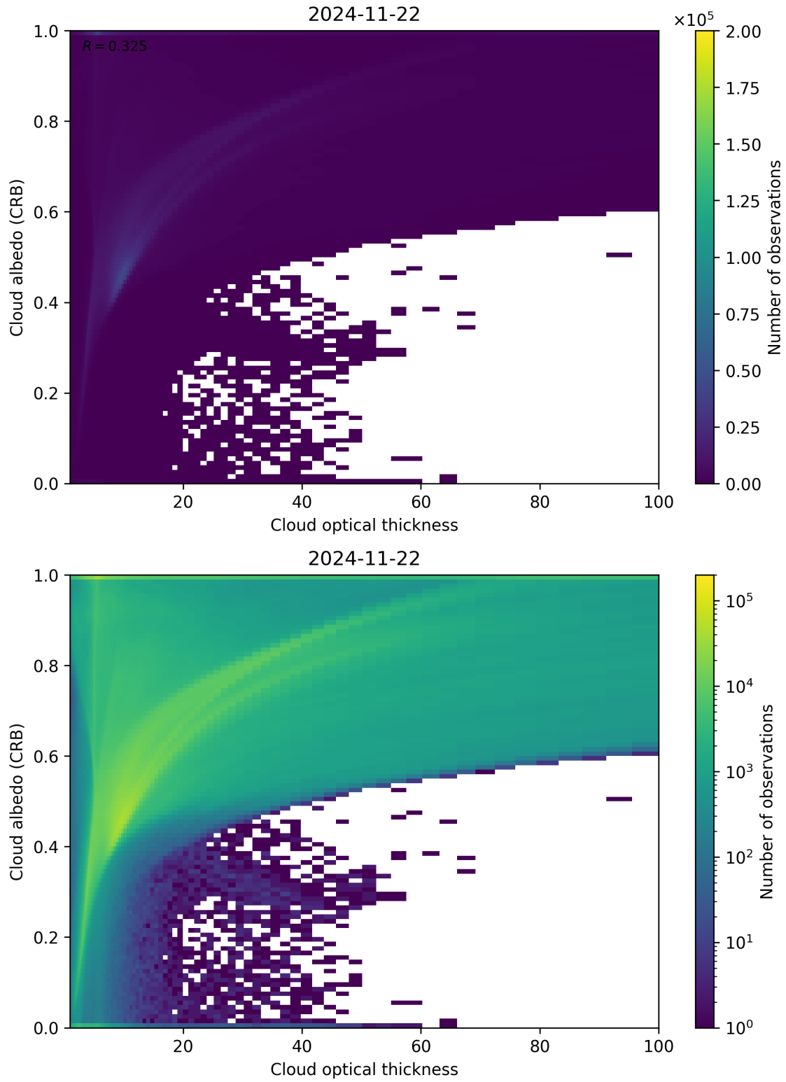
Figure 82: Scatter density plot of “Cloud optical thickness” against “Cloud albedo (CRB)” for 2024-11-21 to 2024-11-23.
