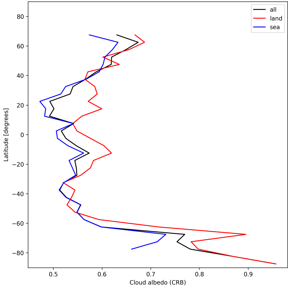
Figure 28: Zonal average of “Cloud albedo (CRB)” for 2024-11-21 to 2024-11-23.
