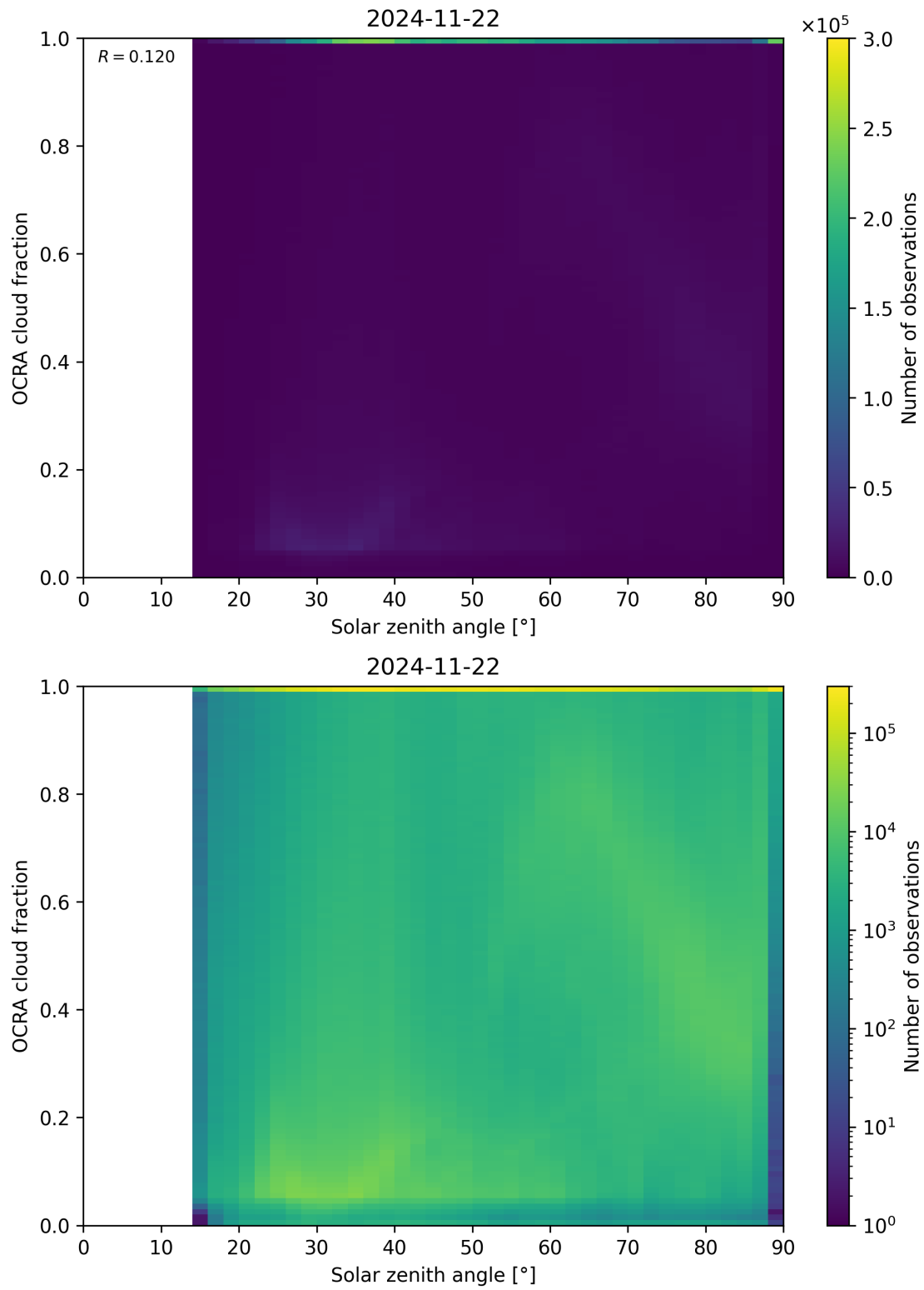
Figure 100: Scatter density plot of “Solar zenith angle” against “OCRA cloud fraction” for 2024-11-21 to 2024-11-23.
