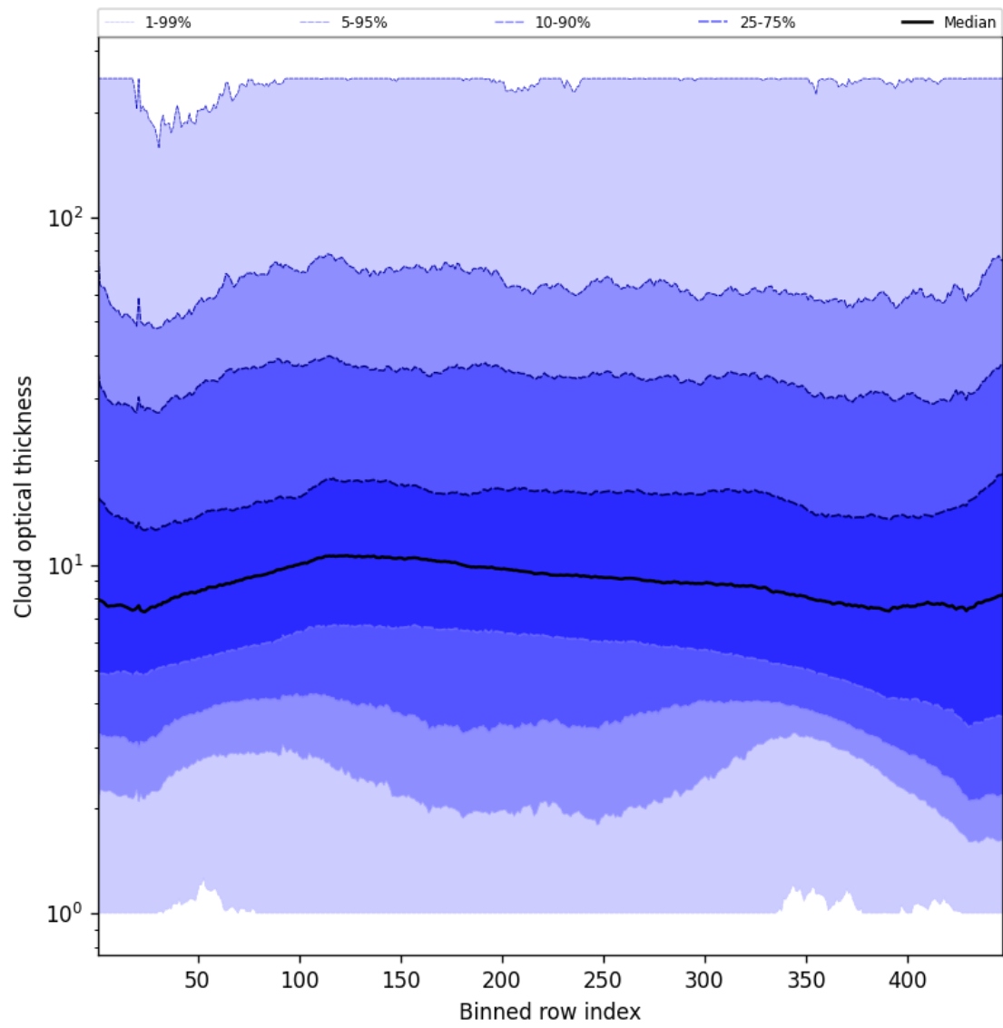
Figure 57: Along track statistics of “Cloud optical thickness” for 2024-11-21 to 2024-11-23
