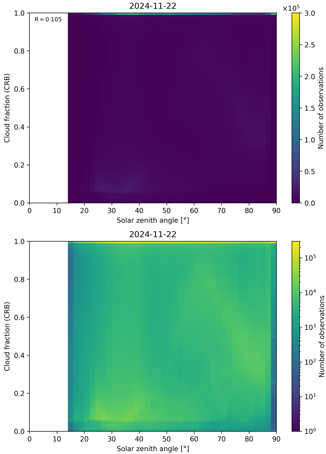
Figure 101: Scatter density plot of “Solar zenith angle” against “Cloud fraction (CRB)” for 2024-11-21 to 2024-11-23.
