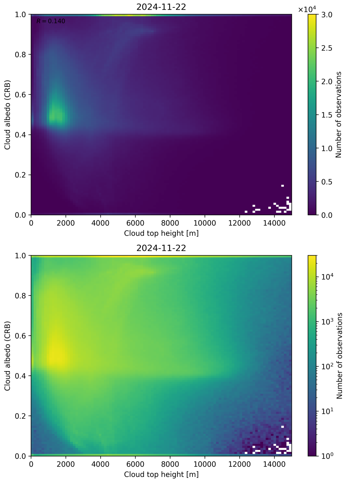
Figure 86: Scatter density plot of “Cloud top height” against “Cloud albedo (CRB)” for 2024-11-21 to 2024-11-23.
