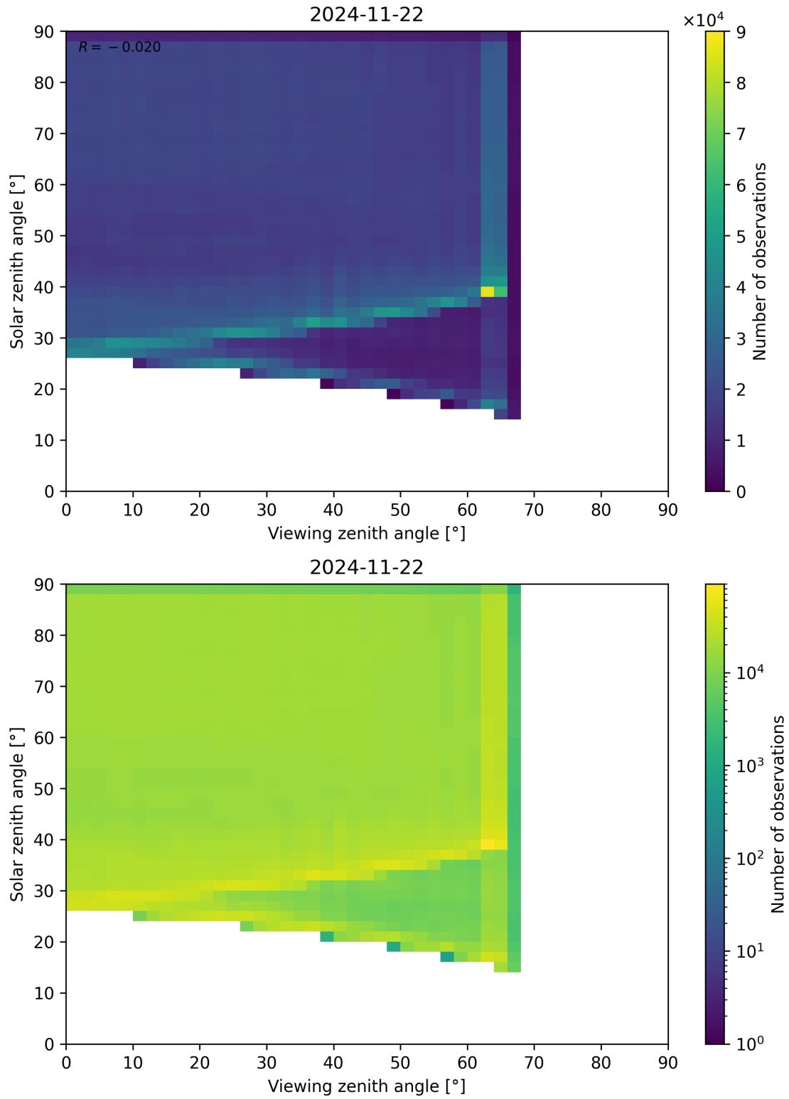
Figure 114: Scatter density plot of “Viewing zenith angle” against “Solar zenith angle” for 2024-11-21 to 2024-11-23.
