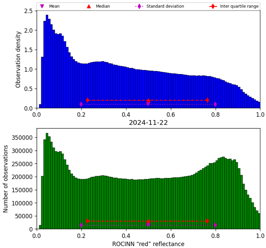
Figure 53: Histogram of “ROCINN “red” reflectance” for 2024-11-21 to 2024-11-23
