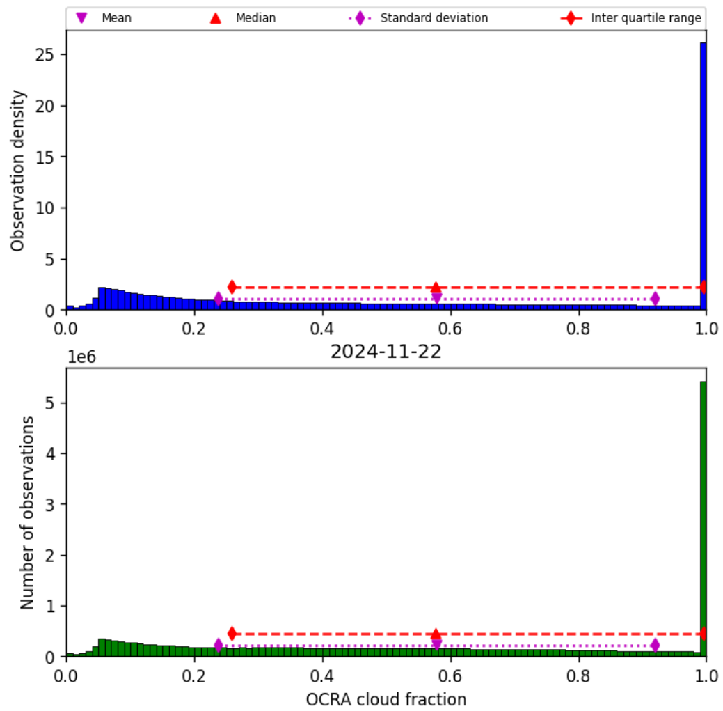
Figure 50: Histogram of “OCRA cloud fraction” for 2024-11-21 to 2024-11-23
