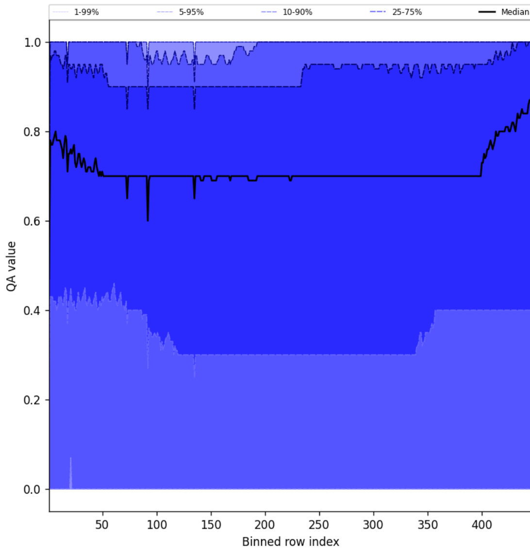
Figure 54: Along track statistics of “QA value” for 2024-11-21 to 2024-11-23
