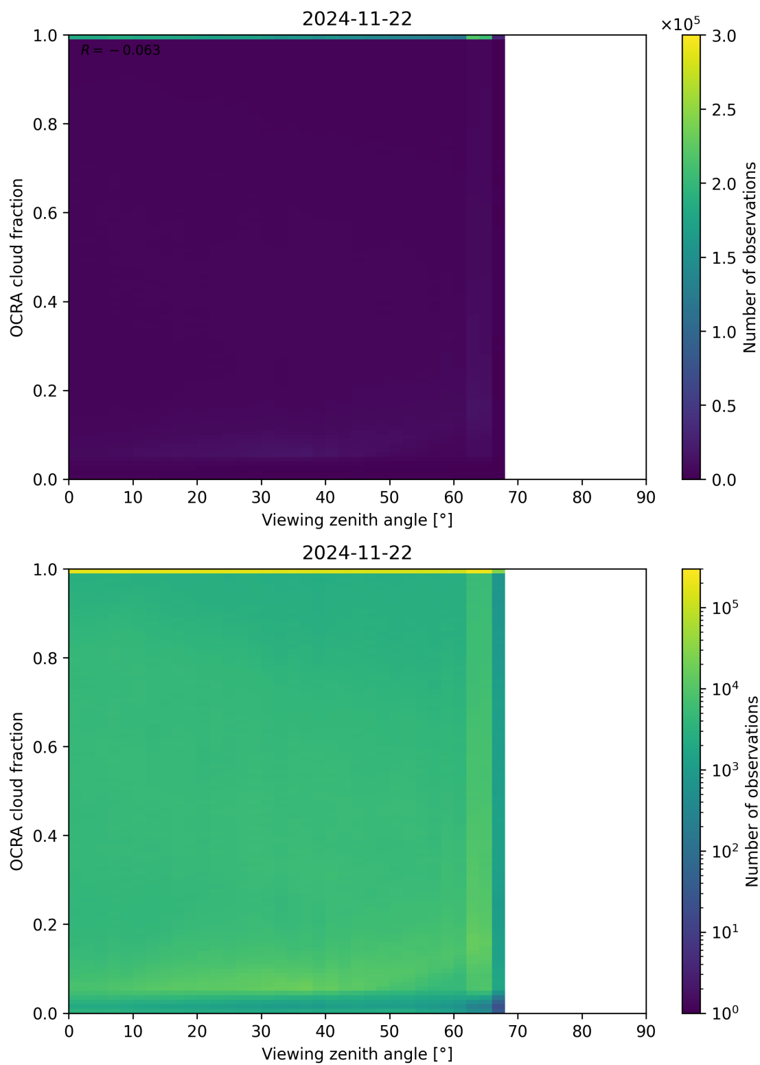
Figure 108: Scatter density plot of “Viewing zenith angle” against “OCRA cloud fraction” for 2024-11-21 to 2024-11-23.
