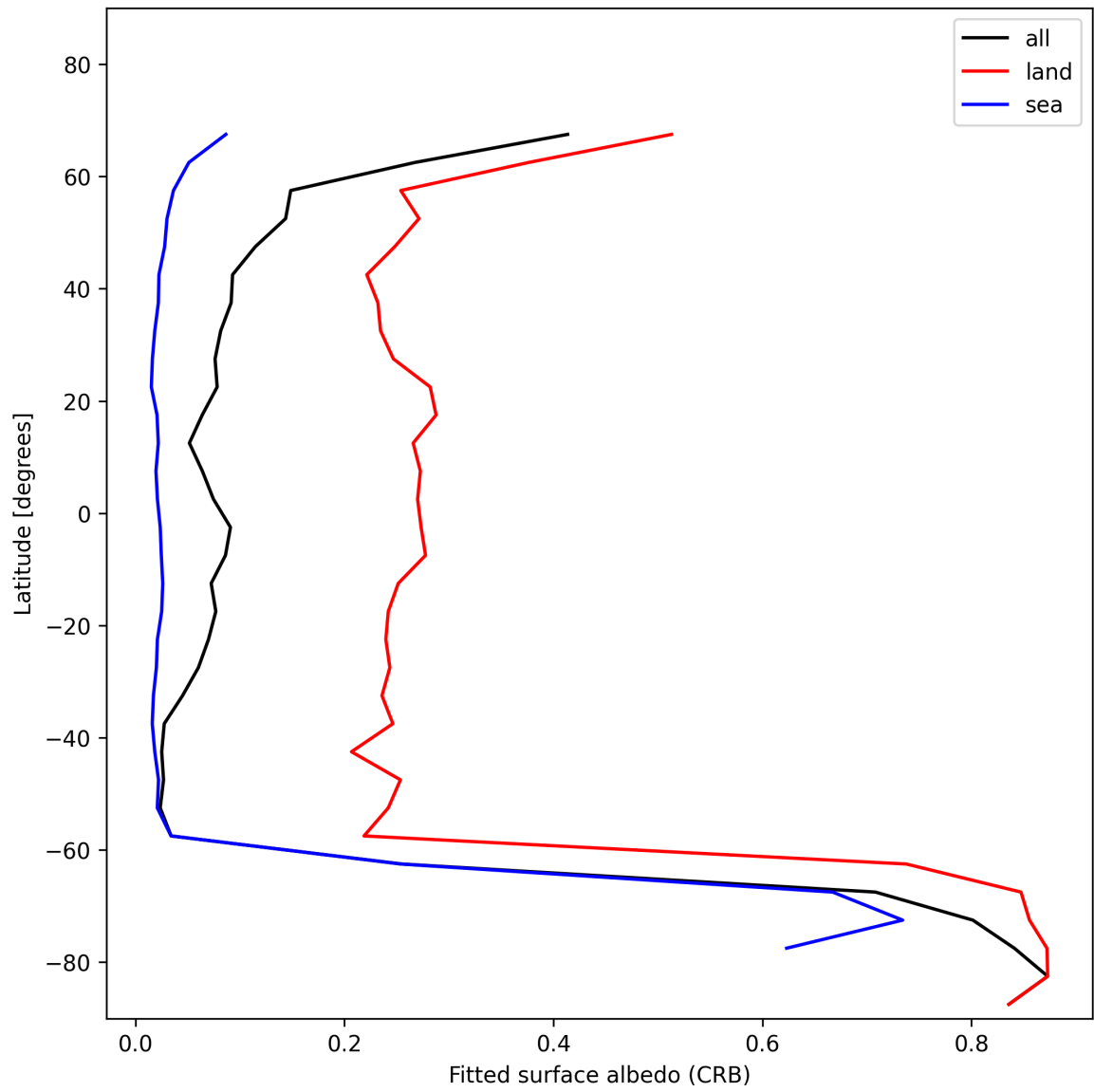
Figure 30: Zonal average of “Fitted surface albedo (CRB)” for 2024-11-21 to 2024-11-23.
