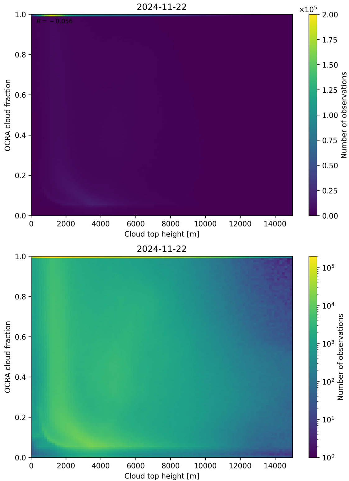
Figure 87: Scatter density plot of “Cloud top height” against “OCRA cloud fraction” for 2024-11-21 to 2024-11-23.
