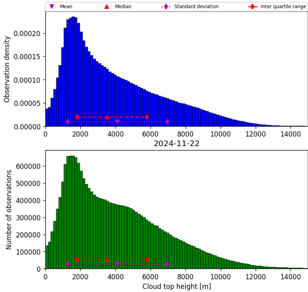
Figure 40: Histogram of “Cloud top height” for 2024-11-21 to 2024-11-23
