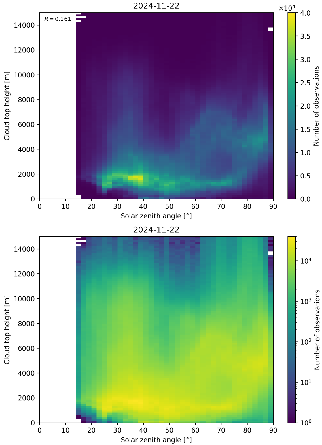
Figure 104: Scatter density plot of “Solar zenith angle” against “Cloud top height” for 2024-11-21 to 2024-11-23.
