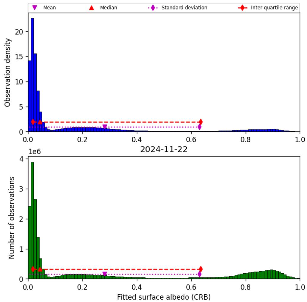
Figure 46: Histogram of “Fitted surface albedo (CRB)” for 2024-11-21 to 2024-11-23
