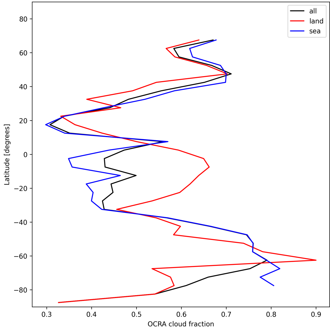
Figure 34: Zonal average of “OCRA cloud fraction” for 2024-11-21 to 2024-11-23.
