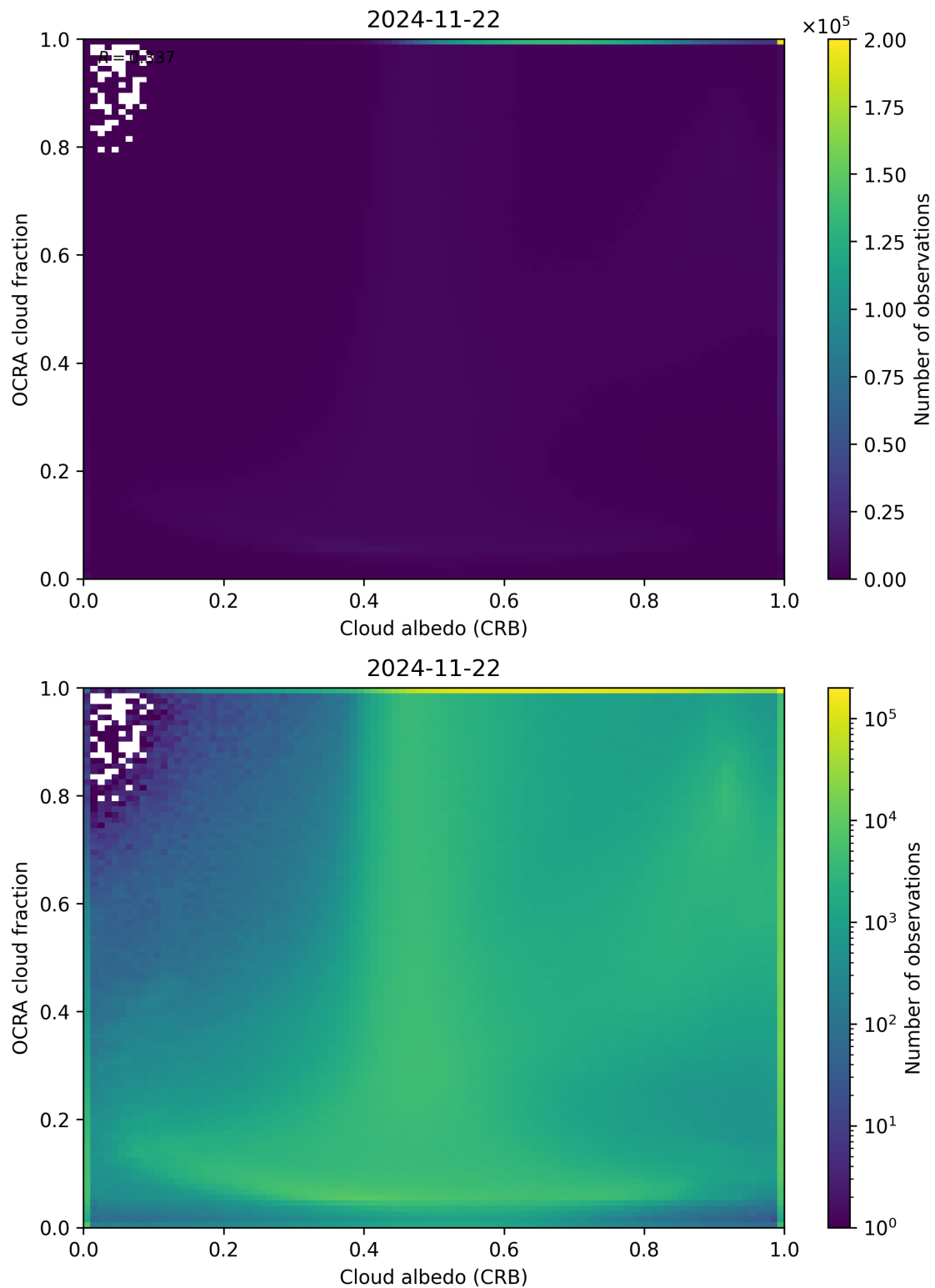
Figure 70: Scatter density plot of “Cloud albedo (CRB)” against “OCRA cloud fraction” for 2024-11-21 to 2024-11-23.
