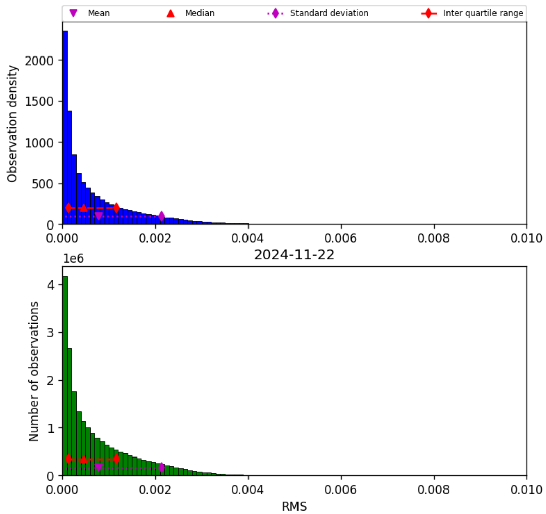
Figure 47: Histogram of “RMS” for 2024-11-21 to 2024-11-23
