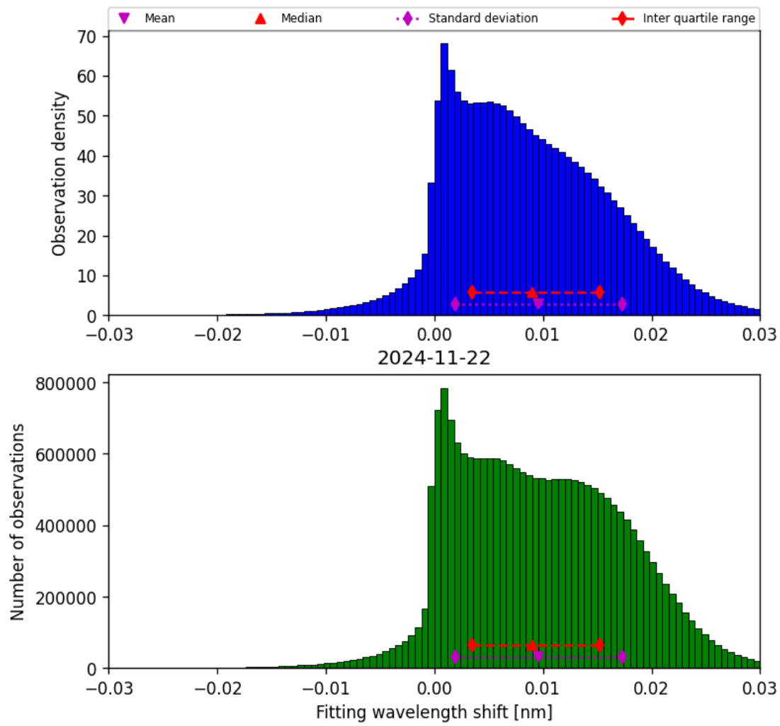
Figure 49: Histogram of “Fitting wavelength shift” for 2024-11-21 to 2024-11-23
