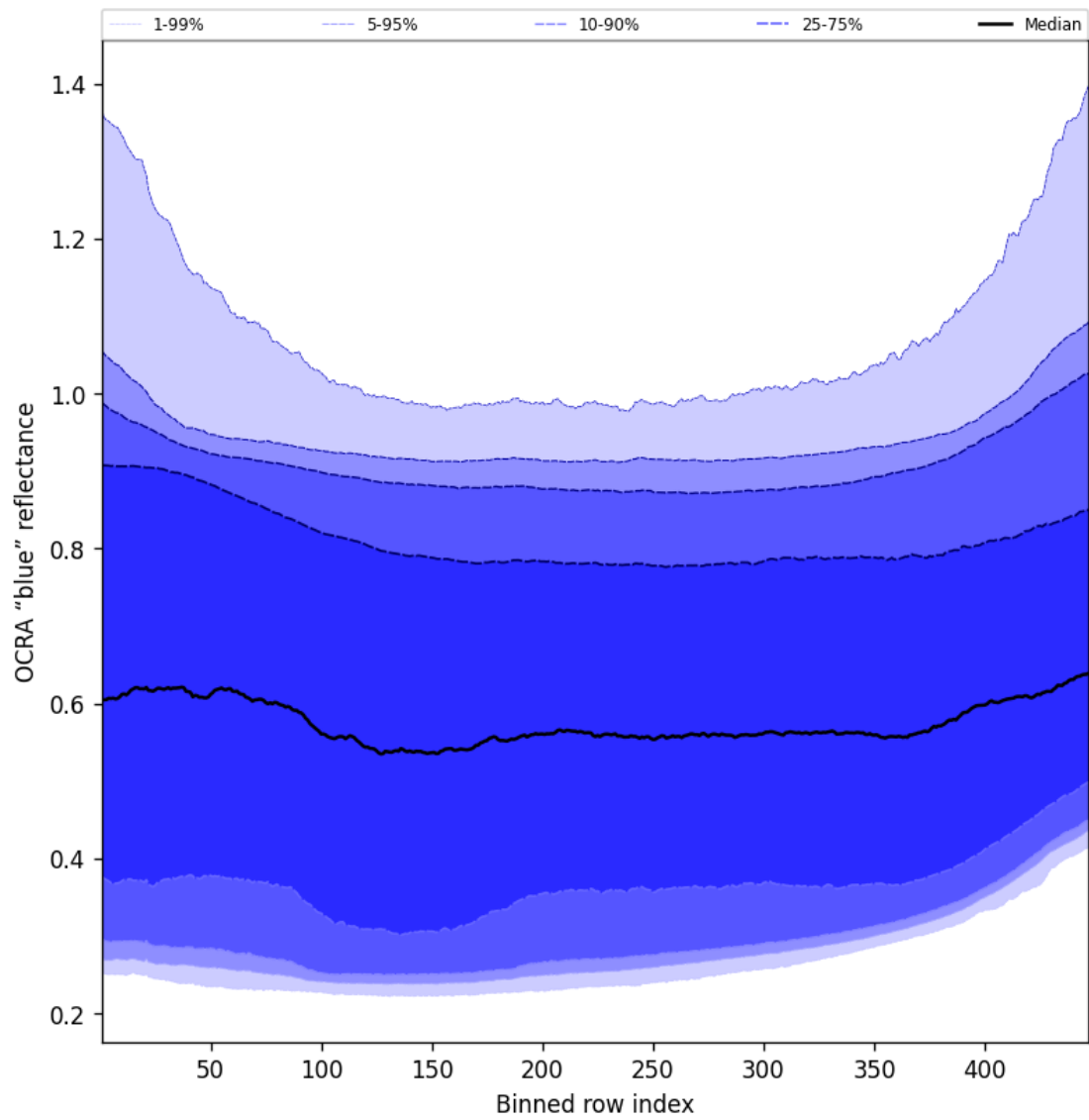
Figure 67: Along track statistics of “OCRA “blue” reflectance” for 2024-11-21 to 2024-11-23
