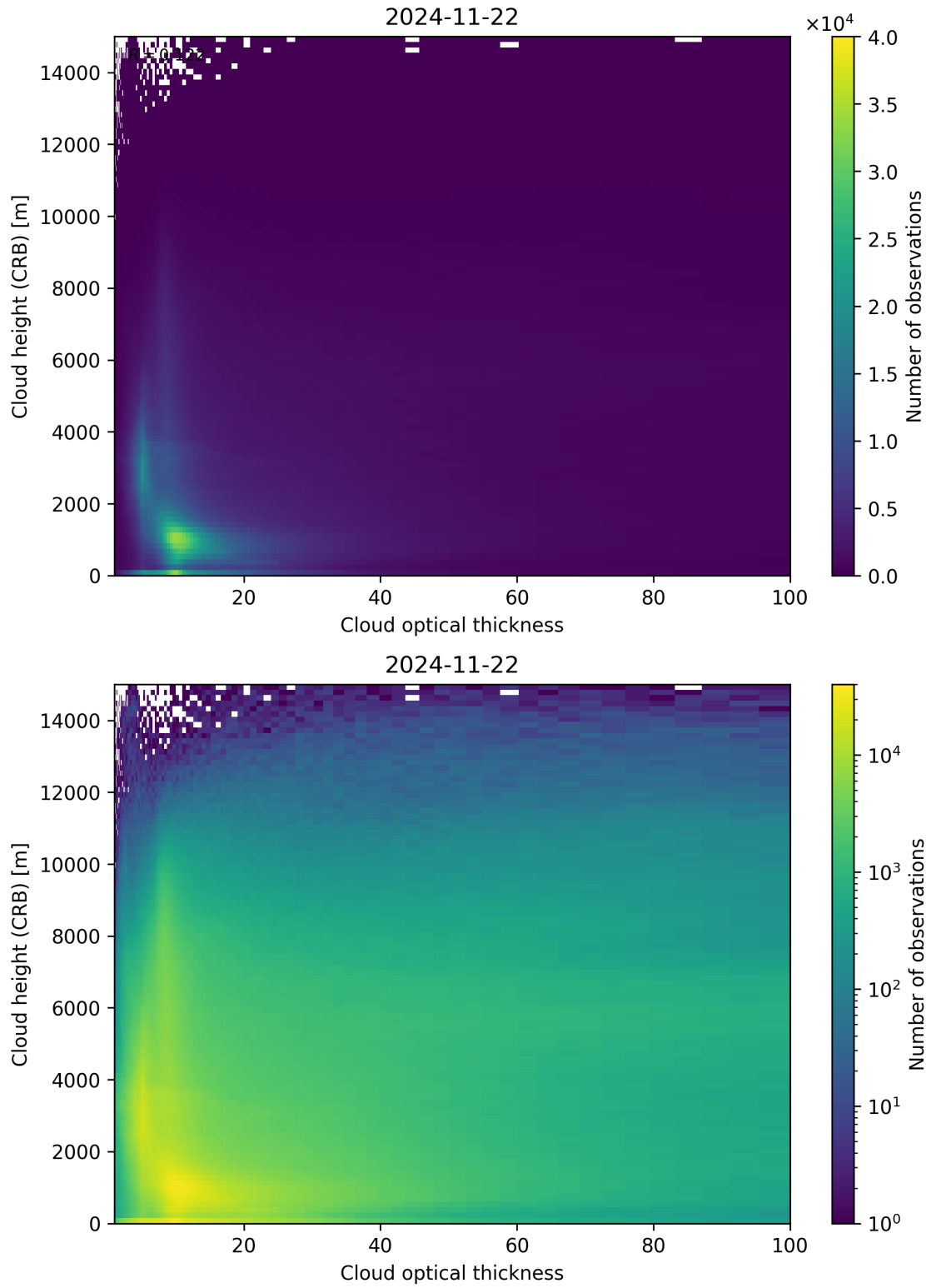
Figure 85: Scatter density plot of “Cloud optical thickness” against “Cloud height (CRB)” for 2024-11-21 to 2024-11-23.
