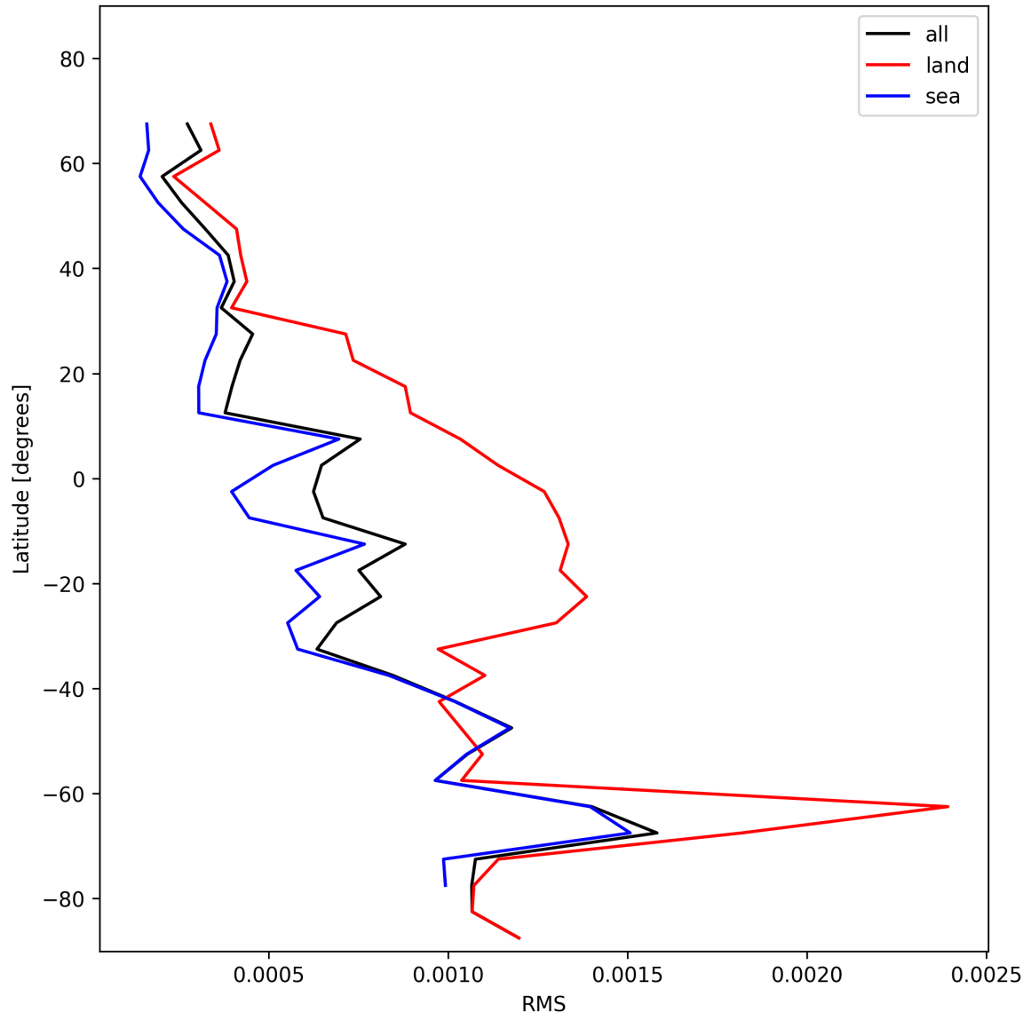
Figure 31: Zonal average of “RMS” for 2024-11-21 to 2024-11-23.
