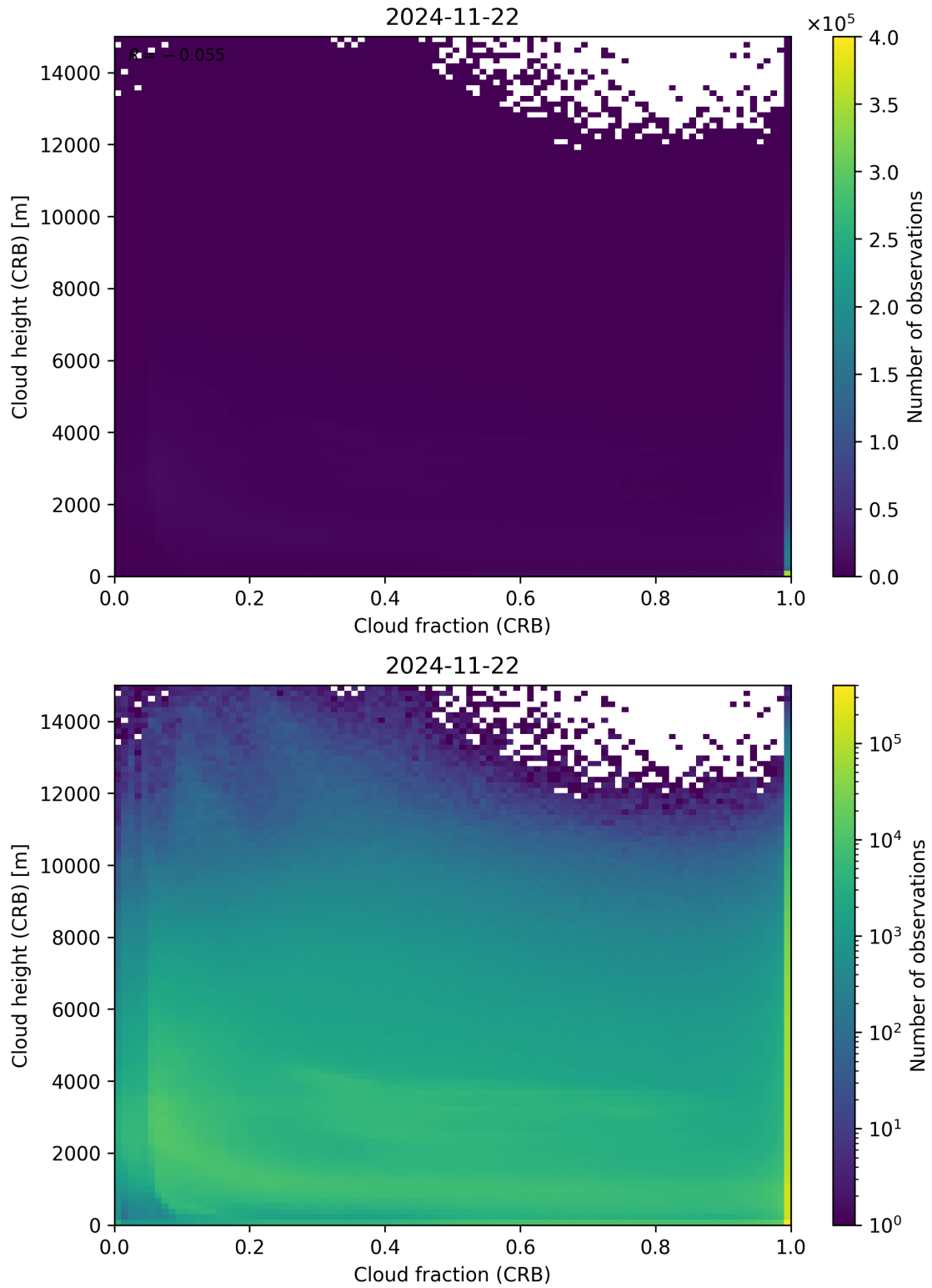
Figure 79: Scatter density plot of “Cloud fraction (CRB)” against “Cloud height (CRB)” for 2024-11-21 to 2024-11-23.
