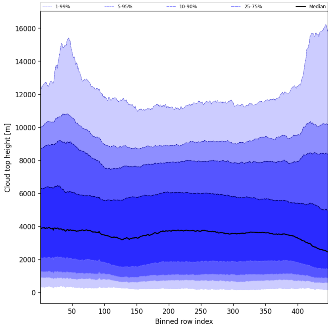
Figure 56: Along track statistics of “Cloud top height” for 2024-11-21 to 2024-11-23
