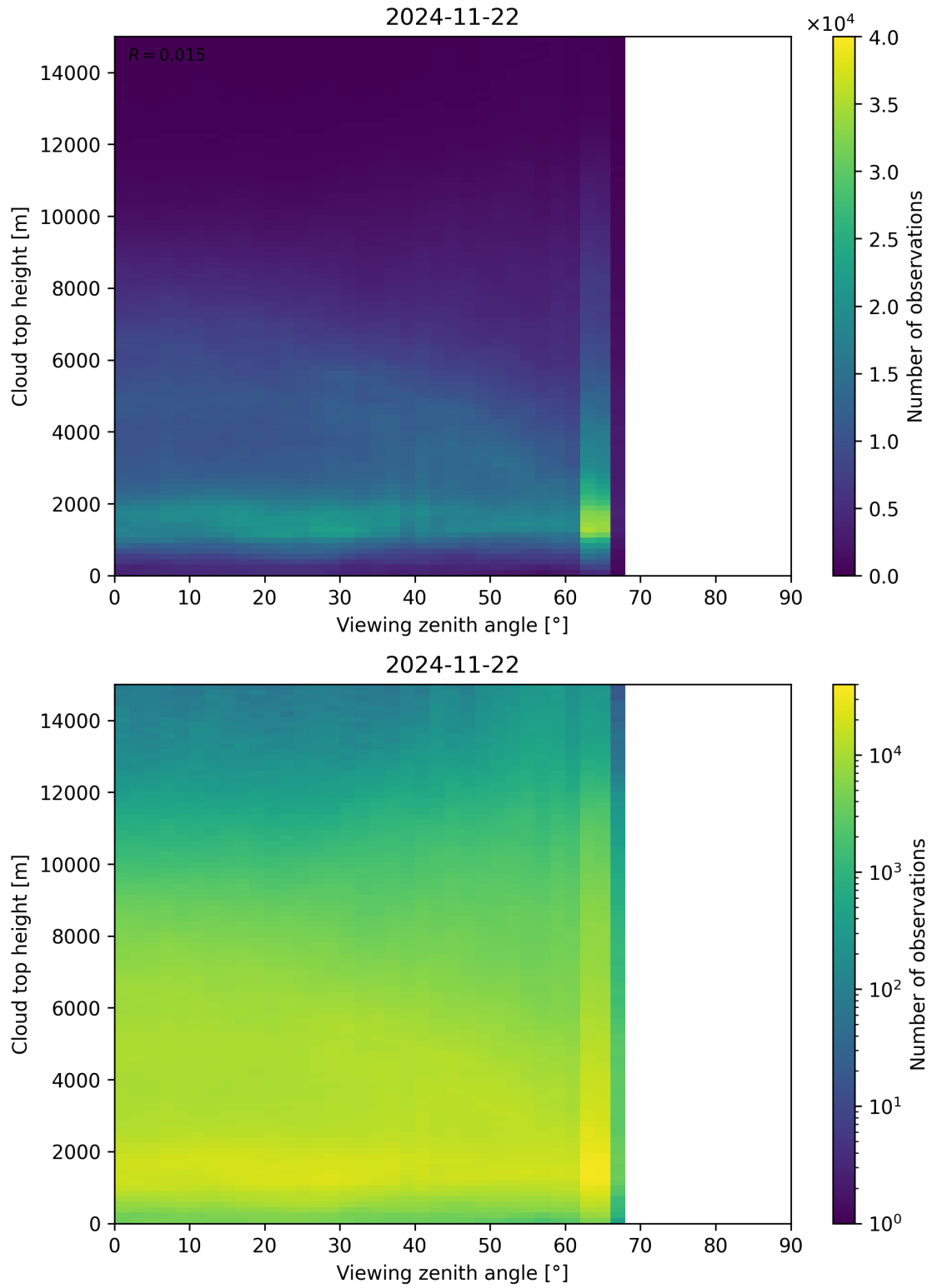
Figure 112: Scatter density plot of “Viewing zenith angle” against “Cloud top height” for 2024-11-21 to 2024-11-23.
