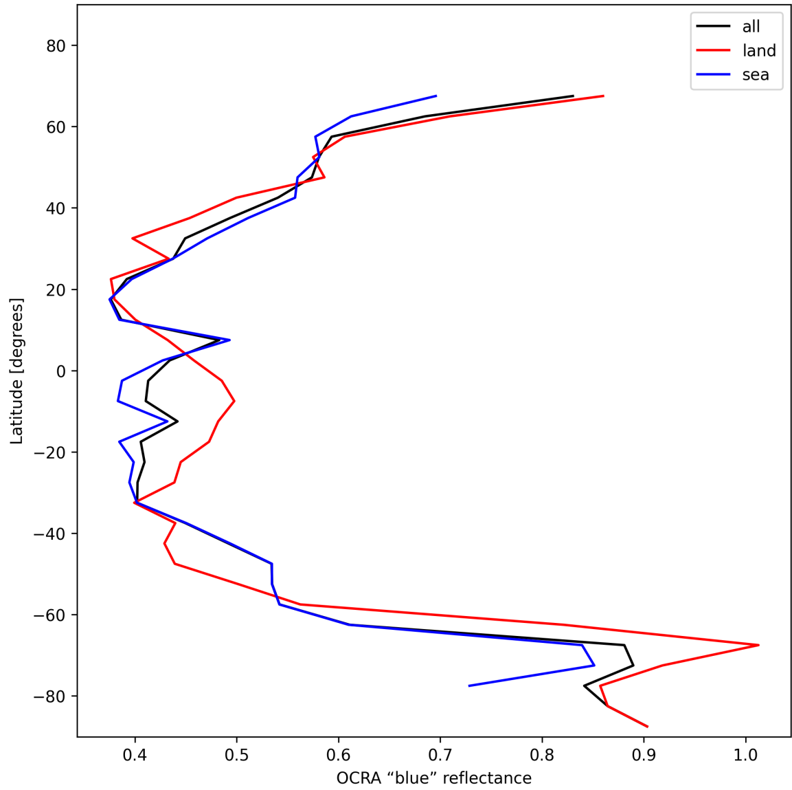
Figure 35: Zonal average of “OCRA “blue” reflectance” for 2024-11-21 to 2024-11-23.
