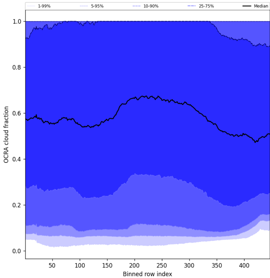
Figure 66: Along track statistics of “OCRA cloud fraction” for 2024-11-21 to 2024-11-23
