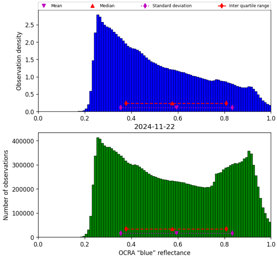
Figure 51: Histogram of "OCRA "blue" reflectance" for 2024-11-21 to 2024-11-23
