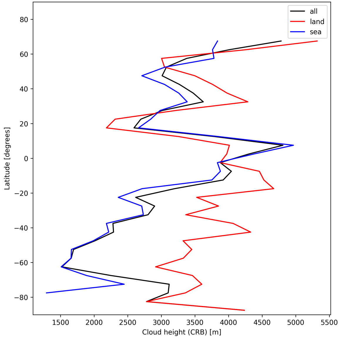
Figure 27: Zonal average of “Cloud height (CRB)” for 2024-11-21 to 2024-11-23.
