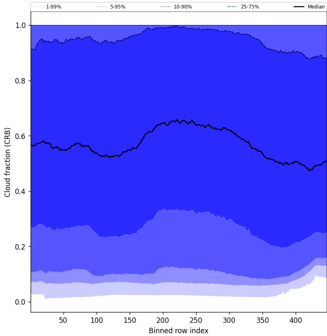
Figure 58: Along track statistics of “Cloud fraction (CRB)” for 2024-11-21 to 2024-11-23
