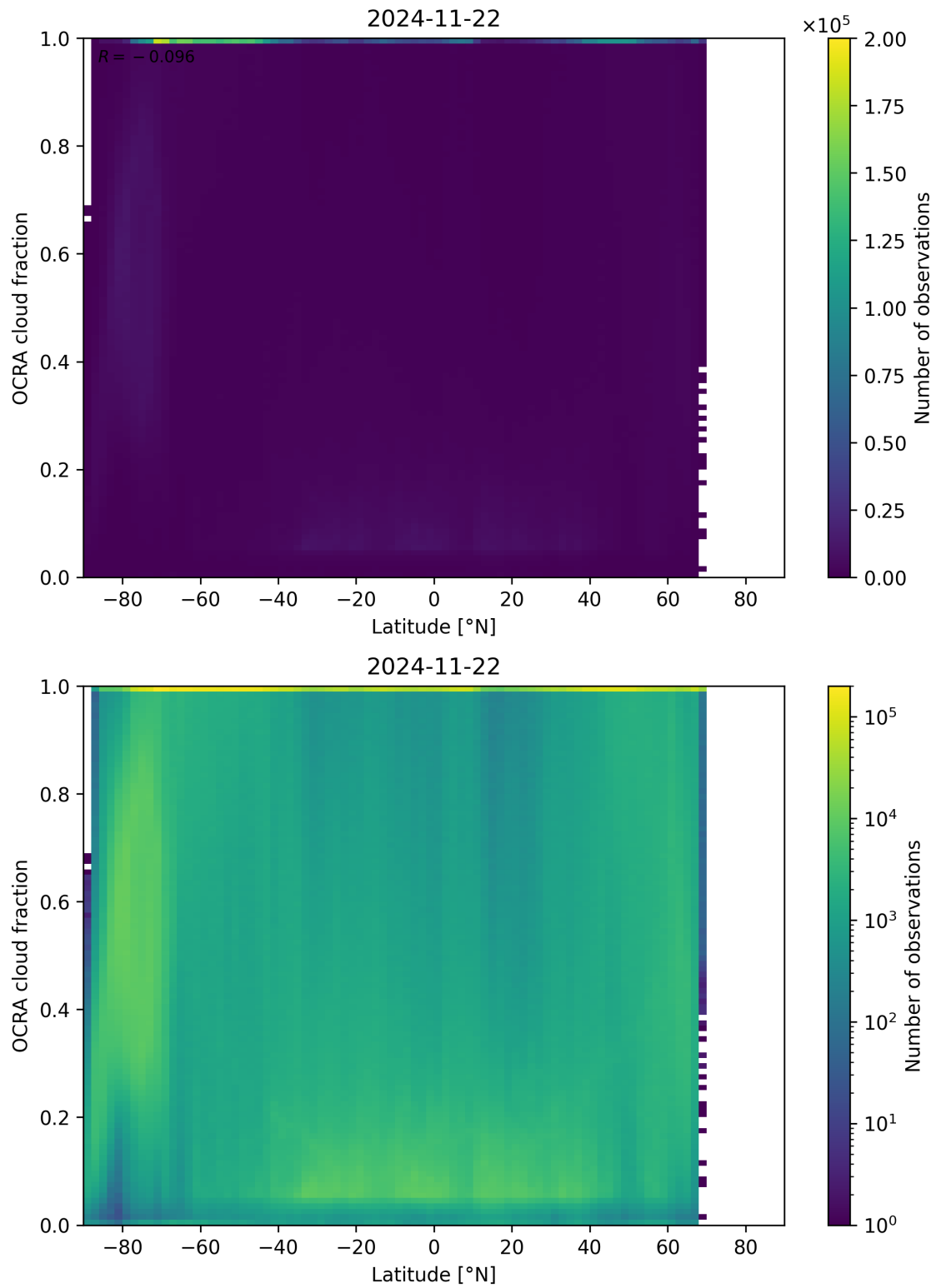
Figure 93: Scatter density plot of “Latitude” against “OCRA cloud fraction” for 2024-11-21 to 2024-11-23.
