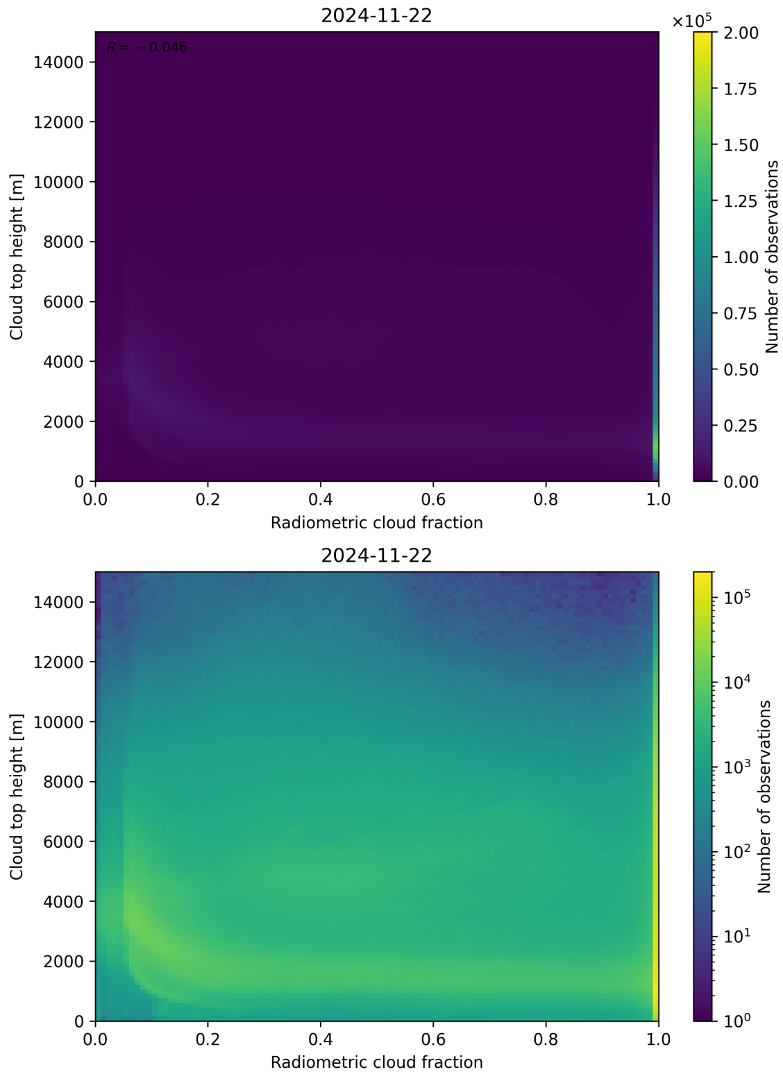
Figure 76: Scatter density plot of “Radiometric cloud fraction” against “Cloud top height” for 2024-11-21 to 2024-11-23.
