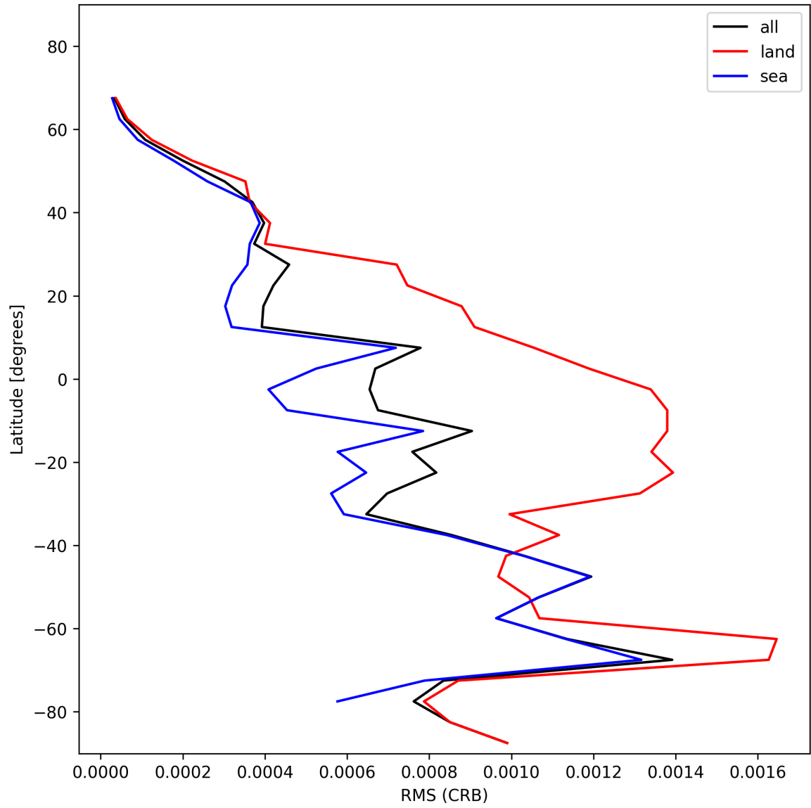
Figure 32: Zonal average of “RMS (CRB)” for 2024-11-21 to 2024-11-23.
