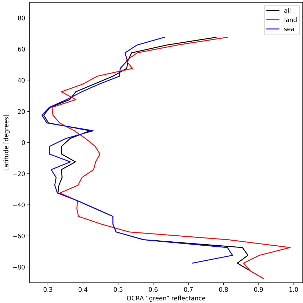
Figure 36: Zonal average of “OCRA “green” reflectance” for 2024-11-21 to 2024-11-23.
