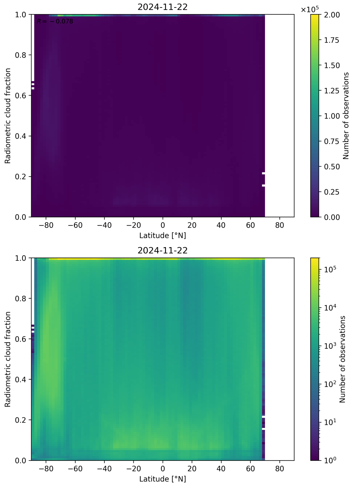
Figure 92: Scatter density plot of “Latitude” against “Radiometric cloud fraction” for 2024-11-21 to 2024-11-23.
