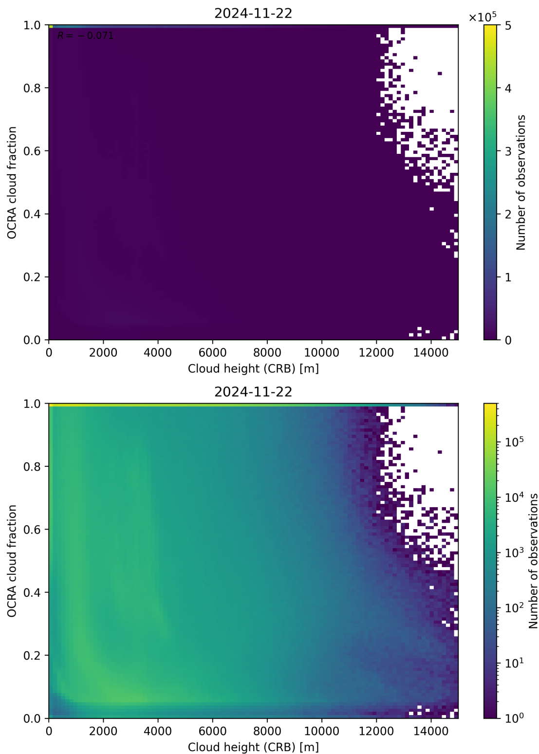
Figure 81: Scatter density plot of “Cloud height (CRB)” against “OCRA cloud fraction” for 2024-11-21 to 2024-11-23.
