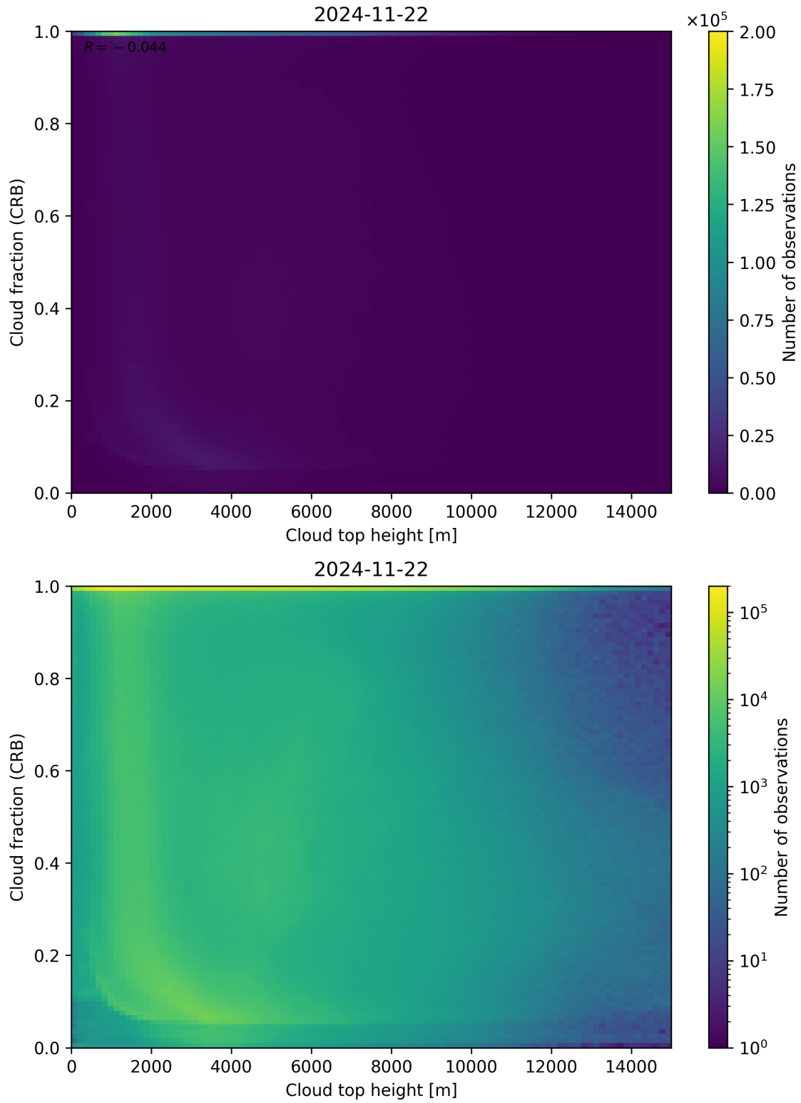
Figure 88: Scatter density plot of “Cloud top height” against “Cloud fraction (CRB)” for 2024-11-21 to 2024-11-23.
