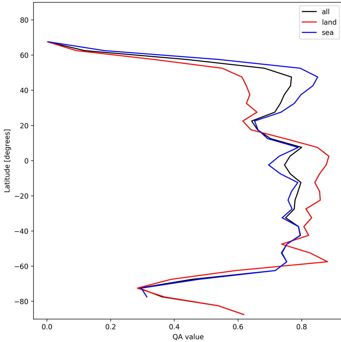
Figure 22: Zonal average of “QA value” for 2024-11-21 to 2024-11-23.
