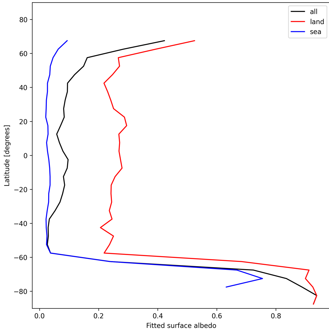
Figure 29: Zonal average of “Fitted surface albedo” for 2024-11-21 to 2024-11-23.
