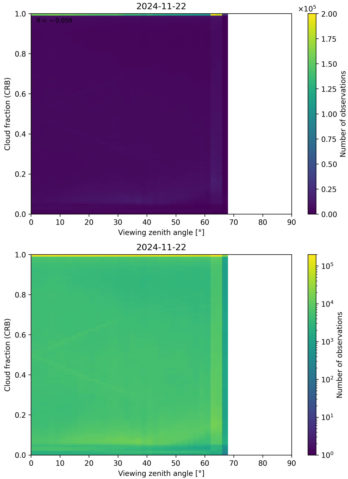
Figure 109: Scatter density plot of “Viewing zenith angle” against “Cloud fraction (CRB)” for 2024-11-21 to 2024-11-23.
