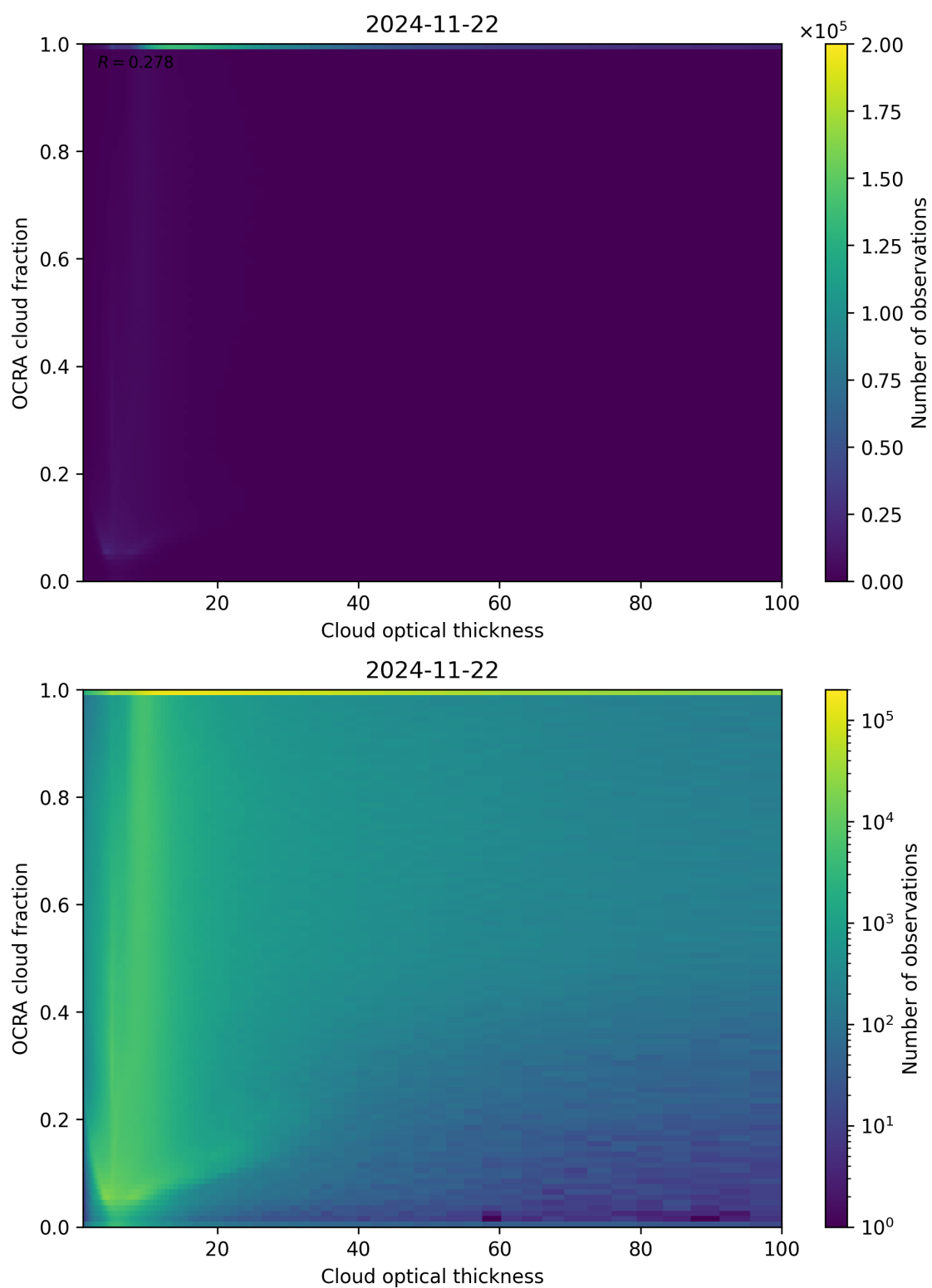
Figure 83: Scatter density plot of “Cloud optical thickness” against “OCRA cloud fraction” for 2024-11-21 to 2024-11-23.
