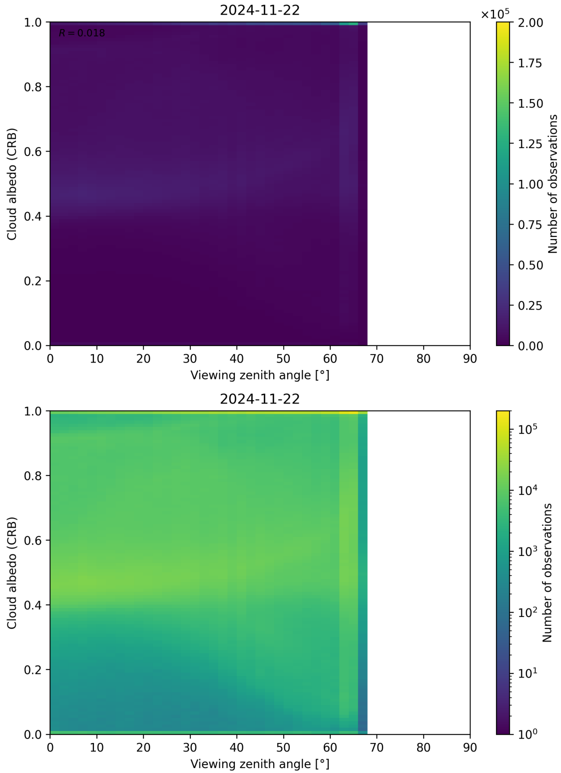
Figure 106: Scatter density plot of “Viewing zenith angle” against “Cloud albedo (CRB)” for 2024-11-21 to 2024-11-23.
