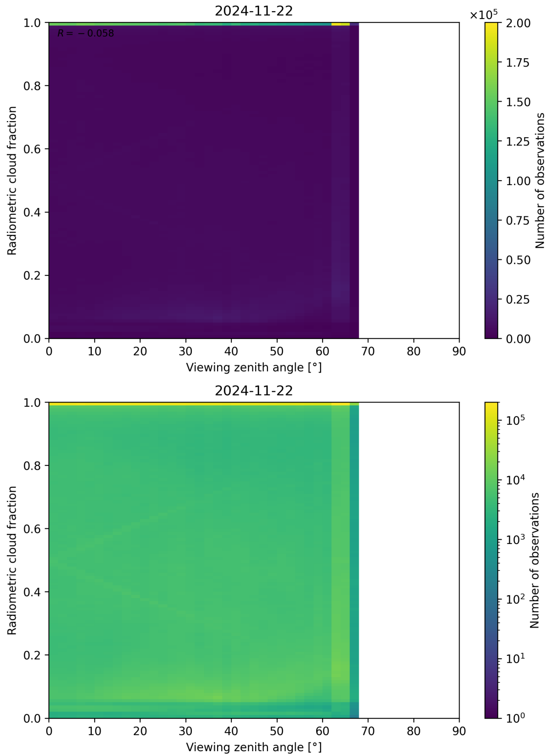
Figure 107: Scatter density plot of “Viewing zenith angle” against “Radiometric cloud fraction” for 2024-11-21 to 2024-11-23.
