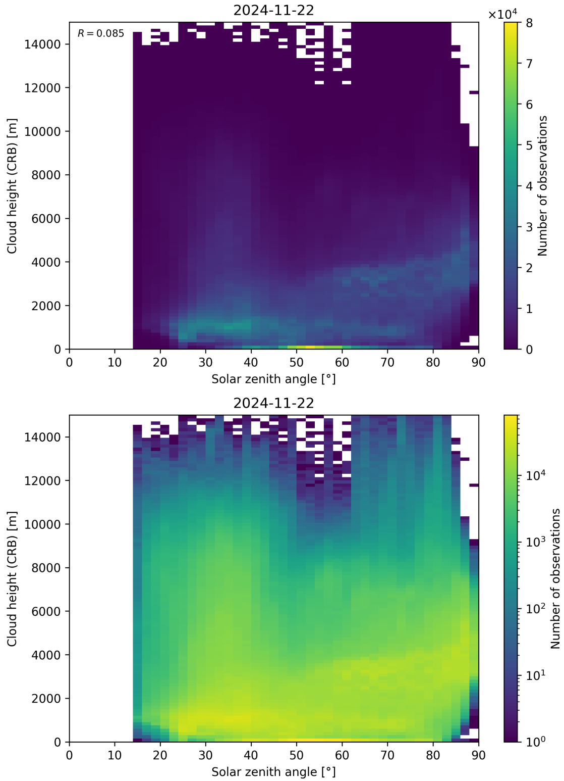
Figure 102: Scatter density plot of “Solar zenith angle” against “Cloud height (CRB)” for 2024-11-21 to 2024-11-23.
