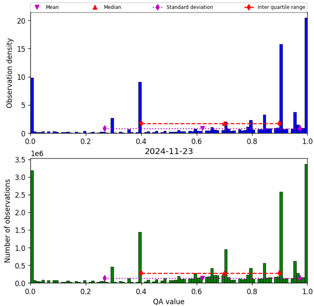
Figure 38: Histogram of “QA value” for 2024-11-22 to 2024-11-24
