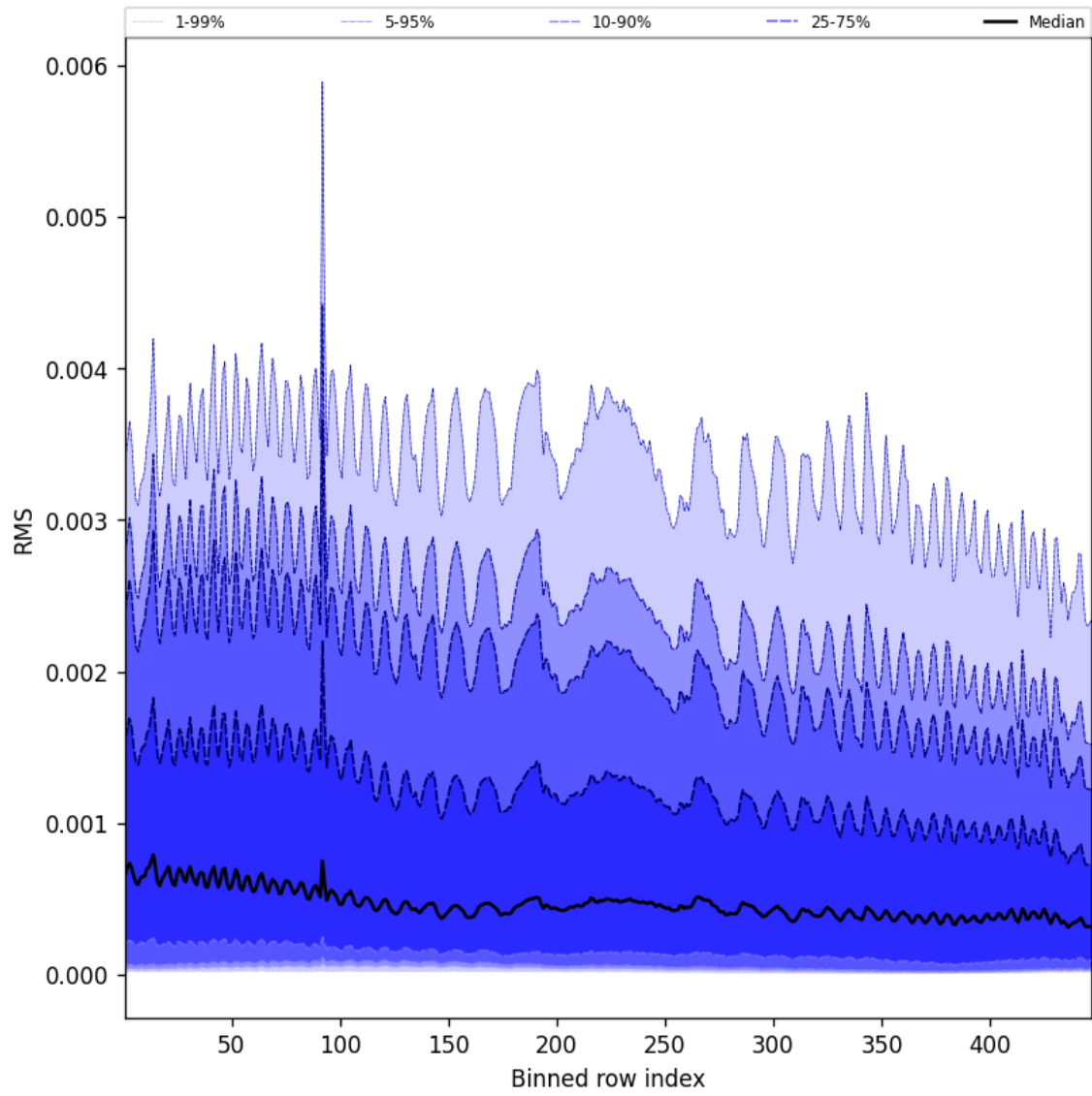
Figure 63: Along track statistics of “RMS” for 2024-11-22 to 2024-11-24
