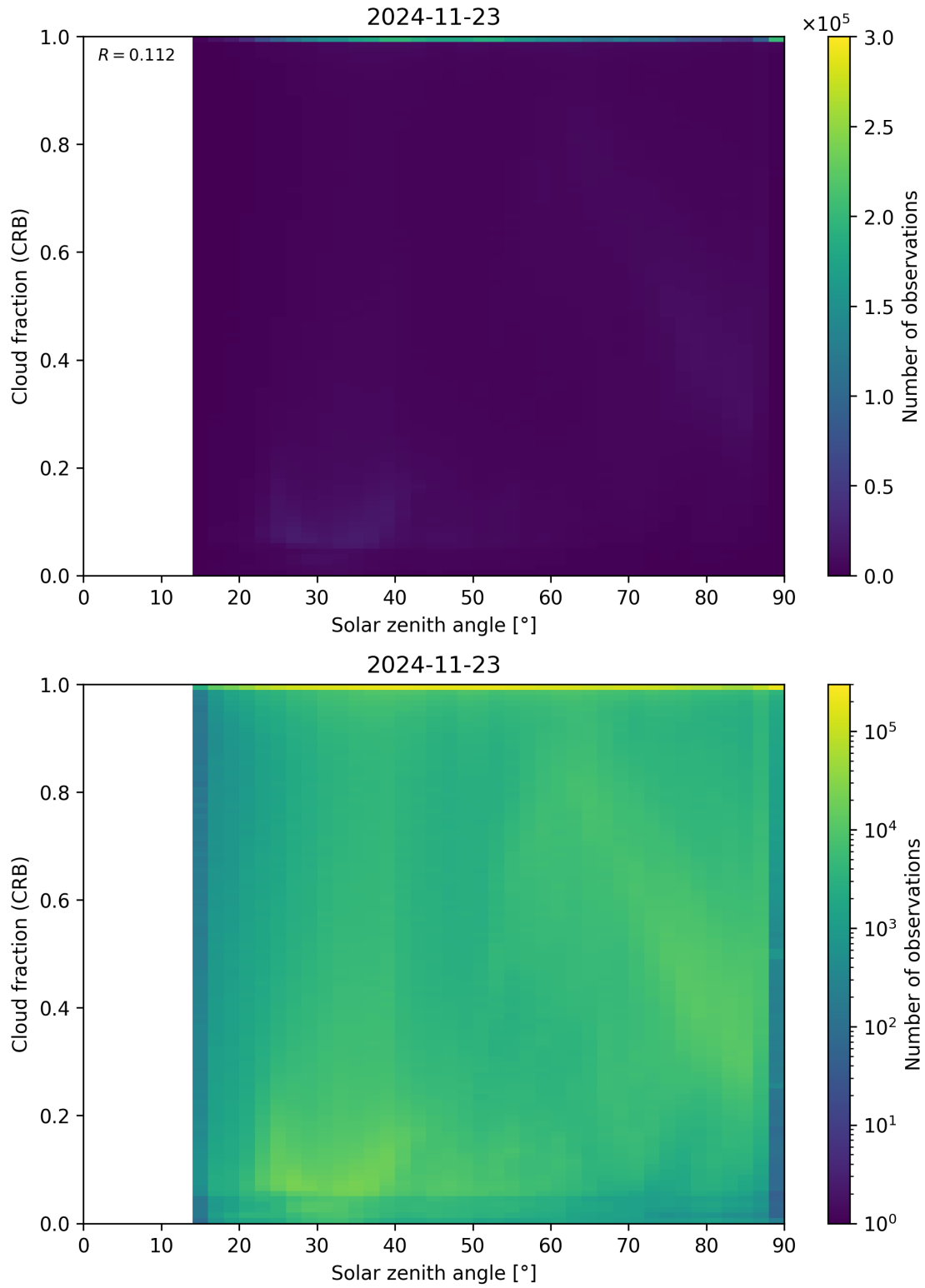
Figure 101: Scatter density plot of “Solar zenith angle” against “Cloud fraction (CRB)” for 2024-11-22 to 2024-11-24.
