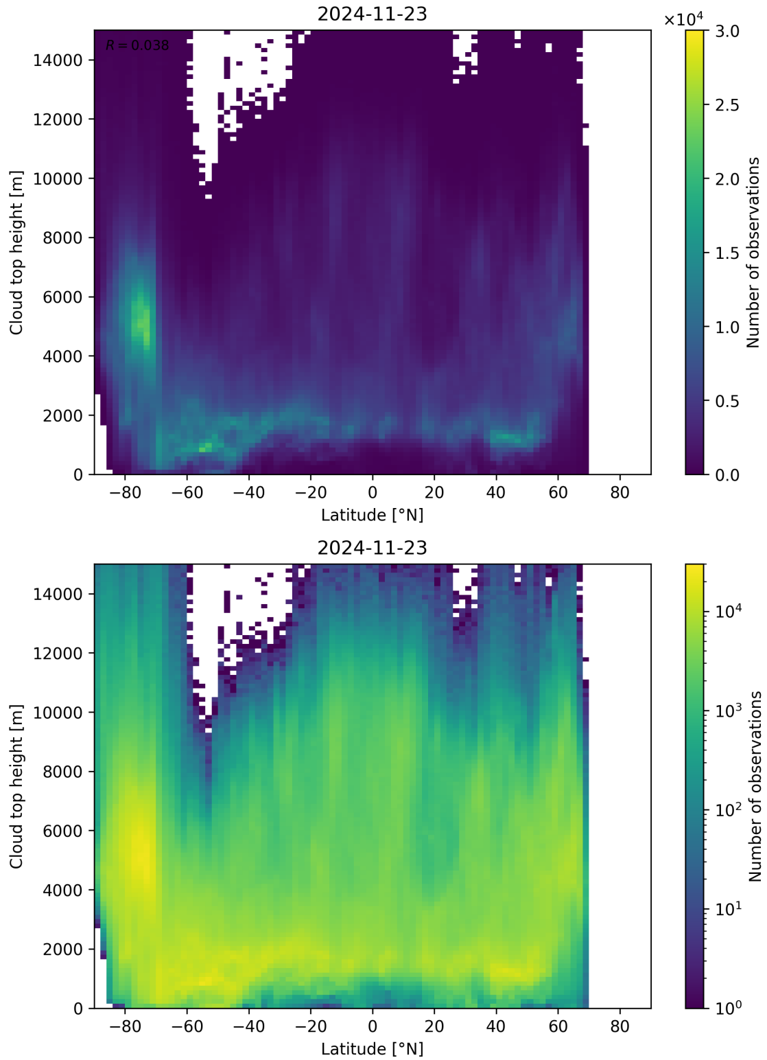
Figure 97: Scatter density plot of “Latitude” against “Cloud top height” for 2024-11-22 to 2024-11-24.
