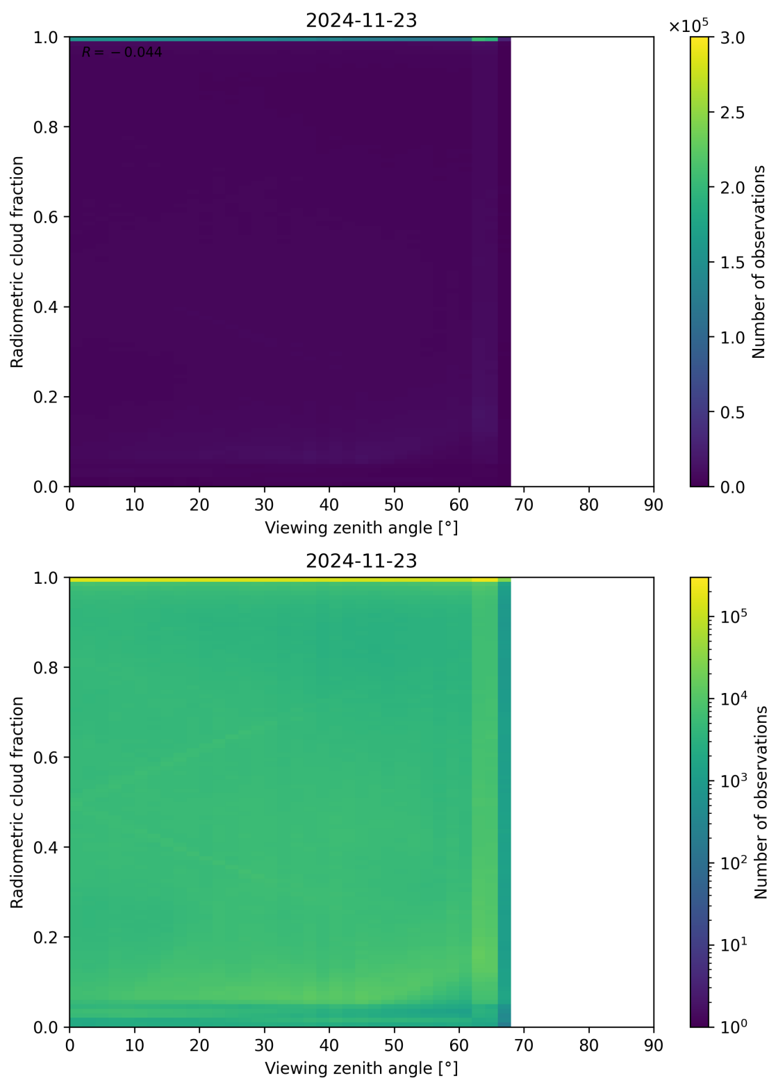
Figure 107: Scatter density plot of “Viewing zenith angle” against “Radiometric cloud fraction” for 2024-11-22 to 2024-11-24.
