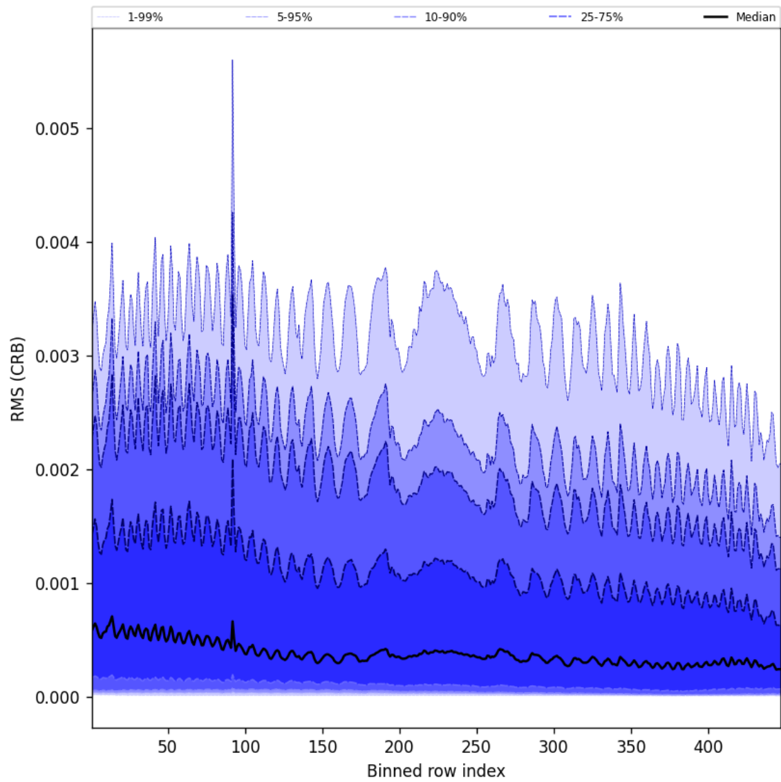
Figure 64: Along track statistics of “RMS (CRB)” for 2024-11-22 to 2024-11-24
