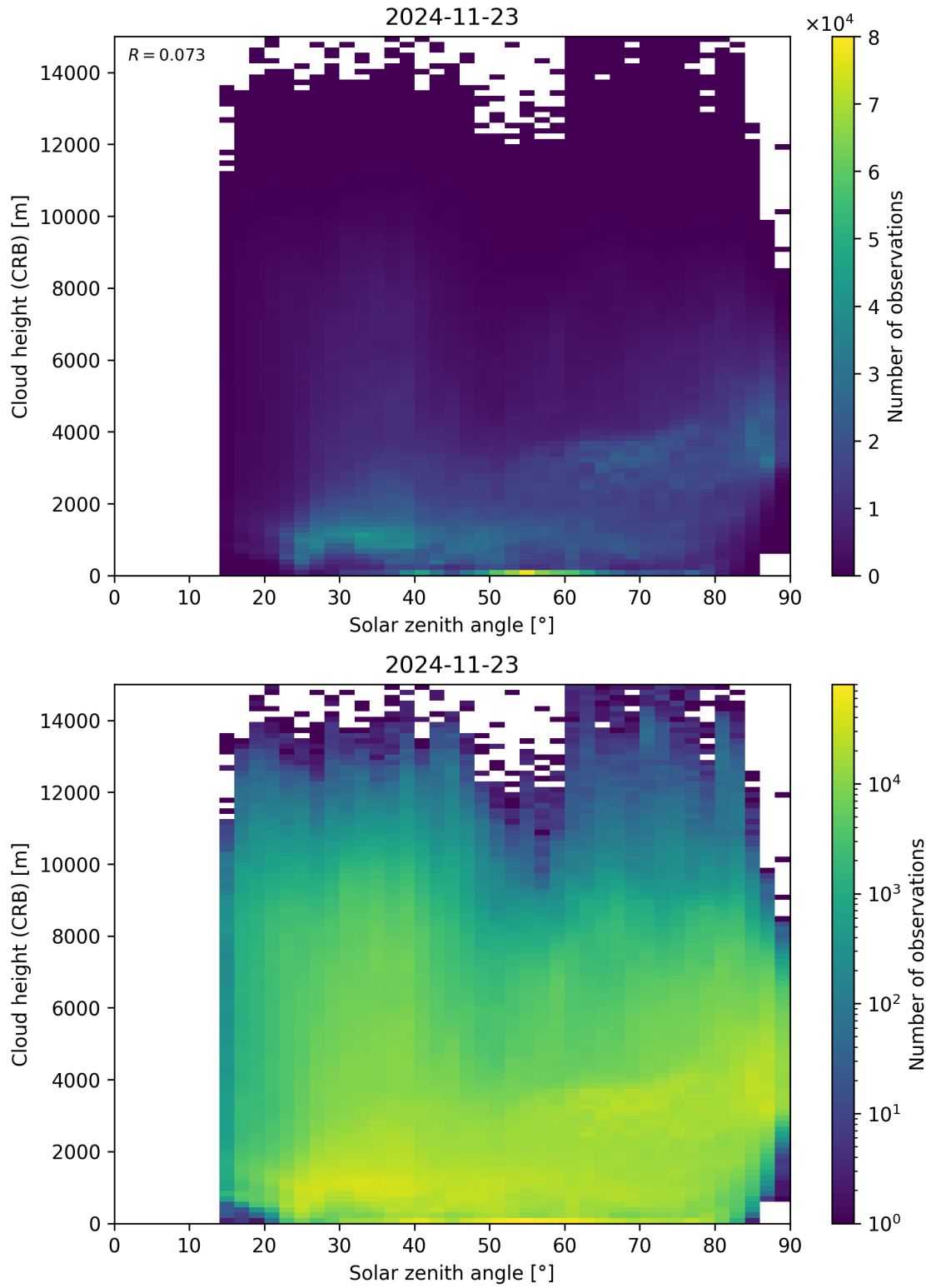
Figure 102: Scatter density plot of “Solar zenith angle” against “Cloud height (CRB)” for 2024-11-22 to 2024-11-24.
