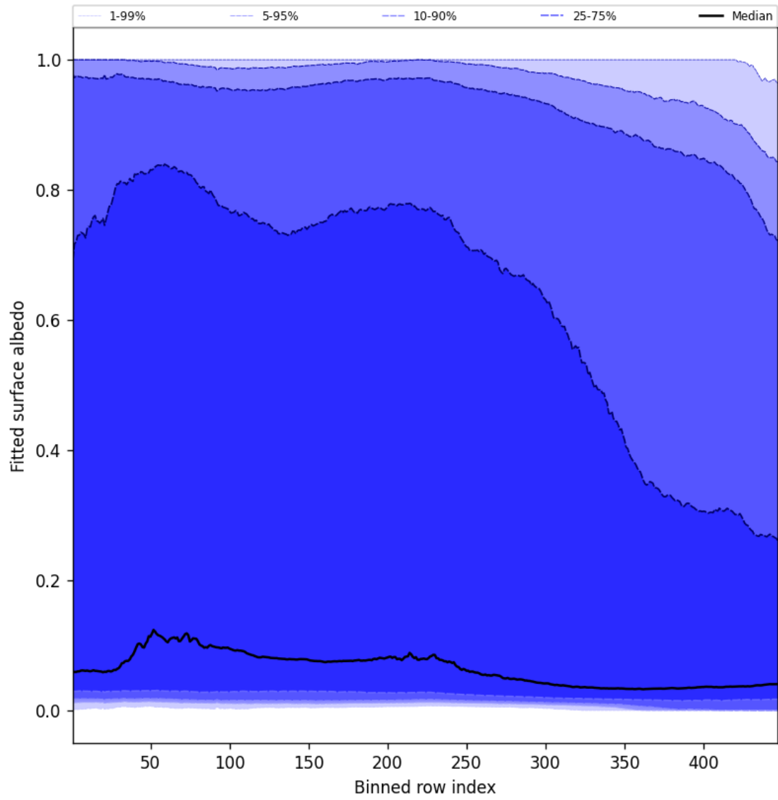
Figure 61: Along track statistics of “Fitted surface albedo” for 2024-11-22 to 2024-11-24
