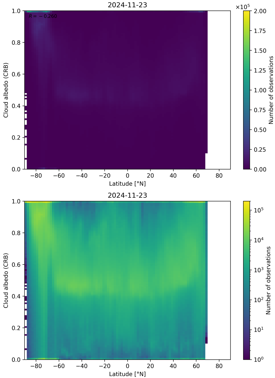
Figure 91: Scatter density plot of “Latitude” against “Cloud albedo (CRB)” for 2024-11-22 to 2024-11-24.
