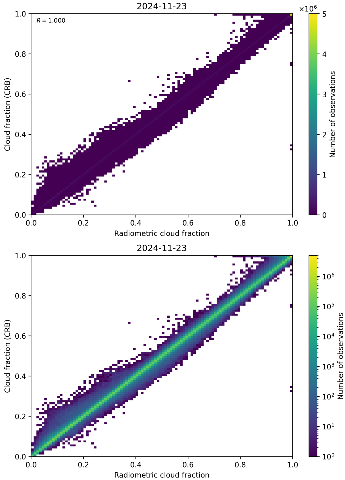
Figure 73: Scatter density plot of “Radiometric cloud fraction” against “Cloud fraction (CRB)” for 2024-11-22 to 2024-11-24.
