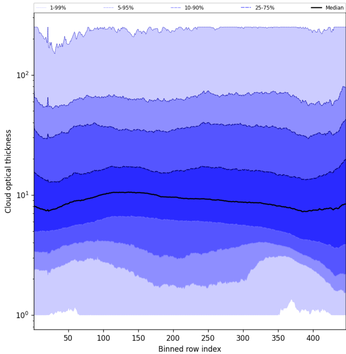
Figure 57: Along track statistics of “Cloud optical thickness” for 2024-11-22 to 2024-11-24
