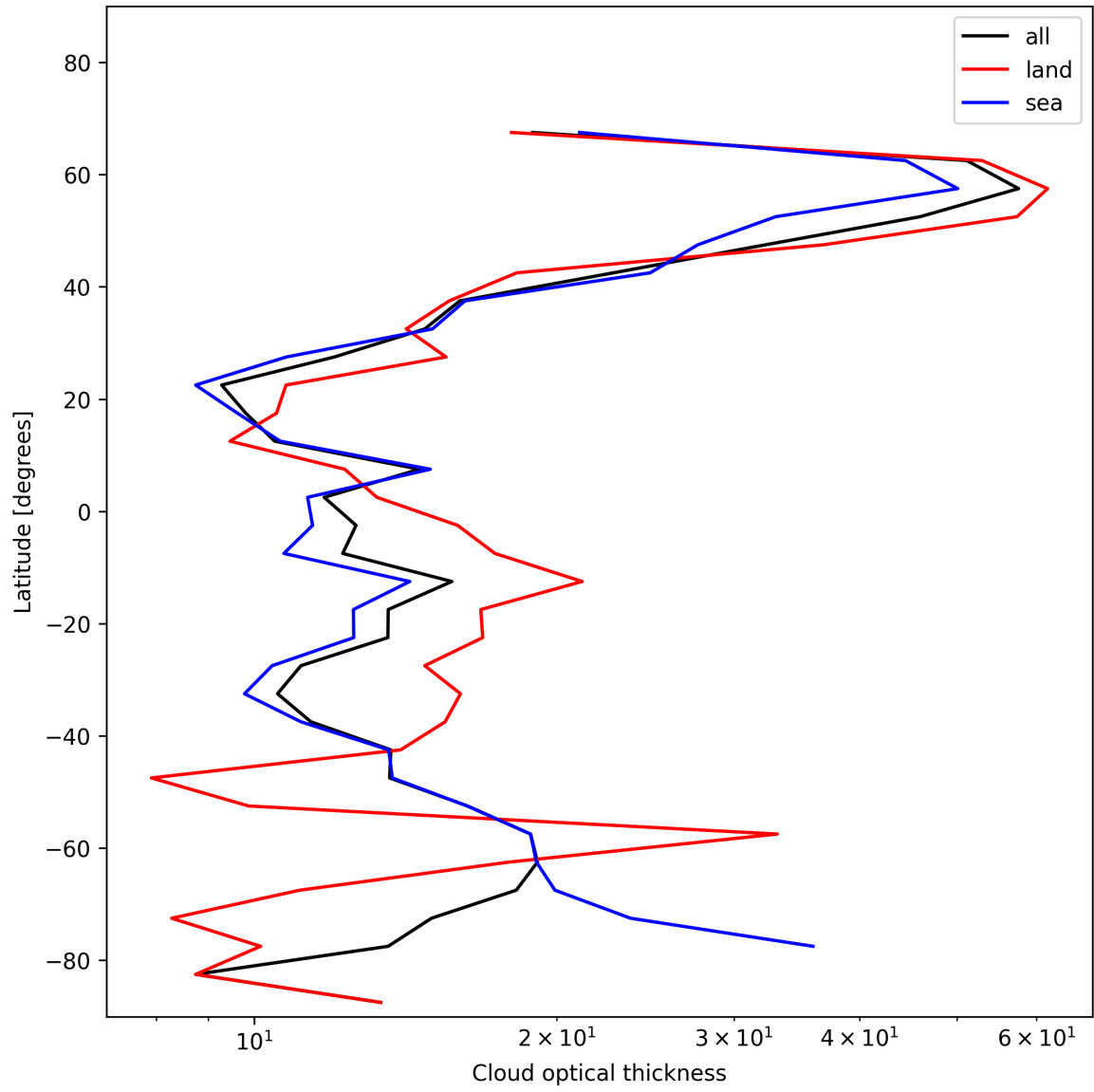
Figure 25: Zonal average of “Cloud optical thickness” for 2024-11-22 to 2024-11-24.
