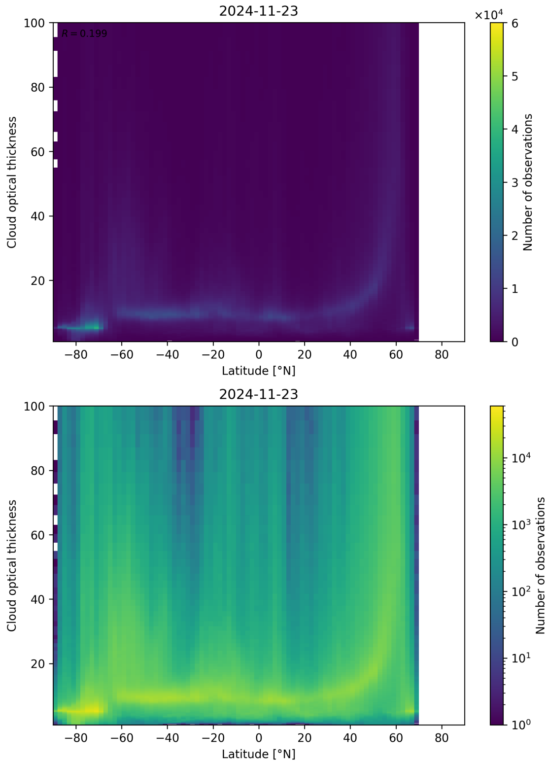
Figure 96: Scatter density plot of “Latitude” against “Cloud optical thickness” for 2024-11-22 to 2024-11-24.
