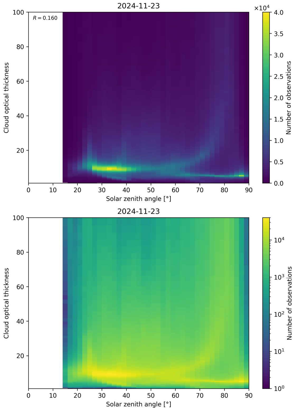
Figure 103: Scatter density plot of “Solar zenith angle” against “Cloud optical thickness” for 2024-11-22 to 2024-11-24.
