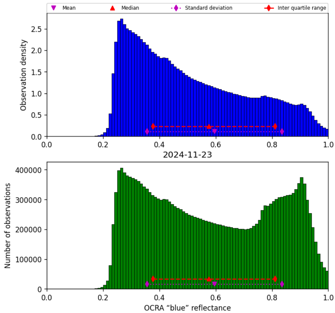
Figure 51: Histogram of “OCRA “blue” reflectance” for 2024-11-22 to 2024-11-24
