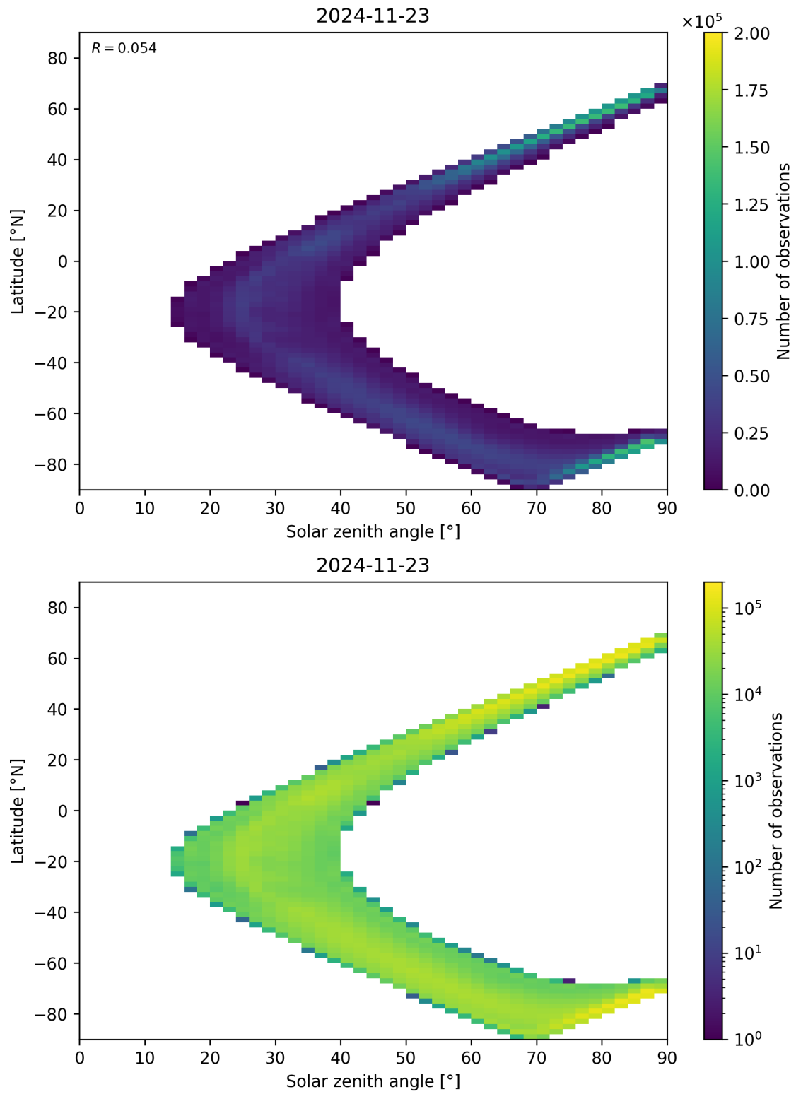
Figure 105: Scatter density plot of “Solar zenith angle” against “Latitude” for 2024-11-22 to 2024-11-24.
