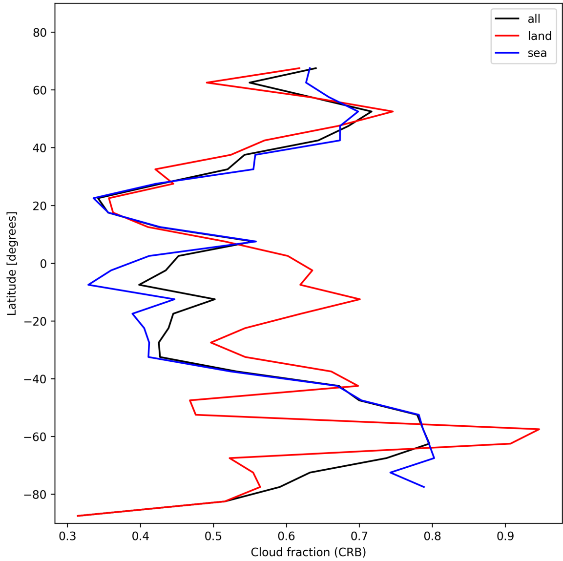
Figure 26: Zonal average of “Cloud fraction (CRB)” for 2024-11-22 to 2024-11-24.
