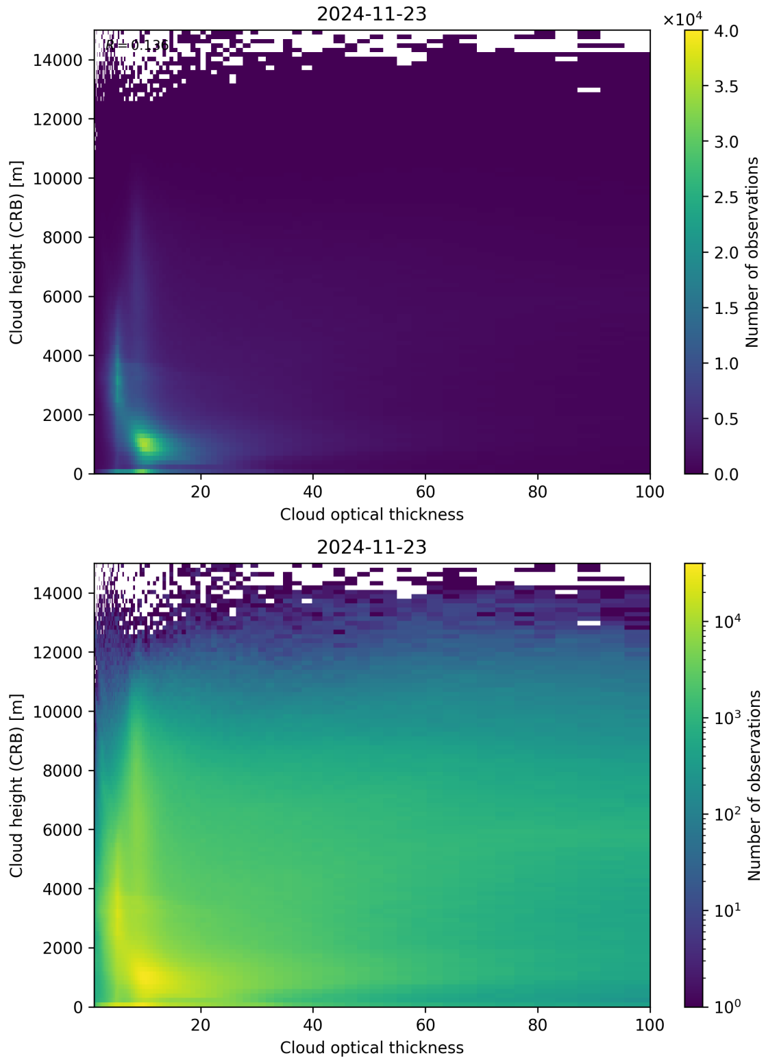
Figure 85: Scatter density plot of “Cloud optical thickness” against “Cloud height (CRB)” for 2024-11-22 to 2024-11-24.
