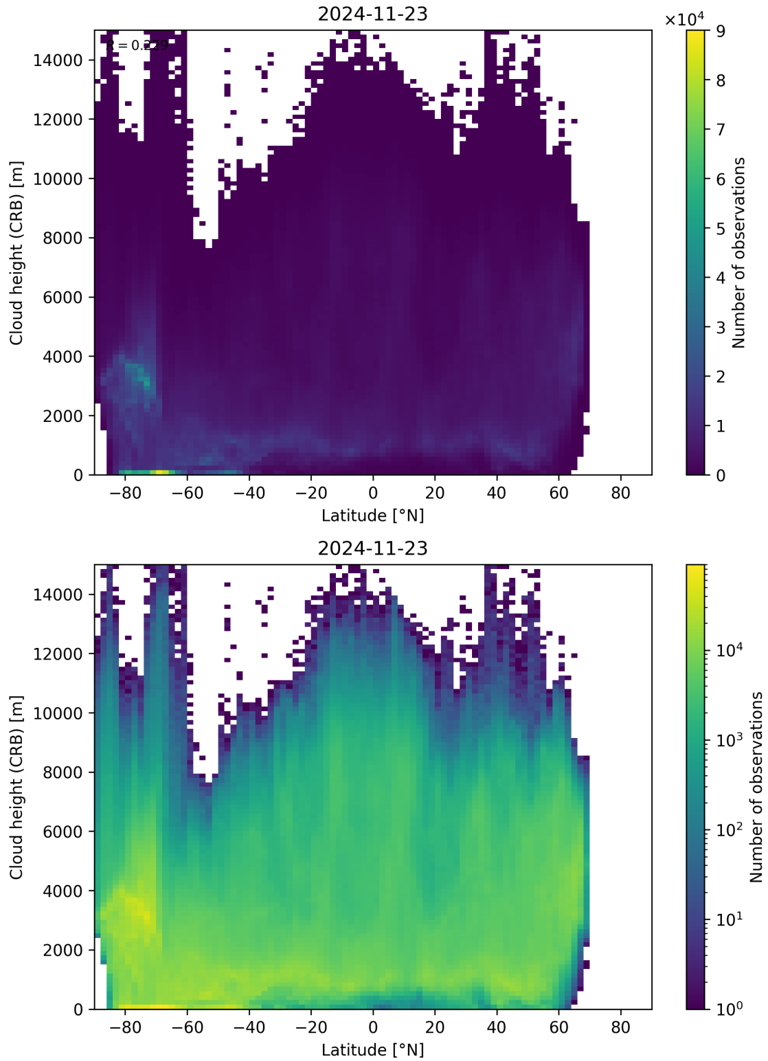
Figure 95: Scatter density plot of “Latitude” against “Cloud height (CRB)” for 2024-11-22 to 2024-11-24.
