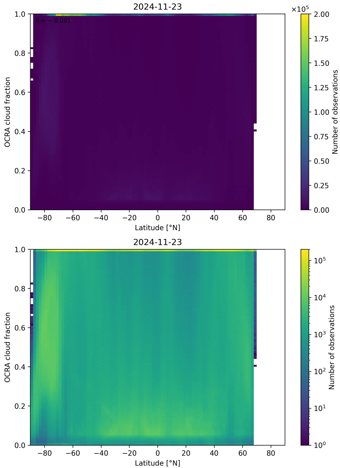
Figure 93: Scatter density plot of “Latitude” against “OCRA cloud fraction” for 2024-11-22 to 2024-11-24.
