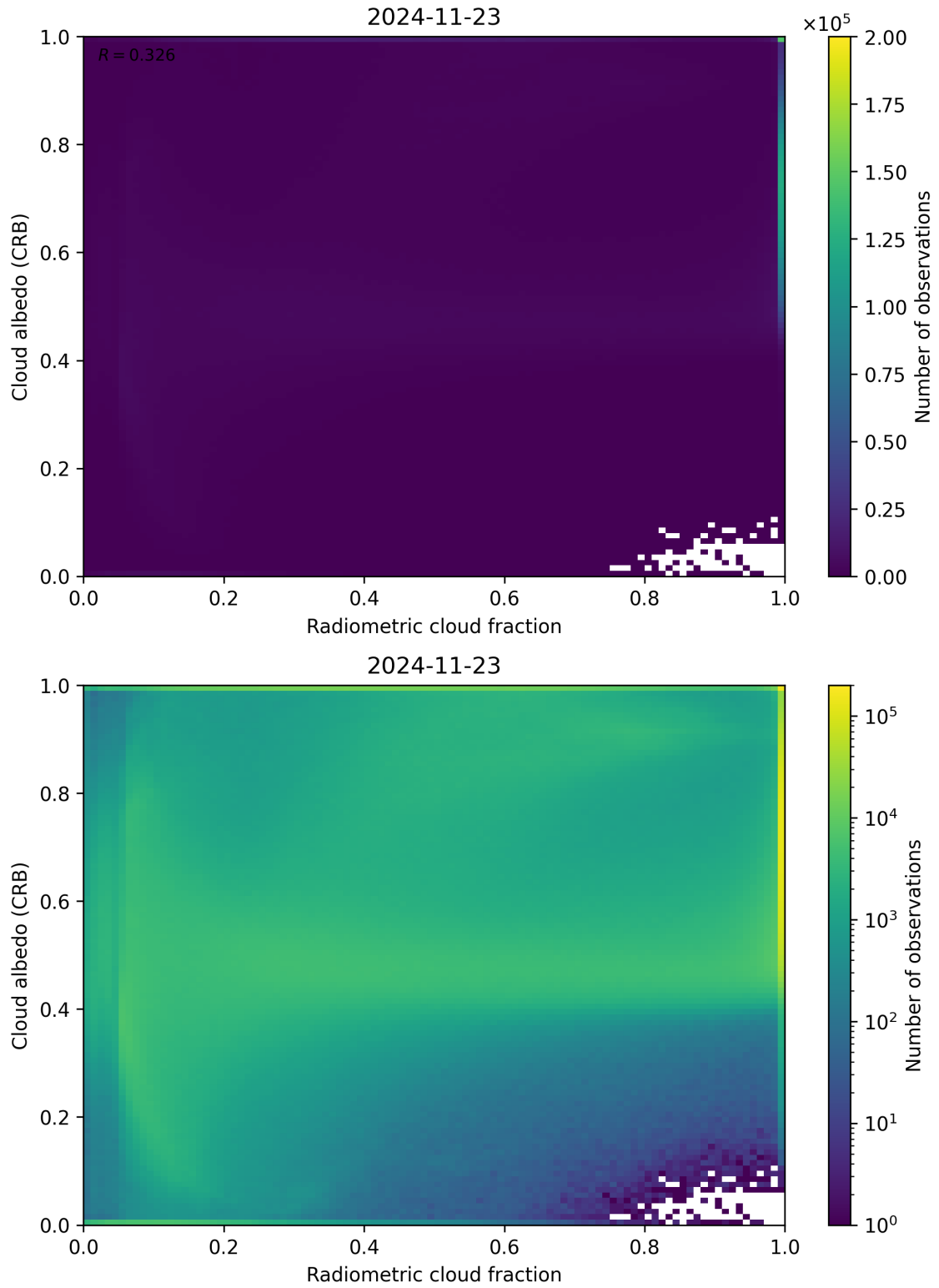
Figure 71: Scatter density plot of “Radiometric cloud fraction” against “Cloud albedo (CRB)” for 2024-11-22 to 2024-11-24.
