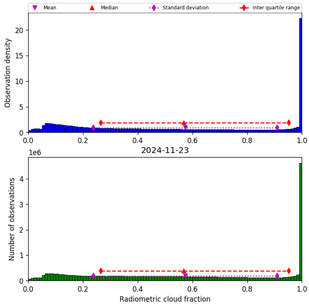
Figure 39: Histogram of “Radiometric cloud fraction” for 2024-11-22 to 2024-11-24
