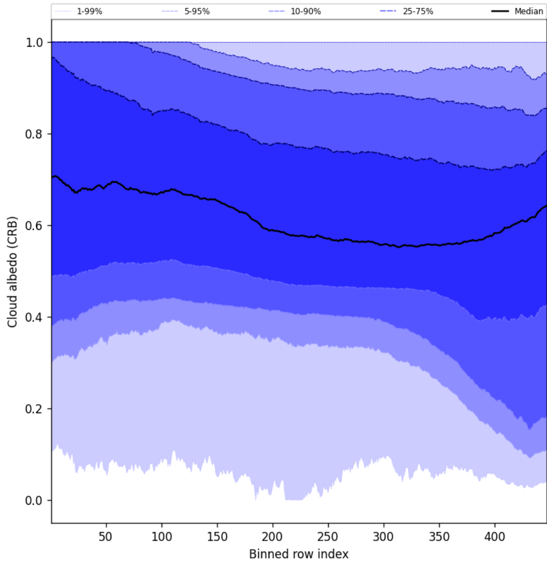
Figure 60: Along track statistics of “Cloud albedo (CRB)” for 2024-11-22 to 2024-11-24
