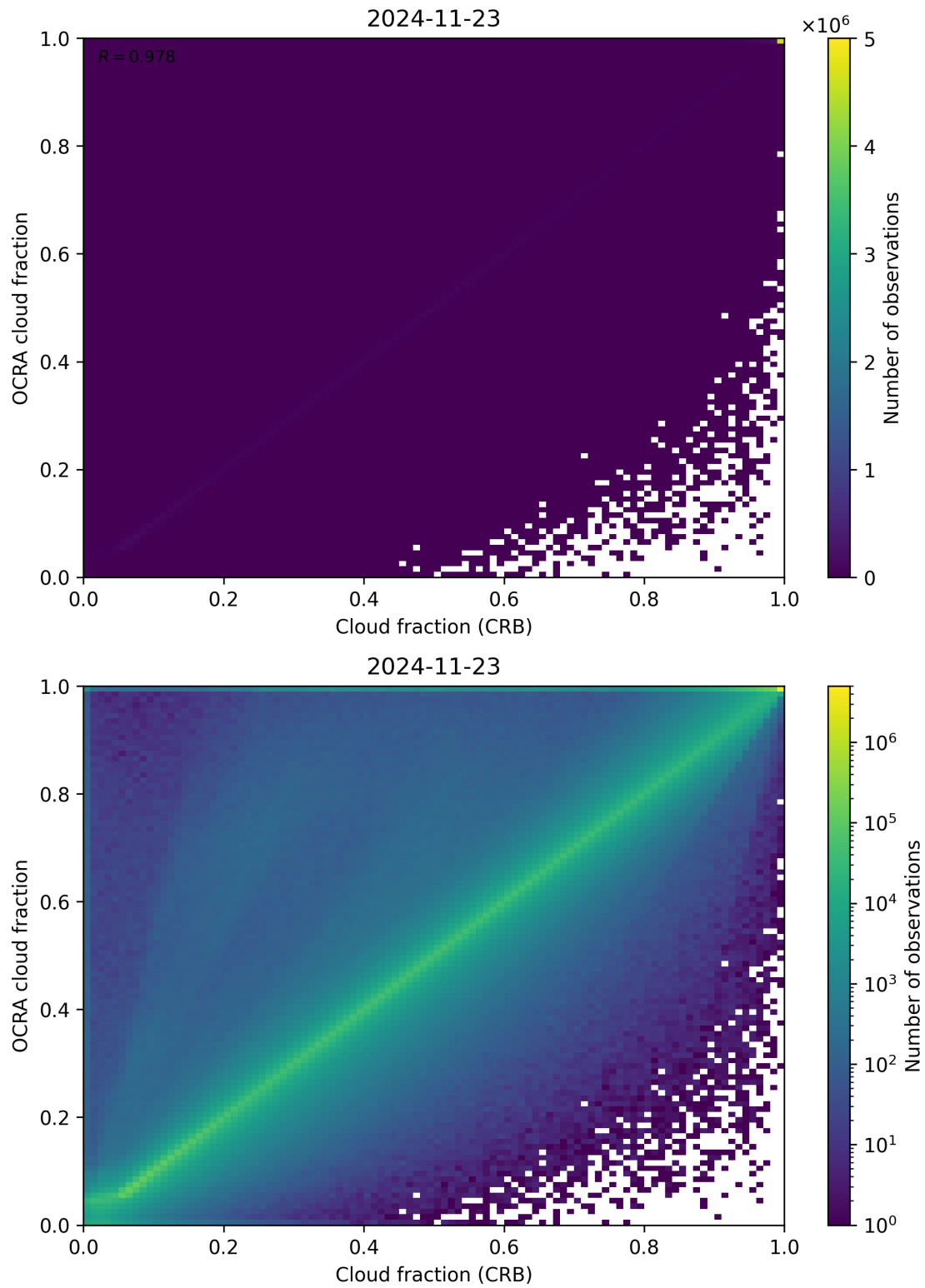
Figure 78: Scatter density plot of “Cloud fraction (CRB)” against “OCRA cloud fraction” for 2024-11-22 to 2024-11-24.
