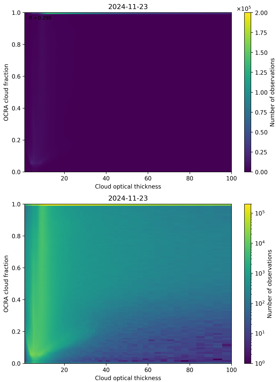
Figure 83: Scatter density plot of “Cloud optical thickness” against “OCRA cloud fraction” for 2024-11-22 to 2024-11-24.
