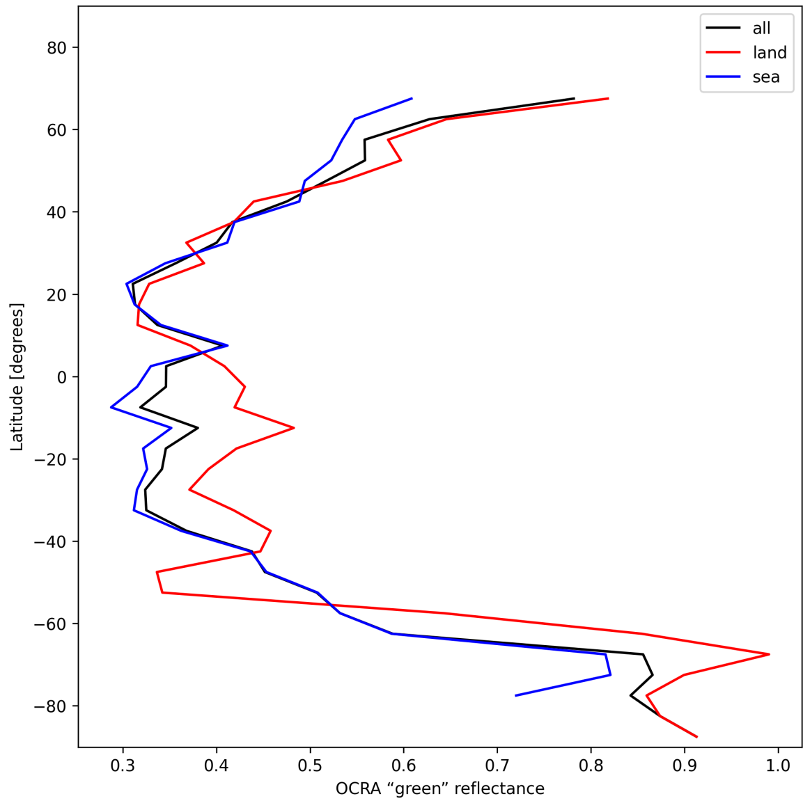
Figure 36: Zonal average of “OCRA “green” reflectance” for 2024-11-22 to 2024-11-24.
