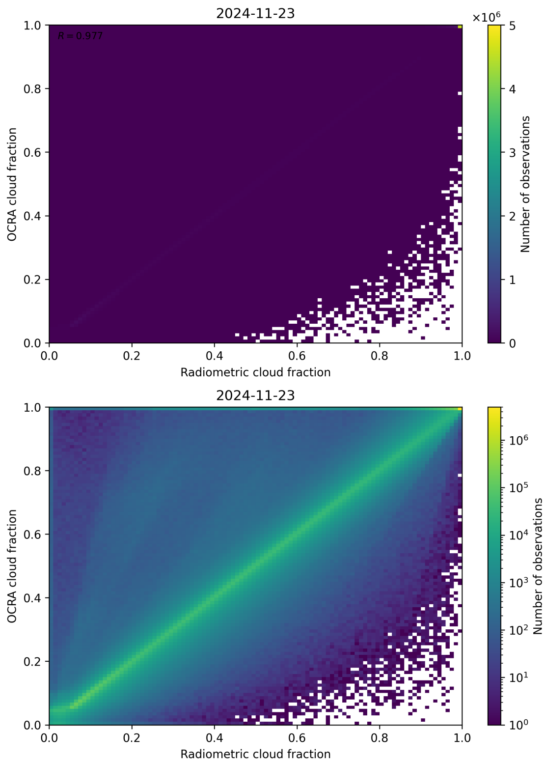
Figure 72: Scatter density plot of “Radiometric cloud fraction” against “OCRA cloud fraction” for 2024-11-22 to 2024-11-24.
