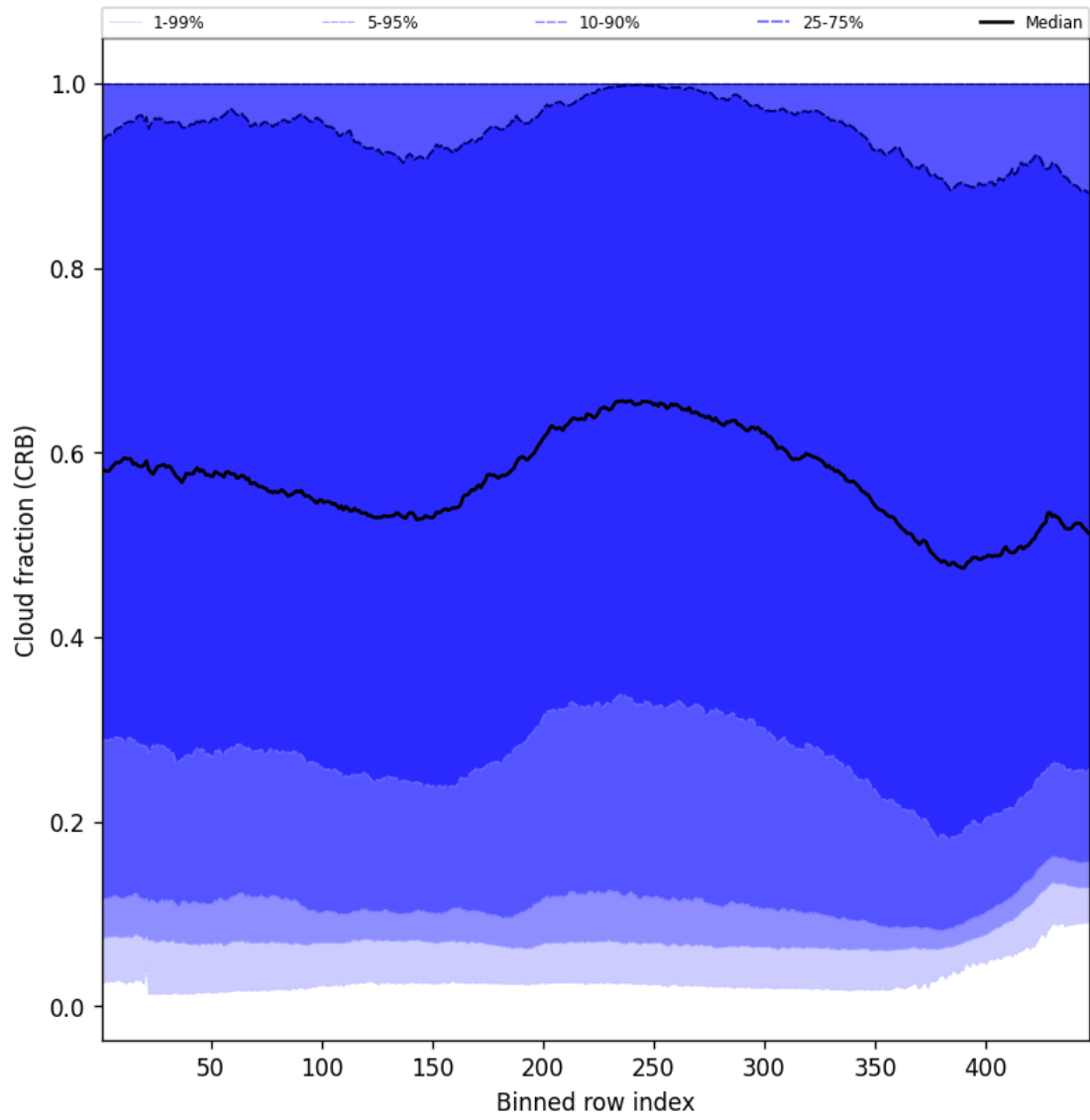
Figure 58: Along track statistics of “Cloud fraction (CRB)” for 2024-11-22 to 2024-11-24
