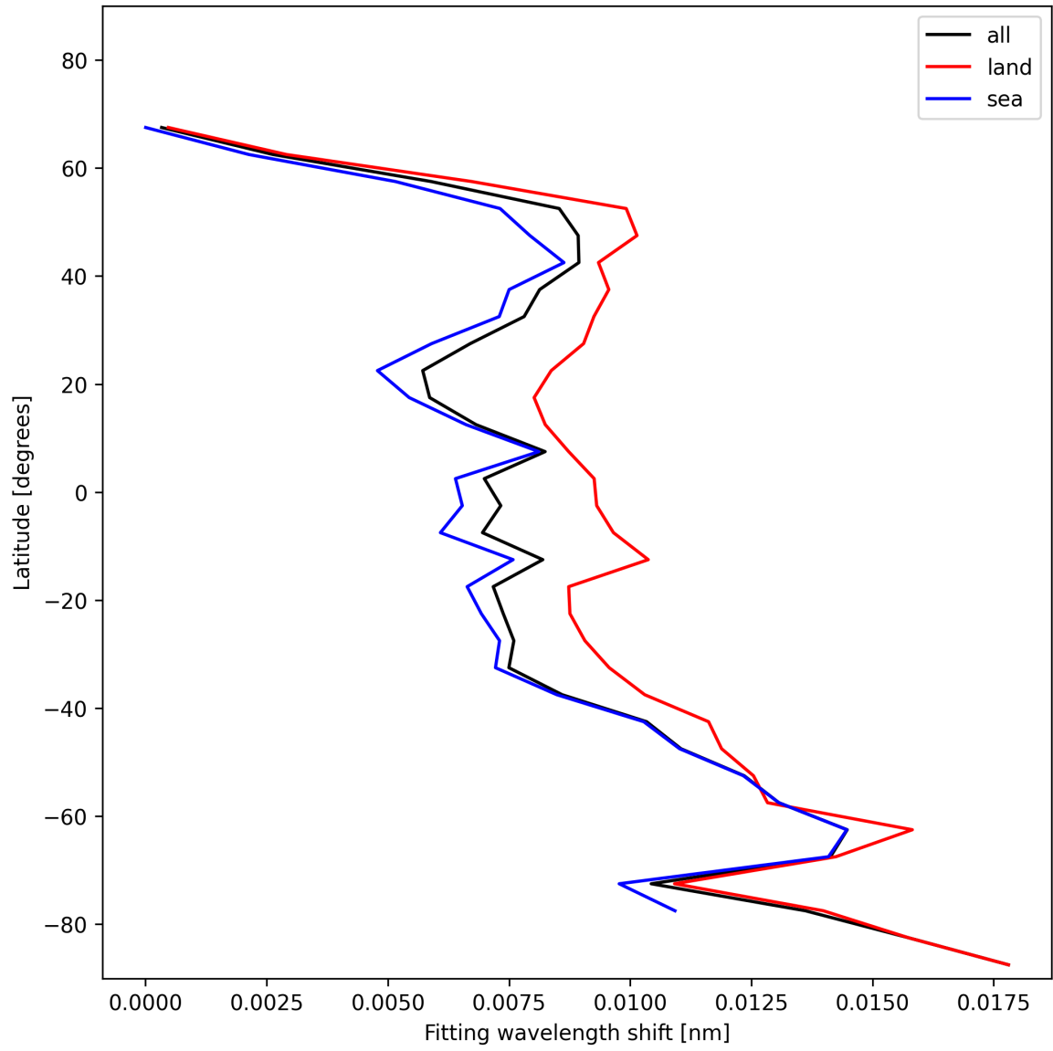
Figure 33: Zonal average of “Fitting wavelength shift” for 2024-11-22 to 2024-11-24.
