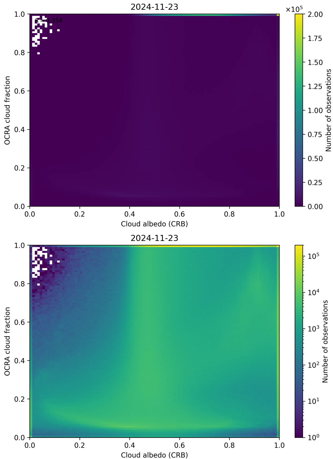
Figure 70: Scatter density plot of “Cloud albedo (CRB)” against “OCRA cloud fraction” for 2024-11-22 to 2024-11-24.
