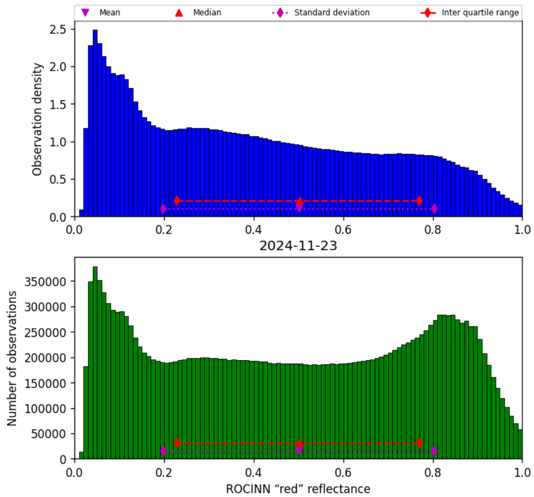
Figure 53: Histogram of “ROCINN “red” reflectance” for 2024-11-22 to 2024-11-24
