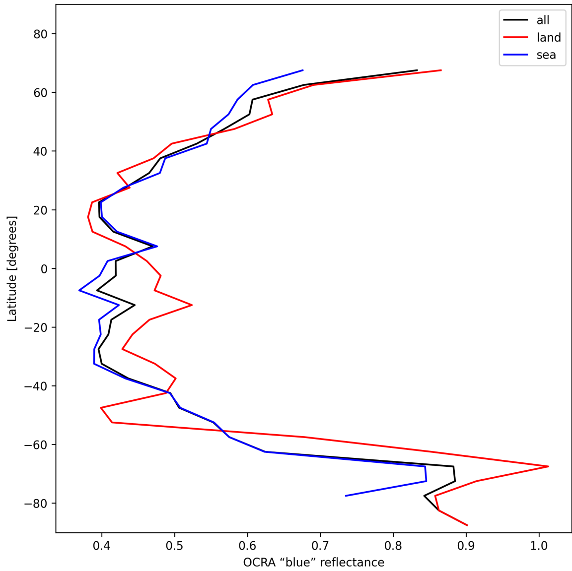
Figure 35: Zonal average of “OCRA “blue” reflectance” for 2024-11-22 to 2024-11-24.
