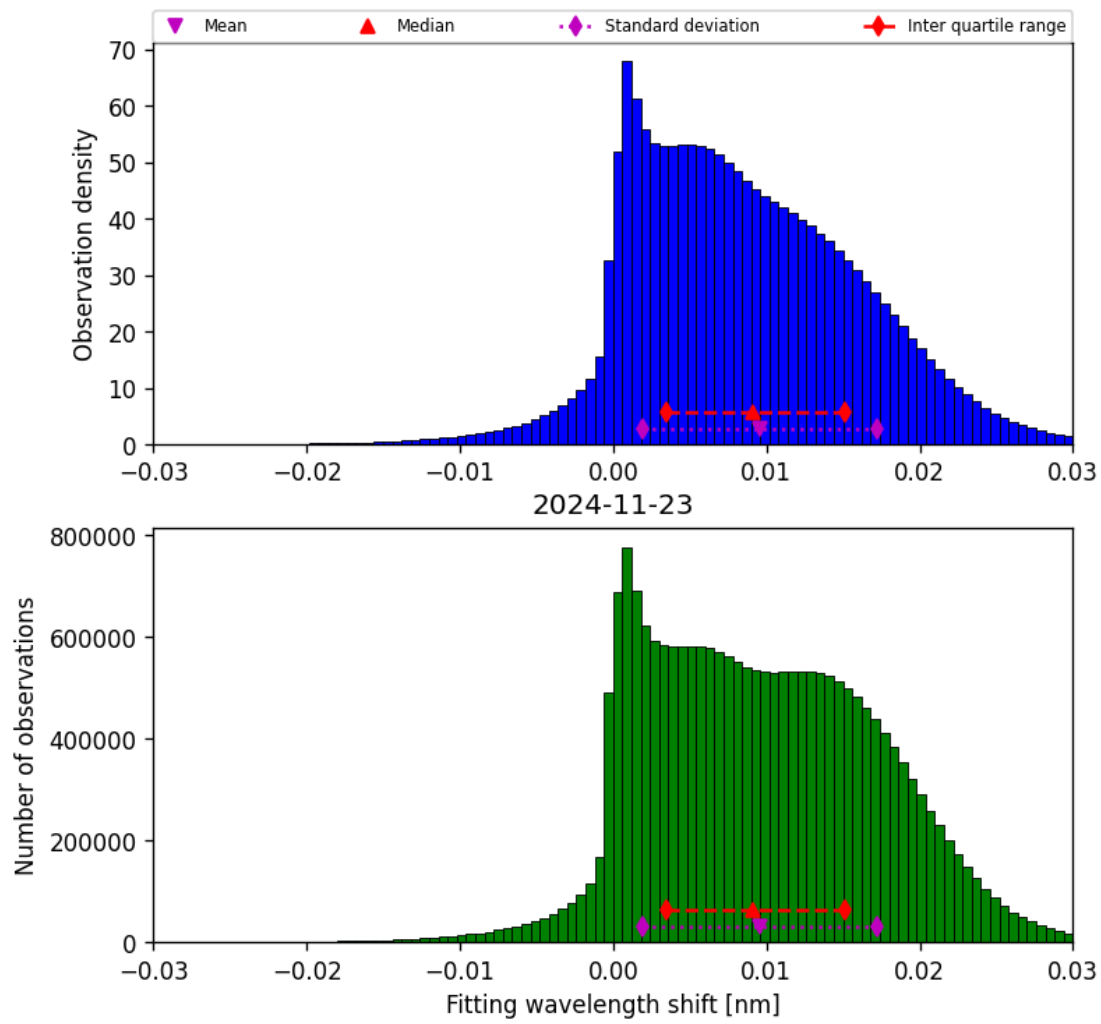
Figure 49: Histogram of “Fitting wavelength shift” for 2024-11-22 to 2024-11-24
