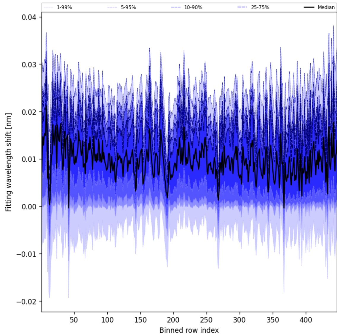
Figure 65: Along track statistics of “Fitting wavelength shift” for 2024-11-22 to 2024-11-24
