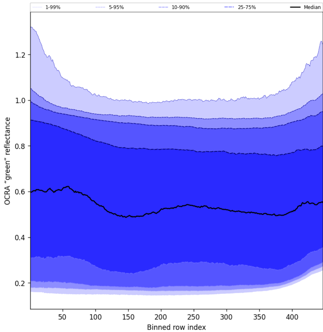
Figure 68: Along track statistics of “OCRA “green” reflectance” for 2024-11-22 to 2024-11-24
