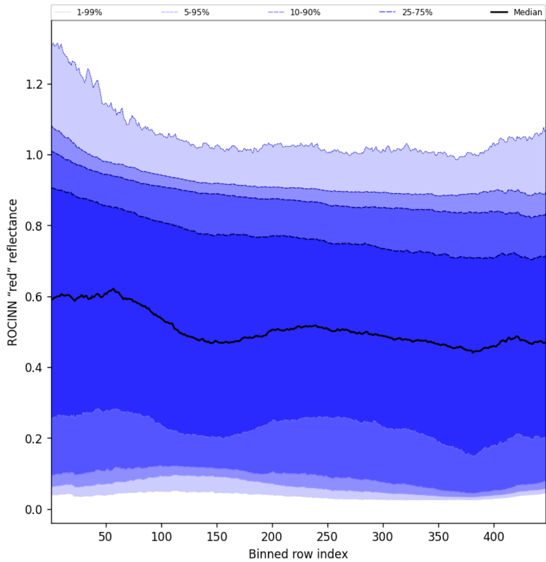
Figure 69: Along track statistics of “ROCINN “red” reflectance” for 2024-11-22 to 2024-11-24
