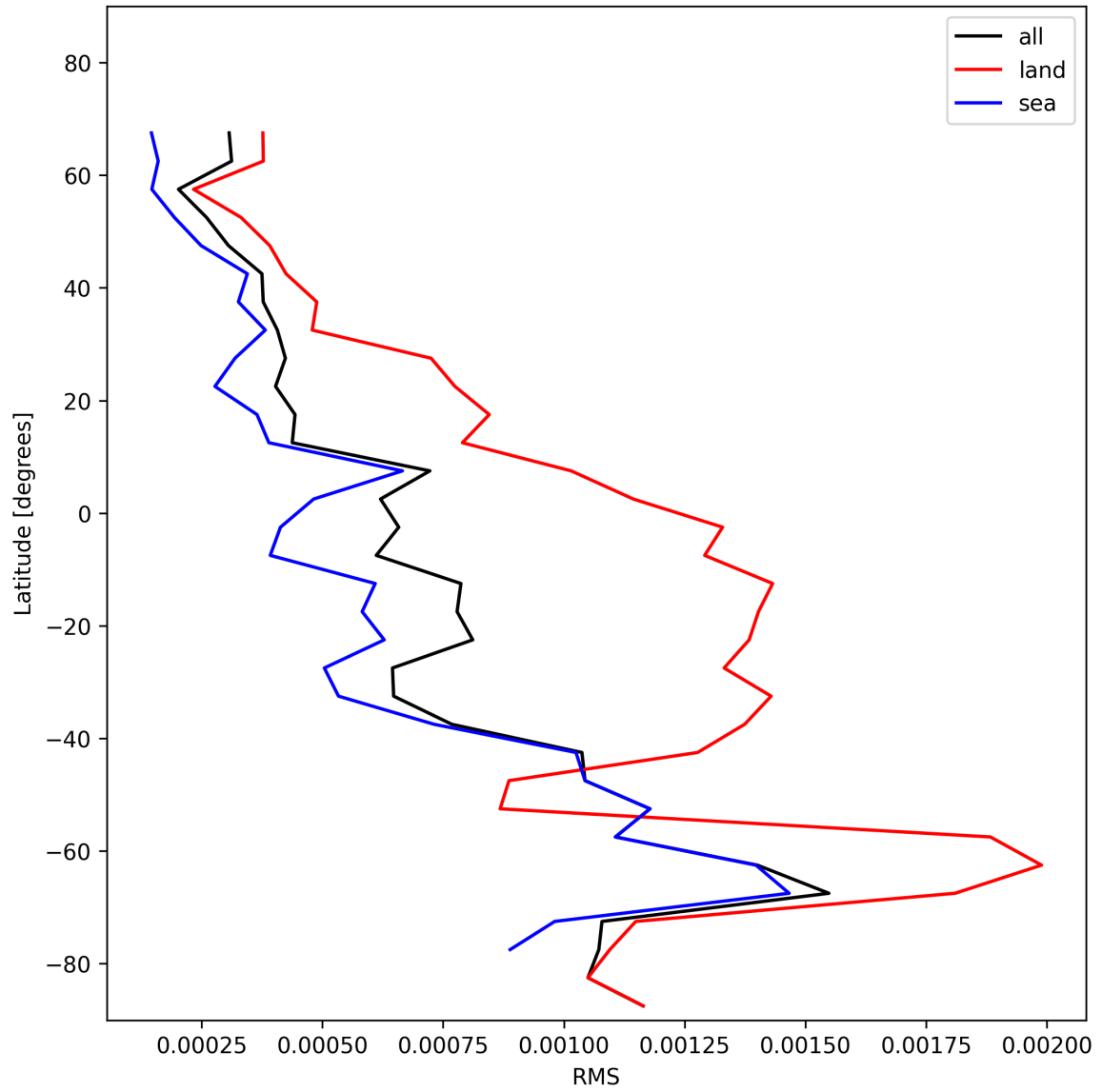
Figure 31: Zonal average of “RMS” for 2024-11-22 to 2024-11-24.
