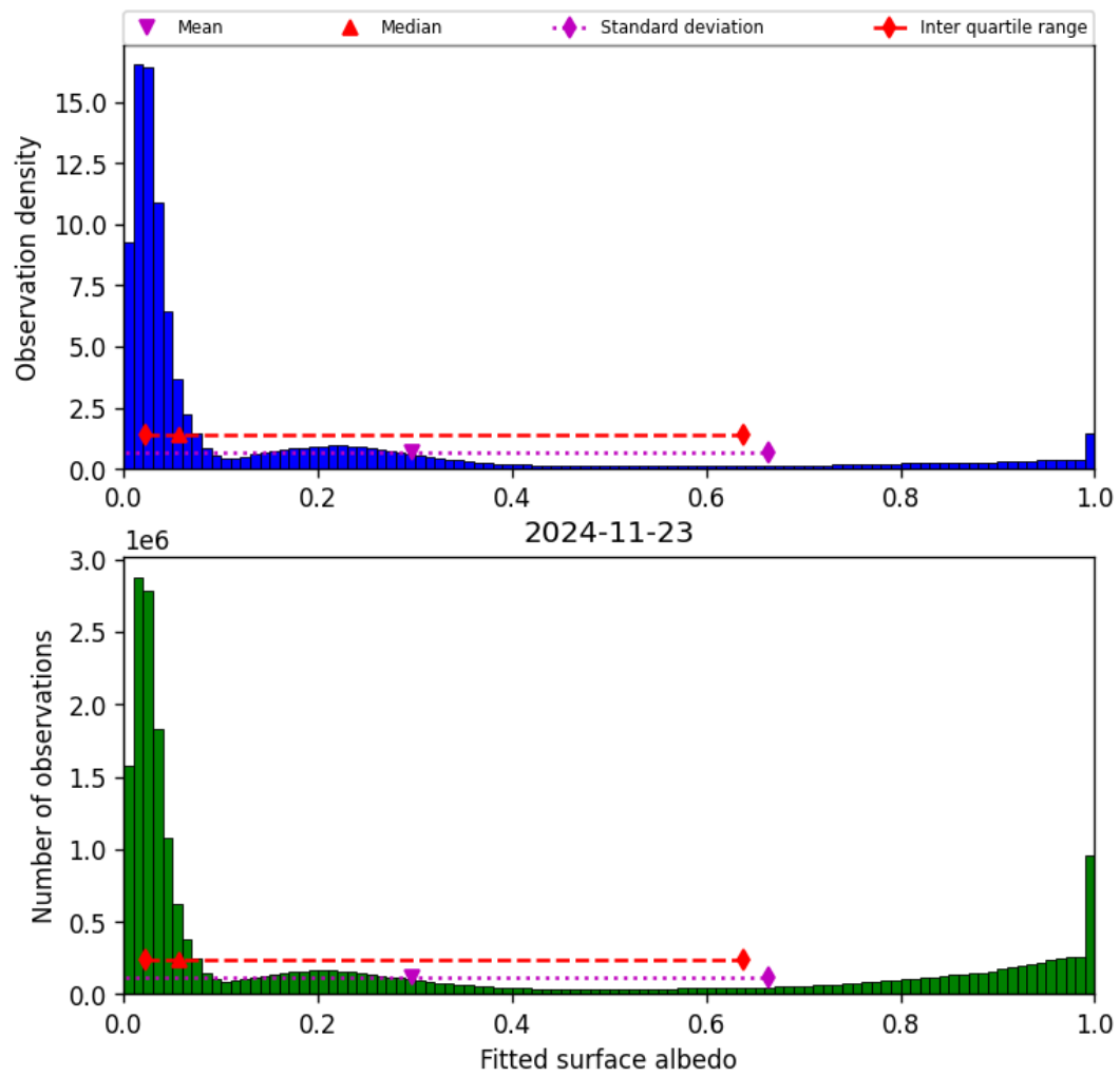
Figure 45: Histogram of “Fitted surface albedo” for 2024-11-22 to 2024-11-24
