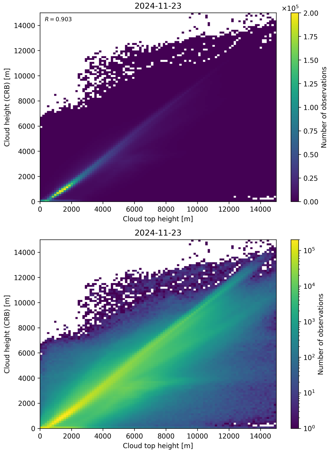
Figure 89: Scatter density plot of “Cloud top height” against “Cloud height (CRB)” for 2024-11-22 to 2024-11-24.
