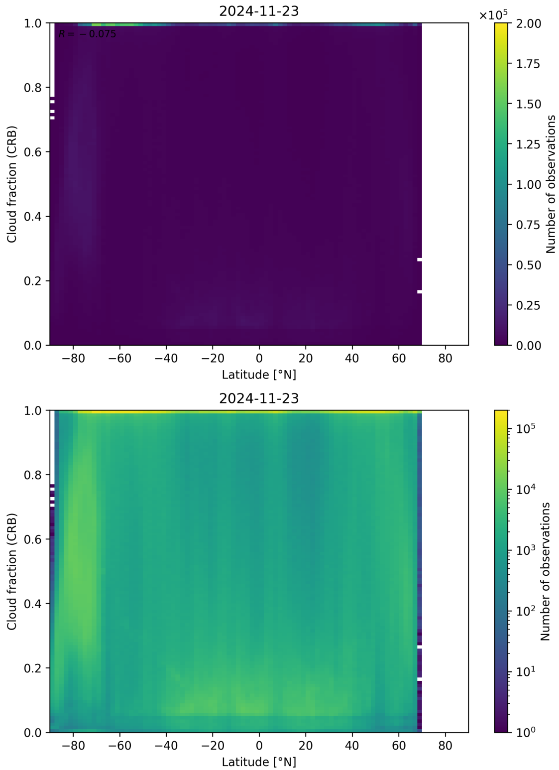
Figure 94: Scatter density plot of “Latitude” against “Cloud fraction (CRB)” for 2024-11-22 to 2024-11-24.
