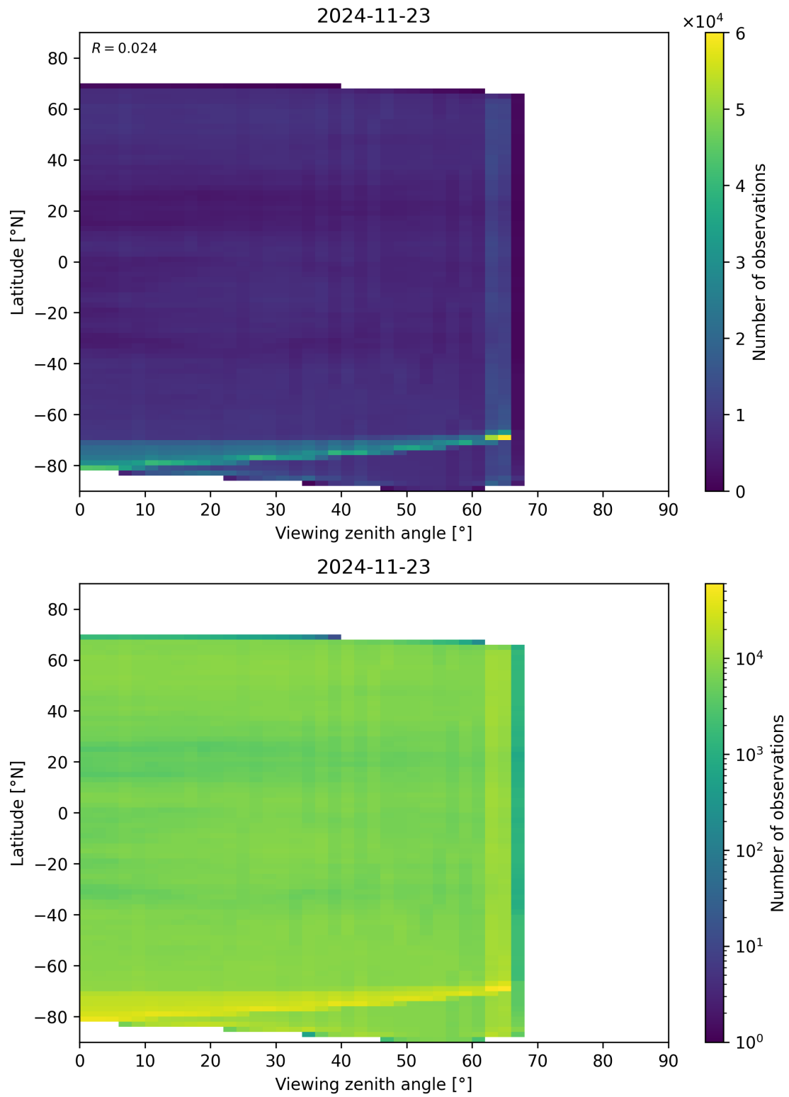
Figure 113: Scatter density plot of “Viewing zenith angle” against “Latitude” for 2024-11-22 to 2024-11-24.
