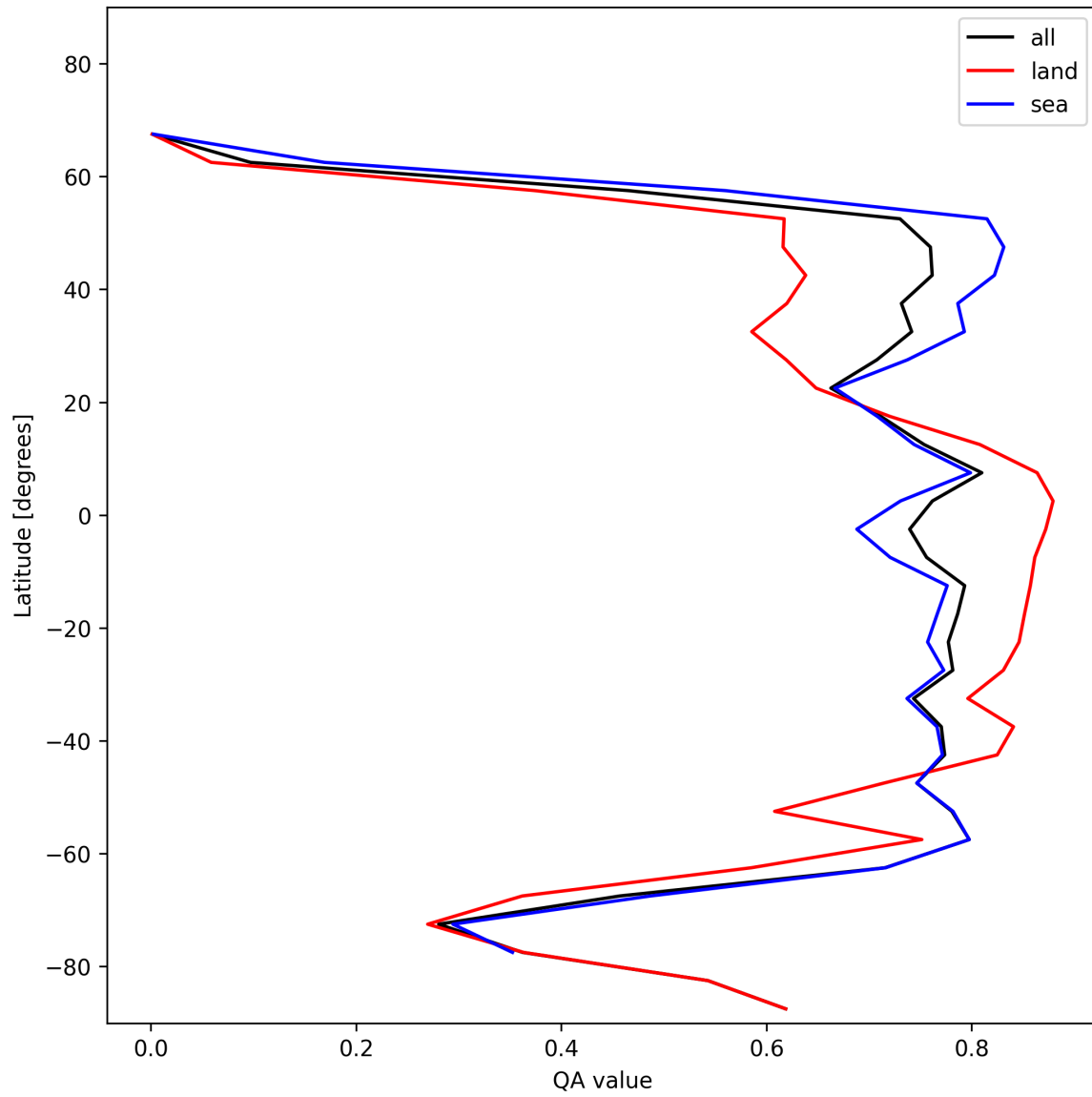
Figure 22: Zonal average of “QA value” for 2024-11-22 to 2024-11-24.
