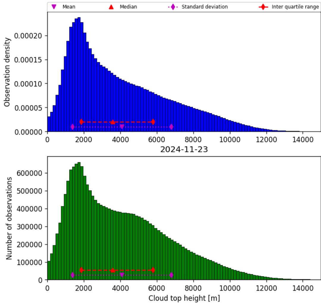
Figure 40: Histogram of “Cloud top height” for 2024-11-22 to 2024-11-24
