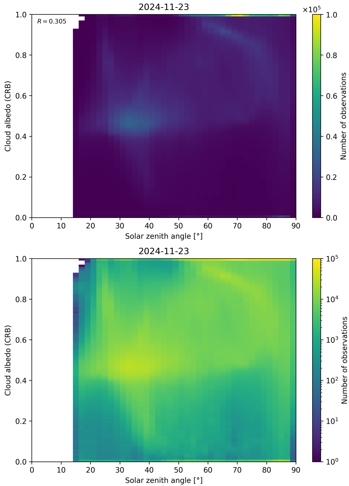
Figure 98: Scatter density plot of “Solar zenith angle” against “Cloud albedo (CRB)” for 2024-11-22 to 2024-11-24.
