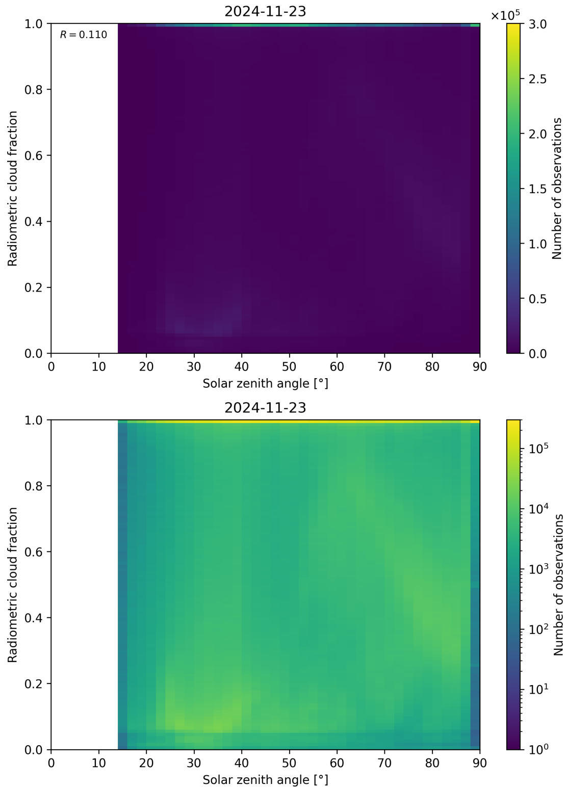
Figure 99: Scatter density plot of “Solar zenith angle” against “Radiometric cloud fraction” for 2024-11-22 to 2024-11-24.
