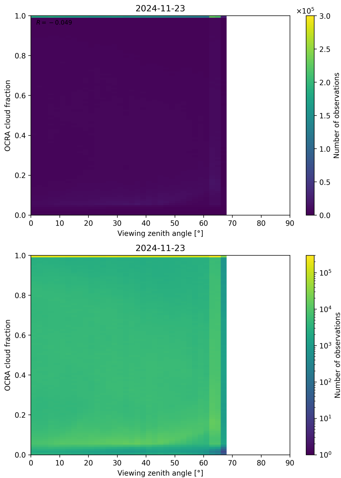
Figure 108: Scatter density plot of “Viewing zenith angle” against “OCRA cloud fraction” for 2024-11-22 to 2024-11-24.
