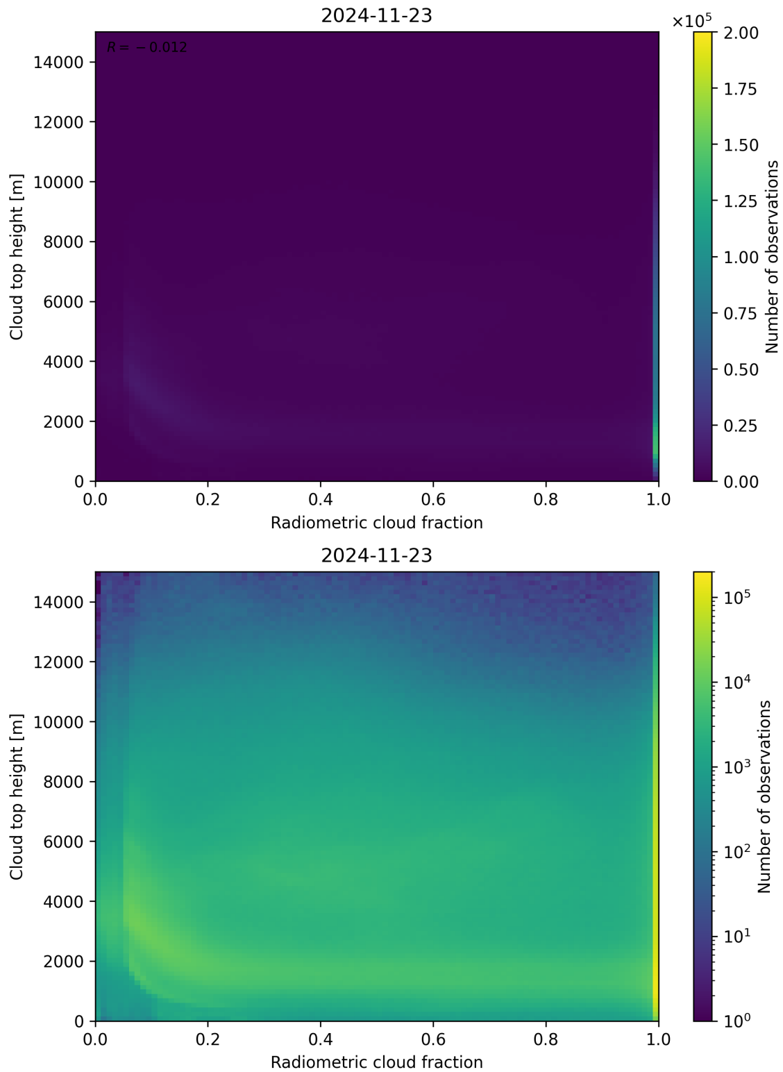
Figure 76: Scatter density plot of “Radiometric cloud fraction” against “Cloud top height” for 2024-11-22 to 2024-11-24.
