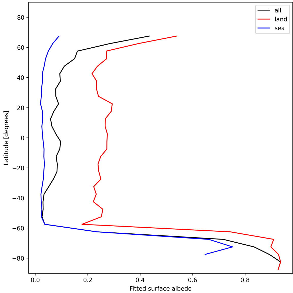
Figure 29: Zonal average of “Fitted surface albedo” for 2024-11-22 to 2024-11-24.
