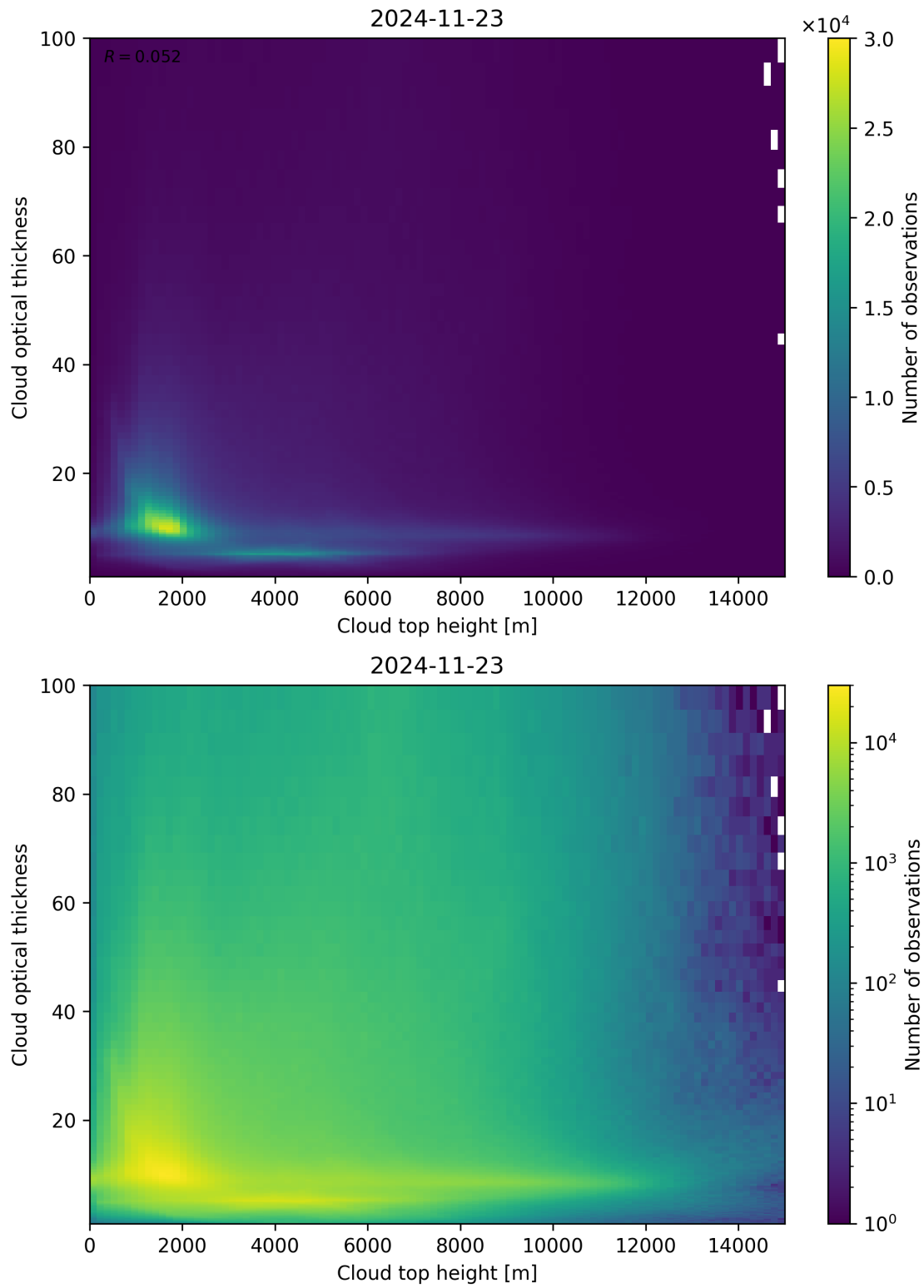
Figure 90: Scatter density plot of “Cloud top height” against “Cloud optical thickness” for 2024-11-22 to 2024-11-24.
