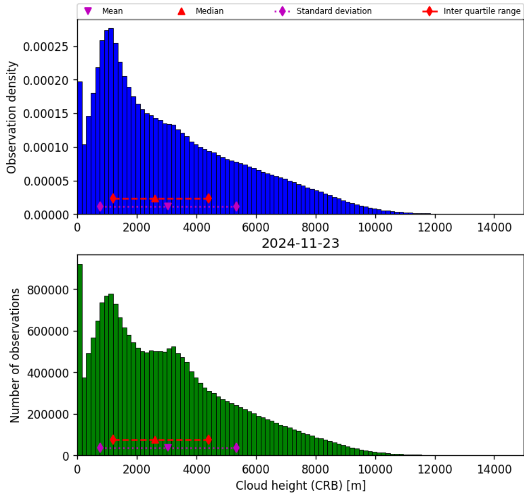
Figure 43: Histogram of “Cloud height (CRB)” for 2024-11-22 to 2024-11-24
