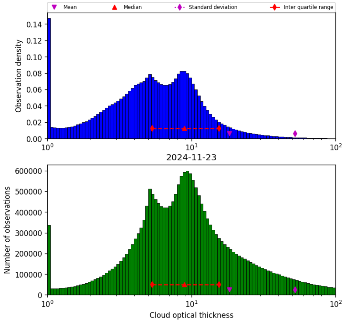
Figure 41: Histogram of “Cloud optical thickness” for 2024-11-22 to 2024-11-24
