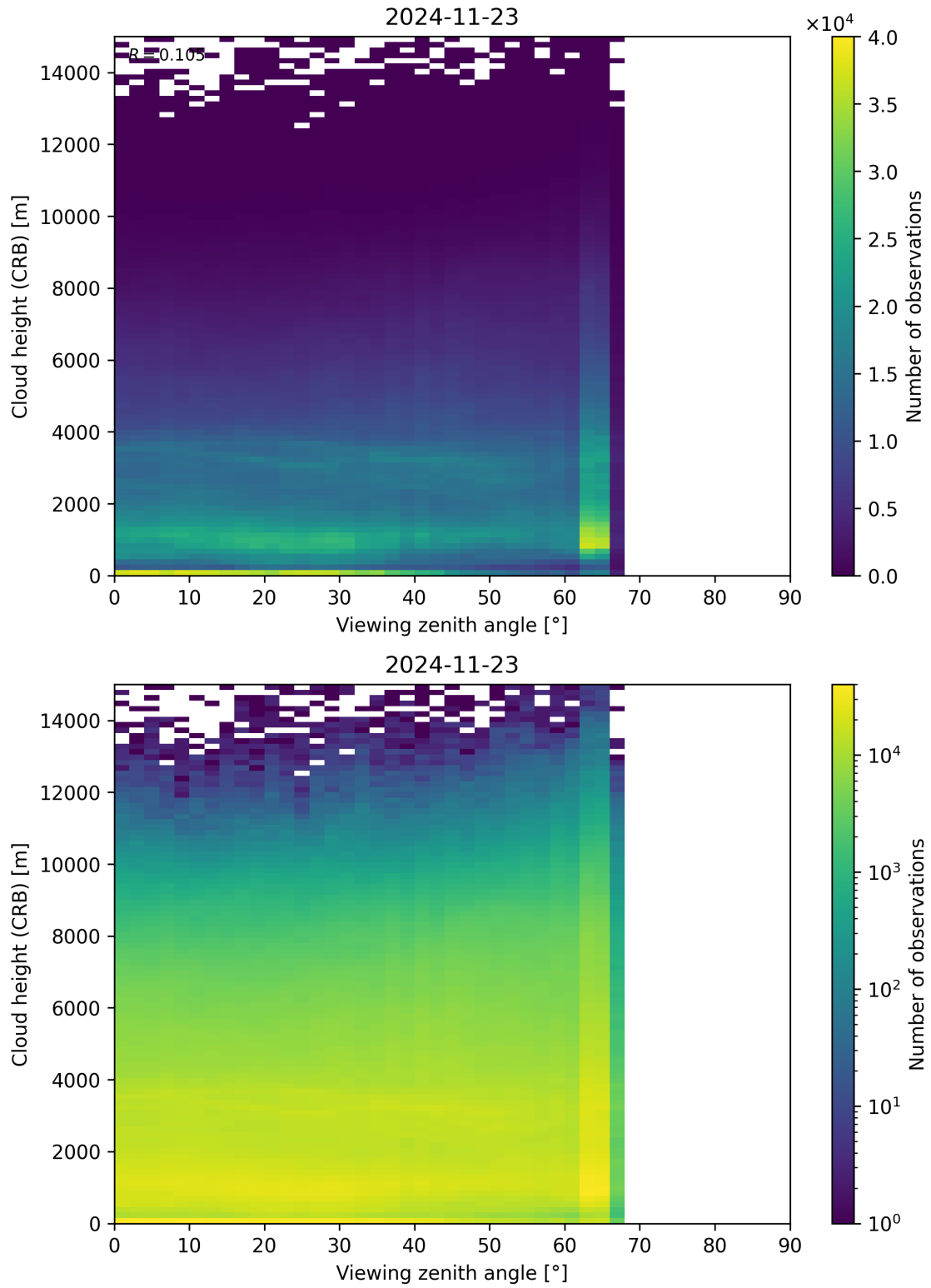
Figure 110: Scatter density plot of “Viewing zenith angle” against “Cloud height (CRB)” for 2024-11-22 to 2024-11-24.
