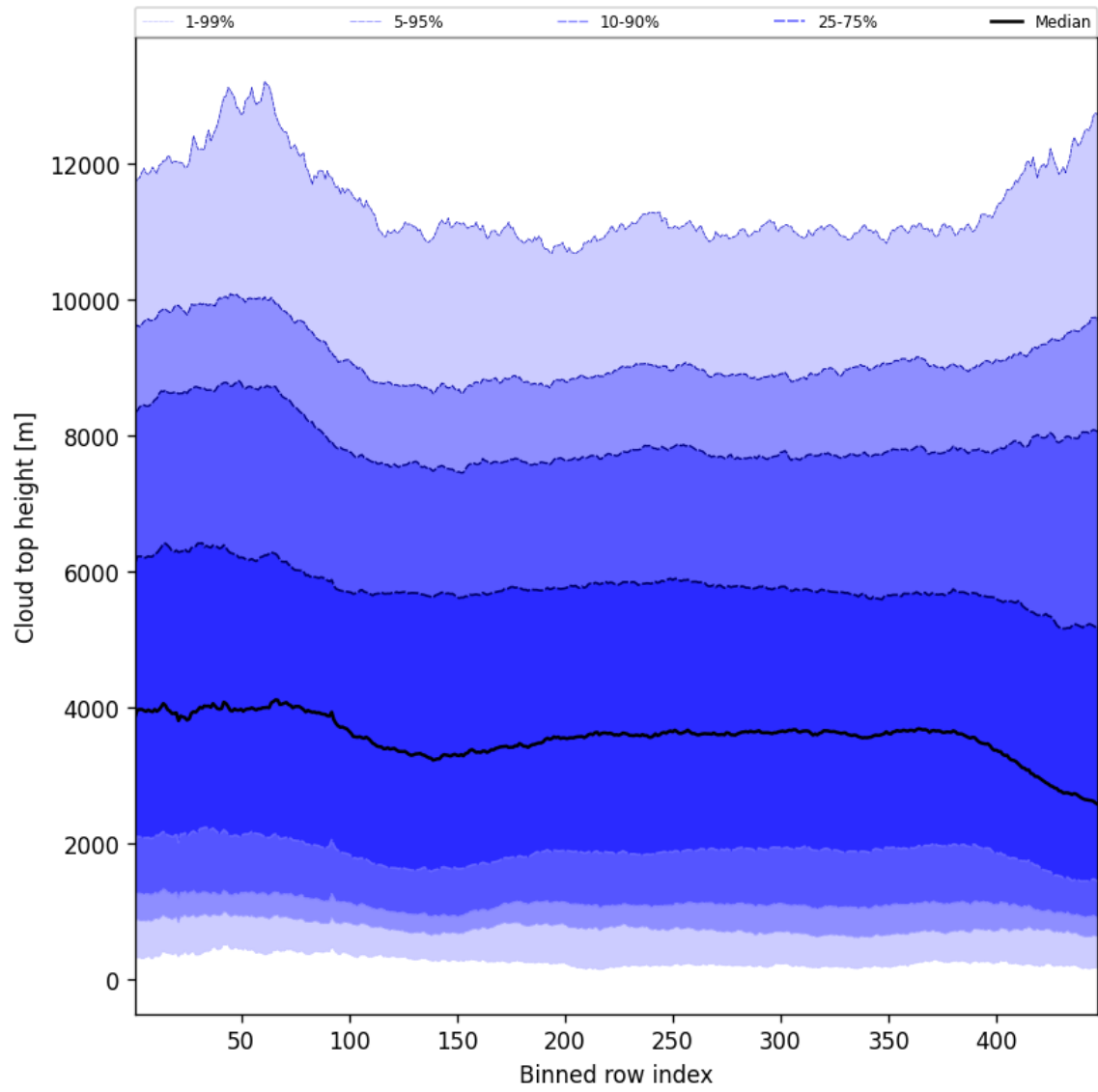
Figure 56: Along track statistics of “Cloud top height” for 2024-11-22 to 2024-11-24
