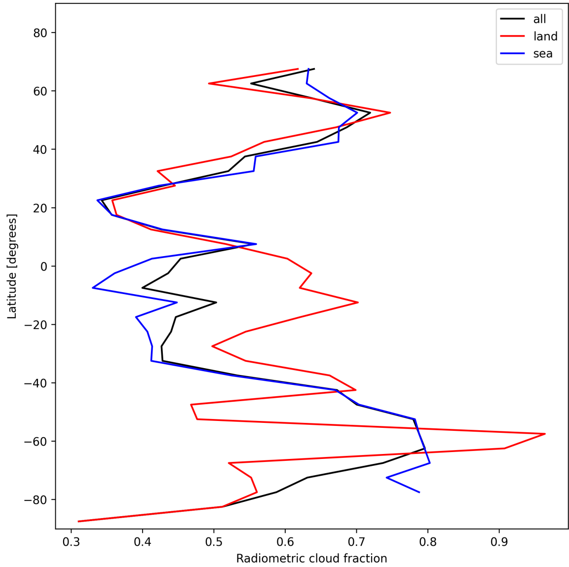
Figure 23: Zonal average of “Radiometric cloud fraction” for 2024-11-22 to 2024-11-24.
