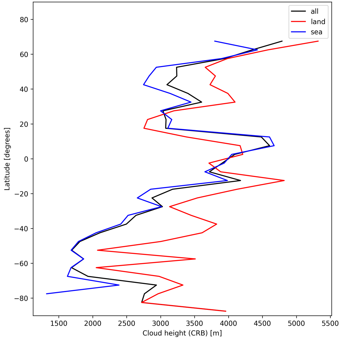
Figure 27: Zonal average of “Cloud height (CRB)” for 2024-11-22 to 2024-11-24.
