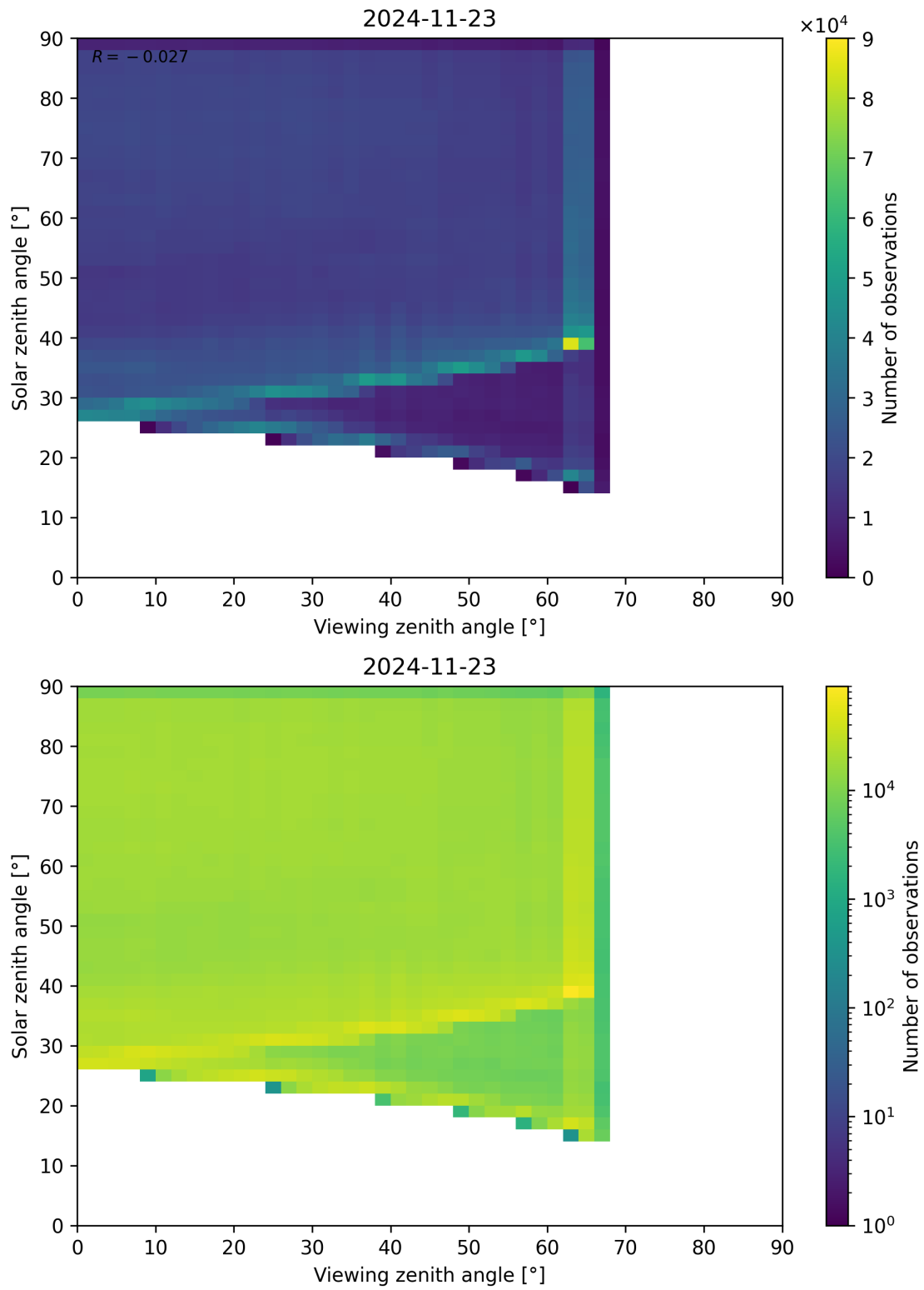
Figure 114: Scatter density plot of “Viewing zenith angle” against “Solar zenith angle” for 2024-11-22 to 2024-11-24.
