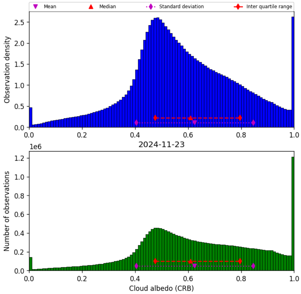
Figure 44: Histogram of “Cloud albedo (CRB)” for 2024-11-22 to 2024-11-24
