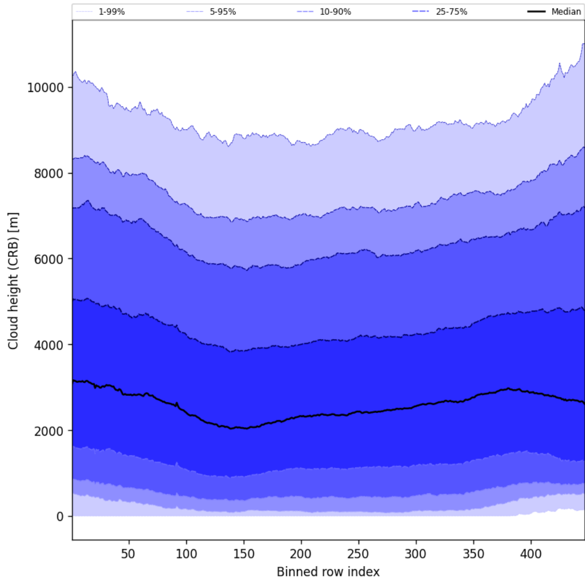
Figure 59: Along track statistics of “Cloud height (CRB)” for 2024-11-22 to 2024-11-24
