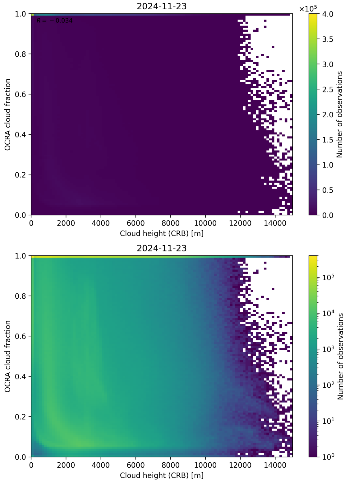
Figure 81: Scatter density plot of “Cloud height (CRB)” against “OCRA cloud fraction” for 2024-11-22 to 2024-11-24.
