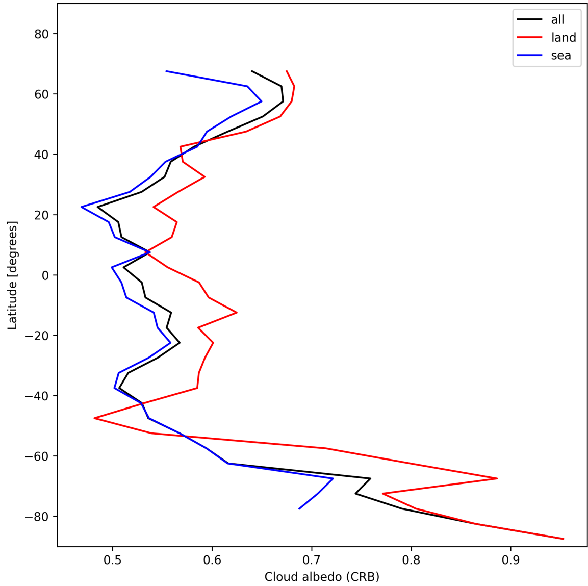
Figure 28: Zonal average of “Cloud albedo (CRB)” for 2024-11-22 to 2024-11-24.
