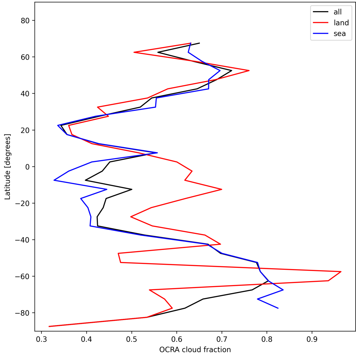
Figure 34: Zonal average of “OCRA cloud fraction” for 2024-11-22 to 2024-11-24.
