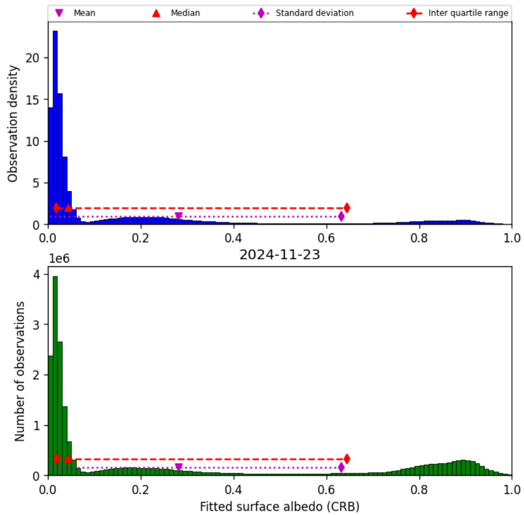
Figure 46: Histogram of “Fitted surface albedo (CRB)” for 2024-11-22 to 2024-11-24
