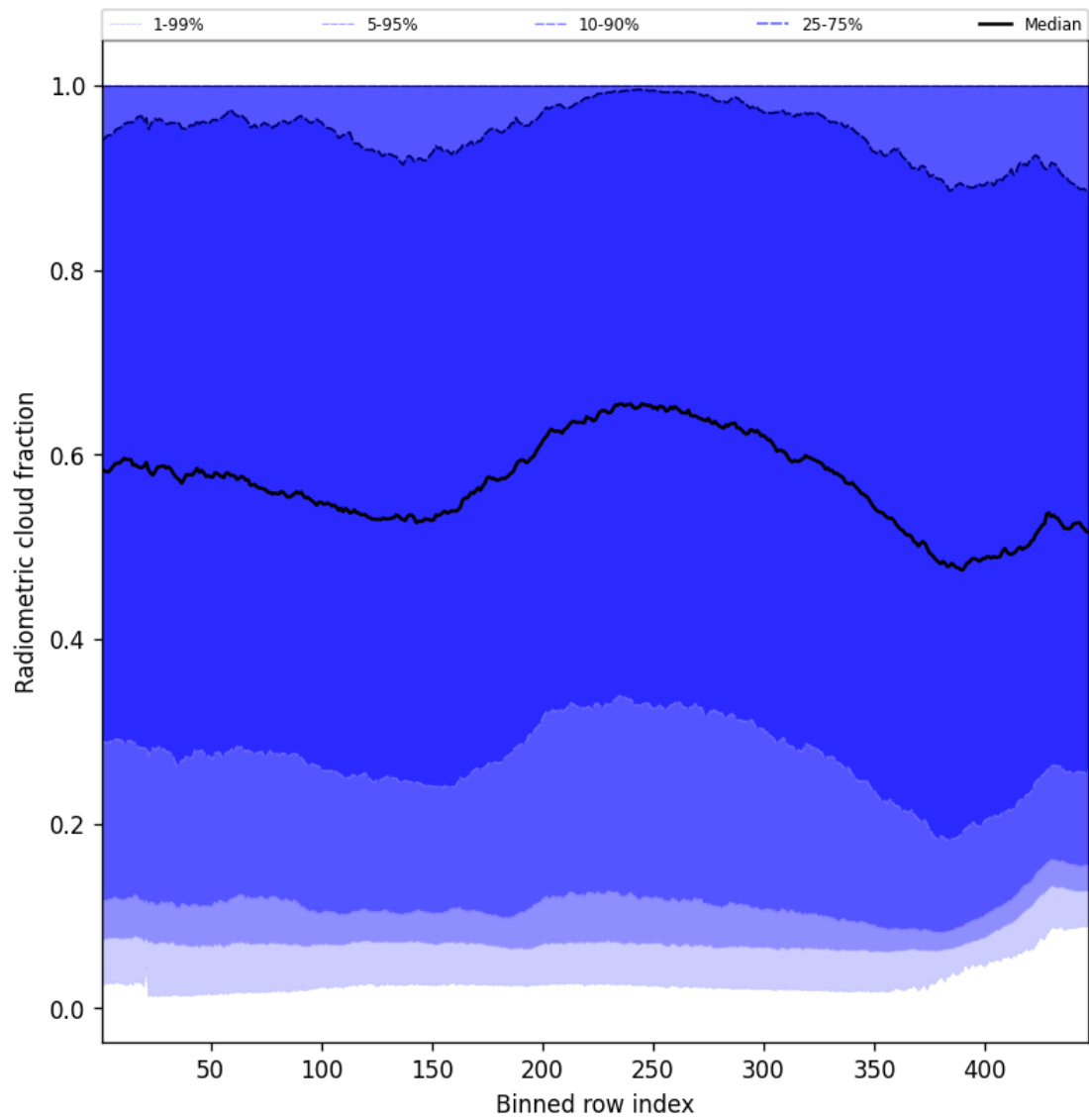
Figure 55: Along track statistics of “Radiometric cloud fraction” for 2024-11-22 to 2024-11-24
