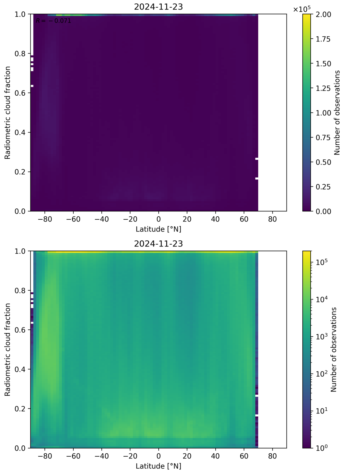
Figure 92: Scatter density plot of “Latitude” against “Radiometric cloud fraction” for 2024-11-22 to 2024-11-24.
