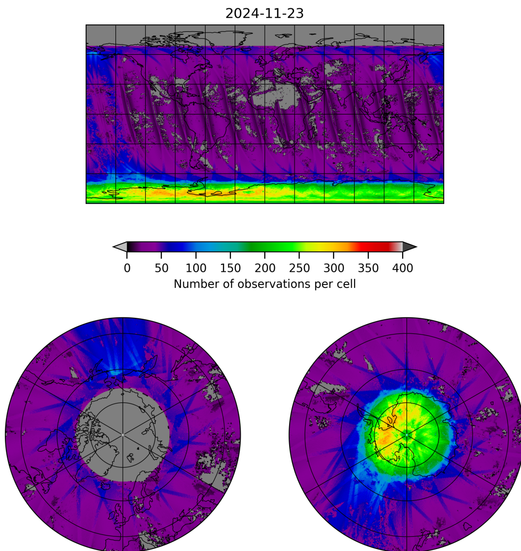
Figure 21: Map of the number of observations for 2024-11-22 to 2024-11-24
