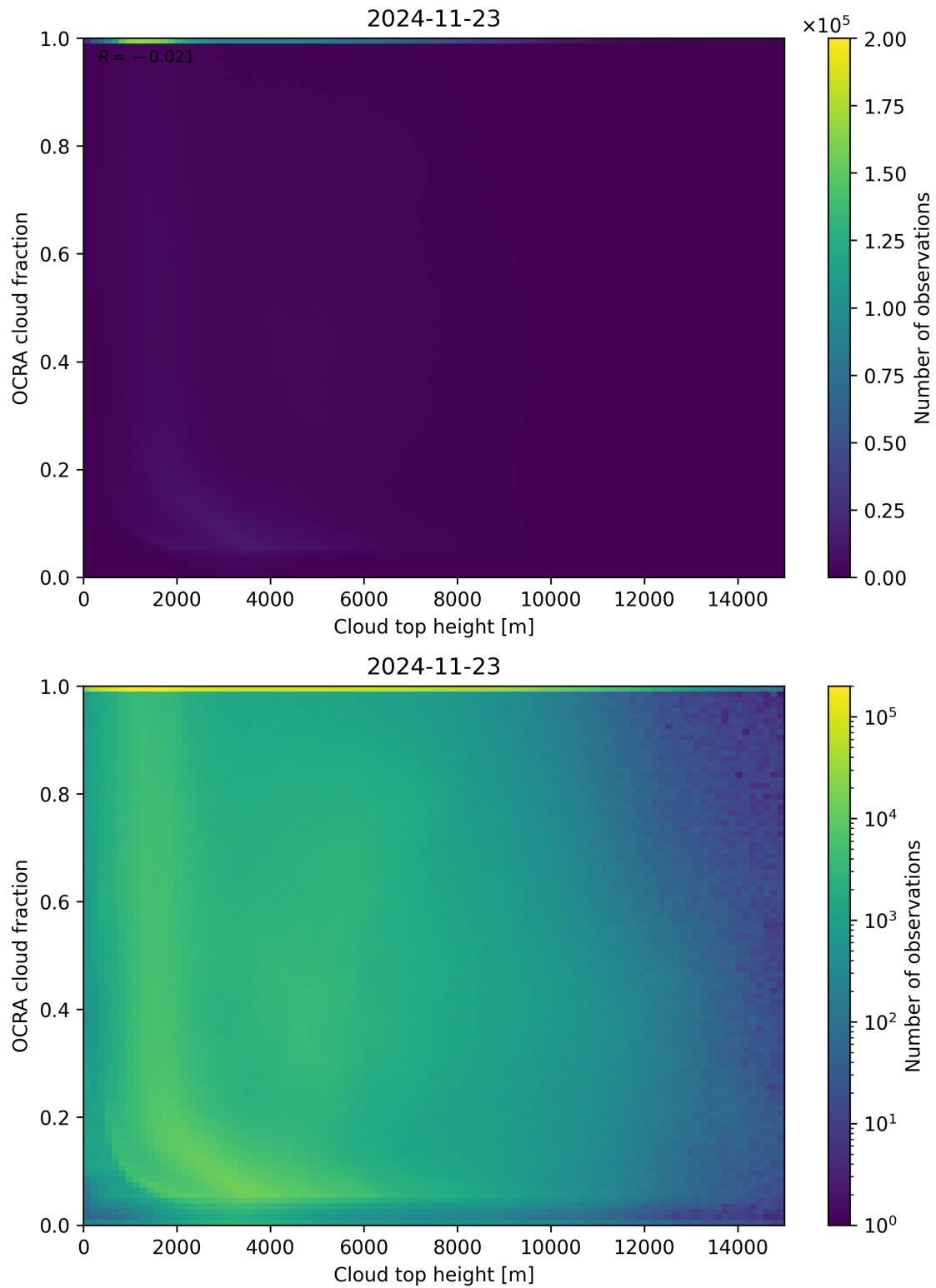
Figure 87: Scatter density plot of “Cloud top height” against “OCRA cloud fraction” for 2024-11-22 to 2024-11-24.
