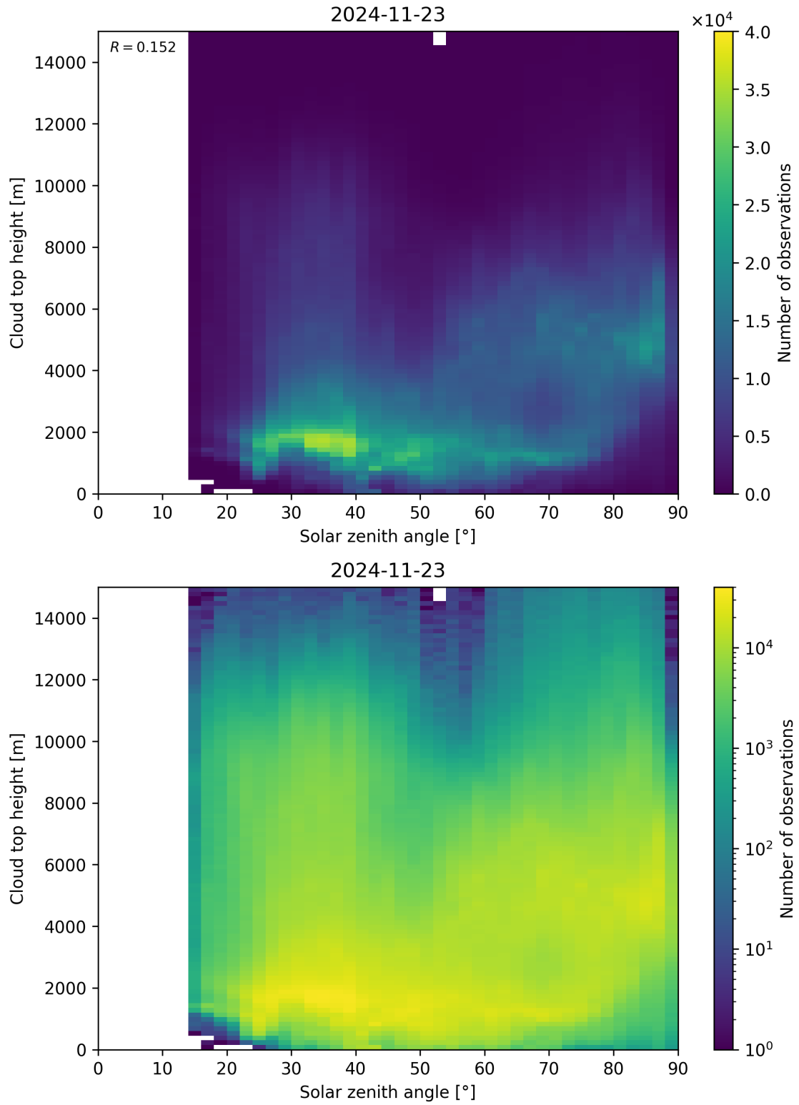
Figure 104: Scatter density plot of “Solar zenith angle” against “Cloud top height” for 2024-11-22 to 2024-11-24.
