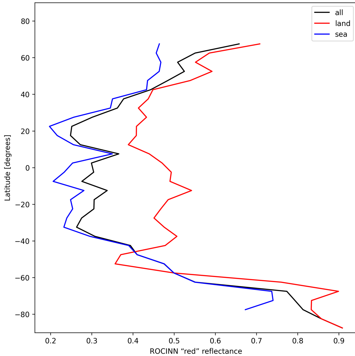
Figure 37: Zonal average of “ROCINN “red” reflectance” for 2024-11-22 to 2024-11-24.
