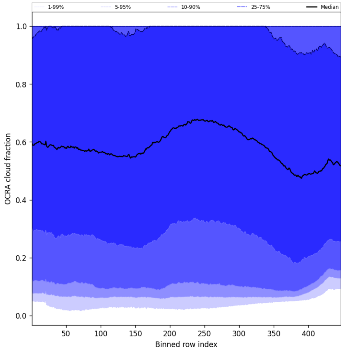
Figure 66: Along track statistics of “OCRA cloud fraction” for 2024-11-22 to 2024-11-24
