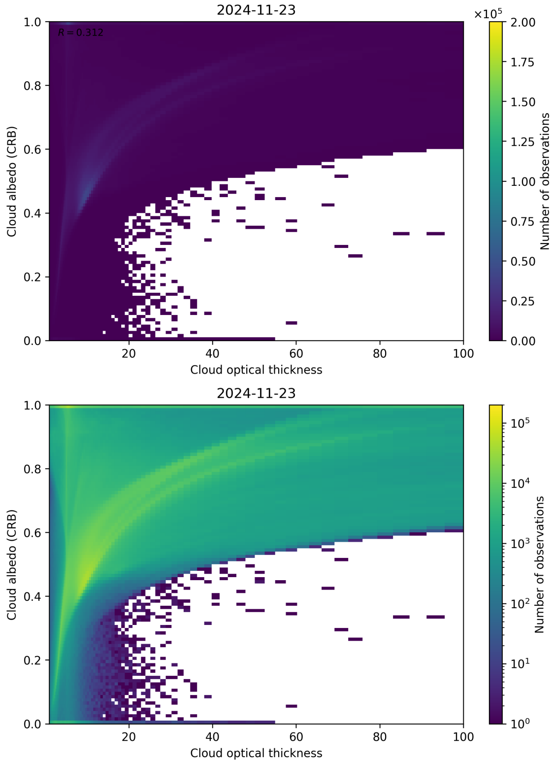
Figure 82: Scatter density plot of “Cloud optical thickness” against “Cloud albedo (CRB)” for 2024-11-22 to 2024-11-24.
