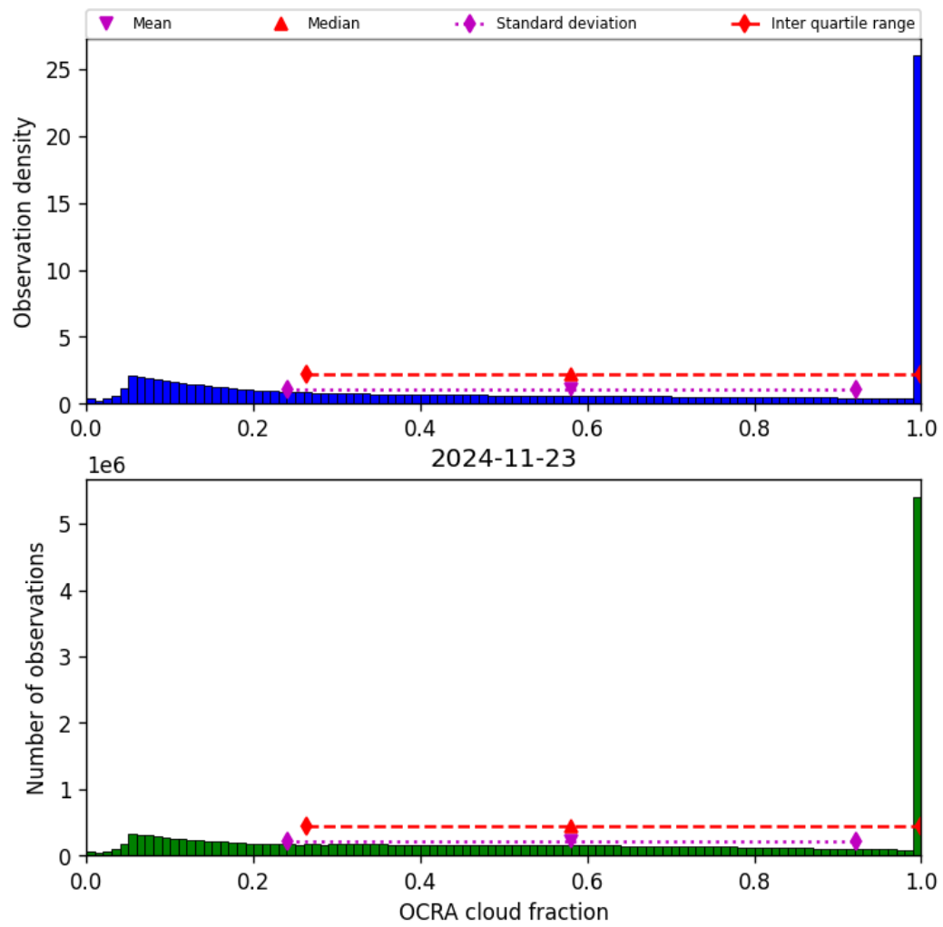
Figure 50: Histogram of “OCRA cloud fraction” for 2024-11-22 to 2024-11-24
