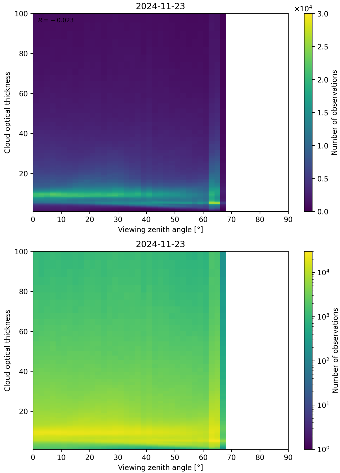
Figure 111: Scatter density plot of “Viewing zenith angle” against “Cloud optical thickness” for 2024-11-22 to 2024-11-24.
