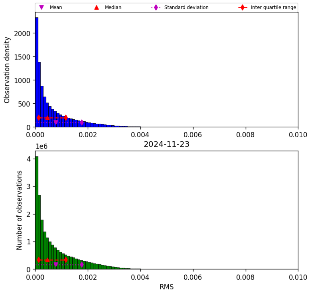
Figure 47: Histogram of “RMS” for 2024-11-22 to 2024-11-24
