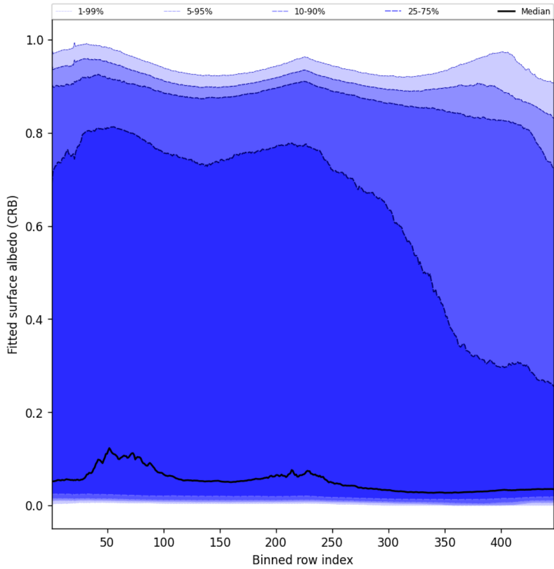
Figure 62: Along track statistics of “Fitted surface albedo (CRB)” for 2024-11-22 to 2024-11-24
