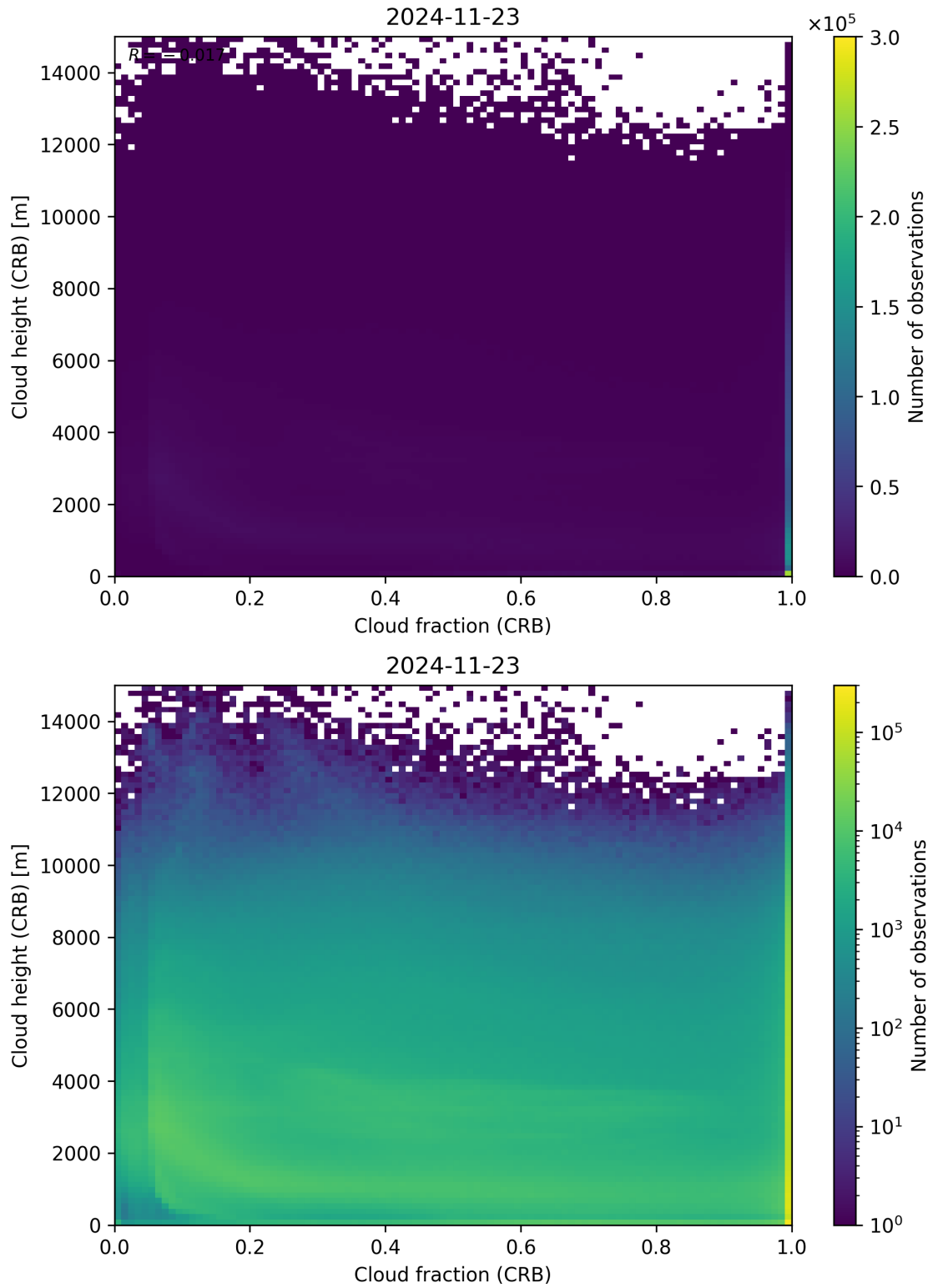
Figure 79: Scatter density plot of “Cloud fraction (CRB)” against “Cloud height (CRB)” for 2024-11-22 to 2024-11-24.
