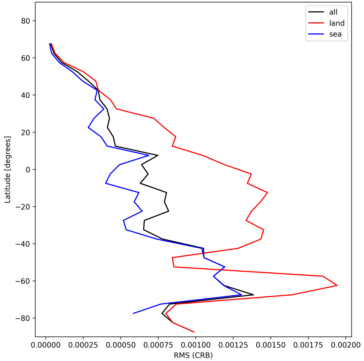
Figure 32: Zonal average of “RMS (CRB)” for 2024-11-22 to 2024-11-24.
