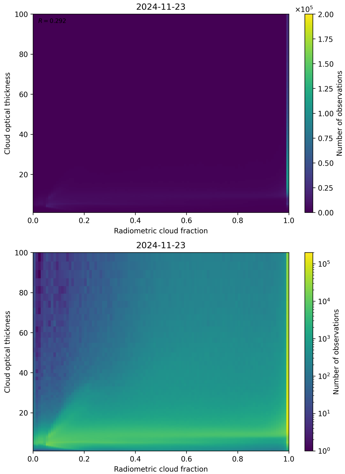
Figure 75: Scatter density plot of “Radiometric cloud fraction” against “Cloud optical thickness” for 2024-11-22 to 2024-11-24.
