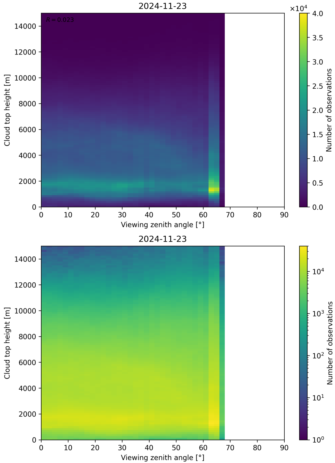
Figure 112: Scatter density plot of “Viewing zenith angle” against “Cloud top height” for 2024-11-22 to 2024-11-24.
