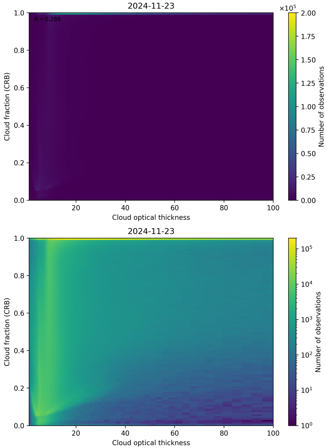
Figure 84: Scatter density plot of “Cloud optical thickness” against “Cloud fraction (CRB)” for 2024-11-22 to 2024-11-24.
