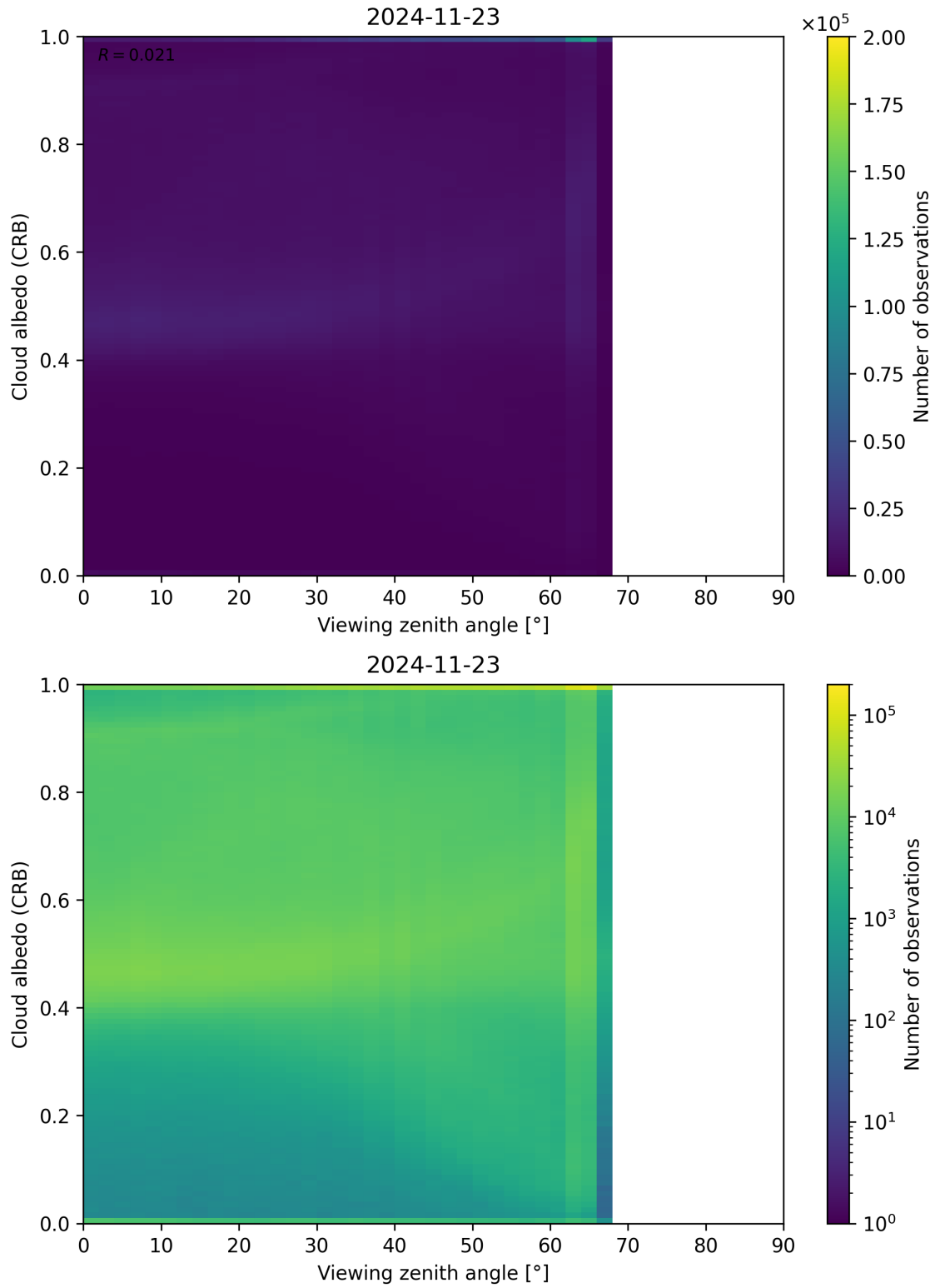
Figure 106: Scatter density plot of “Viewing zenith angle” against “Cloud albedo (CRB)” for 2024-11-22 to 2024-11-24.
