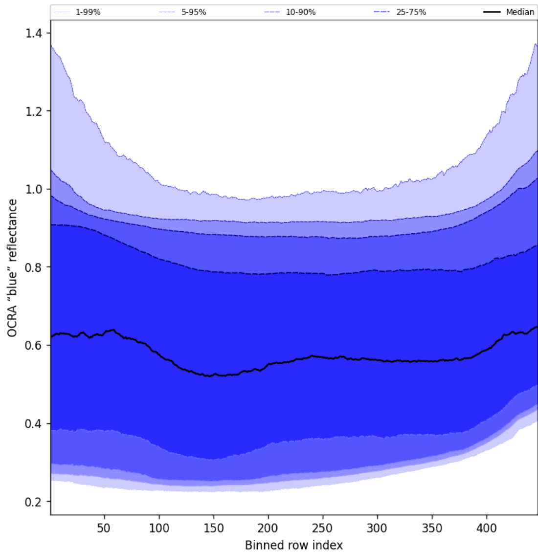
Figure 67: Along track statistics of “OCRA “blue” reflectance” for 2024-11-22 to 2024-11-24
