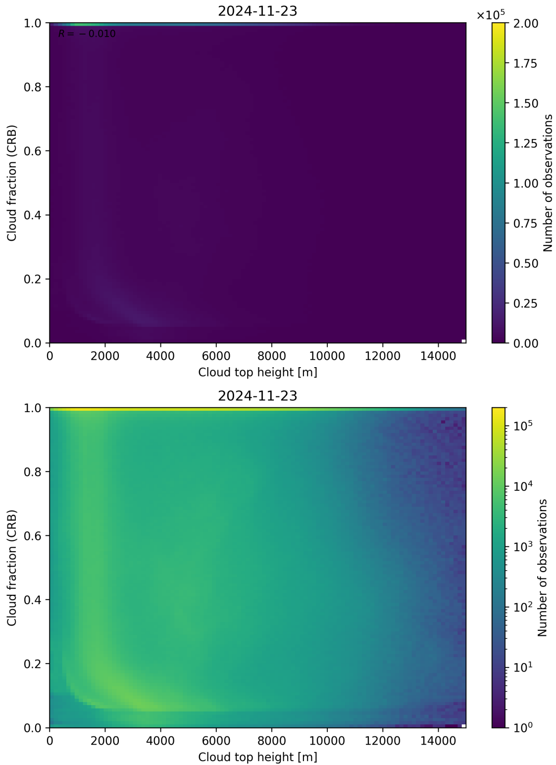
Figure 88: Scatter density plot of “Cloud top height” against “Cloud fraction (CRB)” for 2024-11-22 to 2024-11-24.
