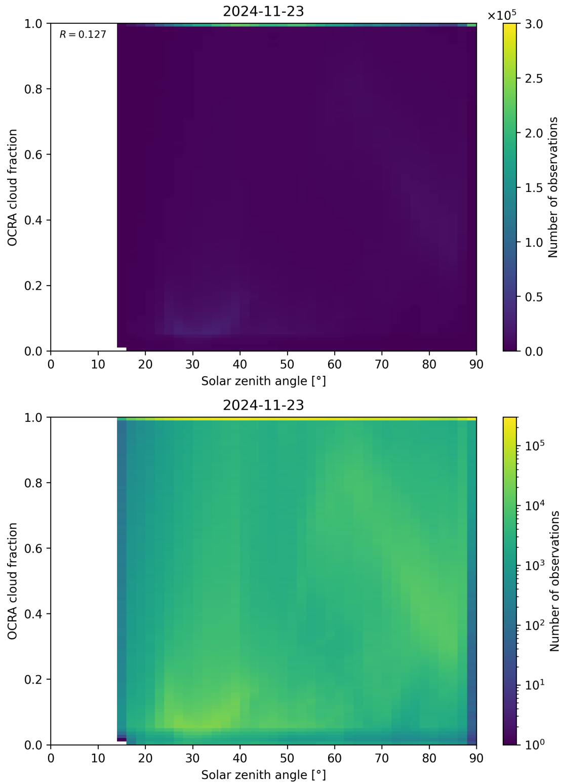
Figure 100: Scatter density plot of “Solar zenith angle” against “OCRA cloud fraction” for 2024-11-22 to 2024-11-24.
