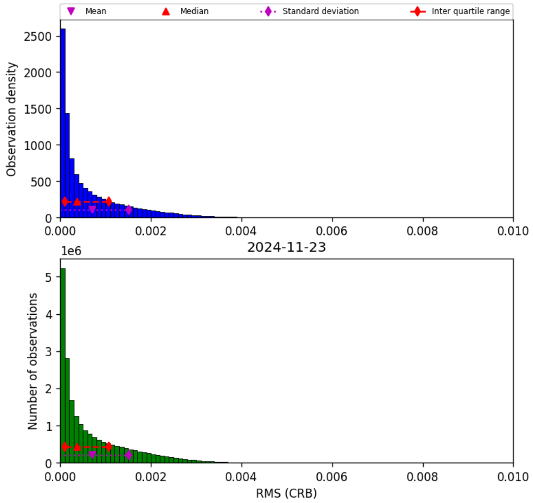
Figure 48: Histogram of “RMS (CRB)” for 2024-11-22 to 2024-11-24
