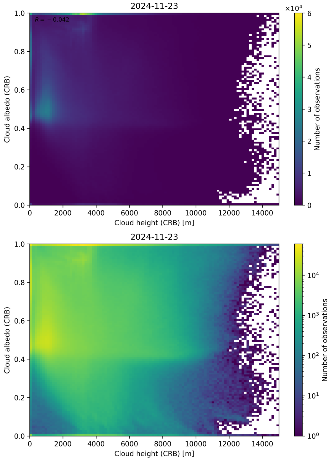
Figure 80: Scatter density plot of “Cloud height (CRB)” against “Cloud albedo (CRB)” for 2024-11-22 to 2024-11-24.
