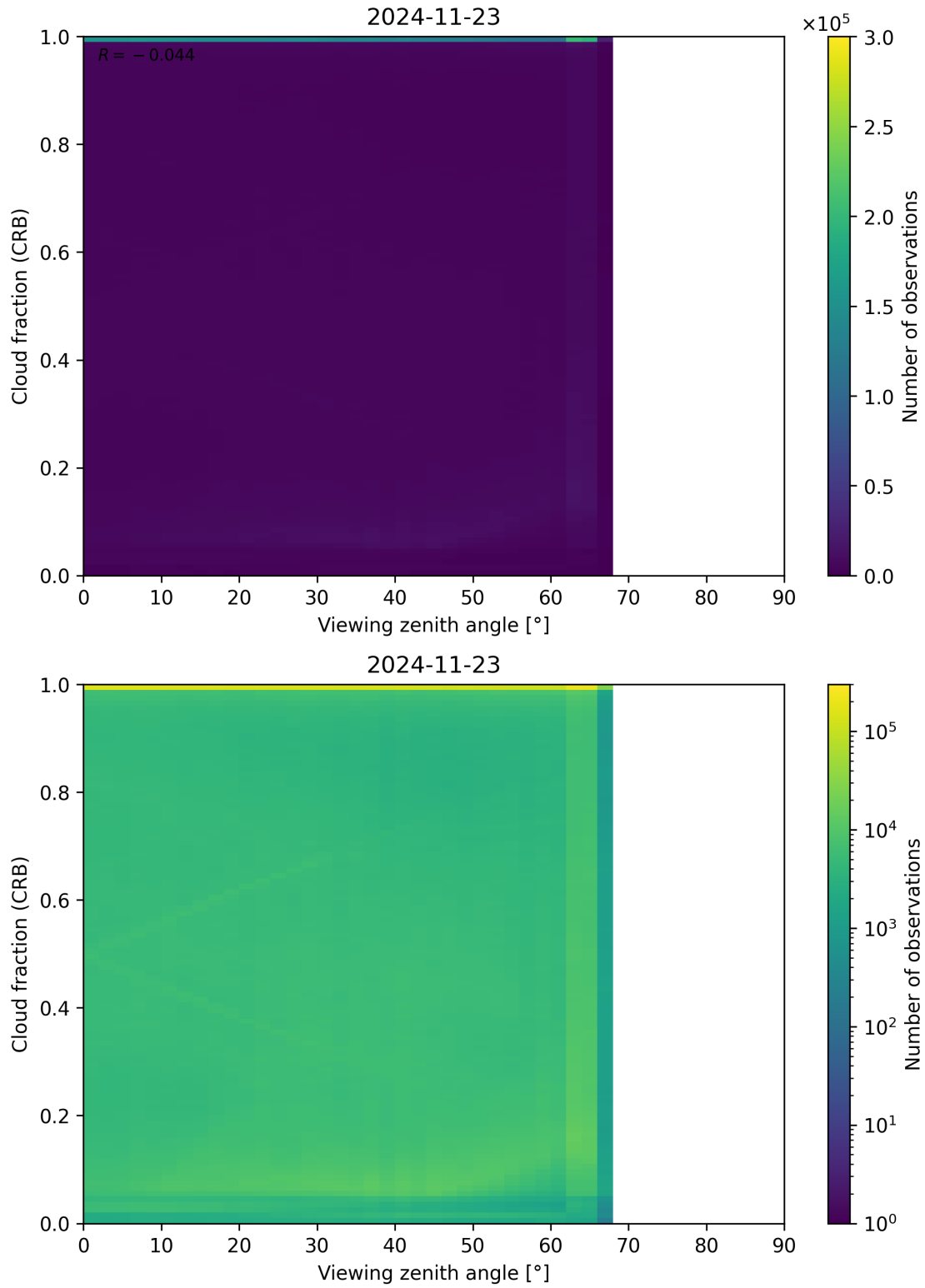
Figure 109: Scatter density plot of “Viewing zenith angle” against “Cloud fraction (CRB)” for 2024-11-22 to 2024-11-24.
