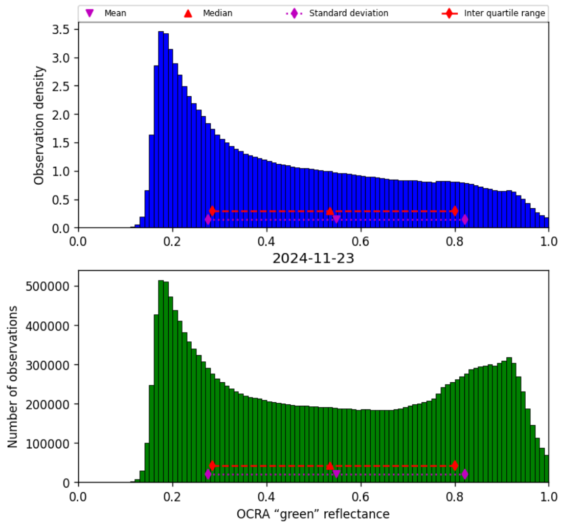
Figure 52: Histogram of “OCRA “green” reflectance” for 2024-11-22 to 2024-11-24
