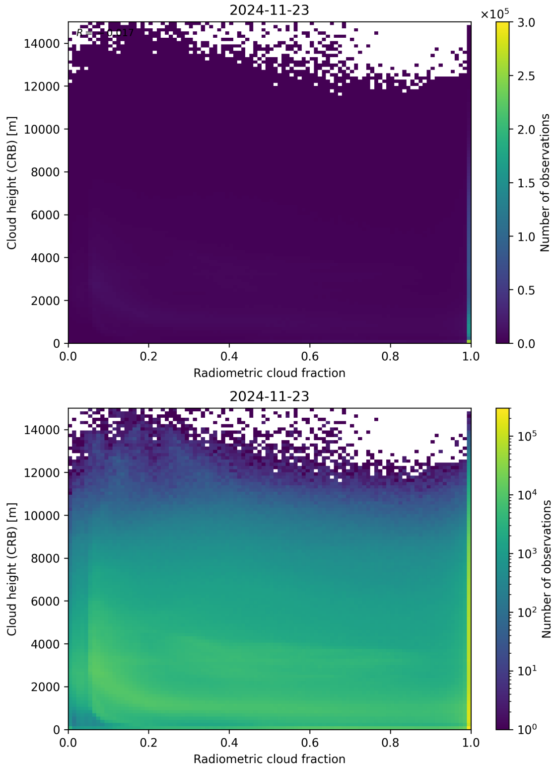
Figure 74: Scatter density plot of “Radiometric cloud fraction” against “Cloud height (CRB)” for 2024-11-22 to 2024-11-24.
