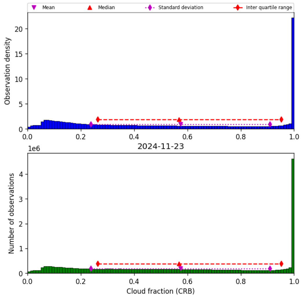
Figure 42: Histogram of “Cloud fraction (CRB)” for 2024-11-22 to 2024-11-24
