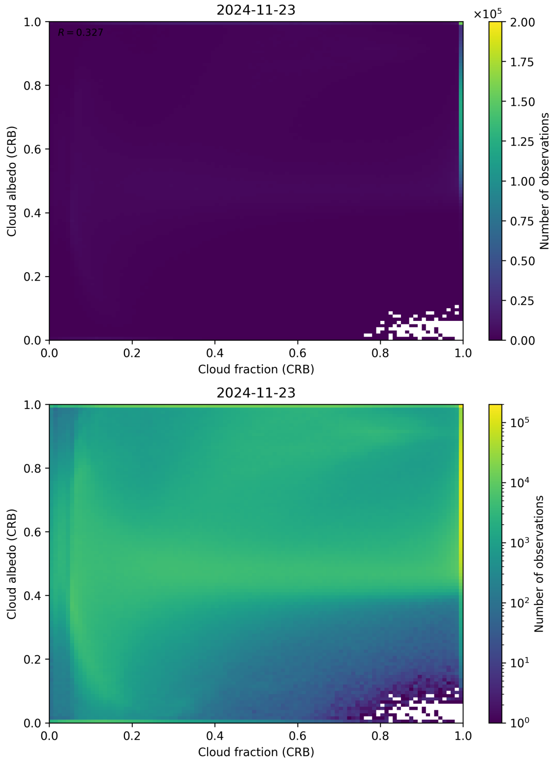
Figure 77: Scatter density plot of “Cloud fraction (CRB)” against “Cloud albedo (CRB)” for 2024-11-22 to 2024-11-24.
