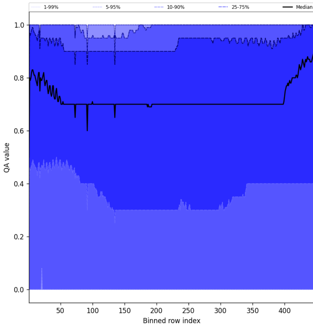
Figure 54: Along track statistics of “QA value” for 2024-11-22 to 2024-11-24
