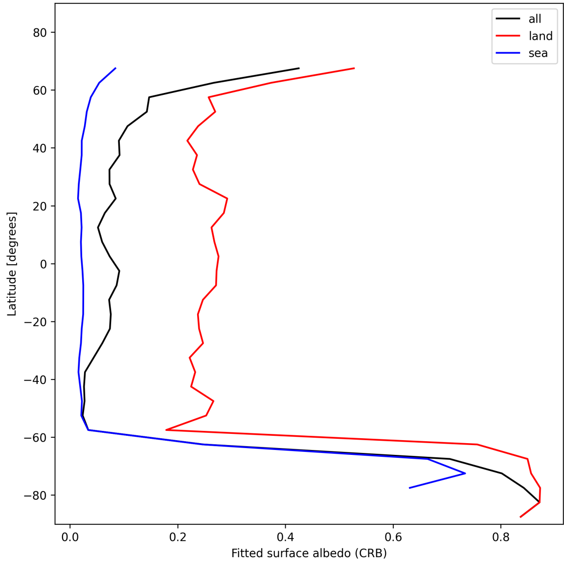
Figure 30: Zonal average of “Fitted surface albedo (CRB)” for 2024-11-22 to 2024-11-24.
