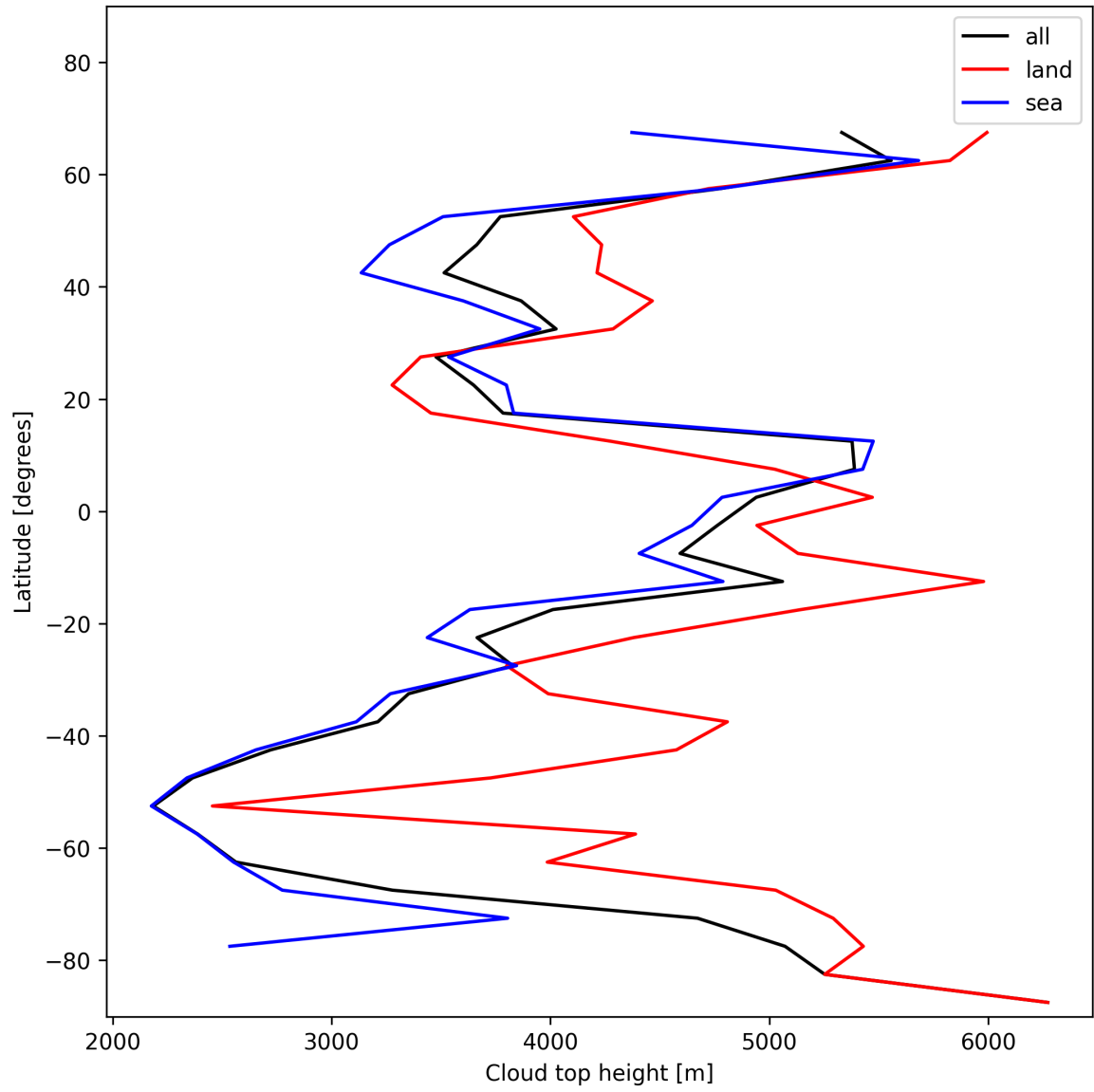
Figure 24: Zonal average of “Cloud top height” for 2024-11-22 to 2024-11-24.
