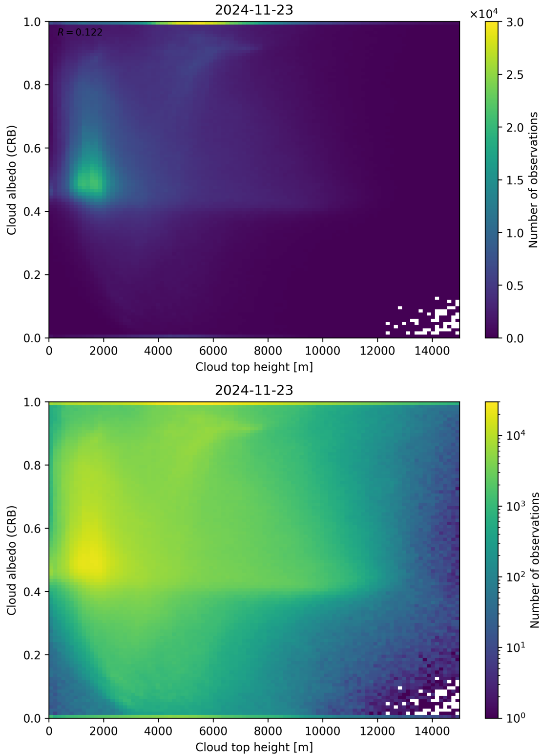
Figure 86: Scatter density plot of “Cloud top height” against “Cloud albedo (CRB)” for 2024-11-22 to 2024-11-24.
