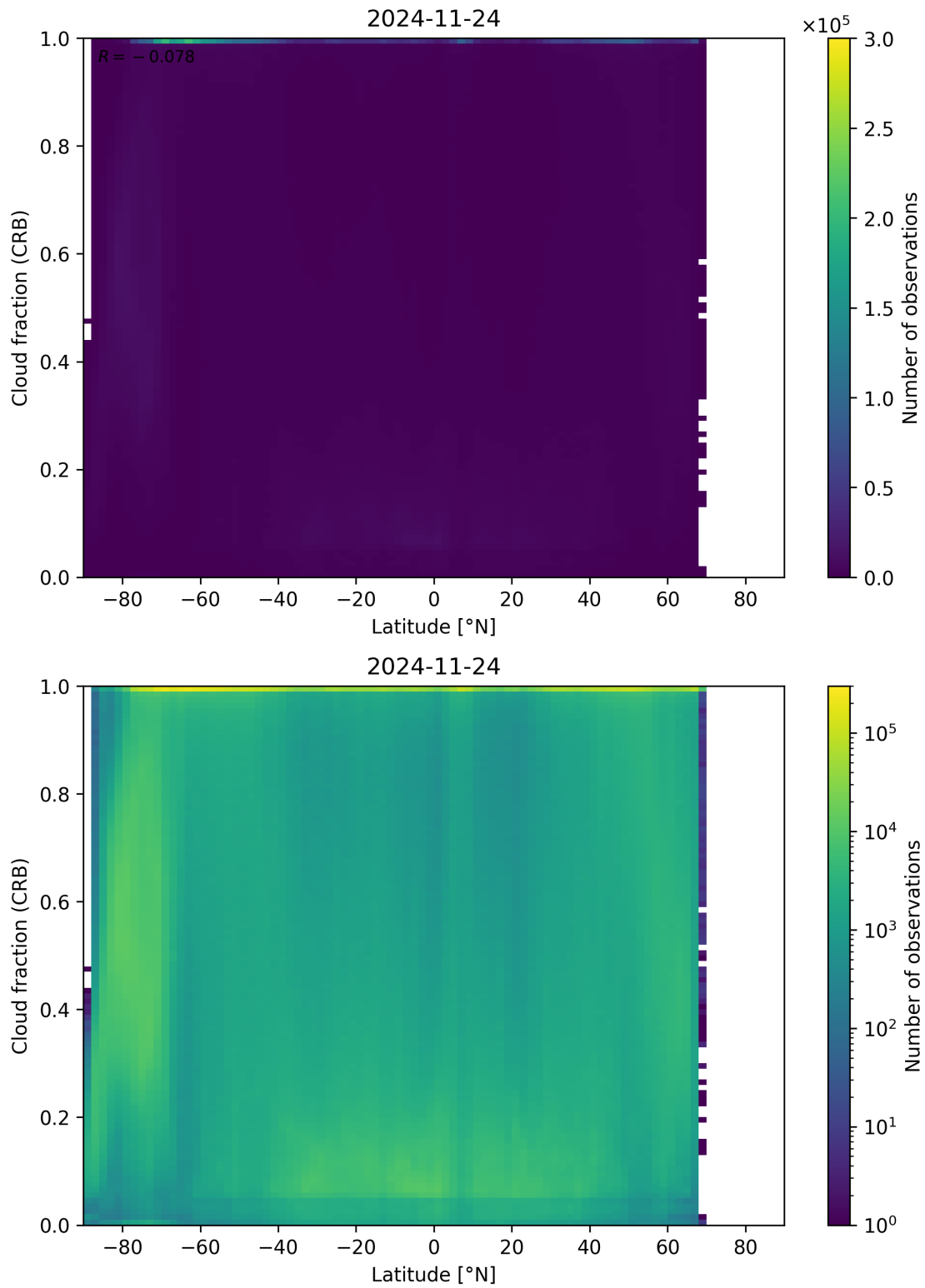
Figure 94: Scatter density plot of “Latitude” against “Cloud fraction (CRB)” for 2024-11-23 to 2024-11-25.
