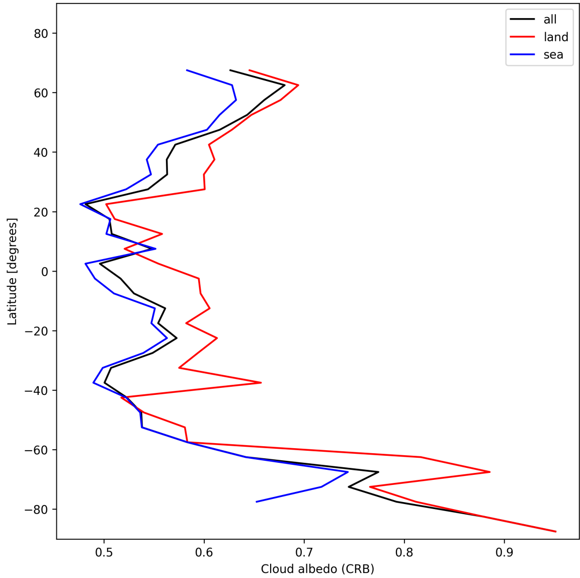
Figure 28: Zonal average of “Cloud albedo (CRB)” for 2024-11-23 to 2024-11-25.
