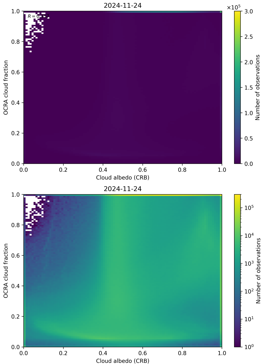
Figure 70: Scatter density plot of “Cloud albedo (CRB)” against “OCRA cloud fraction” for 2024-11-23 to 2024-11-25.
