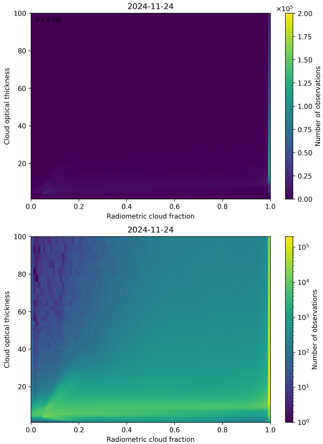
Figure 75: Scatter density plot of “Radiometric cloud fraction” against “Cloud optical thickness” for 2024-11-23 to 2024-11-25.
