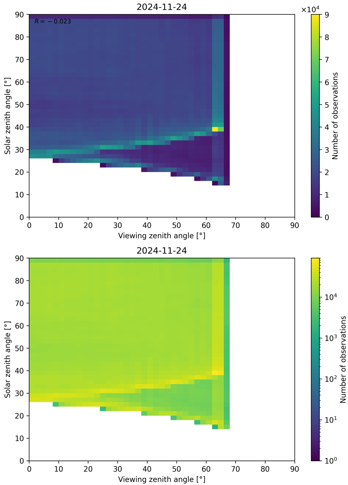
Figure 114: Scatter density plot of “Viewing zenith angle” against “Solar zenith angle” for 2024-11-23 to 2024-11-25.
