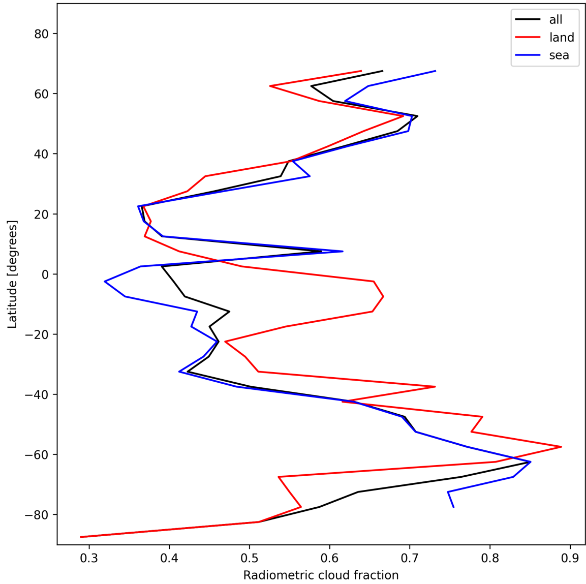
Figure 23: Zonal average of “Radiometric cloud fraction” for 2024-11-23 to 2024-11-25.
