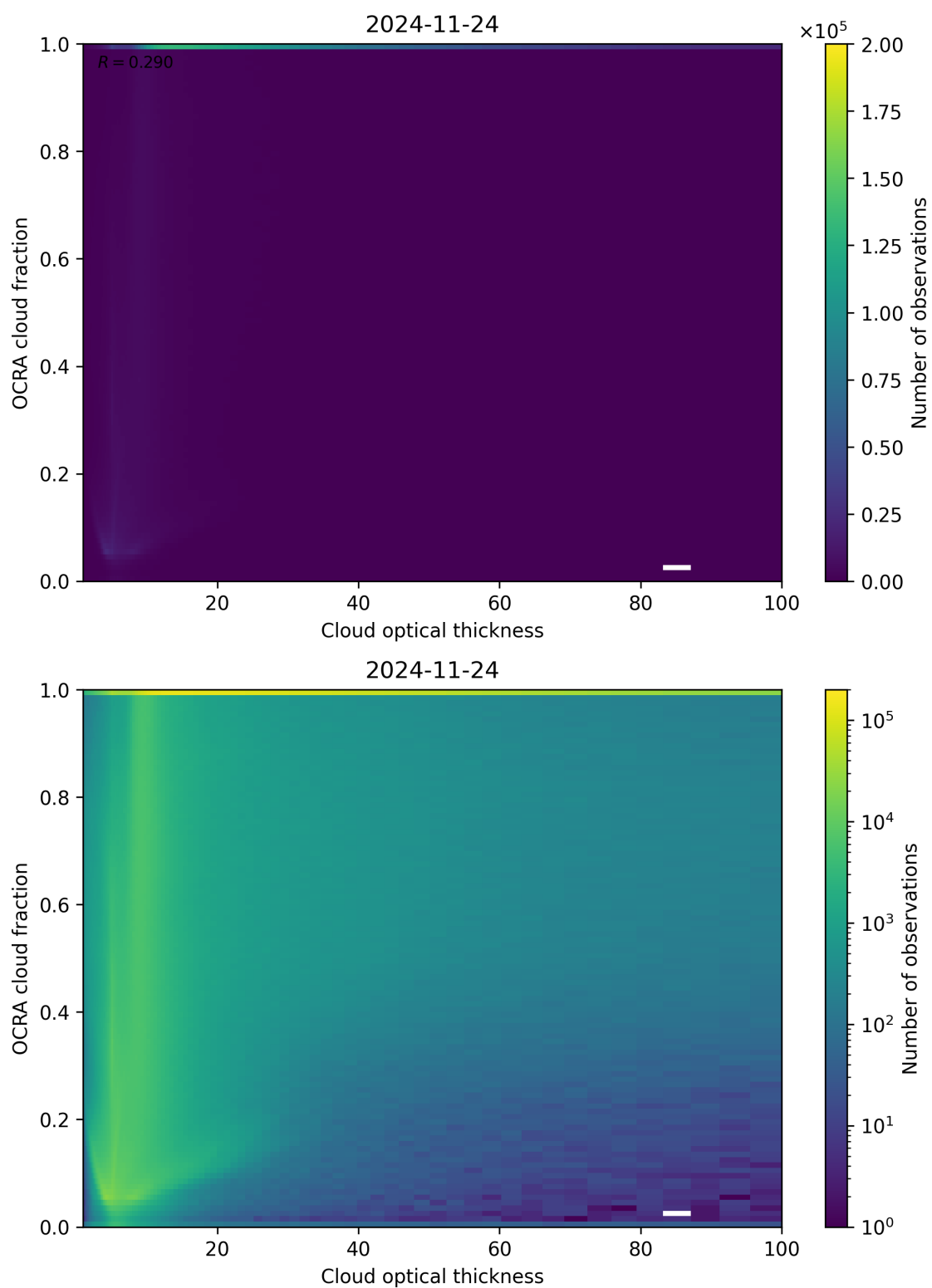
Figure 83: Scatter density plot of “Cloud optical thickness” against “OCRA cloud fraction” for 2024-11-23 to 2024-11-25.
