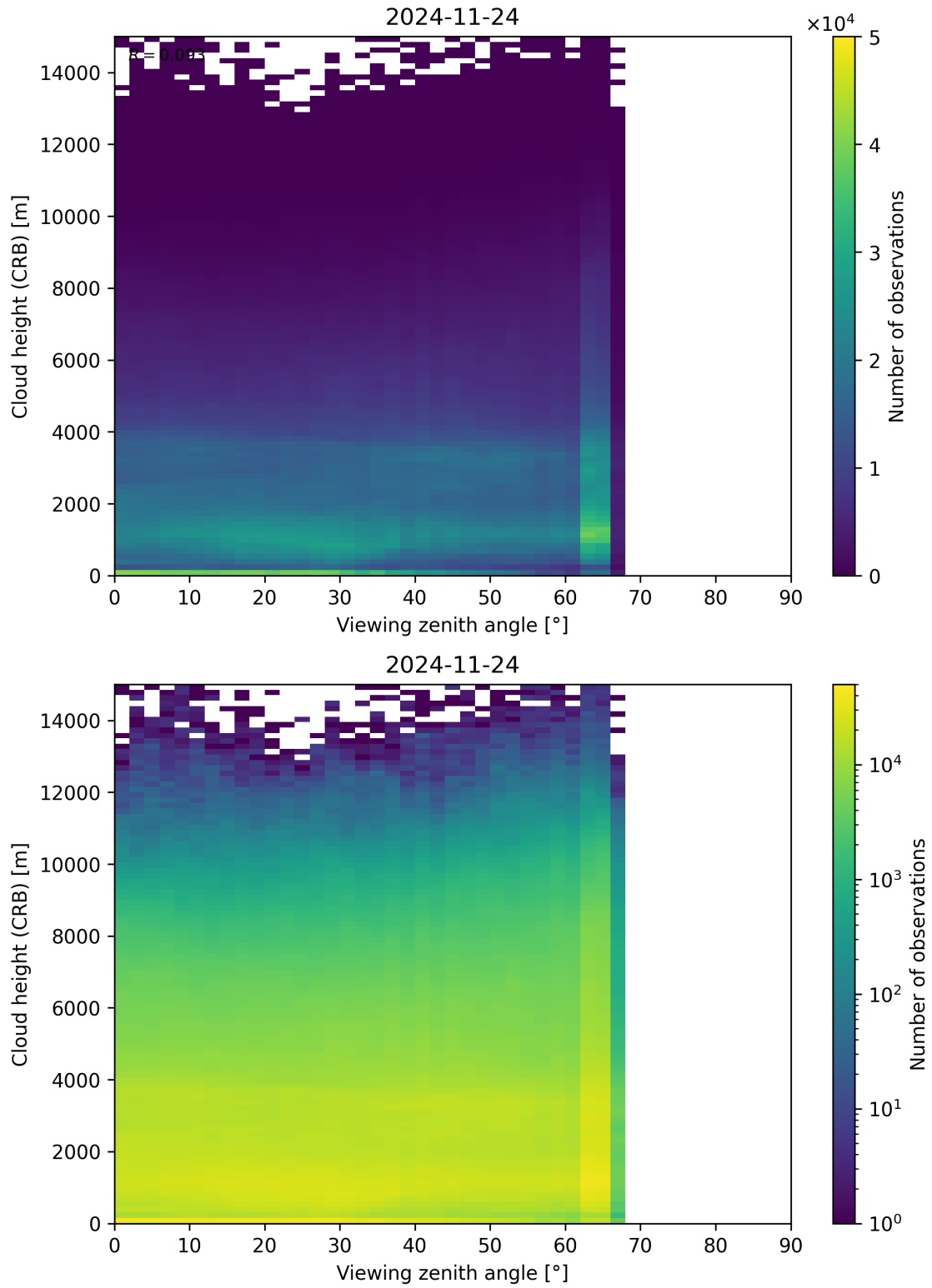
Figure 110: Scatter density plot of “Viewing zenith angle” against “Cloud height (CRB)” for 2024-11-23 to 2024-11-25.
