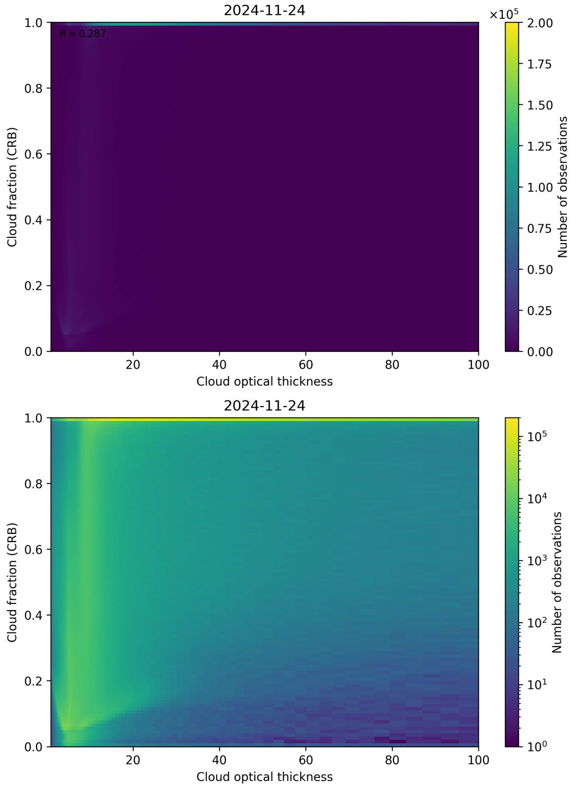
Figure 84: Scatter density plot of “Cloud optical thickness” against “Cloud fraction (CRB)” for 2024-11-23 to 2024-11-25.
