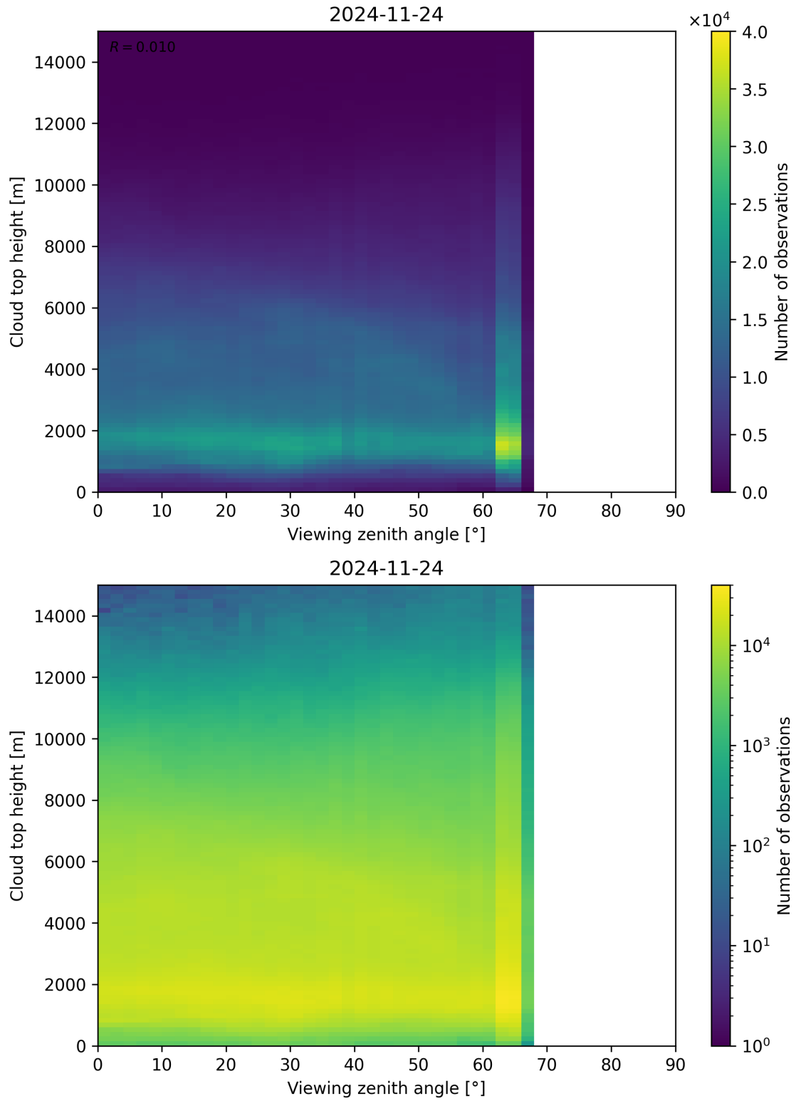
Figure 112: Scatter density plot of “Viewing zenith angle” against “Cloud top height” for 2024-11-23 to 2024-11-25.
