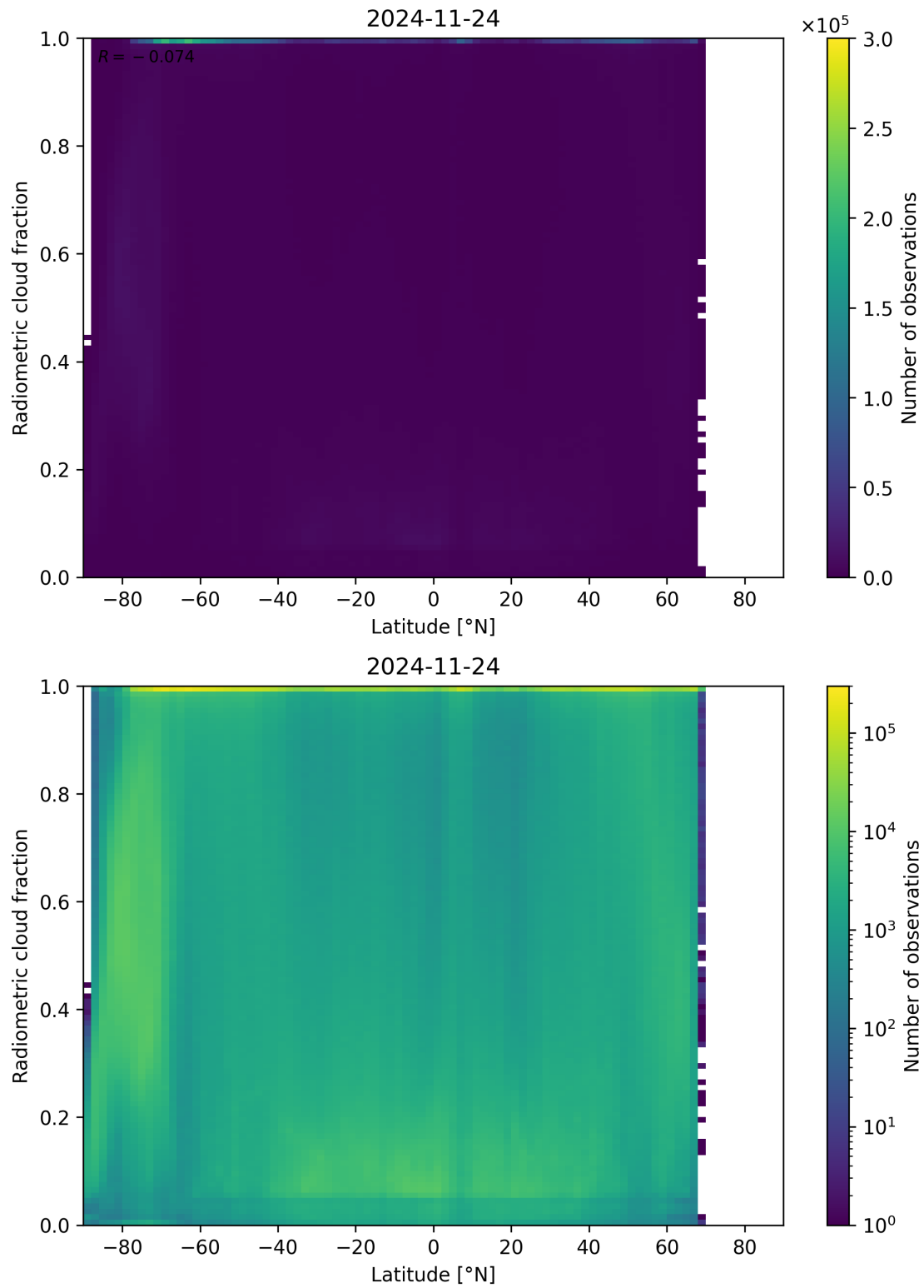
Figure 92: Scatter density plot of “Latitude” against “Radiometric cloud fraction” for 2024-11-23 to 2024-11-25.
