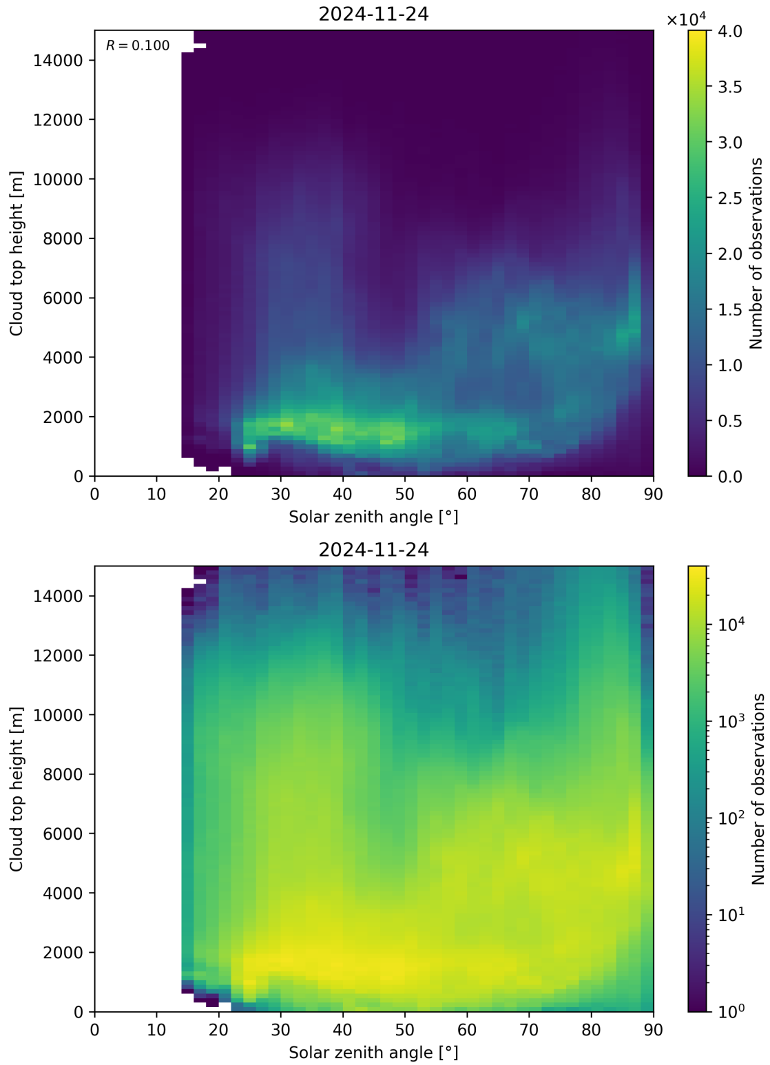
Figure 104: Scatter density plot of “Solar zenith angle” against “Cloud top height” for 2024-11-23 to 2024-11-25.
