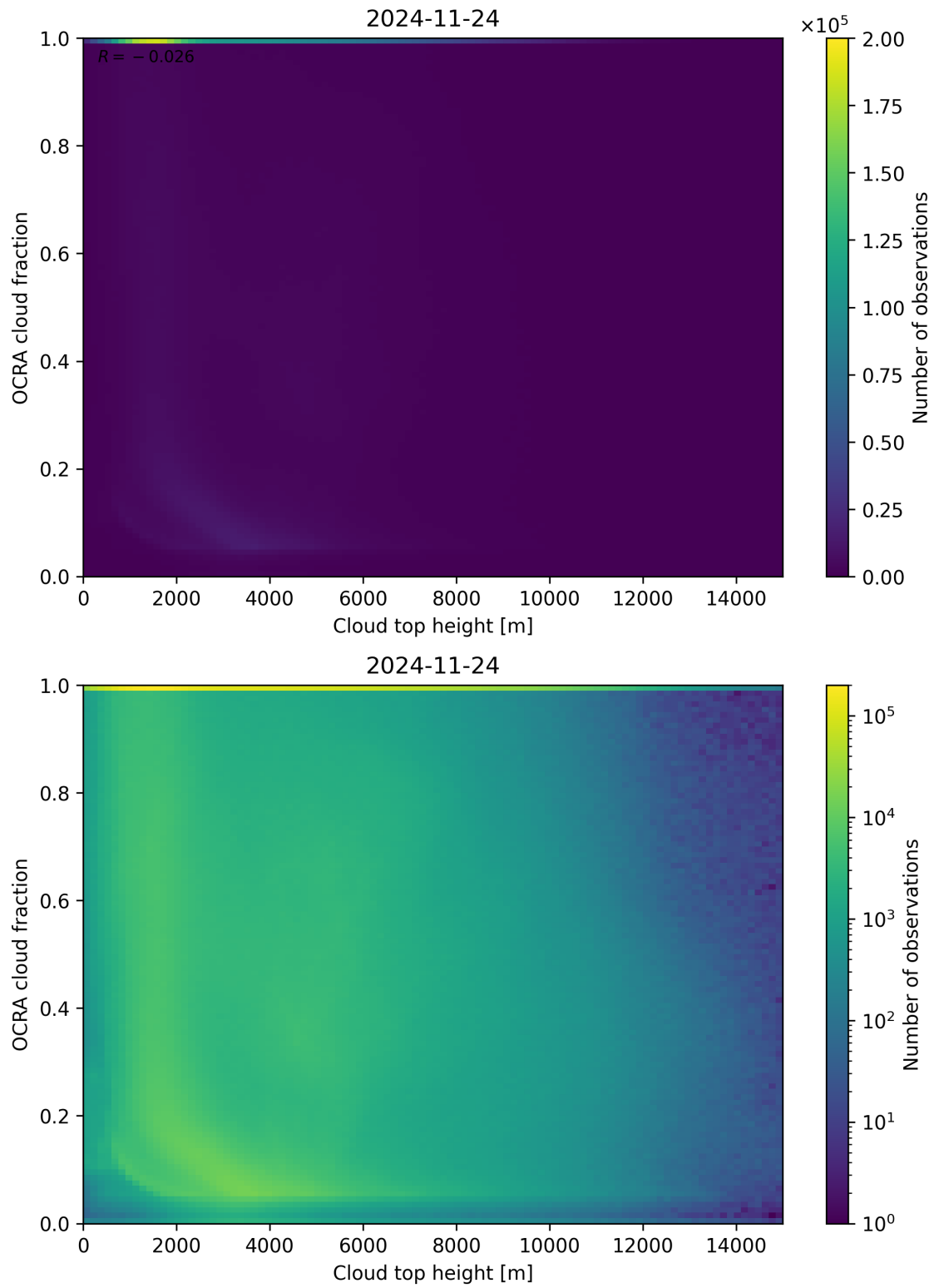
Figure 87: Scatter density plot of “Cloud top height” against “OCRA cloud fraction” for 2024-11-23 to 2024-11-25.
