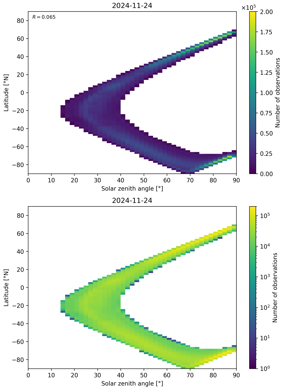
Figure 105: Scatter density plot of “Solar zenith angle” against “Latitude” for 2024-11-23 to 2024-11-25.
