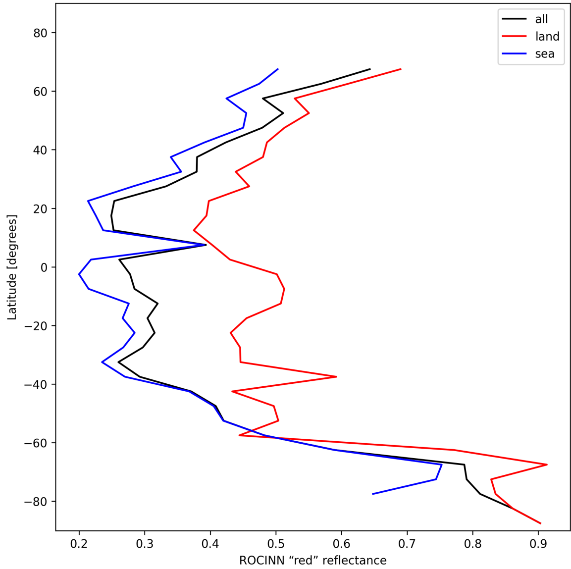
Figure 37: Zonal average of “ROCINN “red” reflectance” for 2024-11-23 to 2024-11-25.
