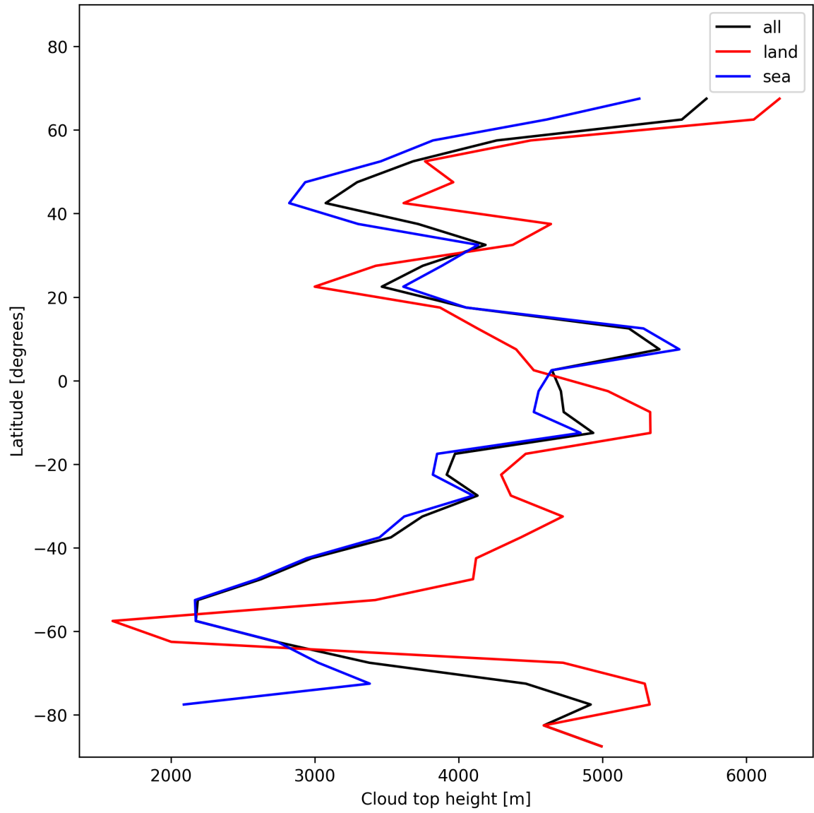
Figure 24: Zonal average of “Cloud top height” for 2024-11-23 to 2024-11-25.
