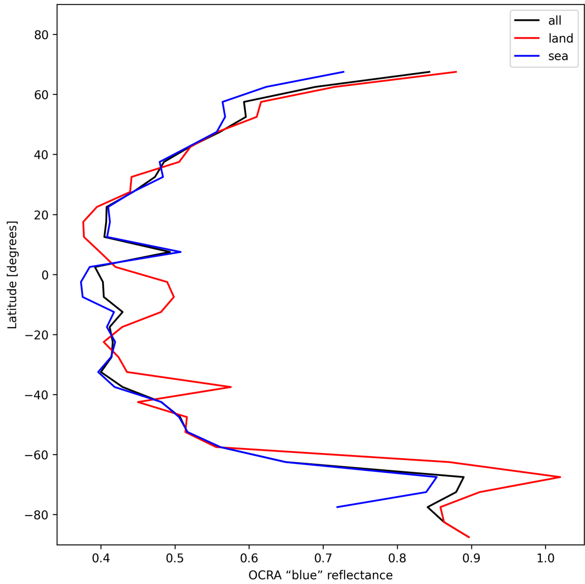
Figure 35: Zonal average of “OCRA “blue” reflectance” for 2024-11-23 to 2024-11-25.
