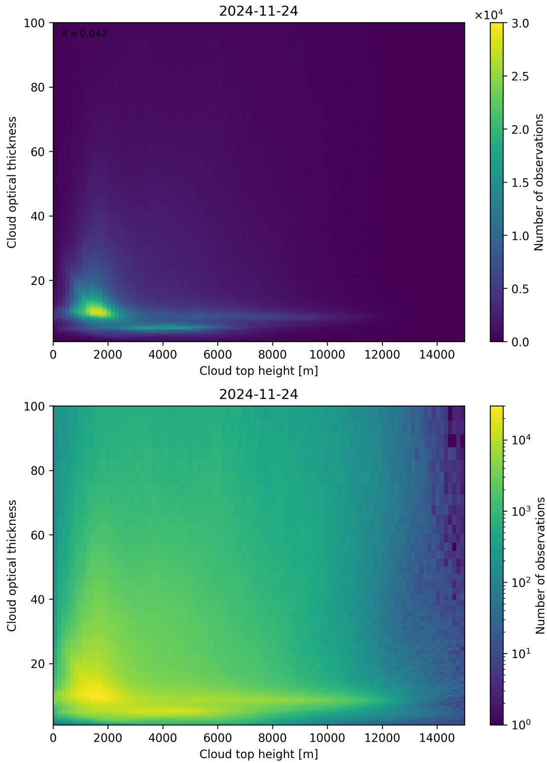
Figure 90: Scatter density plot of “Cloud top height” against “Cloud optical thickness” for 2024-11-23 to 2024-11-25.
