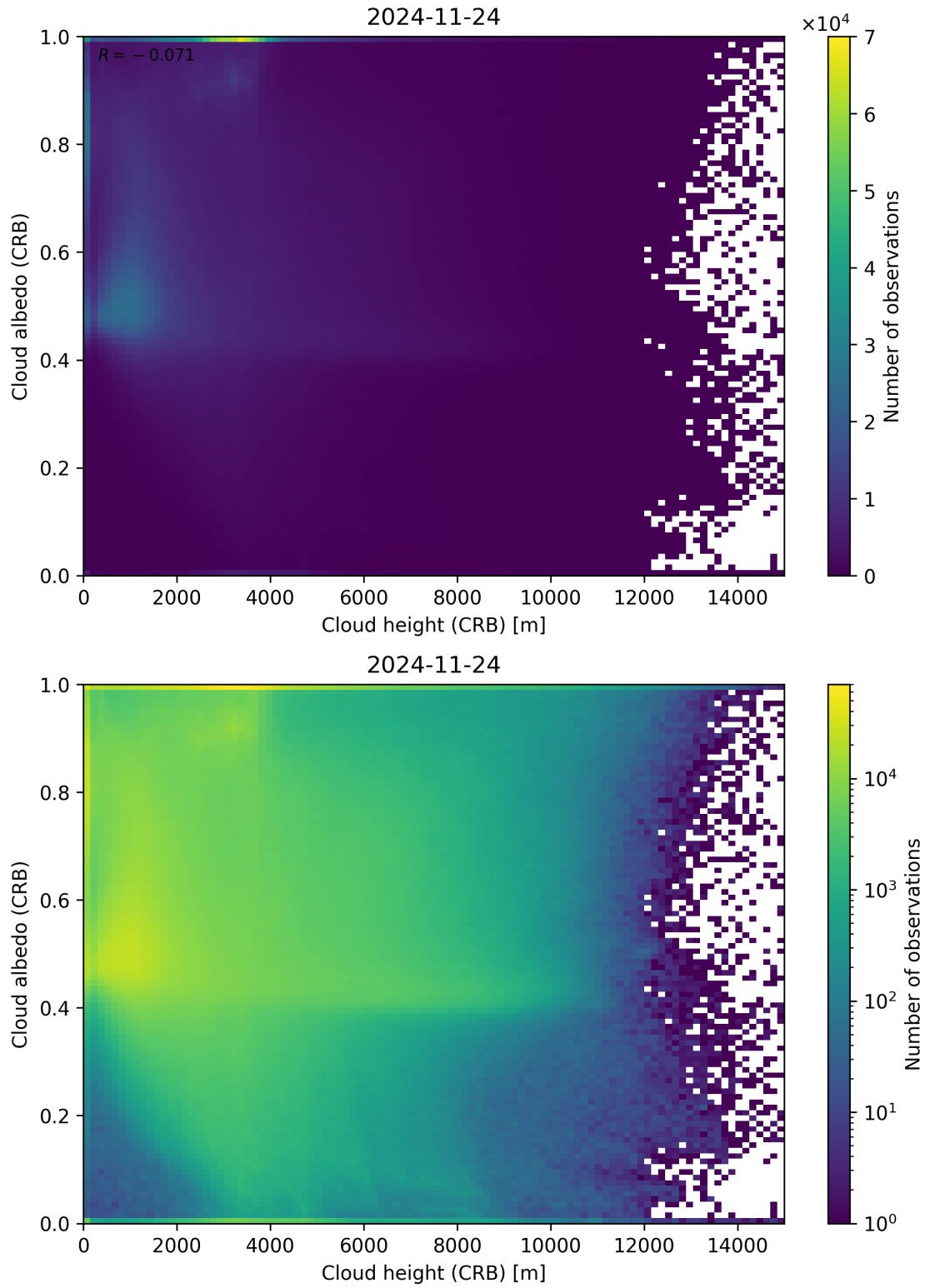
Figure 80: Scatter density plot of “Cloud height (CRB)” against “Cloud albedo (CRB)” for 2024-11-23 to 2024-11-25.
