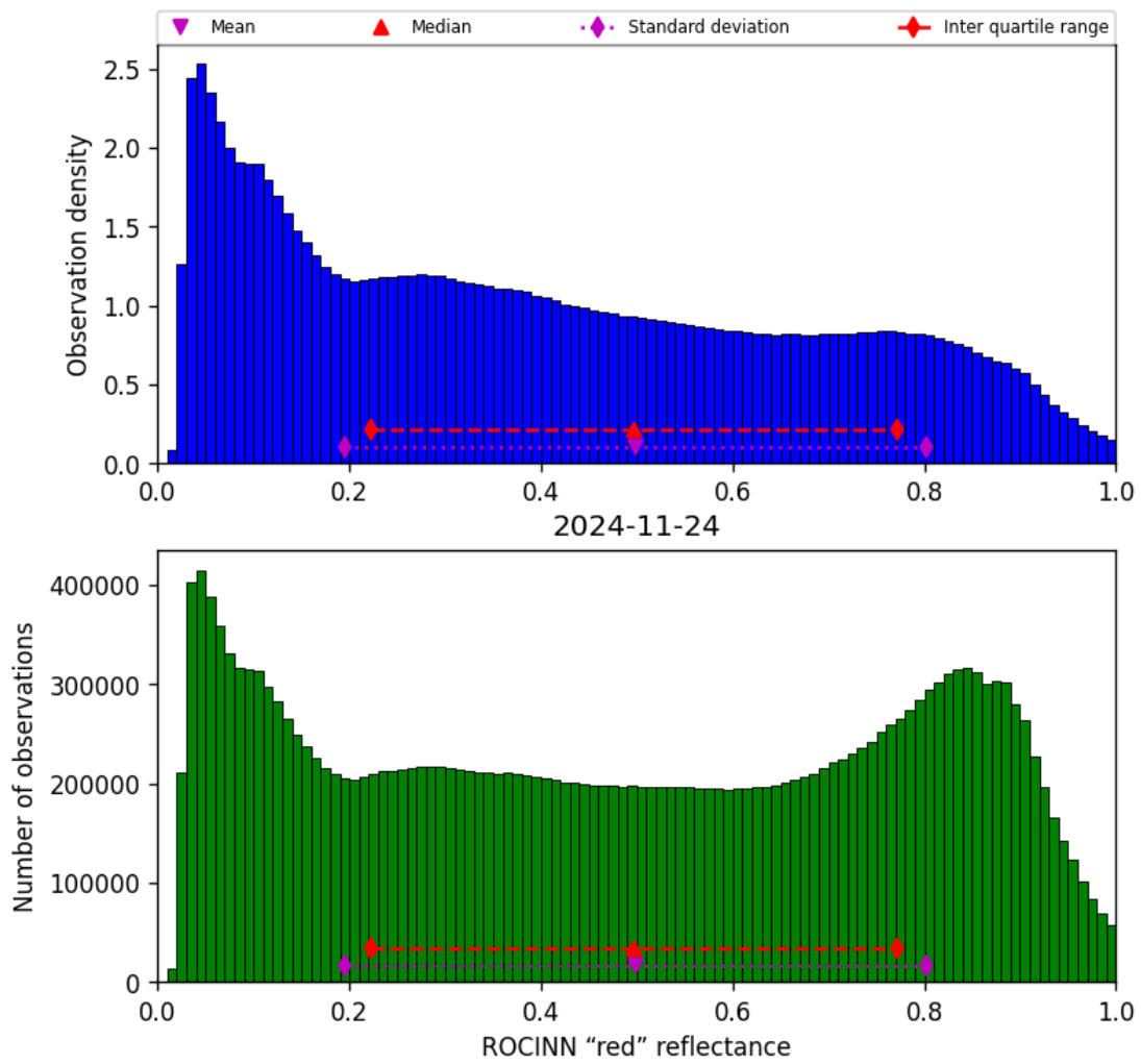
Figure 53: Histogram of “ROCINN “red” reflectance” for 2024-11-23 to 2024-11-25
