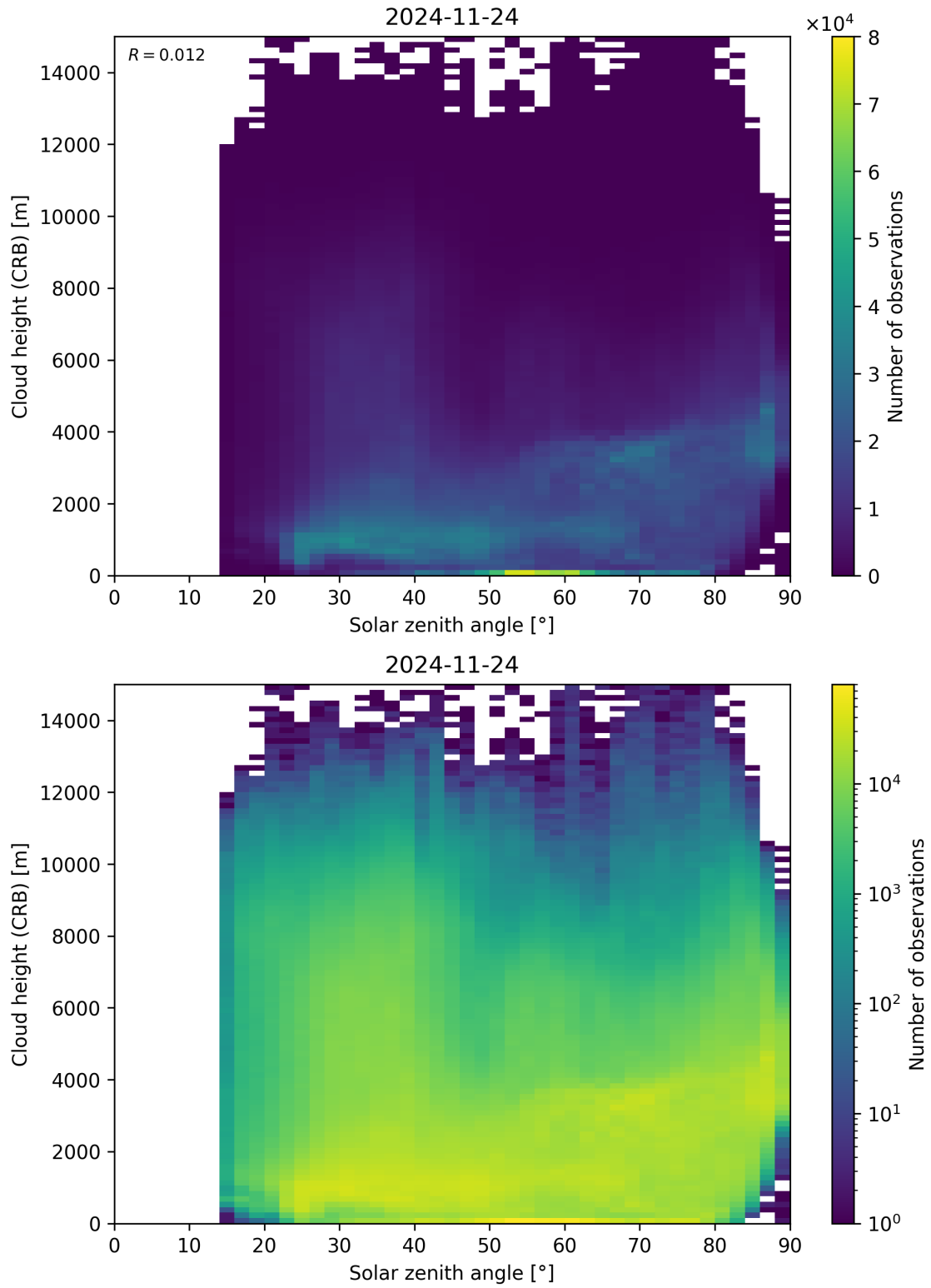
Figure 102: Scatter density plot of “Solar zenith angle” against “Cloud height (CRB)” for 2024-11-23 to 2024-11-25.
