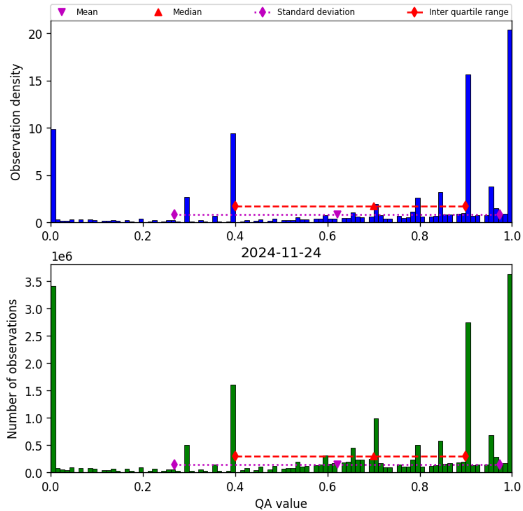
Figure 38: Histogram of “QA value” for 2024-11-23 to 2024-11-25
