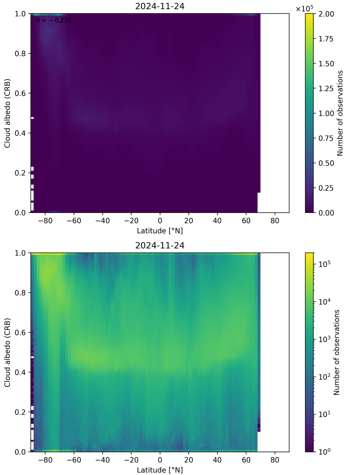
Figure 91: Scatter density plot of “Latitude” against “Cloud albedo (CRB)” for 2024-11-23 to 2024-11-25.
