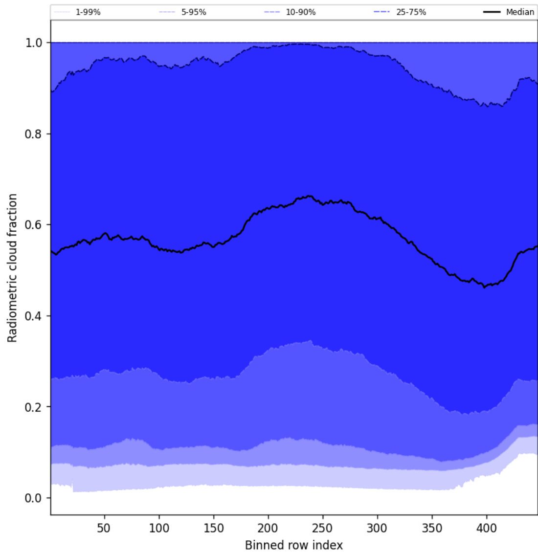
Figure 55: Along track statistics of “Radiometric cloud fraction” for 2024-11-23 to 2024-11-25
