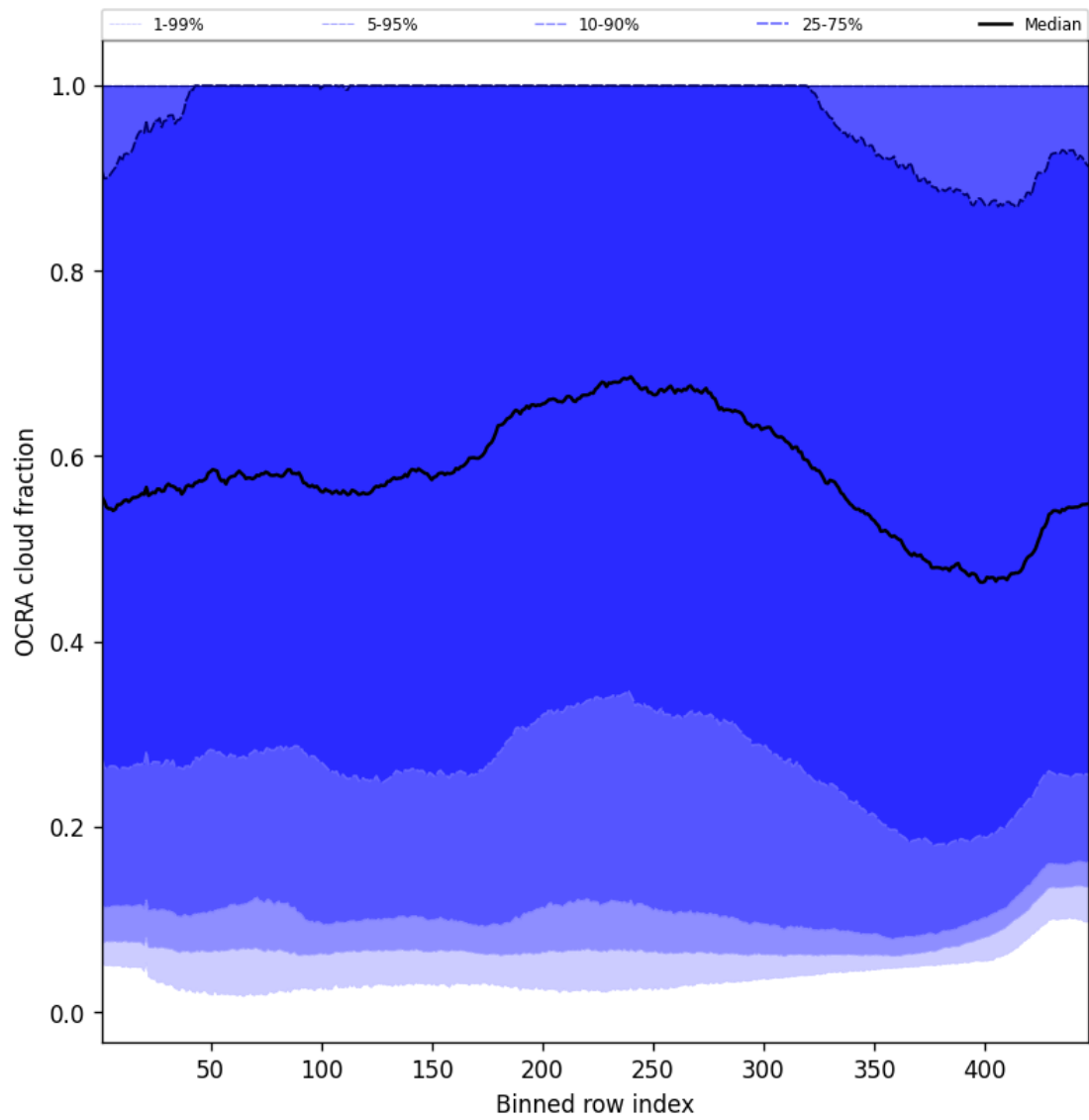
Figure 66: Along track statistics of “OCRA cloud fraction” for 2024-11-23 to 2024-11-25
