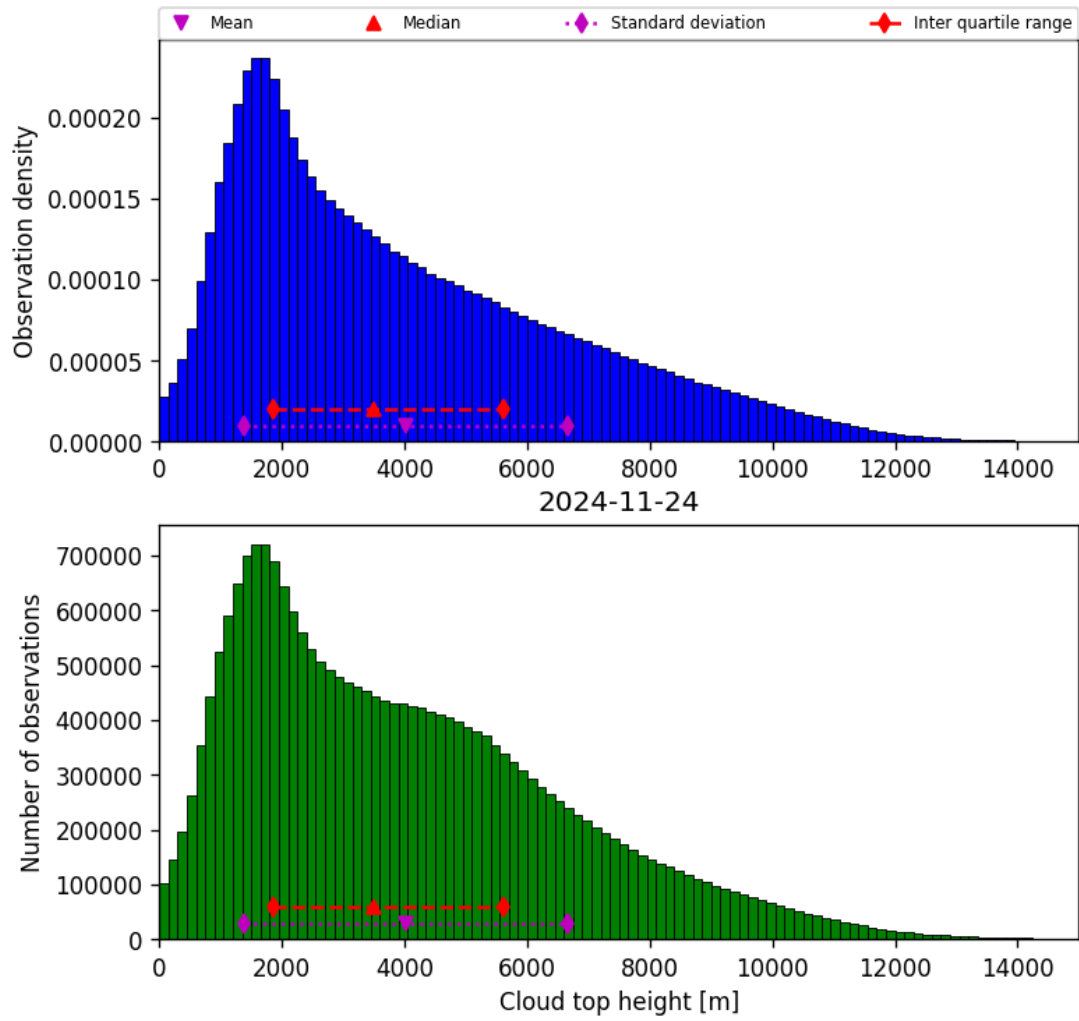
Figure 40: Histogram of “Cloud top height” for 2024-11-23 to 2024-11-25
