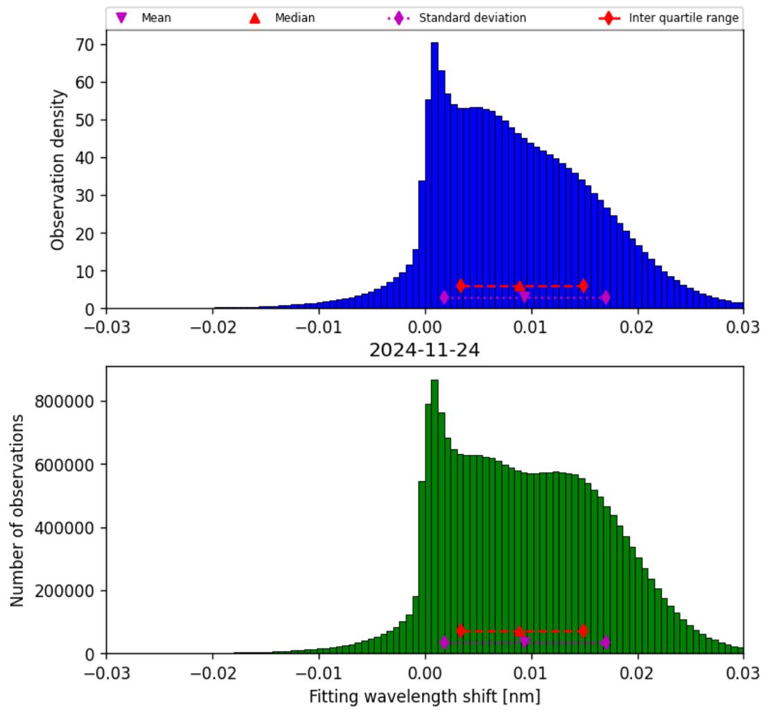
Figure 49: Histogram of “Fitting wavelength shift” for 2024-11-23 to 2024-11-25
