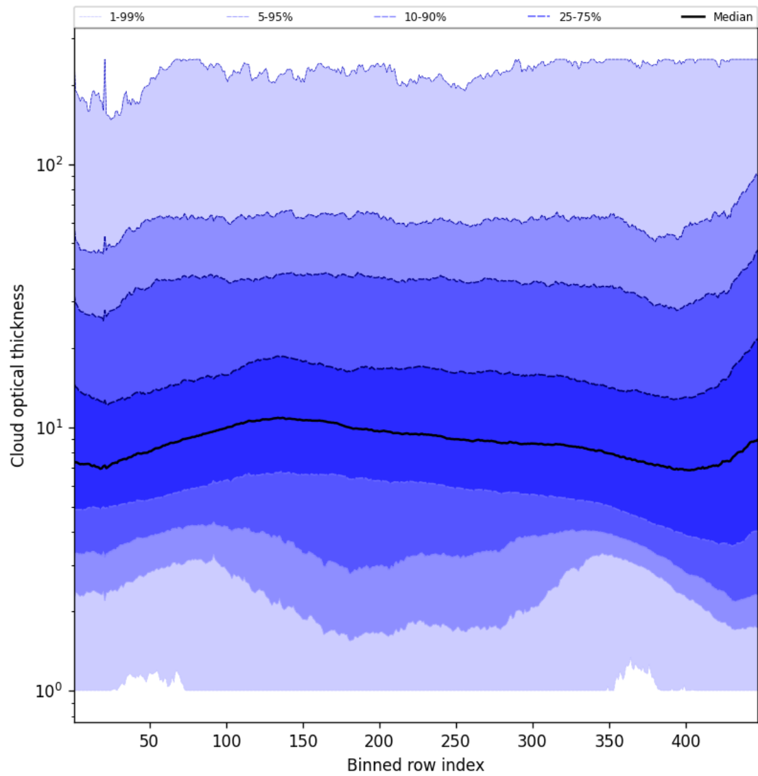
Figure 57: Along track statistics of “Cloud optical thickness” for 2024-11-23 to 2024-11-25
