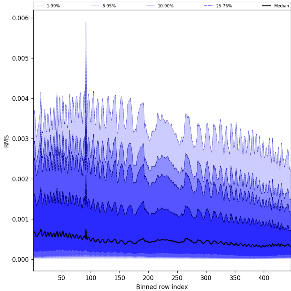
Figure 63: Along track statistics of “RMS” for 2024-11-23 to 2024-11-25
