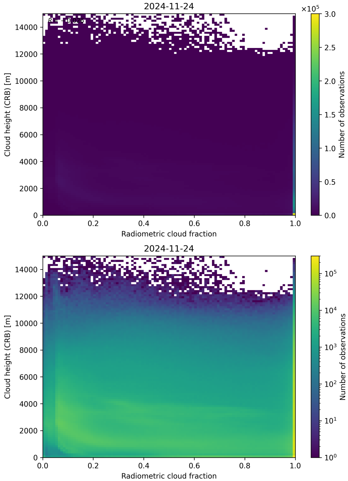
Figure 74: Scatter density plot of “Radiometric cloud fraction” against “Cloud height (CRB)” for 2024-11-23 to 2024-11-25.
