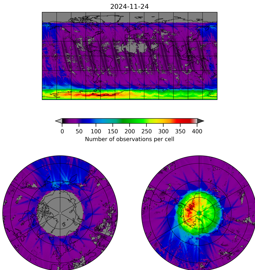
Figure 21: Map of the number of observations for 2024-11-23 to 2024-11-25
