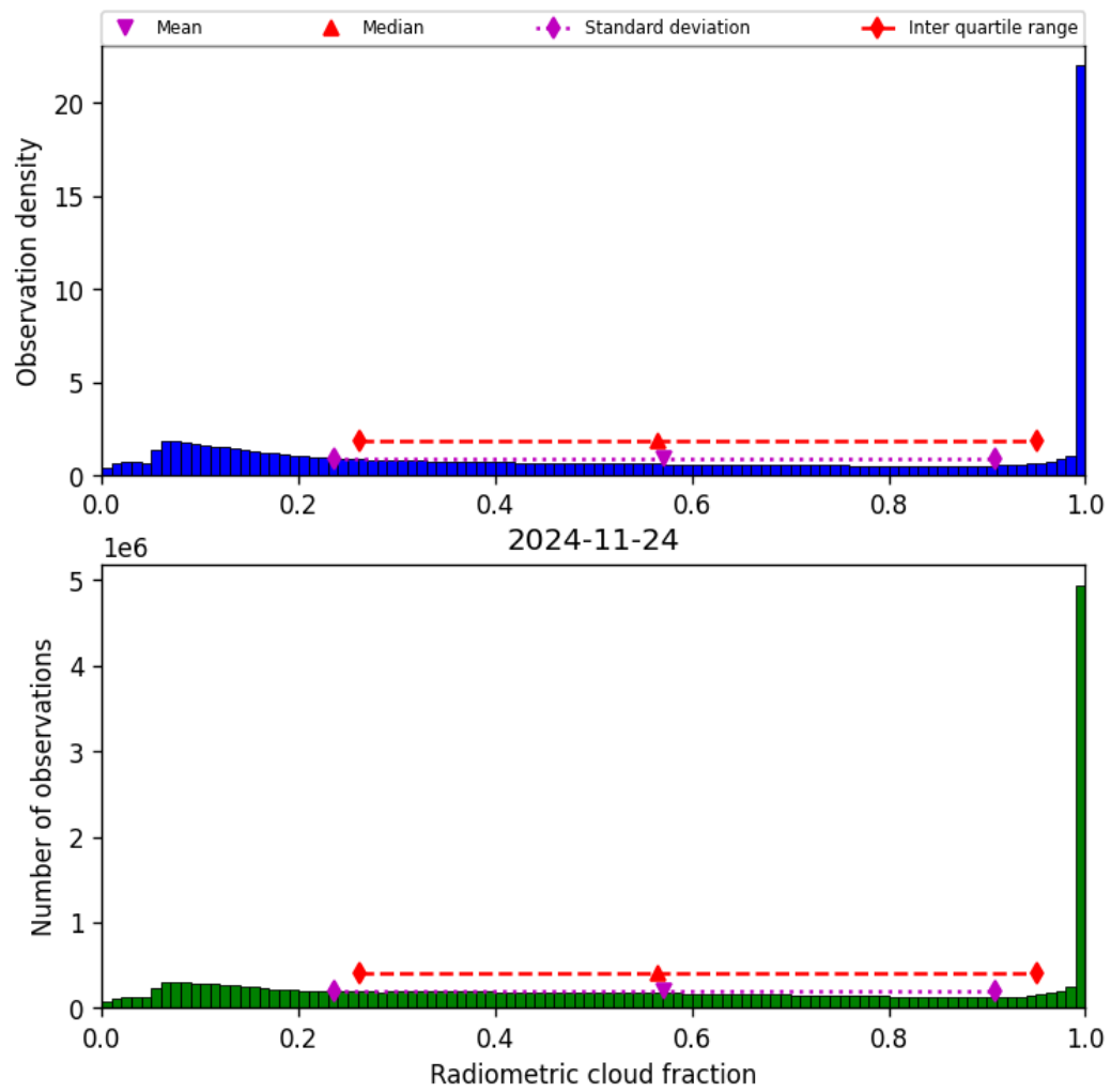
Figure 39: Histogram of “Radiometric cloud fraction” for 2024-11-23 to 2024-11-25
