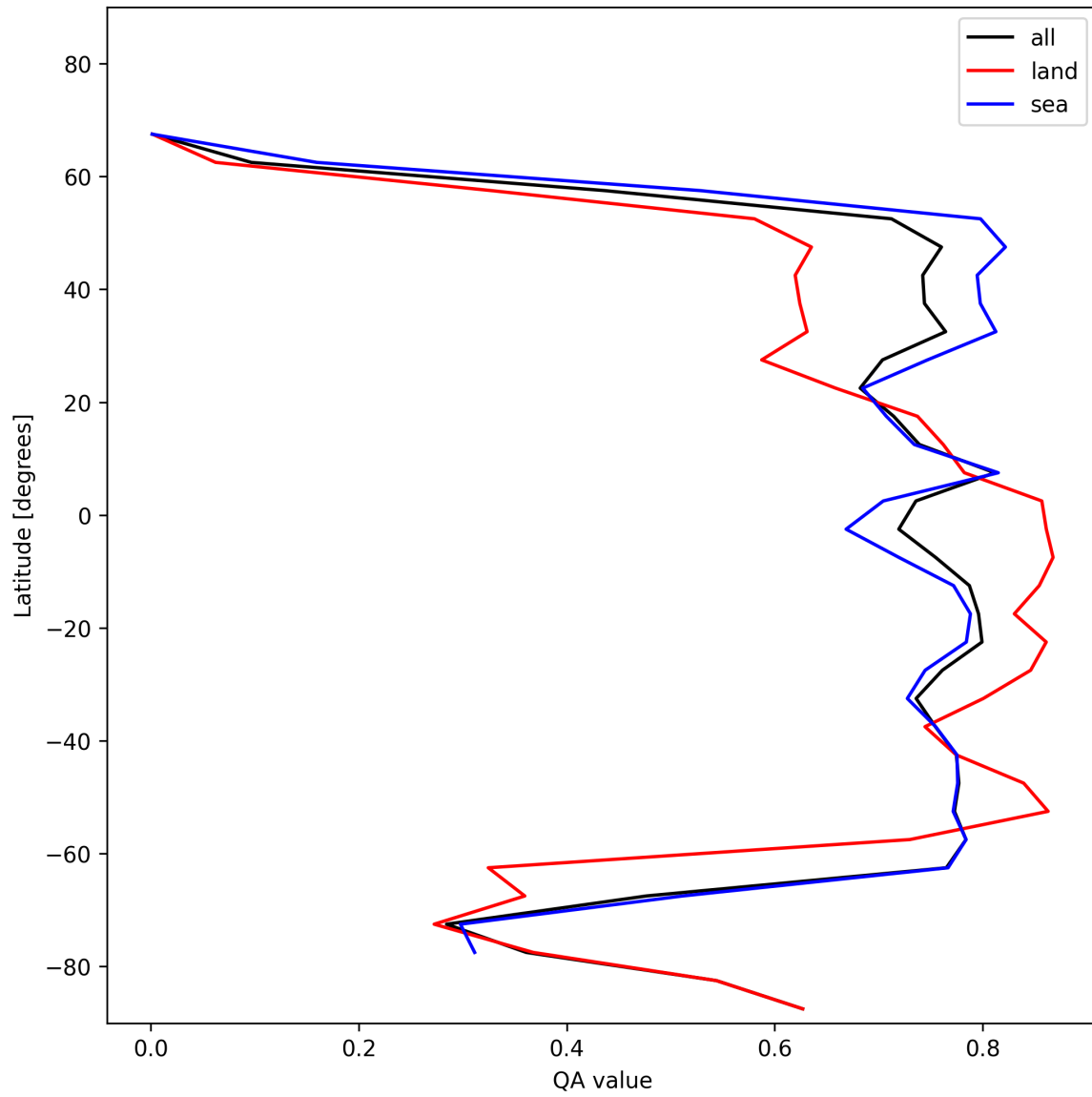
Figure 22: Zonal average of “QA value” for 2024-11-23 to 2024-11-25.
