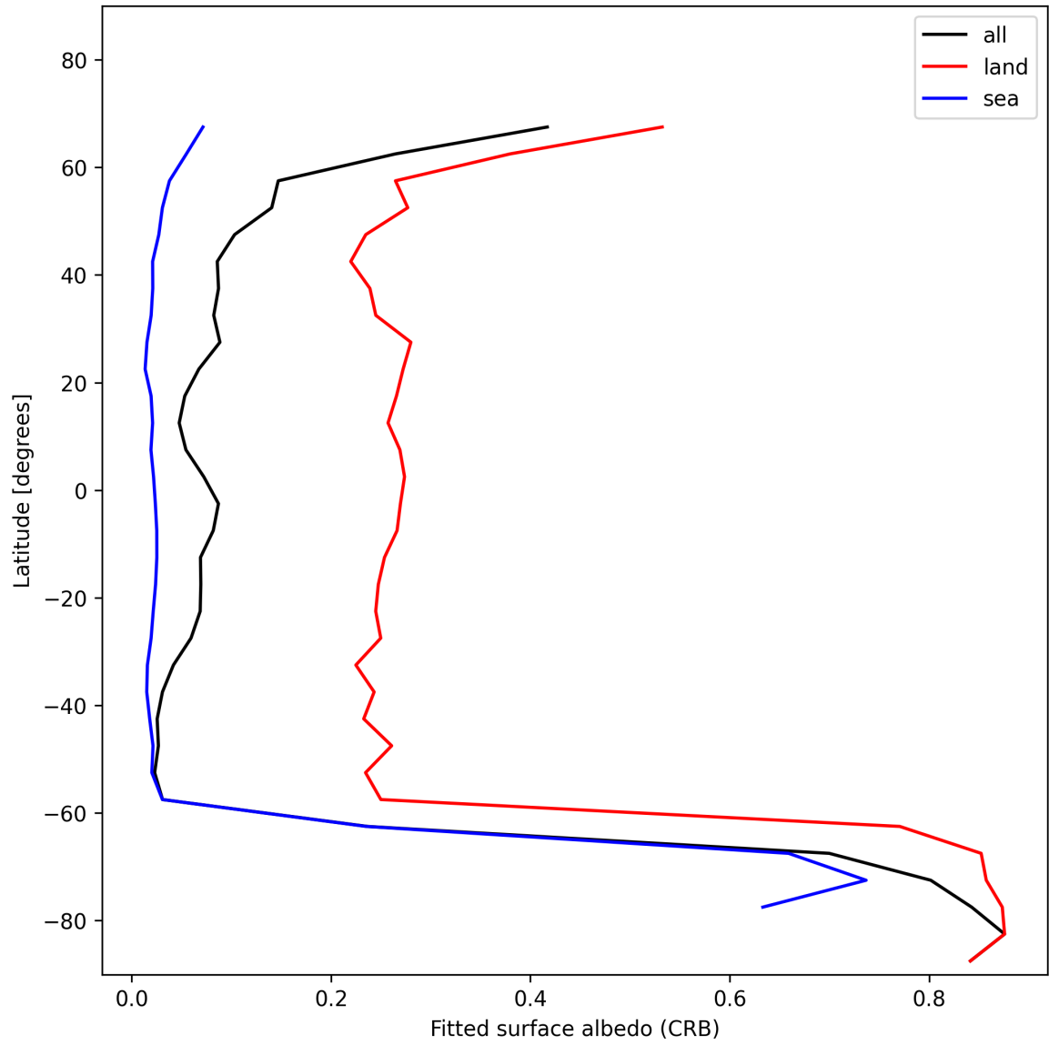
Figure 30: Zonal average of “Fitted surface albedo (CRB)” for 2024-11-23 to 2024-11-25.
