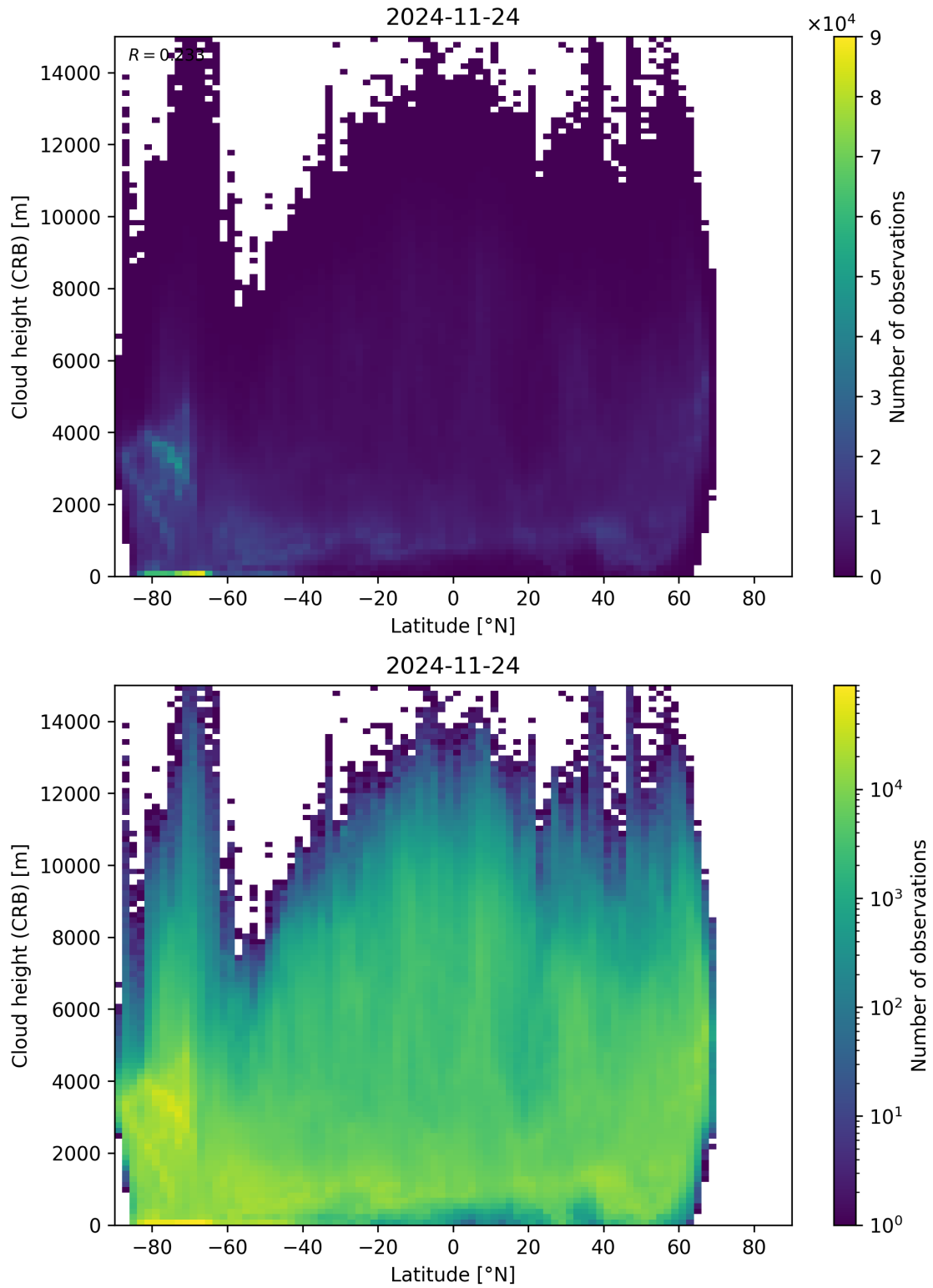
Figure 95: Scatter density plot of “Latitude” against “Cloud height (CRB)” for 2024-11-23 to 2024-11-25.
