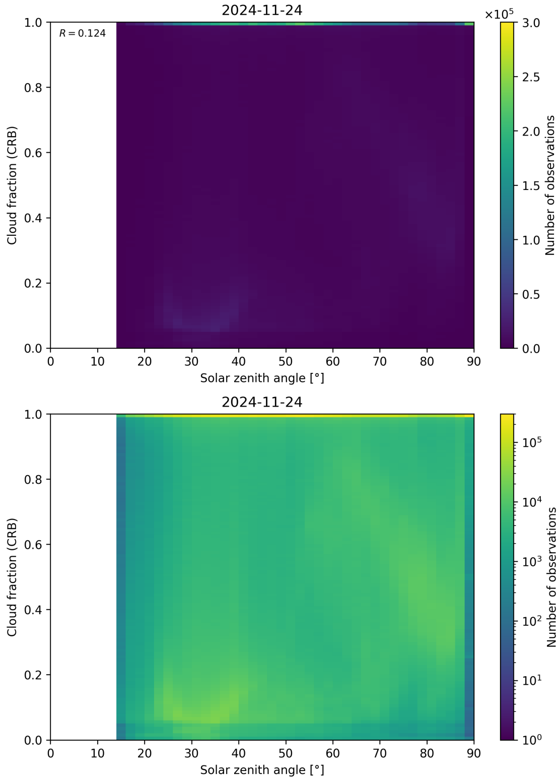
Figure 101: Scatter density plot of “Solar zenith angle” against “Cloud fraction (CRB)” for 2024-11-23 to 2024-11-25.
