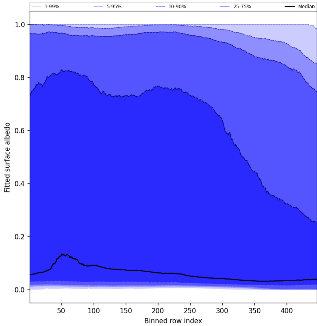
Figure 61: Along track statistics of “Fitted surface albedo” for 2024-11-23 to 2024-11-25
