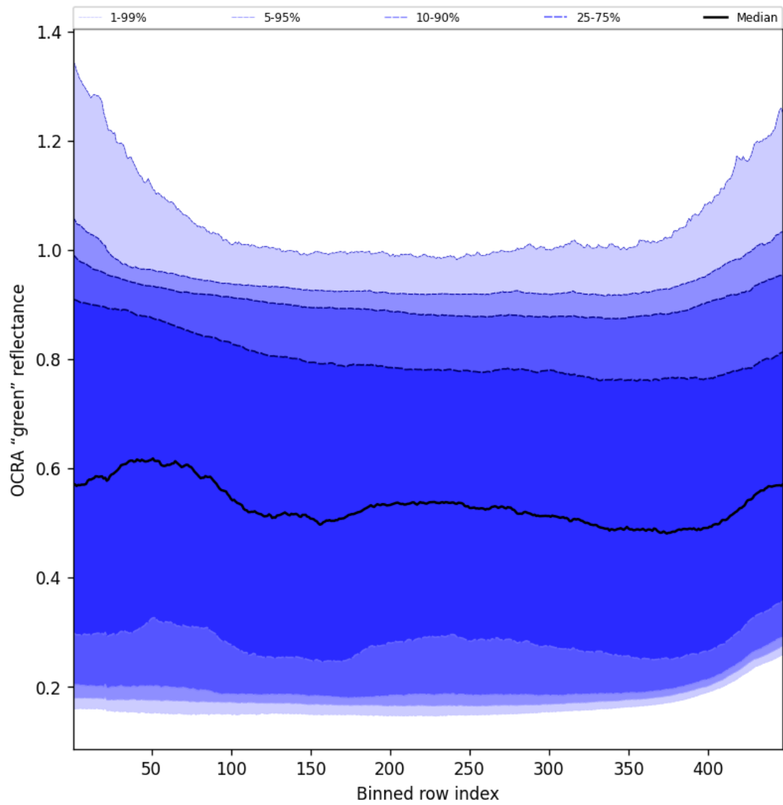
Figure 68: Along track statistics of “OCRA “green” reflectance” for 2024-11-23 to 2024-11-25
