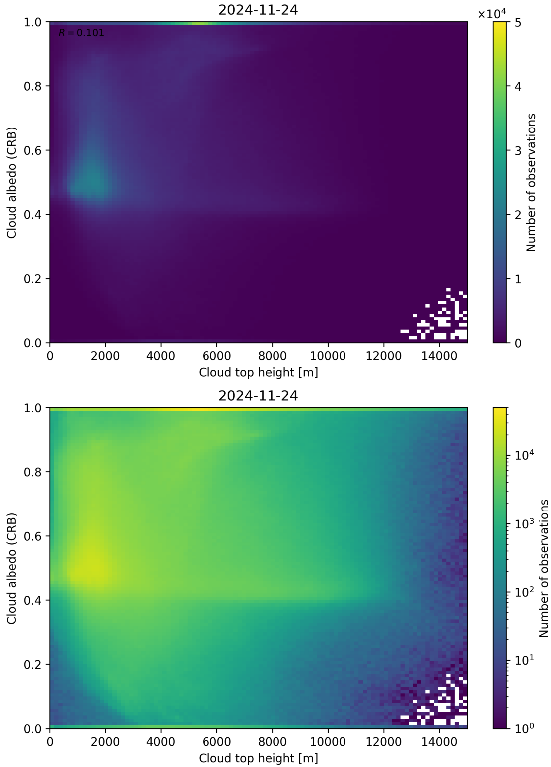
Figure 86: Scatter density plot of “Cloud top height” against “Cloud albedo (CRB)” for 2024-11-23 to 2024-11-25.
