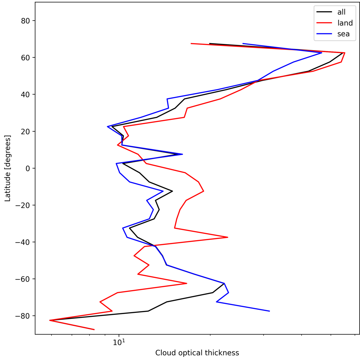
Figure 25: Zonal average of “Cloud optical thickness” for 2024-11-23 to 2024-11-25.
