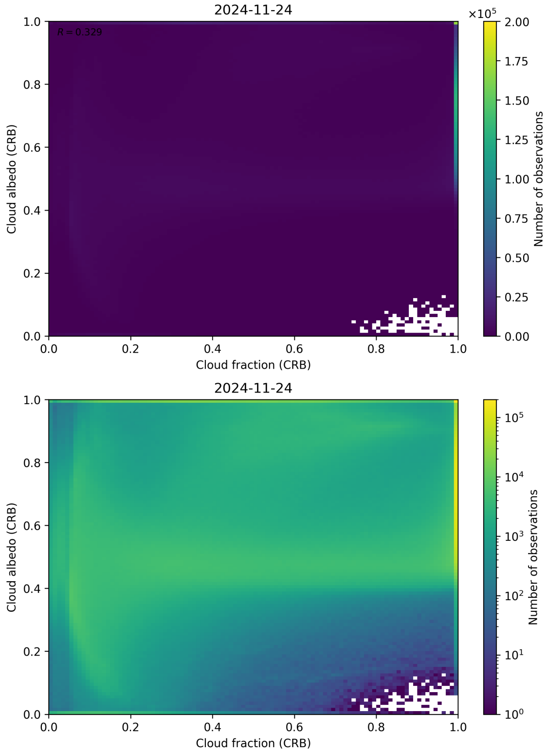
Figure 77: Scatter density plot of “Cloud fraction (CRB)” against “Cloud albedo (CRB)” for 2024-11-23 to 2024-11-25.
