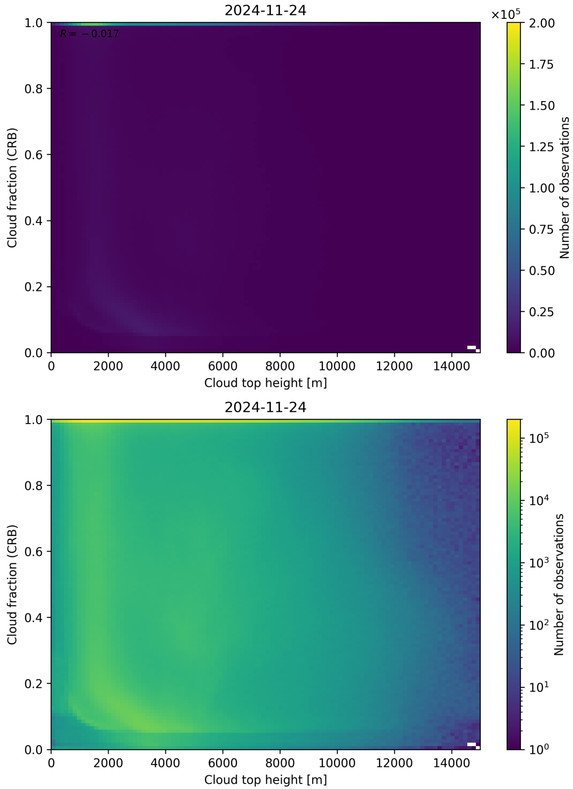
Figure 88: Scatter density plot of “Cloud top height” against “Cloud fraction (CRB)” for 2024-11-23 to 2024-11-25.
