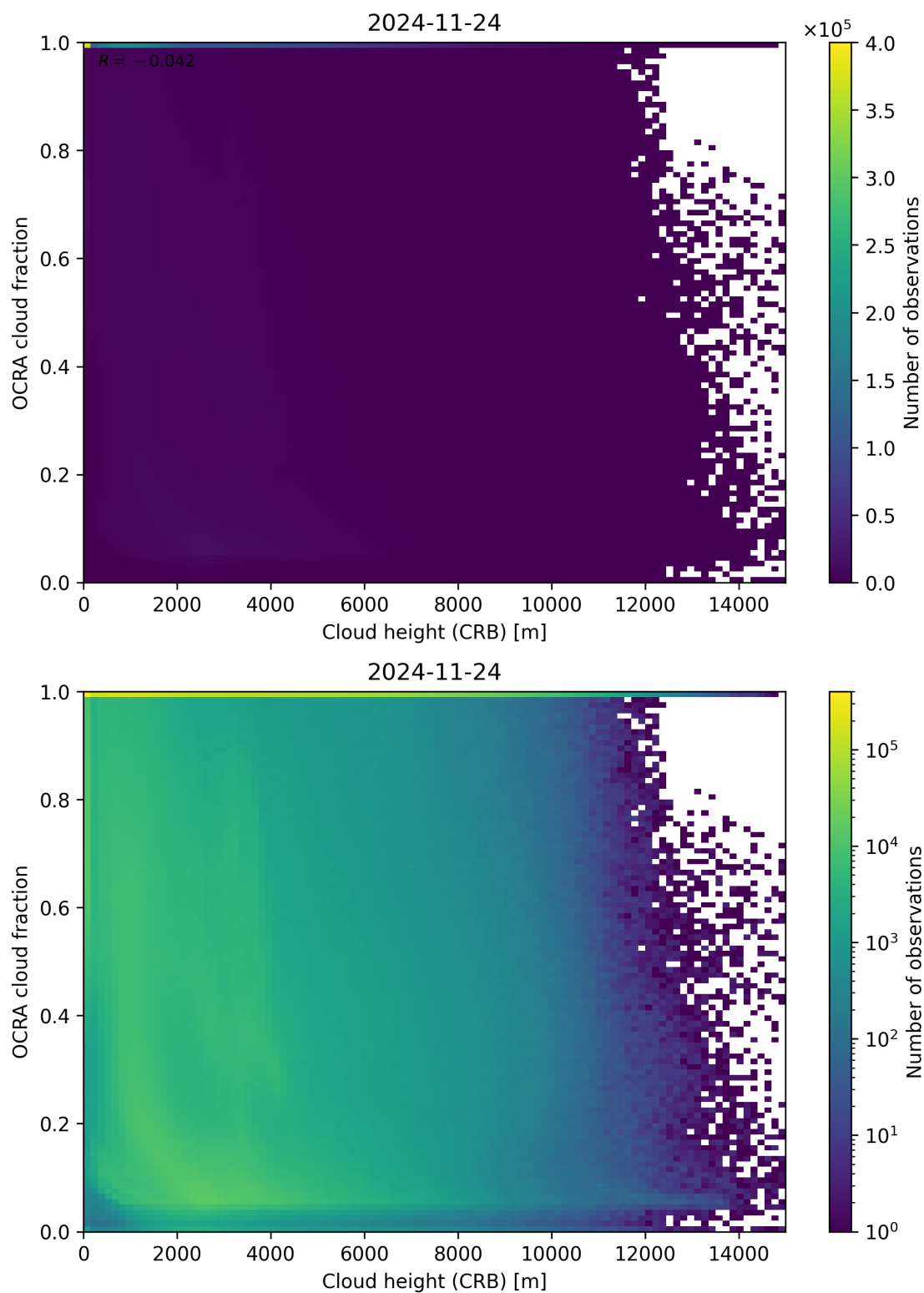
Figure 81: Scatter density plot of “Cloud height (CRB)” against “OCRA cloud fraction” for 2024-11-23 to 2024-11-25.
