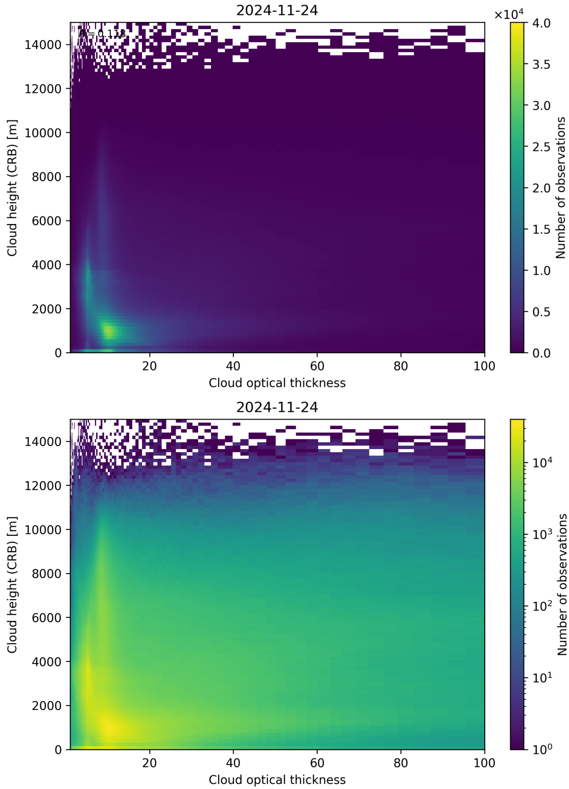
Figure 85: Scatter density plot of “Cloud optical thickness” against “Cloud height (CRB)” for 2024-11-23 to 2024-11-25.
