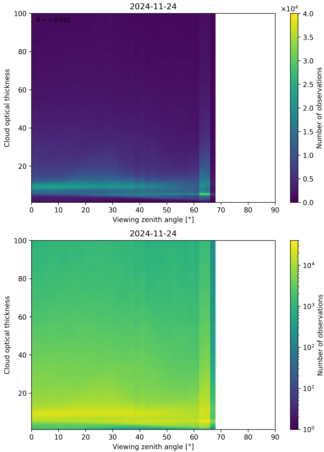
Figure 111: Scatter density plot of “Viewing zenith angle” against “Cloud optical thickness” for 2024-11-23 to 2024-11-25.
