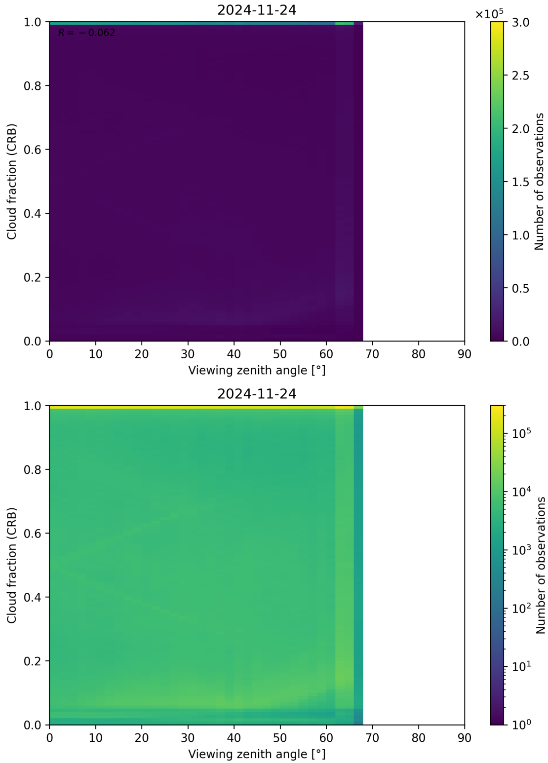
Figure 109: Scatter density plot of “Viewing zenith angle” against “Cloud fraction (CRB)” for 2024-11-23 to 2024-11-25.
