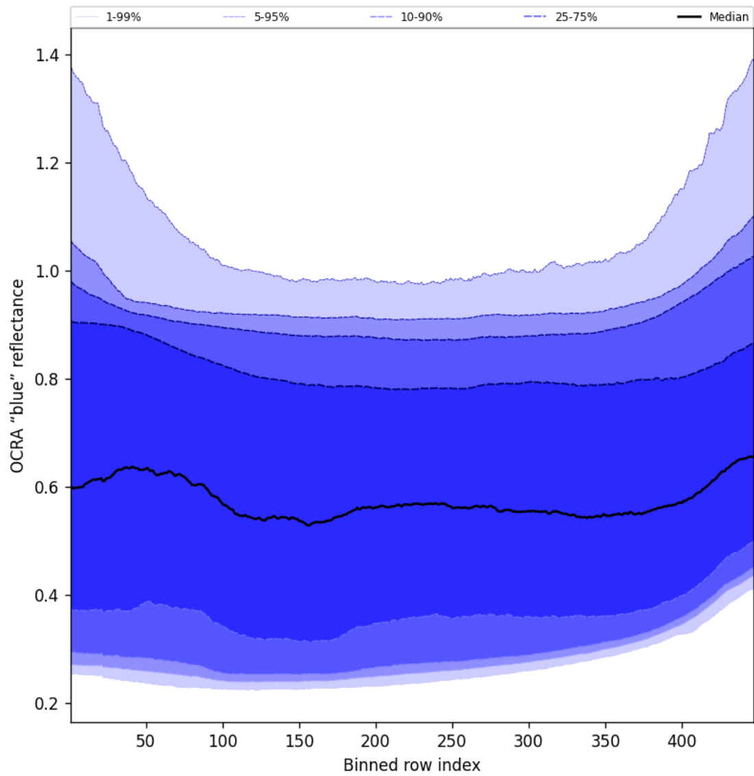
Figure 67: Along track statistics of “OCRA “blue” reflectance” for 2024-11-23 to 2024-11-25
