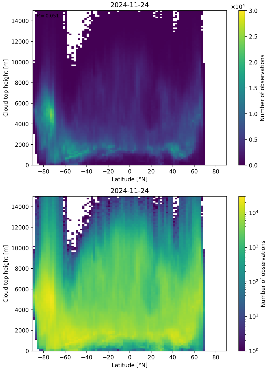
Figure 97: Scatter density plot of “Latitude” against “Cloud top height” for 2024-11-23 to 2024-11-25.
