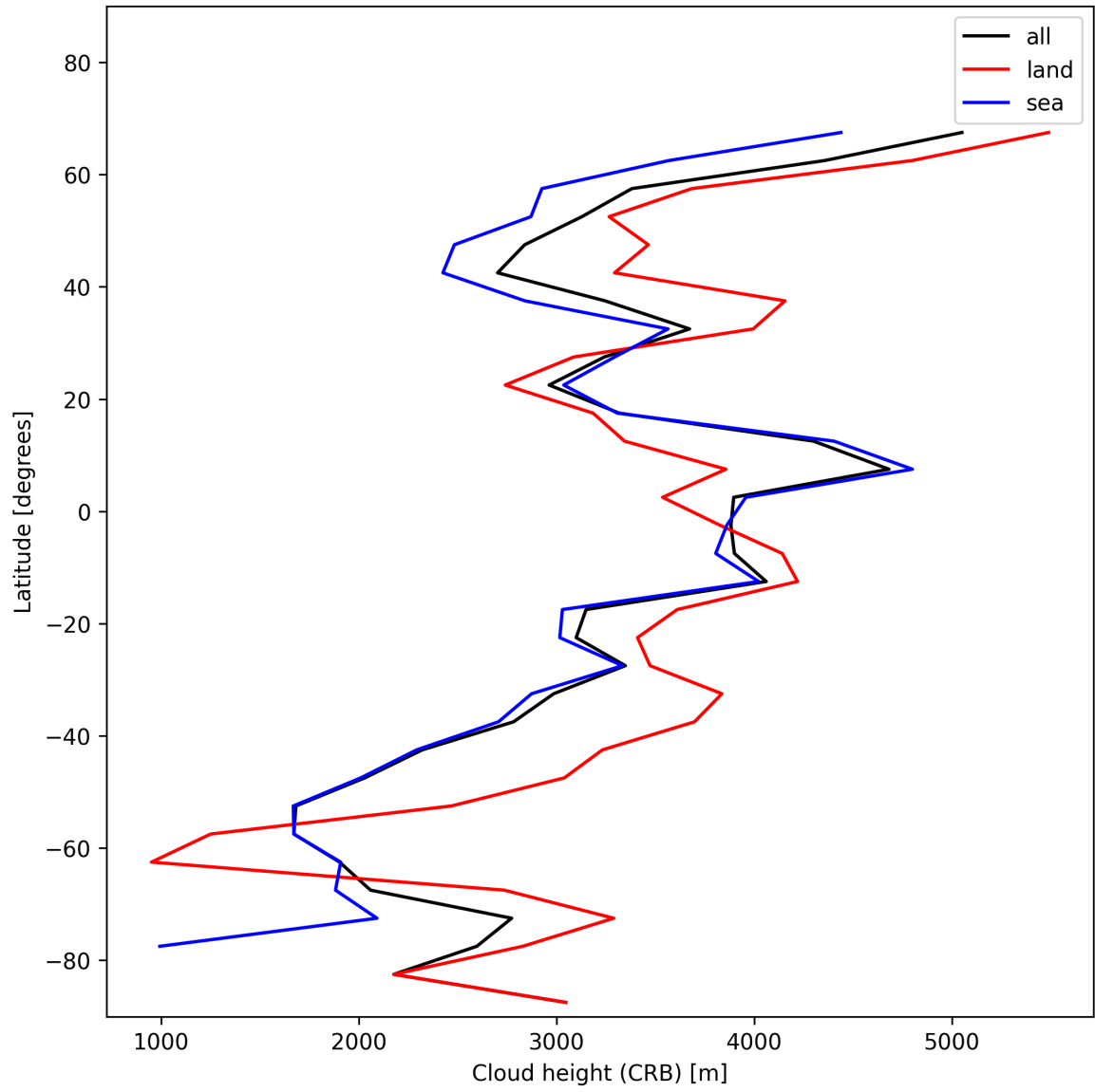
Figure 27: Zonal average of “Cloud height (CRB)” for 2024-11-23 to 2024-11-25.
