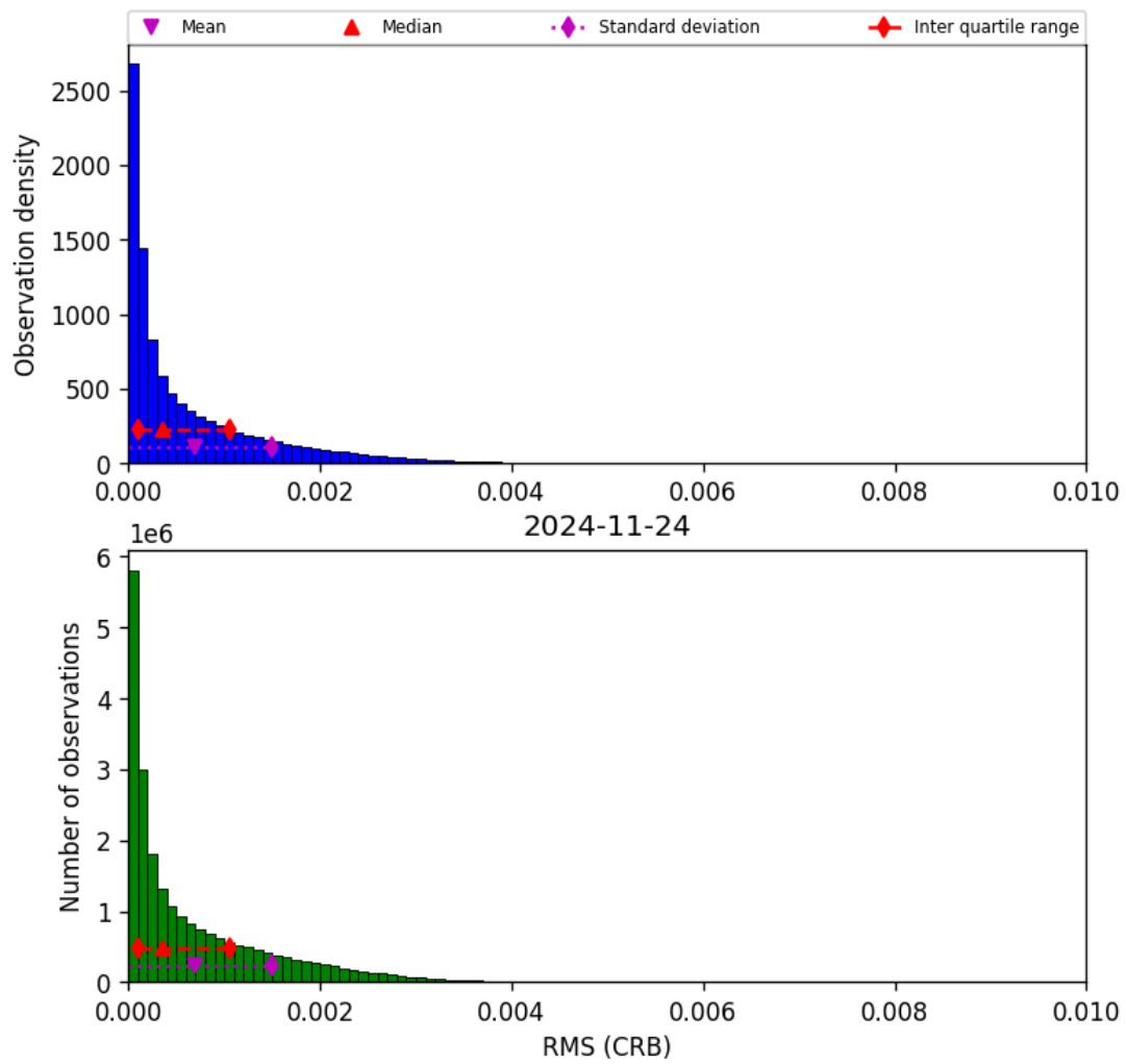
Figure 48: Histogram of “RMS (CRB)” for 2024-11-23 to 2024-11-25
