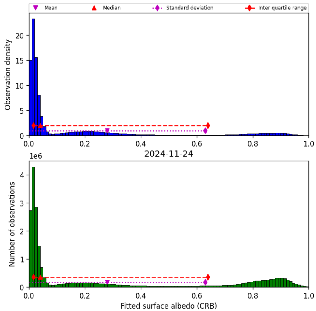
Figure 46: Histogram of “Fitted surface albedo (CRB)” for 2024-11-23 to 2024-11-25
