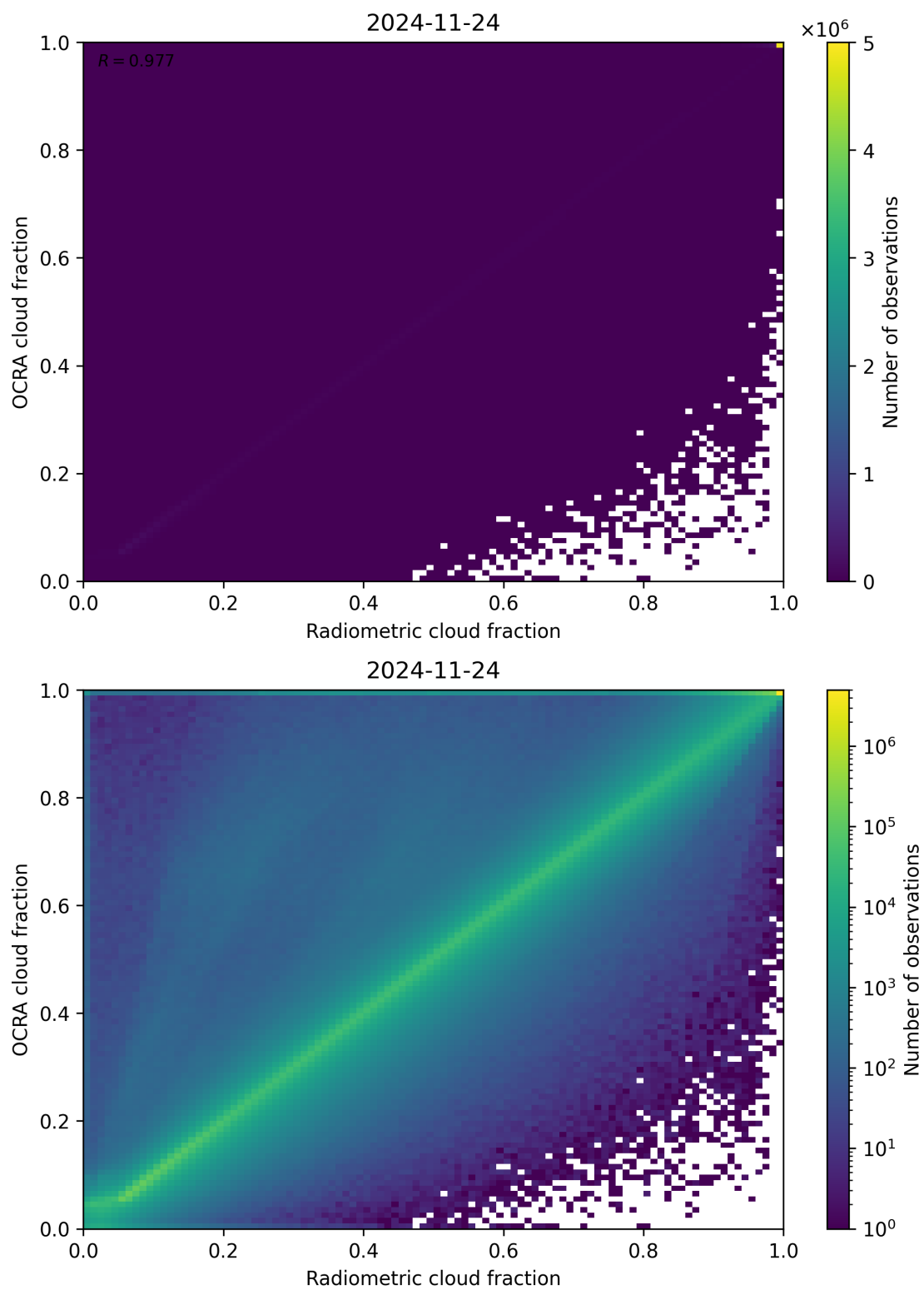
Figure 72: Scatter density plot of “Radiometric cloud fraction” against “OCRA cloud fraction” for 2024-11-23 to 2024-11-25.
