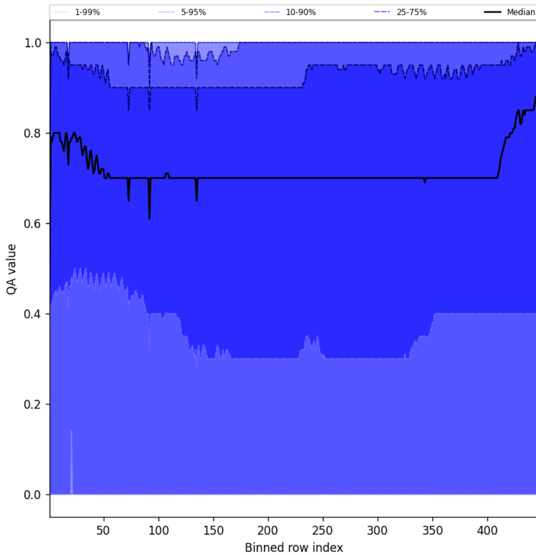
Figure 54: Along track statistics of “QA value” for 2024-11-23 to 2024-11-25
