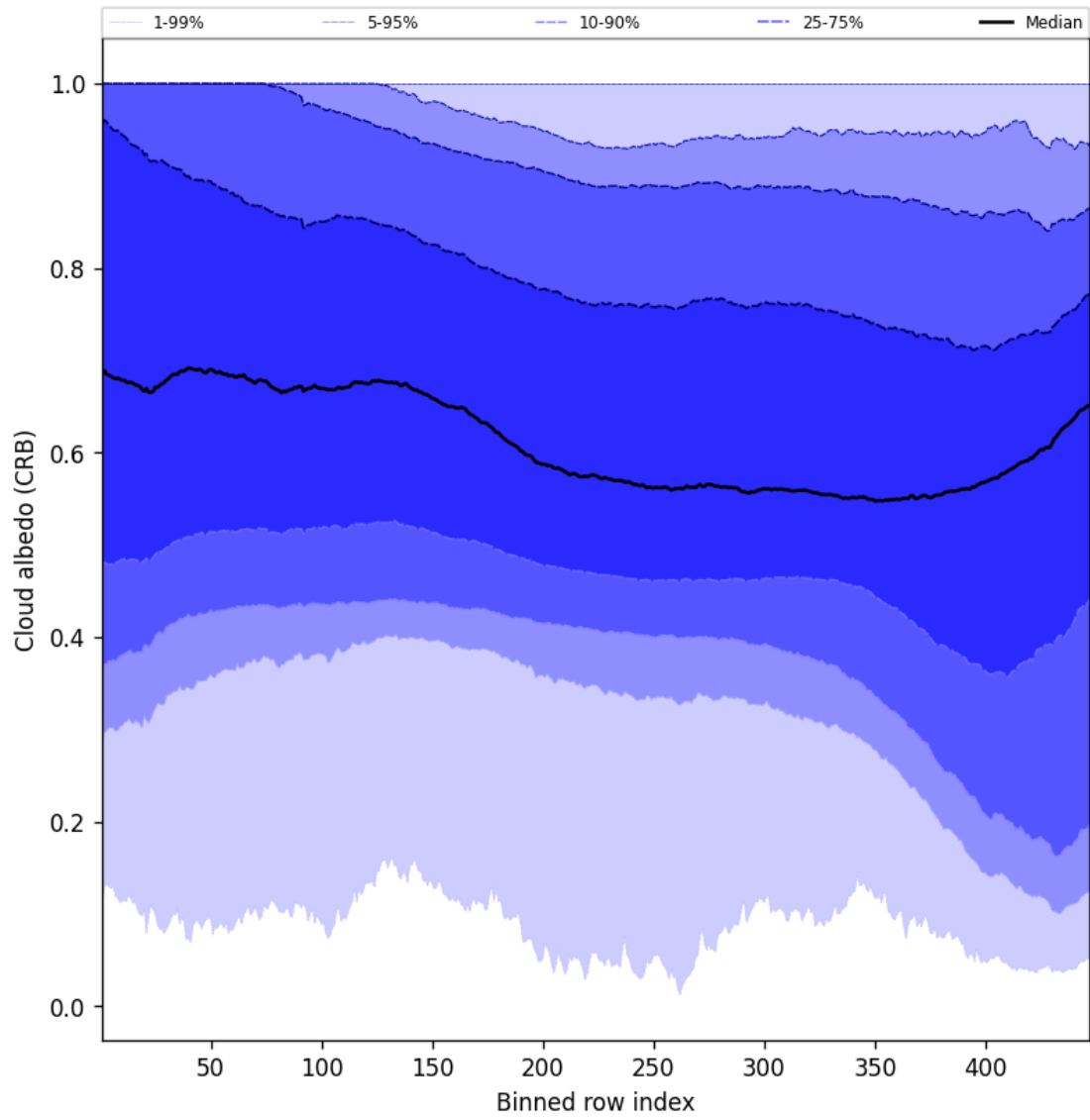
Figure 60: Along track statistics of “Cloud albedo (CRB)” for 2024-11-23 to 2024-11-25
