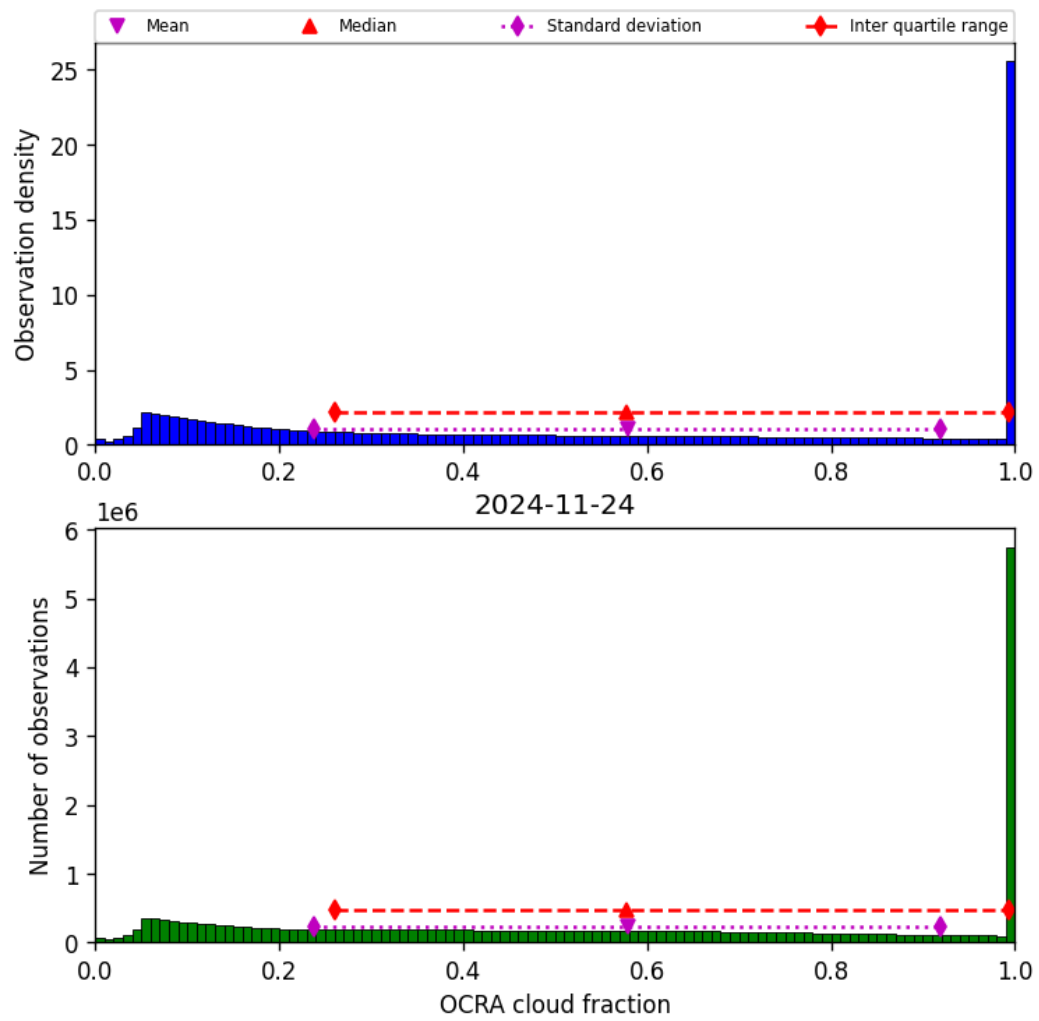
Figure 50: Histogram of “OCRA cloud fraction” for 2024-11-23 to 2024-11-25
