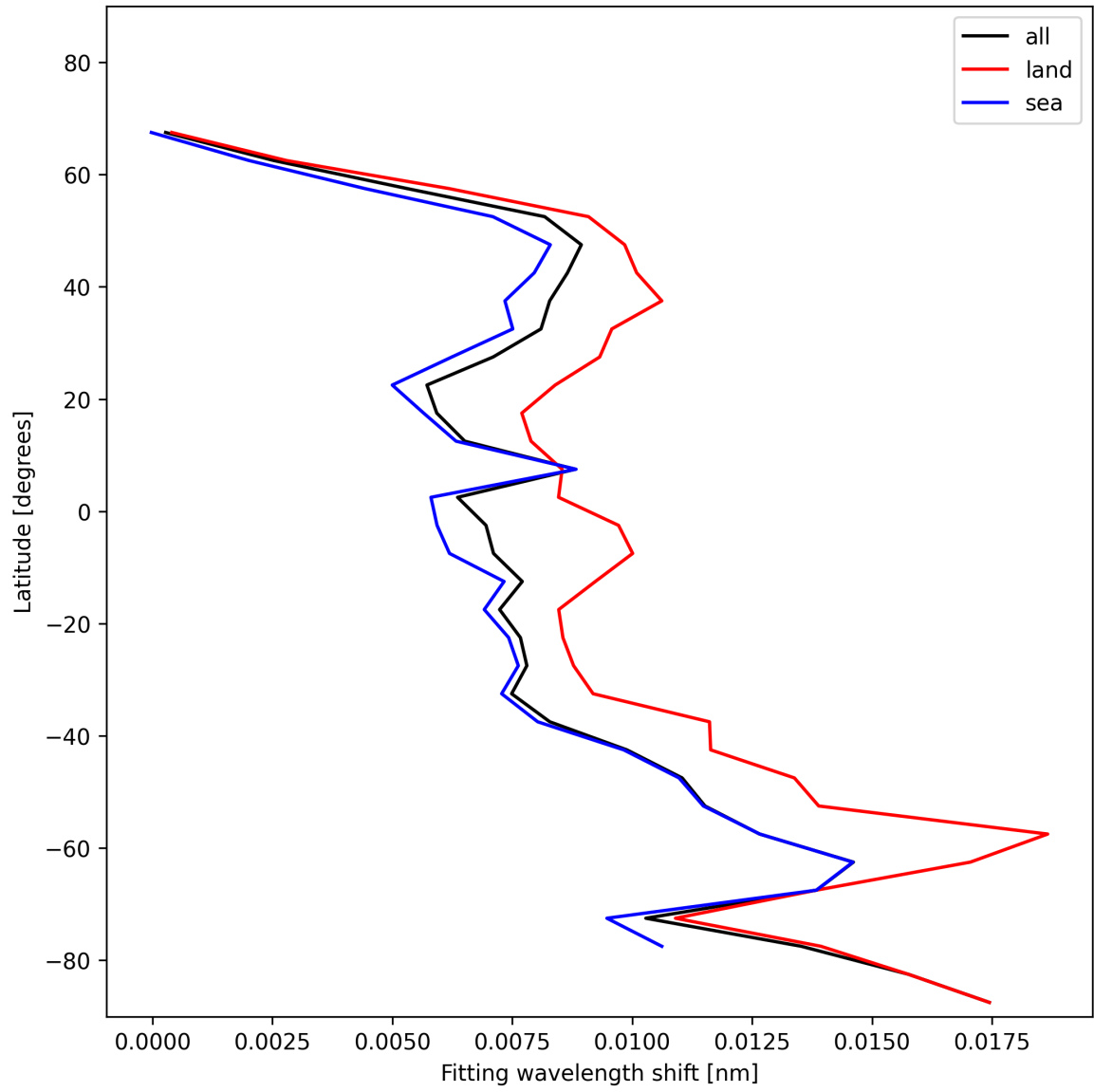
Figure 33: Zonal average of “Fitting wavelength shift” for 2024-11-23 to 2024-11-25.
