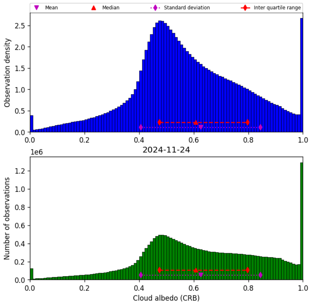
Figure 44: Histogram of “Cloud albedo (CRB)” for 2024-11-23 to 2024-11-25
