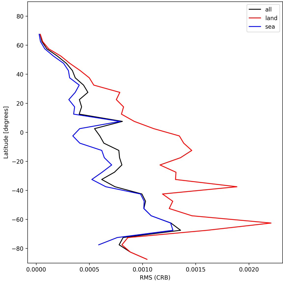
Figure 32: Zonal average of “RMS (CRB)” for 2024-11-23 to 2024-11-25.
