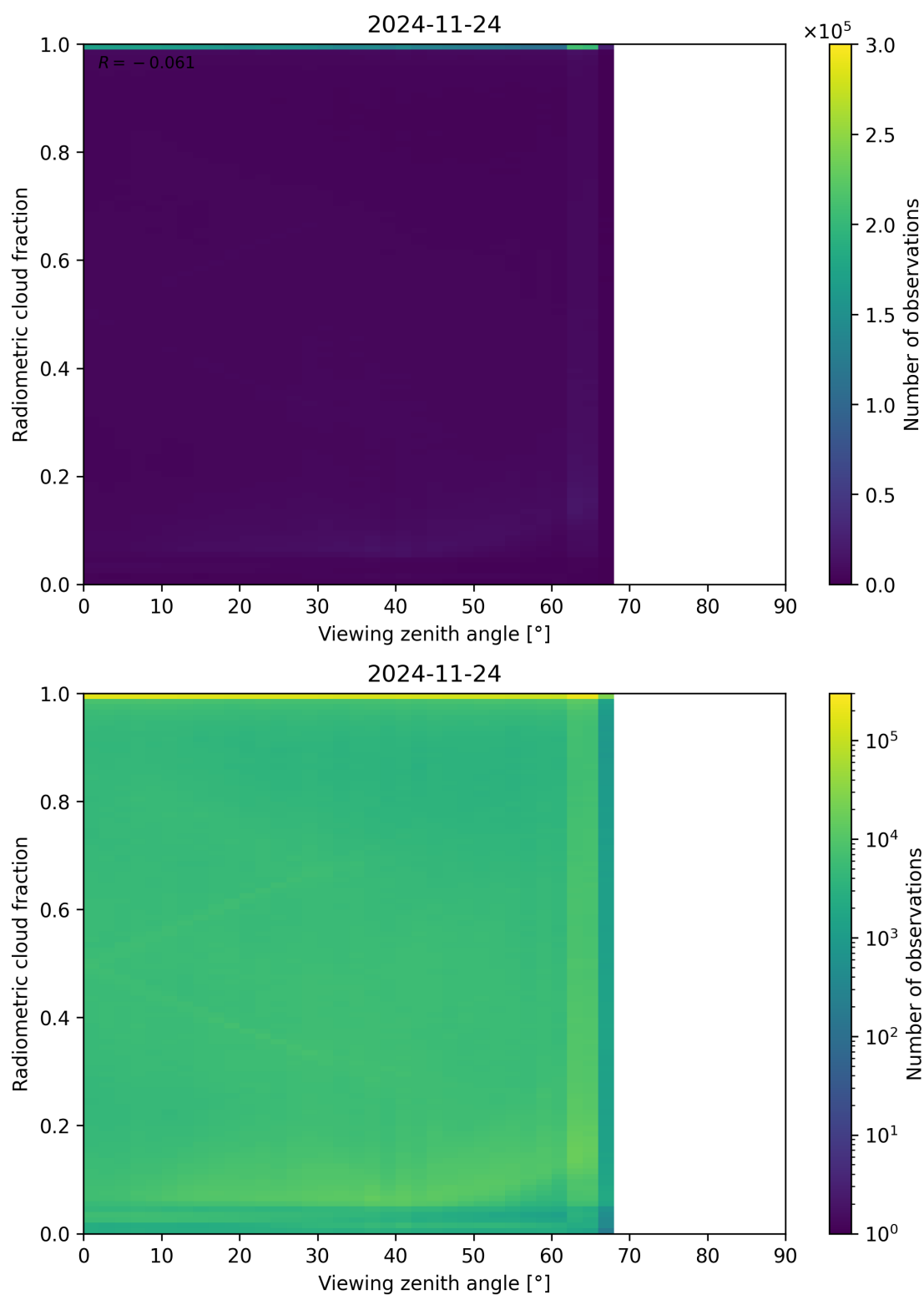
Figure 107: Scatter density plot of “Viewing zenith angle” against “Radiometric cloud fraction” for 2024-11-23 to 2024-11-25.
