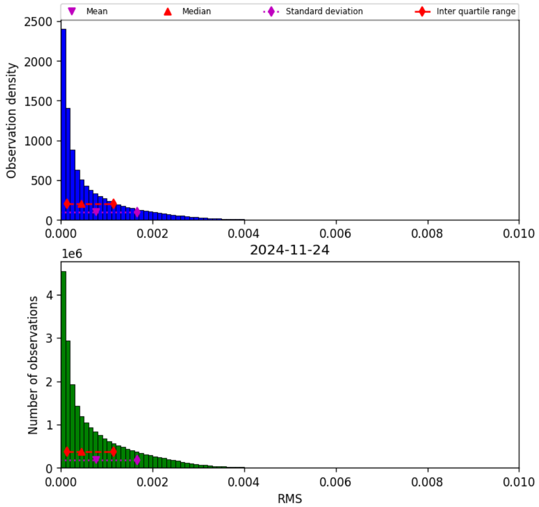
Figure 47: Histogram of “RMS” for 2024-11-23 to 2024-11-25
