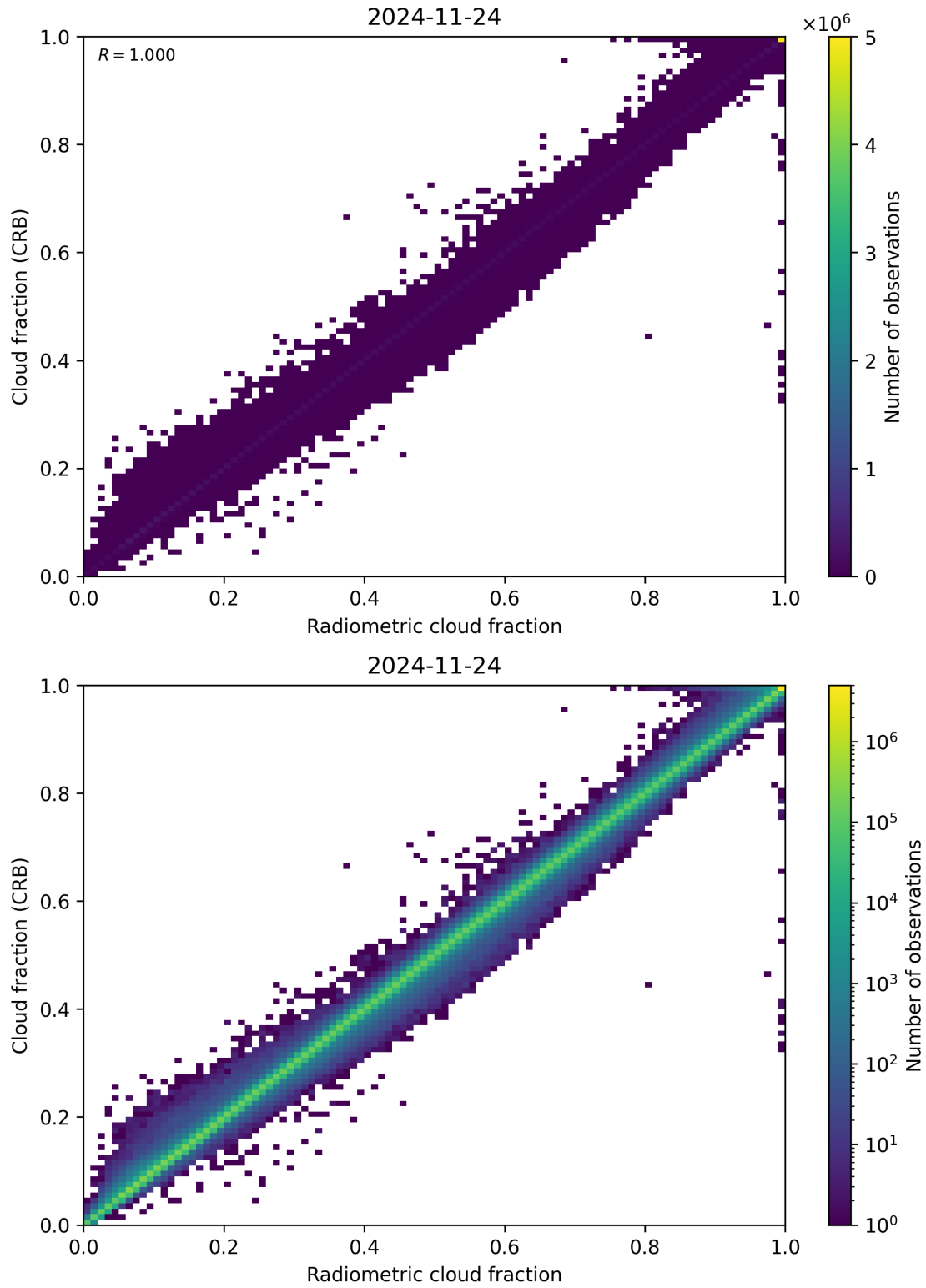
Figure 73: Scatter density plot of “Radiometric cloud fraction” against “Cloud fraction (CRB)” for 2024-11-23 to 2024-11-25.
