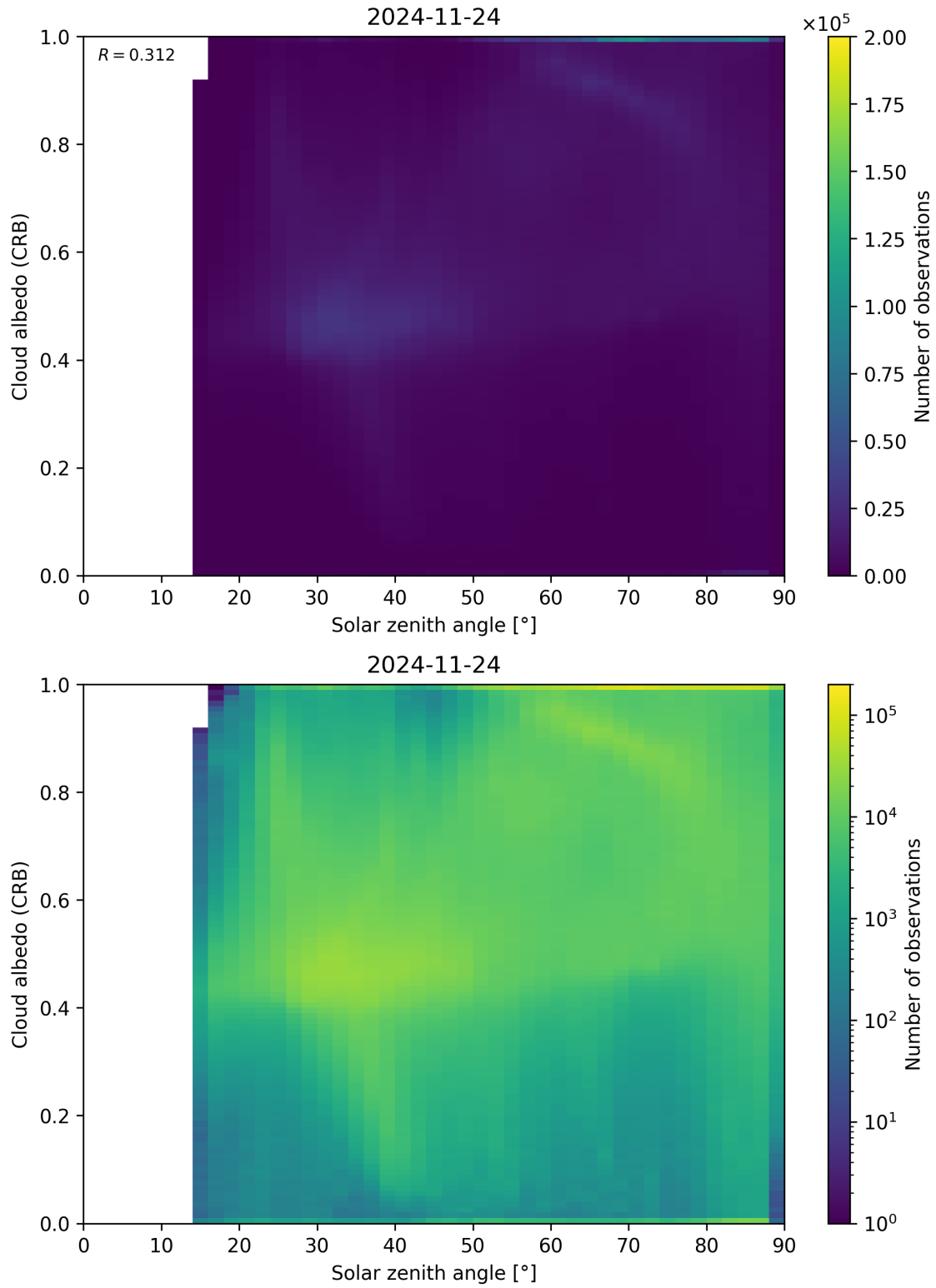
Figure 98: Scatter density plot of “Solar zenith angle” against “Cloud albedo (CRB)” for 2024-11-23 to 2024-11-25.
