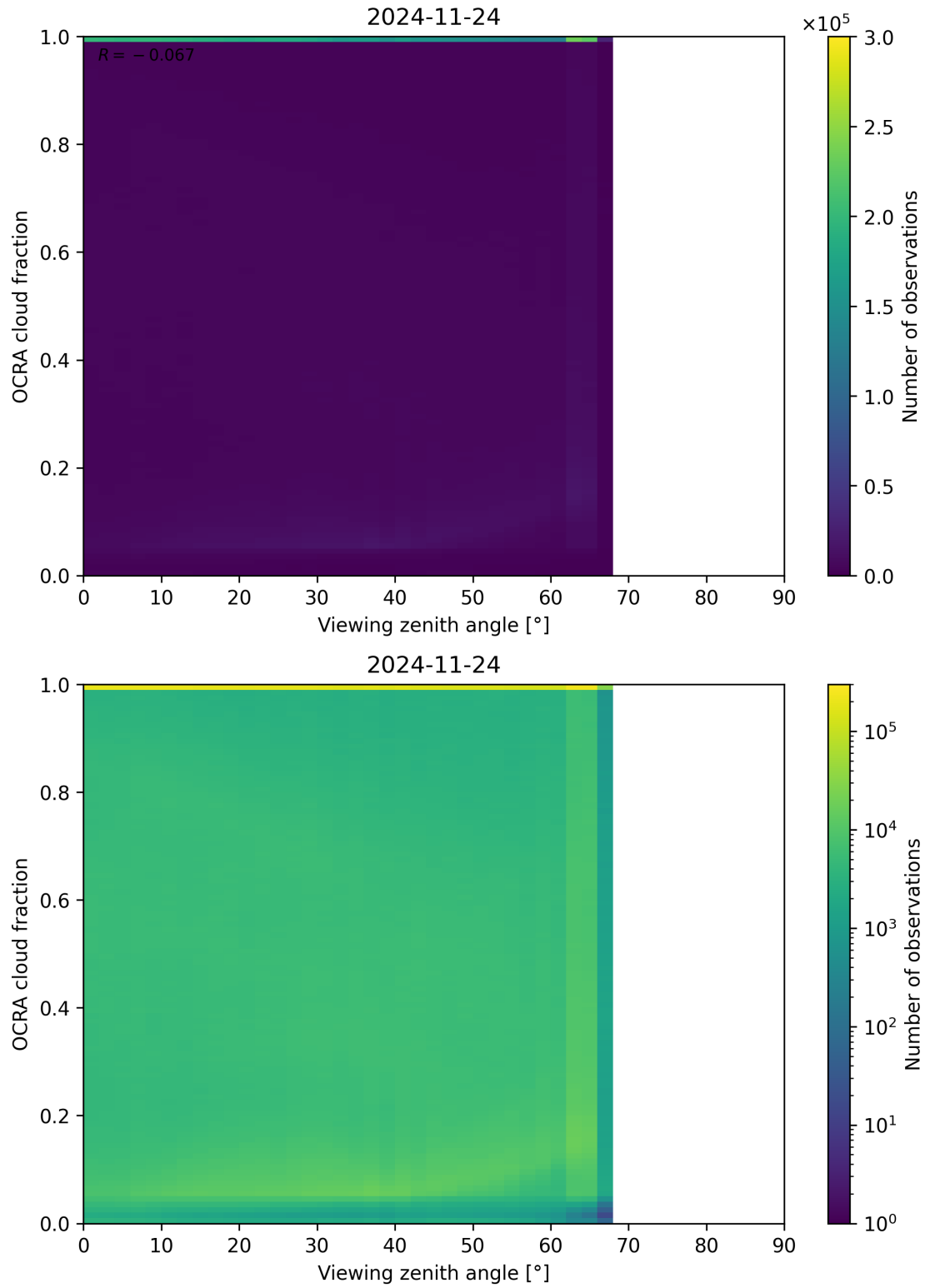
Figure 108: Scatter density plot of “Viewing zenith angle” against “OCRA cloud fraction” for 2024-11-23 to 2024-11-25.
