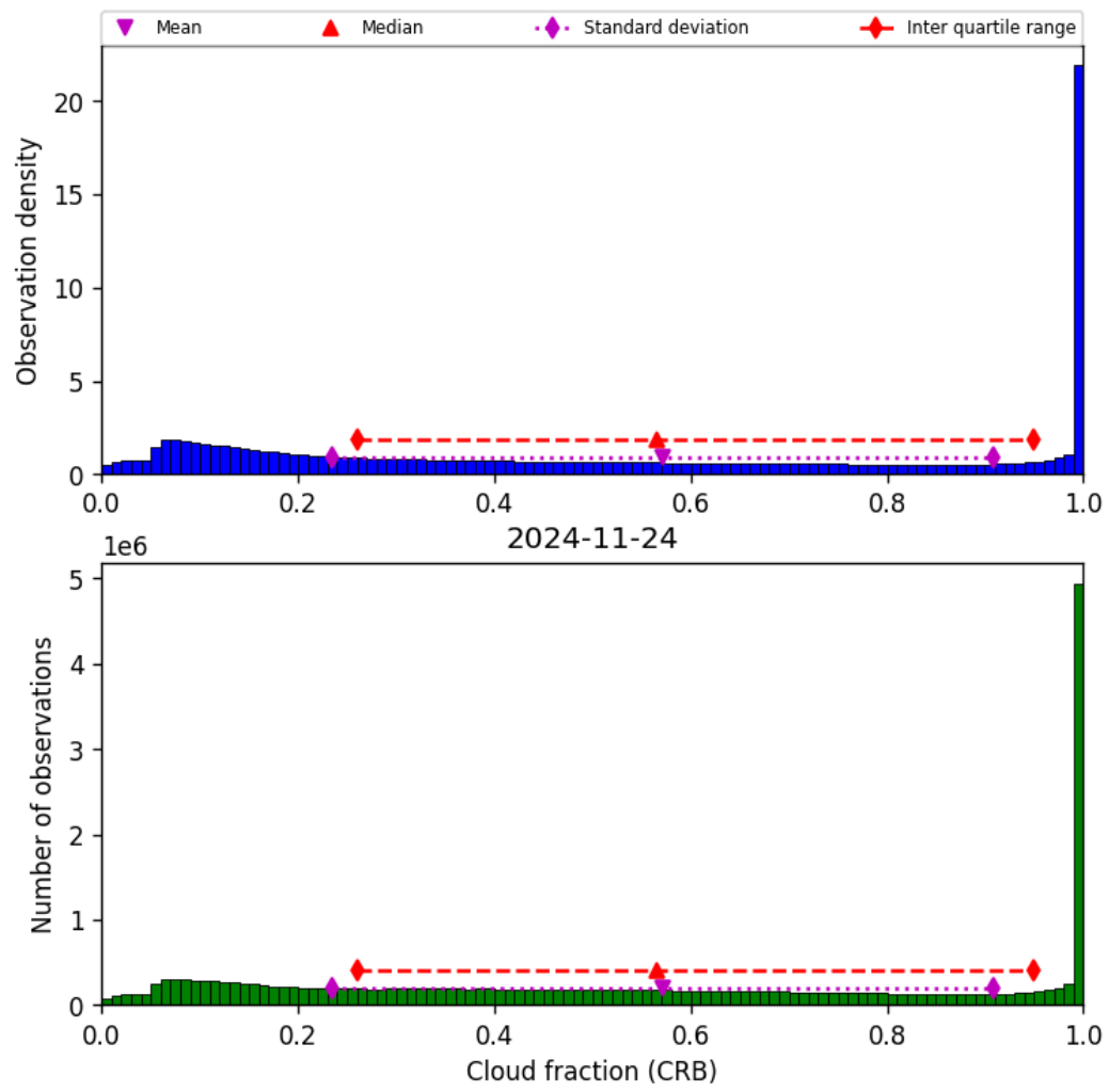
Figure 42: Histogram of “Cloud fraction (CRB)” for 2024-11-23 to 2024-11-25
