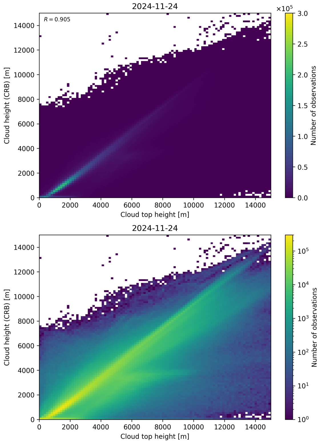
Figure 89: Scatter density plot of “Cloud top height” against “Cloud height (CRB)” for 2024-11-23 to 2024-11-25.
