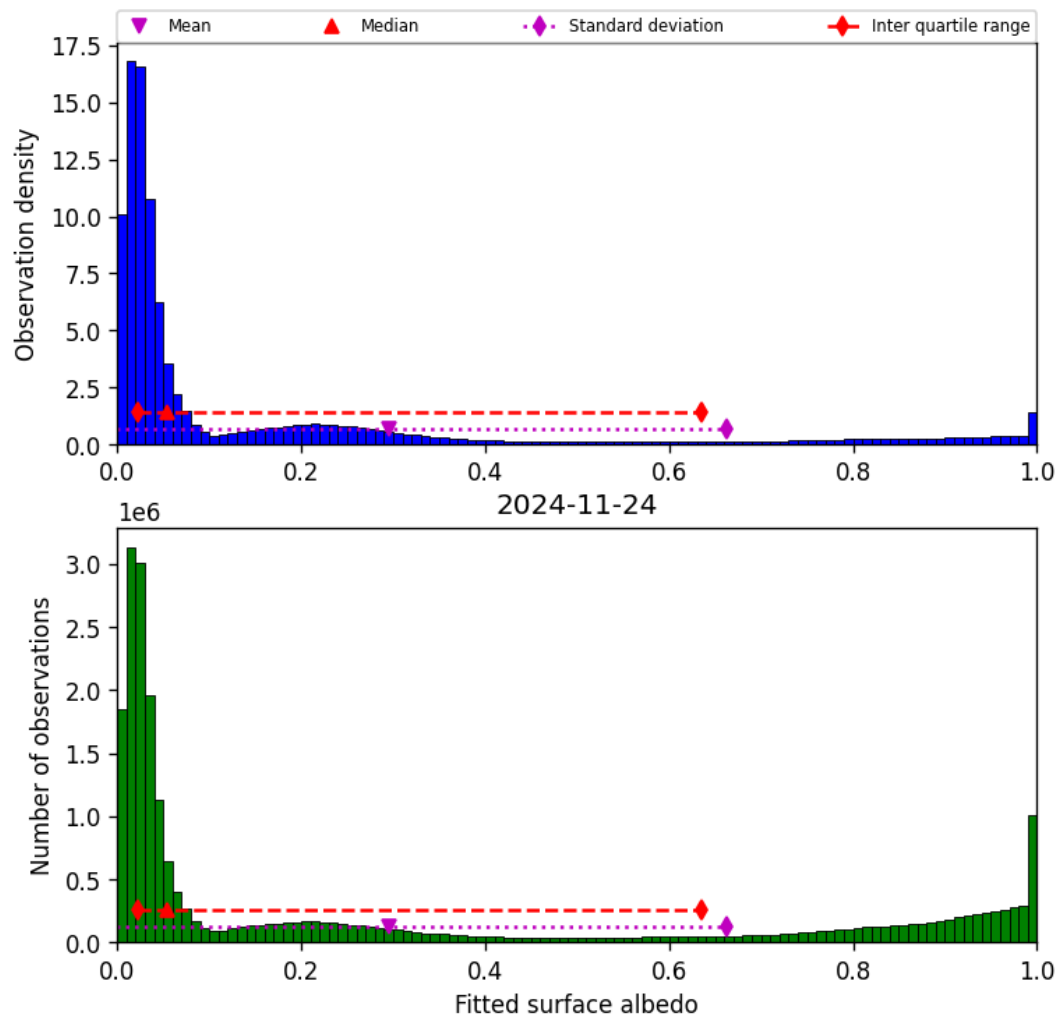
Figure 45: Histogram of “Fitted surface albedo” for 2024-11-23 to 2024-11-25
