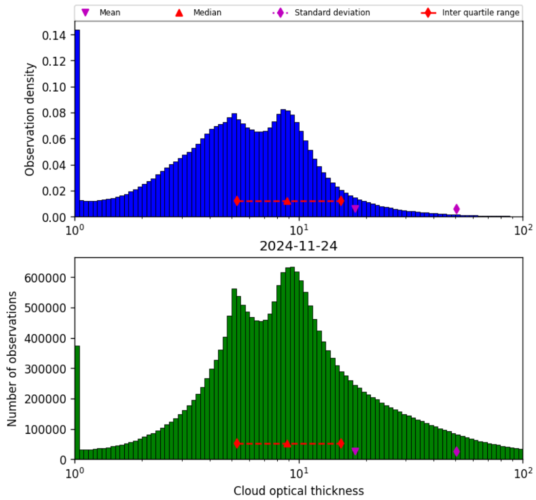
Figure 41: Histogram of “Cloud optical thickness” for 2024-11-23 to 2024-11-25
