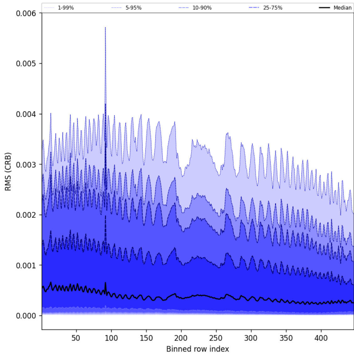
Figure 64: Along track statistics of “RMS (CRB)” for 2024-11-23 to 2024-11-25
