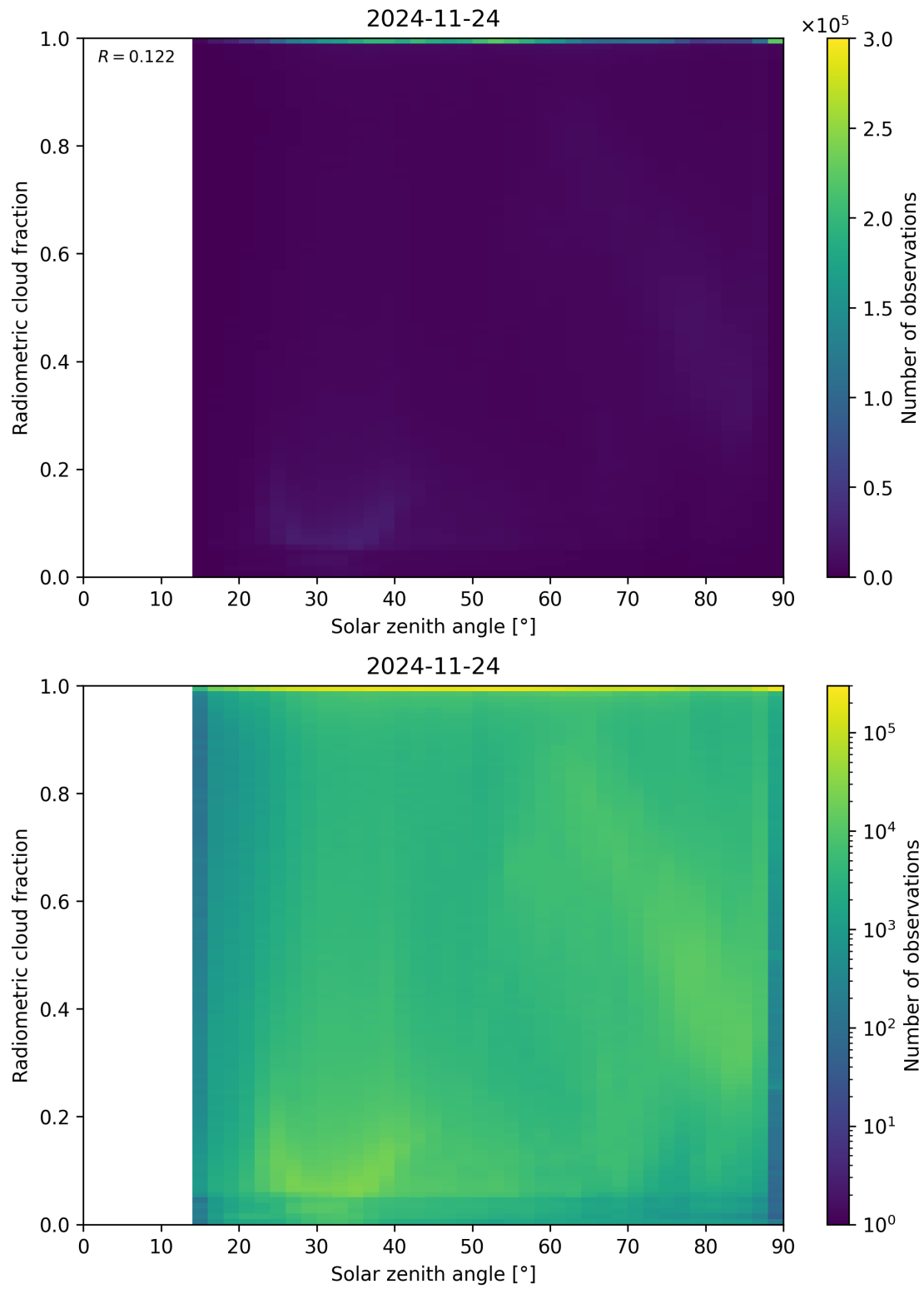
Figure 99: Scatter density plot of “Solar zenith angle” against “Radiometric cloud fraction” for 2024-11-23 to 2024-11-25.
