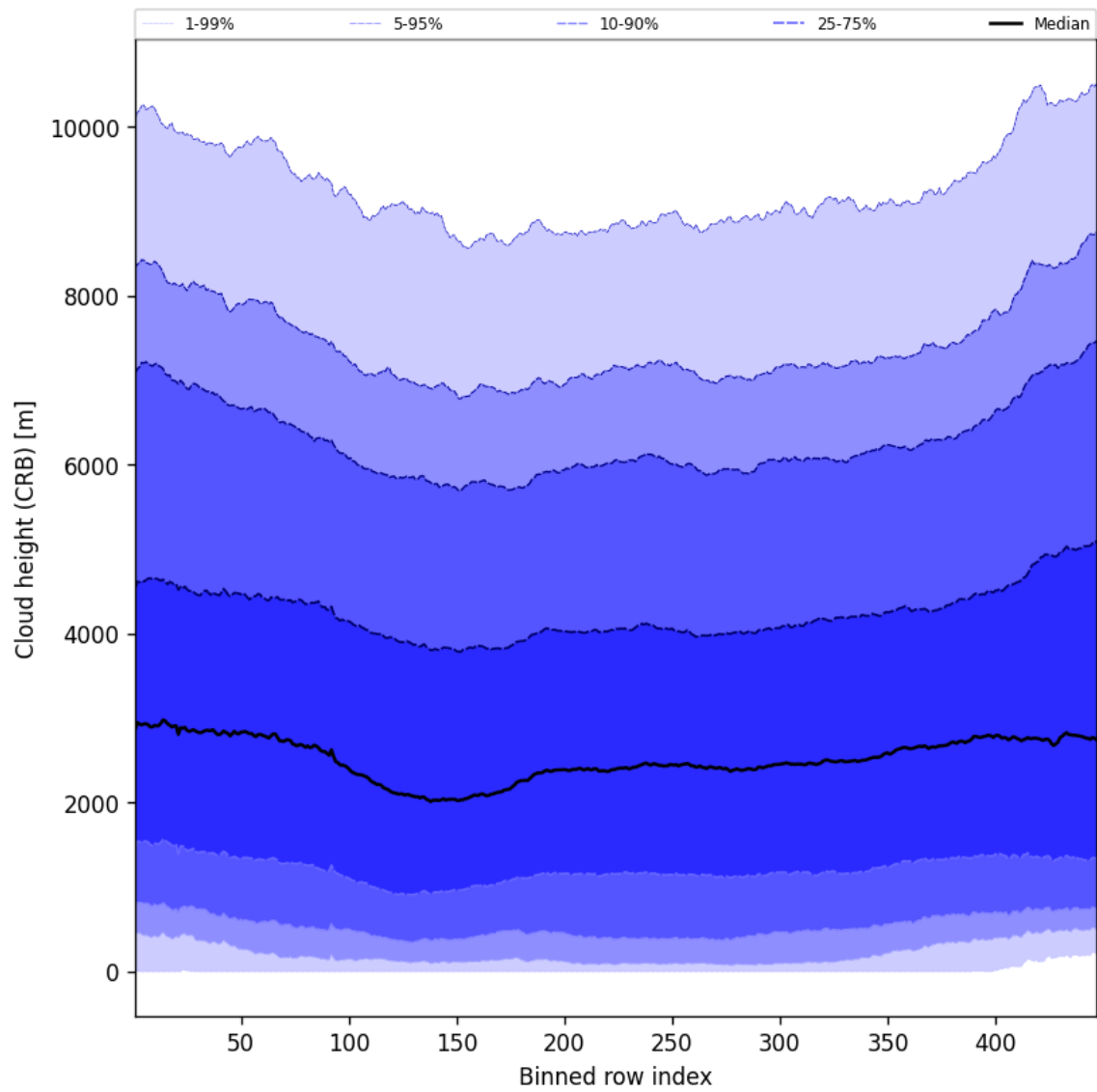
Figure 59: Along track statistics of “Cloud height (CRB)” for 2024-11-23 to 2024-11-25
