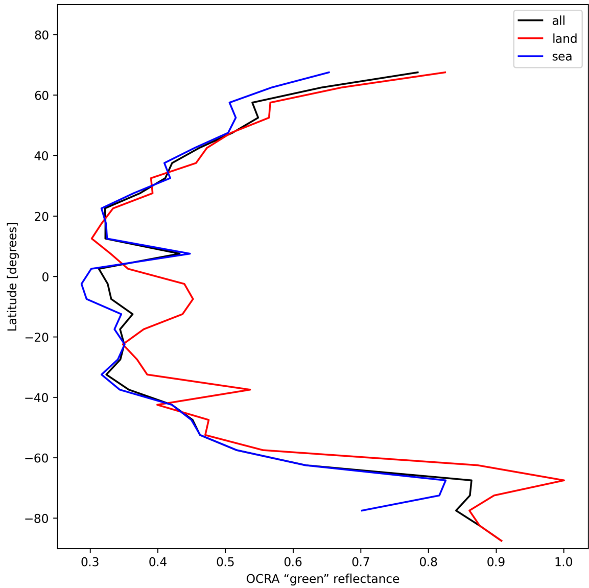
Figure 36: Zonal average of “OCRA “green” reflectance” for 2024-11-23 to 2024-11-25.
