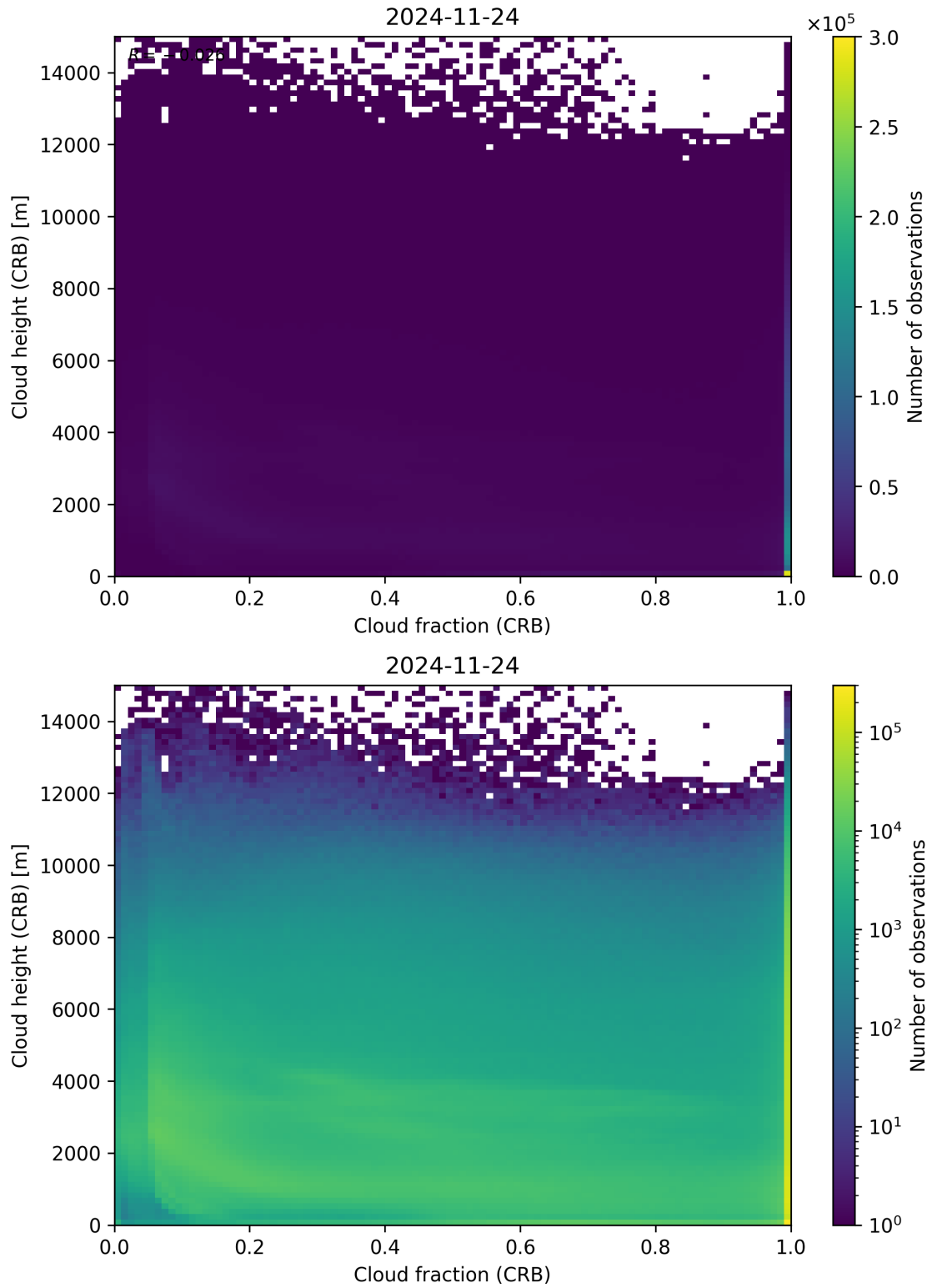
Figure 79: Scatter density plot of “Cloud fraction (CRB)” against “Cloud height (CRB)” for 2024-11-23 to 2024-11-25.
