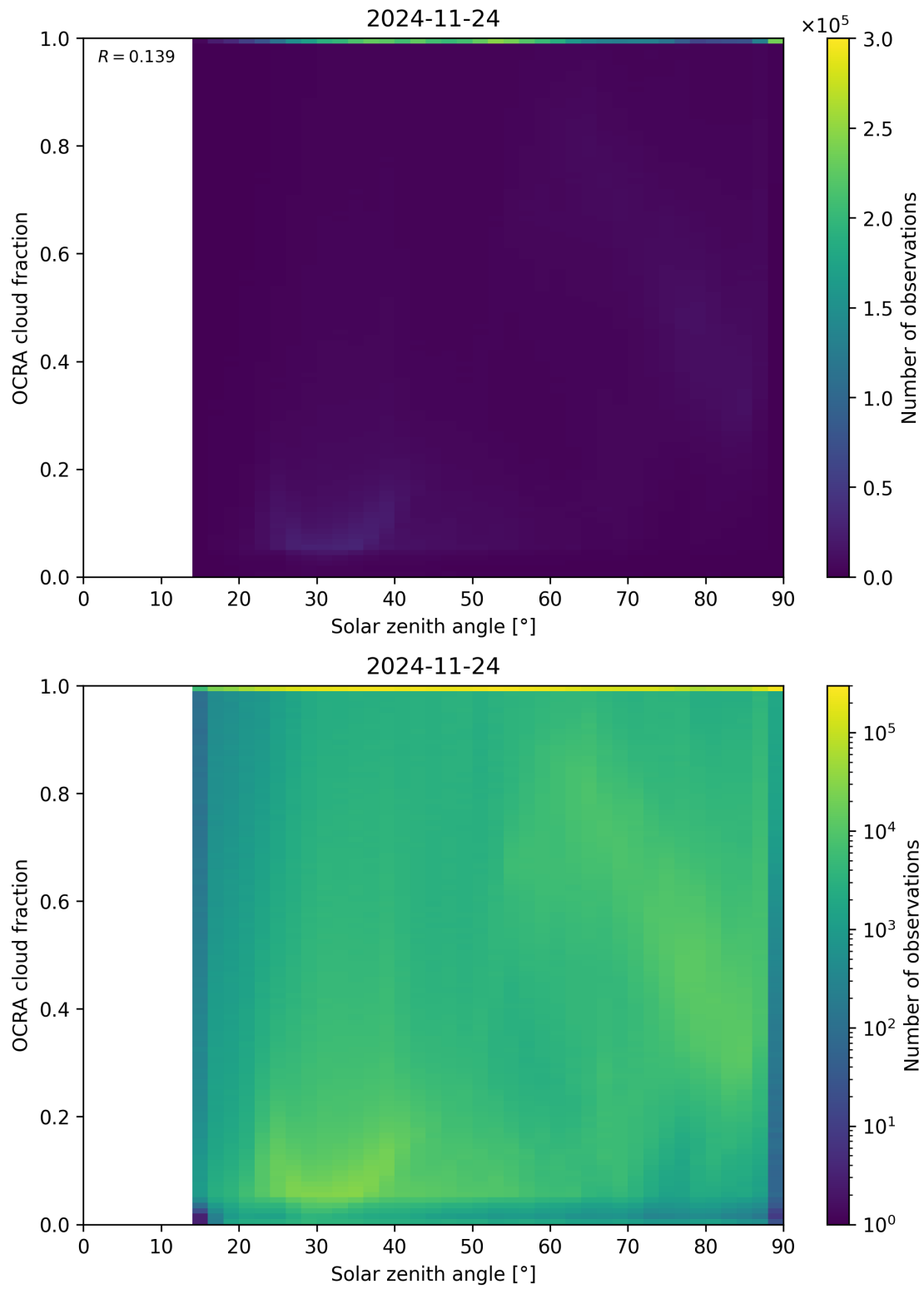
Figure 100: Scatter density plot of “Solar zenith angle” against “OCRA cloud fraction” for 2024-11-23 to 2024-11-25.
