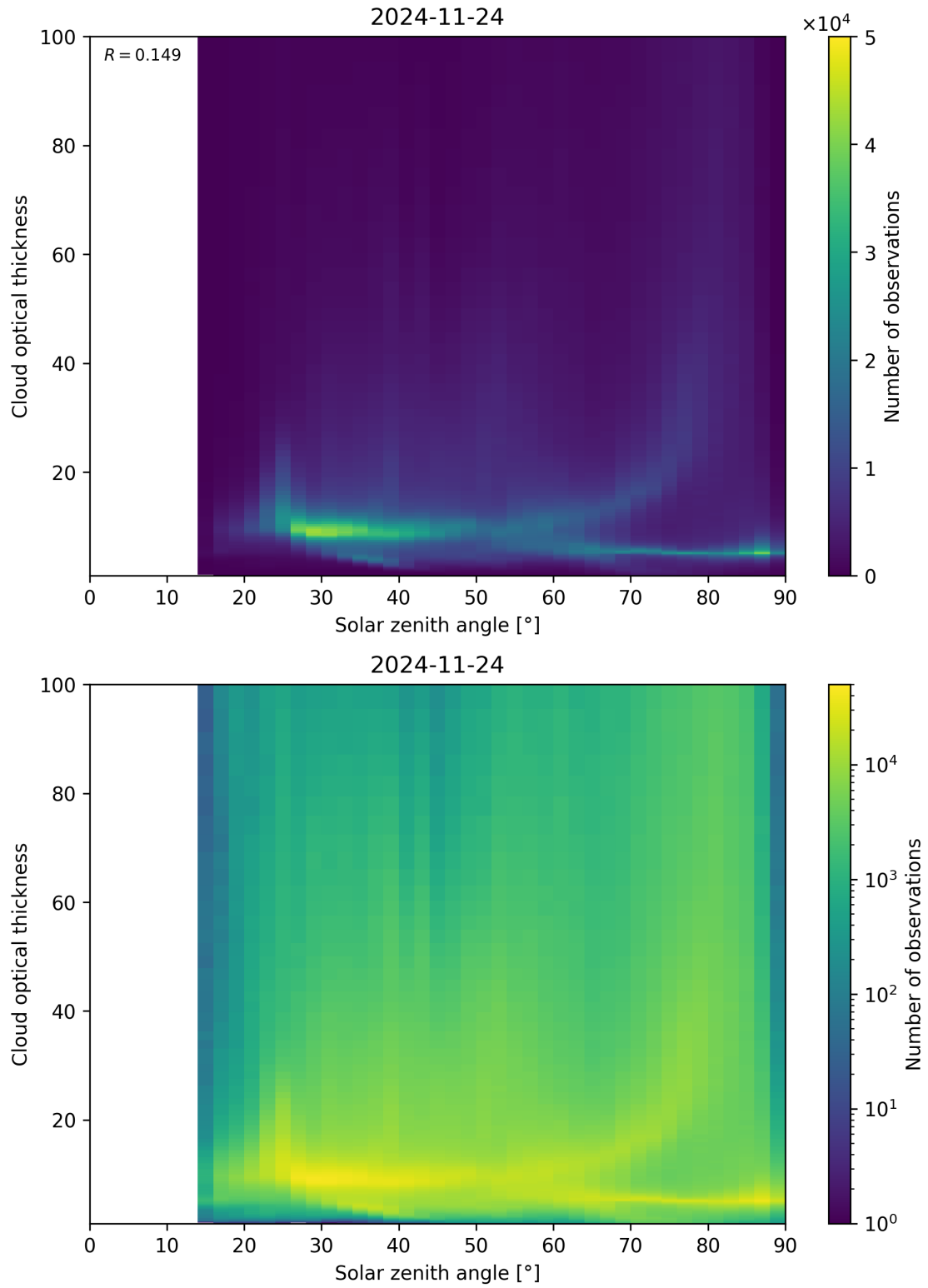
Figure 103: Scatter density plot of “Solar zenith angle” against “Cloud optical thickness” for 2024-11-23 to 2024-11-25.
