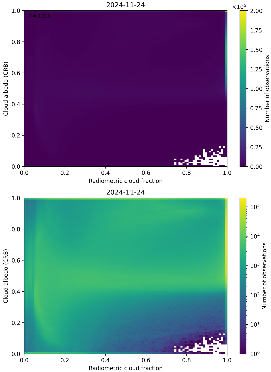
Figure 71: Scatter density plot of “Radiometric cloud fraction” against “Cloud albedo (CRB)” for 2024-11-23 to 2024-11-25.
