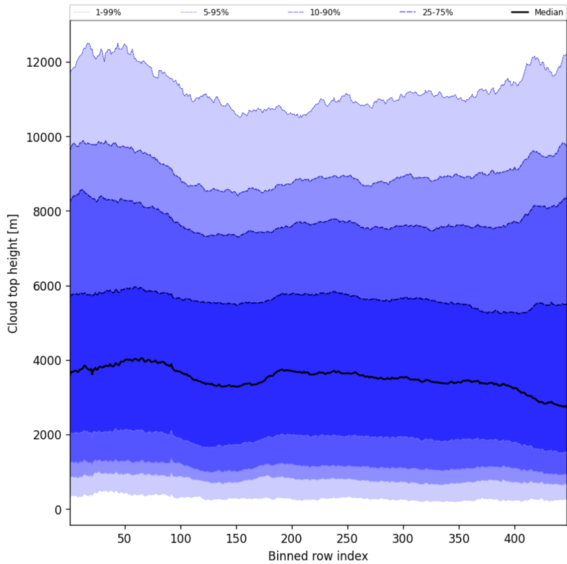
Figure 56: Along track statistics of “Cloud top height” for 2024-11-23 to 2024-11-25
