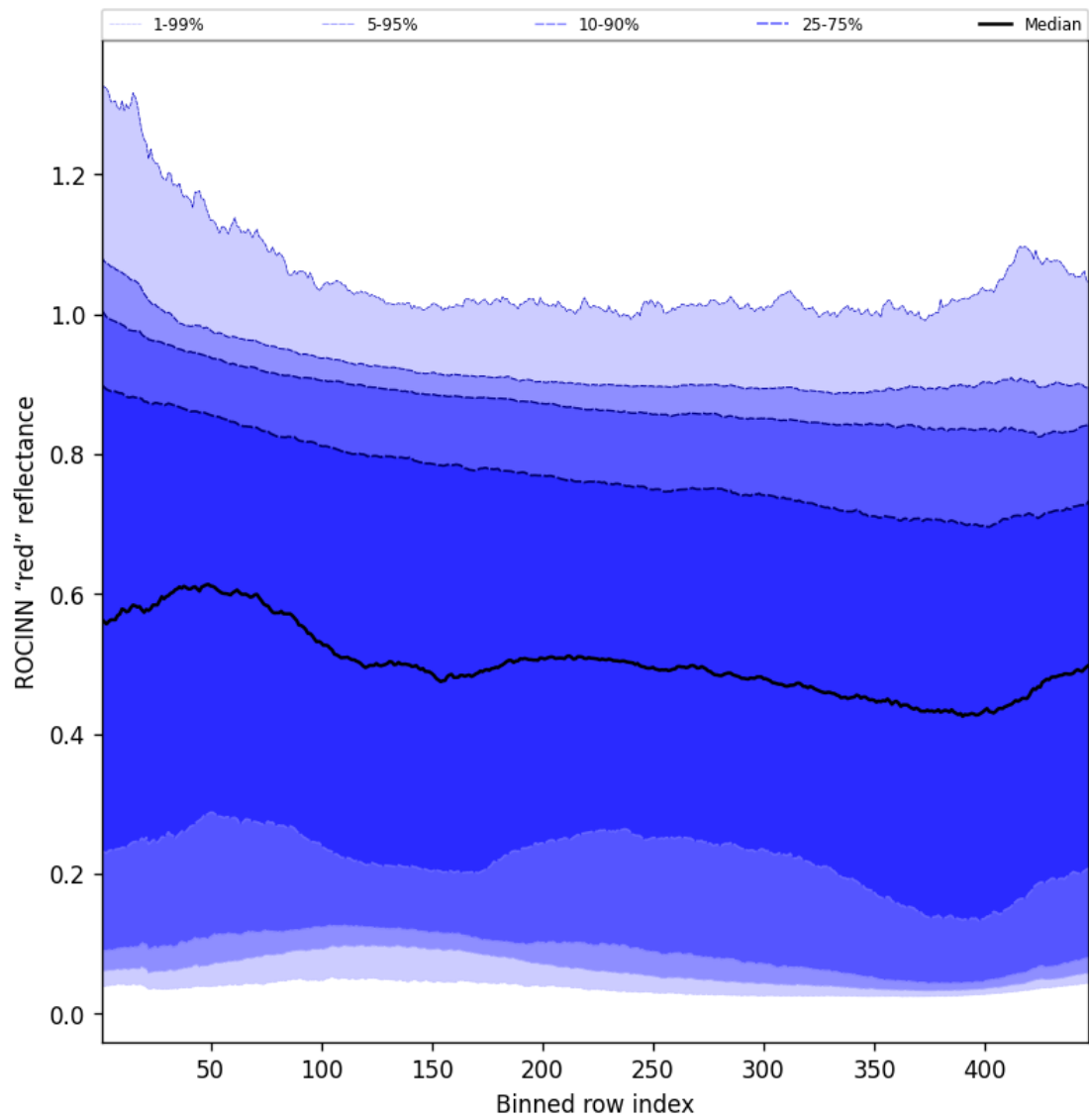
Figure 69: Along track statistics of “ROCINN “red” reflectance” for 2024-11-23 to 2024-11-25
