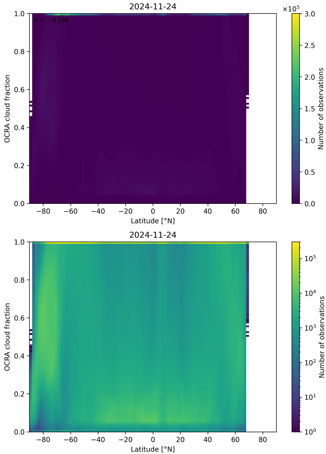
Figure 93: Scatter density plot of “Latitude” against “OCRA cloud fraction” for 2024-11-23 to 2024-11-25.
