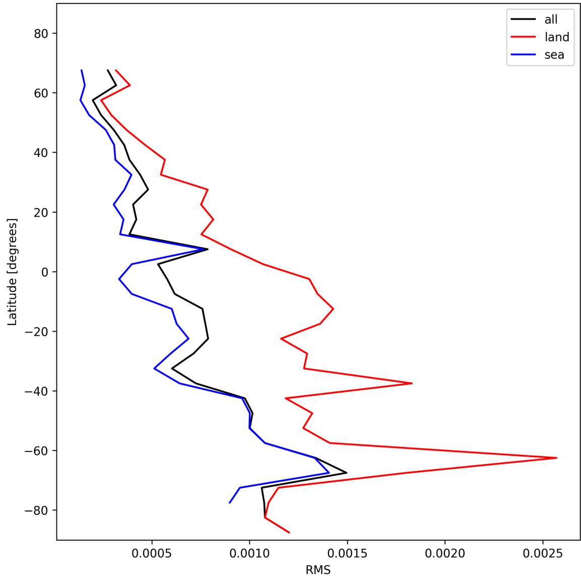
Figure 31: Zonal average of “RMS” for 2024-11-23 to 2024-11-25.
