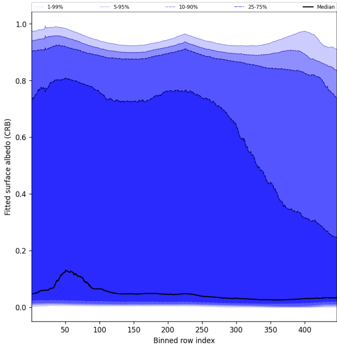
Figure 62: Along track statistics of “Fitted surface albedo (CRB)” for 2024-11-23 to 2024-11-25
