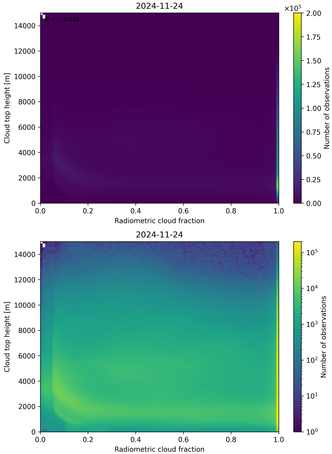
Figure 76: Scatter density plot of “Radiometric cloud fraction” against “Cloud top height” for 2024-11-23 to 2024-11-25.
