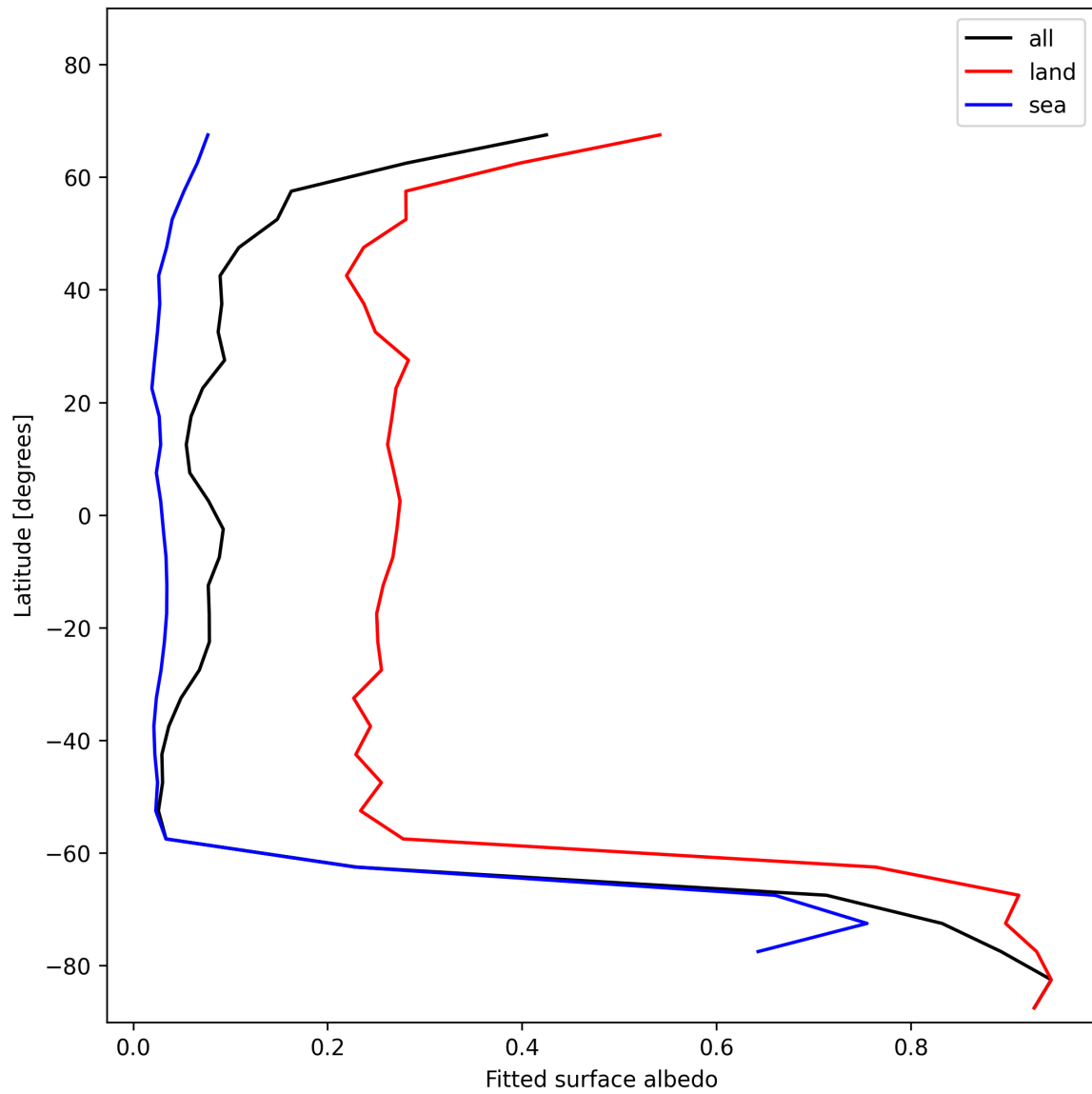
Figure 29: Zonal average of “Fitted surface albedo” for 2024-11-23 to 2024-11-25.
