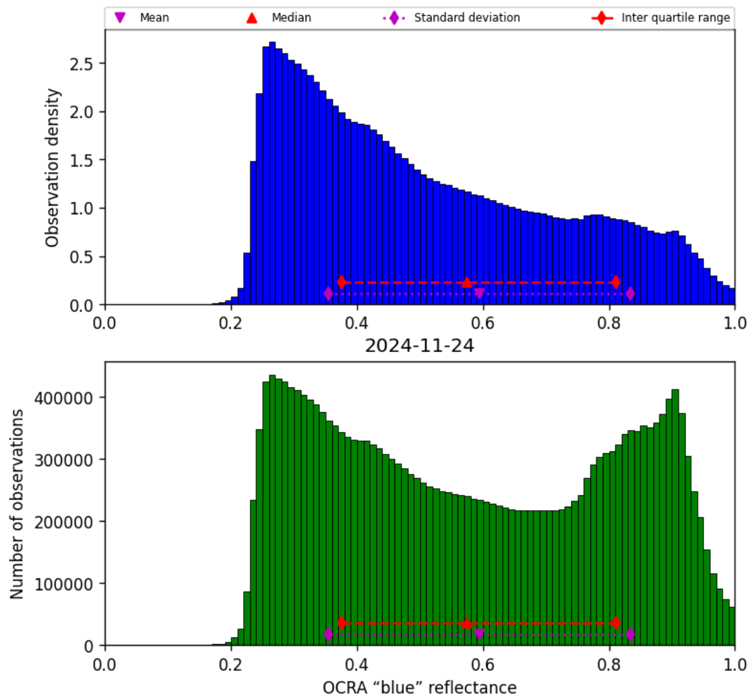
Figure 51: Histogram of “OCRA “blue” reflectance” for 2024-11-23 to 2024-11-25
