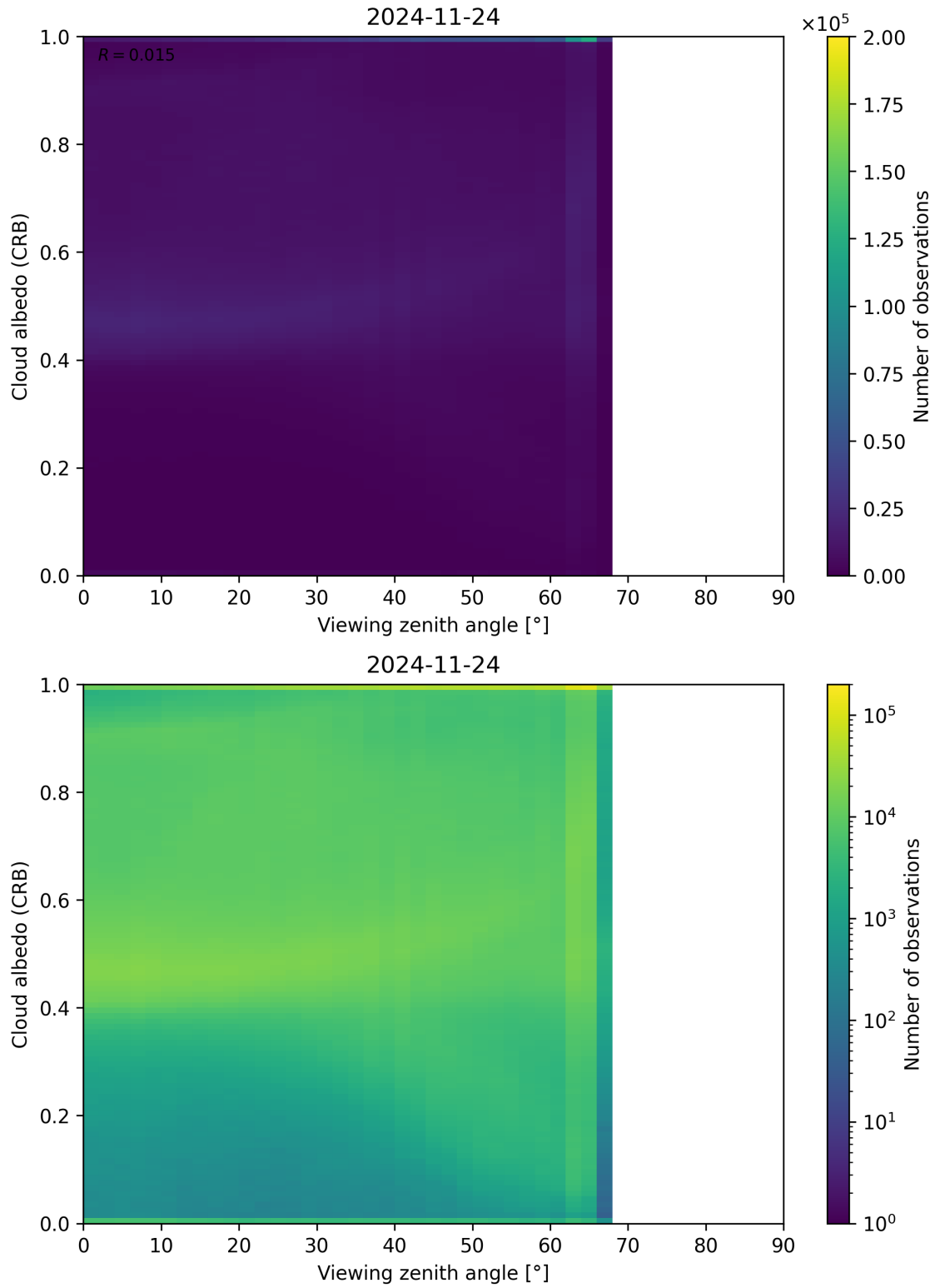
Figure 106: Scatter density plot of “Viewing zenith angle” against “Cloud albedo (CRB)” for 2024-11-23 to 2024-11-25.
