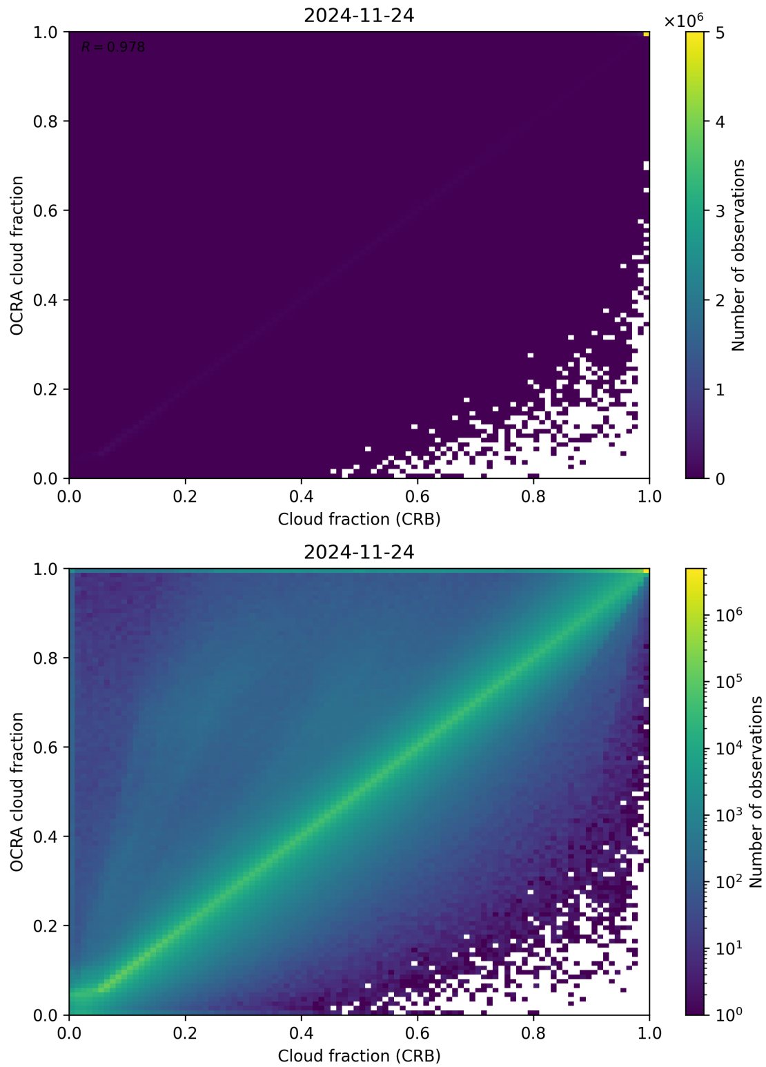
Figure 78: Scatter density plot of “Cloud fraction (CRB)” against “OCRA cloud fraction” for 2024-11-23 to 2024-11-25.
