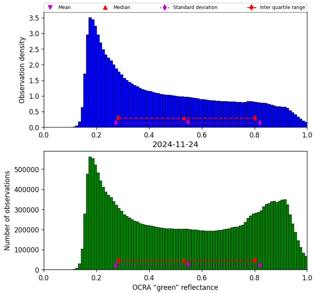
Figure 52: Histogram of “OCRA “green” reflectance” for 2024-11-23 to 2024-11-25
