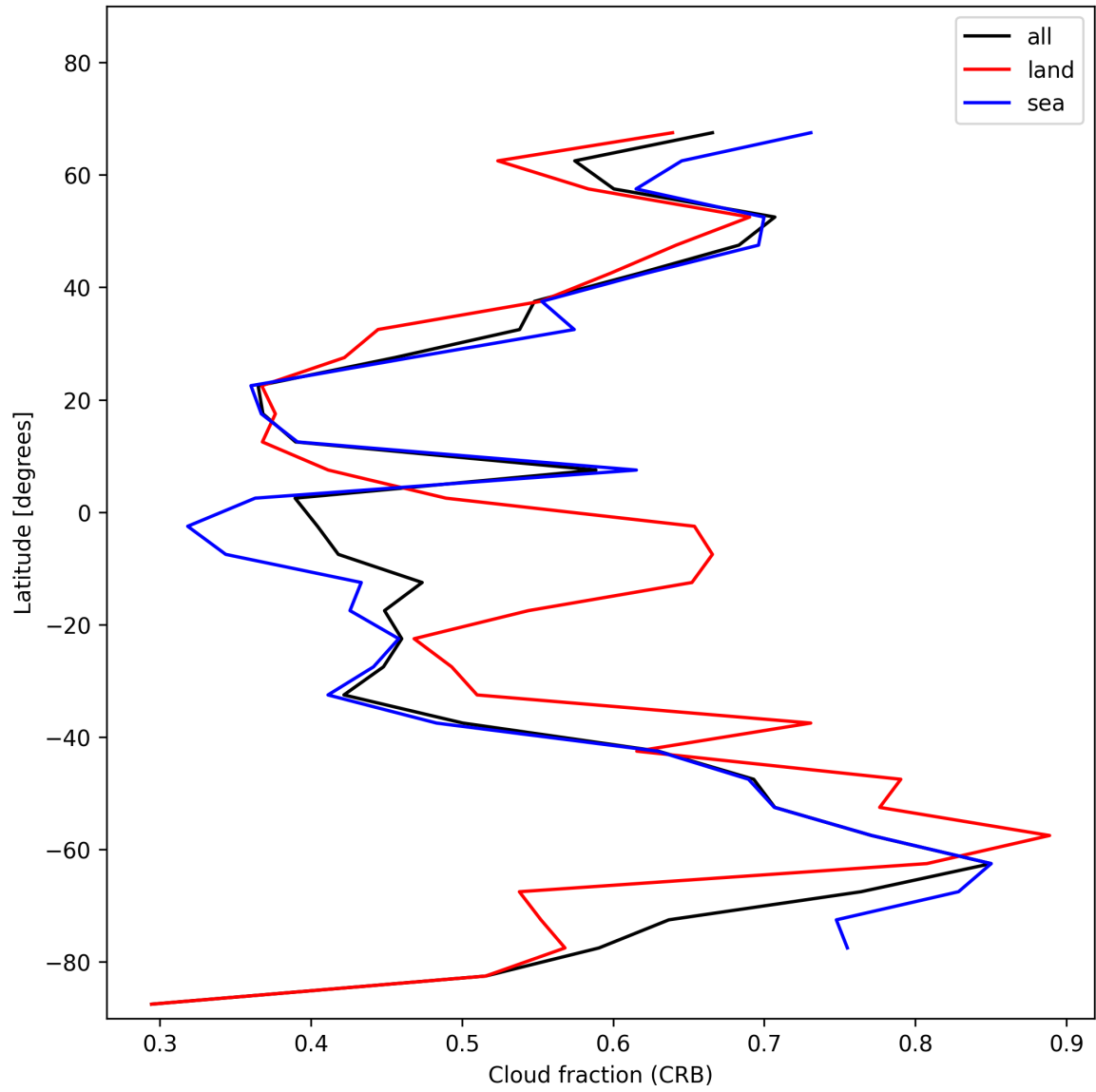
Figure 26: Zonal average of “Cloud fraction (CRB)” for 2024-11-23 to 2024-11-25.
