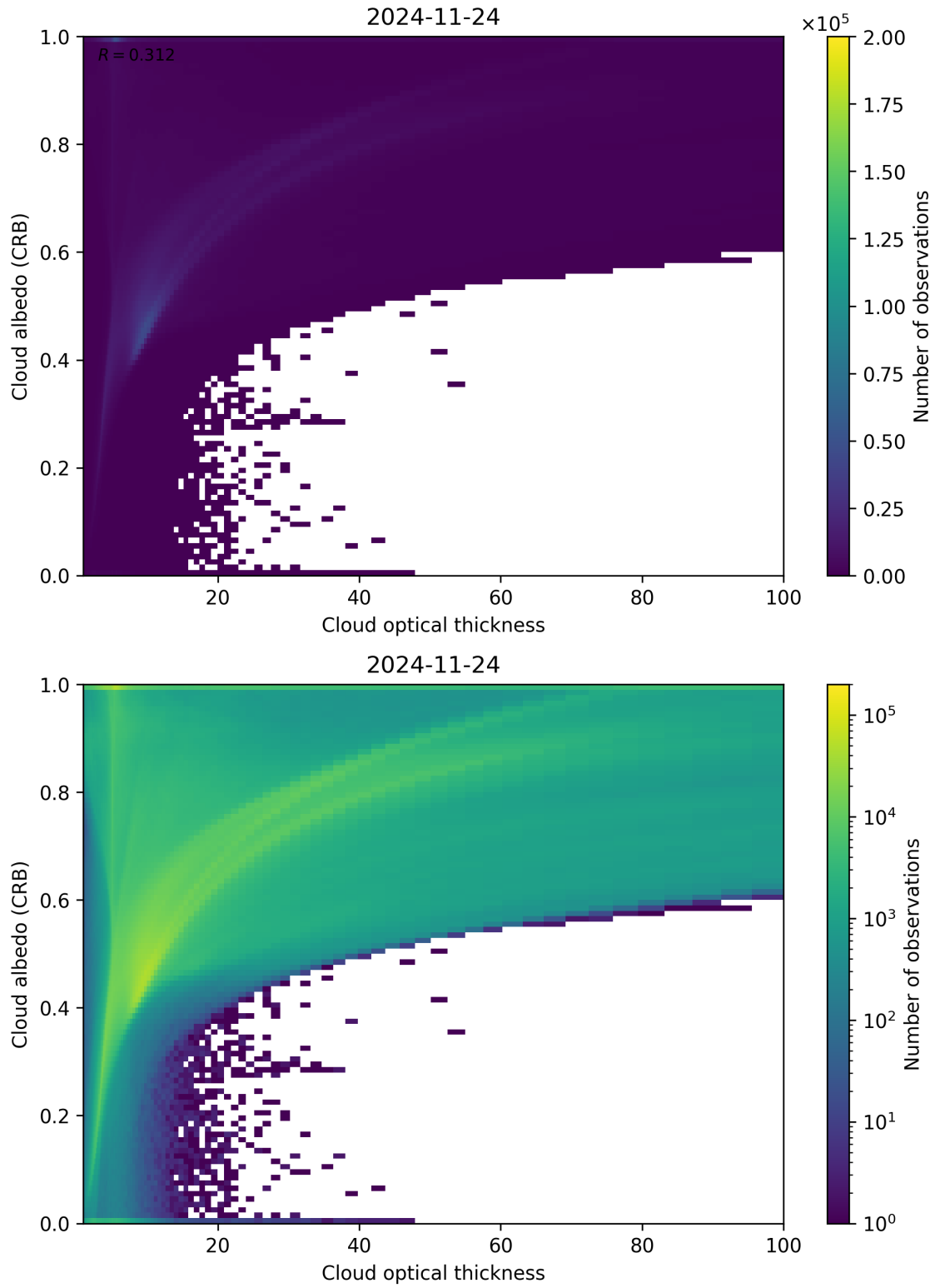
Figure 82: Scatter density plot of “Cloud optical thickness” against “Cloud albedo (CRB)” for 2024-11-23 to 2024-11-25.
