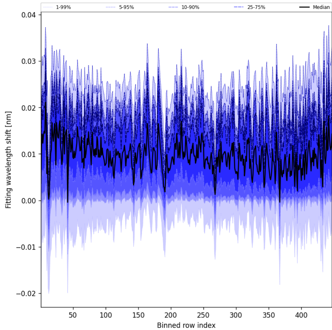
Figure 65: Along track statistics of “Fitting wavelength shift” for 2024-11-23 to 2024-11-25
