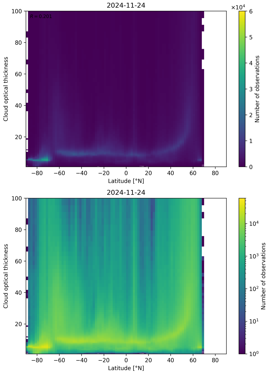
Figure 96: Scatter density plot of “Latitude” against “Cloud optical thickness” for 2024-11-23 to 2024-11-25.
