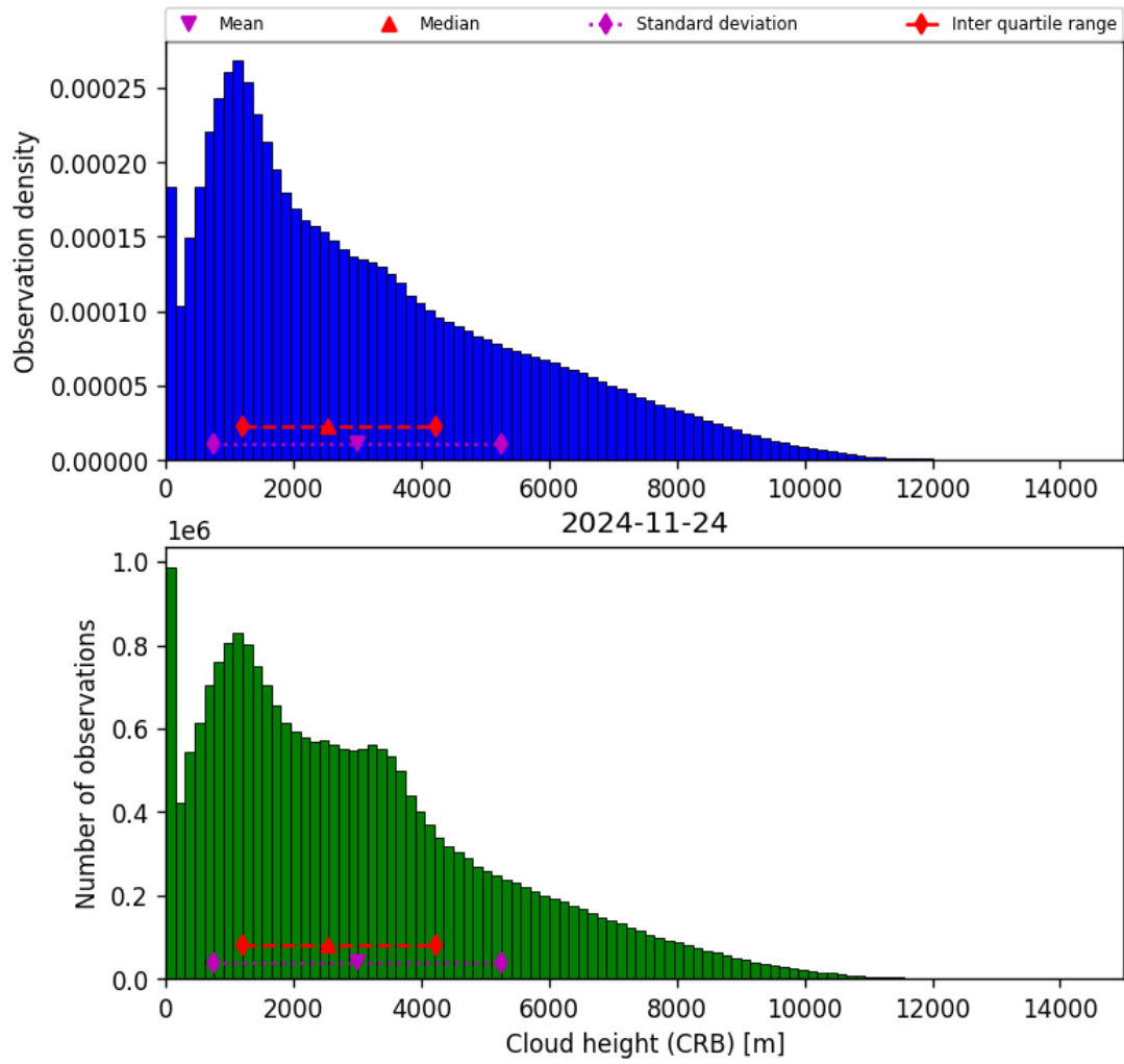
Figure 43: Histogram of “Cloud height (CRB)” for 2024-11-23 to 2024-11-25
