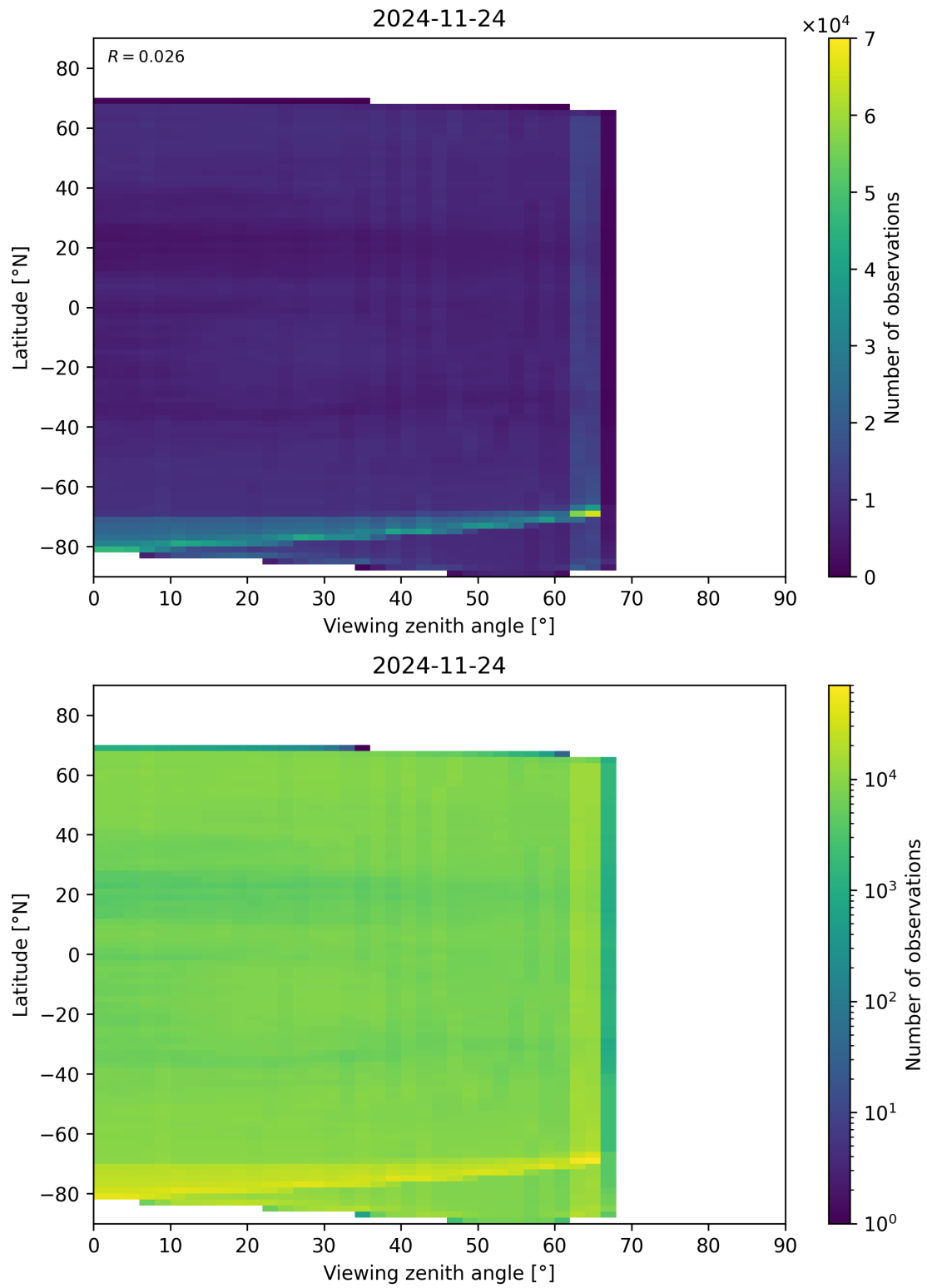
Figure 113: Scatter density plot of “Viewing zenith angle” against “Latitude” for 2024-11-23 to 2024-11-25.
