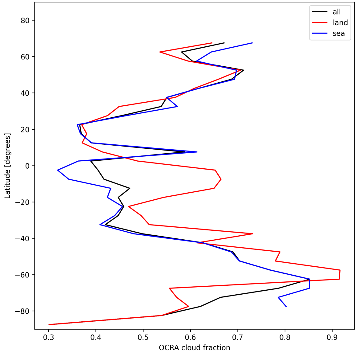
Figure 34: Zonal average of “OCRA cloud fraction” for 2024-11-23 to 2024-11-25.
