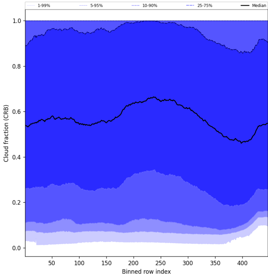
Figure 58: Along track statistics of “Cloud fraction (CRB)” for 2024-11-23 to 2024-11-25
