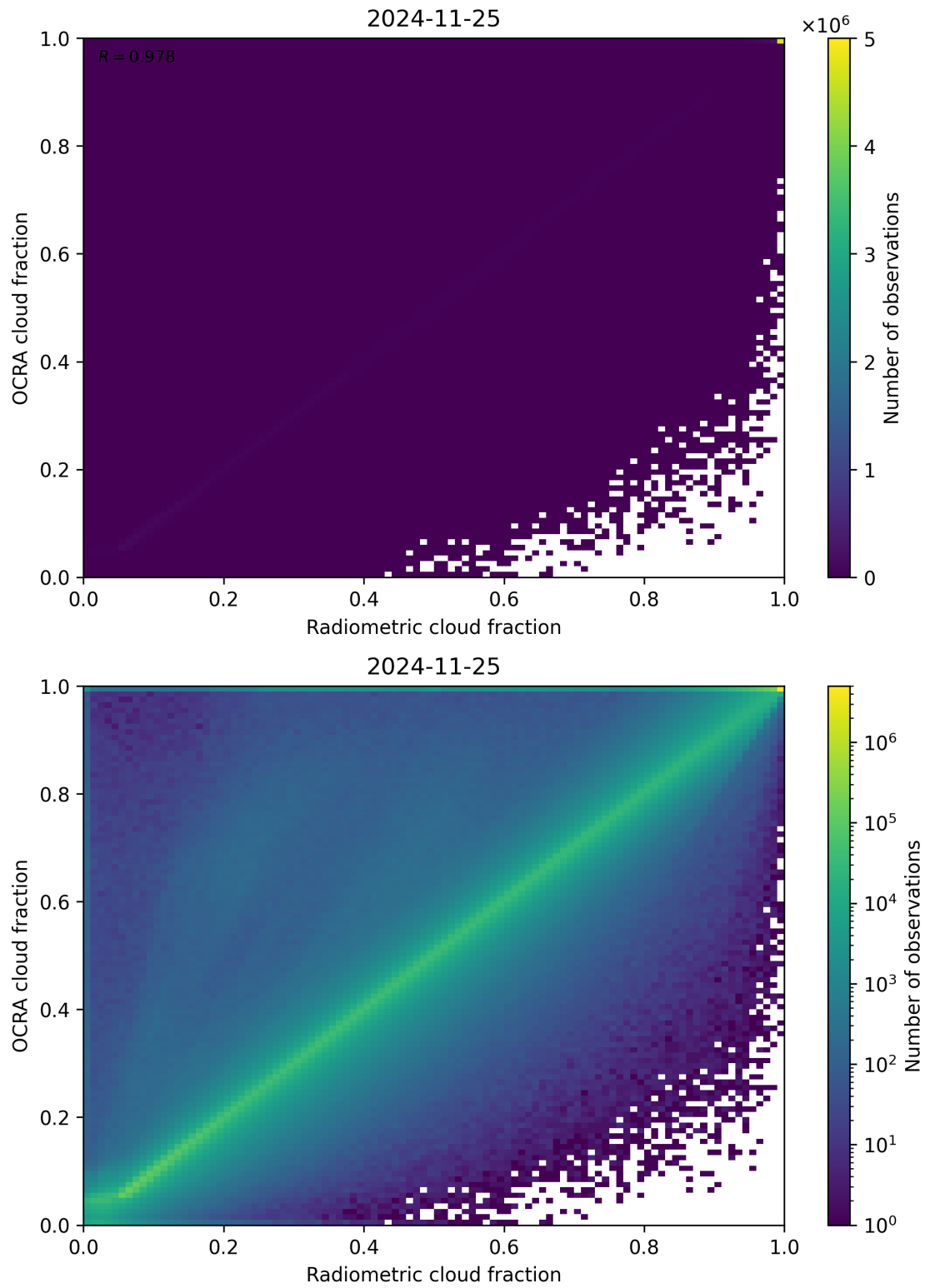
Figure 72: Scatter density plot of “Radiometric cloud fraction” against “OCRA cloud fraction” for 2024-11-25 to 2024-11-26.
