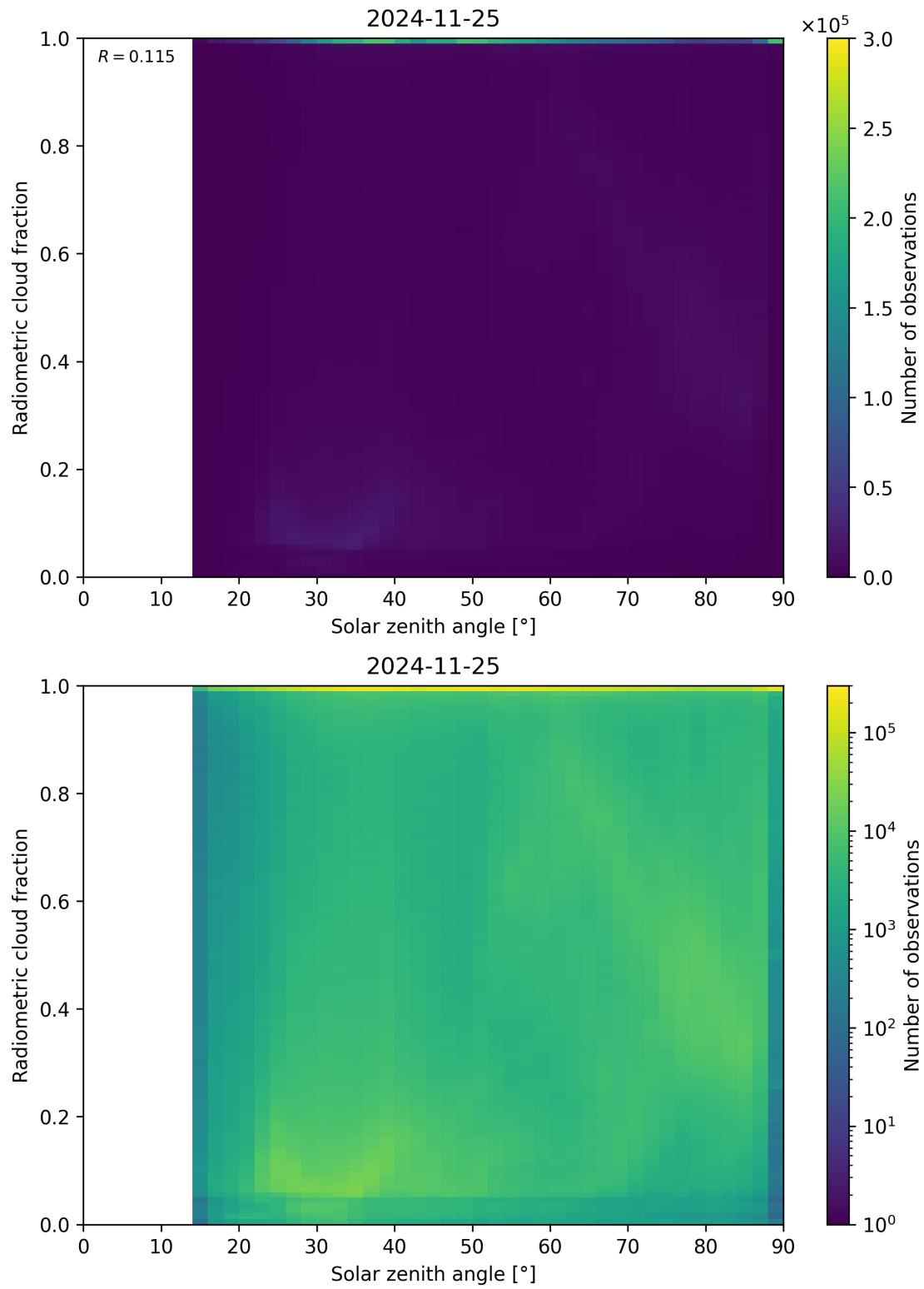
Figure 99: Scatter density plot of “Solar zenith angle” against “Radiometric cloud fraction” for 2024-11-25 to 2024-11-26.
