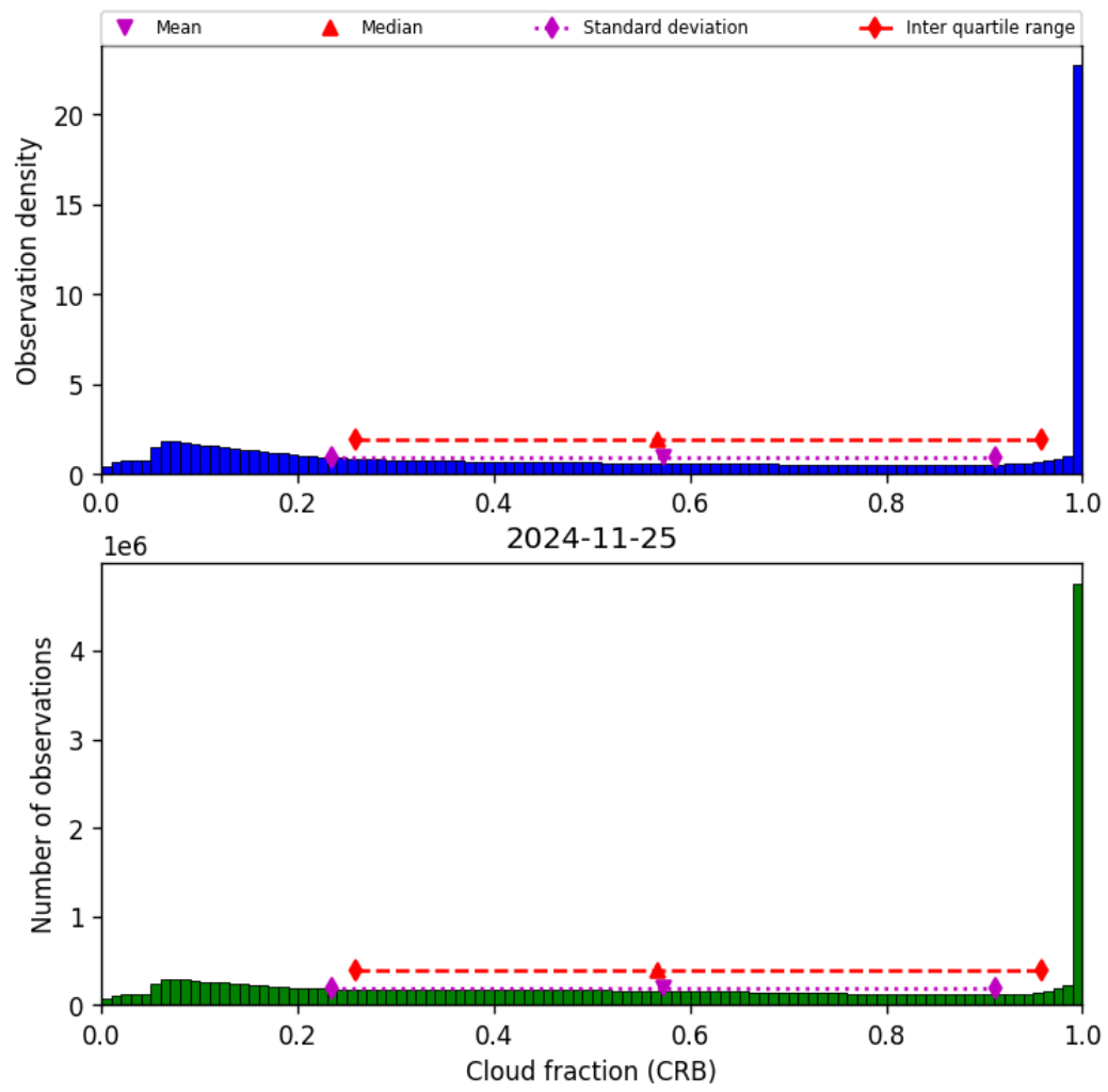
Figure 42: Histogram of “Cloud fraction (CRB)” for 2024-11-25 to 2024-11-26
