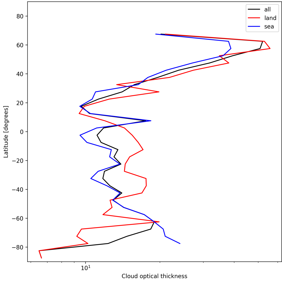
Figure 25: Zonal average of “Cloud optical thickness” for 2024-11-25 to 2024-11-26.
