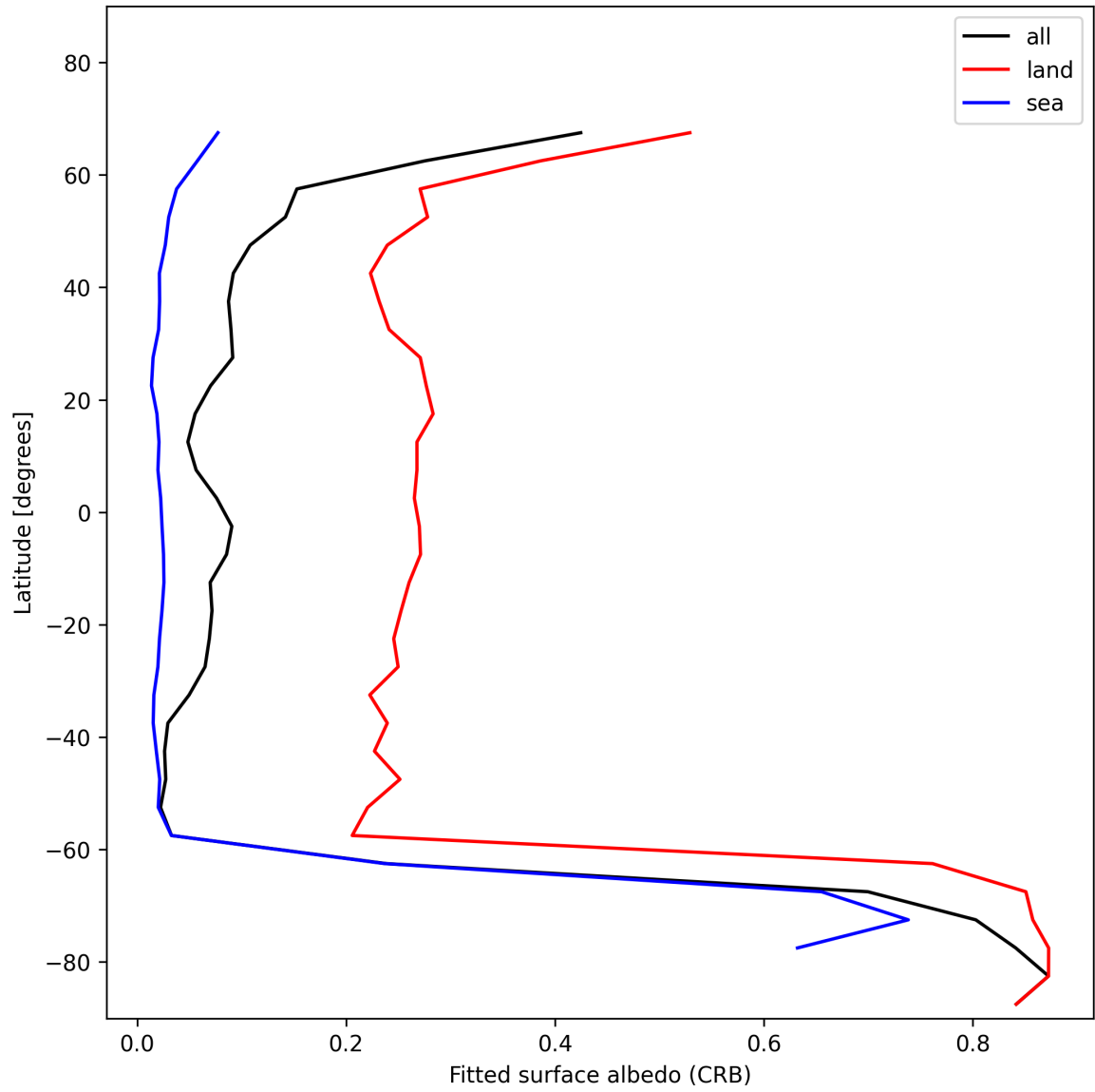
Figure 30: Zonal average of “Fitted surface albedo (CRB)” for 2024-11-25 to 2024-11-26.
