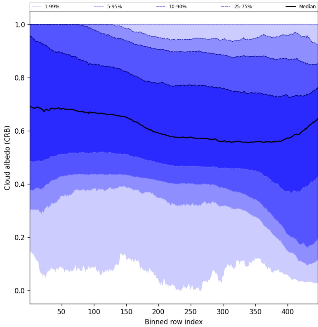
Figure 60: Along track statistics of “Cloud albedo (CRB)” for 2024-11-25 to 2024-11-26
