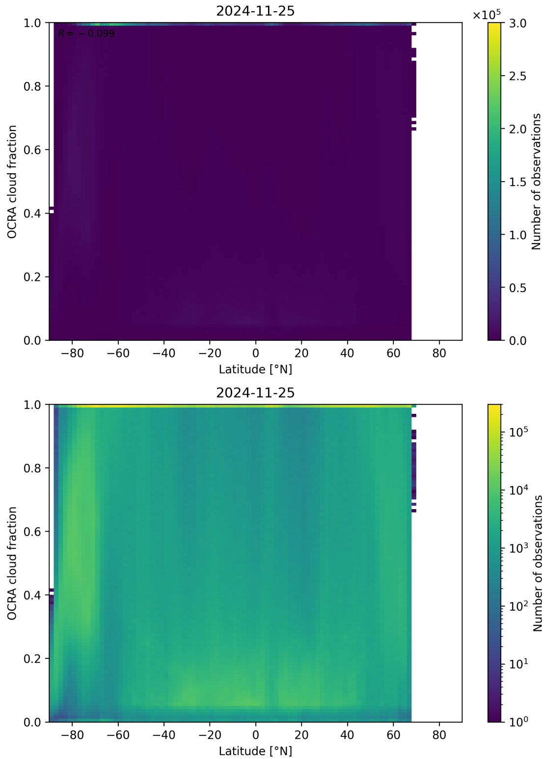
Figure 93: Scatter density plot of “Latitude” against “OCRA cloud fraction” for 2024-11-25 to 2024-11-26.
