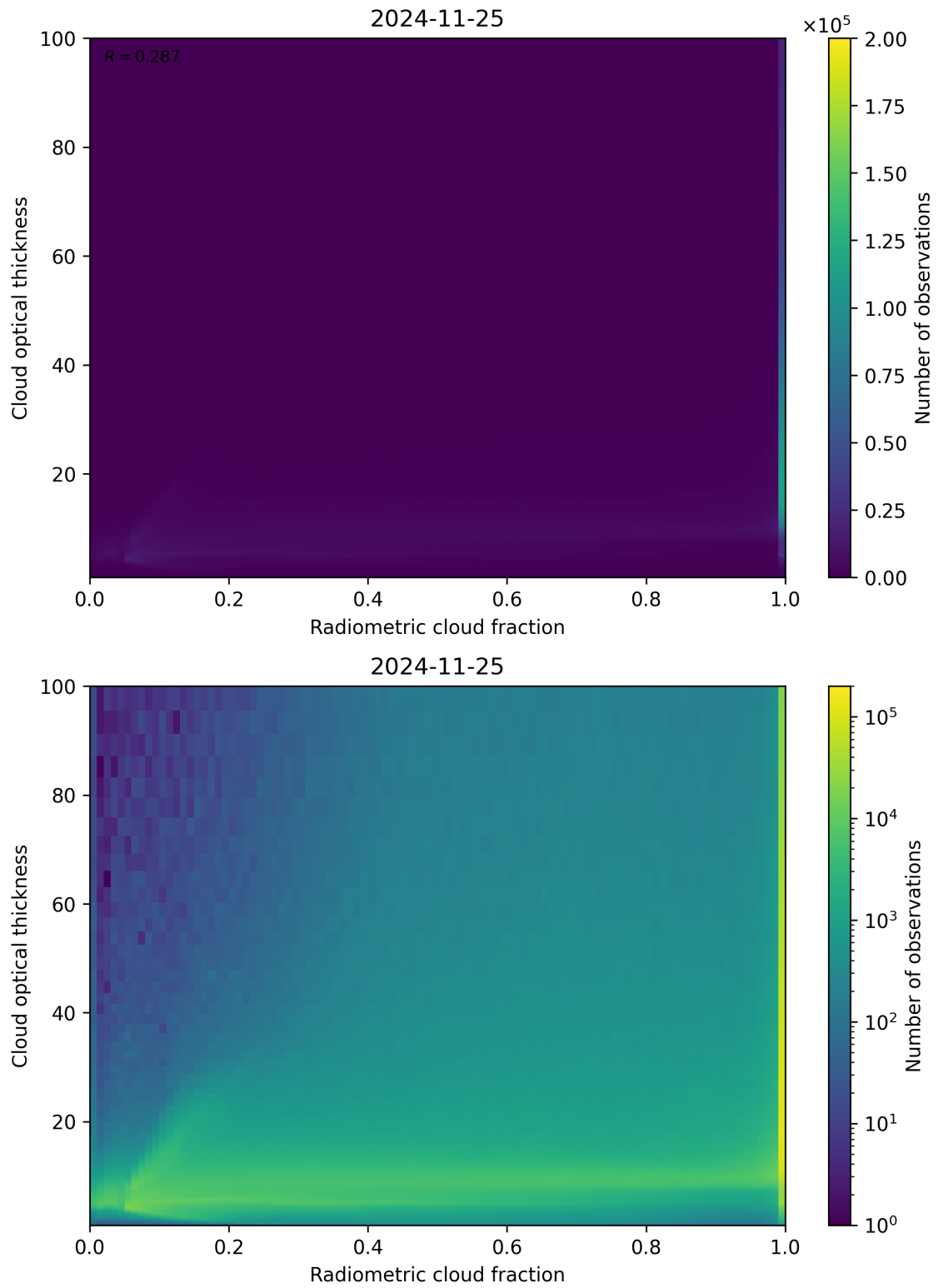
Figure 75: Scatter density plot of “Radiometric cloud fraction” against “Cloud optical thickness” for 2024-11-25 to 2024-11-26.
