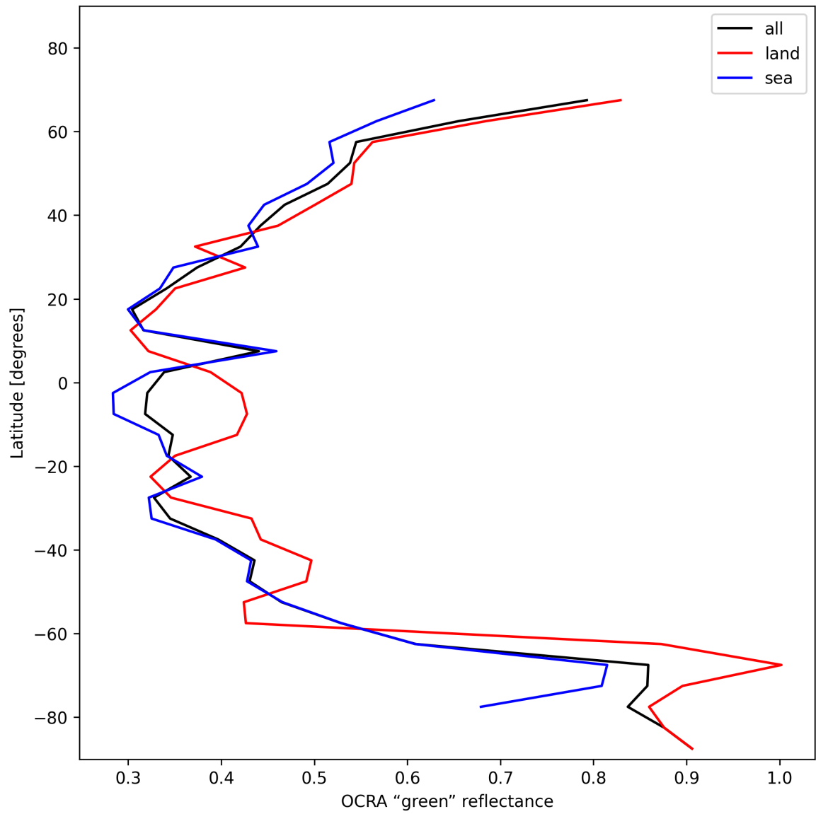
Figure 36: Zonal average of “OCRA “green” reflectance” for 2024-11-25 to 2024-11-26.
