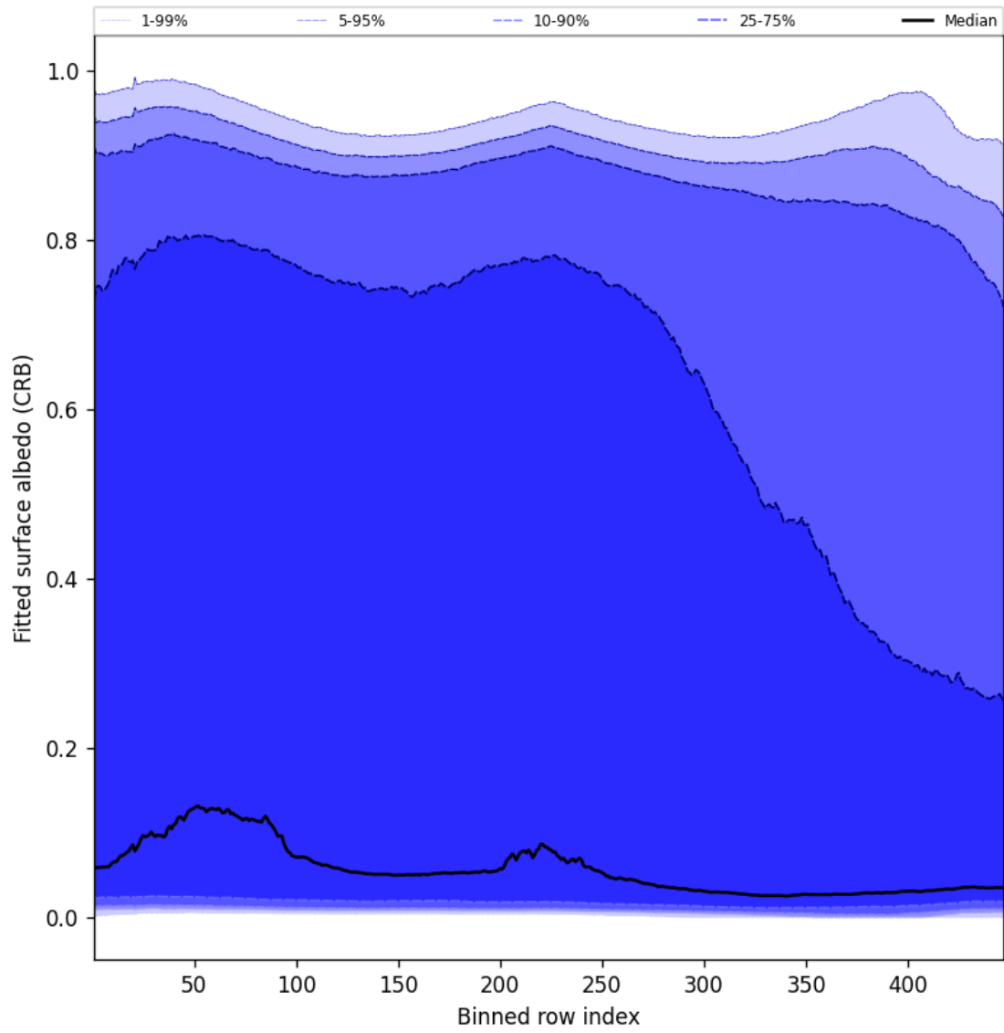
Figure 62: Along track statistics of “Fitted surface albedo (CRB)” for 2024-11-25 to 2024-11-26
