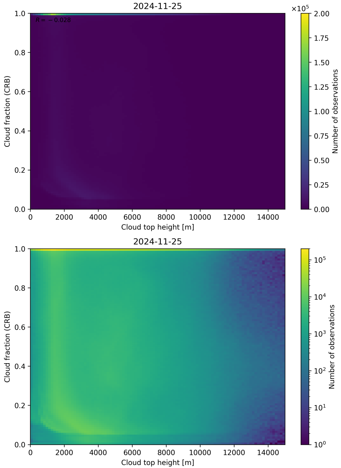
Figure 88: Scatter density plot of “Cloud top height” against “Cloud fraction (CRB)” for 2024-11-25 to 2024-11-26.
