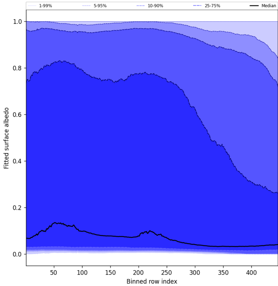
Figure 61: Along track statistics of “Fitted surface albedo” for 2024-11-25 to 2024-11-26
