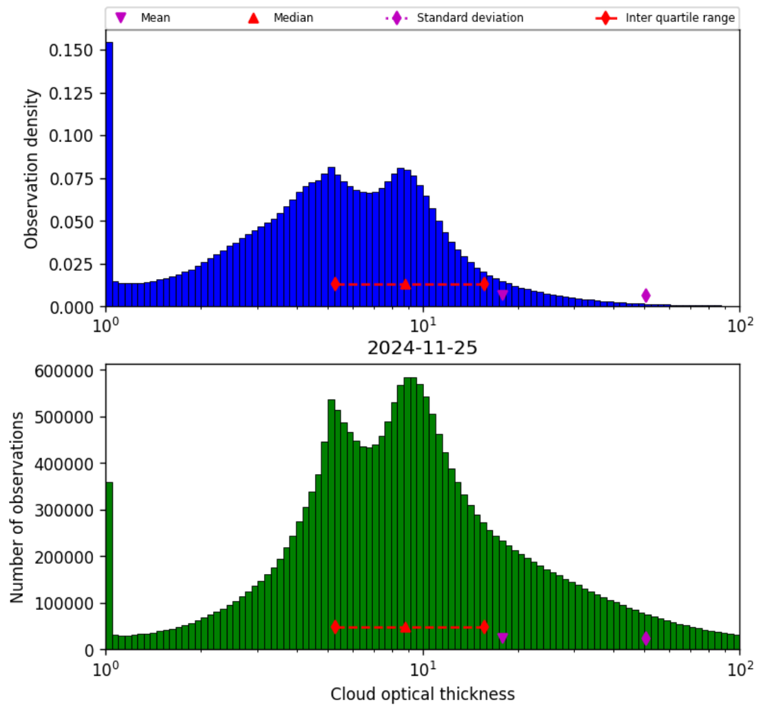
Figure 41: Histogram of “Cloud optical thickness” for 2024-11-25 to 2024-11-26
