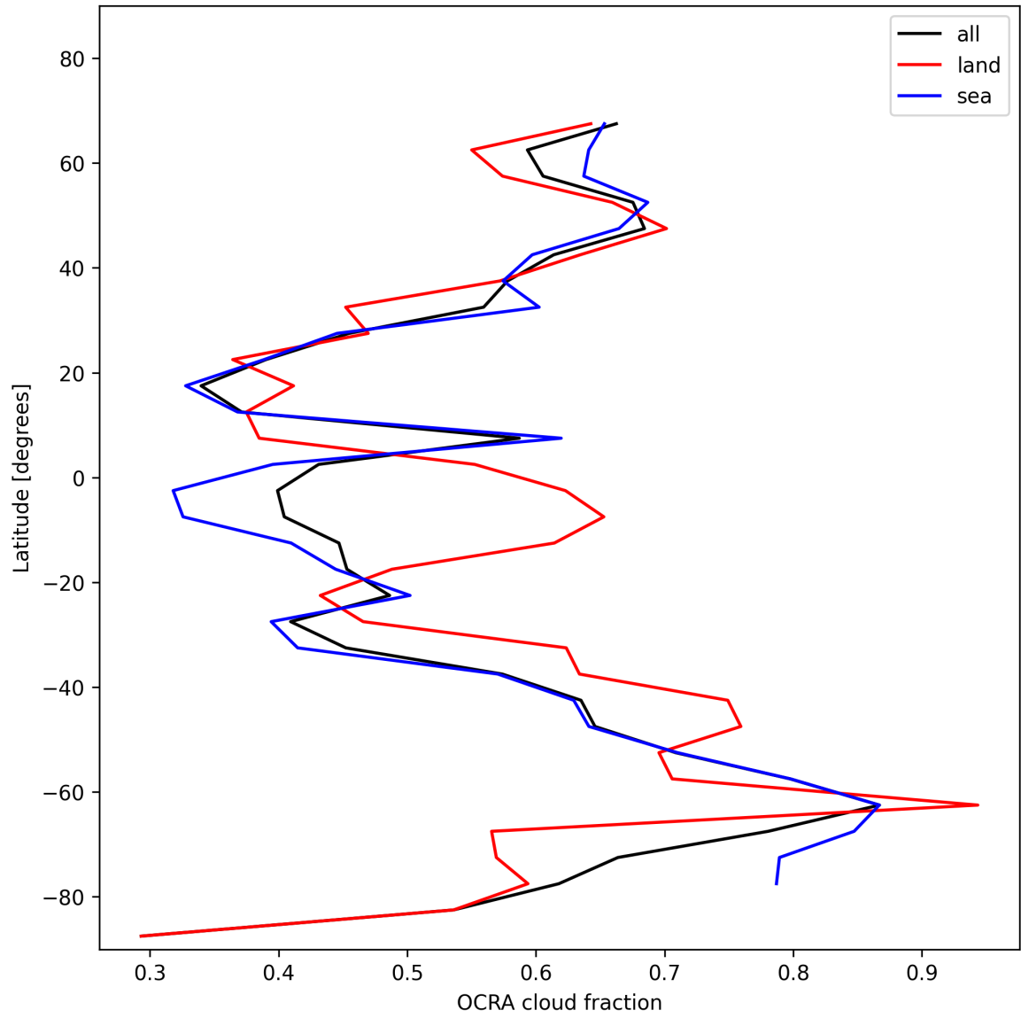
Figure 34: Zonal average of “OCRA cloud fraction” for 2024-11-25 to 2024-11-26.
