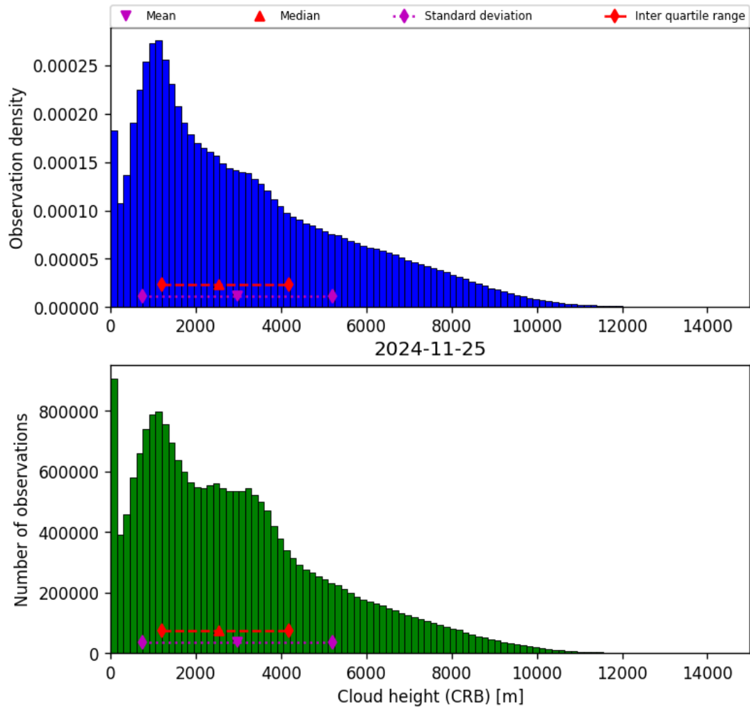
Figure 43: Histogram of “Cloud height (CRB)” for 2024-11-25 to 2024-11-26
