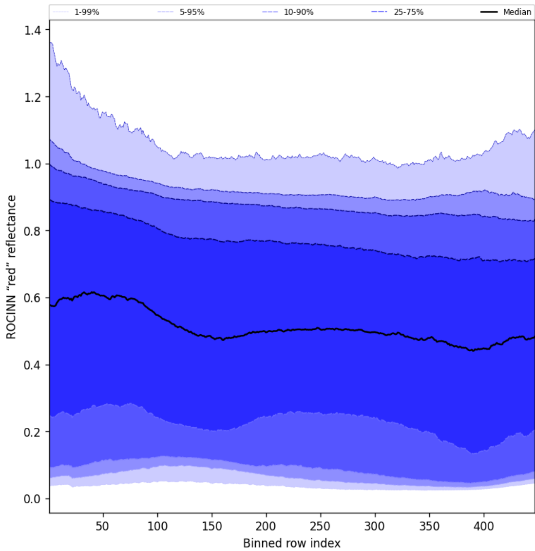
Figure 69: Along track statistics of “ROCINN “red” reflectance” for 2024-11-25 to 2024-11-26
