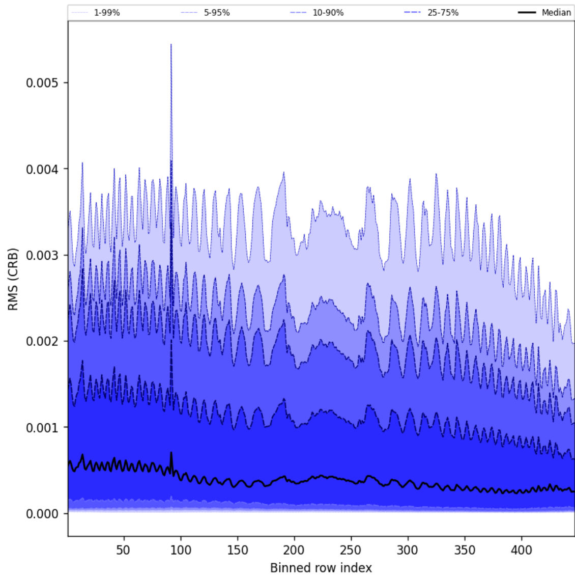
Figure 64: Along track statistics of “RMS (CRB)” for 2024-11-25 to 2024-11-26
