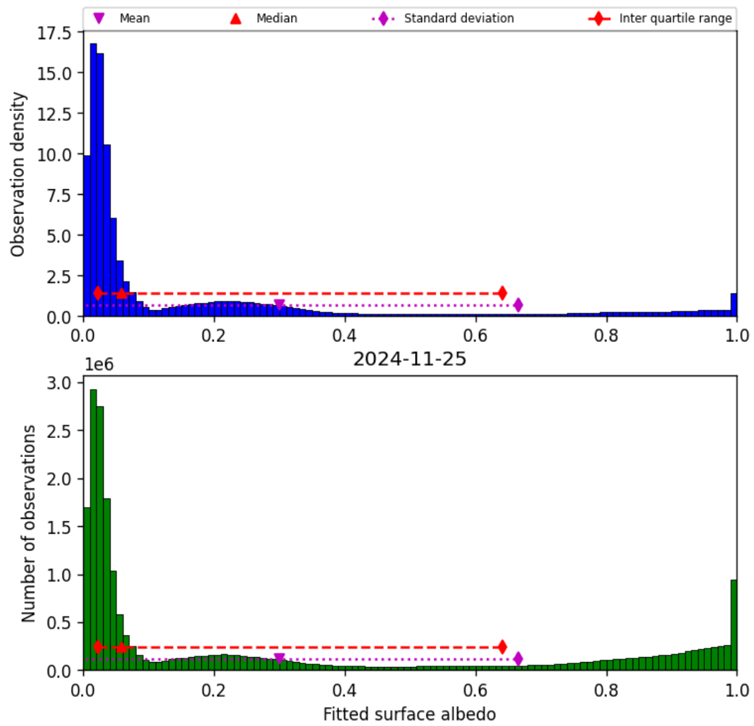
Figure 45: Histogram of “Fitted surface albedo” for 2024-11-25 to 2024-11-26
