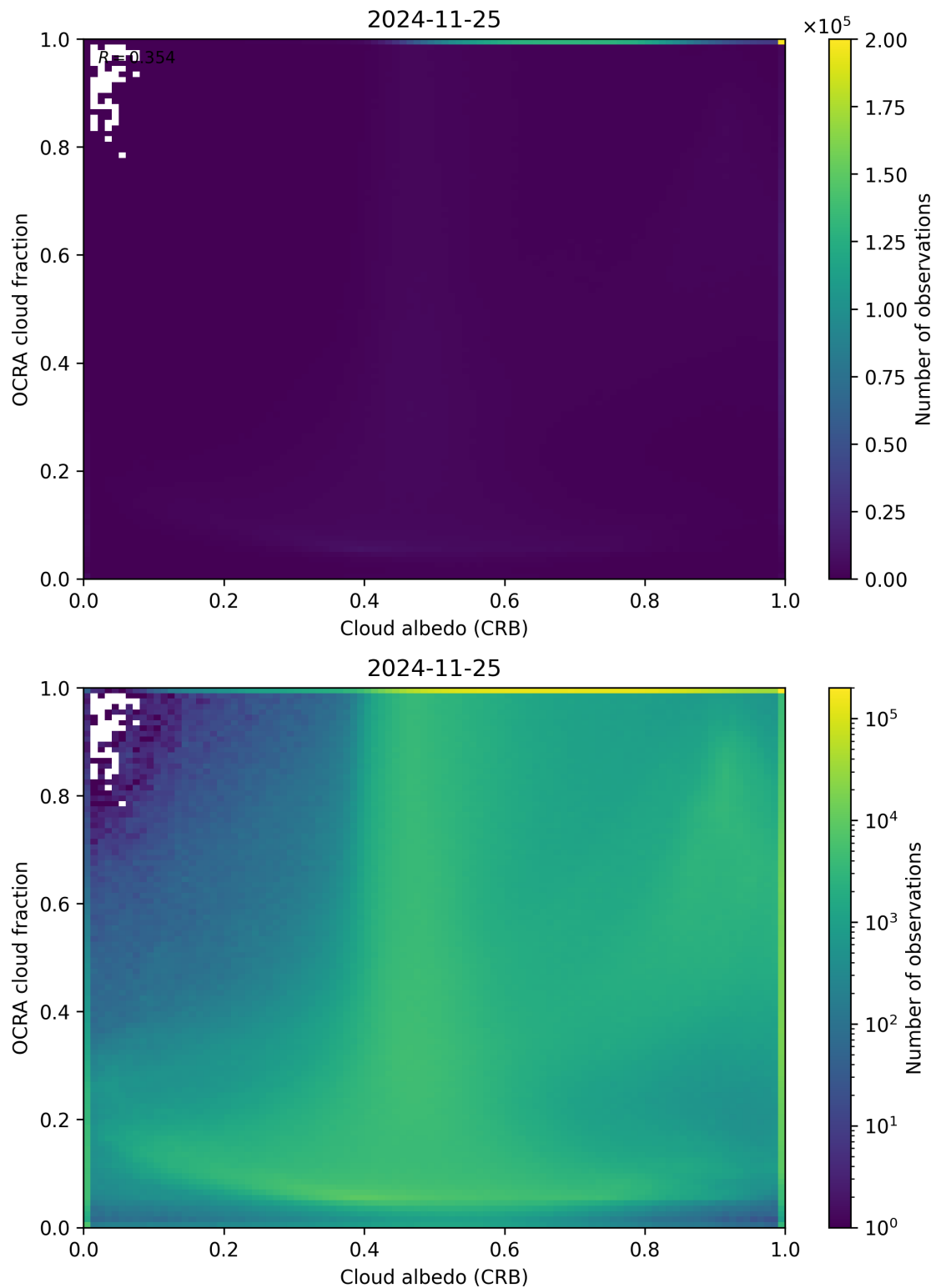
Figure 70: Scatter density plot of “Cloud albedo (CRB)” against “OCRA cloud fraction” for 2024-11-25 to 2024-11-26.
