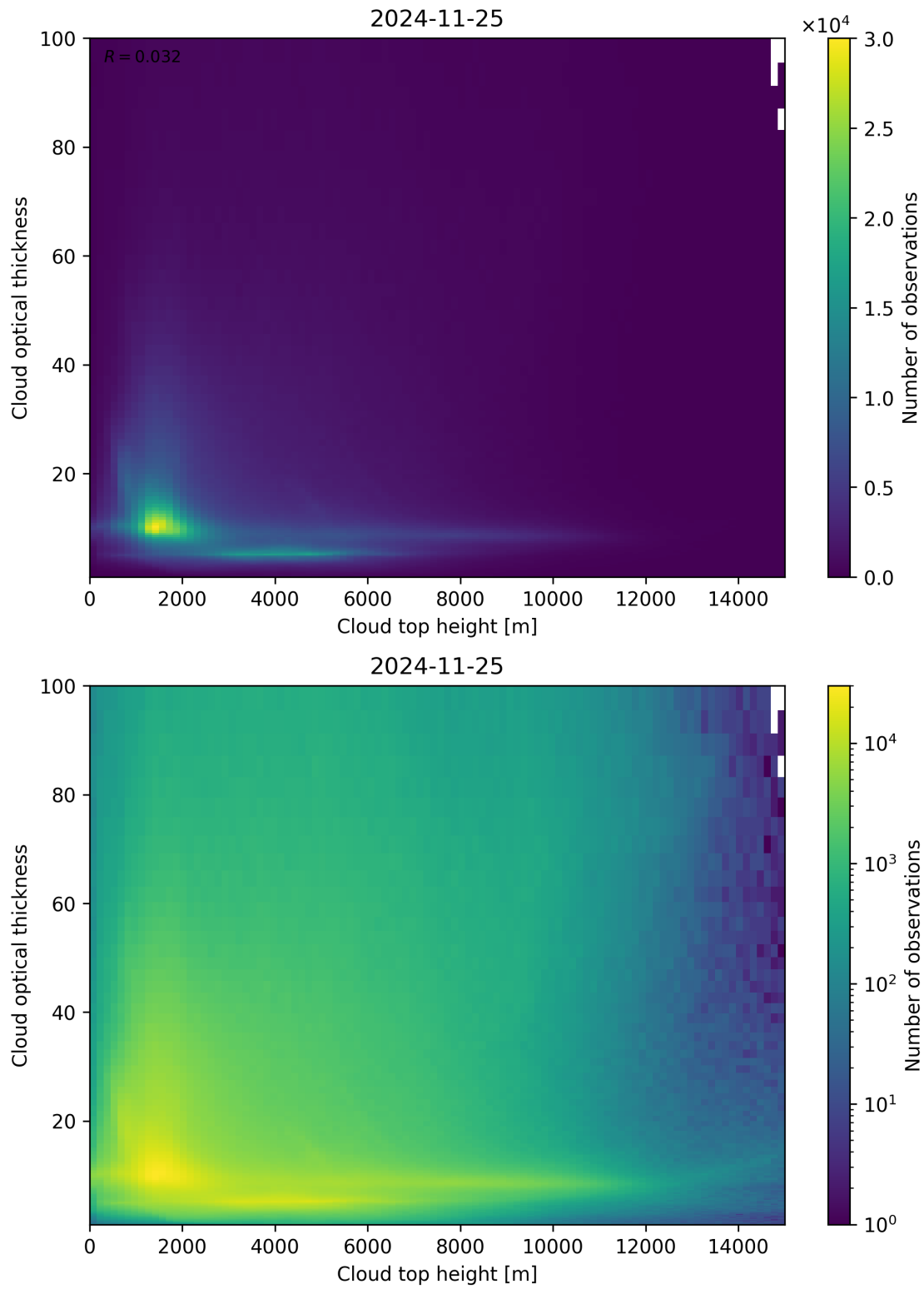
Figure 90: Scatter density plot of “Cloud top height” against “Cloud optical thickness” for 2024-11-25 to 2024-11-26.
