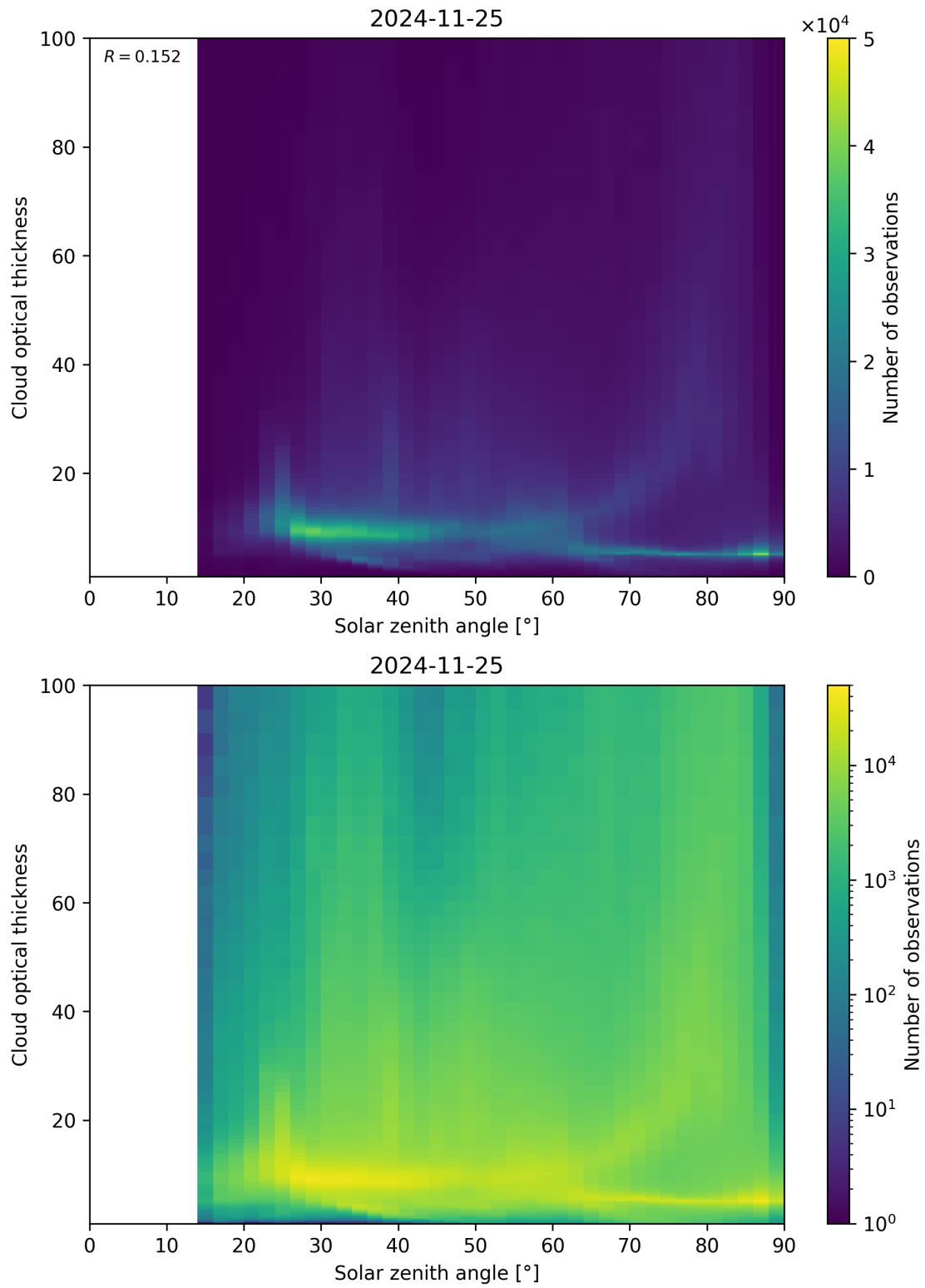
Figure 103: Scatter density plot of “Solar zenith angle” against “Cloud optical thickness” for 2024-11-25 to 2024-11-26.
