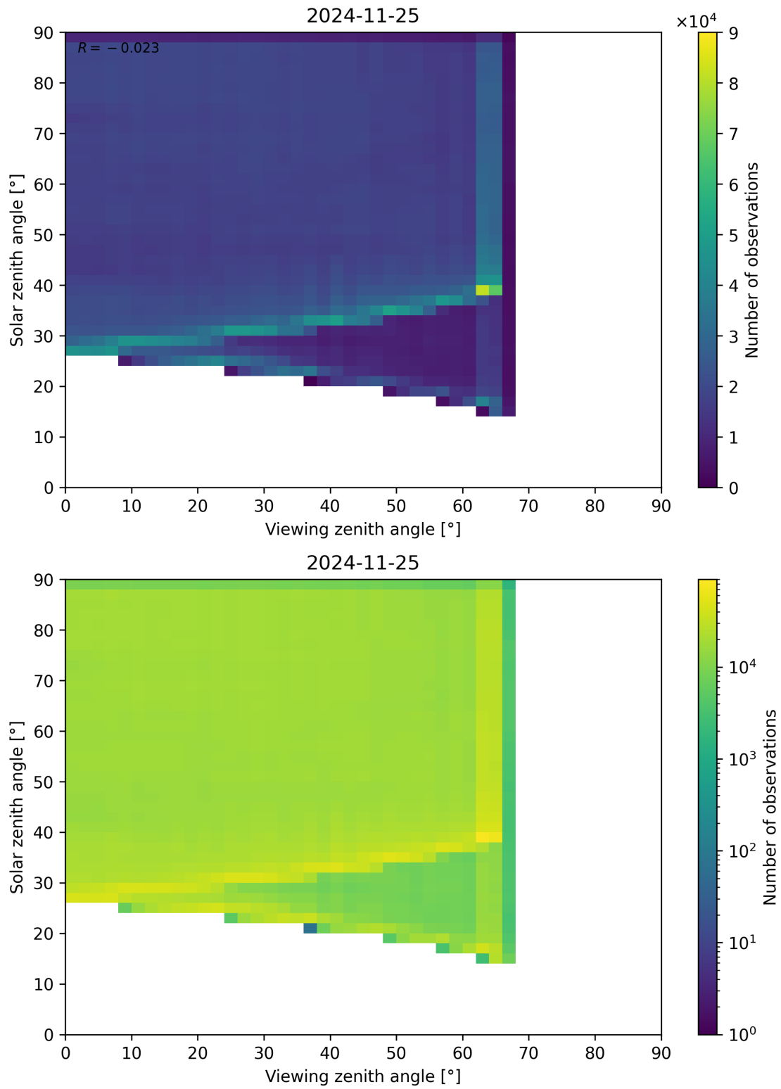
Figure 114: Scatter density plot of “Viewing zenith angle” against “Solar zenith angle” for 2024-11-25 to 2024-11-26.
