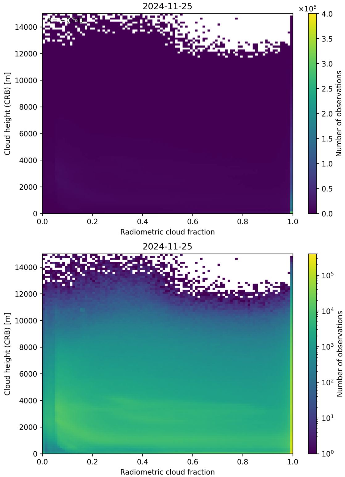
Figure 74: Scatter density plot of “Radiometric cloud fraction” against “Cloud height (CRB)” for 2024-11-25 to 2024-11-26.
