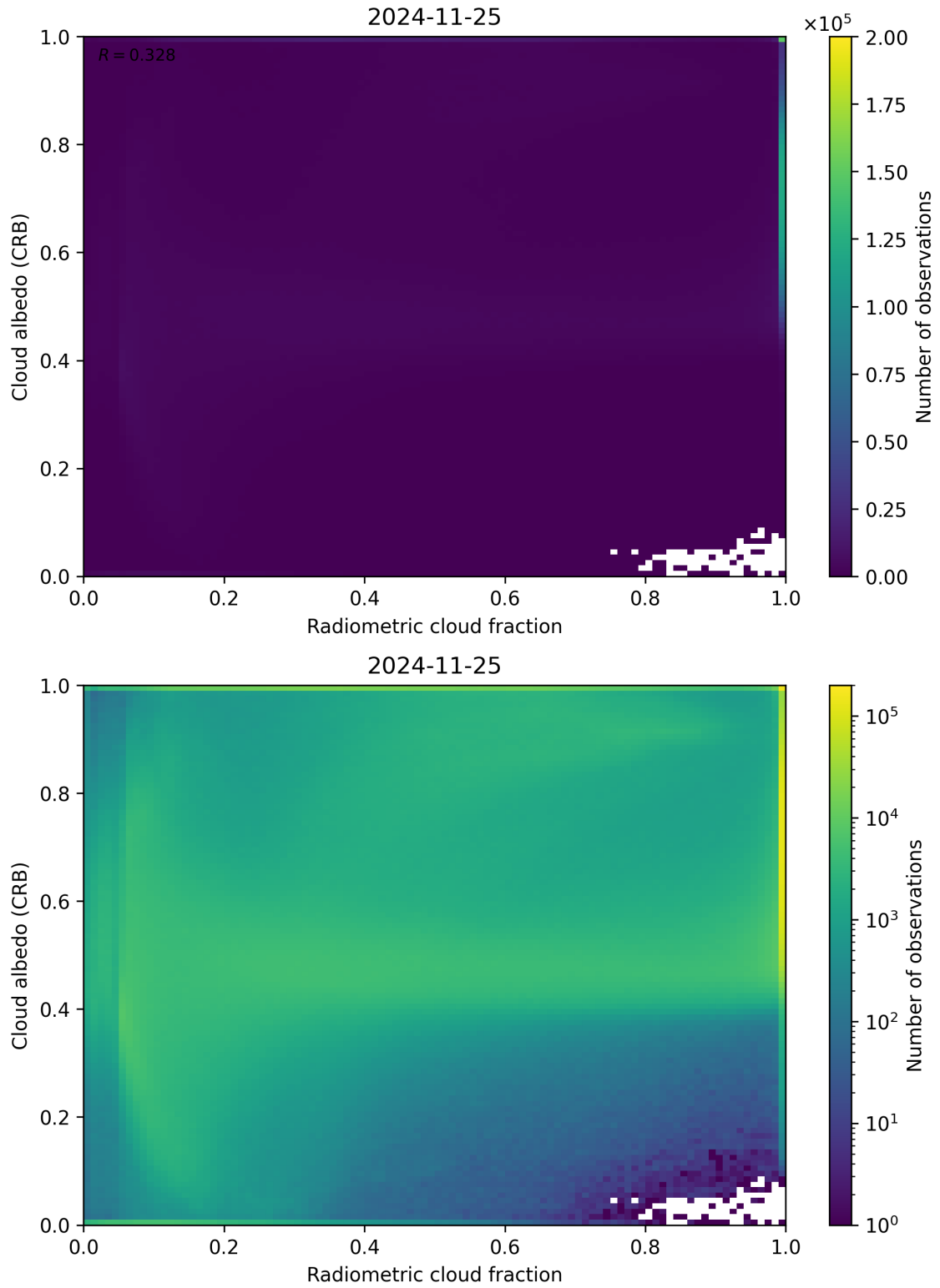
Figure 71: Scatter density plot of “Radiometric cloud fraction” against “Cloud albedo (CRB)” for 2024-11-25 to 2024-11-26.
