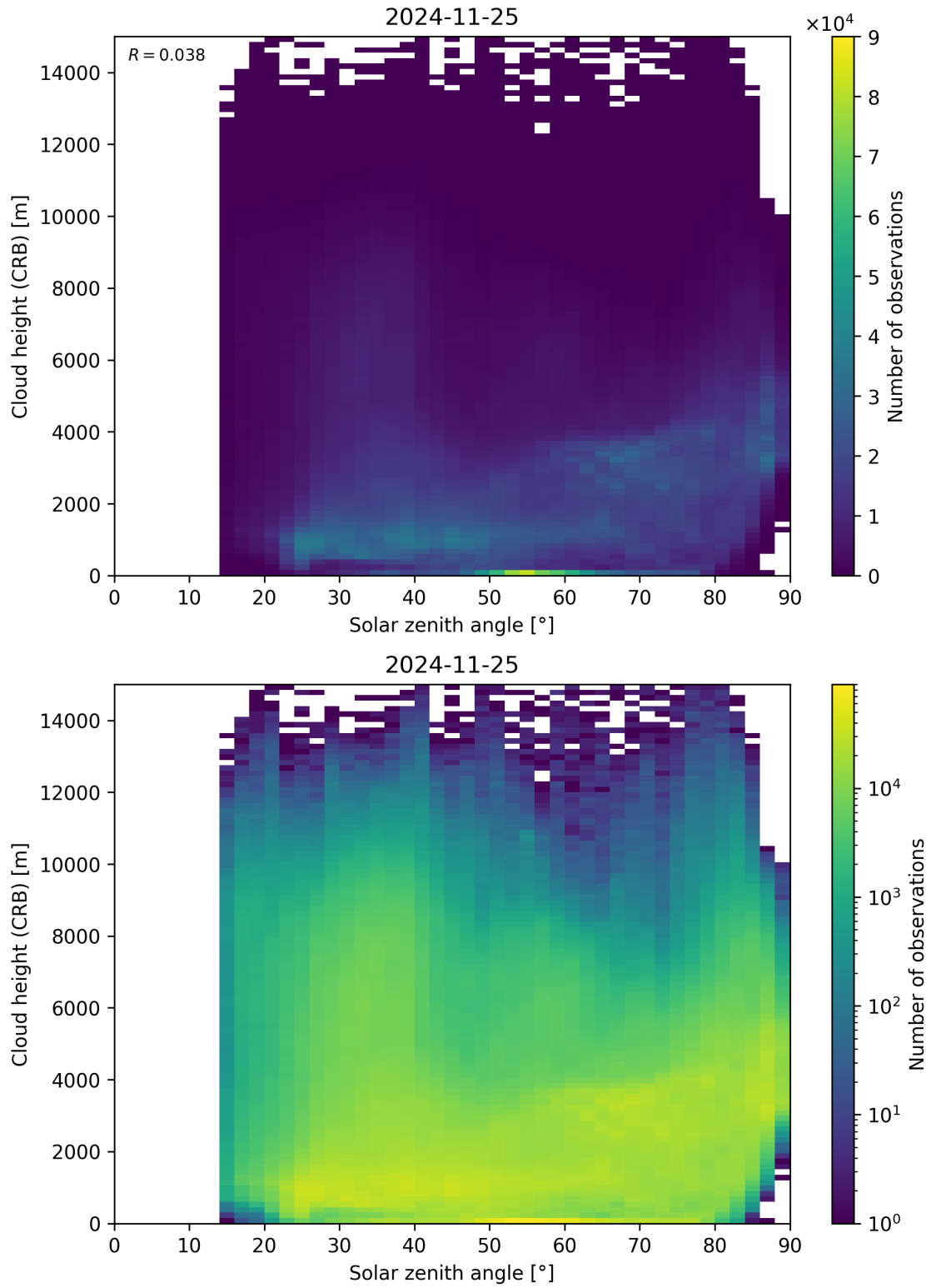
Figure 102: Scatter density plot of “Solar zenith angle” against “Cloud height (CRB)” for 2024-11-25 to 2024-11-26.
