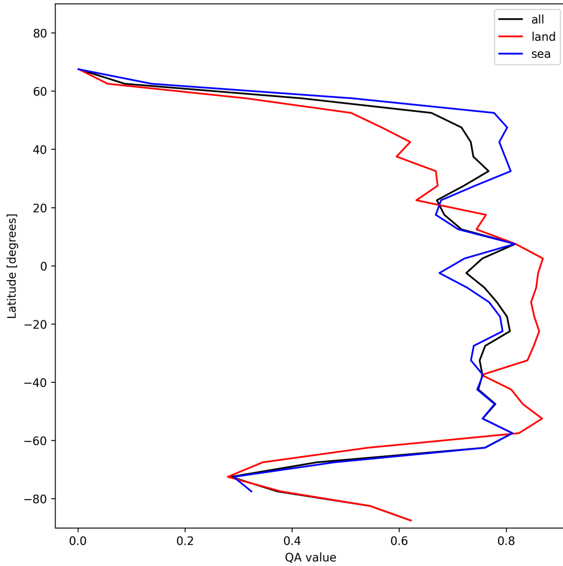
Figure 22: Zonal average of “QA value” for 2024-11-25 to 2024-11-26.
