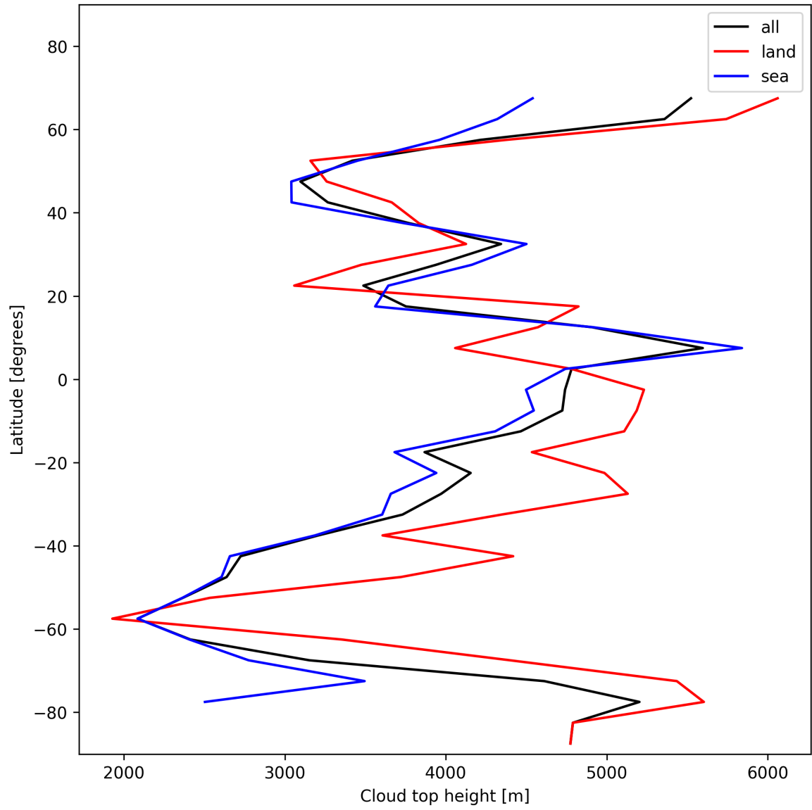
Figure 24: Zonal average of “Cloud top height” for 2024-11-25 to 2024-11-26.
