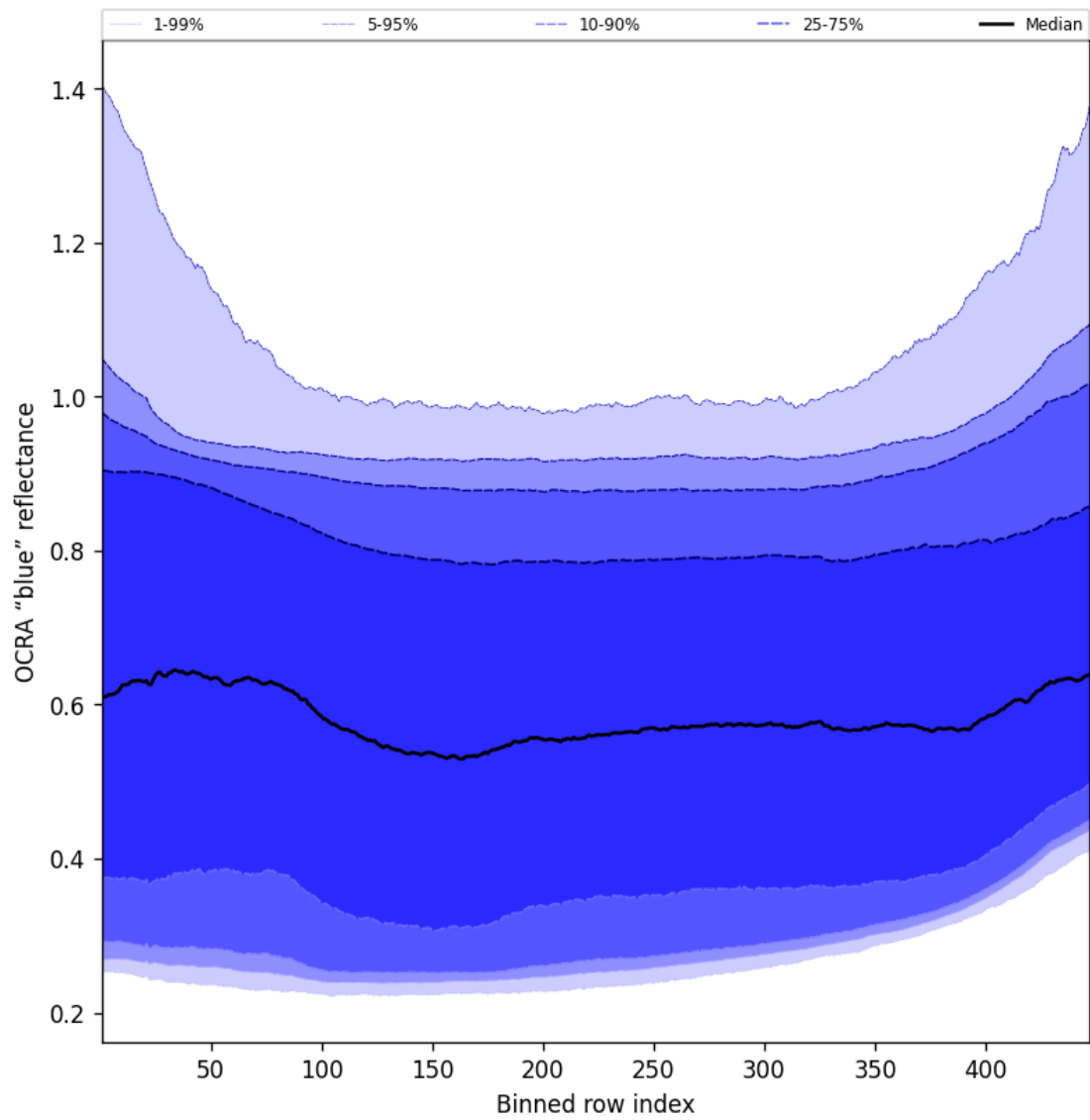
Figure 67: Along track statistics of “OCRA “blue” reflectance” for 2024-11-25 to 2024-11-26
