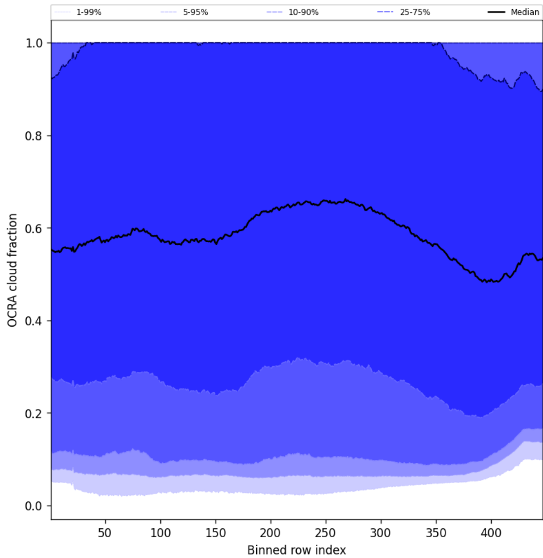
Figure 66: Along track statistics of “OCRA cloud fraction” for 2024-11-25 to 2024-11-26
