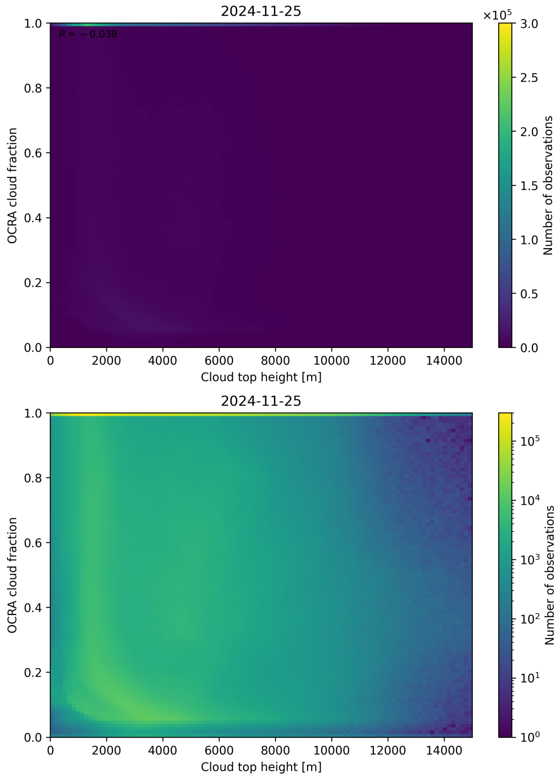
Figure 87: Scatter density plot of “Cloud top height” against “OCRA cloud fraction” for 2024-11-25 to 2024-11-26.
