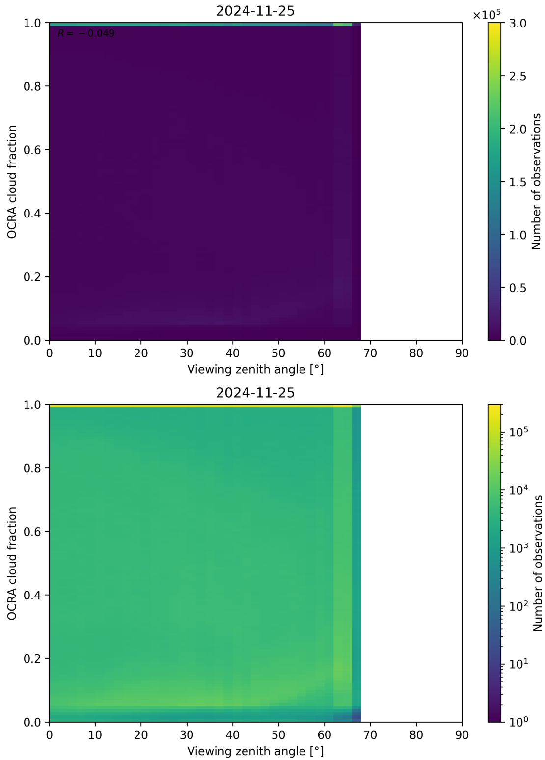
Figure 108: Scatter density plot of “Viewing zenith angle” against “OCRA cloud fraction” for 2024-11-25 to 2024-11-26.
