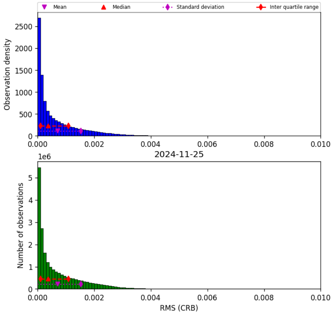
Figure 48: Histogram of “RMS (CRB)” for 2024-11-25 to 2024-11-26
