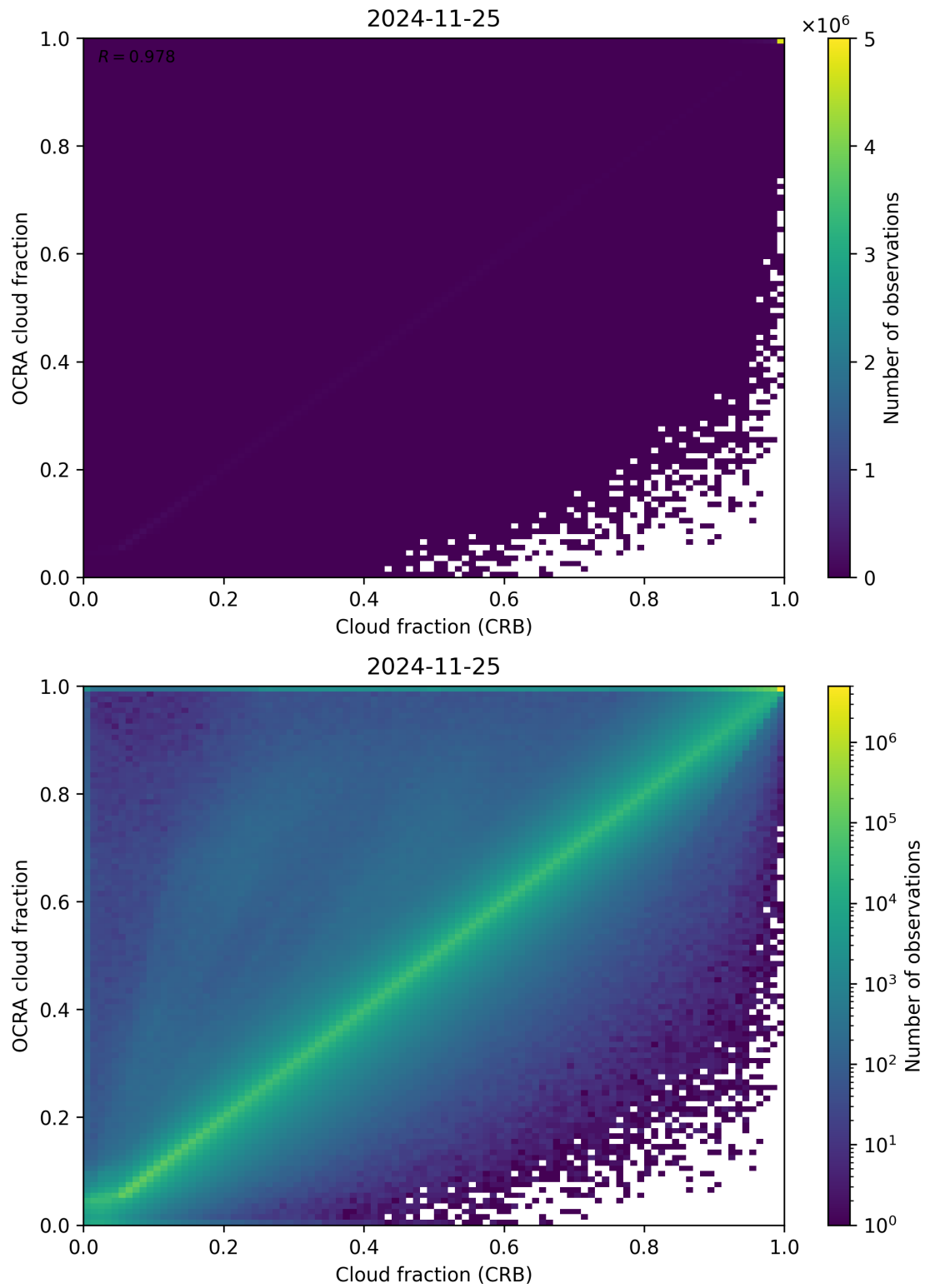
Figure 78: Scatter density plot of “Cloud fraction (CRB)” against “OCRA cloud fraction” for 2024-11-25 to 2024-11-26.
