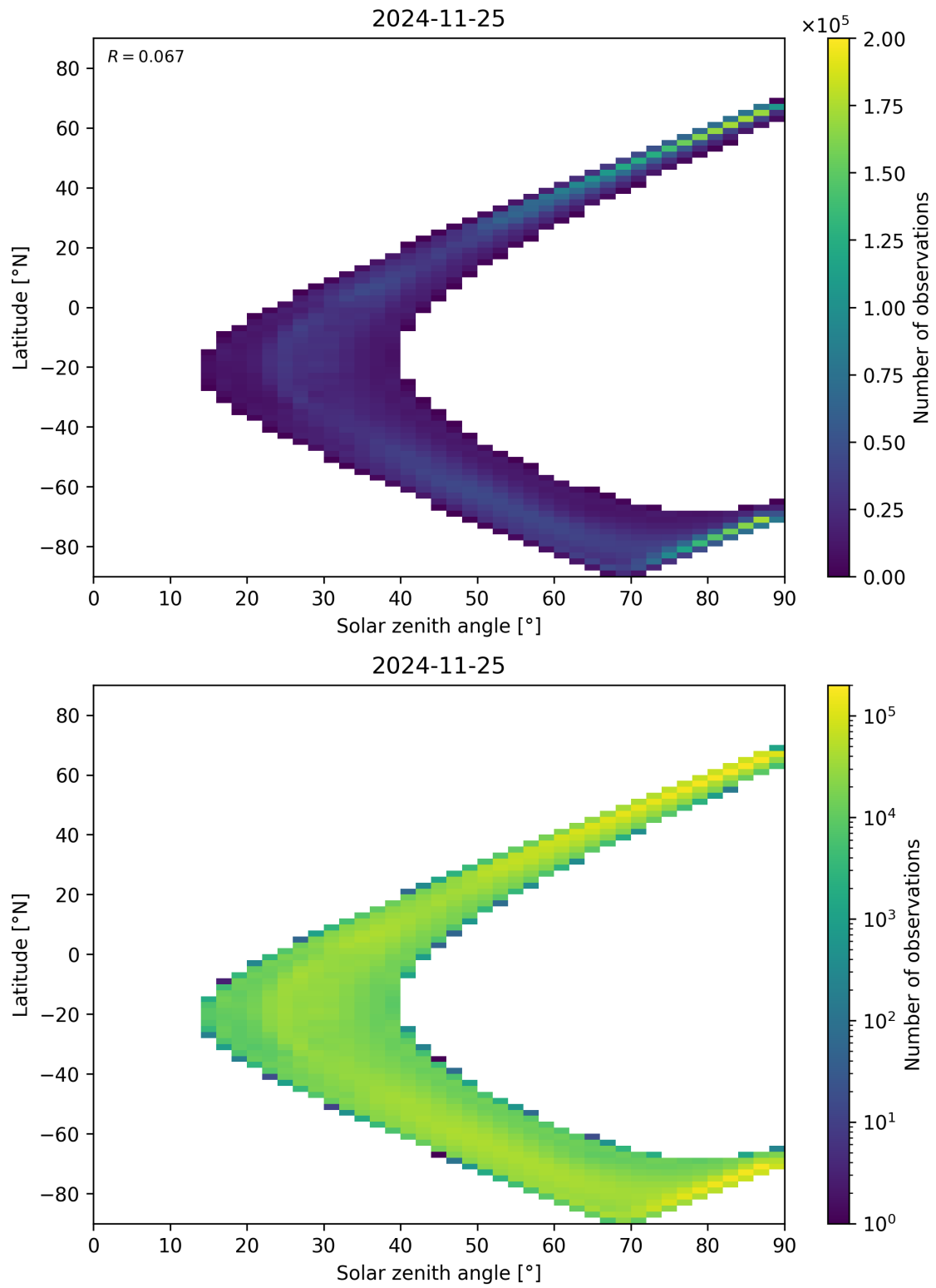
Figure 105: Scatter density plot of “Solar zenith angle” against “Latitude” for 2024-11-25 to 2024-11-26.
