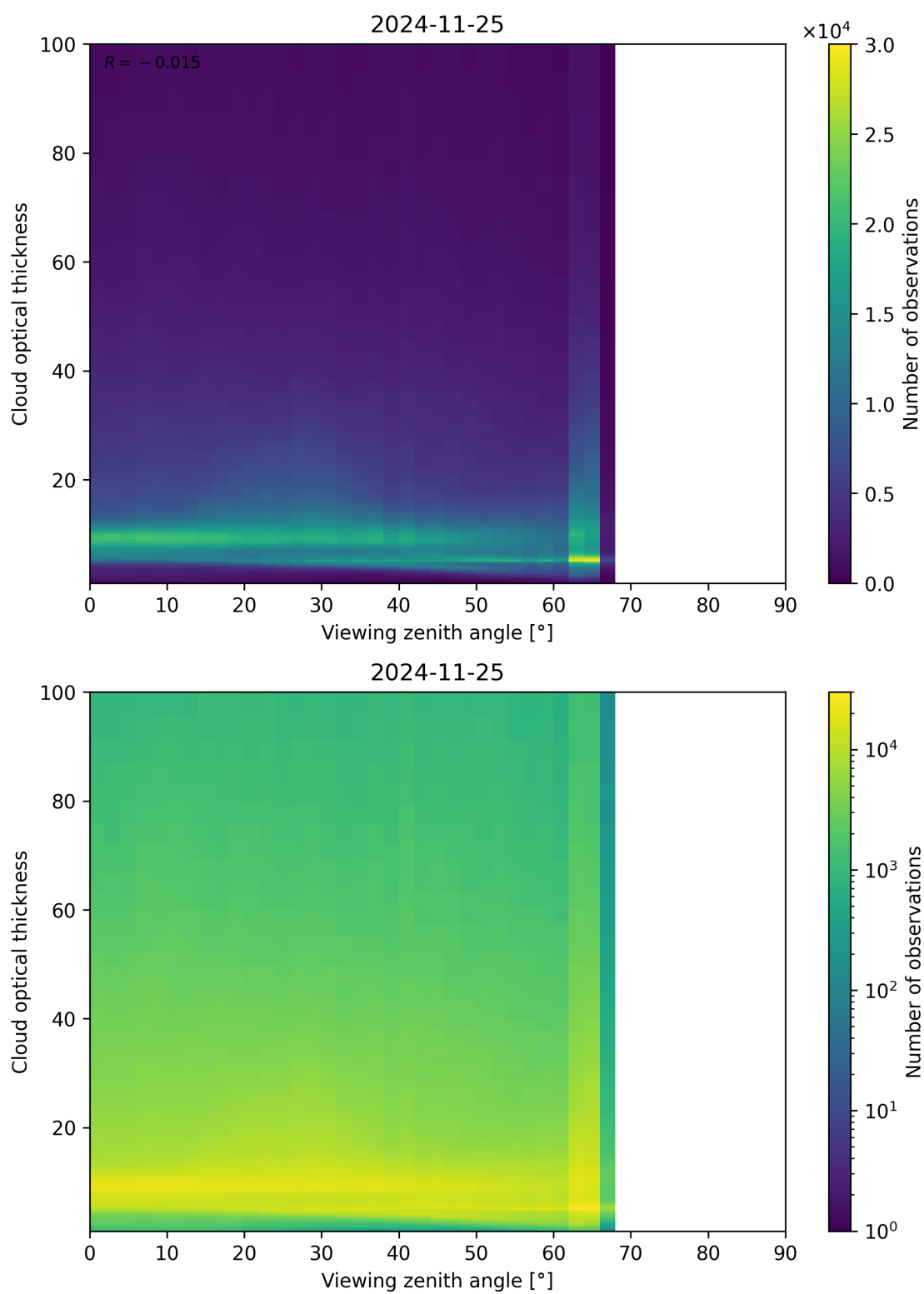
Figure 111: Scatter density plot of “Viewing zenith angle” against “Cloud optical thickness” for 2024-11-25 to 2024-11-26.
