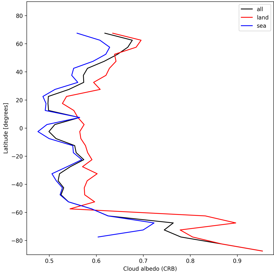
Figure 28: Zonal average of “Cloud albedo (CRB)” for 2024-11-25 to 2024-11-26.
