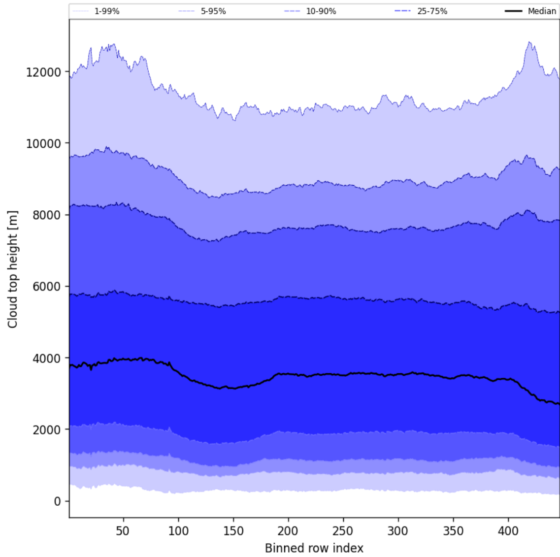
Figure 56: Along track statistics of “Cloud top height” for 2024-11-25 to 2024-11-26
