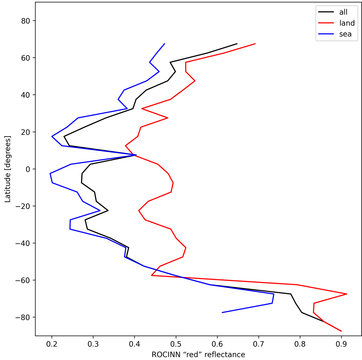
Figure 37: Zonal average of “ROCINN “red” reflectance” for 2024-11-25 to 2024-11-26.
