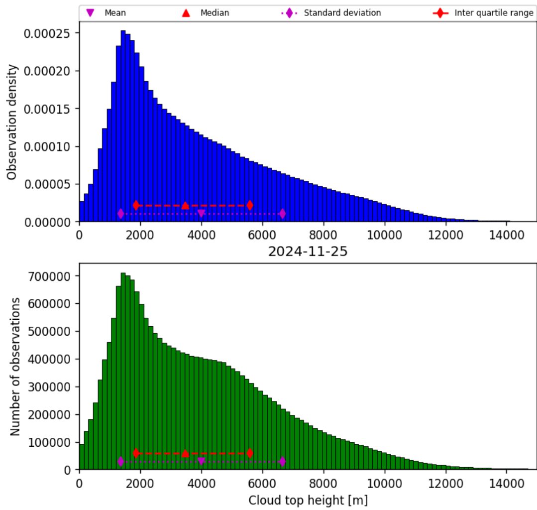
Figure 40: Histogram of “Cloud top height” for 2024-11-25 to 2024-11-26
