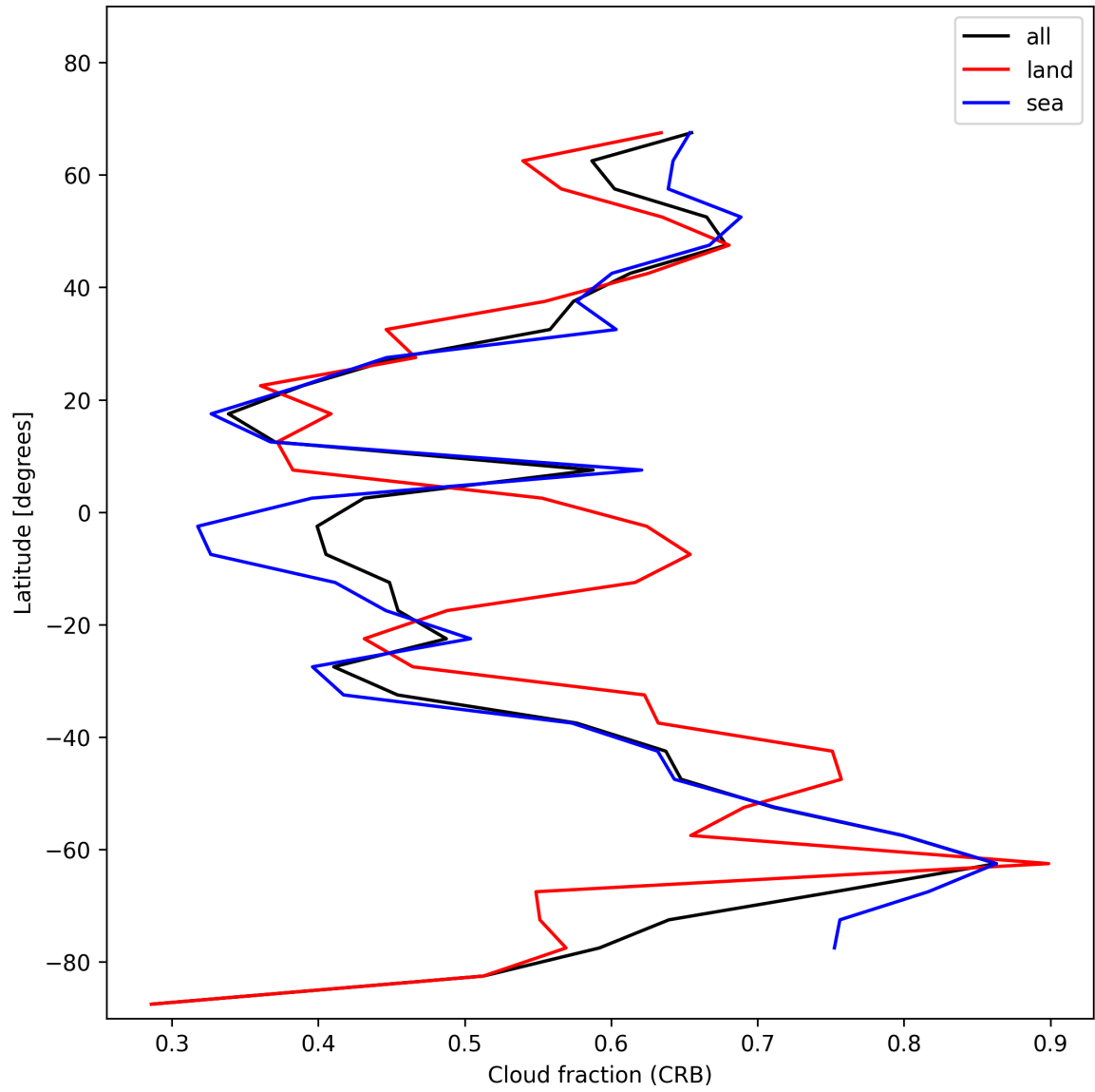
Figure 26: Zonal average of “Cloud fraction (CRB)” for 2024-11-25 to 2024-11-26.
