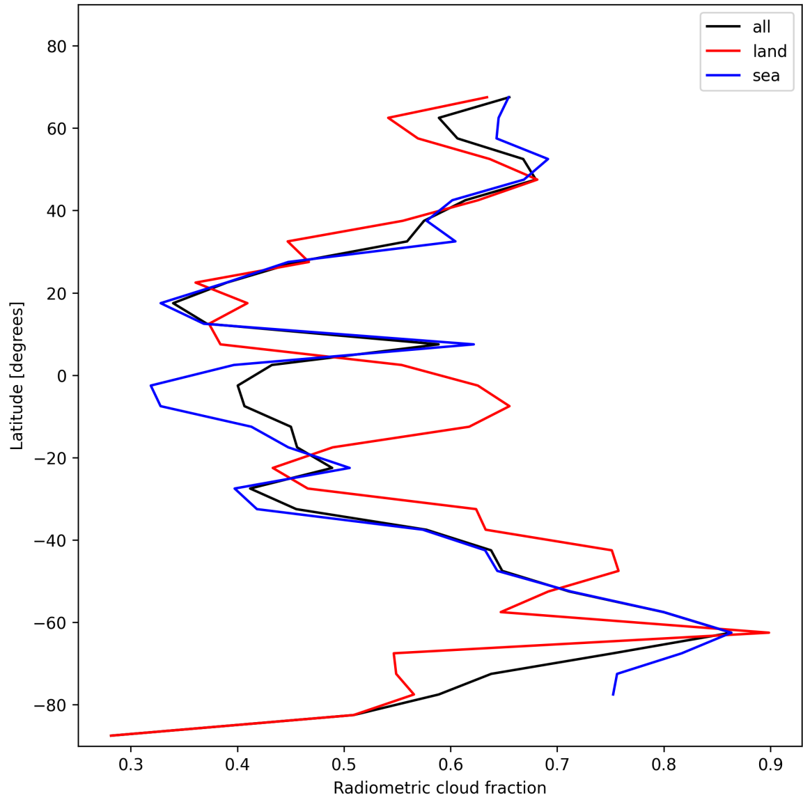
Figure 23: Zonal average of “Radiometric cloud fraction” for 2024-11-25 to 2024-11-26.
