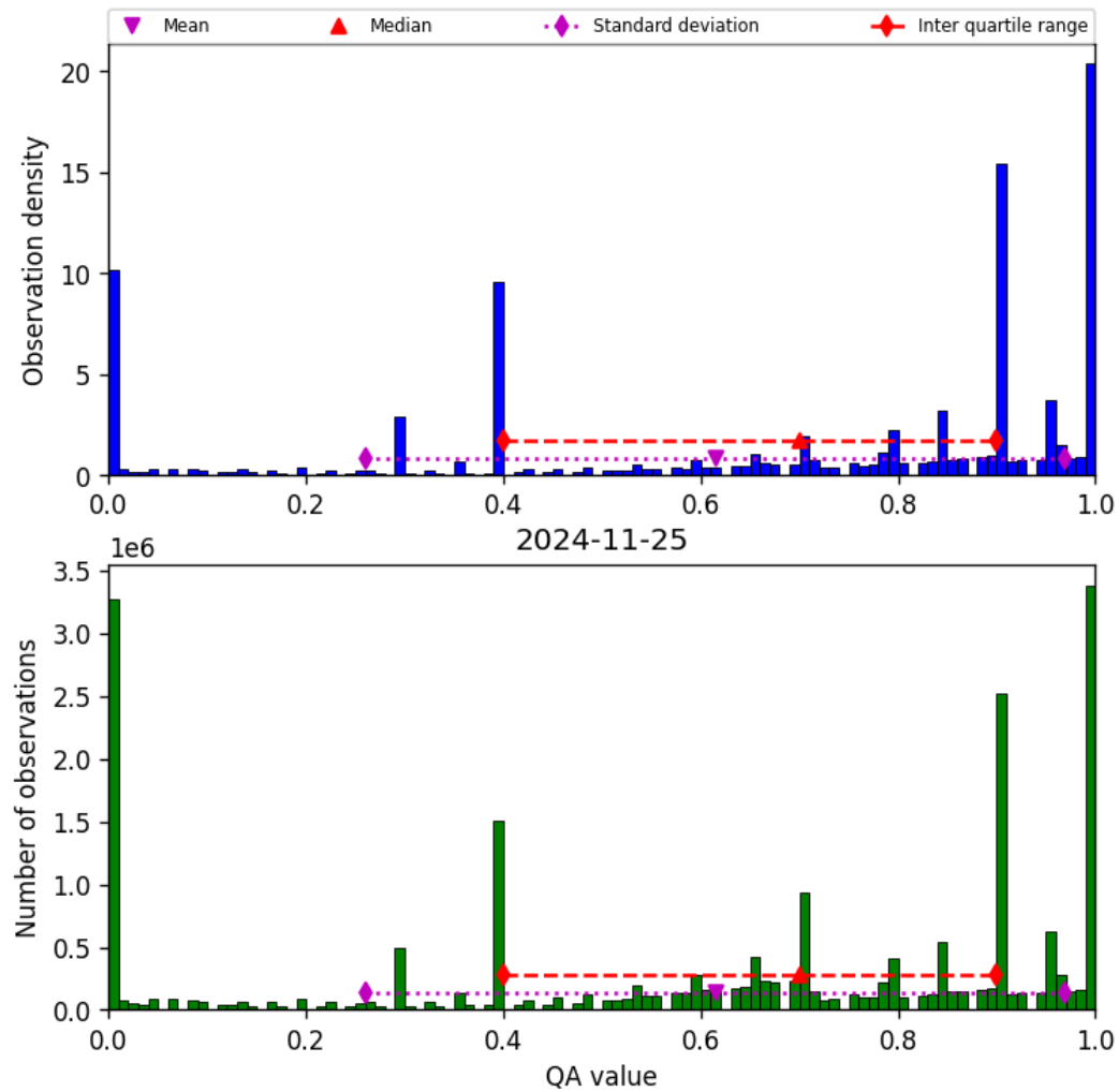
Figure 38: Histogram of “QA value” for 2024-11-25 to 2024-11-26
