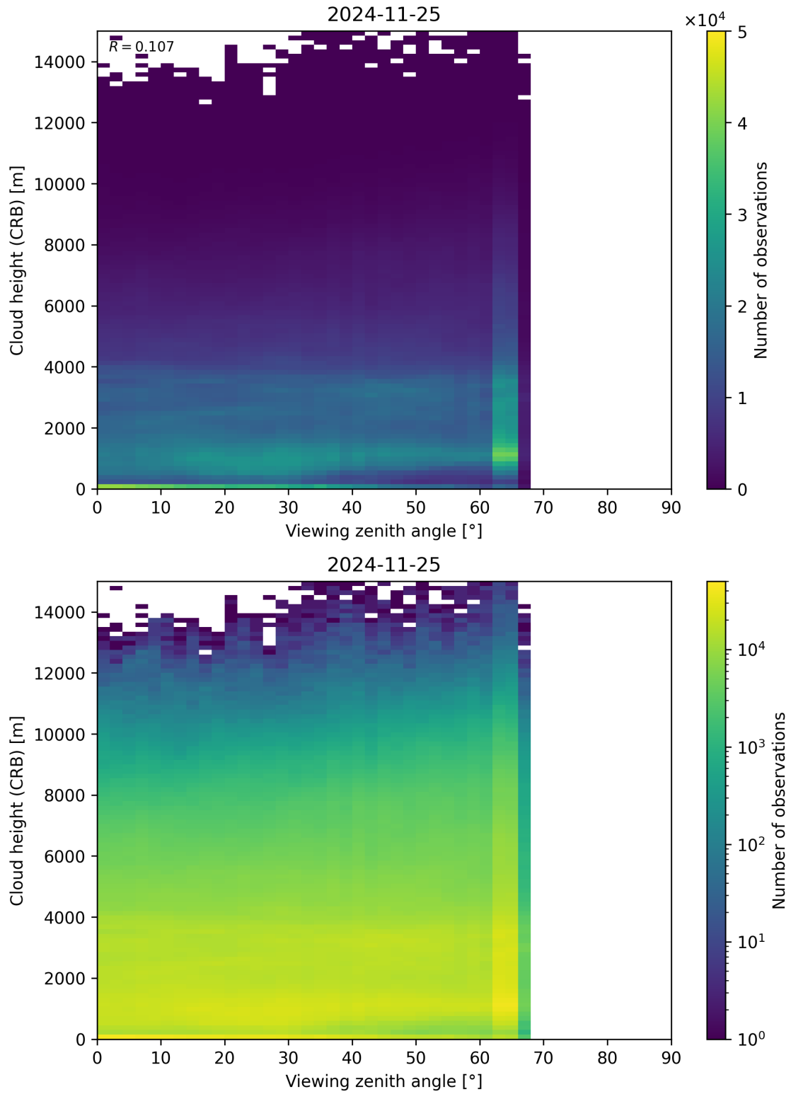
Figure 110: Scatter density plot of “Viewing zenith angle” against “Cloud height (CRB)” for 2024-11-25 to 2024-11-26.
