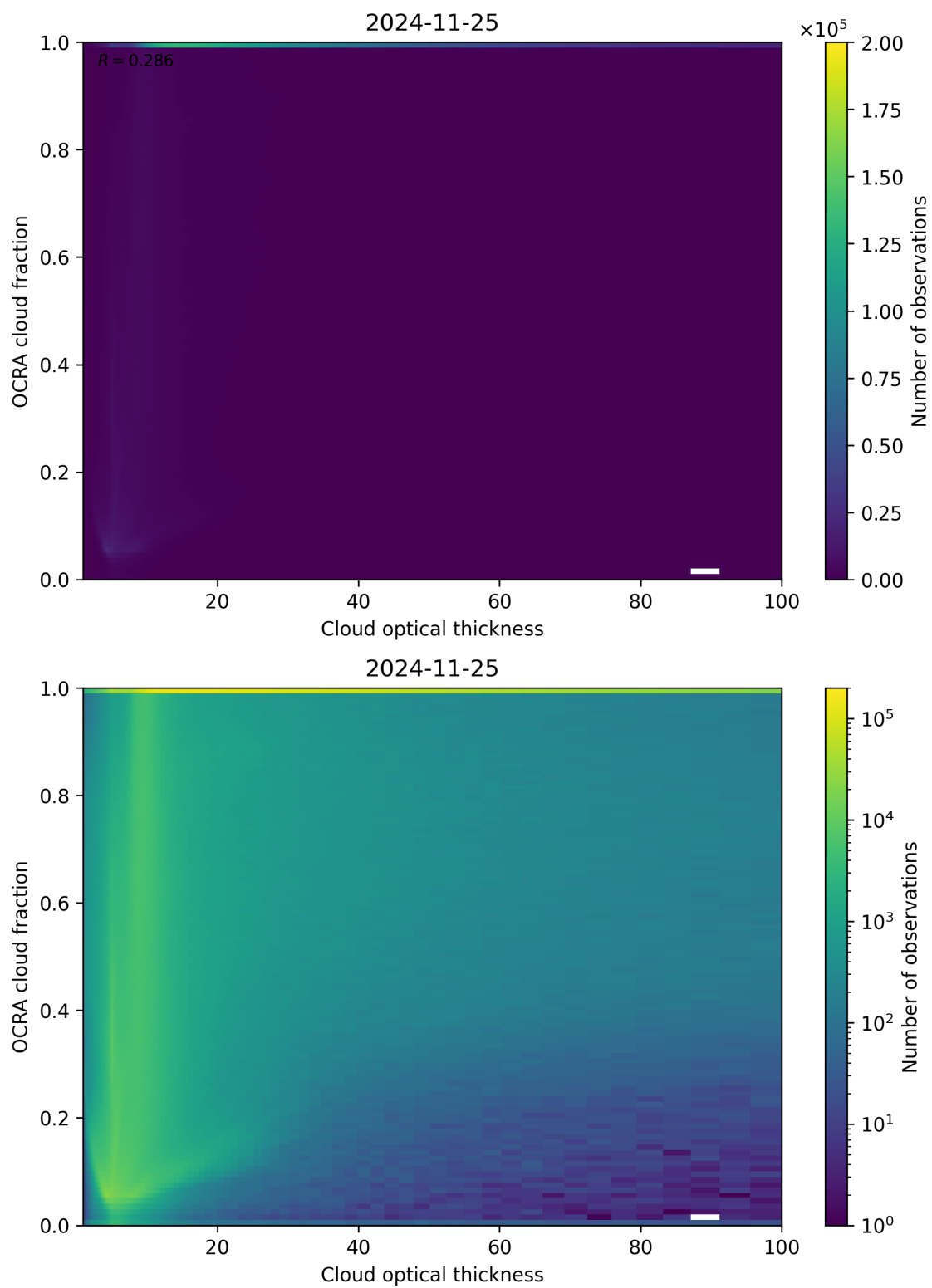
Figure 83: Scatter density plot of “Cloud optical thickness” against “OCRA cloud fraction” for 2024-11-25 to 2024-11-26.
