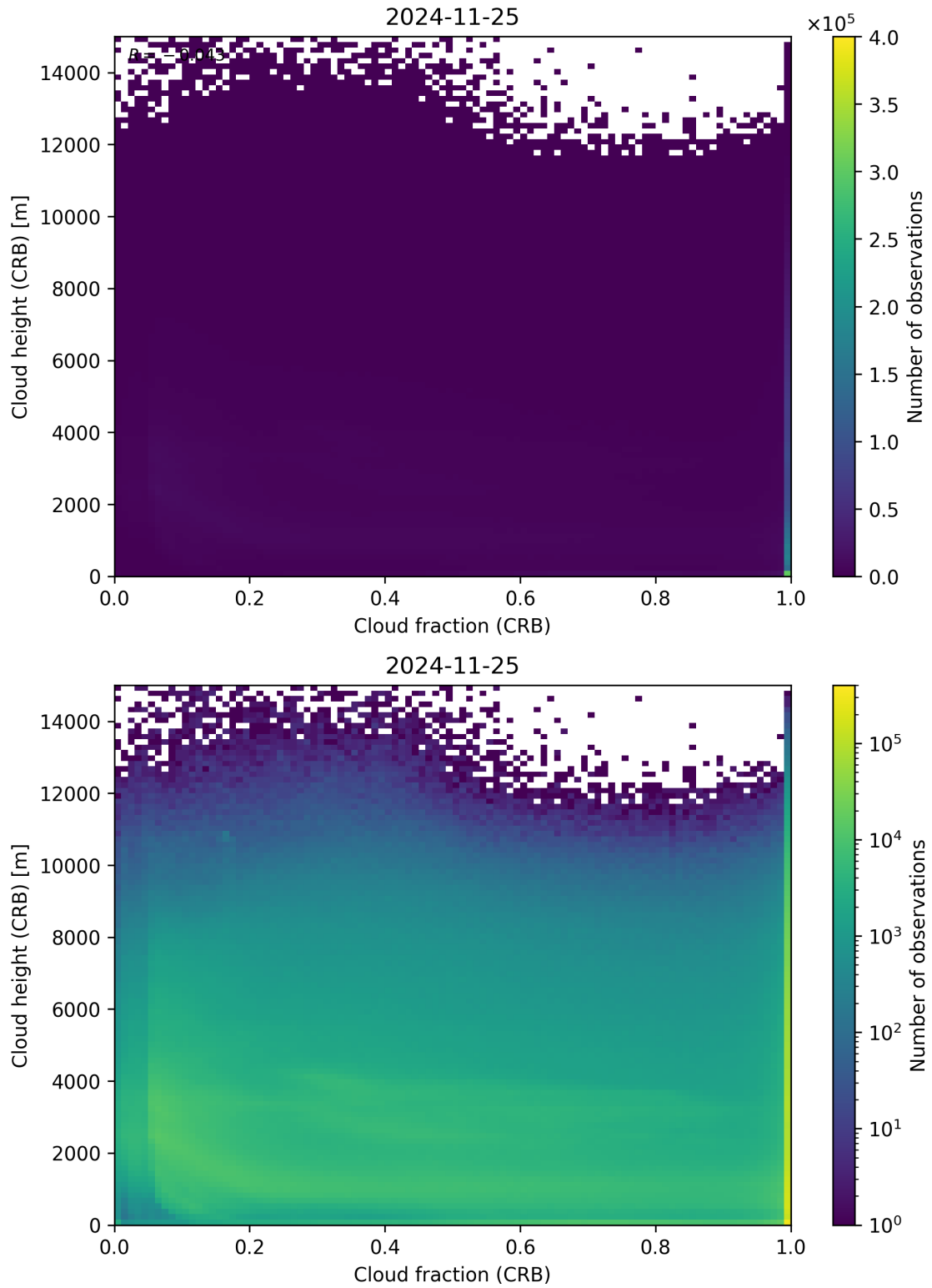
Figure 79: Scatter density plot of “Cloud fraction (CRB)” against “Cloud height (CRB)” for 2024-11-25 to 2024-11-26.
