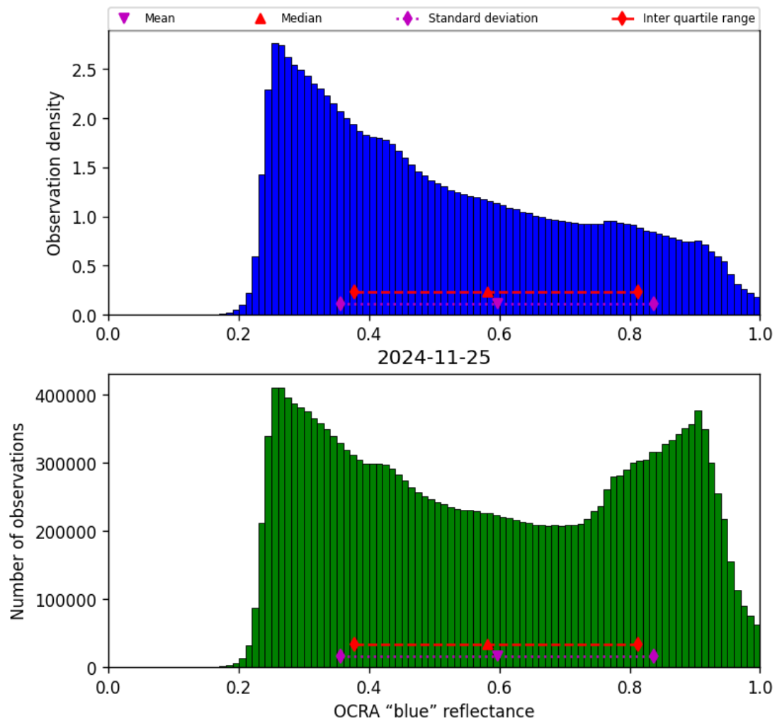
Figure 51: Histogram of “OCRA “blue” reflectance” for 2024-11-25 to 2024-11-26
