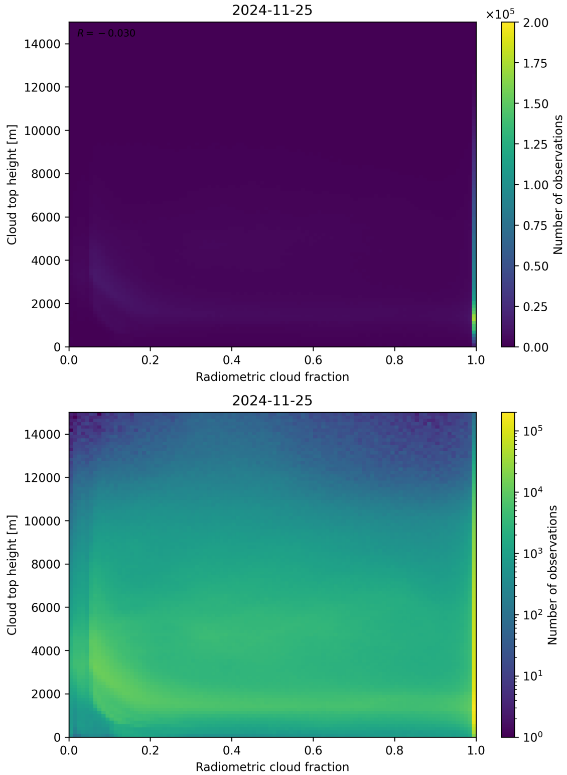
Figure 76: Scatter density plot of “Radiometric cloud fraction” against “Cloud top height” for 2024-11-25 to 2024-11-26.
