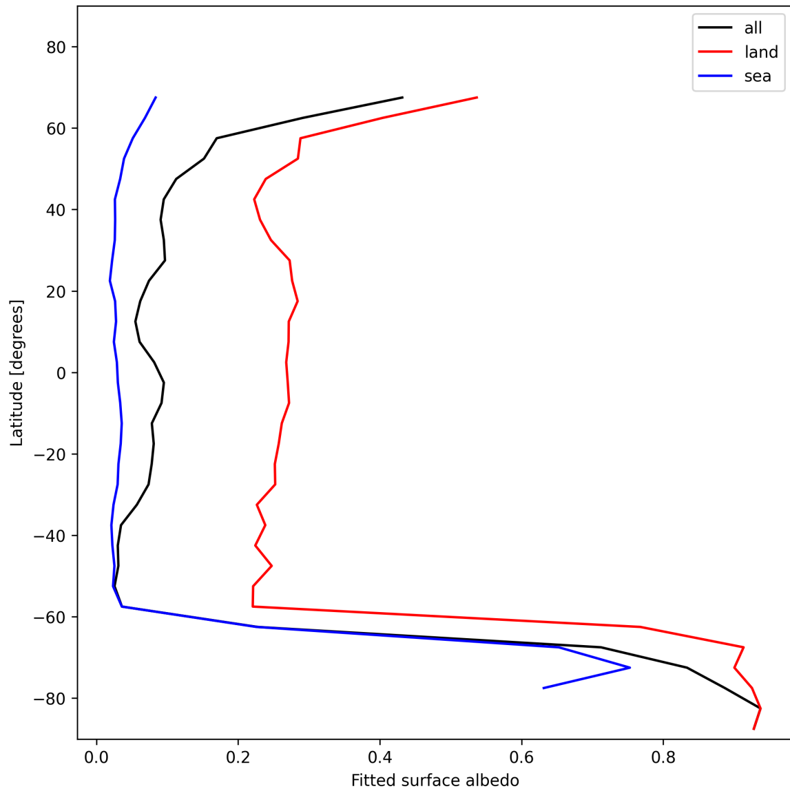
Figure 29: Zonal average of “Fitted surface albedo” for 2024-11-25 to 2024-11-26.
