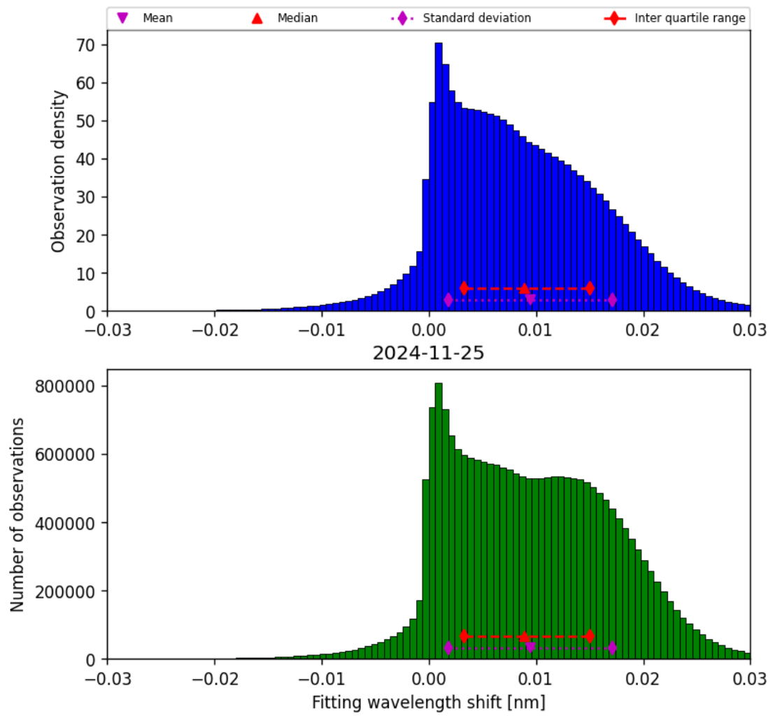
Figure 49: Histogram of “Fitting wavelength shift” for 2024-11-25 to 2024-11-26
