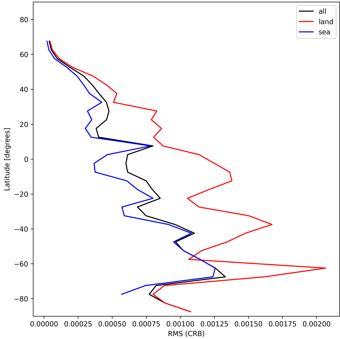
Figure 32: Zonal average of “RMS (CRB)” for 2024-11-25 to 2024-11-26.
