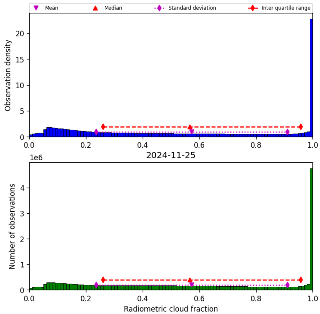
Figure 39: Histogram of “Radiometric cloud fraction” for 2024-11-25 to 2024-11-26
