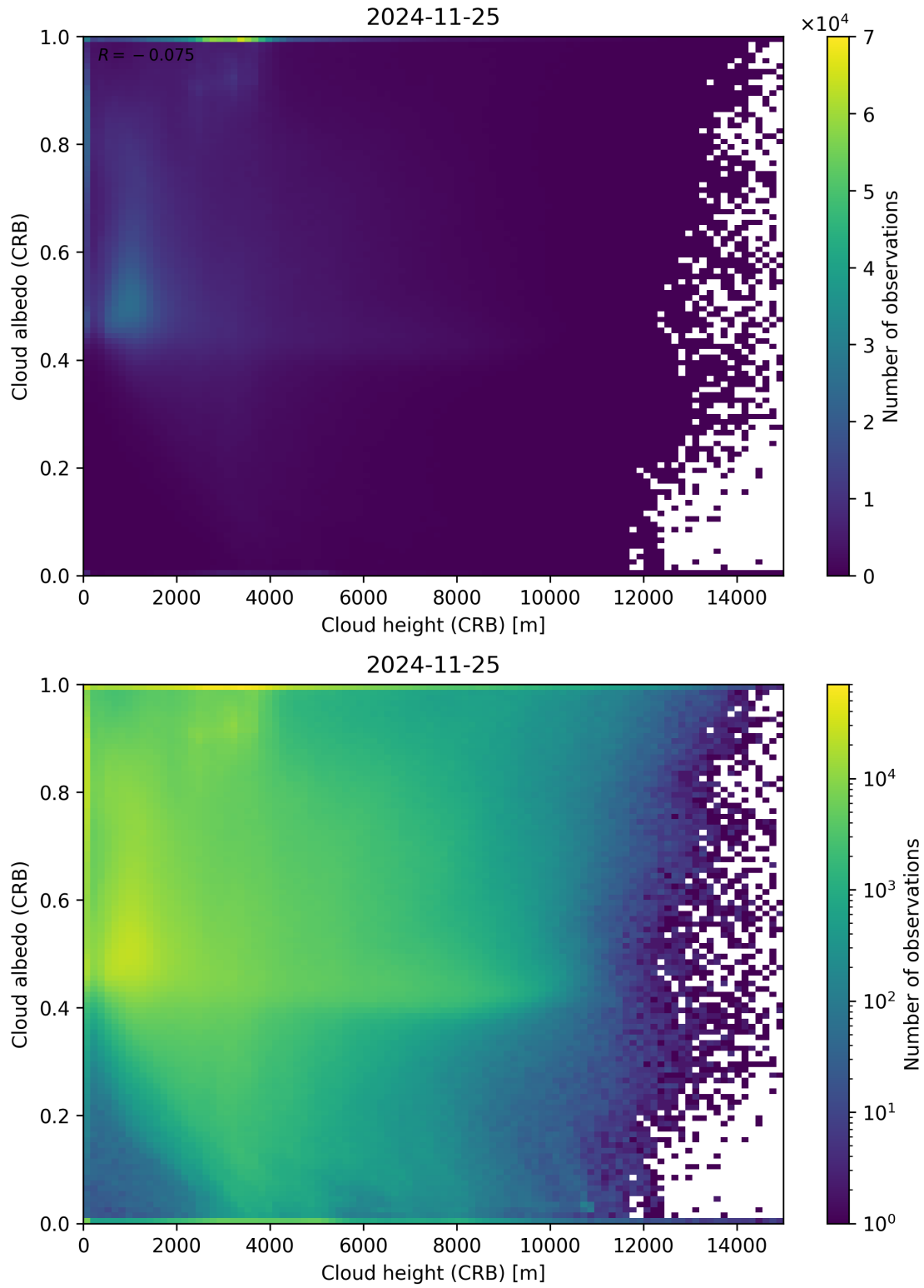
Figure 80: Scatter density plot of “Cloud height (CRB)” against “Cloud albedo (CRB)” for 2024-11-25 to 2024-11-26.
