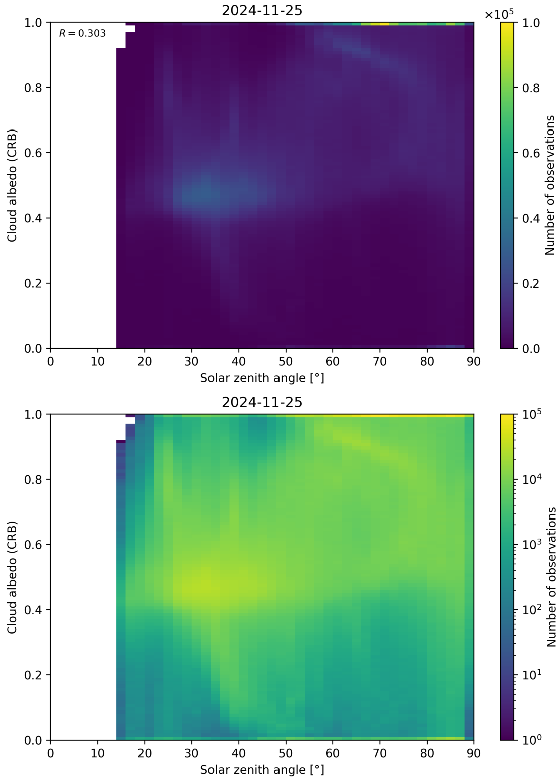
Figure 98: Scatter density plot of “Solar zenith angle” against “Cloud albedo (CRB)” for 2024-11-25 to 2024-11-26.
