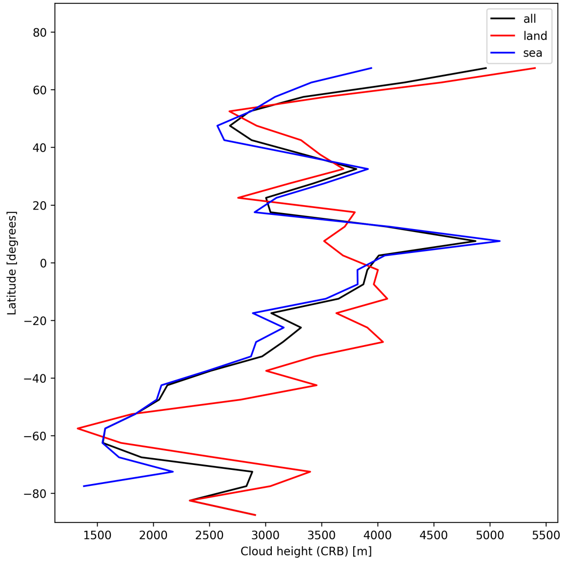
Figure 27: Zonal average of “Cloud height (CRB)” for 2024-11-25 to 2024-11-26.
