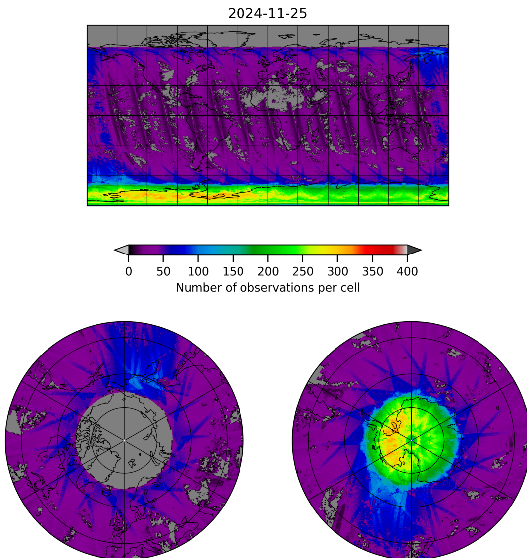
Figure 21: Map of the number of observations for 2024-11-25 to 2024-11-26
