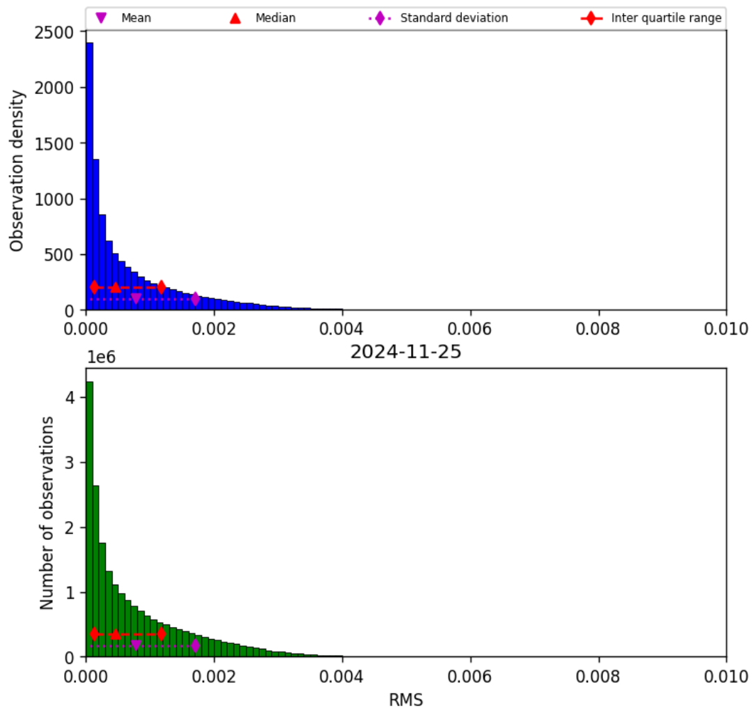
Figure 47: Histogram of “RMS” for 2024-11-25 to 2024-11-26
