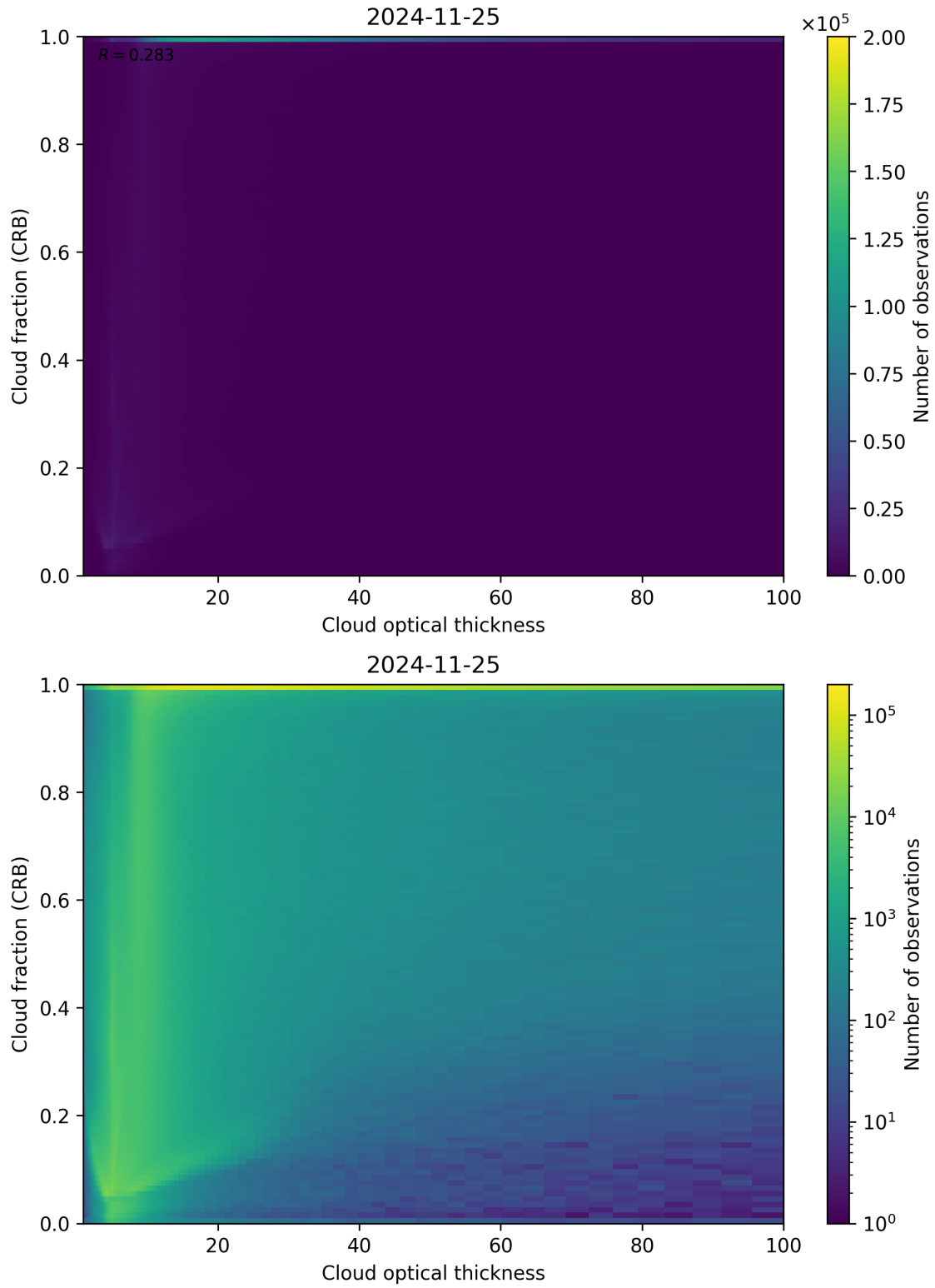
Figure 84: Scatter density plot of “Cloud optical thickness” against “Cloud fraction (CRB)” for 2024-11-25 to 2024-11-26.
