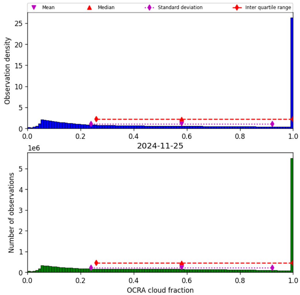
Figure 50: Histogram of “OCRA cloud fraction” for 2024-11-25 to 2024-11-26
