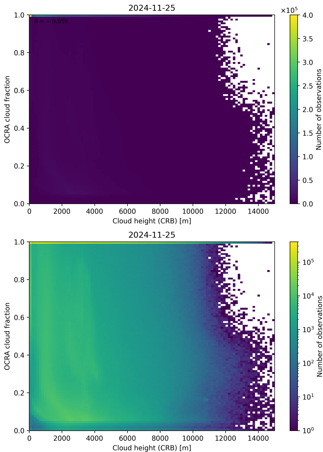
Figure 81: Scatter density plot of “Cloud height (CRB)” against “OCRA cloud fraction” for 2024-11-25 to 2024-11-26.
