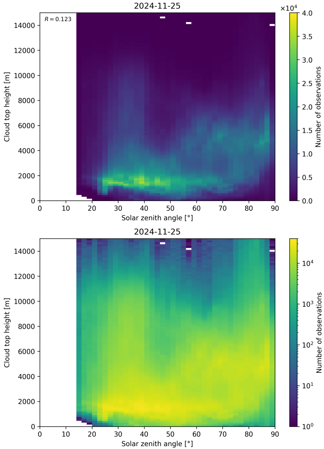
Figure 104: Scatter density plot of “Solar zenith angle” against “Cloud top height” for 2024-11-25 to 2024-11-26.
