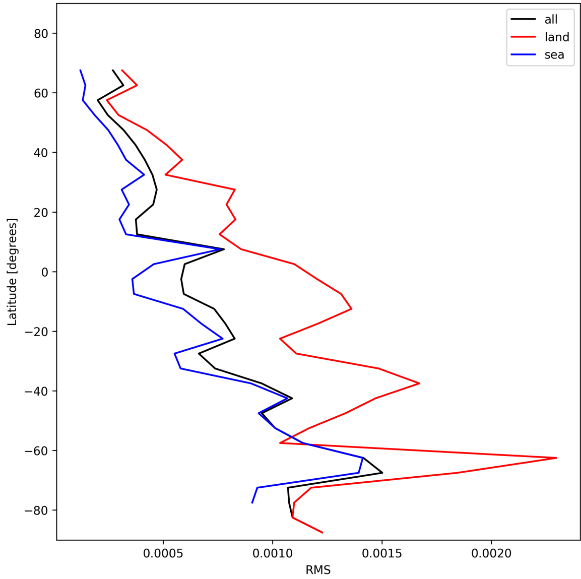
Figure 31: Zonal average of “RMS” for 2024-11-25 to 2024-11-26.
