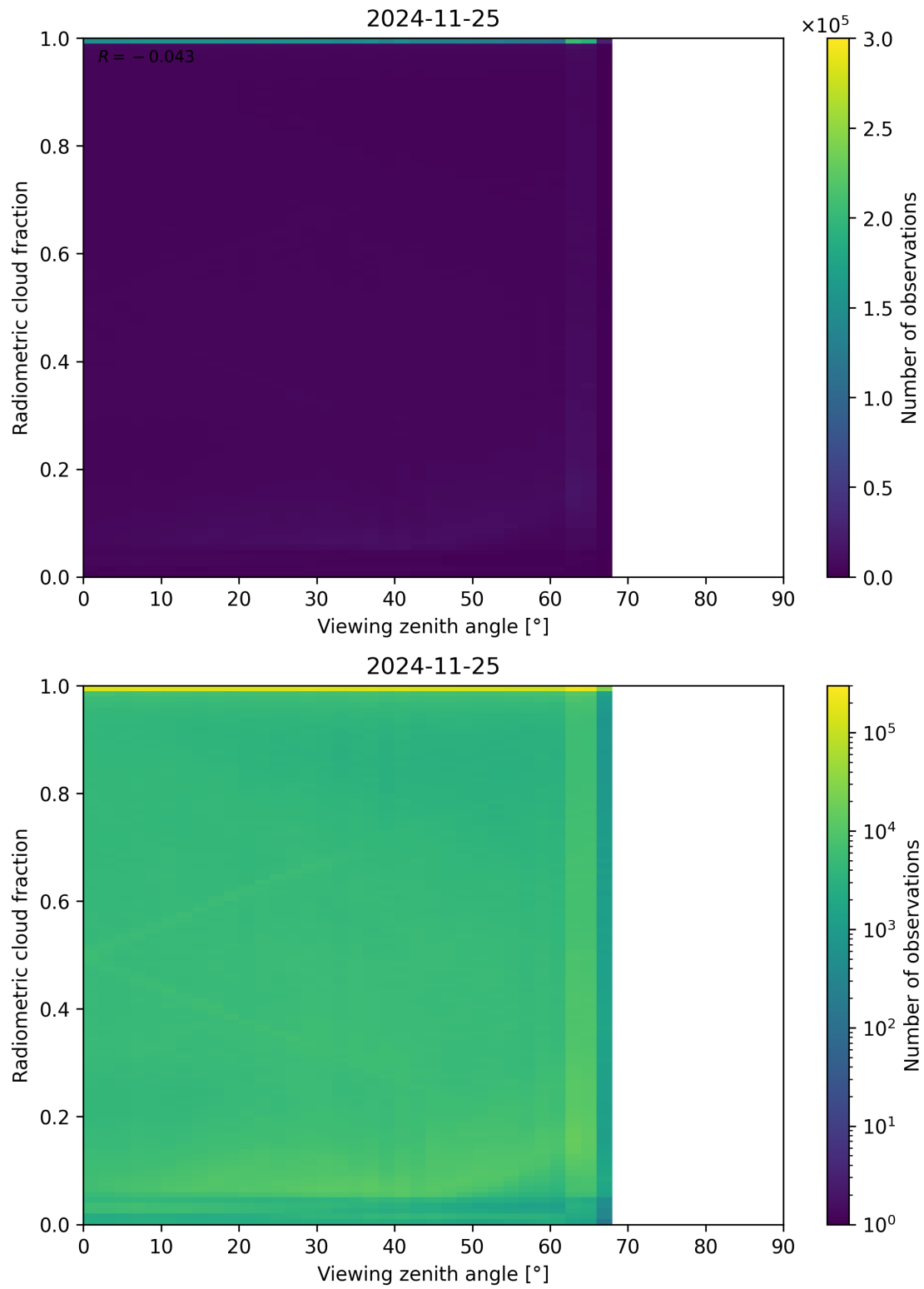
Figure 107: Scatter density plot of “Viewing zenith angle” against “Radiometric cloud fraction” for 2024-11-25 to 2024-11-26.
