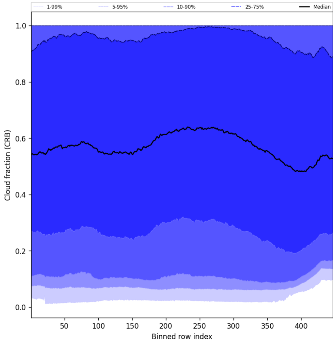
Figure 58: Along track statistics of “Cloud fraction (CRB)” for 2024-11-25 to 2024-11-26
