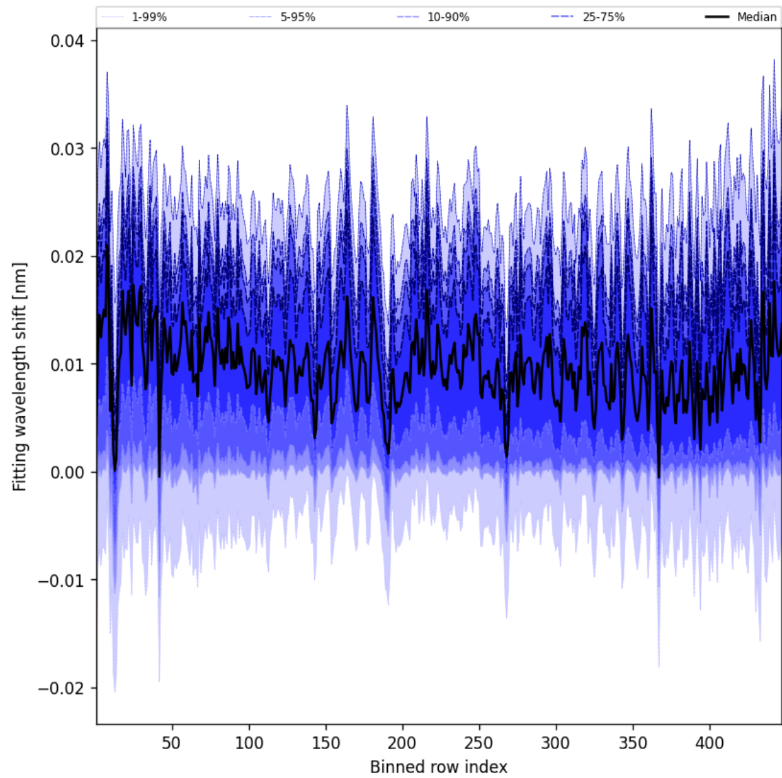
Figure 65: Along track statistics of “Fitting wavelength shift” for 2024-11-25 to 2024-11-26
