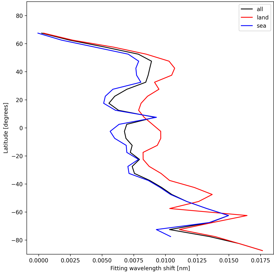
Figure 33: Zonal average of “Fitting wavelength shift” for 2024-11-25 to 2024-11-26.
