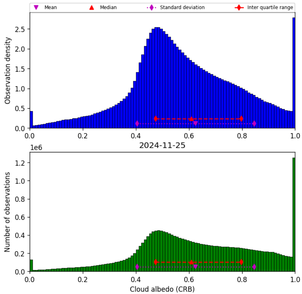
Figure 44: Histogram of “Cloud albedo (CRB)” for 2024-11-25 to 2024-11-26
