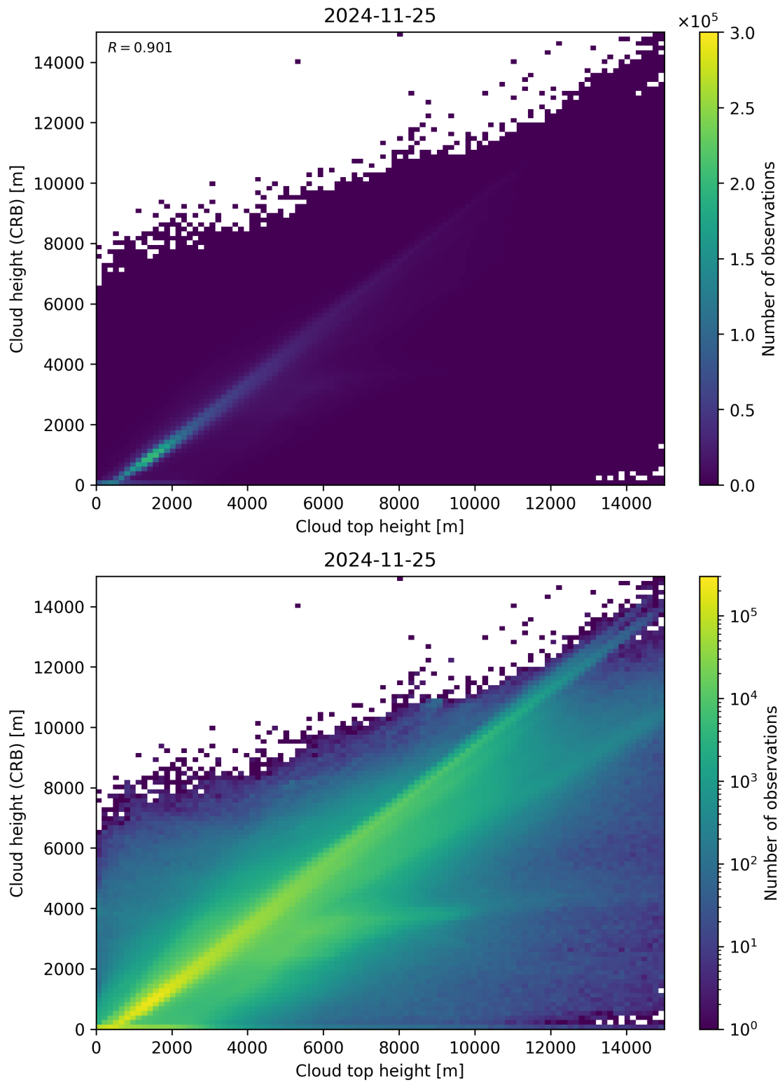
Figure 89: Scatter density plot of “Cloud top height” against “Cloud height (CRB)” for 2024-11-25 to 2024-11-26.
