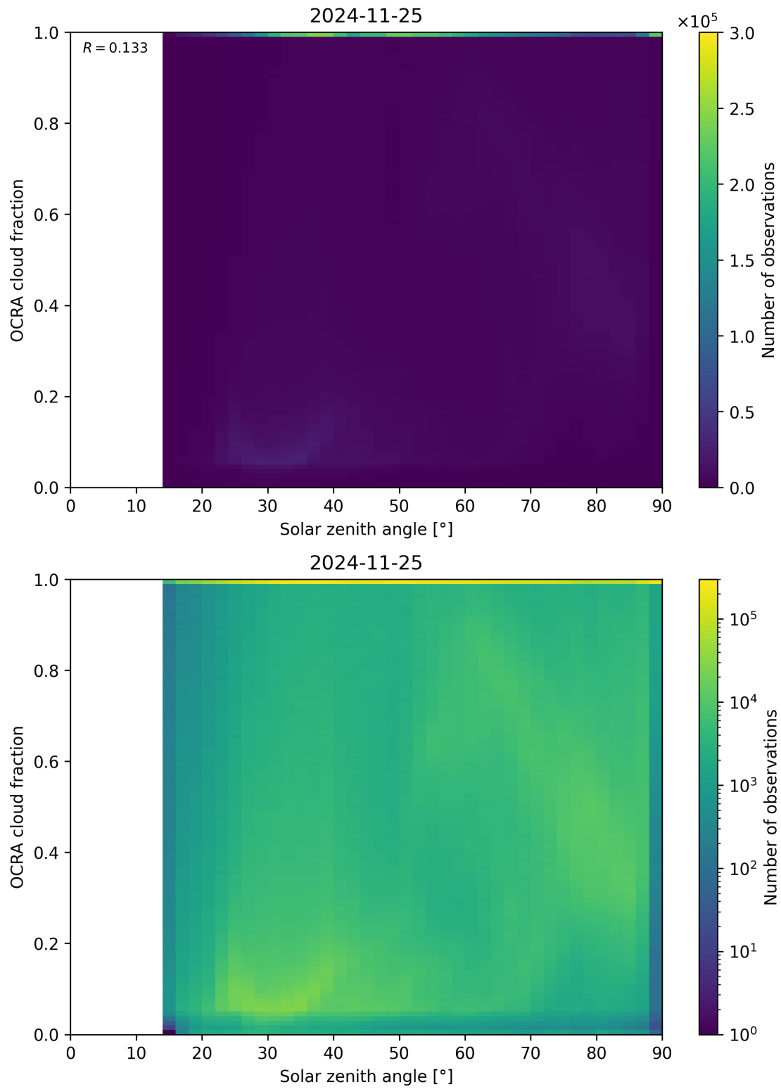
Figure 100: Scatter density plot of “Solar zenith angle” against “OCRA cloud fraction” for 2024-11-25 to 2024-11-26.
