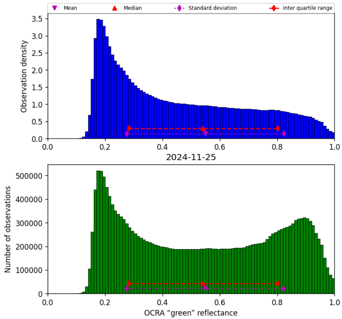
Figure 52: Histogram of “OCRA “green” reflectance” for 2024-11-25 to 2024-11-26
