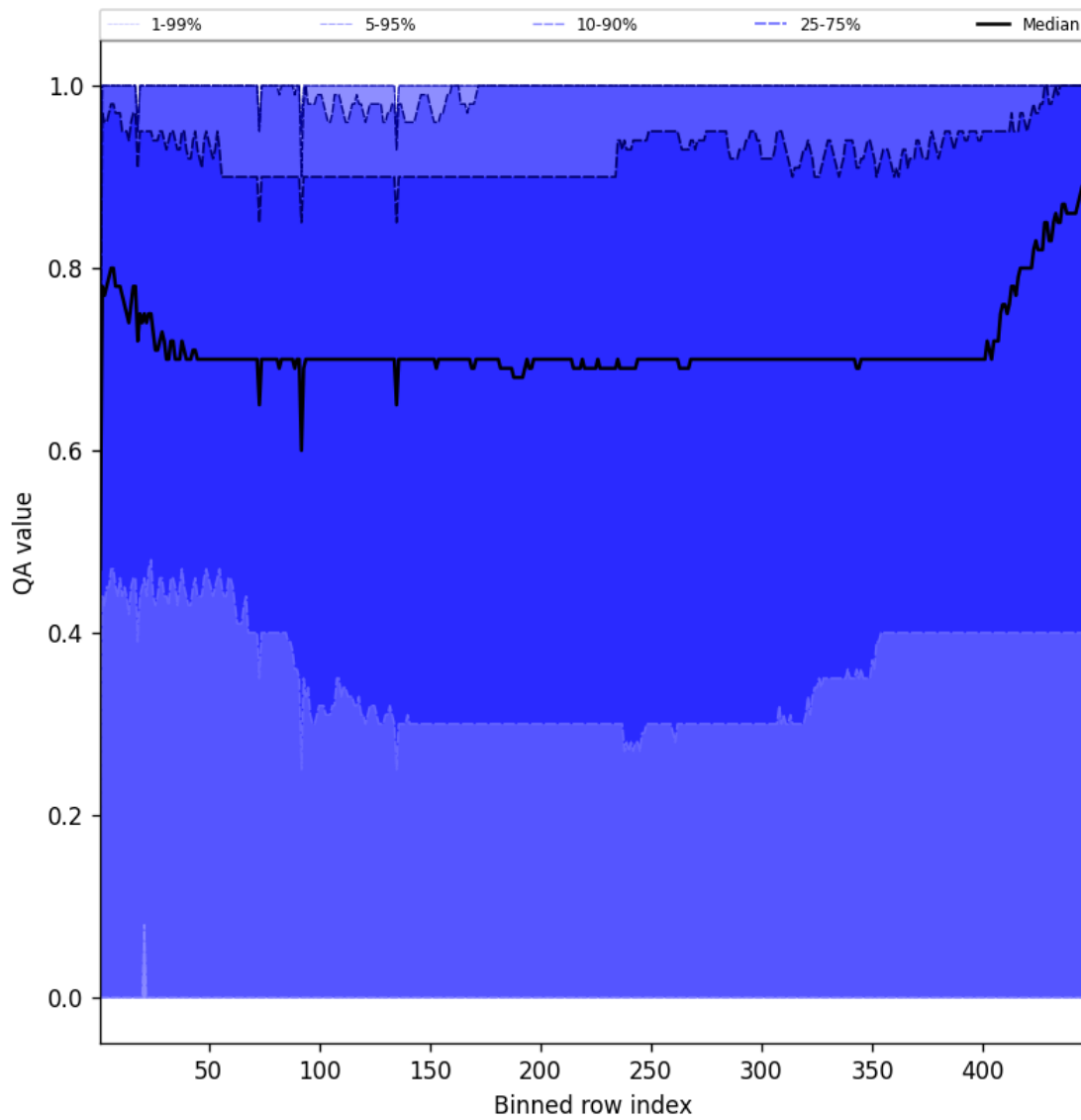
Figure 54: Along track statistics of “QA value” for 2024-11-25 to 2024-11-26
