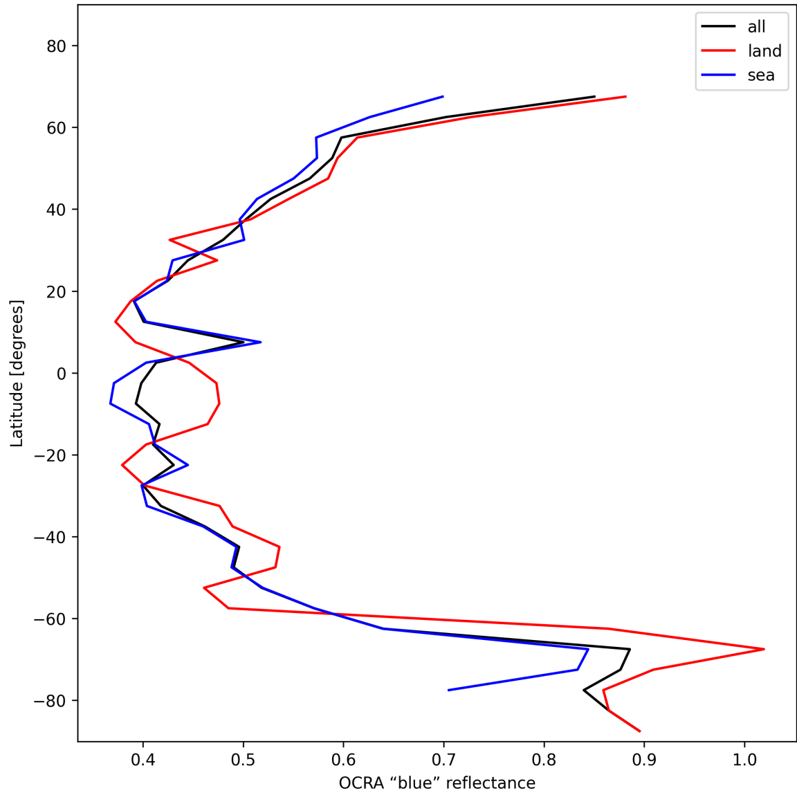
Figure 35: Zonal average of “OCRA “blue” reflectance” for 2024-11-25 to 2024-11-26.
