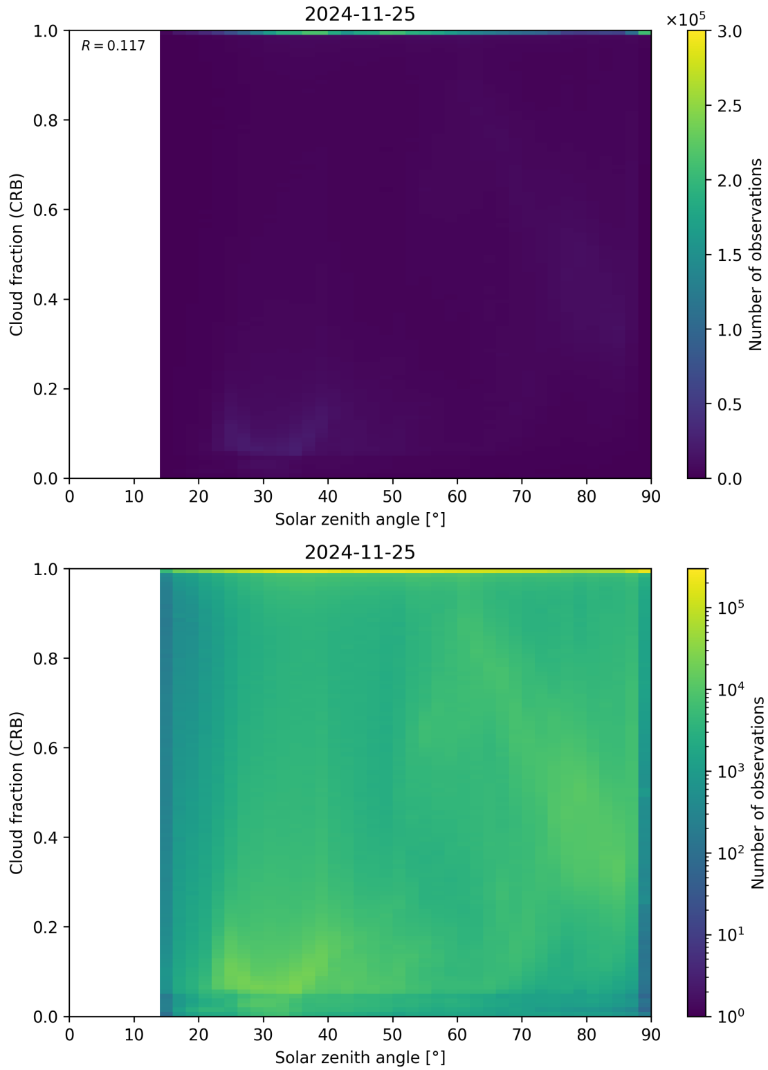
Figure 101: Scatter density plot of “Solar zenith angle” against “Cloud fraction (CRB)” for 2024-11-25 to 2024-11-26.
