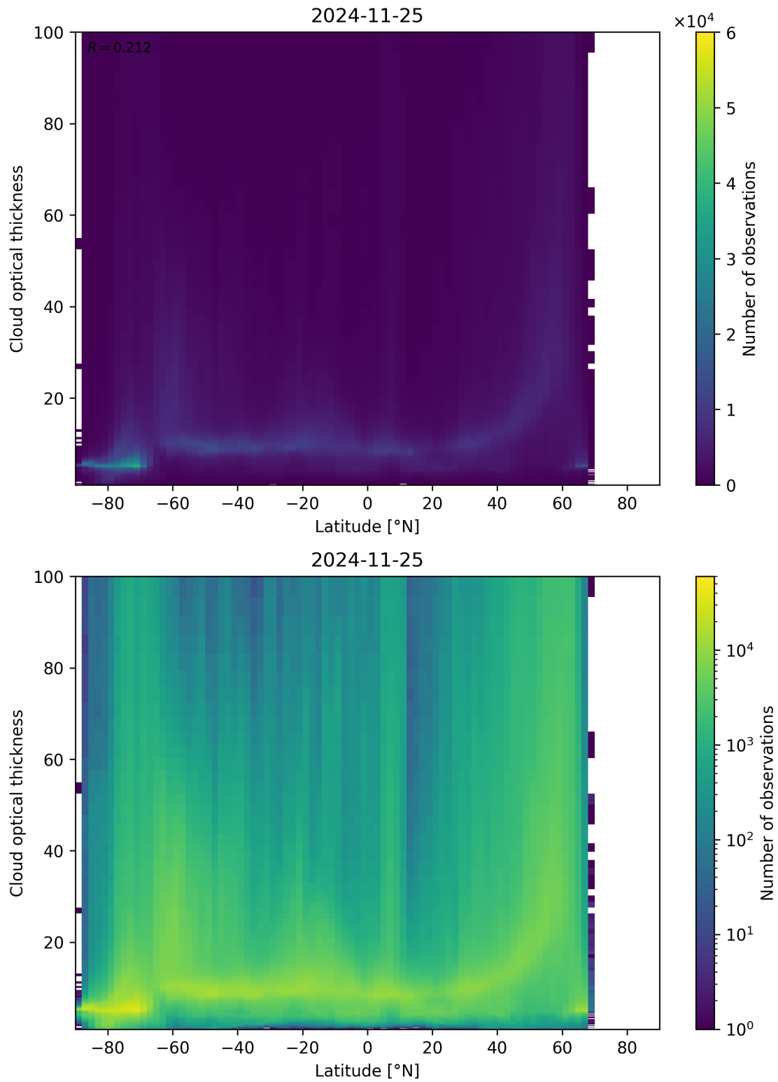
Figure 96: Scatter density plot of “Latitude” against “Cloud optical thickness” for 2024-11-25 to 2024-11-26.
