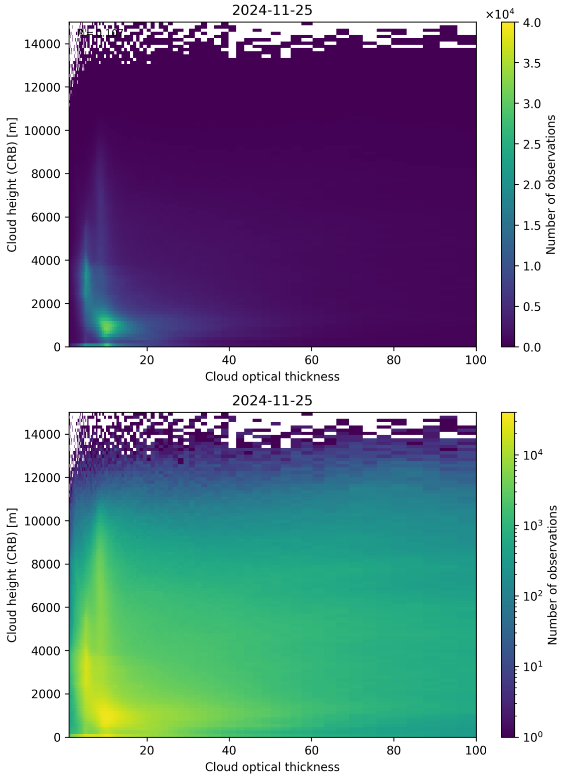
Figure 85: Scatter density plot of “Cloud optical thickness” against “Cloud height (CRB)” for 2024-11-25 to 2024-11-26.
