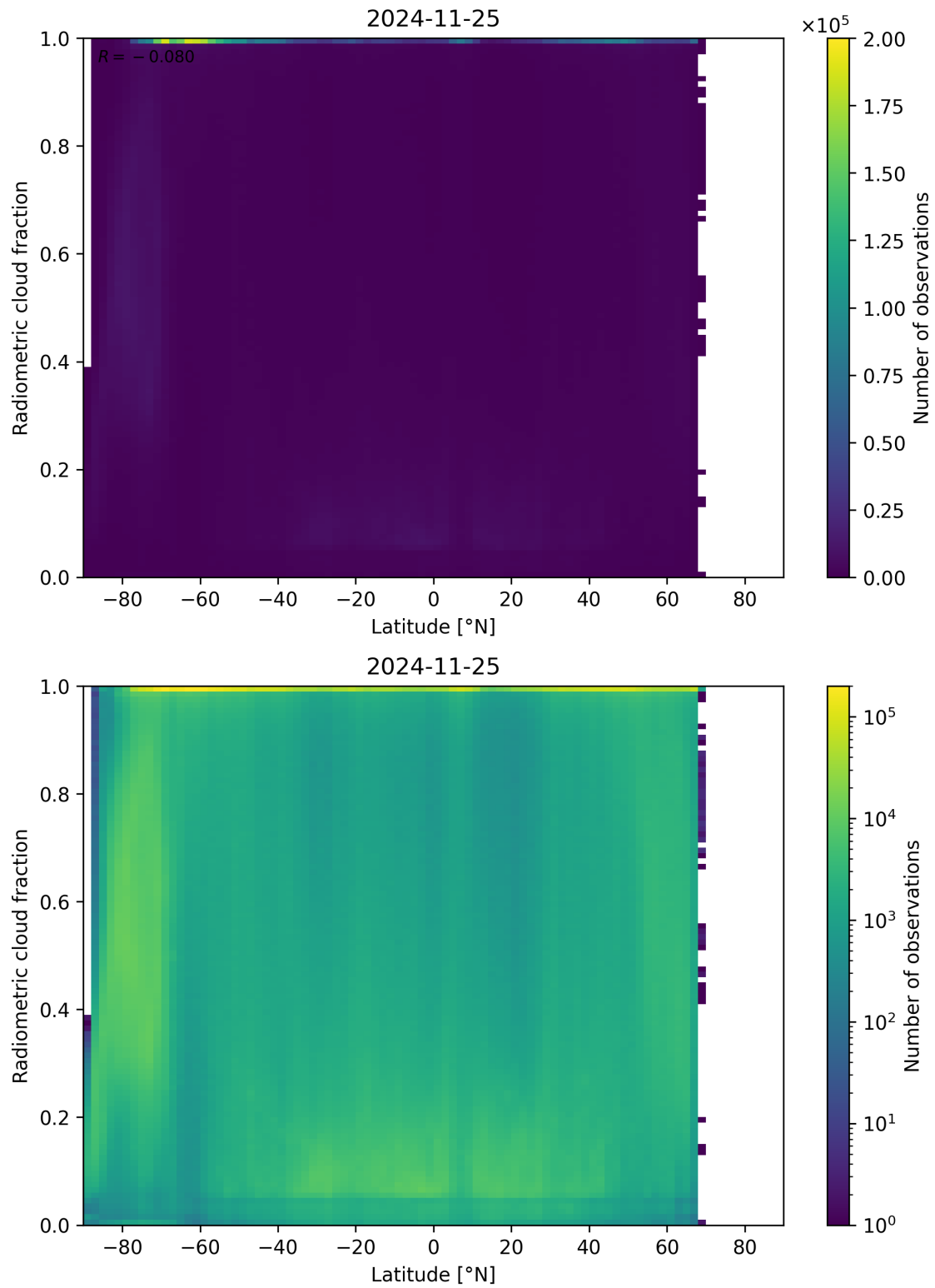
Figure 92: Scatter density plot of “Latitude” against “Radiometric cloud fraction” for 2024-11-25 to 2024-11-26.
