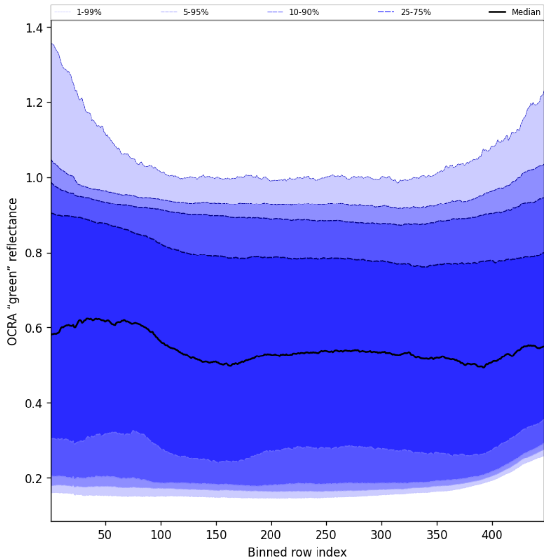
Figure 68: Along track statistics of “OCRA “green” reflectance” for 2024-11-25 to 2024-11-26
