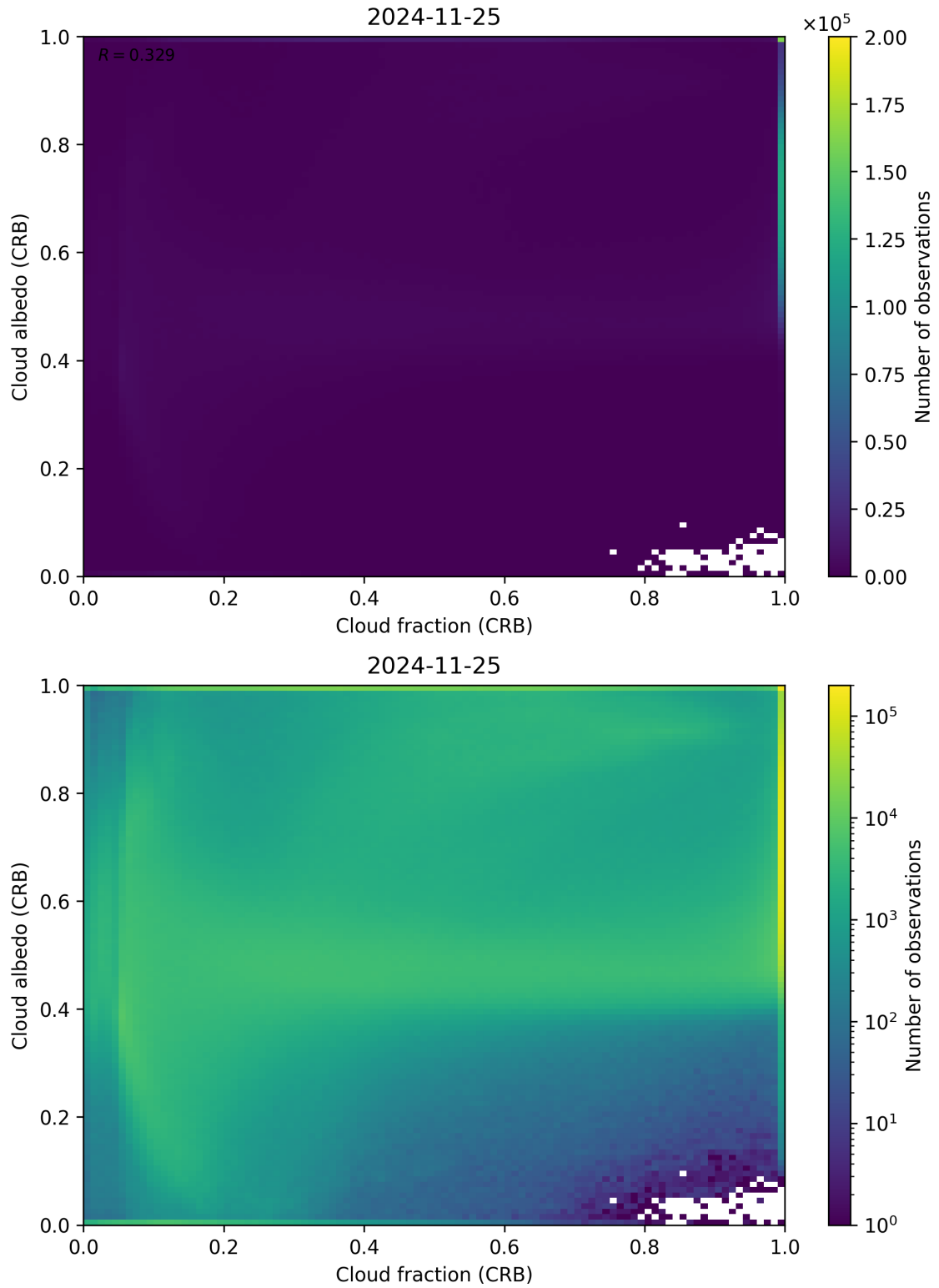
Figure 77: Scatter density plot of “Cloud fraction (CRB)” against “Cloud albedo (CRB)” for 2024-11-25 to 2024-11-26.
