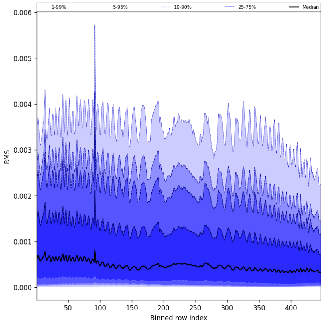
Figure 63: Along track statistics of “RMS” for 2024-11-25 to 2024-11-26
