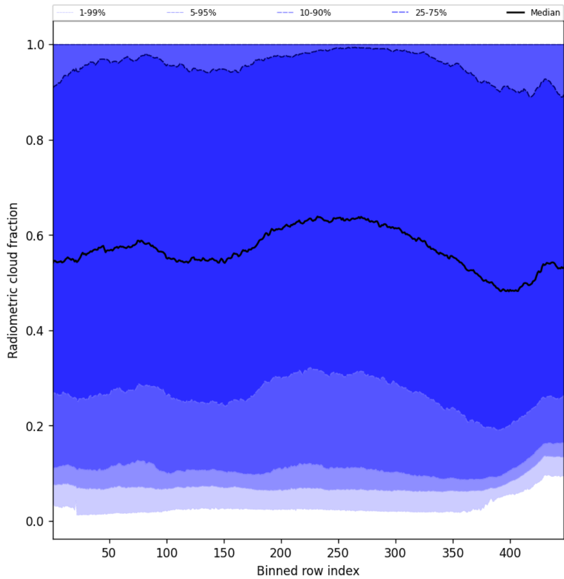
Figure 55: Along track statistics of “Radiometric cloud fraction” for 2024-11-25 to 2024-11-26
