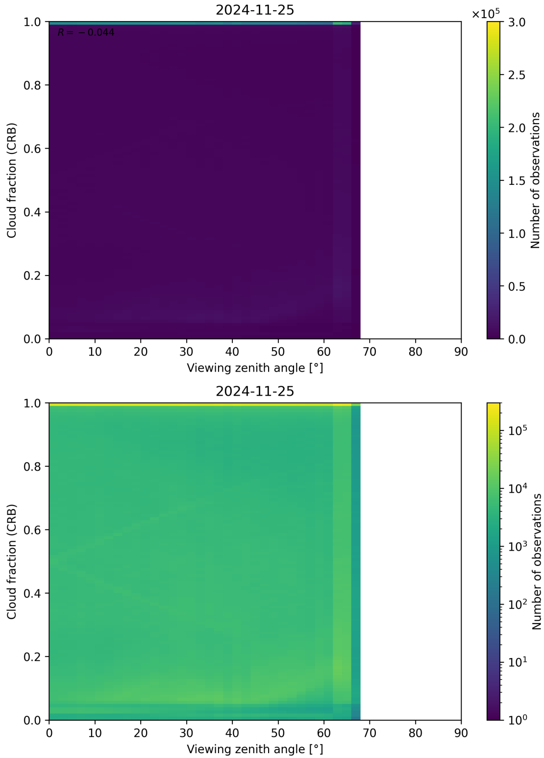
Figure 109: Scatter density plot of “Viewing zenith angle” against “Cloud fraction (CRB)” for 2024-11-25 to 2024-11-26.
