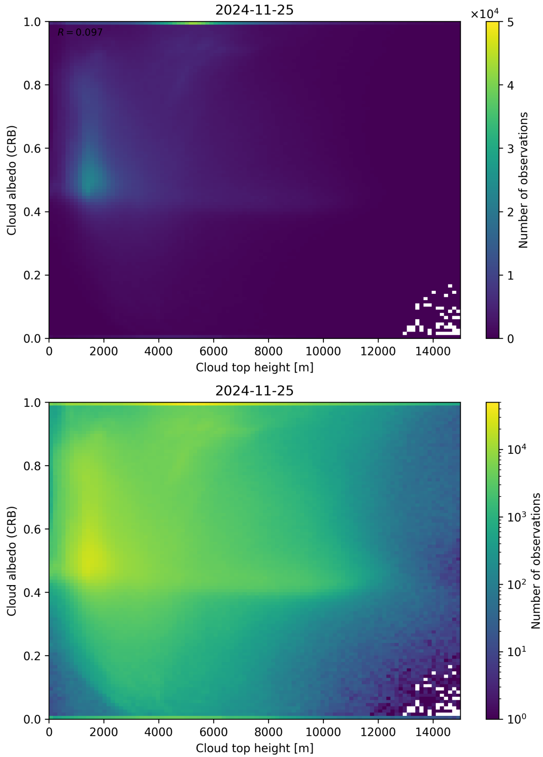
Figure 86: Scatter density plot of “Cloud top height” against “Cloud albedo (CRB)” for 2024-11-25 to 2024-11-26.
