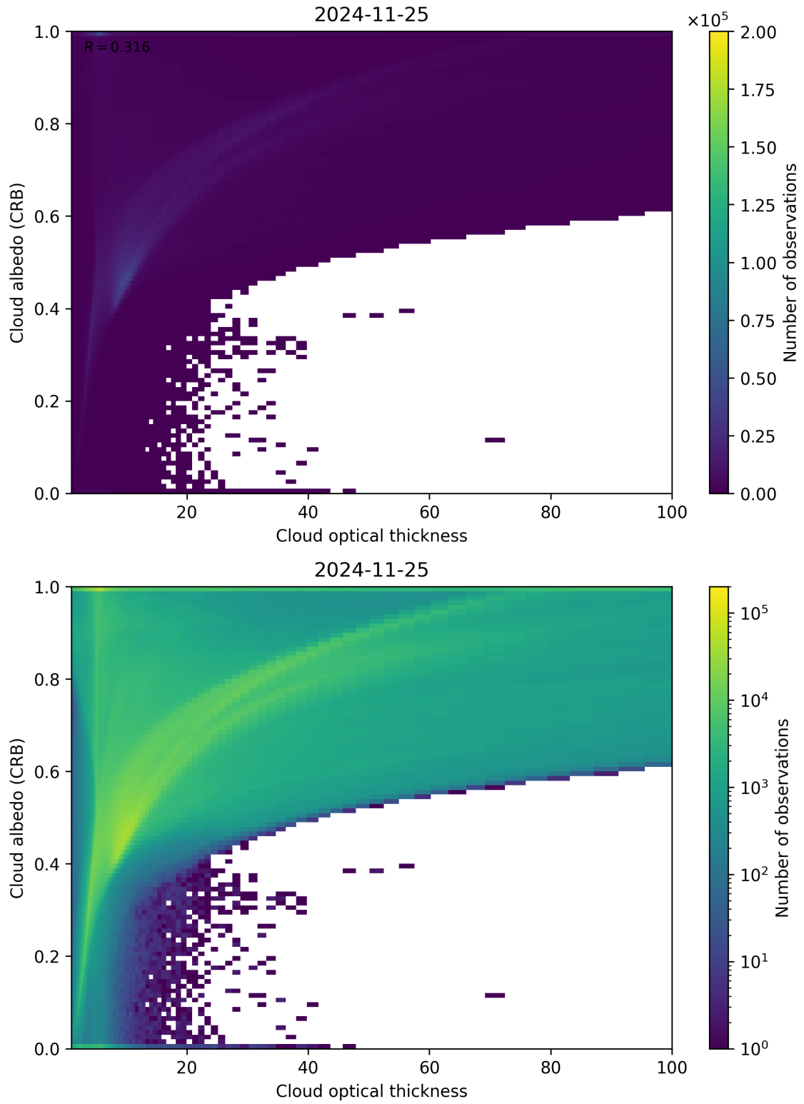
Figure 82: Scatter density plot of “Cloud optical thickness” against “Cloud albedo (CRB)” for 2024-11-25 to 2024-11-26.
