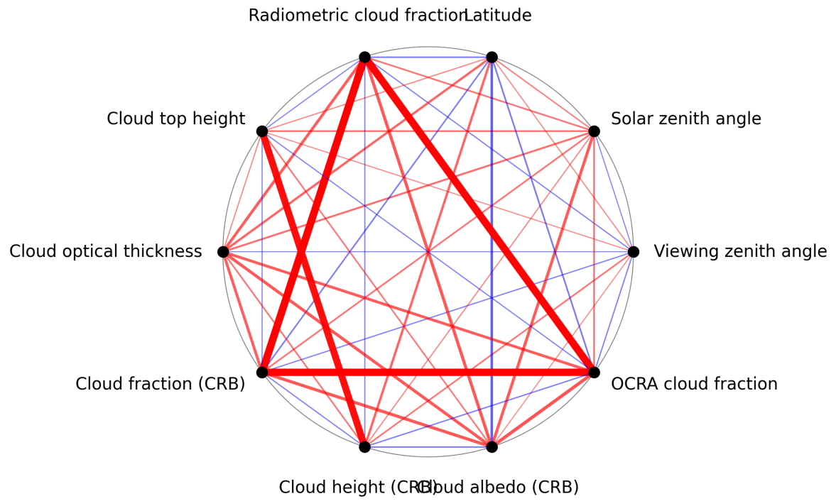
Figure 1: Map of correlation graph for 2024-11-25 to 2024-11-26.
