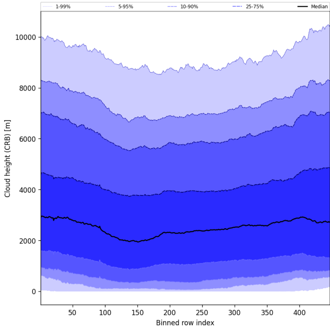
Figure 59: Along track statistics of “Cloud height (CRB)” for 2024-11-25 to 2024-11-26
