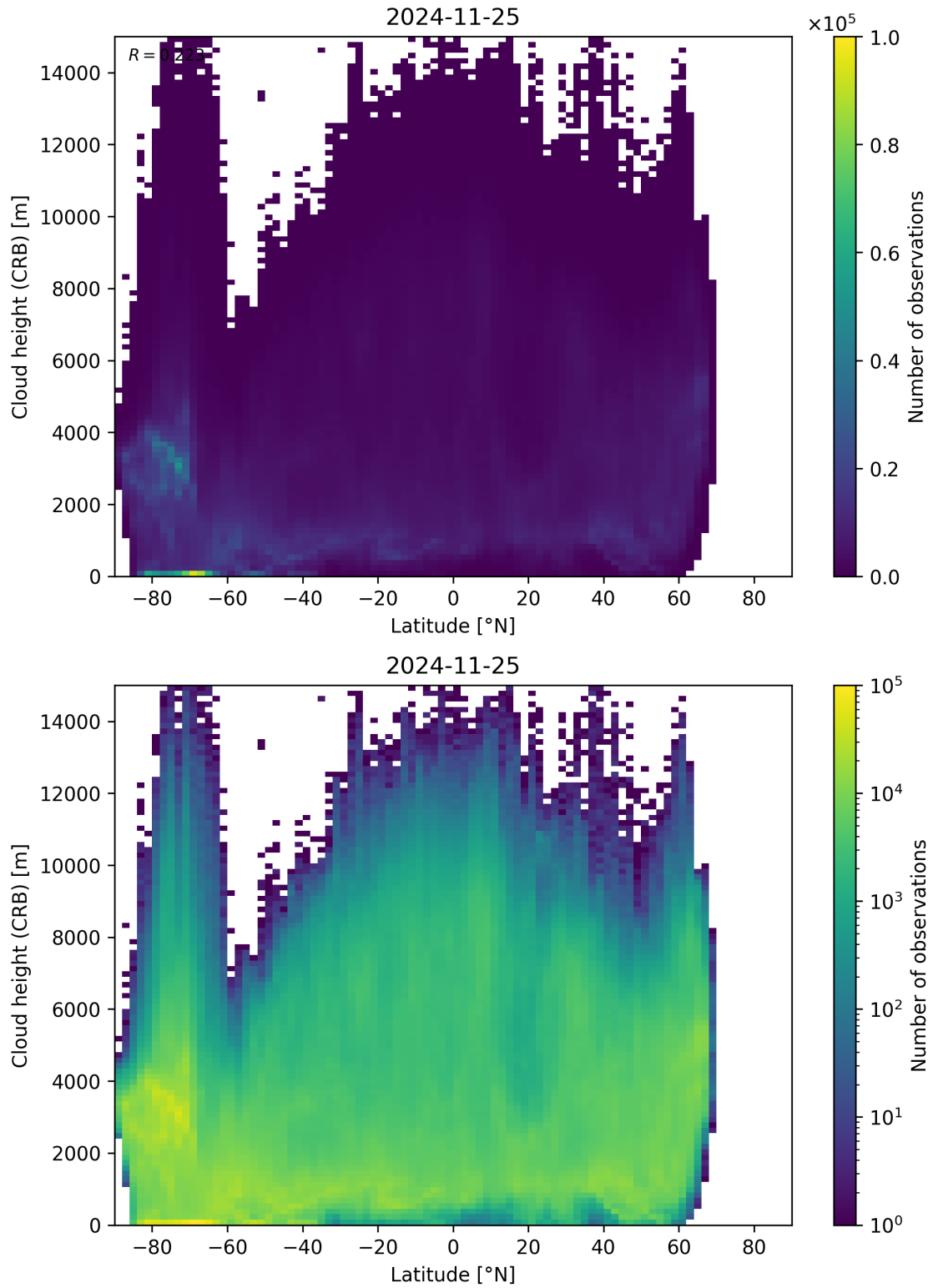
Figure 95: Scatter density plot of “Latitude” against “Cloud height (CRB)” for 2024-11-25 to 2024-11-26.
