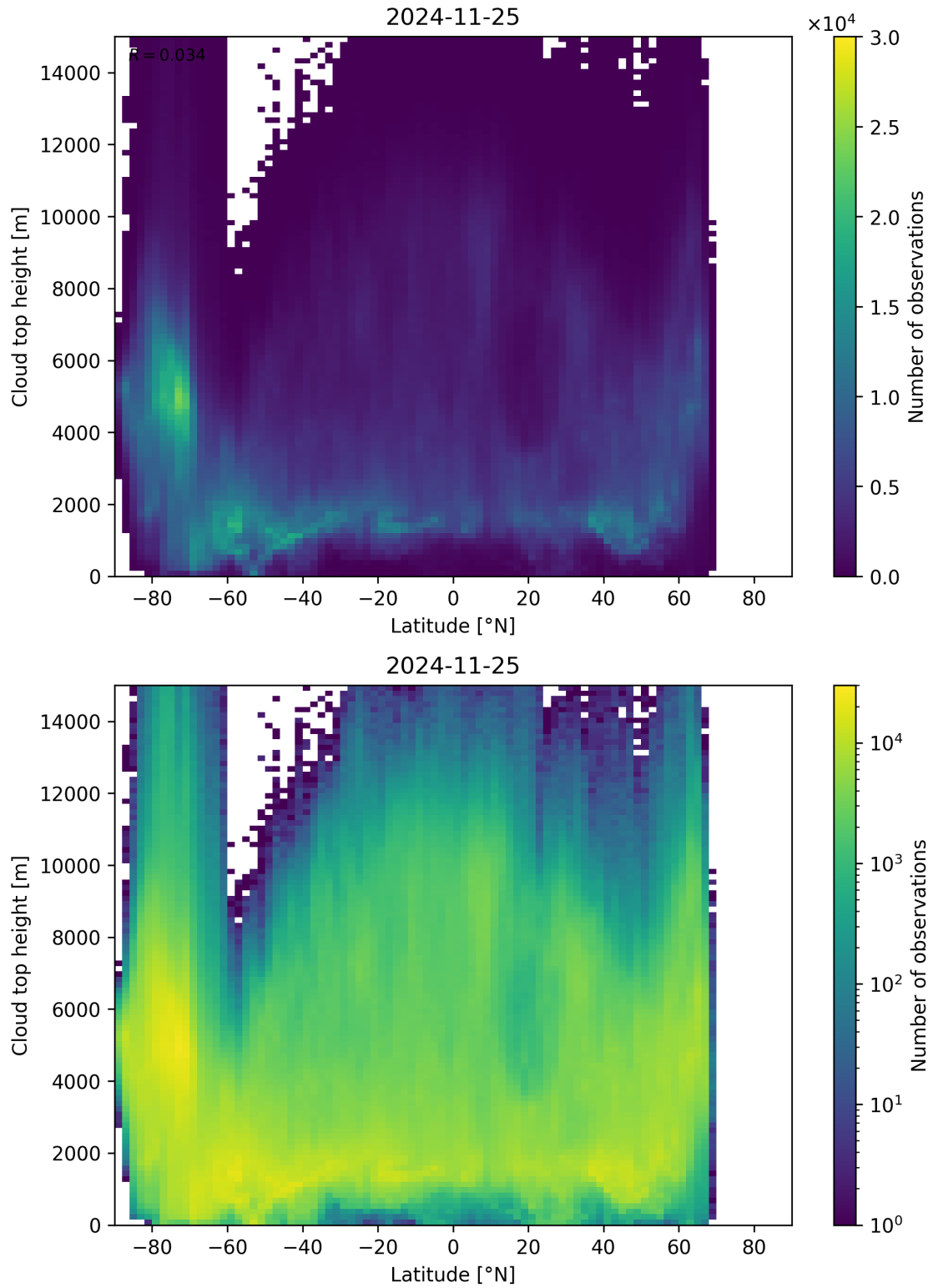
Figure 97: Scatter density plot of “Latitude” against “Cloud top height” for 2024-11-25 to 2024-11-26.
