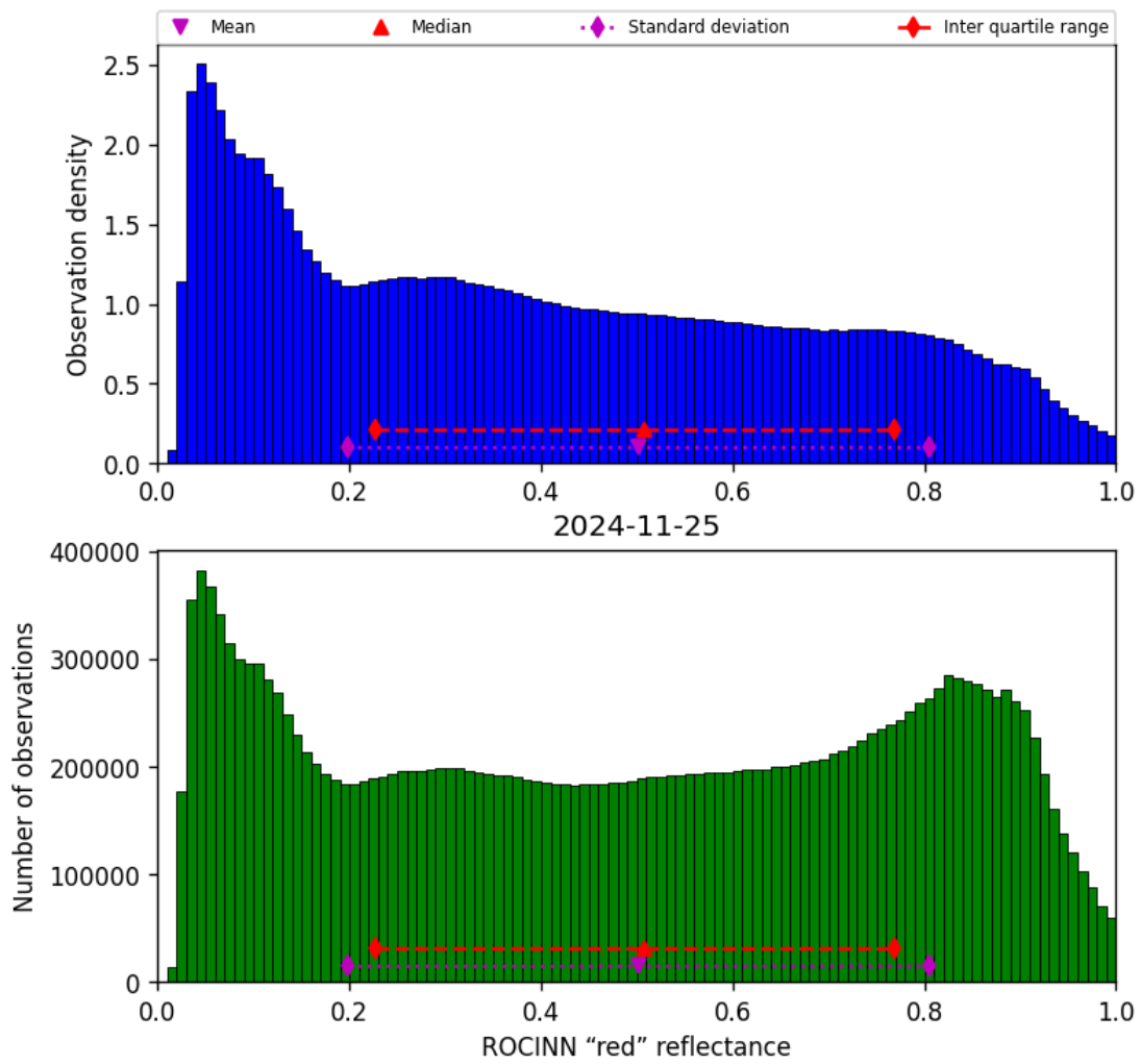
Figure 53: Histogram of “ROCINN “red” reflectance” for 2024-11-25 to 2024-11-26
