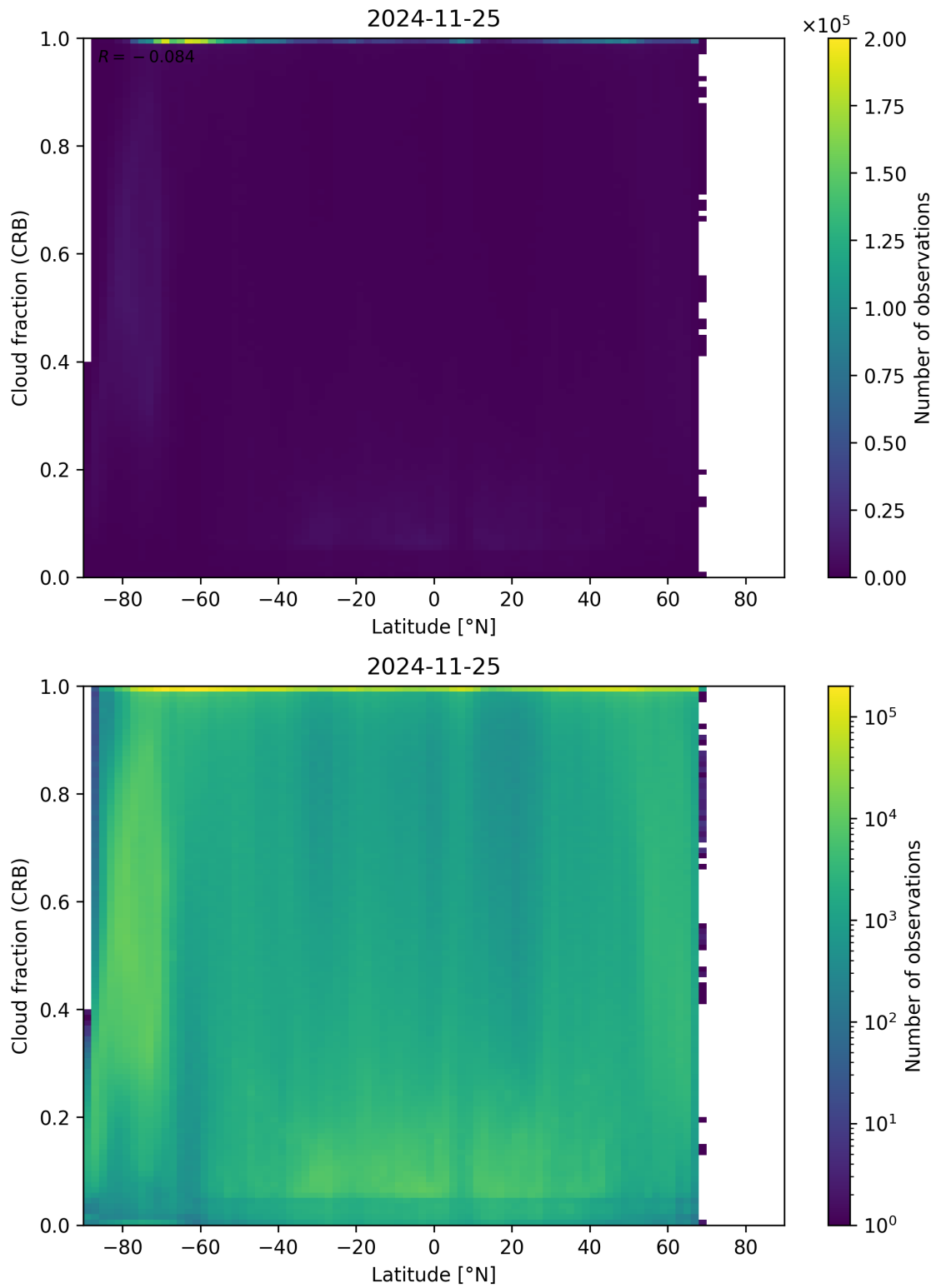
Figure 94: Scatter density plot of “Latitude” against “Cloud fraction (CRB)” for 2024-11-25 to 2024-11-26.
