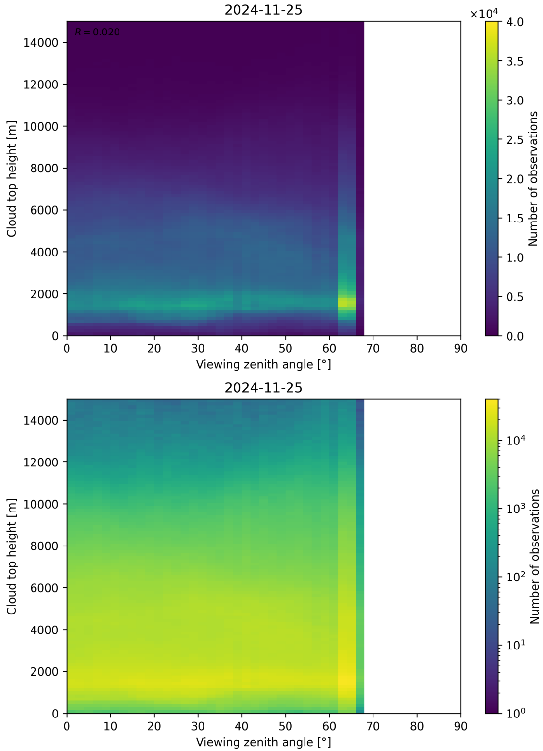
Figure 112: Scatter density plot of “Viewing zenith angle” against “Cloud top height” for 2024-11-25 to 2024-11-26.
