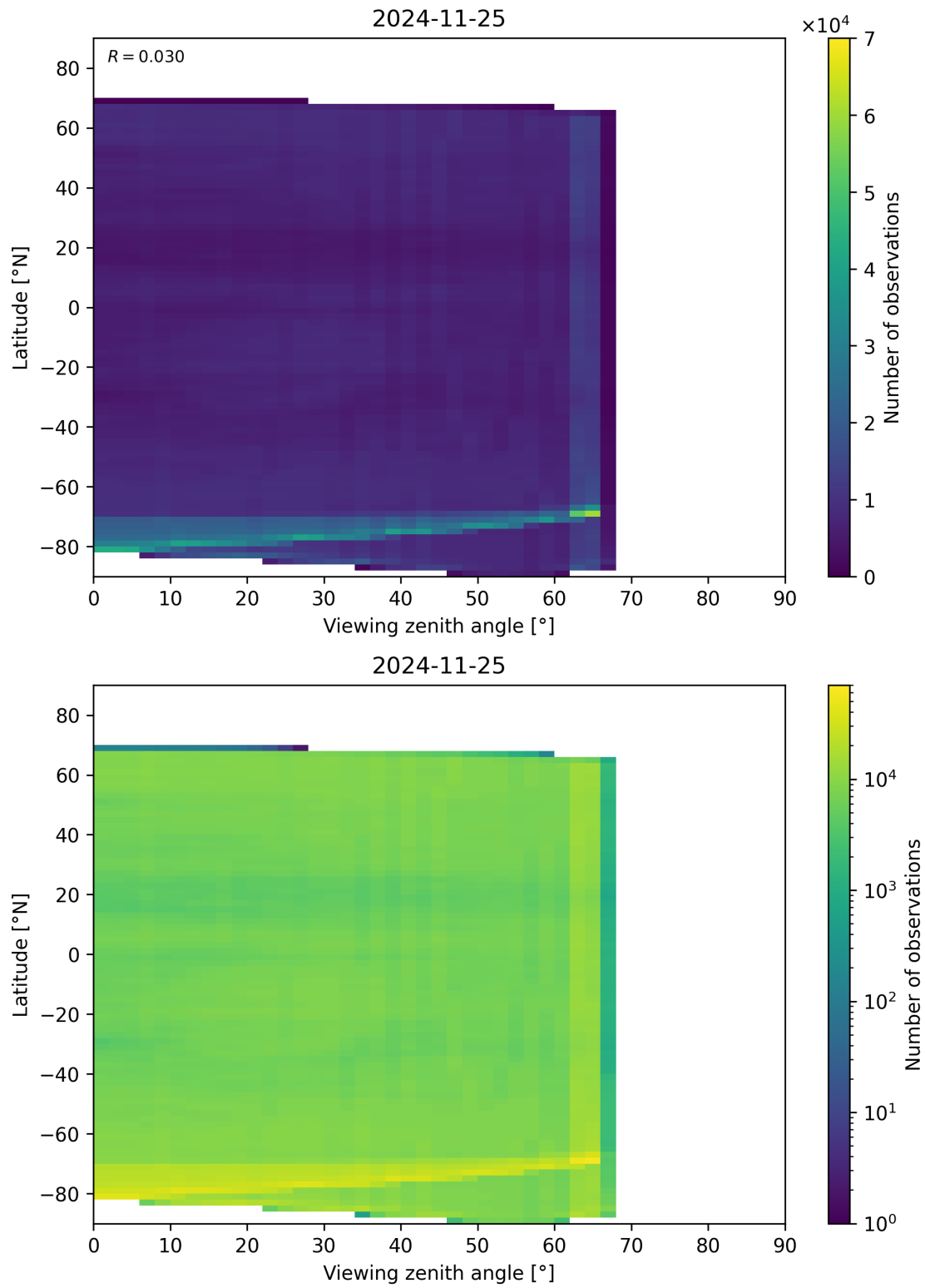
Figure 113: Scatter density plot of “Viewing zenith angle” against “Latitude” for 2024-11-25 to 2024-11-26.
