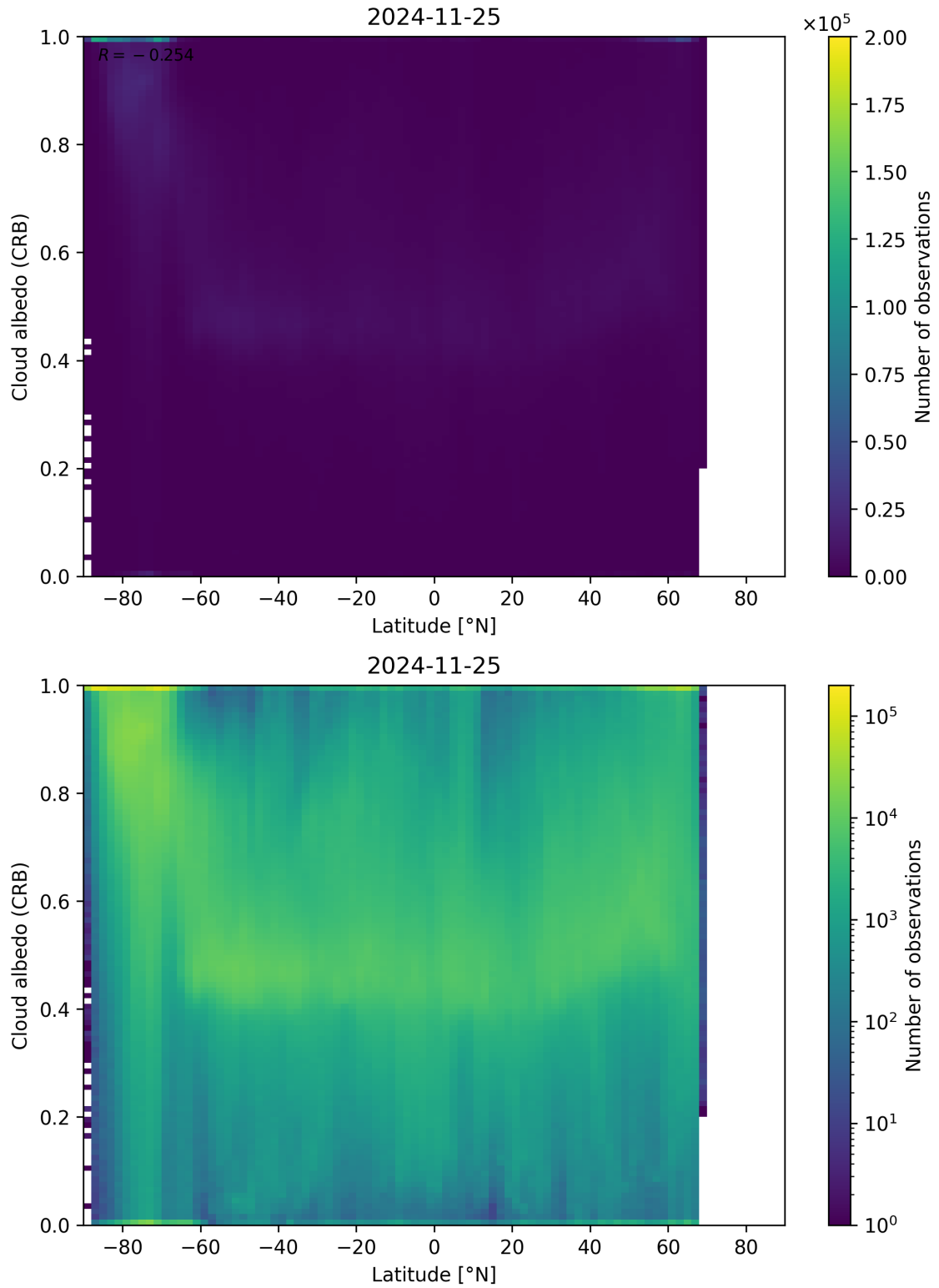
Figure 91: Scatter density plot of “Latitude” against “Cloud albedo (CRB)” for 2024-11-25 to 2024-11-26.
