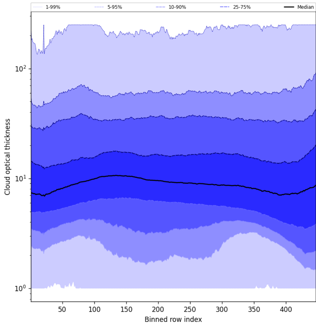
Figure 57: Along track statistics of “Cloud optical thickness” for 2024-11-25 to 2024-11-26
