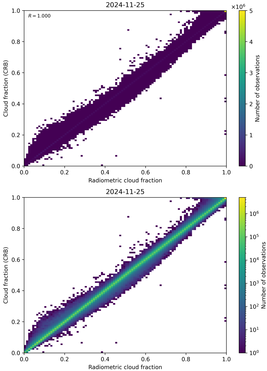
Figure 73: Scatter density plot of “Radiometric cloud fraction” against “Cloud fraction (CRB)” for 2024-11-25 to 2024-11-26.
