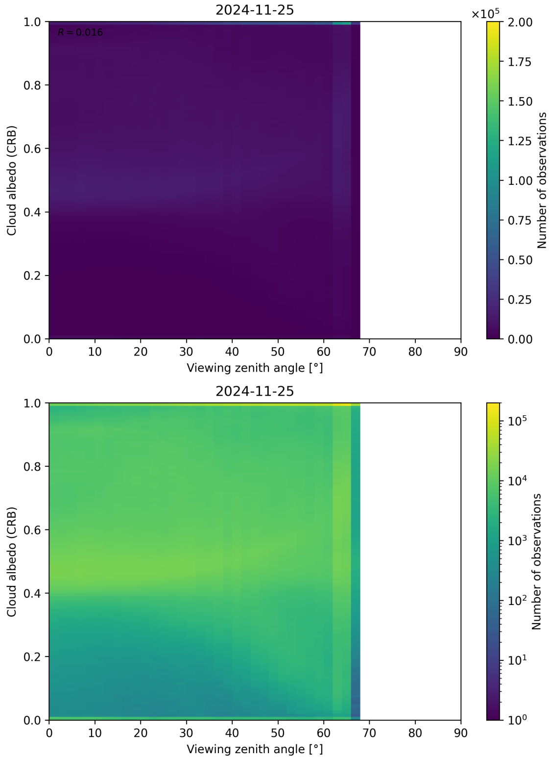
Figure 106: Scatter density plot of “Viewing zenith angle” against “Cloud albedo (CRB)” for 2024-11-25 to 2024-11-26.
