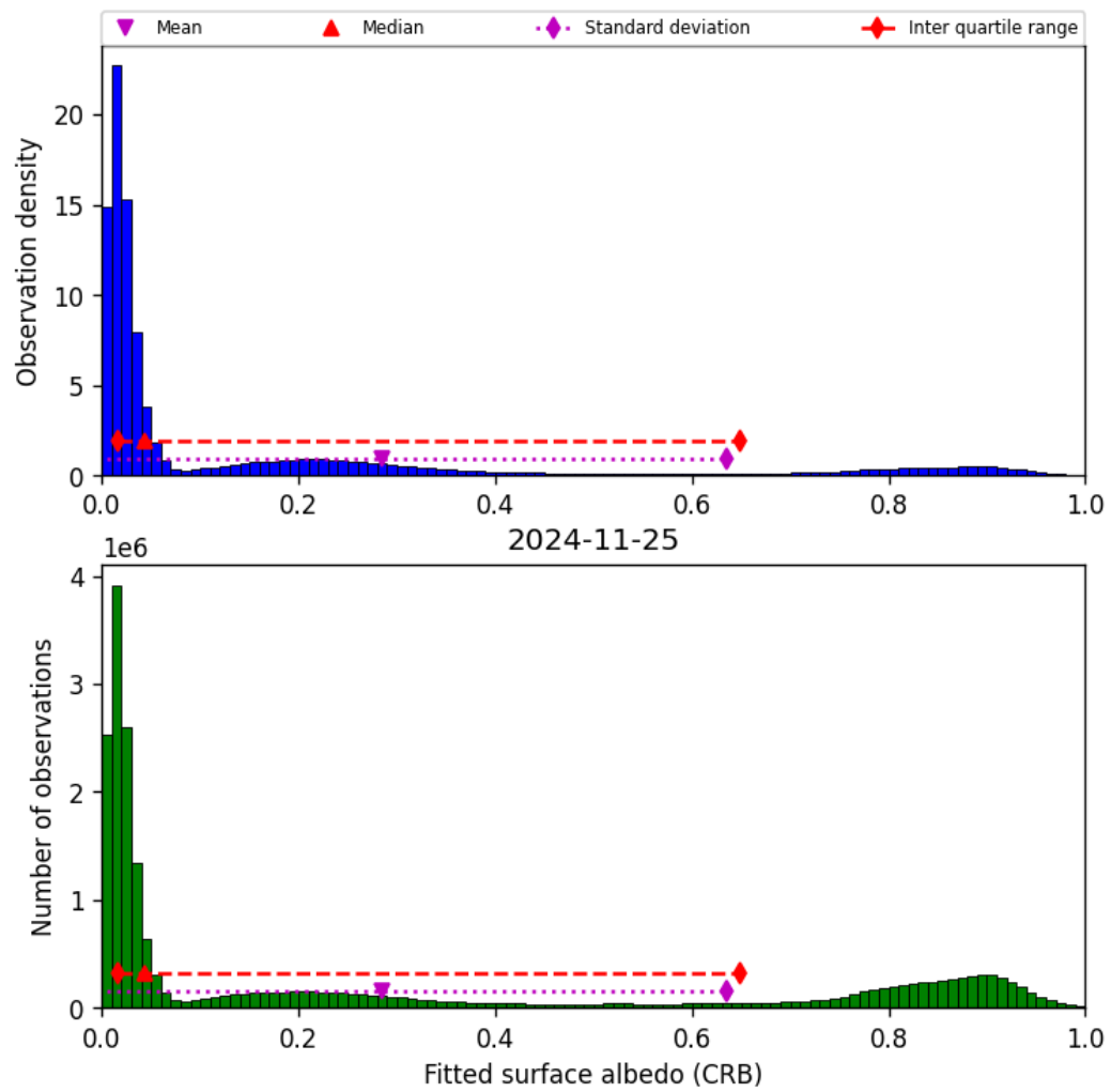
Figure 46: Histogram of “Fitted surface albedo (CRB)” for 2024-11-25 to 2024-11-26
