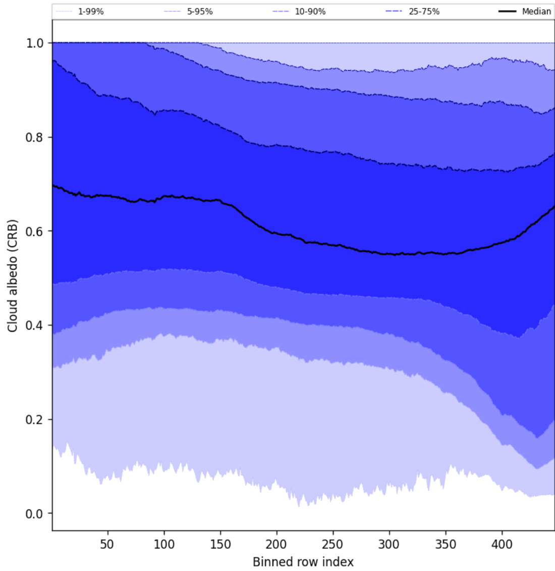
Figure 60: Along track statistics of “Cloud albedo (CRB)” for 2024-11-25 to 2024-11-27
