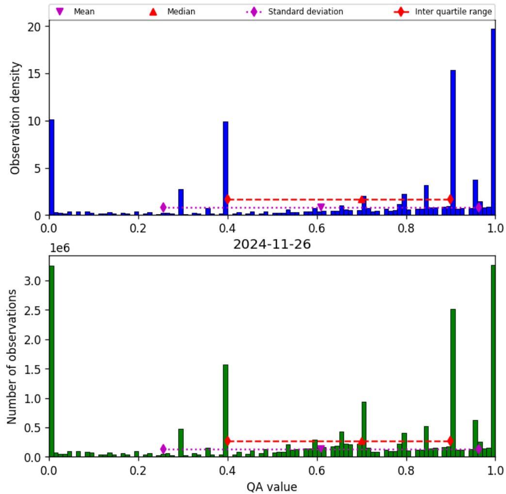
Figure 38: Histogram of “QA value” for 2024-11-25 to 2024-11-27
