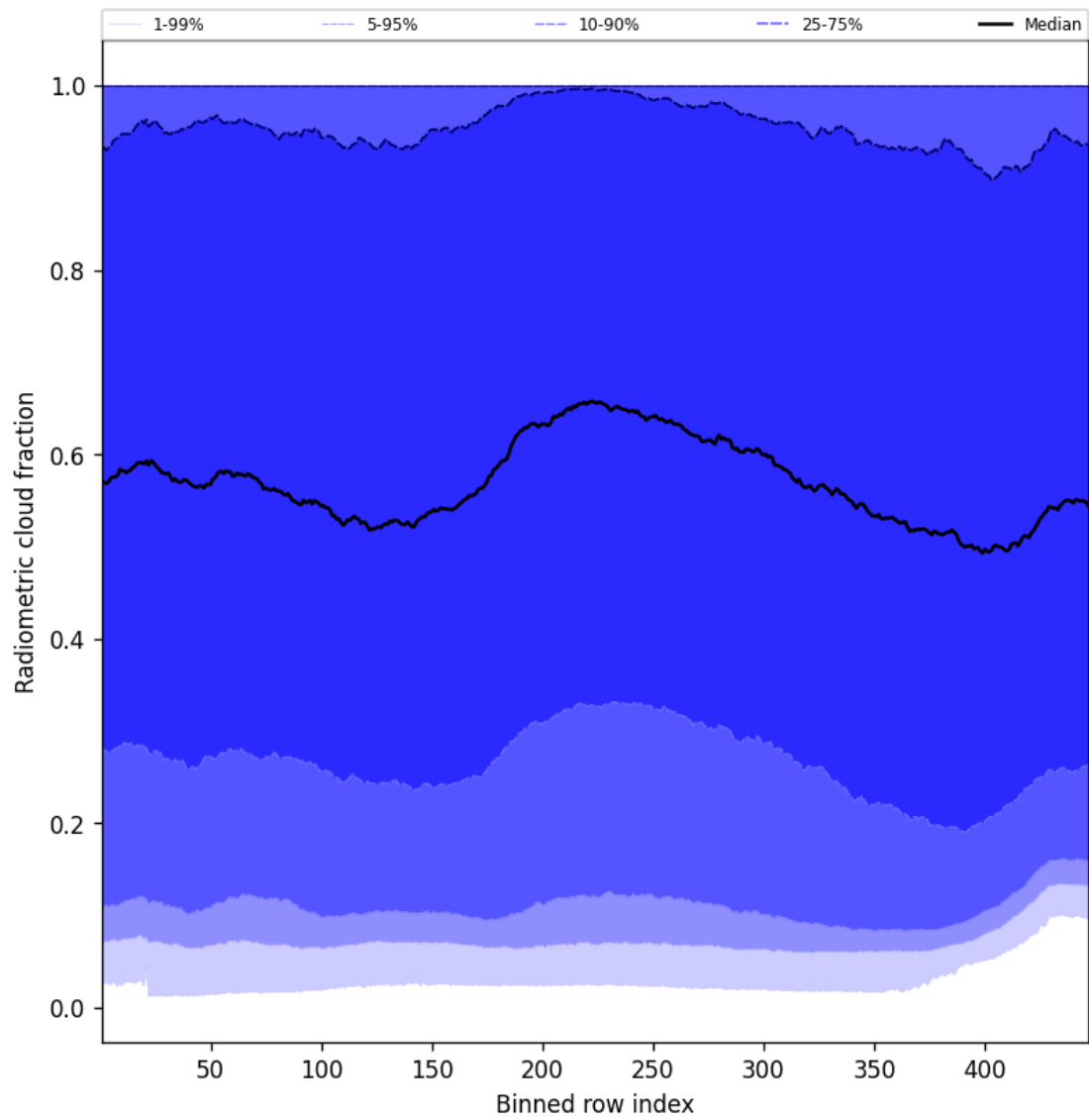
Figure 55: Along track statistics of “Radiometric cloud fraction” for 2024-11-25 to 2024-11-27
