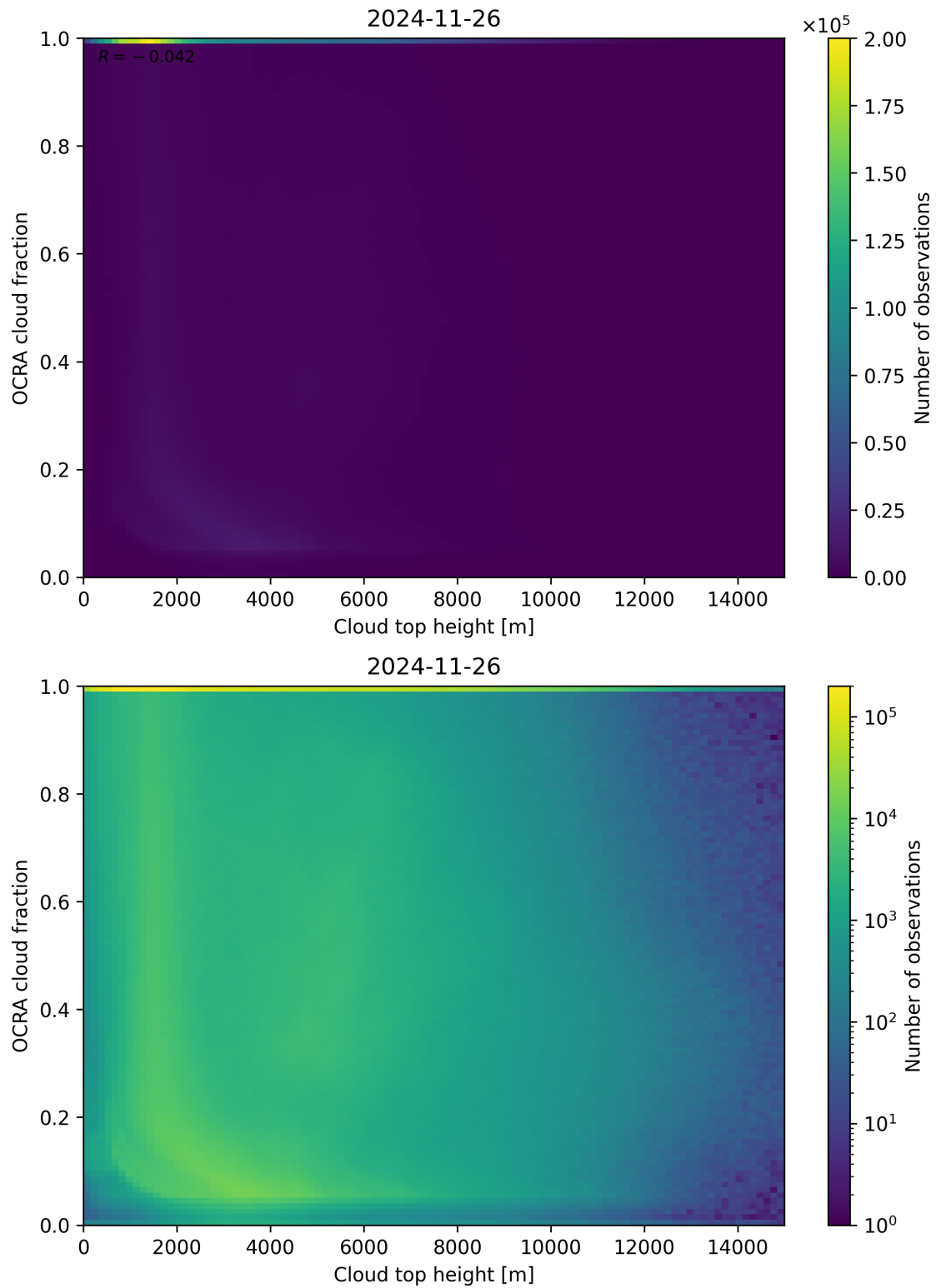
Figure 87: Scatter density plot of “Cloud top height” against “OCRA cloud fraction” for 2024-11-25 to 2024-11-27.
