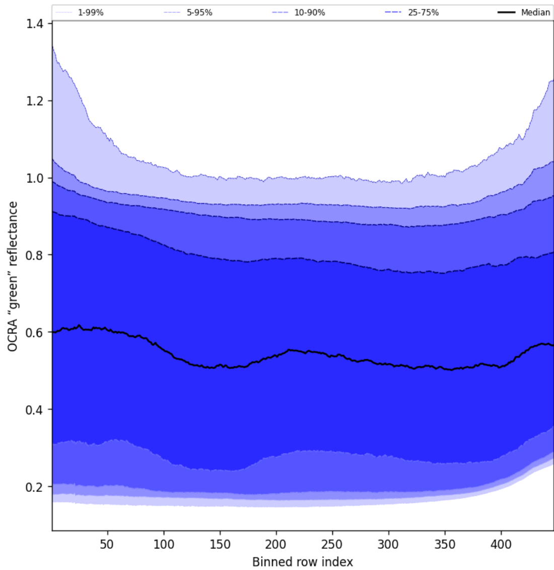
Figure 68: Along track statistics of “OCRA “green” reflectance” for 2024-11-25 to 2024-11-27
