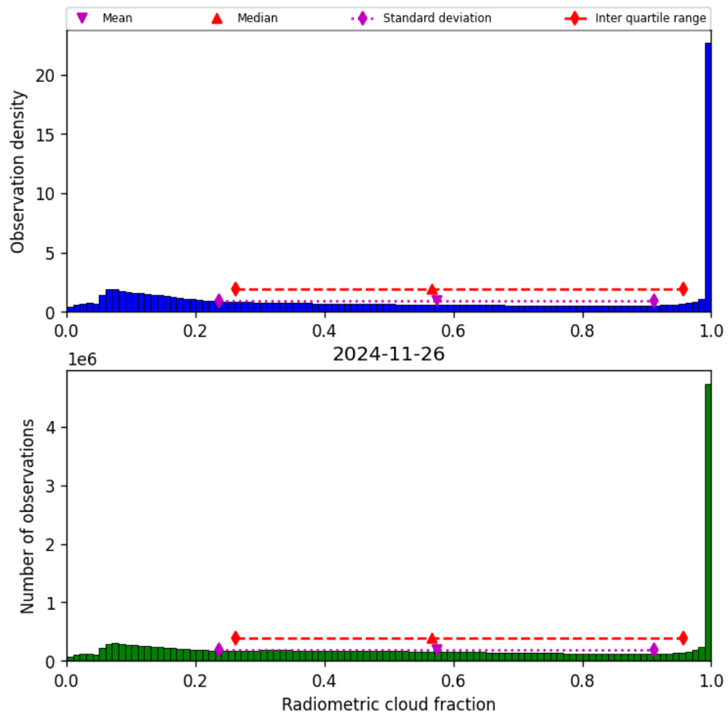
Figure 39: Histogram of “Radiometric cloud fraction” for 2024-11-25 to 2024-11-27
