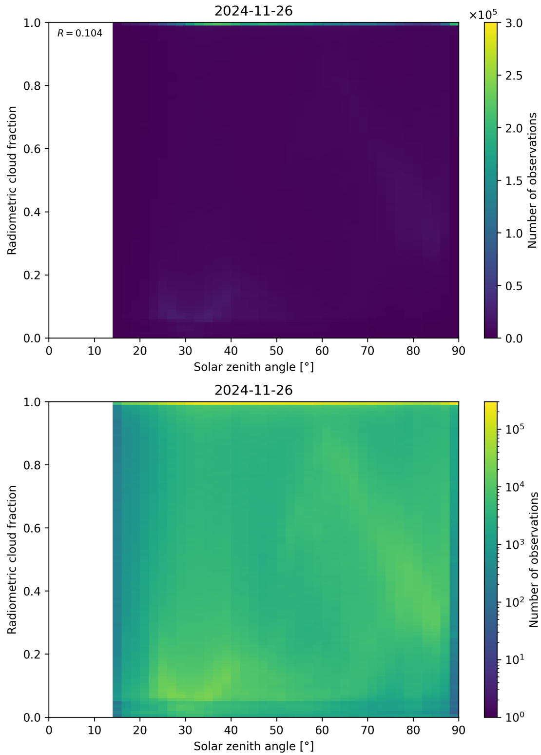
Figure 99: Scatter density plot of “Solar zenith angle” against “Radiometric cloud fraction” for 2024-11-25 to 2024-11-27.
