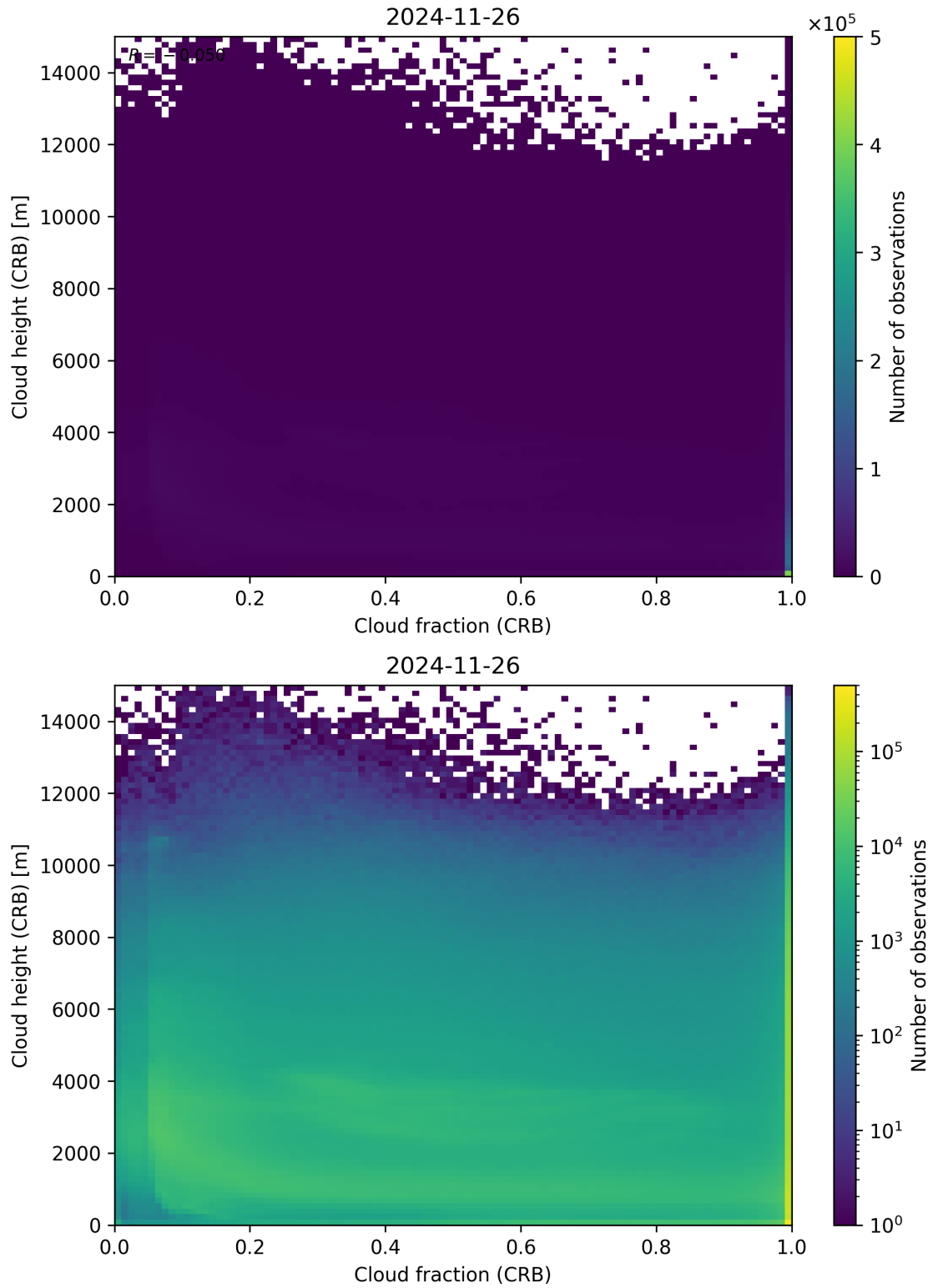
Figure 79: Scatter density plot of “Cloud fraction (CRB)” against “Cloud height (CRB)” for 2024-11-25 to 2024-11-27.
