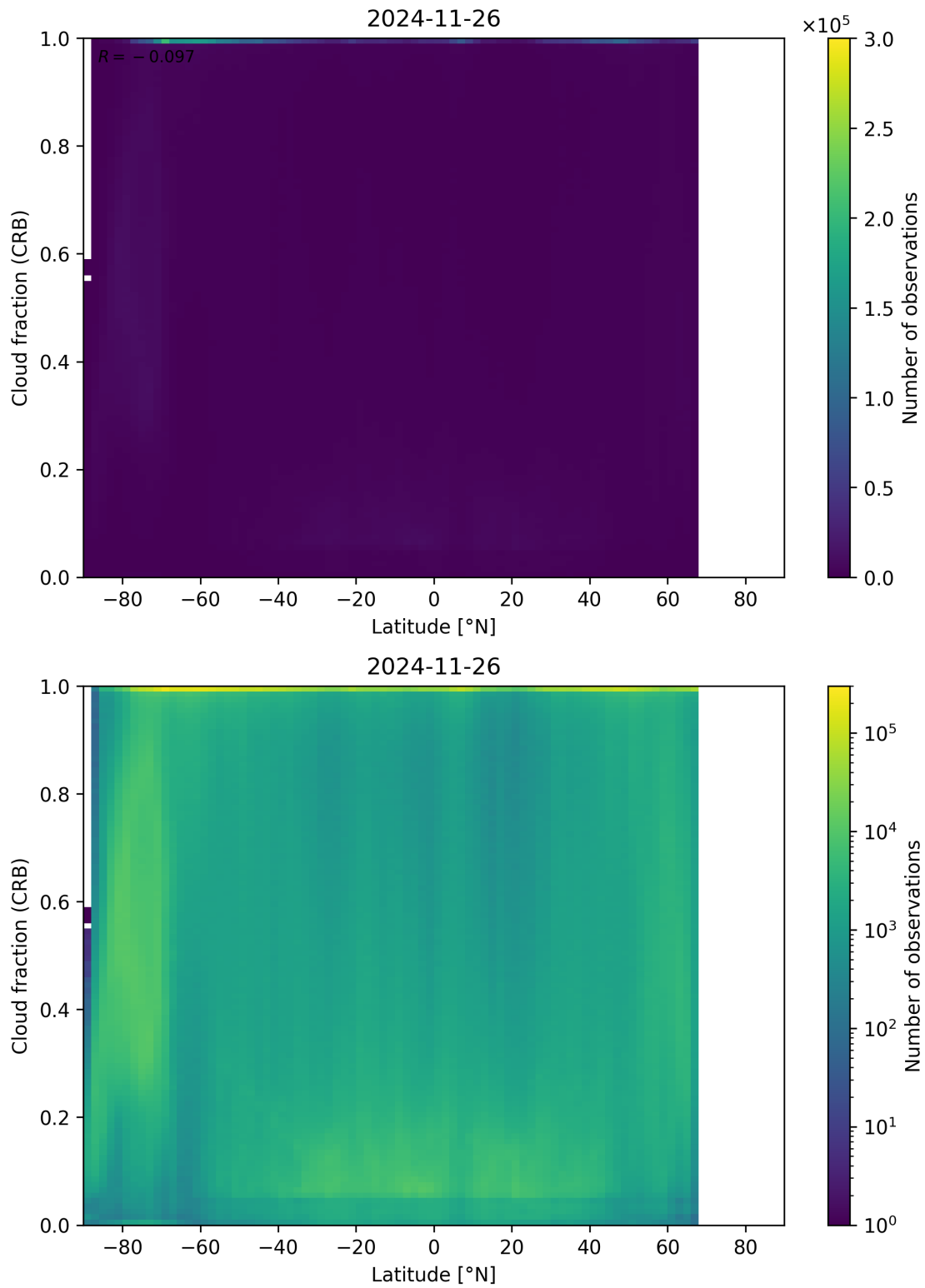
Figure 94: Scatter density plot of “Latitude” against “Cloud fraction (CRB)” for 2024-11-25 to 2024-11-27.
