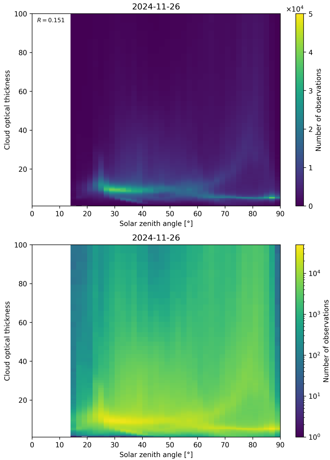
Figure 103: Scatter density plot of “Solar zenith angle” against “Cloud optical thickness” for 2024-11-25 to 2024-11-27.
