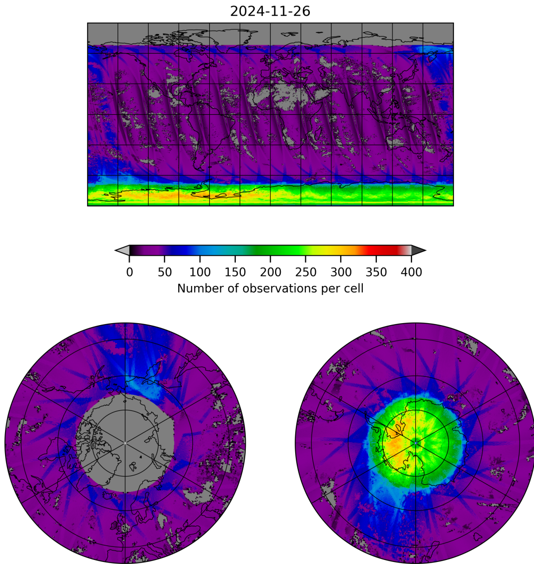
Figure 21: Map of the number of observations for 2024-11-25 to 2024-11-27
