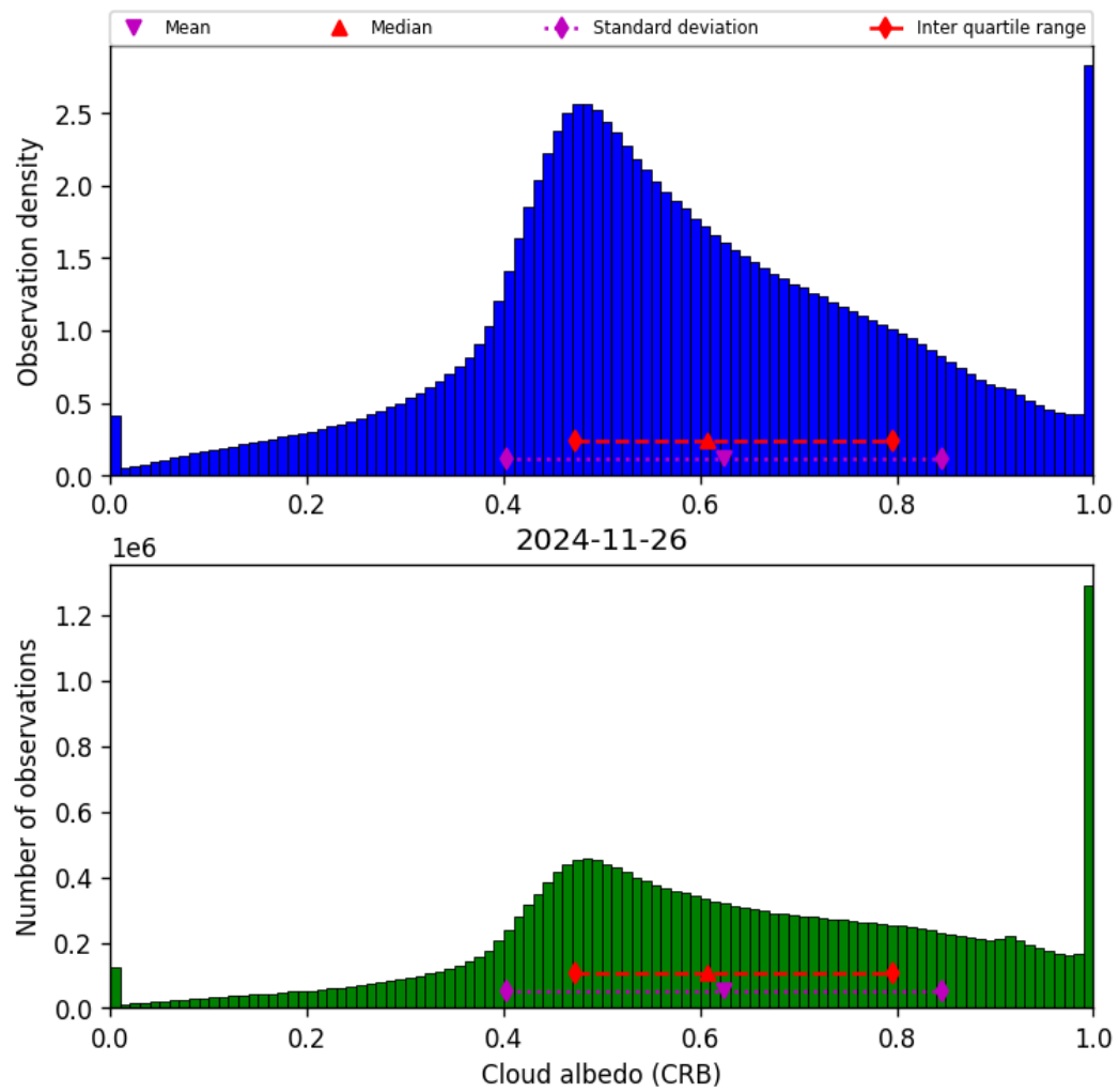
Figure 44: Histogram of “Cloud albedo (CRB)” for 2024-11-25 to 2024-11-27
