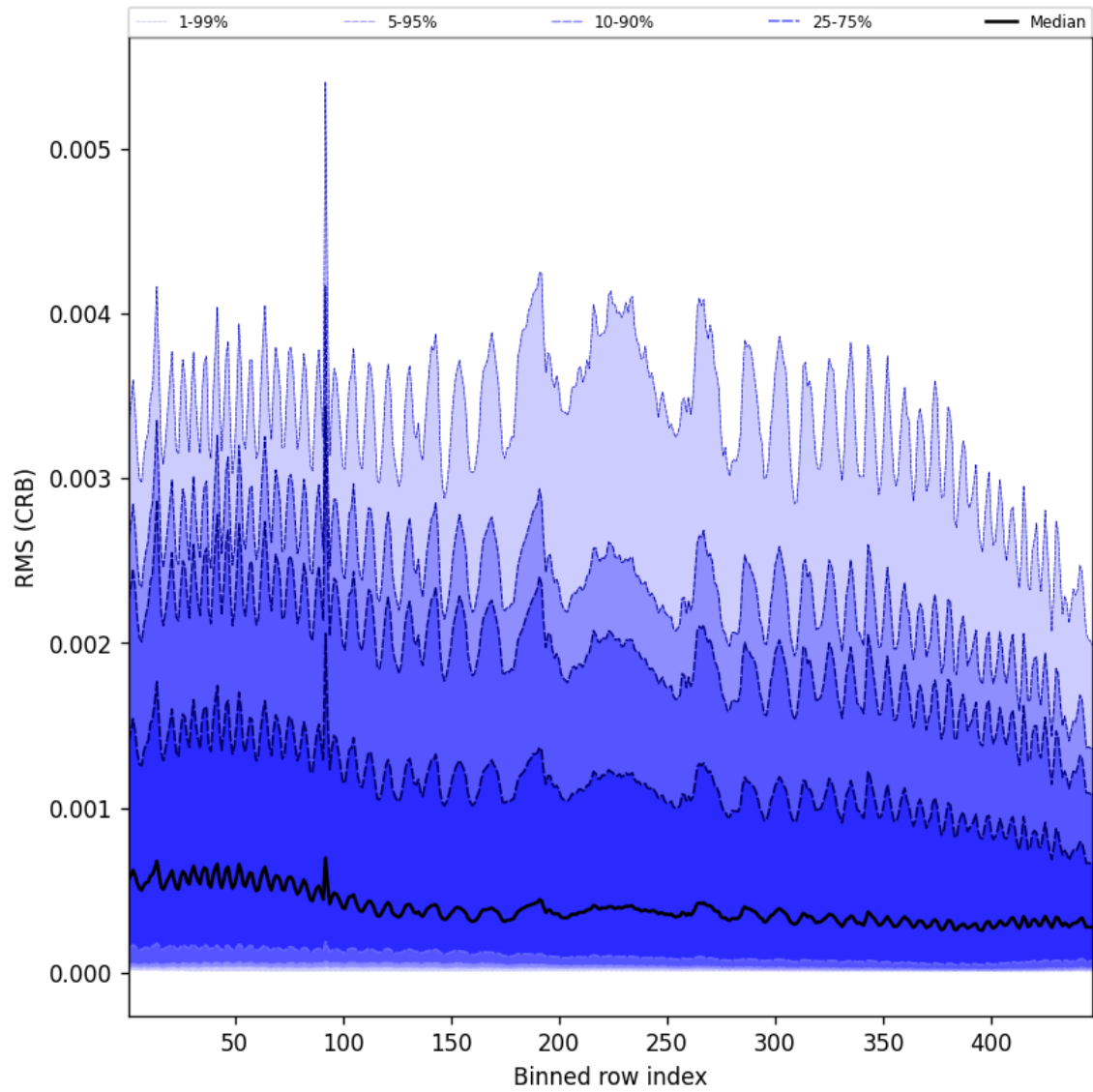
Figure 64: Along track statistics of “RMS (CRB)” for 2024-11-27 to 2024-11-29
