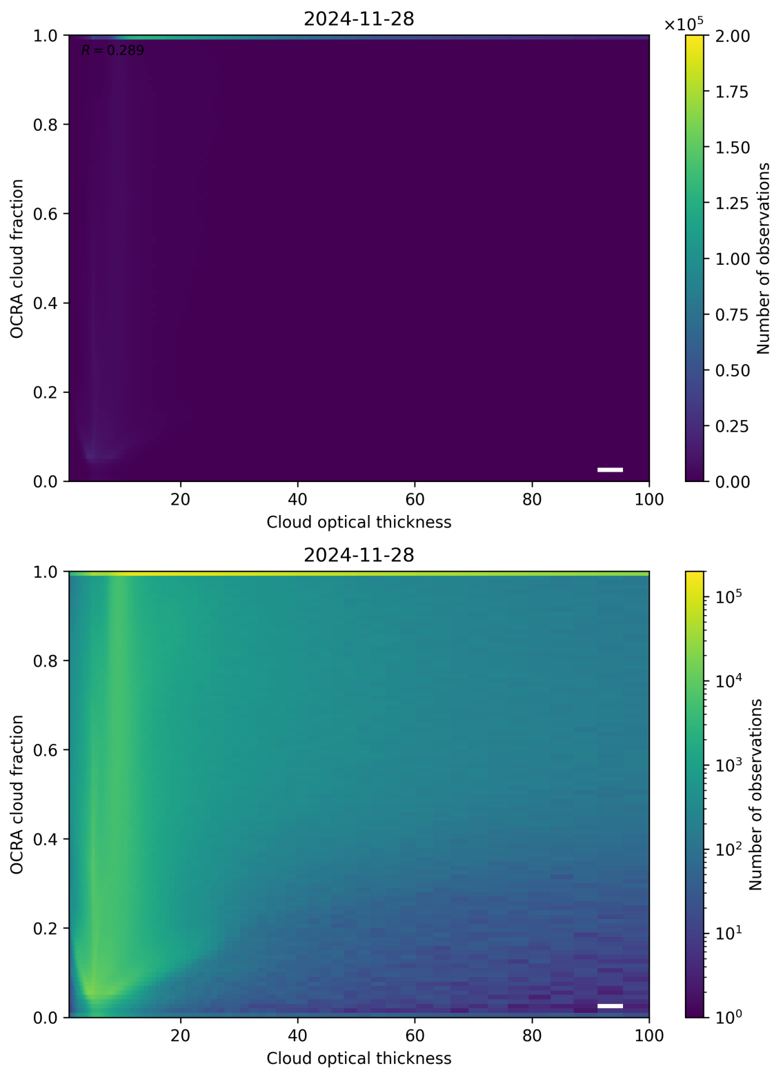
Figure 83: Scatter density plot of “Cloud optical thickness” against “OCRA cloud fraction” for 2024-11-27 to 2024-11-29.
