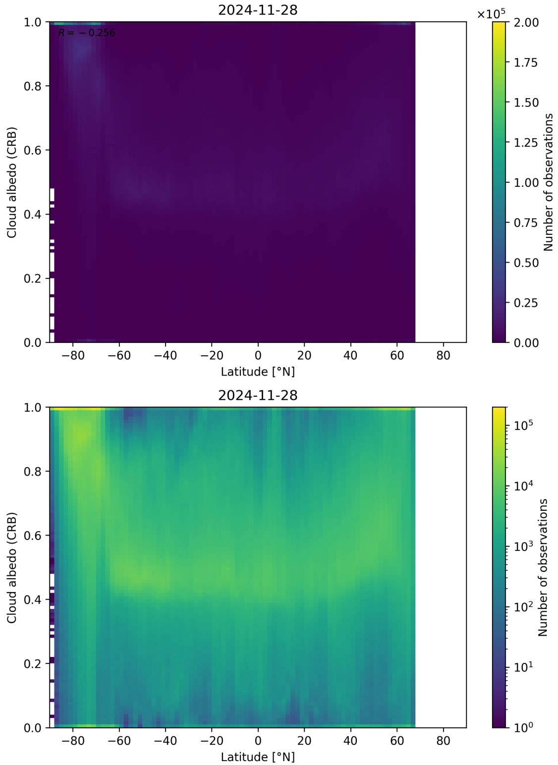
Figure 91: Scatter density plot of “Latitude” against “Cloud albedo (CRB)” for 2024-11-27 to 2024-11-29.
