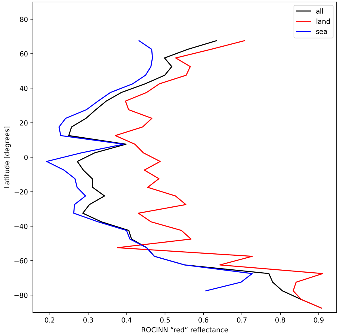
Figure 37: Zonal average of “ROCINN “red” reflectance” for 2024-11-27 to 2024-11-29.
