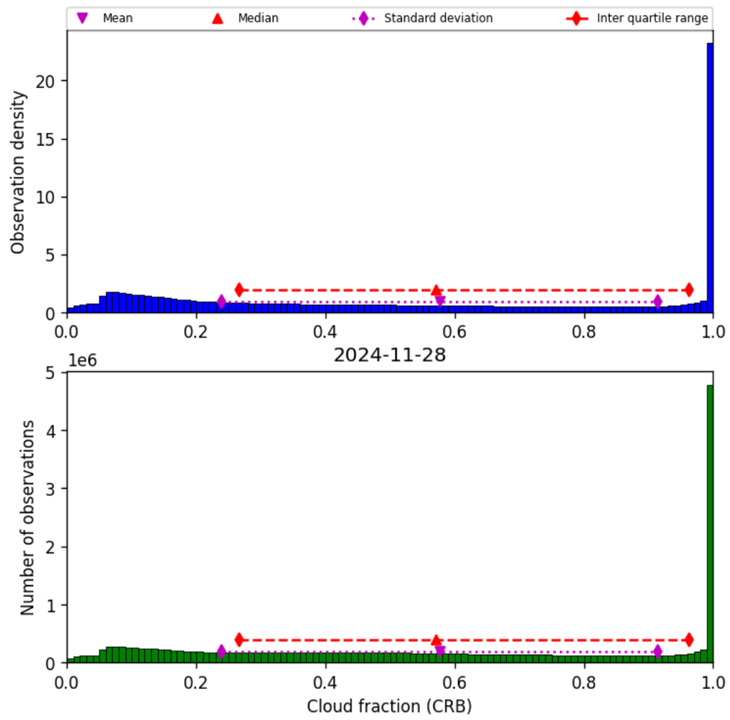
Figure 42: Histogram of “Cloud fraction (CRB)” for 2024-11-27 to 2024-11-29
