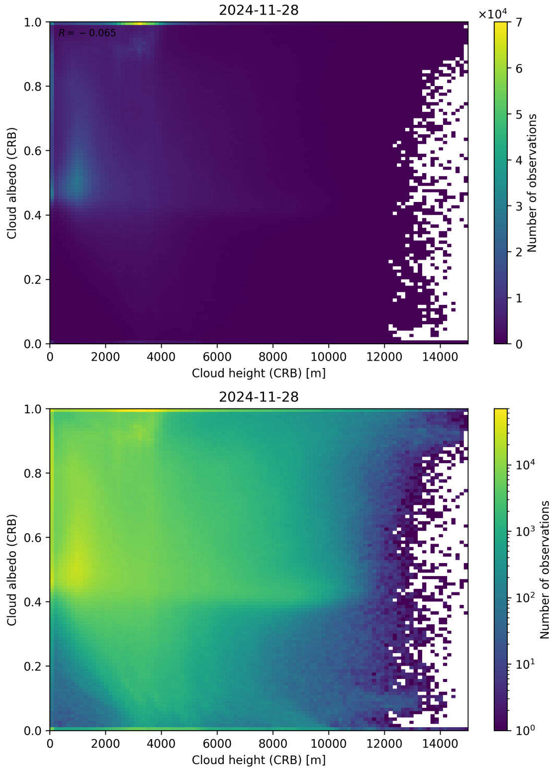
Figure 80: Scatter density plot of “Cloud height (CRB)” against “Cloud albedo (CRB)” for 2024-11-27 to 2024-11-29.
