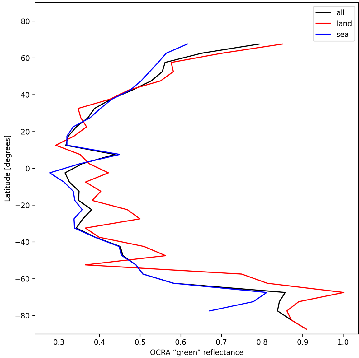
Figure 36: Zonal average of “OCRA “green” reflectance” for 2024-11-27 to 2024-11-29.
