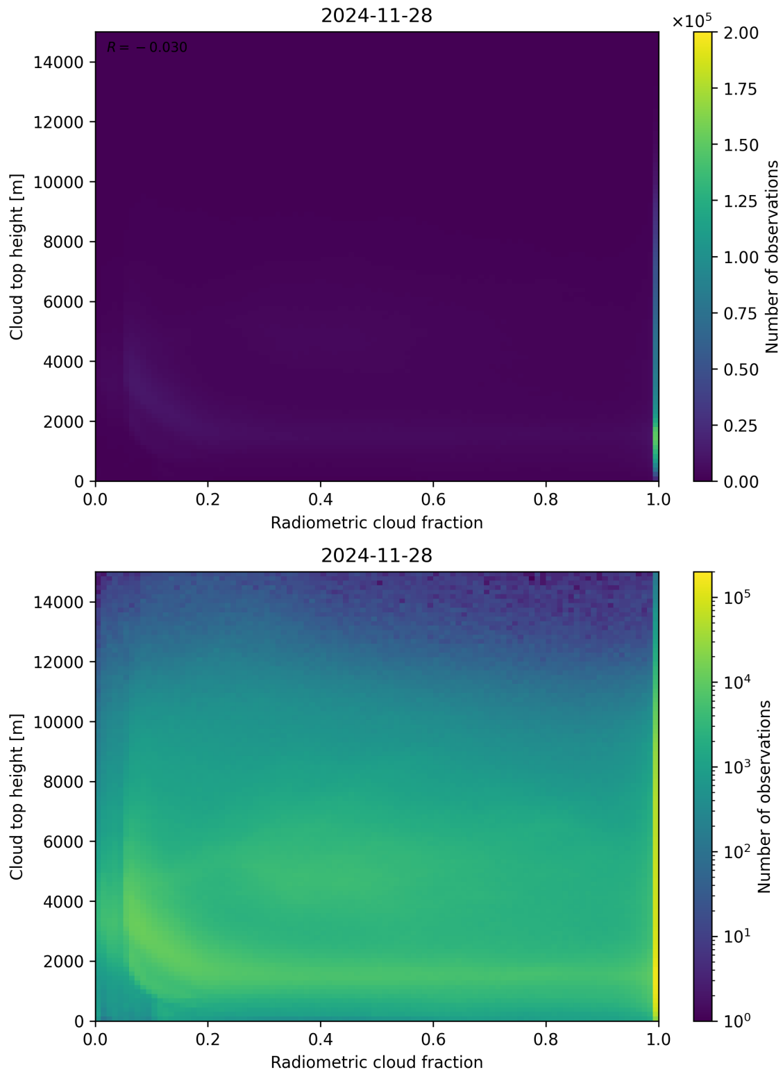
Figure 76: Scatter density plot of “Radiometric cloud fraction” against “Cloud top height” for 2024-11-27 to 2024-11-29.
