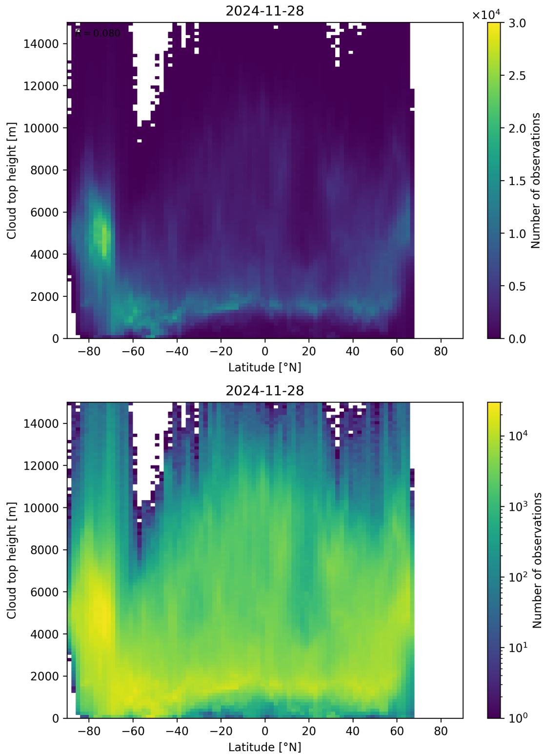
Figure 97: Scatter density plot of “Latitude” against “Cloud top height” for 2024-11-27 to 2024-11-29.
