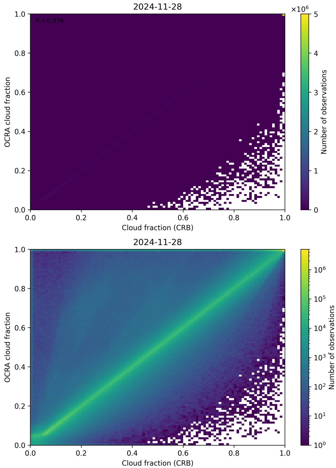
Figure 78: Scatter density plot of “Cloud fraction (CRB)” against “OCRA cloud fraction” for 2024-11-27 to 2024-11-29.
