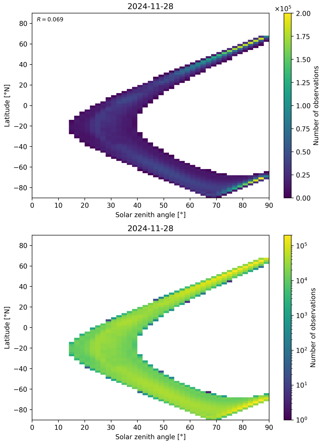
Figure 105: Scatter density plot of “Solar zenith angle” against “Latitude” for 2024-11-27 to 2024-11-29.
