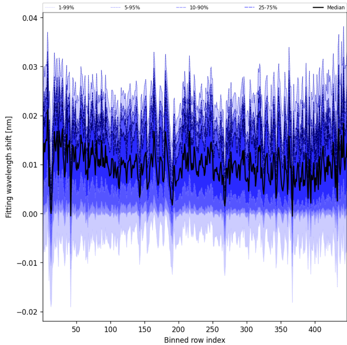
Figure 65: Along track statistics of “Fitting wavelength shift” for 2024-11-27 to 2024-11-29
