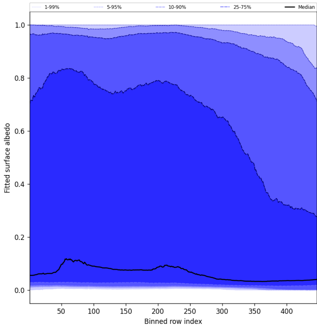
Figure 61: Along track statistics of “Fitted surface albedo” for 2024-11-27 to 2024-11-29
