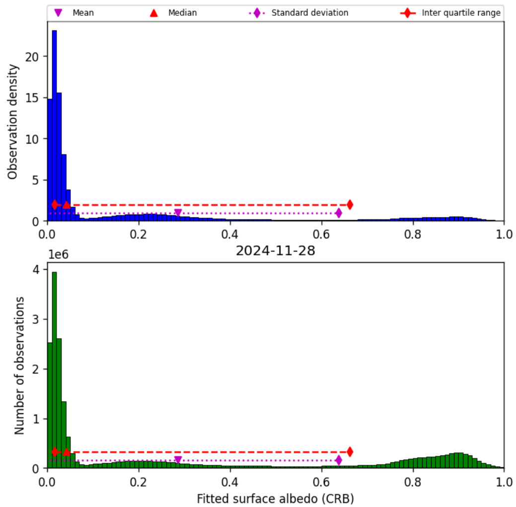
Figure 46: Histogram of “Fitted surface albedo (CRB)” for 2024-11-27 to 2024-11-29
