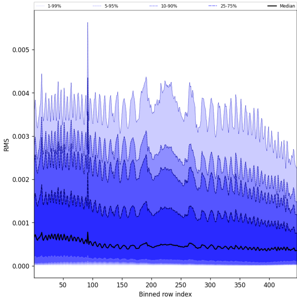
Figure 63: Along track statistics of “RMS” for 2024-11-27 to 2024-11-29
