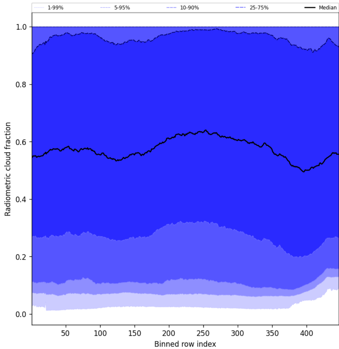
Figure 55: Along track statistics of “Radiometric cloud fraction” for 2024-11-27 to 2024-11-29
