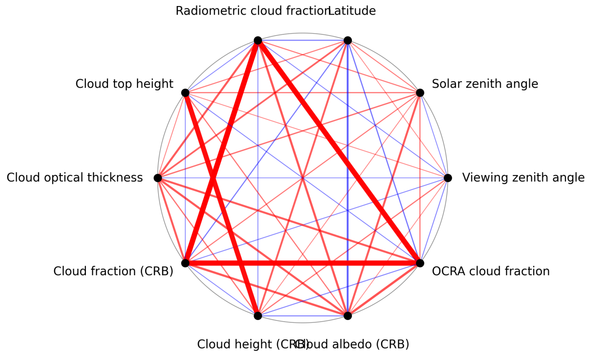
Figure 1: Map of correlation graph for 2024-11-27 to 2024-11-29.
