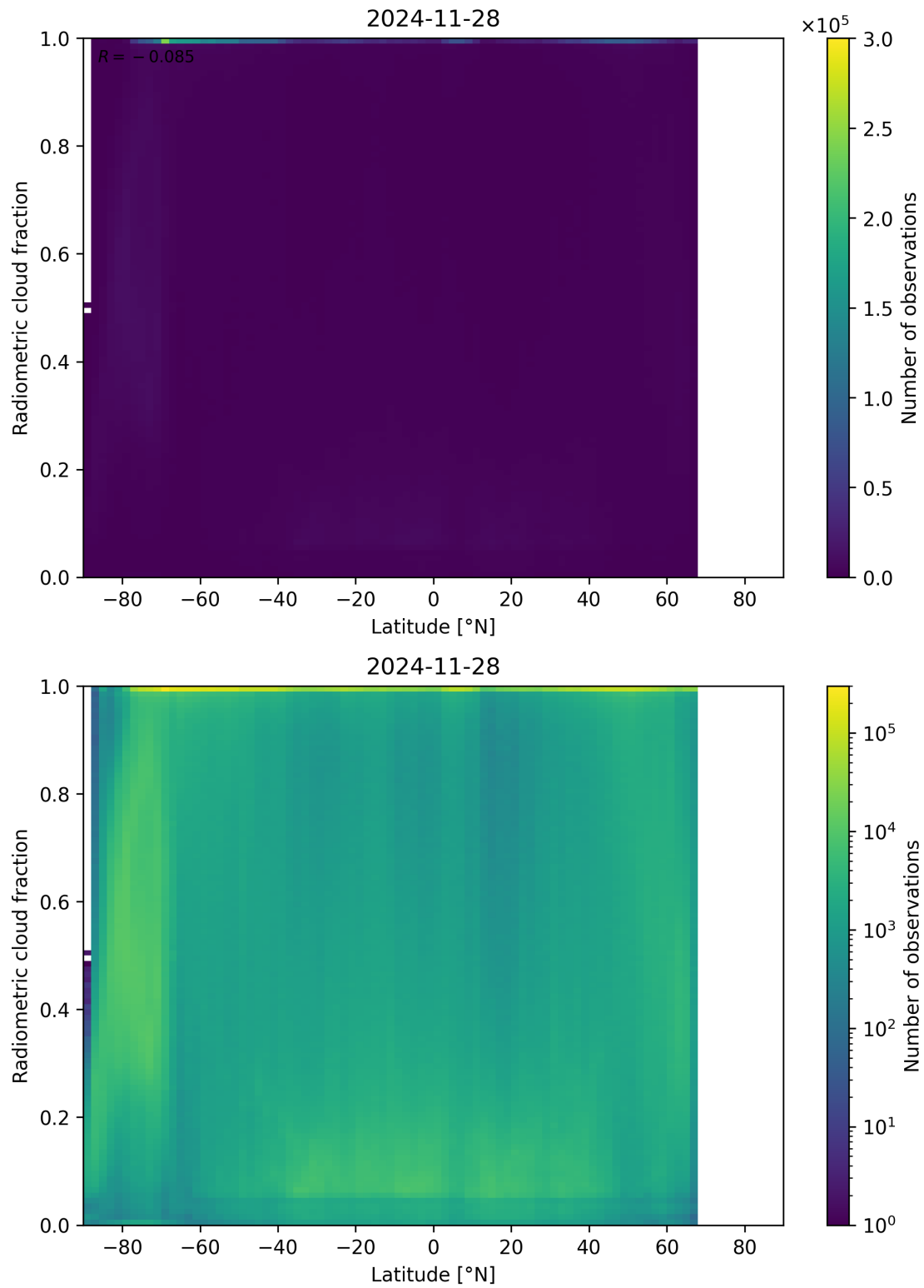
Figure 92: Scatter density plot of “Latitude” against “Radiometric cloud fraction” for 2024-11-27 to 2024-11-29.
