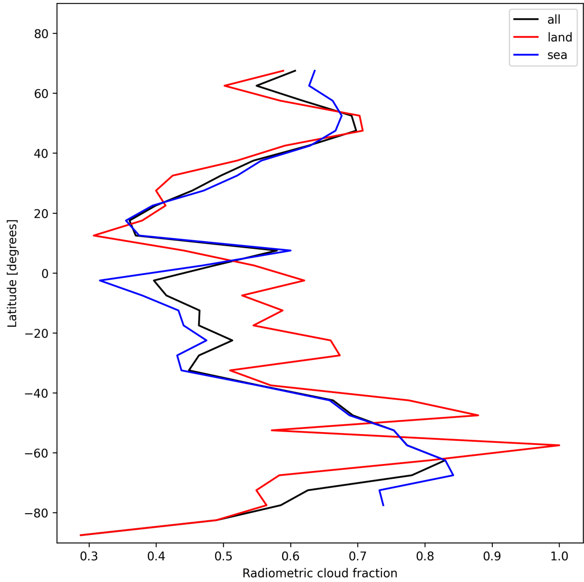
Figure 23: Zonal average of “Radiometric cloud fraction” for 2024-11-27 to 2024-11-29.
