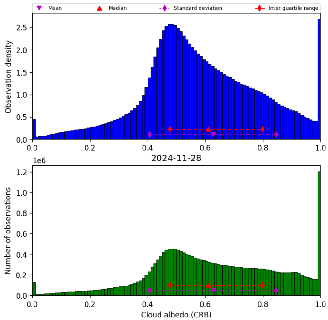
Figure 44: Histogram of “Cloud albedo (CRB)” for 2024-11-27 to 2024-11-29
