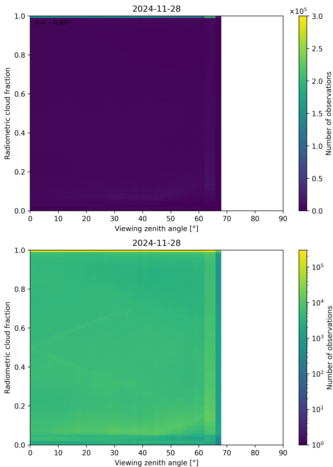
Figure 107: Scatter density plot of “Viewing zenith angle” against “Radiometric cloud fraction” for 2024-11-27 to 2024-11-29.
