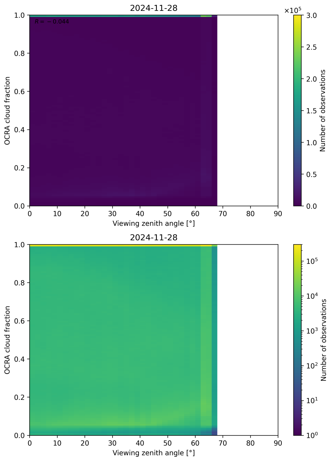
Figure 108: Scatter density plot of “Viewing zenith angle” against “OCRA cloud fraction” for 2024-11-27 to 2024-11-29.
