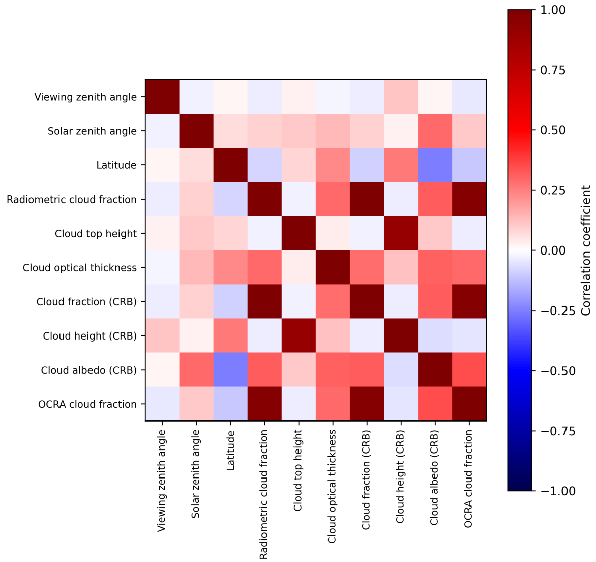
Figure 2: Map of correlation matrix for 2024-11-27 to 2024-11-29.
