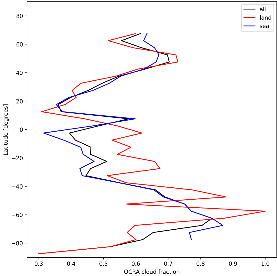
Figure 34: Zonal average of “OCRA cloud fraction” for 2024-11-27 to 2024-11-29.
