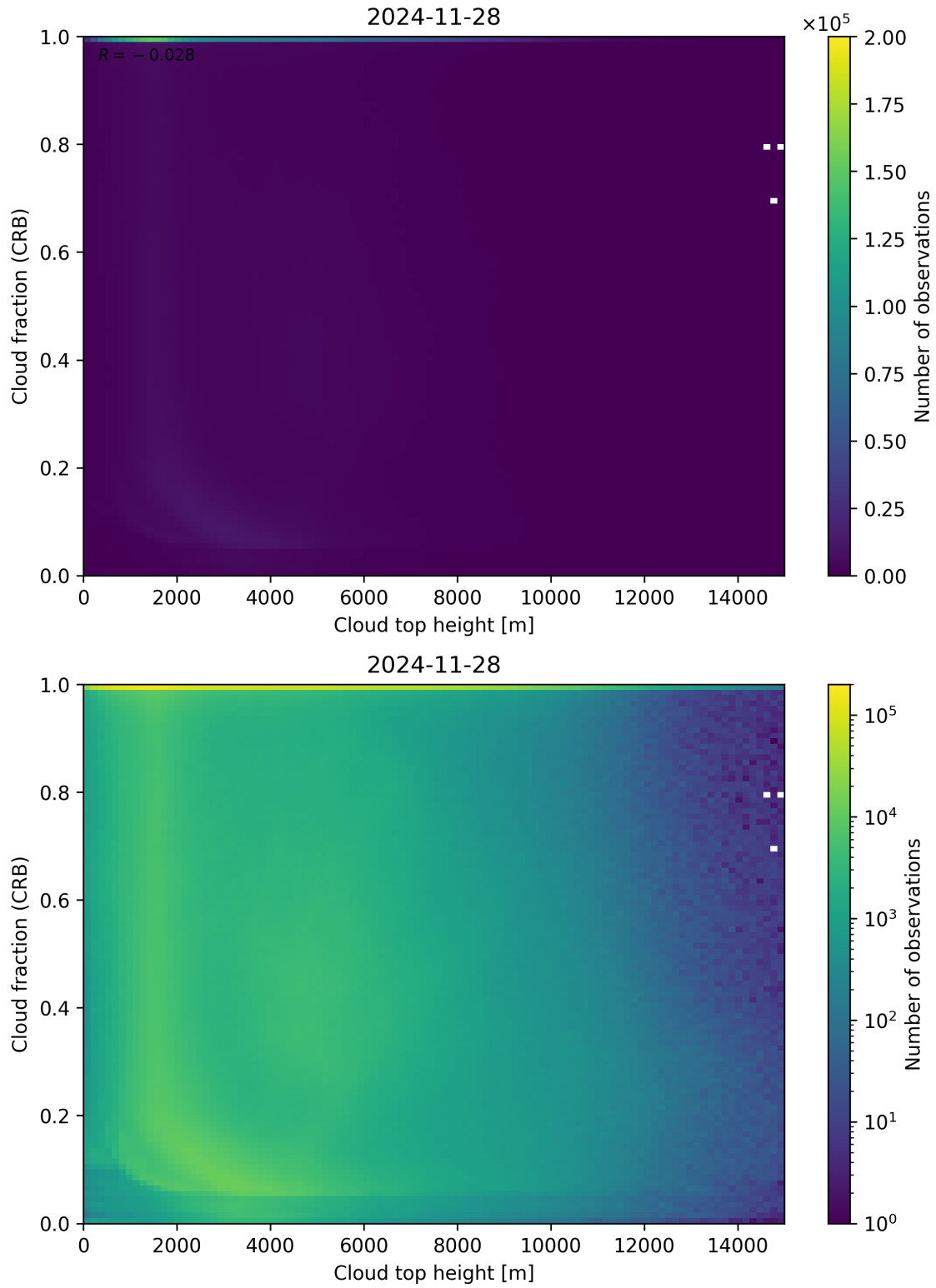
Figure 88: Scatter density plot of “Cloud top height” against “Cloud fraction (CRB)” for 2024-11-27 to 2024-11-29.
