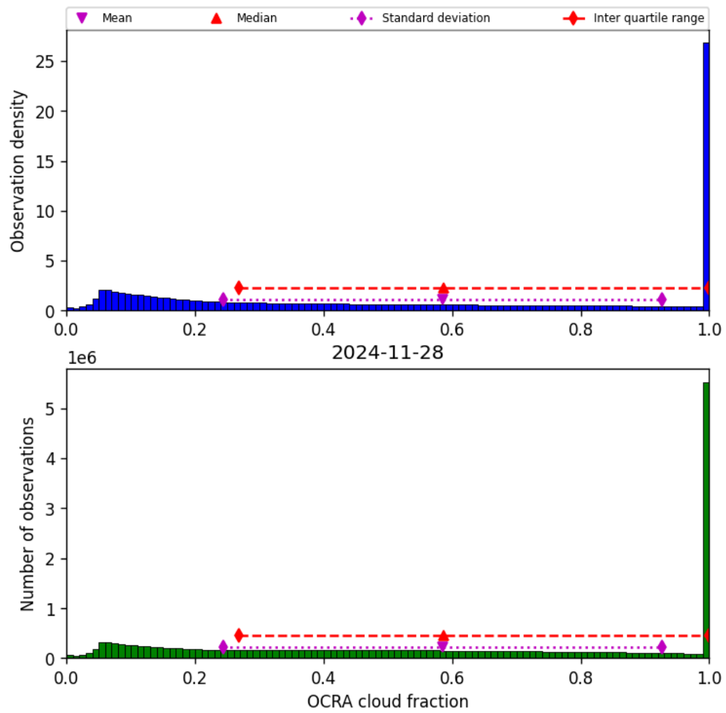
Figure 50: Histogram of “OCRA cloud fraction” for 2024-11-27 to 2024-11-29
