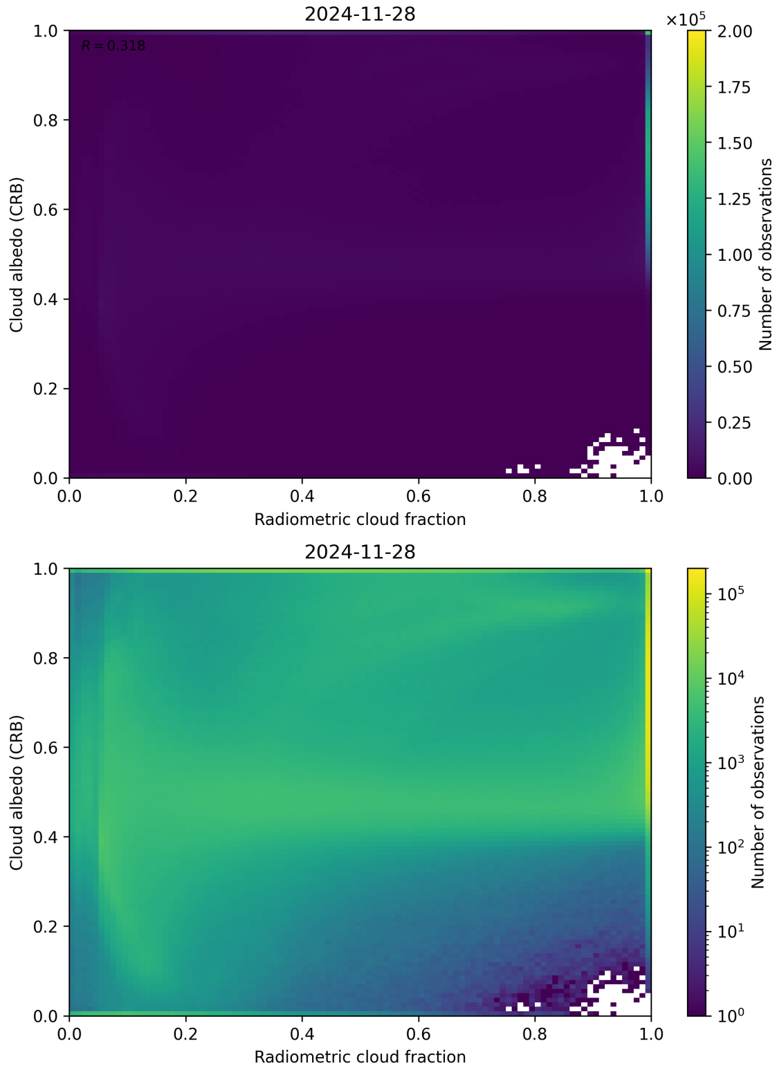
Figure 71: Scatter density plot of “Radiometric cloud fraction” against “Cloud albedo (CRB)” for 2024-11-27 to 2024-11-29.
