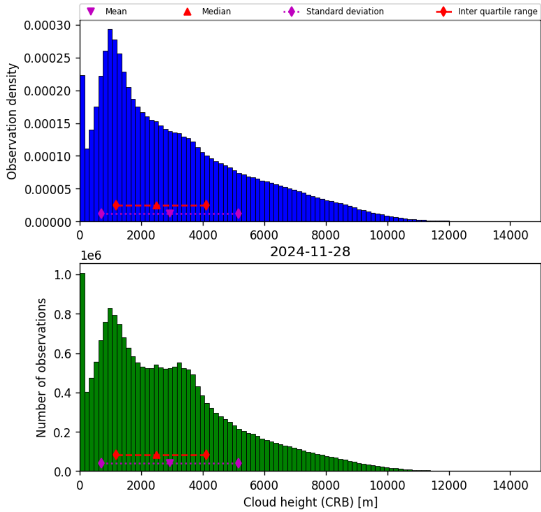
Figure 43: Histogram of “Cloud height (CRB)” for 2024-11-27 to 2024-11-29
