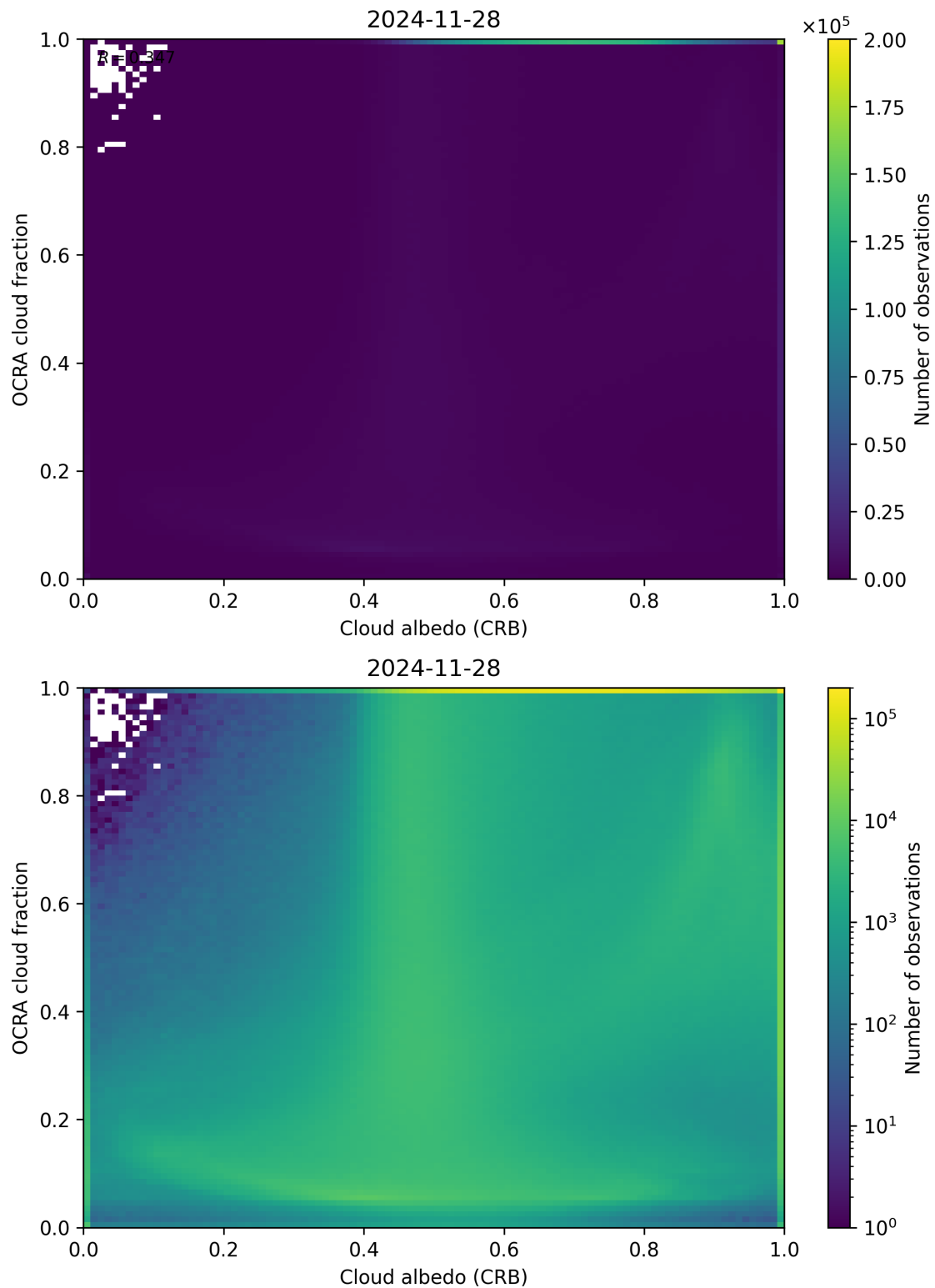
Figure 70: Scatter density plot of “Cloud albedo (CRB)” against “OCRA cloud fraction” for 2024-11-27 to 2024-11-29.
