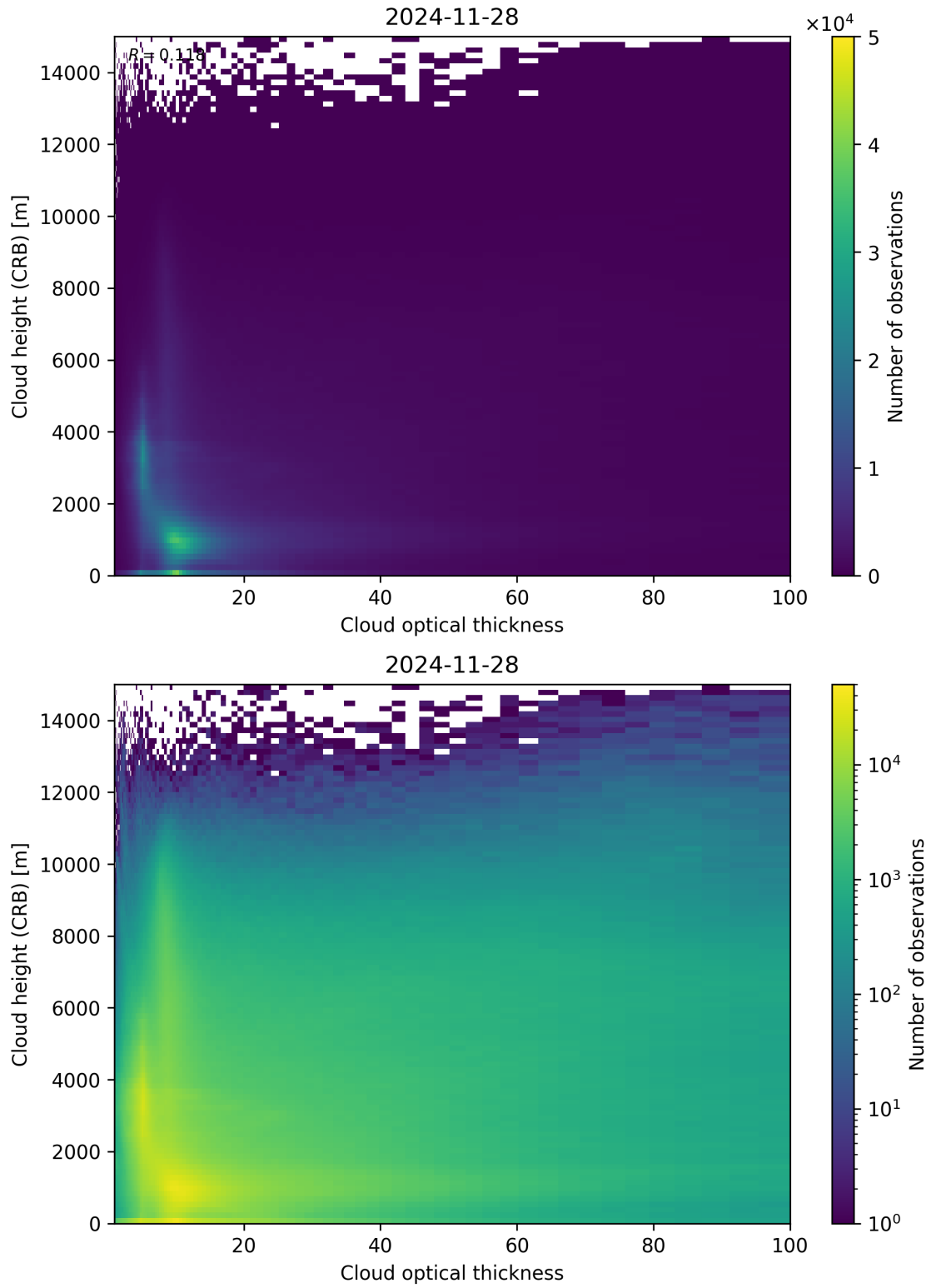
Figure 85: Scatter density plot of “Cloud optical thickness” against “Cloud height (CRB)” for 2024-11-27 to 2024-11-29.
