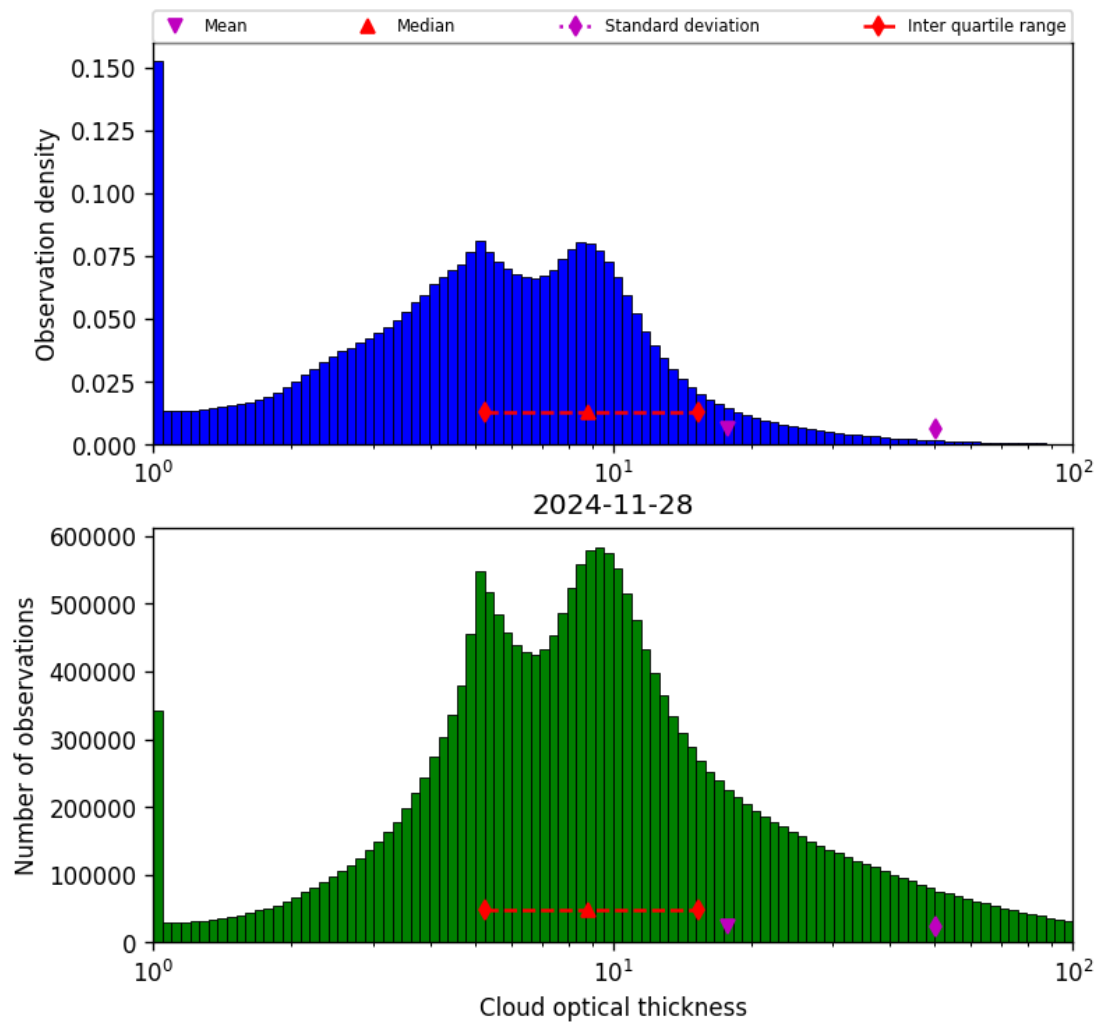
Figure 41: Histogram of “Cloud optical thickness” for 2024-11-27 to 2024-11-29
