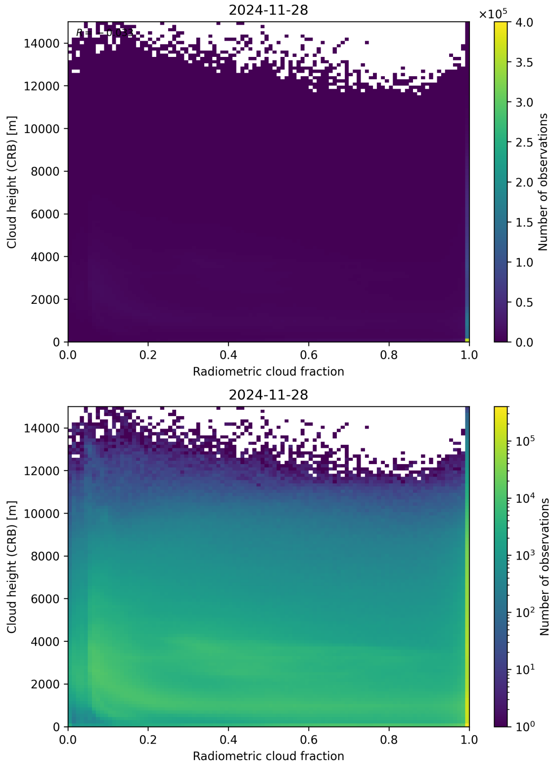
Figure 74: Scatter density plot of “Radiometric cloud fraction” against “Cloud height (CRB)” for 2024-11-27 to 2024-11-29.
