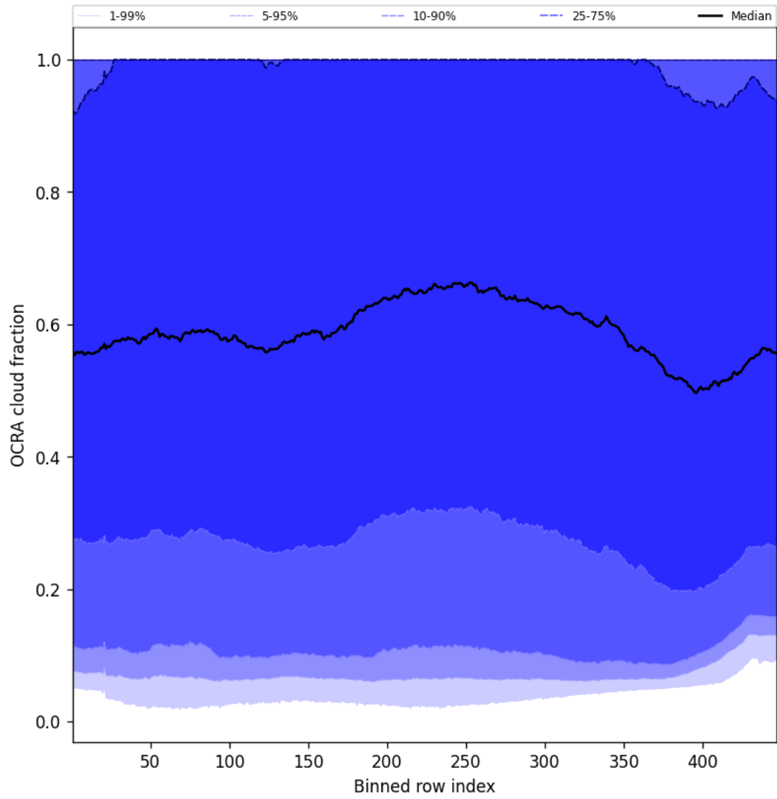
Figure 66: Along track statistics of “OCRA cloud fraction” for 2024-11-27 to 2024-11-29
