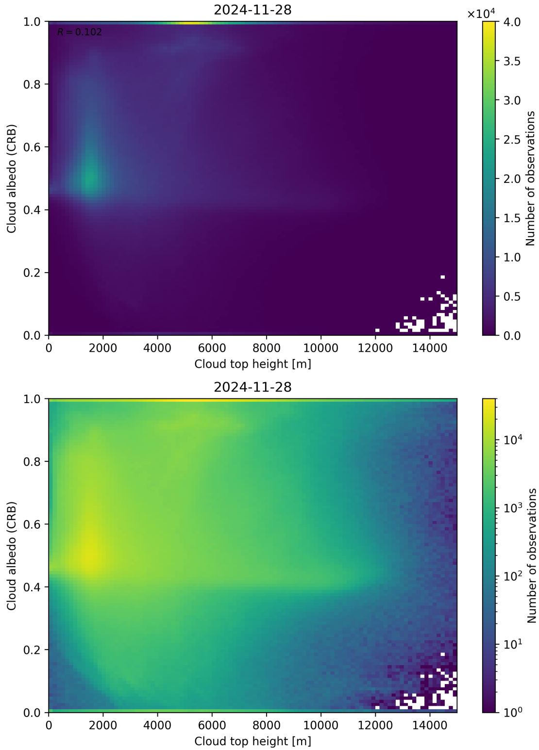
Figure 86: Scatter density plot of “Cloud top height” against “Cloud albedo (CRB)” for 2024-11-27 to 2024-11-29.
