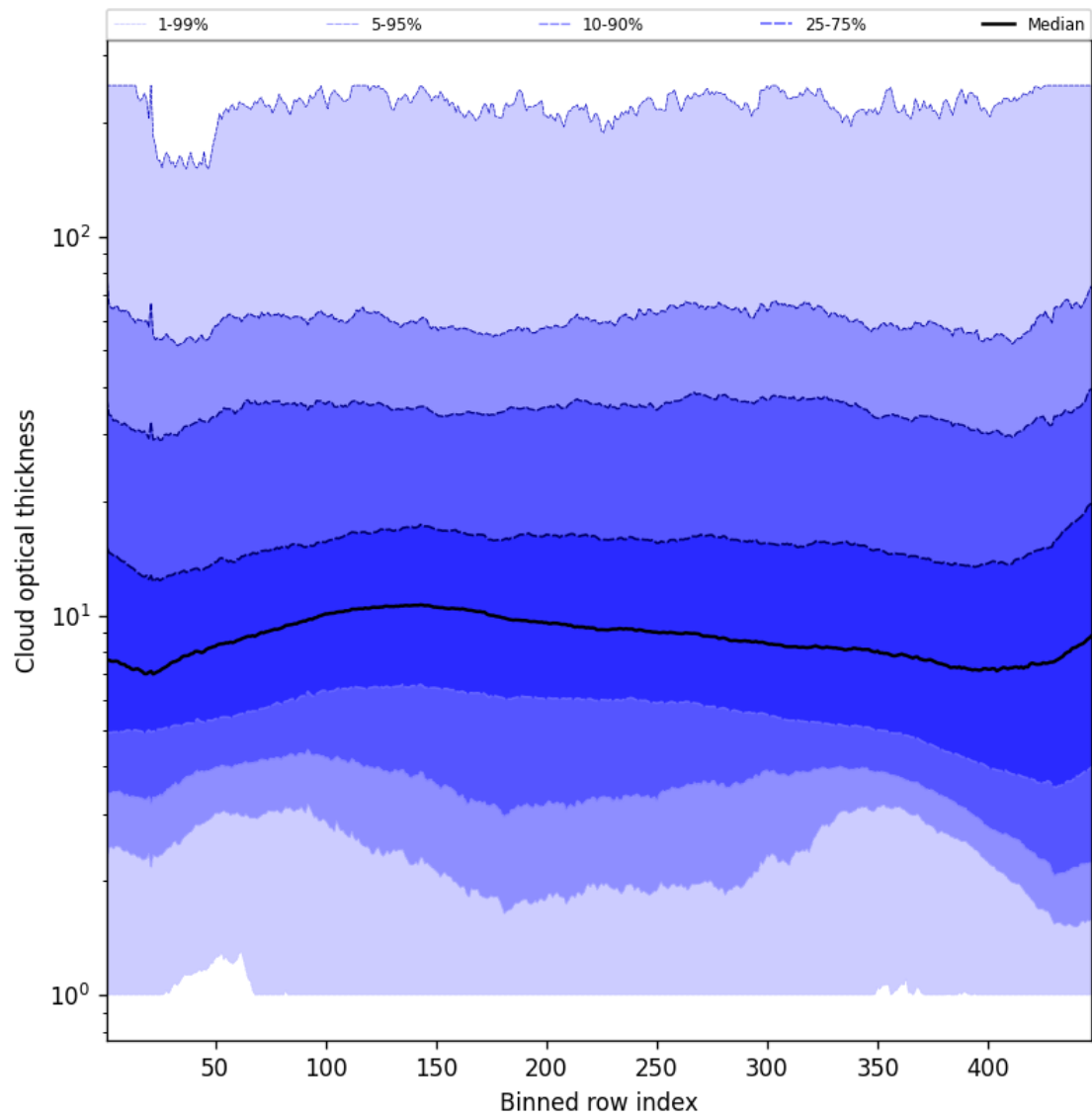
Figure 57: Along track statistics of “Cloud optical thickness” for 2024-11-27 to 2024-11-29
