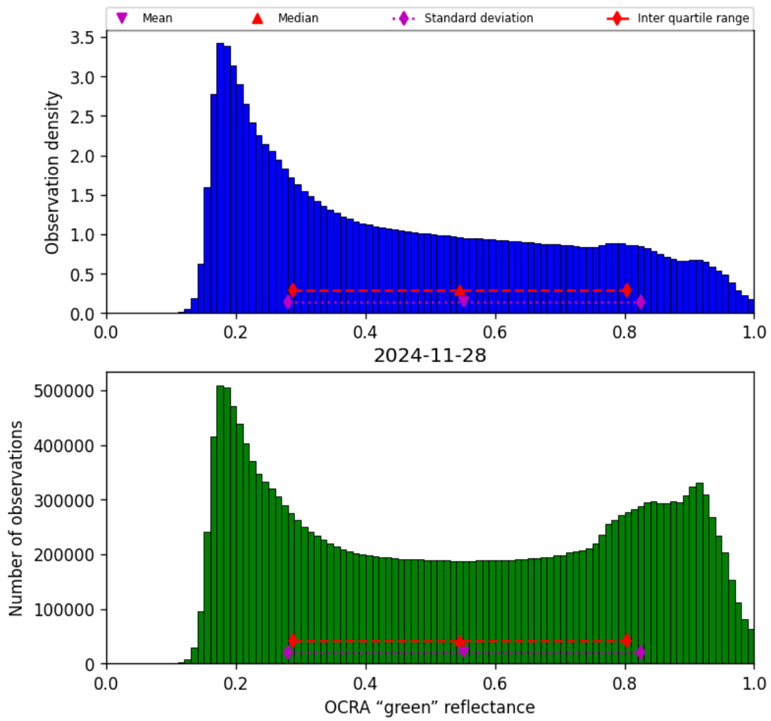
Figure 52: Histogram of “OCRA “green” reflectance” for 2024-11-27 to 2024-11-29
