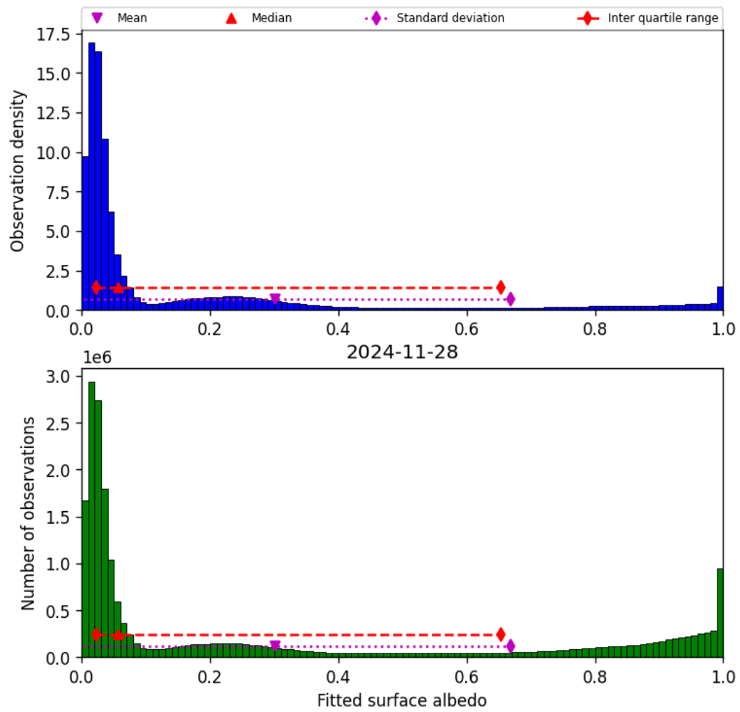
Figure 45: Histogram of “Fitted surface albedo” for 2024-11-27 to 2024-11-29
