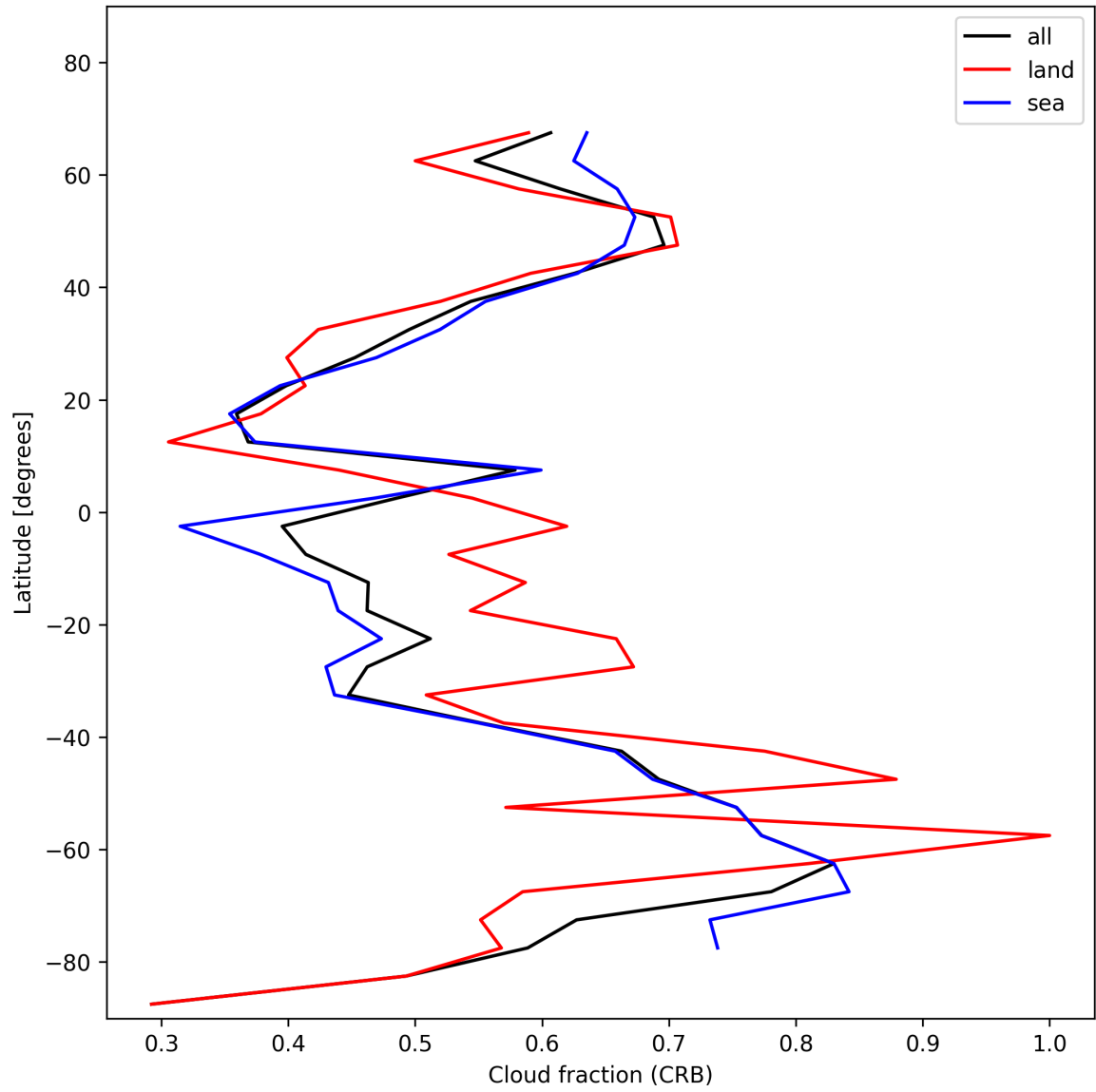
Figure 26: Zonal average of “Cloud fraction (CRB)” for 2024-11-27 to 2024-11-29.
