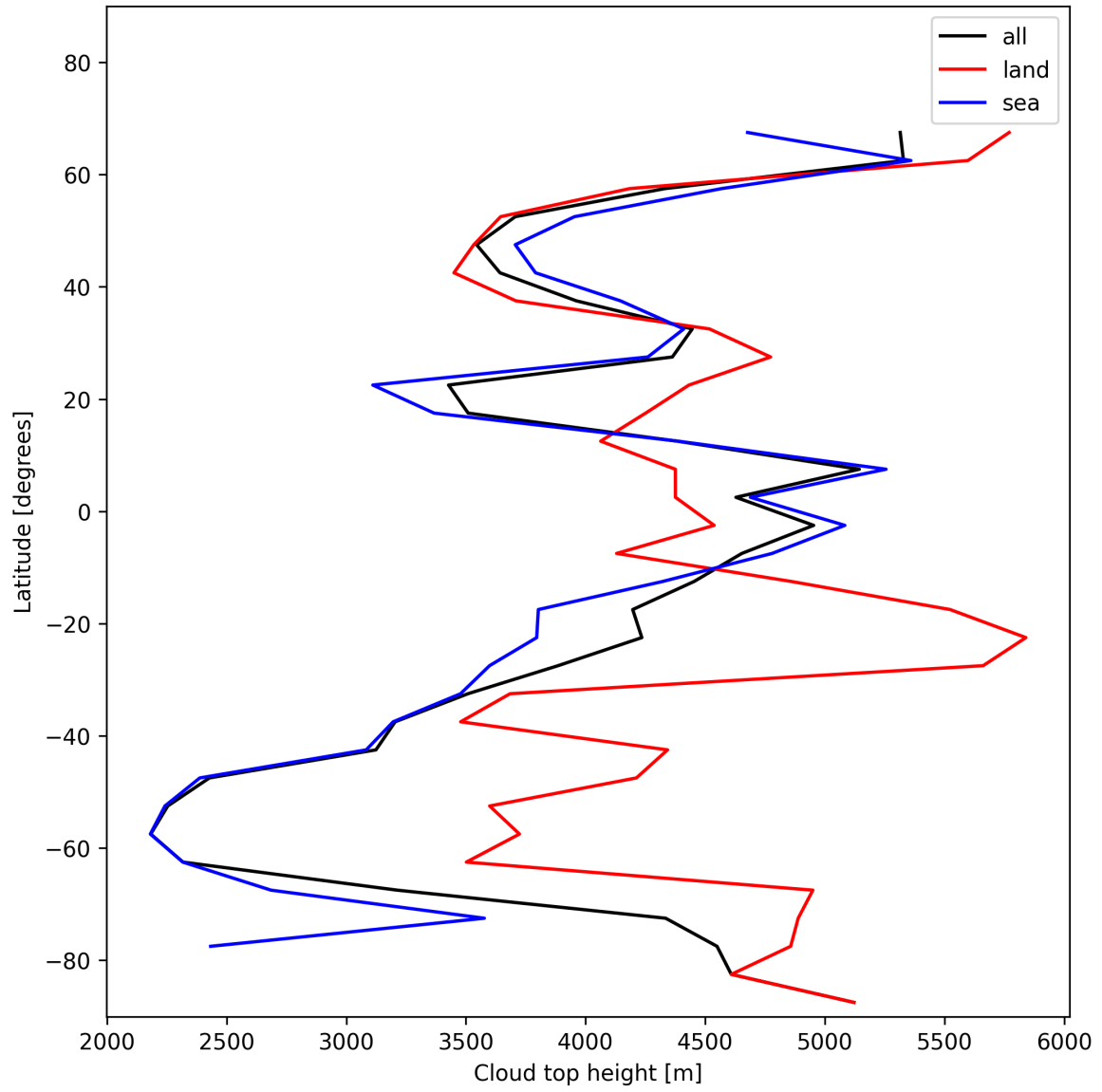
Figure 24: Zonal average of “Cloud top height” for 2024-11-27 to 2024-11-29.
