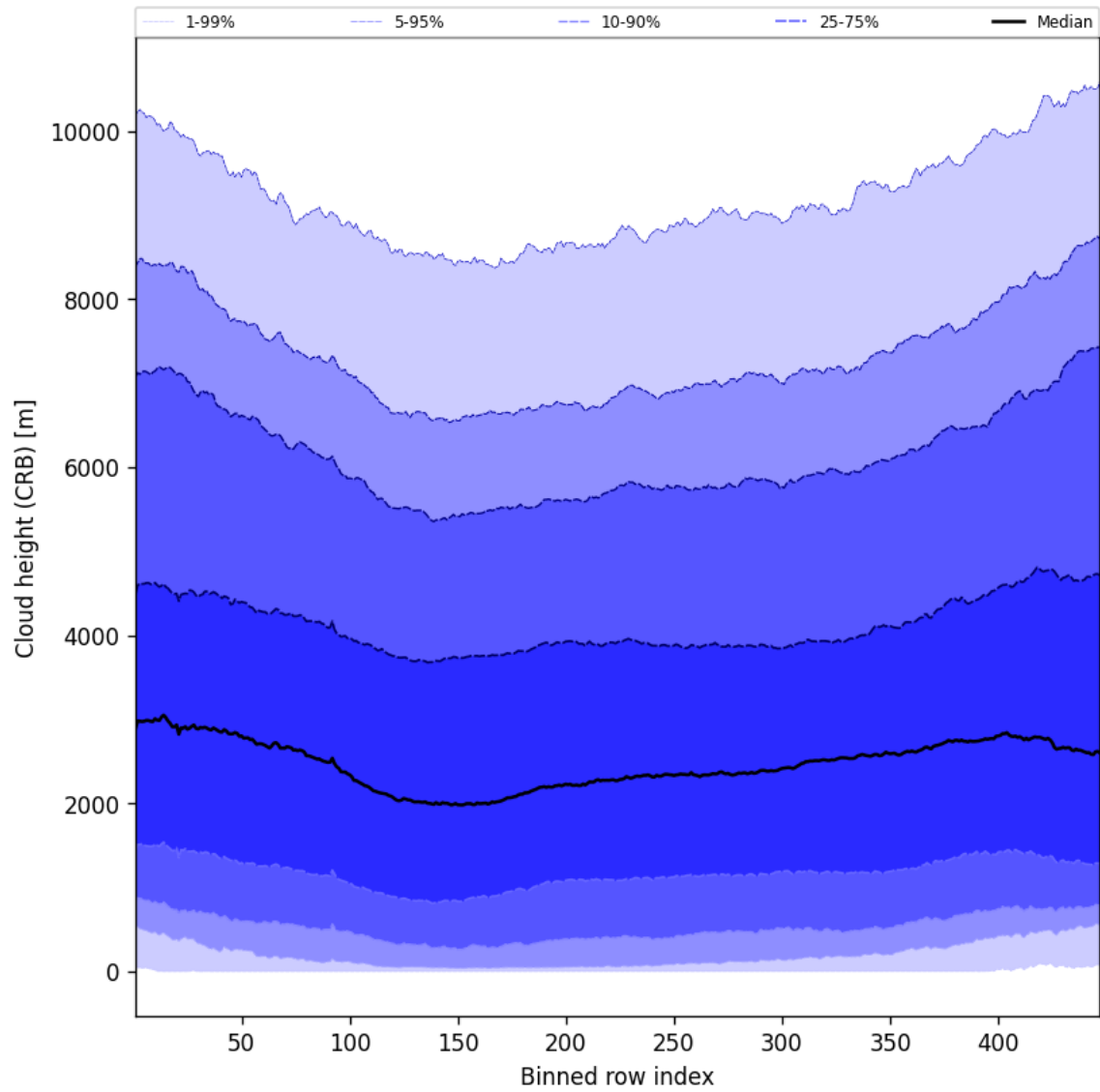
Figure 59: Along track statistics of “Cloud height (CRB)” for 2024-11-27 to 2024-11-29
