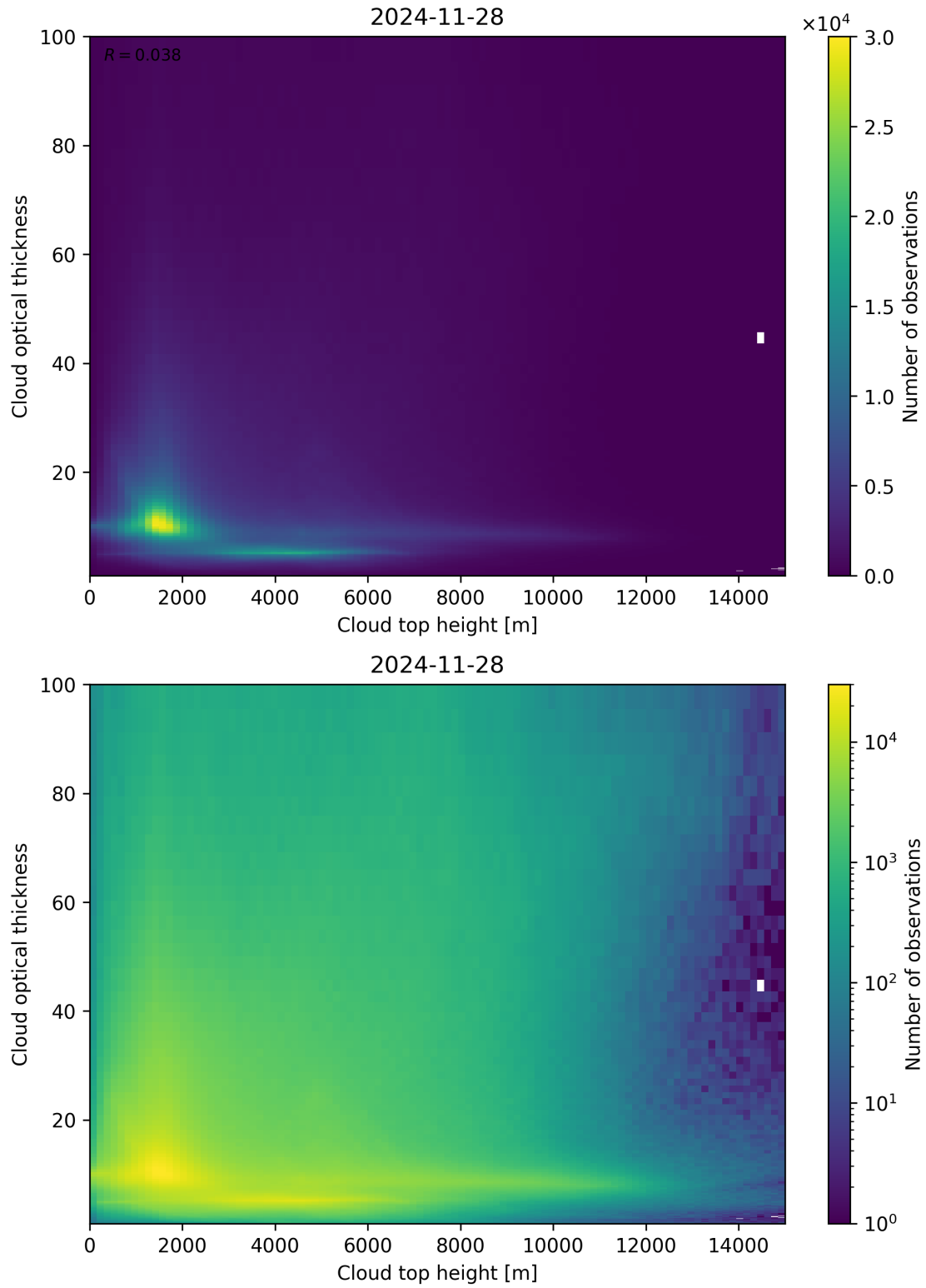
Figure 90: Scatter density plot of “Cloud top height” against “Cloud optical thickness” for 2024-11-27 to 2024-11-29.
