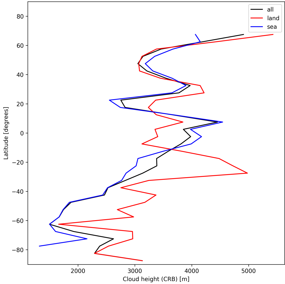
Figure 27: Zonal average of “Cloud height (CRB)” for 2024-11-27 to 2024-11-29.
