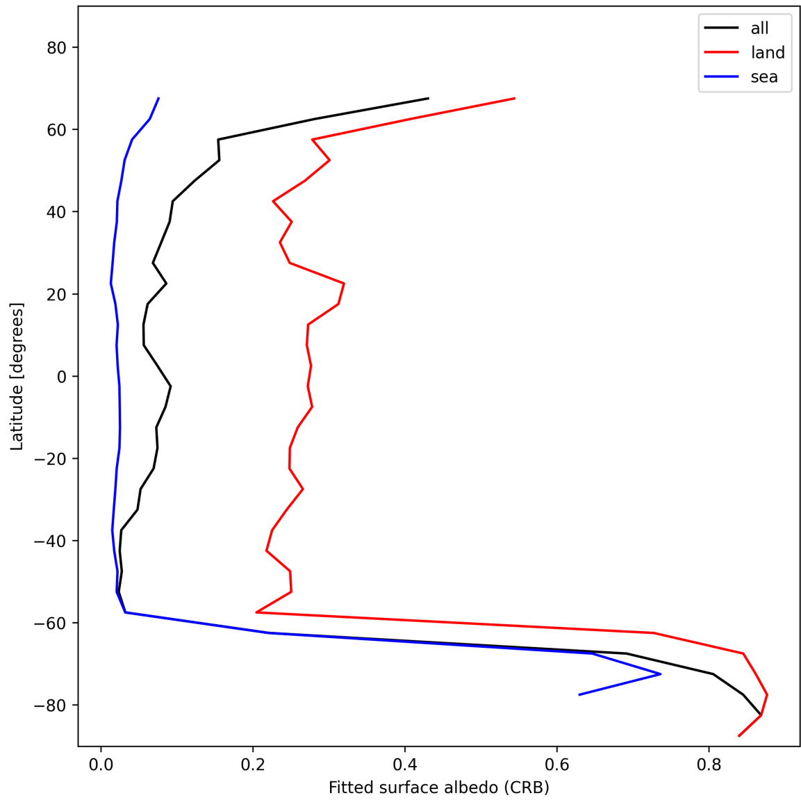
Figure 30: Zonal average of “Fitted surface albedo (CRB)” for 2024-11-27 to 2024-11-29.
