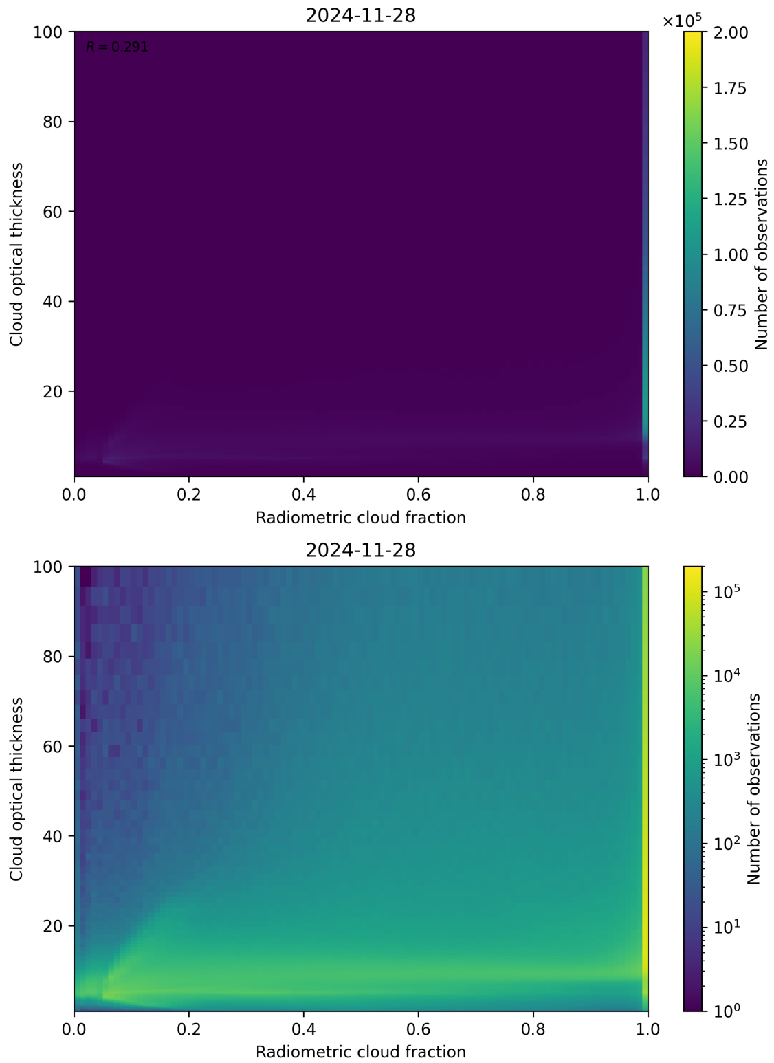
Figure 75: Scatter density plot of “Radiometric cloud fraction” against “Cloud optical thickness” for 2024-11-27 to 2024-11-29.
