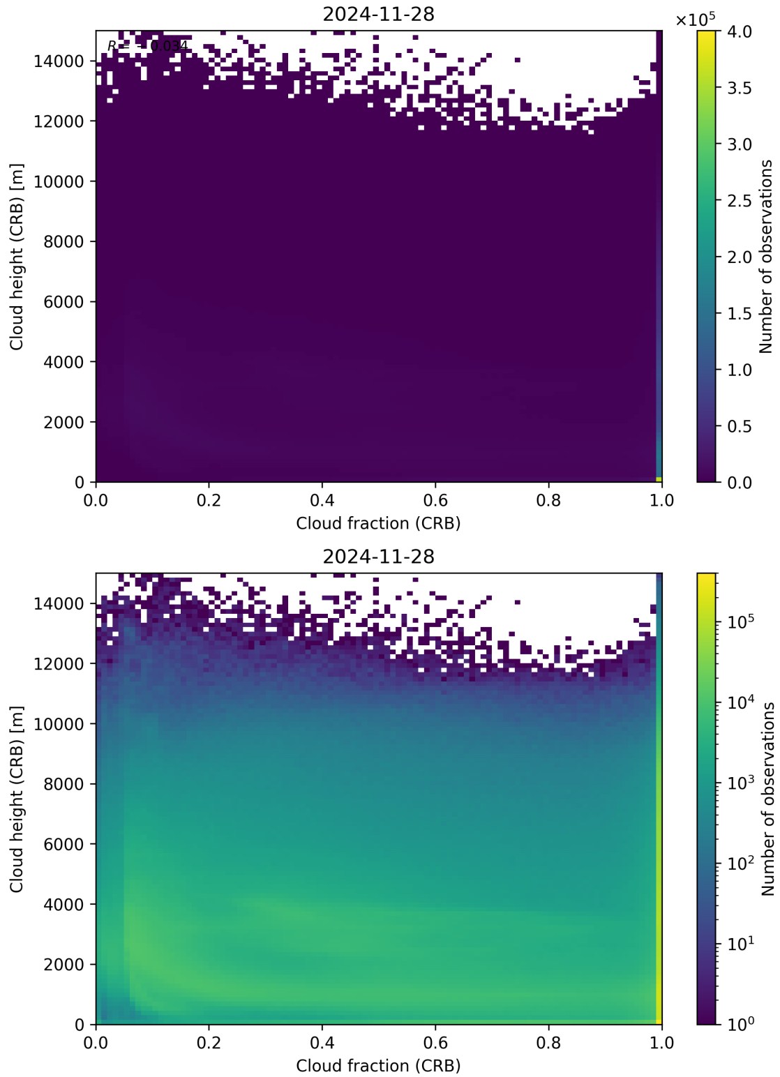
Figure 79: Scatter density plot of “Cloud fraction (CRB)” against “Cloud height (CRB)” for 2024-11-27 to 2024-11-29.
