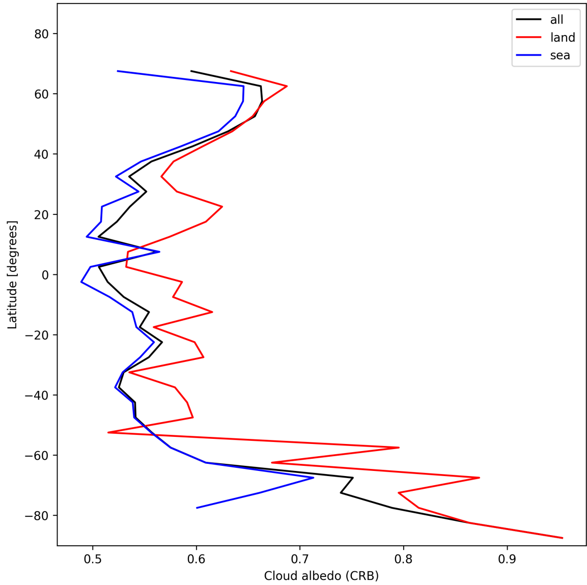
Figure 28: Zonal average of “Cloud albedo (CRB)” for 2024-11-27 to 2024-11-29.
