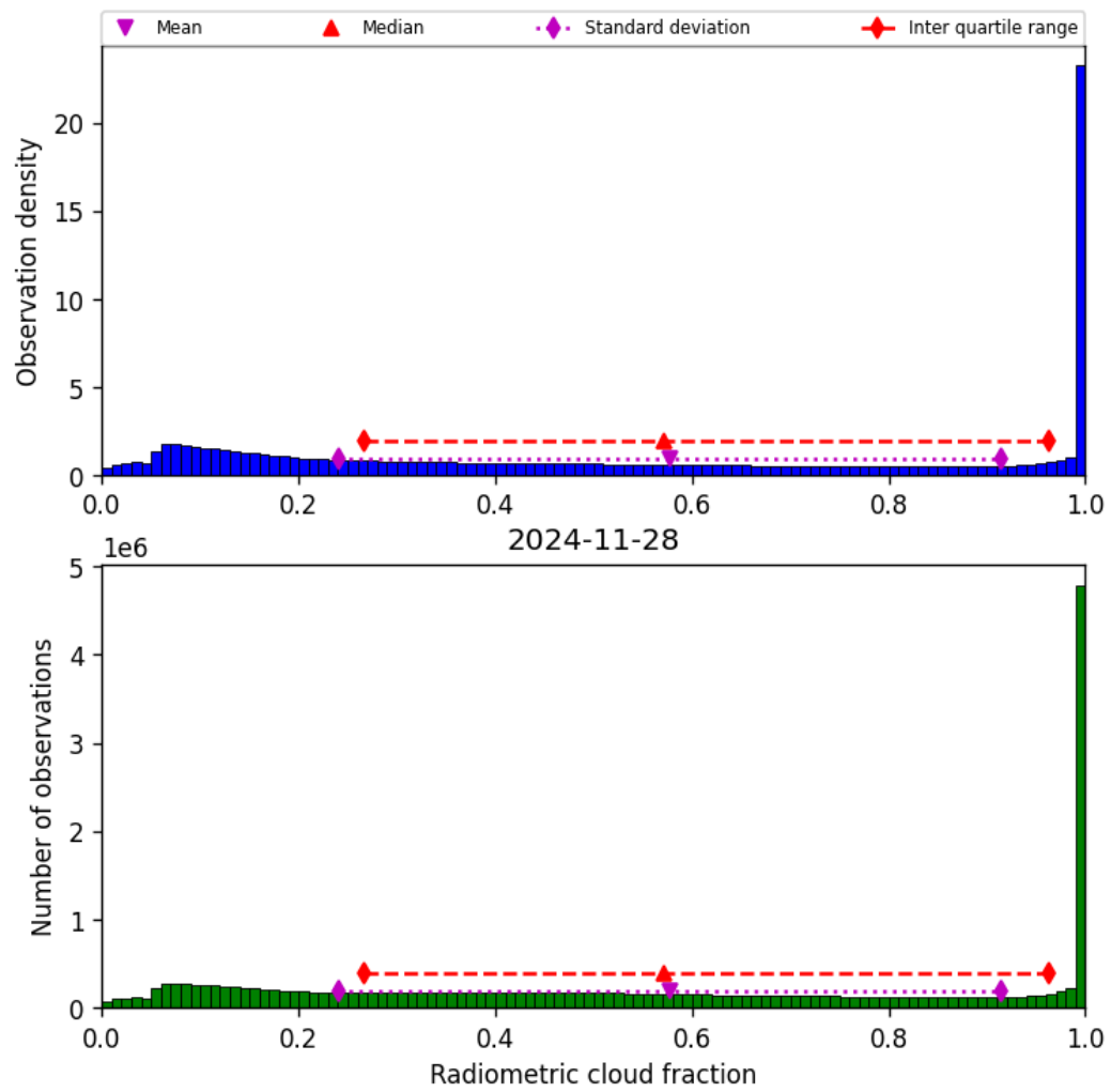
Figure 39: Histogram of “Radiometric cloud fraction” for 2024-11-27 to 2024-11-29
