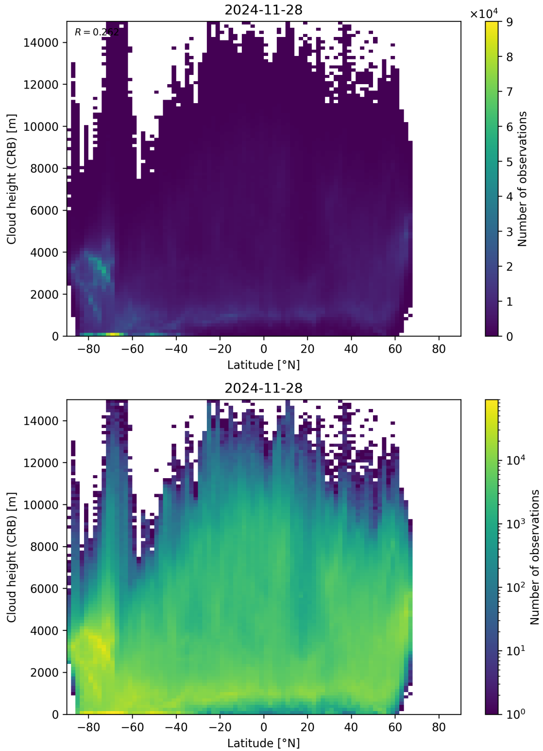
Figure 95: Scatter density plot of “Latitude” against “Cloud height (CRB)” for 2024-11-27 to 2024-11-29.
