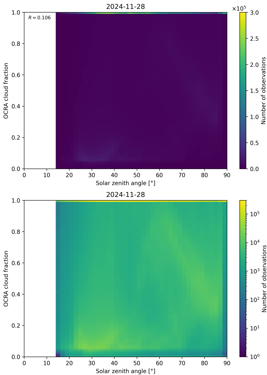
Figure 100: Scatter density plot of “Solar zenith angle” against “OCRA cloud fraction” for 2024-11-27 to 2024-11-29.
