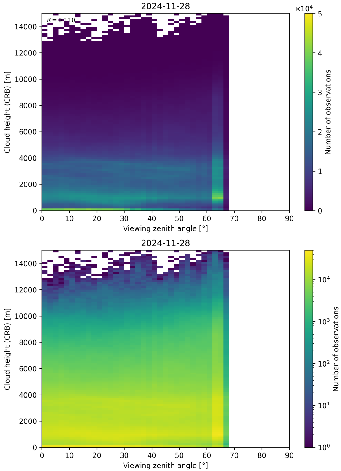
Figure 110: Scatter density plot of “Viewing zenith angle” against “Cloud height (CRB)” for 2024-11-27 to 2024-11-29.
