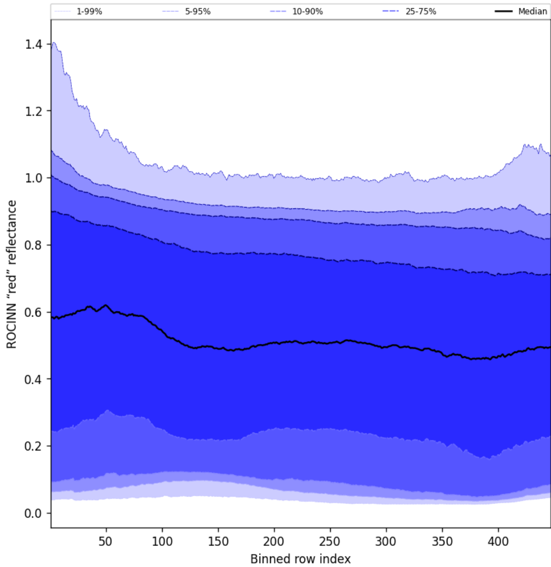
Figure 69: Along track statistics of “ROCINN “red” reflectance” for 2024-11-27 to 2024-11-29
