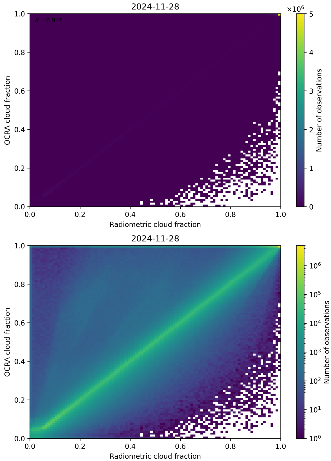
Figure 72: Scatter density plot of “Radiometric cloud fraction” against “OCRA cloud fraction” for 2024-11-27 to 2024-11-29.
