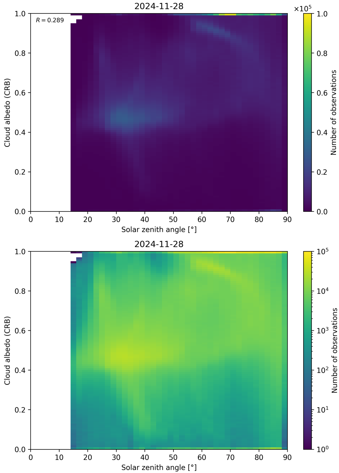
Figure 98: Scatter density plot of “Solar zenith angle” against “Cloud albedo (CRB)” for 2024-11-27 to 2024-11-29.
