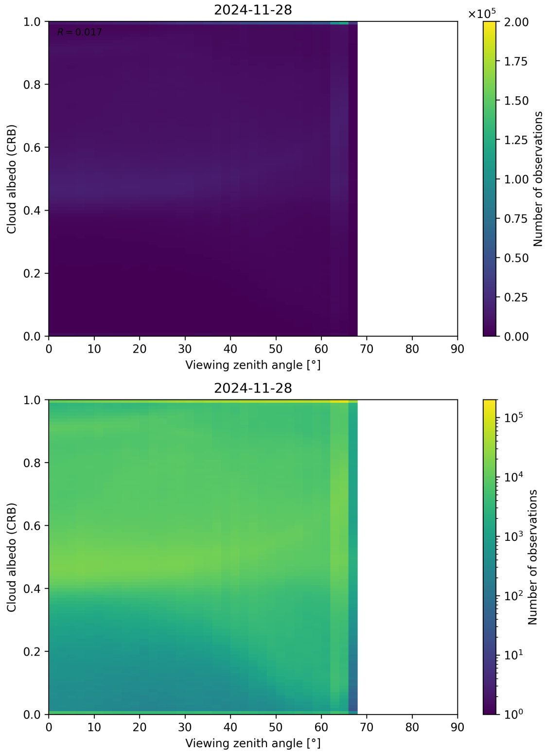
Figure 106: Scatter density plot of “Viewing zenith angle” against “Cloud albedo (CRB)” for 2024-11-27 to 2024-11-29.
