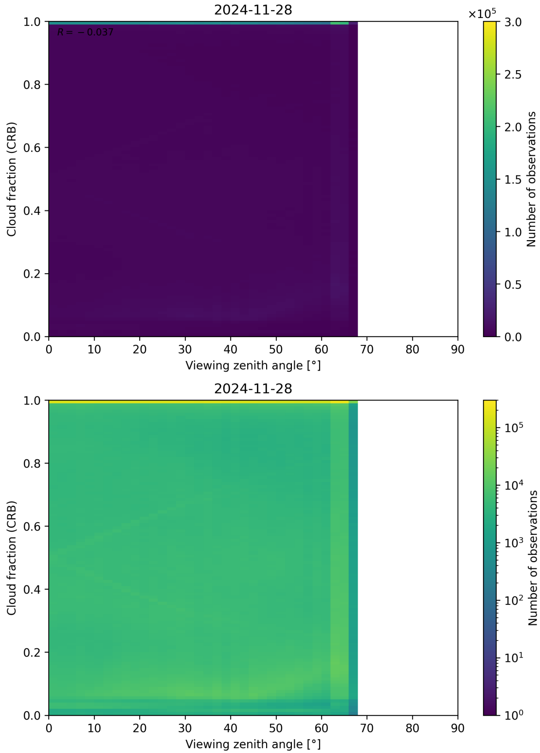
Figure 109: Scatter density plot of “Viewing zenith angle” against “Cloud fraction (CRB)” for 2024-11-27 to 2024-11-29.
