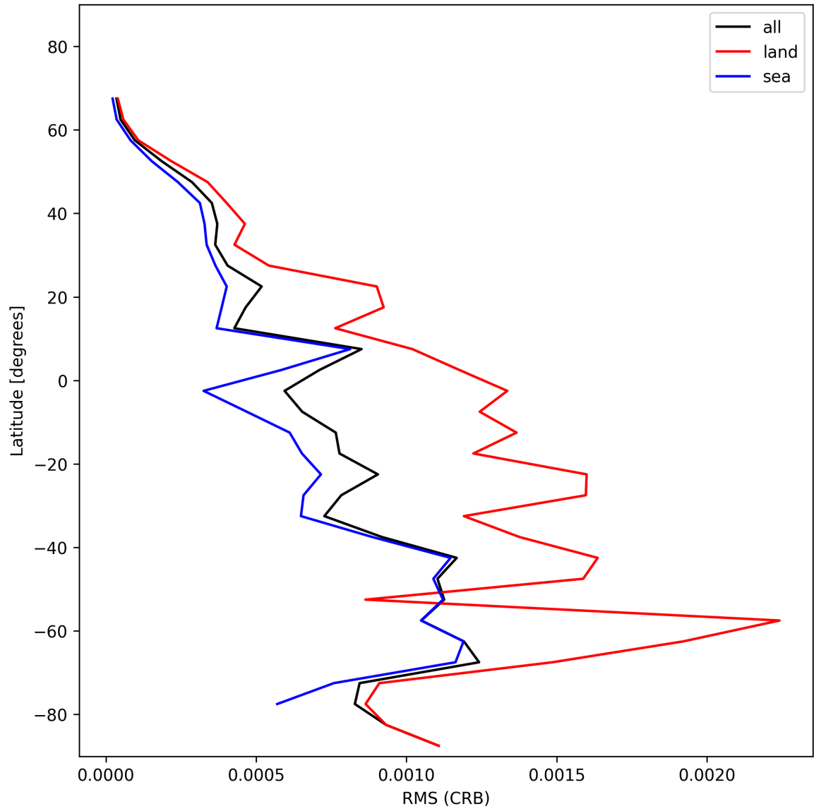
Figure 32: Zonal average of “RMS (CRB)” for 2024-11-27 to 2024-11-29.
