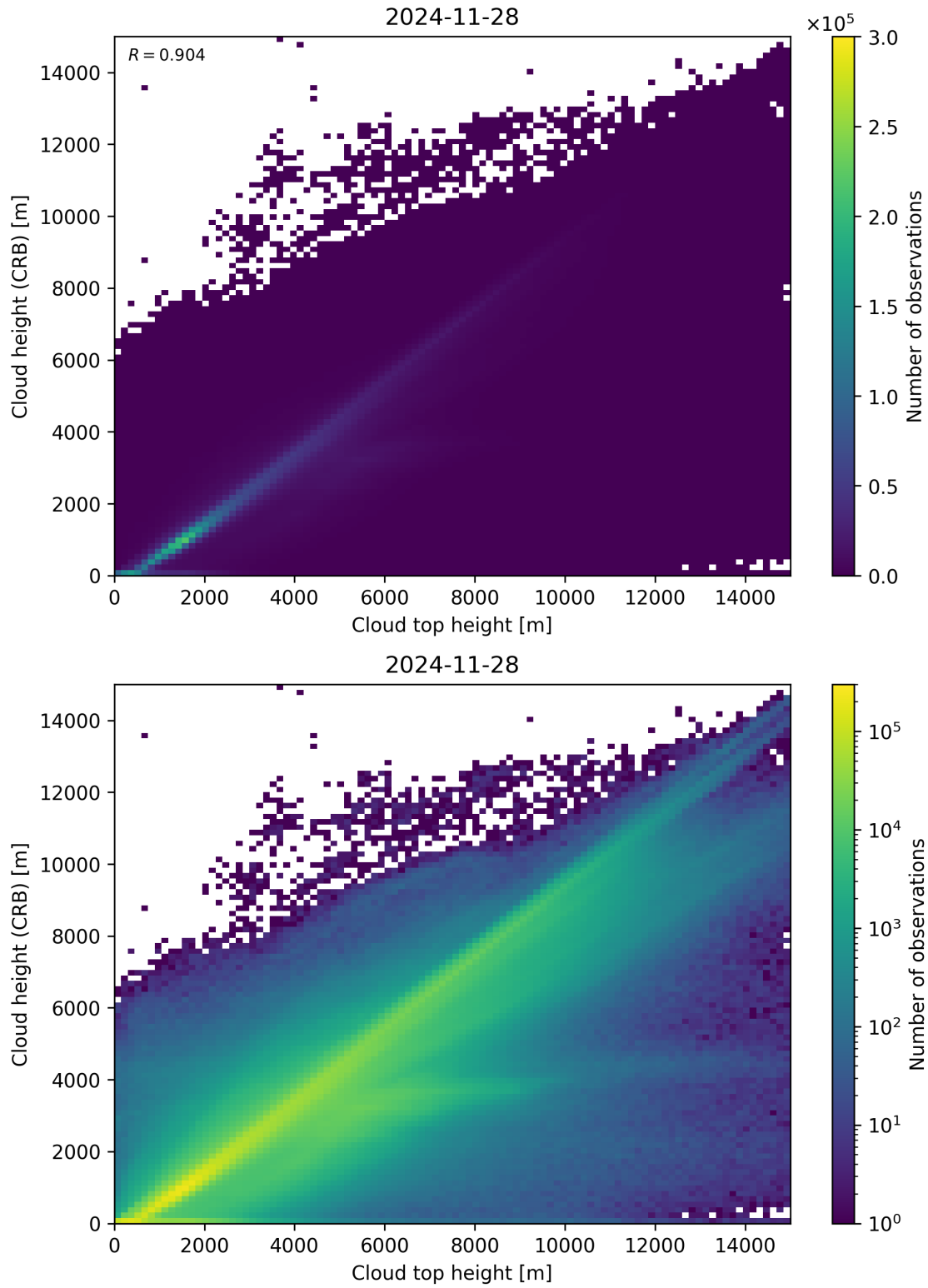
Figure 89: Scatter density plot of “Cloud top height” against “Cloud height (CRB)” for 2024-11-27 to 2024-11-29.
