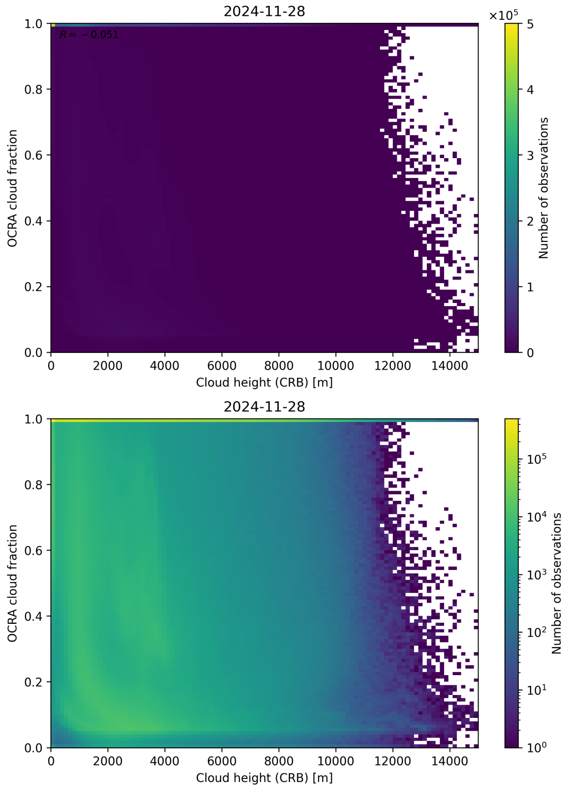
Figure 81: Scatter density plot of “Cloud height (CRB)” against “OCRA cloud fraction” for 2024-11-27 to 2024-11-29.
