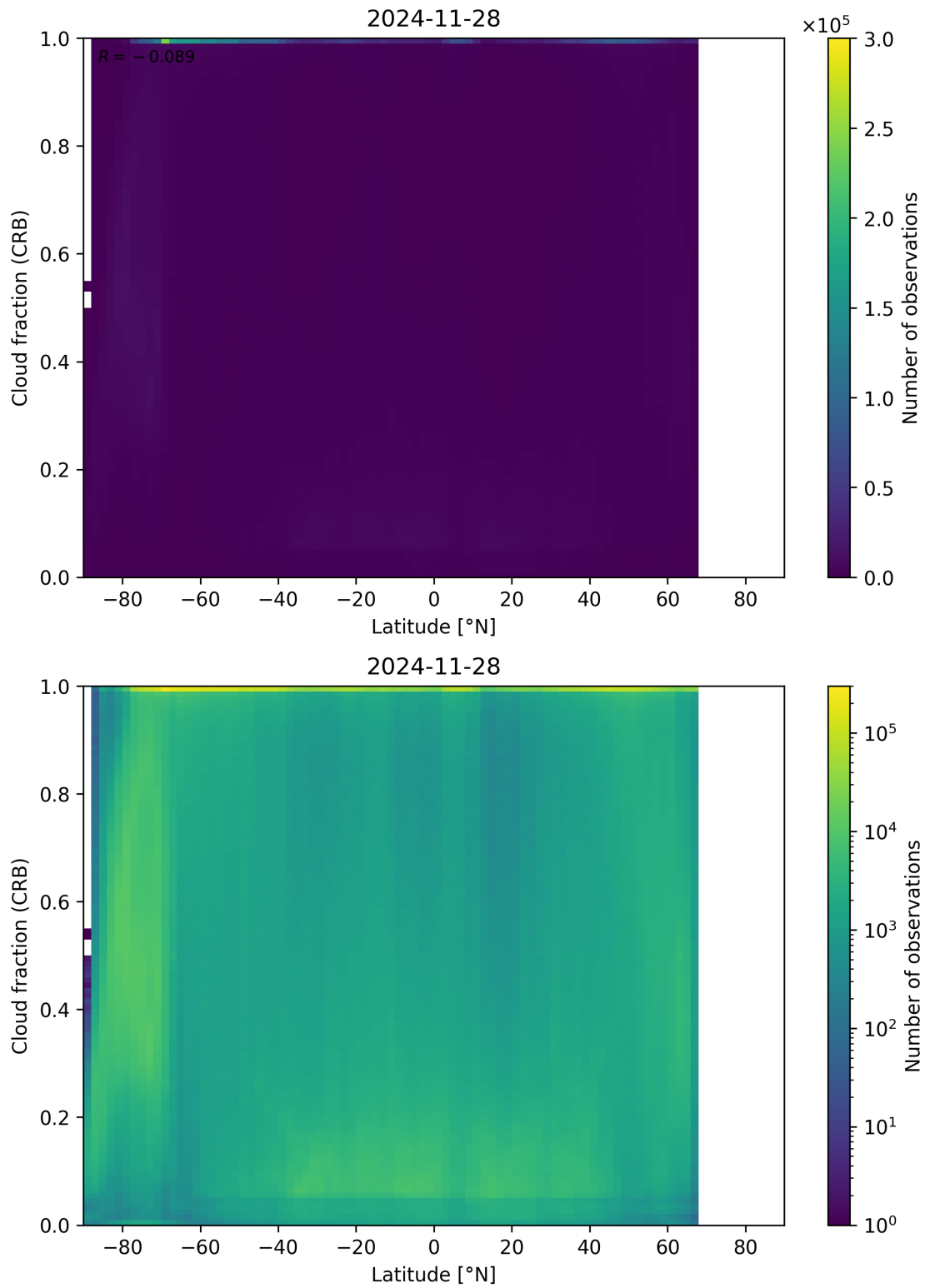
Figure 94: Scatter density plot of “Latitude” against “Cloud fraction (CRB)” for 2024-11-27 to 2024-11-29.
