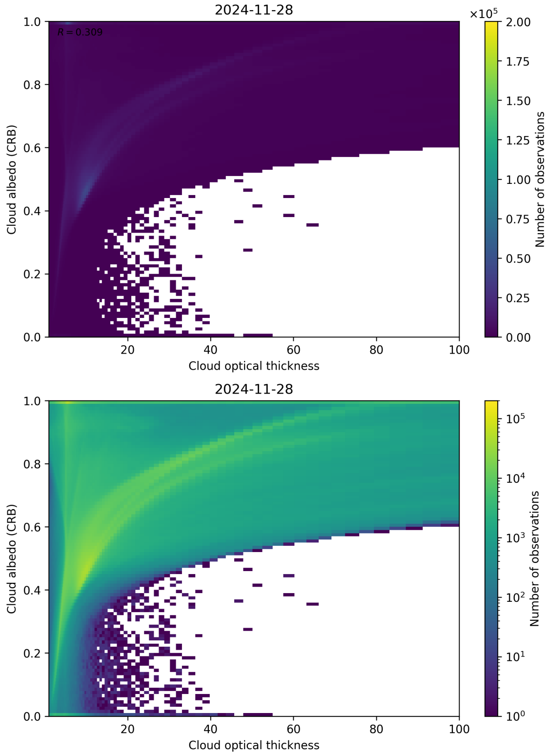
Figure 82: Scatter density plot of “Cloud optical thickness” against “Cloud albedo (CRB)” for 2024-11-27 to 2024-11-29.
