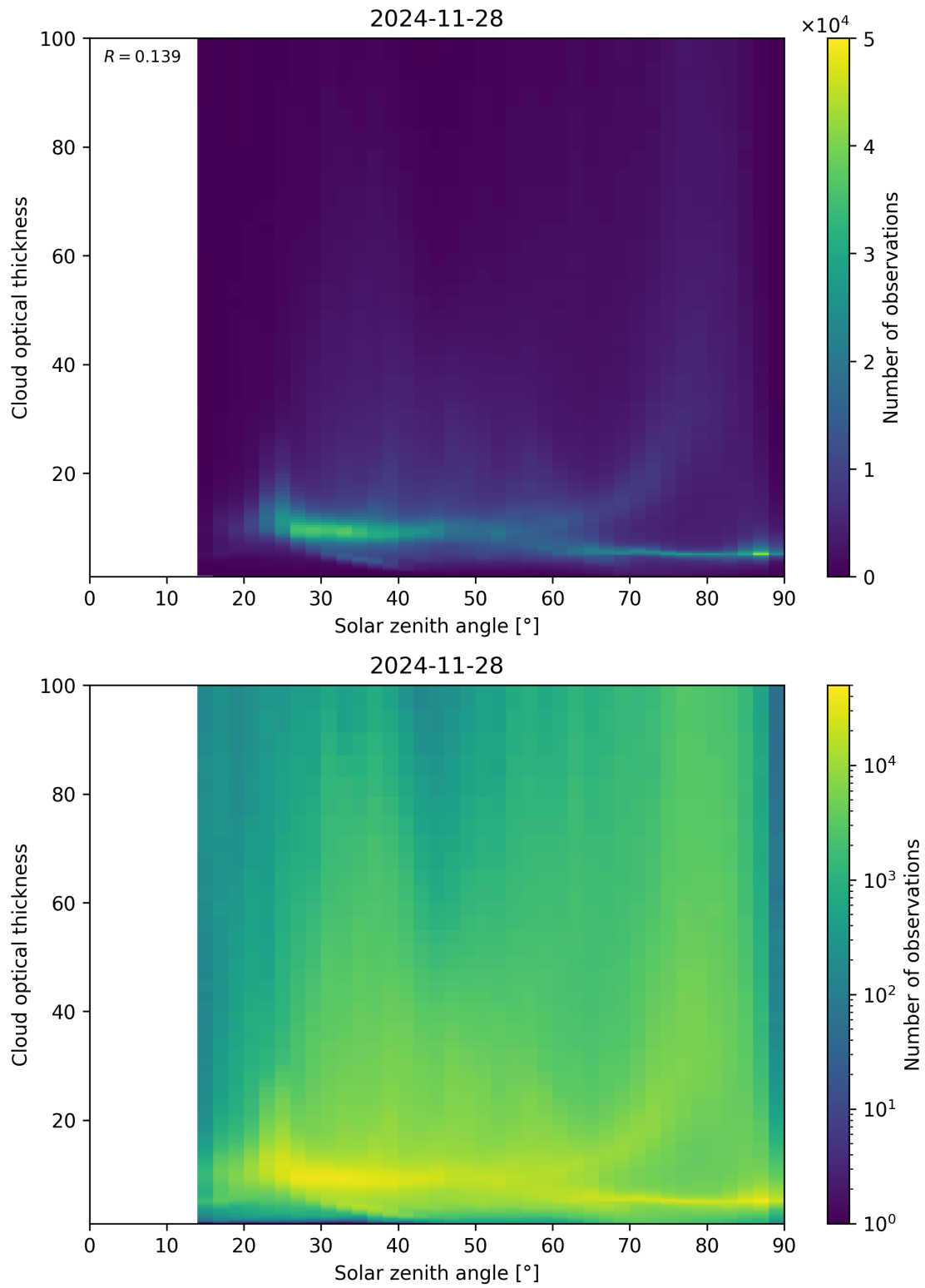
Figure 103: Scatter density plot of “Solar zenith angle” against “Cloud optical thickness” for 2024-11-27 to 2024-11-29.
