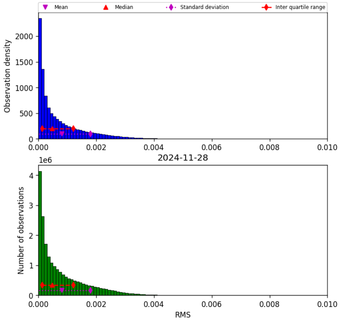
Figure 47: Histogram of “RMS” for 2024-11-27 to 2024-11-29
