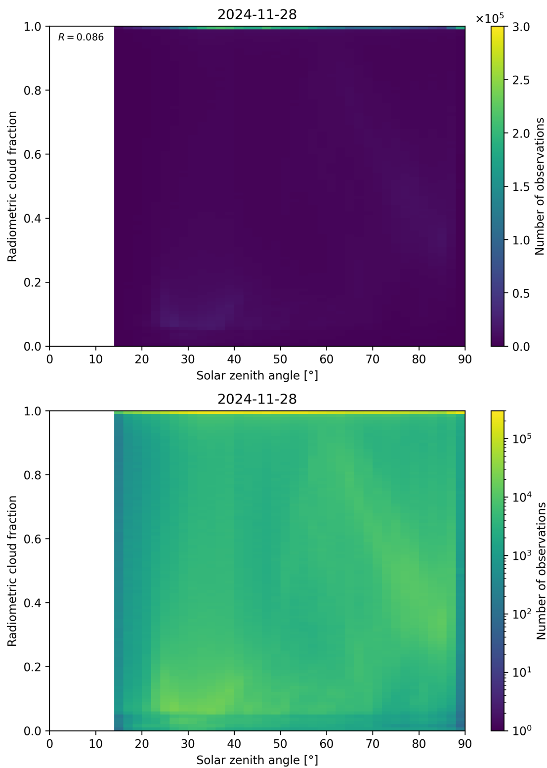
Figure 99: Scatter density plot of “Solar zenith angle” against “Radiometric cloud fraction” for 2024-11-27 to 2024-11-29.
