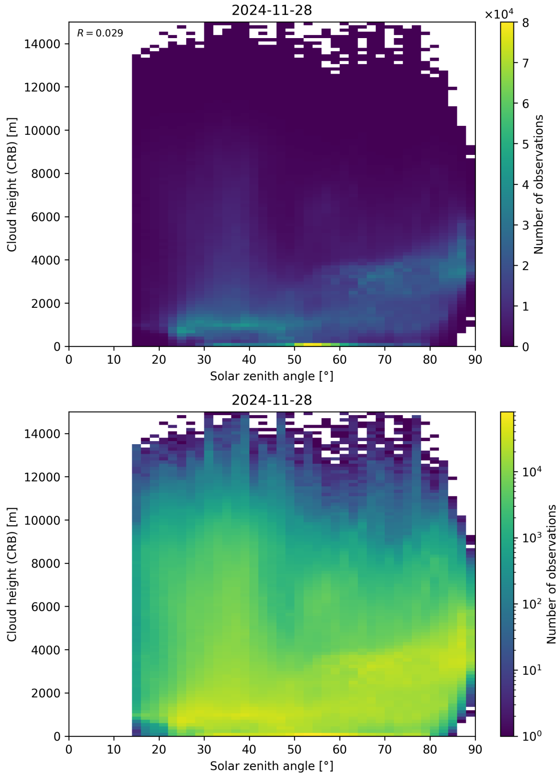
Figure 102: Scatter density plot of “Solar zenith angle” against “Cloud height (CRB)” for 2024-11-27 to 2024-11-29.
