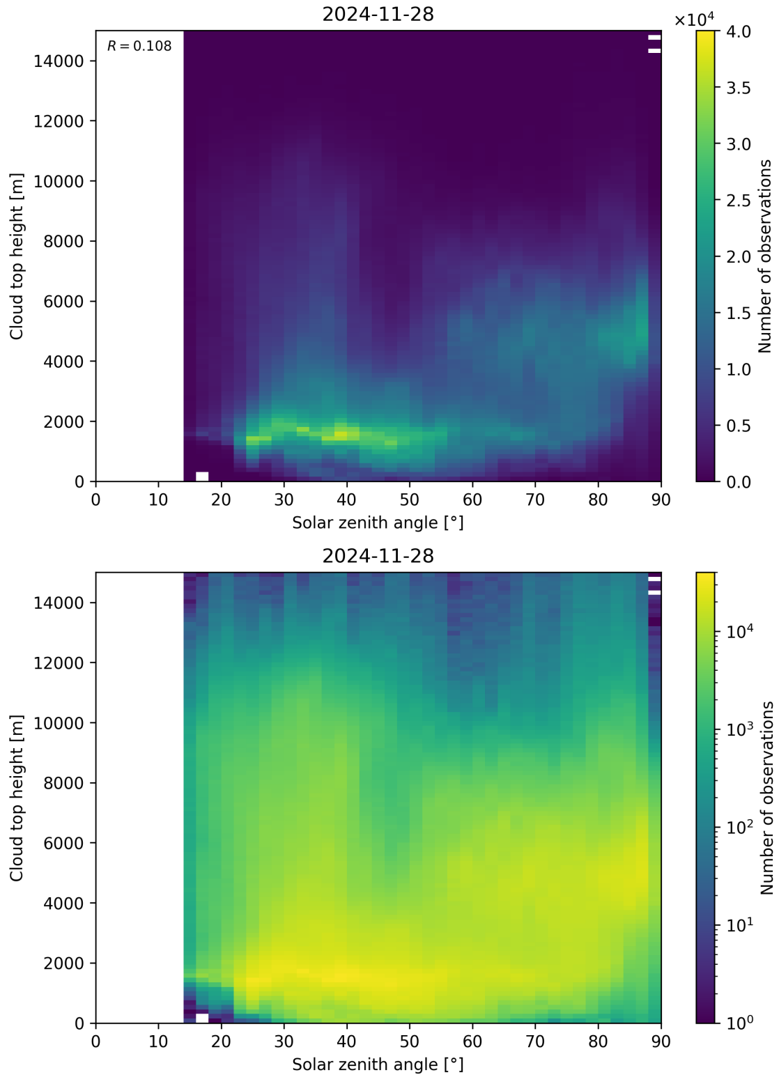
Figure 104: Scatter density plot of “Solar zenith angle” against “Cloud top height” for 2024-11-27 to 2024-11-29.
