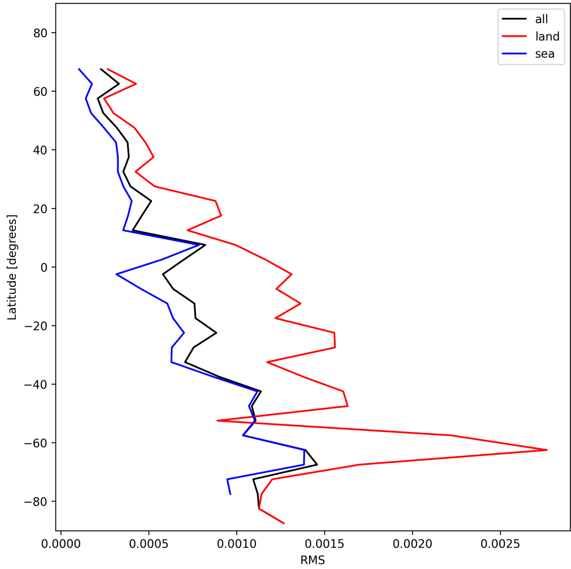
Figure 31: Zonal average of “RMS” for 2024-11-27 to 2024-11-29.
