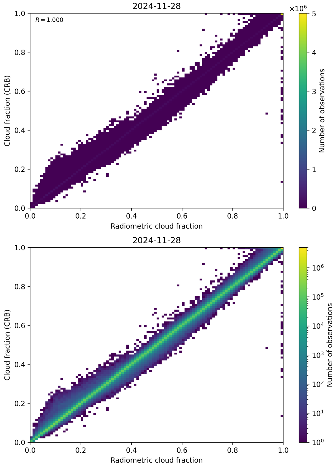
Figure 73: Scatter density plot of “Radiometric cloud fraction” against “Cloud fraction (CRB)” for 2024-11-27 to 2024-11-29.
