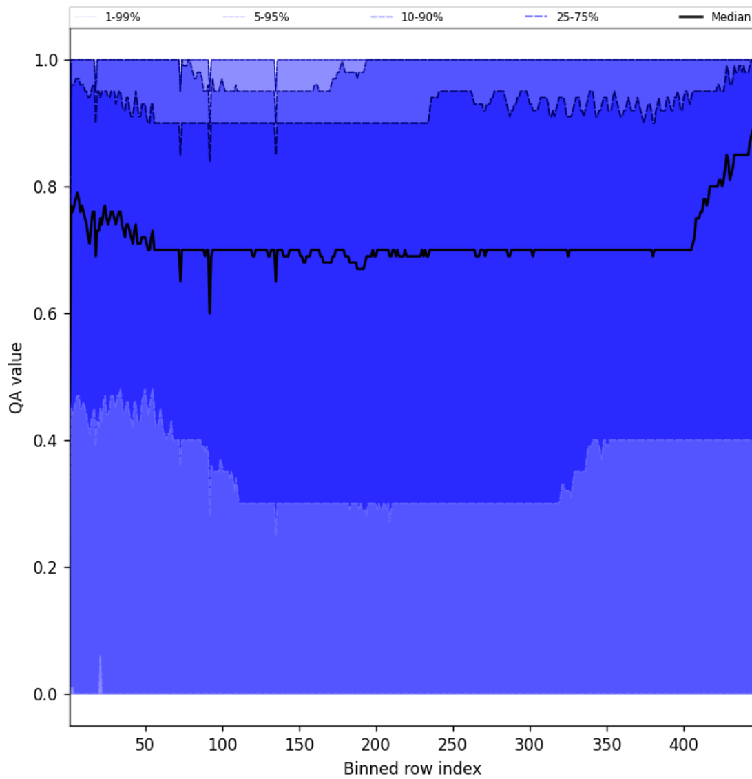
Figure 54: Along track statistics of “QA value” for 2024-11-27 to 2024-11-29
