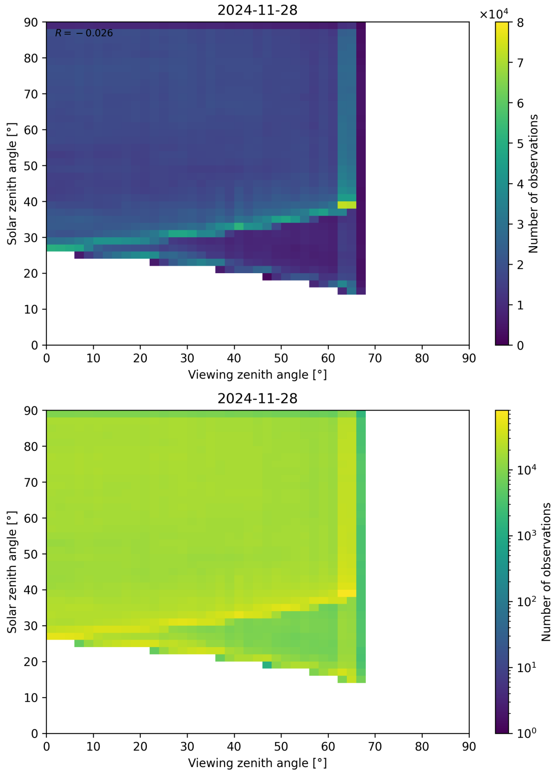
Figure 114: Scatter density plot of “Viewing zenith angle” against “Solar zenith angle” for 2024-11-27 to 2024-11-29.
