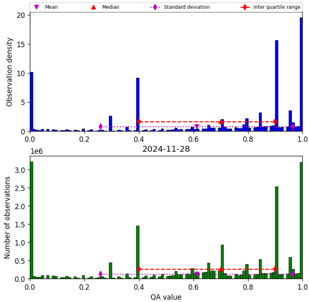
Figure 38: Histogram of “QA value” for 2024-11-27 to 2024-11-29
