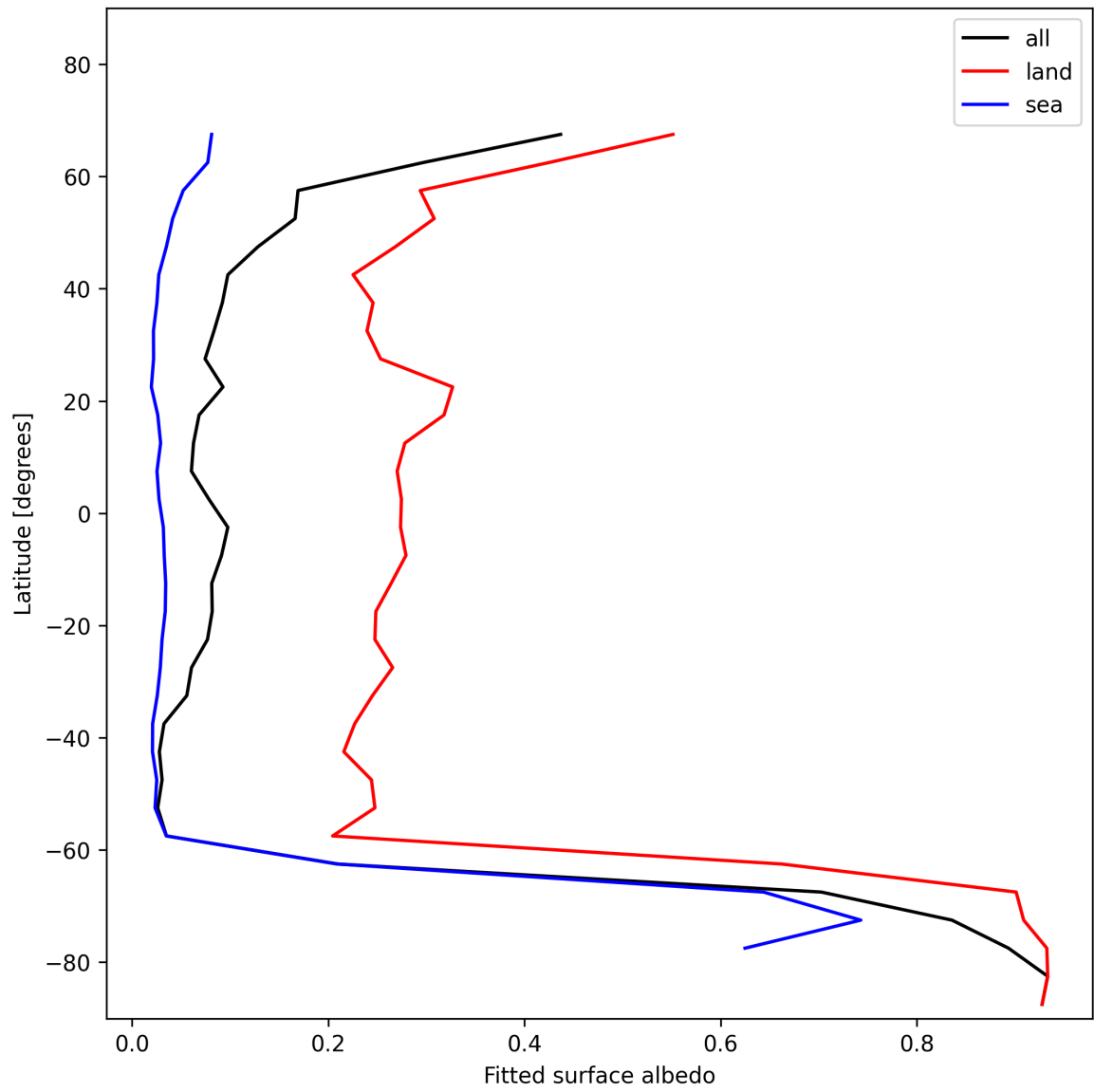
Figure 29: Zonal average of “Fitted surface albedo” for 2024-11-27 to 2024-11-29.
