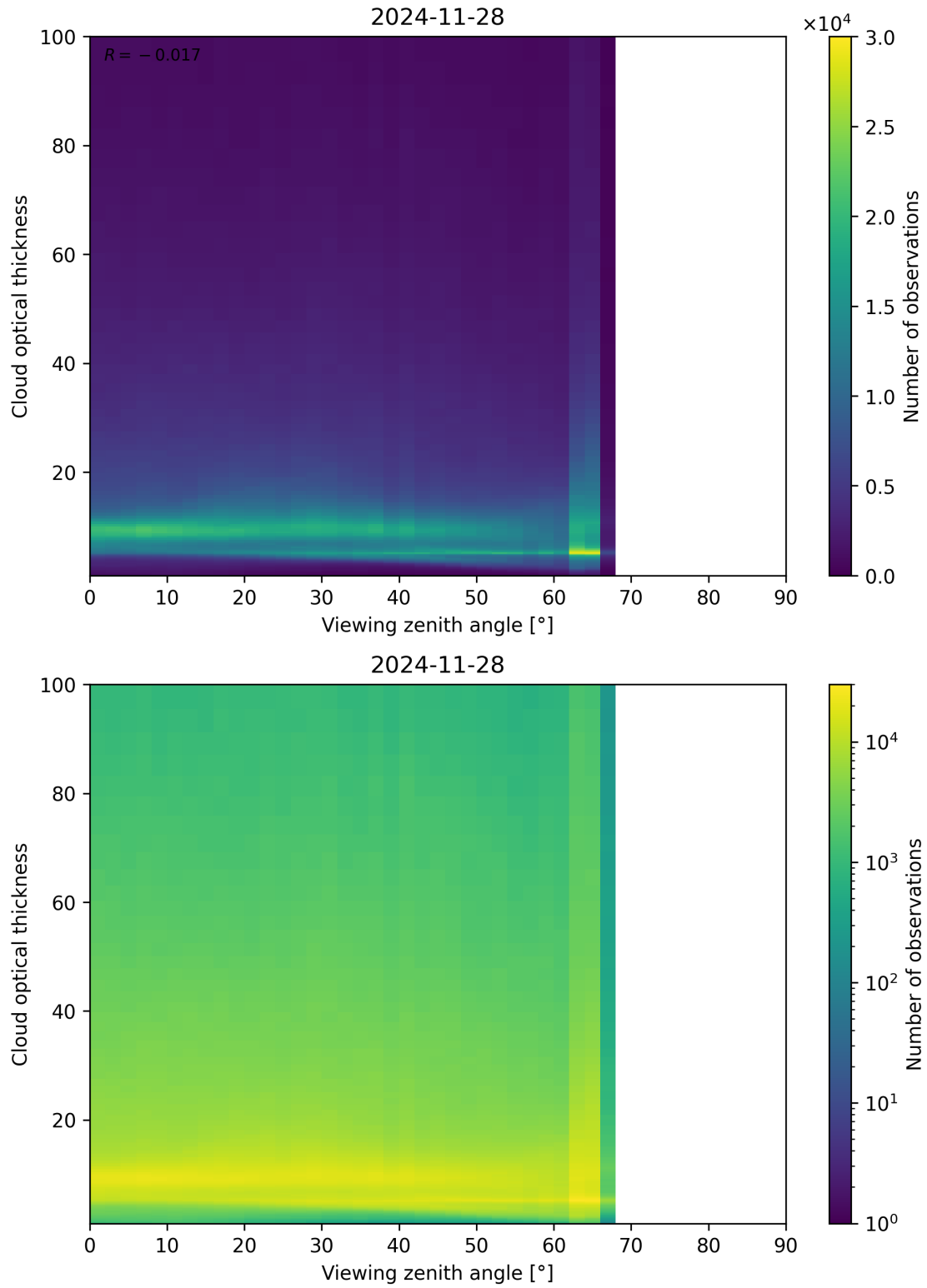
Figure 111: Scatter density plot of “Viewing zenith angle” against “Cloud optical thickness” for 2024-11-27 to 2024-11-29.
