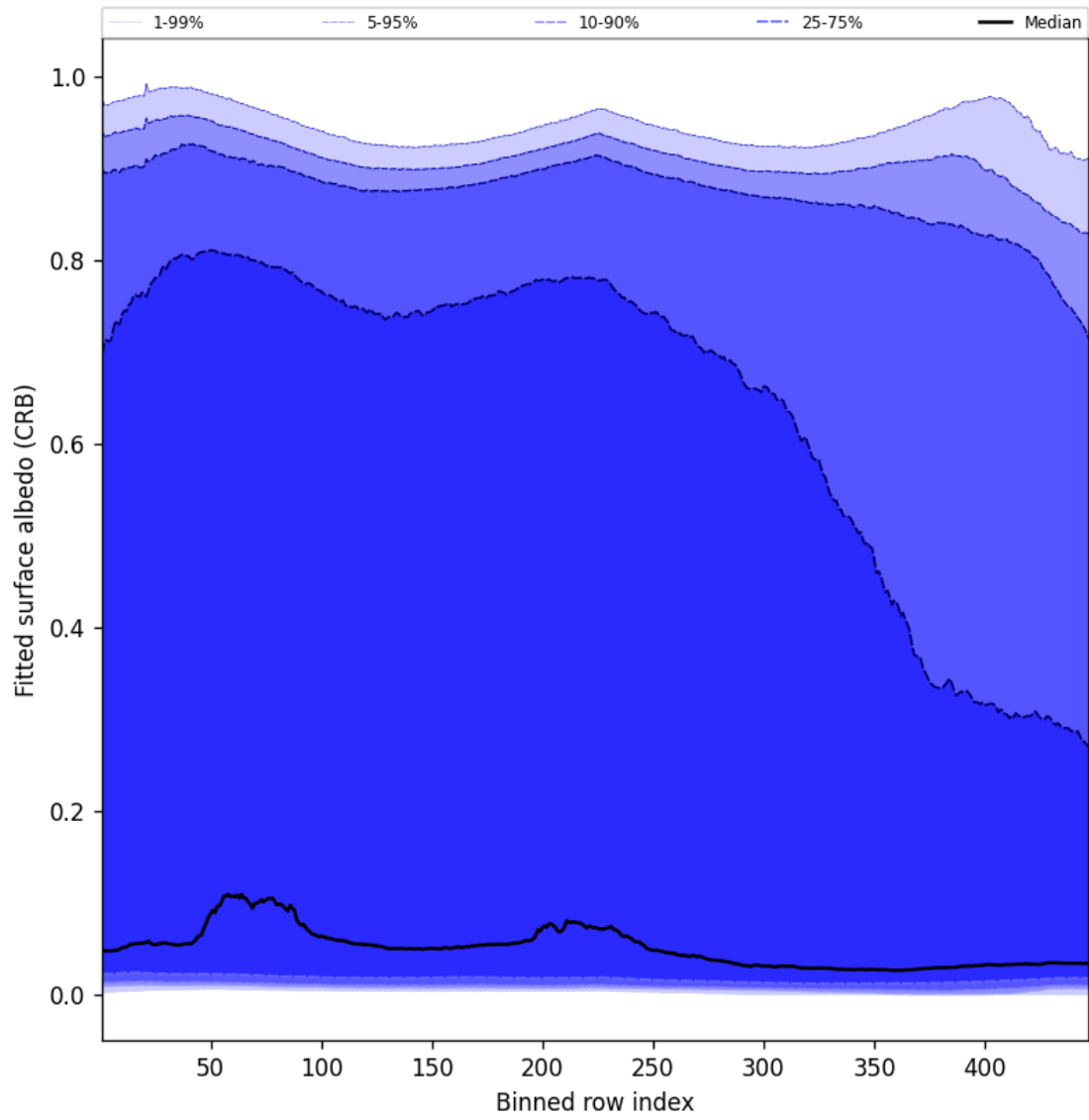
Figure 62: Along track statistics of “Fitted surface albedo (CRB)” for 2024-11-27 to 2024-11-29
