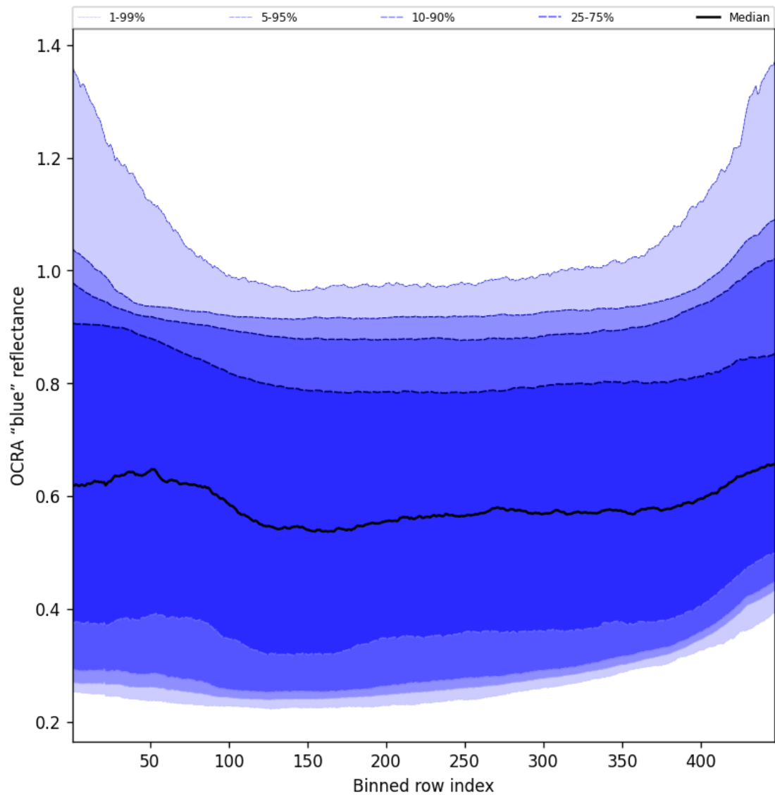
Figure 67: Along track statistics of “OCRA “blue” reflectance” for 2024-11-27 to 2024-11-29
