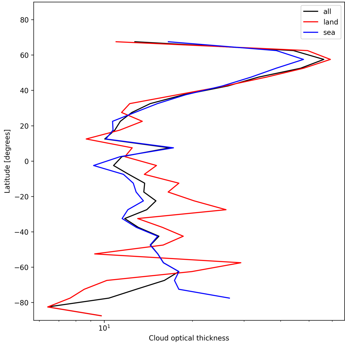
Figure 25: Zonal average of “Cloud optical thickness” for 2024-11-27 to 2024-11-29.
