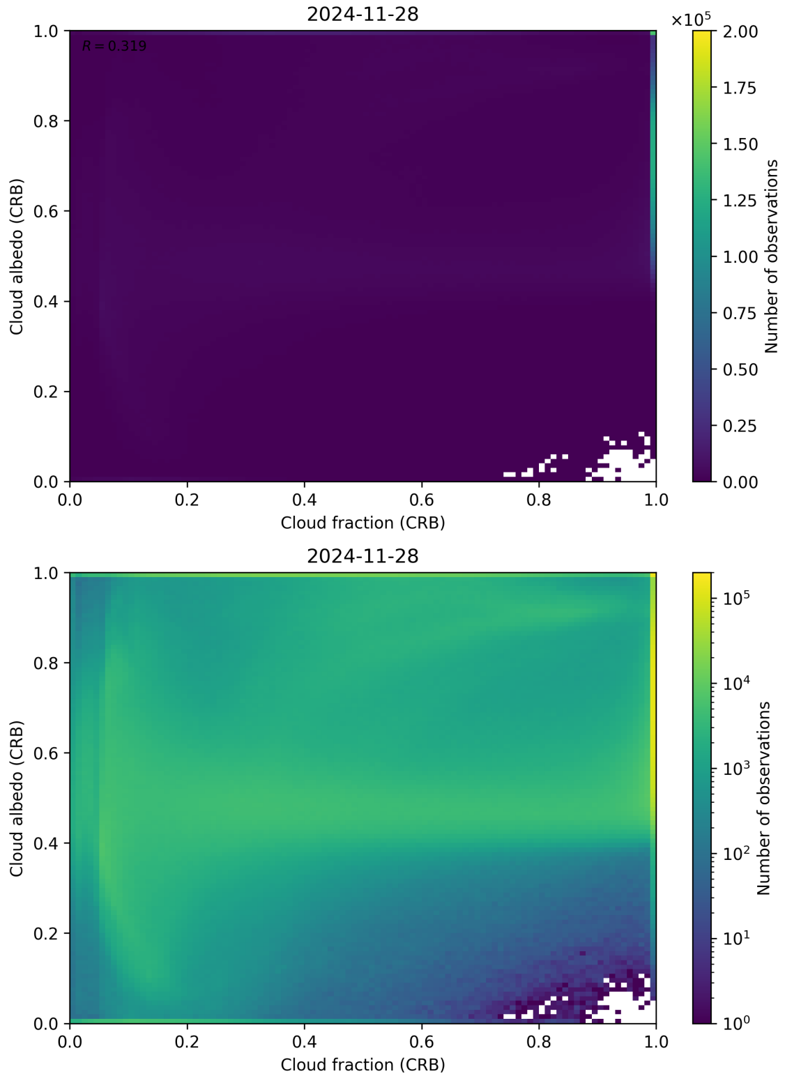
Figure 77: Scatter density plot of “Cloud fraction (CRB)” against “Cloud albedo (CRB)” for 2024-11-27 to 2024-11-29.
