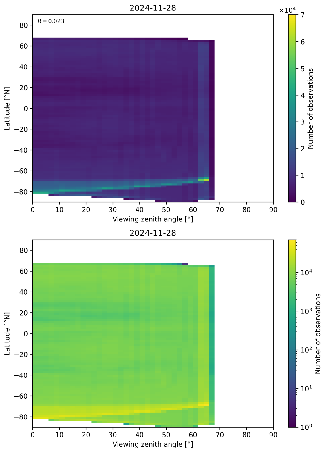
Figure 113: Scatter density plot of “Viewing zenith angle” against “Latitude” for 2024-11-27 to 2024-11-29.
