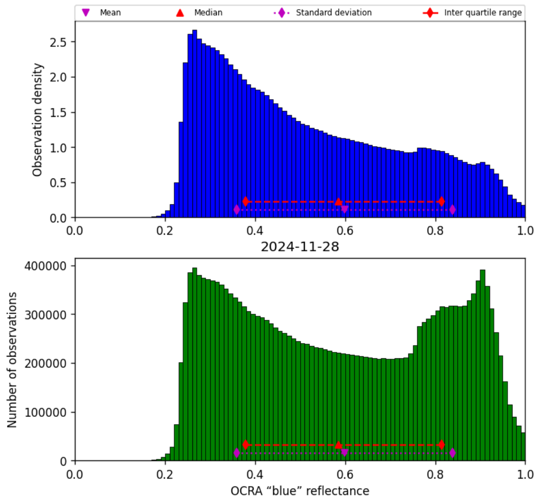
Figure 51: Histogram of “OCRA “blue” reflectance” for 2024-11-27 to 2024-11-29
