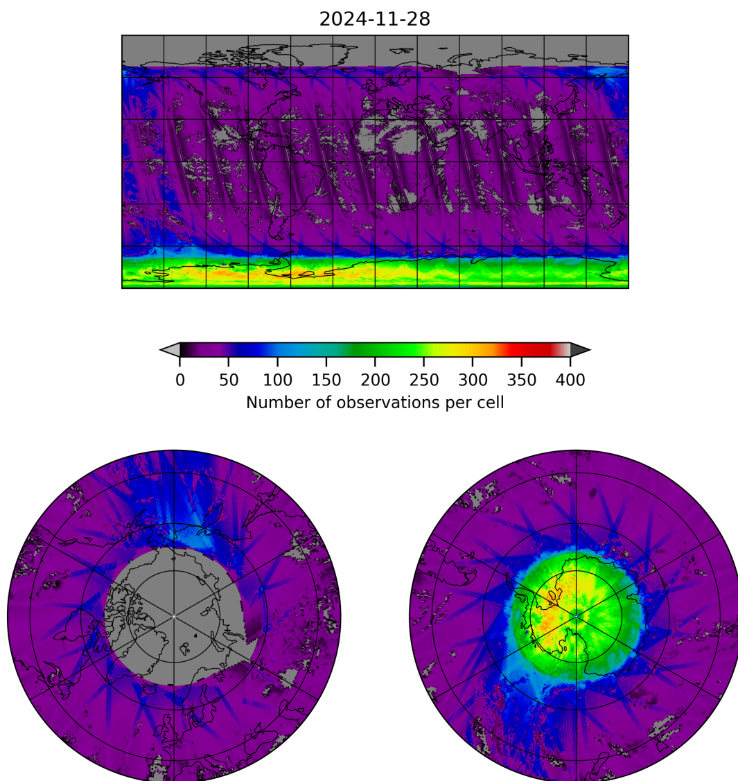
Figure 21: Map of the number of observations for 2024-11-27 to 2024-11-29
