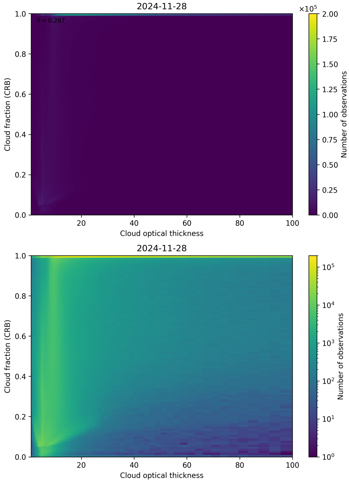
Figure 84: Scatter density plot of “Cloud optical thickness” against “Cloud fraction (CRB)” for 2024-11-27 to 2024-11-29.
