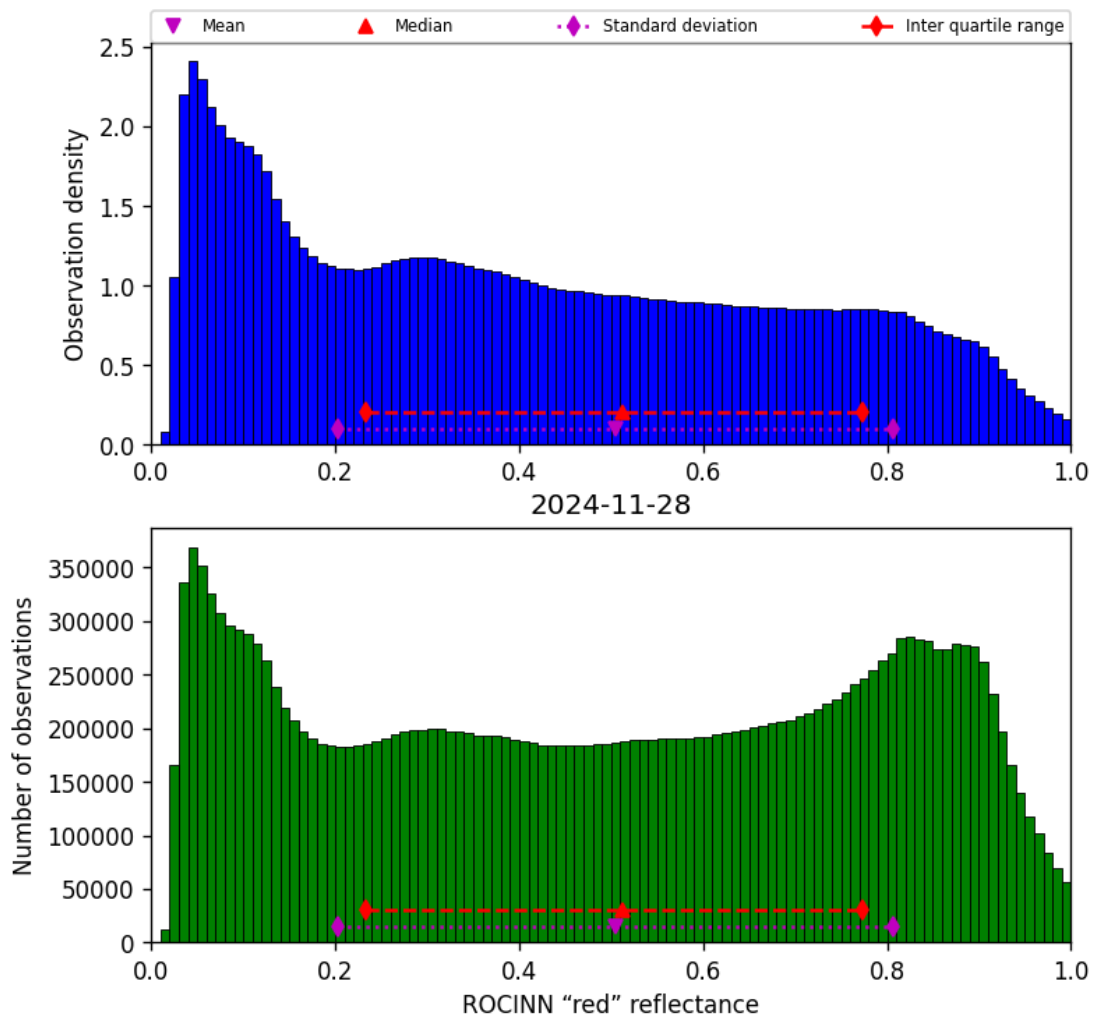
Figure 53: Histogram of “ROCINN “red” reflectance” for 2024-11-27 to 2024-11-29
