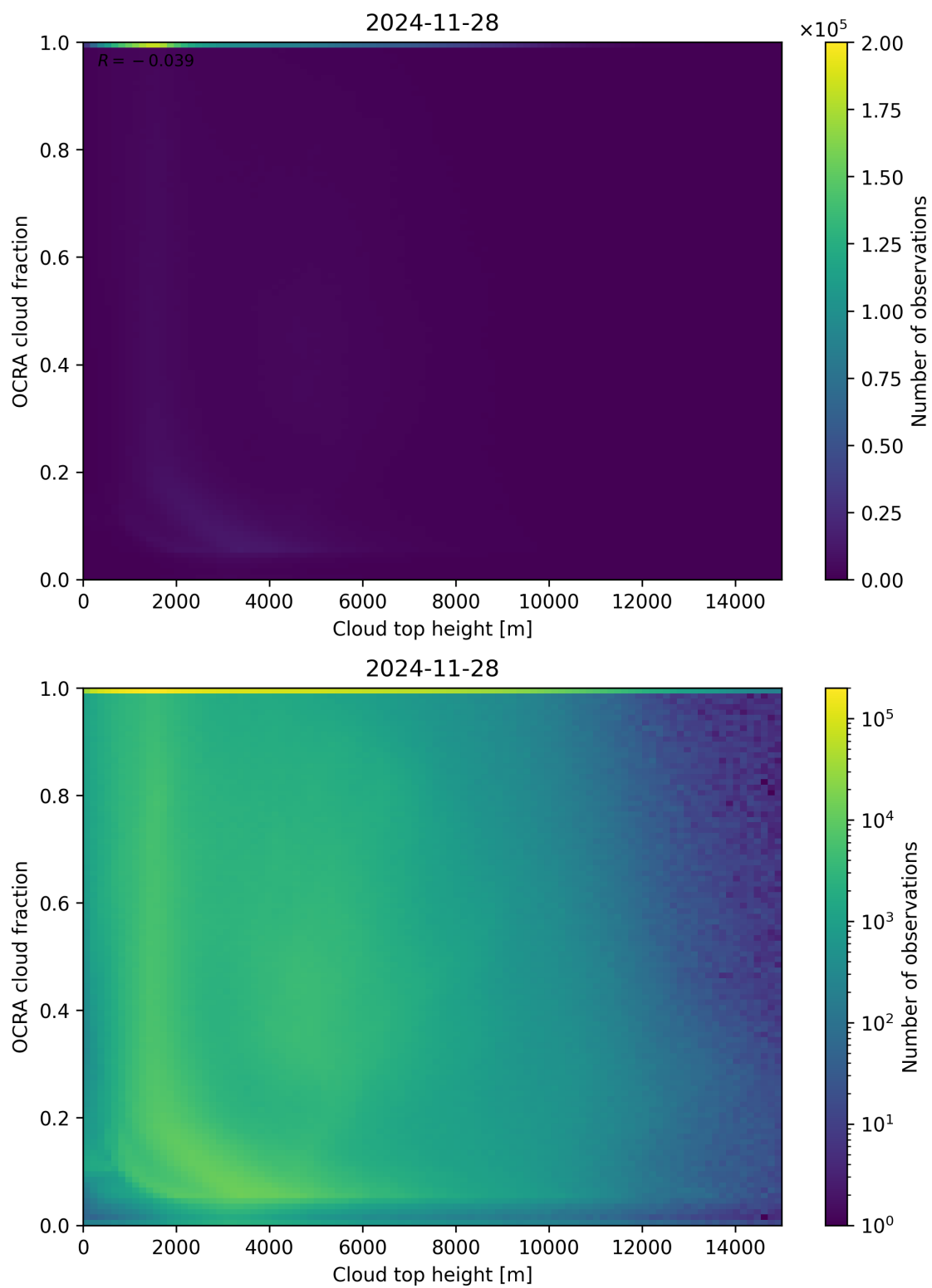
Figure 87: Scatter density plot of “Cloud top height” against “OCRA cloud fraction” for 2024-11-27 to 2024-11-29.
