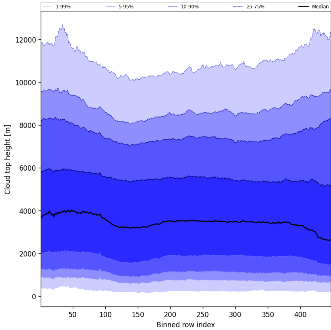
Figure 56: Along track statistics of “Cloud top height” for 2024-11-27 to 2024-11-29
