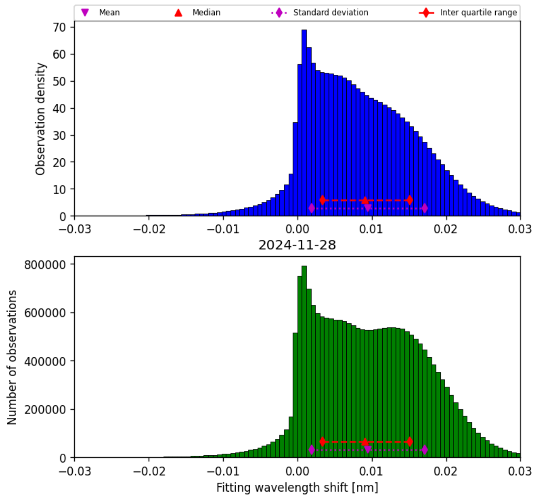
Figure 49: Histogram of “Fitting wavelength shift” for 2024-11-27 to 2024-11-29
