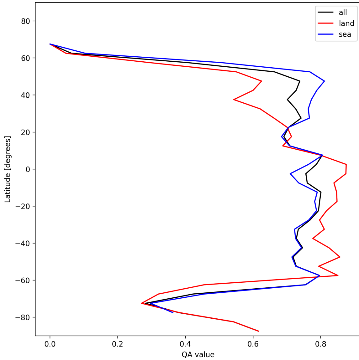
Figure 22: Zonal average of “QA value” for 2024-11-27 to 2024-11-29.
