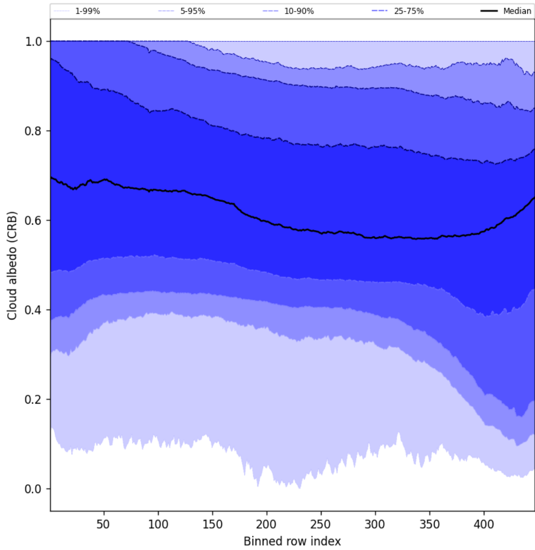
Figure 60: Along track statistics of “Cloud albedo (CRB)” for 2024-11-27 to 2024-11-29
