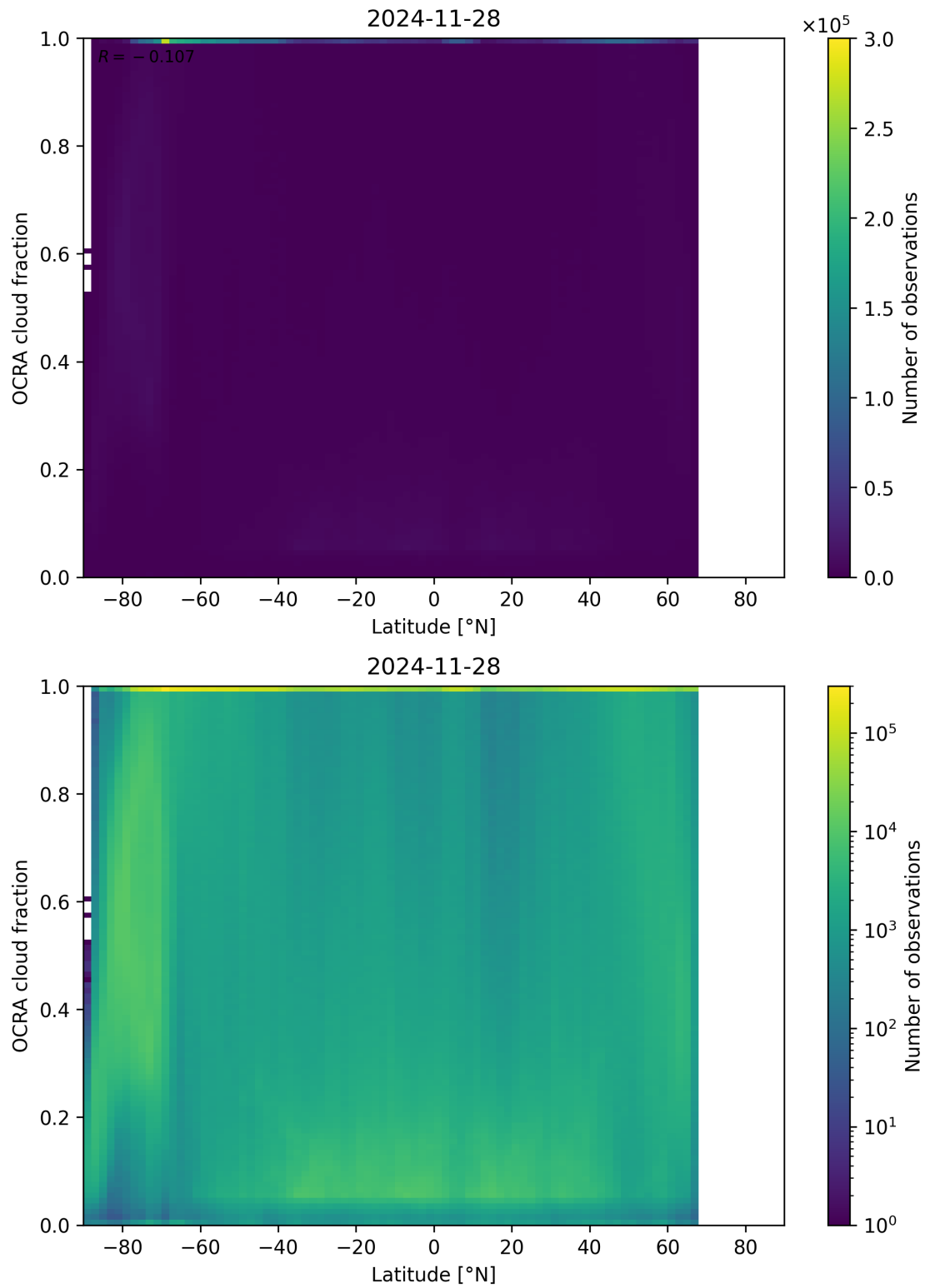
Figure 93: Scatter density plot of “Latitude” against “OCRA cloud fraction” for 2024-11-27 to 2024-11-29.
