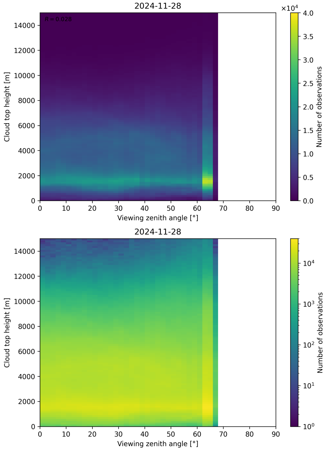
Figure 112: Scatter density plot of “Viewing zenith angle” against “Cloud top height” for 2024-11-27 to 2024-11-29.
