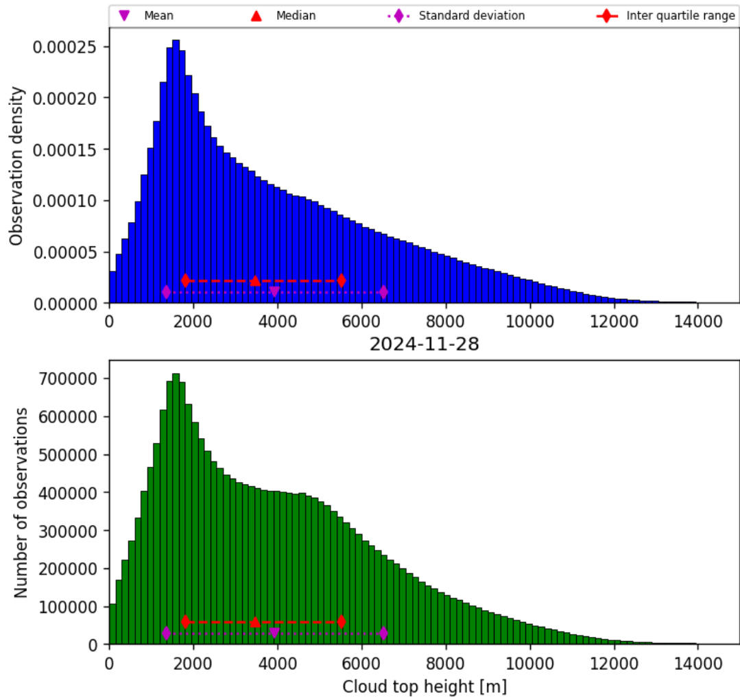
Figure 40: Histogram of “Cloud top height” for 2024-11-27 to 2024-11-29
