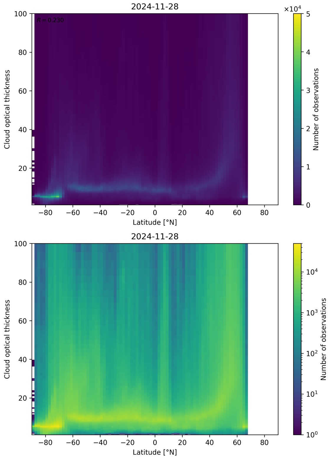
Figure 96: Scatter density plot of “Latitude” against “Cloud optical thickness” for 2024-11-27 to 2024-11-29.
