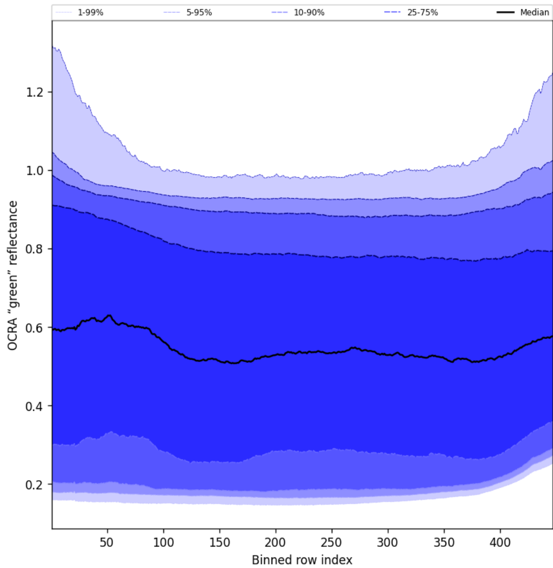
Figure 68: Along track statistics of “OCRA “green” reflectance” for 2024-11-27 to 2024-11-29
