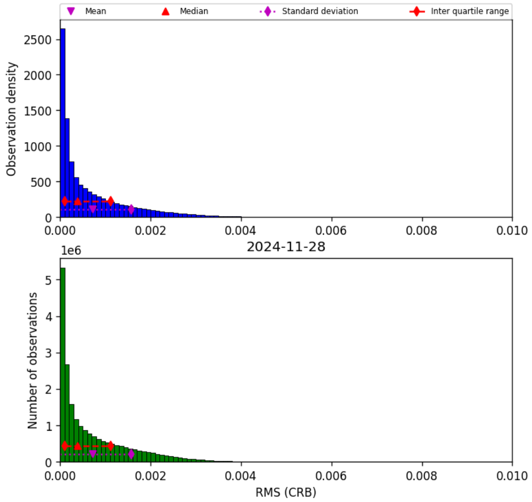
Figure 48: Histogram of “RMS (CRB)” for 2024-11-27 to 2024-11-29
