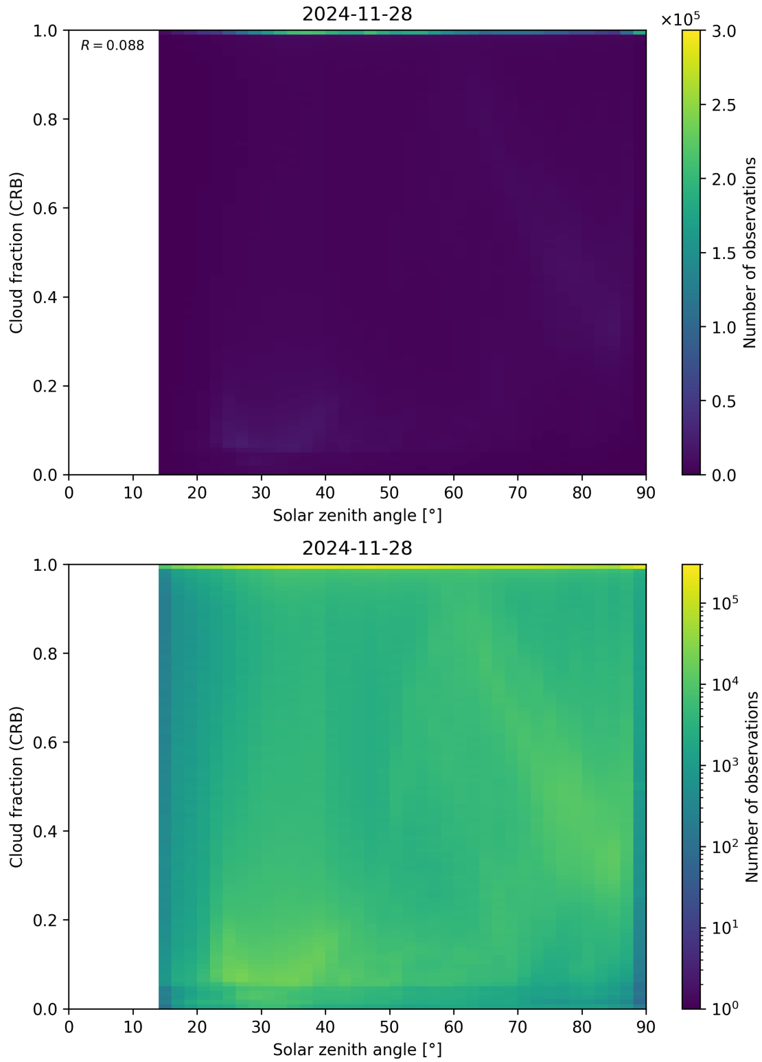
Figure 101: Scatter density plot of “Solar zenith angle” against “Cloud fraction (CRB)” for 2024-11-27 to 2024-11-29.
