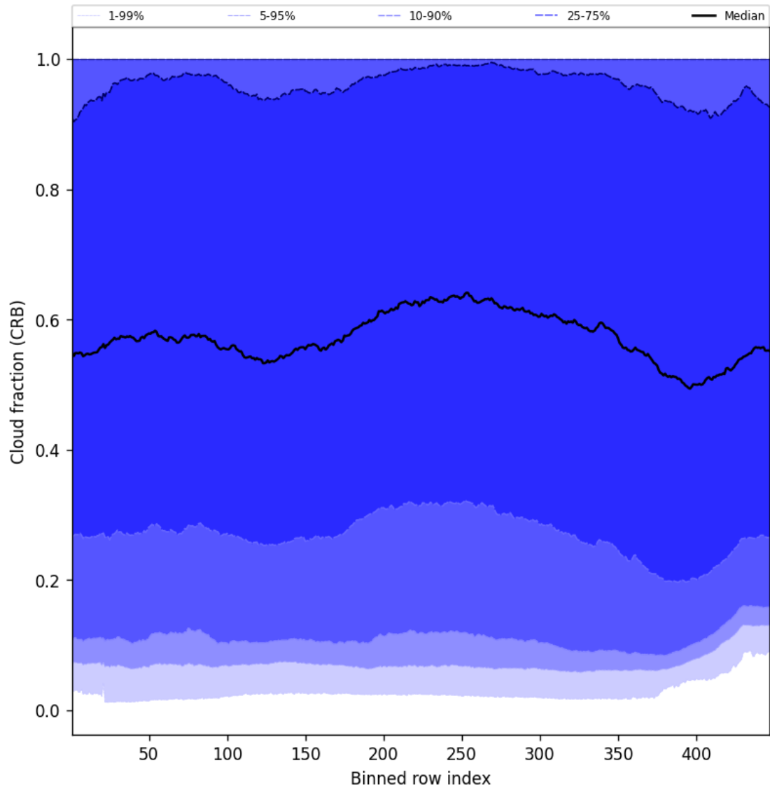
Figure 58: Along track statistics of “Cloud fraction (CRB)” for 2024-11-27 to 2024-11-29
