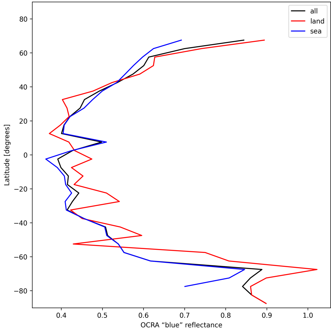
Figure 35: Zonal average of “OCRA “blue” reflectance” for 2024-11-27 to 2024-11-29.
