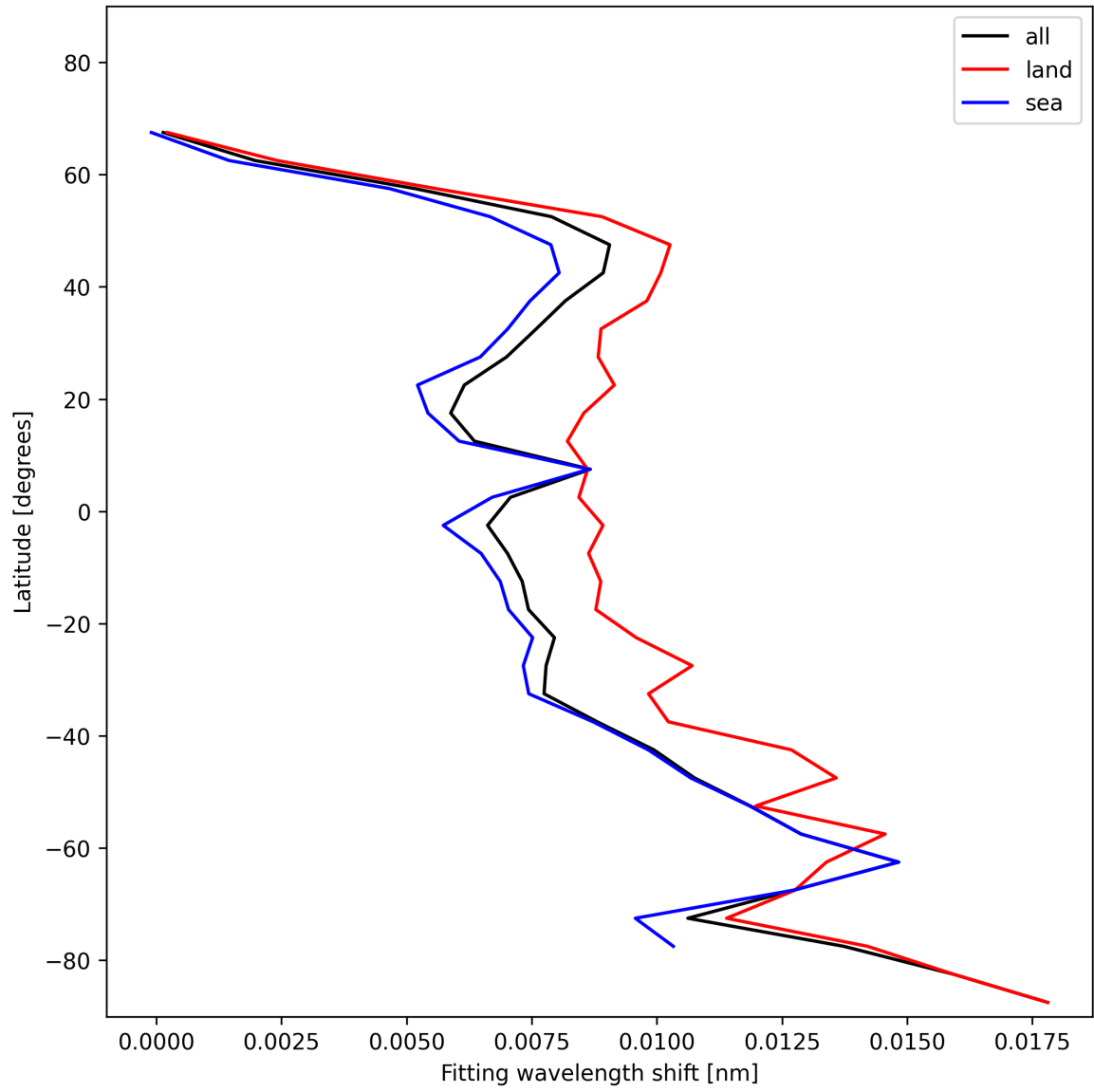
Figure 33: Zonal average of “Fitting wavelength shift” for 2024-11-27 to 2024-11-29.
