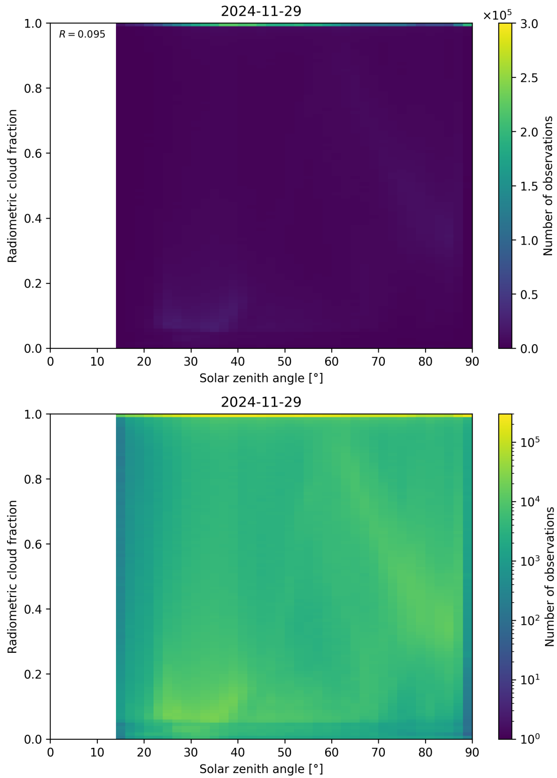
Figure 99: Scatter density plot of “Solar zenith angle” against “Radiometric cloud fraction” for 2024-11-28 to 2024-11-30.
