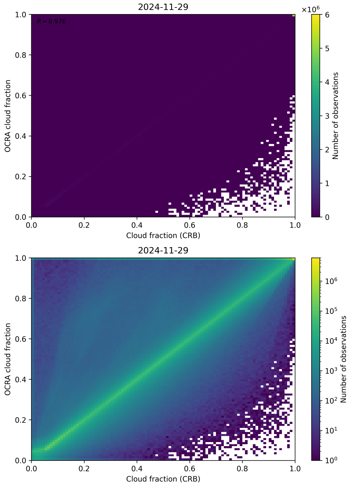
Figure 78: Scatter density plot of “Cloud fraction (CRB)” against “OCRA cloud fraction” for 2024-11-28 to 2024-11-30.
