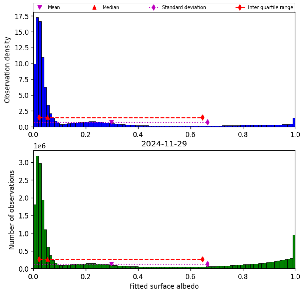
Figure 45: Histogram of “Fitted surface albedo” for 2024-11-28 to 2024-11-30
