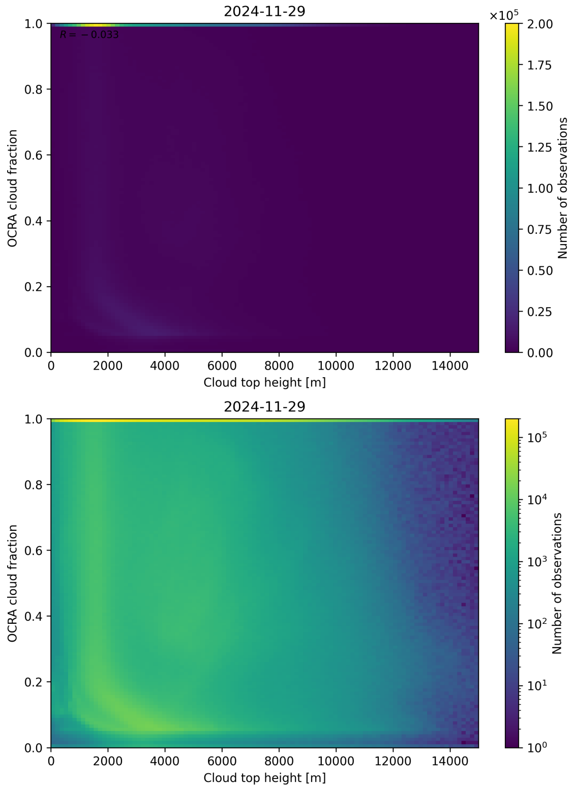
Figure 87: Scatter density plot of “Cloud top height” against “OCRA cloud fraction” for 2024-11-28 to 2024-11-30.
