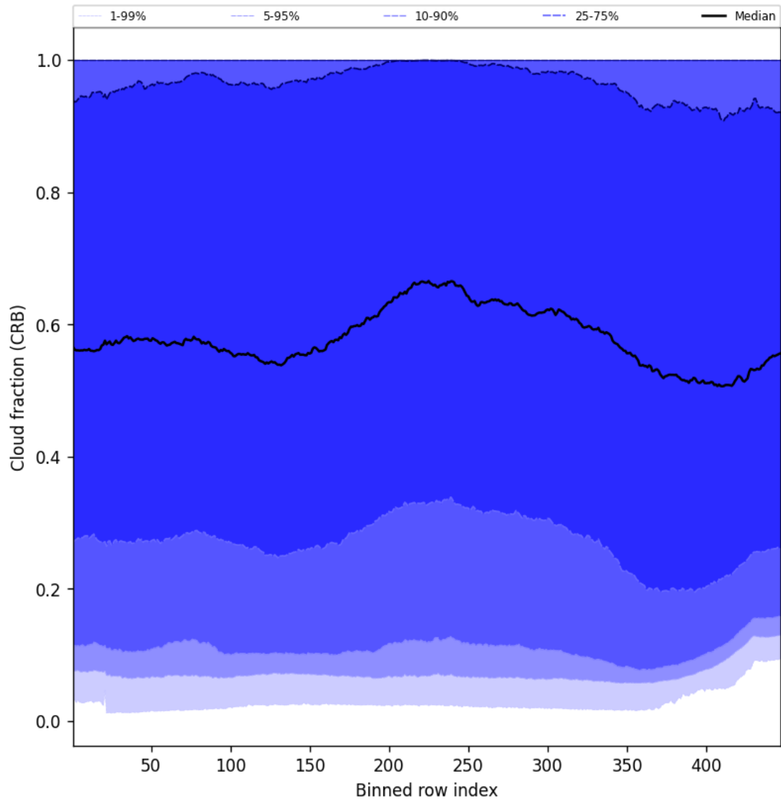
Figure 58: Along track statistics of “Cloud fraction (CRB)” for 2024-11-28 to 2024-11-30
