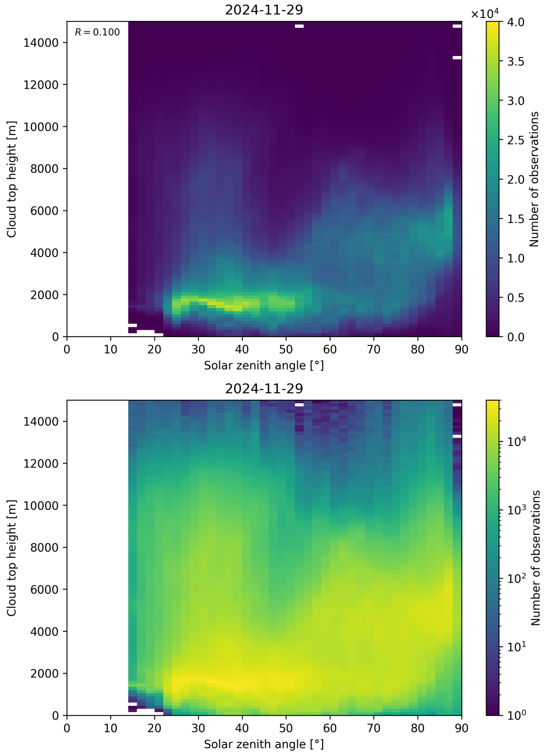
Figure 104: Scatter density plot of “Solar zenith angle” against “Cloud top height” for 2024-11-28 to 2024-11-30.
