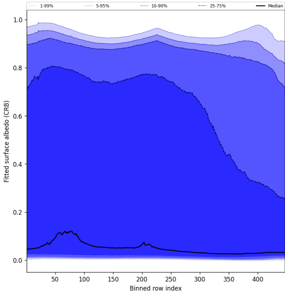
Figure 62: Along track statistics of “Fitted surface albedo (CRB)” for 2024-11-28 to 2024-11-30
