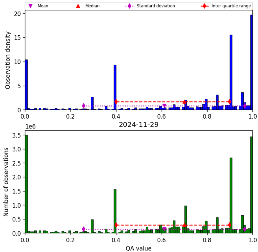
Figure 38: Histogram of “QA value” for 2024-11-28 to 2024-11-30
