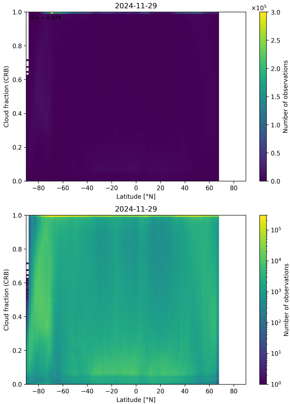
Figure 94: Scatter density plot of “Latitude” against “Cloud fraction (CRB)” for 2024-11-28 to 2024-11-30.
