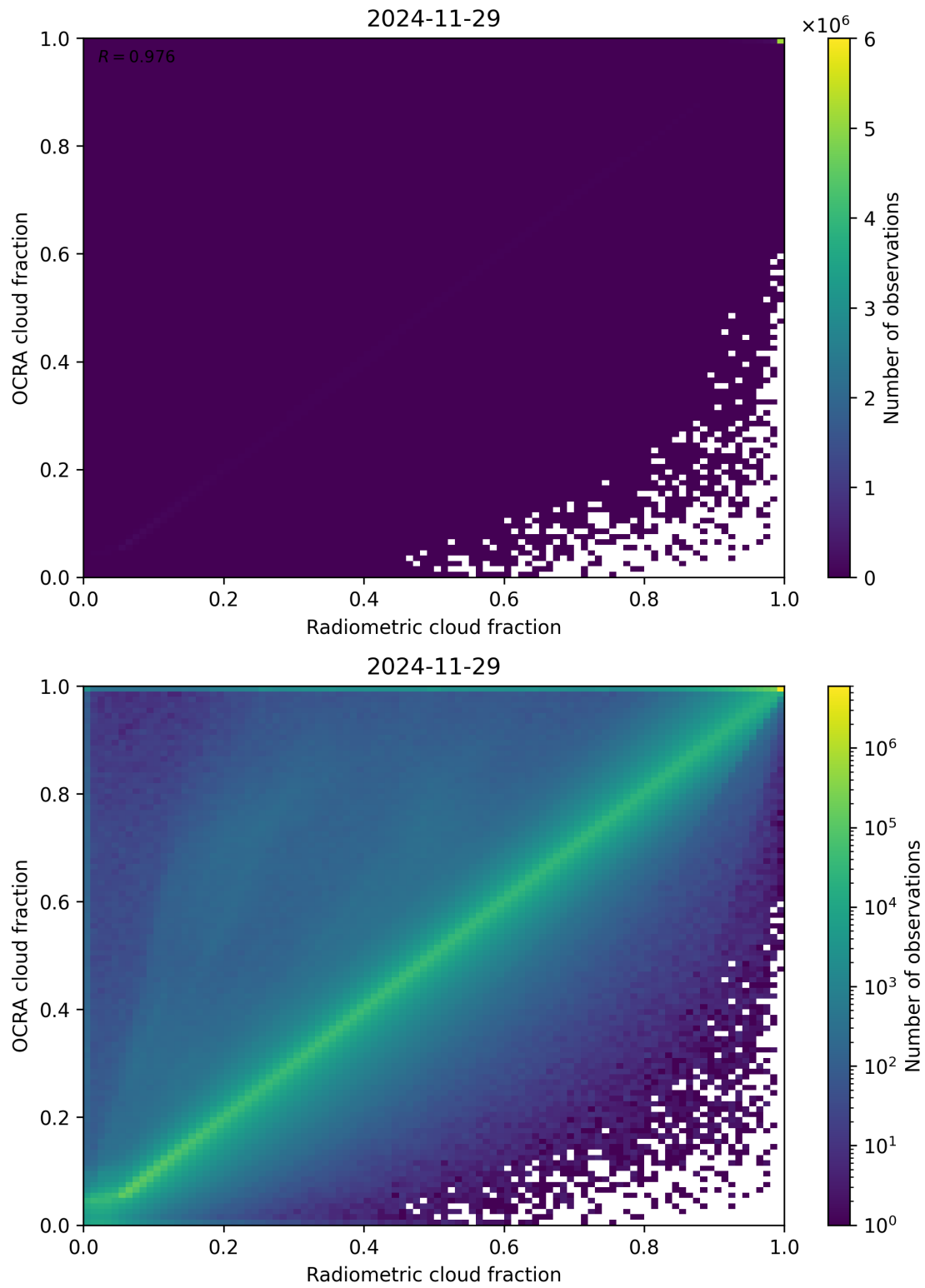
Figure 72: Scatter density plot of “Radiometric cloud fraction” against “OCRA cloud fraction” for 2024-11-28 to 2024-11-30.
