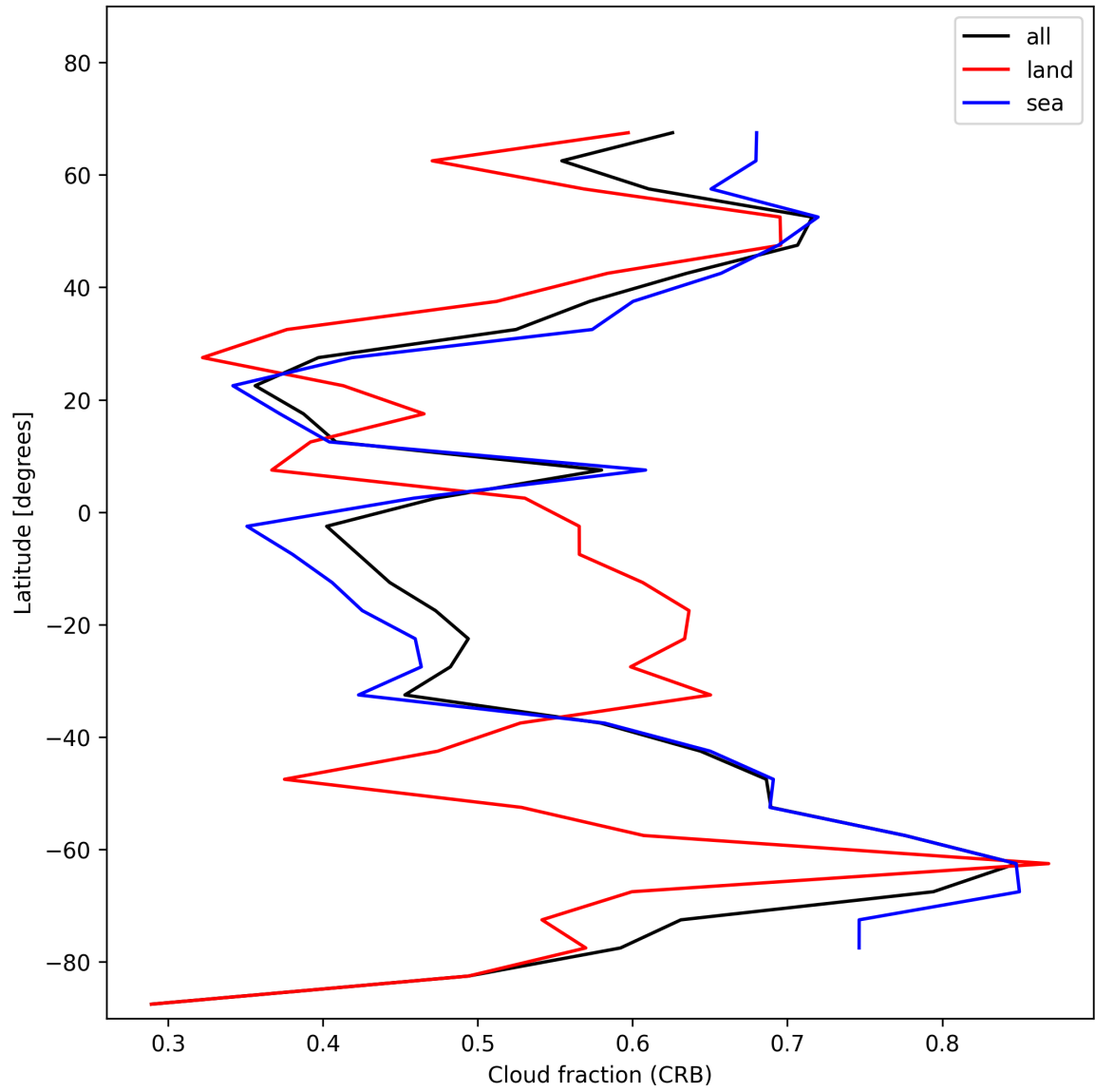
Figure 26: Zonal average of “Cloud fraction (CRB)” for 2024-11-28 to 2024-11-30.
