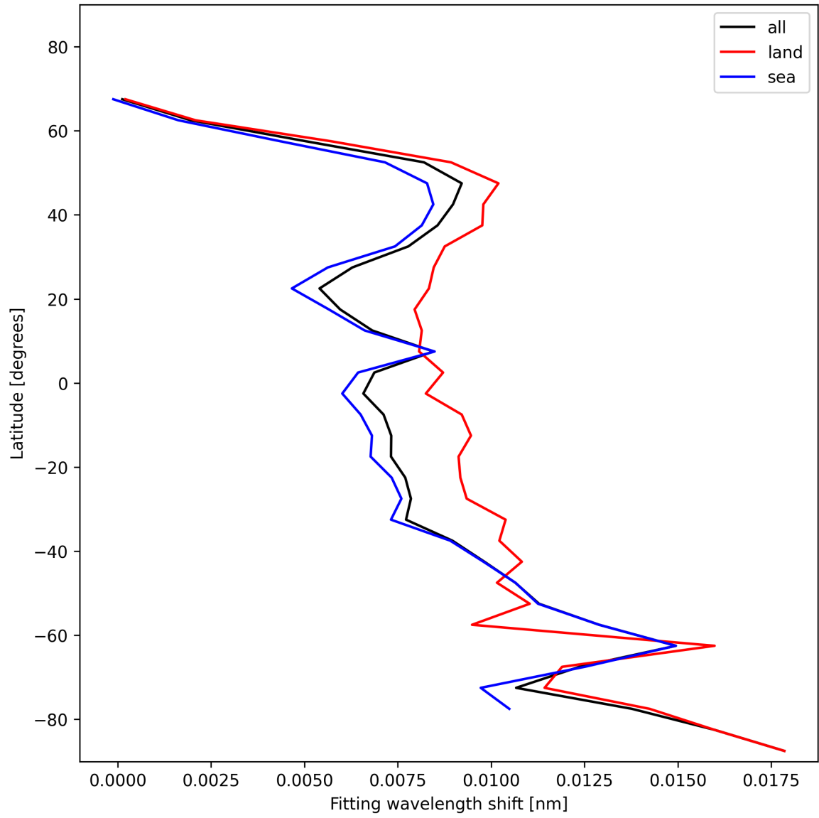
Figure 33: Zonal average of “Fitting wavelength shift” for 2024-11-28 to 2024-11-30.
