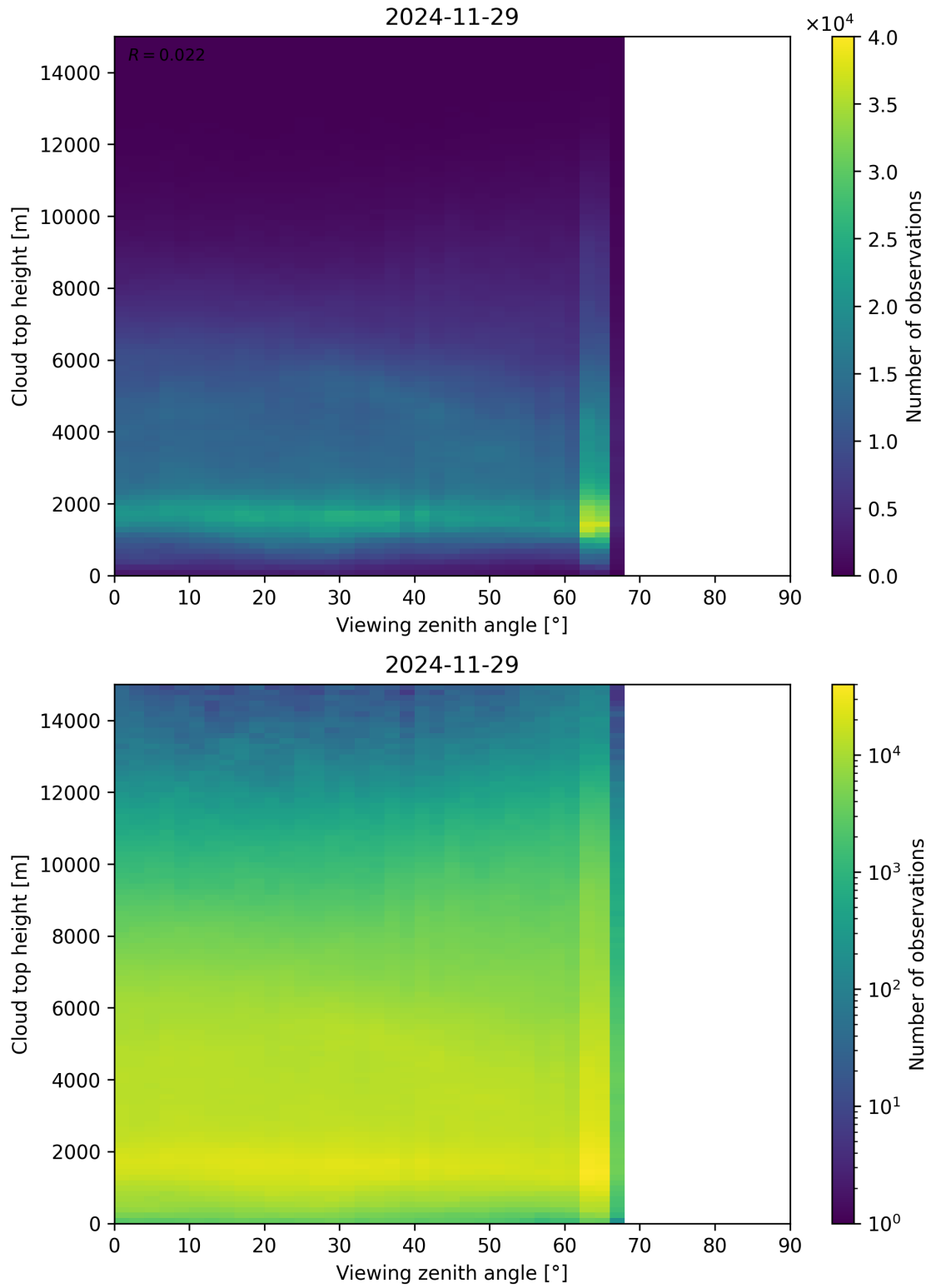
Figure 112: Scatter density plot of “Viewing zenith angle” against “Cloud top height” for 2024-11-28 to 2024-11-30.
