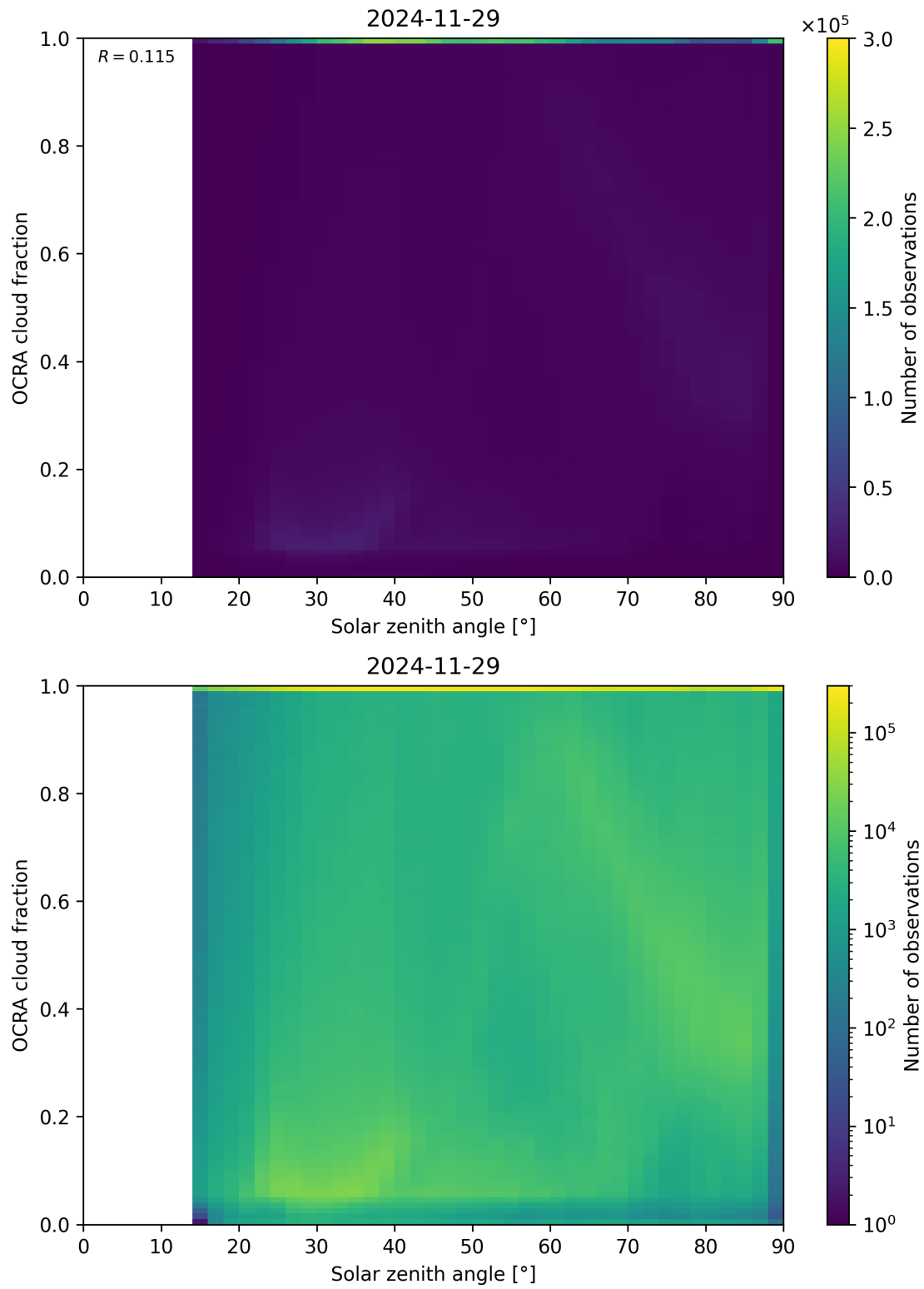
Figure 100: Scatter density plot of “Solar zenith angle” against “OCRA cloud fraction” for 2024-11-28 to 2024-11-30.
