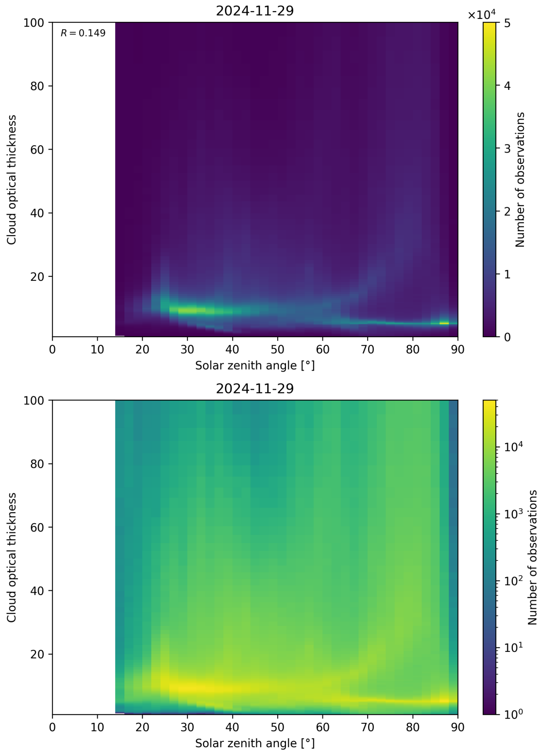
Figure 103: Scatter density plot of “Solar zenith angle” against “Cloud optical thickness” for 2024-11-28 to 2024-11-30.
