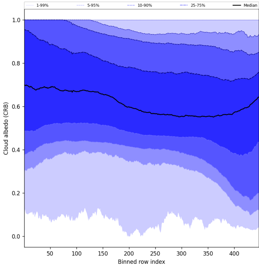
Figure 60: Along track statistics of “Cloud albedo (CRB)” for 2024-11-28 to 2024-11-30
