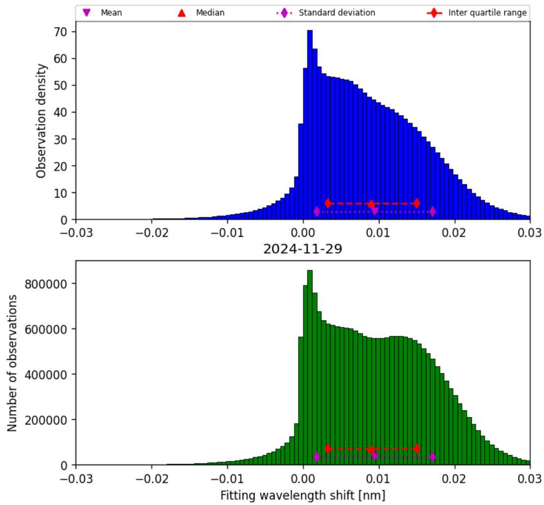
Figure 49: Histogram of “Fitting wavelength shift” for 2024-11-28 to 2024-11-30
