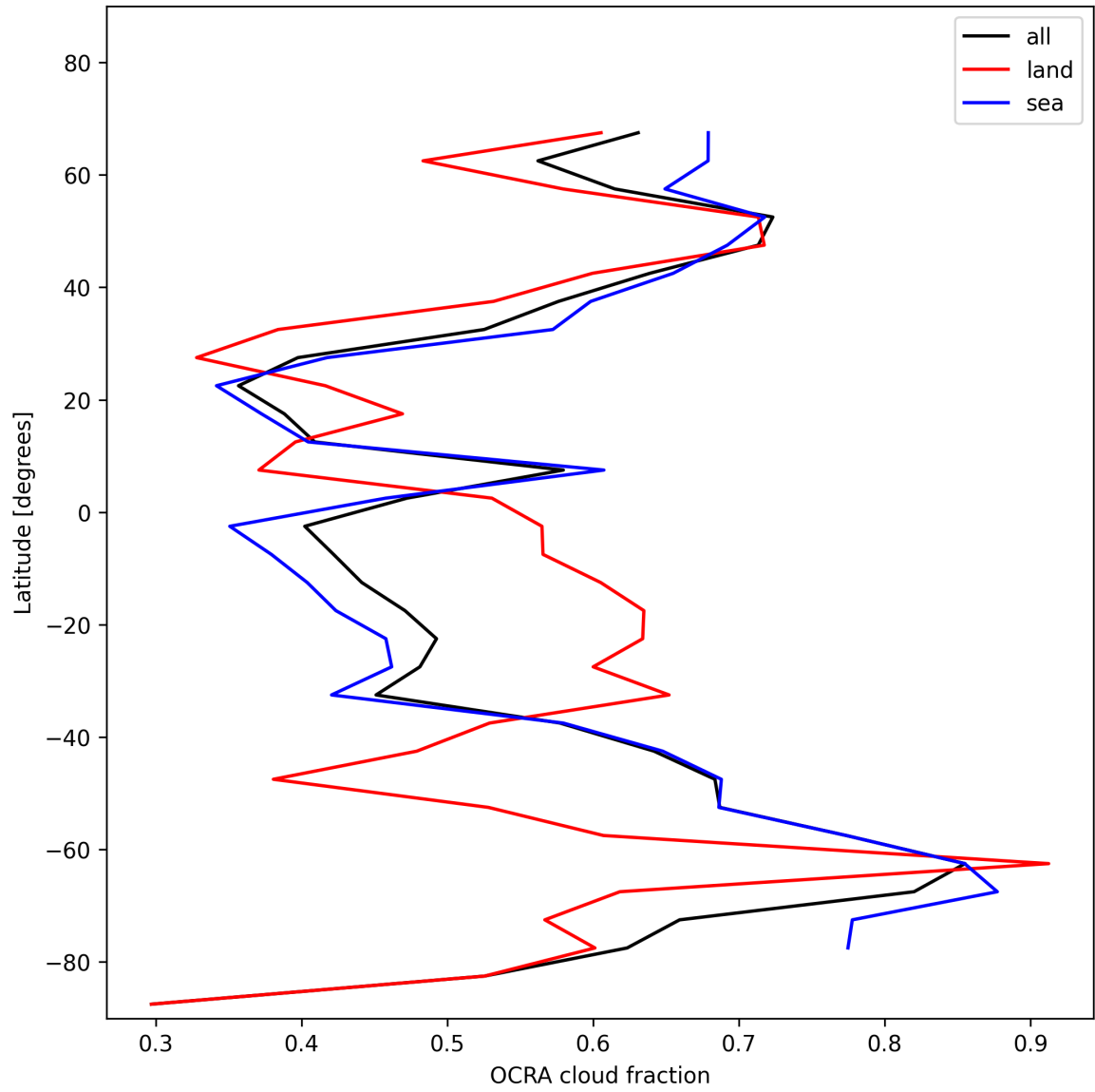
Figure 34: Zonal average of “OCRA cloud fraction” for 2024-11-28 to 2024-11-30.
