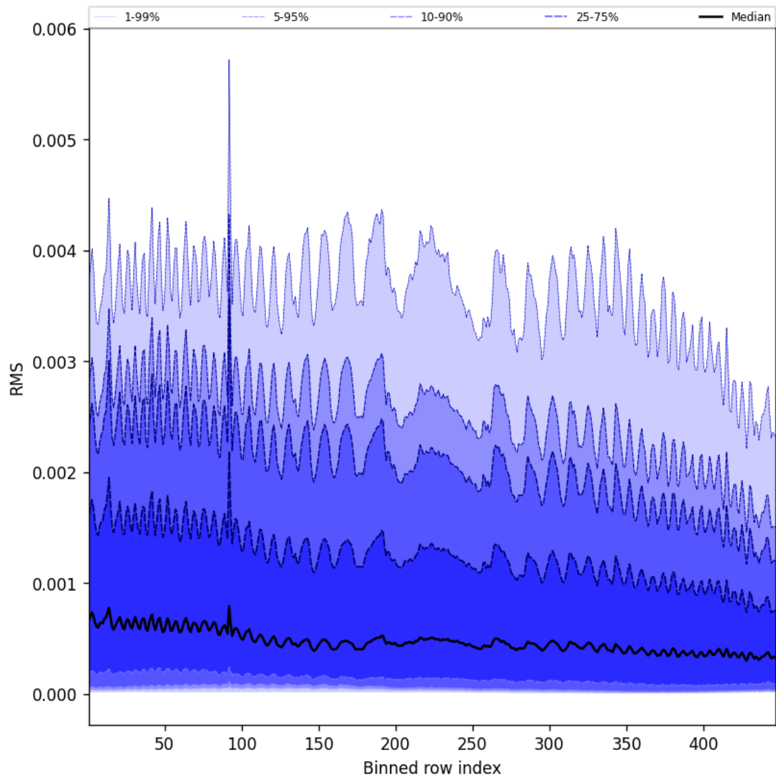
Figure 63: Along track statistics of “RMS” for 2024-11-28 to 2024-11-30
