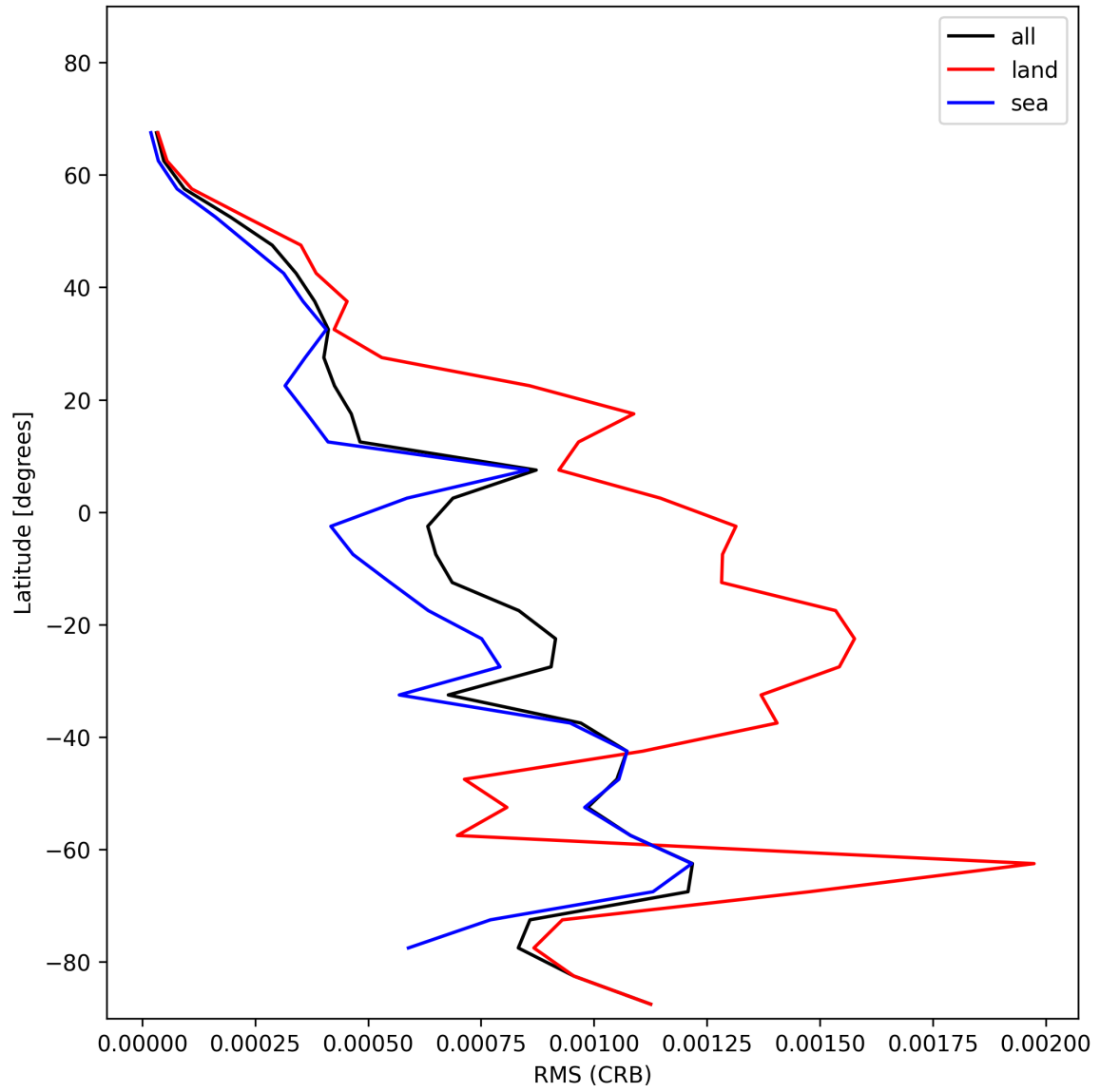
Figure 32: Zonal average of “RMS (CRB)” for 2024-11-28 to 2024-11-30.
