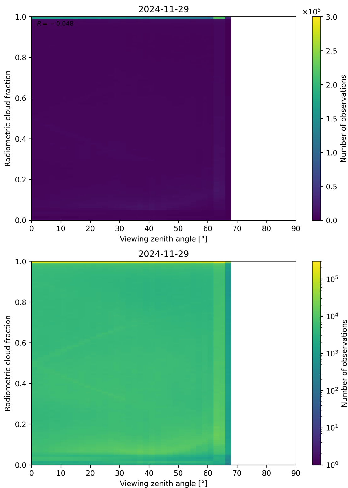
Figure 107: Scatter density plot of “Viewing zenith angle” against “Radiometric cloud fraction” for 2024-11-28 to 2024-11-30.
