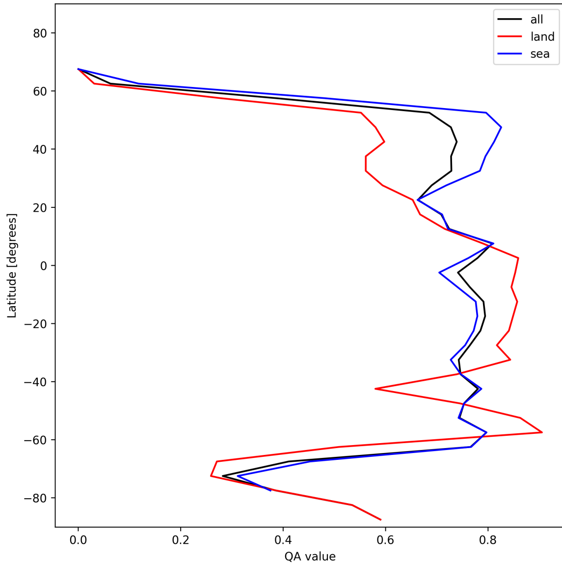
Figure 22: Zonal average of “QA value” for 2024-11-28 to 2024-11-30.
