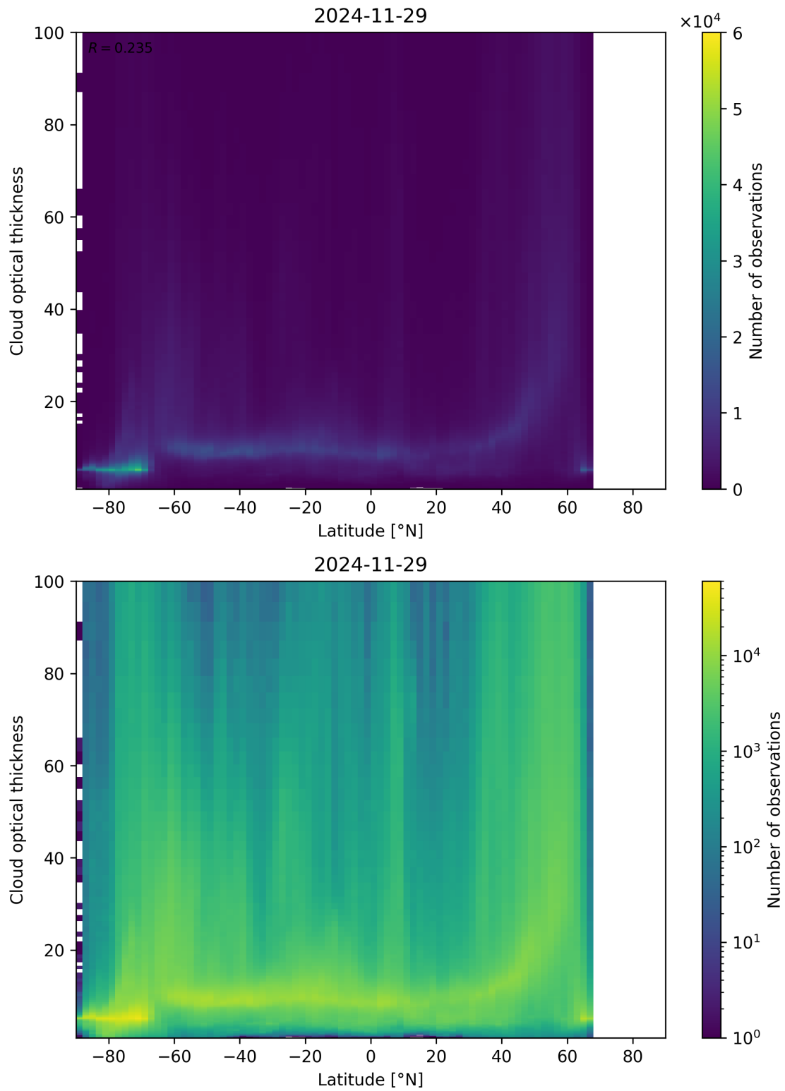
Figure 96: Scatter density plot of “Latitude” against “Cloud optical thickness” for 2024-11-28 to 2024-11-30.
