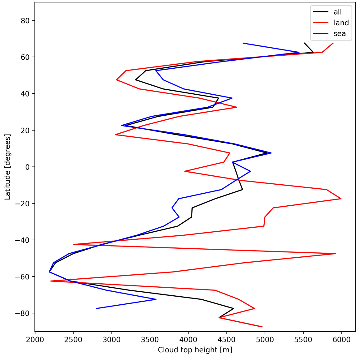
Figure 24: Zonal average of “Cloud top height” for 2024-11-28 to 2024-11-30.
