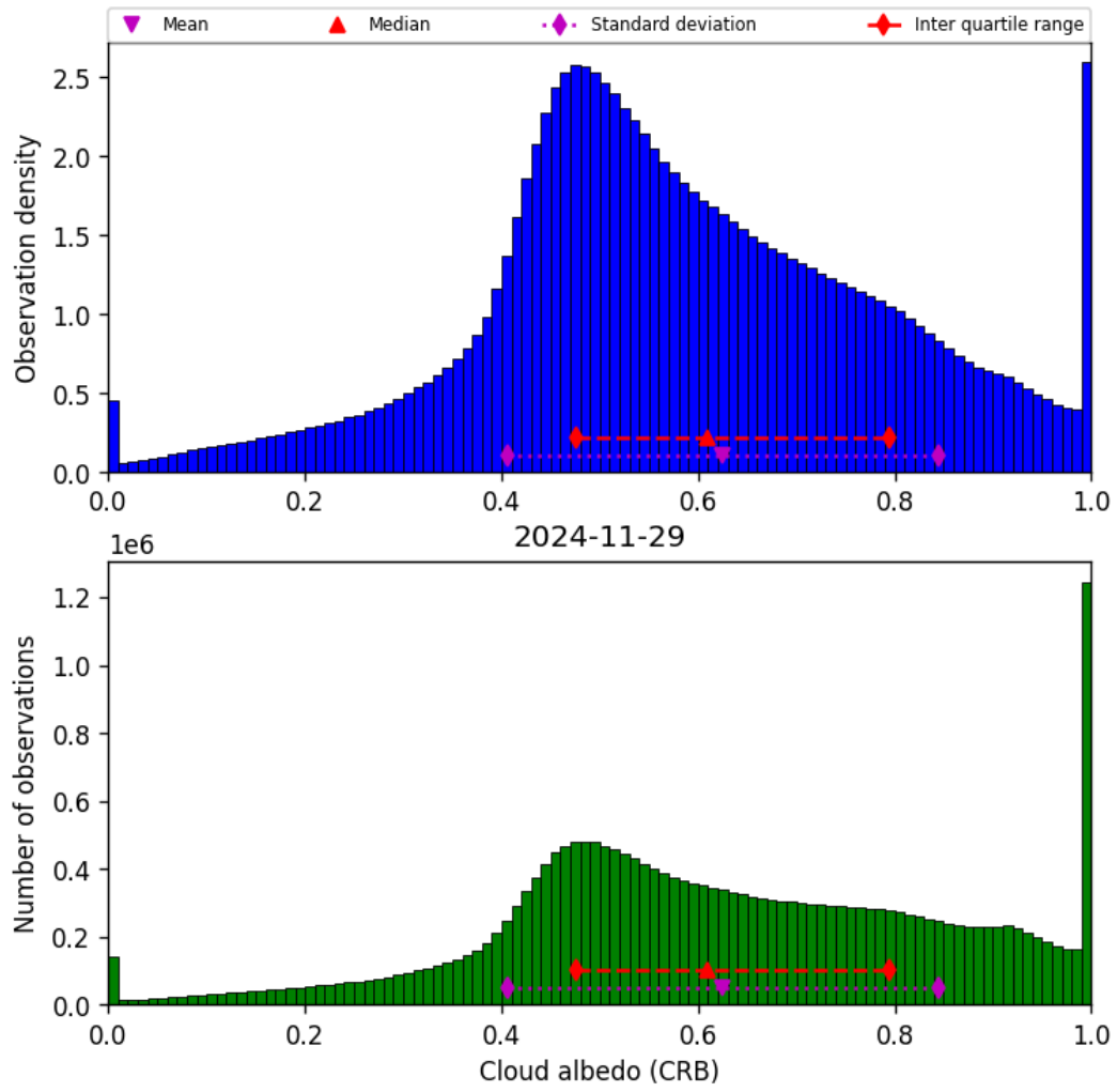
Figure 44: Histogram of “Cloud albedo (CRB)” for 2024-11-28 to 2024-11-30
