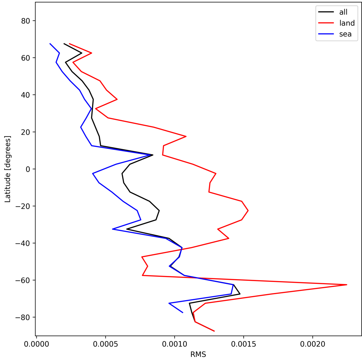
Figure 31: Zonal average of “RMS” for 2024-11-28 to 2024-11-30.
