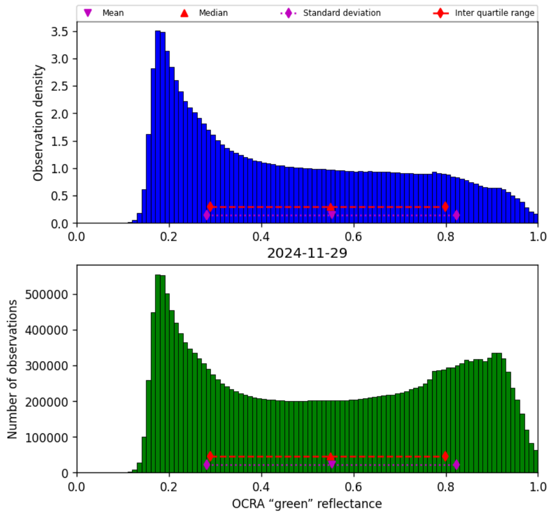
Figure 52: Histogram of “OCRA “green” reflectance” for 2024-11-28 to 2024-11-30
