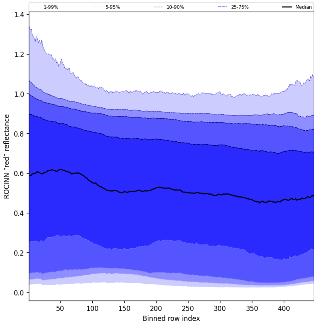
Figure 69: Along track statistics of “ROCINN “red” reflectance” for 2024-11-28 to 2024-11-30
