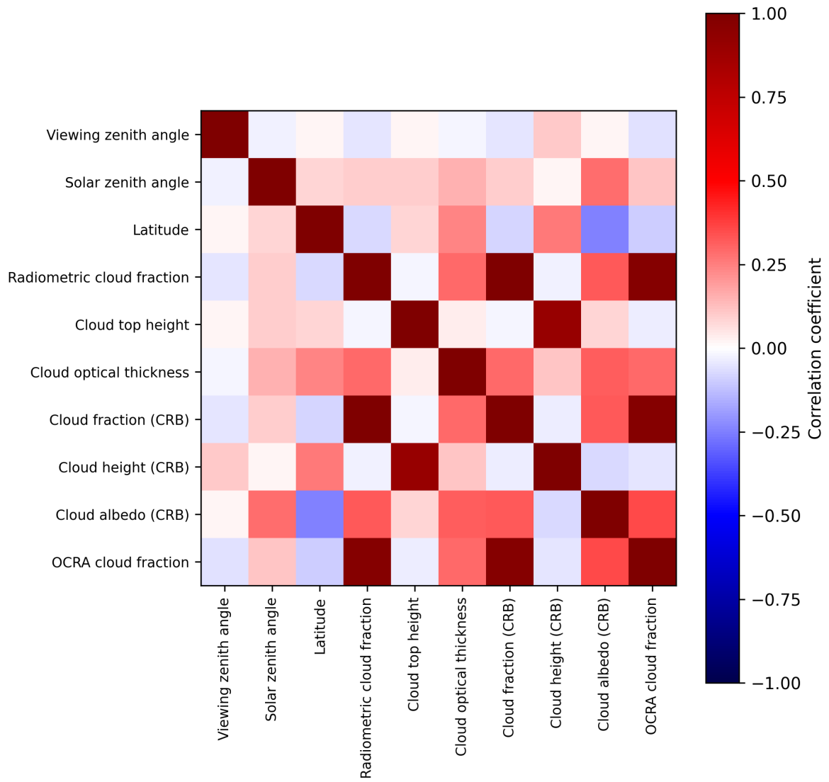
Figure 2: Map of correlation matrix for 2024-11-28 to 2024-11-30.
