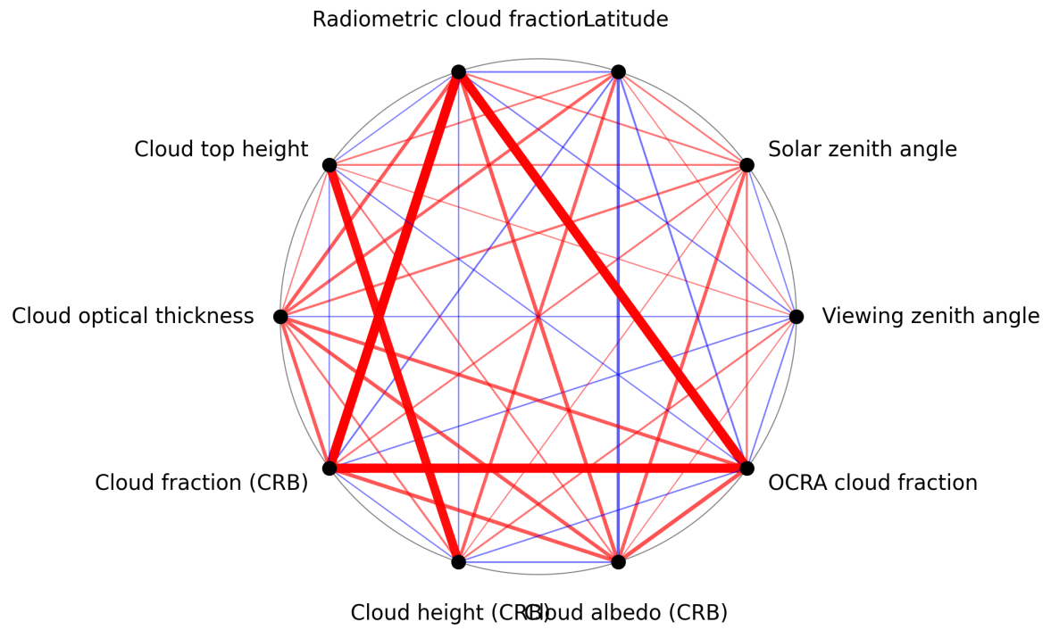
Figure 1: Map of correlation graph for 2024-11-28 to 2024-11-30.
