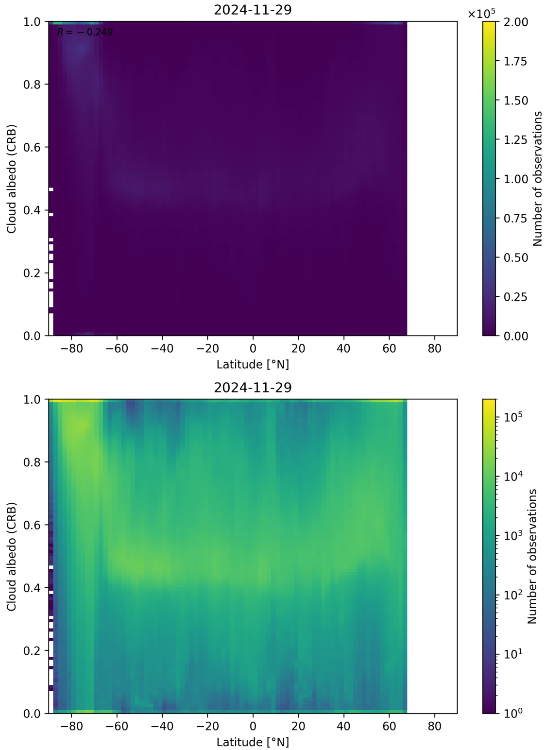
Figure 91: Scatter density plot of “Latitude” against “Cloud albedo (CRB)” for 2024-11-28 to 2024-11-30.
