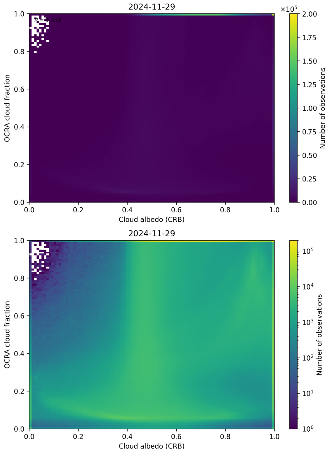
Figure 70: Scatter density plot of “Cloud albedo (CRB)” against “OCRA cloud fraction” for 2024-11-28 to 2024-11-30.
