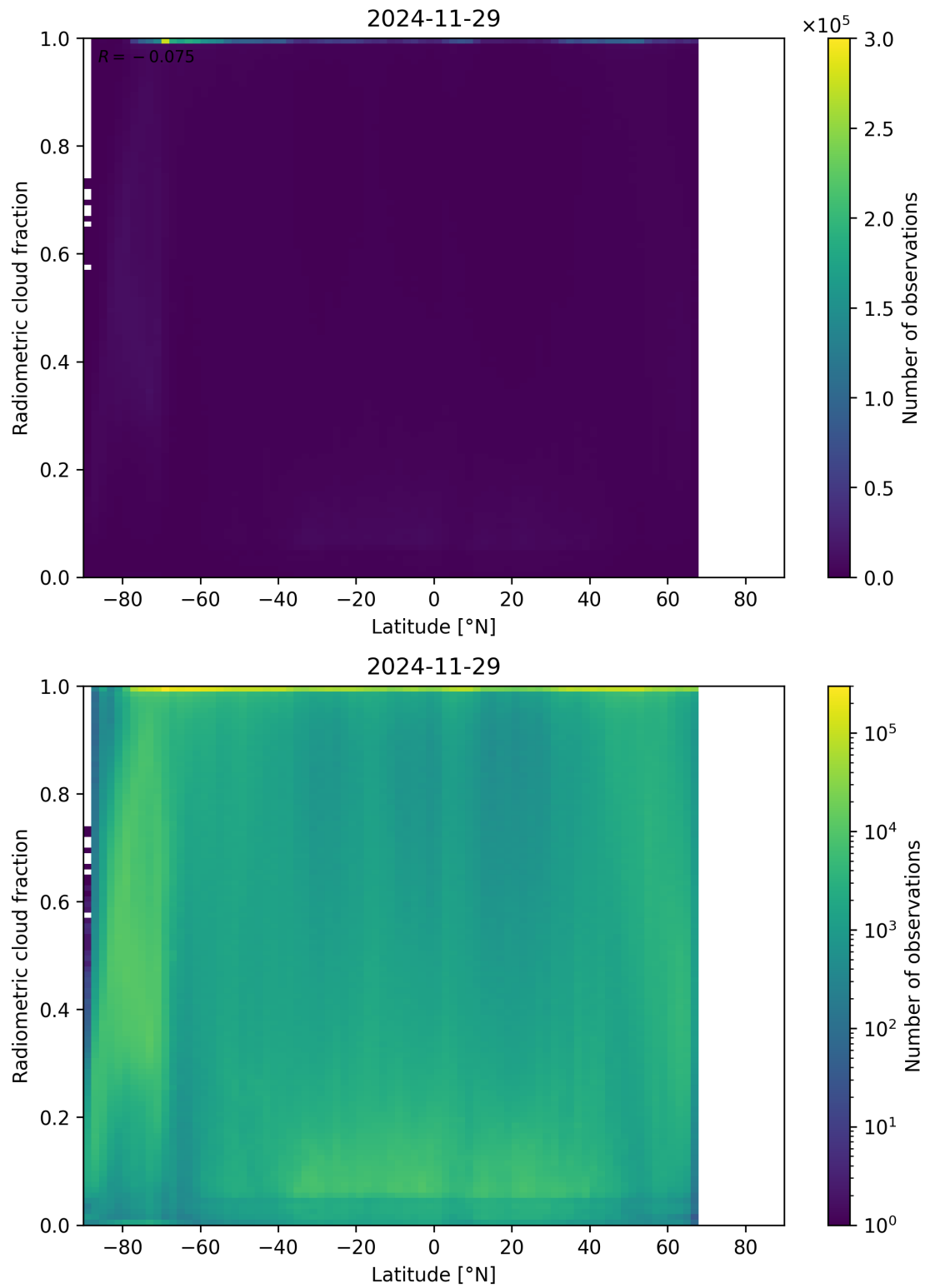
Figure 92: Scatter density plot of “Latitude” against “Radiometric cloud fraction” for 2024-11-28 to 2024-11-30.
