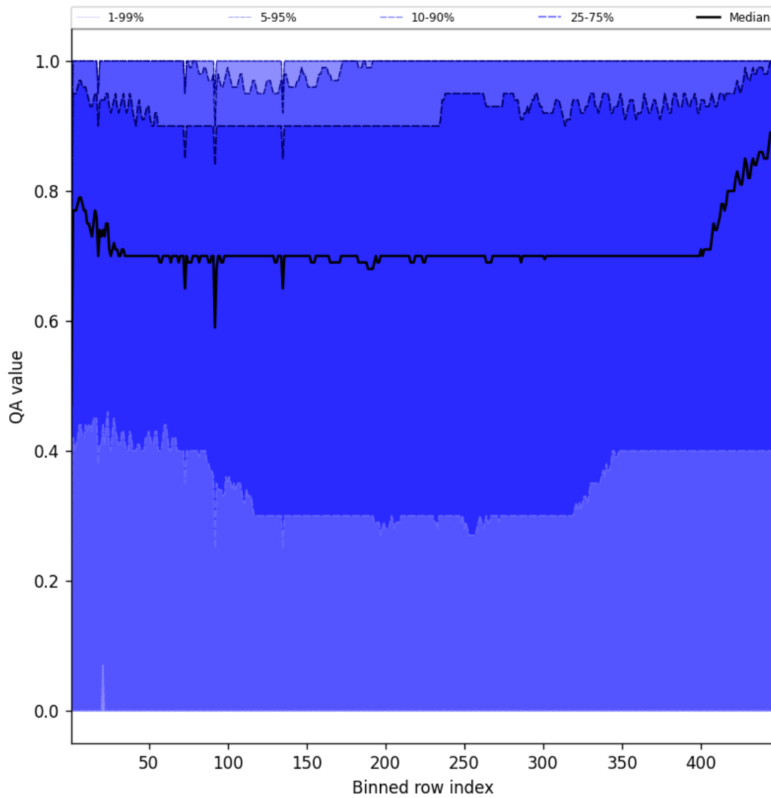
Figure 54: Along track statistics of “QA value” for 2024-11-28 to 2024-11-30
