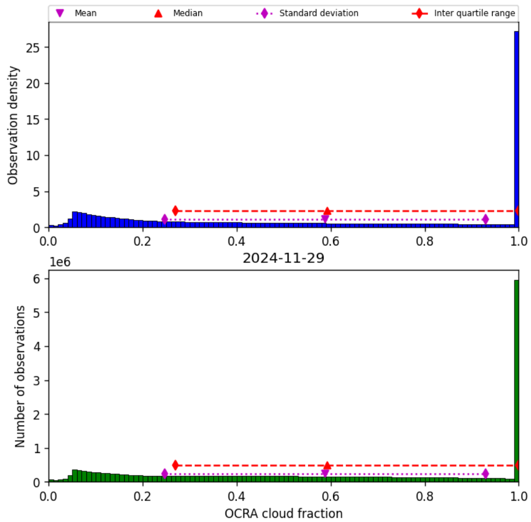
Figure 50: Histogram of “OCRA cloud fraction” for 2024-11-28 to 2024-11-30
