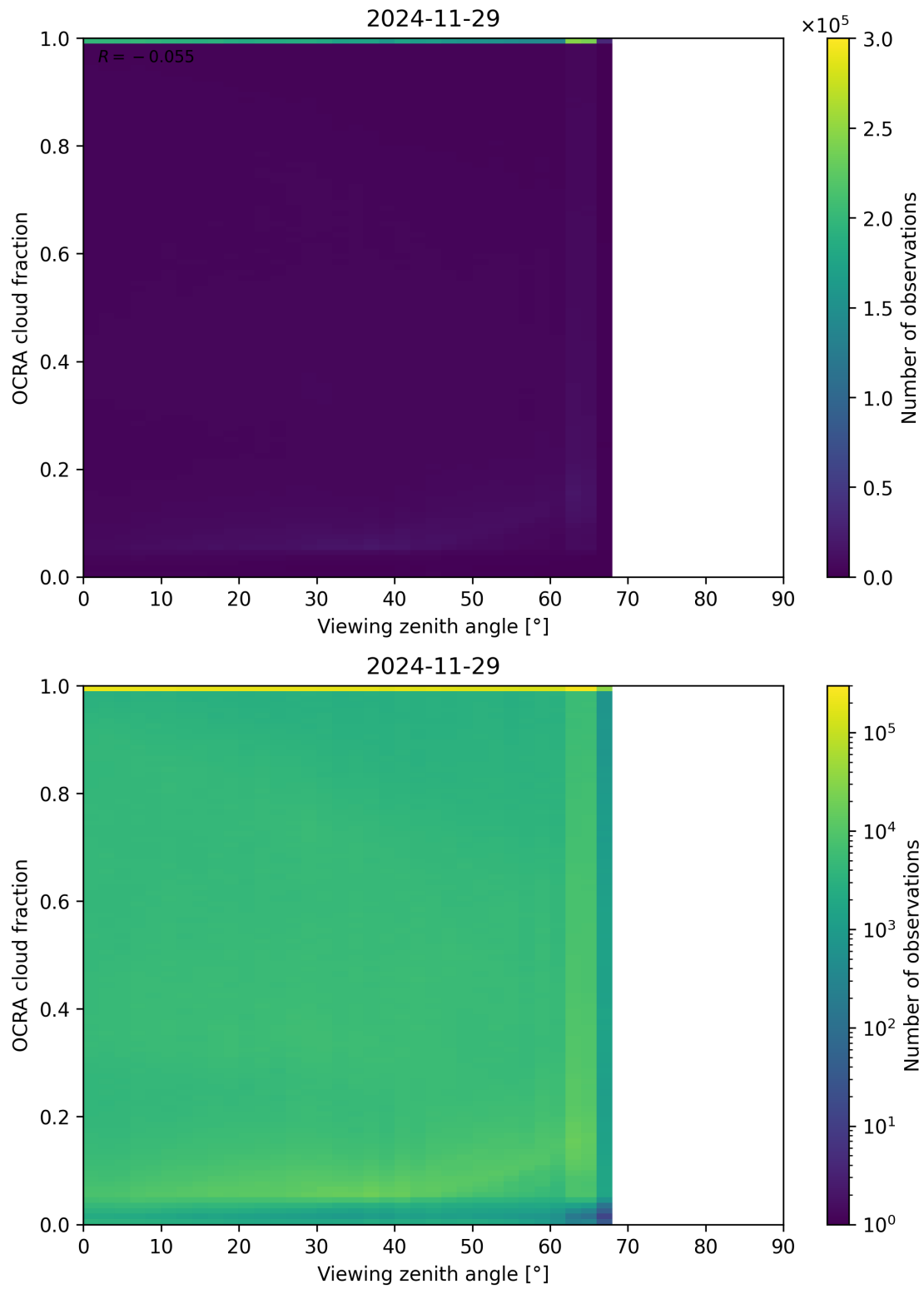
Figure 108: Scatter density plot of “Viewing zenith angle” against “OCRA cloud fraction” for 2024-11-28 to 2024-11-30.
