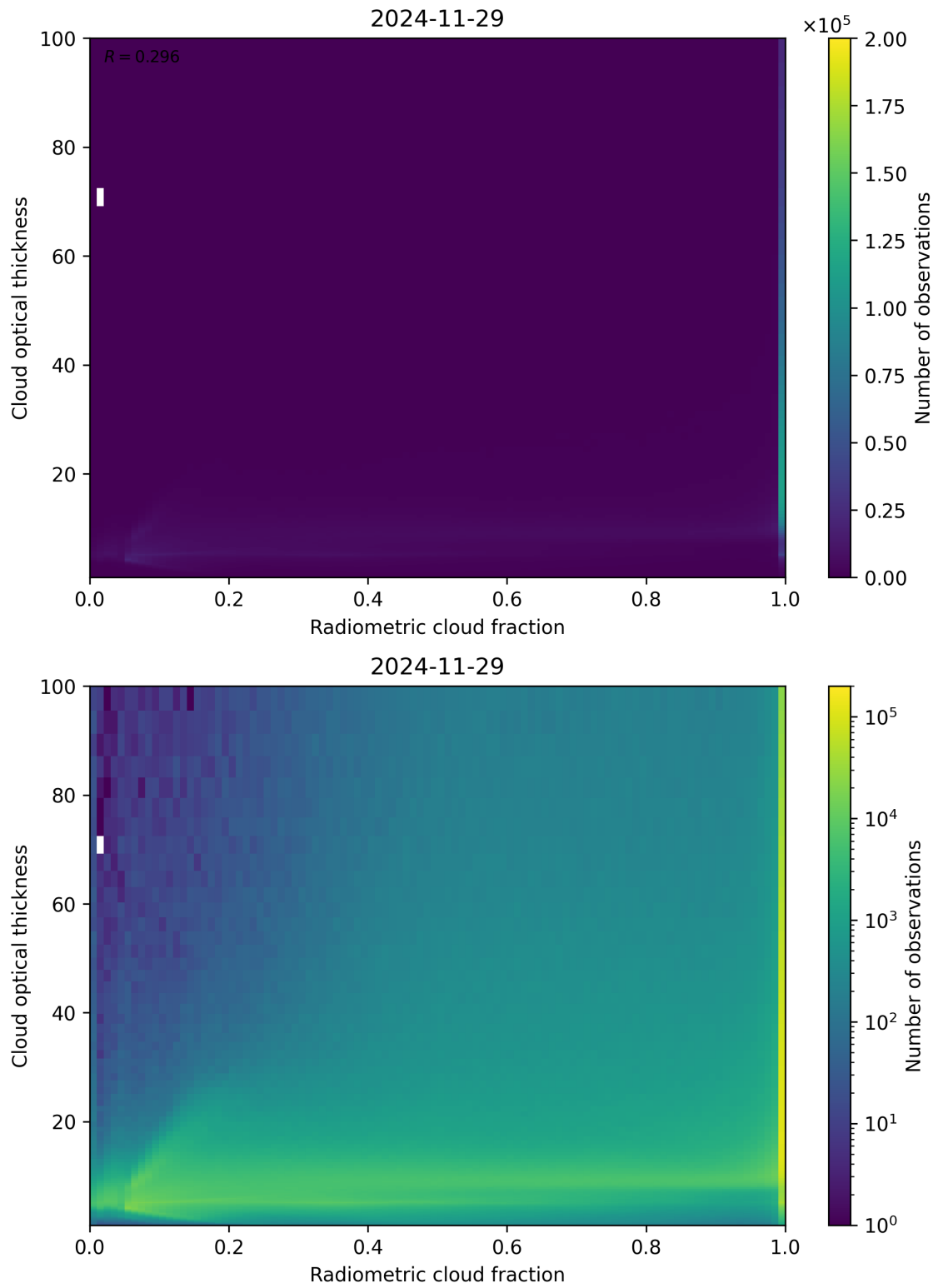
Figure 75: Scatter density plot of “Radiometric cloud fraction” against “Cloud optical thickness” for 2024-11-28 to 2024-11-30.
