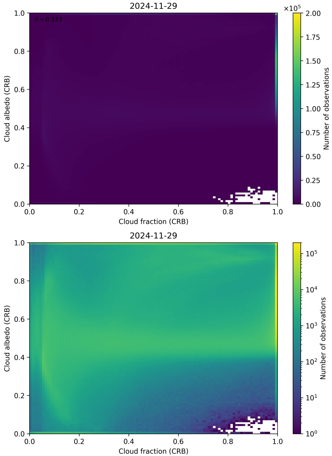
Figure 77: Scatter density plot of “Cloud fraction (CRB)” against “Cloud albedo (CRB)” for 2024-11-28 to 2024-11-30.
