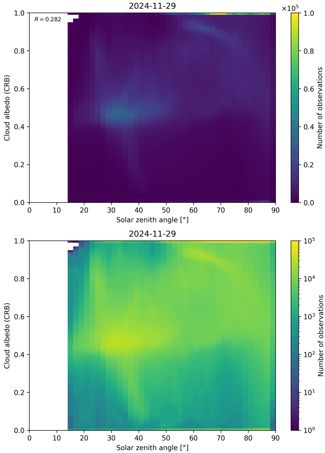
Figure 98: Scatter density plot of “Solar zenith angle” against “Cloud albedo (CRB)” for 2024-11-28 to 2024-11-30.
