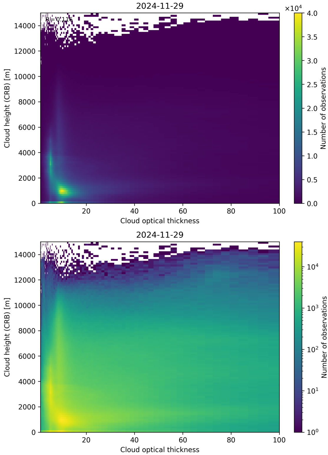
Figure 85: Scatter density plot of “Cloud optical thickness” against “Cloud height (CRB)” for 2024-11-28 to 2024-11-30.
