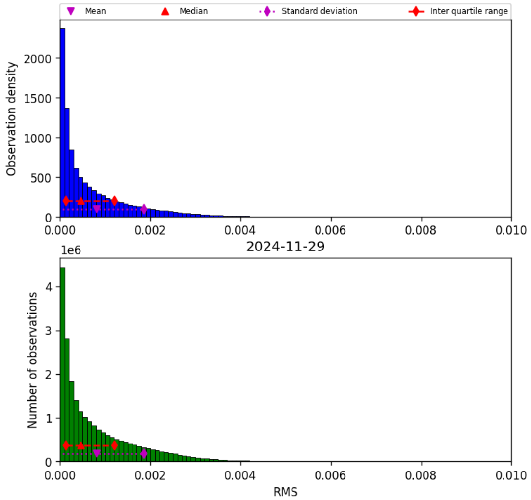
Figure 47: Histogram of “RMS” for 2024-11-28 to 2024-11-30
