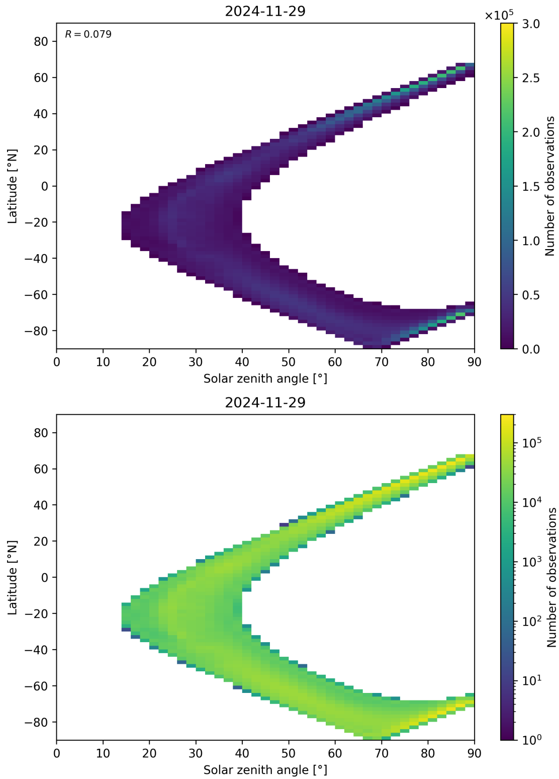
Figure 105: Scatter density plot of “Solar zenith angle” against “Latitude” for 2024-11-28 to 2024-11-30.
