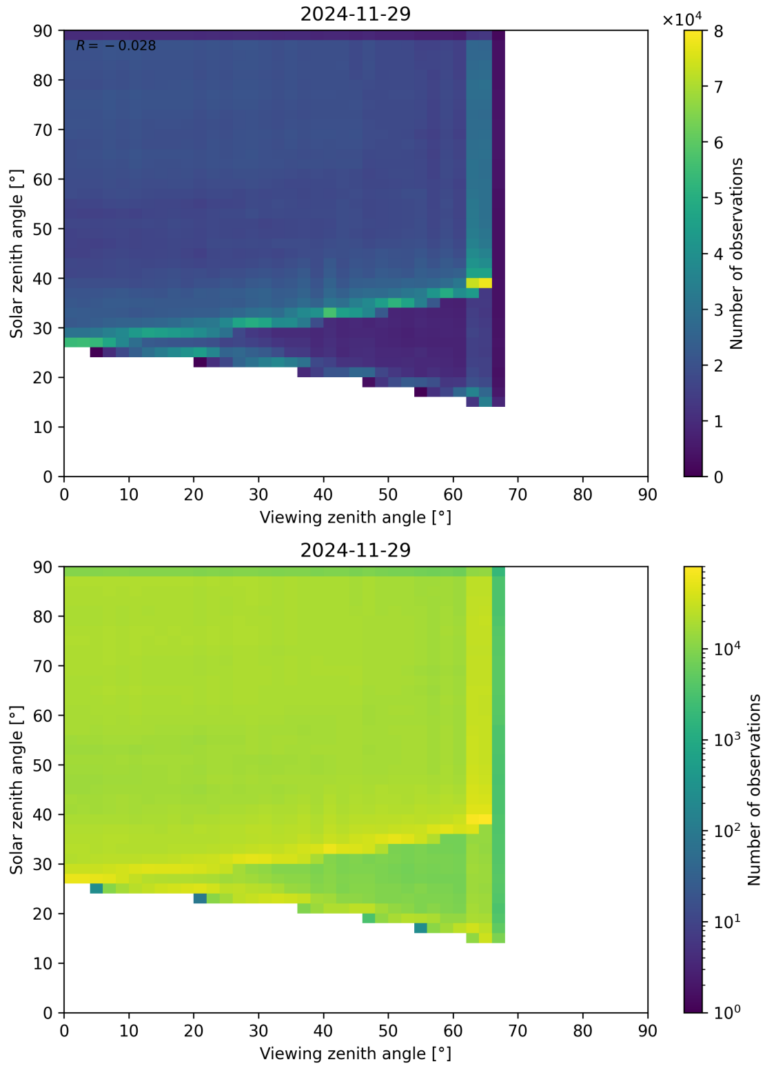
Figure 114: Scatter density plot of “Viewing zenith angle” against “Solar zenith angle” for 2024-11-28 to 2024-11-30.
