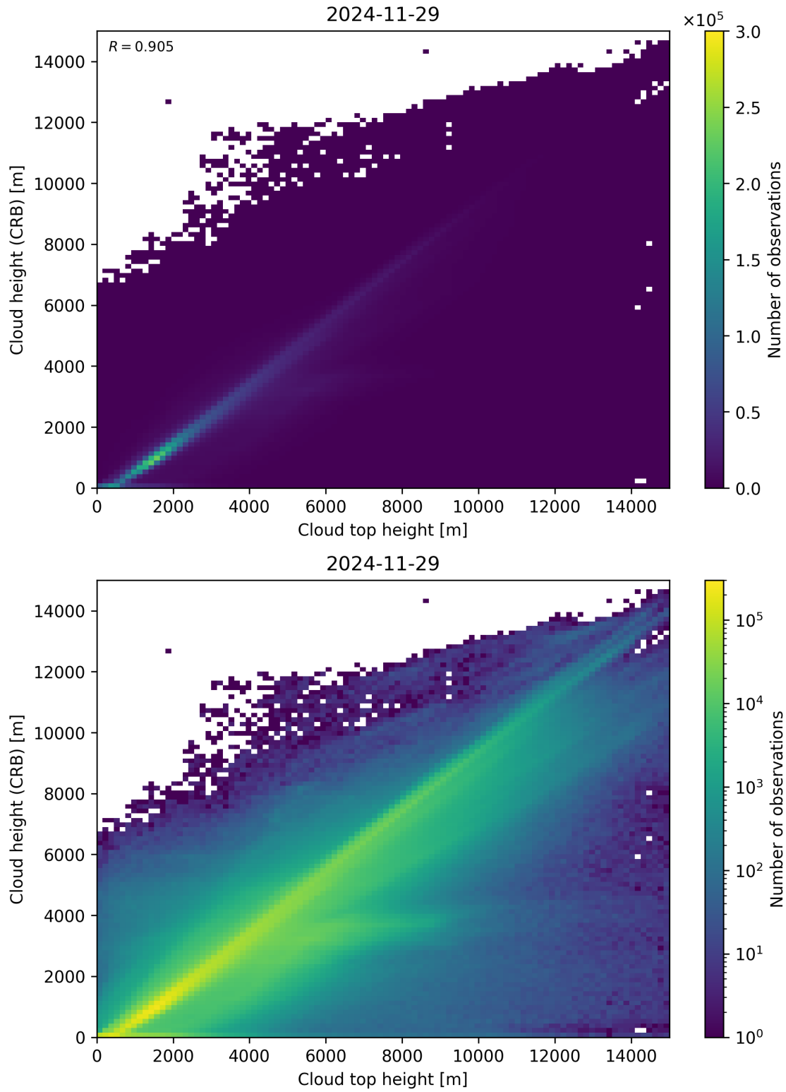
Figure 89: Scatter density plot of “Cloud top height” against “Cloud height (CRB)” for 2024-11-28 to 2024-11-30.
