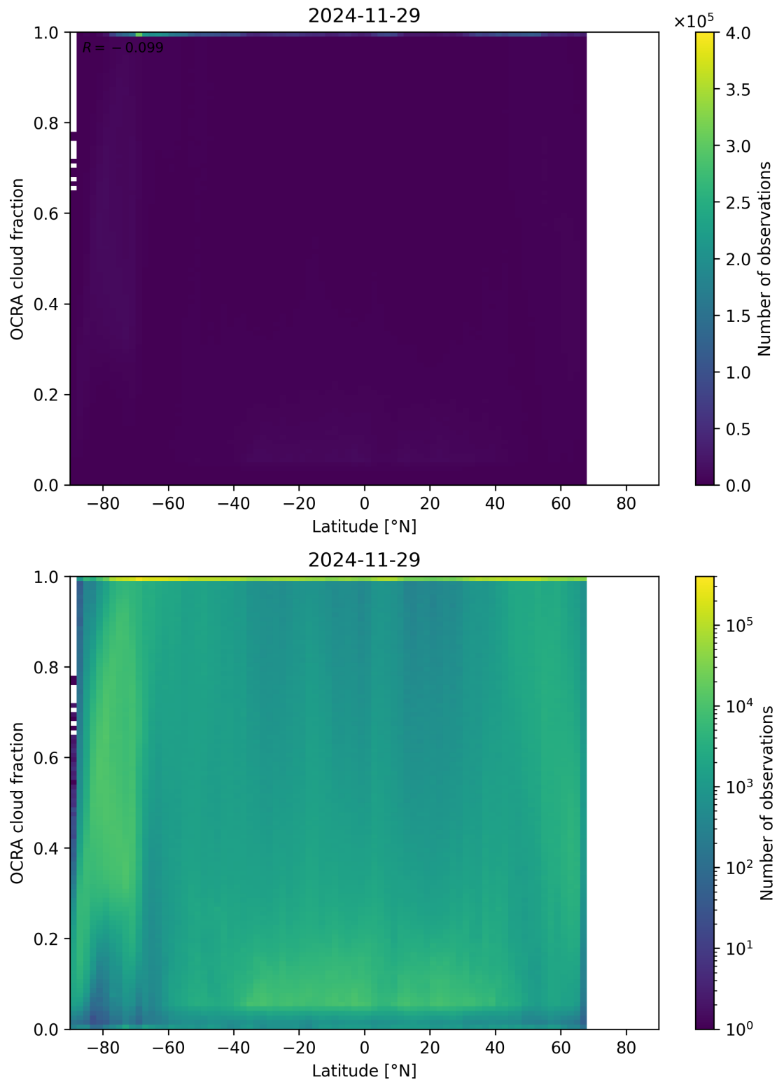
Figure 93: Scatter density plot of “Latitude” against “OCRA cloud fraction” for 2024-11-28 to 2024-11-30.
