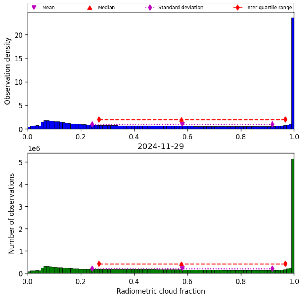
Figure 39: Histogram of “Radiometric cloud fraction” for 2024-11-28 to 2024-11-30
