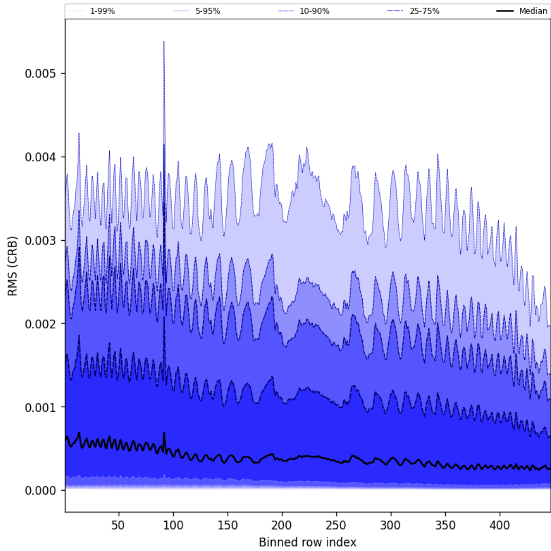
Figure 64: Along track statistics of “RMS (CRB)” for 2024-11-28 to 2024-11-30
