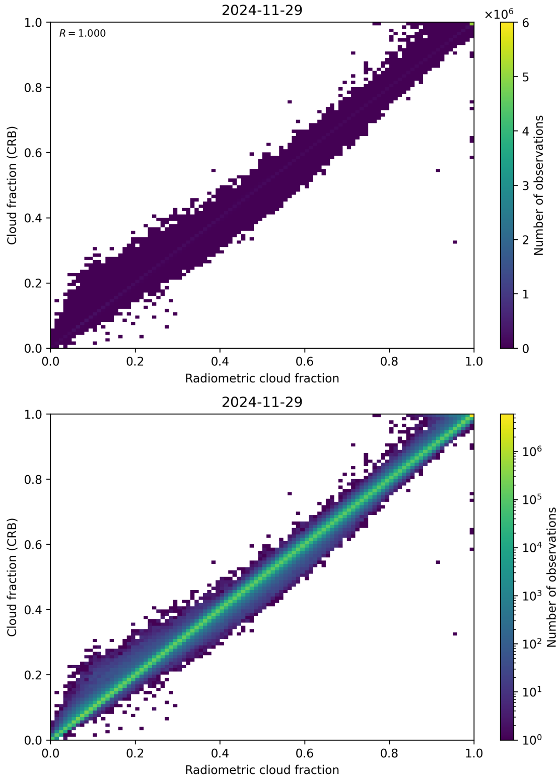
Figure 73: Scatter density plot of “Radiometric cloud fraction” against “Cloud fraction (CRB)” for 2024-11-28 to 2024-11-30.
