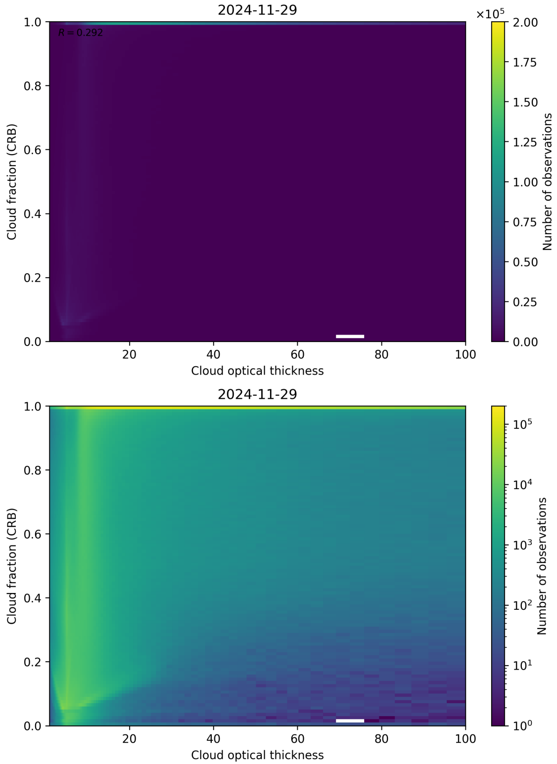
Figure 84: Scatter density plot of “Cloud optical thickness” against “Cloud fraction (CRB)” for 2024-11-28 to 2024-11-30.
