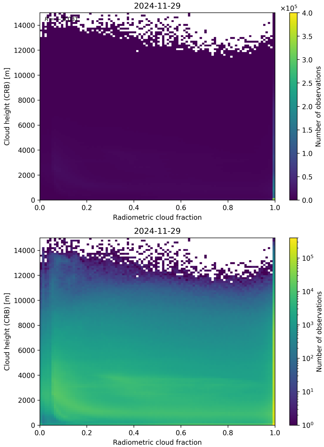
Figure 74: Scatter density plot of “Radiometric cloud fraction” against “Cloud height (CRB)” for 2024-11-28 to 2024-11-30.
