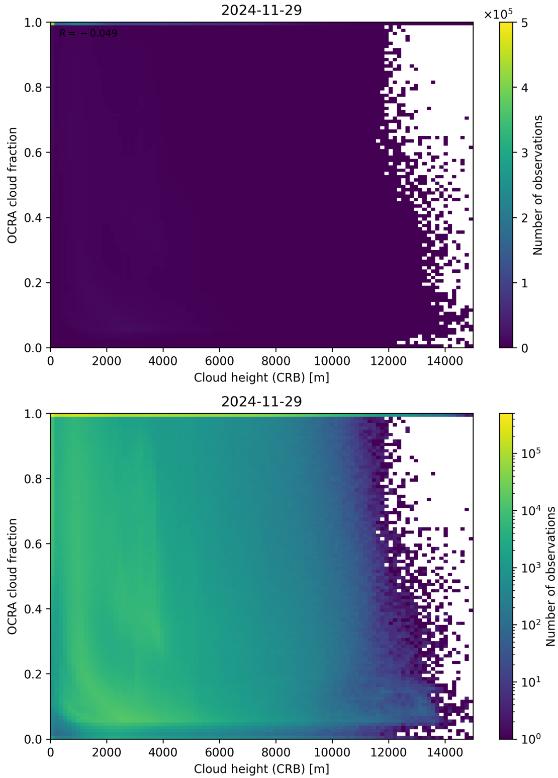
Figure 81: Scatter density plot of “Cloud height (CRB)” against “OCRA cloud fraction” for 2024-11-28 to 2024-11-30.
