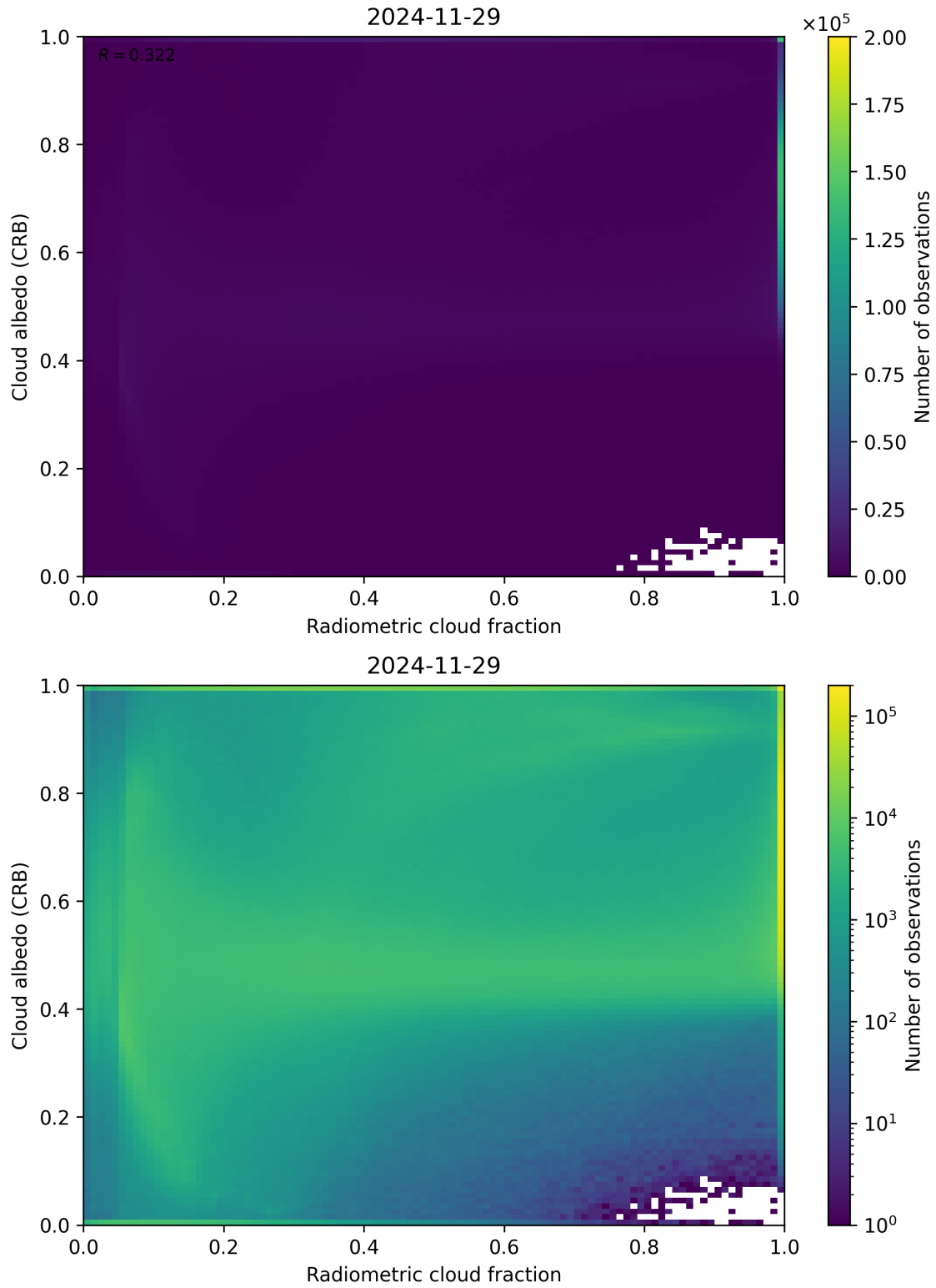
Figure 71: Scatter density plot of “Radiometric cloud fraction” against “Cloud albedo (CRB)” for 2024-11-28 to 2024-11-30.
