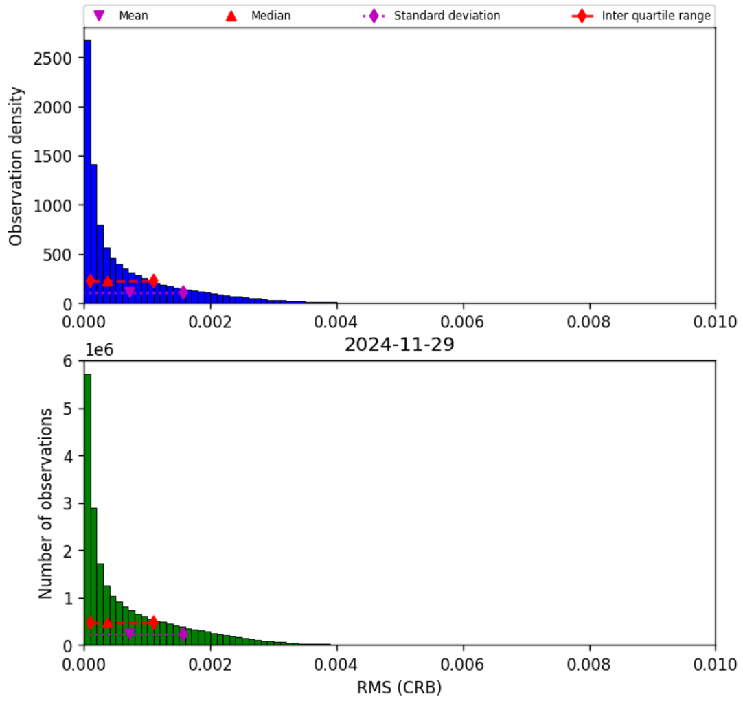
Figure 48: Histogram of “RMS (CRB)” for 2024-11-28 to 2024-11-30
