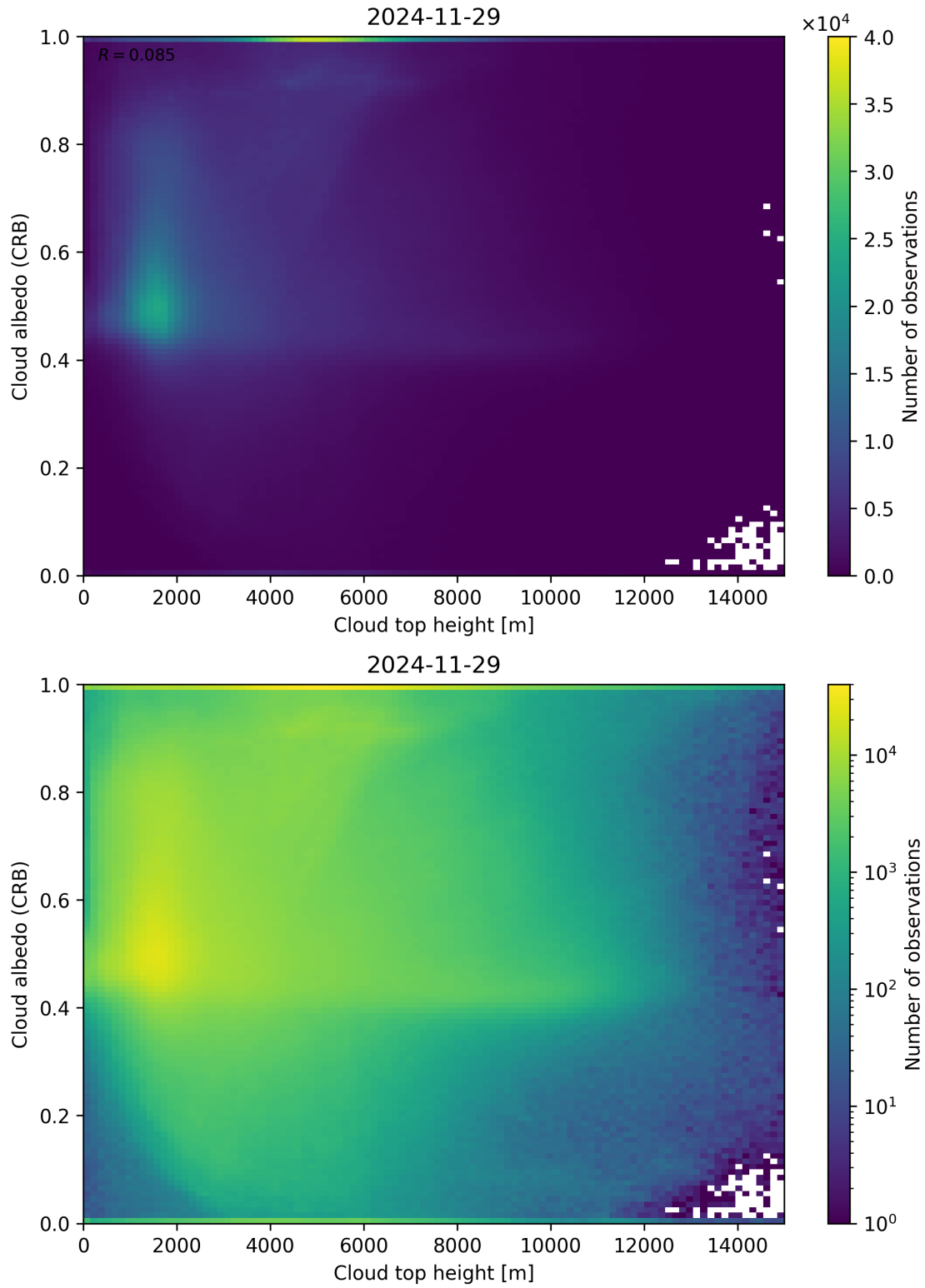
Figure 86: Scatter density plot of “Cloud top height” against “Cloud albedo (CRB)” for 2024-11-28 to 2024-11-30.
