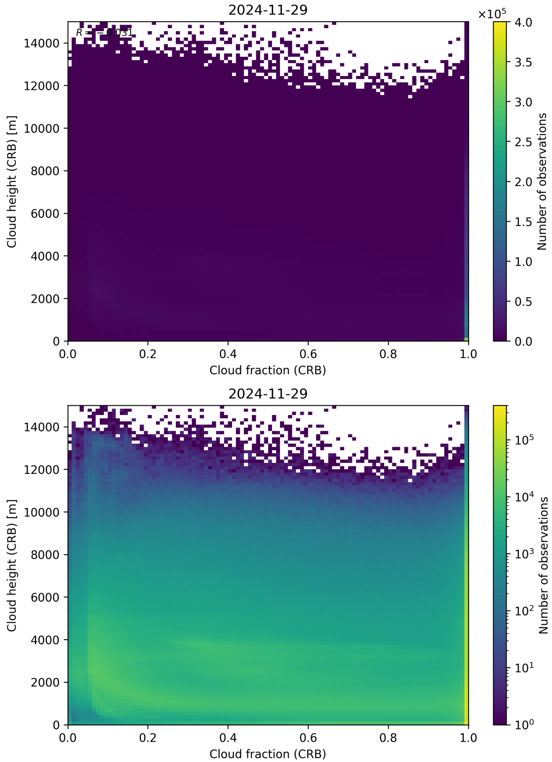
Figure 79: Scatter density plot of “Cloud fraction (CRB)” against “Cloud height (CRB)” for 2024-11-28 to 2024-11-30.
