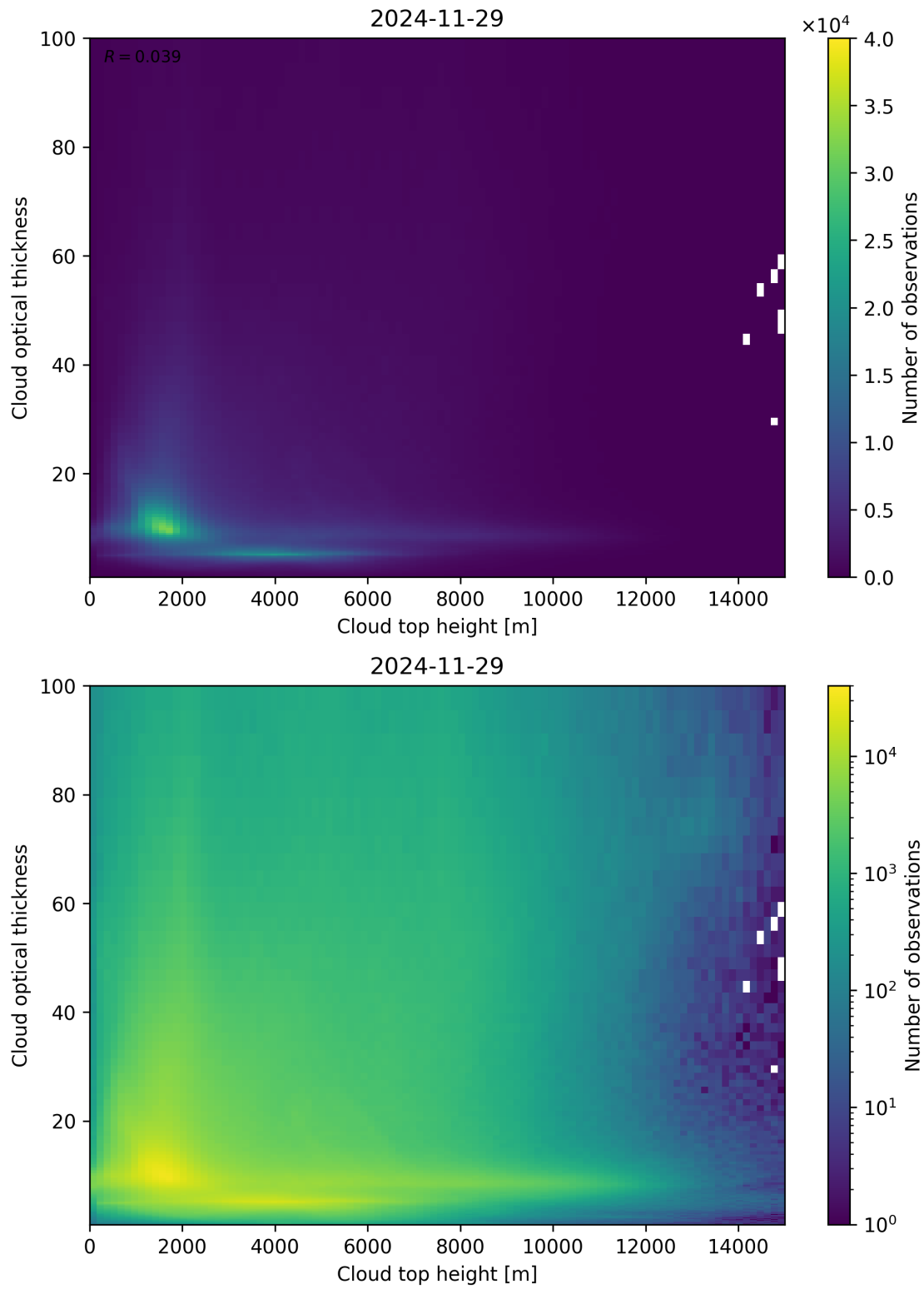
Figure 90: Scatter density plot of “Cloud top height” against “Cloud optical thickness” for 2024-11-28 to 2024-11-30.
