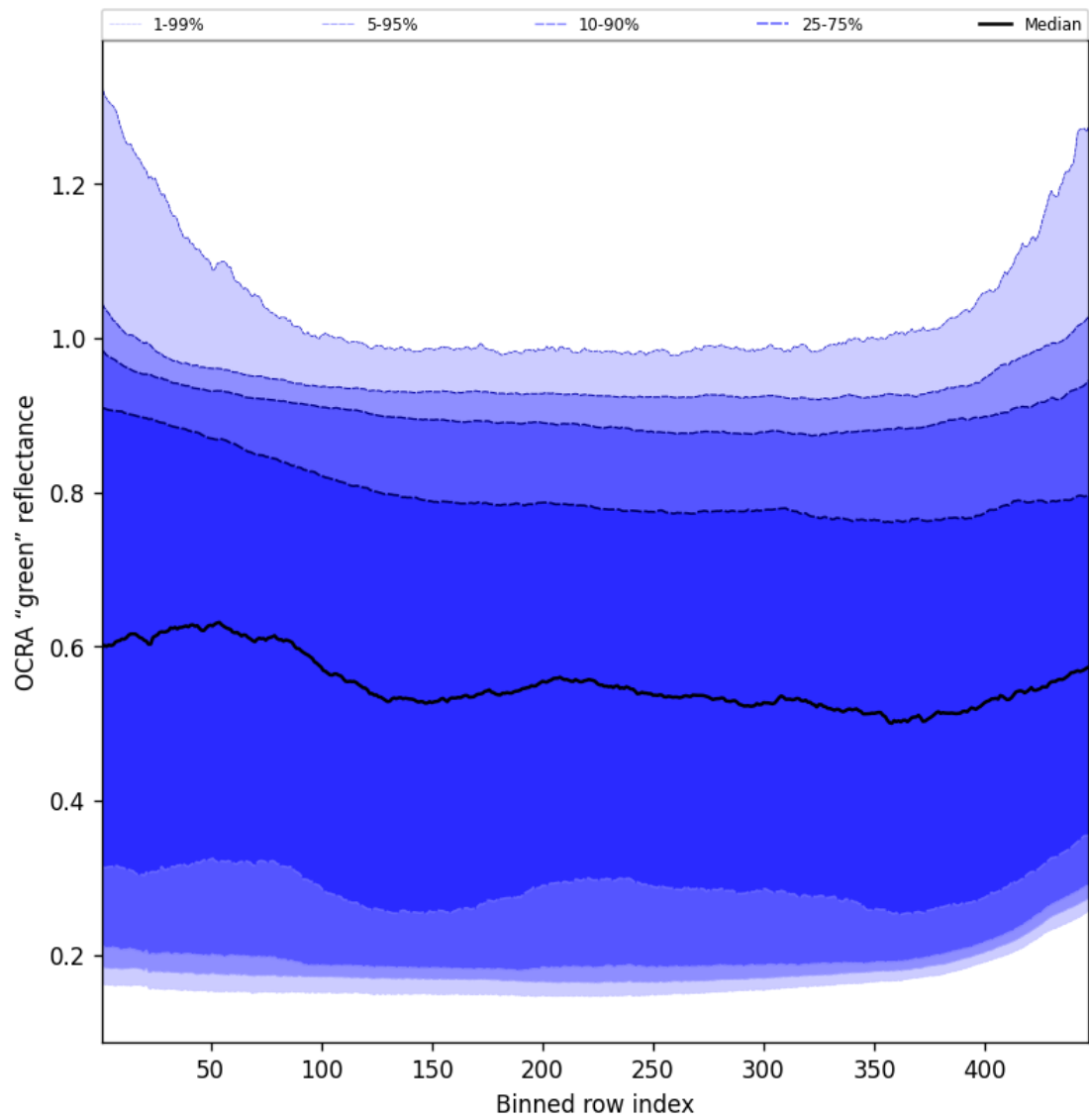
Figure 68: Along track statistics of "OCRA "green" reflectance" for 2024-11-28 to 2024-11-30
