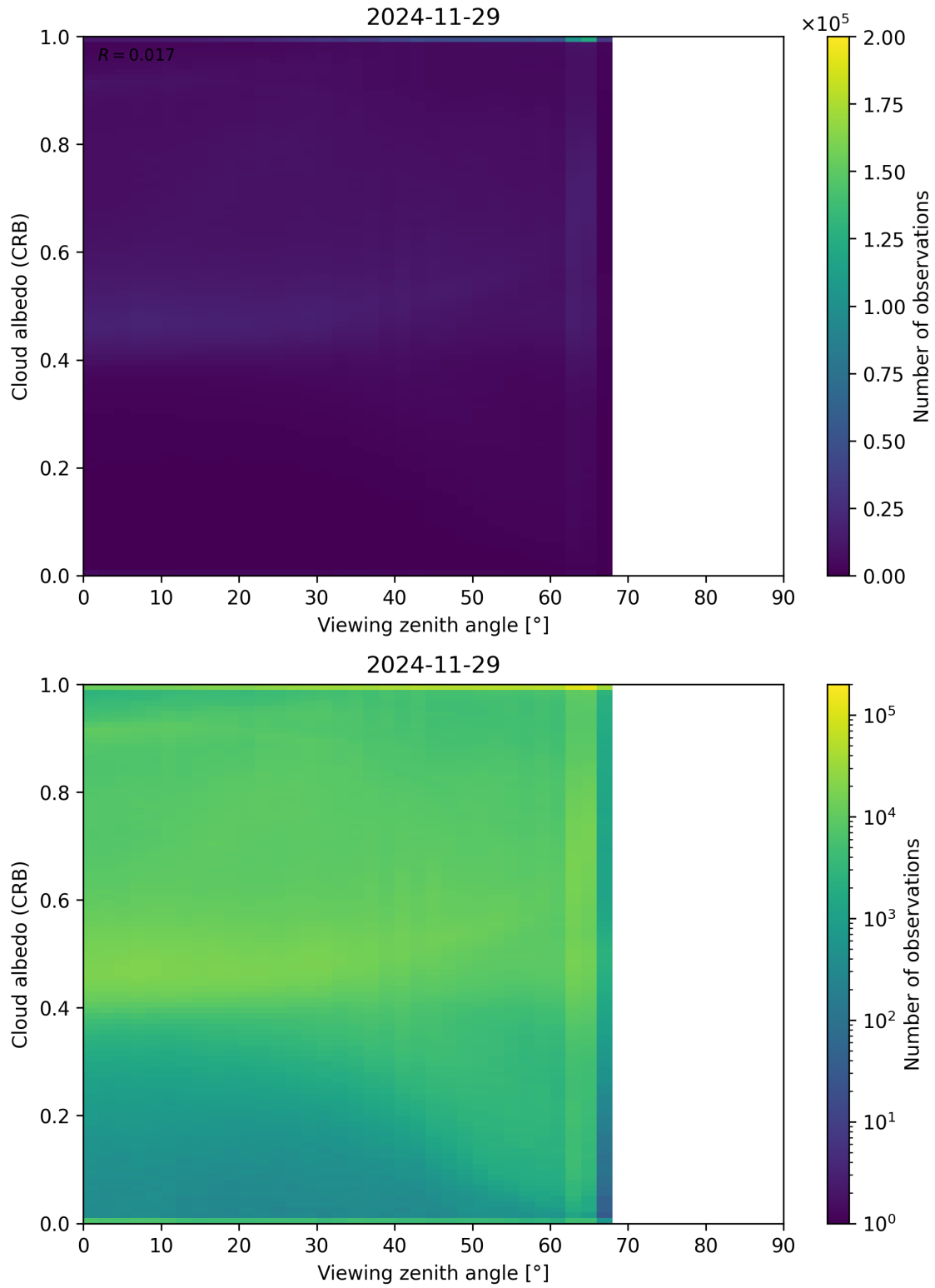
Figure 106: Scatter density plot of “Viewing zenith angle” against “Cloud albedo (CRB)” for 2024-11-28 to 2024-11-30.
