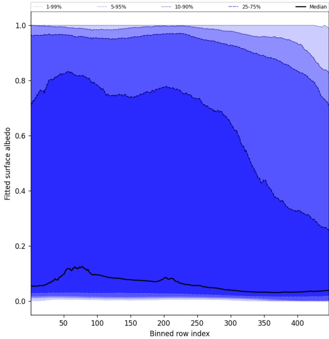
Figure 61: Along track statistics of “Fitted surface albedo” for 2024-11-28 to 2024-11-30
