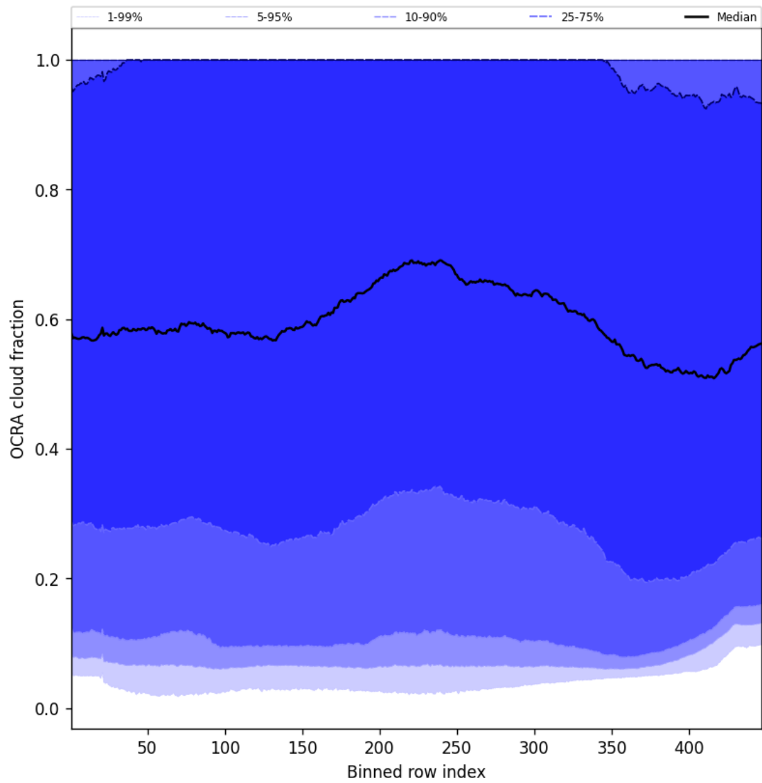
Figure 66: Along track statistics of “OCRA cloud fraction” for 2024-11-28 to 2024-11-30
