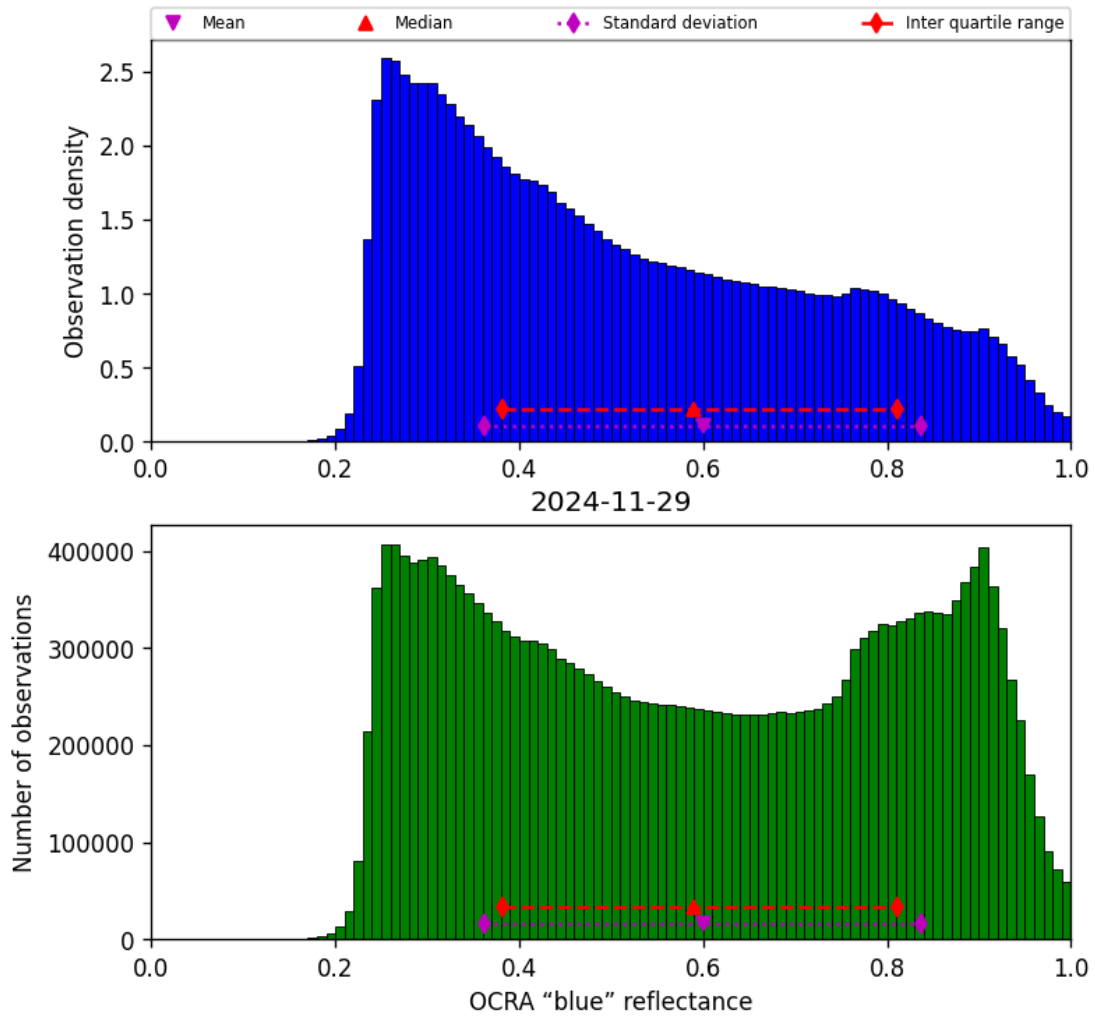
Figure 51: Histogram of “OCRA “blue” reflectance” for 2024-11-28 to 2024-11-30
