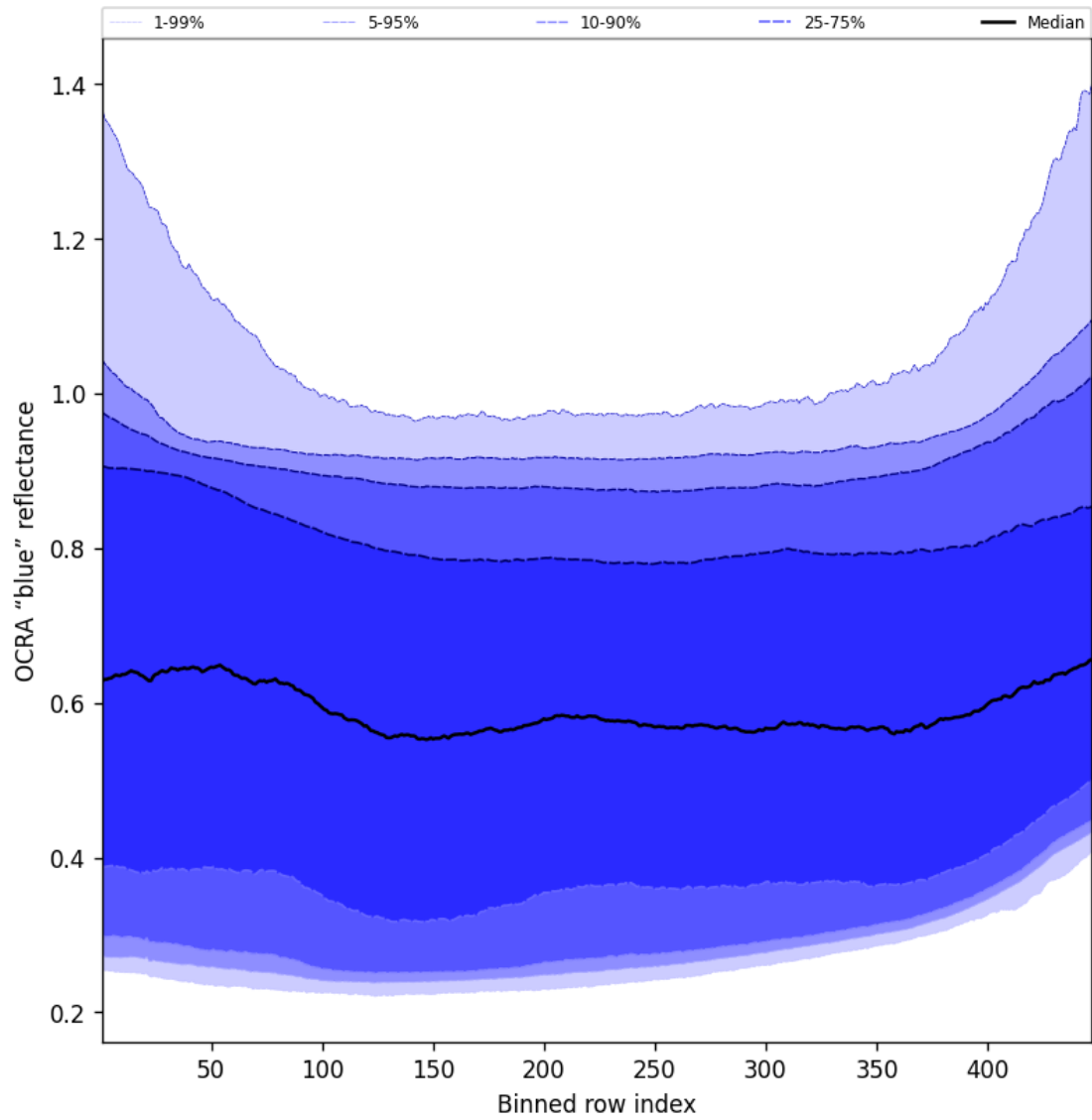
Figure 67: Along track statistics of “OCRA “blue” reflectance” for 2024-11-28 to 2024-11-30
