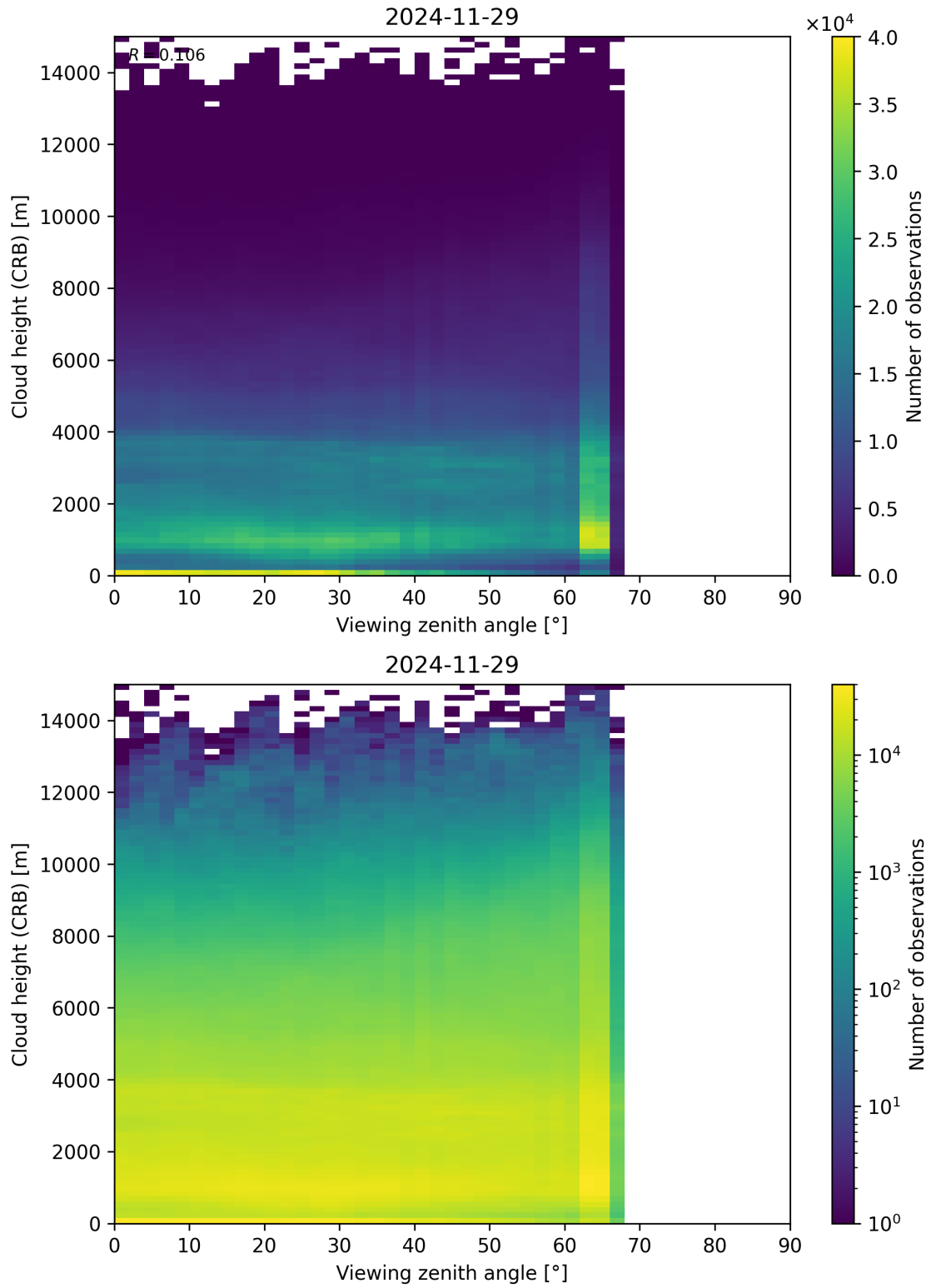
Figure 110: Scatter density plot of “Viewing zenith angle” against “Cloud height (CRB)” for 2024-11-28 to 2024-11-30.
