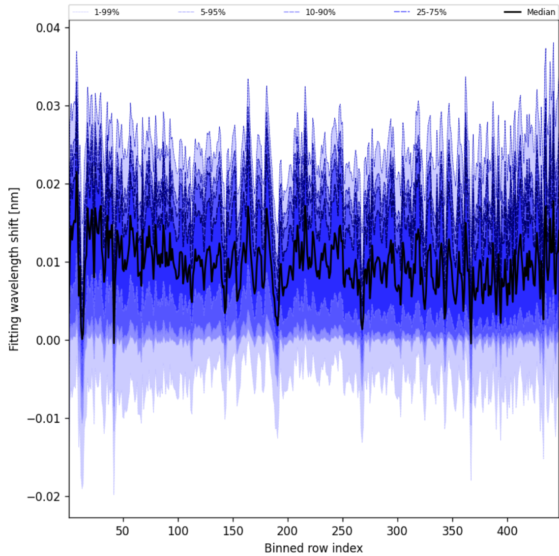
Figure 65: Along track statistics of “Fitting wavelength shift” for 2024-11-28 to 2024-11-30
