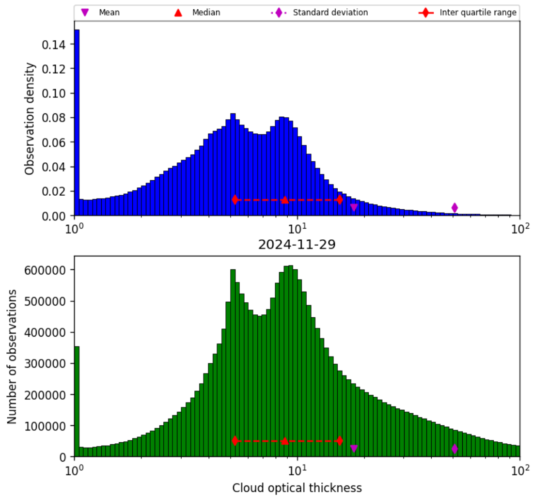
Figure 41: Histogram of “Cloud optical thickness” for 2024-11-28 to 2024-11-30
