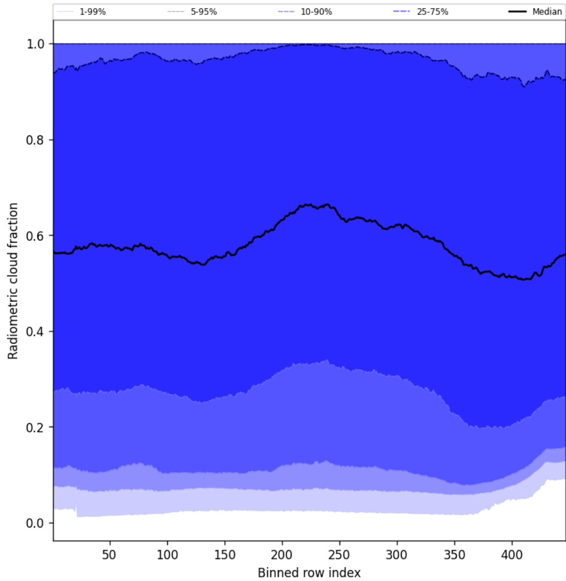
Figure 55: Along track statistics of “Radiometric cloud fraction” for 2024-11-28 to 2024-11-30
