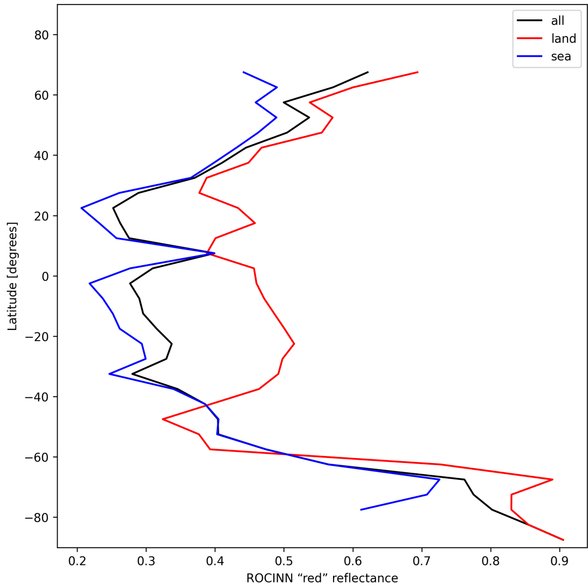
Figure 37: Zonal average of "ROCINN "red" reflectance" for 2024-11-28 to 2024-11-30.
