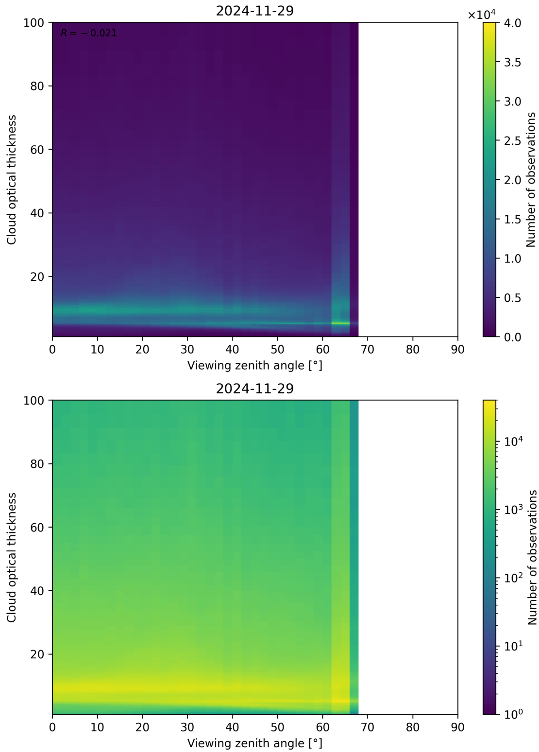
Figure 111: Scatter density plot of “Viewing zenith angle” against “Cloud optical thickness” for 2024-11-28 to 2024-11-30.
