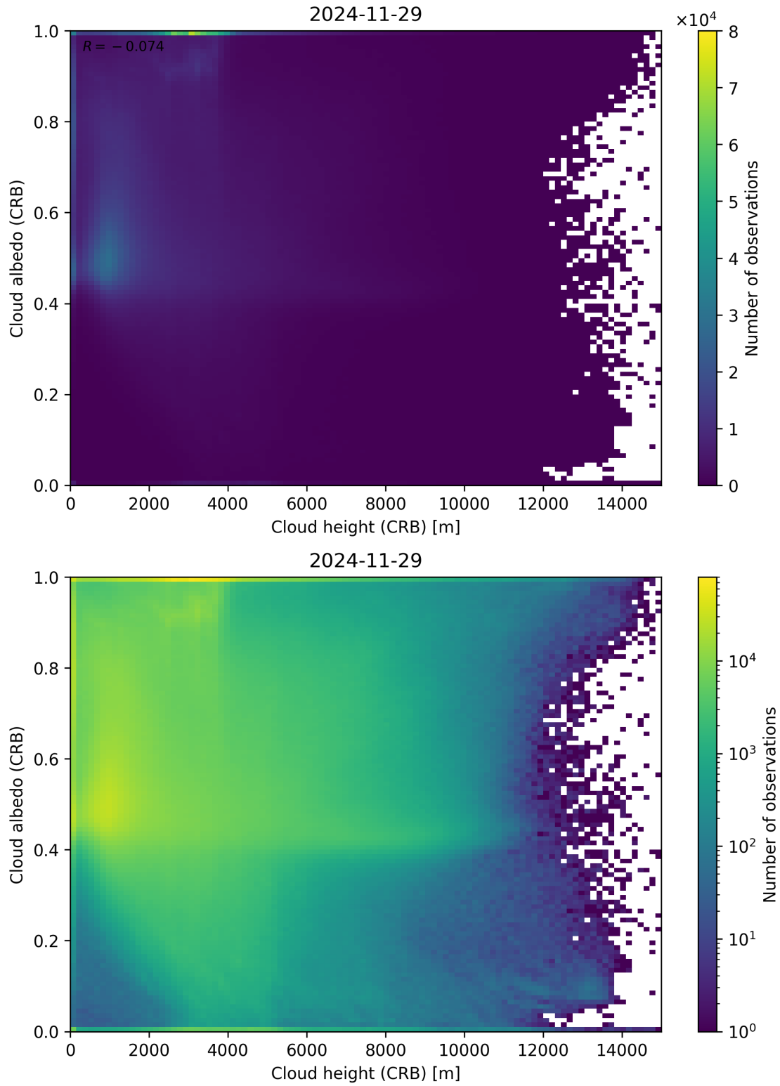
Figure 80: Scatter density plot of “Cloud height (CRB)” against “Cloud albedo (CRB)” for 2024-11-28 to 2024-11-30.
