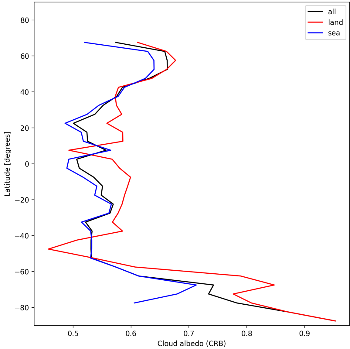
Figure 28: Zonal average of “Cloud albedo (CRB)” for 2024-11-28 to 2024-11-30.
