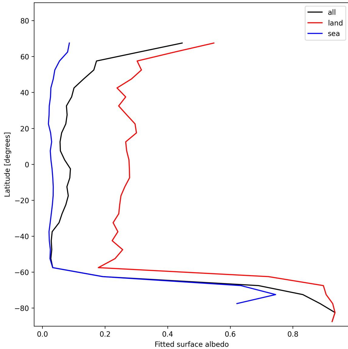
Figure 29: Zonal average of “Fitted surface albedo” for 2024-11-28 to 2024-11-30.
