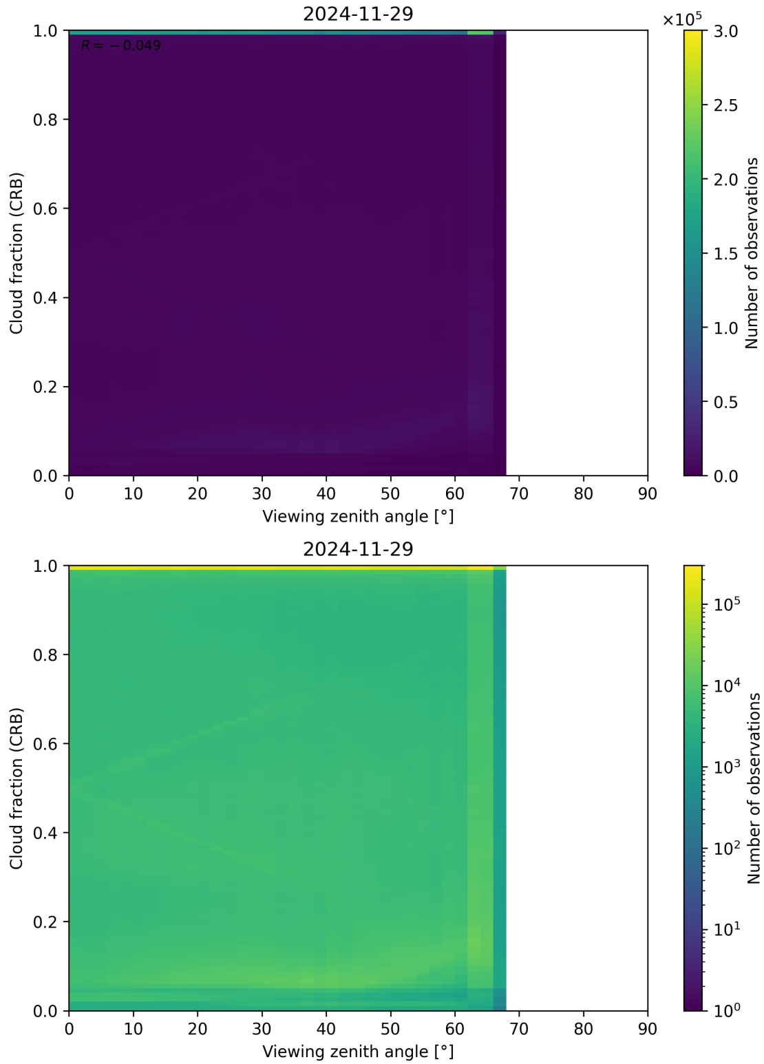
Figure 109: Scatter density plot of “Viewing zenith angle” against “Cloud fraction (CRB)” for 2024-11-28 to 2024-11-30.
