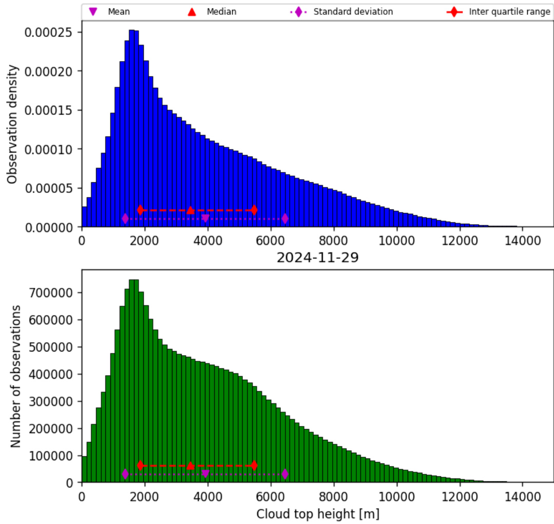
Figure 40: Histogram of “Cloud top height” for 2024-11-28 to 2024-11-30
