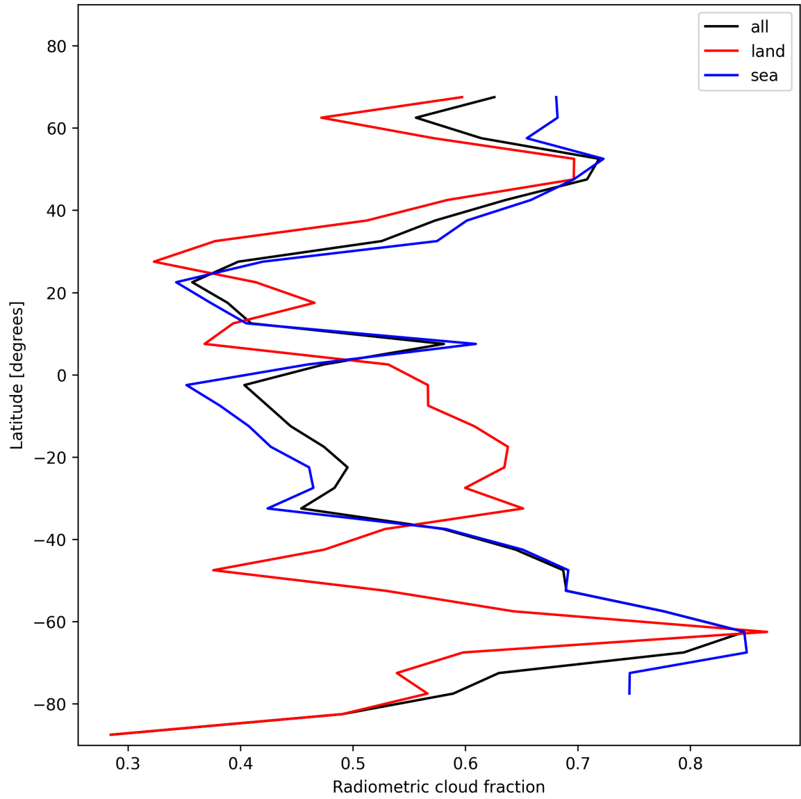
Figure 23: Zonal average of “Radiometric cloud fraction” for 2024-11-28 to 2024-11-30.
