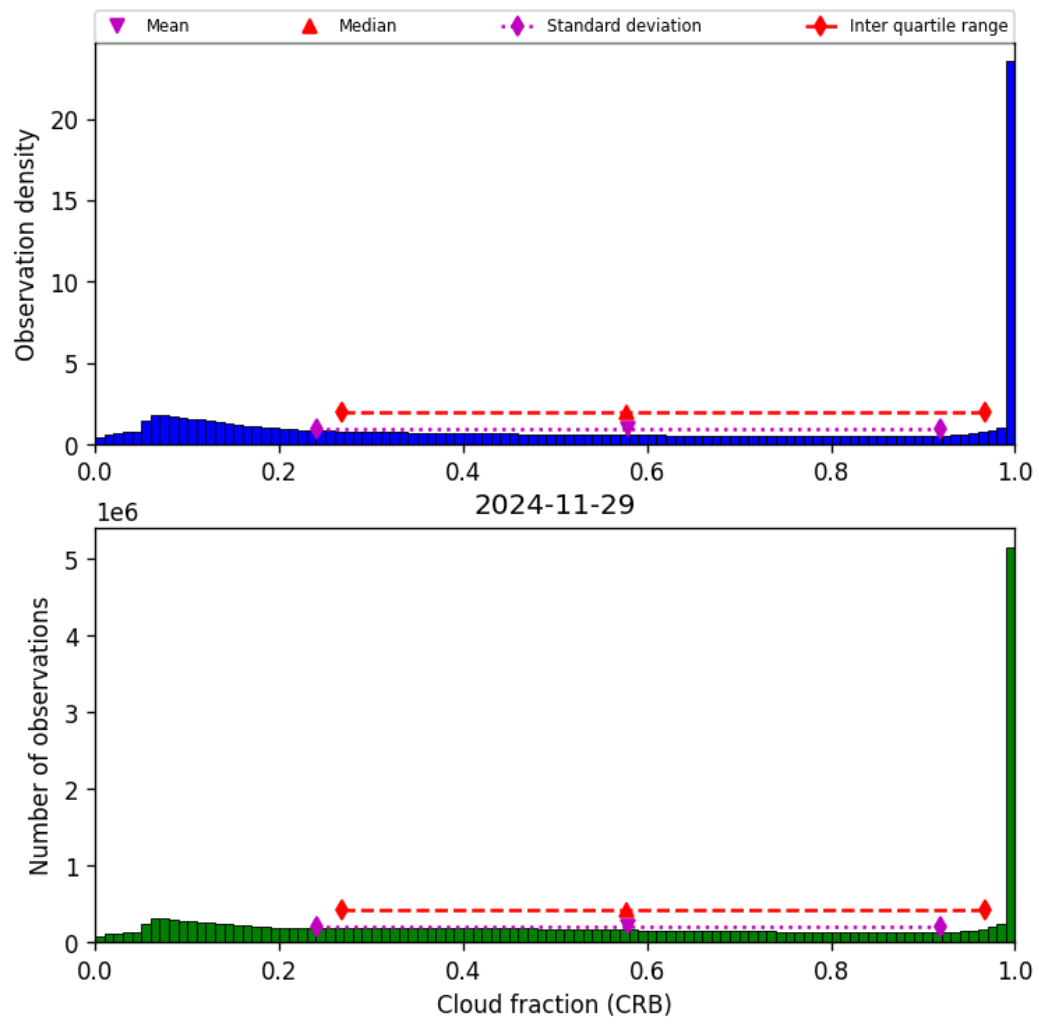
Figure 42: Histogram of “Cloud fraction (CRB)” for 2024-11-28 to 2024-11-30
