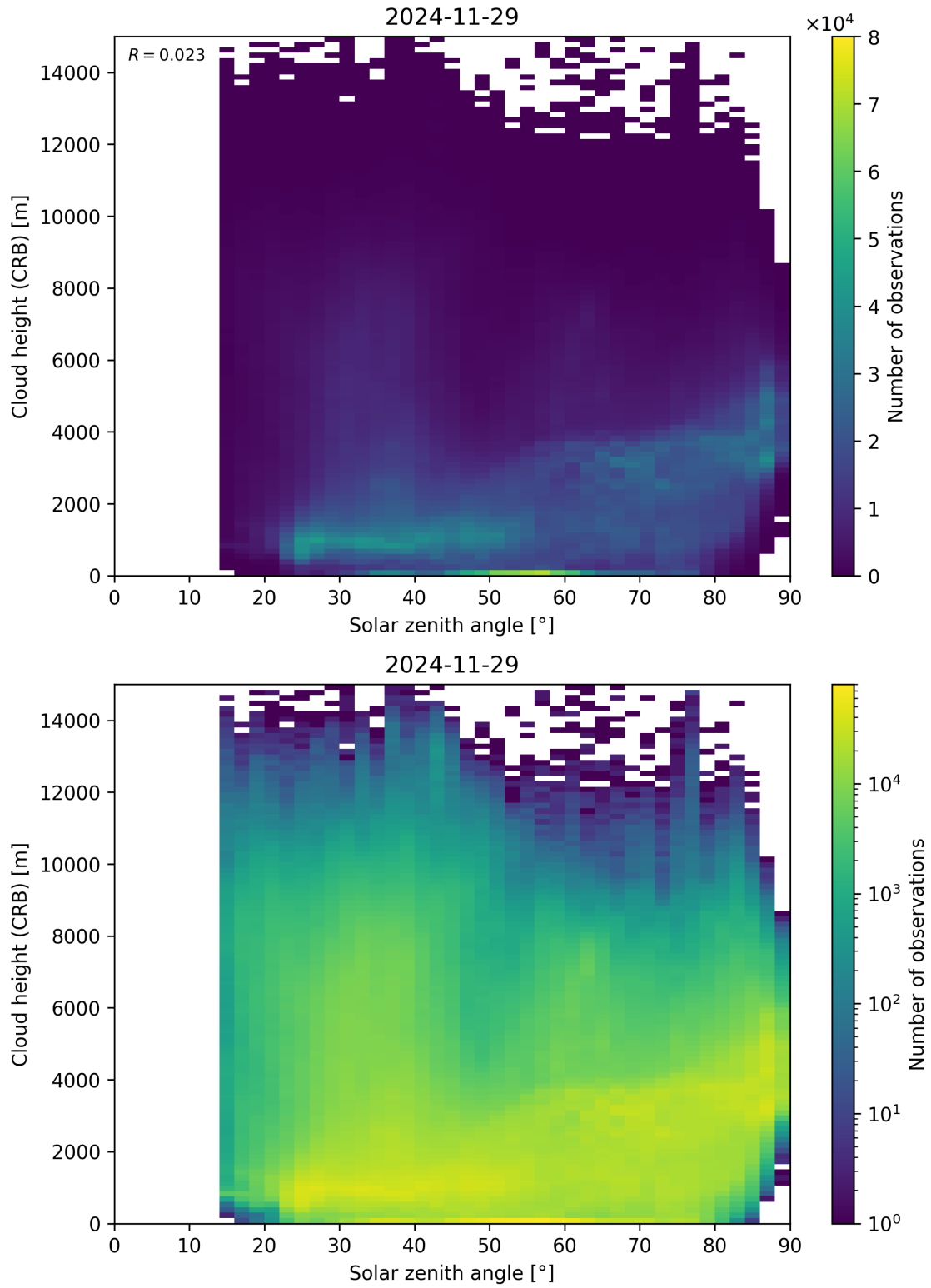
Figure 102: Scatter density plot of “Solar zenith angle” against “Cloud height (CRB)” for 2024-11-28 to 2024-11-30.
