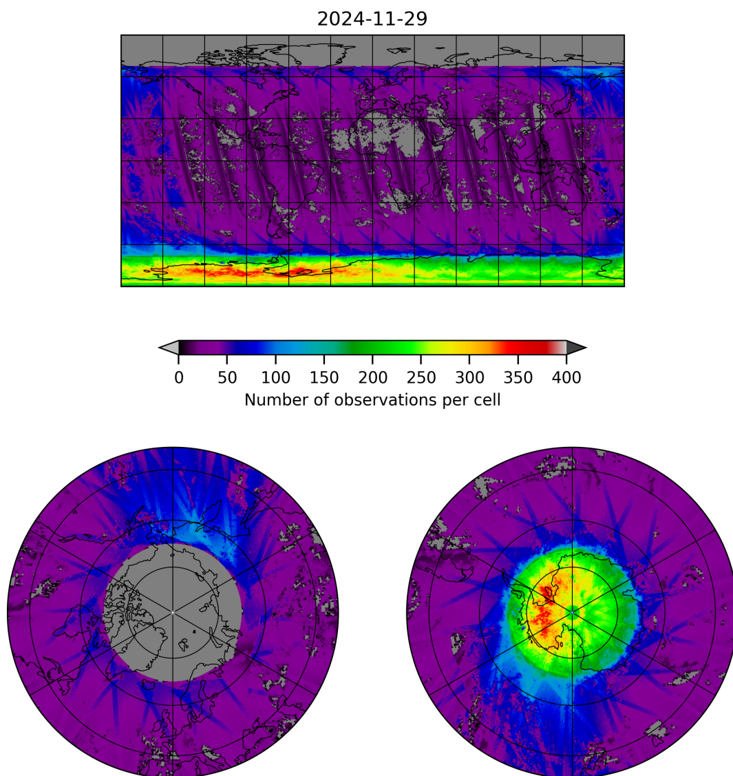
Figure 21: Map of the number of observations for 2024-11-28 to 2024-11-30
