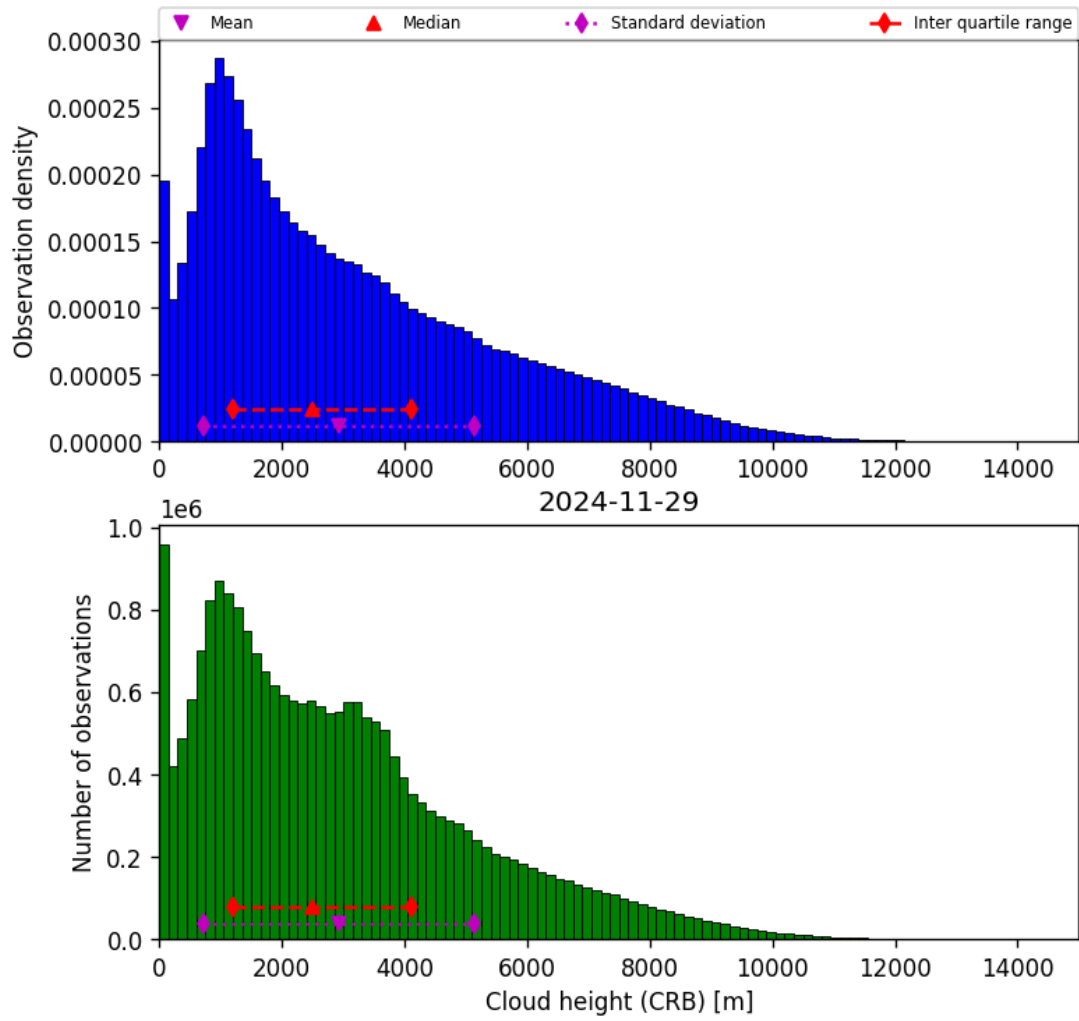
Figure 43: Histogram of “Cloud height (CRB)” for 2024-11-28 to 2024-11-30
