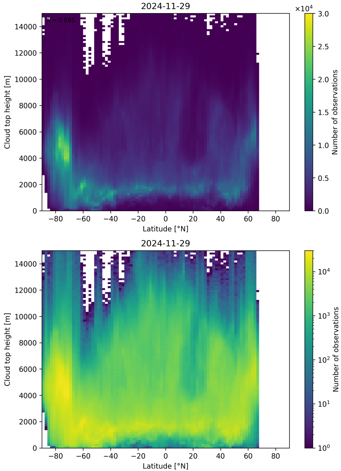
Figure 97: Scatter density plot of “Latitude” against “Cloud top height” for 2024-11-28 to 2024-11-30.
