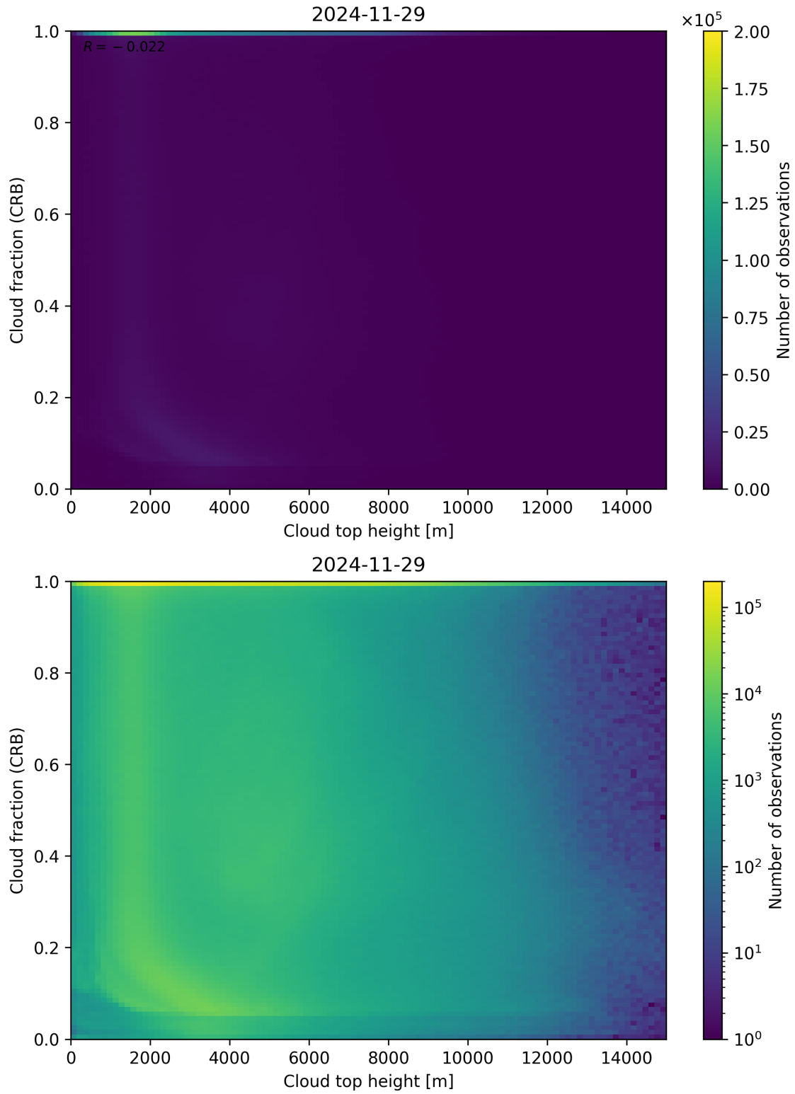
Figure 88: Scatter density plot of “Cloud top height” against “Cloud fraction (CRB)” for 2024-11-28 to 2024-11-30.
