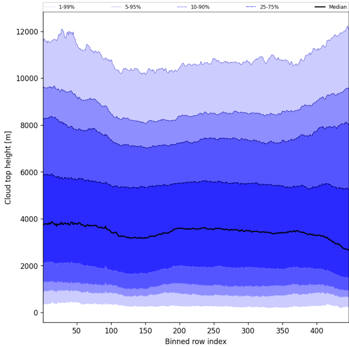
Figure 56: Along track statistics of “Cloud top height” for 2024-11-28 to 2024-11-30
