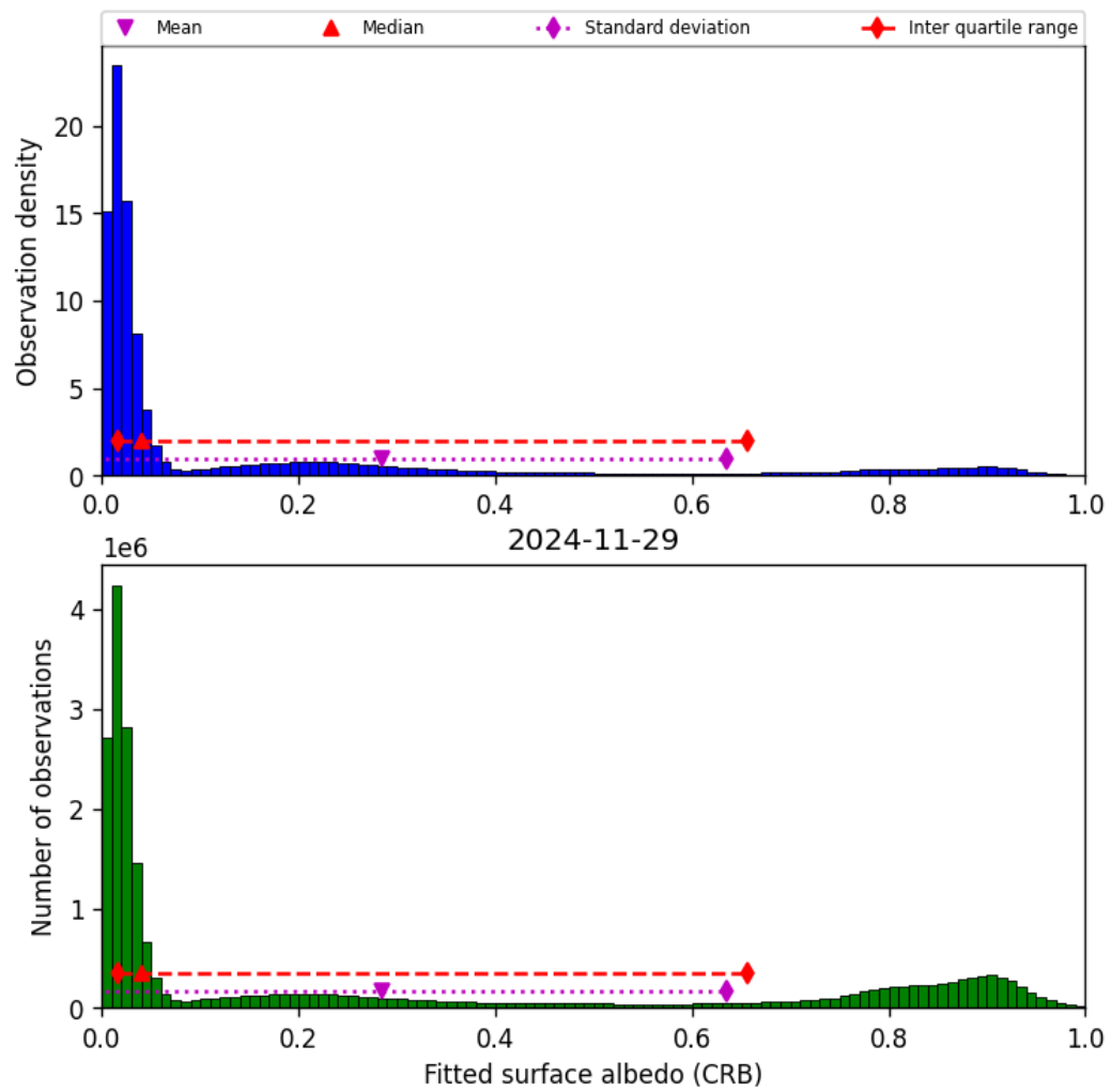
Figure 46: Histogram of “Fitted surface albedo (CRB)” for 2024-11-28 to 2024-11-30
