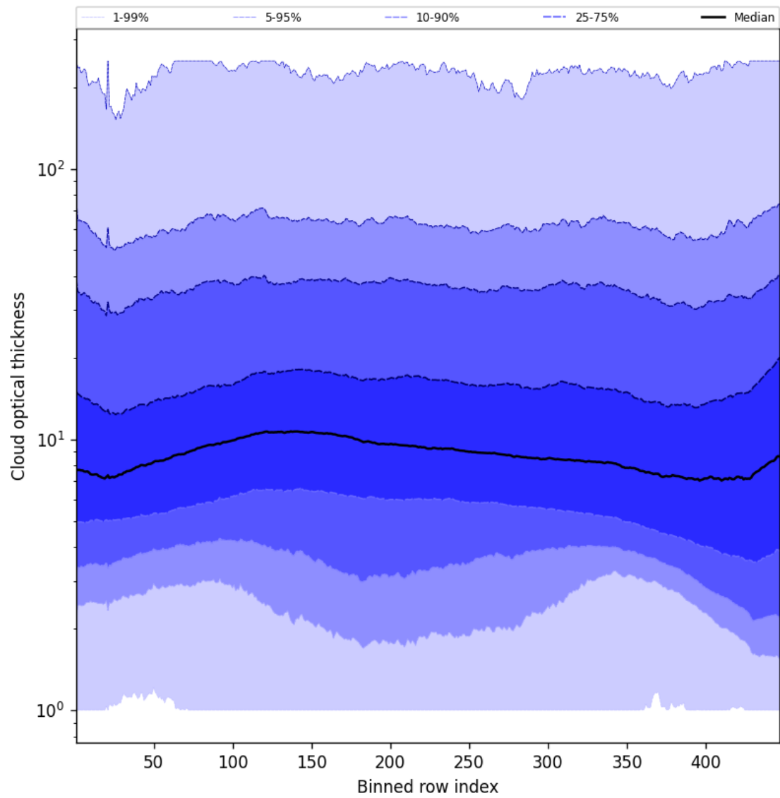
Figure 57: Along track statistics of “Cloud optical thickness” for 2024-11-28 to 2024-11-30
