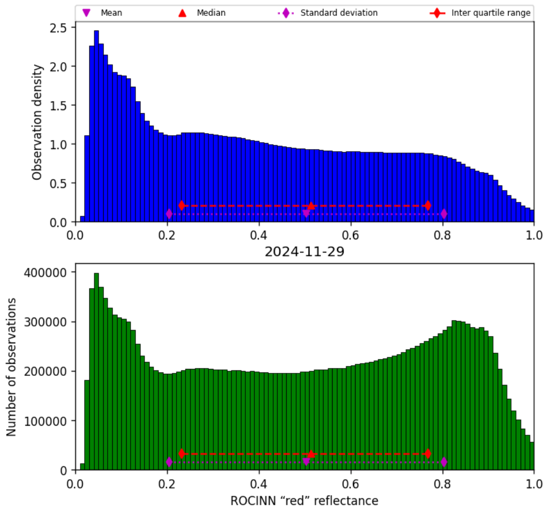
Figure 53: Histogram of “ROCINN “red” reflectance” for 2024-11-28 to 2024-11-30
