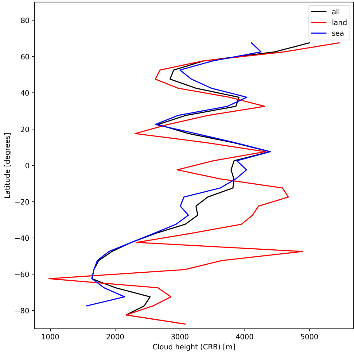
Figure 27: Zonal average of “Cloud height (CRB)” for 2024-11-28 to 2024-11-30.
