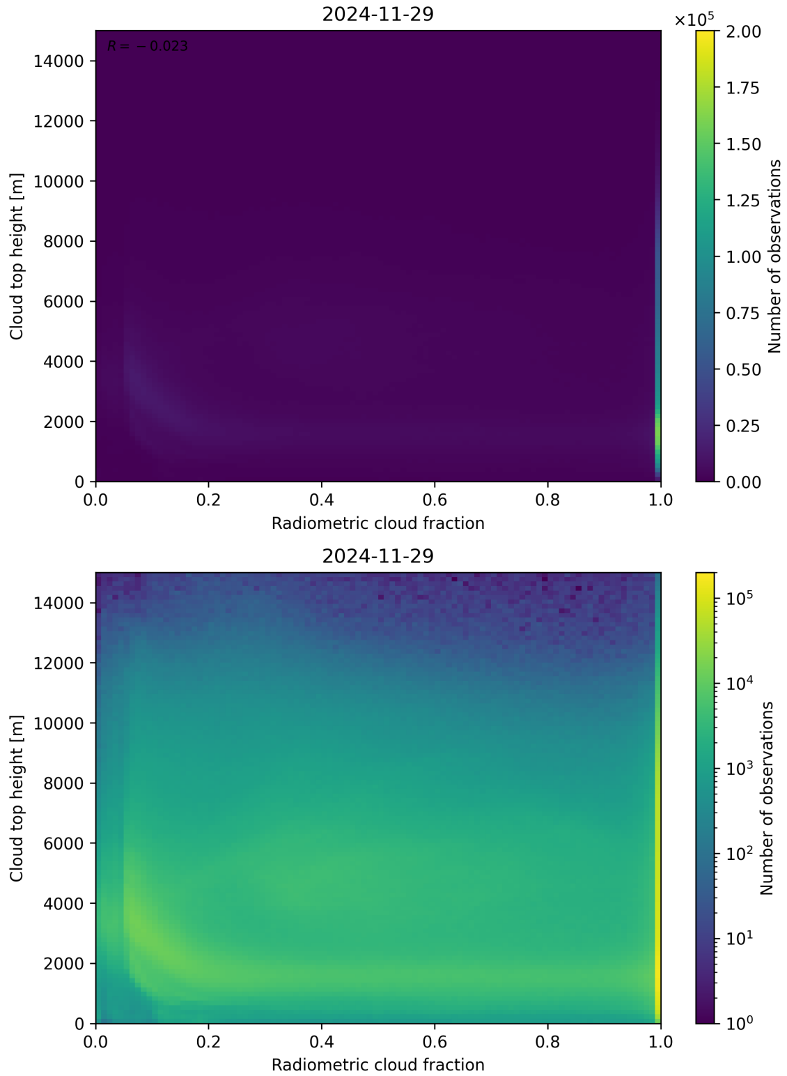
Figure 76: Scatter density plot of “Radiometric cloud fraction” against “Cloud top height” for 2024-11-28 to 2024-11-30.
