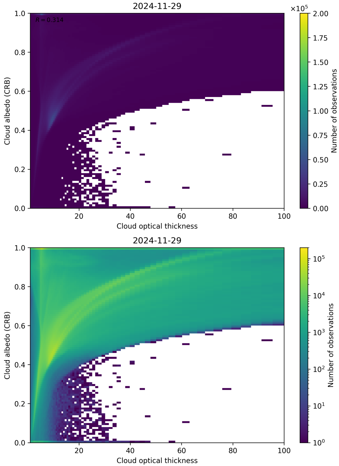
Figure 82: Scatter density plot of “Cloud optical thickness” against “Cloud albedo (CRB)” for 2024-11-28 to 2024-11-30.
