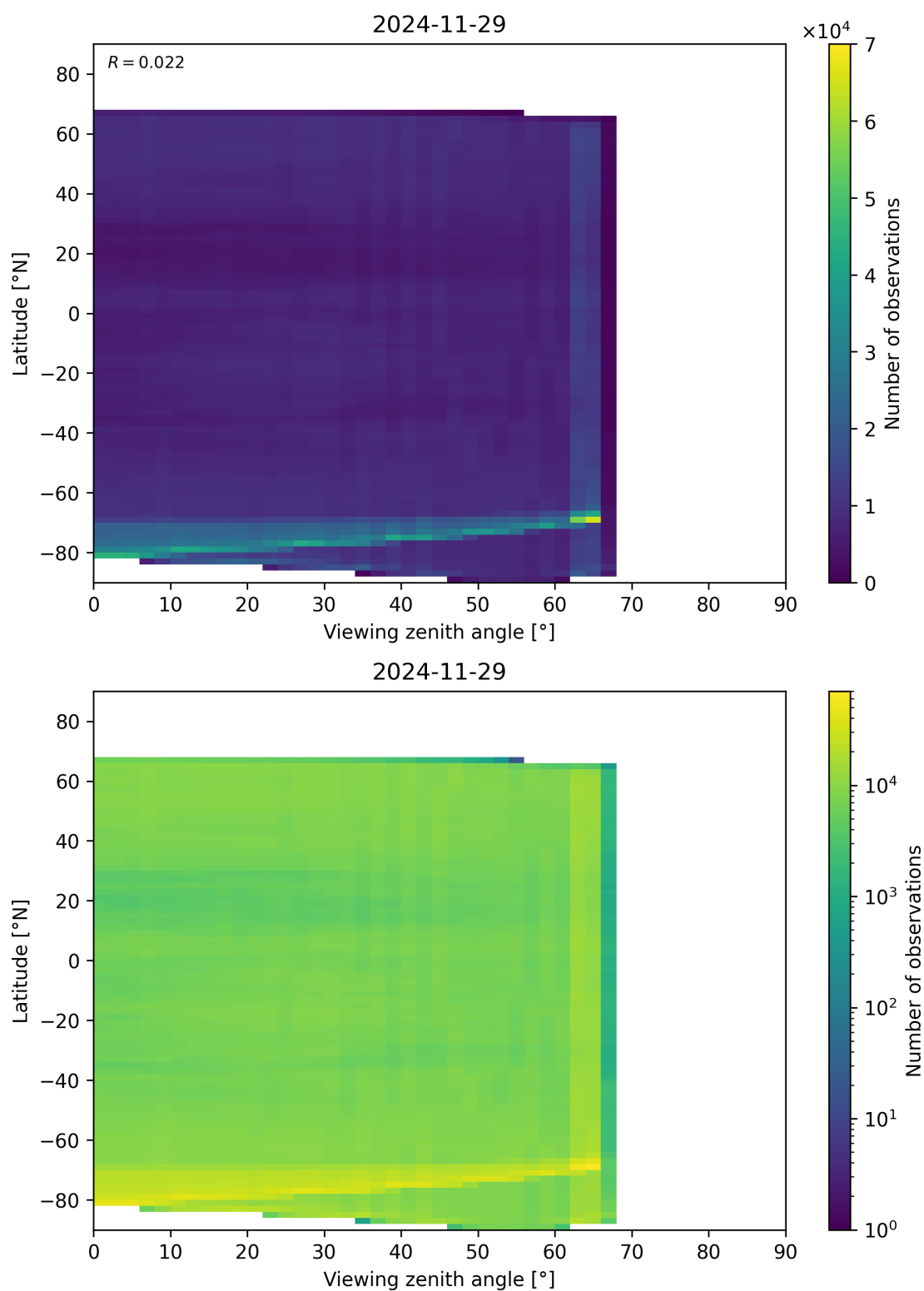
Figure 113: Scatter density plot of “Viewing zenith angle” against “Latitude” for 2024-11-28 to 2024-11-30.
