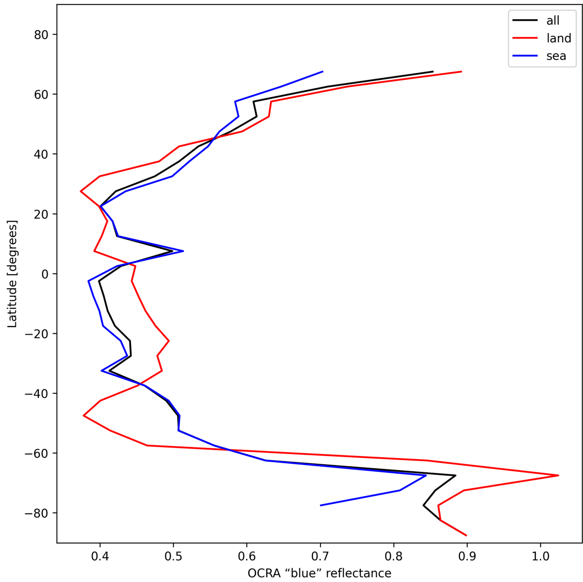
Figure 35: Zonal average of “OCRA “blue” reflectance” for 2024-11-28 to 2024-11-30.
