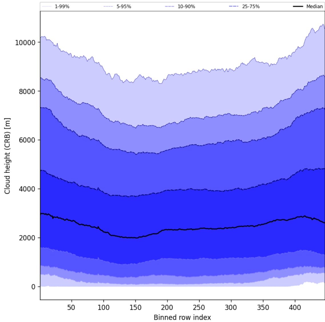
Figure 59: Along track statistics of “Cloud height (CRB)” for 2024-11-28 to 2024-11-30
