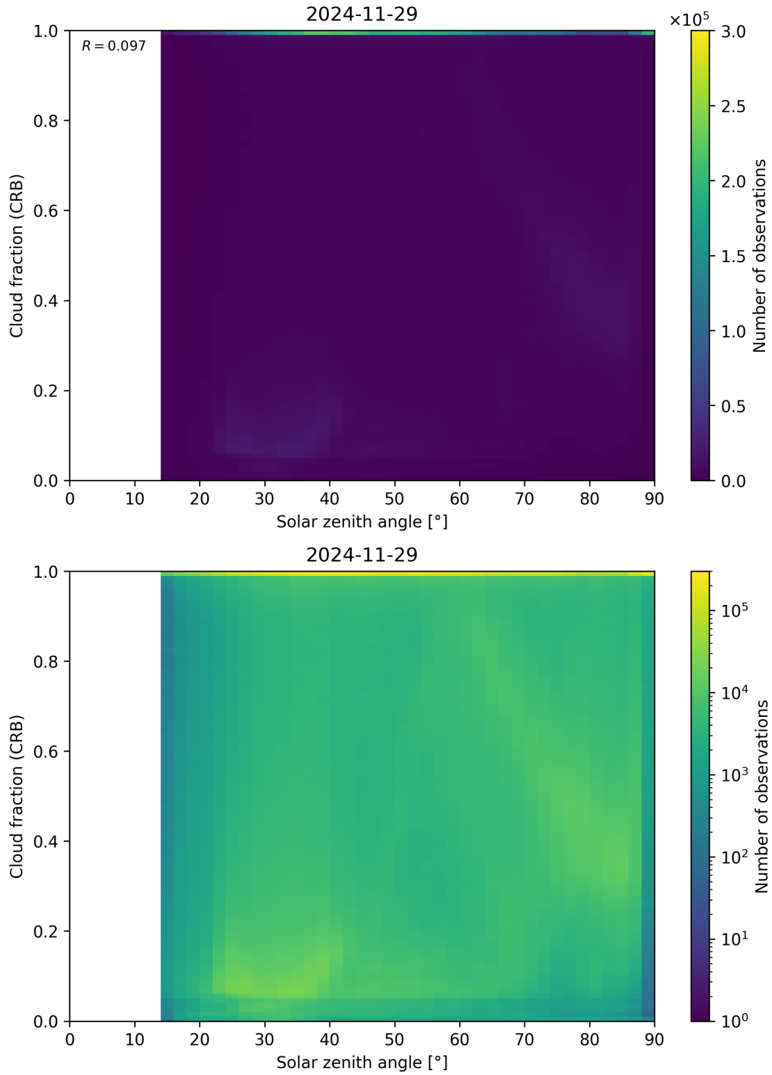
Figure 101: Scatter density plot of “Solar zenith angle” against “Cloud fraction (CRB)” for 2024-11-28 to 2024-11-30.
