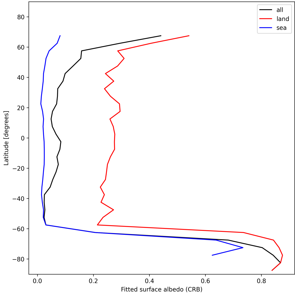
Figure 30: Zonal average of “Fitted surface albedo (CRB)” for 2024-11-28 to 2024-11-30.
