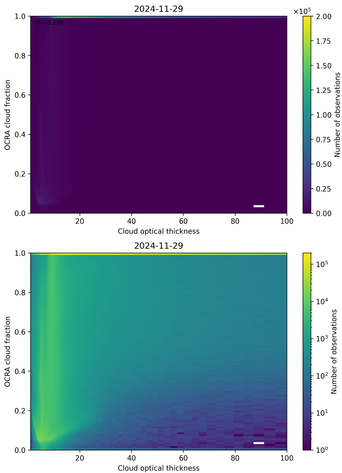
Figure 83: Scatter density plot of “Cloud optical thickness” against “OCRA cloud fraction” for 2024-11-28 to 2024-11-30.
