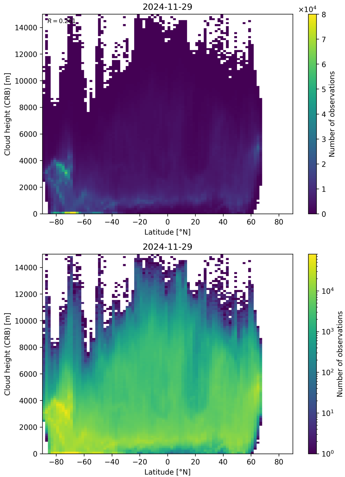
Figure 95: Scatter density plot of “Latitude” against “Cloud height (CRB)” for 2024-11-28 to 2024-11-30.
