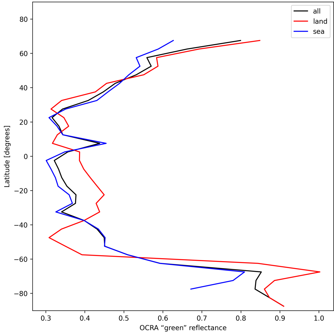
Figure 36: Zonal average of “OCRA “green” reflectance” for 2024-11-28 to 2024-11-30.
