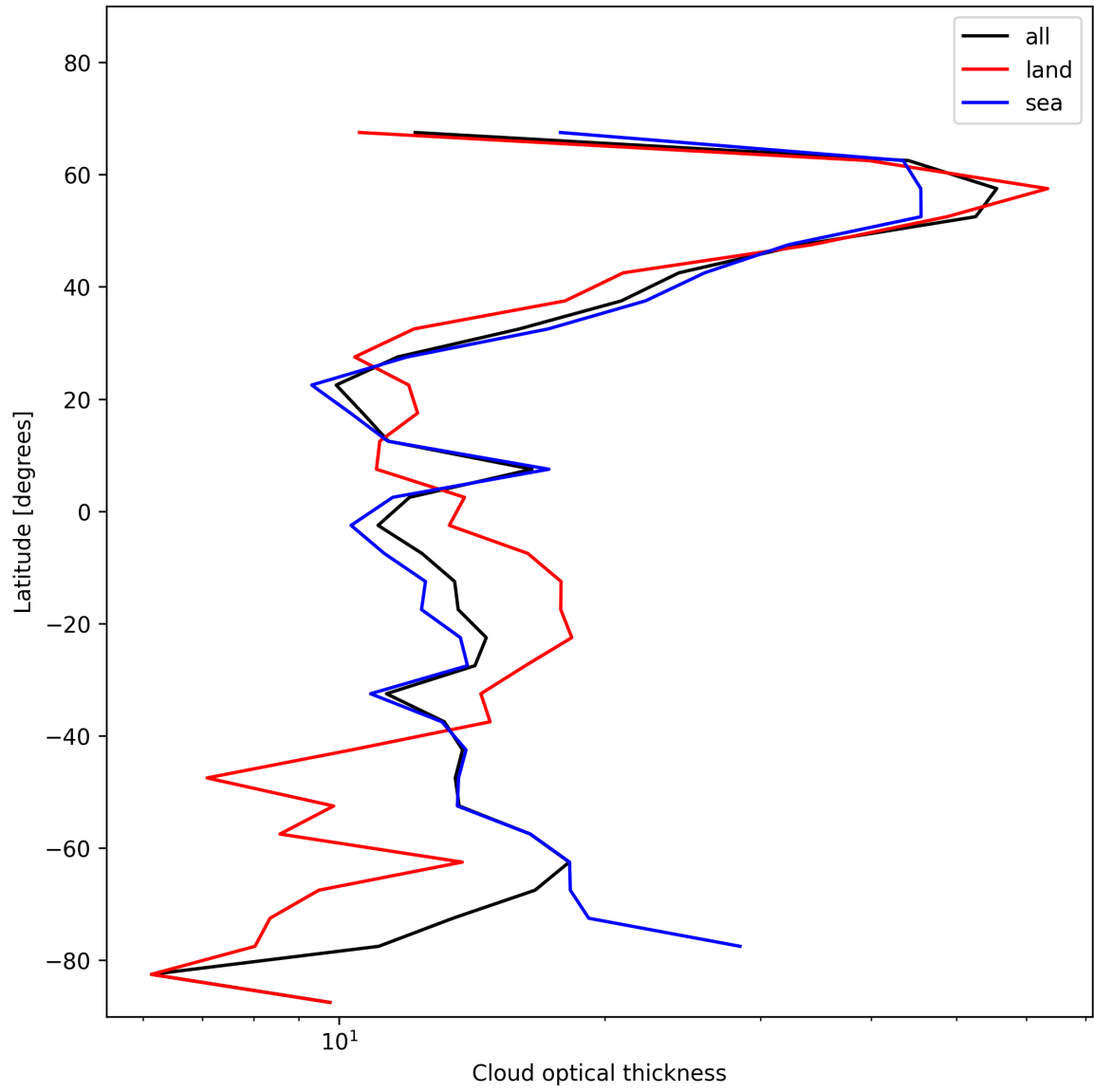
Figure 25: Zonal average of “Cloud optical thickness” for 2024-11-28 to 2024-11-30.
