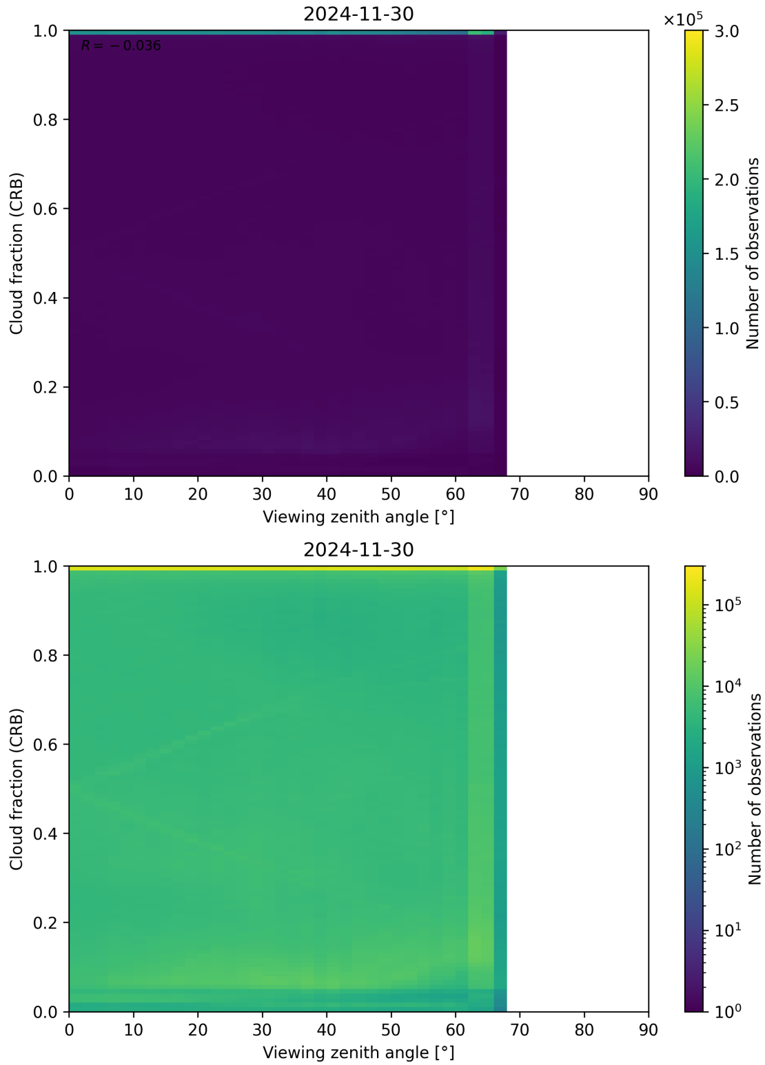
Figure 109: Scatter density plot of “Viewing zenith angle” against “Cloud fraction (CRB)” for 2024-11-30 to 2024-12-01.
