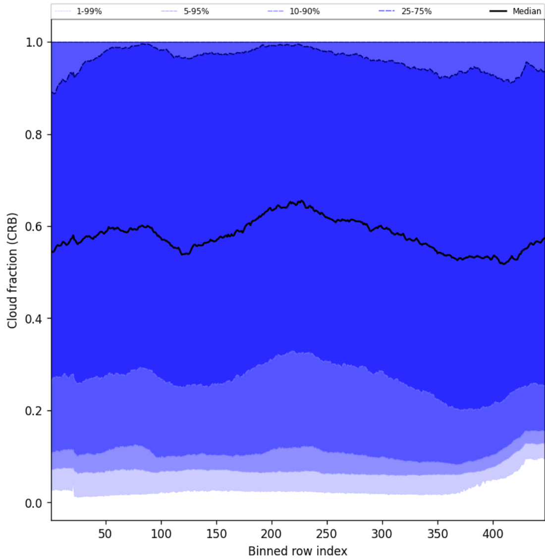
Figure 58: Along track statistics of “Cloud fraction (CRB)” for 2024-11-30 to 2024-12-01
