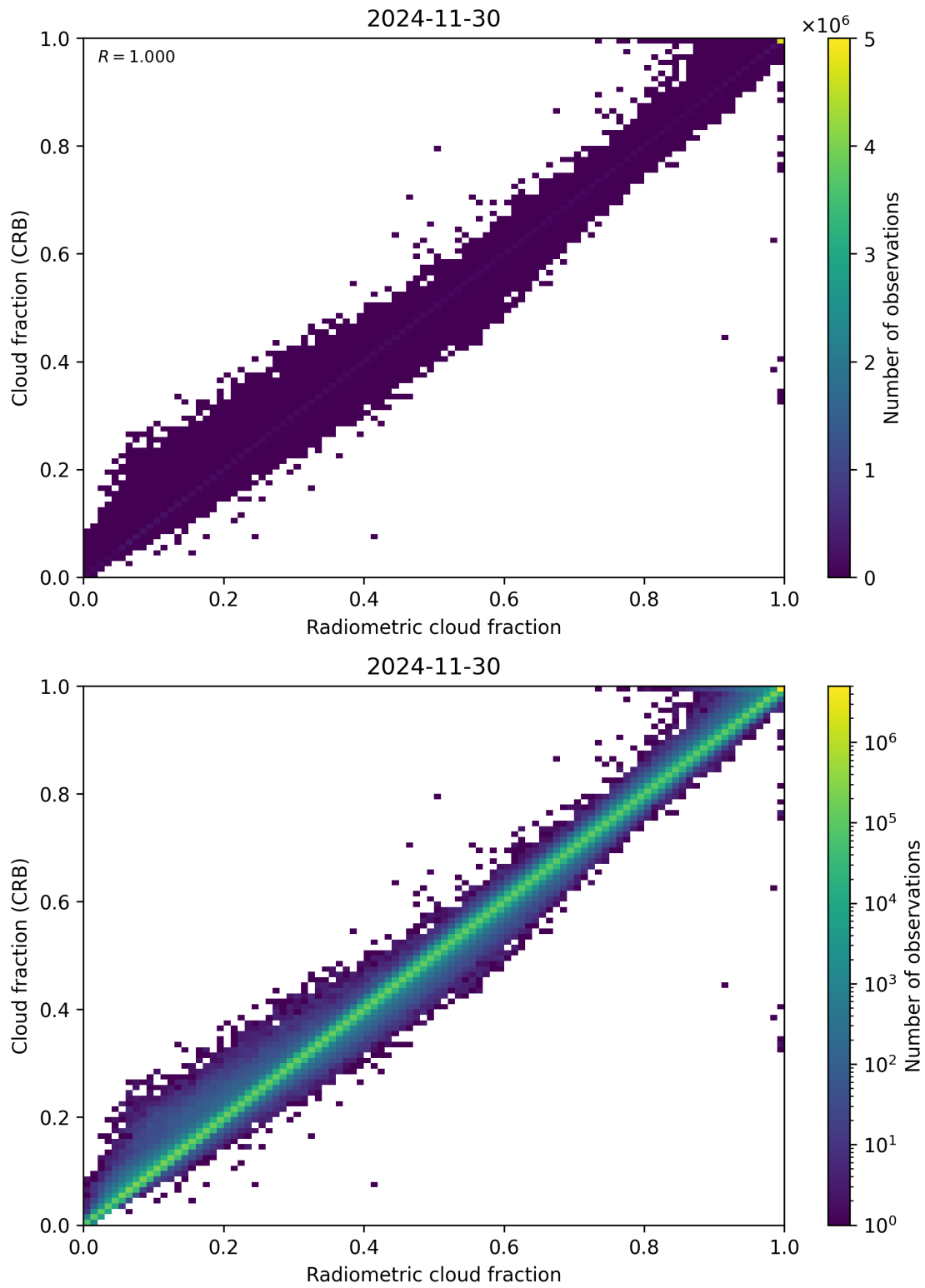
Figure 73: Scatter density plot of “Radiometric cloud fraction” against “Cloud fraction (CRB)” for 2024-11-30 to 2024-12-01.
