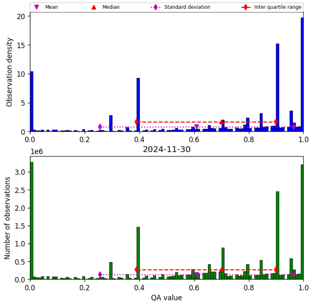
Figure 38: Histogram of “QA value” for 2024-11-30 to 2024-12-01
