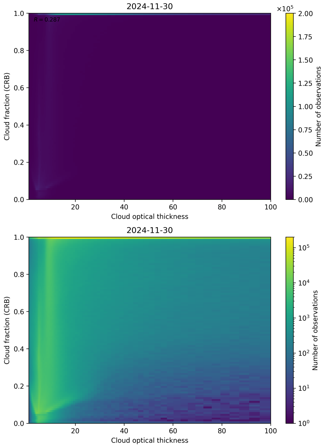
Figure 84: Scatter density plot of “Cloud optical thickness” against “Cloud fraction (CRB)” for 2024-11-30 to 2024-12-01.
