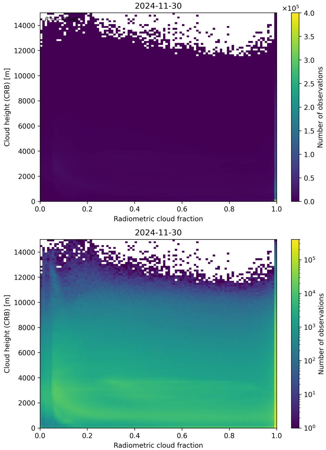
Figure 74: Scatter density plot of “Radiometric cloud fraction” against “Cloud height (CRB)” for 2024-11-30 to 2024-12-01.
