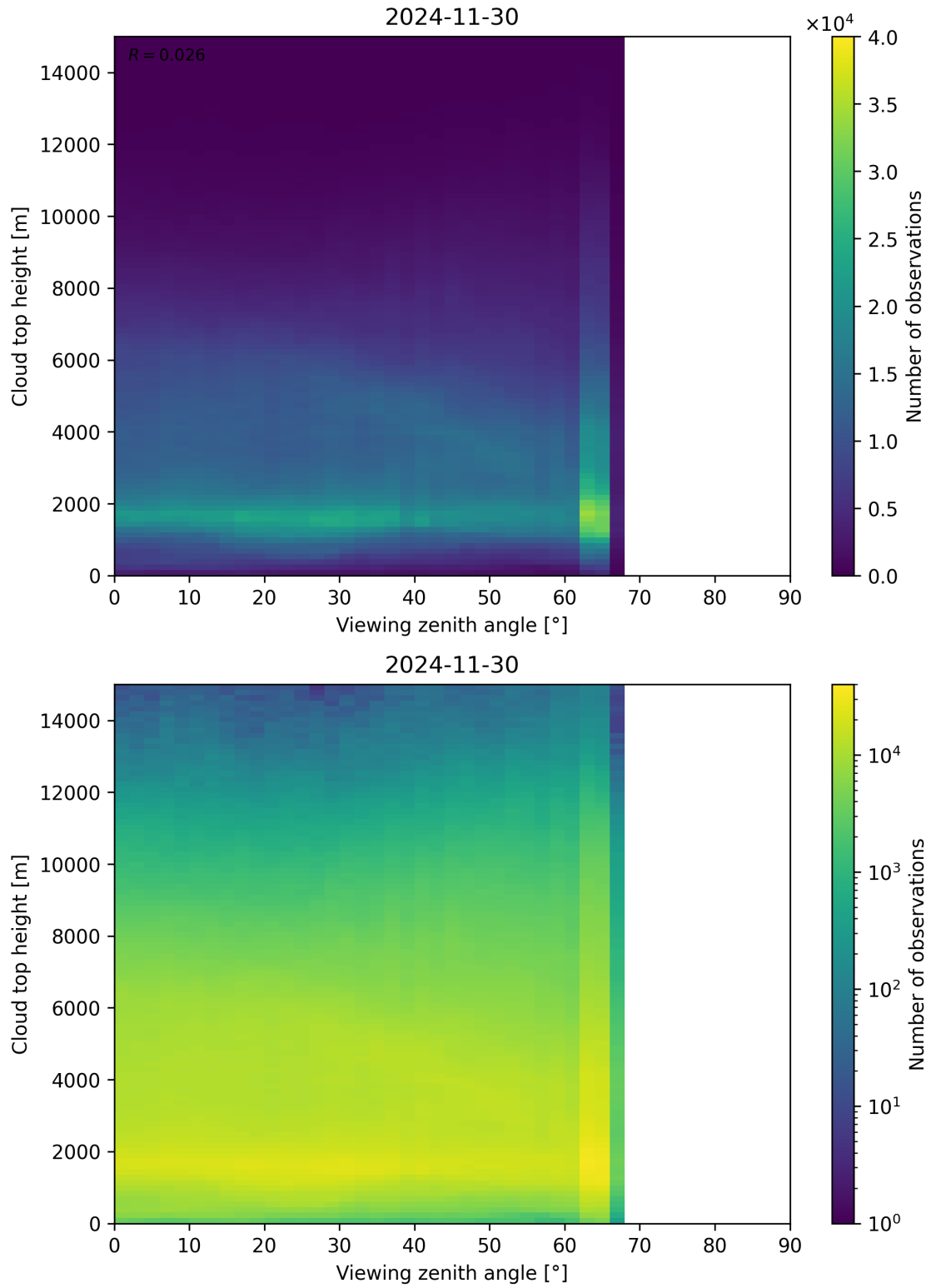
Figure 112: Scatter density plot of “Viewing zenith angle” against “Cloud top height” for 2024-11-30 to 2024-12-01.
