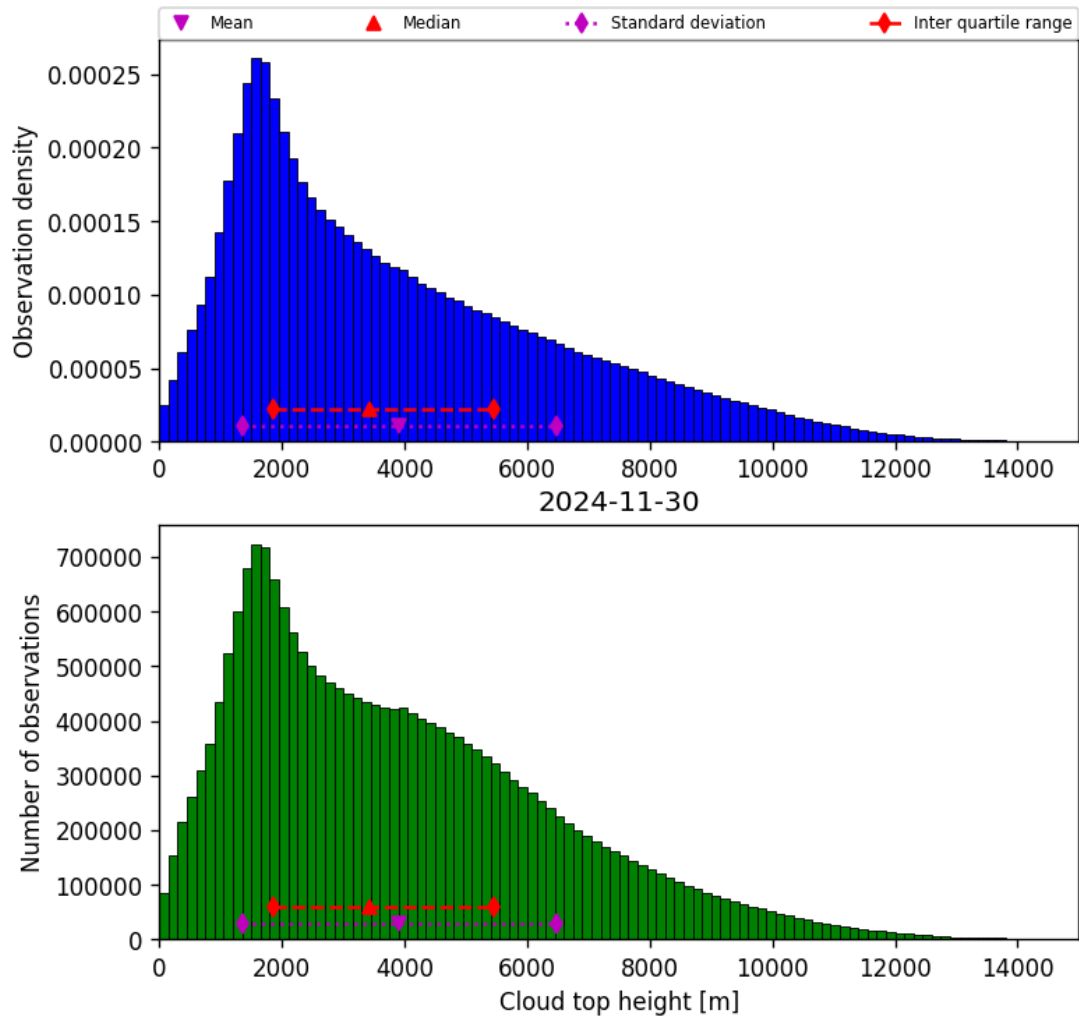
Figure 40: Histogram of “Cloud top height” for 2024-11-30 to 2024-12-01
