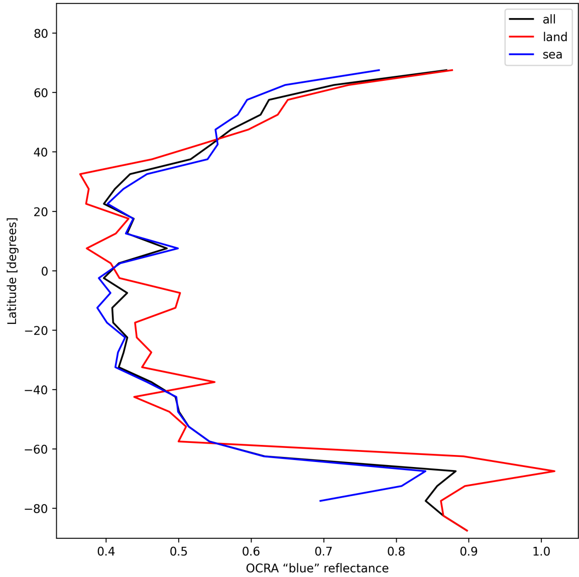
Figure 35: Zonal average of "OCRA "blue" reflectance" for 2024-11-30 to 2024-12-01.
