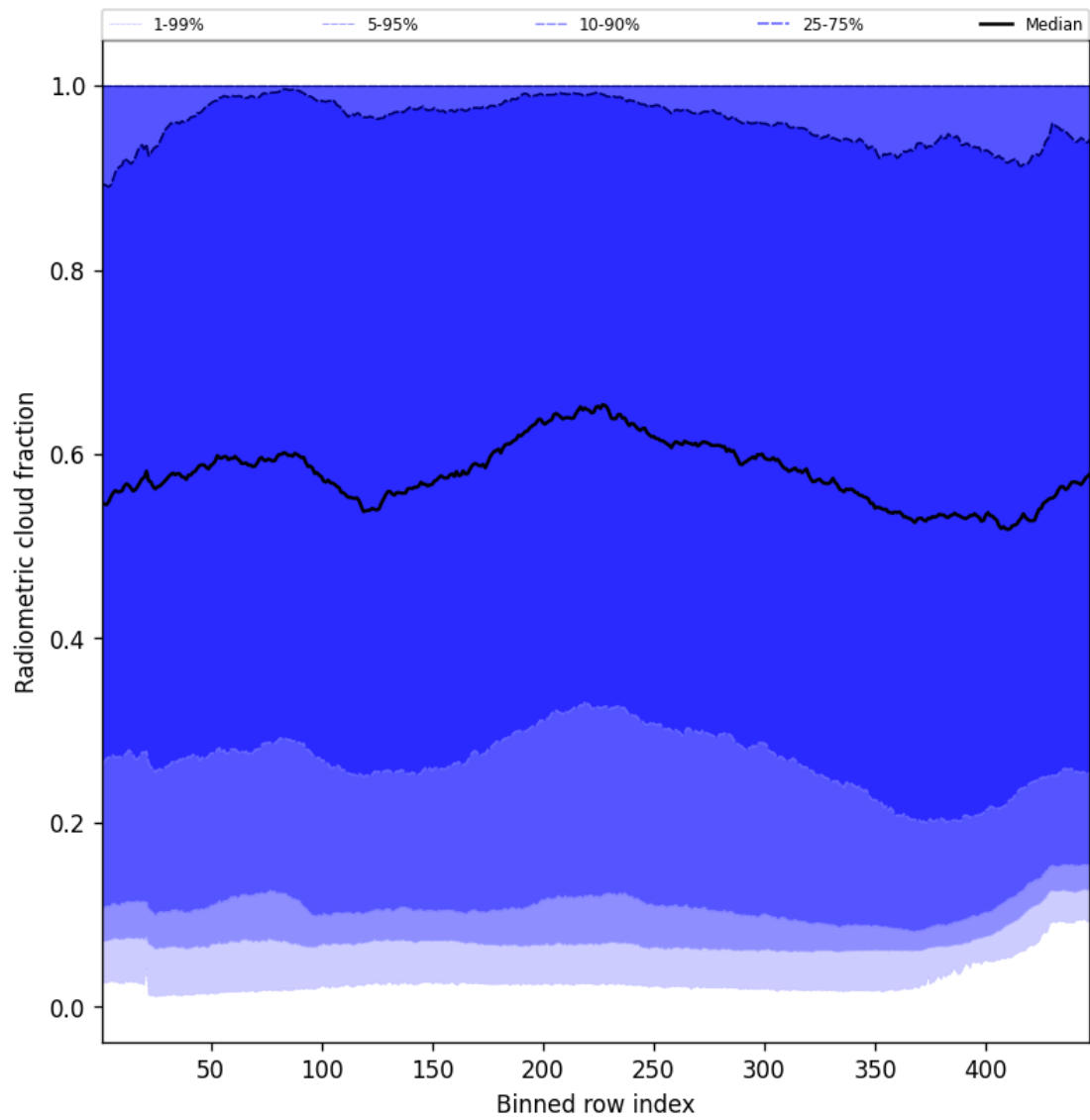
Figure 55: Along track statistics of “Radiometric cloud fraction” for 2024-11-30 to 2024-12-01
