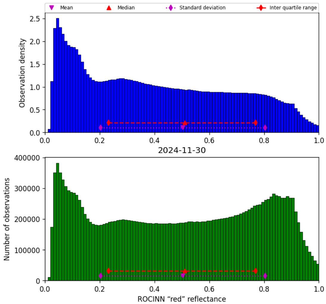
Figure 53: Histogram of “ROCINN “red” reflectance” for 2024-11-30 to 2024-12-01
