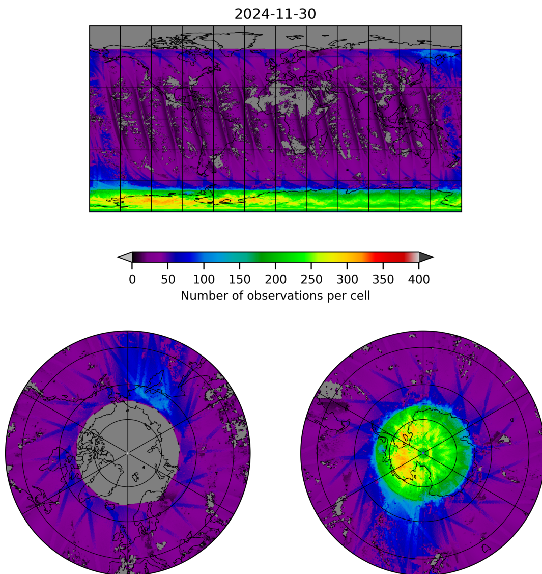
Figure 21: Map of the number of observations for 2024-11-30 to 2024-12-01
