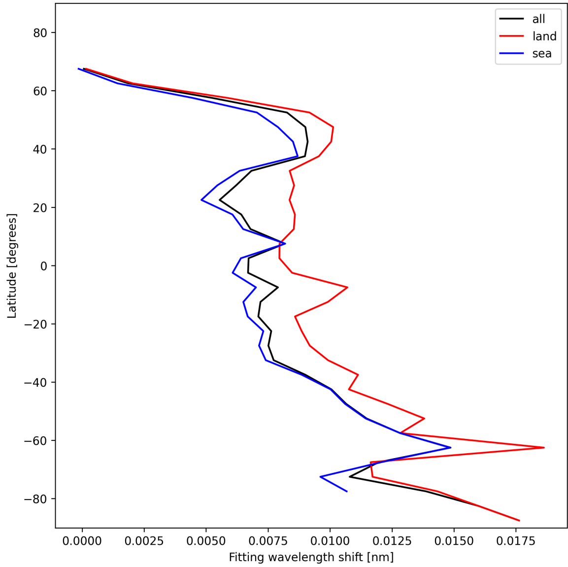
Figure 33: Zonal average of “Fitting wavelength shift” for 2024-11-30 to 2024-12-01.
