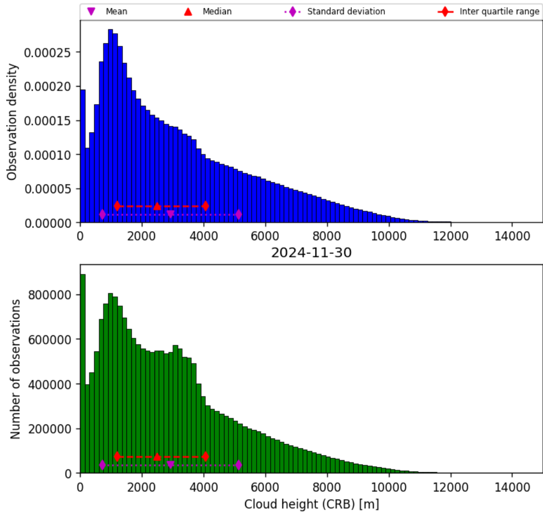
Figure 43: Histogram of “Cloud height (CRB)” for 2024-11-30 to 2024-12-01
