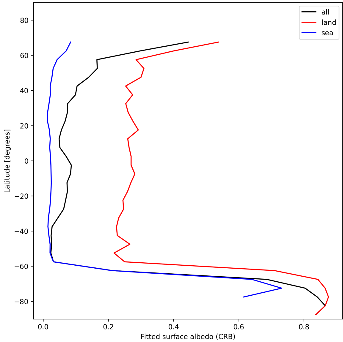
Figure 30: Zonal average of “Fitted surface albedo (CRB)” for 2024-11-30 to 2024-12-01.
