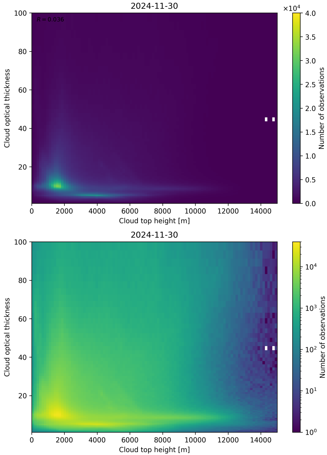
Figure 90: Scatter density plot of “Cloud top height” against “Cloud optical thickness” for 2024-11-30 to 2024-12-01.
