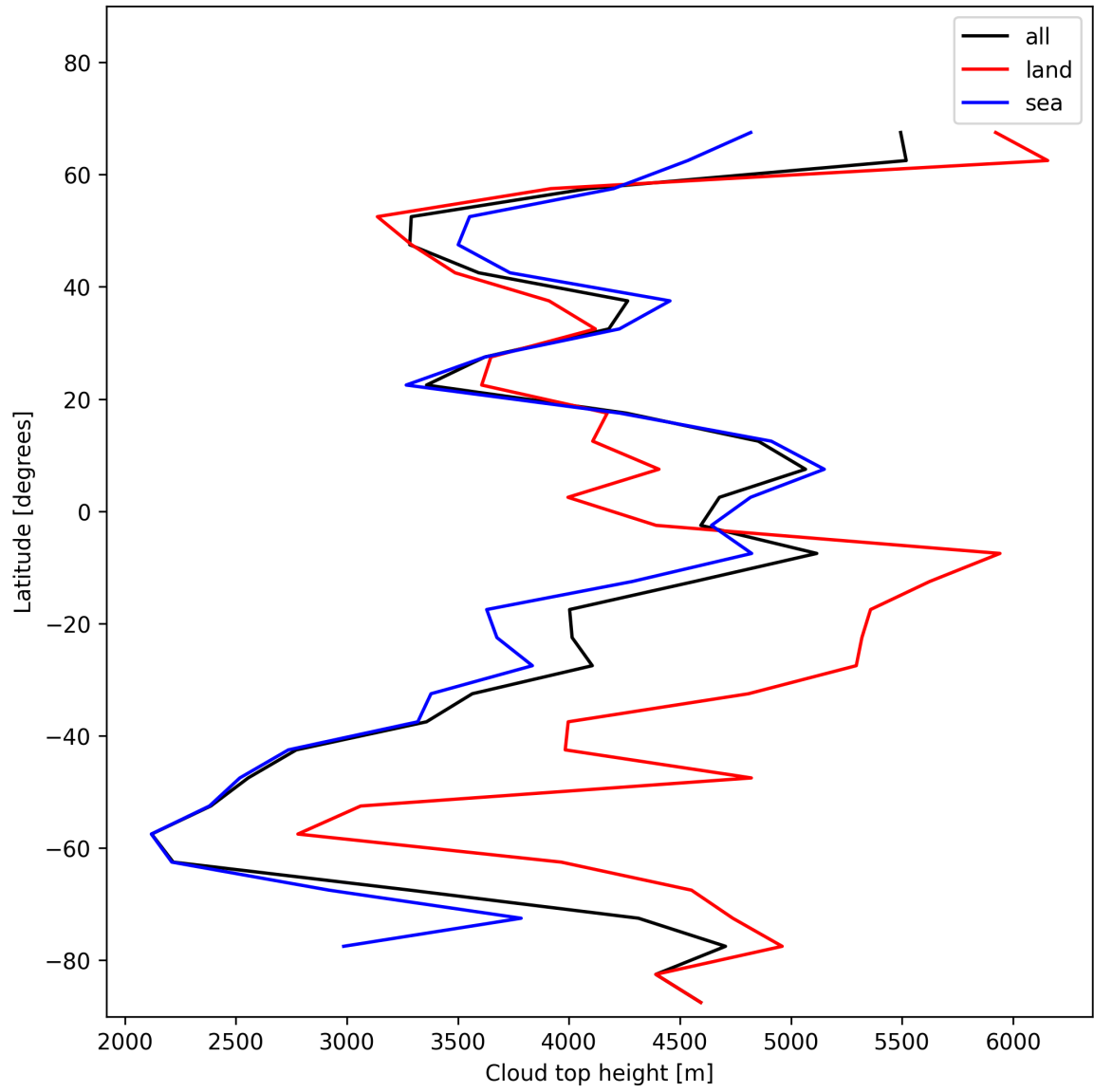
Figure 24: Zonal average of “Cloud top height” for 2024-11-30 to 2024-12-01.
