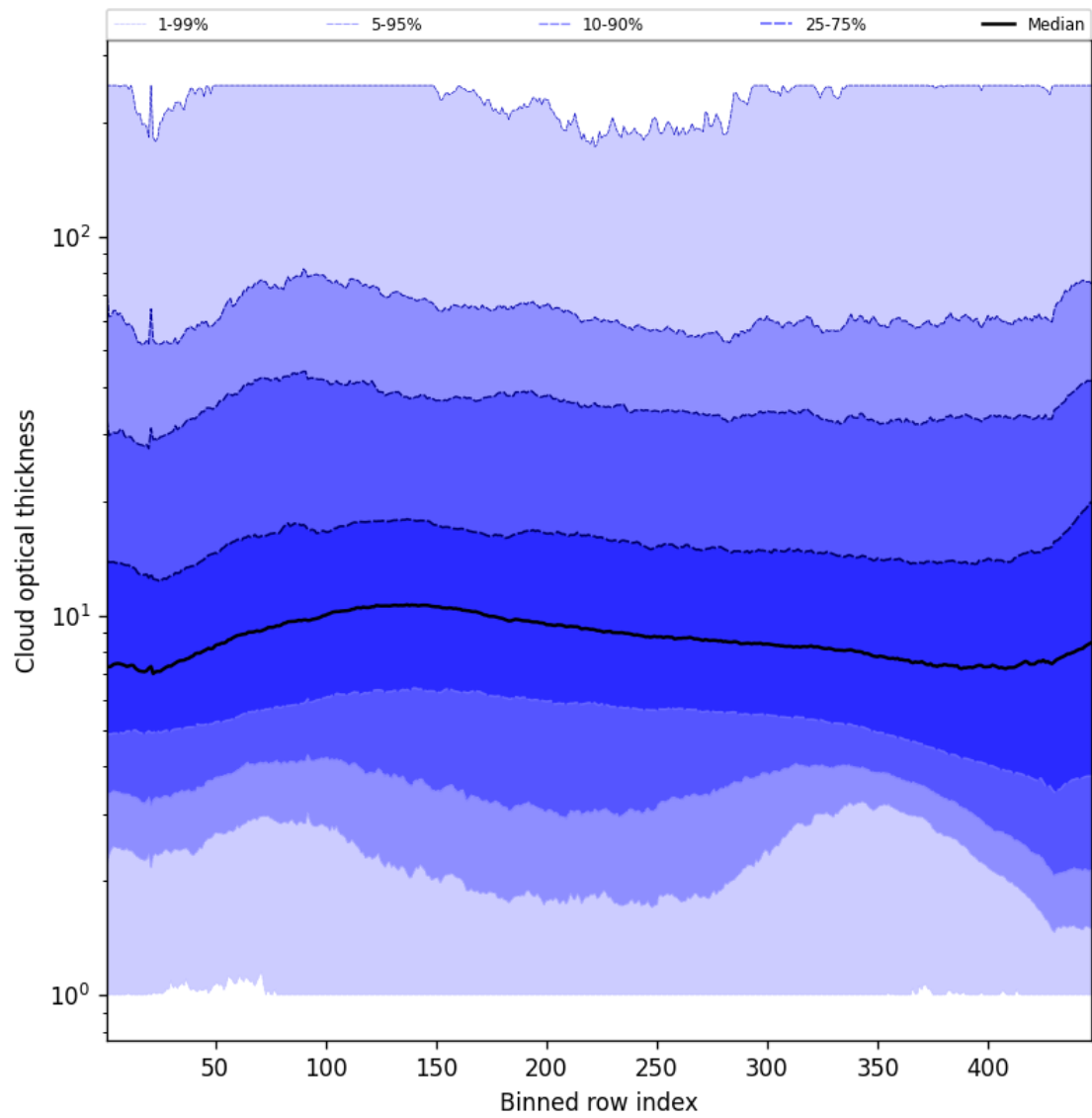
Figure 57: Along track statistics of “Cloud optical thickness” for 2024-11-30 to 2024-12-01
