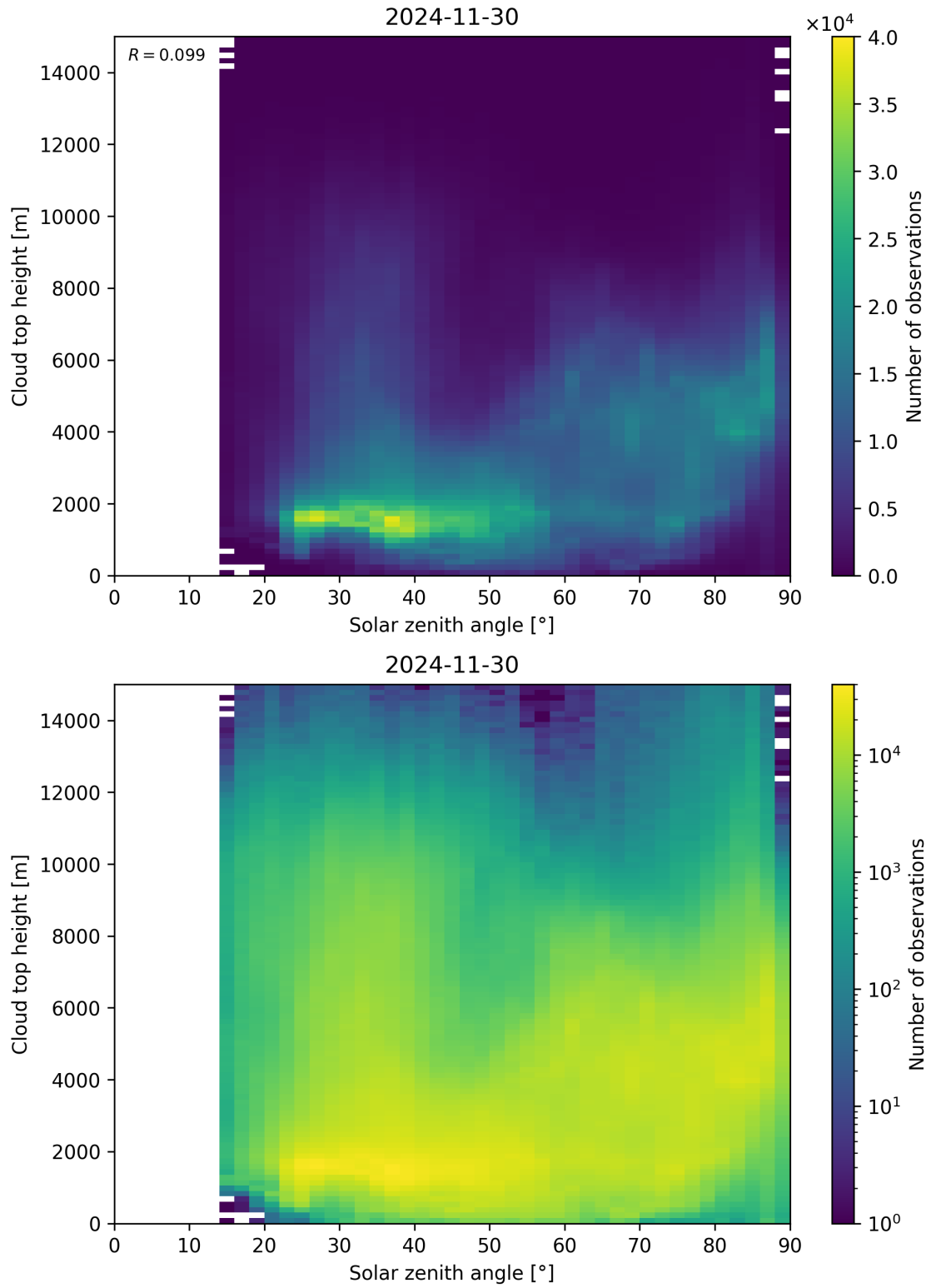
Figure 104: Scatter density plot of “Solar zenith angle” against “Cloud top height” for 2024-11-30 to 2024-12-01.
