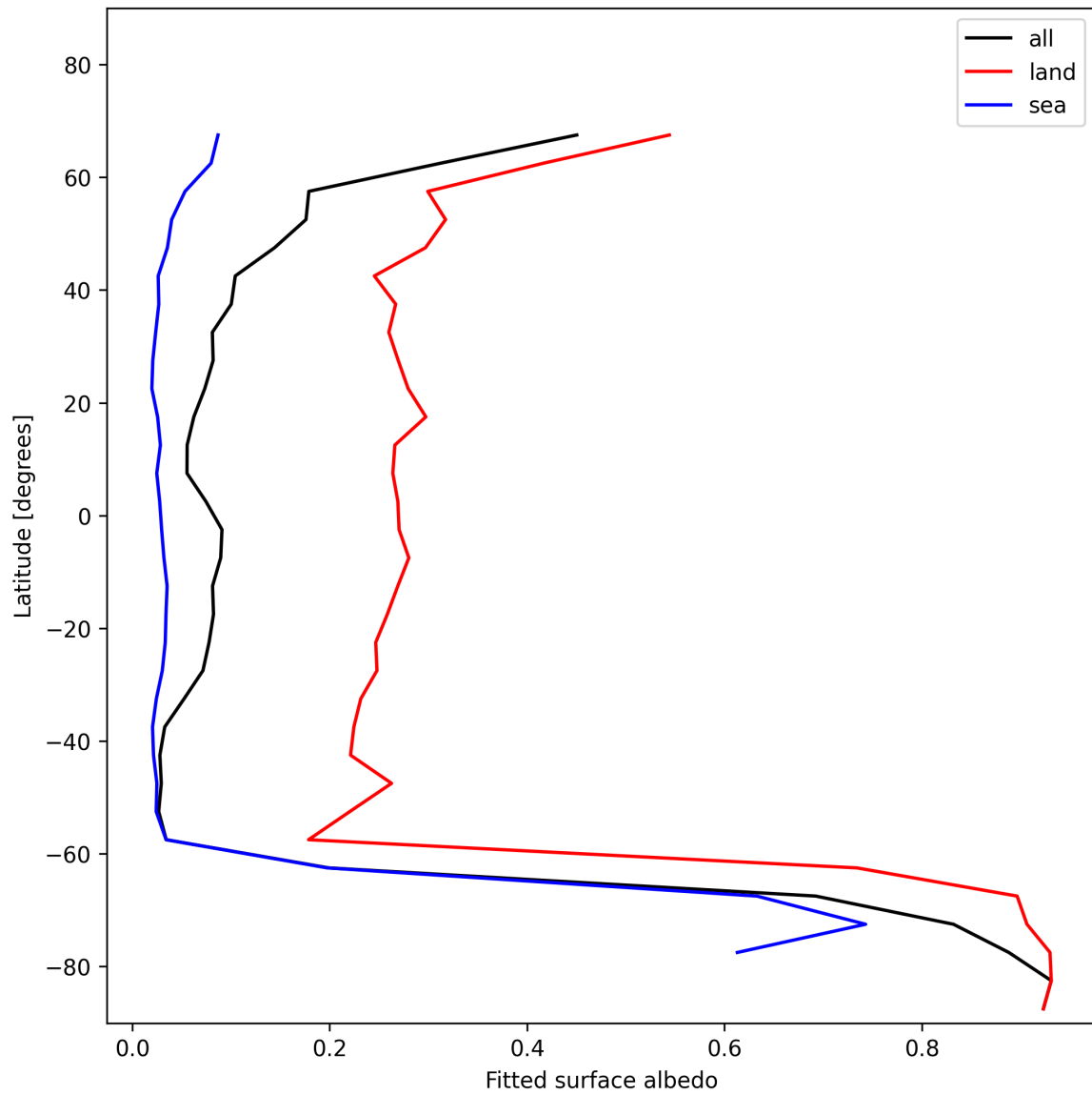
Figure 29: Zonal average of “Fitted surface albedo” for 2024-11-30 to 2024-12-01.
