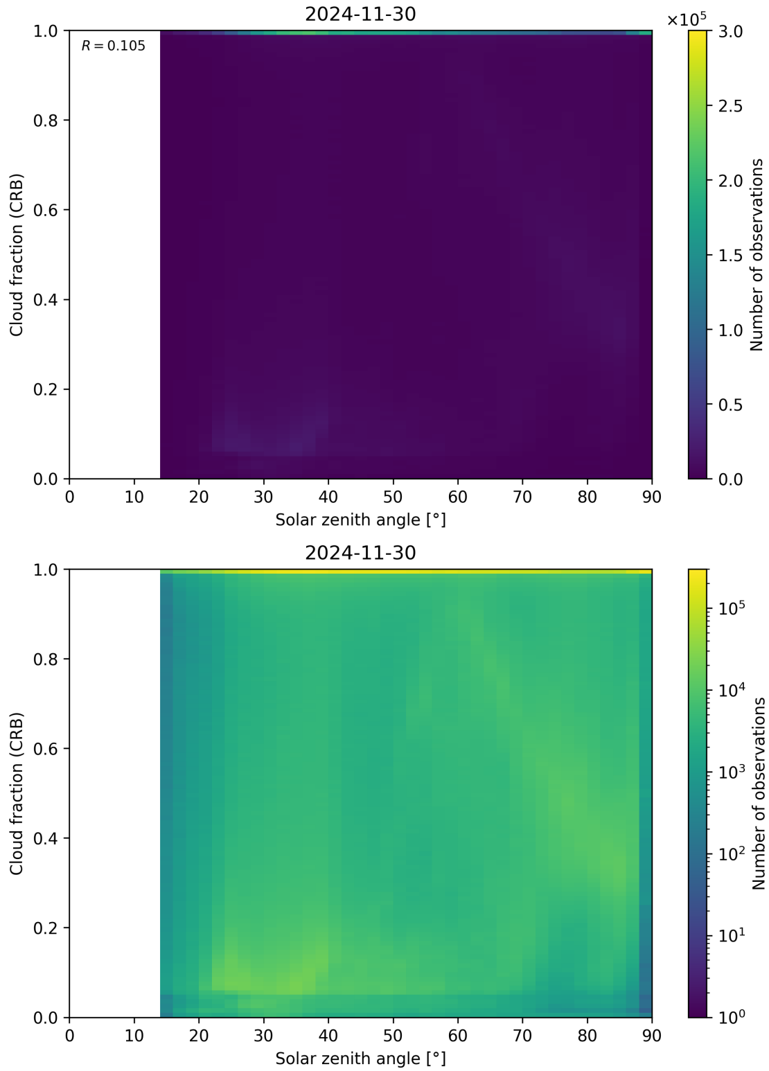
Figure 101: Scatter density plot of “Solar zenith angle” against “Cloud fraction (CRB)” for 2024-11-30 to 2024-12-01.
