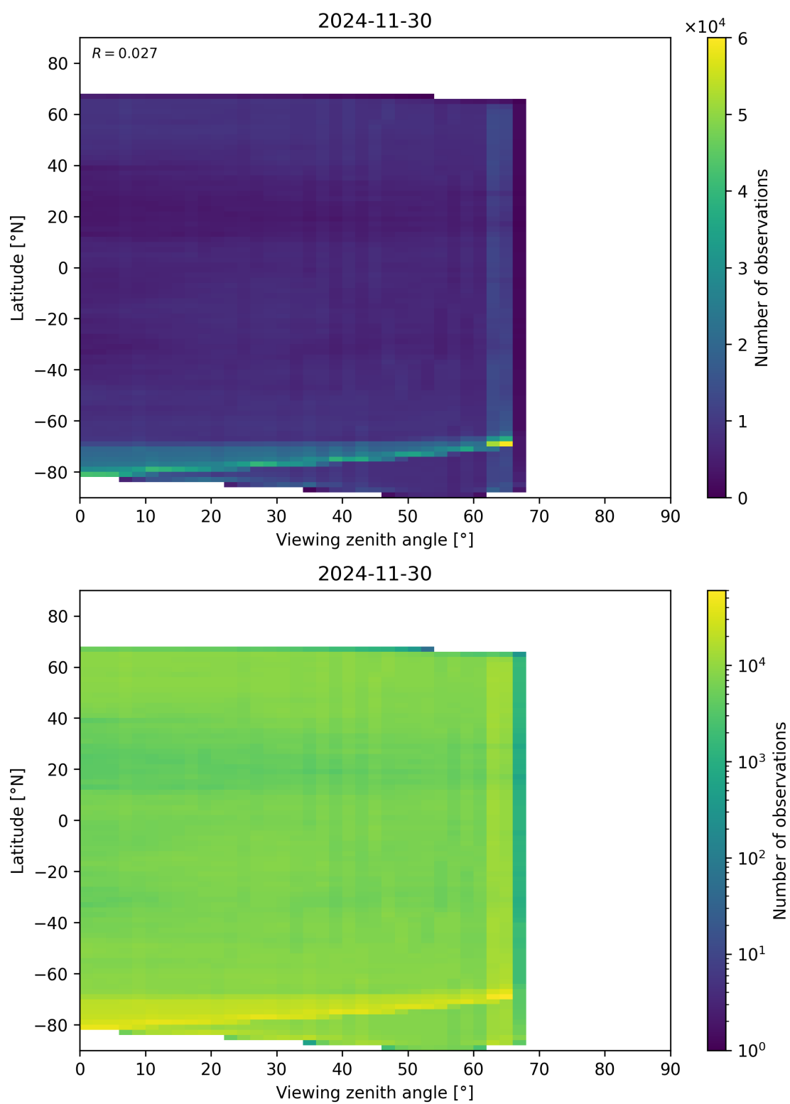
Figure 113: Scatter density plot of “Viewing zenith angle” against “Latitude” for 2024-11-30 to 2024-12-01.
