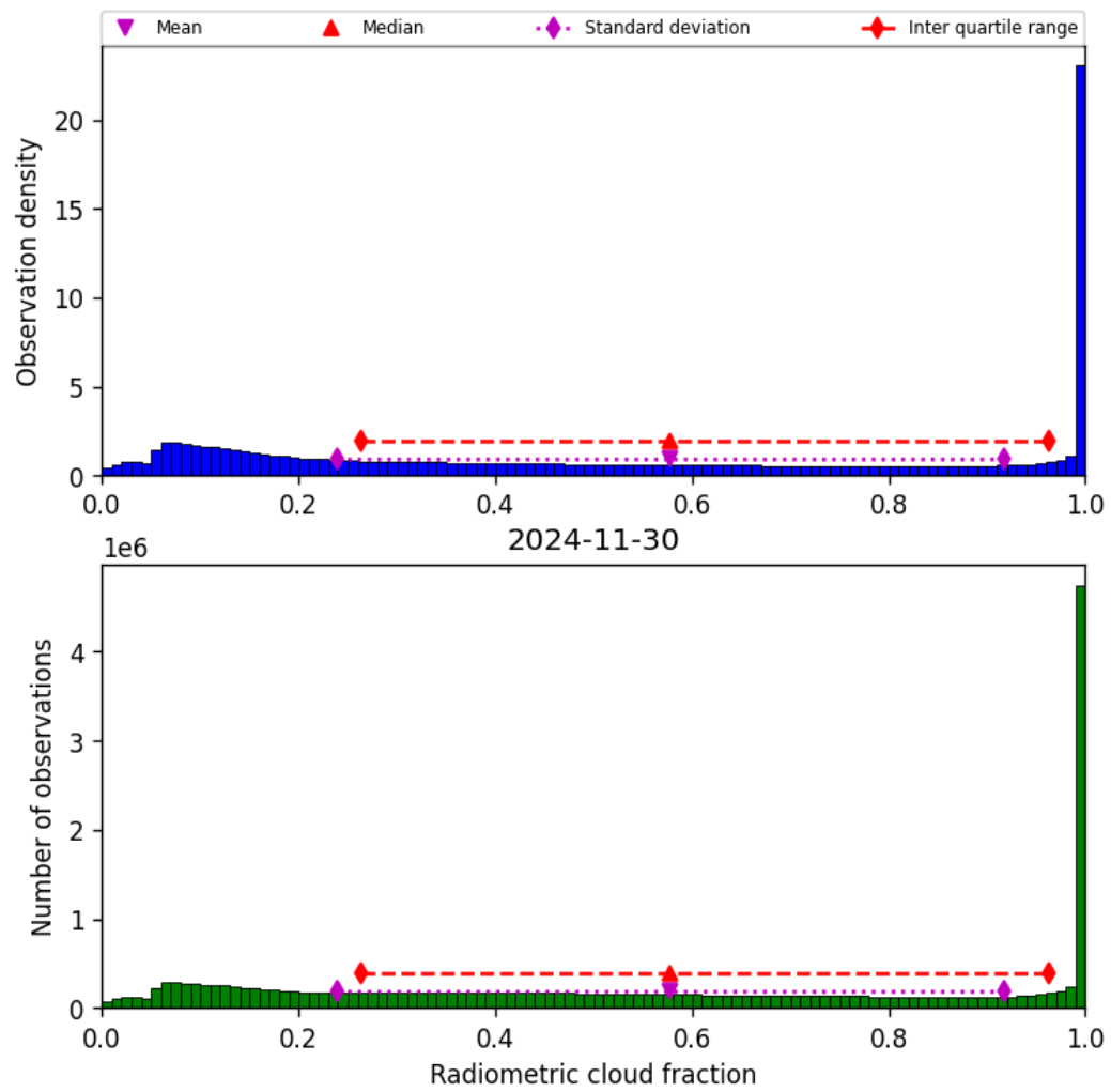
Figure 39: Histogram of “Radiometric cloud fraction” for 2024-11-30 to 2024-12-01
