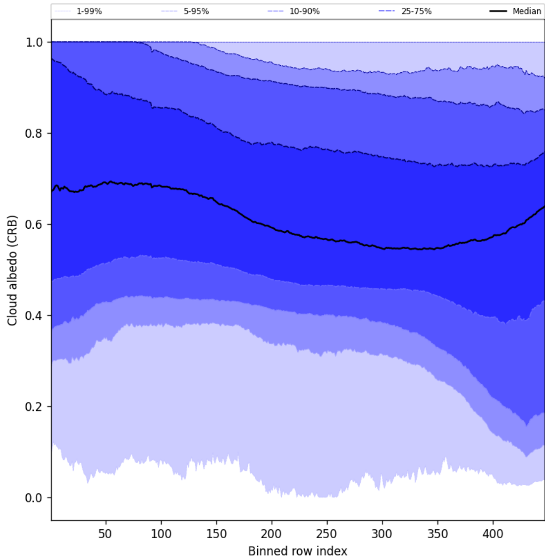
Figure 60: Along track statistics of “Cloud albedo (CRB)” for 2024-11-30 to 2024-12-01
