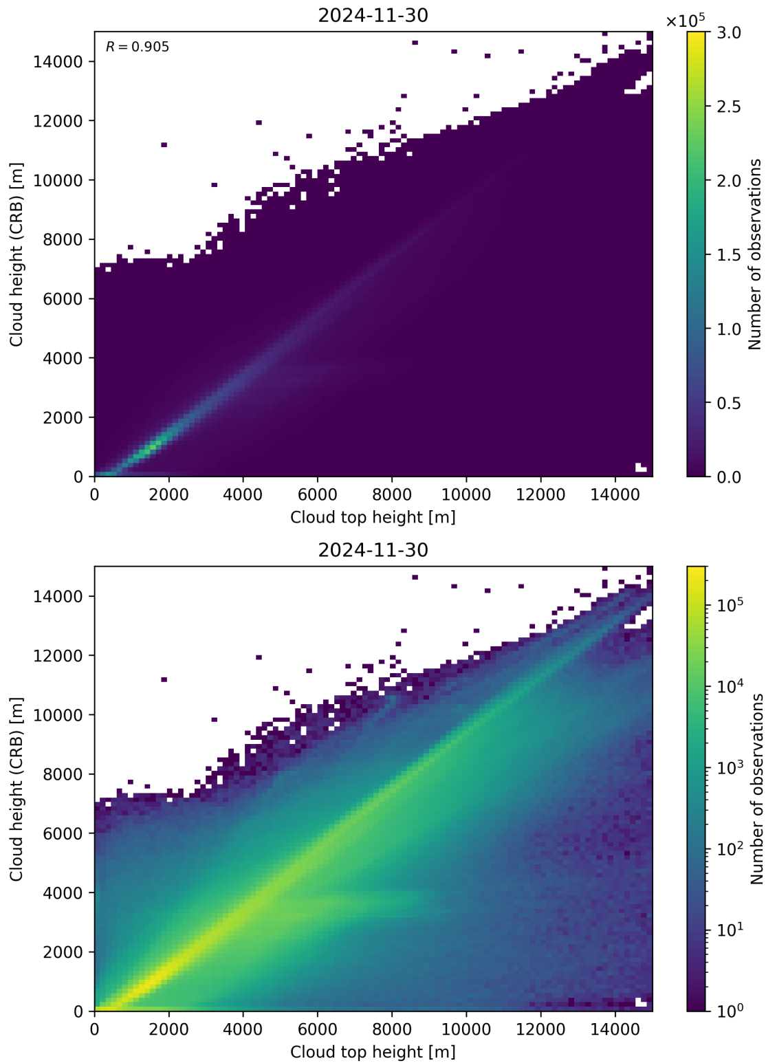
Figure 89: Scatter density plot of “Cloud top height” against “Cloud height (CRB)” for 2024-11-30 to 2024-12-01.
