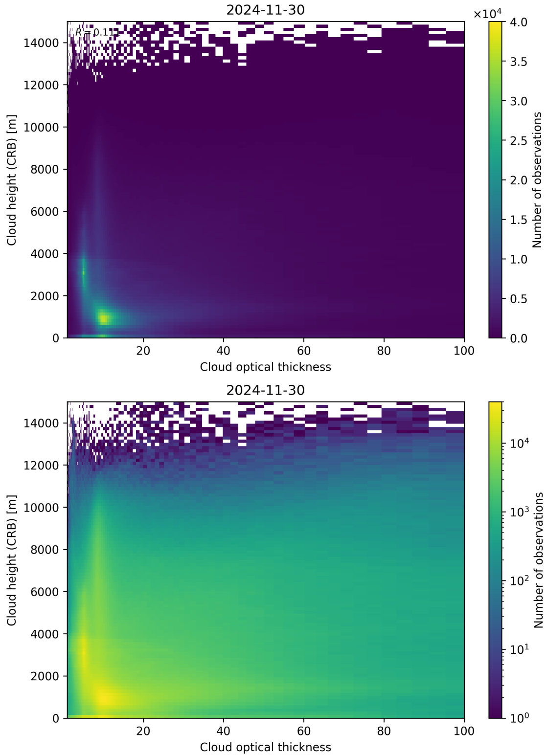
Figure 85: Scatter density plot of “Cloud optical thickness” against “Cloud height (CRB)” for 2024-11-30 to 2024-12-01.
