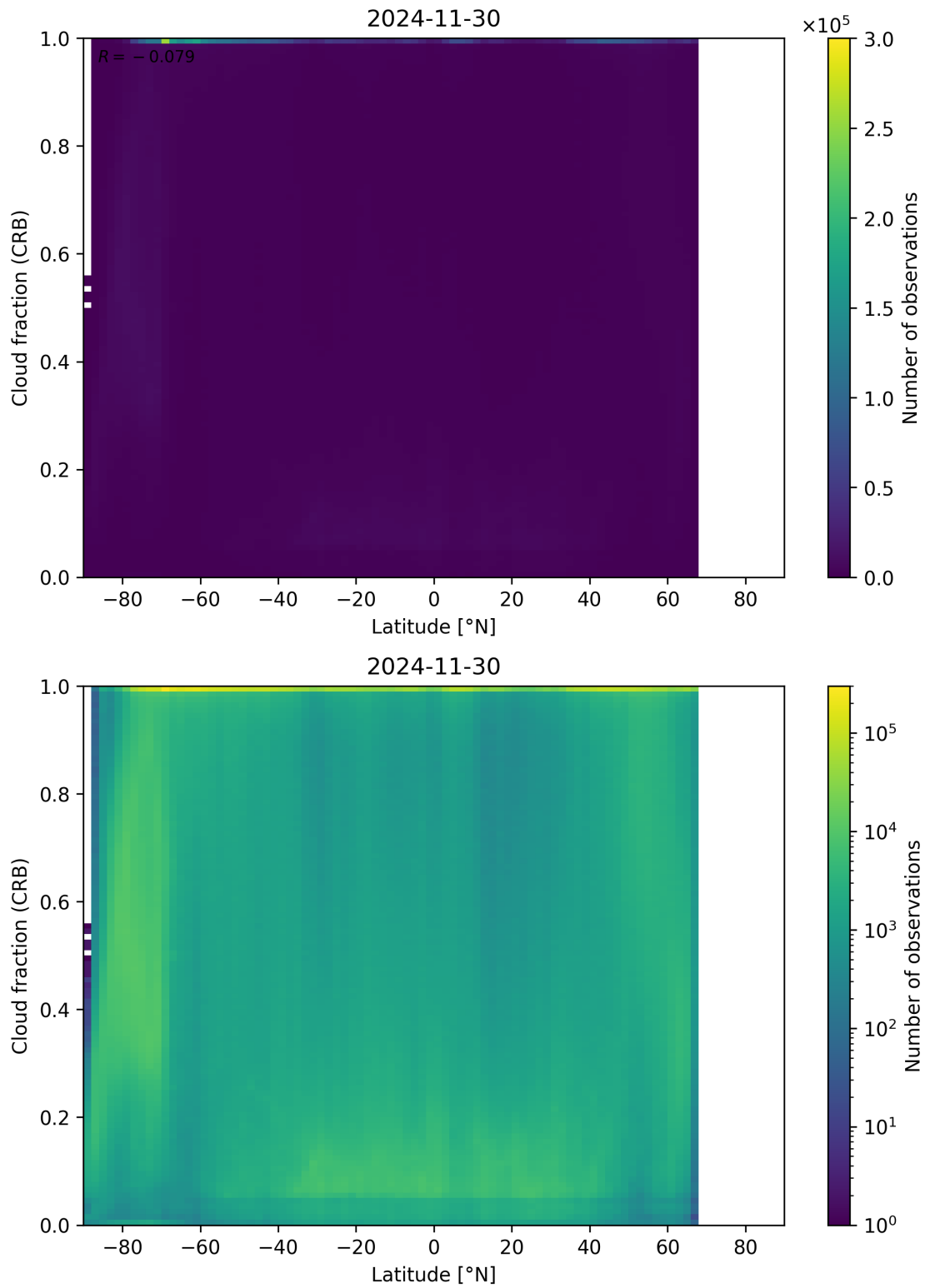
Figure 94: Scatter density plot of “Latitude” against “Cloud fraction (CRB)” for 2024-11-30 to 2024-12-01.
