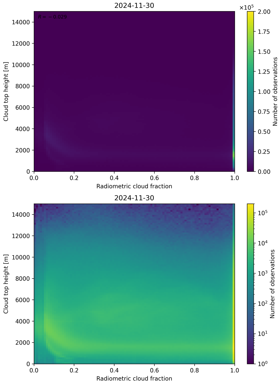
Figure 76: Scatter density plot of “Radiometric cloud fraction” against “Cloud top height” for 2024-11-30 to 2024-12-01.
