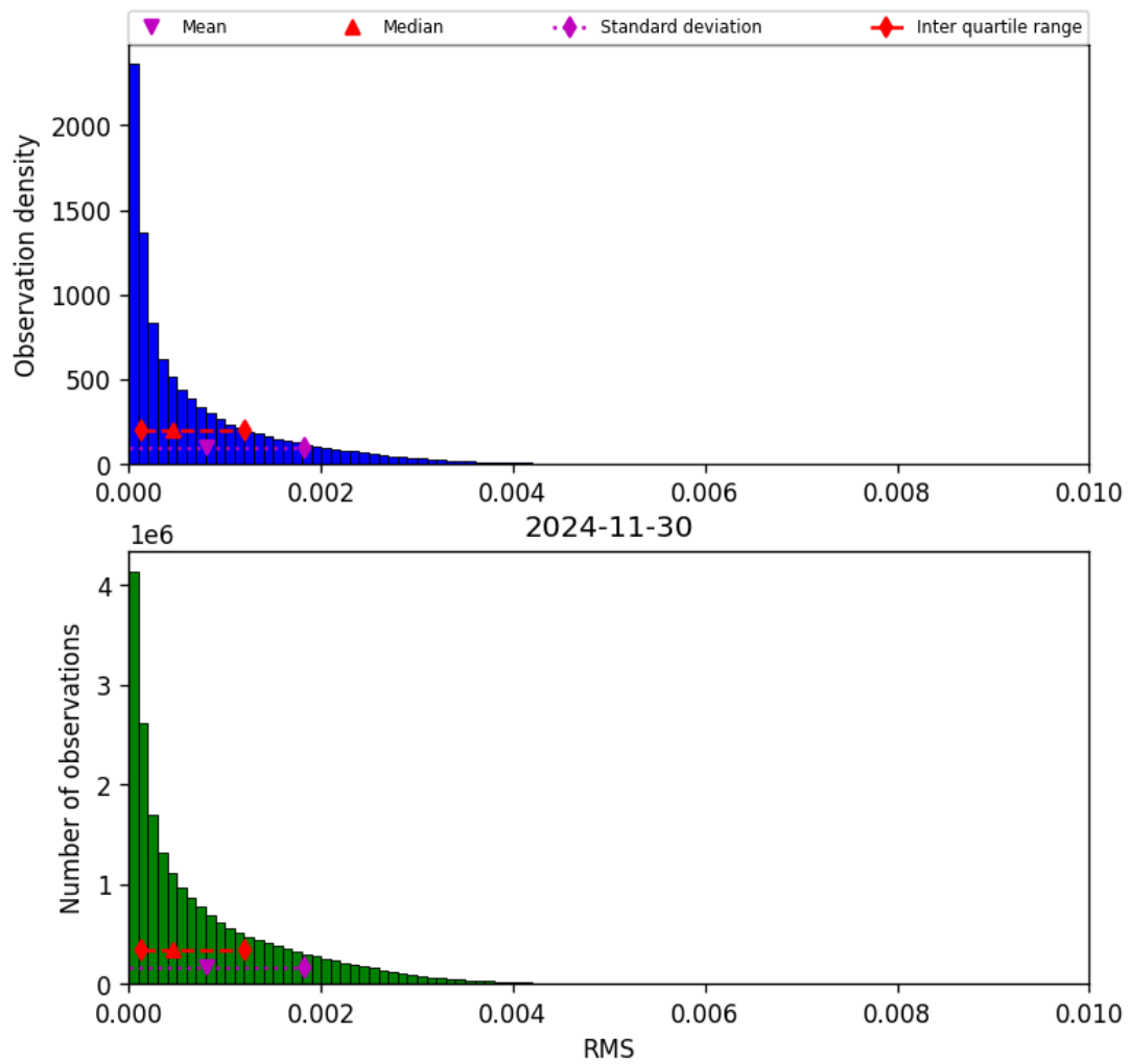
Figure 47: Histogram of “RMS” for 2024-11-30 to 2024-12-01
