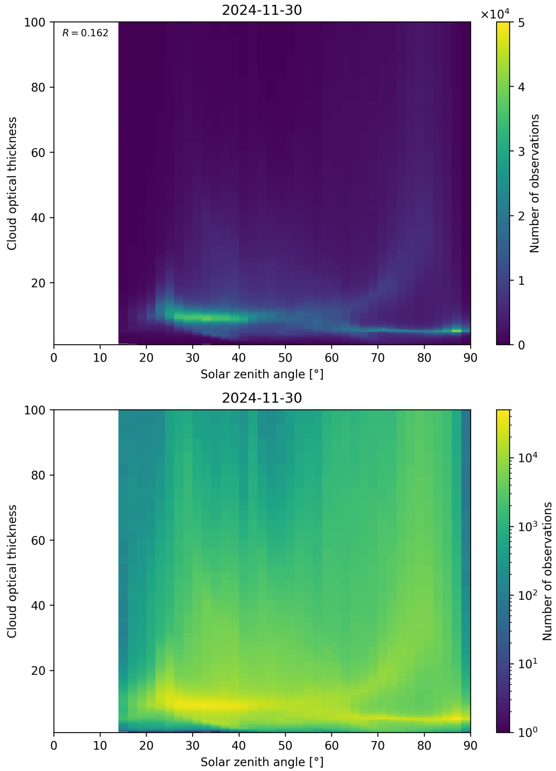
Figure 103: Scatter density plot of “Solar zenith angle” against “Cloud optical thickness” for 2024-11-30 to 2024-12-01.
