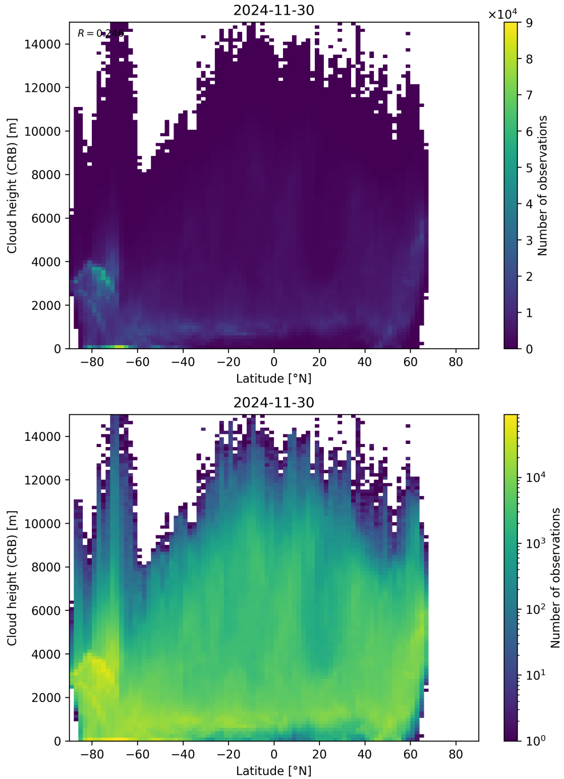
Figure 95: Scatter density plot of “Latitude” against “Cloud height (CRB)” for 2024-11-30 to 2024-12-01.
