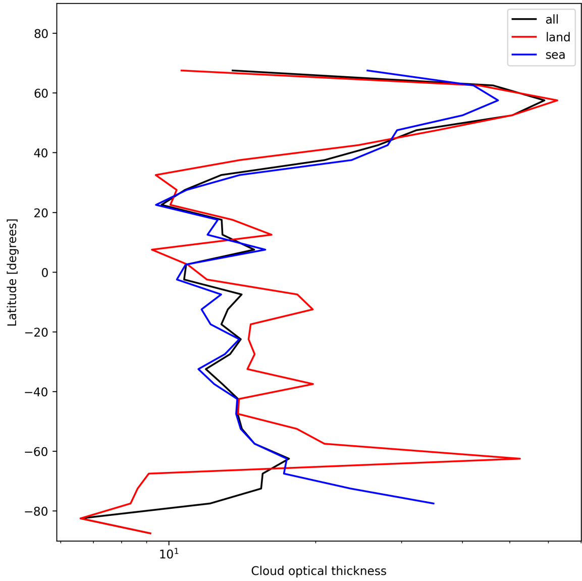
Figure 25: Zonal average of “Cloud optical thickness” for 2024-11-30 to 2024-12-01.
