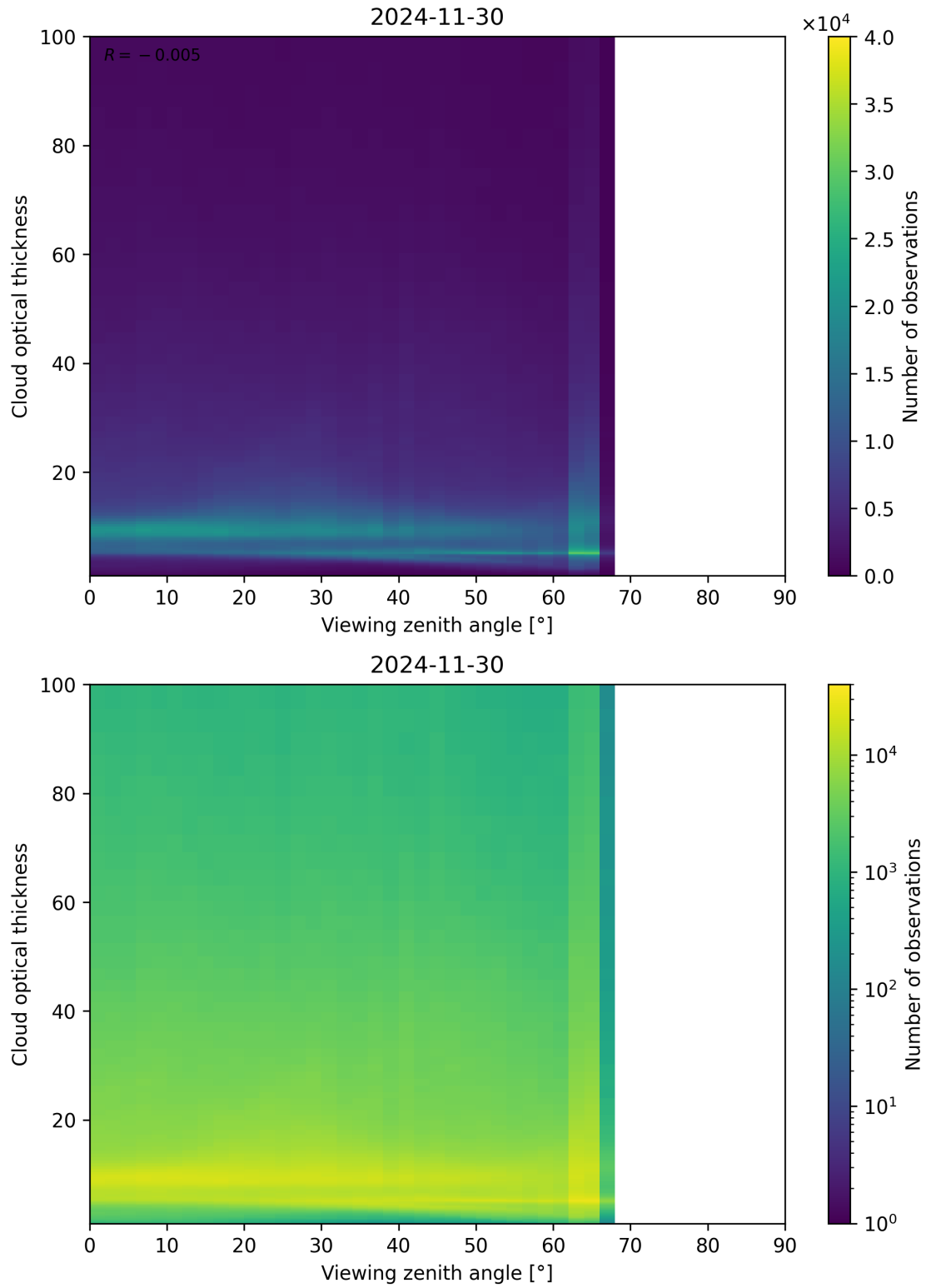
Figure 111: Scatter density plot of “Viewing zenith angle” against “Cloud optical thickness” for 2024-11-30 to 2024-12-01.
