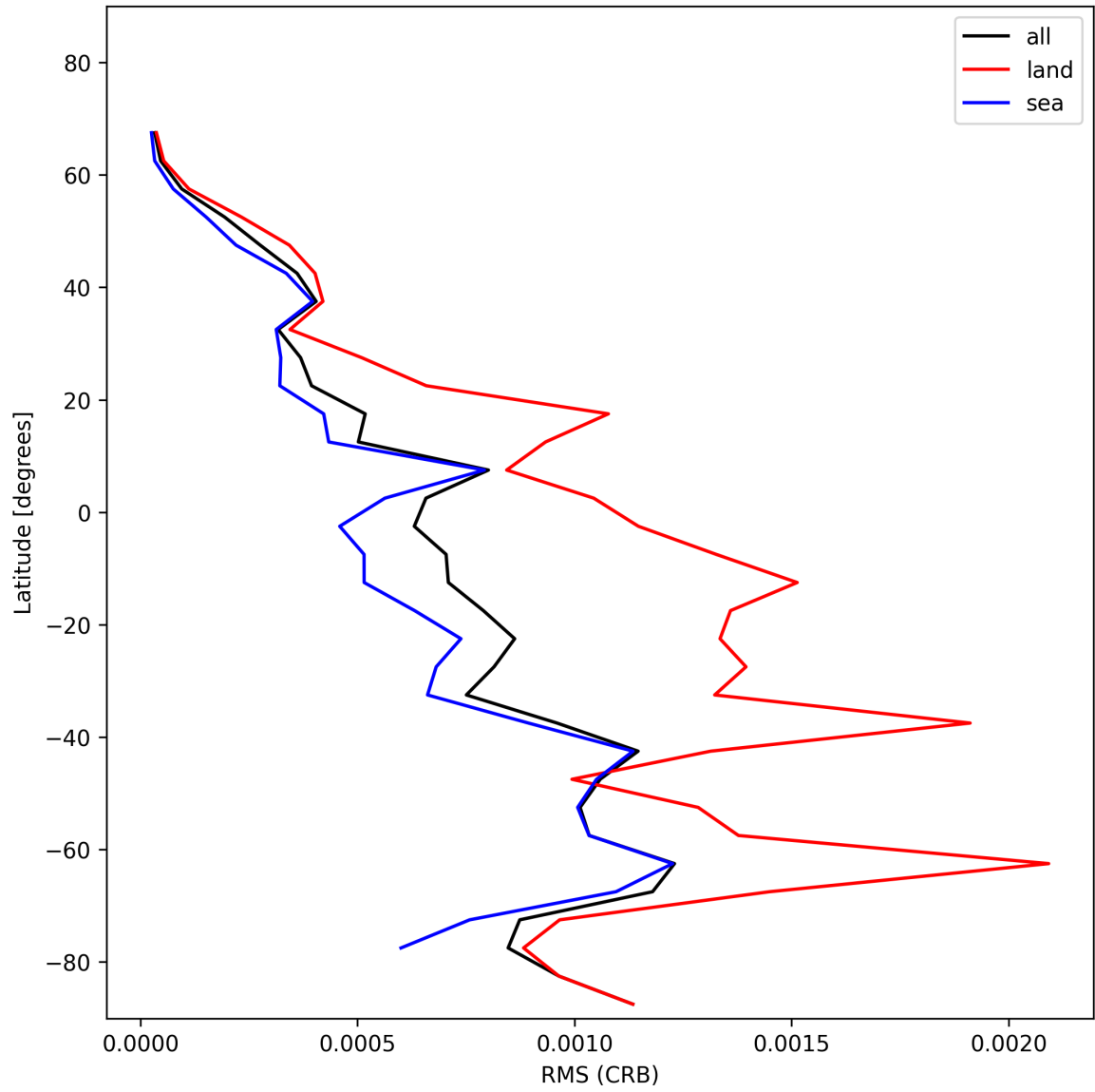
Figure 32: Zonal average of “RMS (CRB)” for 2024-11-30 to 2024-12-01.
