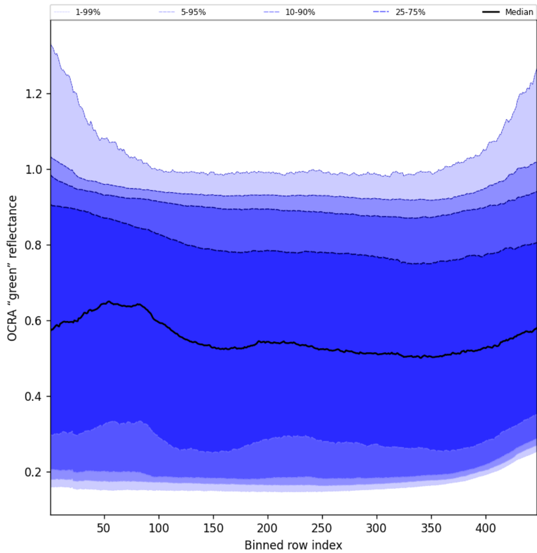
Figure 68: Along track statistics of “OCRA “green” reflectance” for 2024-11-30 to 2024-12-01
