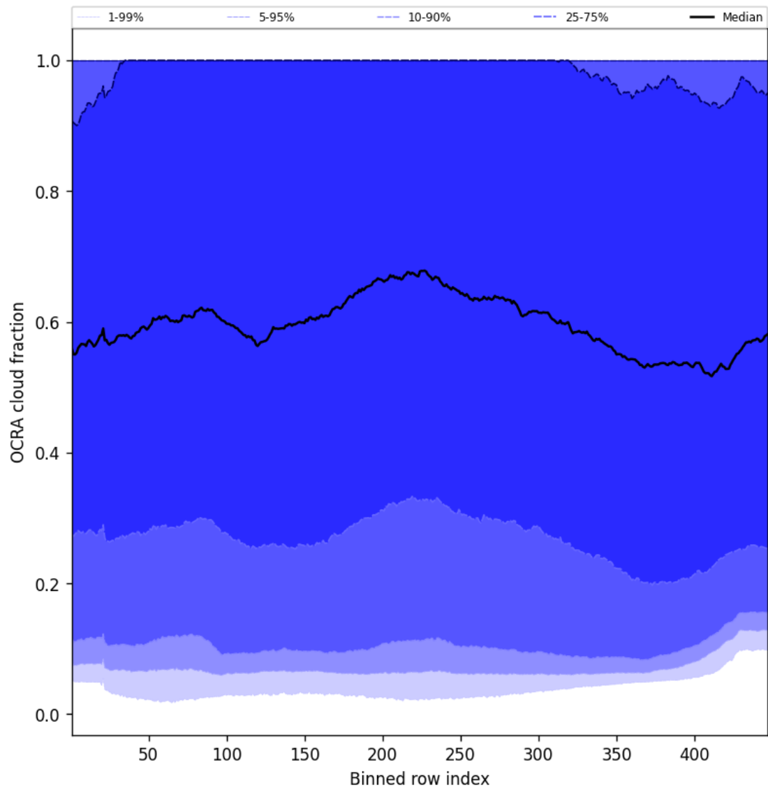
Figure 66: Along track statistics of “OCRA cloud fraction” for 2024-11-30 to 2024-12-01
