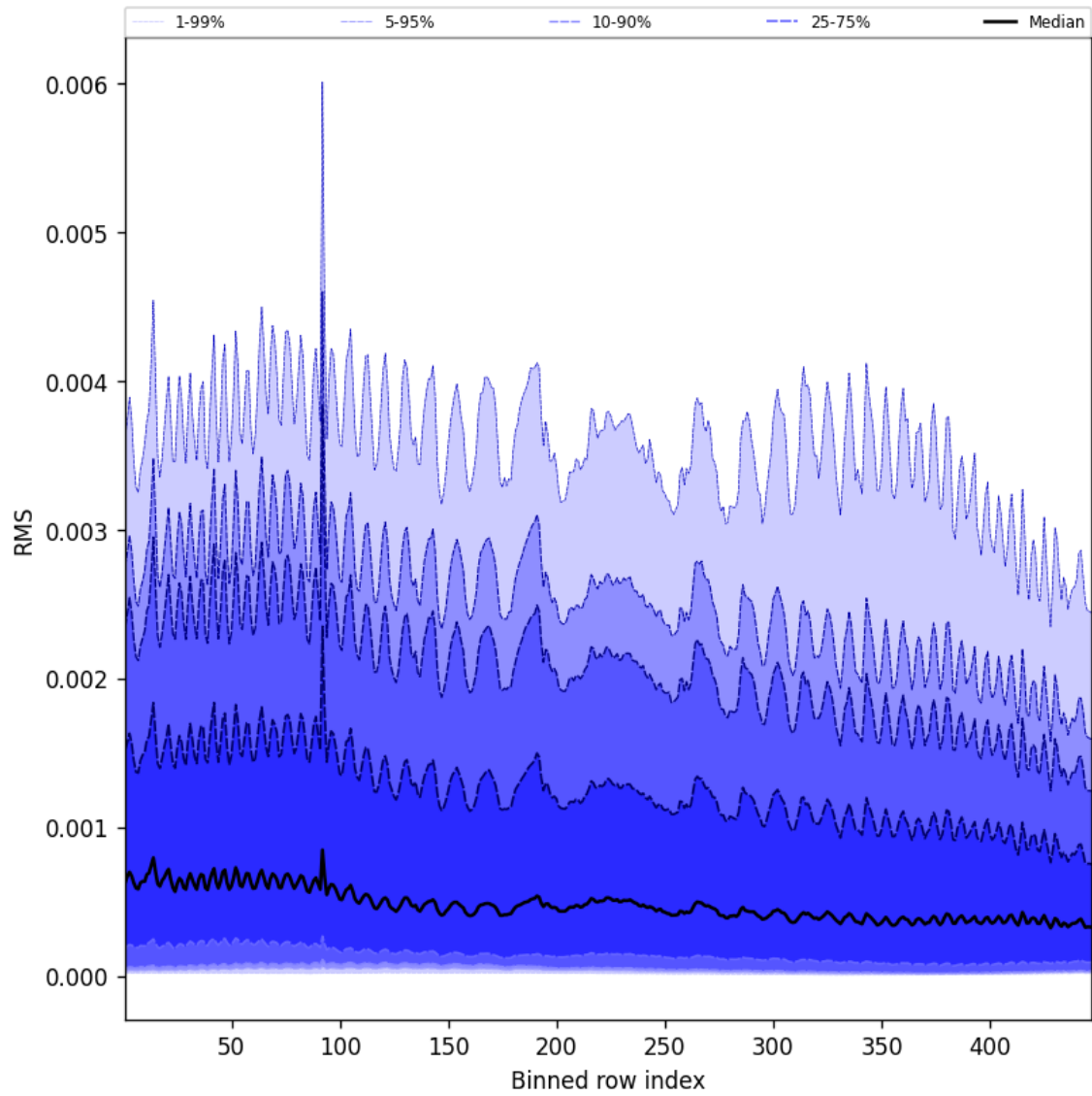
Figure 63: Along track statistics of “RMS” for 2024-11-30 to 2024-12-01
