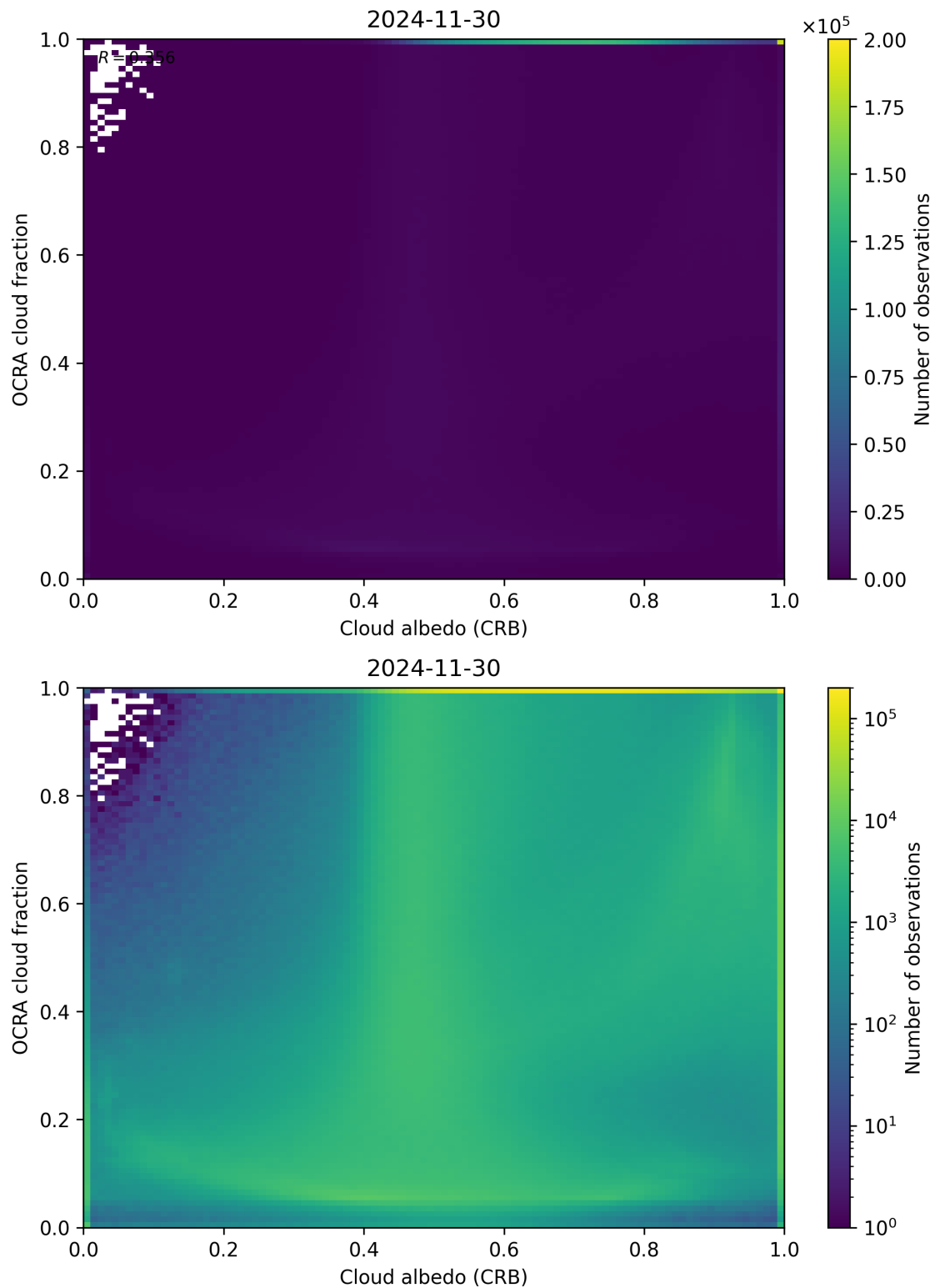
Figure 70: Scatter density plot of “Cloud albedo (CRB)” against “OCRA cloud fraction” for 2024-11-30 to 2024-12-01.
