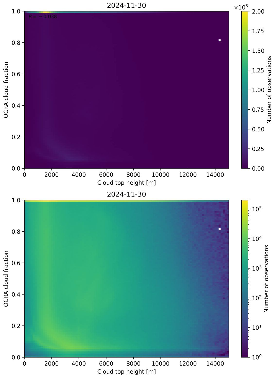
Figure 87: Scatter density plot of “Cloud top height” against “OCRA cloud fraction” for 2024-11-30 to 2024-12-01.
