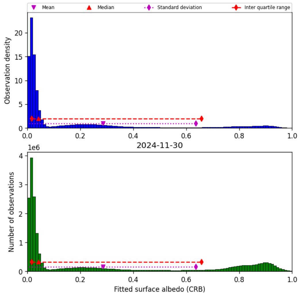
Figure 46: Histogram of “Fitted surface albedo (CRB)” for 2024-11-30 to 2024-12-01
