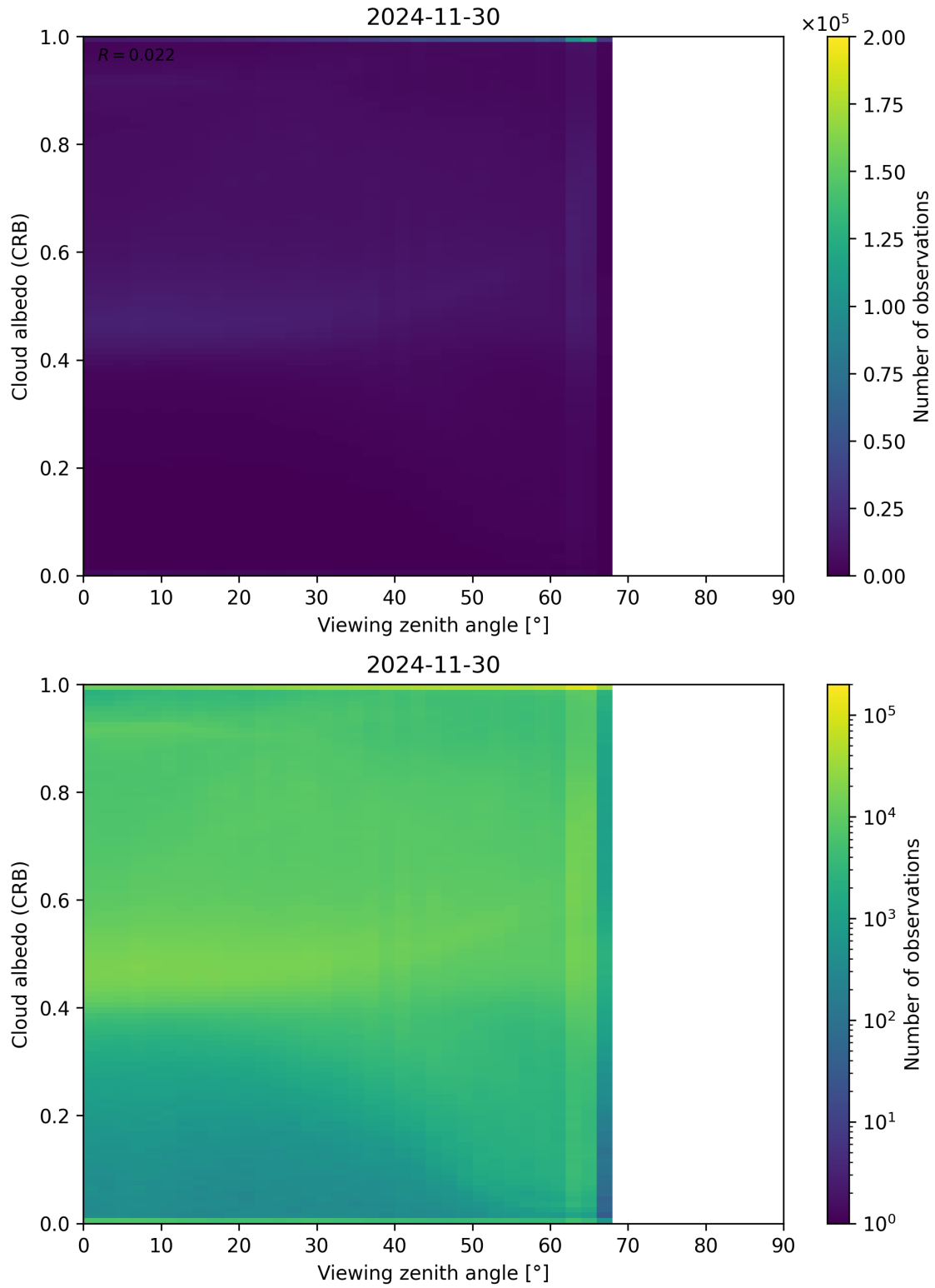
Figure 106: Scatter density plot of “Viewing zenith angle” against “Cloud albedo (CRB)” for 2024-11-30 to 2024-12-01.
