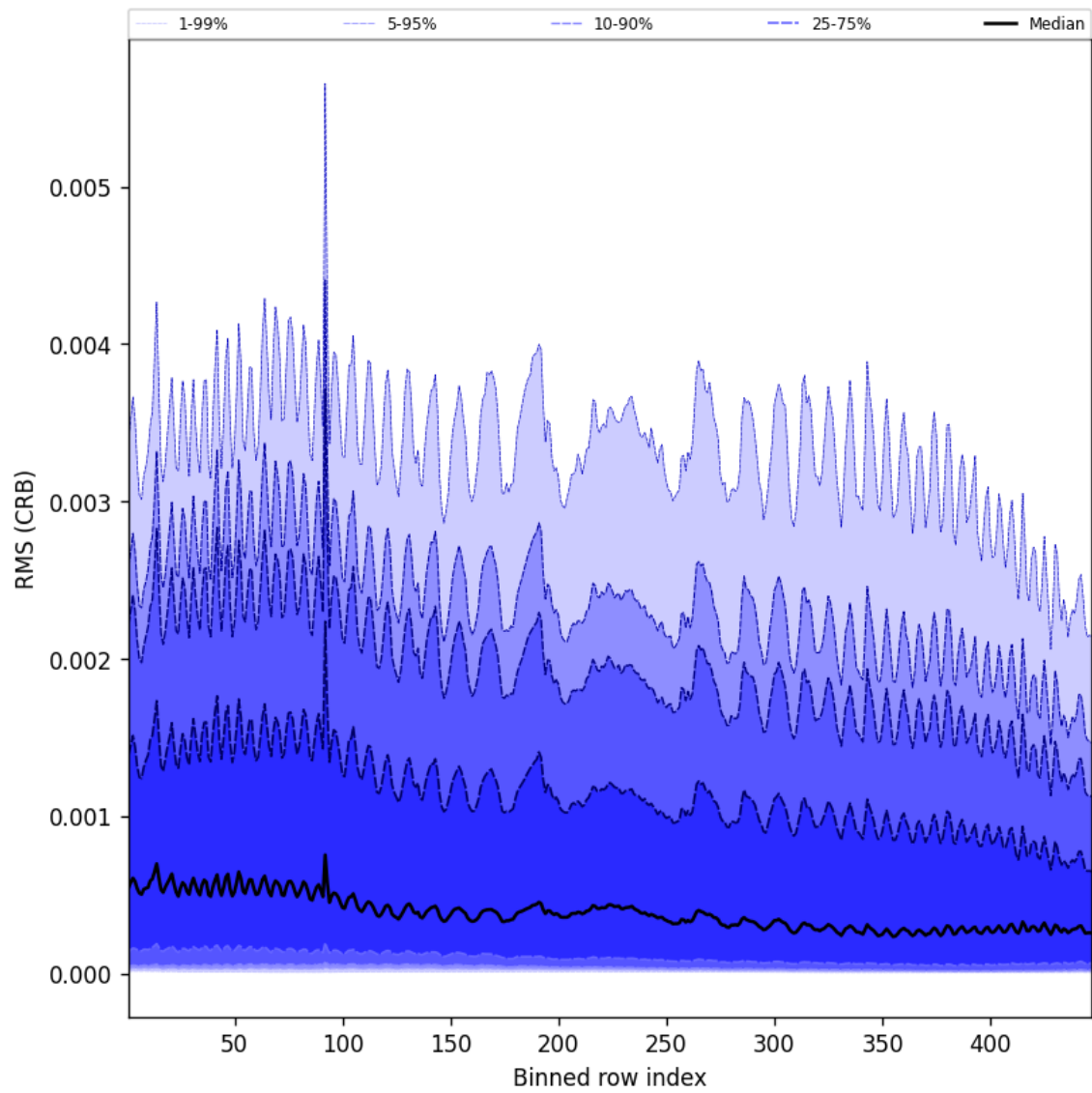
Figure 64: Along track statistics of “RMS (CRB)” for 2024-11-30 to 2024-12-01
