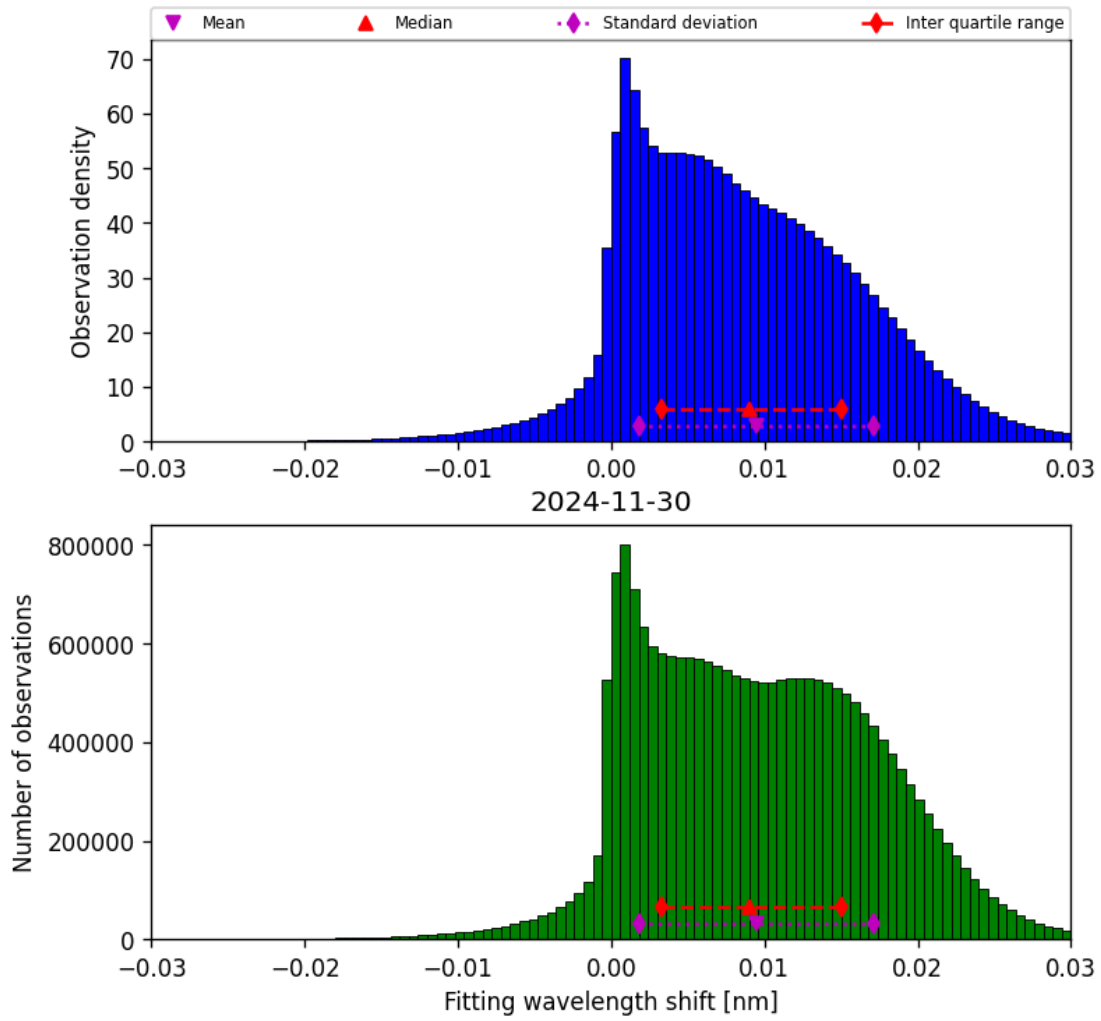
Figure 49: Histogram of “Fitting wavelength shift” for 2024-11-30 to 2024-12-01
