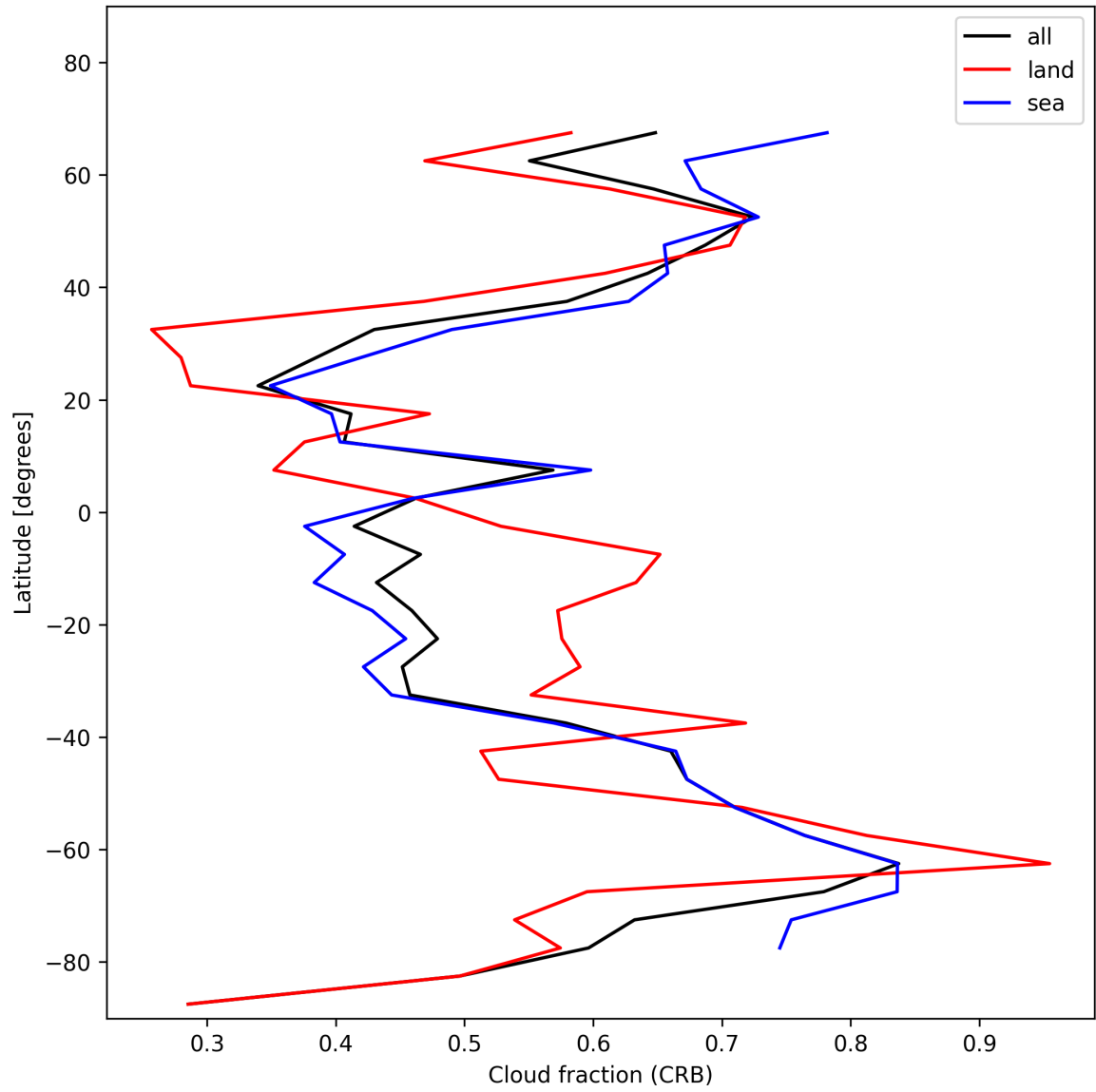
Figure 26: Zonal average of “Cloud fraction (CRB)” for 2024-11-30 to 2024-12-01.
