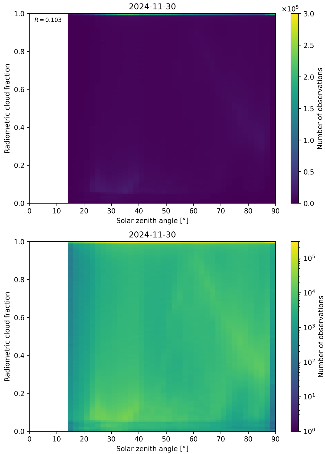
Figure 99: Scatter density plot of “Solar zenith angle” against “Radiometric cloud fraction” for 2024-11-30 to 2024-12-01.
