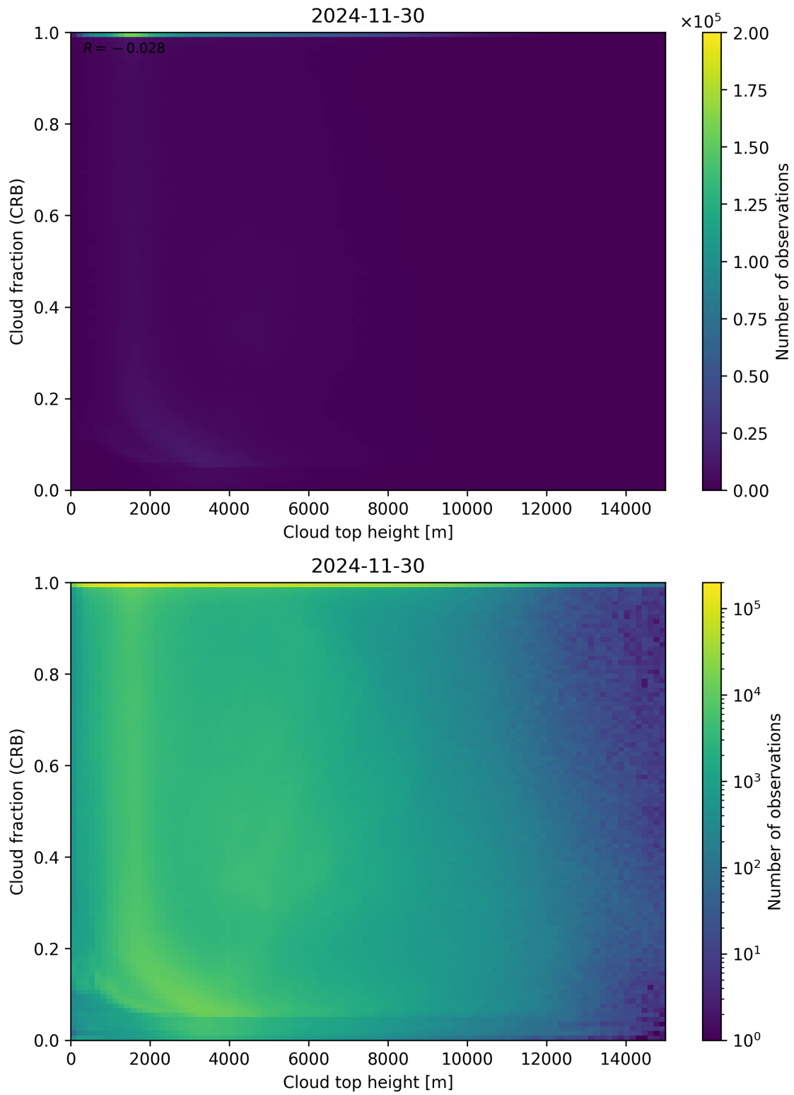
Figure 88: Scatter density plot of “Cloud top height” against “Cloud fraction (CRB)” for 2024-11-30 to 2024-12-01.
