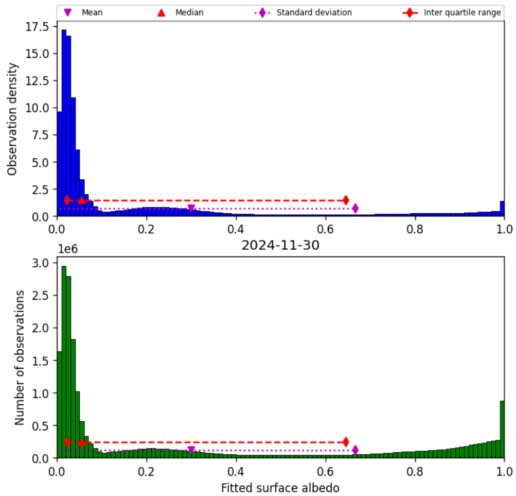
Figure 45: Histogram of “Fitted surface albedo” for 2024-11-30 to 2024-12-01
