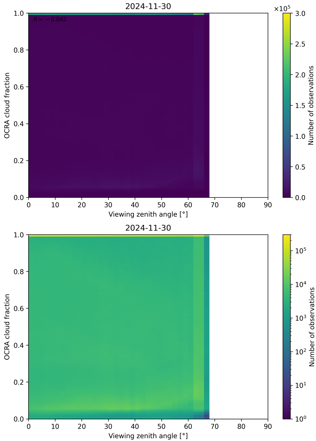
Figure 108: Scatter density plot of “Viewing zenith angle” against “OCRA cloud fraction” for 2024-11-30 to 2024-12-01.
