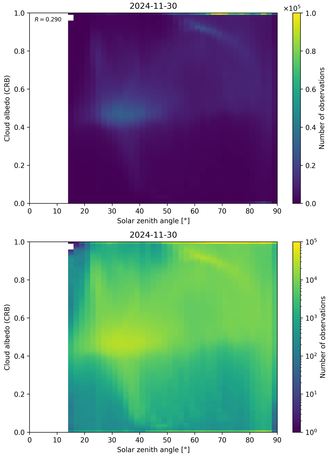
Figure 98: Scatter density plot of “Solar zenith angle” against “Cloud albedo (CRB)” for 2024-11-30 to 2024-12-01.
