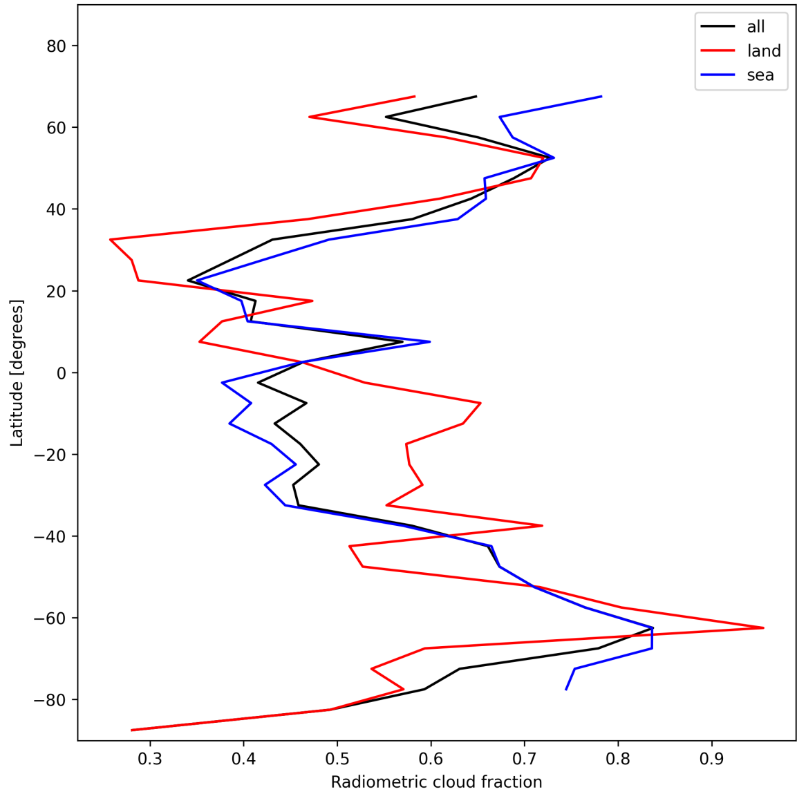
Figure 23: Zonal average of “Radiometric cloud fraction” for 2024-11-30 to 2024-12-01.
