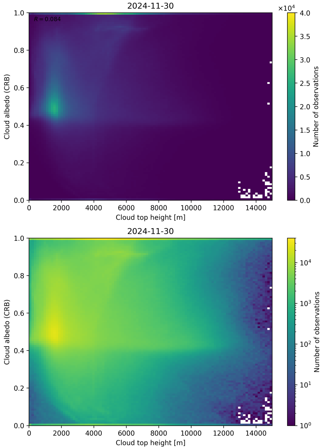
Figure 86: Scatter density plot of “Cloud top height” against “Cloud albedo (CRB)” for 2024-11-30 to 2024-12-01.
