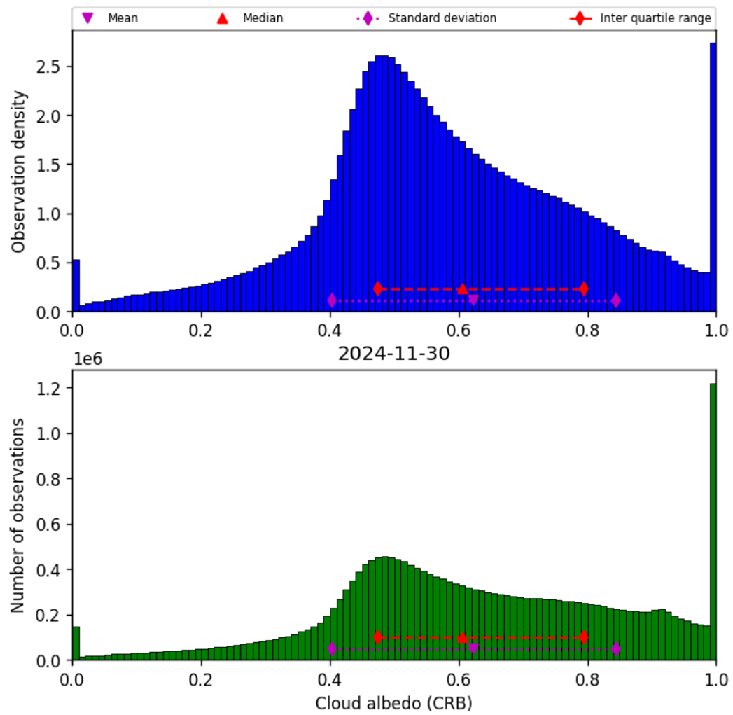
Figure 44: Histogram of “Cloud albedo (CRB)” for 2024-11-30 to 2024-12-01
