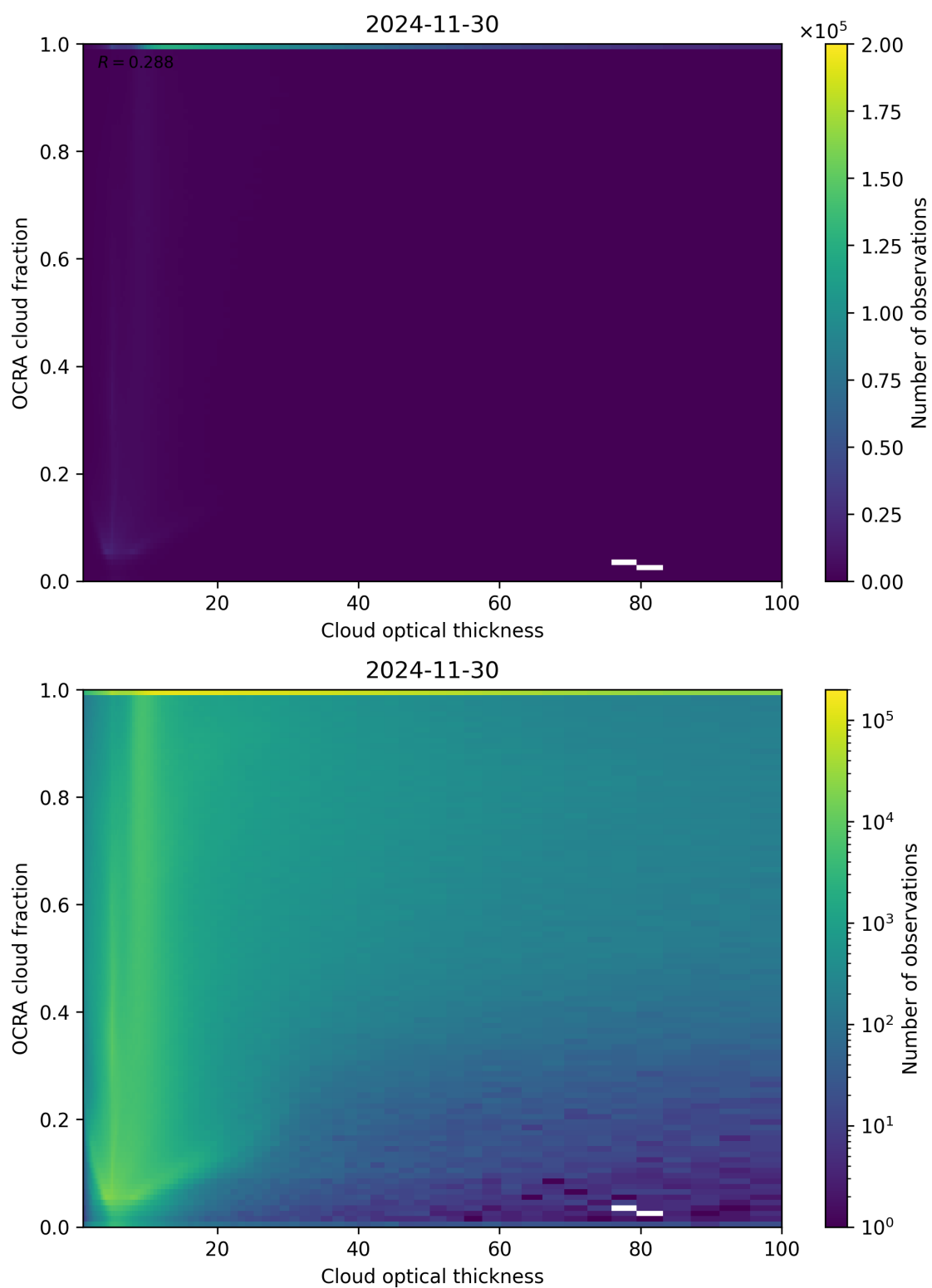
Figure 83: Scatter density plot of “Cloud optical thickness” against “OCRA cloud fraction” for 2024-11-30 to 2024-12-01.
