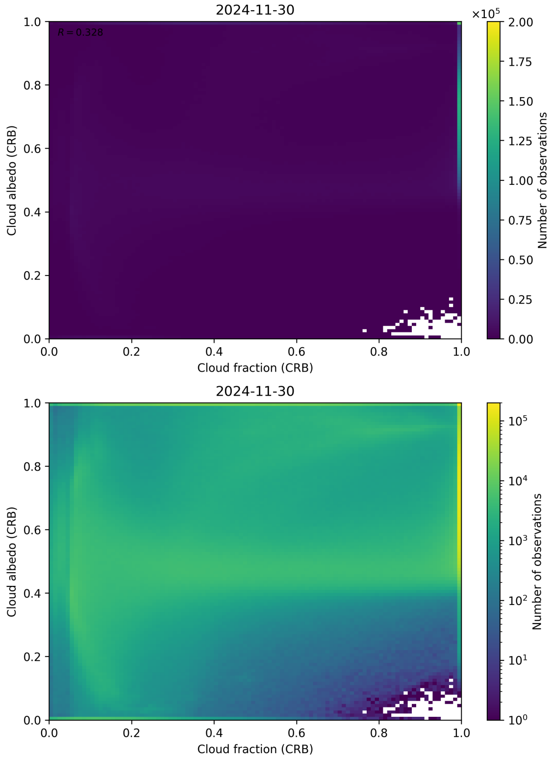
Figure 77: Scatter density plot of “Cloud fraction (CRB)” against “Cloud albedo (CRB)” for 2024-11-30 to 2024-12-01.
