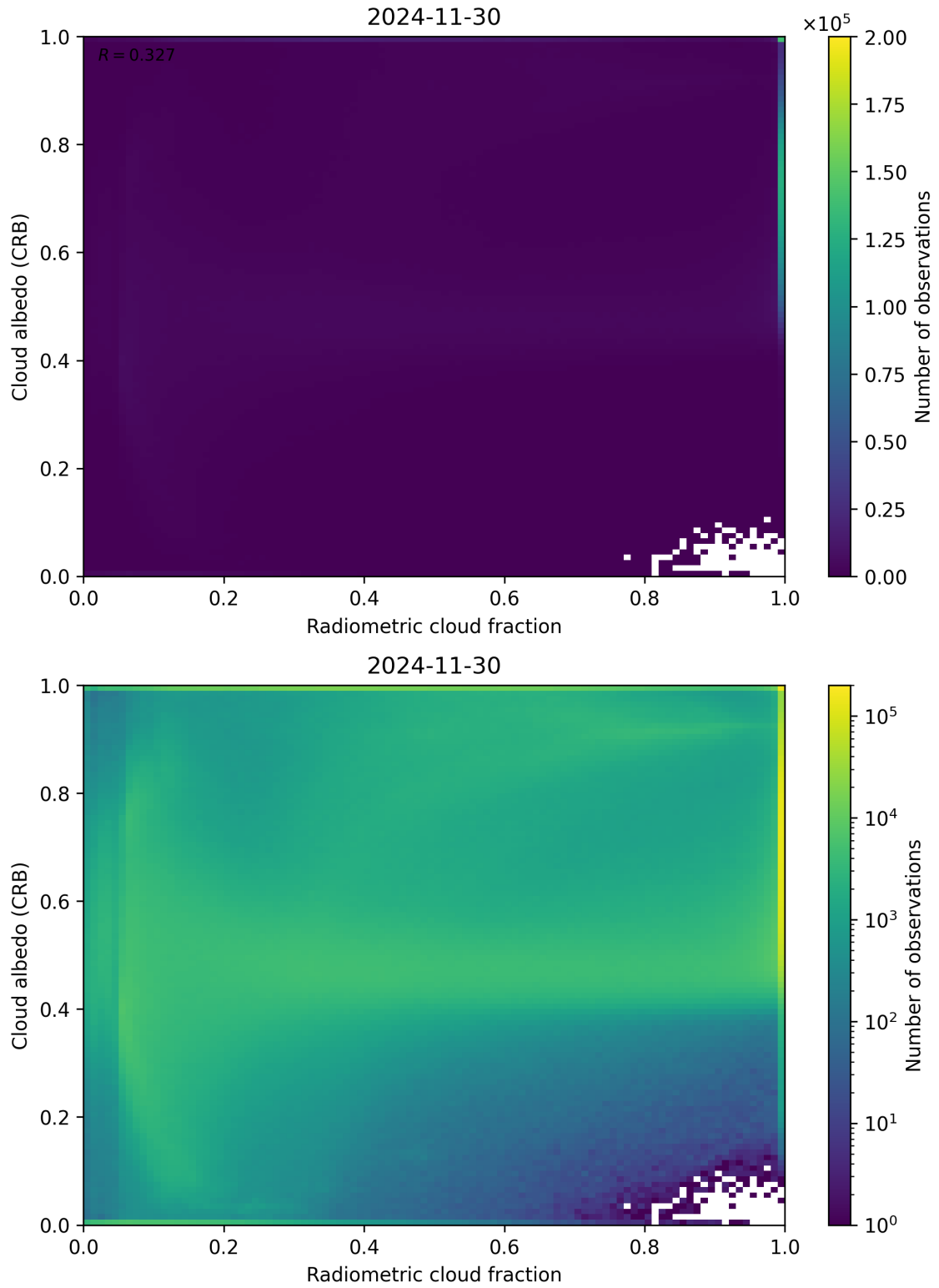
Figure 71: Scatter density plot of “Radiometric cloud fraction” against “Cloud albedo (CRB)” for 2024-11-30 to 2024-12-01.
