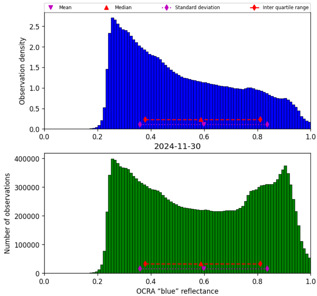
Figure 51: Histogram of “OCRA “blue” reflectance” for 2024-11-30 to 2024-12-01
