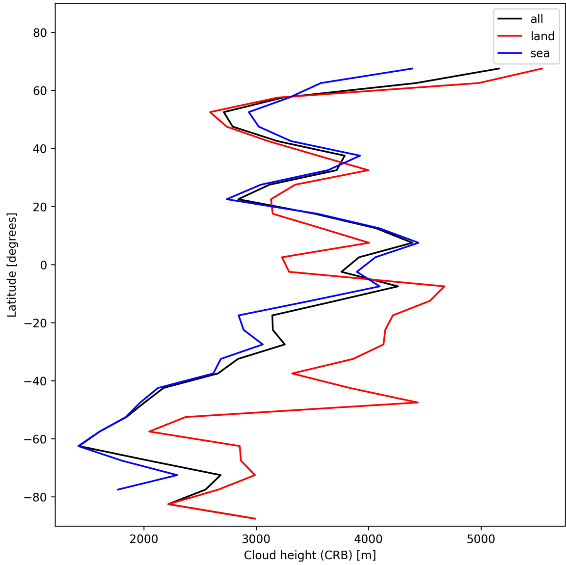
Figure 27: Zonal average of “Cloud height (CRB)” for 2024-11-30 to 2024-12-01.
