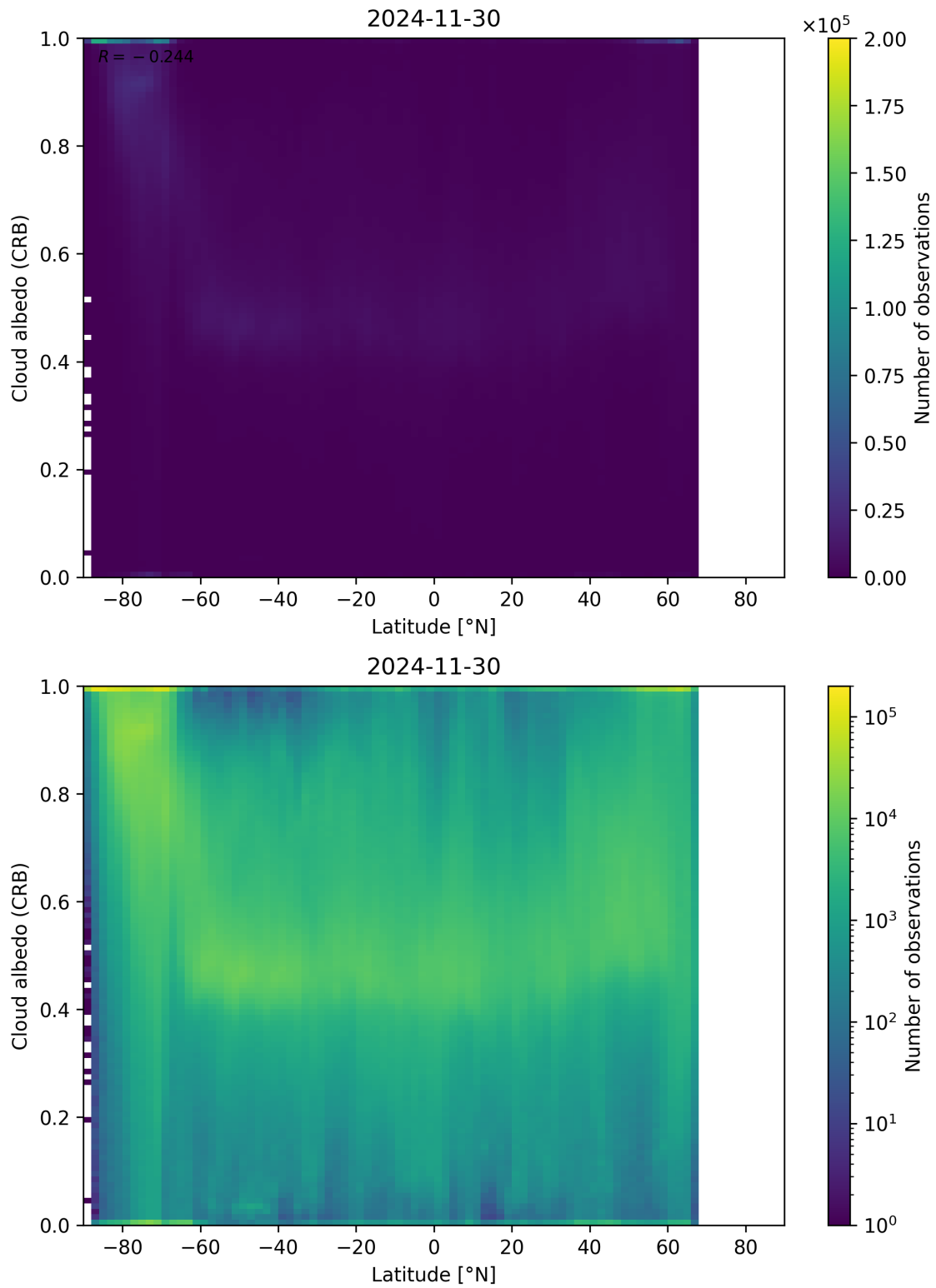
Figure 91: Scatter density plot of “Latitude” against “Cloud albedo (CRB)” for 2024-11-30 to 2024-12-01.
