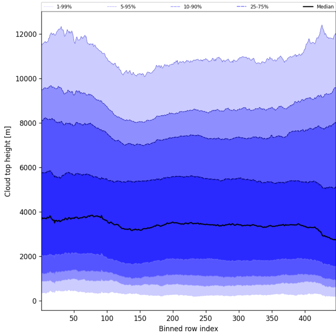
Figure 56: Along track statistics of “Cloud top height” for 2024-11-30 to 2024-12-01
