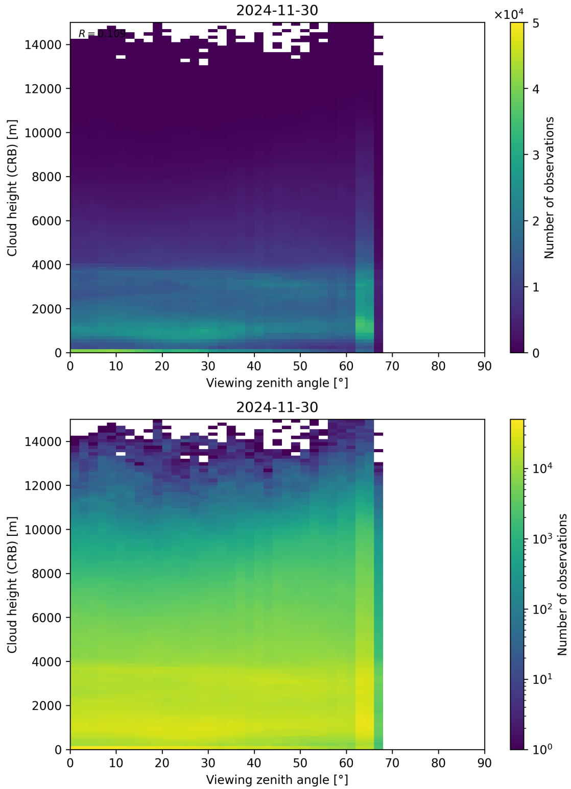
Figure 110: Scatter density plot of “Viewing zenith angle” against “Cloud height (CRB)” for 2024-11-30 to 2024-12-01.
