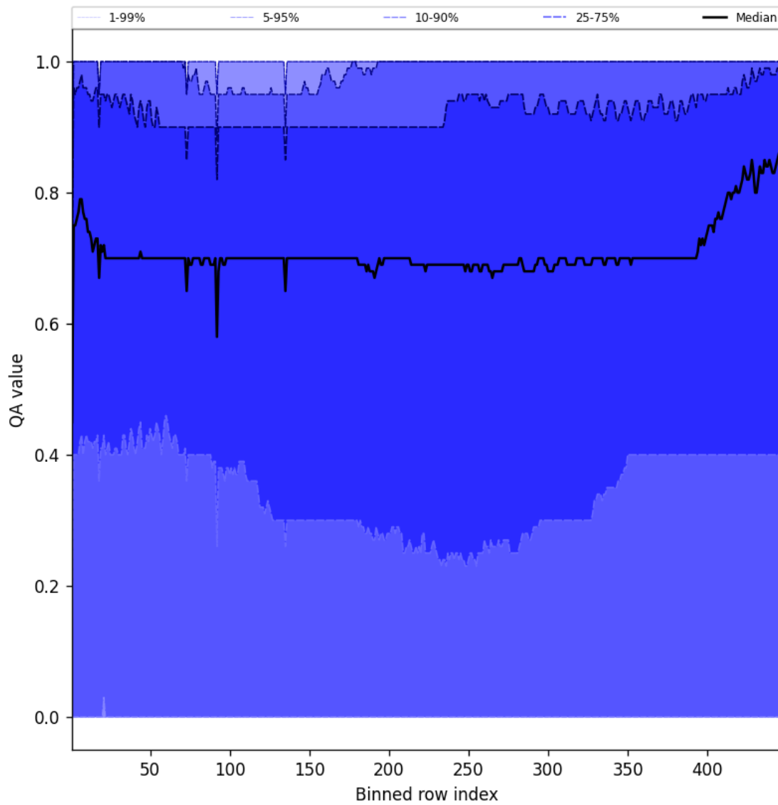
Figure 54: Along track statistics of “QA value” for 2024-11-30 to 2024-12-01
