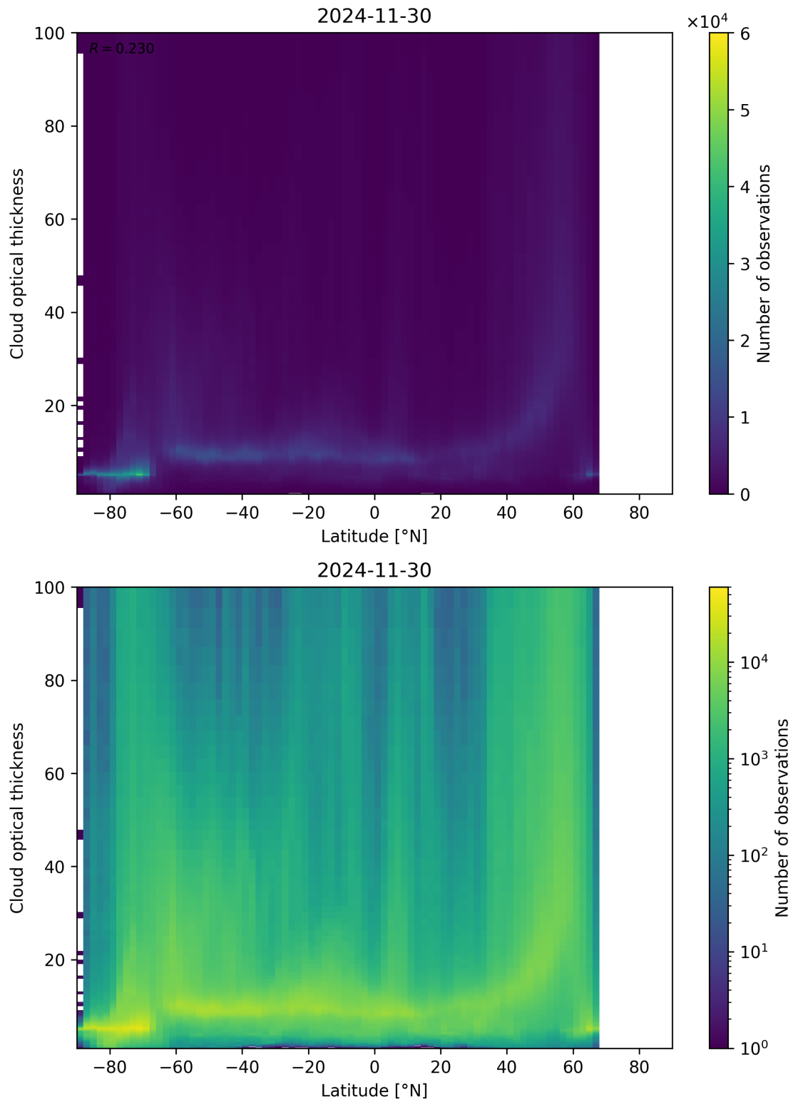
Figure 96: Scatter density plot of “Latitude” against “Cloud optical thickness” for 2024-11-30 to 2024-12-01.
