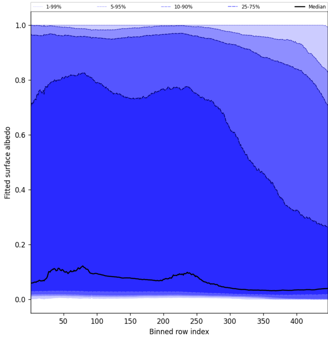
Figure 61: Along track statistics of “Fitted surface albedo” for 2024-11-30 to 2024-12-01
