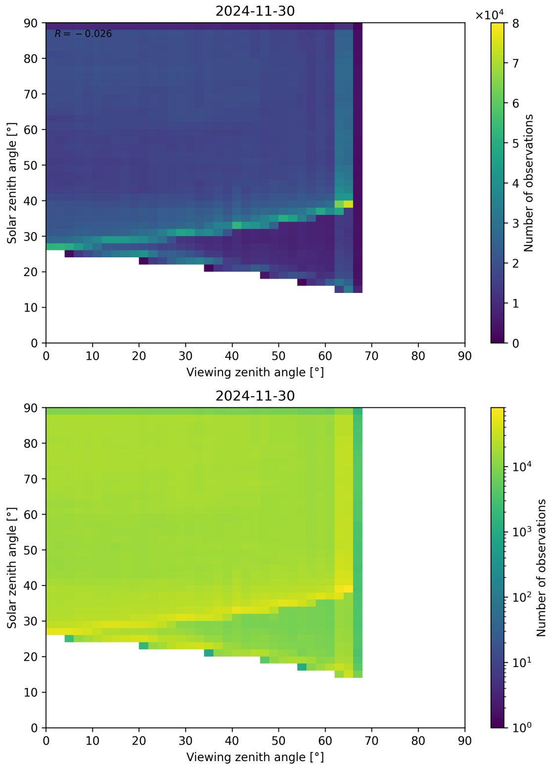
Figure 114: Scatter density plot of “Viewing zenith angle” against “Solar zenith angle” for 2024-11-30 to 2024-12-01.
