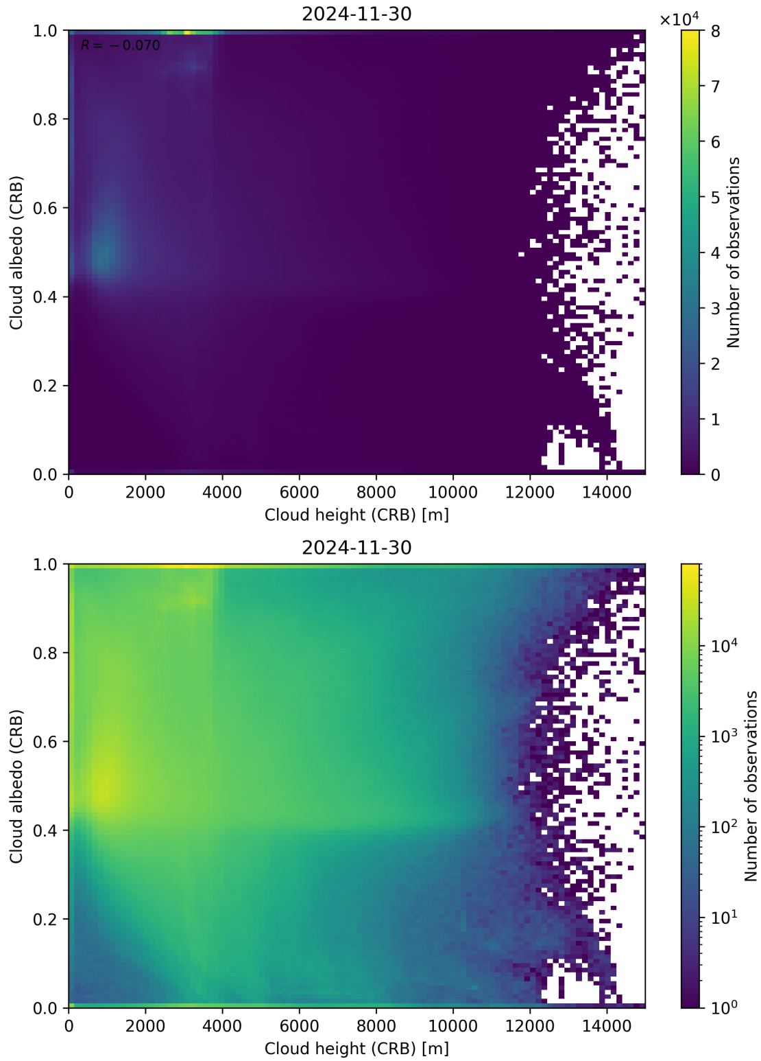
Figure 80: Scatter density plot of “Cloud height (CRB)” against “Cloud albedo (CRB)” for 2024-11-30 to 2024-12-01.
