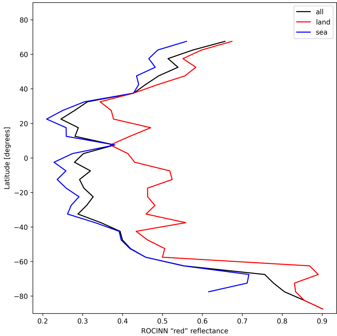
Figure 37: Zonal average of “ROCINN “red” reflectance” for 2024-11-30 to 2024-12-01.
