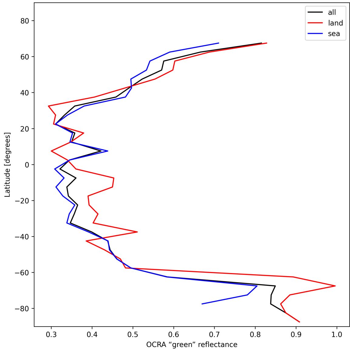
Figure 36: Zonal average of “OCRA “green” reflectance” for 2024-11-30 to 2024-12-01.
