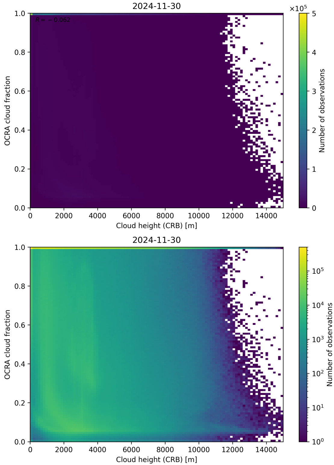
Figure 81: Scatter density plot of “Cloud height (CRB)” against “OCRA cloud fraction” for 2024-11-30 to 2024-12-01.
