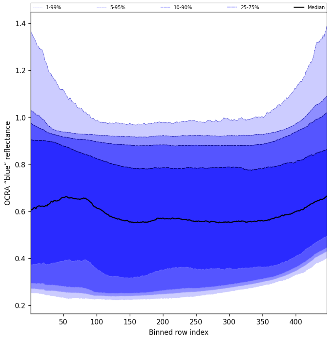
Figure 67: Along track statistics of "OCRA "blue" reflectance" for 2024-11-30 to 2024-12-01
