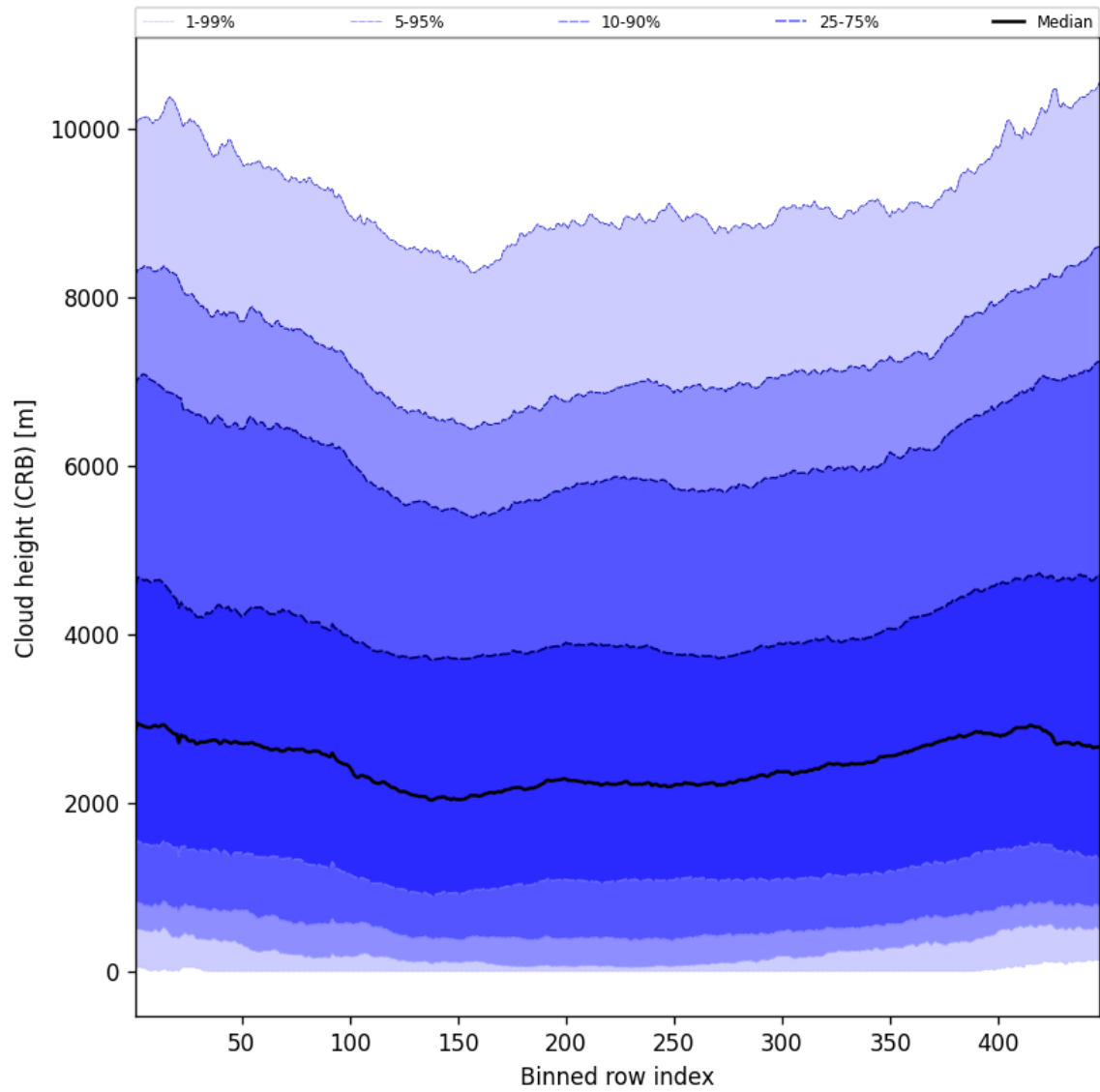
Figure 59: Along track statistics of “Cloud height (CRB)” for 2024-11-30 to 2024-12-01
