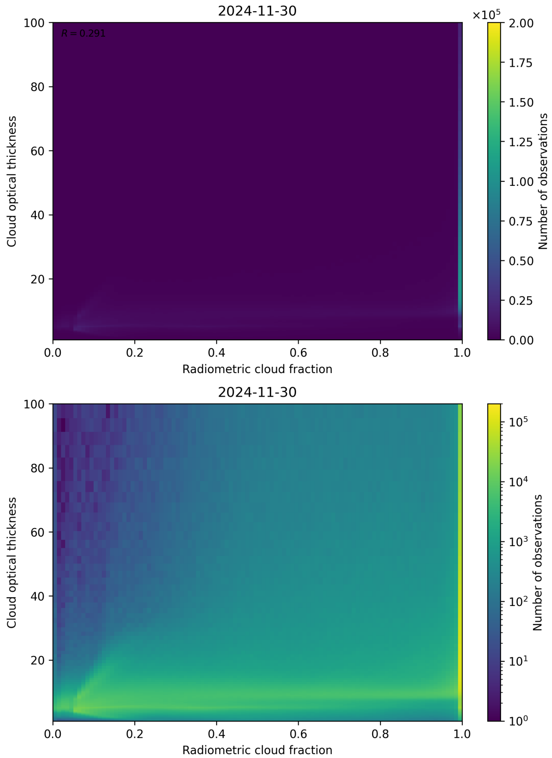
Figure 75: Scatter density plot of “Radiometric cloud fraction” against “Cloud optical thickness” for 2024-11-30 to 2024-12-01.
