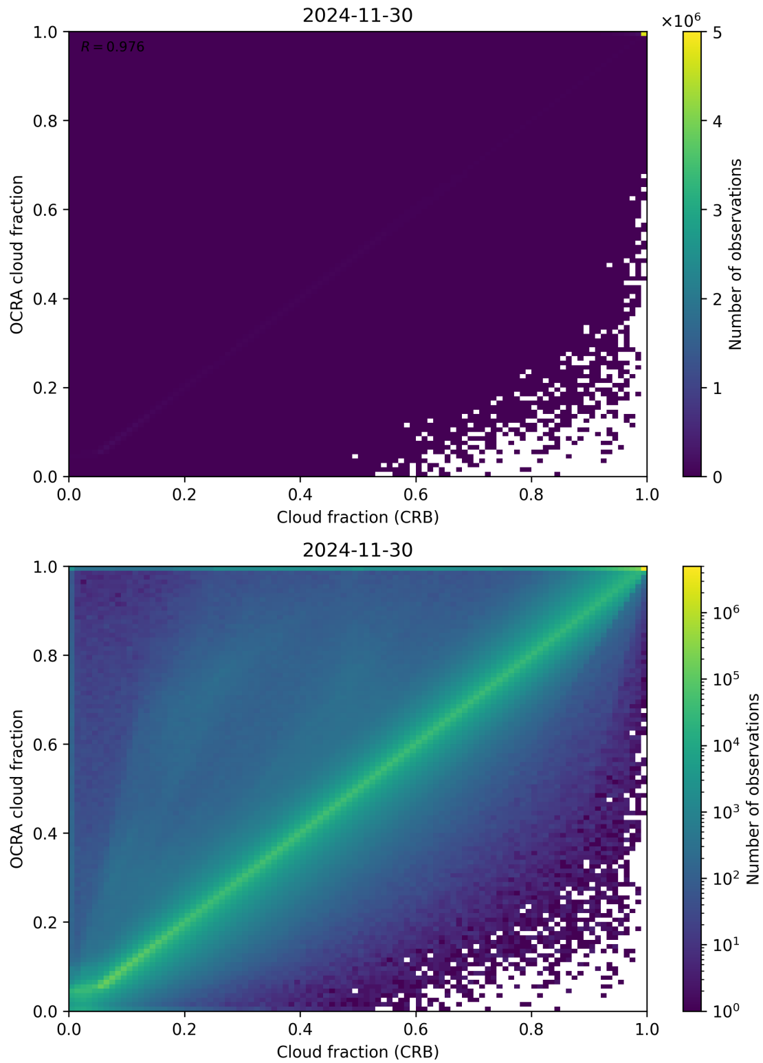
Figure 78: Scatter density plot of “Cloud fraction (CRB)” against “OCRA cloud fraction” for 2024-11-30 to 2024-12-01.
