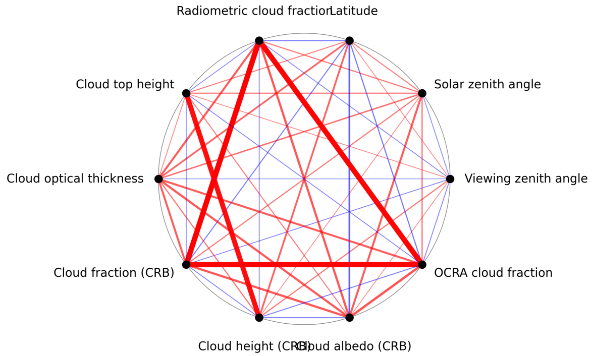
Figure 1: Map of correlation graph for 2024-11-30 to 2024-12-01.
