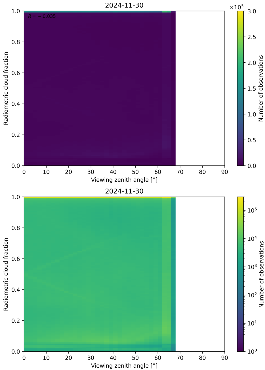
Figure 107: Scatter density plot of “Viewing zenith angle” against “Radiometric cloud fraction” for 2024-11-30 to 2024-12-01.
