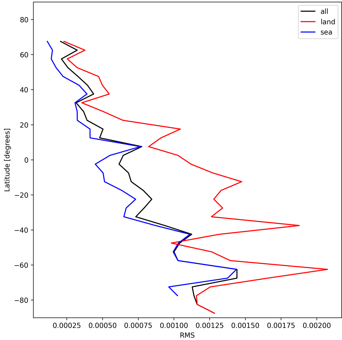
Figure 31: Zonal average of “RMS” for 2024-11-30 to 2024-12-01.
