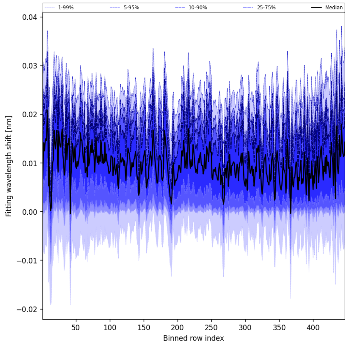
Figure 65: Along track statistics of “Fitting wavelength shift” for 2024-11-30 to 2024-12-01
