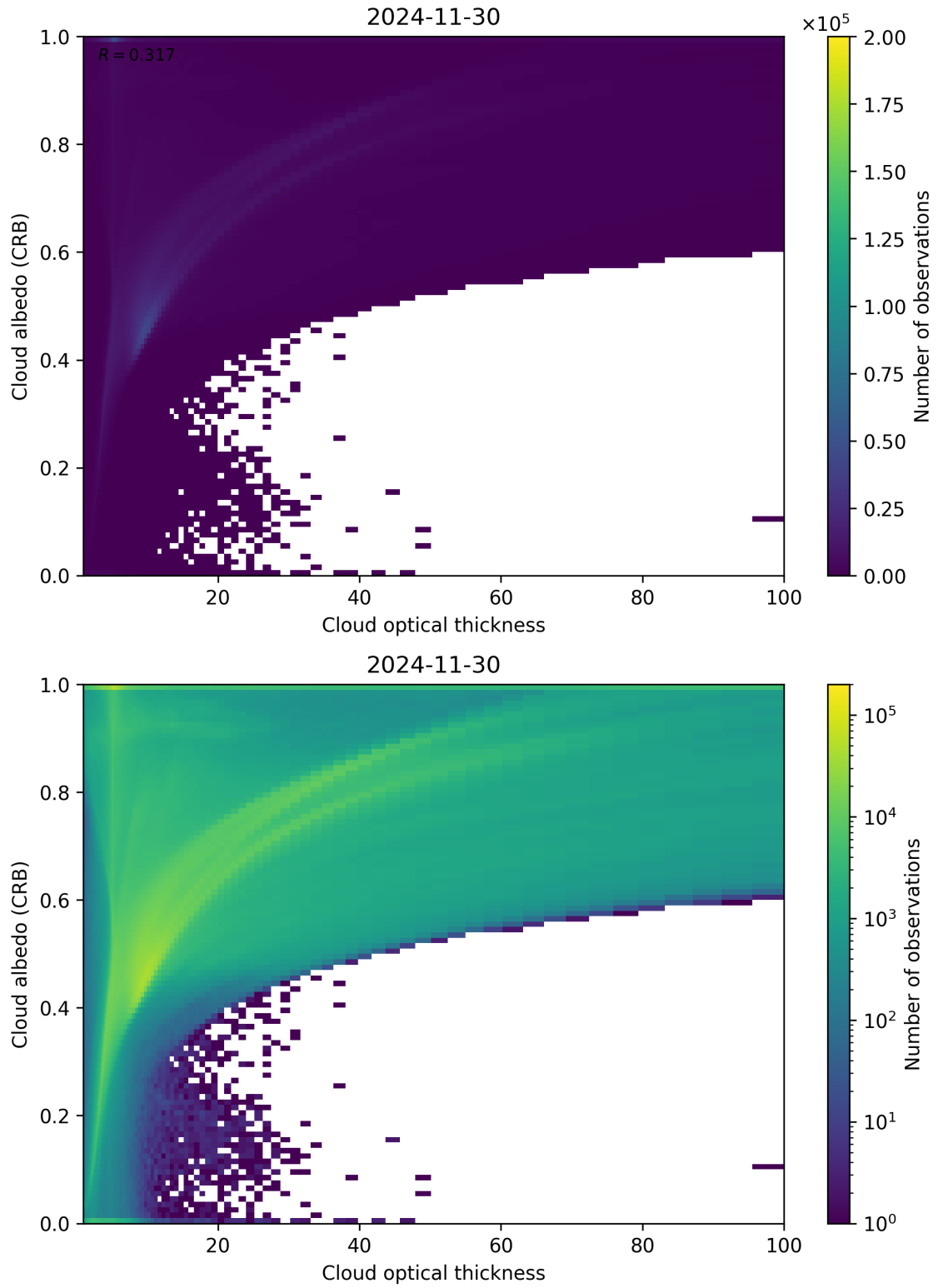
Figure 82: Scatter density plot of “Cloud optical thickness” against “Cloud albedo (CRB)” for 2024-11-30 to 2024-12-01.
