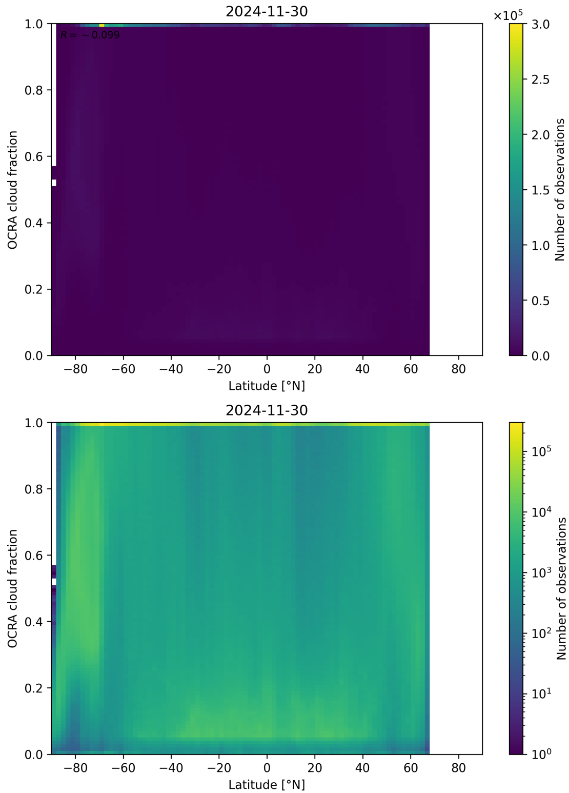
Figure 93: Scatter density plot of “Latitude” against “OCRA cloud fraction” for 2024-11-30 to 2024-12-01.
