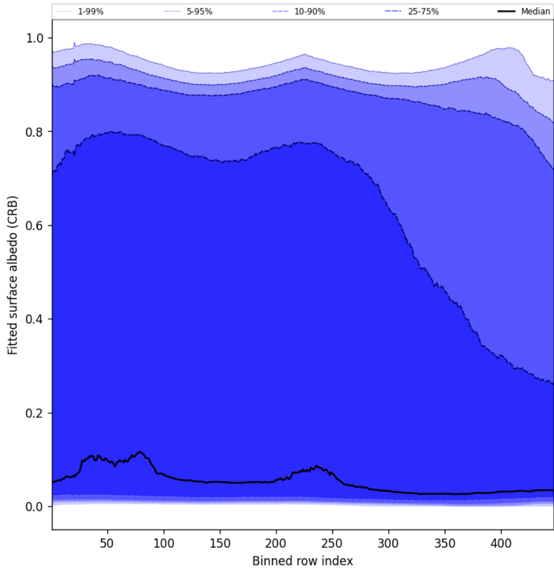
Figure 62: Along track statistics of “Fitted surface albedo (CRB)” for 2024-11-30 to 2024-12-01
