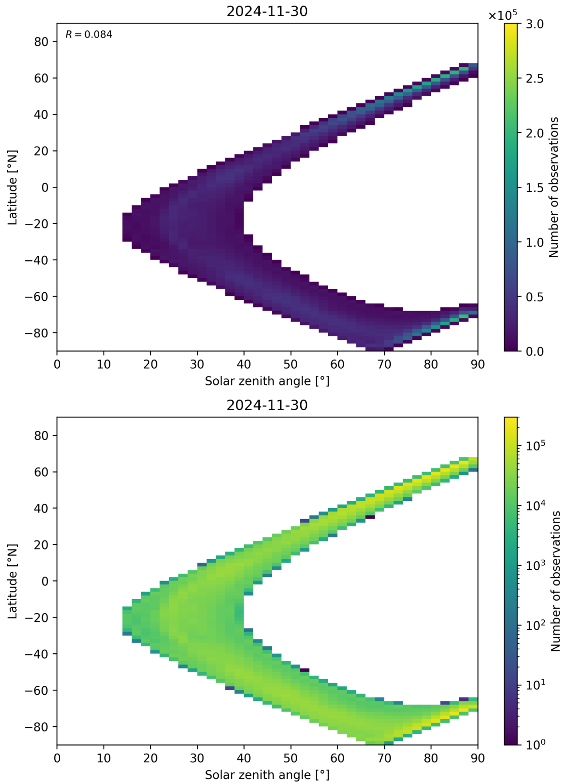
Figure 105: Scatter density plot of “Solar zenith angle” against “Latitude” for 2024-11-30 to 2024-12-01.
