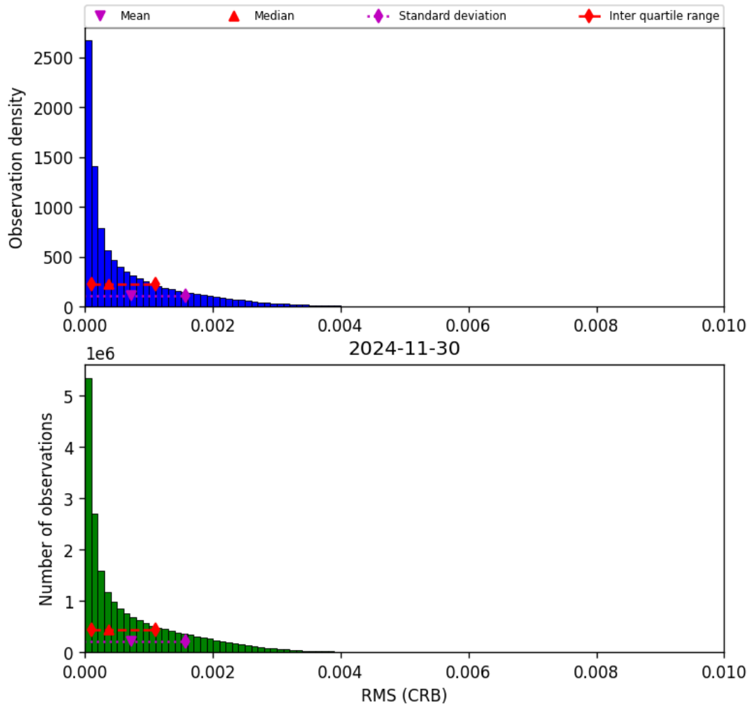
Figure 48: Histogram of “RMS (CRB)” for 2024-11-30 to 2024-12-01
