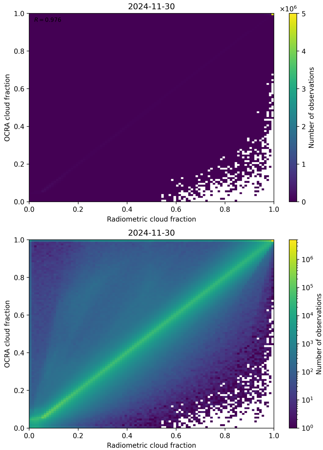
Figure 72: Scatter density plot of “Radiometric cloud fraction” against “OCRA cloud fraction” for 2024-11-30 to 2024-12-01.
