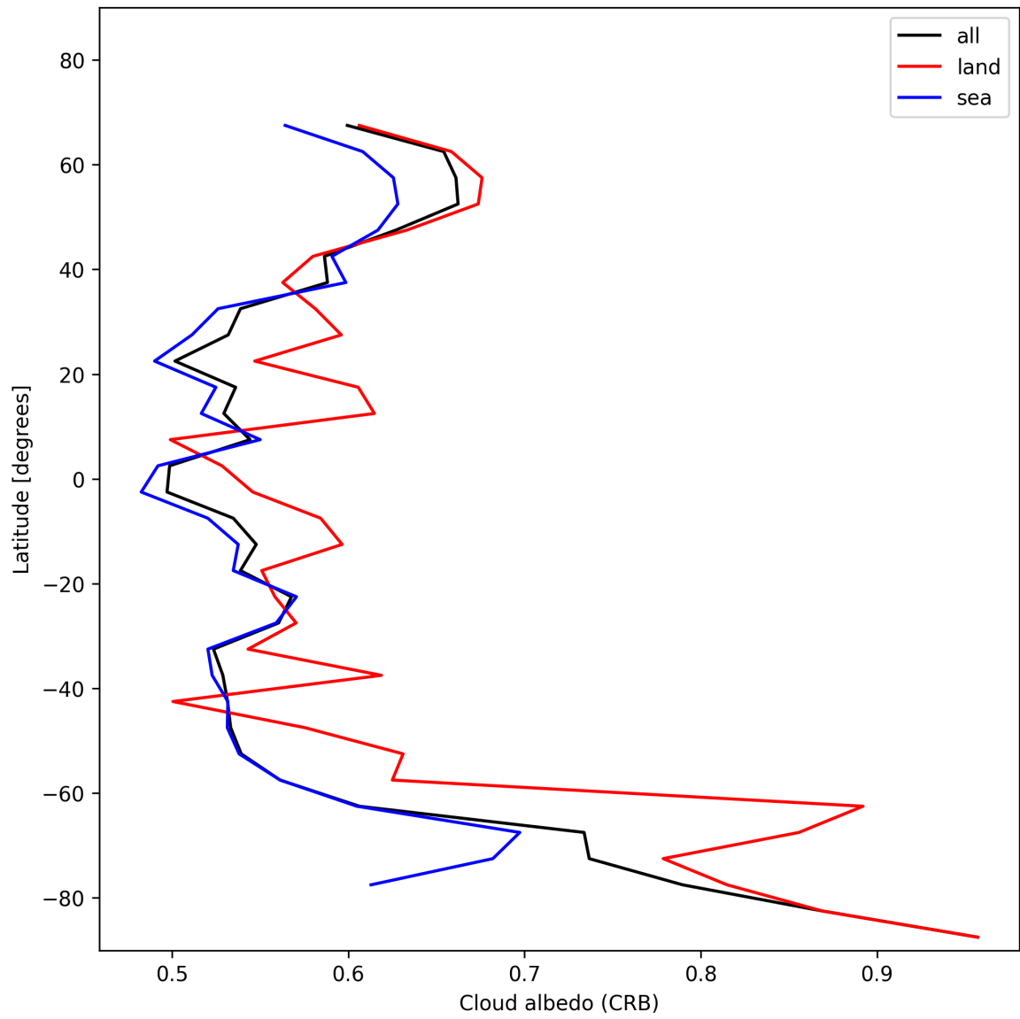
Figure 28: Zonal average of “Cloud albedo (CRB)” for 2024-11-30 to 2024-12-01.
