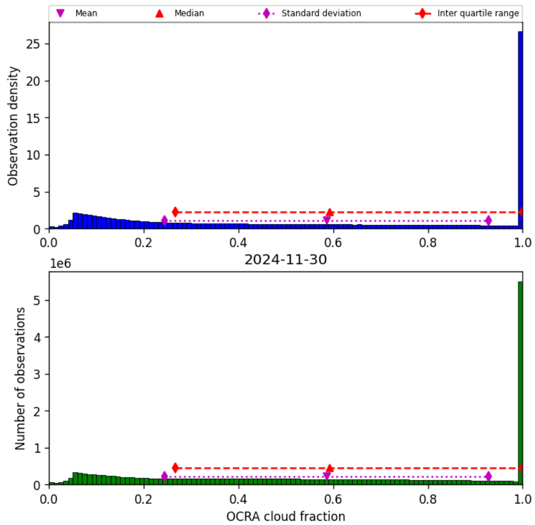
Figure 50: Histogram of “OCRA cloud fraction” for 2024-11-30 to 2024-12-01
