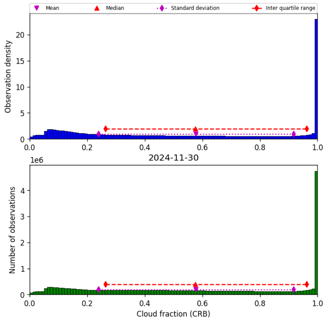
Figure 42: Histogram of “Cloud fraction (CRB)” for 2024-11-30 to 2024-12-01
