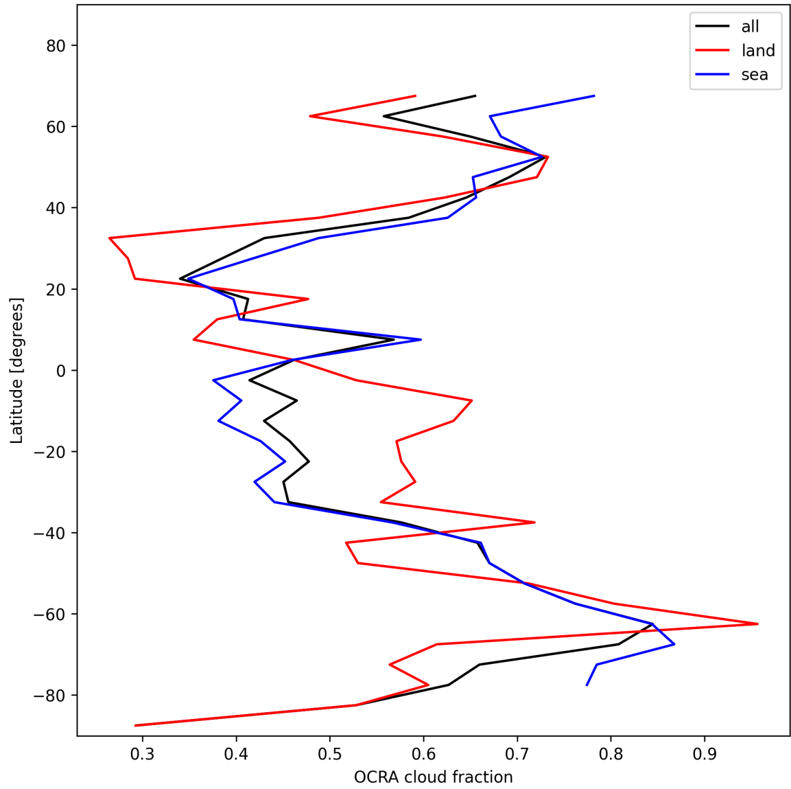
Figure 34: Zonal average of “OCRA cloud fraction” for 2024-11-30 to 2024-12-01.
