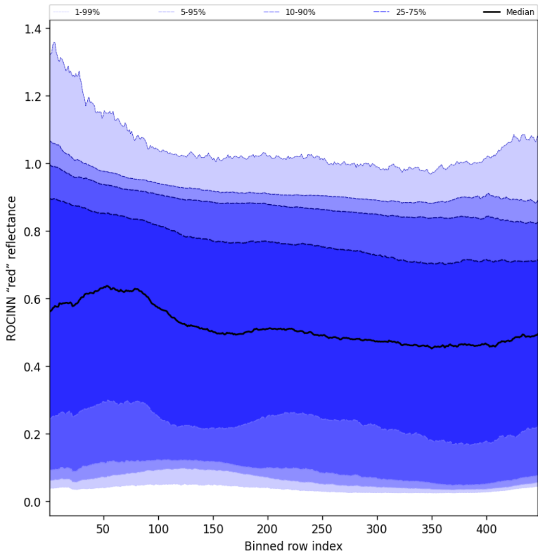
Figure 69: Along track statistics of “ROCINN “red” reflectance” for 2024-11-30 to 2024-12-01
