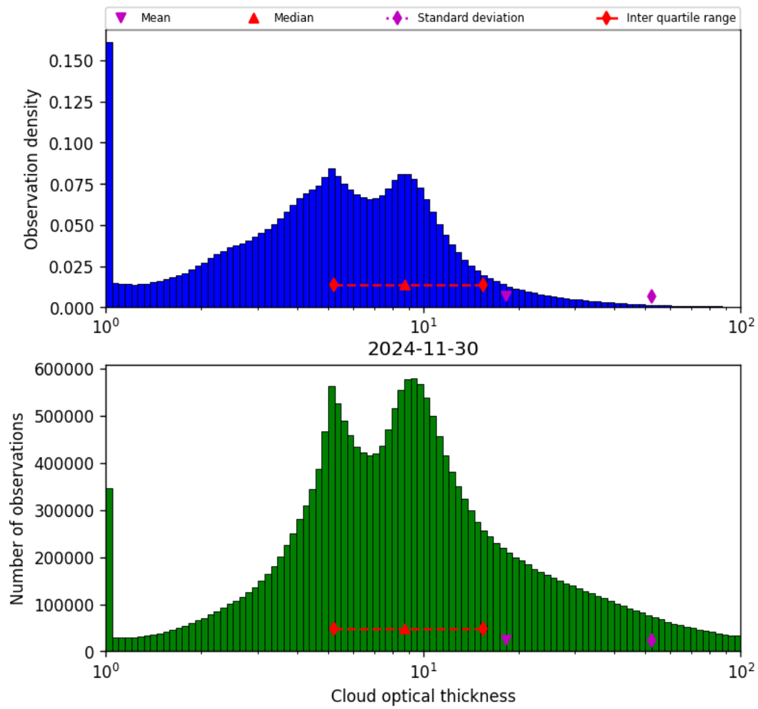
Figure 41: Histogram of “Cloud optical thickness” for 2024-11-30 to 2024-12-01
