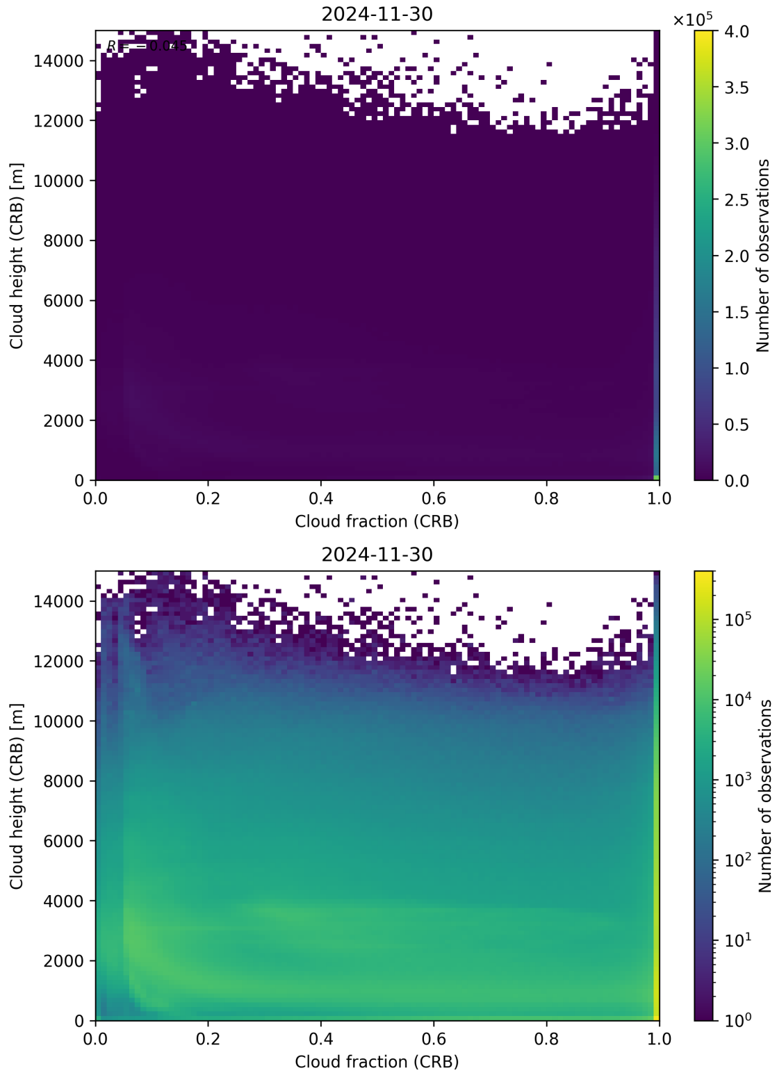
Figure 79: Scatter density plot of “Cloud fraction (CRB)” against “Cloud height (CRB)” for 2024-11-30 to 2024-12-01.
