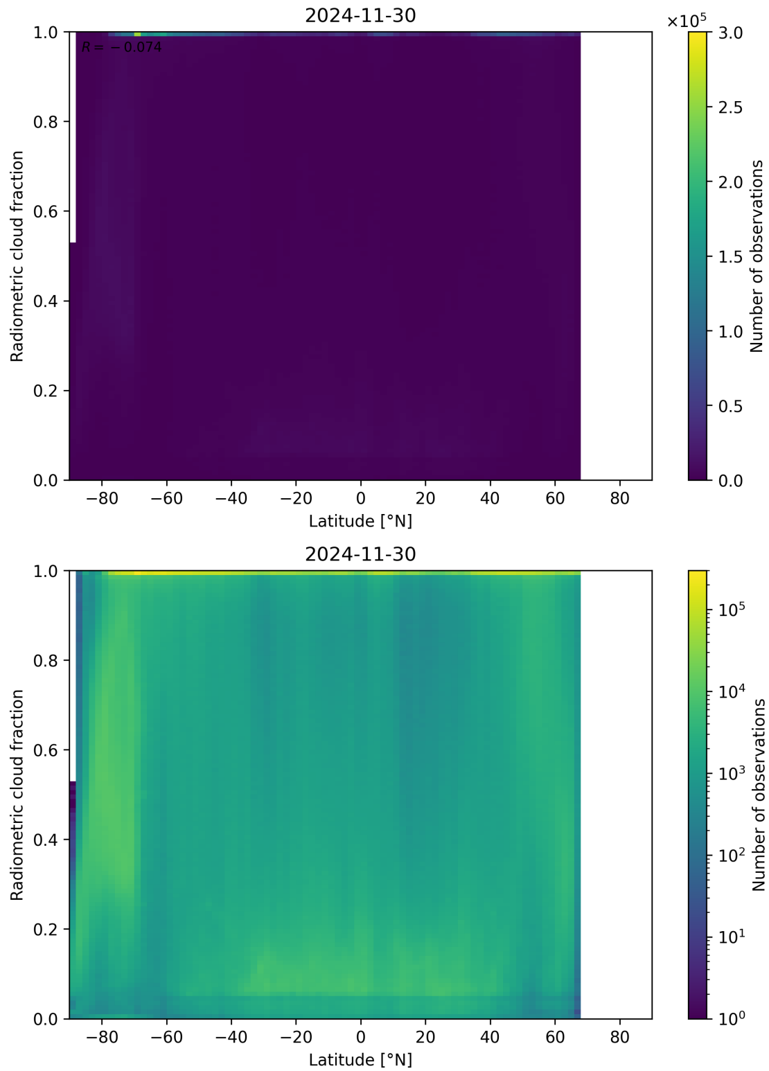
Figure 92: Scatter density plot of “Latitude” against “Radiometric cloud fraction” for 2024-11-30 to 2024-12-01.
