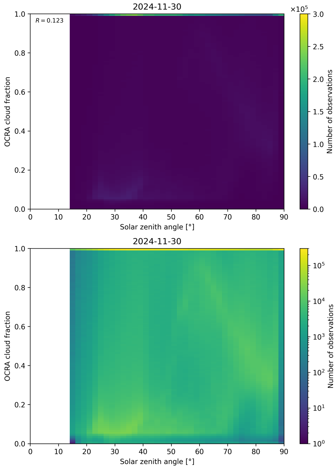
Figure 100: Scatter density plot of “Solar zenith angle” against “OCRA cloud fraction” for 2024-11-30 to 2024-12-01.
