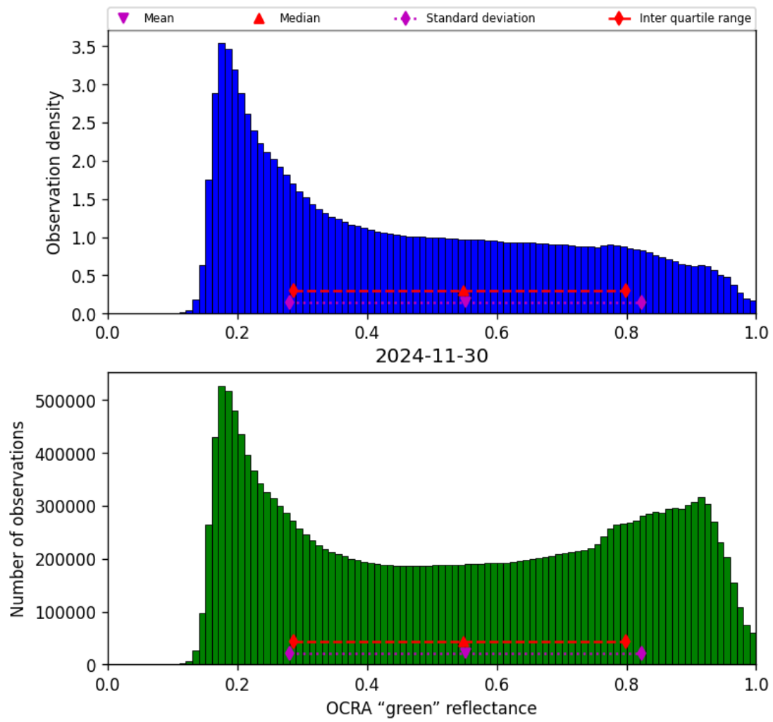
Figure 52: Histogram of “OCRA “green” reflectance” for 2024-11-30 to 2024-12-01
