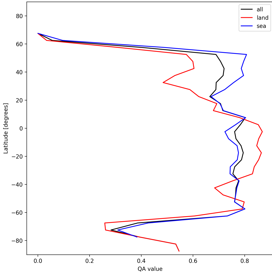
Figure 22: Zonal average of “QA value” for 2024-11-30 to 2024-12-01.
