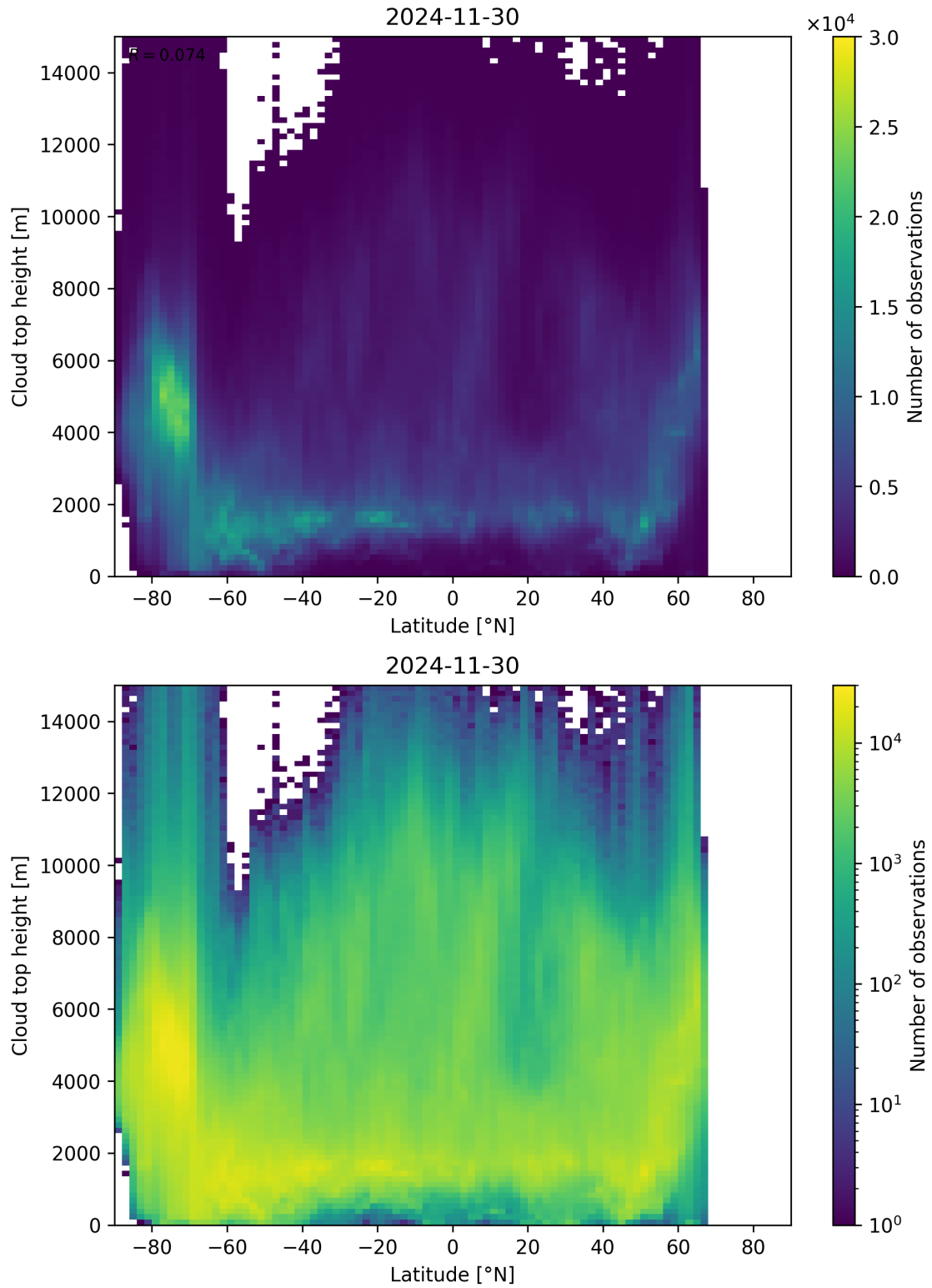
Figure 97: Scatter density plot of “Latitude” against “Cloud top height” for 2024-11-30 to 2024-12-01.
