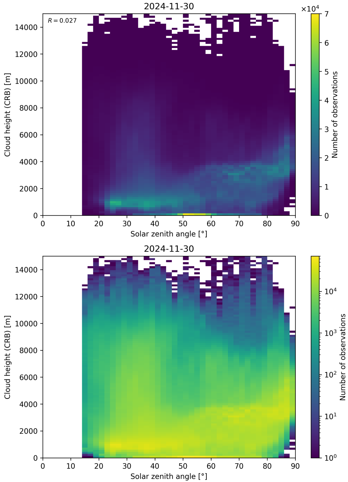
Figure 102: Scatter density plot of “Solar zenith angle” against “Cloud height (CRB)” for 2024-11-30 to 2024-12-01.
