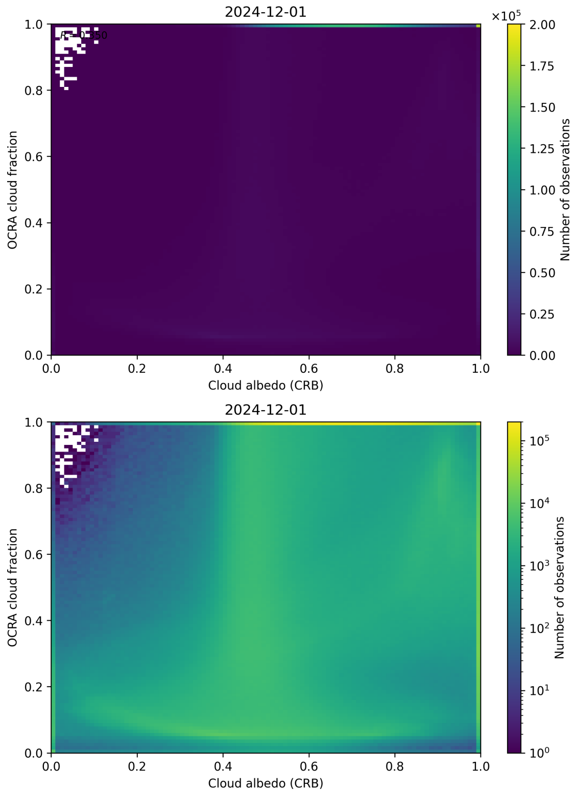
Figure 70: Scatter density plot of “Cloud albedo (CRB)” against “OCRA cloud fraction” for 2024-11-30 to 2024-12-02.
