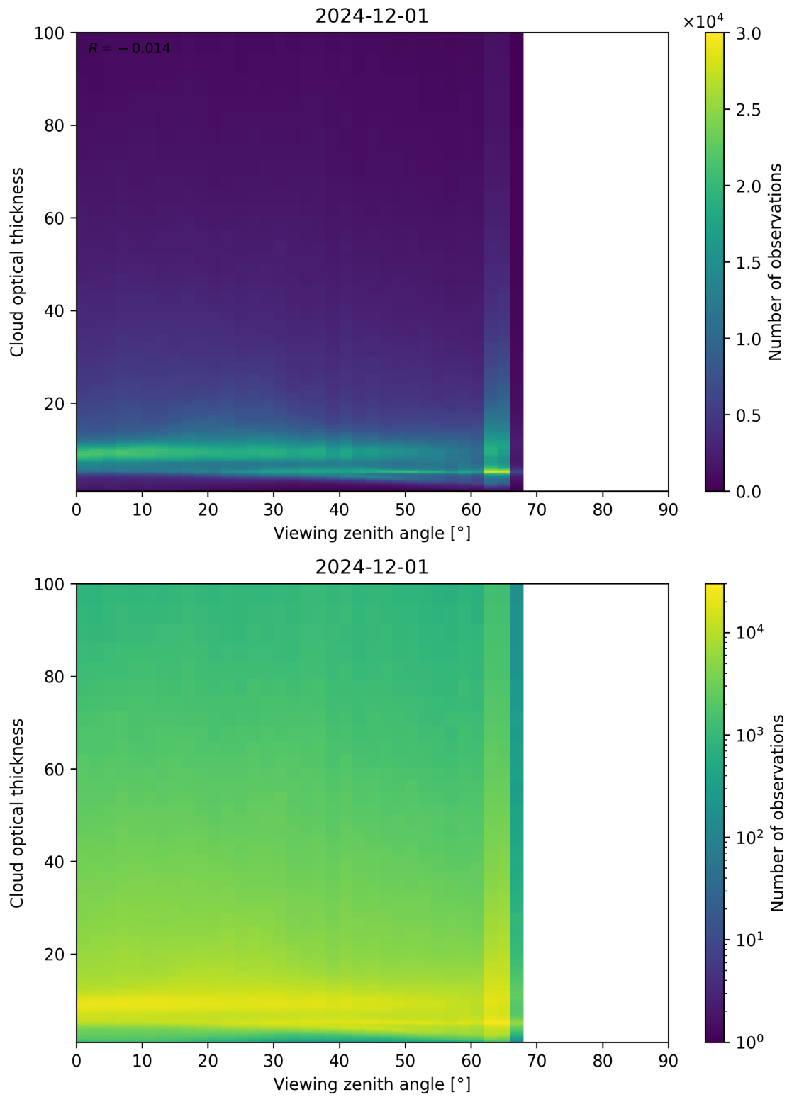
Figure 111: Scatter density plot of “Viewing zenith angle” against “Cloud optical thickness” for 2024-11-30 to 2024-12-02.
