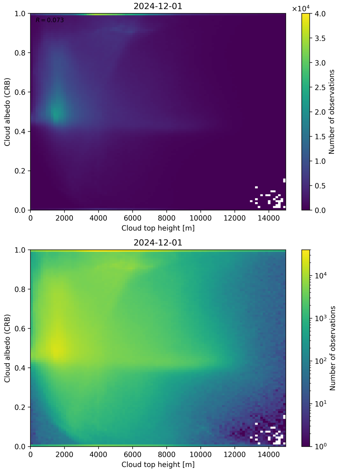
Figure 86: Scatter density plot of “Cloud top height” against “Cloud albedo (CRB)” for 2024-11-30 to 2024-12-02.
