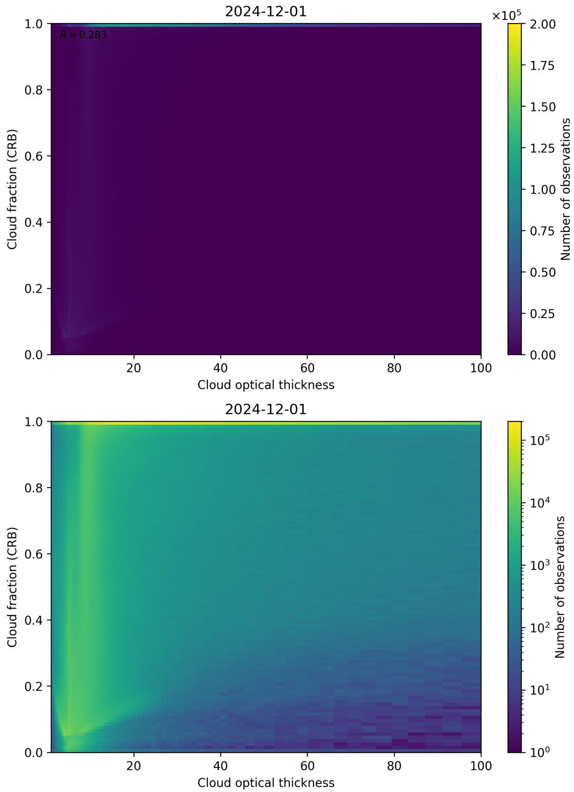
Figure 84: Scatter density plot of “Cloud optical thickness” against “Cloud fraction (CRB)” for 2024-11-30 to 2024-12-02.
