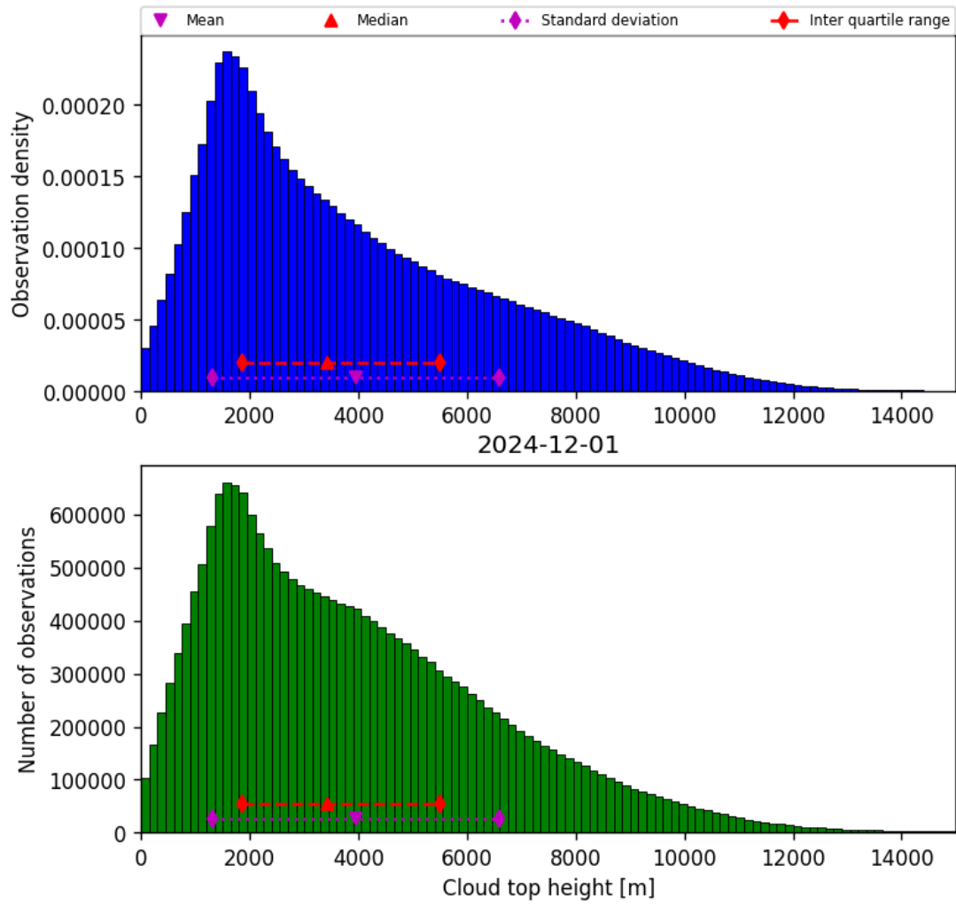
Figure 40: Histogram of “Cloud top height” for 2024-11-30 to 2024-12-02
