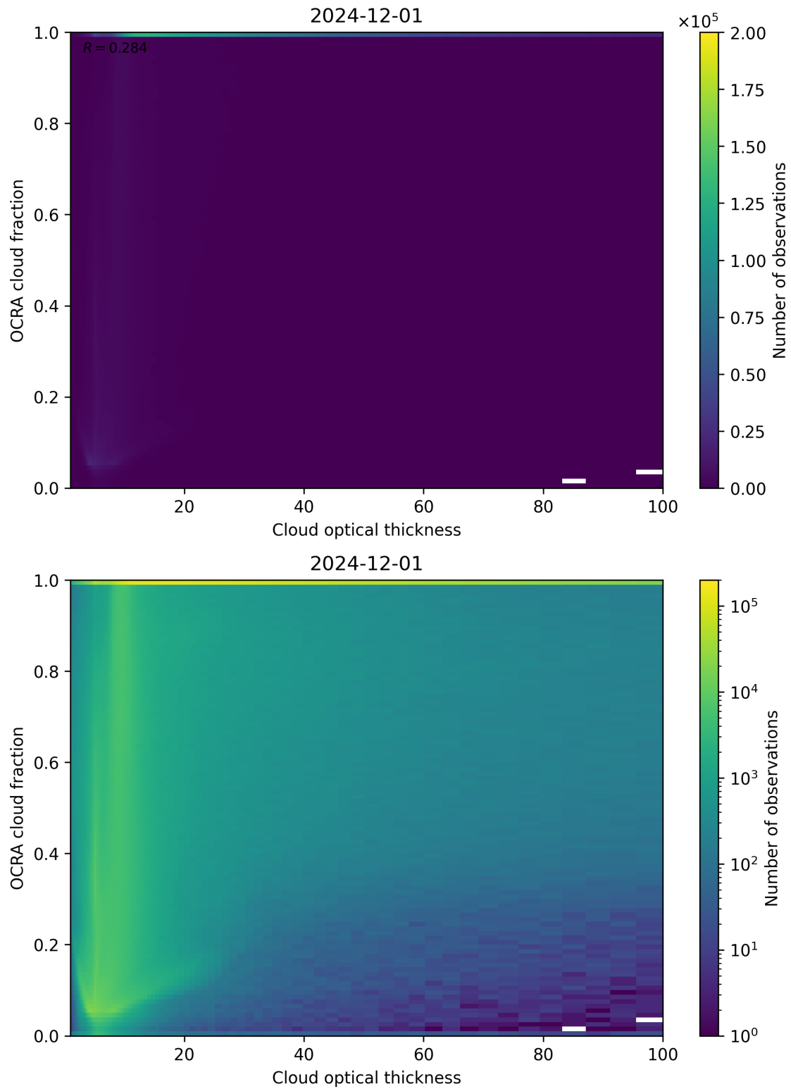
Figure 83: Scatter density plot of “Cloud optical thickness” against “OCRA cloud fraction” for 2024-11-30 to 2024-12-02.
