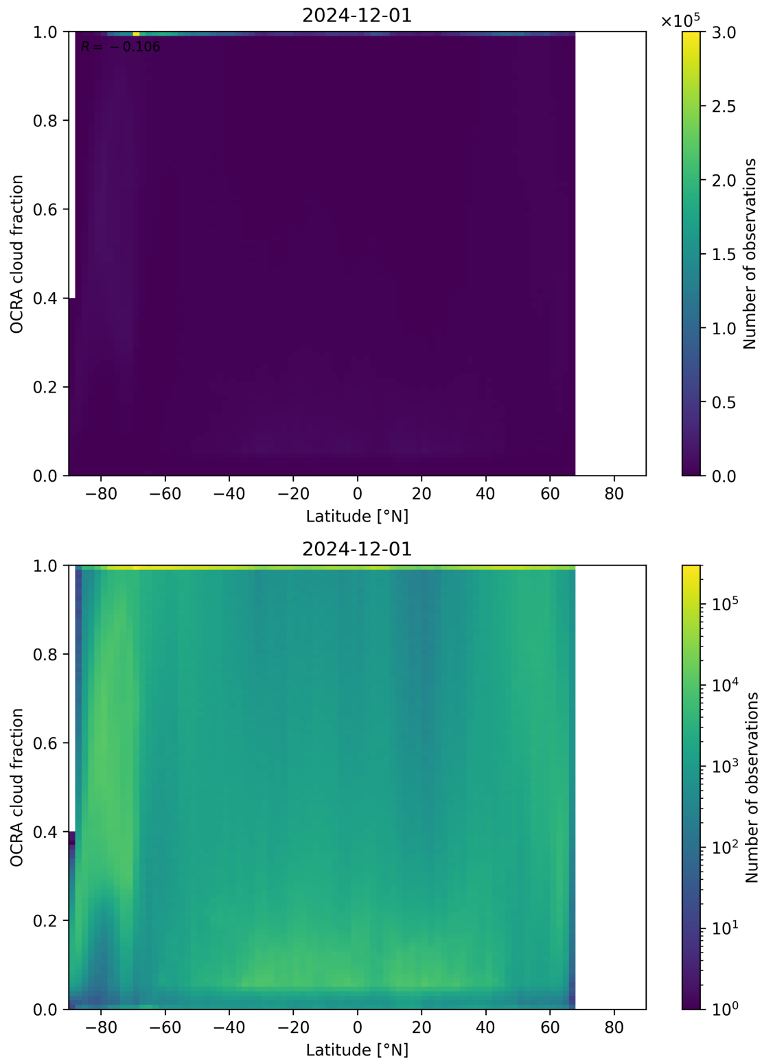
Figure 93: Scatter density plot of “Latitude” against “OCRA cloud fraction” for 2024-11-30 to 2024-12-02.
