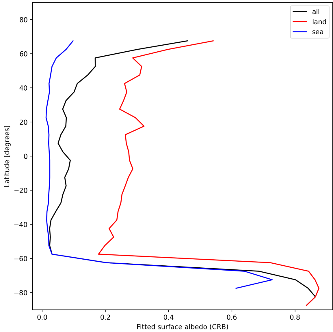
Figure 30: Zonal average of “Fitted surface albedo (CRB)” for 2024-11-30 to 2024-12-02.
