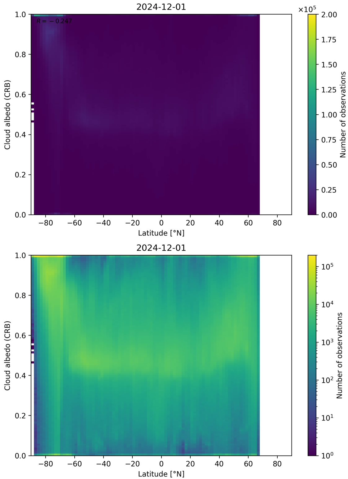
Figure 91: Scatter density plot of “Latitude” against “Cloud albedo (CRB)” for 2024-11-30 to 2024-12-02.
