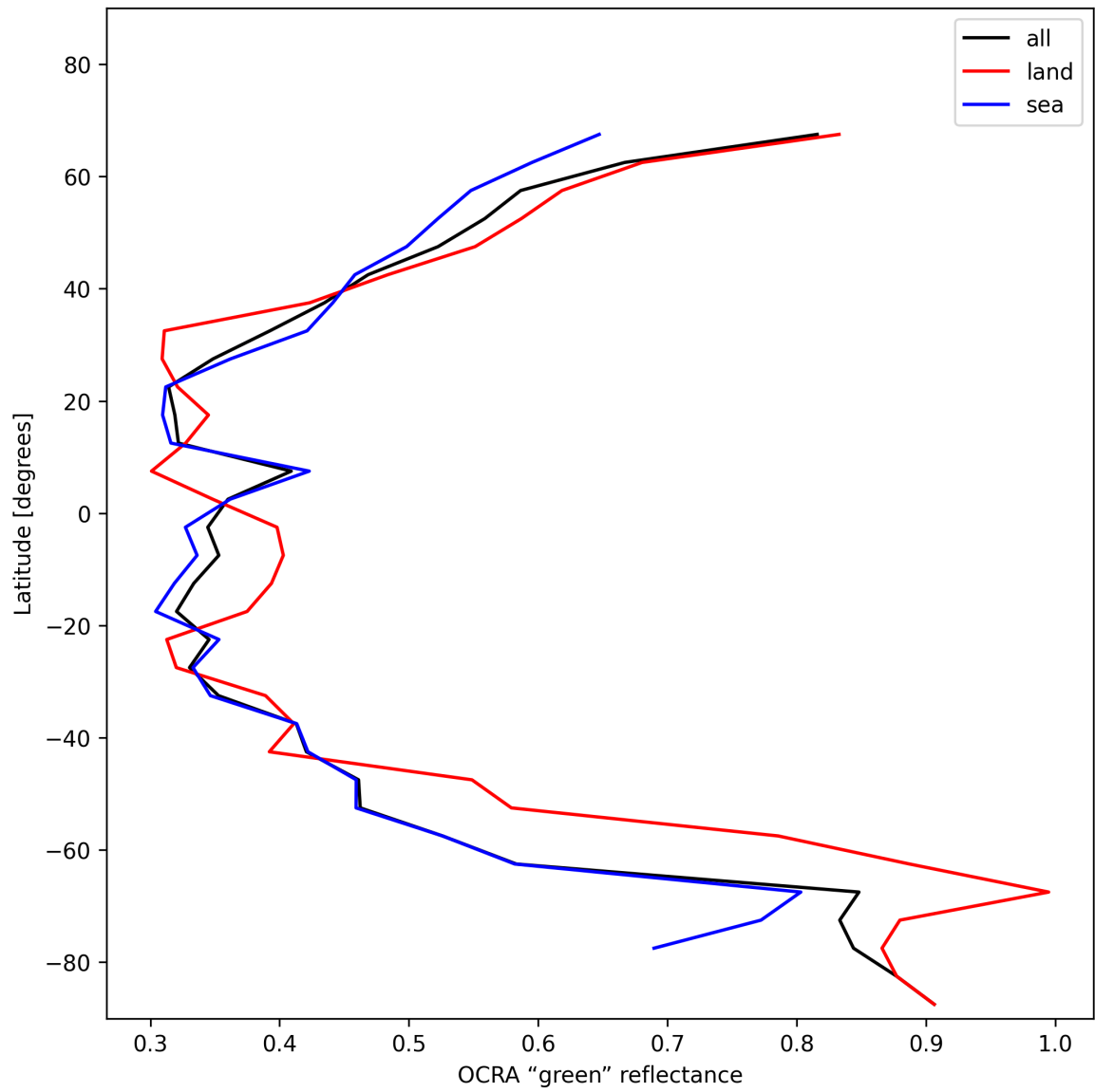
Figure 36: Zonal average of “OCRA “green” reflectance” for 2024-11-30 to 2024-12-02.
