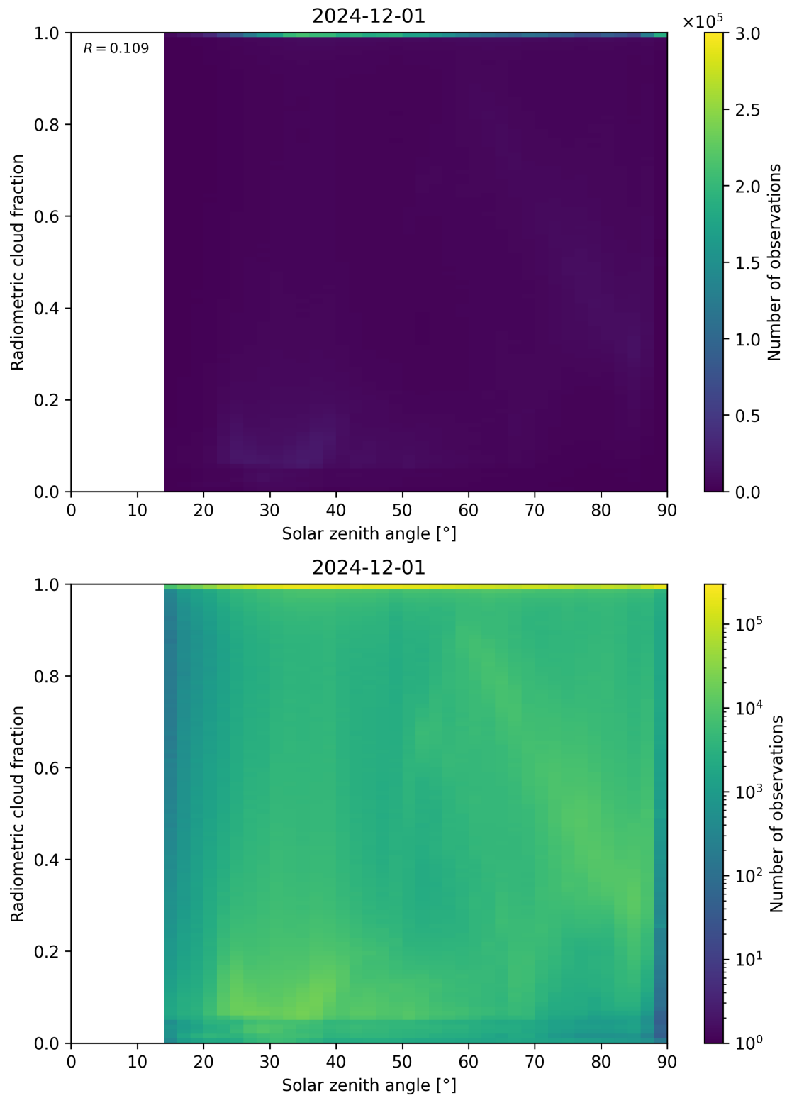
Figure 99: Scatter density plot of “Solar zenith angle” against “Radiometric cloud fraction” for 2024-11-30 to 2024-12-02.
