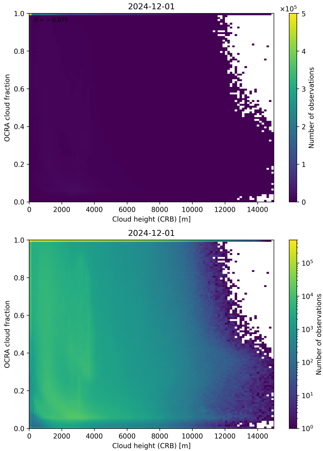
Figure 81: Scatter density plot of “Cloud height (CRB)” against “OCRA cloud fraction” for 2024-11-30 to 2024-12-02.
