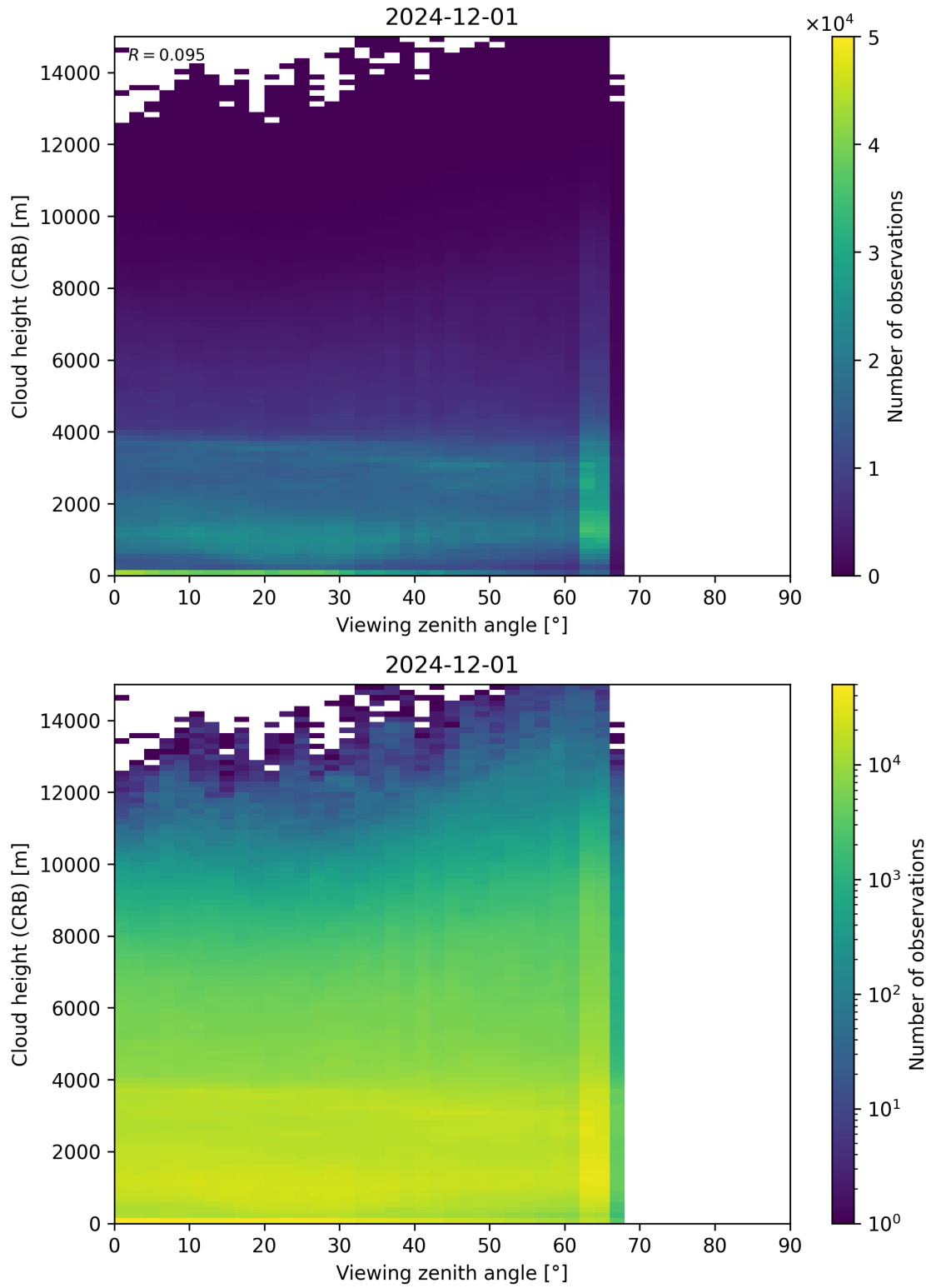
Figure 110: Scatter density plot of “Viewing zenith angle” against “Cloud height (CRB)” for 2024-11-30 to 2024-12-02.
