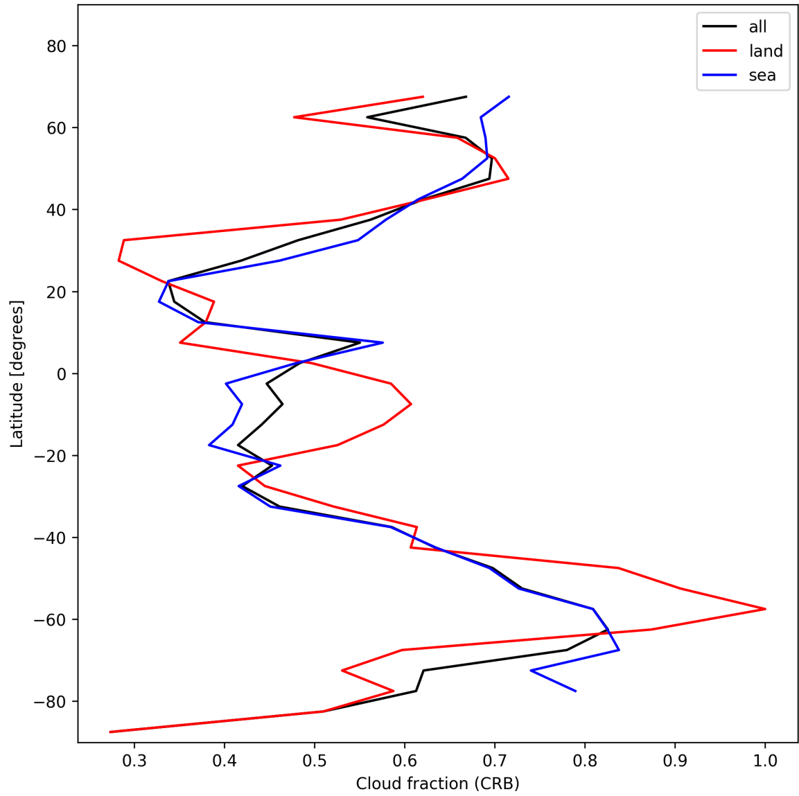
Figure 26: Zonal average of “Cloud fraction (CRB)” for 2024-11-30 to 2024-12-02.
