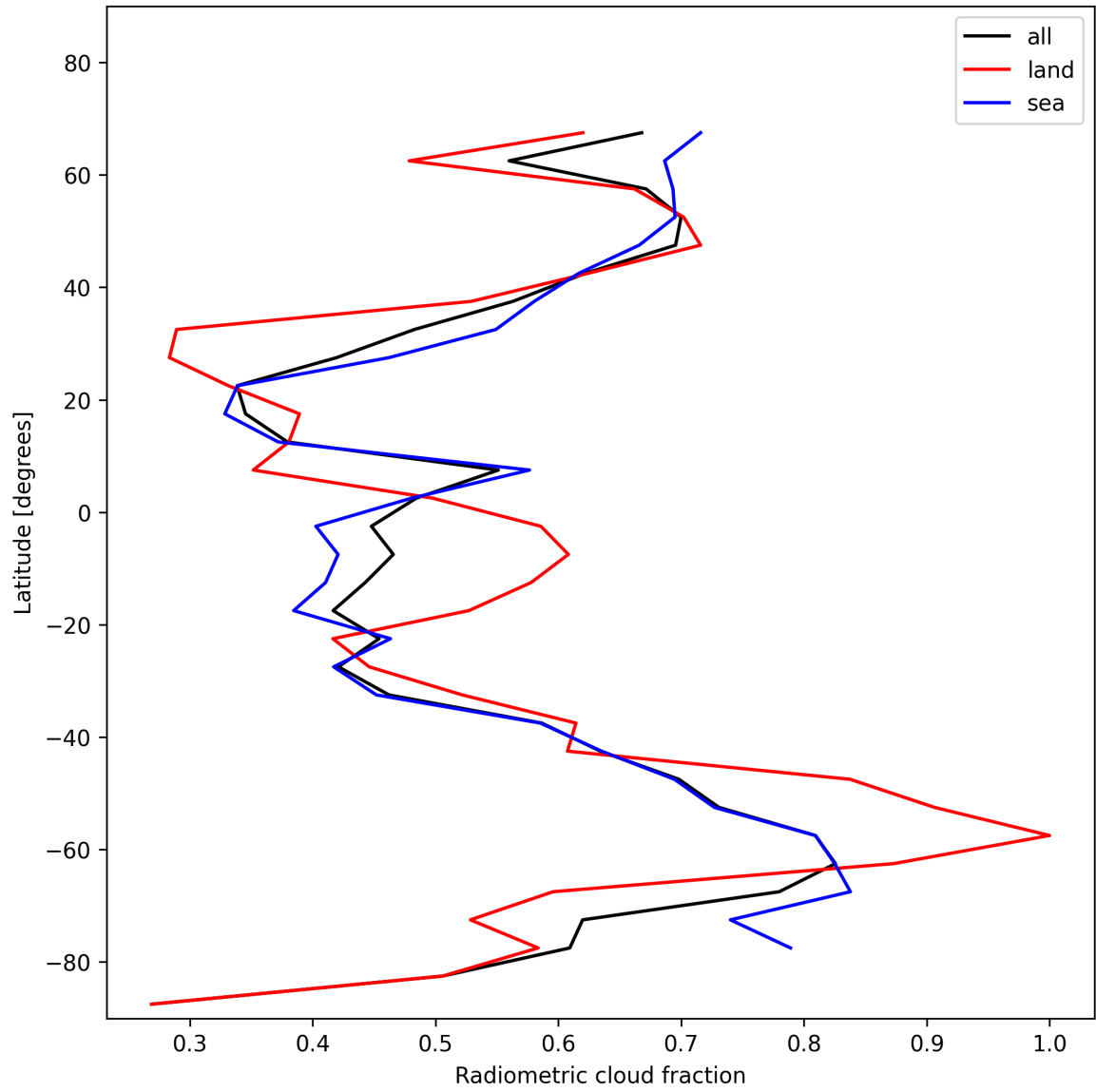
Figure 23: Zonal average of “Radiometric cloud fraction” for 2024-11-30 to 2024-12-02.
