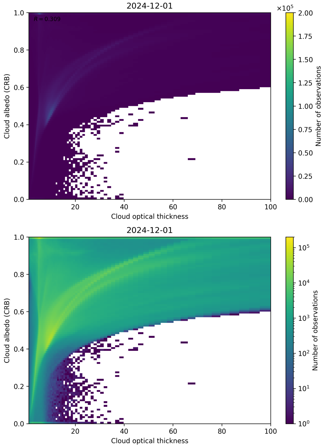
Figure 82: Scatter density plot of “Cloud optical thickness” against “Cloud albedo (CRB)” for 2024-11-30 to 2024-12-02.
