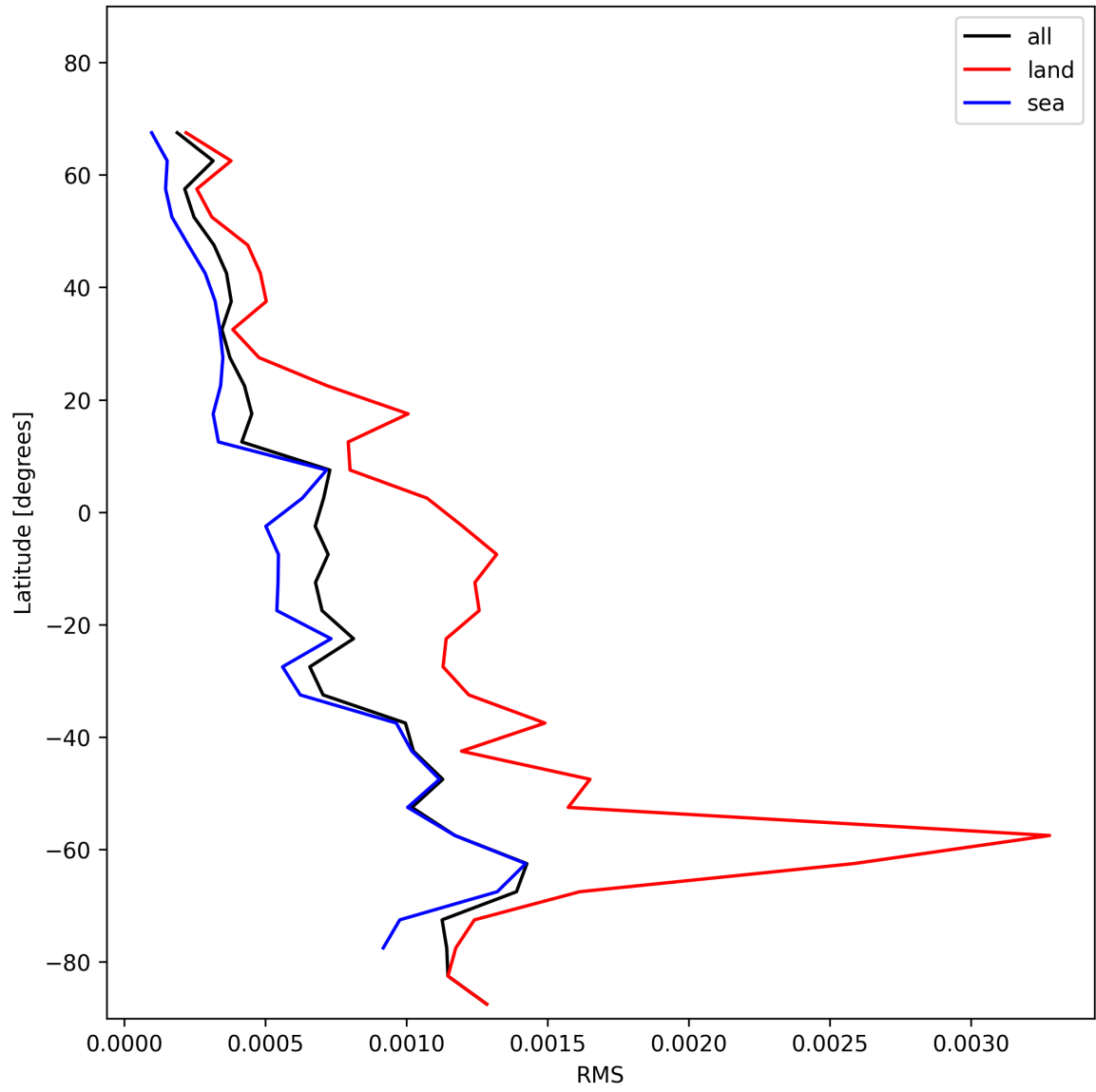
Figure 31: Zonal average of “RMS” for 2024-11-30 to 2024-12-02.
