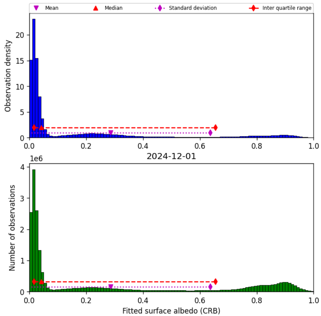
Figure 46: Histogram of “Fitted surface albedo (CRB)” for 2024-11-30 to 2024-12-02
