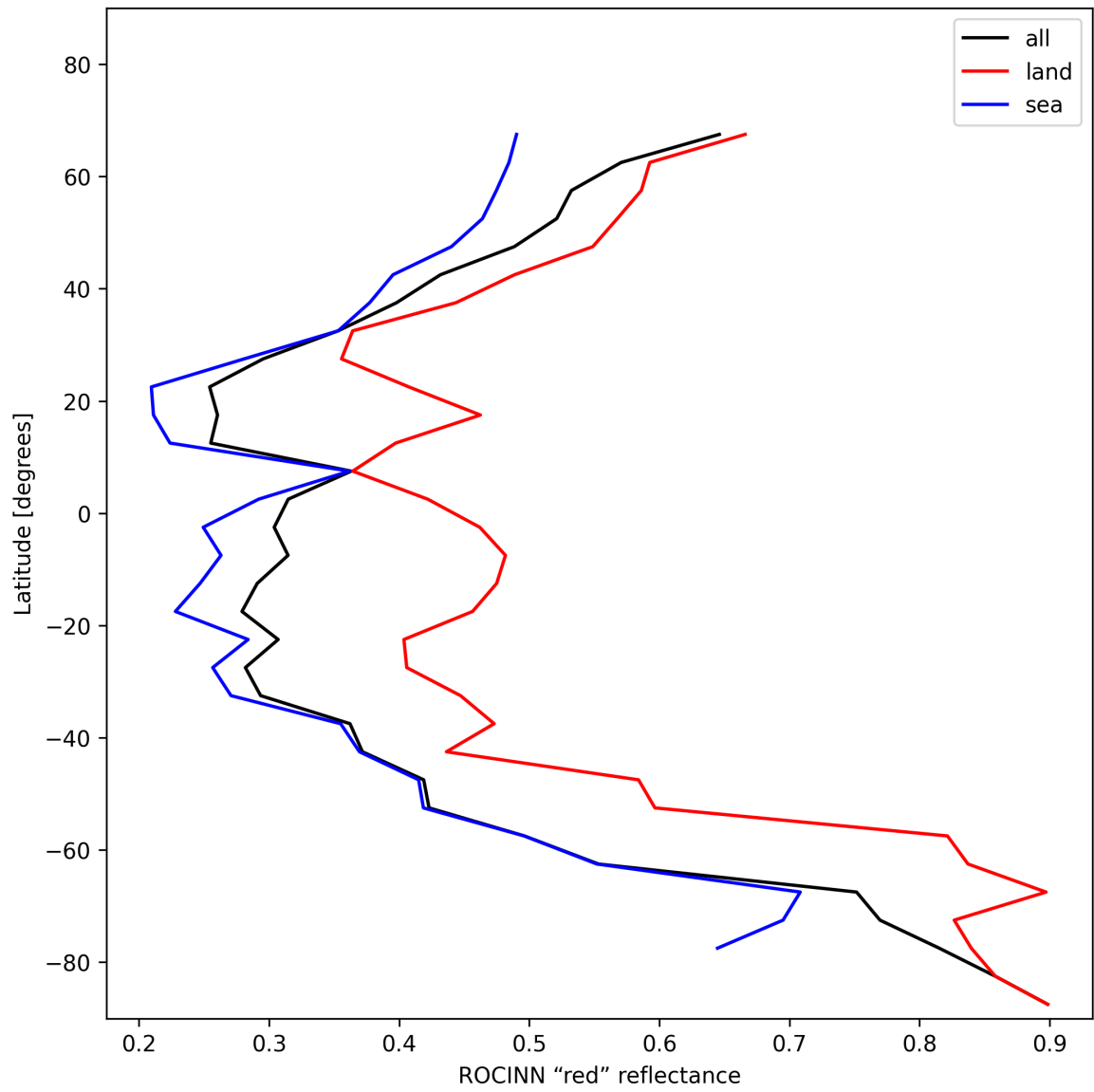
Figure 37: Zonal average of “ROCINN “red” reflectance” for 2024-11-30 to 2024-12-02.
