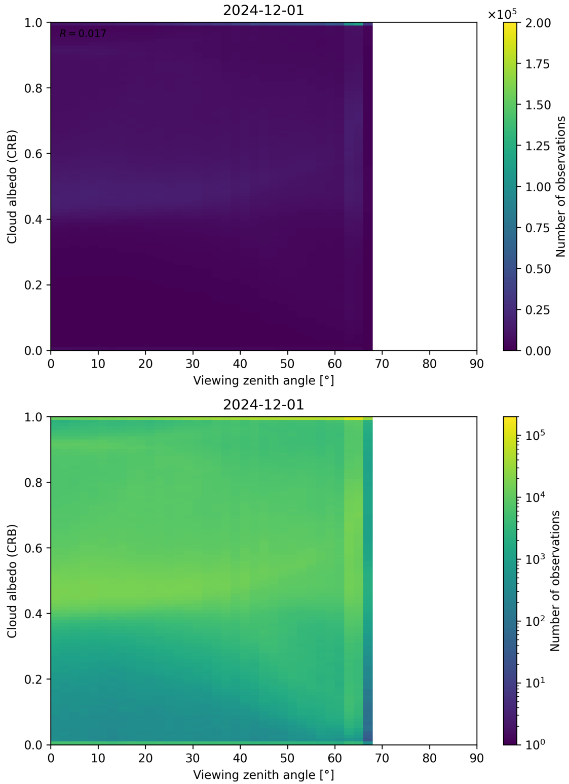
Figure 106: Scatter density plot of “Viewing zenith angle” against “Cloud albedo (CRB)” for 2024-11-30 to 2024-12-02.
