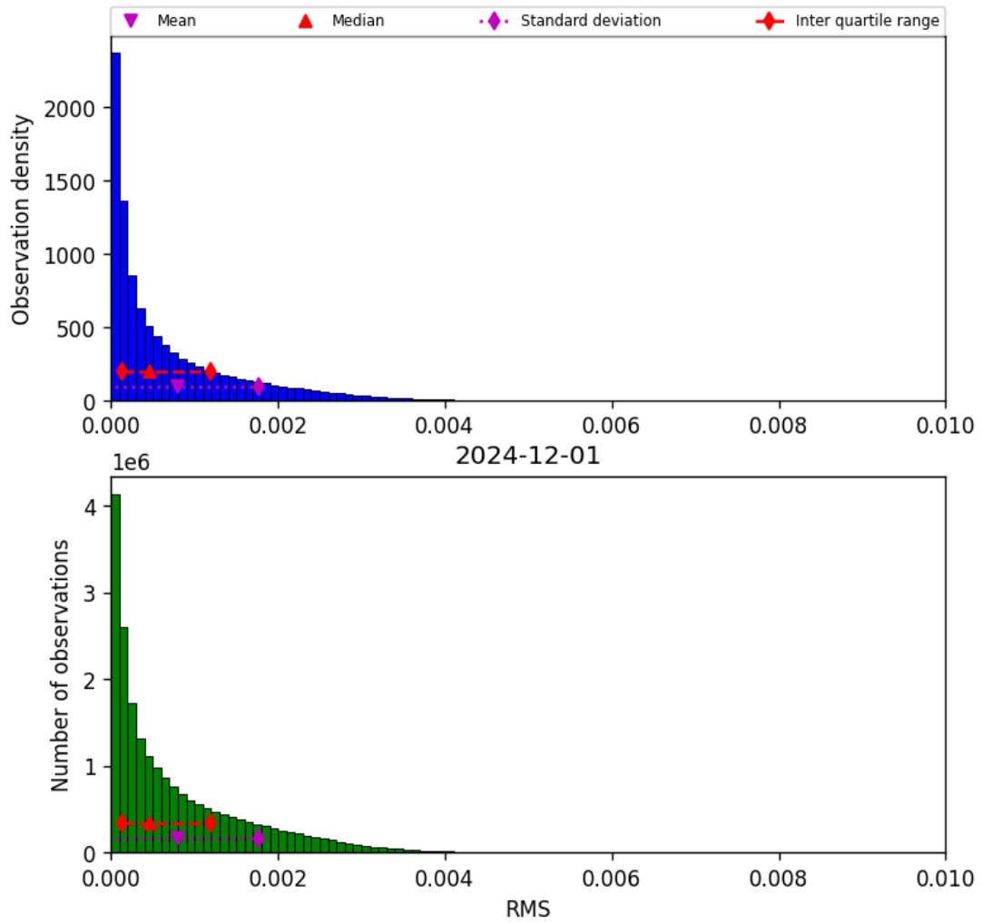
Figure 47: Histogram of “RMS” for 2024-11-30 to 2024-12-02
