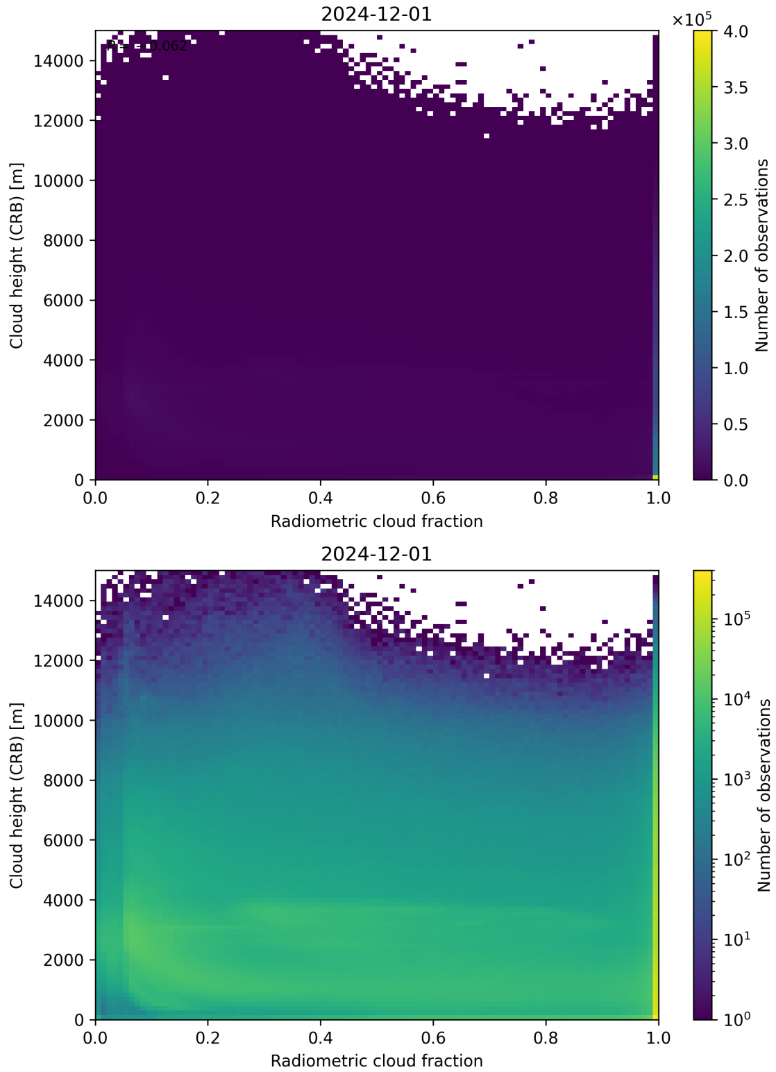
Figure 74: Scatter density plot of “Radiometric cloud fraction” against “Cloud height (CRB)” for 2024-11-30 to 2024-12-02.
