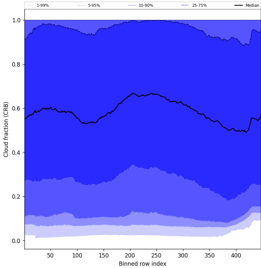
Figure 58: Along track statistics of “Cloud fraction (CRB)” for 2024-11-30 to 2024-12-02
