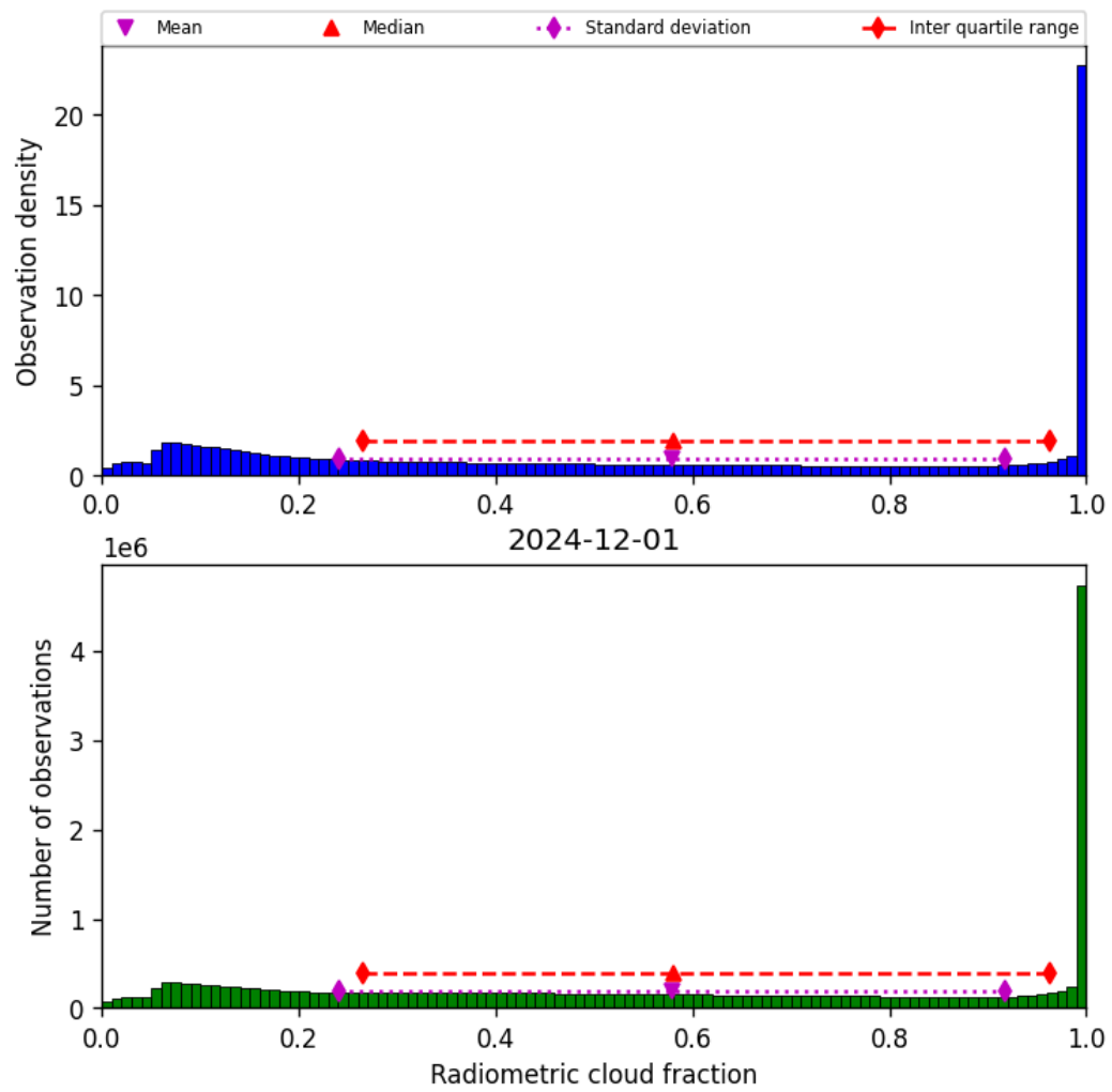
Figure 39: Histogram of “Radiometric cloud fraction” for 2024-11-30 to 2024-12-02
