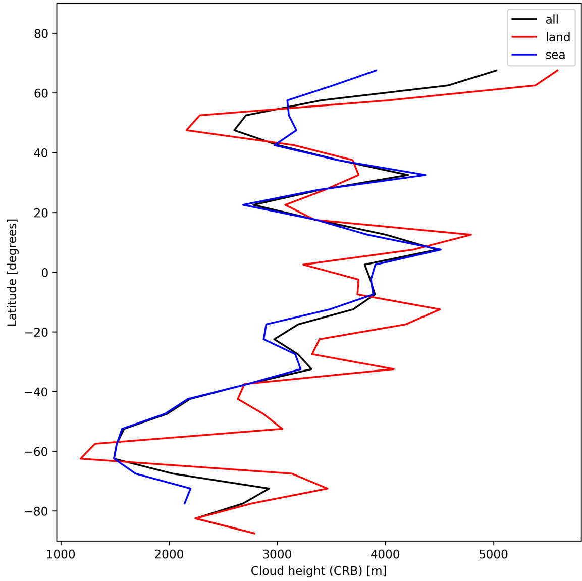
Figure 27: Zonal average of “Cloud height (CRB)” for 2024-11-30 to 2024-12-02.
