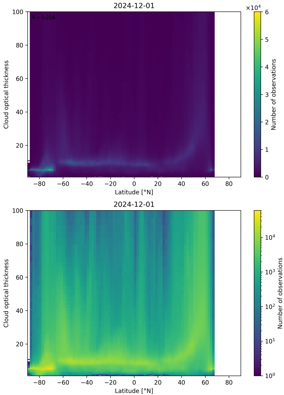
Figure 96: Scatter density plot of “Latitude” against “Cloud optical thickness” for 2024-11-30 to 2024-12-02.
