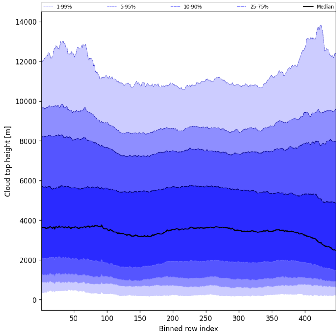
Figure 56: Along track statistics of “Cloud top height” for 2024-11-30 to 2024-12-02
