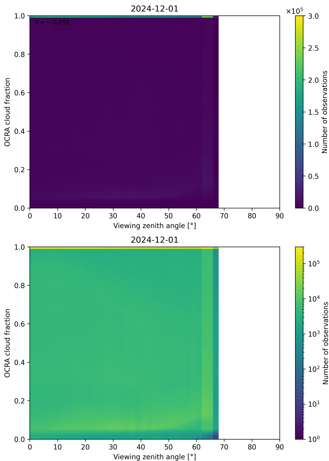
Figure 108: Scatter density plot of “Viewing zenith angle” against “OCRA cloud fraction” for 2024-11-30 to 2024-12-02.
