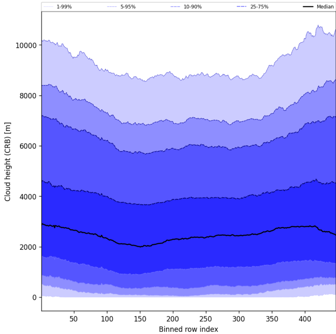
Figure 59: Along track statistics of “Cloud height (CRB)” for 2024-11-30 to 2024-12-02
