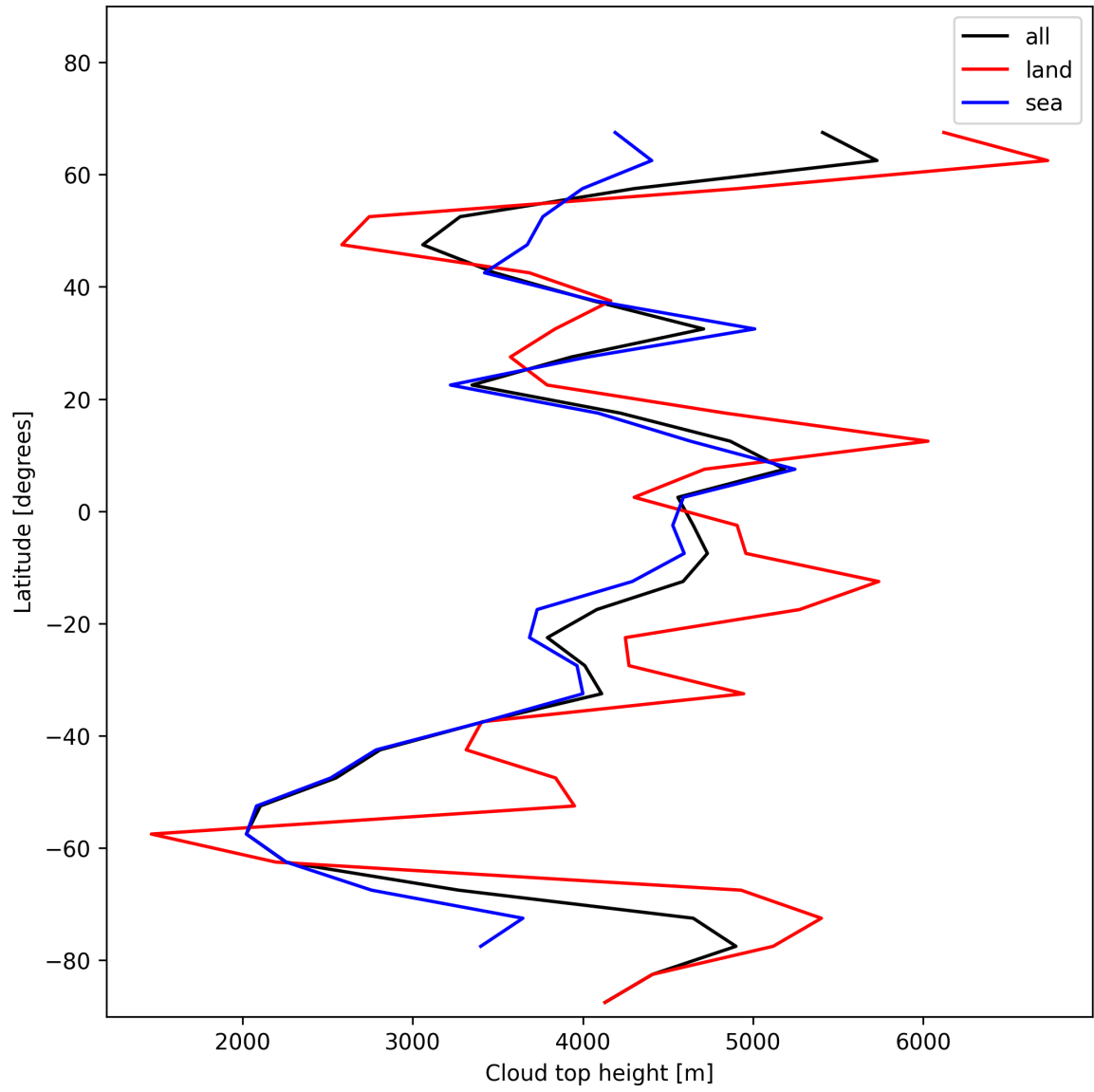
Figure 24: Zonal average of “Cloud top height” for 2024-11-30 to 2024-12-02.
