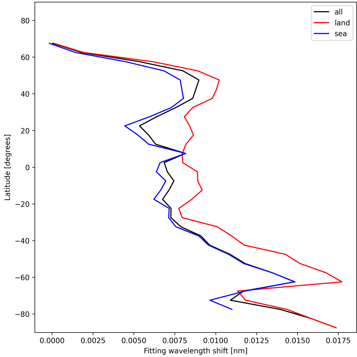
Figure 33: Zonal average of “Fitting wavelength shift” for 2024-11-30 to 2024-12-02.
