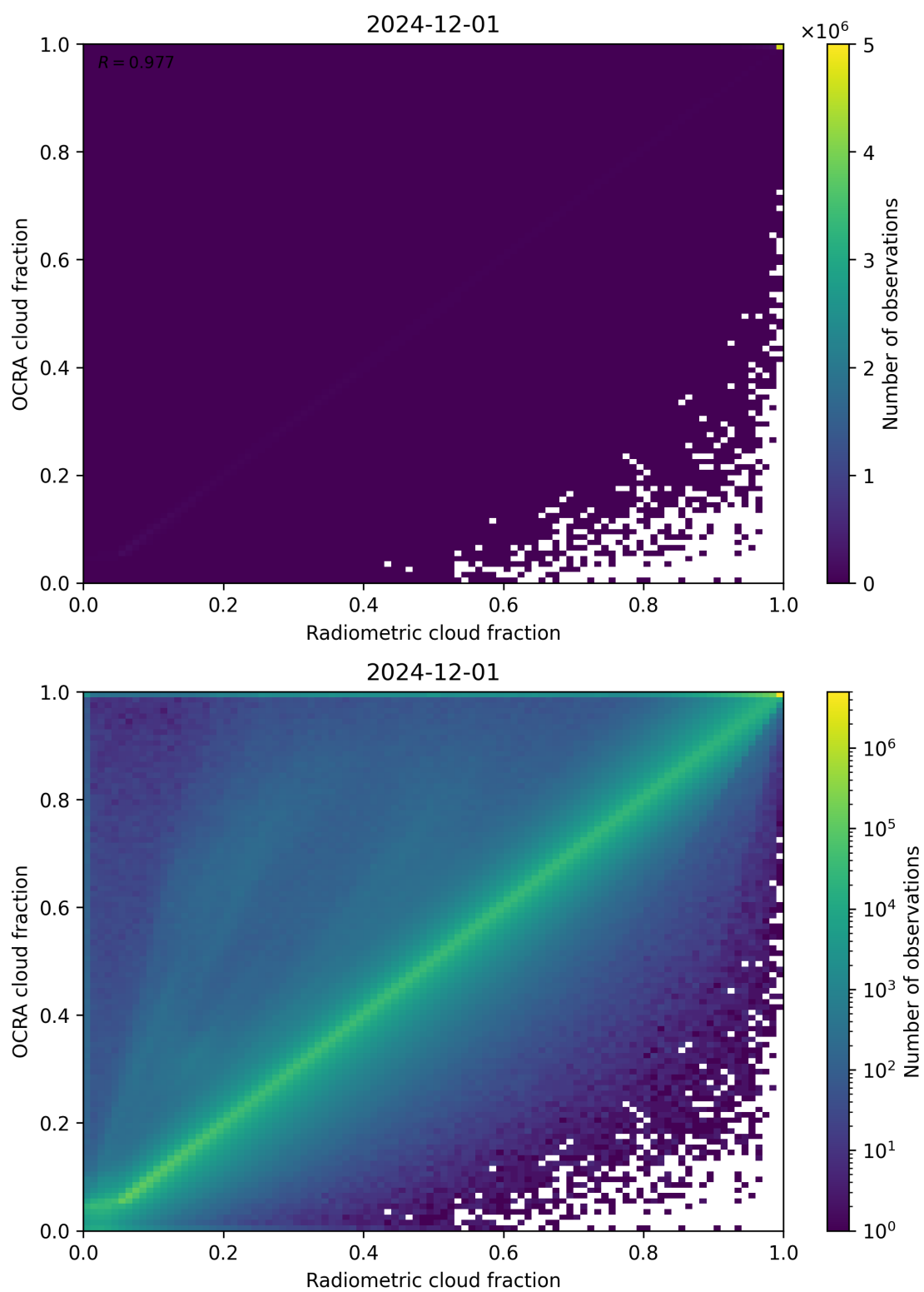
Figure 72: Scatter density plot of “Radiometric cloud fraction” against “OCRA cloud fraction” for 2024-11-30 to 2024-12-02.
