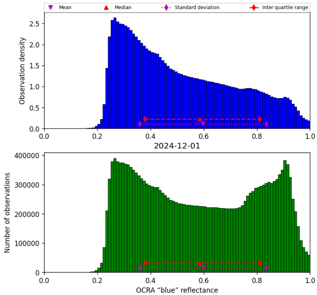
Figure 51: Histogram of “OCRA “blue” reflectance” for 2024-11-30 to 2024-12-02
