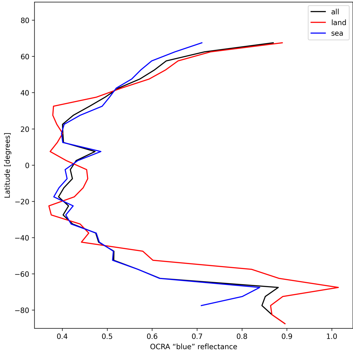
Figure 35: Zonal average of “OCRA “blue” reflectance” for 2024-11-30 to 2024-12-02.
