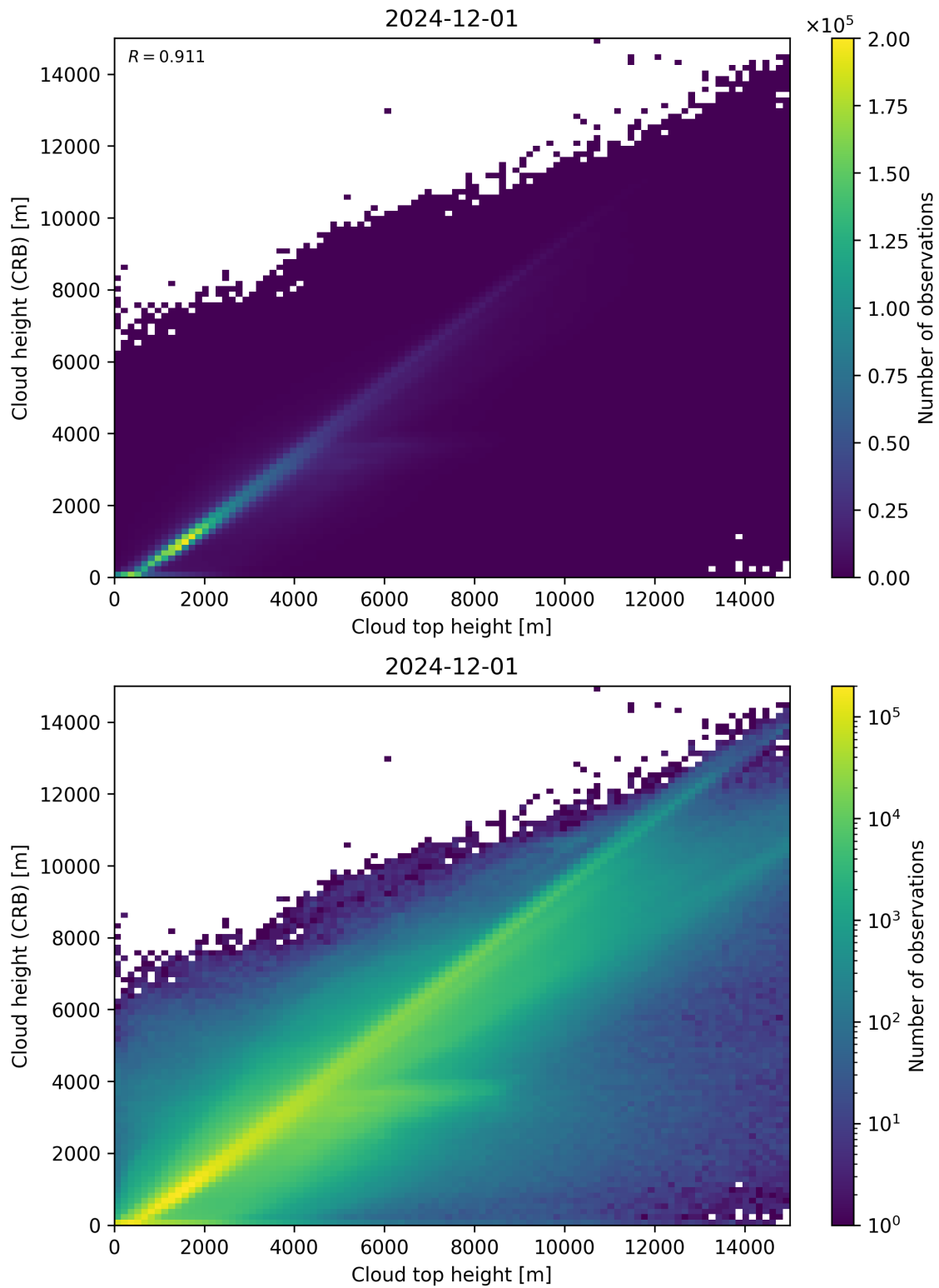
Figure 89: Scatter density plot of “Cloud top height” against “Cloud height (CRB)” for 2024-11-30 to 2024-12-02.
