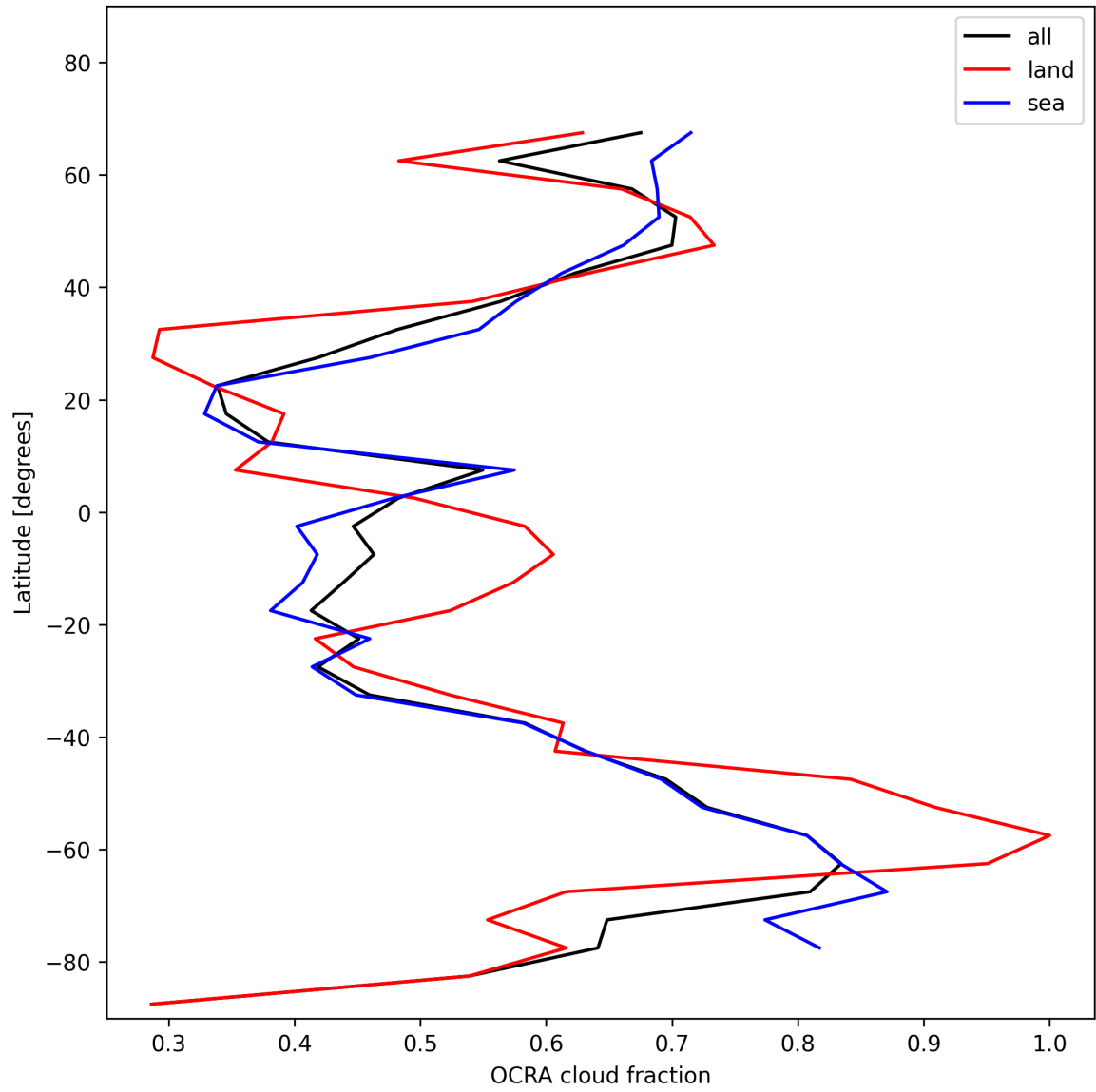
Figure 34: Zonal average of “OCRA cloud fraction” for 2024-11-30 to 2024-12-02.
