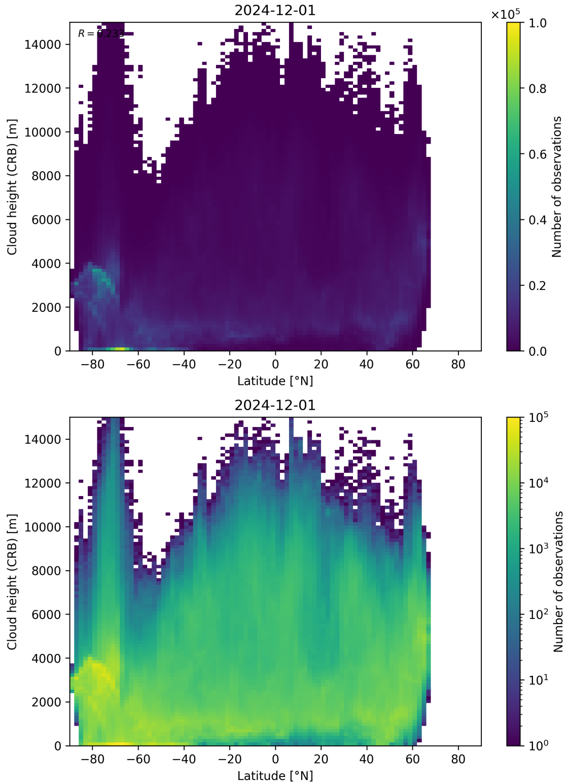
Figure 95: Scatter density plot of “Latitude” against “Cloud height (CRB)” for 2024-11-30 to 2024-12-02.
