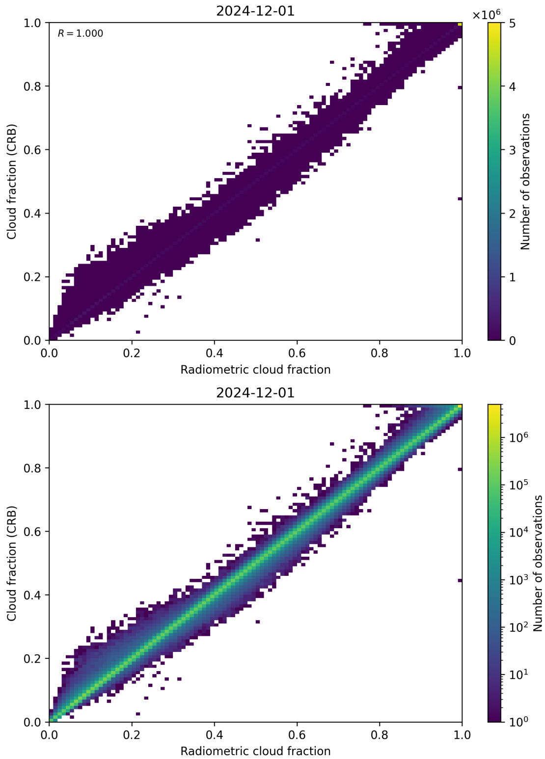
Figure 73: Scatter density plot of “Radiometric cloud fraction” against “Cloud fraction (CRB)” for 2024-11-30 to 2024-12-02.
