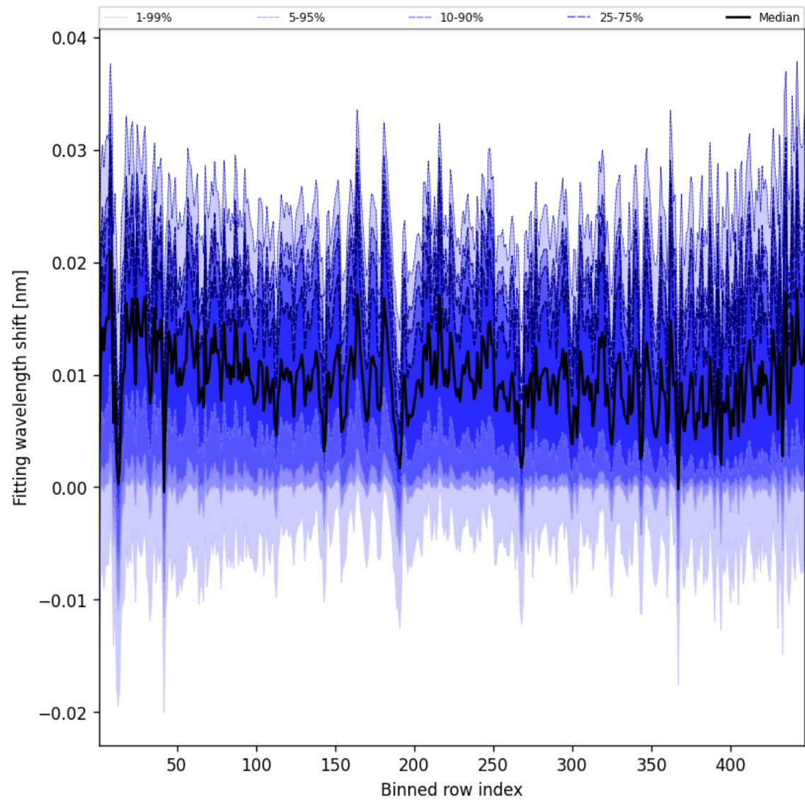
Figure 65: Along track statistics of “Fitting wavelength shift” for 2024-11-30 to 2024-12-02
