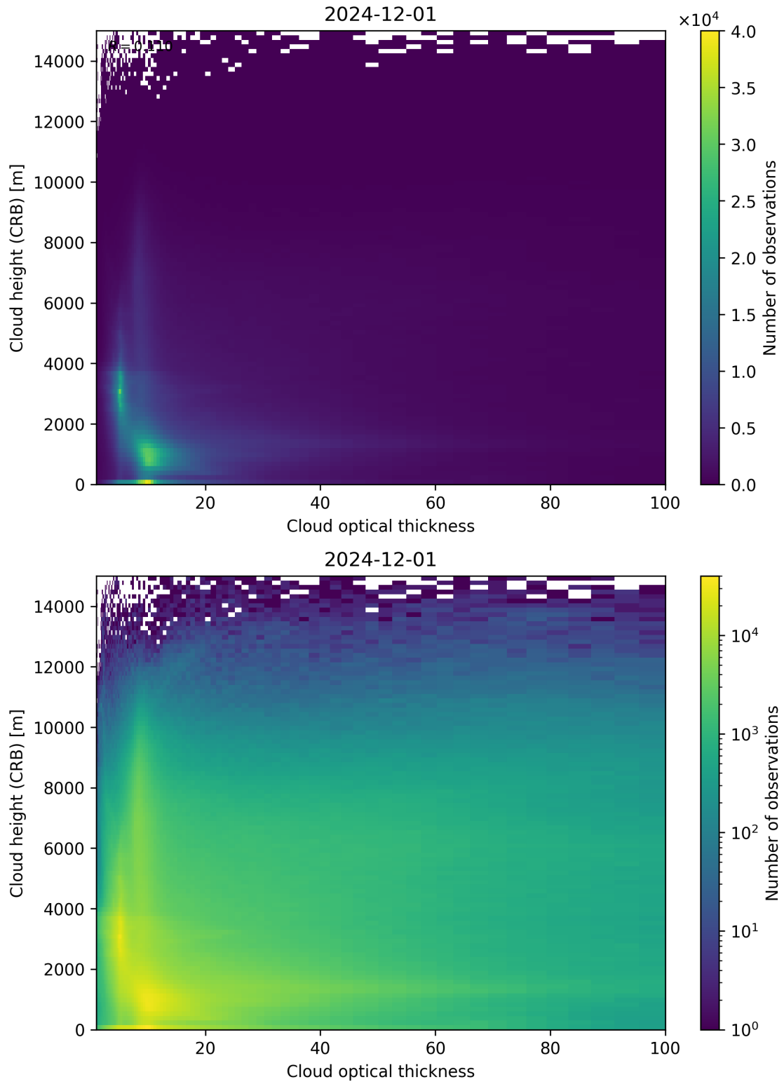
Figure 85: Scatter density plot of “Cloud optical thickness” against “Cloud height (CRB)” for 2024-11-30 to 2024-12-02.
