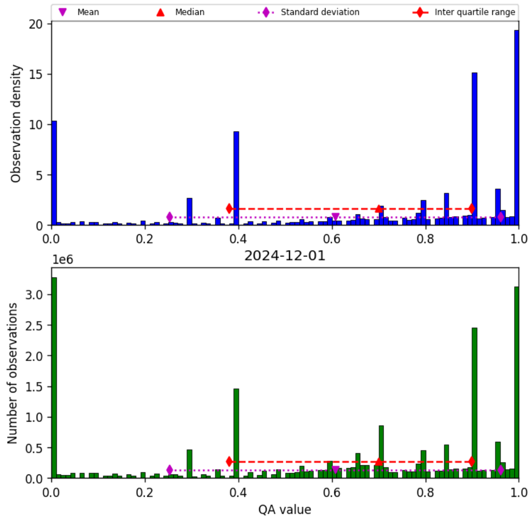
Figure 38: Histogram of “QA value” for 2024-11-30 to 2024-12-02
