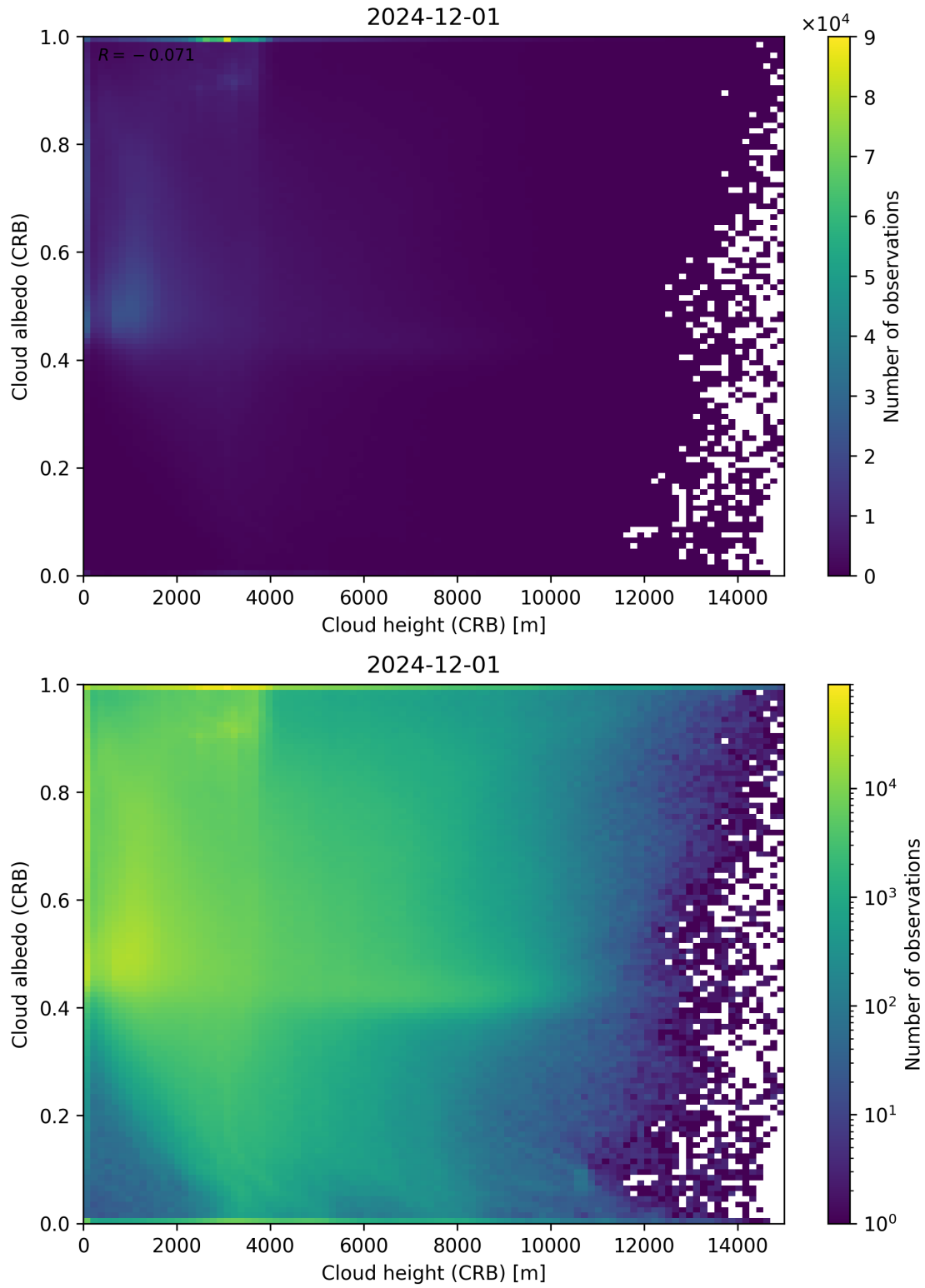
Figure 80: Scatter density plot of “Cloud height (CRB)” against “Cloud albedo (CRB)” for 2024-11-30 to 2024-12-02.
