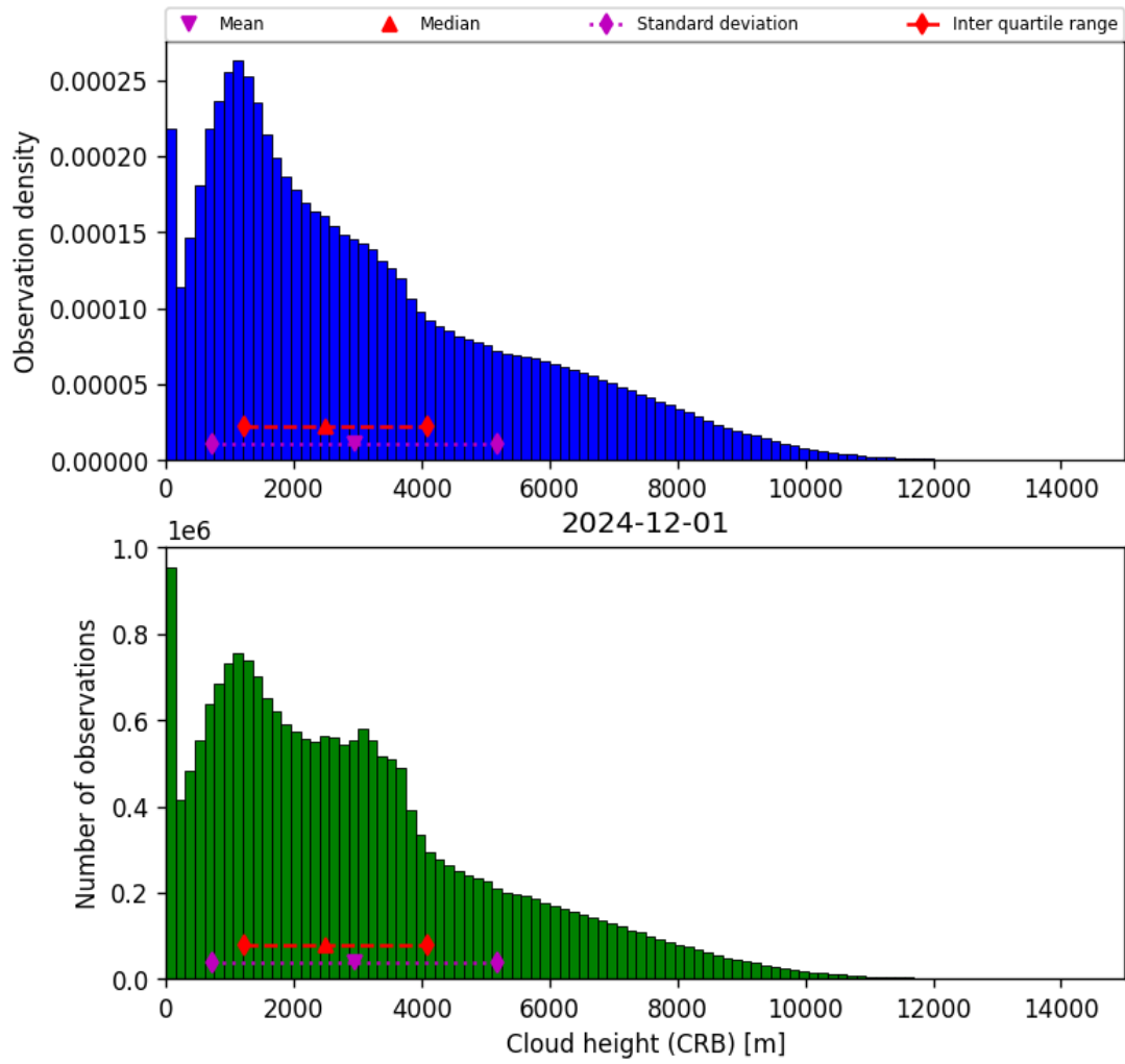
Figure 43: Histogram of “Cloud height (CRB)” for 2024-11-30 to 2024-12-02
