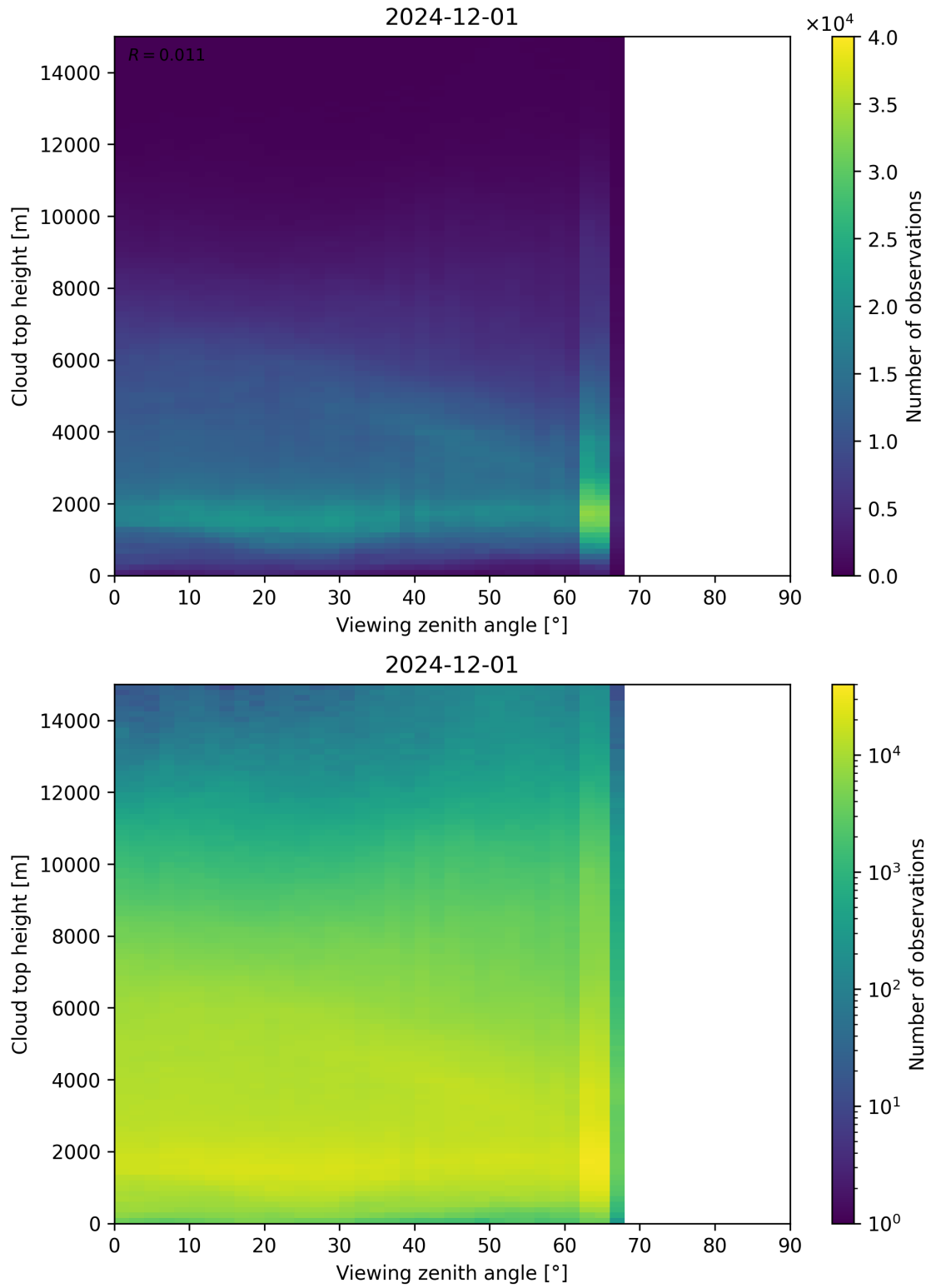
Figure 112: Scatter density plot of “Viewing zenith angle” against “Cloud top height” for 2024-11-30 to 2024-12-02.
