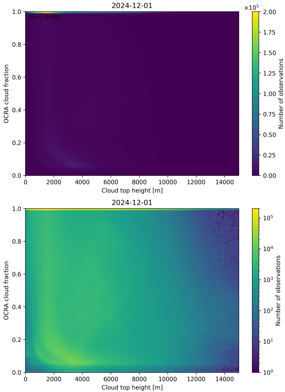
Figure 87: Scatter density plot of “Cloud top height” against “OCRA cloud fraction” for 2024-11-30 to 2024-12-02.
