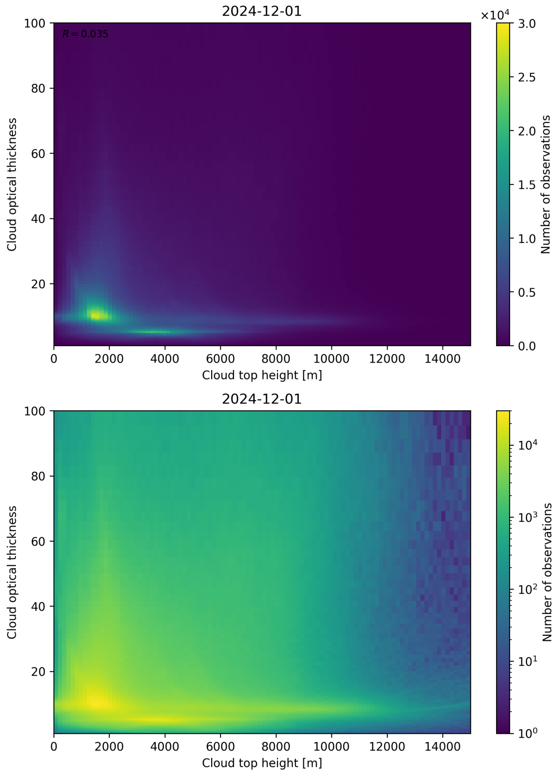
Figure 90: Scatter density plot of “Cloud top height” against “Cloud optical thickness” for 2024-11-30 to 2024-12-02.
