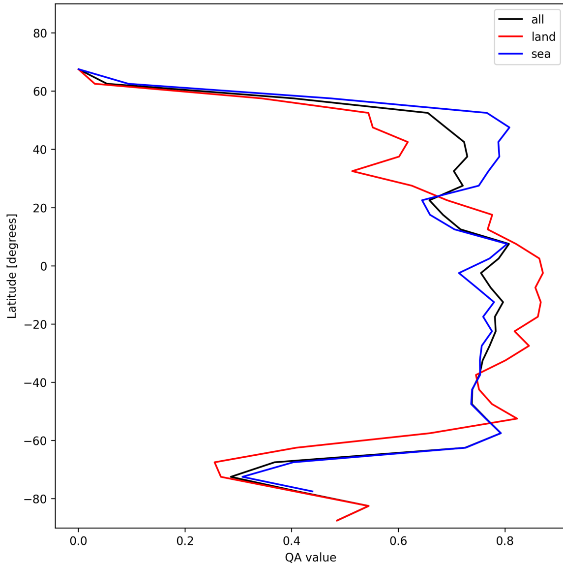
Figure 22: Zonal average of “QA value” for 2024-11-30 to 2024-12-02.
