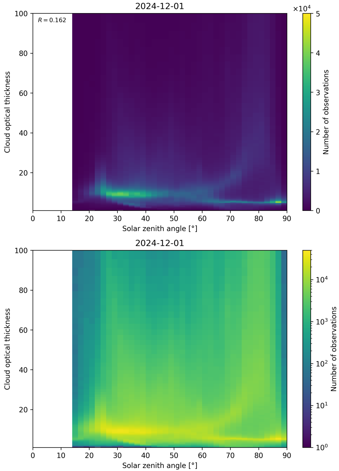
Figure 103: Scatter density plot of “Solar zenith angle” against “Cloud optical thickness” for 2024-11-30 to 2024-12-02.
