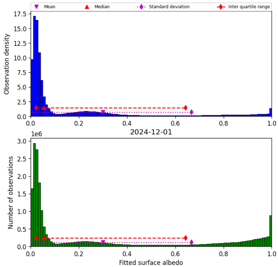
Figure 45: Histogram of “Fitted surface albedo” for 2024-11-30 to 2024-12-02
