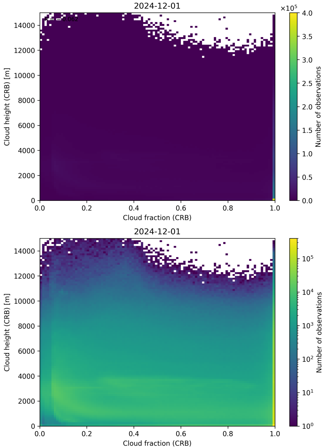
Figure 79: Scatter density plot of “Cloud fraction (CRB)” against “Cloud height (CRB)” for 2024-11-30 to 2024-12-02.
