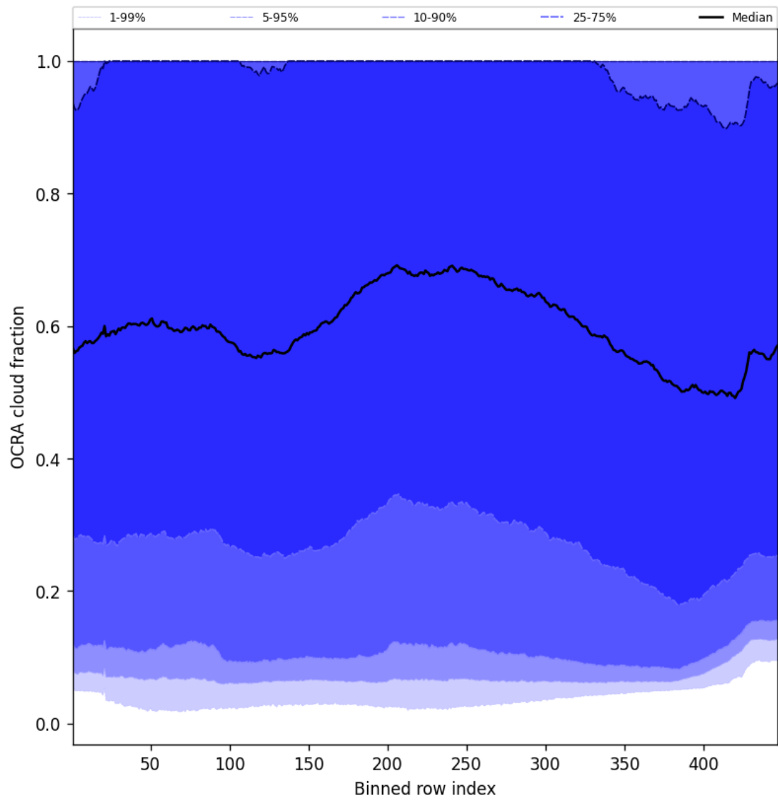
Figure 66: Along track statistics of “OCRA cloud fraction” for 2024-11-30 to 2024-12-02
