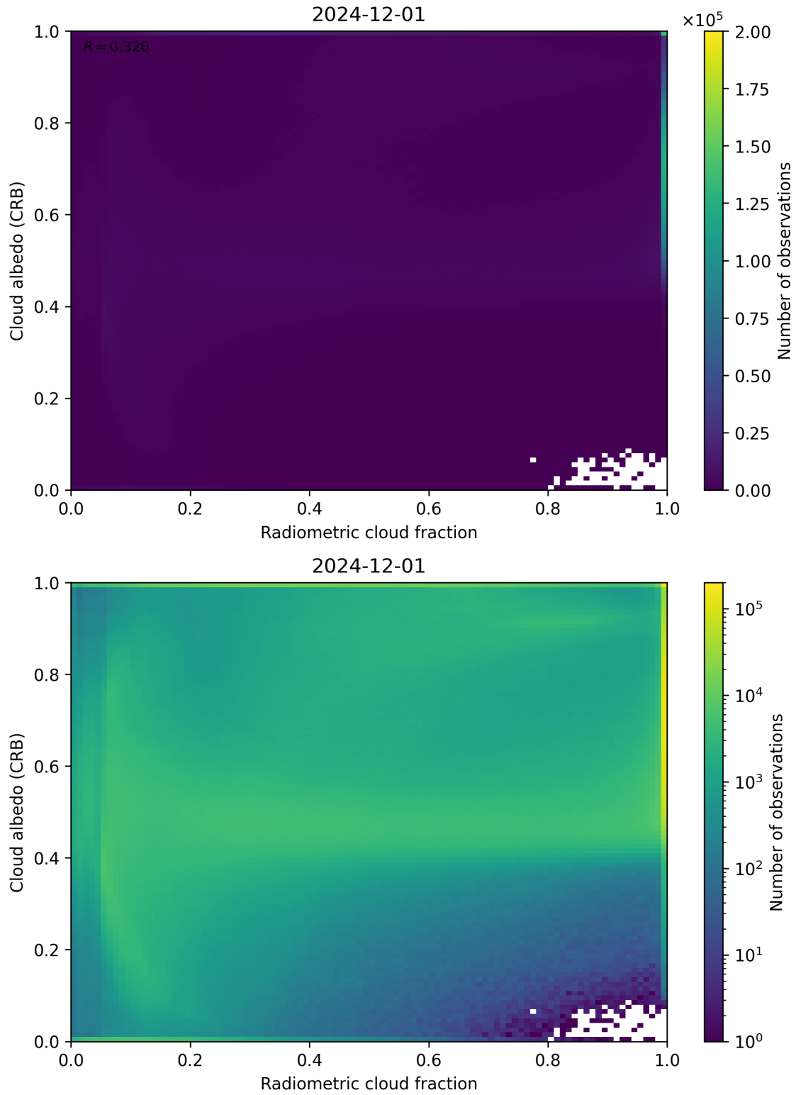
Figure 71: Scatter density plot of “Radiometric cloud fraction” against “Cloud albedo (CRB)” for 2024-11-30 to 2024-12-02.
