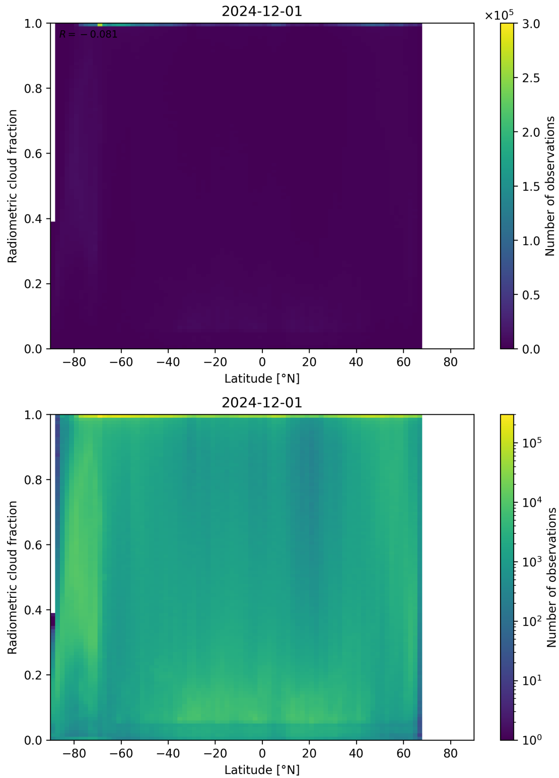
Figure 92: Scatter density plot of “Latitude” against “Radiometric cloud fraction” for 2024-11-30 to 2024-12-02.
