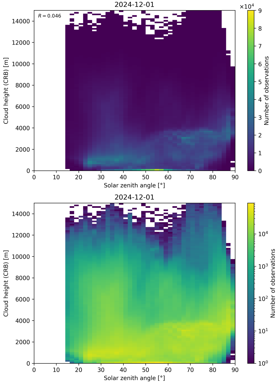
Figure 102: Scatter density plot of “Solar zenith angle” against “Cloud height (CRB)” for 2024-11-30 to 2024-12-02.
