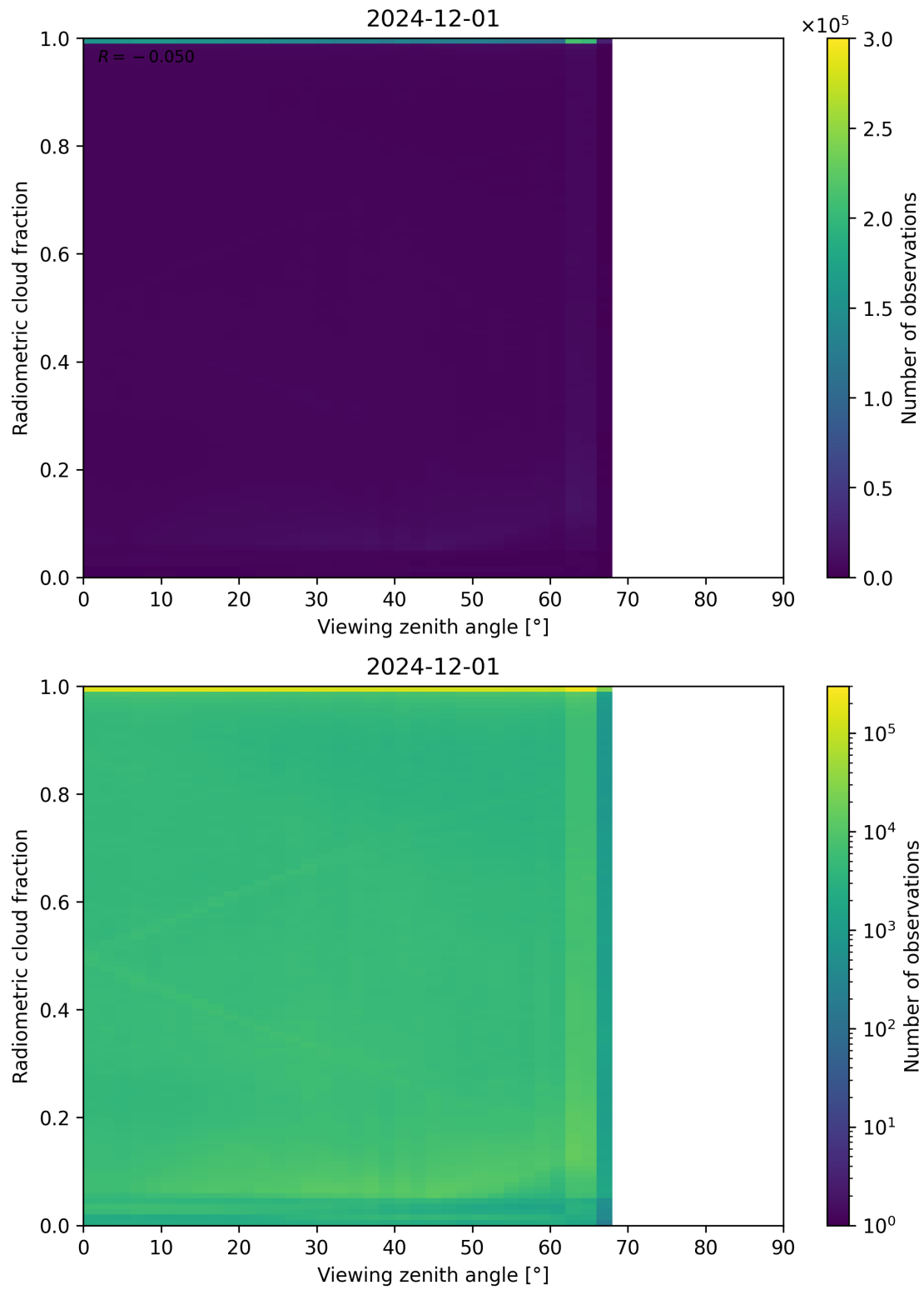
Figure 107: Scatter density plot of “Viewing zenith angle” against “Radiometric cloud fraction” for 2024-11-30 to 2024-12-02.
