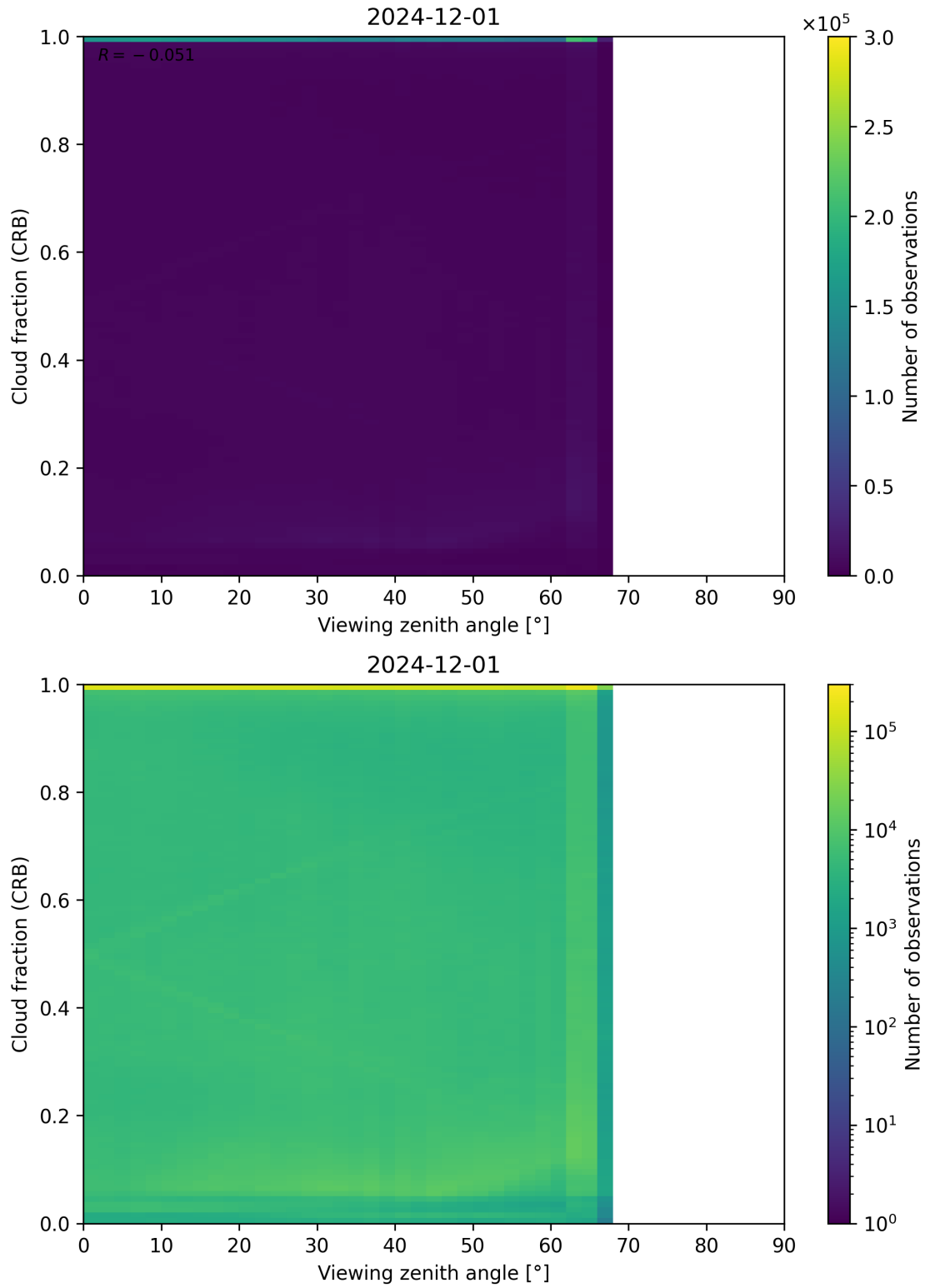
Figure 109: Scatter density plot of “Viewing zenith angle” against “Cloud fraction (CRB)” for 2024-11-30 to 2024-12-02.
