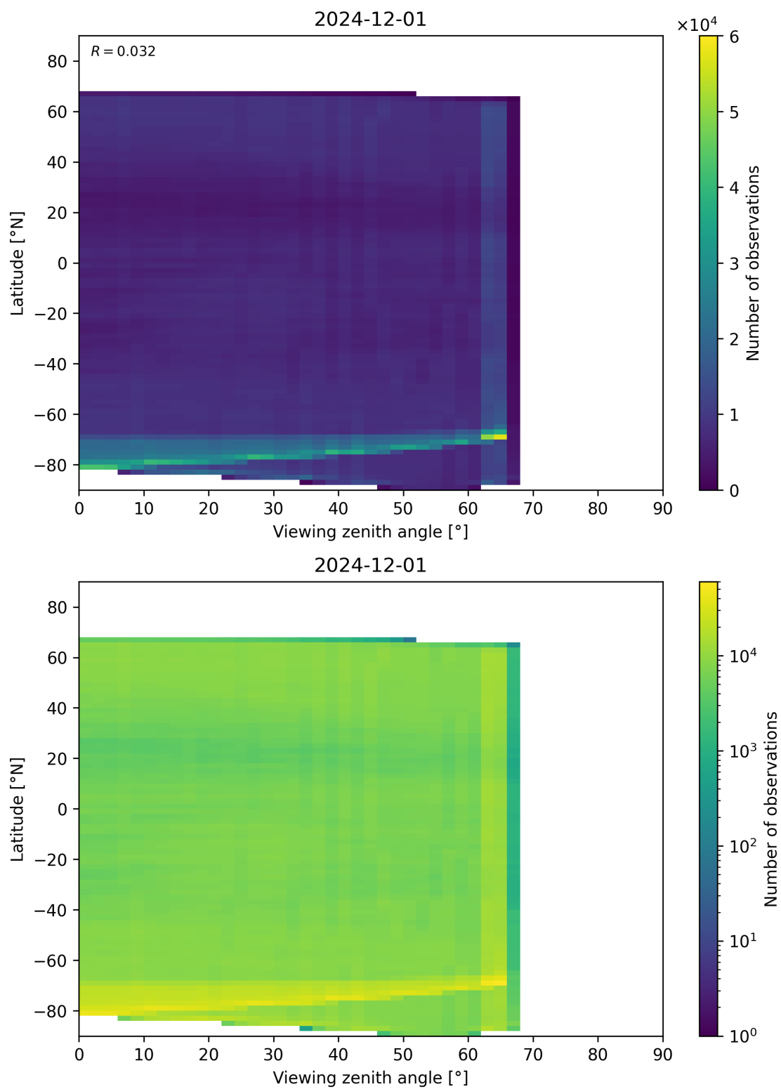
Figure 113: Scatter density plot of “Viewing zenith angle” against “Latitude” for 2024-11-30 to 2024-12-02.
