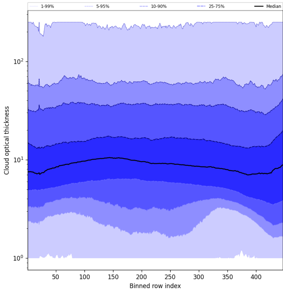
Figure 57: Along track statistics of “Cloud optical thickness” for 2024-11-30 to 2024-12-02
