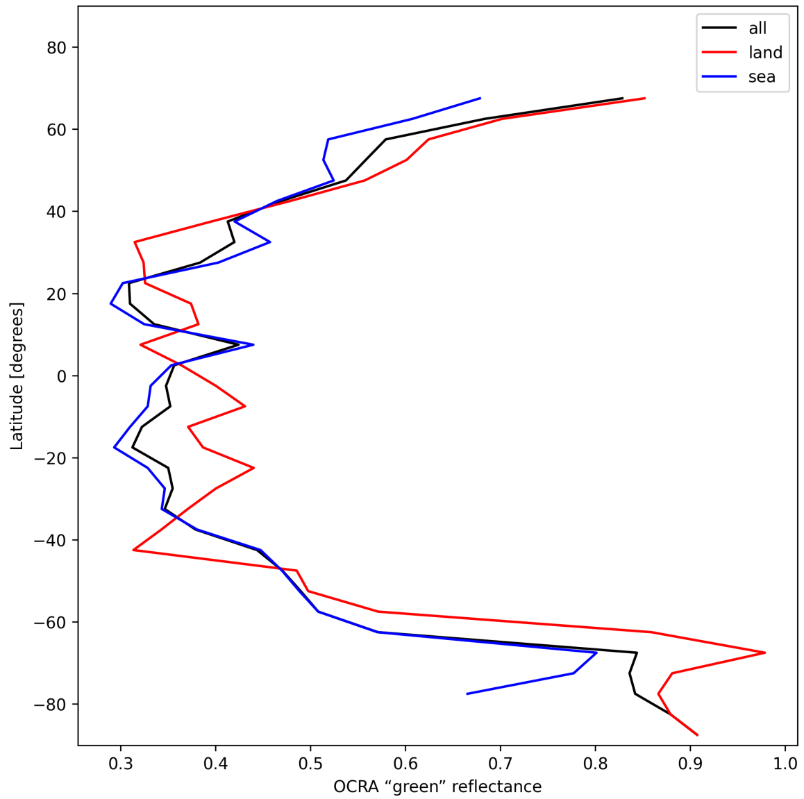
Figure 36: Zonal average of “OCRA “green” reflectance” for 2024-12-01 to 2024-12-03.
