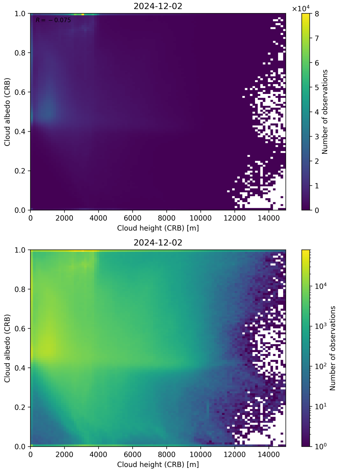
Figure 80: Scatter density plot of “Cloud height (CRB)” against “Cloud albedo (CRB)” for 2024-12-01 to 2024-12-03.
