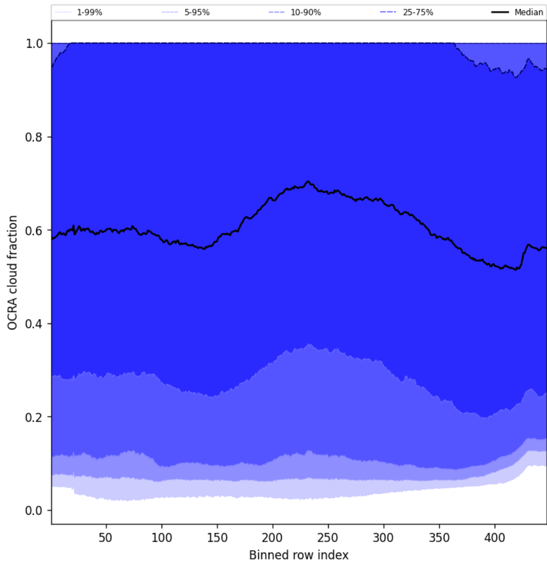
Figure 66: Along track statistics of “OCRA cloud fraction” for 2024-12-01 to 2024-12-03
