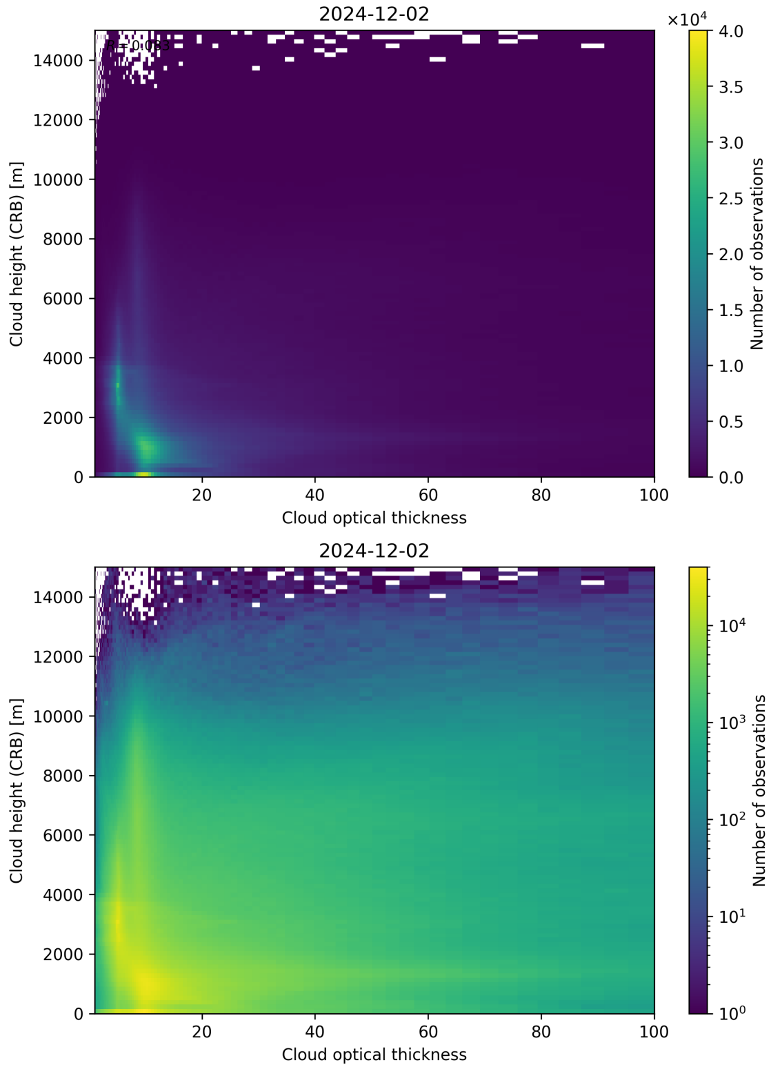
Figure 85: Scatter density plot of “Cloud optical thickness” against “Cloud height (CRB)” for 2024-12-01 to 2024-12-03.
