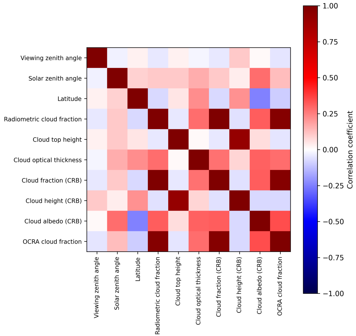
Figure 2: Map of correlation matrix for 2024-12-01 to 2024-12-03.
