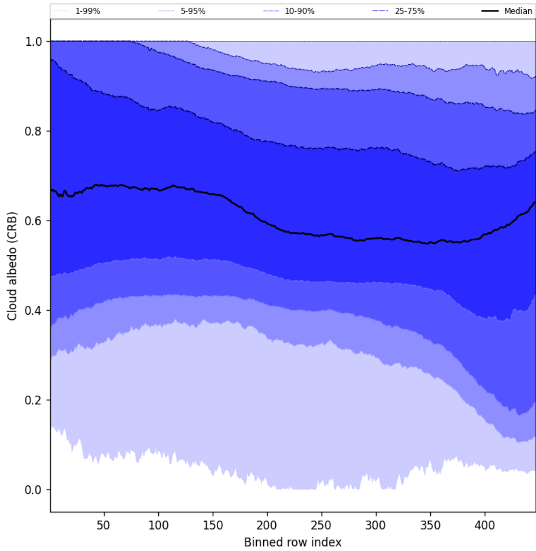
Figure 60: Along track statistics of “Cloud albedo (CRB)” for 2024-12-01 to 2024-12-03
