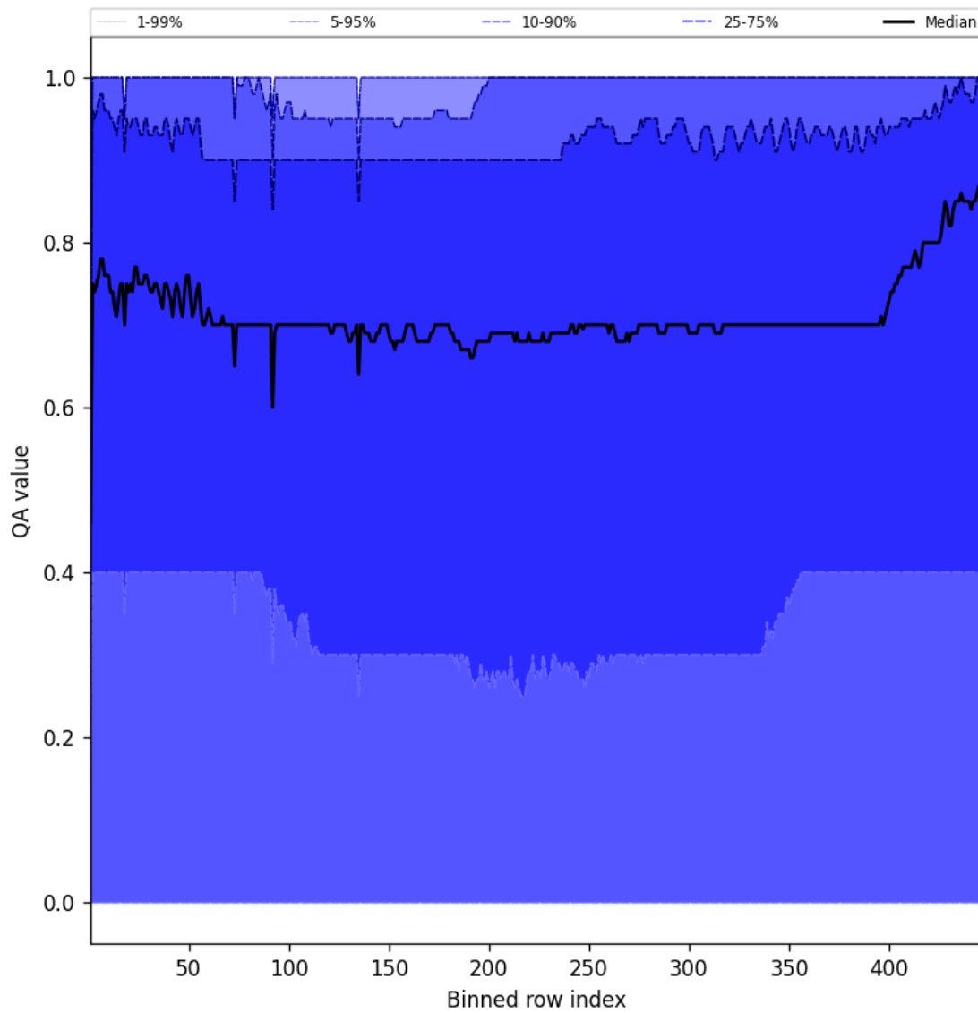
Figure 54: Along track statistics of “QA value” for 2024-12-01 to 2024-12-03
