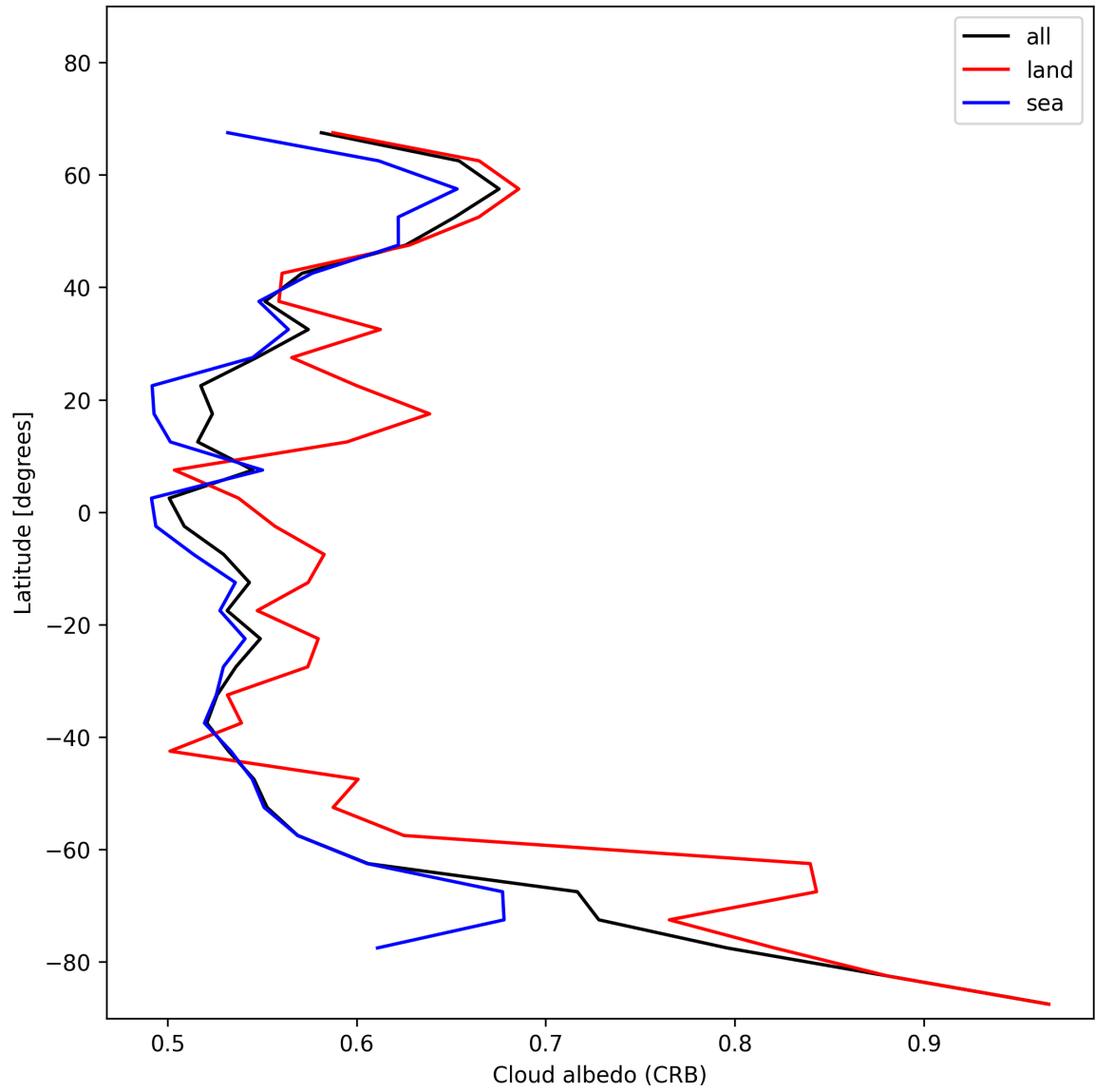
Figure 28: Zonal average of “Cloud albedo (CRB)” for 2024-12-01 to 2024-12-03.
