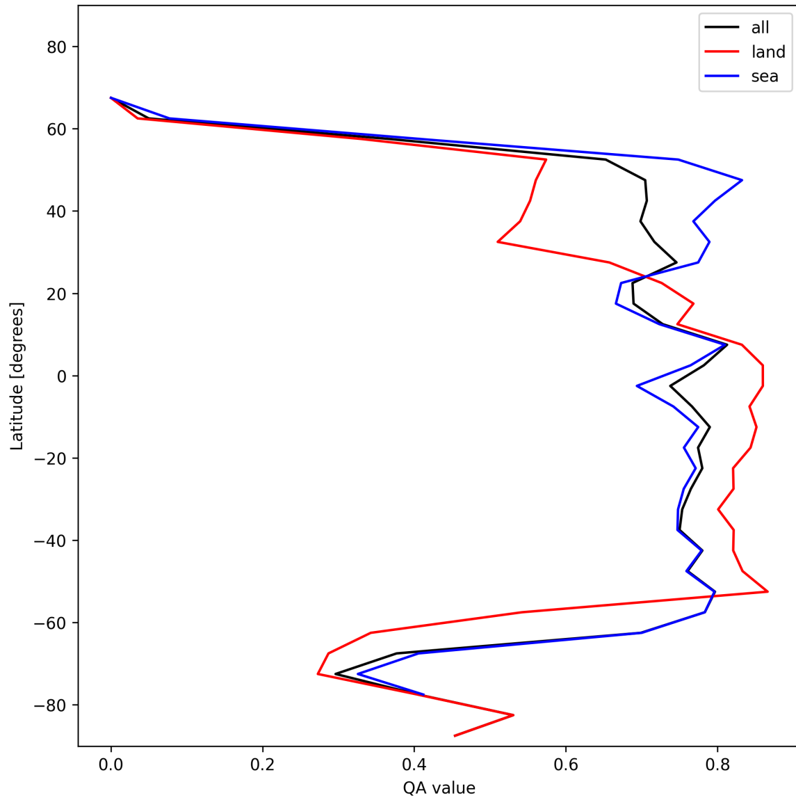
Figure 22: Zonal average of “QA value” for 2024-12-01 to 2024-12-03.
