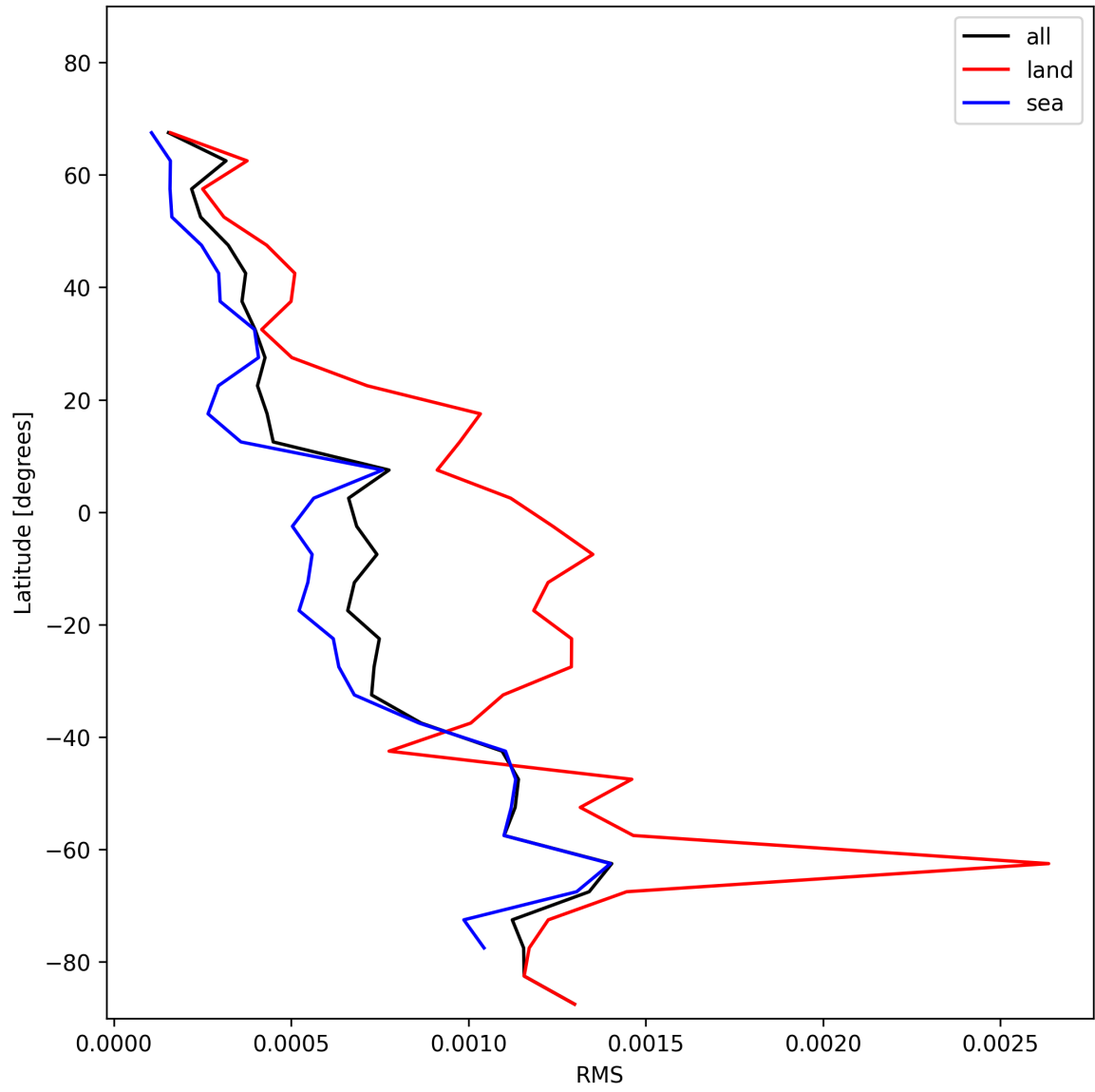
Figure 31: Zonal average of “RMS” for 2024-12-01 to 2024-12-03.
