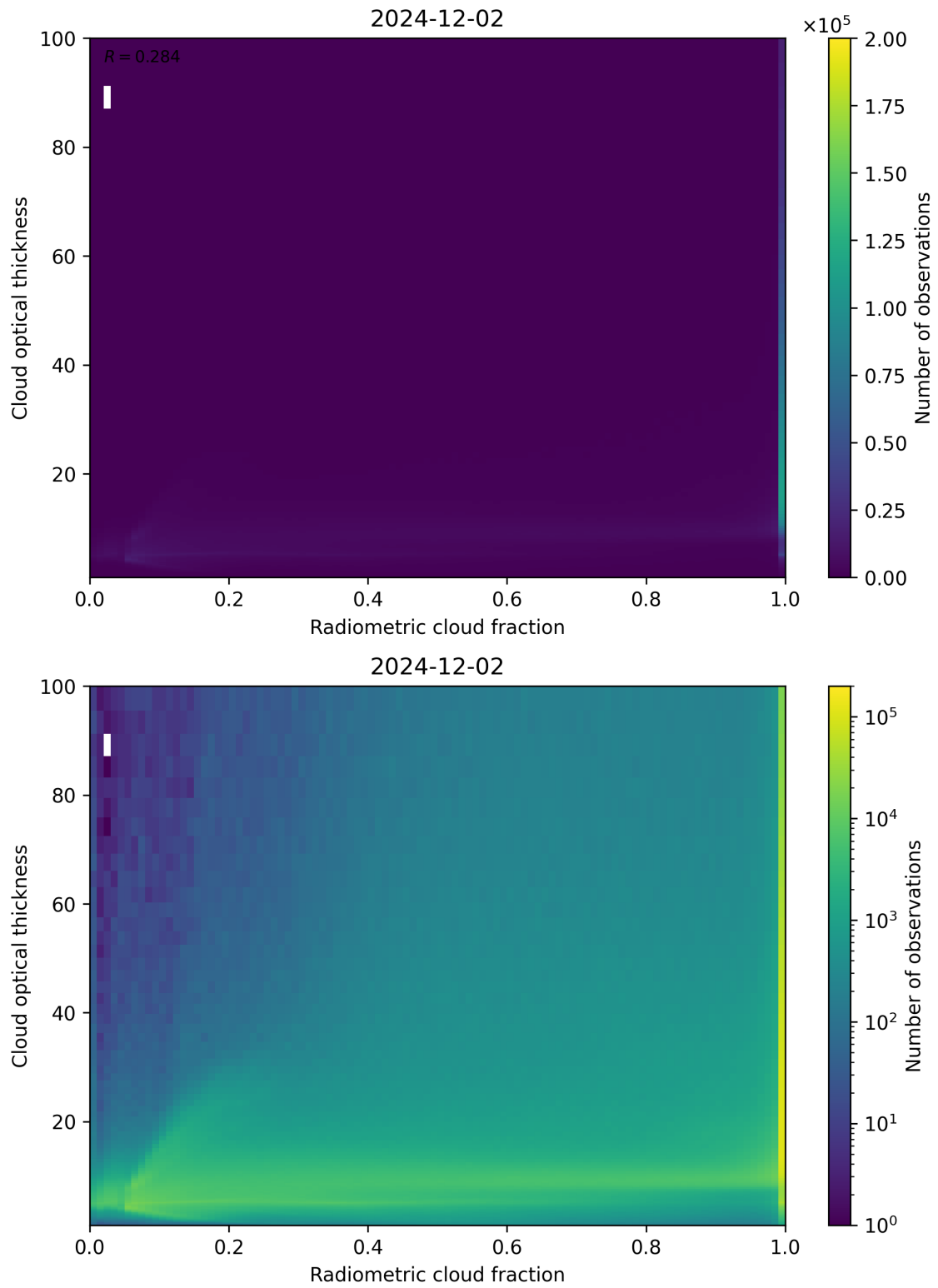
Figure 75: Scatter density plot of “Radiometric cloud fraction” against “Cloud optical thickness” for 2024-12-01 to 2024-12-03.
