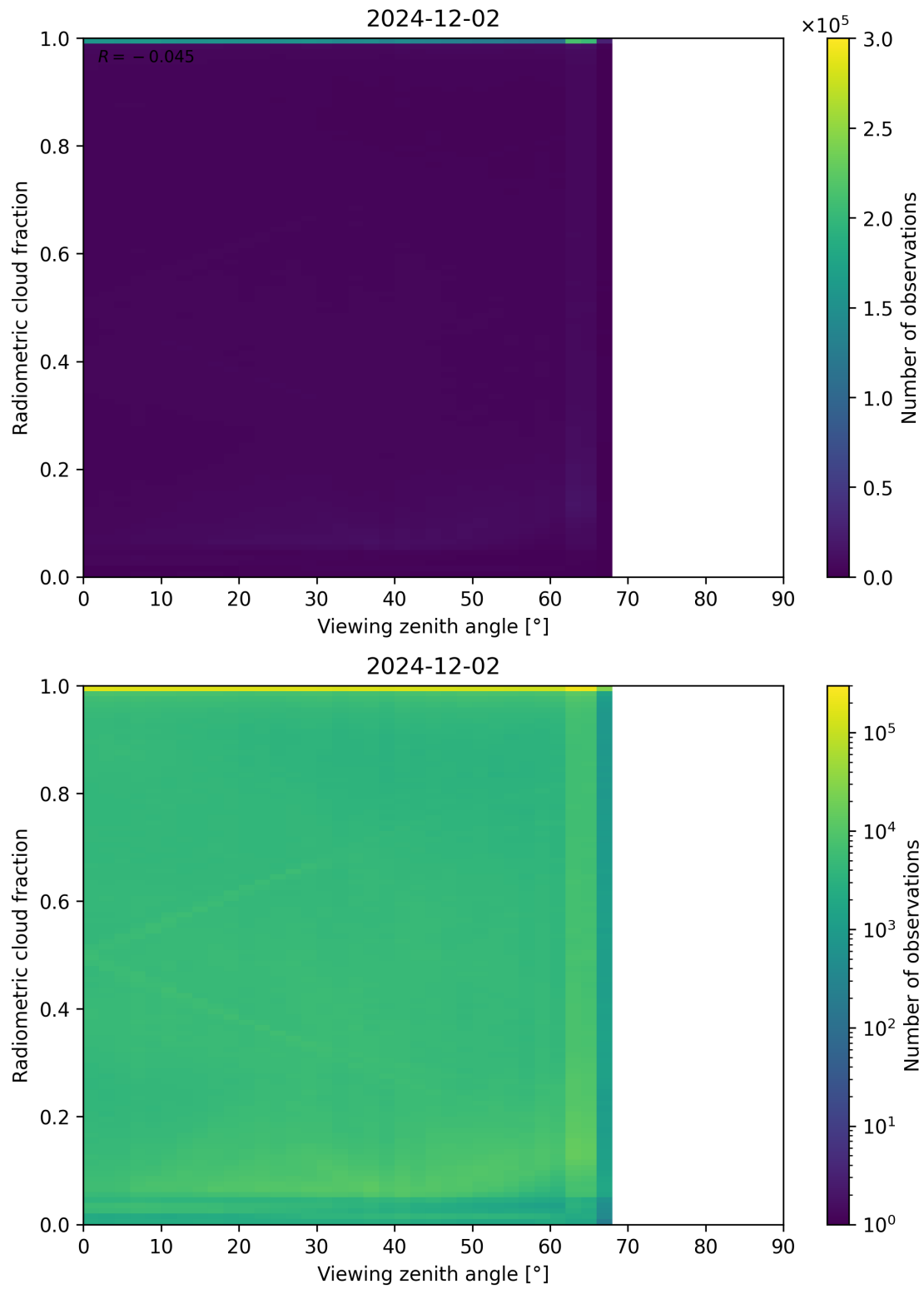
Figure 107: Scatter density plot of “Viewing zenith angle” against “Radiometric cloud fraction” for 2024-12-01 to 2024-12-03.
