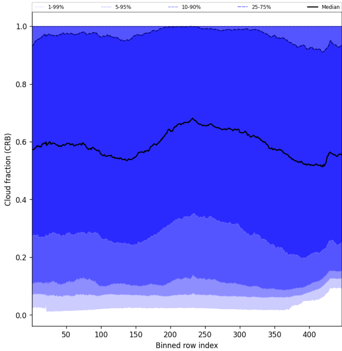
Figure 58: Along track statistics of “Cloud fraction (CRB)” for 2024-12-01 to 2024-12-03
