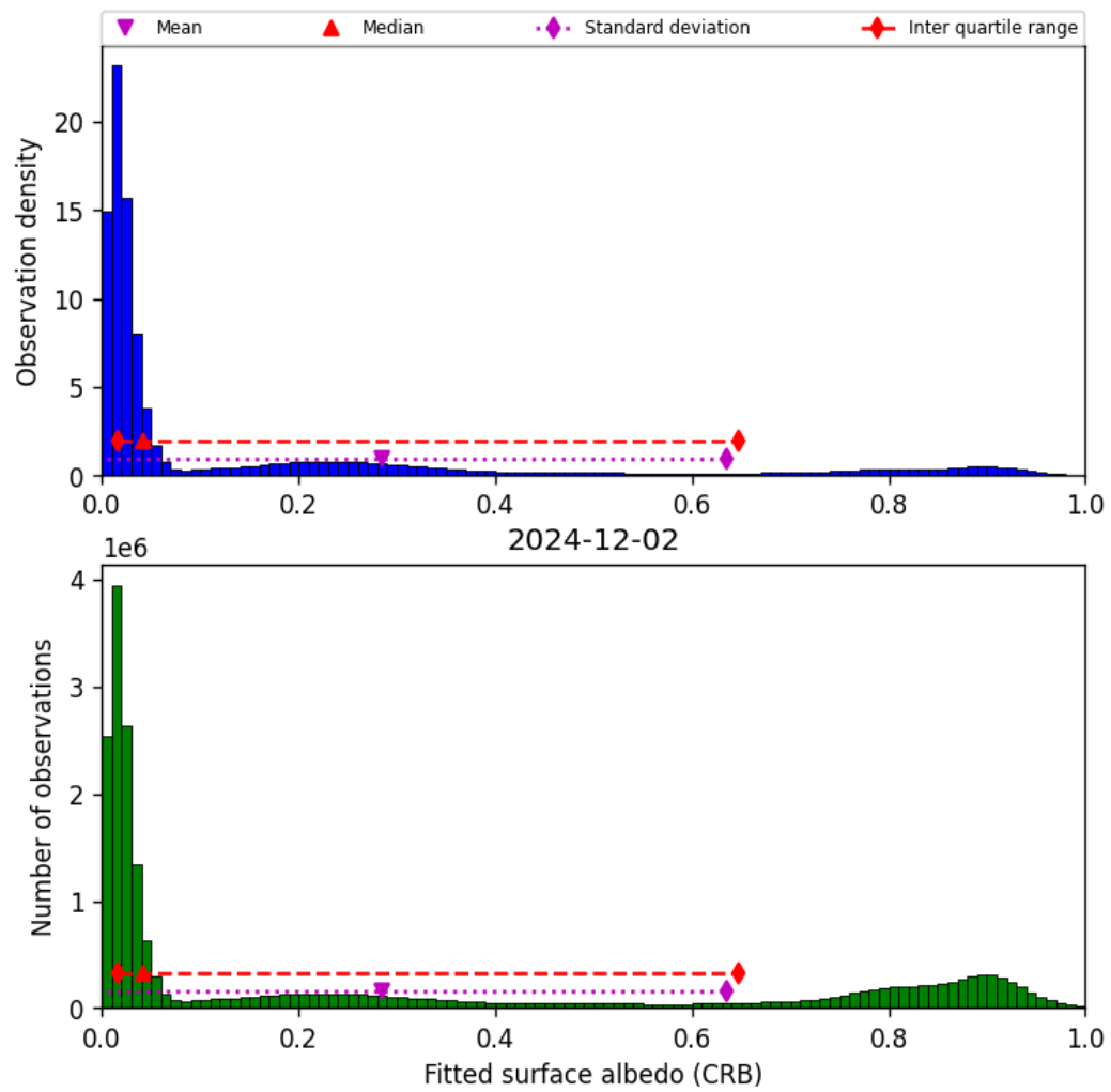
Figure 46: Histogram of “Fitted surface albedo (CRB)” for 2024-12-01 to 2024-12-03
