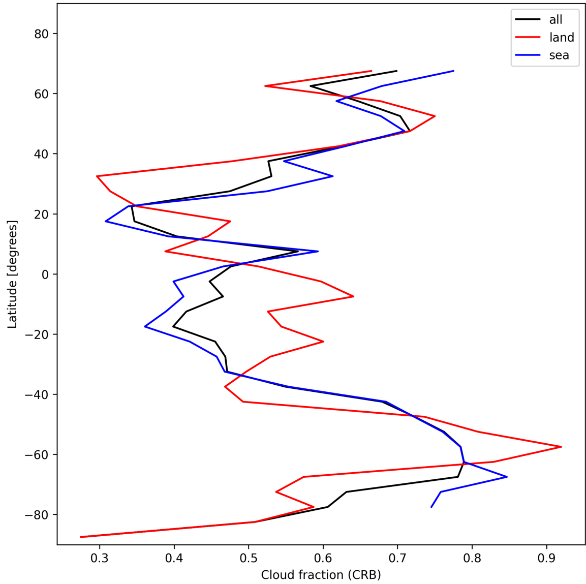
Figure 26: Zonal average of “Cloud fraction (CRB)” for 2024-12-01 to 2024-12-03.
