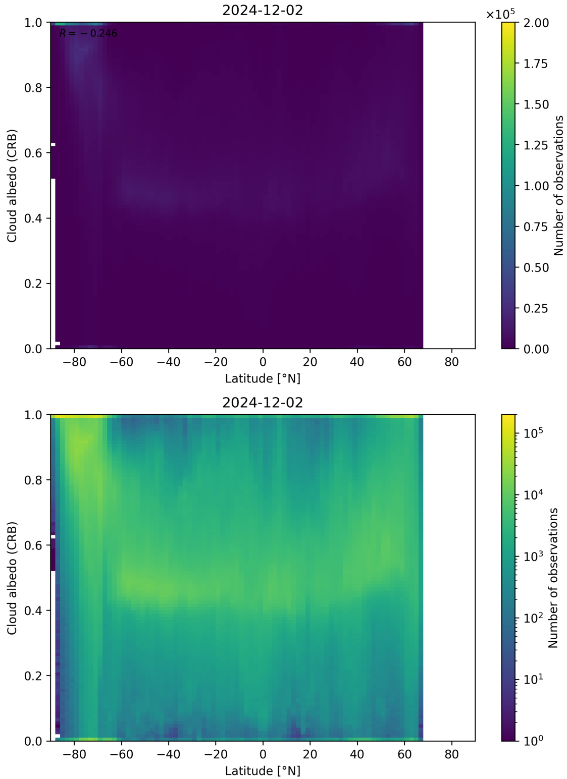
Figure 91: Scatter density plot of “Latitude” against “Cloud albedo (CRB)” for 2024-12-01 to 2024-12-03.
