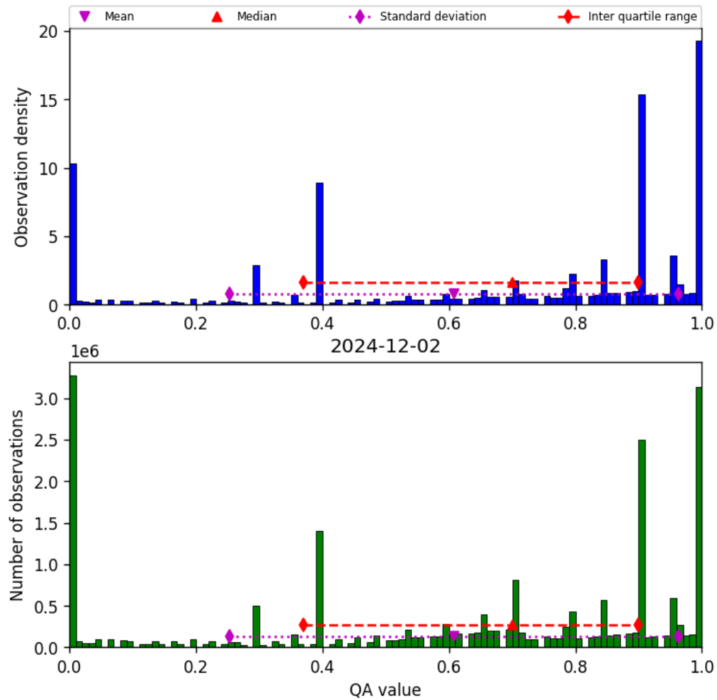
Figure 38: Histogram of “QA value” for 2024-12-01 to 2024-12-03
