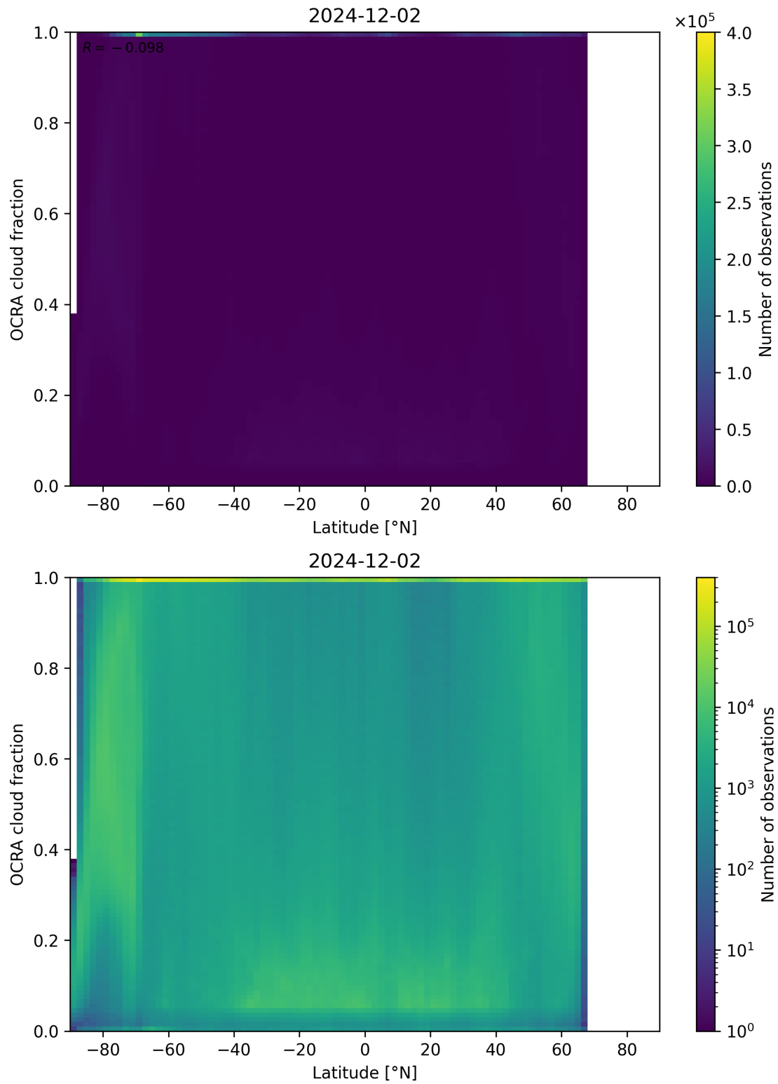
Figure 93: Scatter density plot of “Latitude” against “OCRA cloud fraction” for 2024-12-01 to 2024-12-03.
