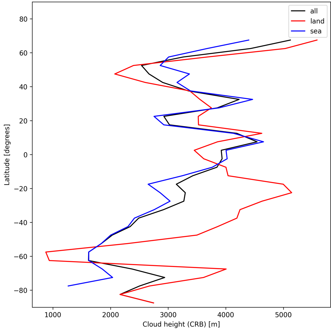
Figure 27: Zonal average of “Cloud height (CRB)” for 2024-12-01 to 2024-12-03.
