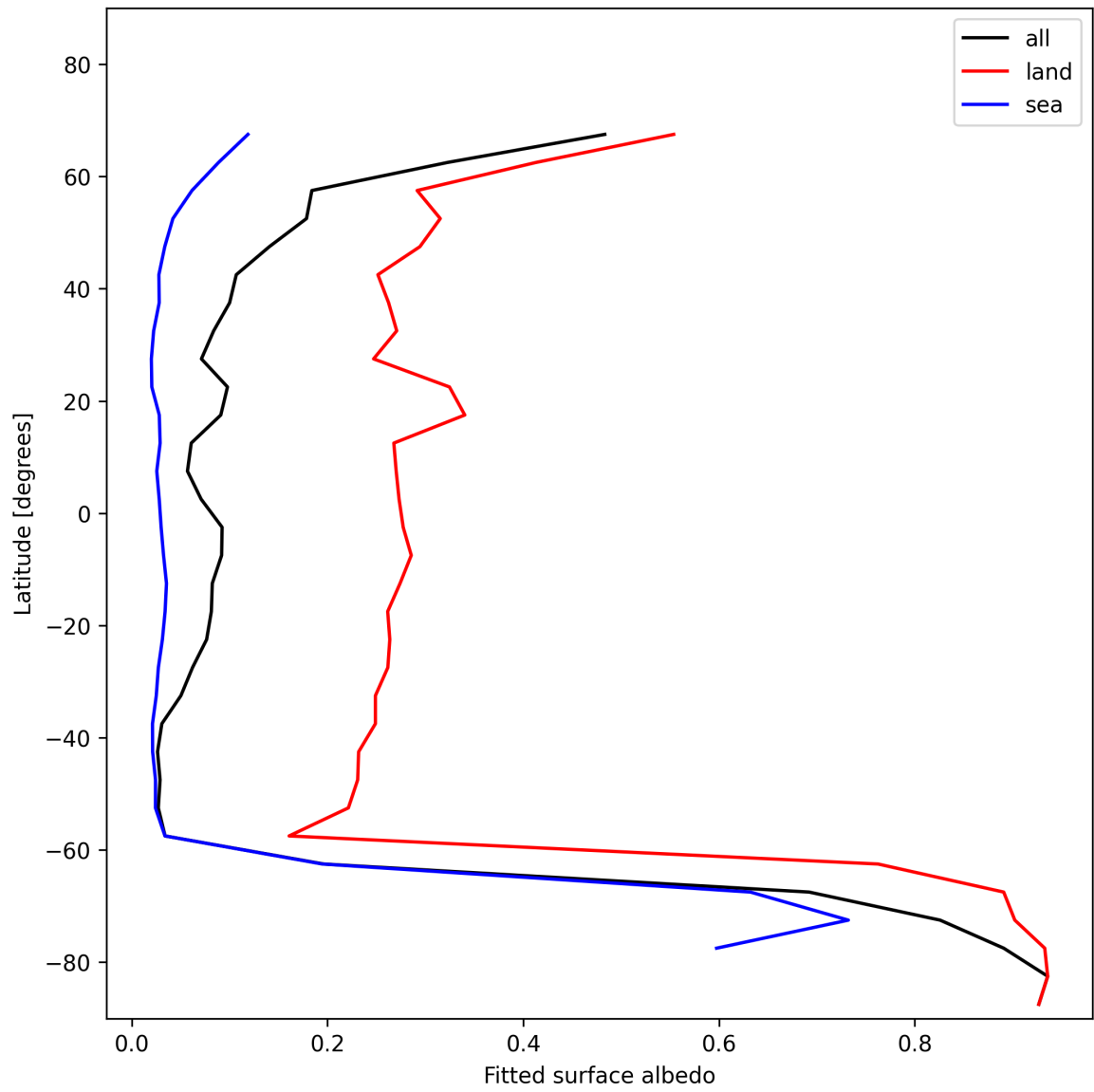
Figure 29: Zonal average of “Fitted surface albedo” for 2024-12-01 to 2024-12-03.
