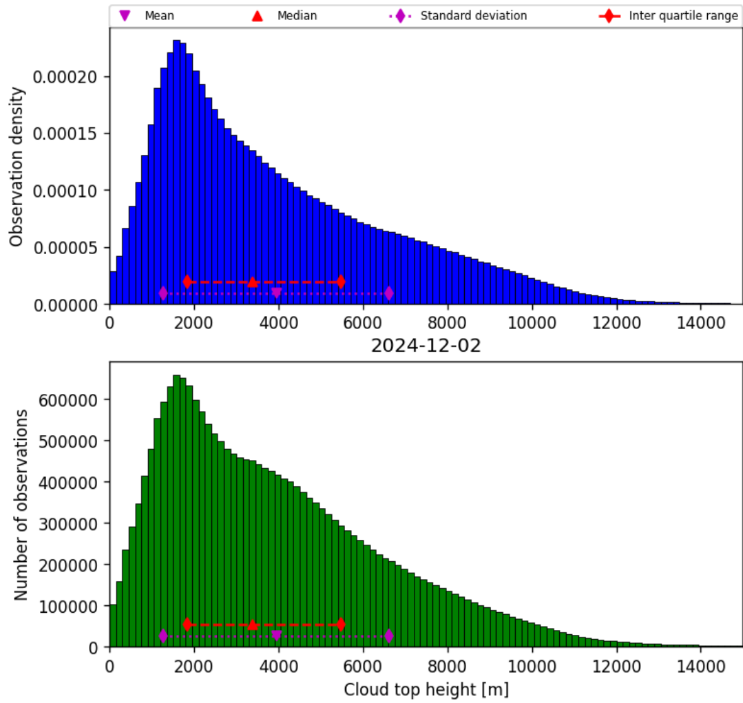
Figure 40: Histogram of “Cloud top height” for 2024-12-01 to 2024-12-03
