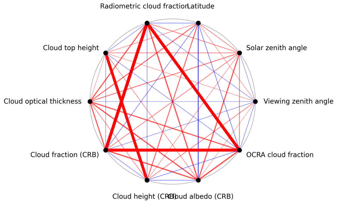
Figure 1: Map of correlation graph for 2024-12-01 to 2024-12-03.
