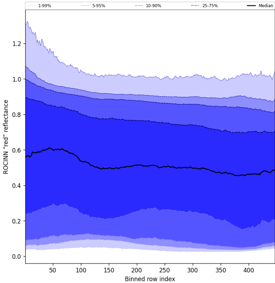
Figure 69: Along track statistics of “ROCINN “red” reflectance” for 2024-12-01 to 2024-12-03
