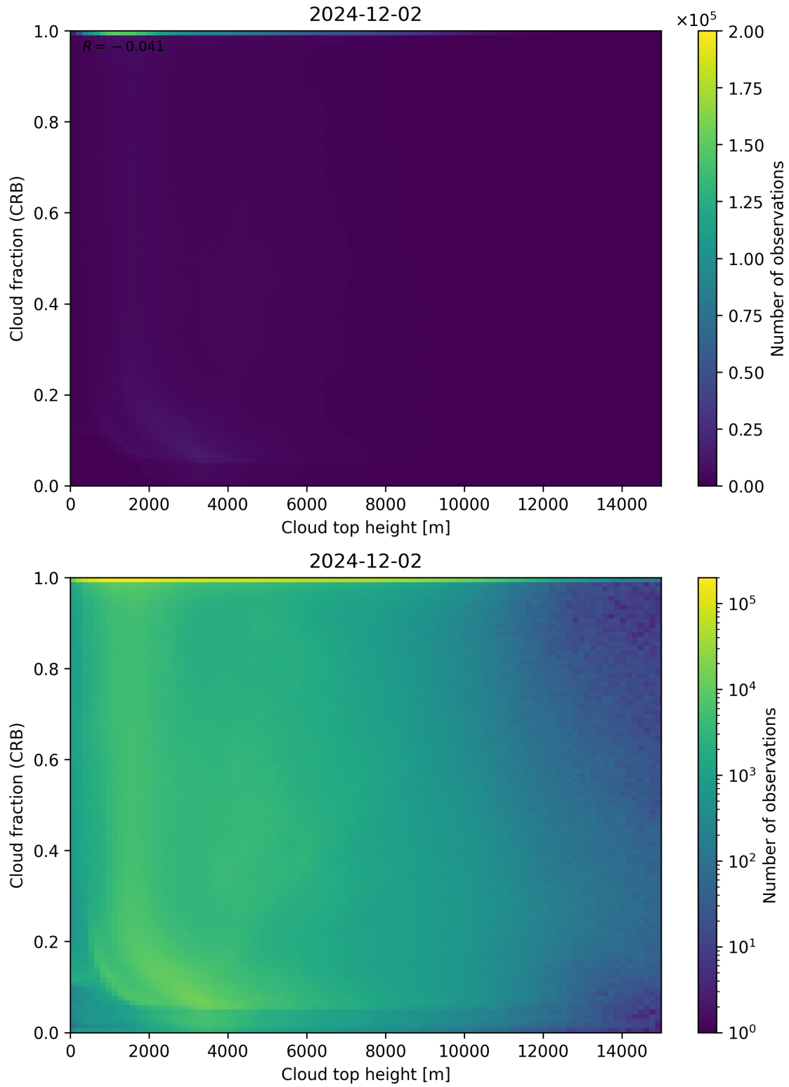
Figure 88: Scatter density plot of “Cloud top height” against “Cloud fraction (CRB)” for 2024-12-01 to 2024-12-03.
