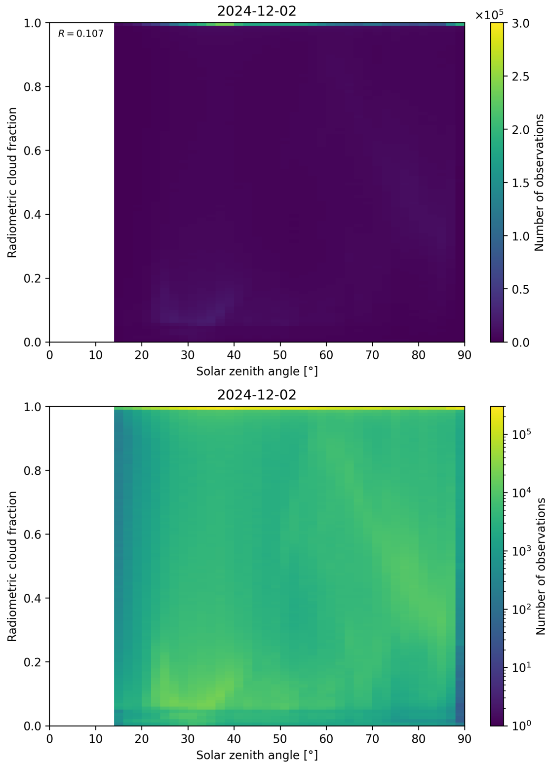
Figure 99: Scatter density plot of “Solar zenith angle” against “Radiometric cloud fraction” for 2024-12-01 to 2024-12-03.
