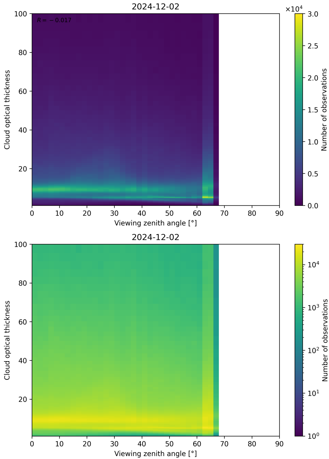
Figure 111: Scatter density plot of “Viewing zenith angle” against “Cloud optical thickness” for 2024-12-01 to 2024-12-03.
