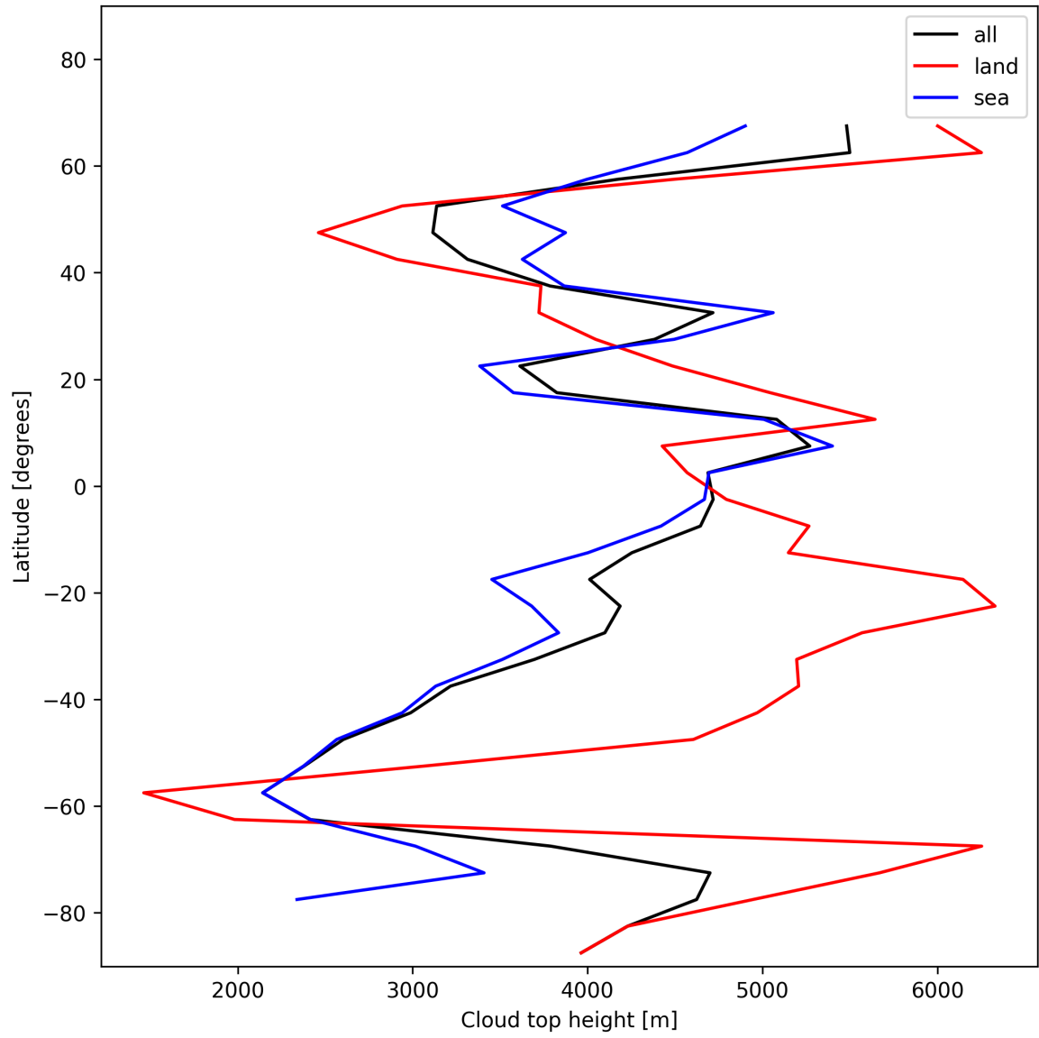
Figure 24: Zonal average of “Cloud top height” for 2024-12-01 to 2024-12-03.
