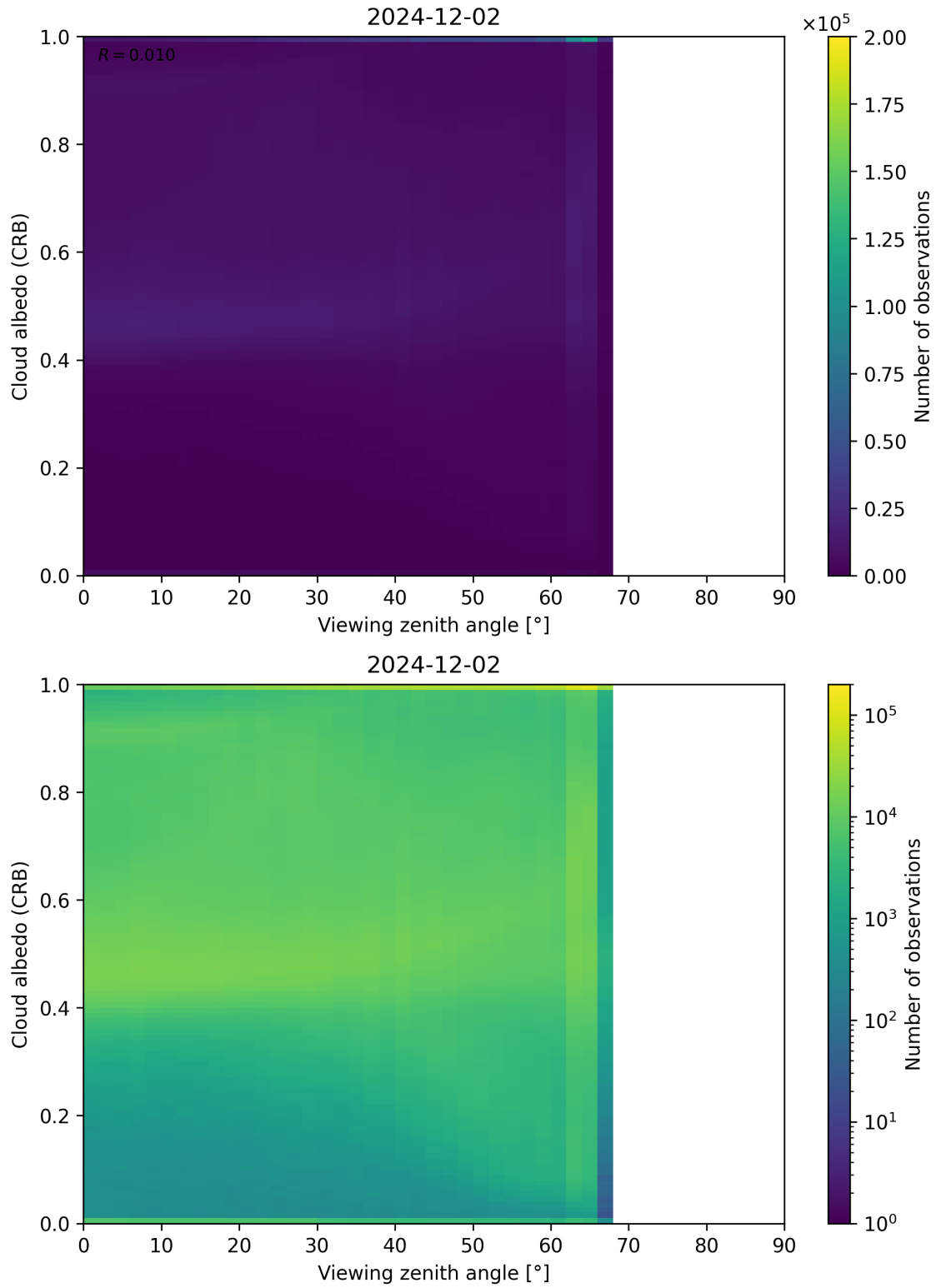
Figure 106: Scatter density plot of “Viewing zenith angle” against “Cloud albedo (CRB)” for 2024-12-01 to 2024-12-03.
