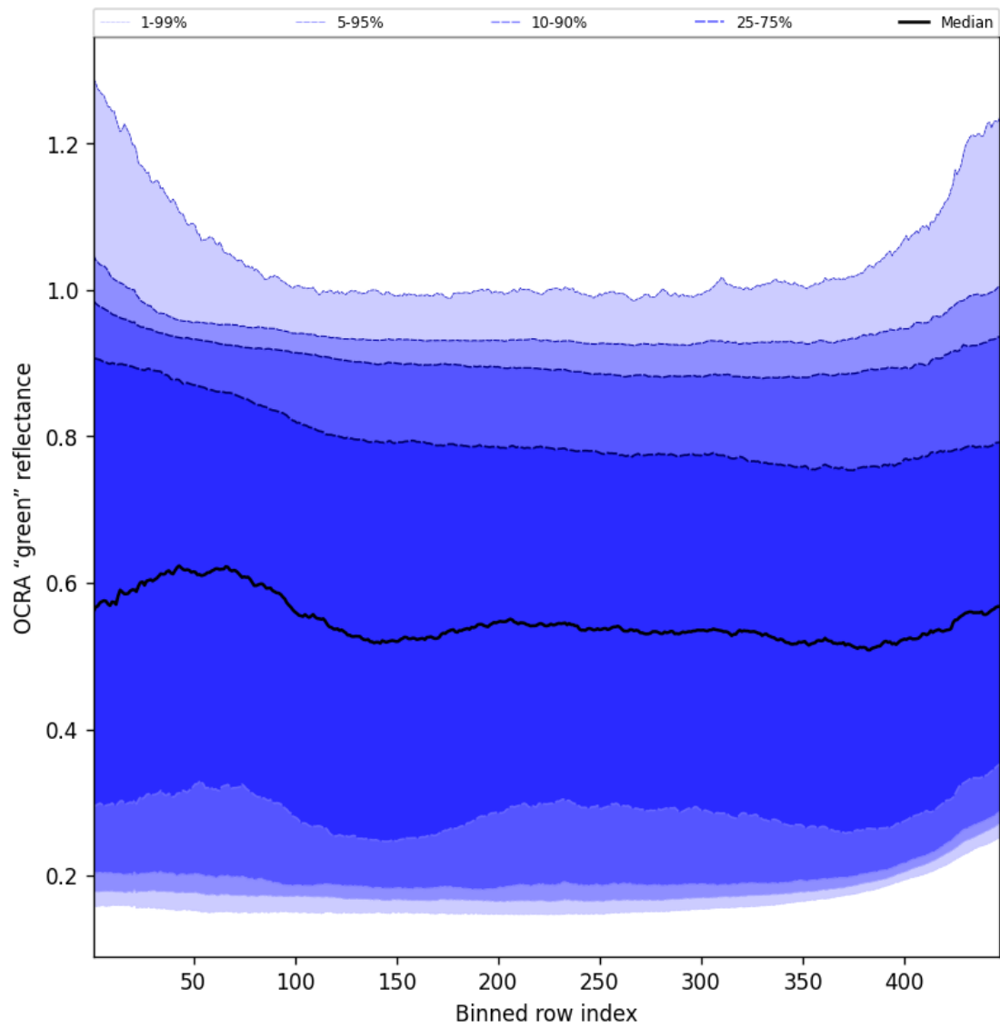
Figure 68: Along track statistics of "OCRA "green" reflectance" for 2024-12-01 to 2024-12-03
