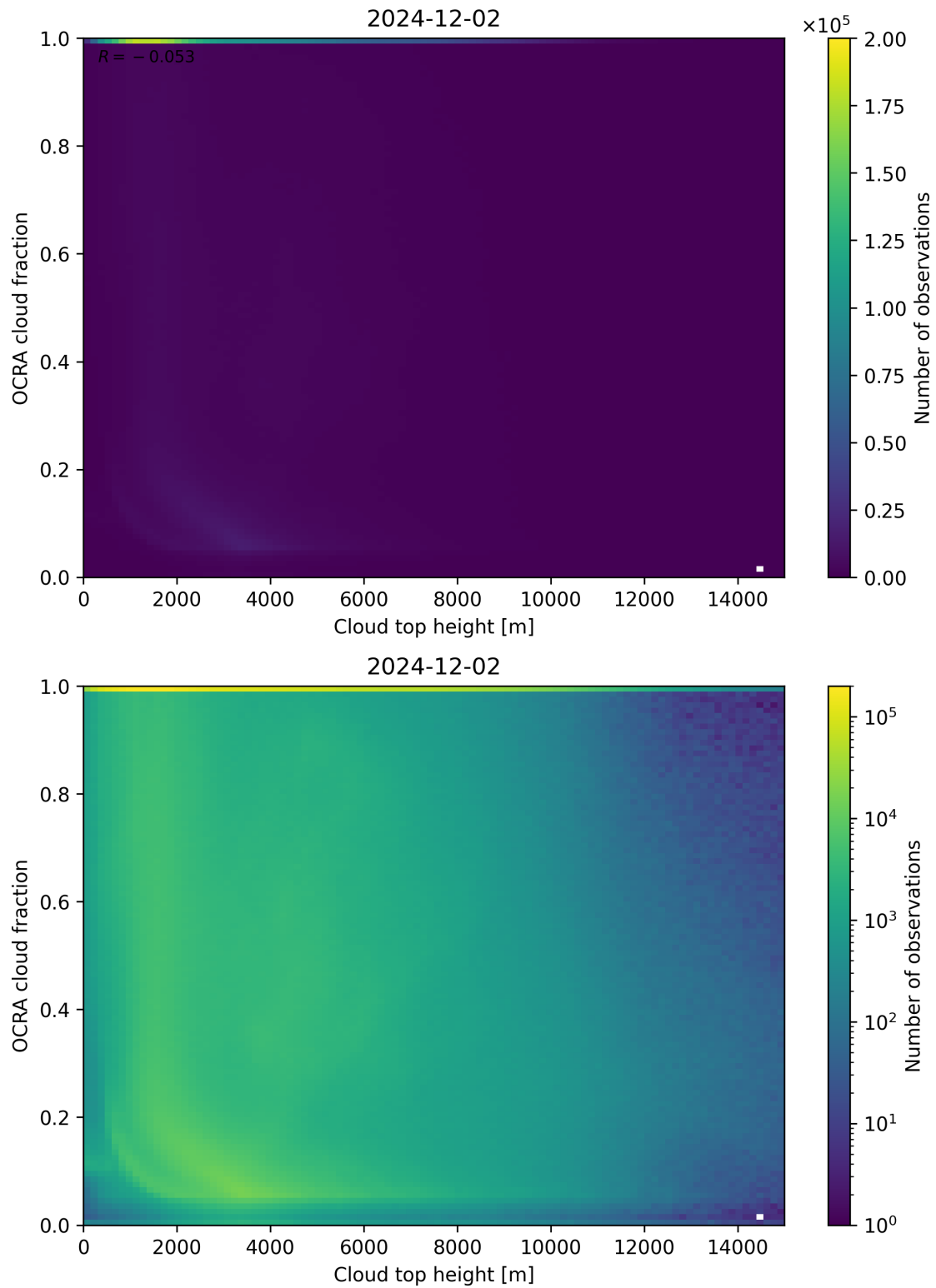
Figure 87: Scatter density plot of “Cloud top height” against “OCRA cloud fraction” for 2024-12-01 to 2024-12-03.
