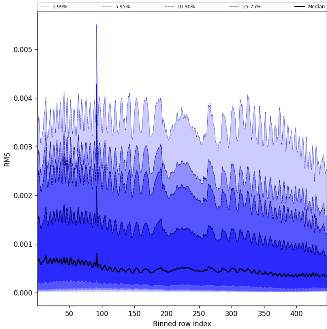
Figure 63: Along track statistics of “RMS” for 2024-12-01 to 2024-12-03
