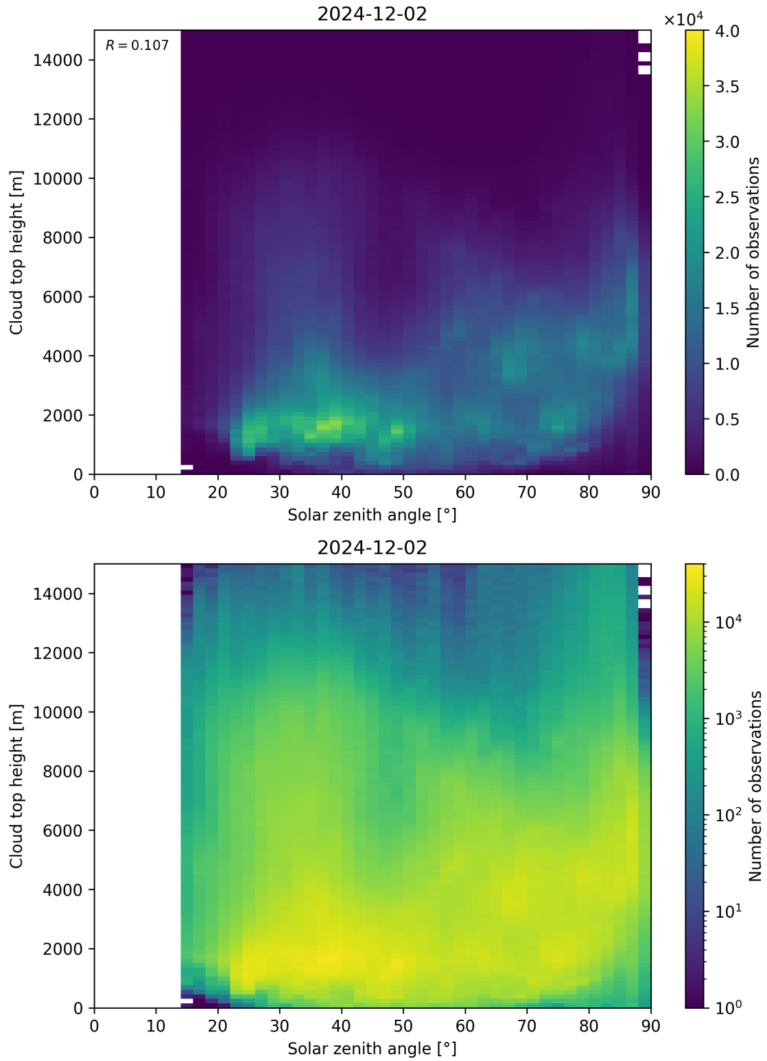
Figure 104: Scatter density plot of “Solar zenith angle” against “Cloud top height” for 2024-12-01 to 2024-12-03.
