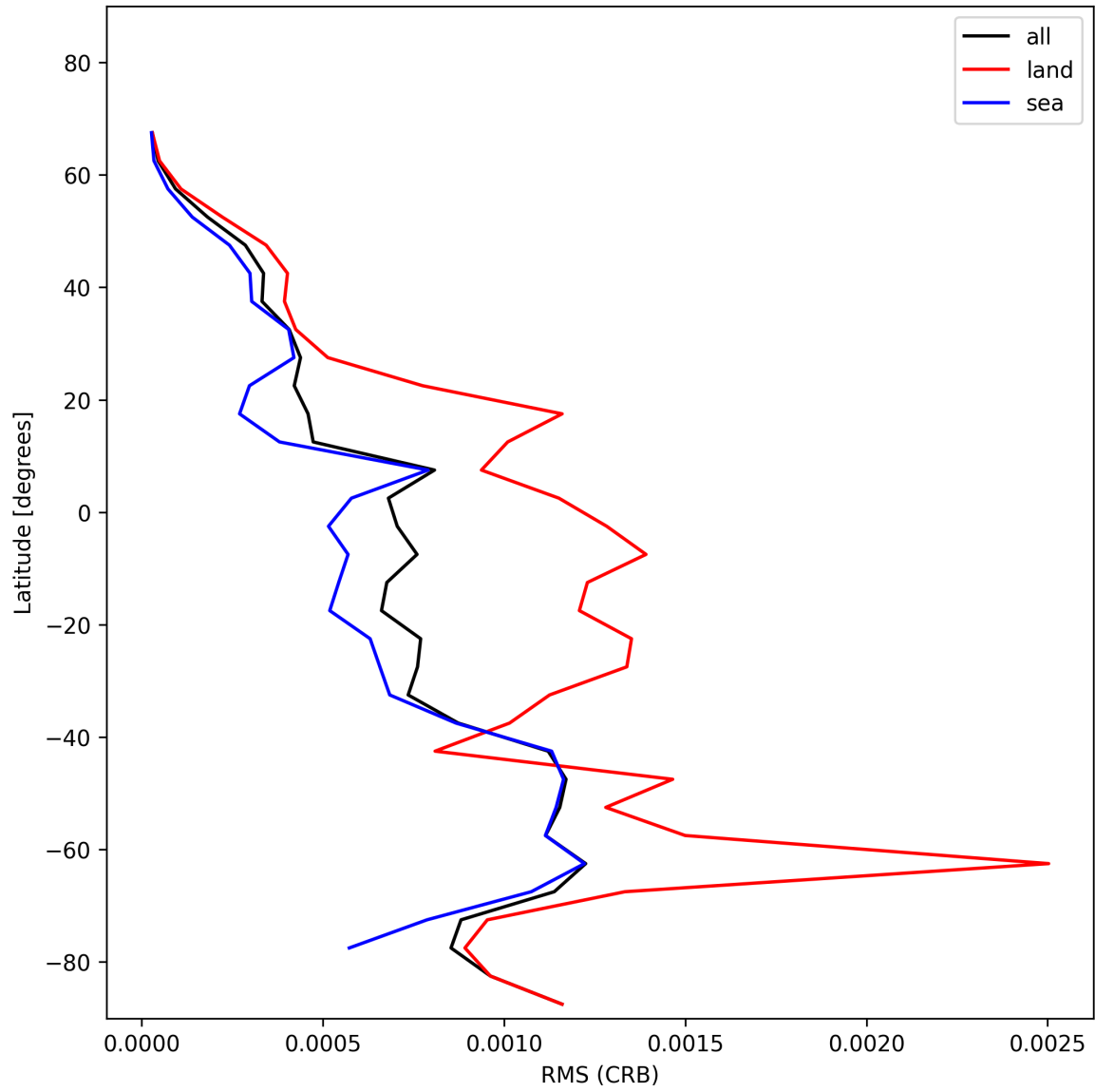
Figure 32: Zonal average of “RMS (CRB)” for 2024-12-01 to 2024-12-03.
