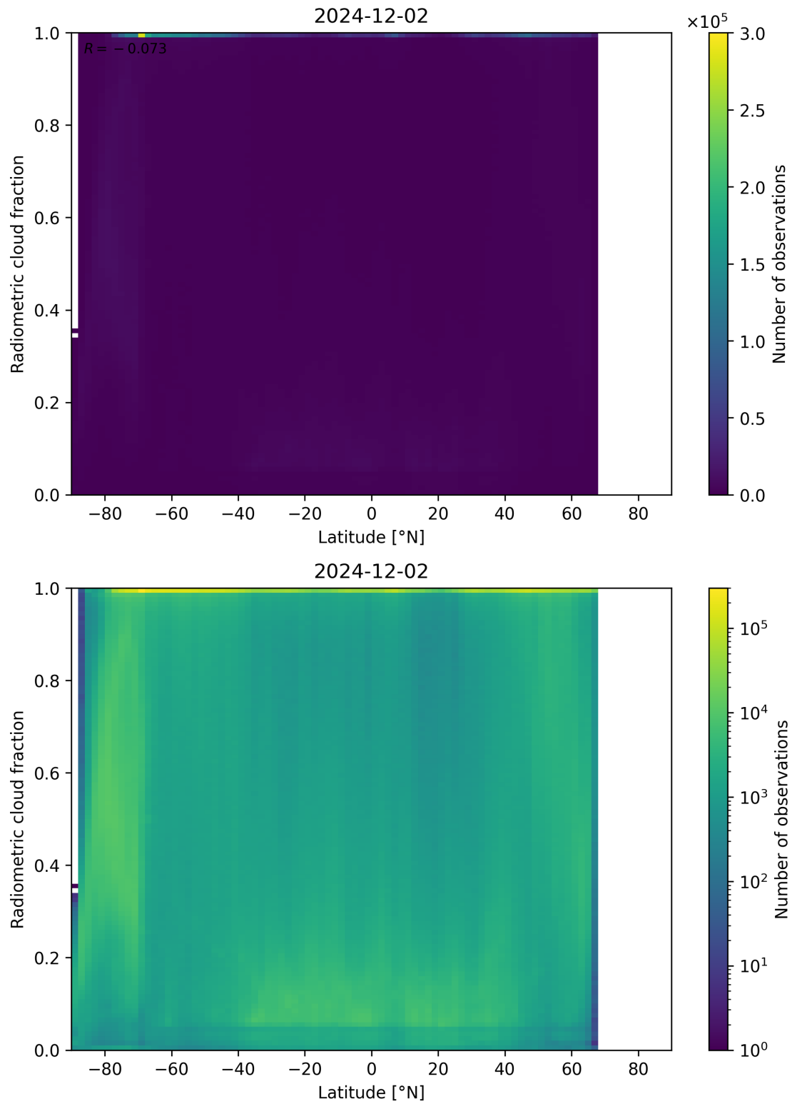
Figure 92: Scatter density plot of “Latitude” against “Radiometric cloud fraction” for 2024-12-01 to 2024-12-03.
