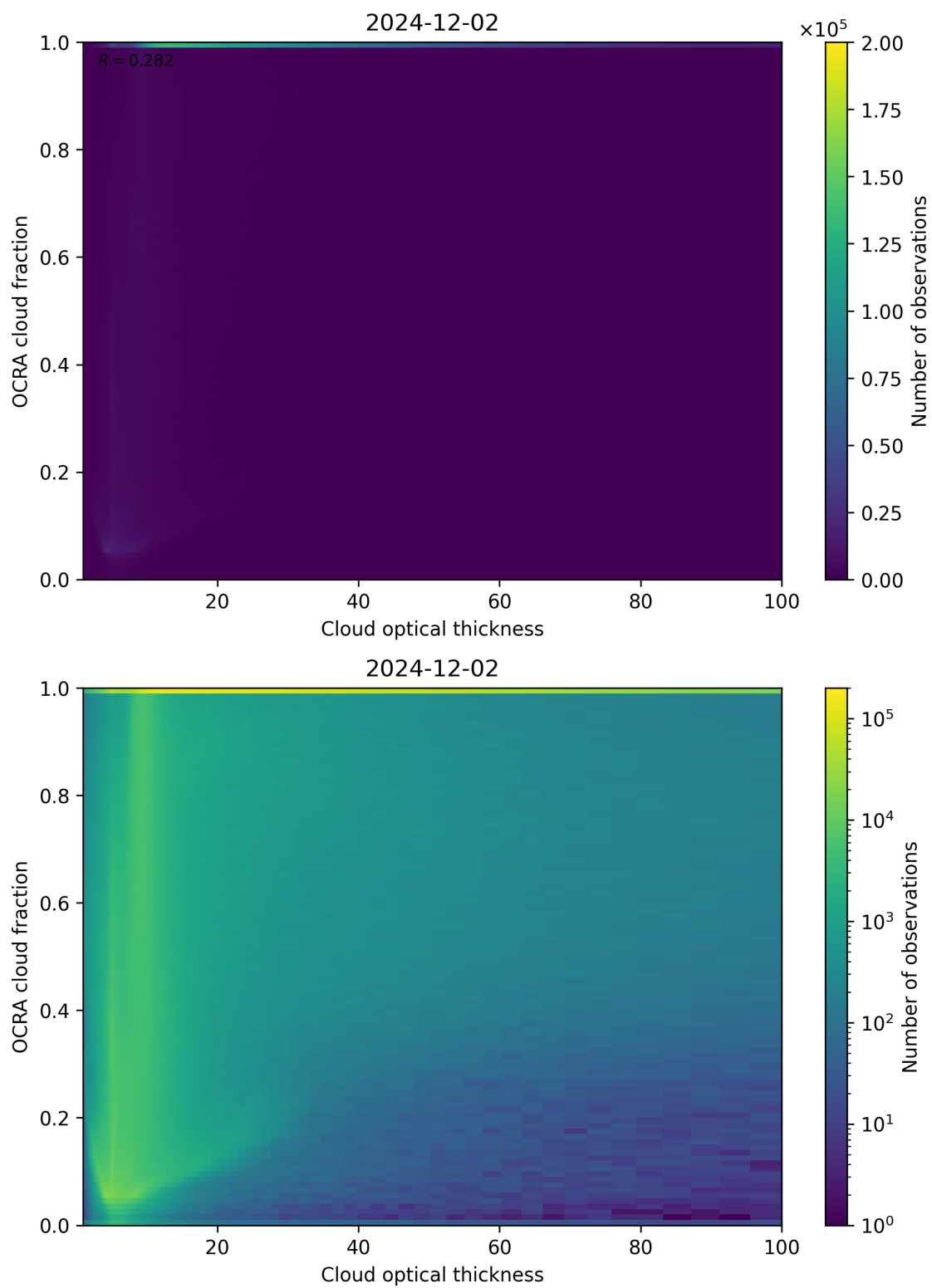
Figure 83: Scatter density plot of “Cloud optical thickness” against “OCRA cloud fraction” for 2024-12-01 to 2024-12-03.
