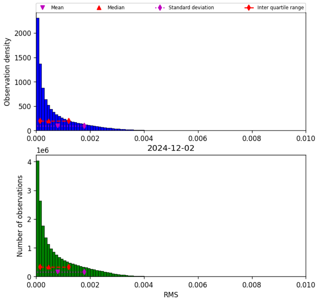
Figure 47: Histogram of “RMS” for 2024-12-01 to 2024-12-03
