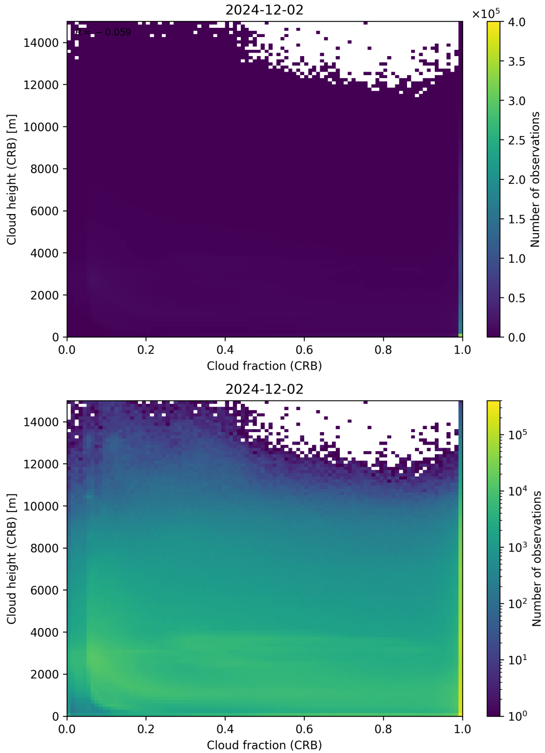
Figure 79: Scatter density plot of “Cloud fraction (CRB)” against “Cloud height (CRB)” for 2024-12-01 to 2024-12-03.
