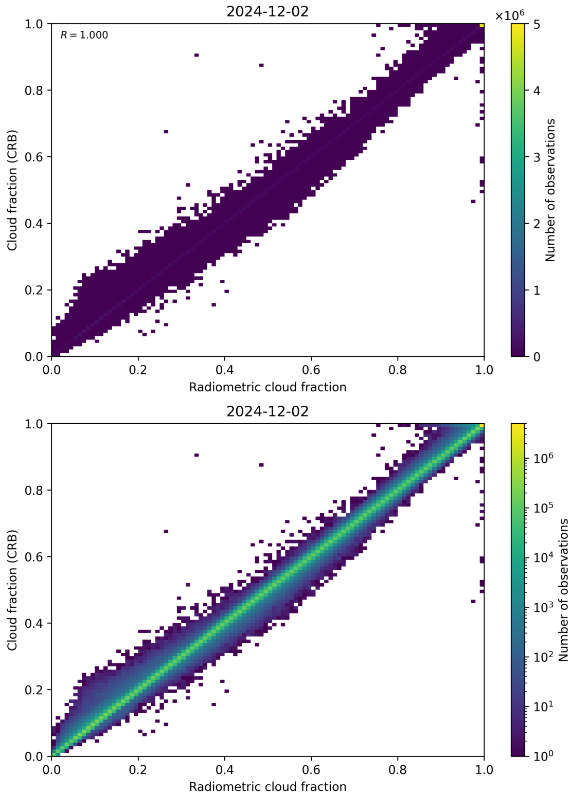
Figure 73: Scatter density plot of “Radiometric cloud fraction” against “Cloud fraction (CRB)” for 2024-12-01 to 2024-12-03.
