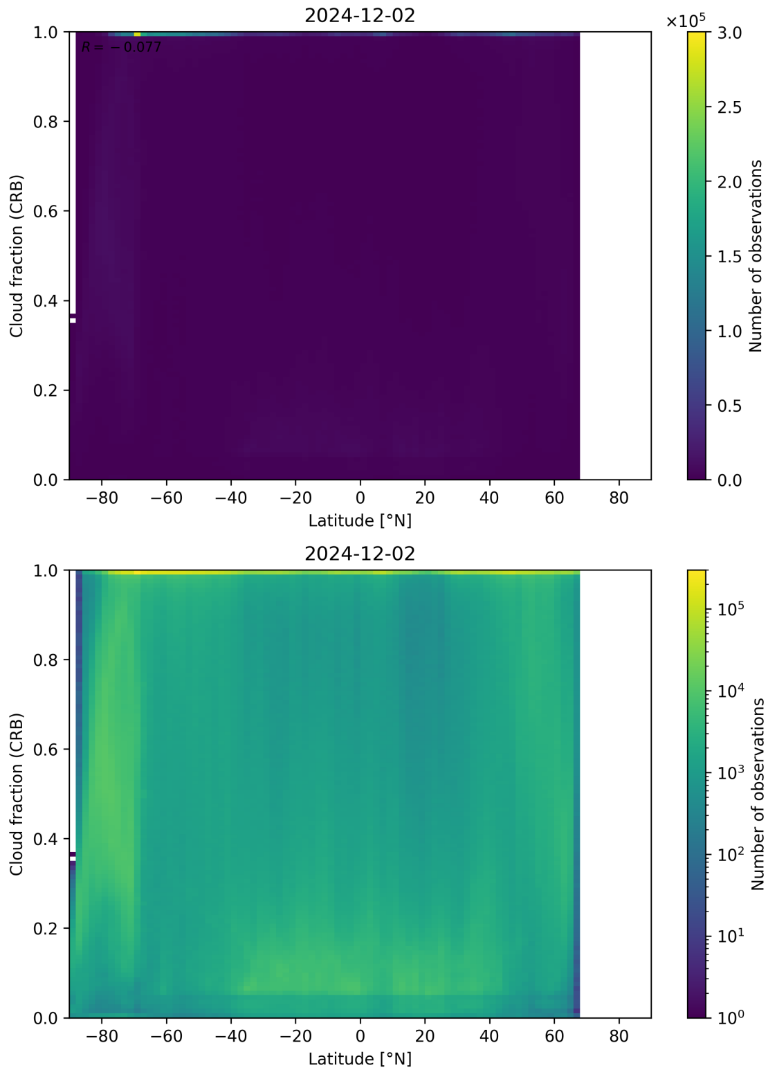
Figure 94: Scatter density plot of “Latitude” against “Cloud fraction (CRB)” for 2024-12-01 to 2024-12-03.
