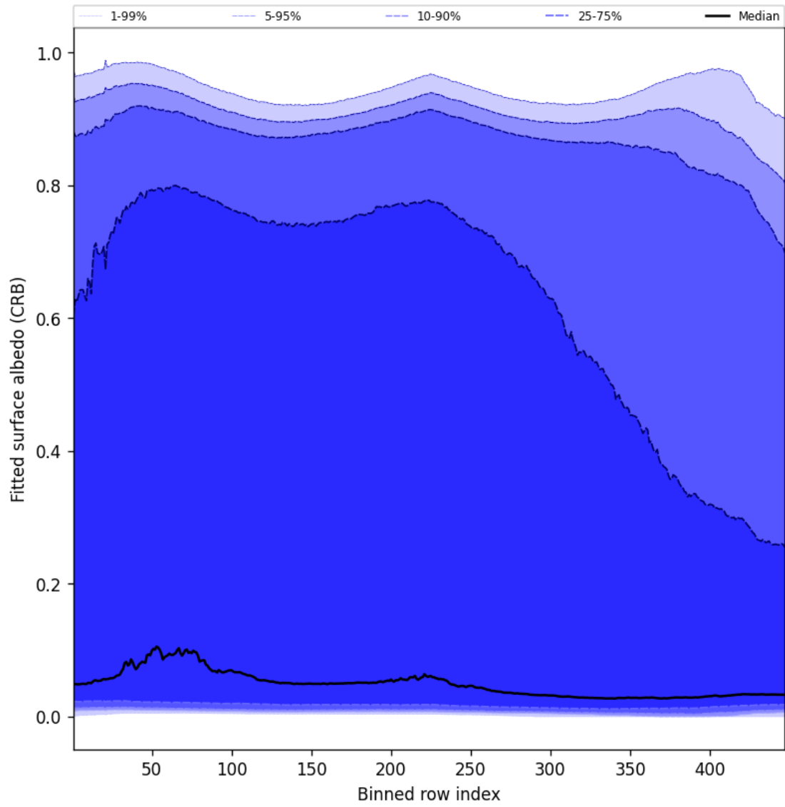
Figure 62: Along track statistics of “Fitted surface albedo (CRB)” for 2024-12-01 to 2024-12-03
