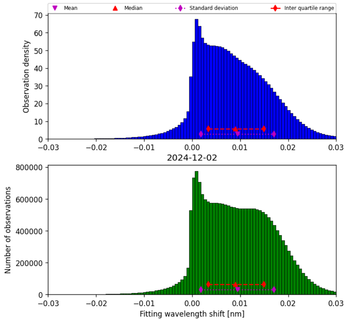
Figure 49: Histogram of “Fitting wavelength shift” for 2024-12-01 to 2024-12-03
