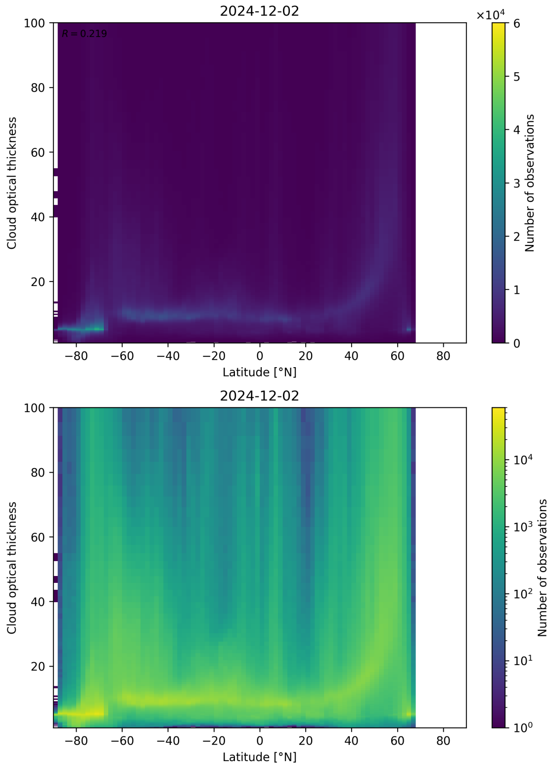
Figure 96: Scatter density plot of “Latitude” against “Cloud optical thickness” for 2024-12-01 to 2024-12-03.
