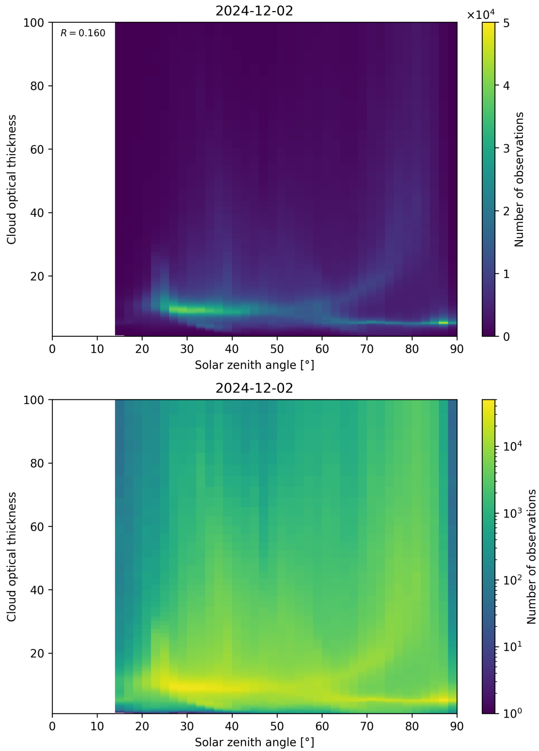
Figure 103: Scatter density plot of “Solar zenith angle” against “Cloud optical thickness” for 2024-12-01 to 2024-12-03.
