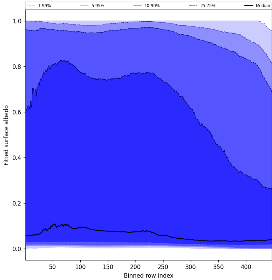
Figure 61: Along track statistics of “Fitted surface albedo” for 2024-12-01 to 2024-12-03
