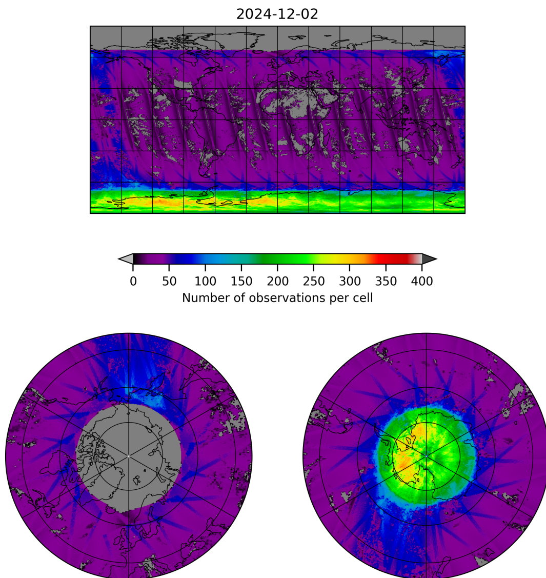
Figure 21: Map of the number of observations for 2024-12-01 to 2024-12-03
