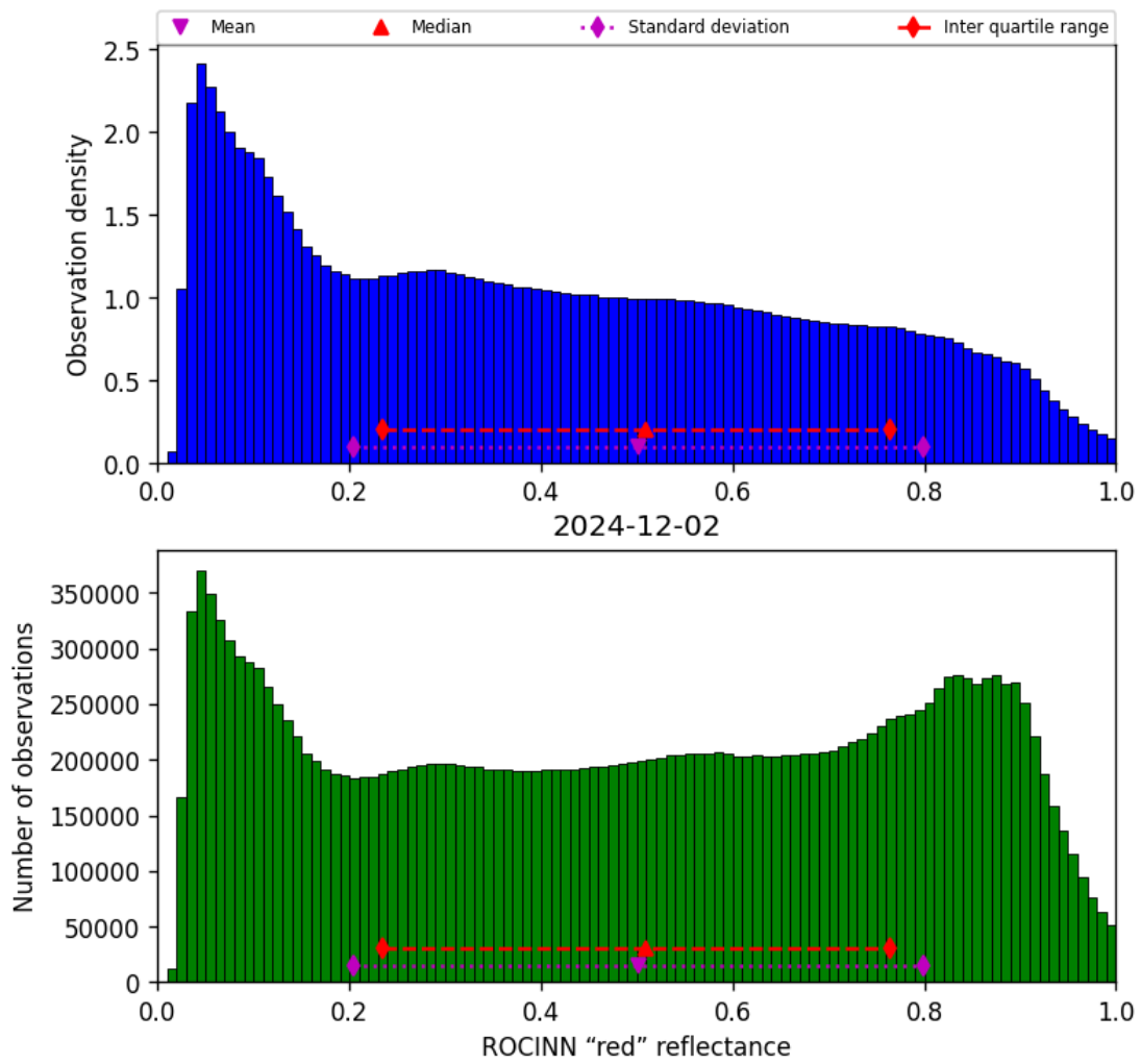
Figure 53: Histogram of “ROCINN “red” reflectance” for 2024-12-01 to 2024-12-03
