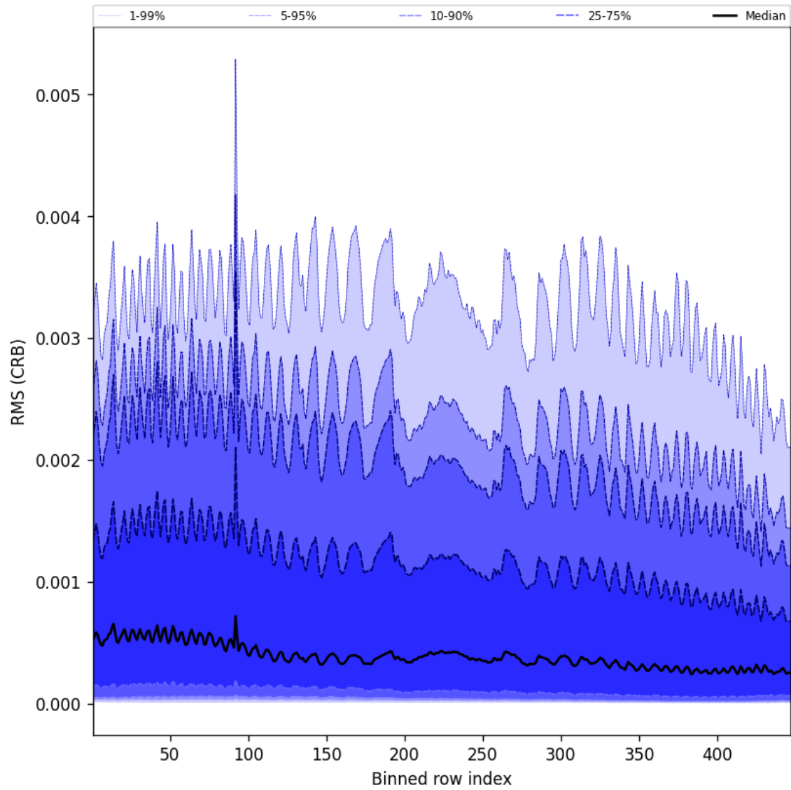
Figure 64: Along track statistics of “RMS (CRB)” for 2024-12-01 to 2024-12-03
