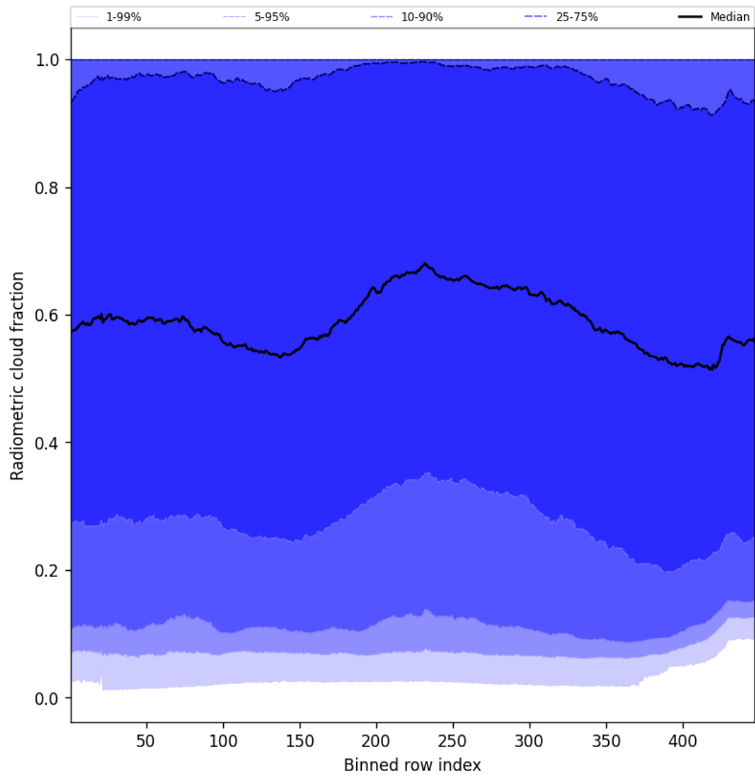
Figure 55: Along track statistics of “Radiometric cloud fraction” for 2024-12-01 to 2024-12-03
