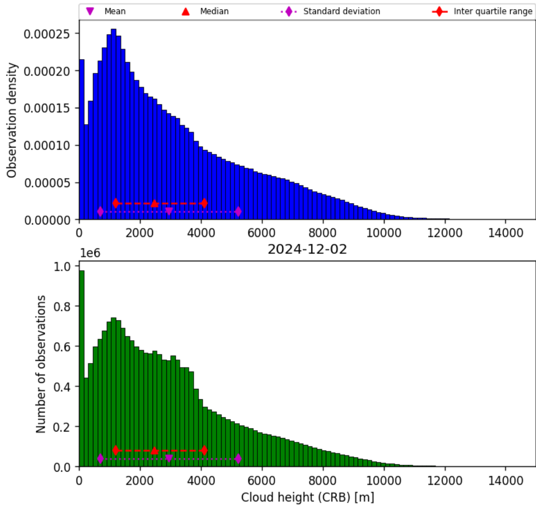
Figure 43: Histogram of “Cloud height (CRB)” for 2024-12-01 to 2024-12-03
