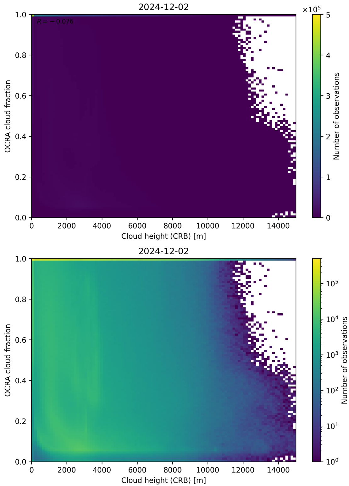
Figure 81: Scatter density plot of “Cloud height (CRB)” against “OCRA cloud fraction” for 2024-12-01 to 2024-12-03.
