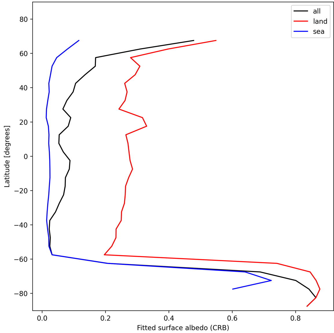
Figure 30: Zonal average of “Fitted surface albedo (CRB)” for 2024-12-01 to 2024-12-03.
