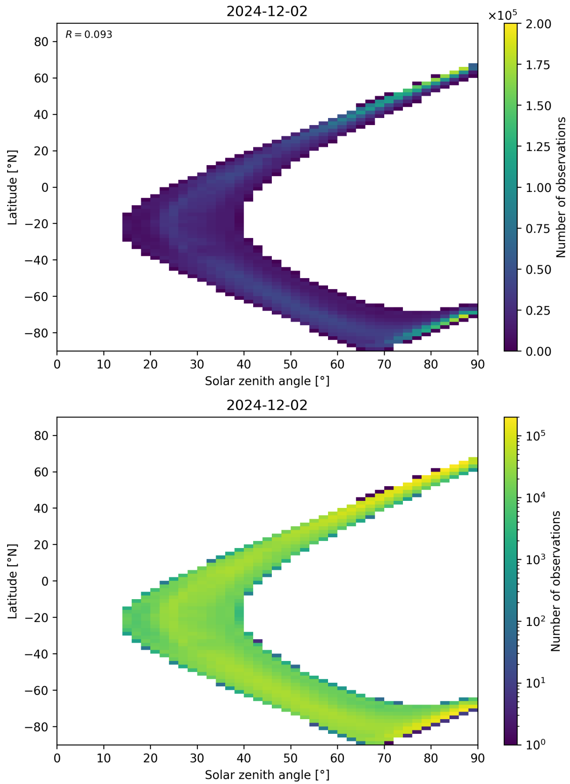
Figure 105: Scatter density plot of “Solar zenith angle” against “Latitude” for 2024-12-01 to 2024-12-03.
