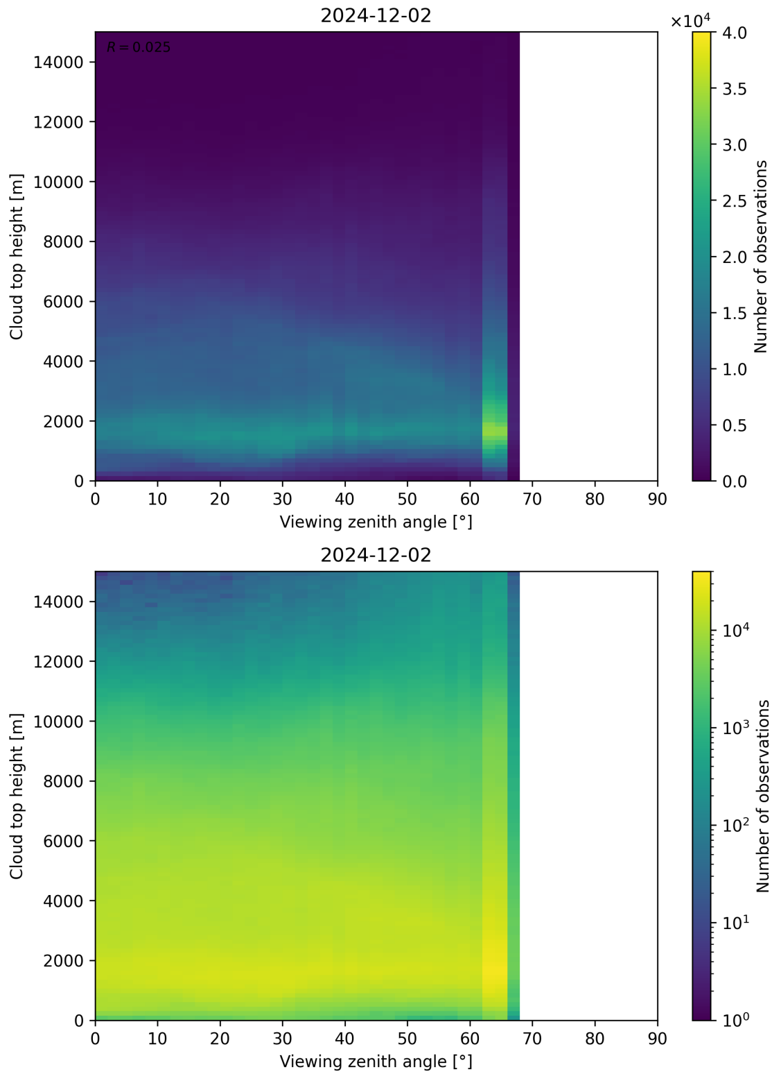
Figure 112: Scatter density plot of “Viewing zenith angle” against “Cloud top height” for 2024-12-01 to 2024-12-03.
