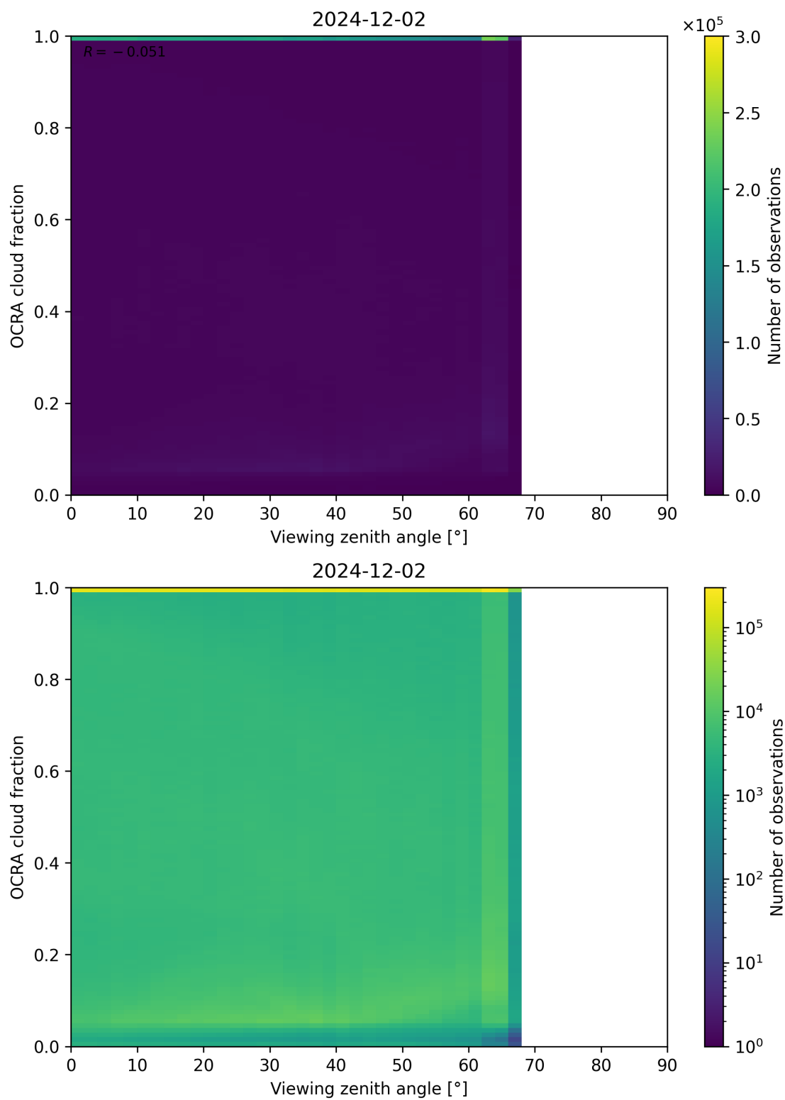
Figure 108: Scatter density plot of “Viewing zenith angle” against “OCRA cloud fraction” for 2024-12-01 to 2024-12-03.
