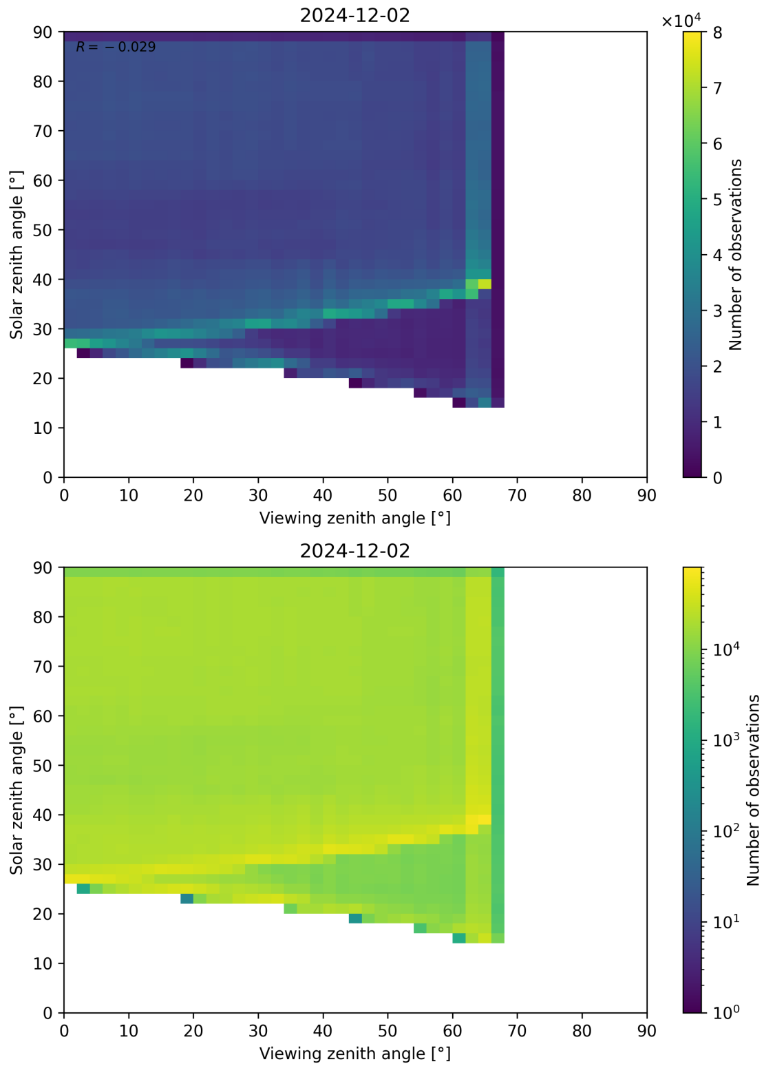
Figure 114: Scatter density plot of “Viewing zenith angle” against “Solar zenith angle” for 2024-12-01 to 2024-12-03.
