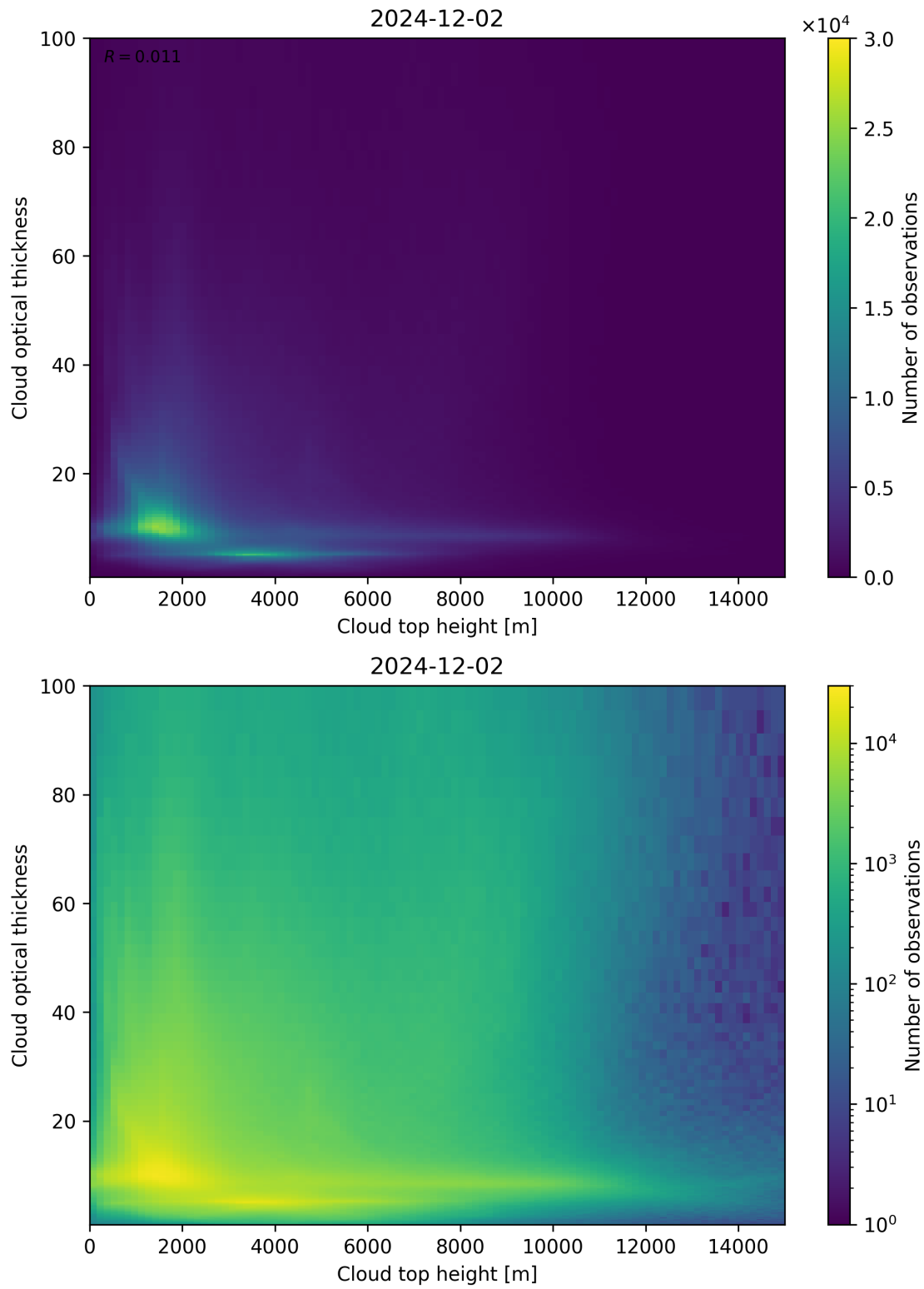
Figure 90: Scatter density plot of “Cloud top height” against “Cloud optical thickness” for 2024-12-01 to 2024-12-03.
