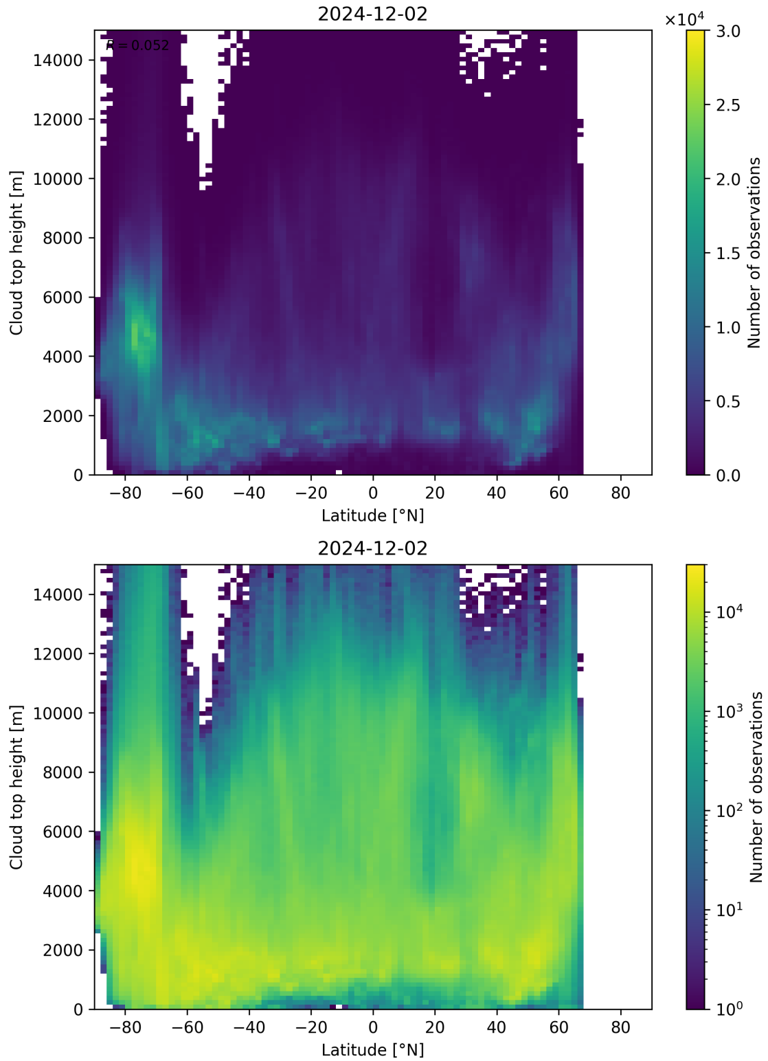
Figure 97: Scatter density plot of “Latitude” against “Cloud top height” for 2024-12-01 to 2024-12-03.
