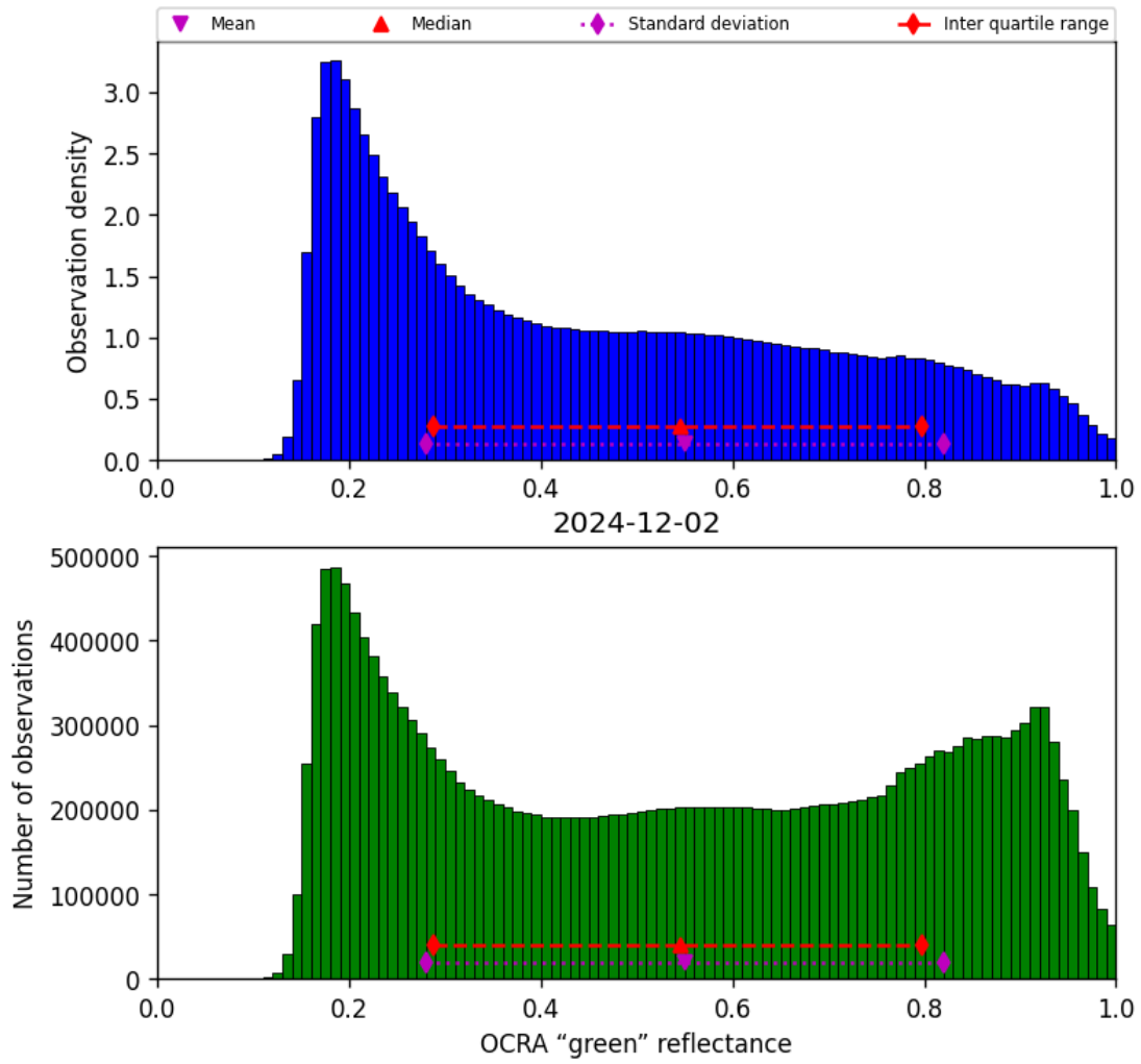
Figure 52: Histogram of “OCRA “green” reflectance” for 2024-12-01 to 2024-12-03
