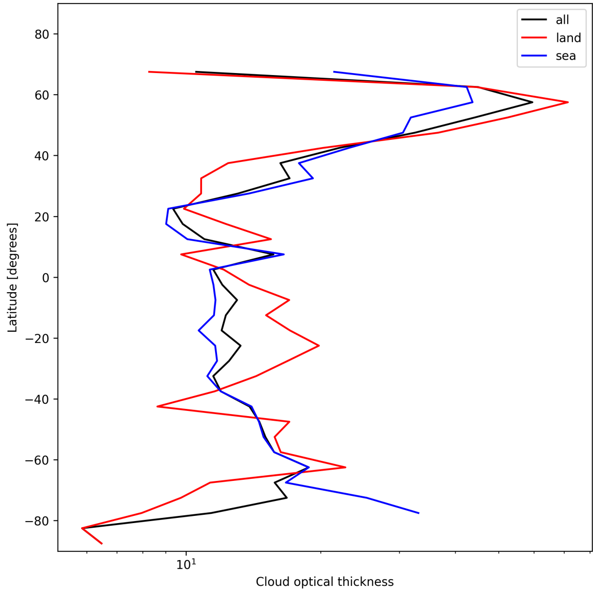
Figure 25: Zonal average of “Cloud optical thickness” for 2024-12-01 to 2024-12-03.
