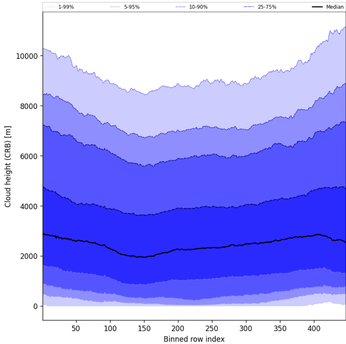
Figure 59: Along track statistics of “Cloud height (CRB)” for 2024-12-01 to 2024-12-03
