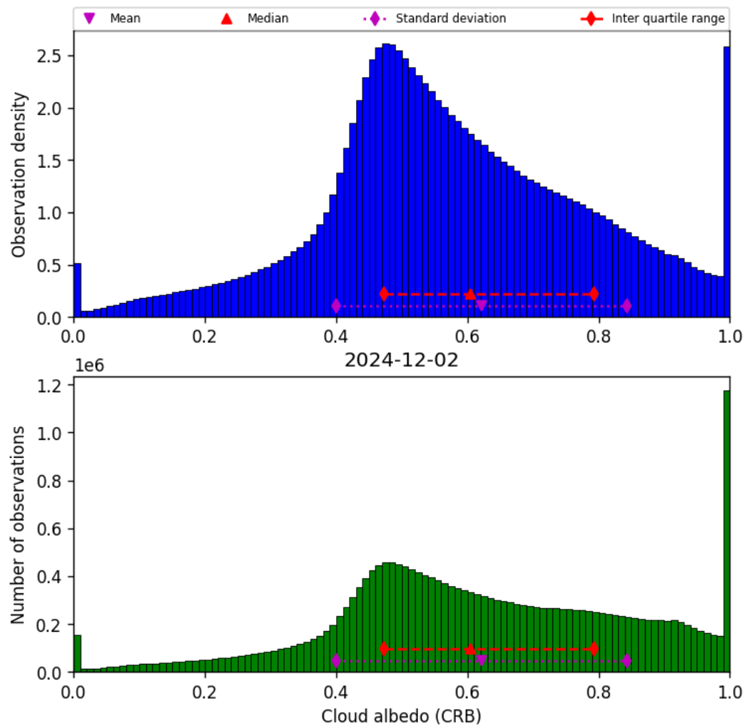
Figure 44: Histogram of “Cloud albedo (CRB)” for 2024-12-01 to 2024-12-03
