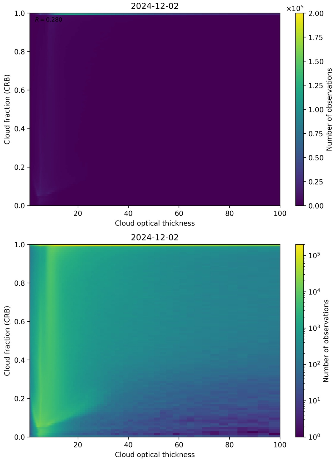
Figure 84: Scatter density plot of “Cloud optical thickness” against “Cloud fraction (CRB)” for 2024-12-01 to 2024-12-03.
