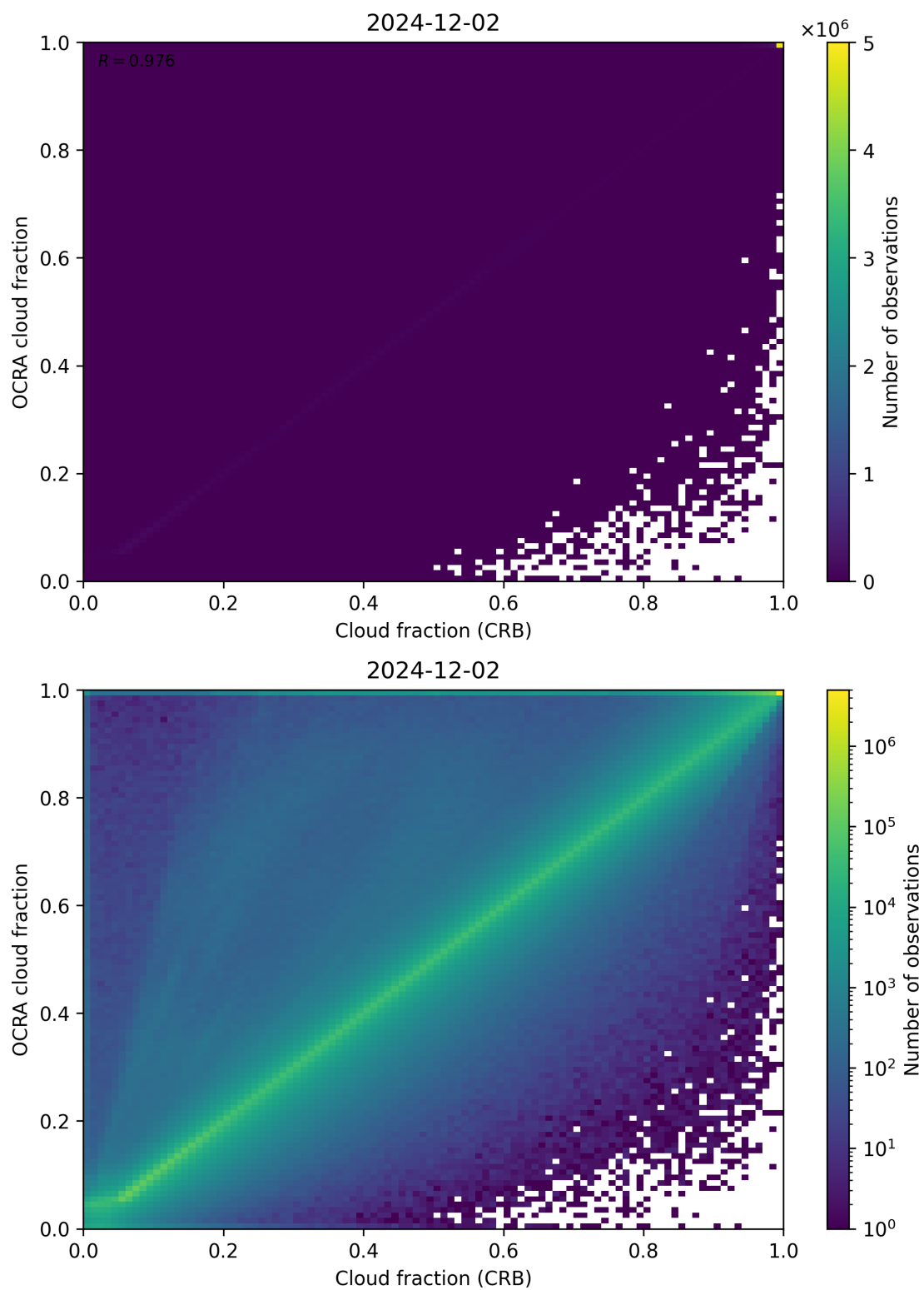
Figure 78: Scatter density plot of “Cloud fraction (CRB)” against “OCRA cloud fraction” for 2024-12-01 to 2024-12-03.
