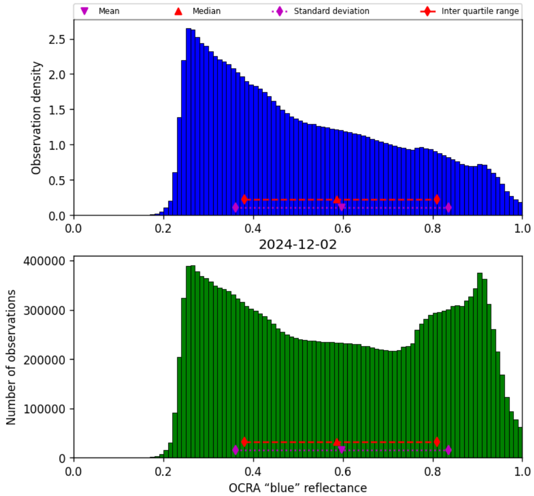
Figure 51: Histogram of “OCRA “blue” reflectance” for 2024-12-01 to 2024-12-03
