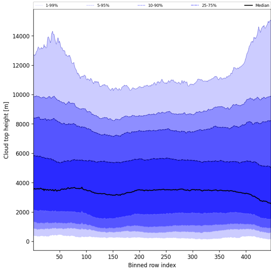
Figure 56: Along track statistics of “Cloud top height” for 2024-12-01 to 2024-12-03
