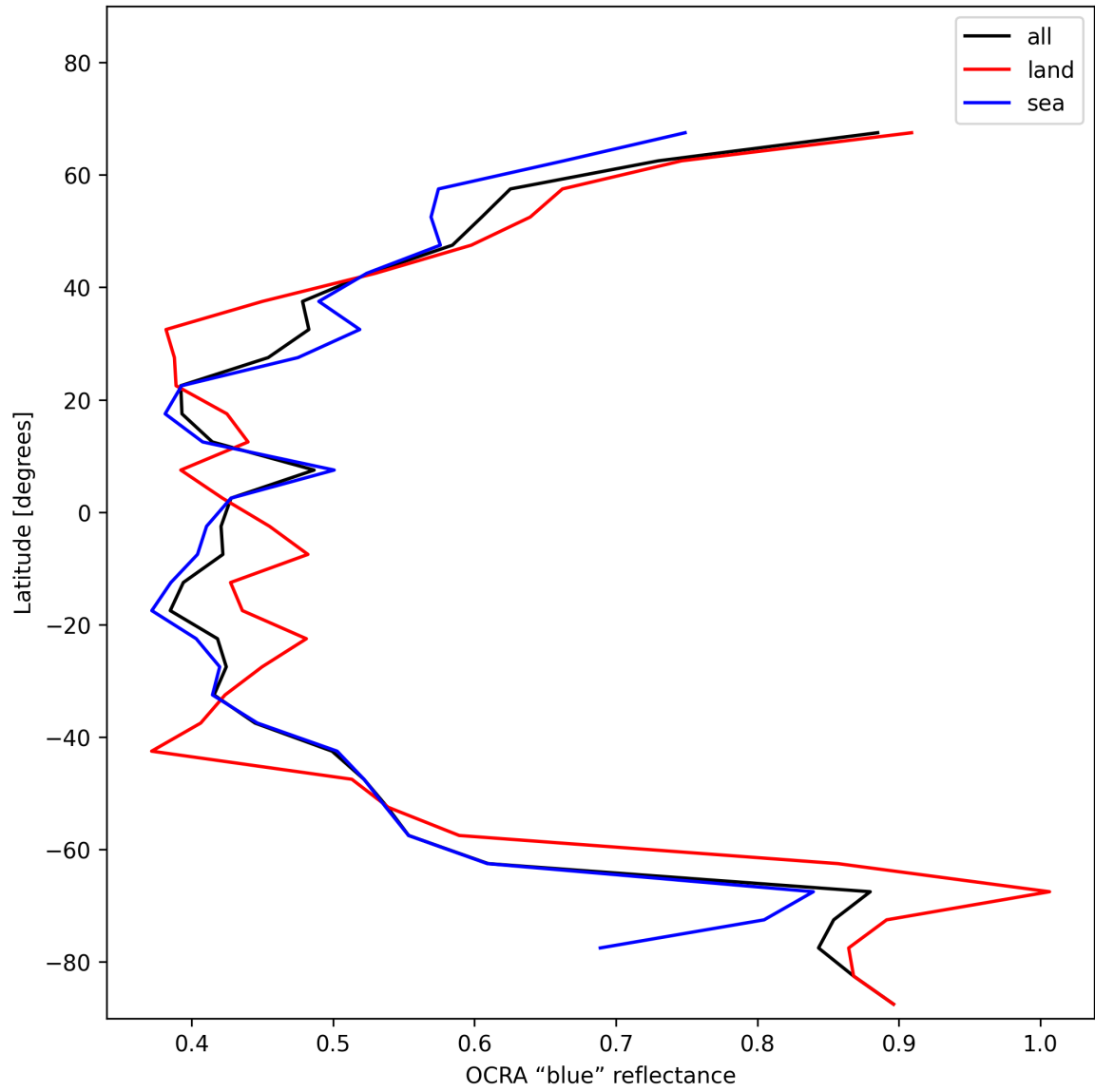
Figure 35: Zonal average of “OCRA “blue” reflectance” for 2024-12-01 to 2024-12-03.
