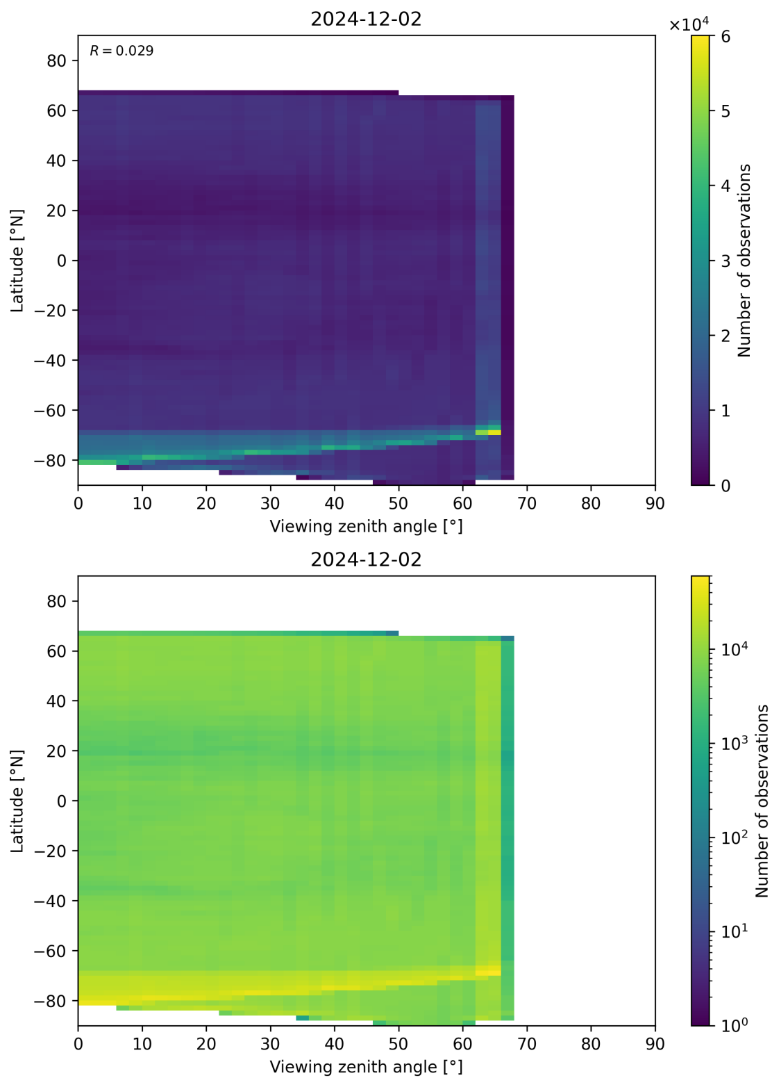
Figure 113: Scatter density plot of “Viewing zenith angle” against “Latitude” for 2024-12-01 to 2024-12-03.
