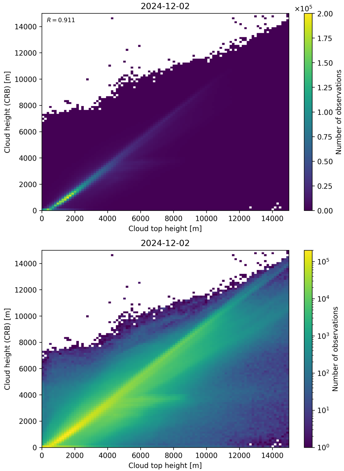
Figure 89: Scatter density plot of “Cloud top height” against “Cloud height (CRB)” for 2024-12-01 to 2024-12-03.
