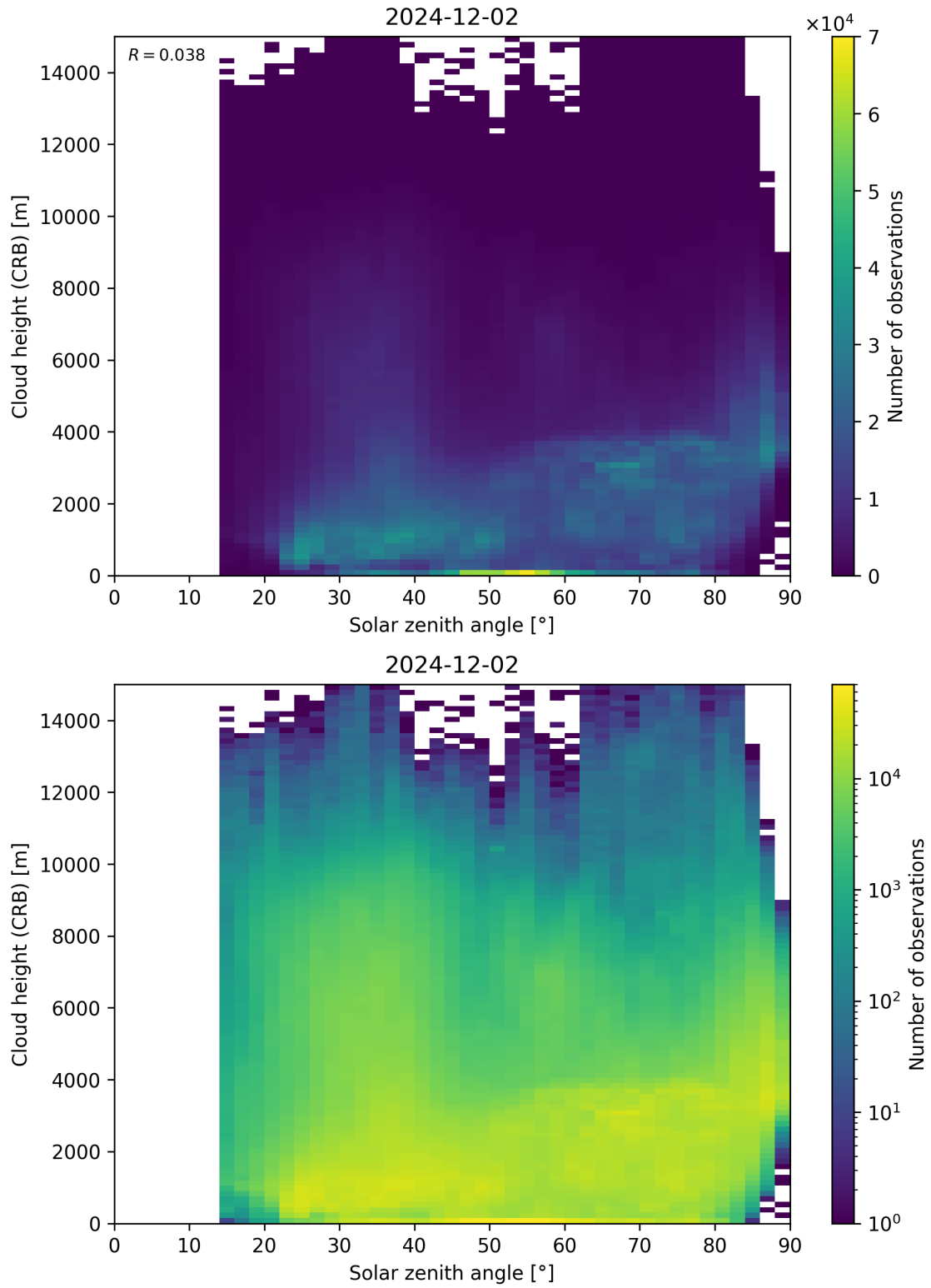
Figure 102: Scatter density plot of “Solar zenith angle” against “Cloud height (CRB)” for 2024-12-01 to 2024-12-03.
