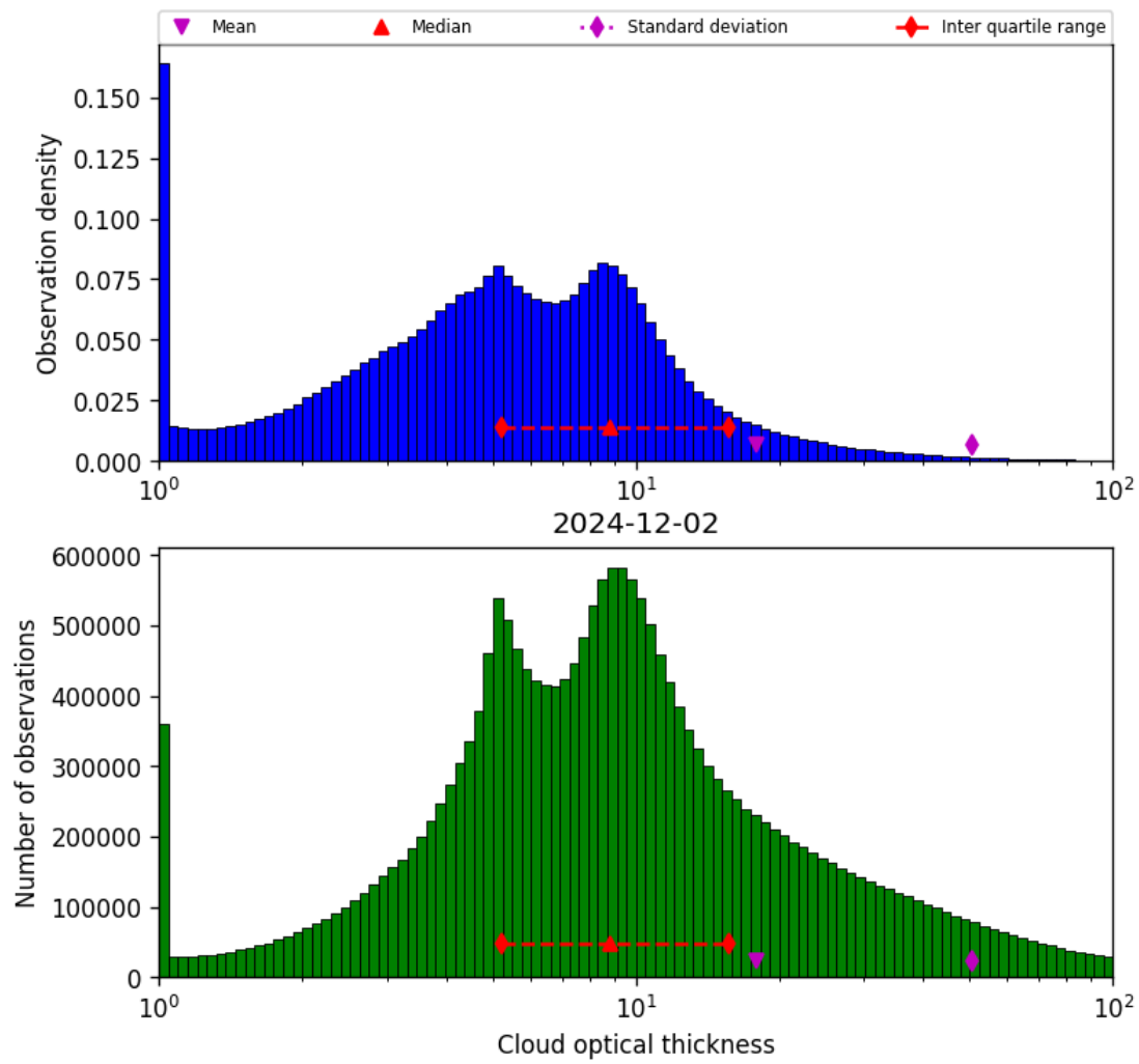
Figure 41: Histogram of “Cloud optical thickness” for 2024-12-01 to 2024-12-03
