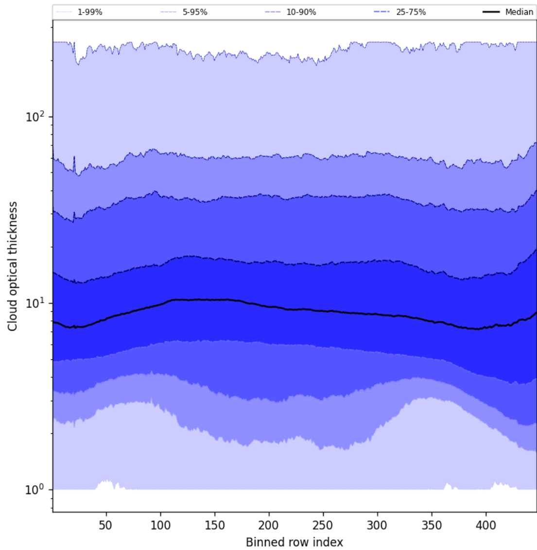
Figure 57: Along track statistics of “Cloud optical thickness” for 2024-12-01 to 2024-12-03
