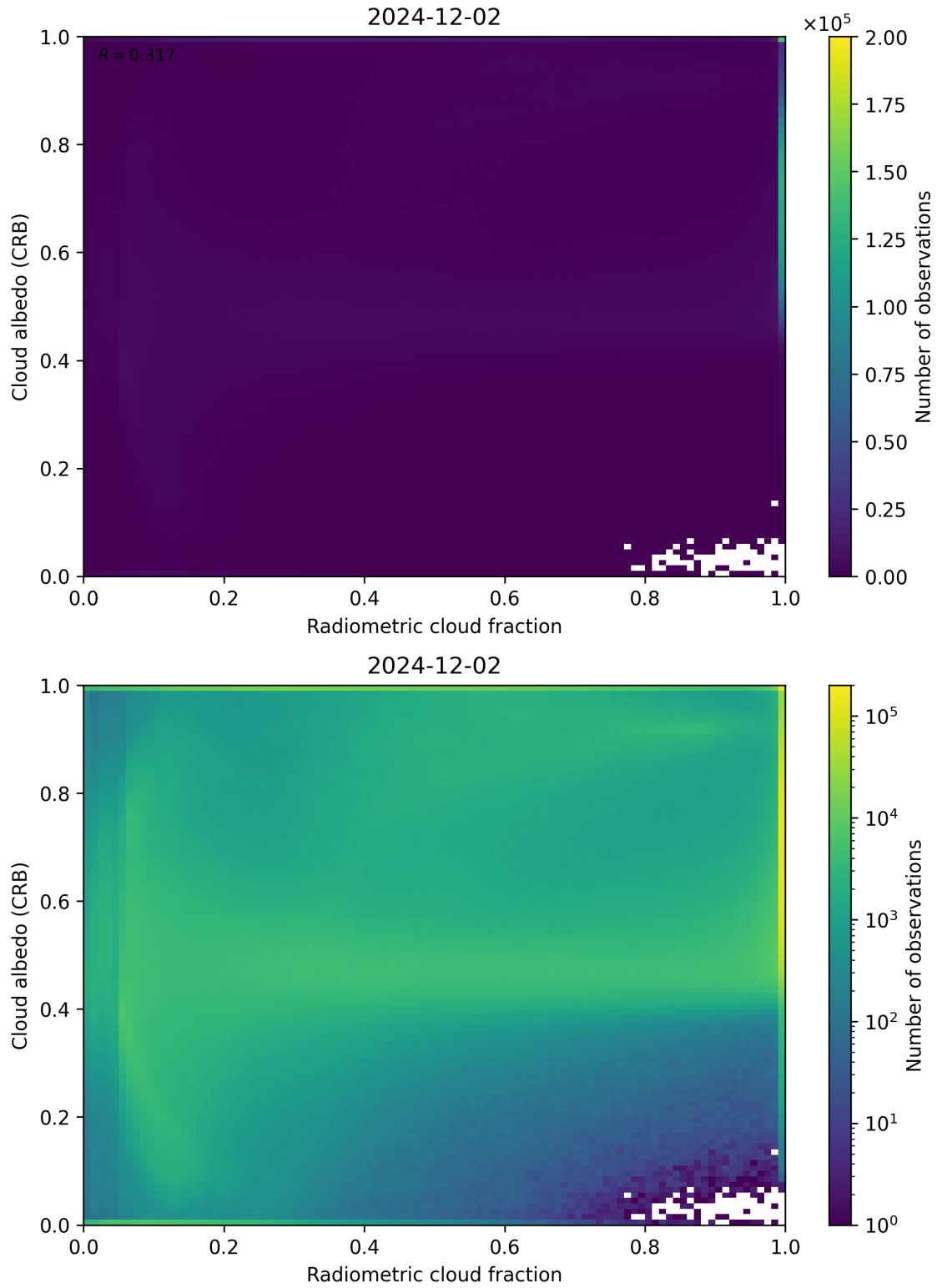
Figure 71: Scatter density plot of “Radiometric cloud fraction” against “Cloud albedo (CRB)” for 2024-12-01 to 2024-12-03.
