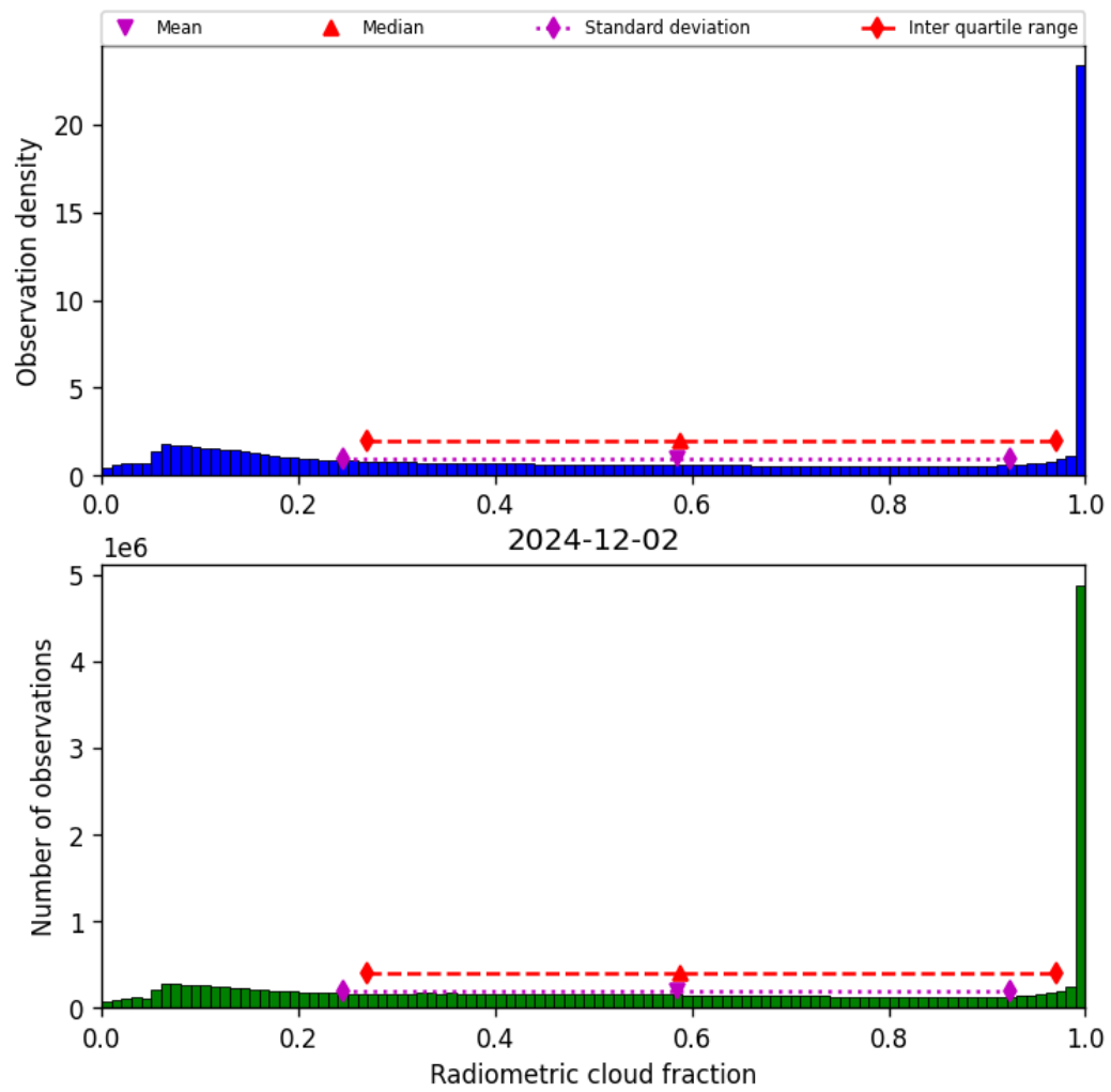
Figure 39: Histogram of “Radiometric cloud fraction” for 2024-12-01 to 2024-12-03
