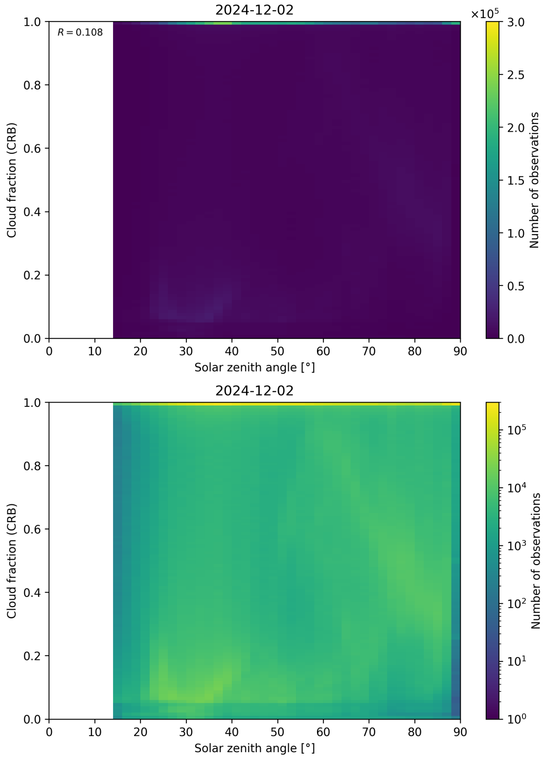
Figure 101: Scatter density plot of “Solar zenith angle” against “Cloud fraction (CRB)” for 2024-12-01 to 2024-12-03.
