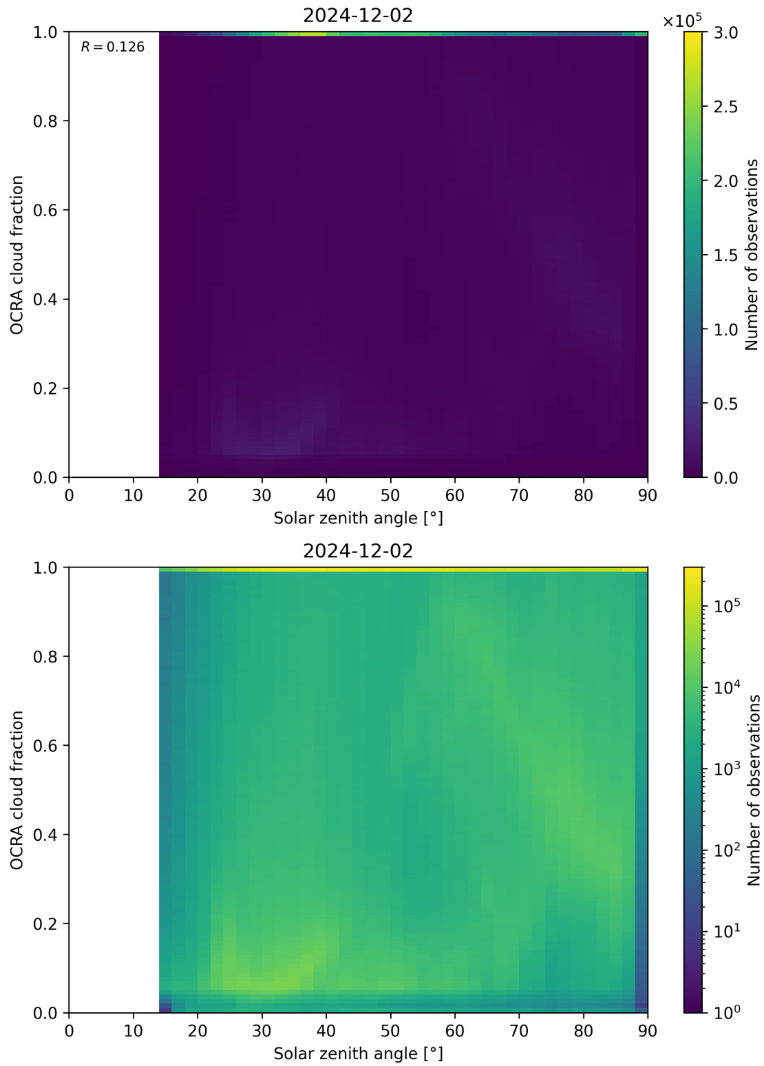
Figure 100: Scatter density plot of “Solar zenith angle” against “OCRA cloud fraction” for 2024-12-01 to 2024-12-03.
