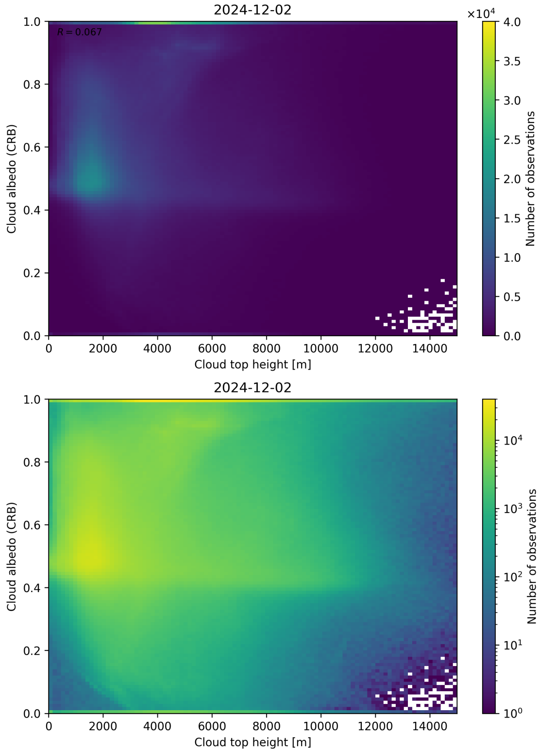
Figure 86: Scatter density plot of “Cloud top height” against “Cloud albedo (CRB)” for 2024-12-01 to 2024-12-03.
