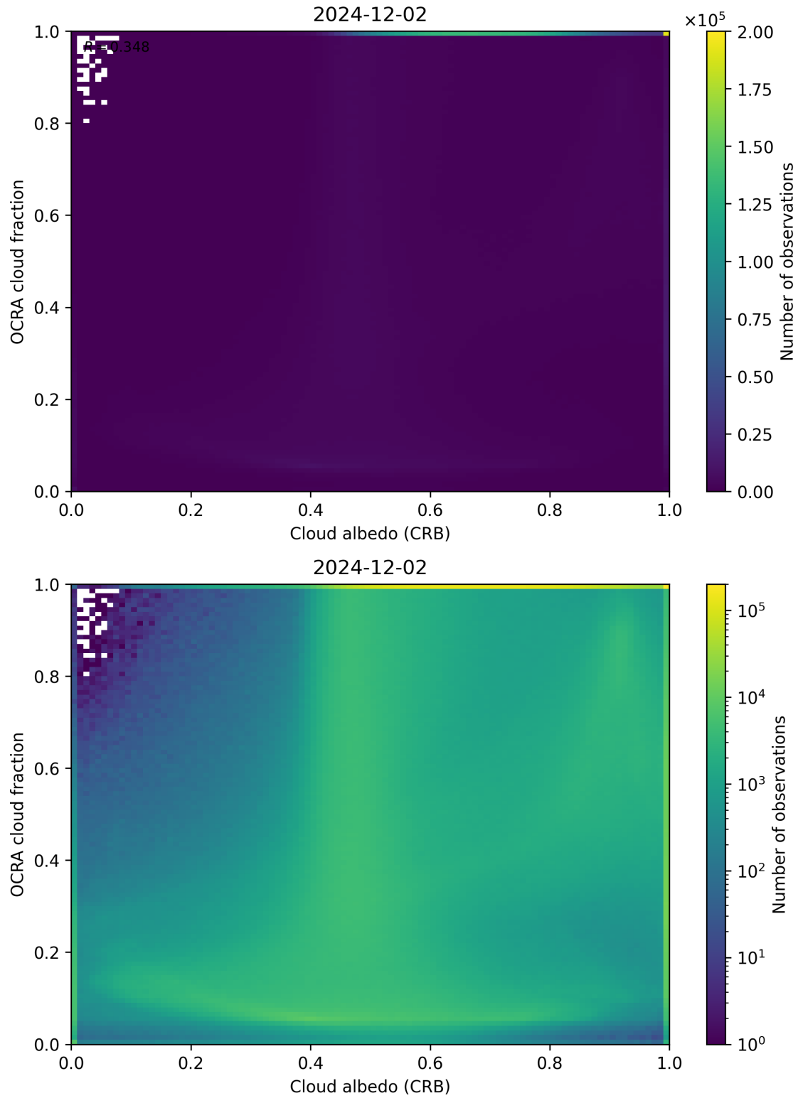
Figure 70: Scatter density plot of “Cloud albedo (CRB)” against “OCRA cloud fraction” for 2024-12-01 to 2024-12-03.
