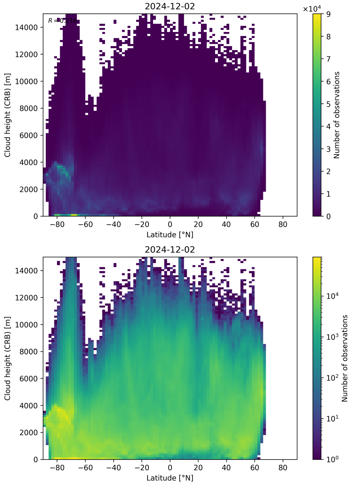
Figure 95: Scatter density plot of “Latitude” against “Cloud height (CRB)” for 2024-12-01 to 2024-12-03.
