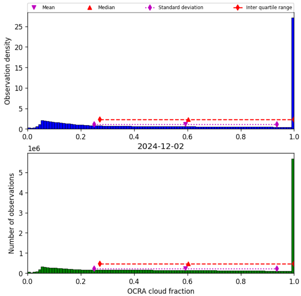
Figure 50: Histogram of “OCRA cloud fraction” for 2024-12-01 to 2024-12-03
