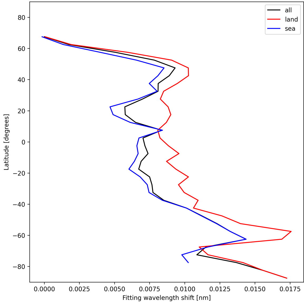
Figure 33: Zonal average of “Fitting wavelength shift” for 2024-12-01 to 2024-12-03.
