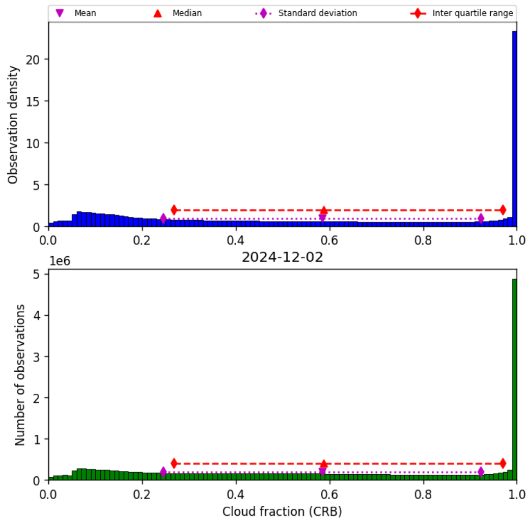
Figure 42: Histogram of “Cloud fraction (CRB)” for 2024-12-01 to 2024-12-03
