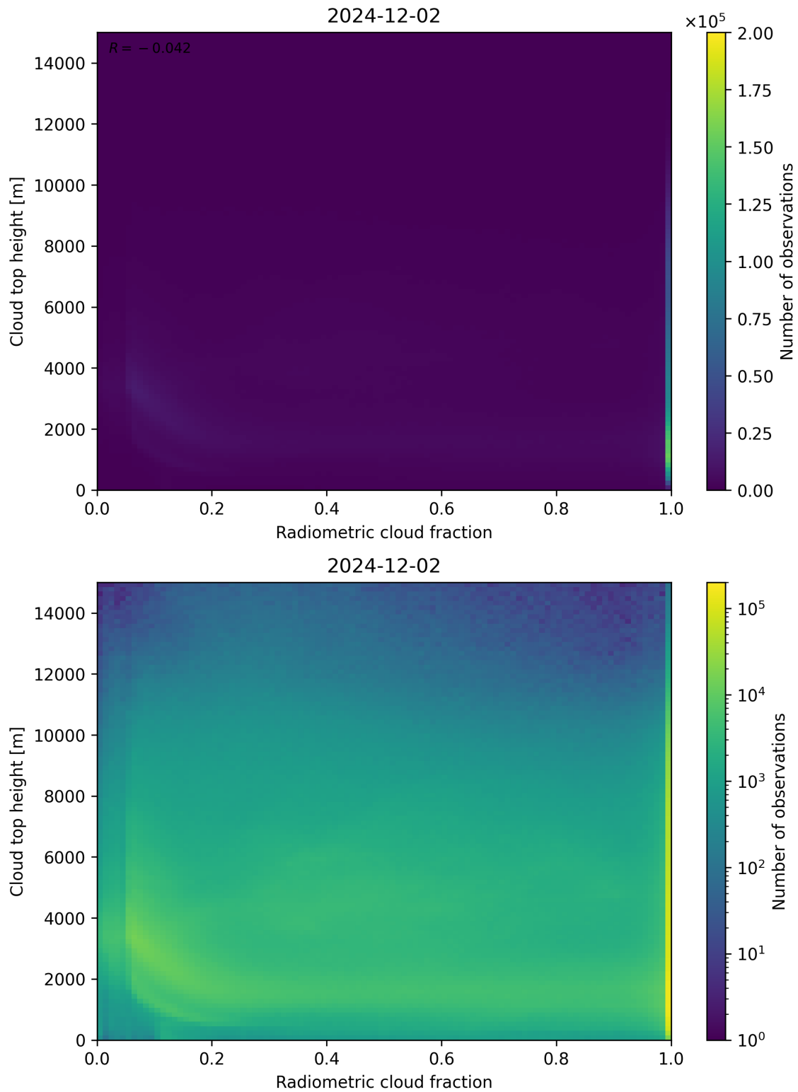
Figure 76: Scatter density plot of “Radiometric cloud fraction” against “Cloud top height” for 2024-12-01 to 2024-12-03.
