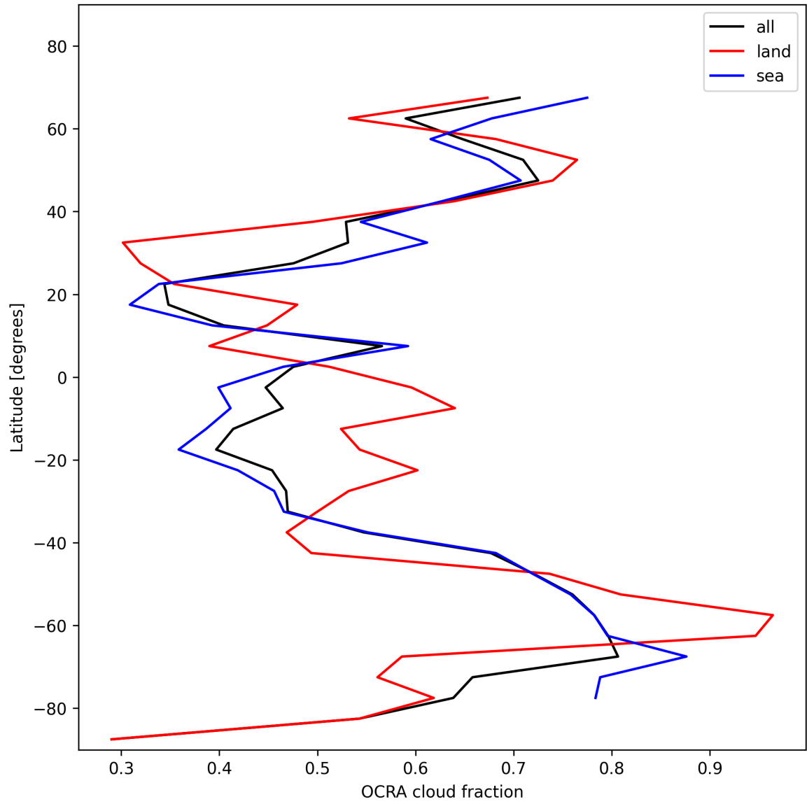
Figure 34: Zonal average of “OCRA cloud fraction” for 2024-12-01 to 2024-12-03.
