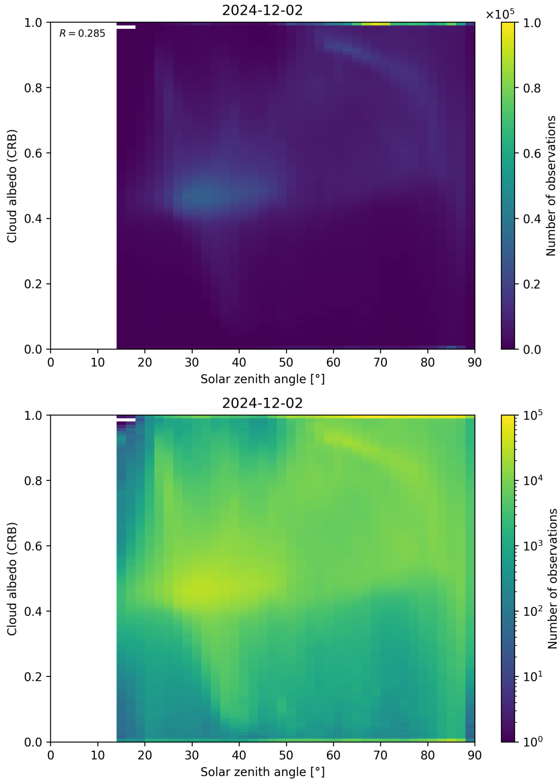
Figure 98: Scatter density plot of “Solar zenith angle” against “Cloud albedo (CRB)” for 2024-12-01 to 2024-12-03.
