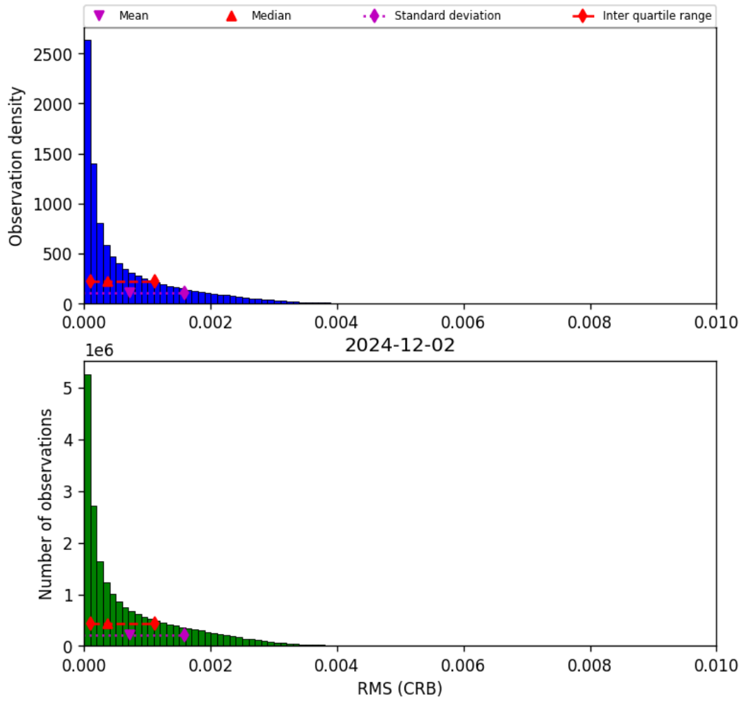
Figure 48: Histogram of “RMS (CRB)” for 2024-12-01 to 2024-12-03
