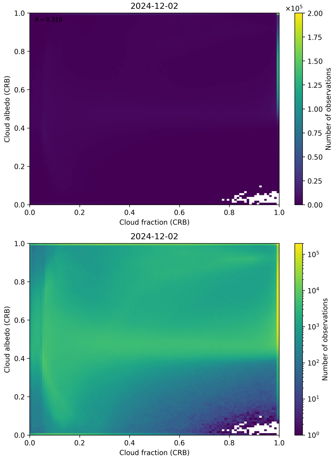
Figure 77: Scatter density plot of “Cloud fraction (CRB)” against “Cloud albedo (CRB)” for 2024-12-01 to 2024-12-03.
