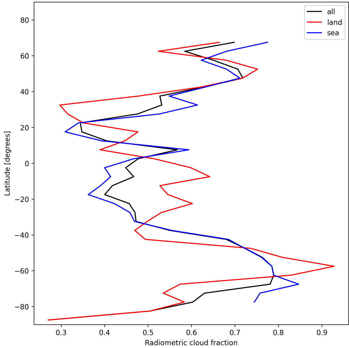
Figure 23: Zonal average of “Radiometric cloud fraction” for 2024-12-01 to 2024-12-03.
