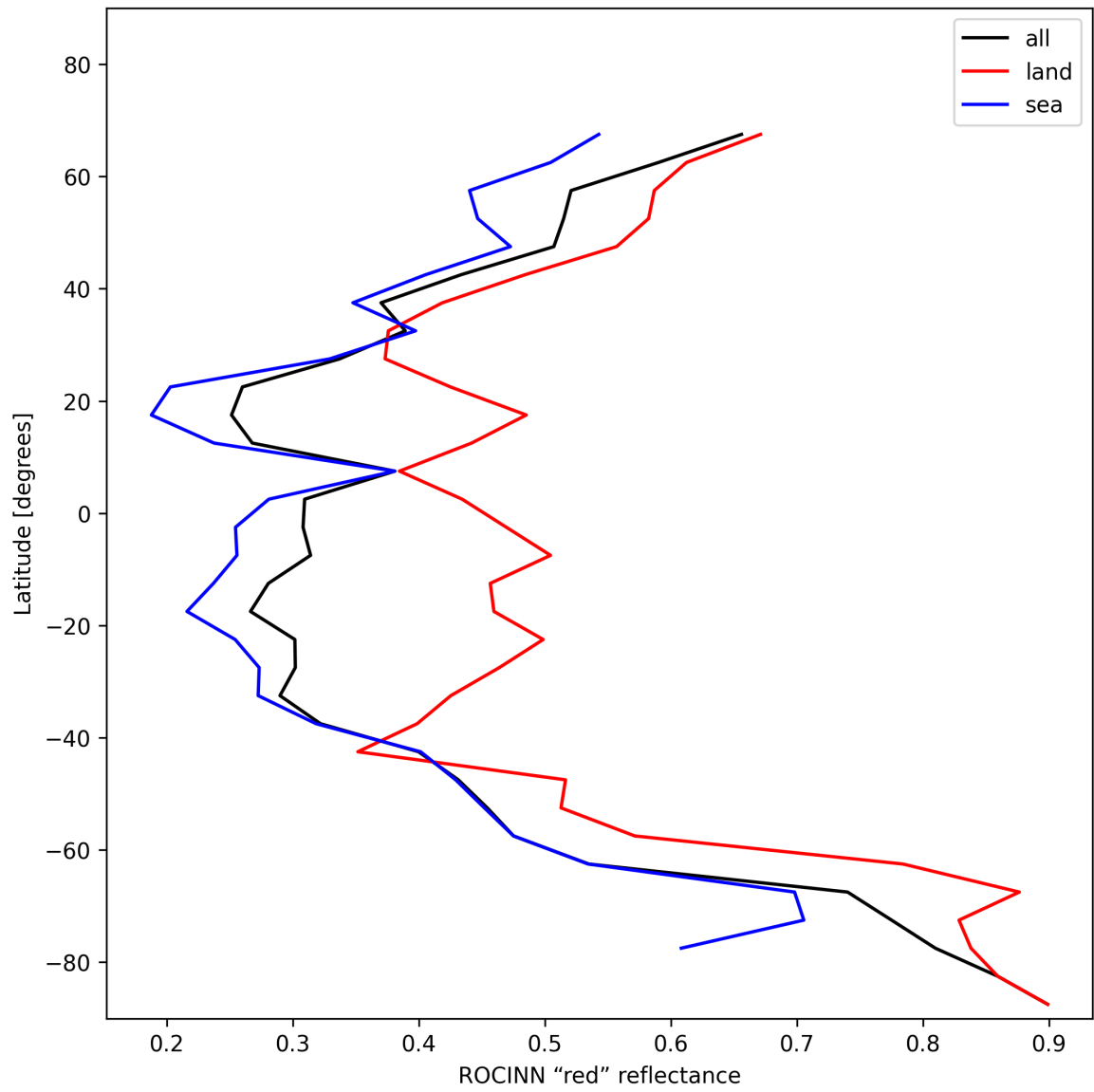
Figure 37: Zonal average of "ROCINN "red" reflectance" for 2024-12-01 to 2024-12-03.
