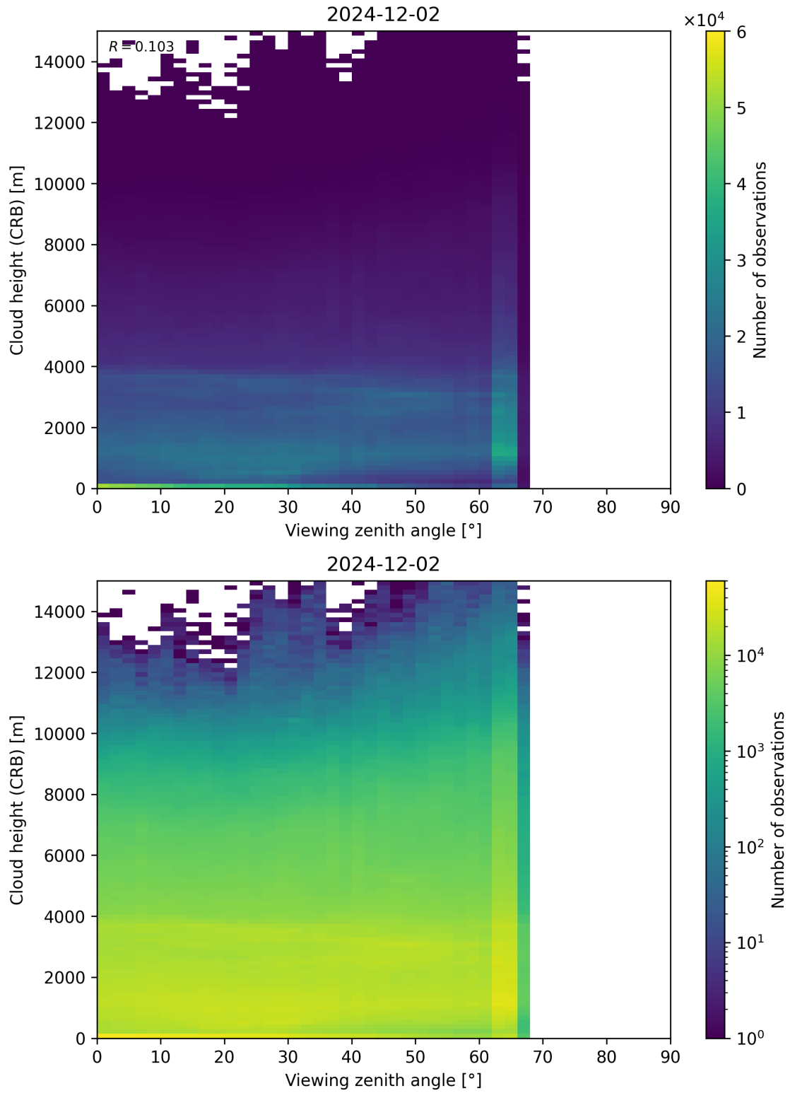
Figure 110: Scatter density plot of “Viewing zenith angle” against “Cloud height (CRB)” for 2024-12-01 to 2024-12-03.
