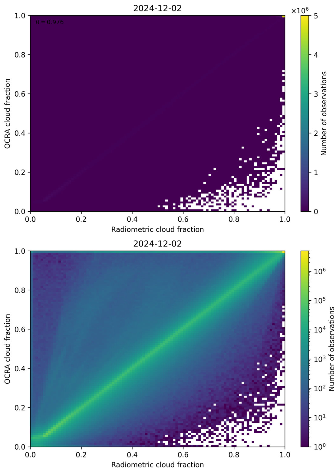
Figure 72: Scatter density plot of “Radiometric cloud fraction” against “OCRA cloud fraction” for 2024-12-01 to 2024-12-03.
