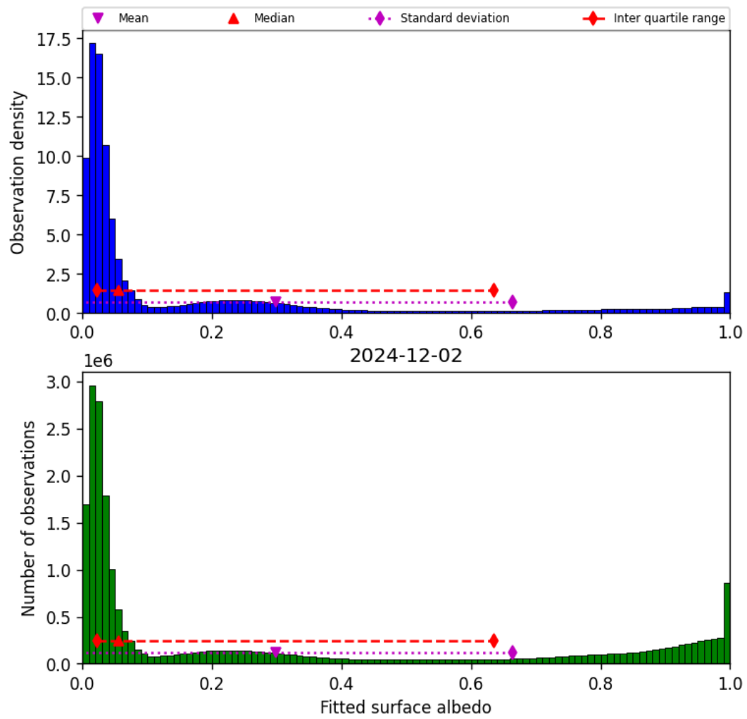
Figure 45: Histogram of “Fitted surface albedo” for 2024-12-01 to 2024-12-03
