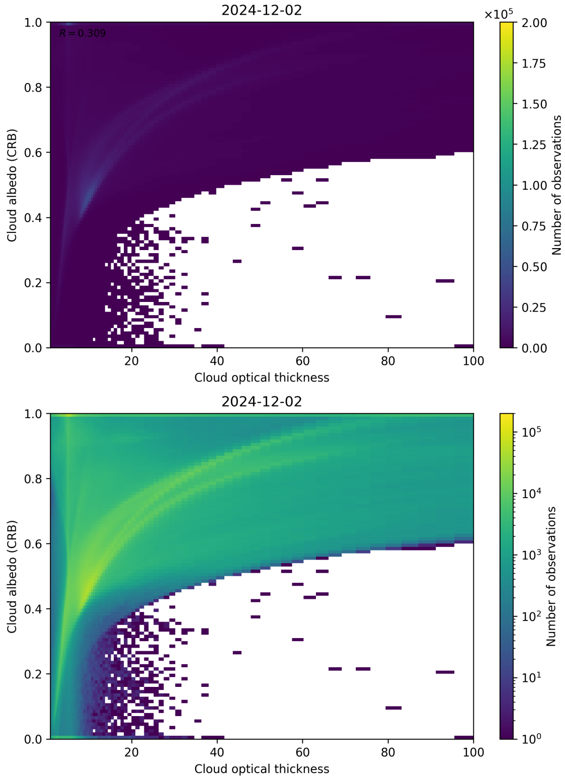
Figure 82: Scatter density plot of “Cloud optical thickness” against “Cloud albedo (CRB)” for 2024-12-01 to 2024-12-03.
