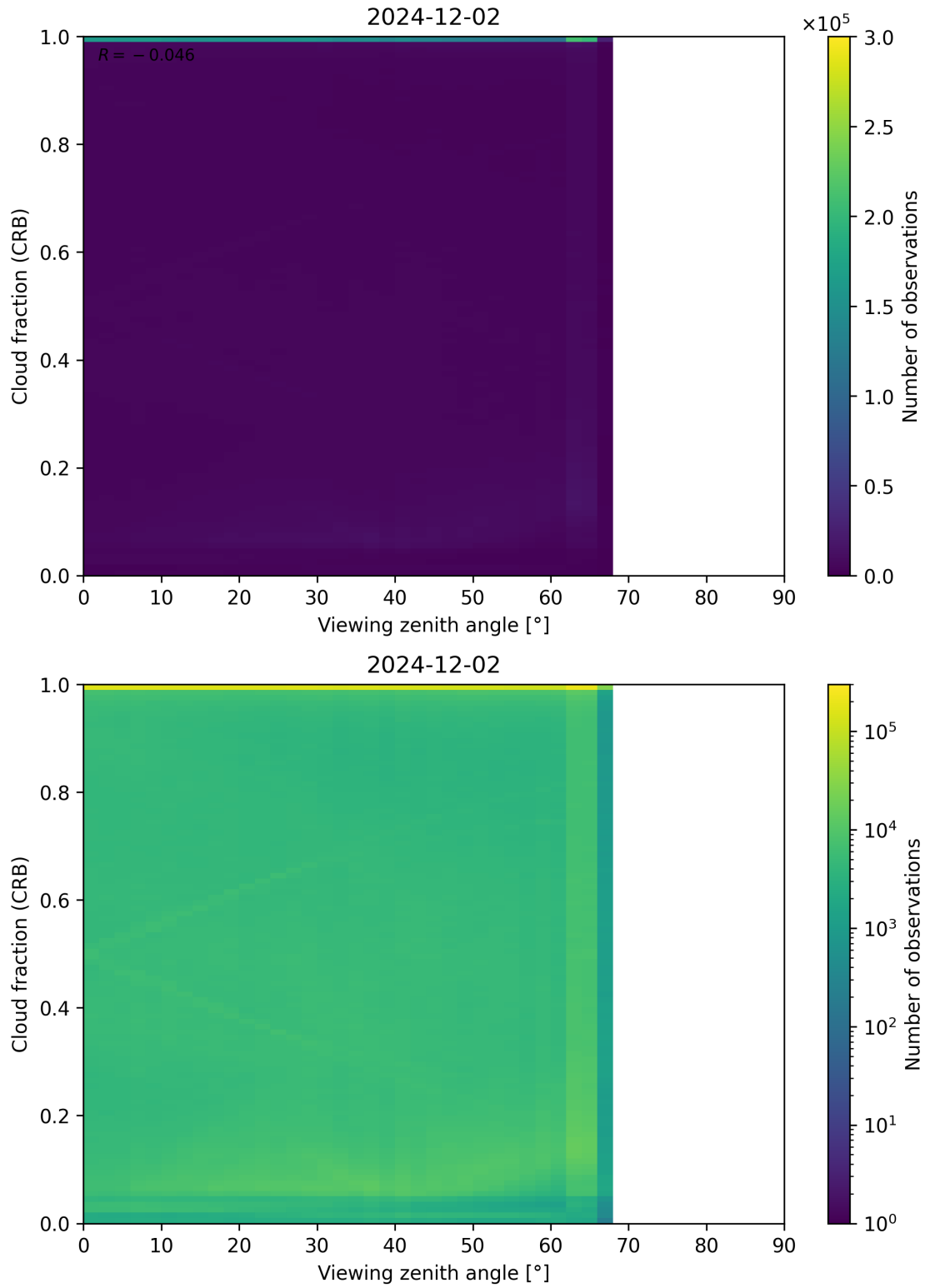
Figure 109: Scatter density plot of “Viewing zenith angle” against “Cloud fraction (CRB)” for 2024-12-01 to 2024-12-03.
