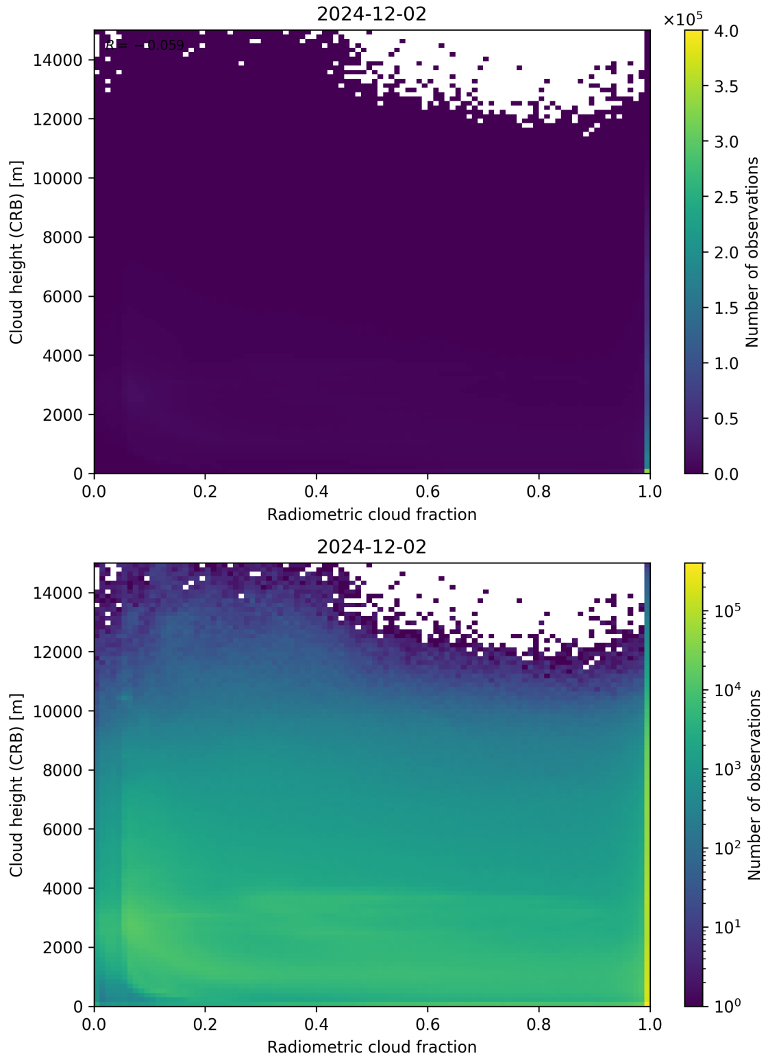
Figure 74: Scatter density plot of “Radiometric cloud fraction” against “Cloud height (CRB)” for 2024-12-01 to 2024-12-03.
