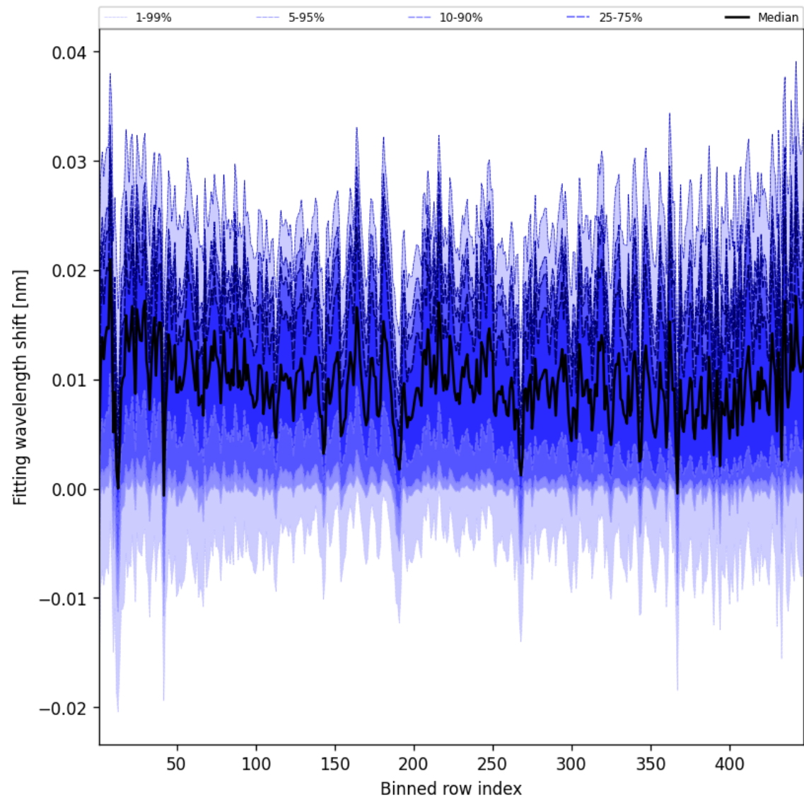
Figure 65: Along track statistics of “Fitting wavelength shift” for 2024-12-01 to 2024-12-03
