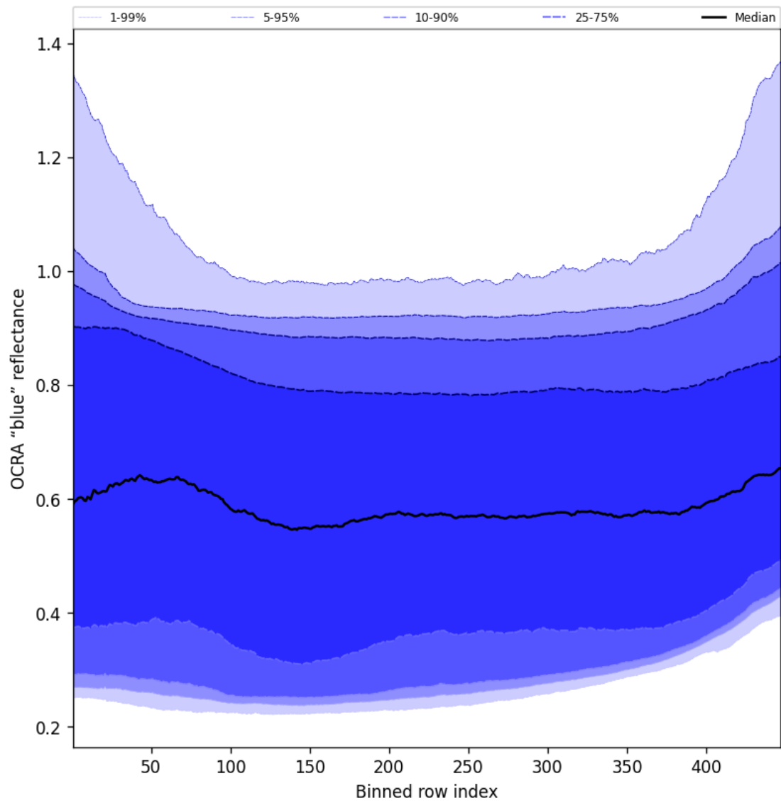
Figure 67: Along track statistics of “OCRA “blue” reflectance” for 2024-12-01 to 2024-12-03
