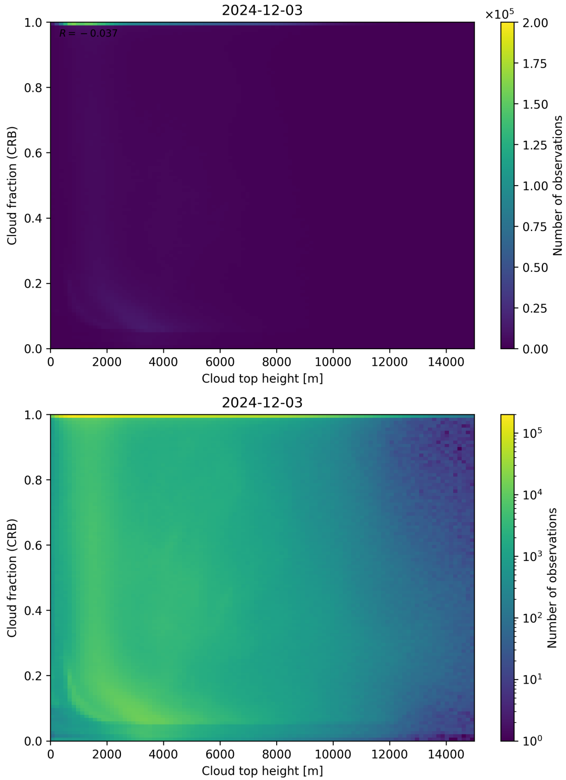
Figure 88: Scatter density plot of “Cloud top height” against “Cloud fraction (CRB)” for 2024-12-02 to 2024-12-04.
