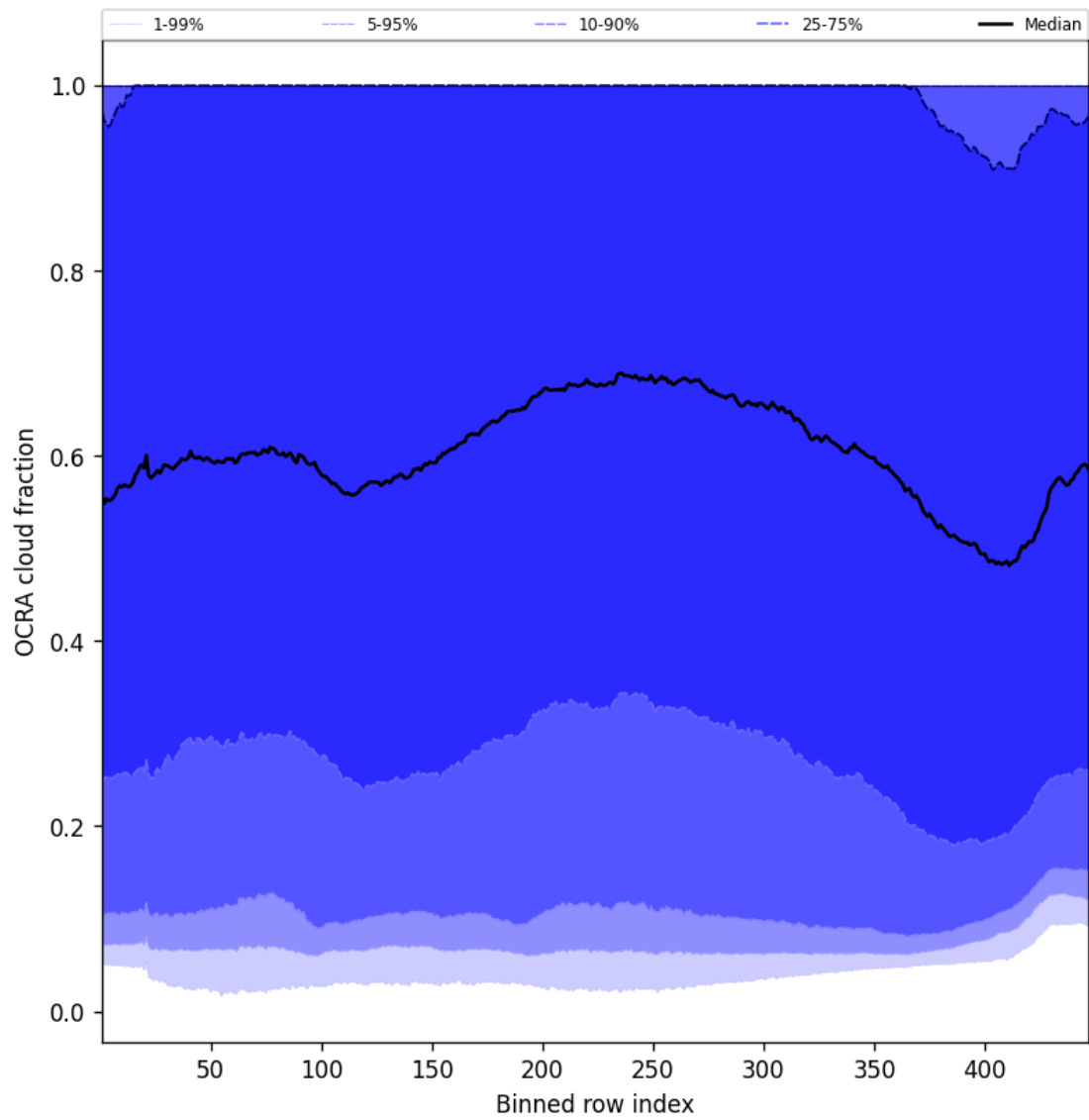
Figure 66: Along track statistics of “OCRA cloud fraction” for 2024-12-02 to 2024-12-04
