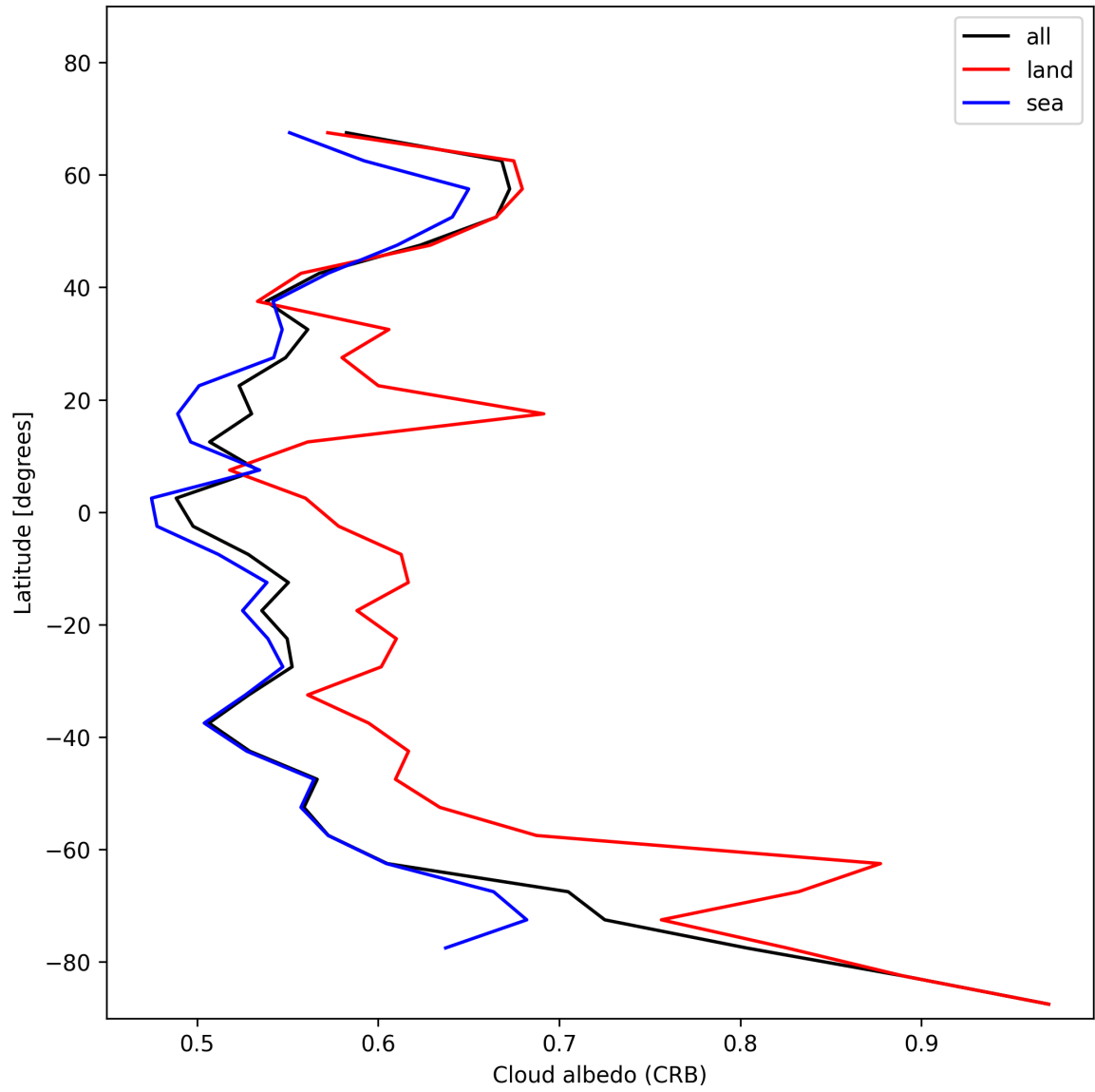
Figure 28: Zonal average of “Cloud albedo (CRB)” for 2024-12-02 to 2024-12-04.
