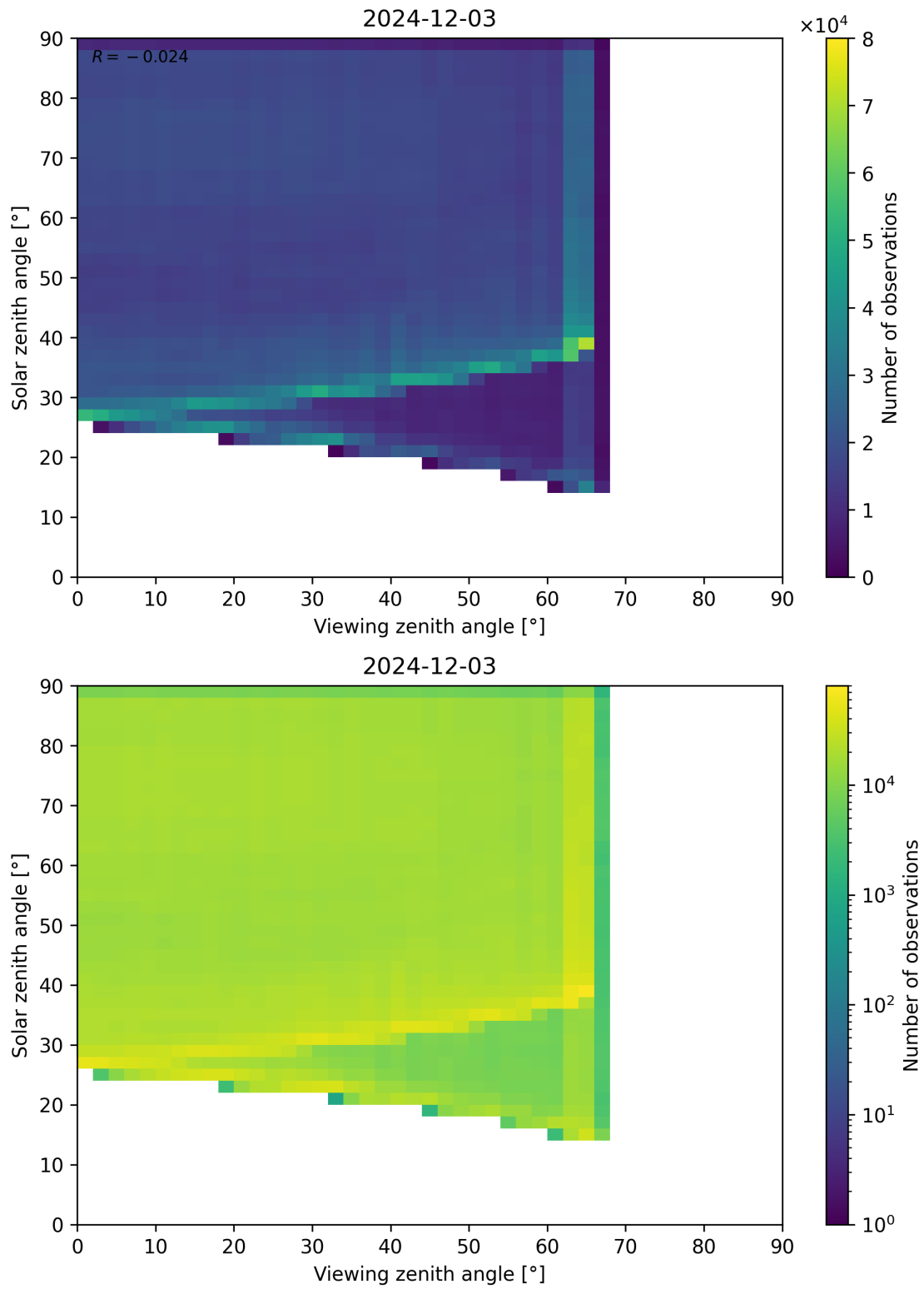
Figure 114: Scatter density plot of “Viewing zenith angle” against “Solar zenith angle” for 2024-12-02 to 2024-12-04.
