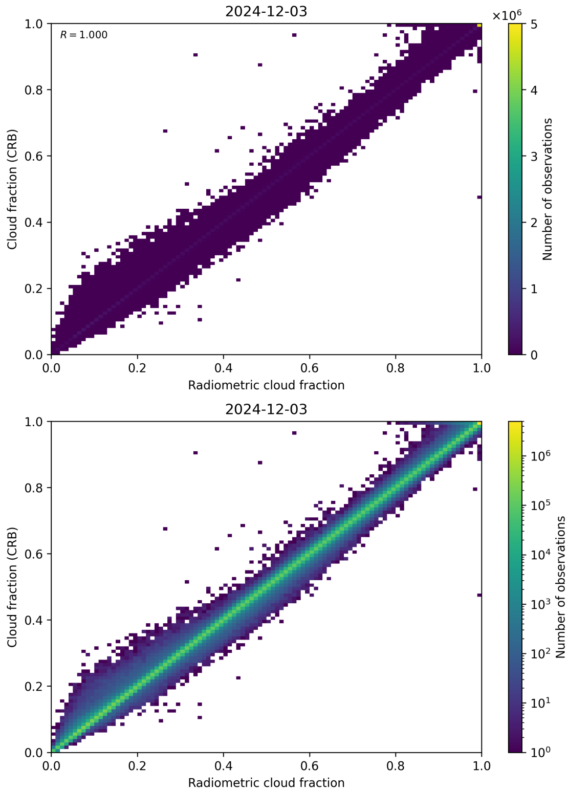
Figure 73: Scatter density plot of “Radiometric cloud fraction” against “Cloud fraction (CRB)” for 2024-12-02 to 2024-12-04.
