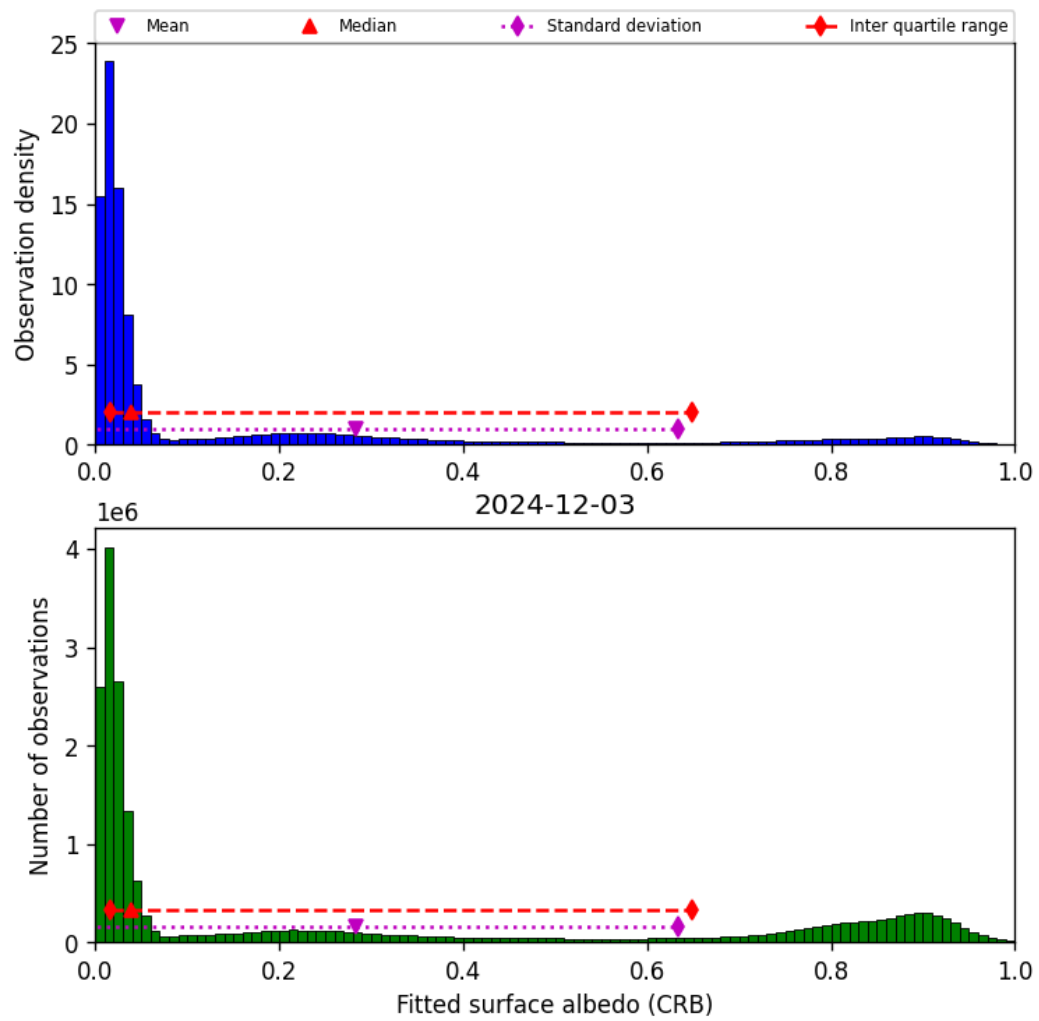
Figure 46: Histogram of “Fitted surface albedo (CRB)” for 2024-12-02 to 2024-12-04
