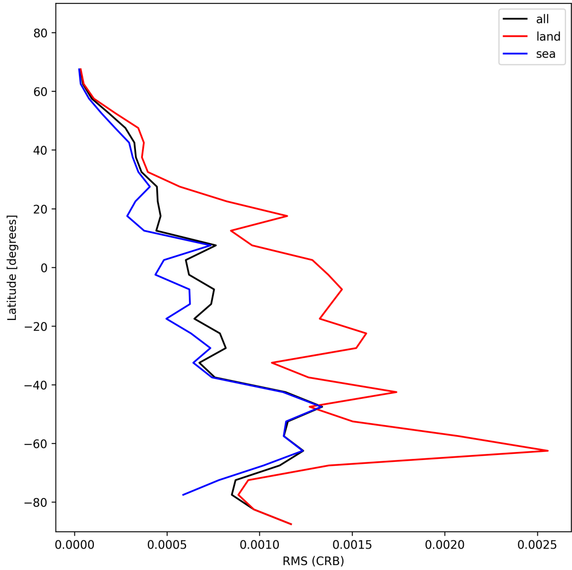
Figure 32: Zonal average of “RMS (CRB)” for 2024-12-02 to 2024-12-04.
