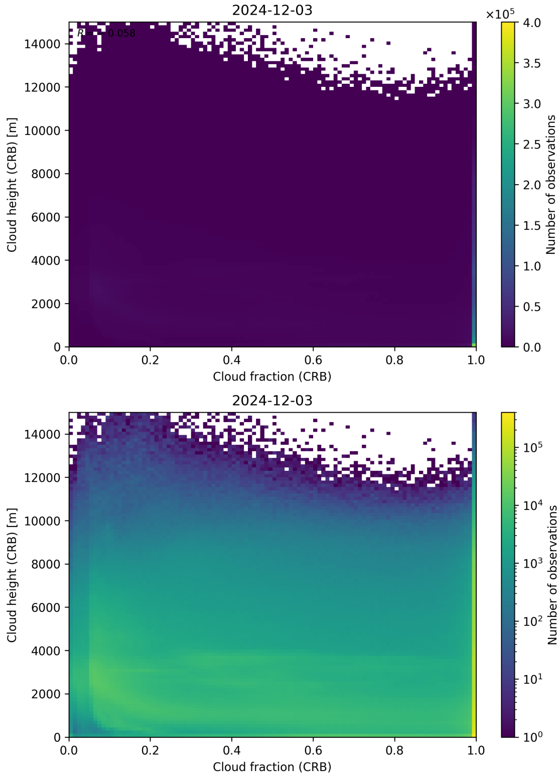
Figure 79: Scatter density plot of “Cloud fraction (CRB)” against “Cloud height (CRB)” for 2024-12-02 to 2024-12-04.
