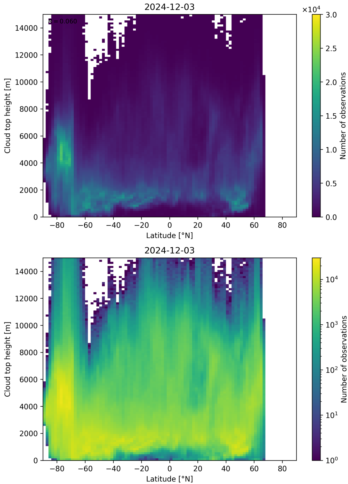
Figure 97: Scatter density plot of “Latitude” against “Cloud top height” for 2024-12-02 to 2024-12-04.
