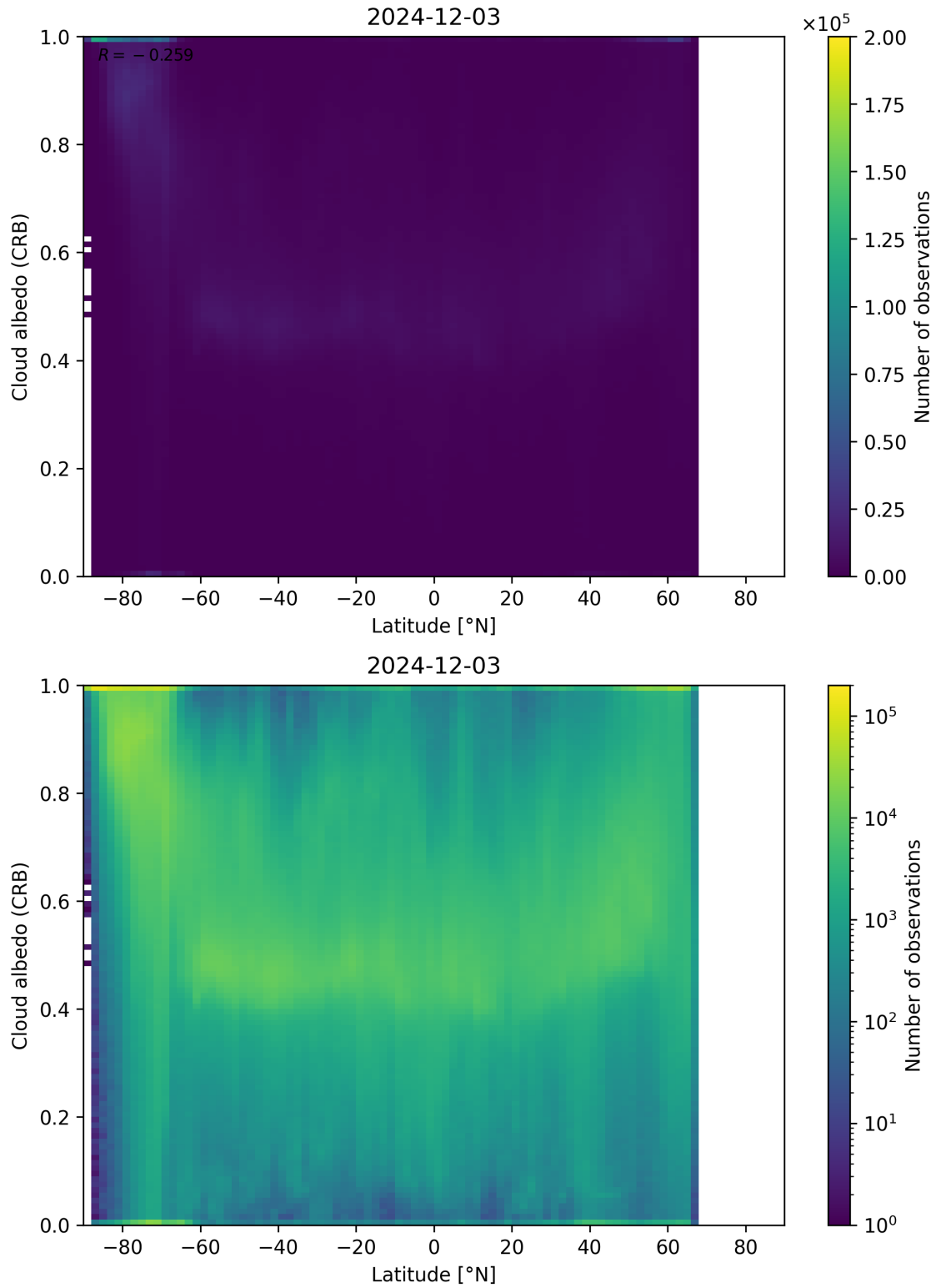
Figure 91: Scatter density plot of “Latitude” against “Cloud albedo (CRB)” for 2024-12-02 to 2024-12-04.
