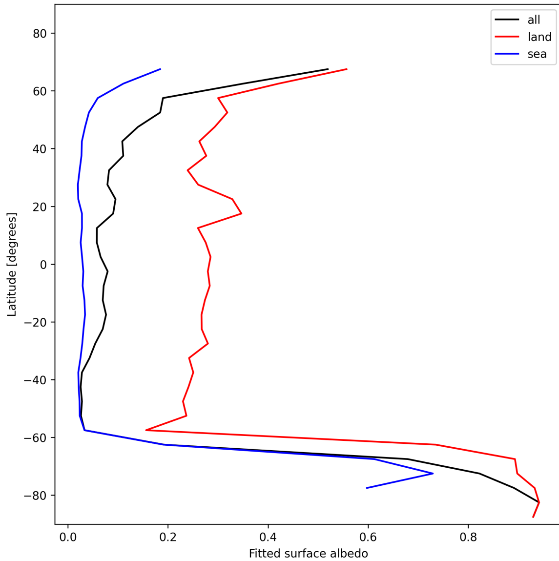
Figure 29: Zonal average of “Fitted surface albedo” for 2024-12-02 to 2024-12-04.
