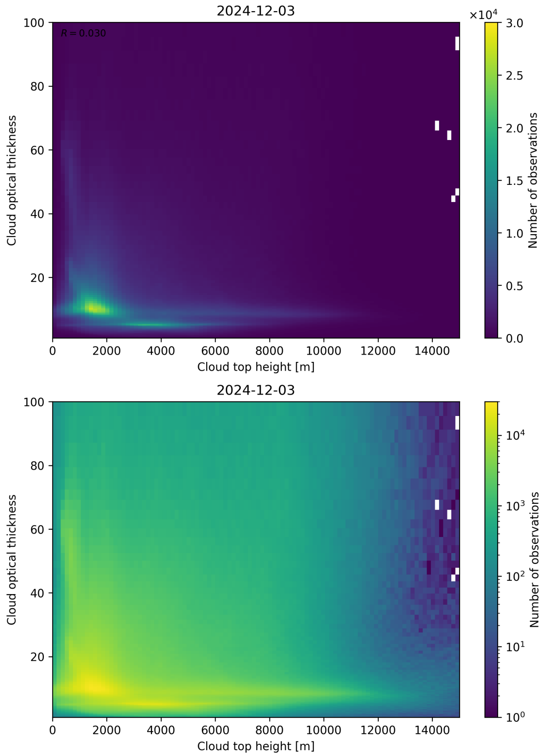
Figure 90: Scatter density plot of “Cloud top height” against “Cloud optical thickness” for 2024-12-02 to 2024-12-04.
