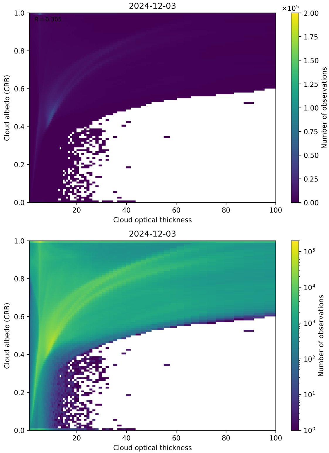
Figure 82: Scatter density plot of “Cloud optical thickness” against “Cloud albedo (CRB)” for 2024-12-02 to 2024-12-04.
