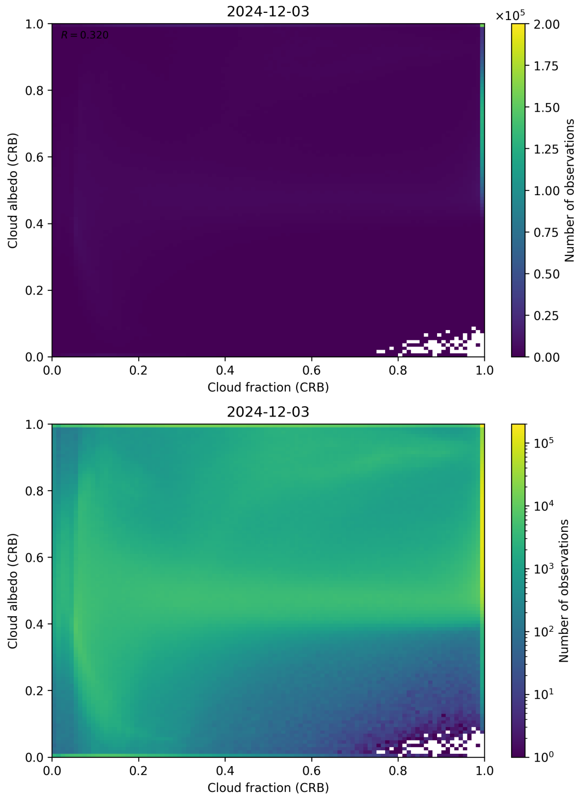
Figure 77: Scatter density plot of “Cloud fraction (CRB)” against “Cloud albedo (CRB)” for 2024-12-02 to 2024-12-04.
