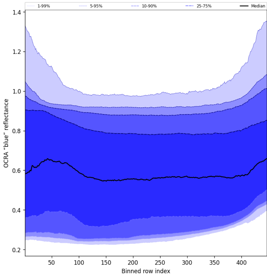
Figure 67: Along track statistics of “OCRA “blue” reflectance” for 2024-12-02 to 2024-12-04
