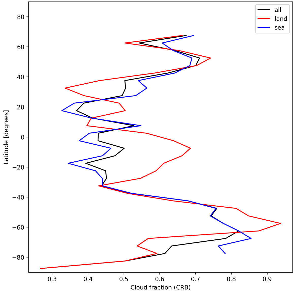
Figure 26: Zonal average of “Cloud fraction (CRB)” for 2024-12-02 to 2024-12-04.
