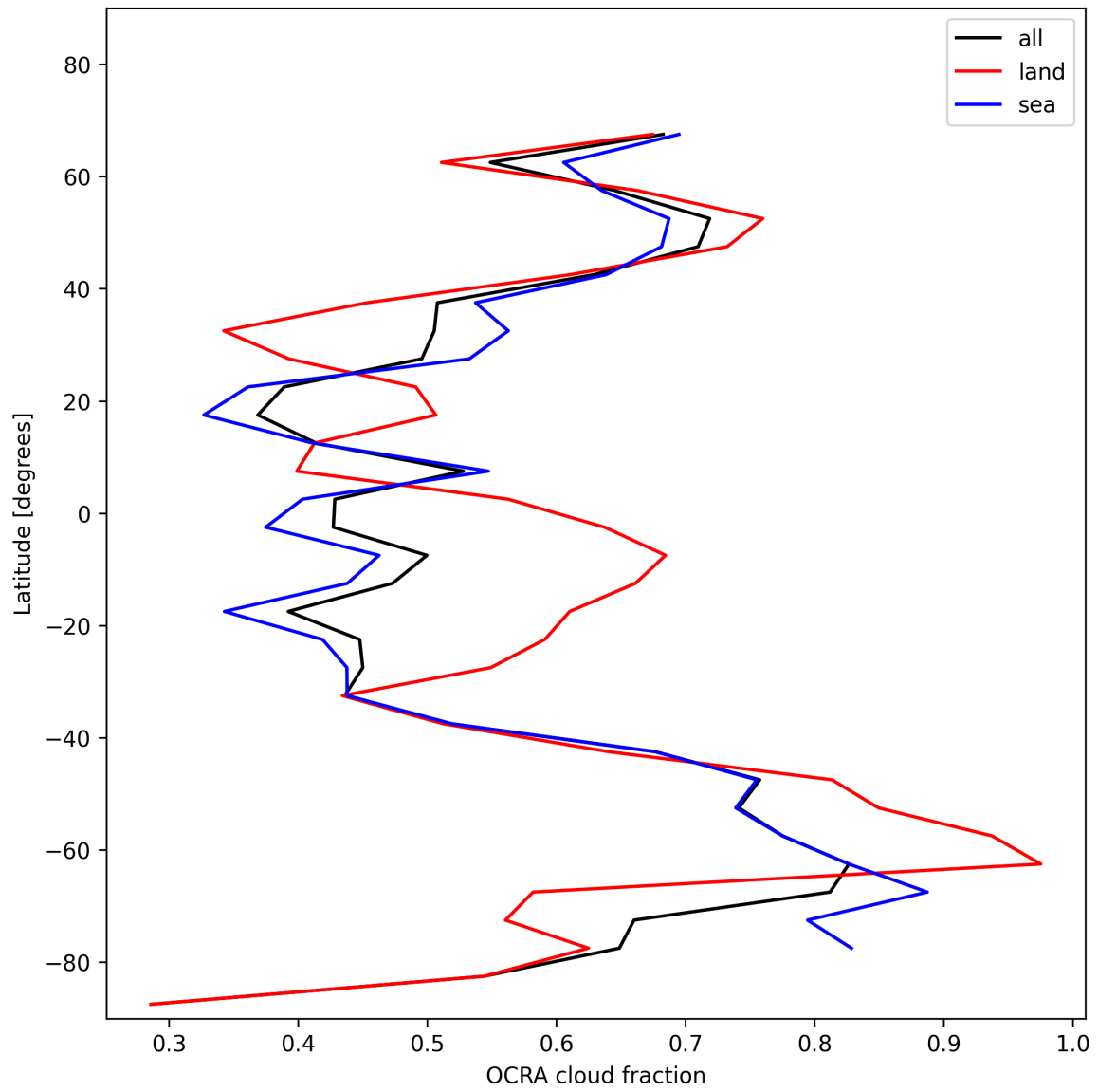
Figure 34: Zonal average of “OCRA cloud fraction” for 2024-12-02 to 2024-12-04.
