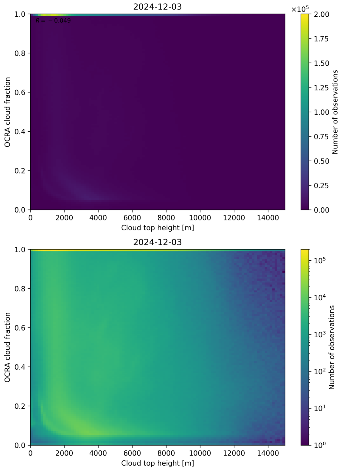
Figure 87: Scatter density plot of “Cloud top height” against “OCRA cloud fraction” for 2024-12-02 to 2024-12-04.
