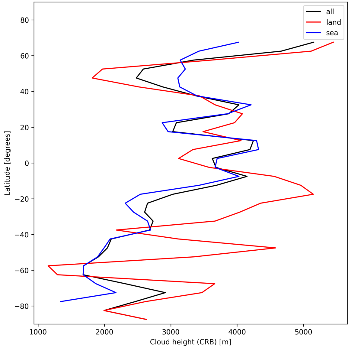
Figure 27: Zonal average of “Cloud height (CRB)” for 2024-12-02 to 2024-12-04.
