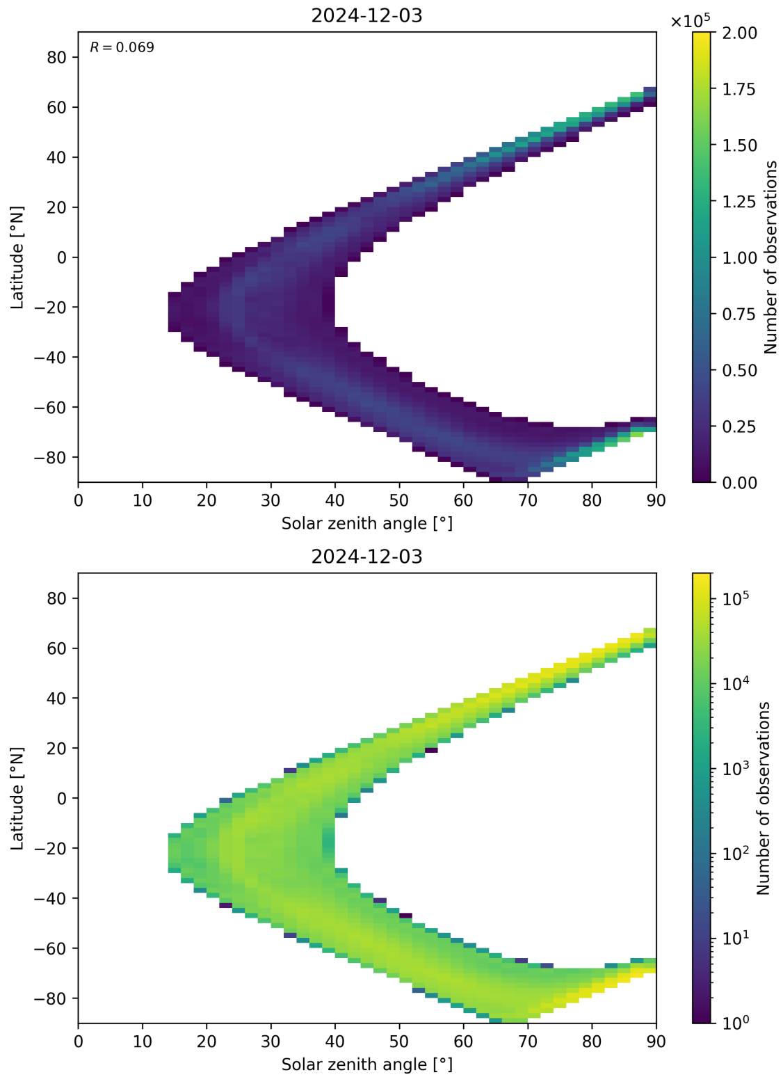
Figure 105: Scatter density plot of “Solar zenith angle” against “Latitude” for 2024-12-02 to 2024-12-04.
