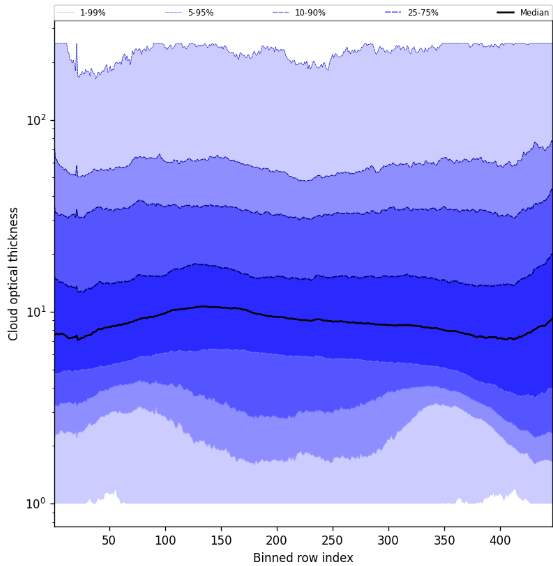
Figure 57: Along track statistics of “Cloud optical thickness” for 2024-12-02 to 2024-12-04
