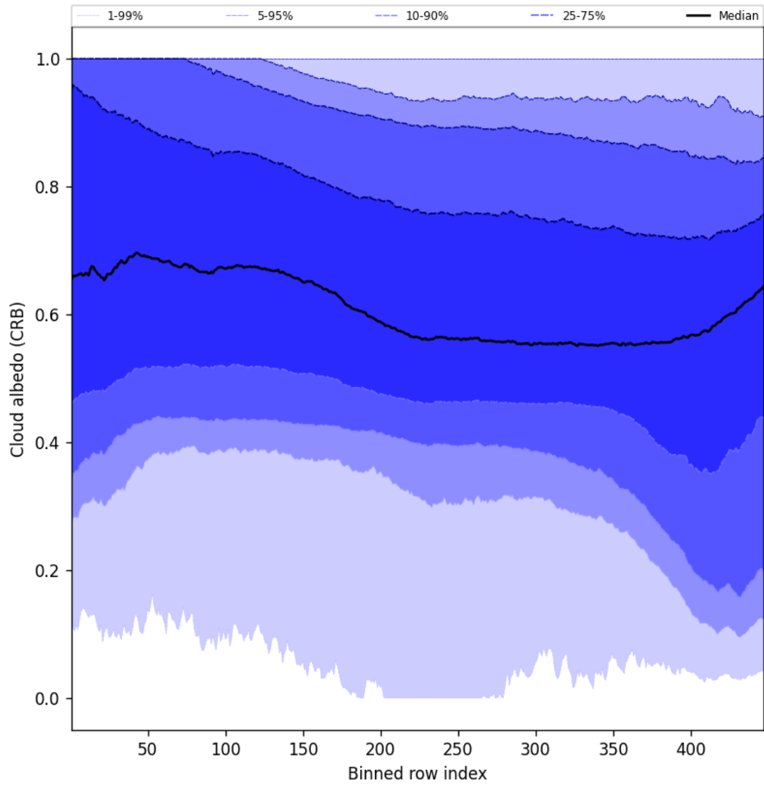
Figure 60: Along track statistics of “Cloud albedo (CRB)” for 2024-12-02 to 2024-12-04
