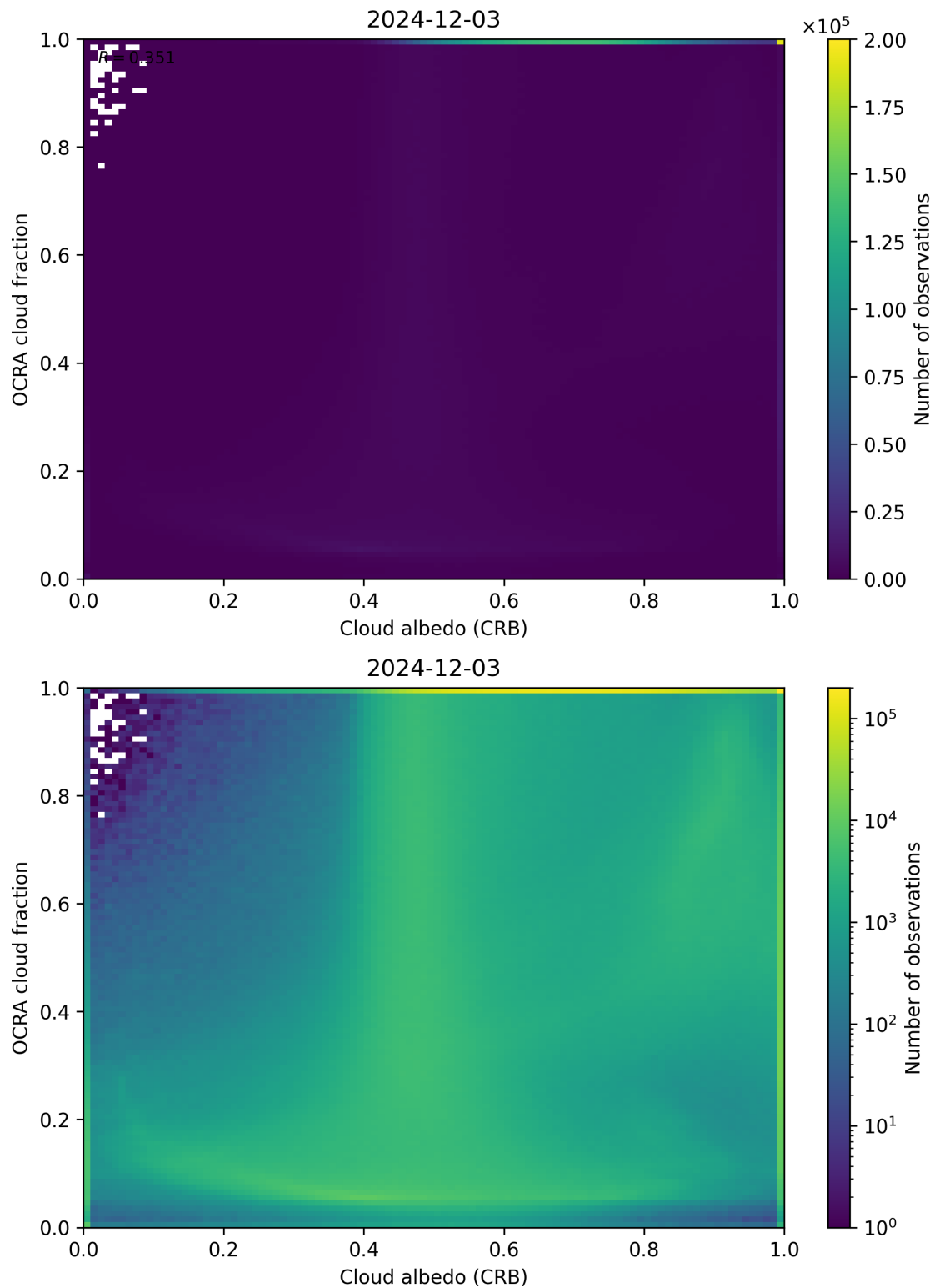
Figure 70: Scatter density plot of “Cloud albedo (CRB)” against “OCRA cloud fraction” for 2024-12-02 to 2024-12-04.
