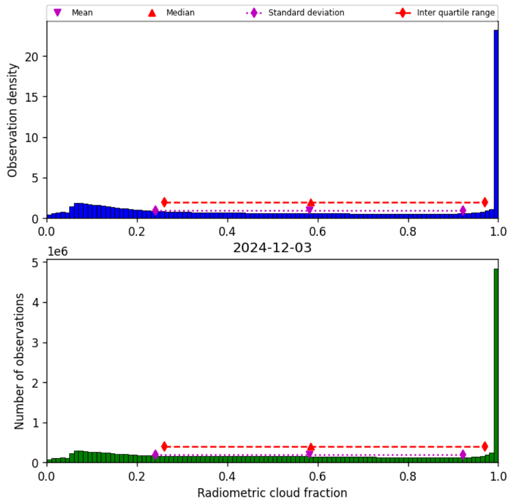
Figure 39: Histogram of “Radiometric cloud fraction” for 2024-12-02 to 2024-12-04
