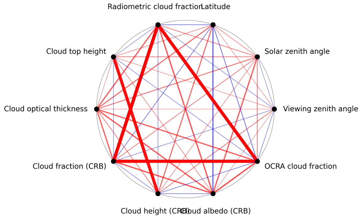
Figure 1: Map of correlation graph for 2024-12-02 to 2024-12-04.
