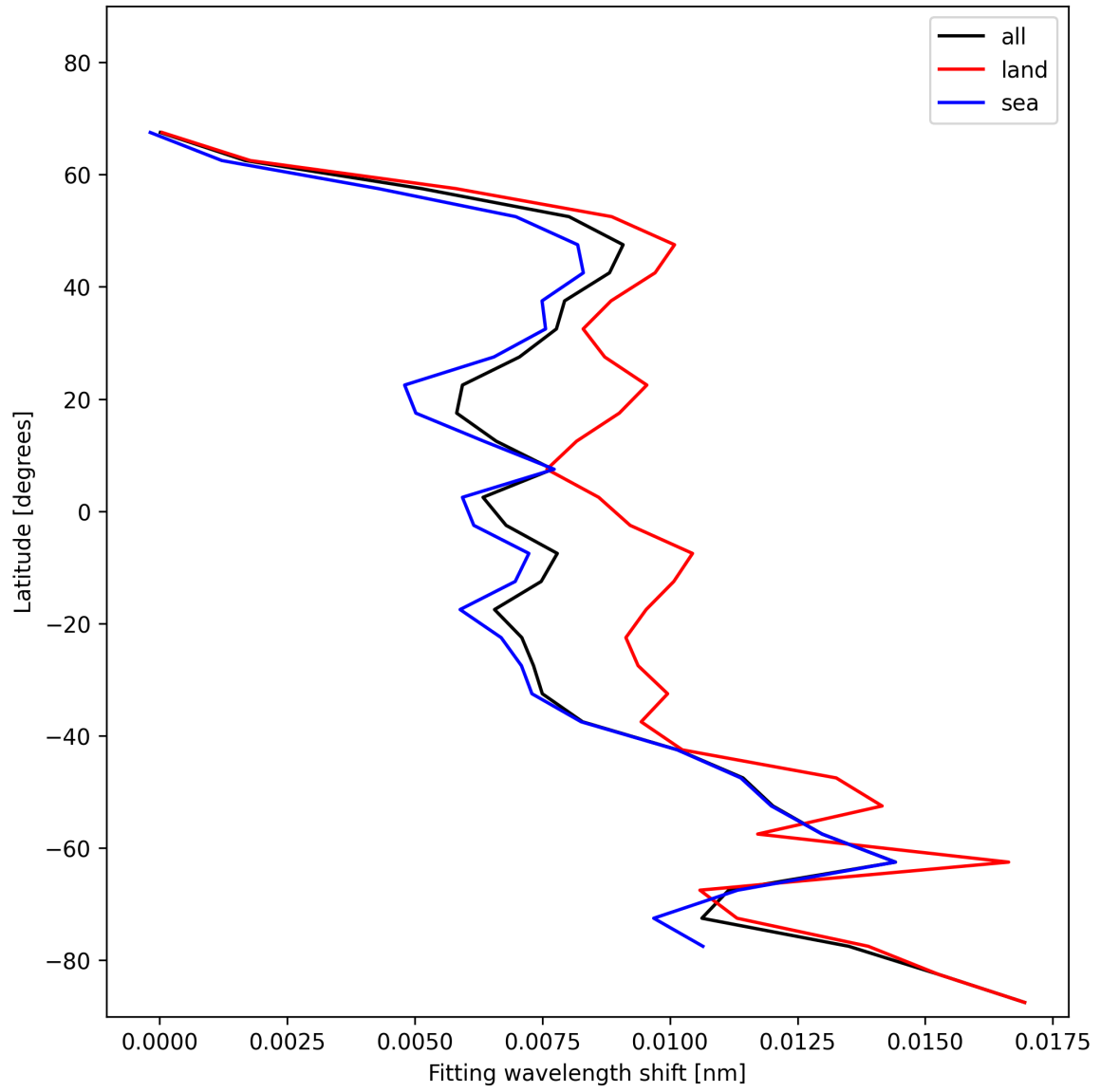
Figure 33: Zonal average of “Fitting wavelength shift” for 2024-12-02 to 2024-12-04.
