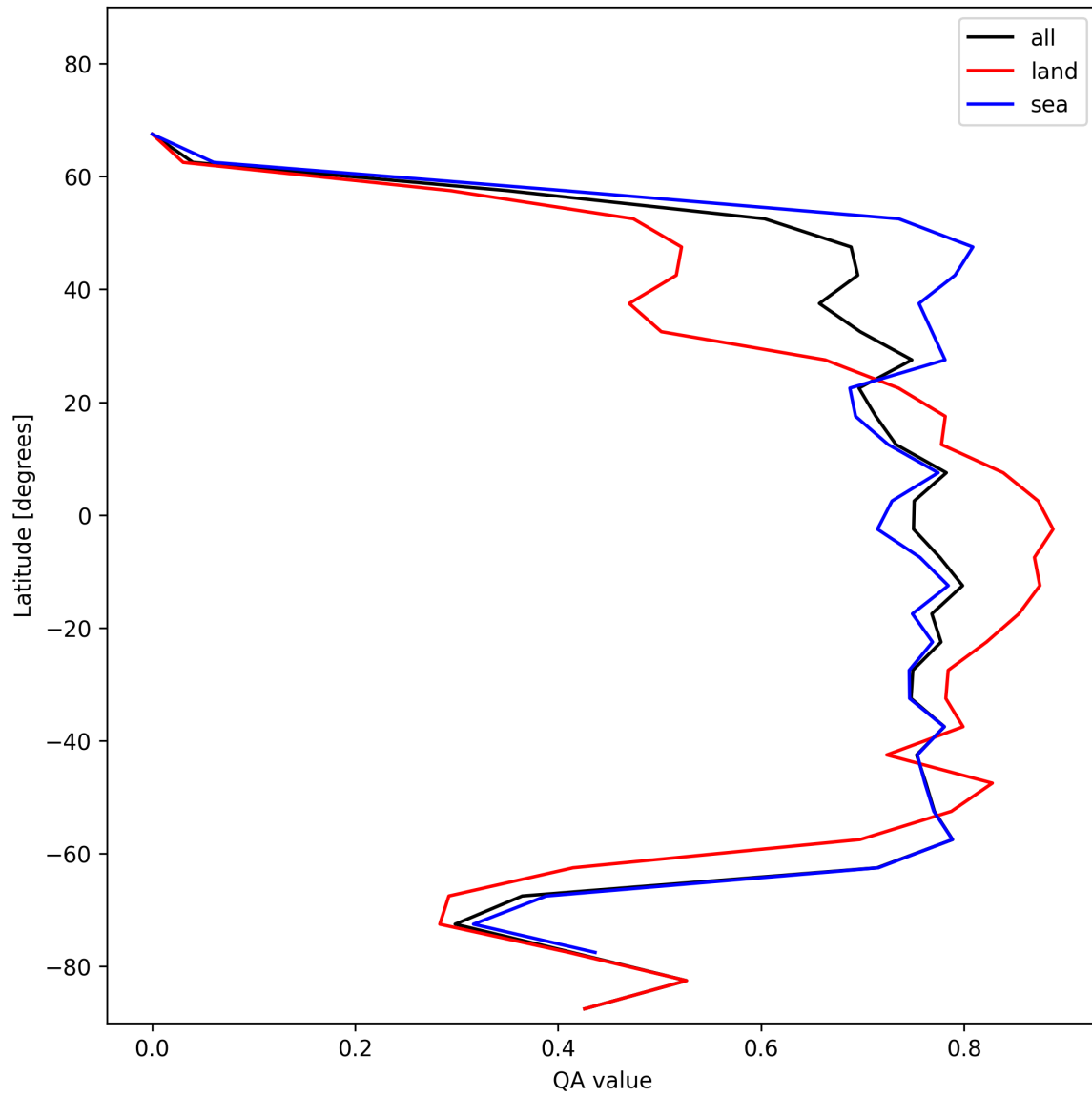
Figure 22: Zonal average of “QA value” for 2024-12-02 to 2024-12-04.
