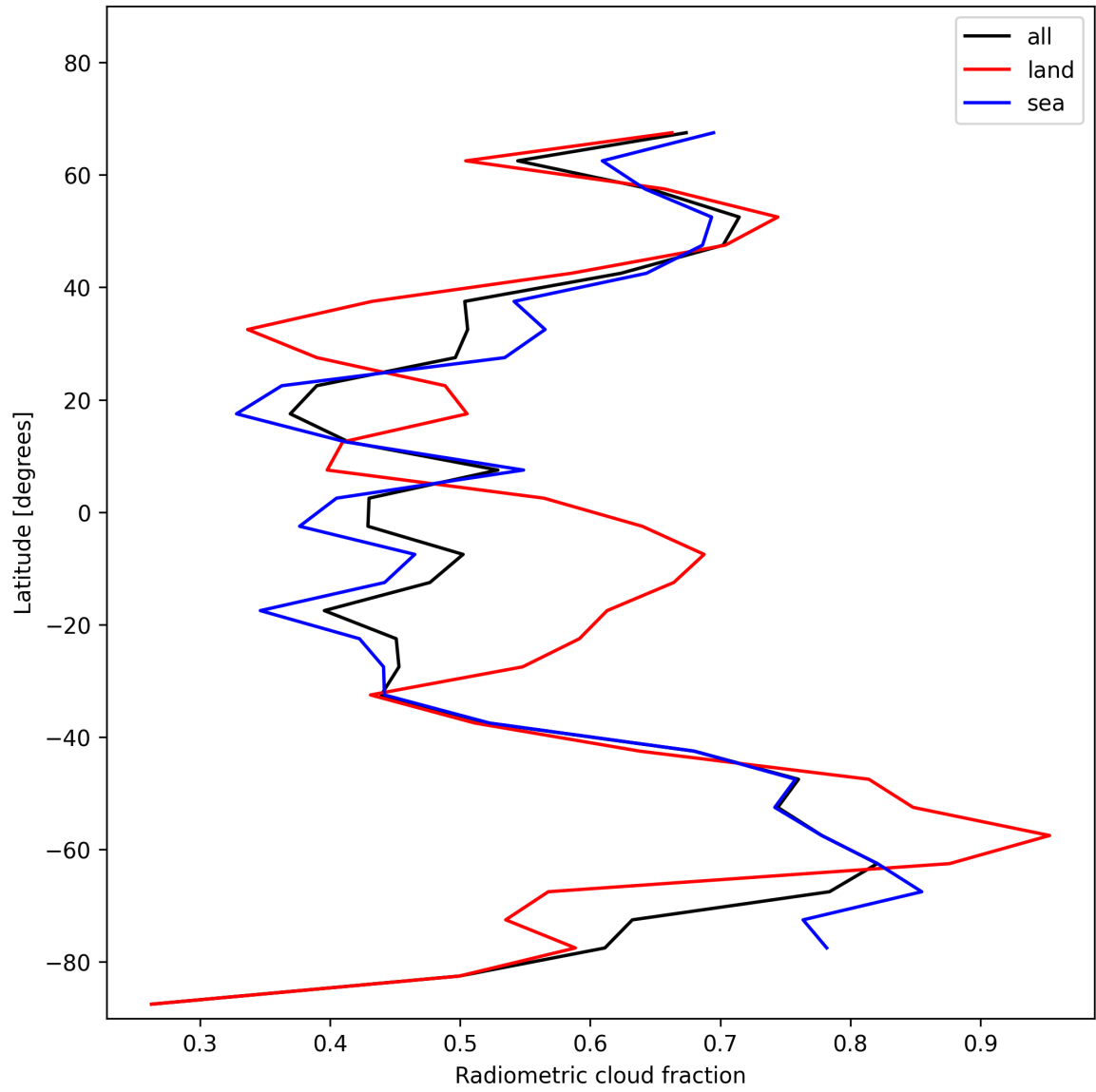
Figure 23: Zonal average of “Radiometric cloud fraction” for 2024-12-02 to 2024-12-04.
