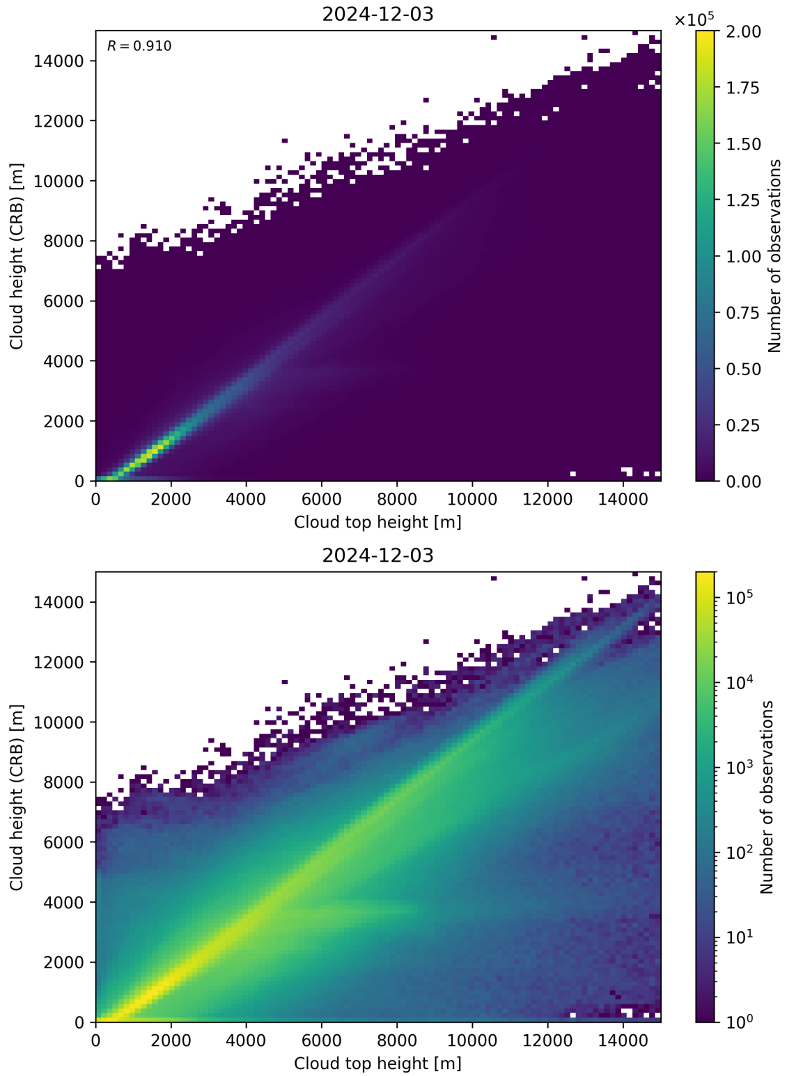
Figure 89: Scatter density plot of “Cloud top height” against “Cloud height (CRB)” for 2024-12-02 to 2024-12-04.
