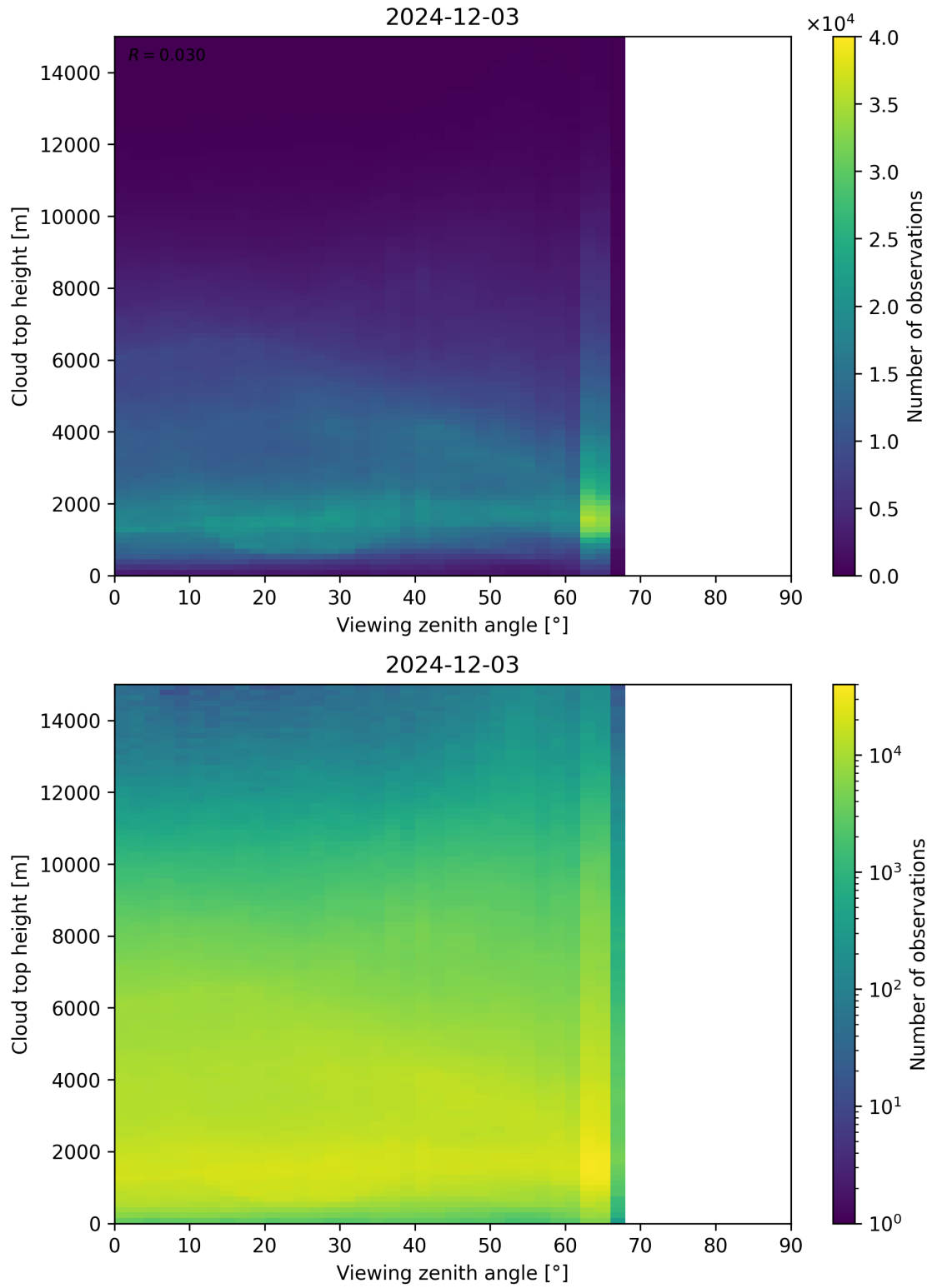
Figure 112: Scatter density plot of “Viewing zenith angle” against “Cloud top height” for 2024-12-02 to 2024-12-04.
