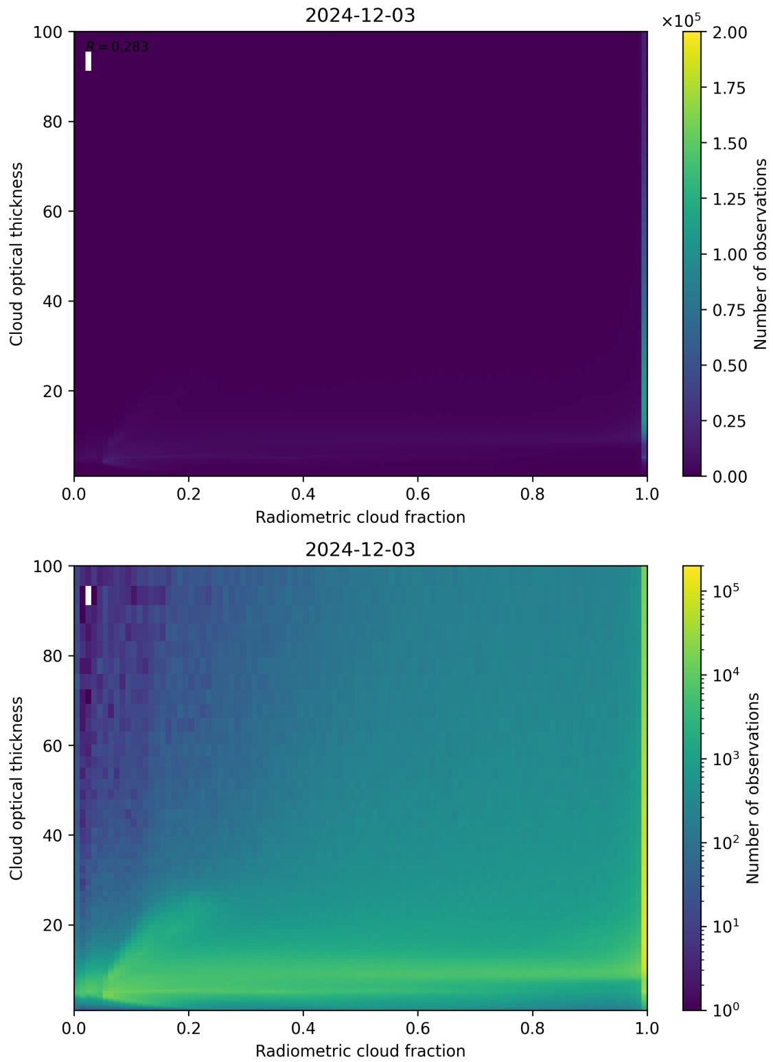
Figure 75: Scatter density plot of “Radiometric cloud fraction” against “Cloud optical thickness” for 2024-12-02 to 2024-12-04.
