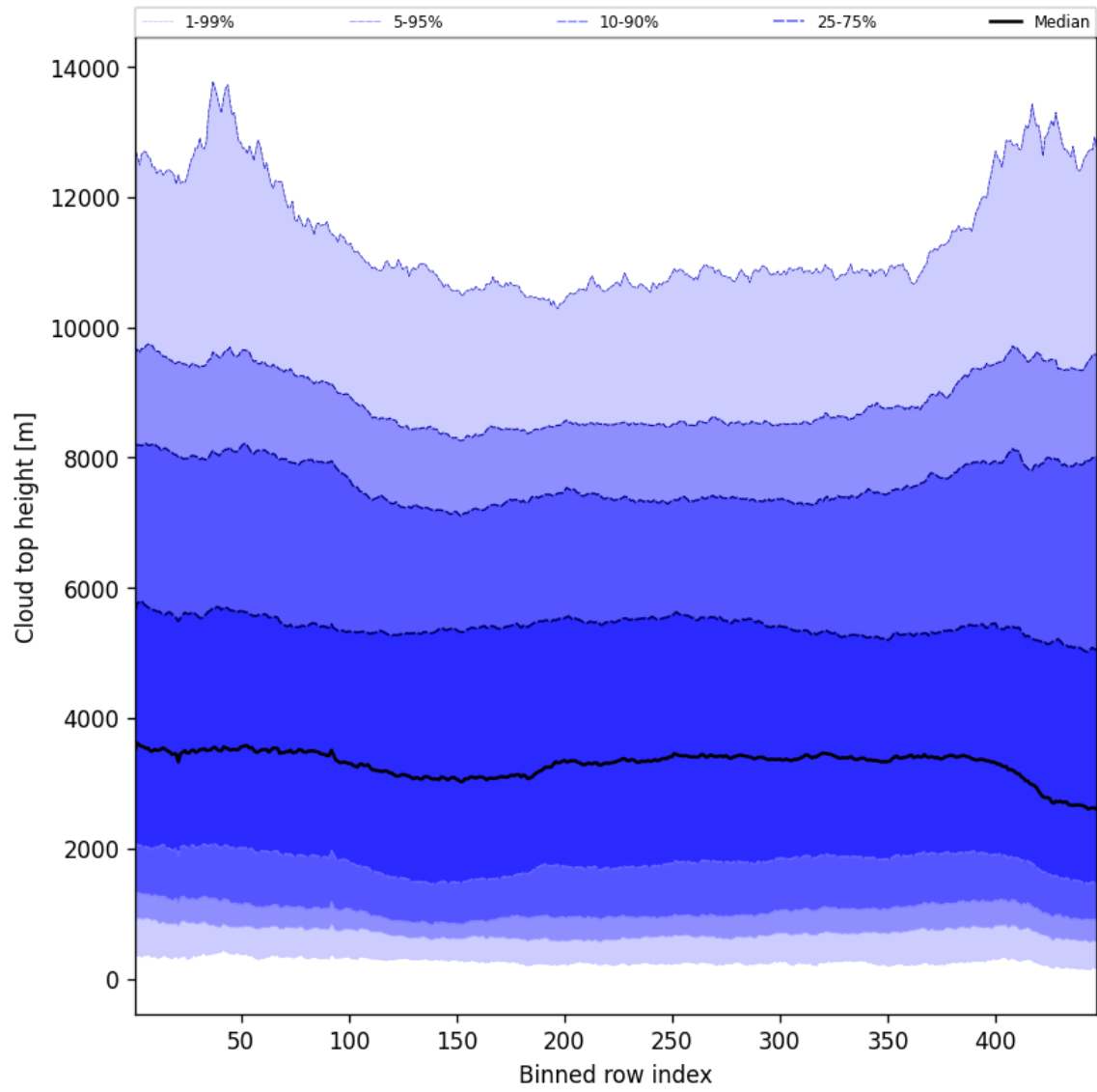
Figure 56: Along track statistics of “Cloud top height” for 2024-12-02 to 2024-12-04
