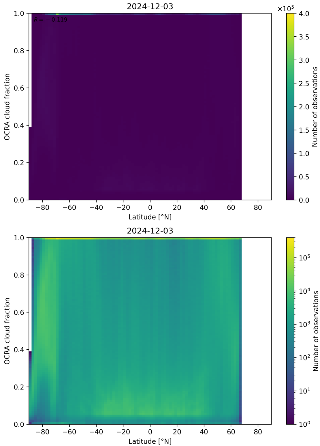
Figure 93: Scatter density plot of “Latitude” against “OCRA cloud fraction” for 2024-12-02 to 2024-12-04.
