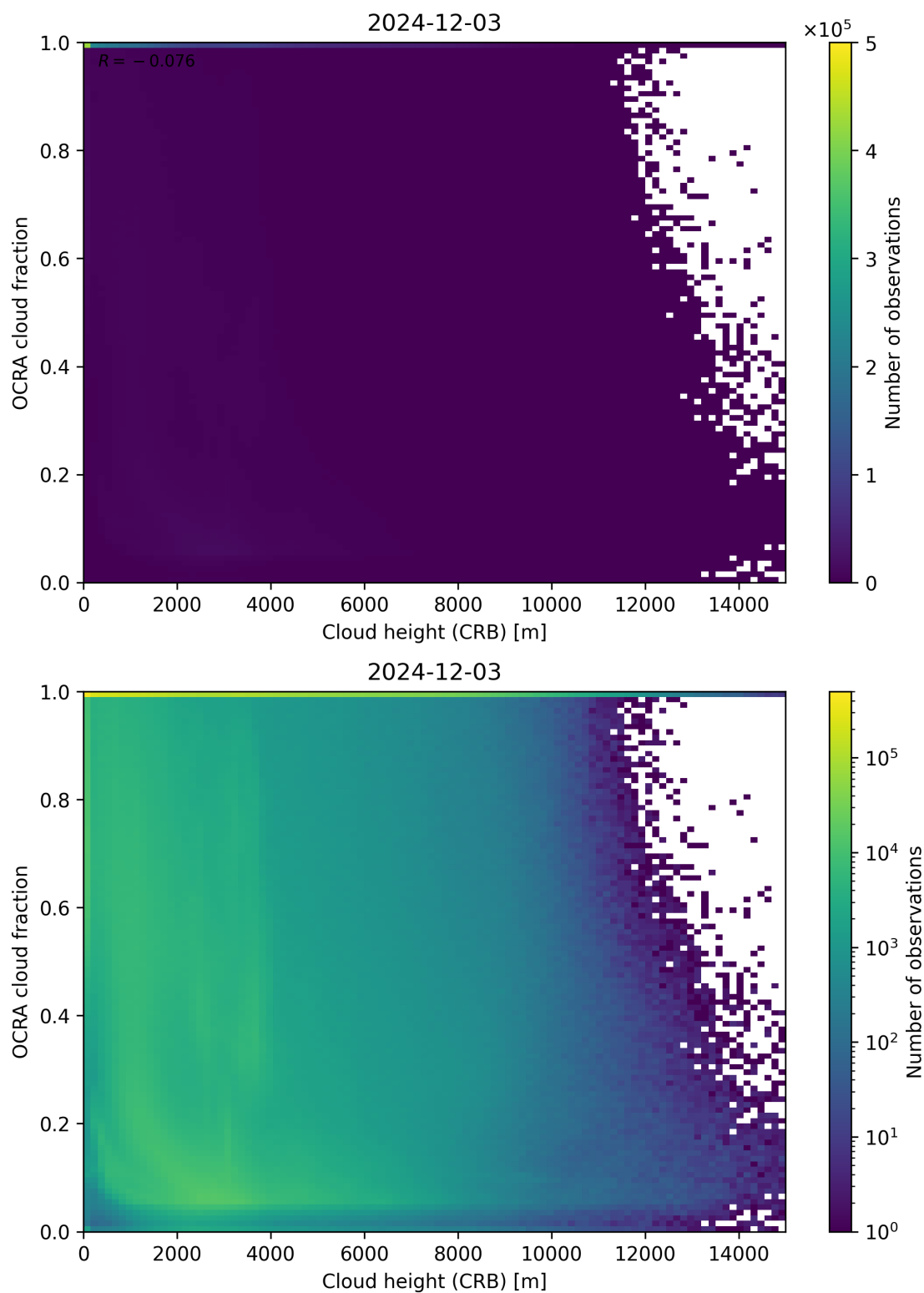
Figure 81: Scatter density plot of “Cloud height (CRB)” against “OCRA cloud fraction” for 2024-12-02 to 2024-12-04.
