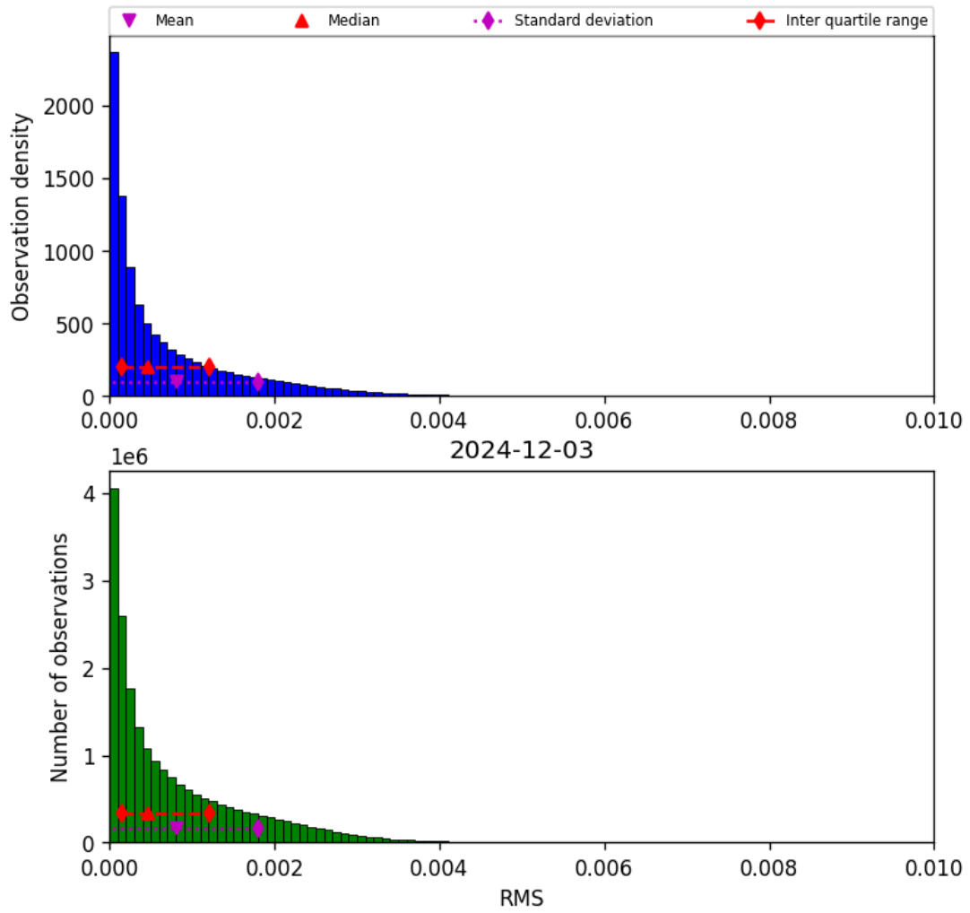
Figure 47: Histogram of “RMS” for 2024-12-02 to 2024-12-04
