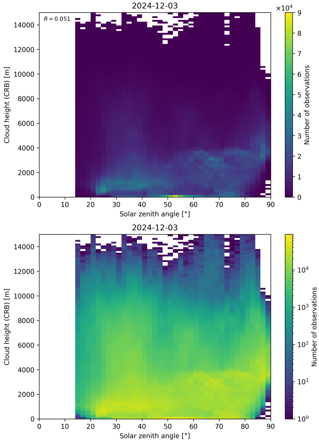
Figure 102: Scatter density plot of “Solar zenith angle” against “Cloud height (CRB)” for 2024-12-02 to 2024-12-04.
