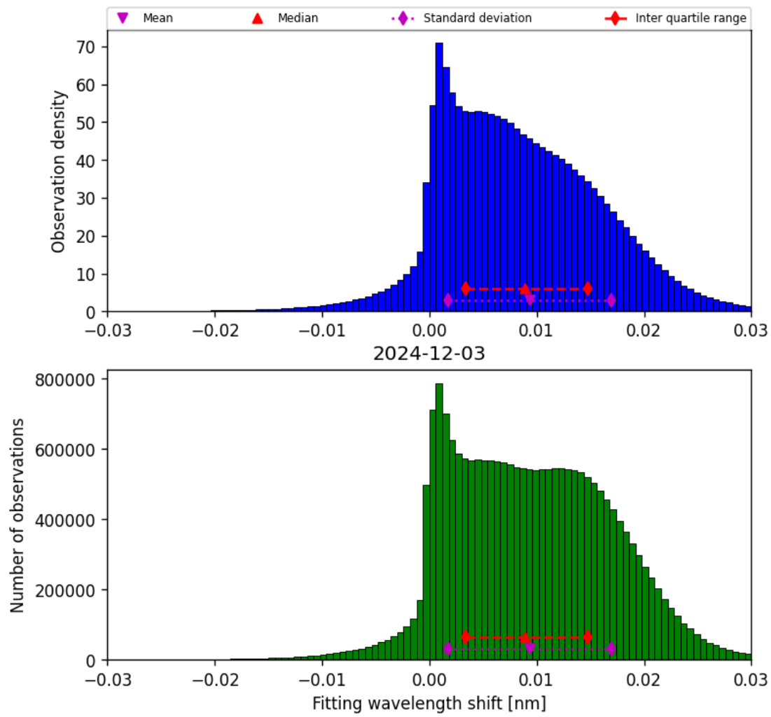
Figure 49: Histogram of “Fitting wavelength shift” for 2024-12-02 to 2024-12-04
