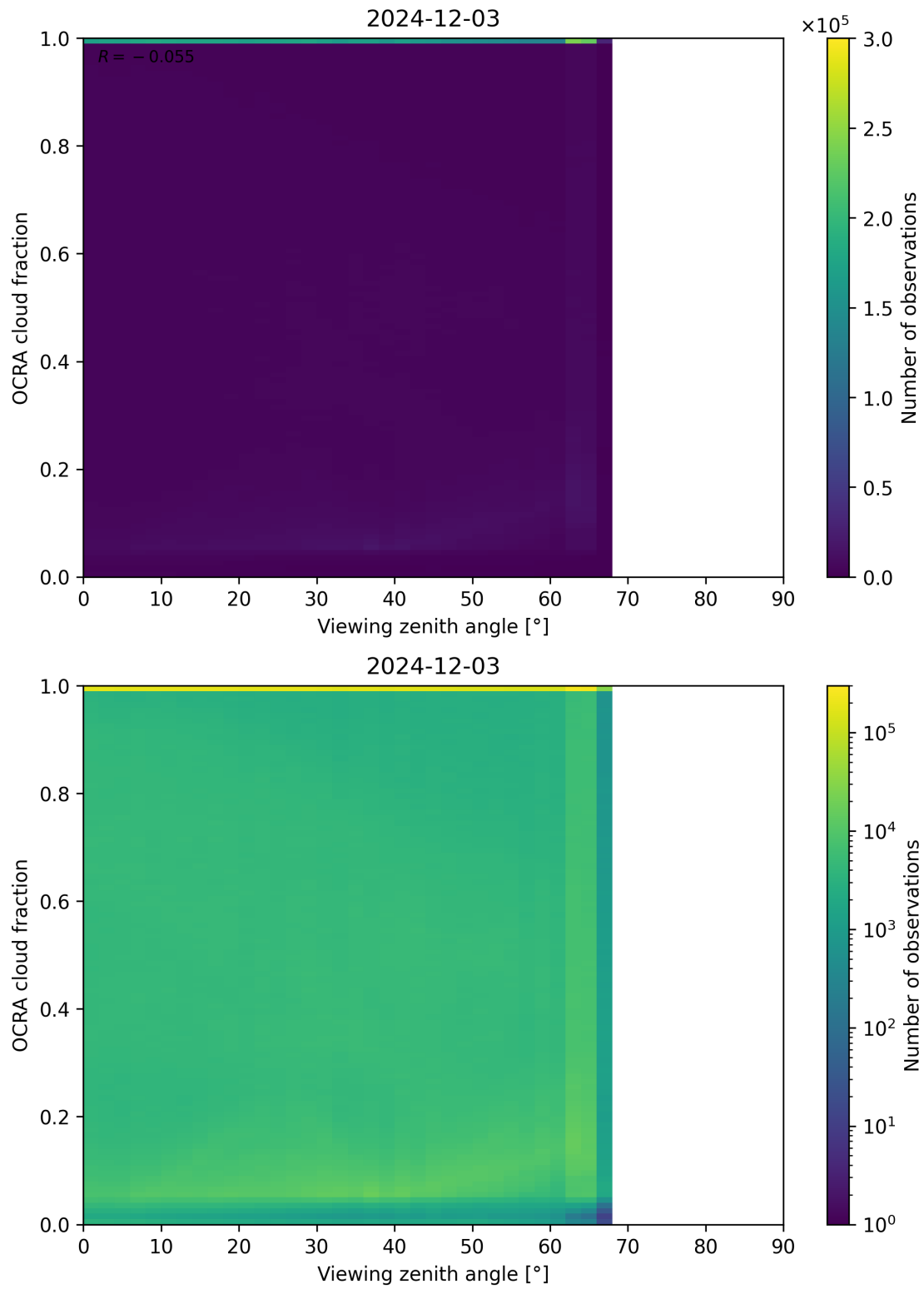
Figure 108: Scatter density plot of “Viewing zenith angle” against “OCRA cloud fraction” for 2024-12-02 to 2024-12-04.
