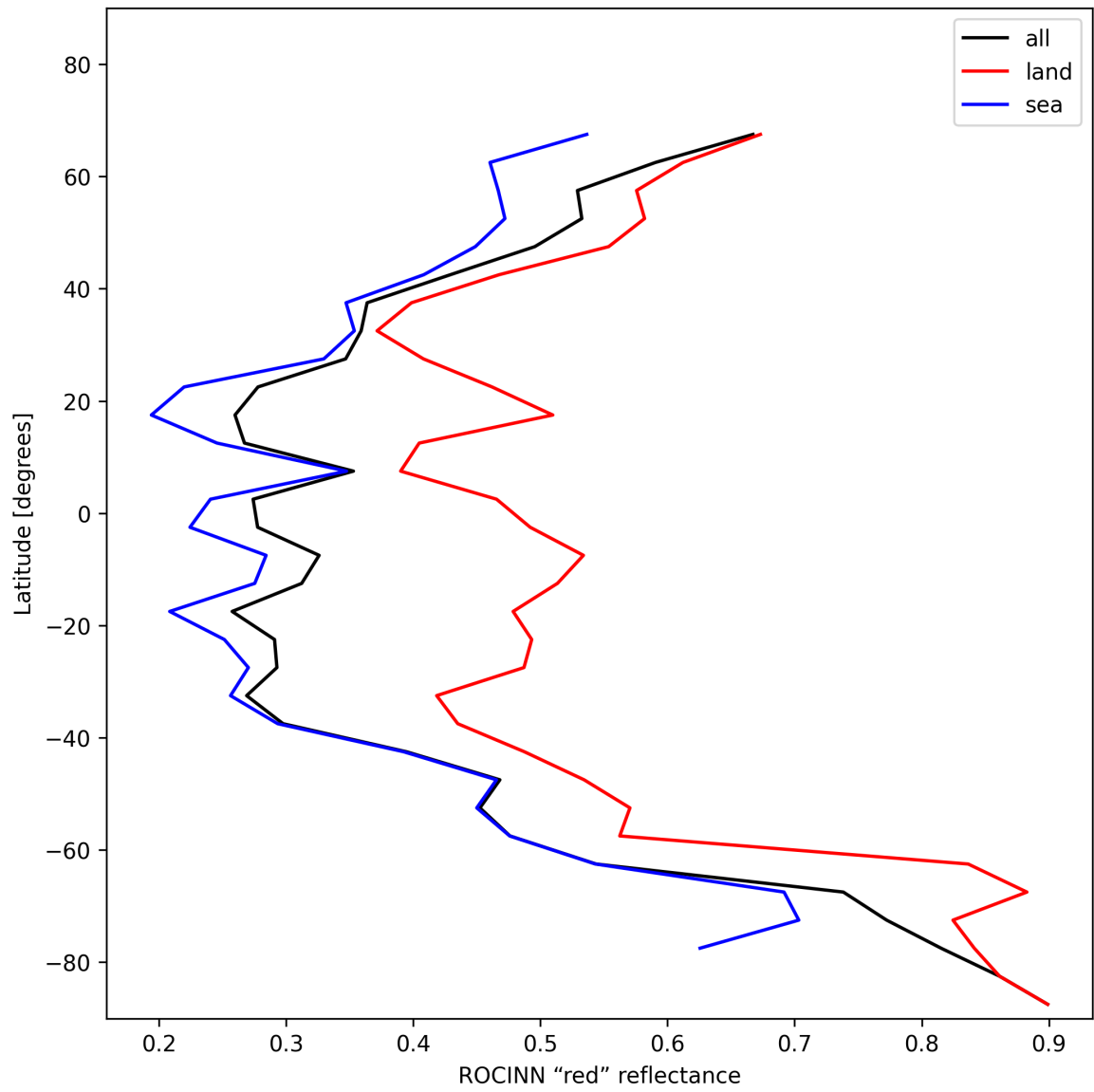
Figure 37: Zonal average of “ROCINN “red” reflectance” for 2024-12-02 to 2024-12-04.
