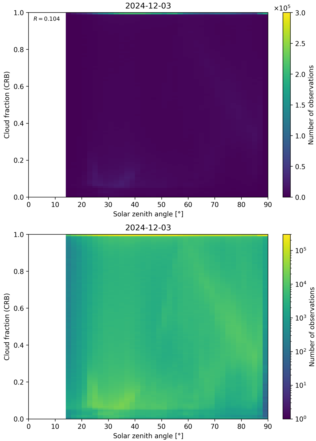
Figure 101: Scatter density plot of “Solar zenith angle” against “Cloud fraction (CRB)” for 2024-12-02 to 2024-12-04.
