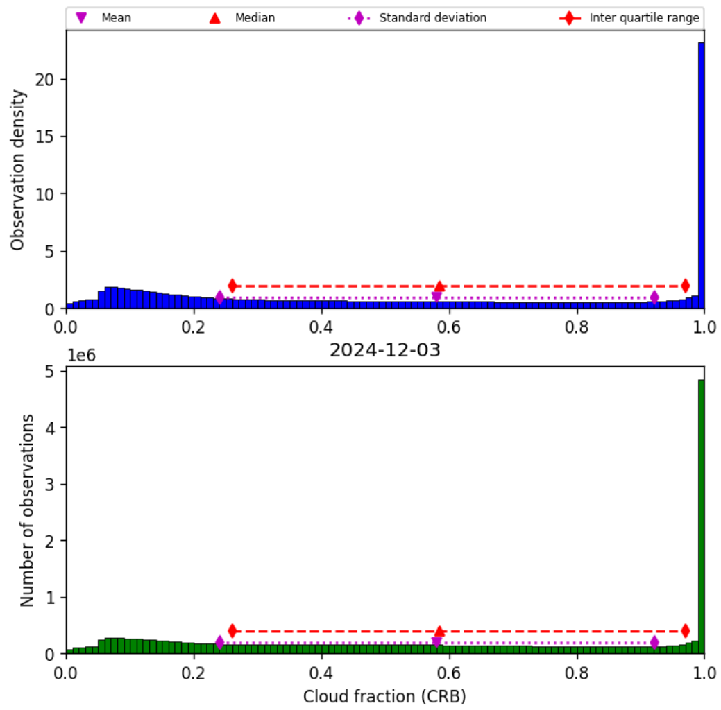
Figure 42: Histogram of “Cloud fraction (CRB)” for 2024-12-02 to 2024-12-04
