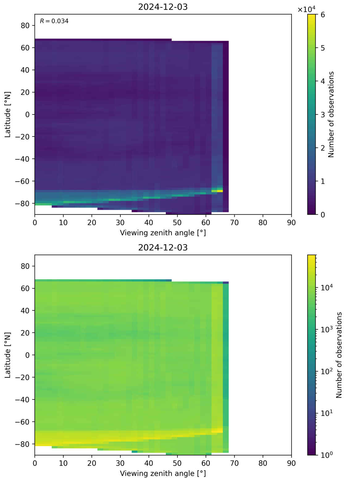
Figure 113: Scatter density plot of “Viewing zenith angle” against “Latitude” for 2024-12-02 to 2024-12-04.
