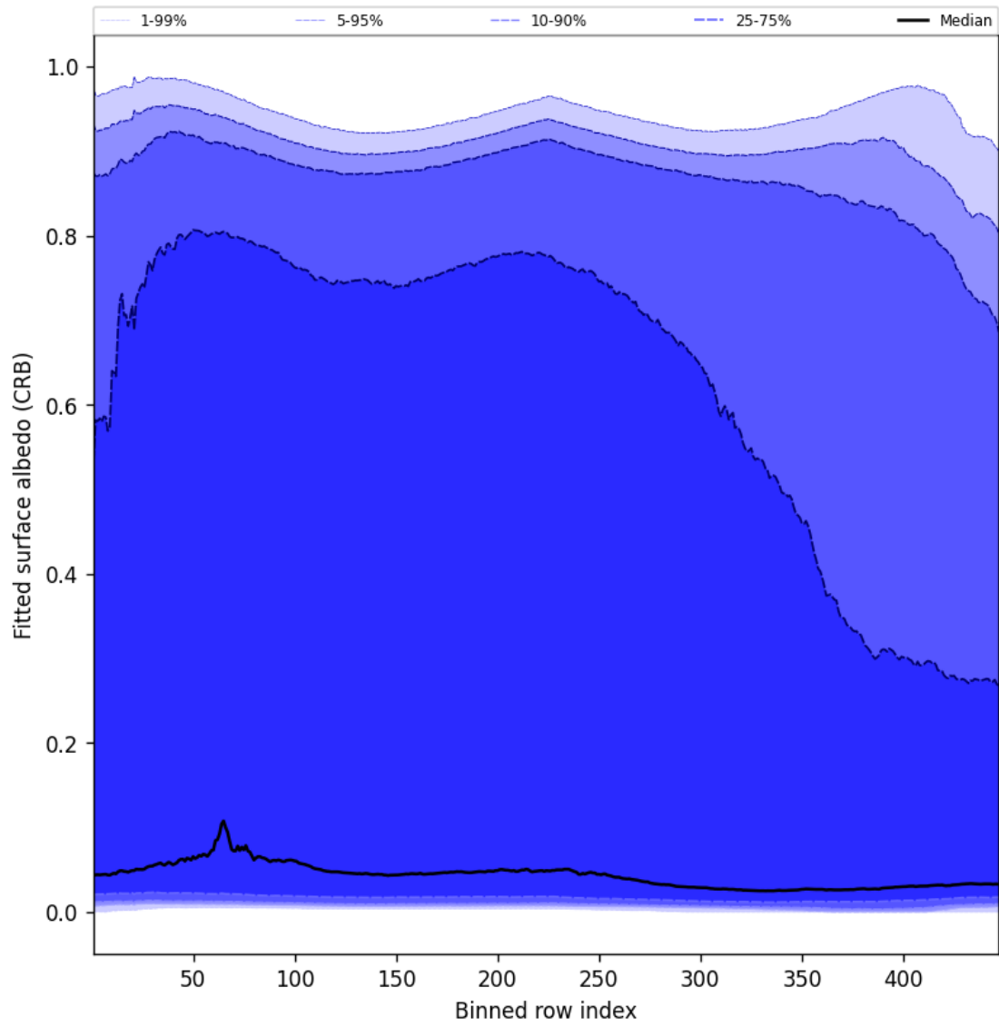
Figure 62: Along track statistics of “Fitted surface albedo (CRB)” for 2024-12-02 to 2024-12-04
