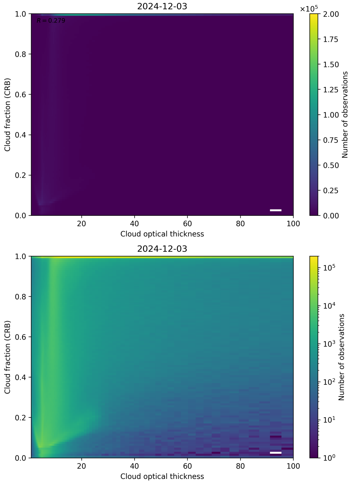
Figure 84: Scatter density plot of “Cloud optical thickness” against “Cloud fraction (CRB)” for 2024-12-02 to 2024-12-04.
