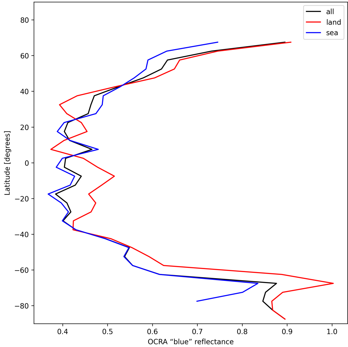
Figure 35: Zonal average of "OCRA "blue" reflectance" for 2024-12-02 to 2024-12-04.
