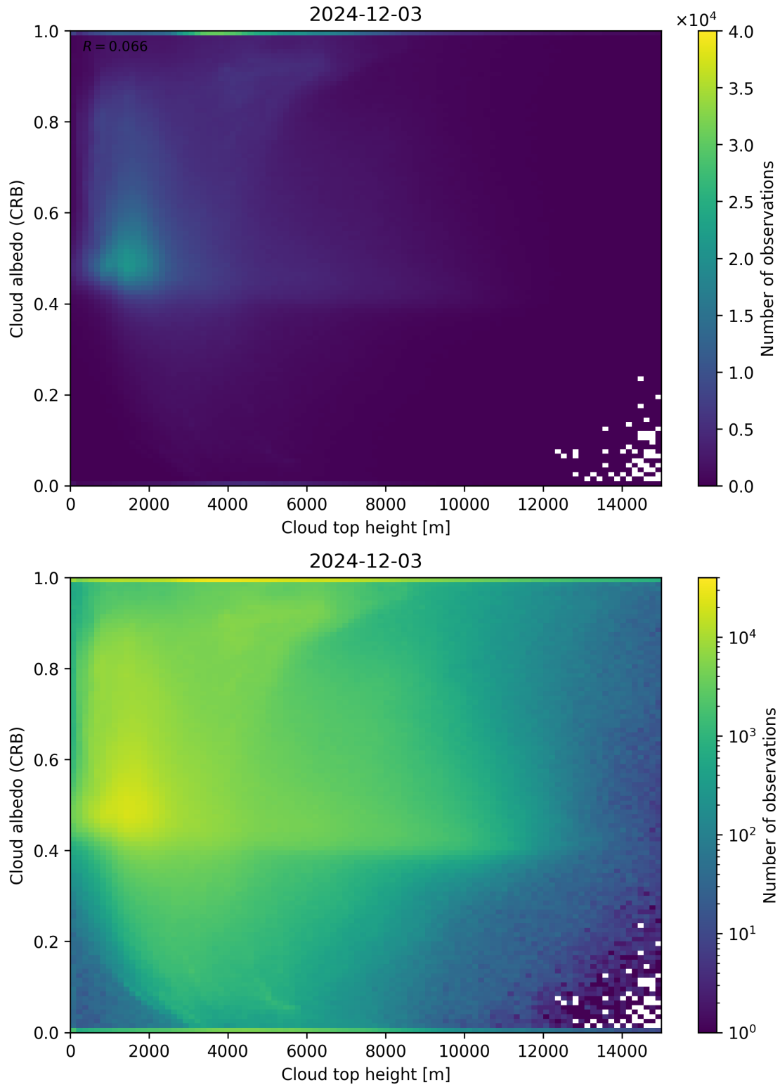
Figure 86: Scatter density plot of “Cloud top height” against “Cloud albedo (CRB)” for 2024-12-02 to 2024-12-04.
