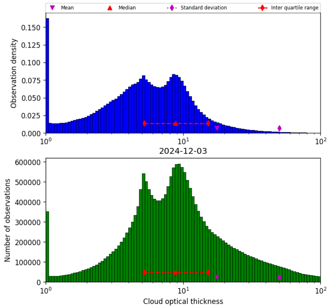
Figure 41: Histogram of “Cloud optical thickness” for 2024-12-02 to 2024-12-04
