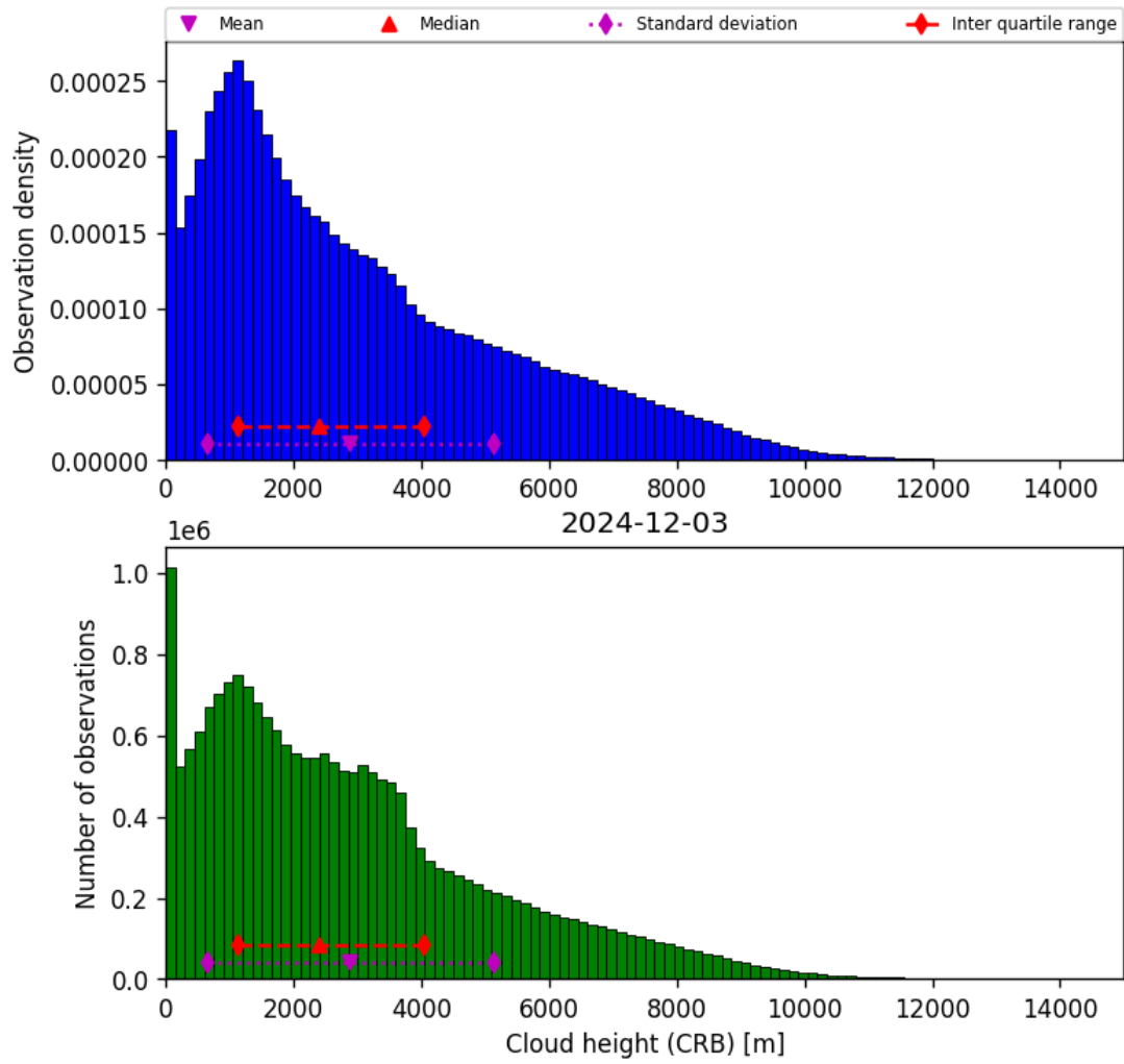
Figure 43: Histogram of “Cloud height (CRB)” for 2024-12-02 to 2024-12-04
