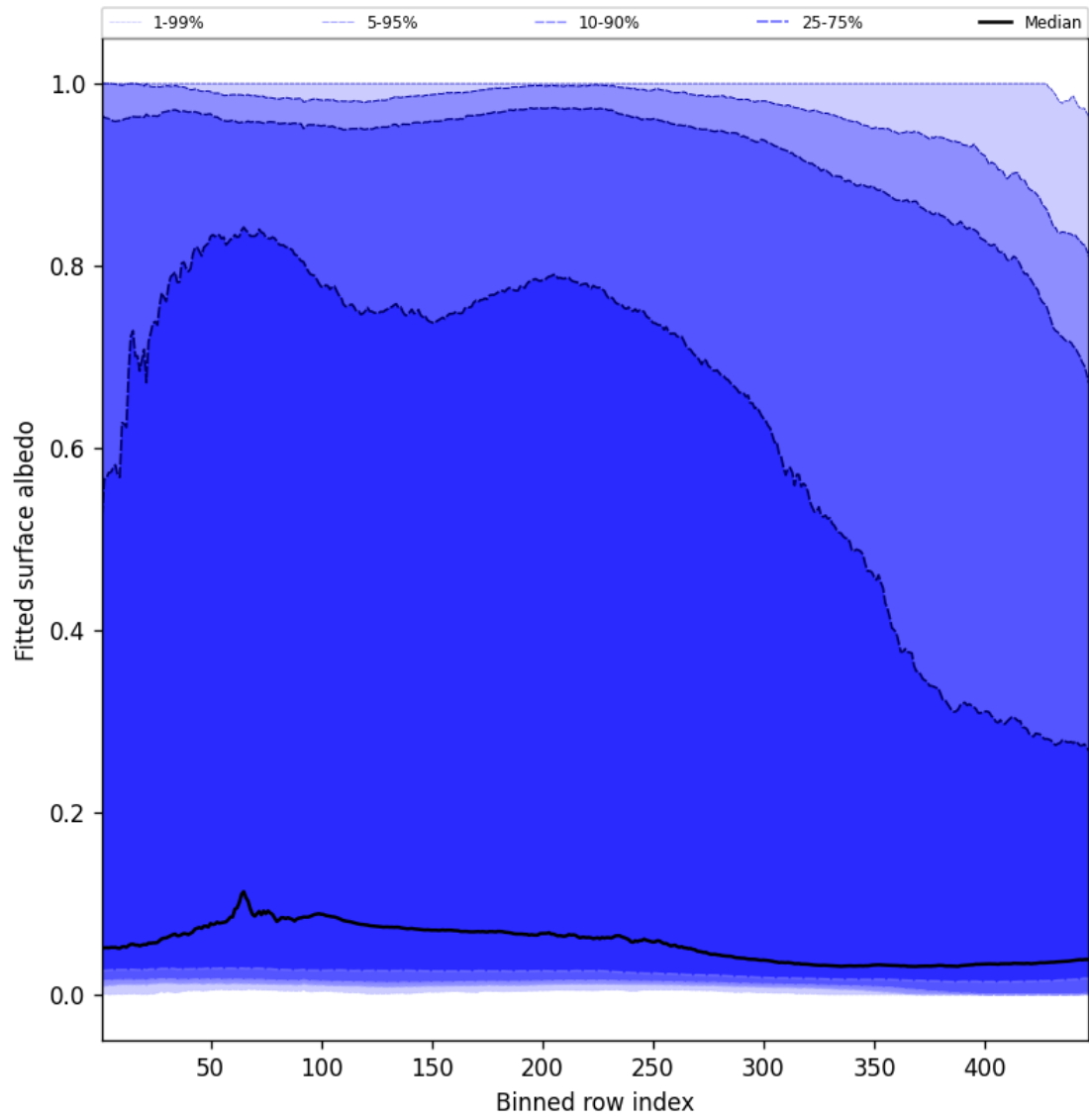
Figure 61: Along track statistics of “Fitted surface albedo” for 2024-12-02 to 2024-12-04
