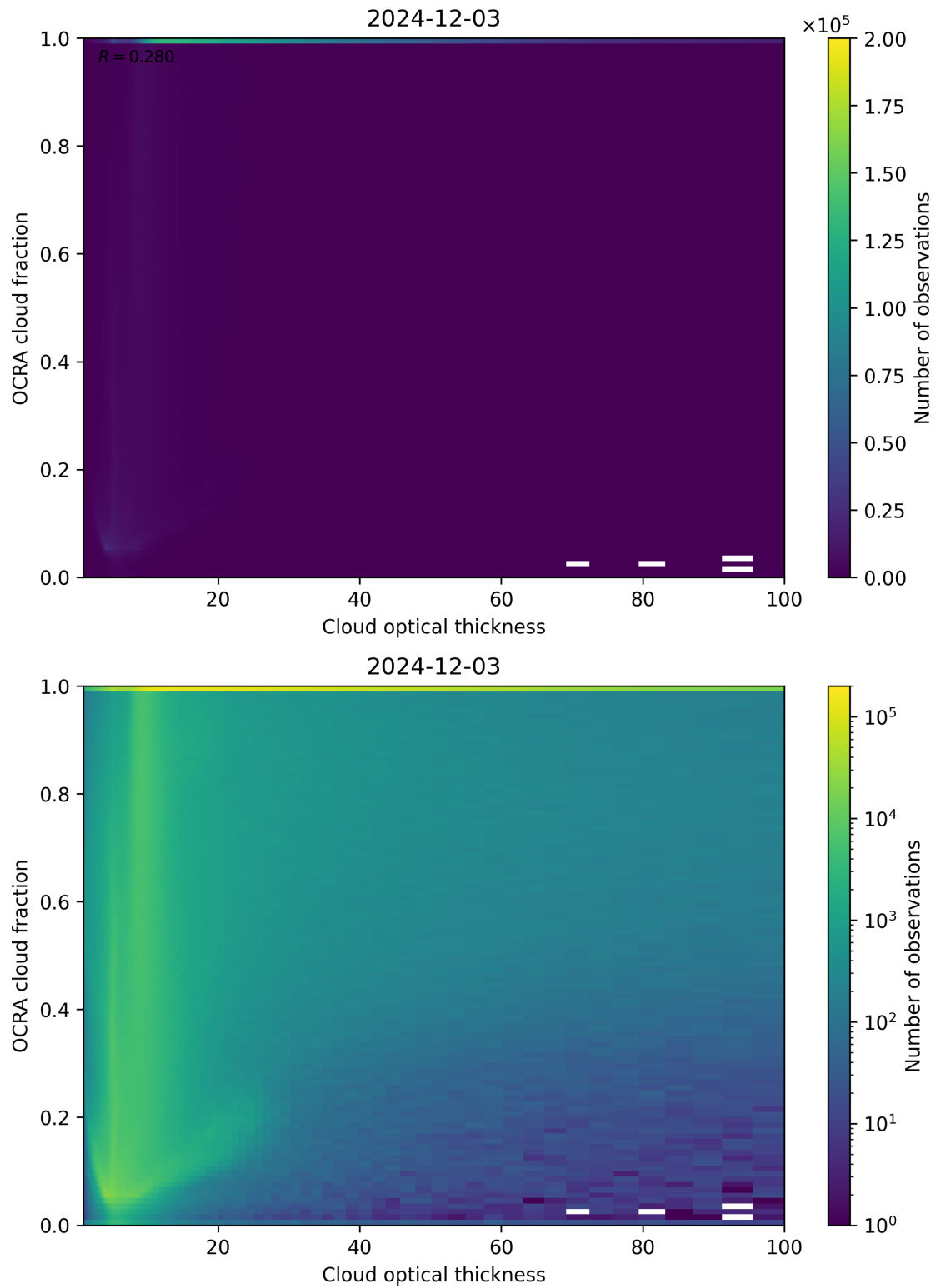
Figure 83: Scatter density plot of “Cloud optical thickness” against “OCRA cloud fraction” for 2024-12-02 to 2024-12-04.
