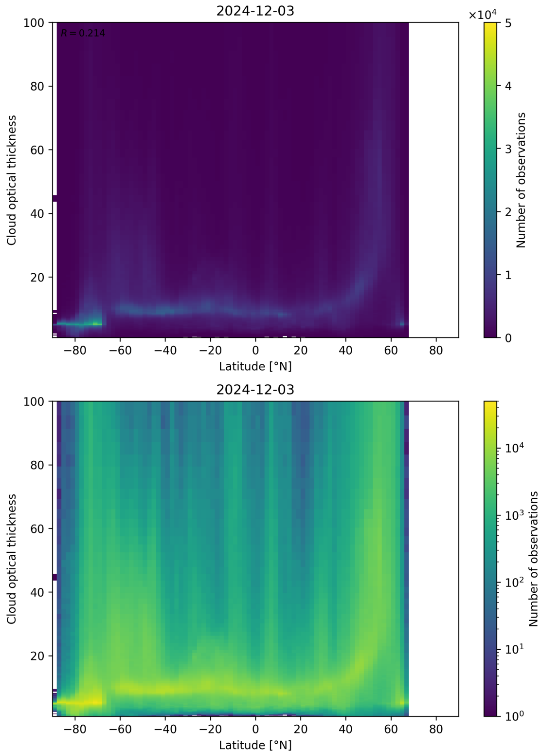
Figure 96: Scatter density plot of “Latitude” against “Cloud optical thickness” for 2024-12-02 to 2024-12-04.
