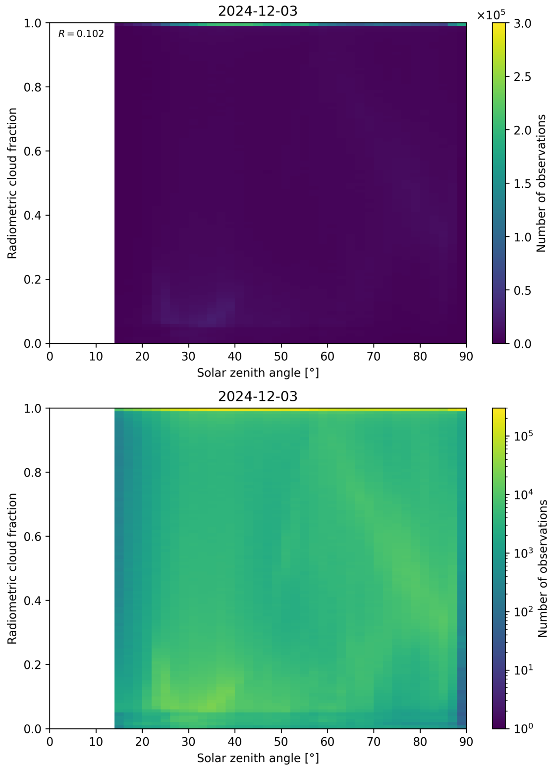
Figure 99: Scatter density plot of “Solar zenith angle” against “Radiometric cloud fraction” for 2024-12-02 to 2024-12-04.
