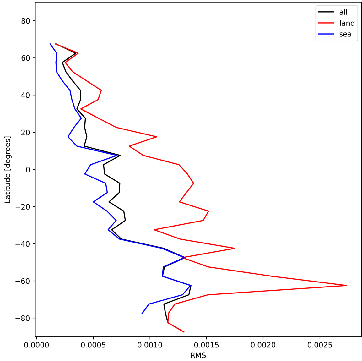
Figure 31: Zonal average of “RMS” for 2024-12-02 to 2024-12-04.
