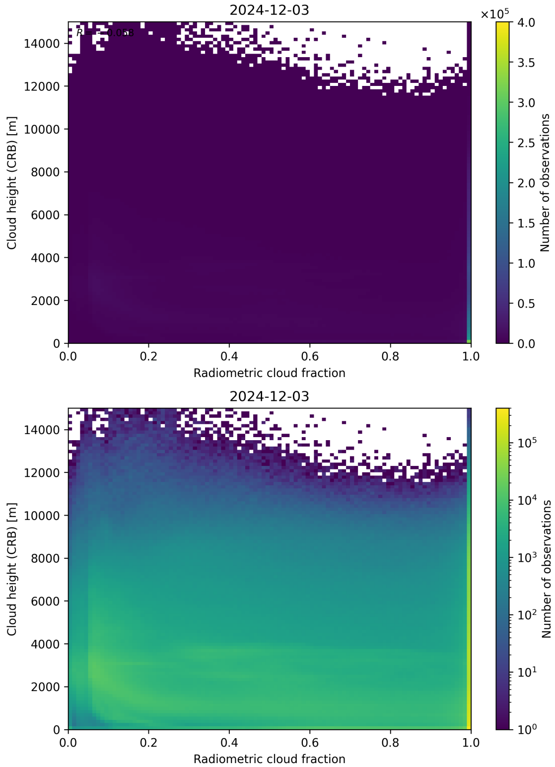
Figure 74: Scatter density plot of “Radiometric cloud fraction” against “Cloud height (CRB)” for 2024-12-02 to 2024-12-04.
