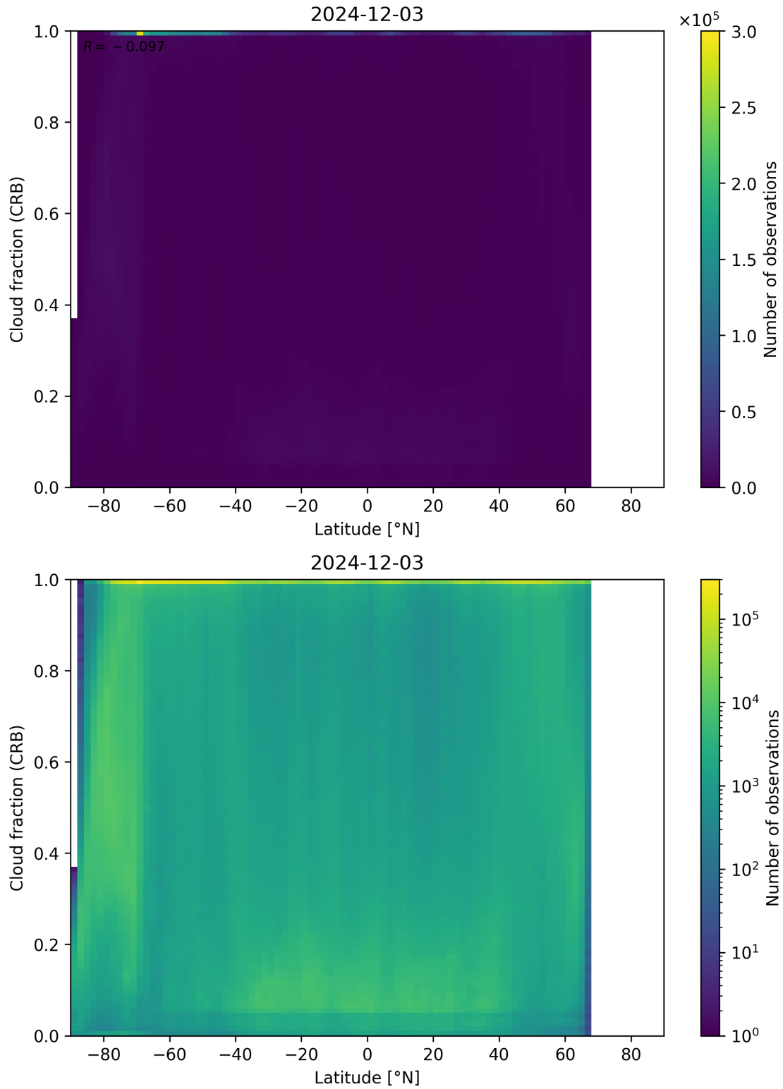
Figure 94: Scatter density plot of “Latitude” against “Cloud fraction (CRB)” for 2024-12-02 to 2024-12-04.
