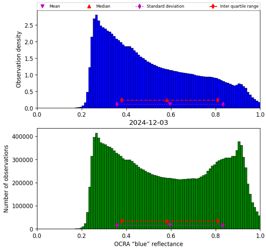
Figure 51: Histogram of “OCRA “blue” reflectance” for 2024-12-02 to 2024-12-04
