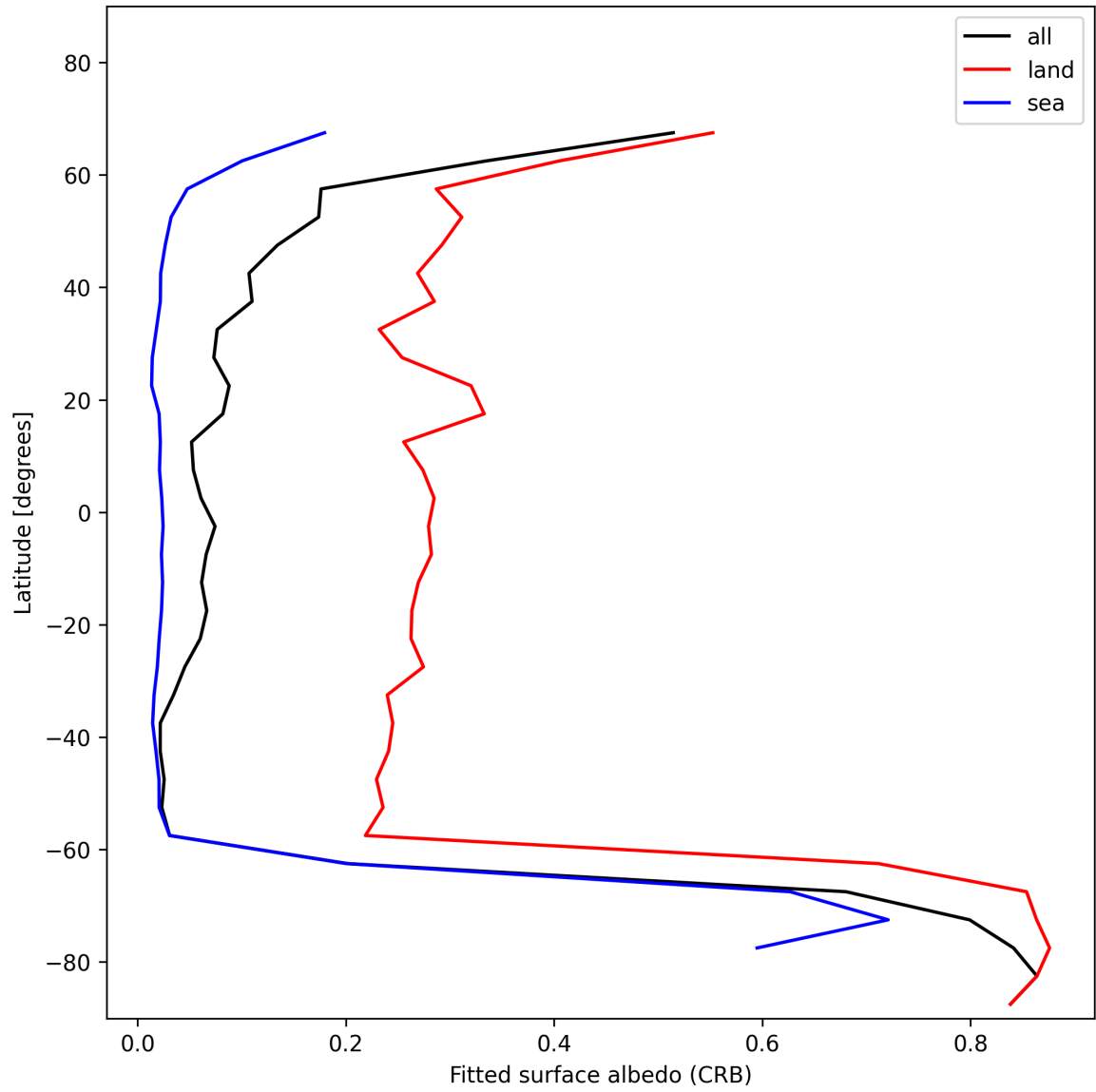
Figure 30: Zonal average of “Fitted surface albedo (CRB)” for 2024-12-02 to 2024-12-04.
