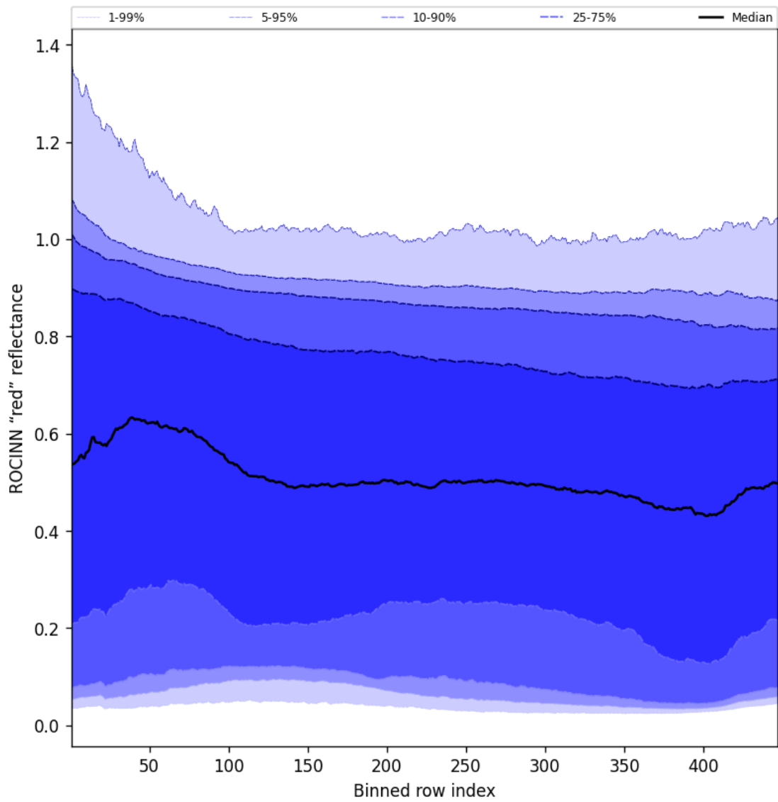
Figure 69: Along track statistics of "ROCINN "red" reflectance" for 2024-12-02 to 2024-12-04
