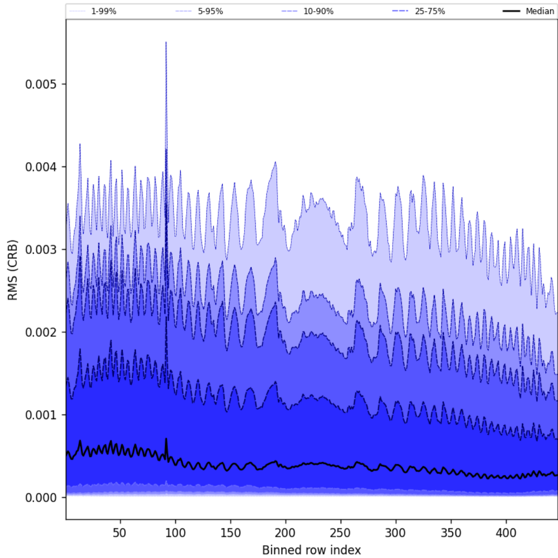
Figure 64: Along track statistics of “RMS (CRB)” for 2024-12-02 to 2024-12-04
