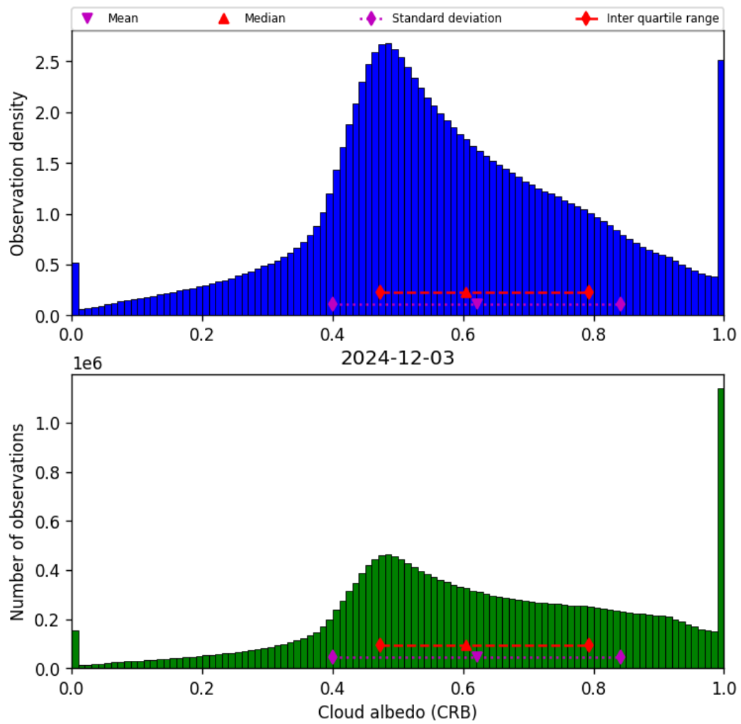
Figure 44: Histogram of “Cloud albedo (CRB)” for 2024-12-02 to 2024-12-04
