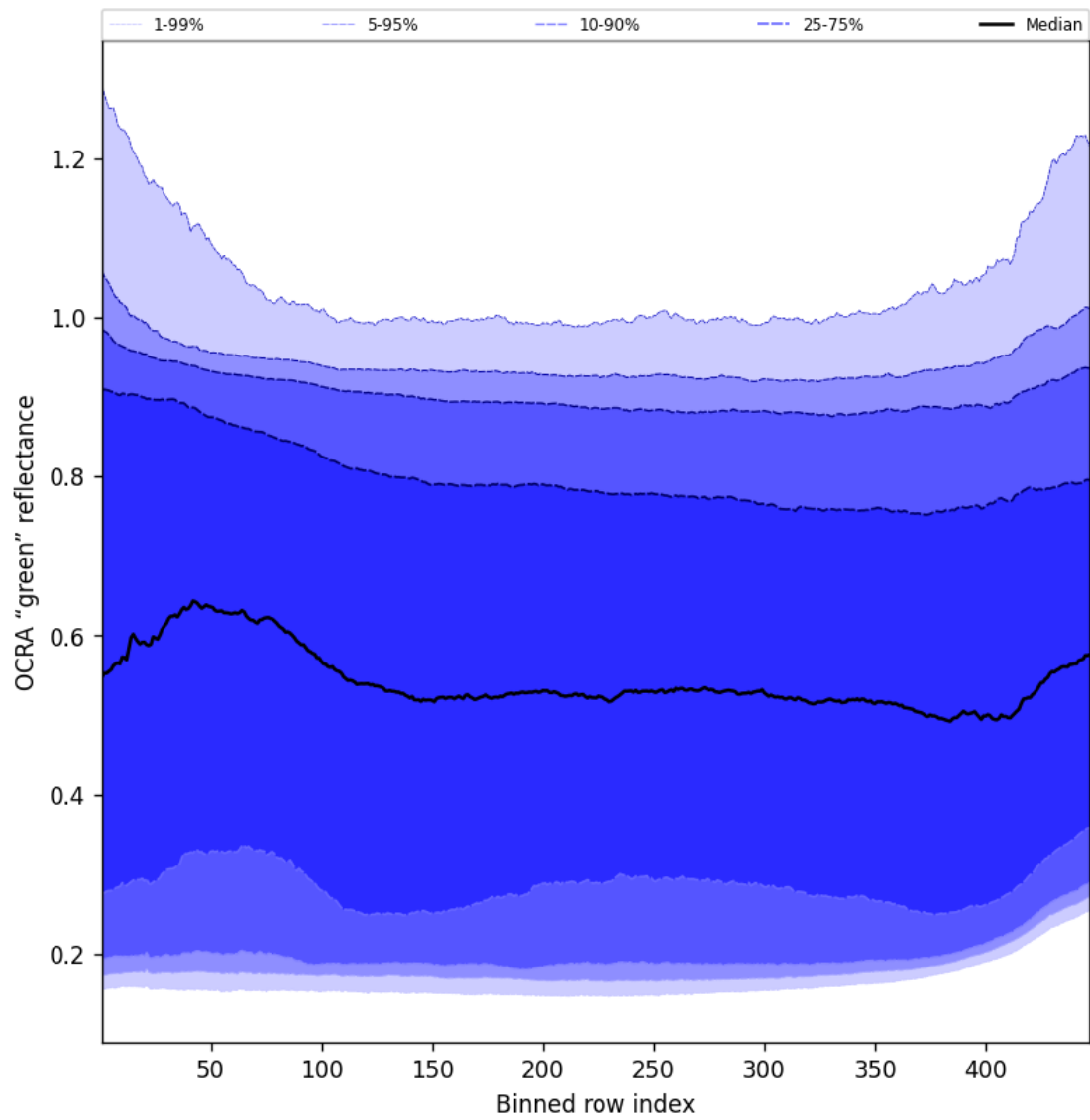
Figure 68: Along track statistics of "OCRA "green" reflectance" for 2024-12-02 to 2024-12-04
