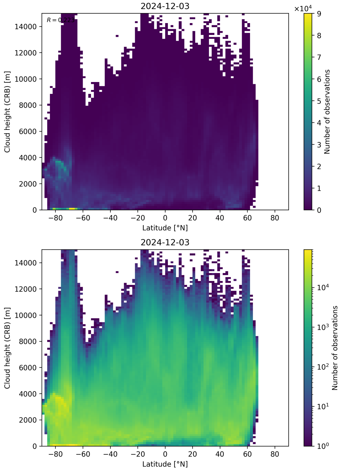
Figure 95: Scatter density plot of “Latitude” against “Cloud height (CRB)” for 2024-12-02 to 2024-12-04.
