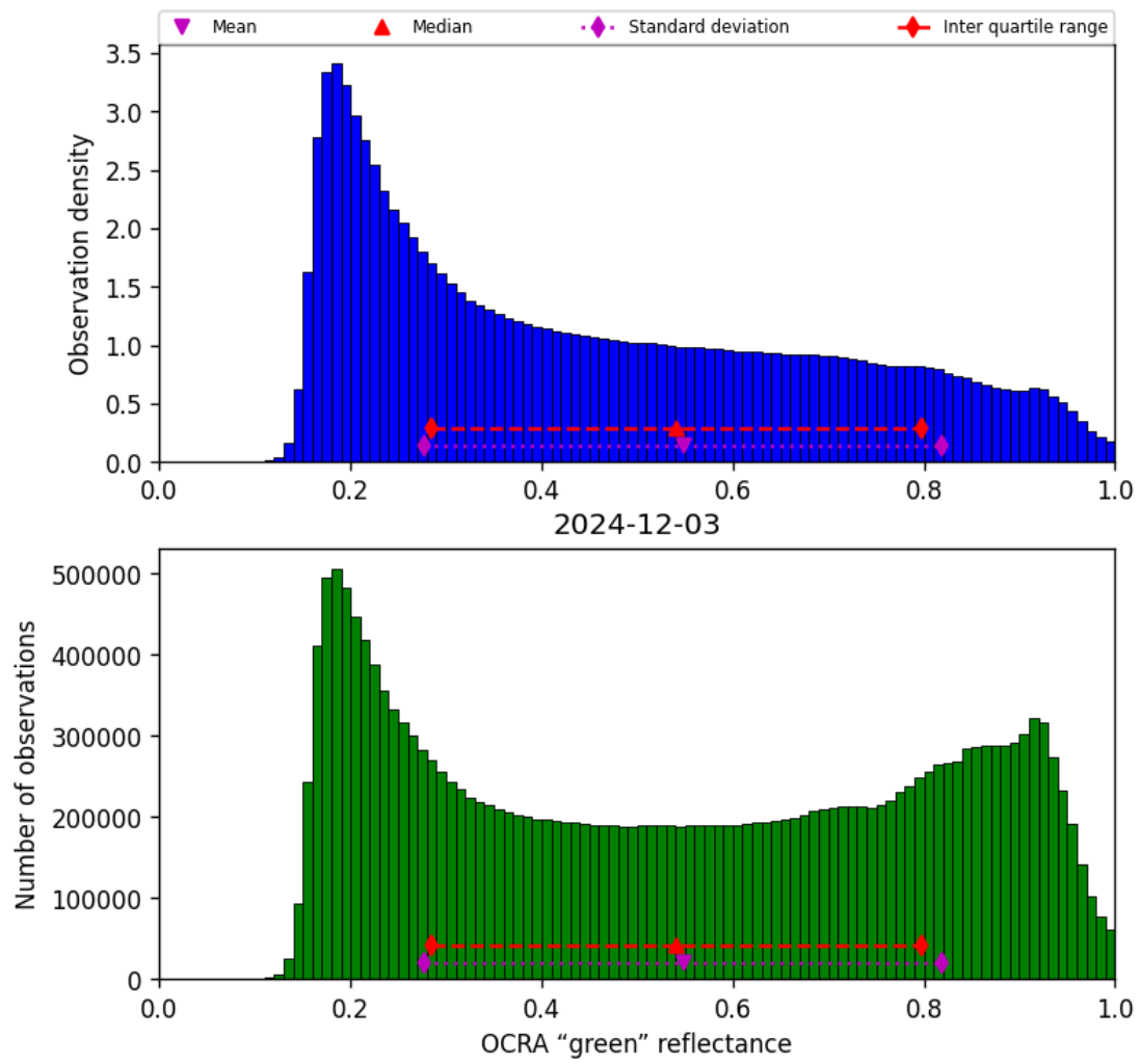
Figure 52: Histogram of “OCRA “green” reflectance” for 2024-12-02 to 2024-12-04
