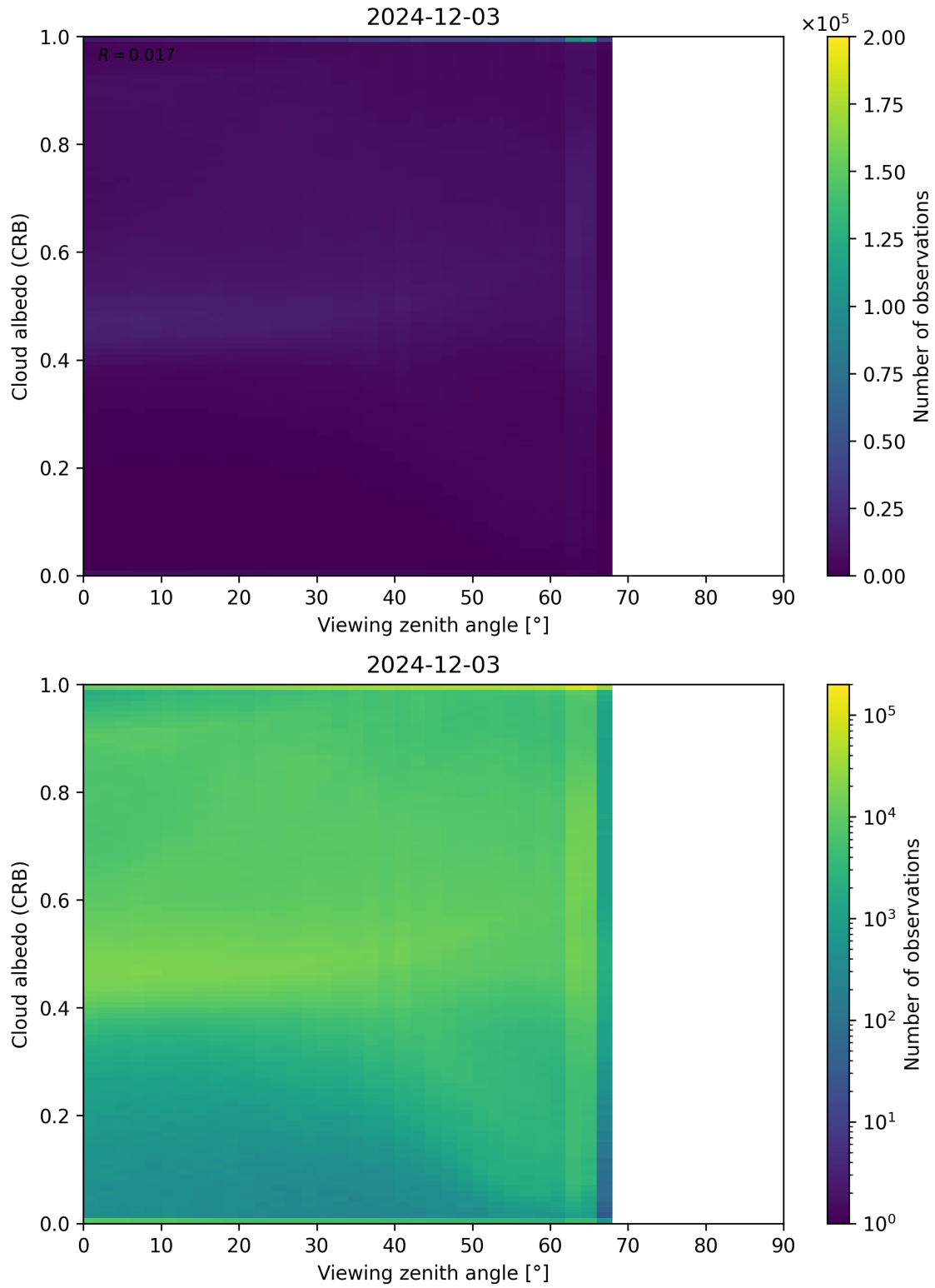
Figure 106: Scatter density plot of “Viewing zenith angle” against “Cloud albedo (CRB)” for 2024-12-02 to 2024-12-04.
