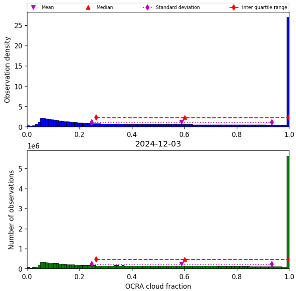
Figure 50: Histogram of “OCRA cloud fraction” for 2024-12-02 to 2024-12-04
