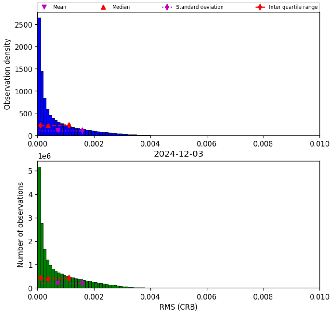
Figure 48: Histogram of “RMS (CRB)” for 2024-12-02 to 2024-12-04
