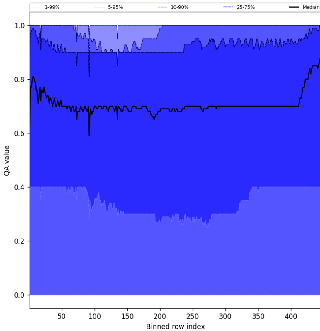
Figure 54: Along track statistics of “QA value” for 2024-12-02 to 2024-12-04
