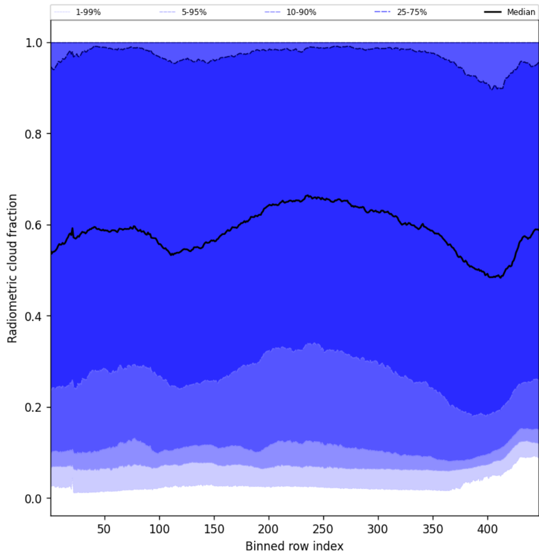
Figure 55: Along track statistics of “Radiometric cloud fraction” for 2024-12-02 to 2024-12-04
