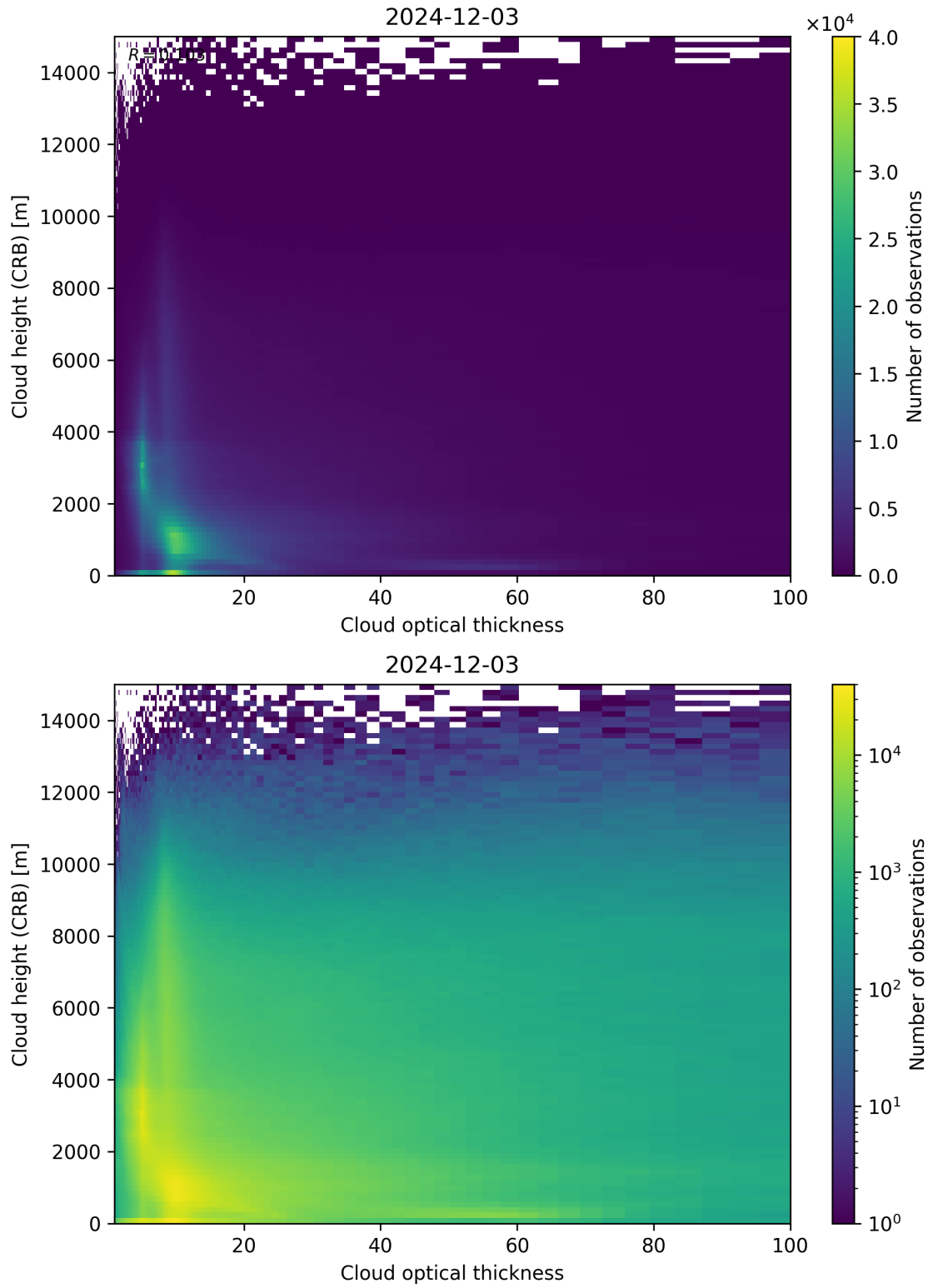
Figure 85: Scatter density plot of “Cloud optical thickness” against “Cloud height (CRB)” for 2024-12-02 to 2024-12-04.
