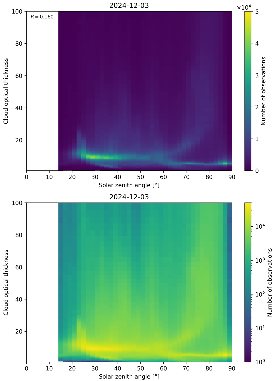
Figure 103: Scatter density plot of “Solar zenith angle” against “Cloud optical thickness” for 2024-12-02 to 2024-12-04.
