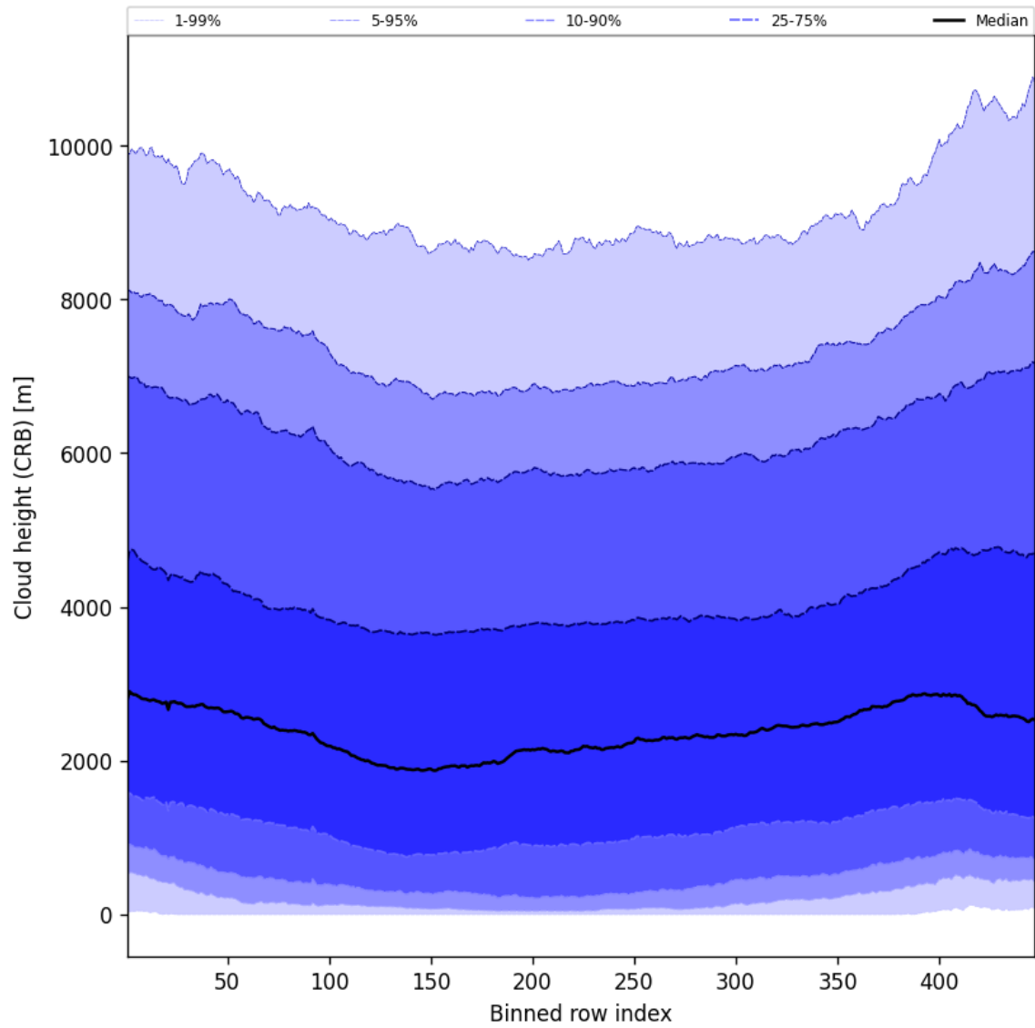
Figure 59: Along track statistics of “Cloud height (CRB)” for 2024-12-02 to 2024-12-04
