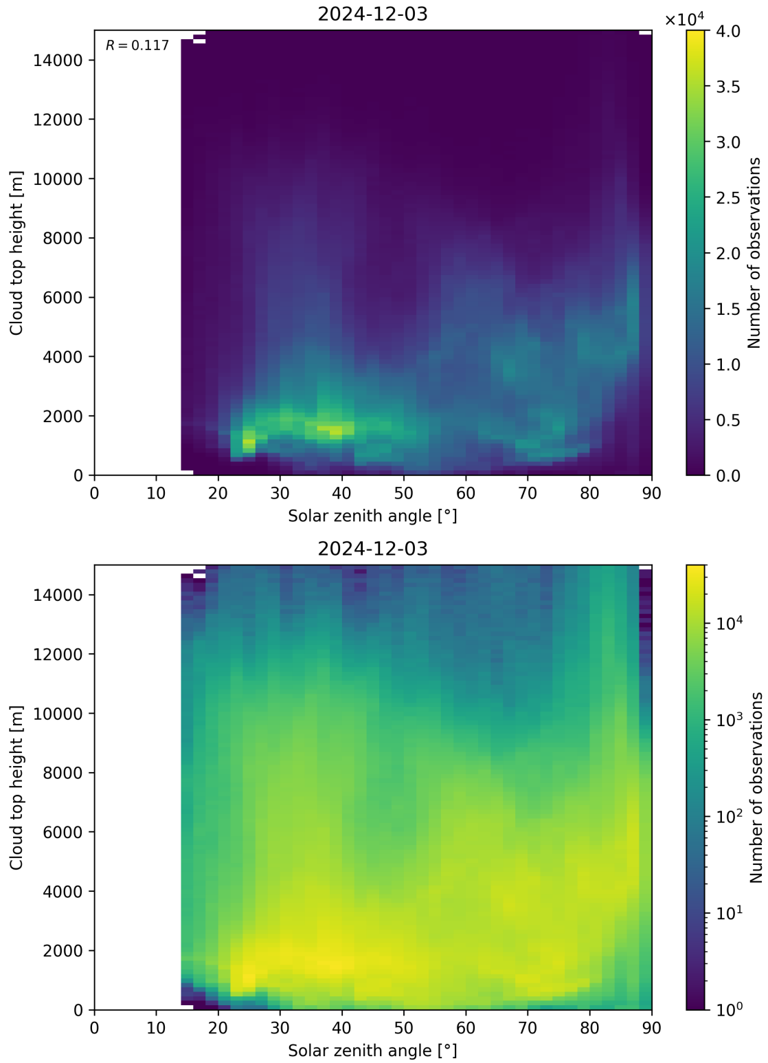
Figure 104: Scatter density plot of “Solar zenith angle” against “Cloud top height” for 2024-12-02 to 2024-12-04.
