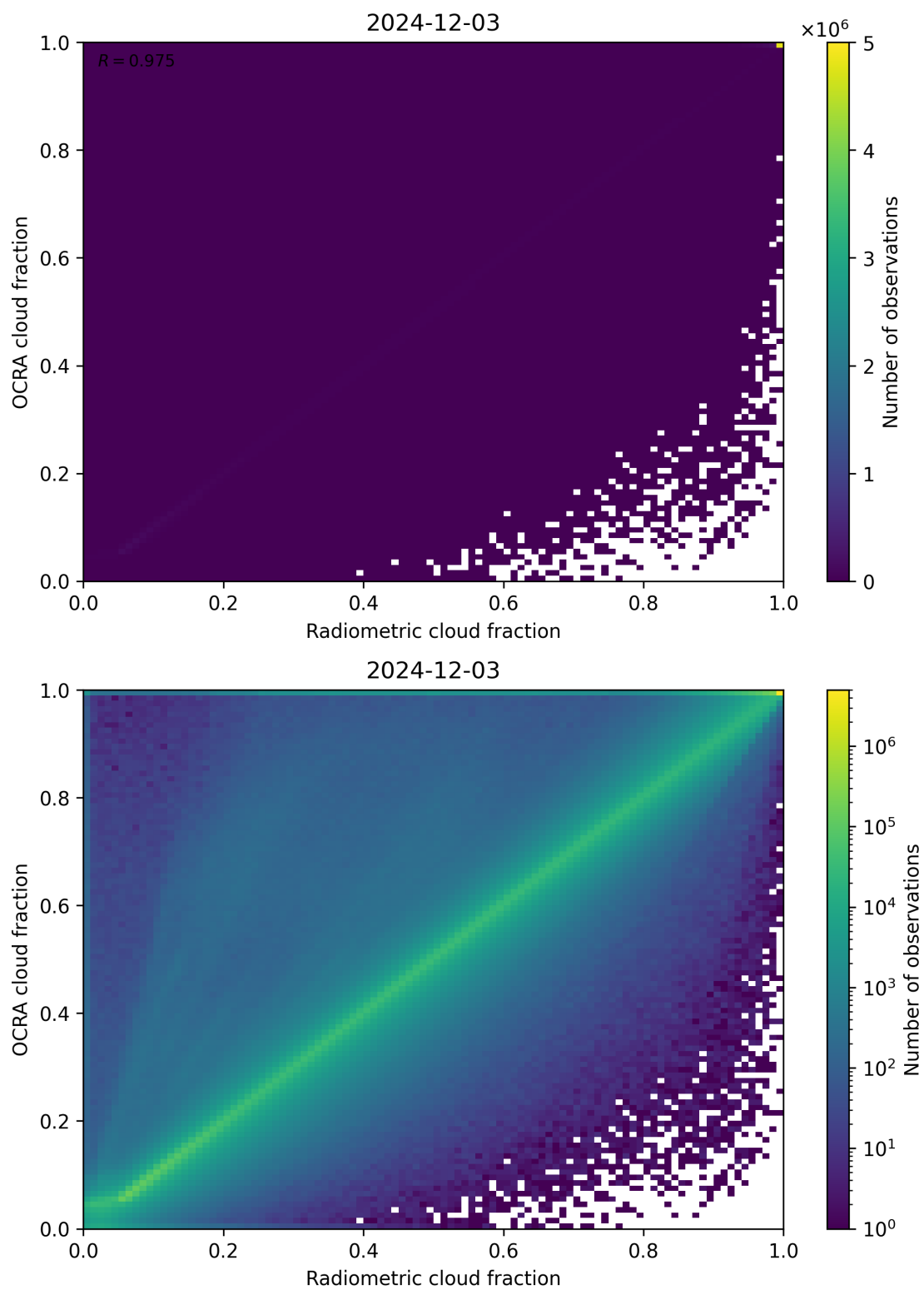
Figure 72: Scatter density plot of “Radiometric cloud fraction” against “OCRA cloud fraction” for 2024-12-02 to 2024-12-04.
