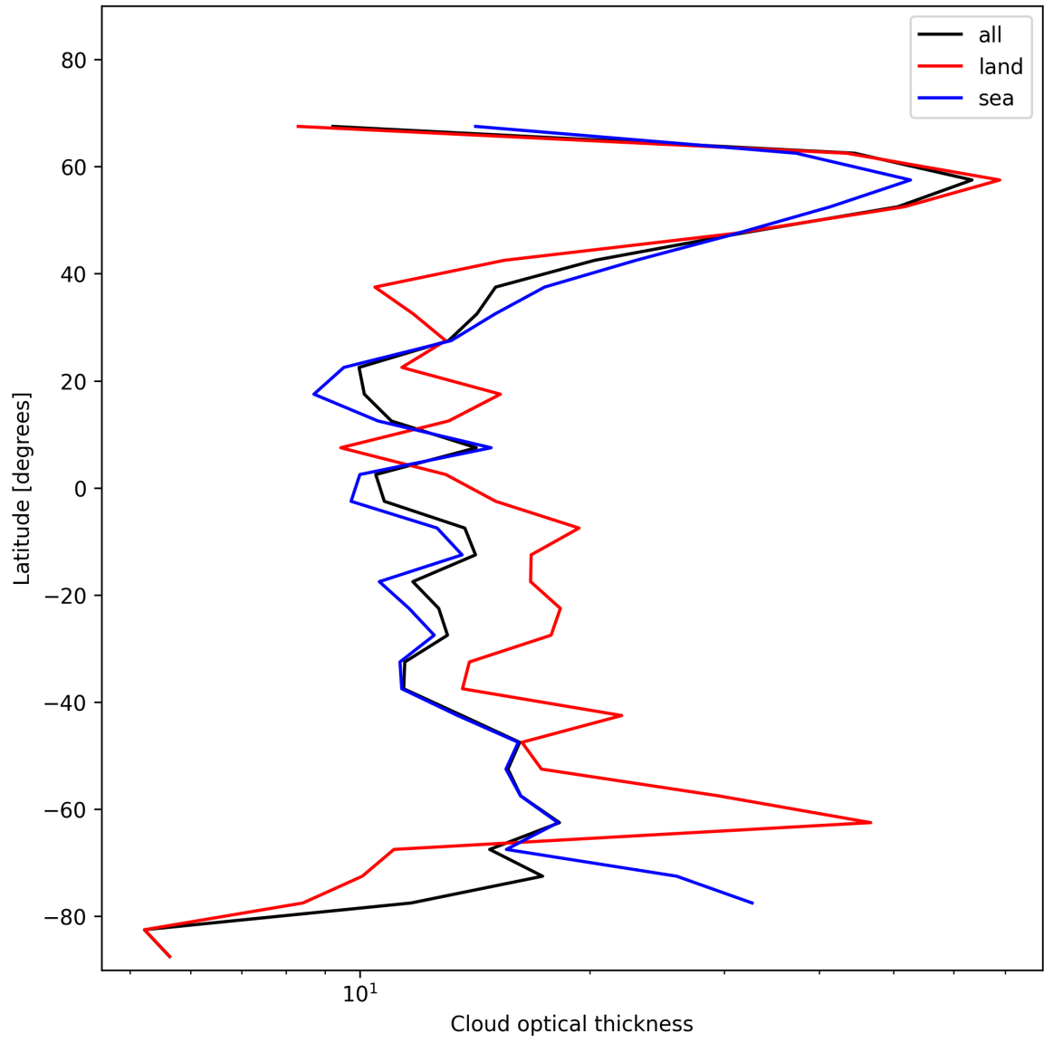
Figure 25: Zonal average of “Cloud optical thickness” for 2024-12-02 to 2024-12-04.
