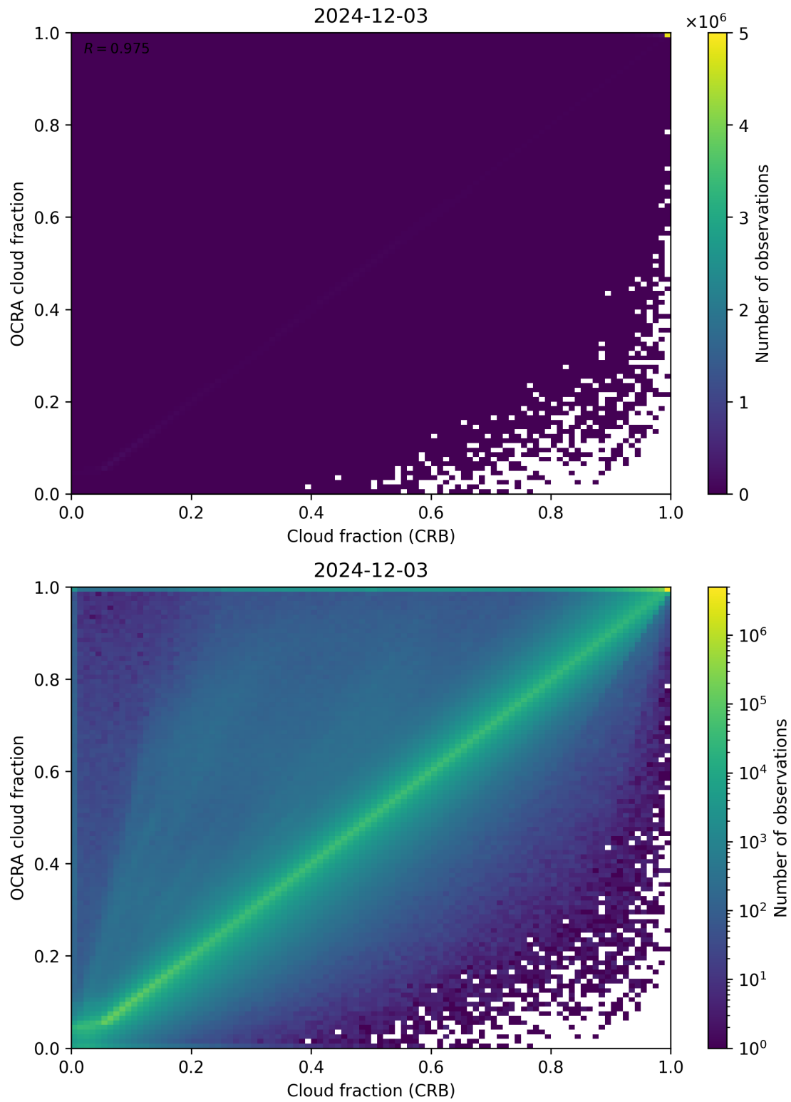
Figure 78: Scatter density plot of “Cloud fraction (CRB)” against “OCRA cloud fraction” for 2024-12-02 to 2024-12-04.
