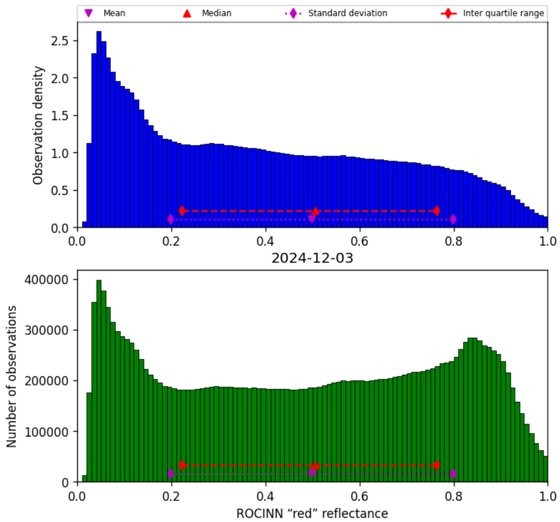
Figure 53: Histogram of “ROCINN “red” reflectance” for 2024-12-02 to 2024-12-04
