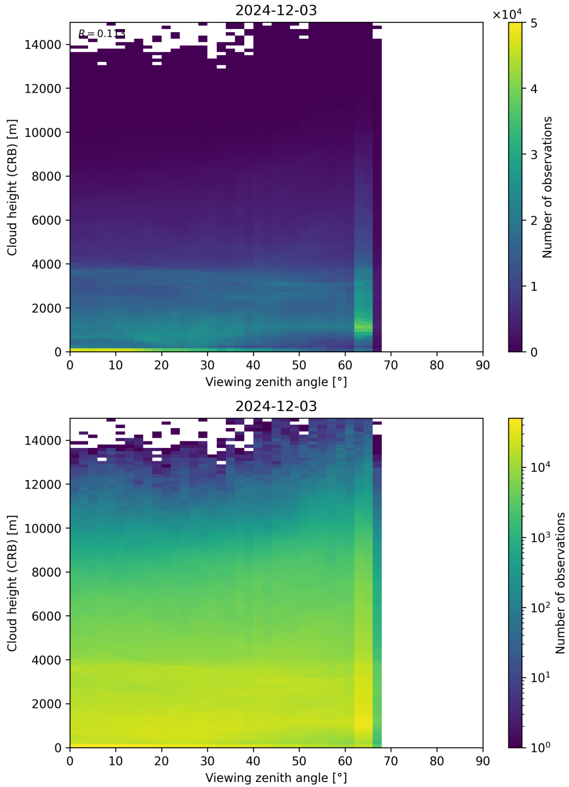
Figure 110: Scatter density plot of “Viewing zenith angle” against “Cloud height (CRB)” for 2024-12-02 to 2024-12-04.
