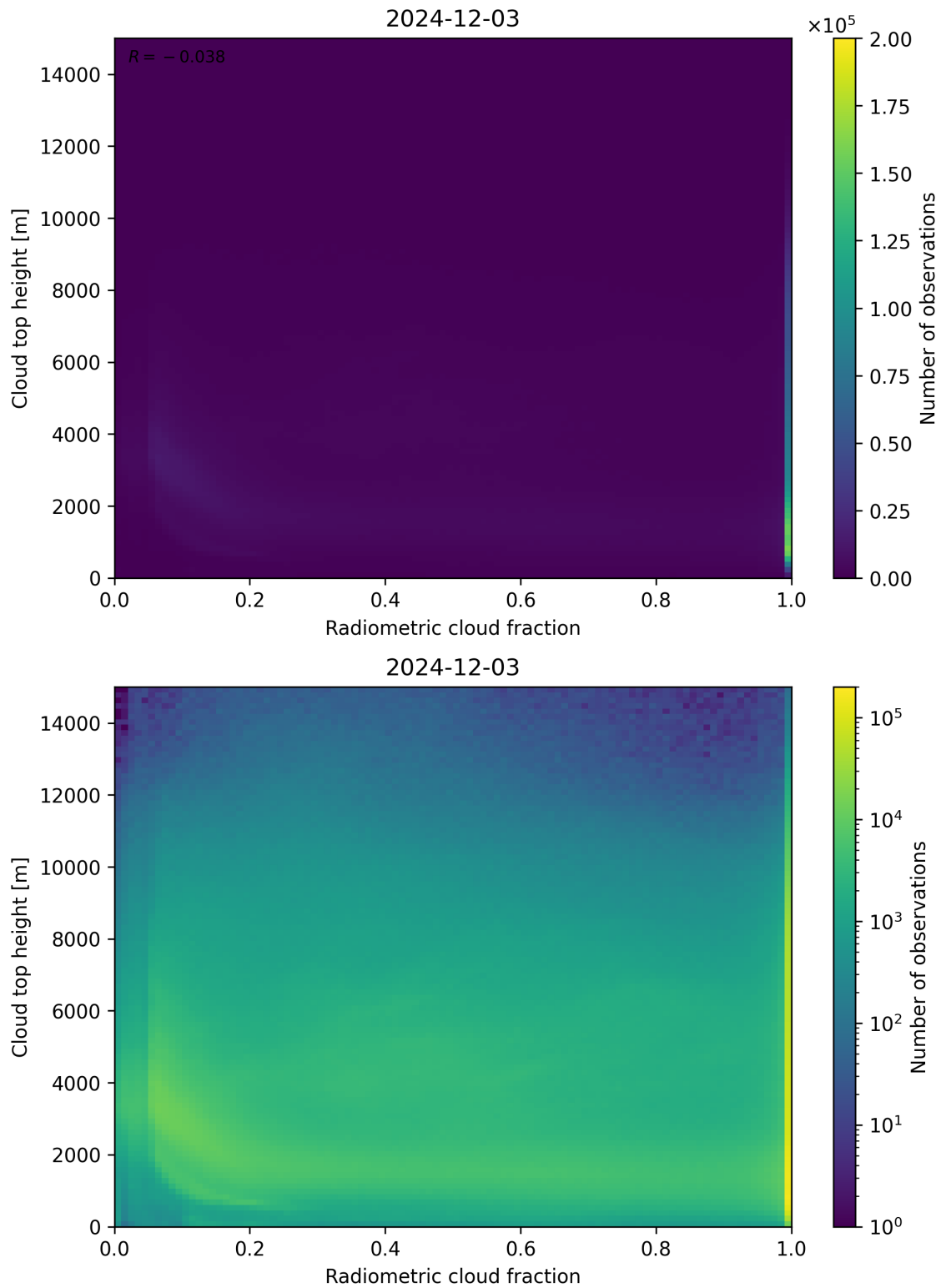
Figure 76: Scatter density plot of “Radiometric cloud fraction” against “Cloud top height” for 2024-12-02 to 2024-12-04.
