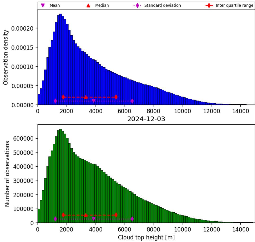
Figure 40: Histogram of “Cloud top height” for 2024-12-02 to 2024-12-04
