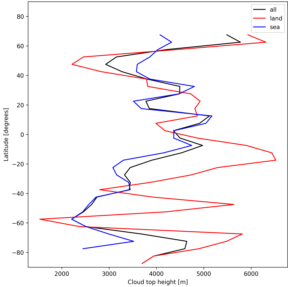
Figure 24: Zonal average of “Cloud top height” for 2024-12-02 to 2024-12-04.
