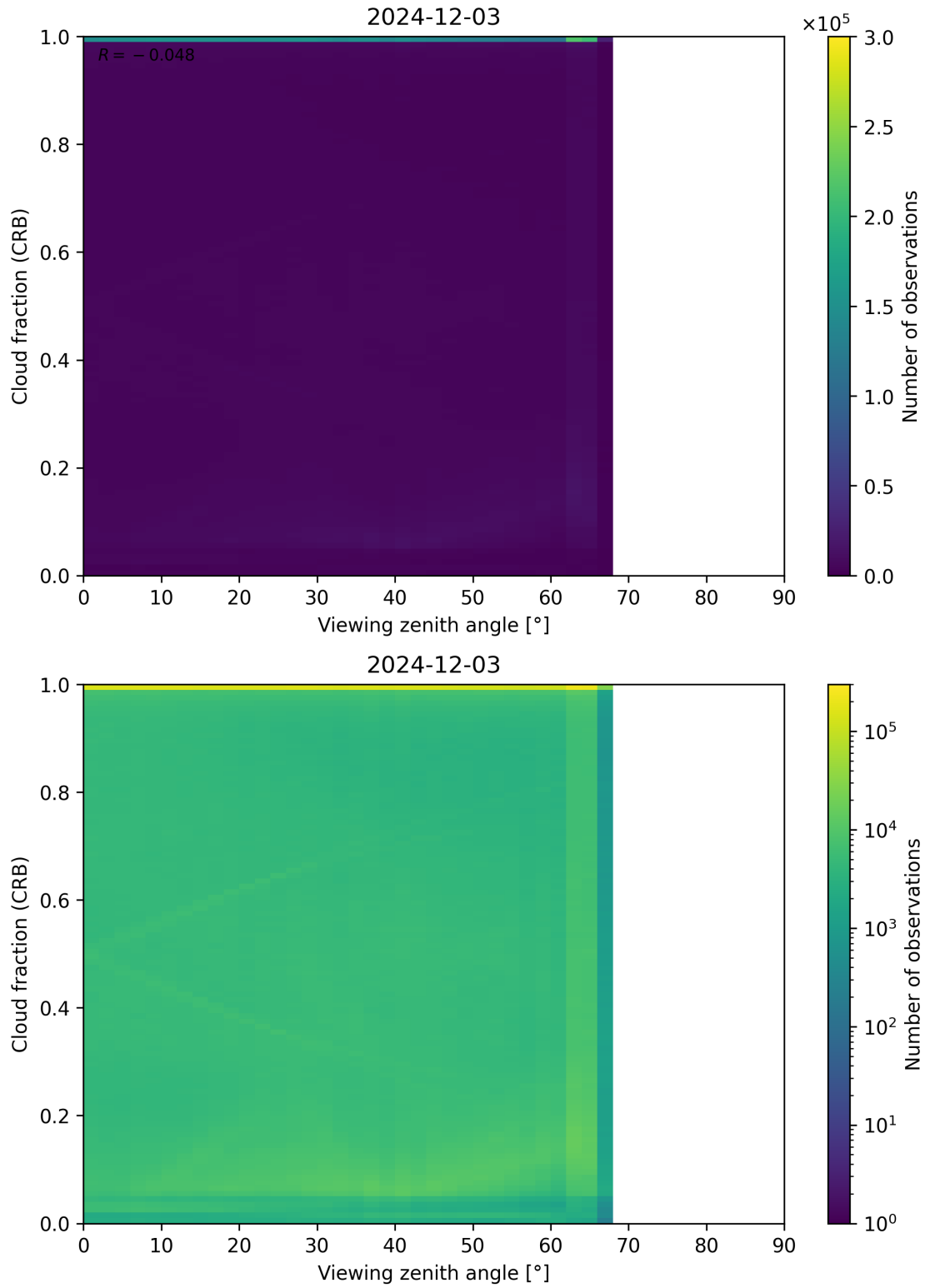
Figure 109: Scatter density plot of “Viewing zenith angle” against “Cloud fraction (CRB)” for 2024-12-02 to 2024-12-04.
