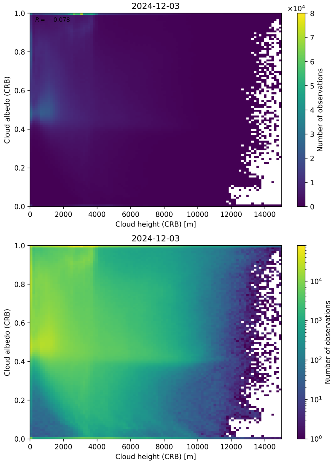
Figure 80: Scatter density plot of “Cloud height (CRB)” against “Cloud albedo (CRB)” for 2024-12-02 to 2024-12-04.
