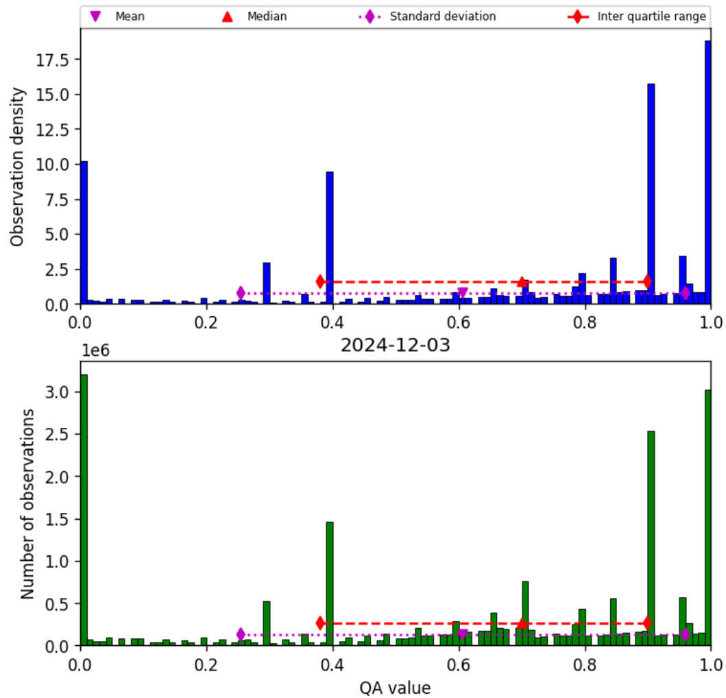
Figure 38: Histogram of “QA value” for 2024-12-02 to 2024-12-04
