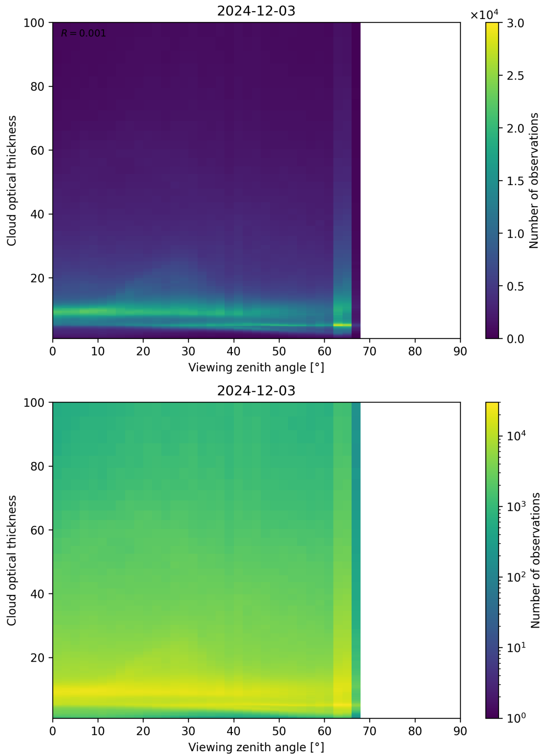
Figure 111: Scatter density plot of “Viewing zenith angle” against “Cloud optical thickness” for 2024-12-02 to 2024-12-04.
