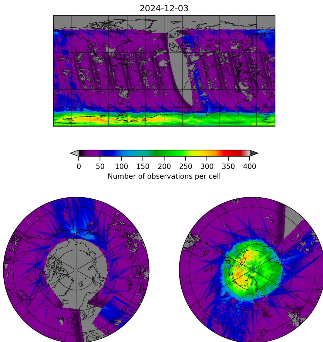
Figure 21: Map of the number of observations for 2024-12-02 to 2024-12-04
