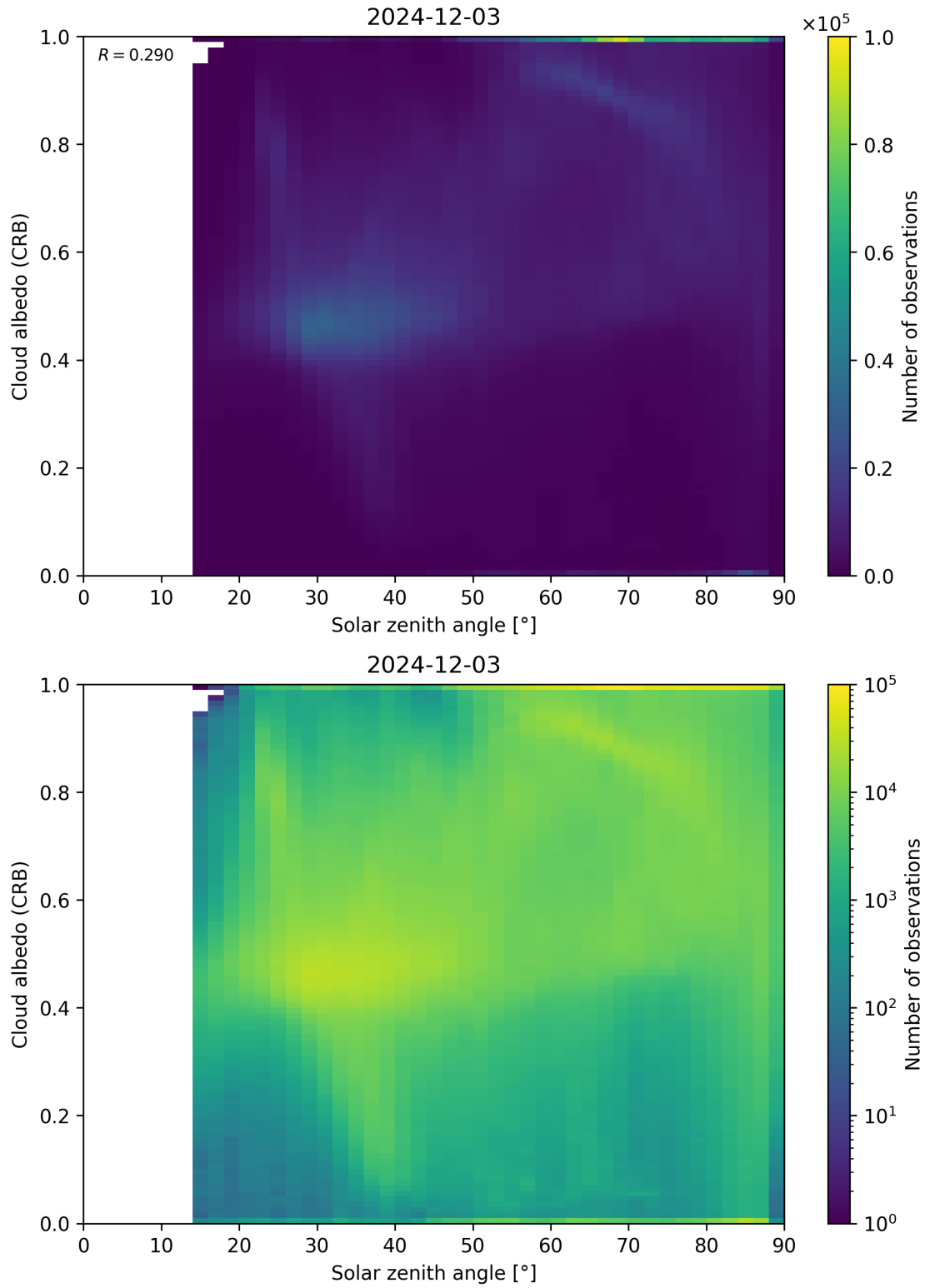
Figure 98: Scatter density plot of “Solar zenith angle” against “Cloud albedo (CRB)” for 2024-12-02 to 2024-12-04.
