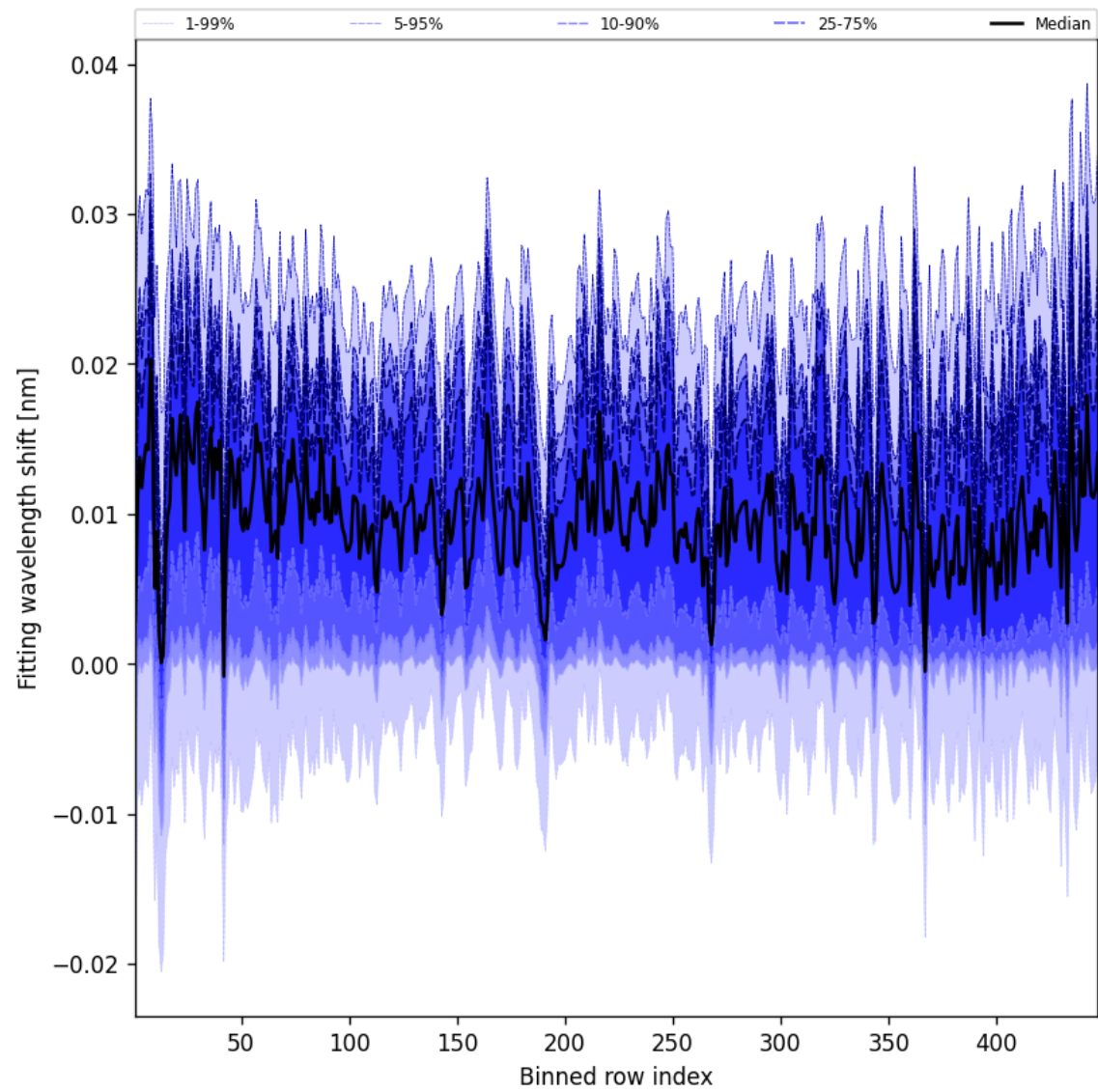
Figure 65: Along track statistics of “Fitting wavelength shift” for 2024-12-02 to 2024-12-04
