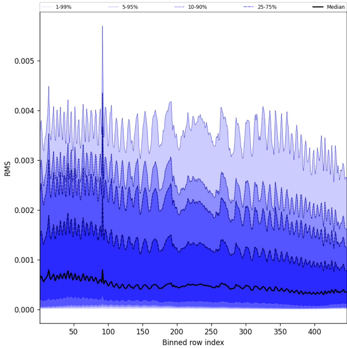
Figure 63: Along track statistics of “RMS” for 2024-12-02 to 2024-12-04
