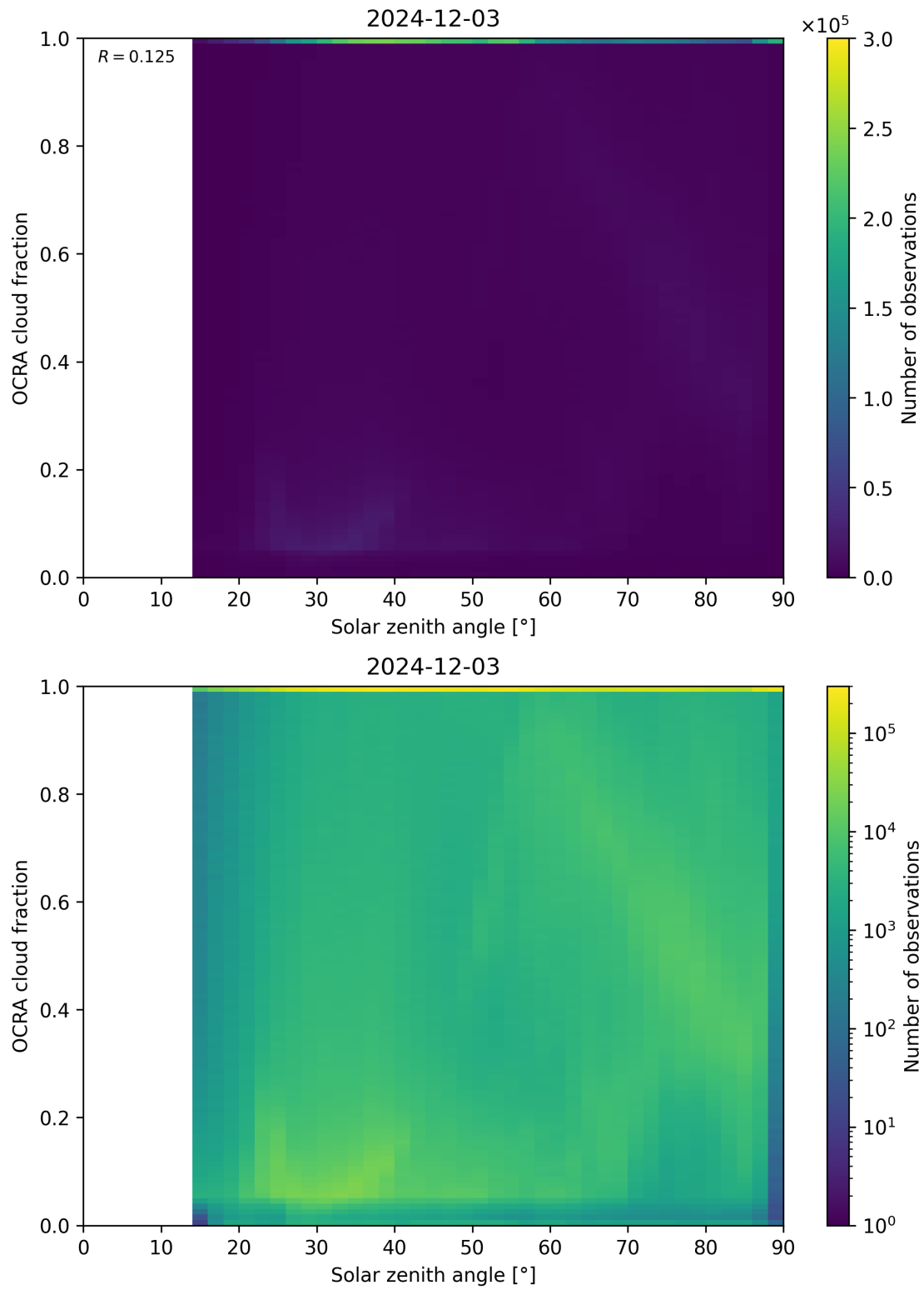
Figure 100: Scatter density plot of “Solar zenith angle” against “OCRA cloud fraction” for 2024-12-02 to 2024-12-04.
