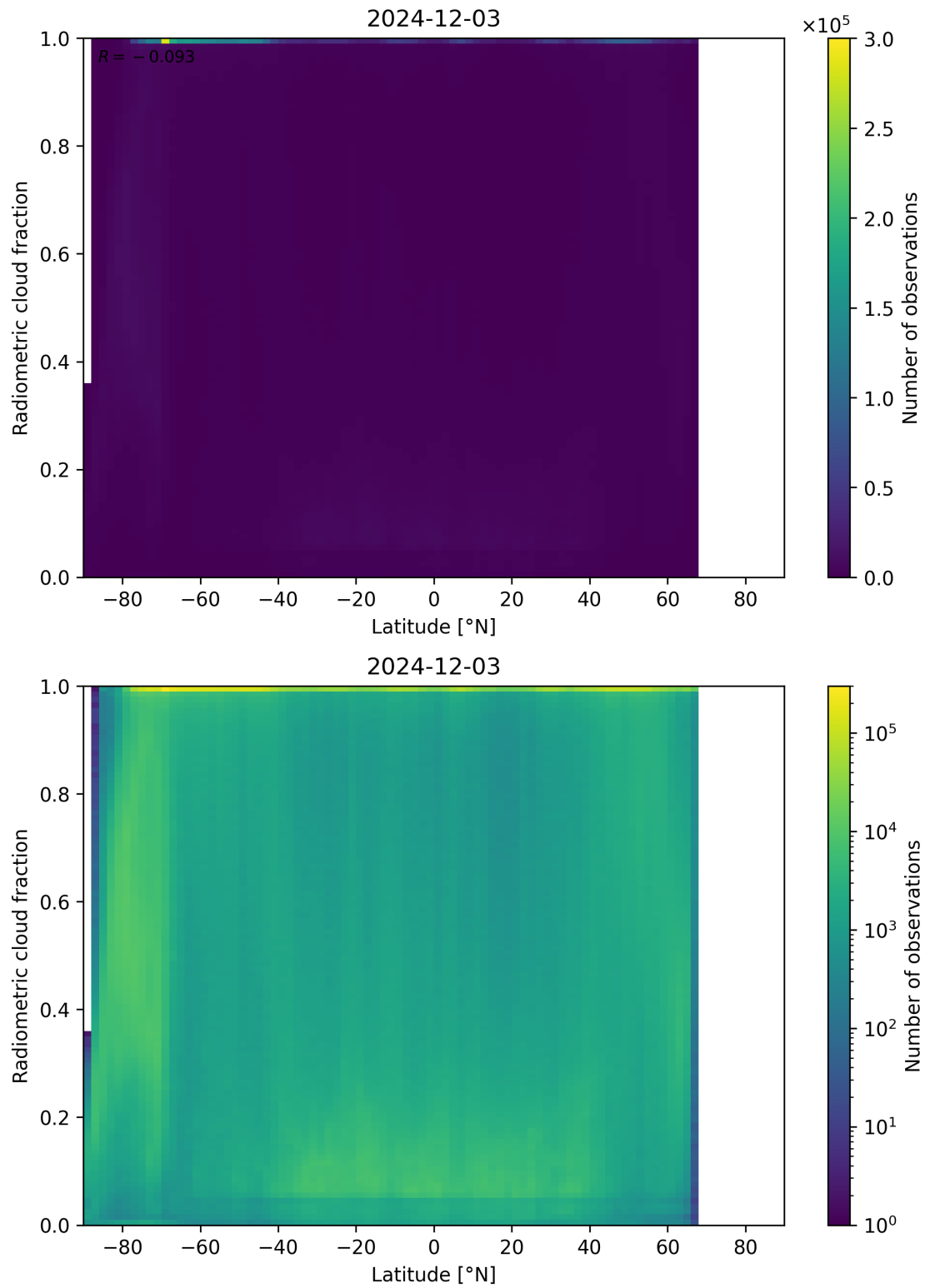
Figure 92: Scatter density plot of “Latitude” against “Radiometric cloud fraction” for 2024-12-02 to 2024-12-04.
