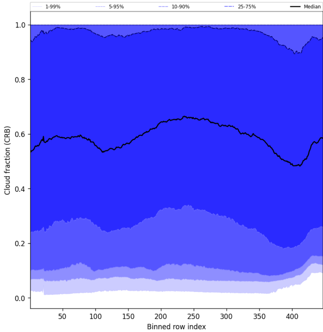
Figure 58: Along track statistics of “Cloud fraction (CRB)” for 2024-12-02 to 2024-12-04
