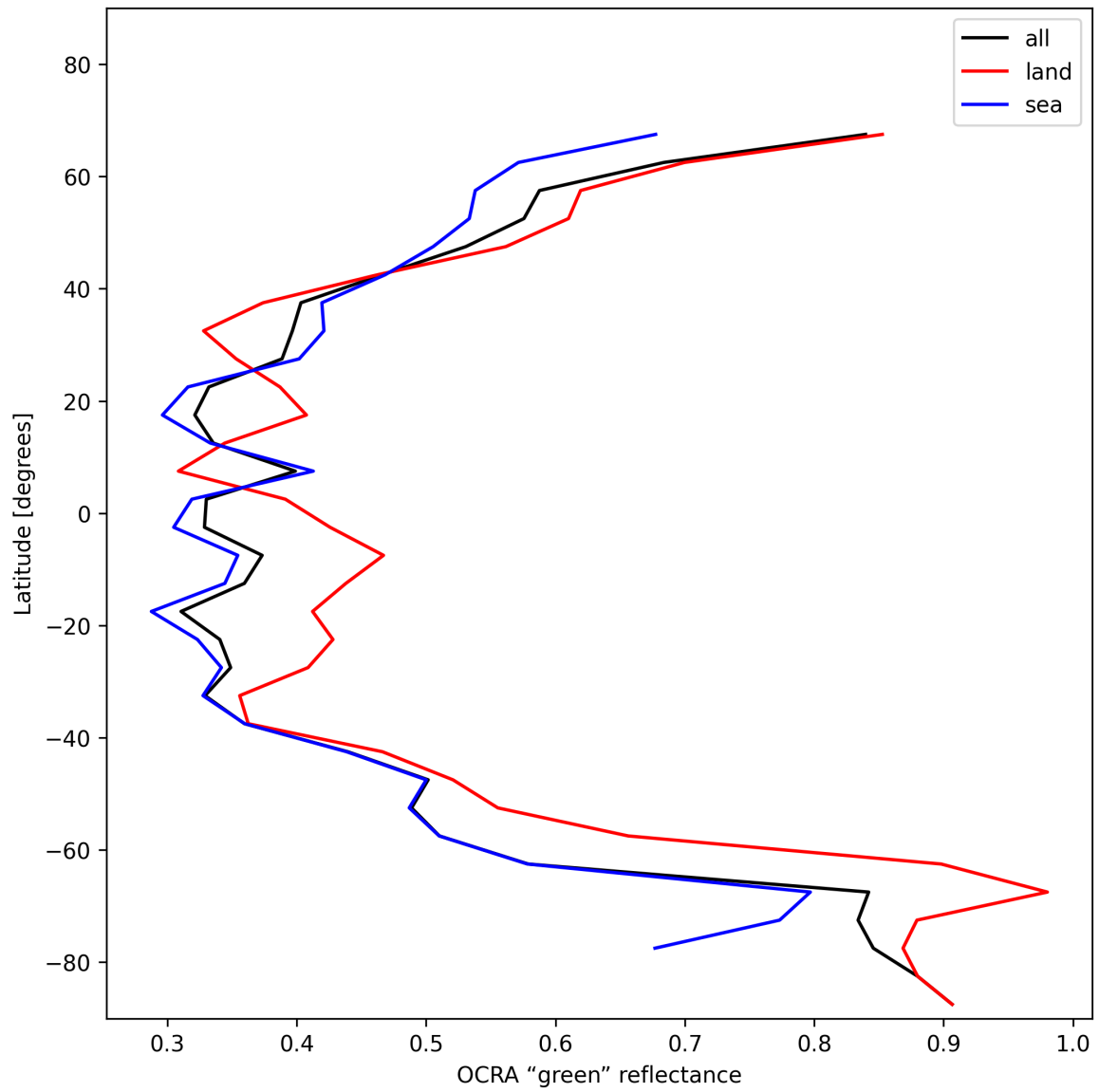
Figure 36: Zonal average of “OCRA “green” reflectance” for 2024-12-02 to 2024-12-04.
