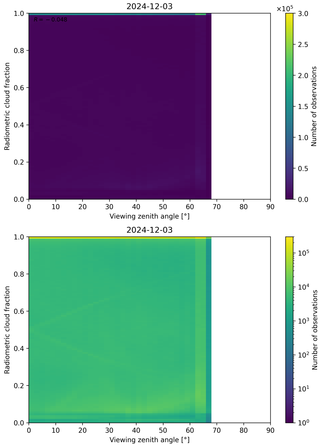
Figure 107: Scatter density plot of “Viewing zenith angle” against “Radiometric cloud fraction” for 2024-12-02 to 2024-12-04.
