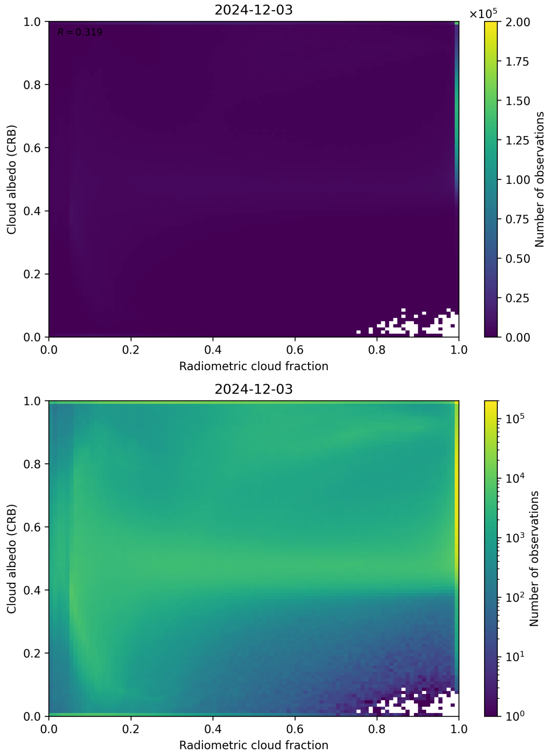
Figure 71: Scatter density plot of “Radiometric cloud fraction” against “Cloud albedo (CRB)” for 2024-12-02 to 2024-12-04.
