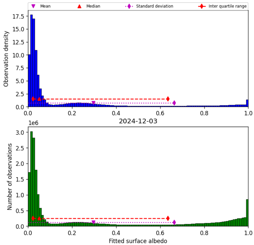
Figure 45: Histogram of “Fitted surface albedo” for 2024-12-02 to 2024-12-04
