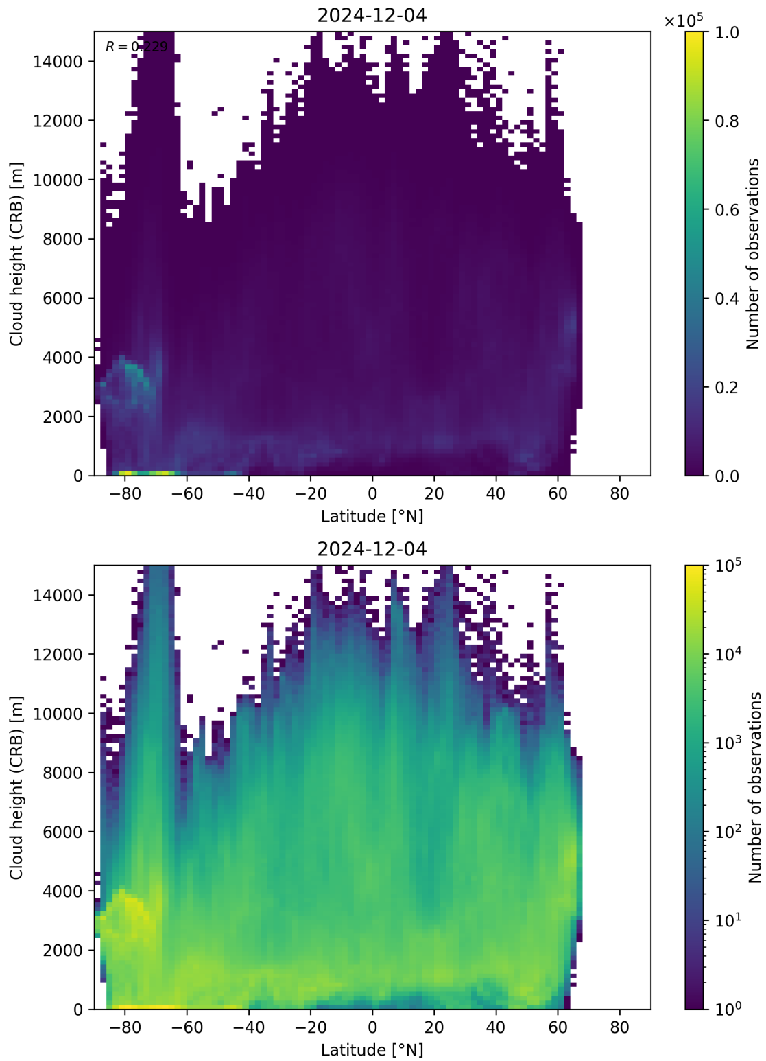
Figure 95: Scatter density plot of “Latitude” against “Cloud height (CRB)” for 2024-12-03 to 2024-12-05.
