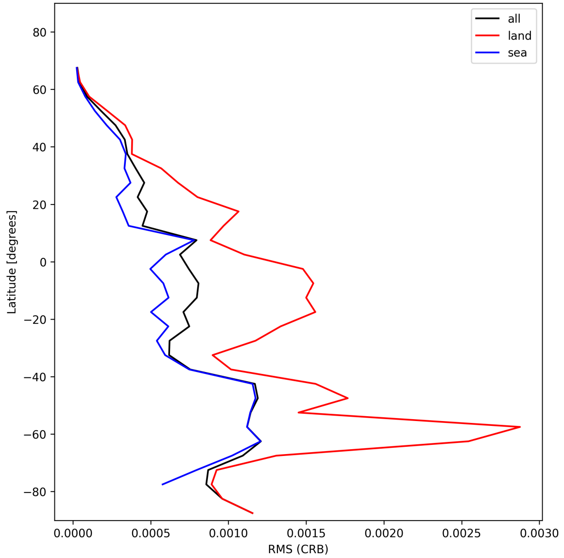
Figure 32: Zonal average of “RMS (CRB)” for 2024-12-03 to 2024-12-05.
