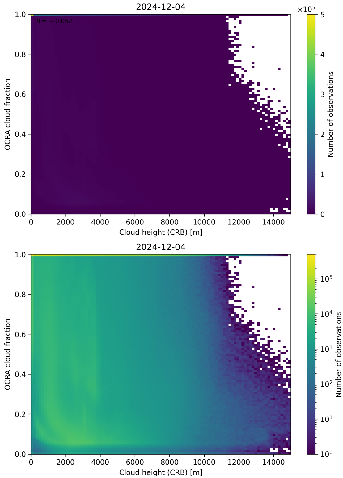
Figure 81: Scatter density plot of “Cloud height (CRB)” against “OCRA cloud fraction” for 2024-12-03 to 2024-12-05.
