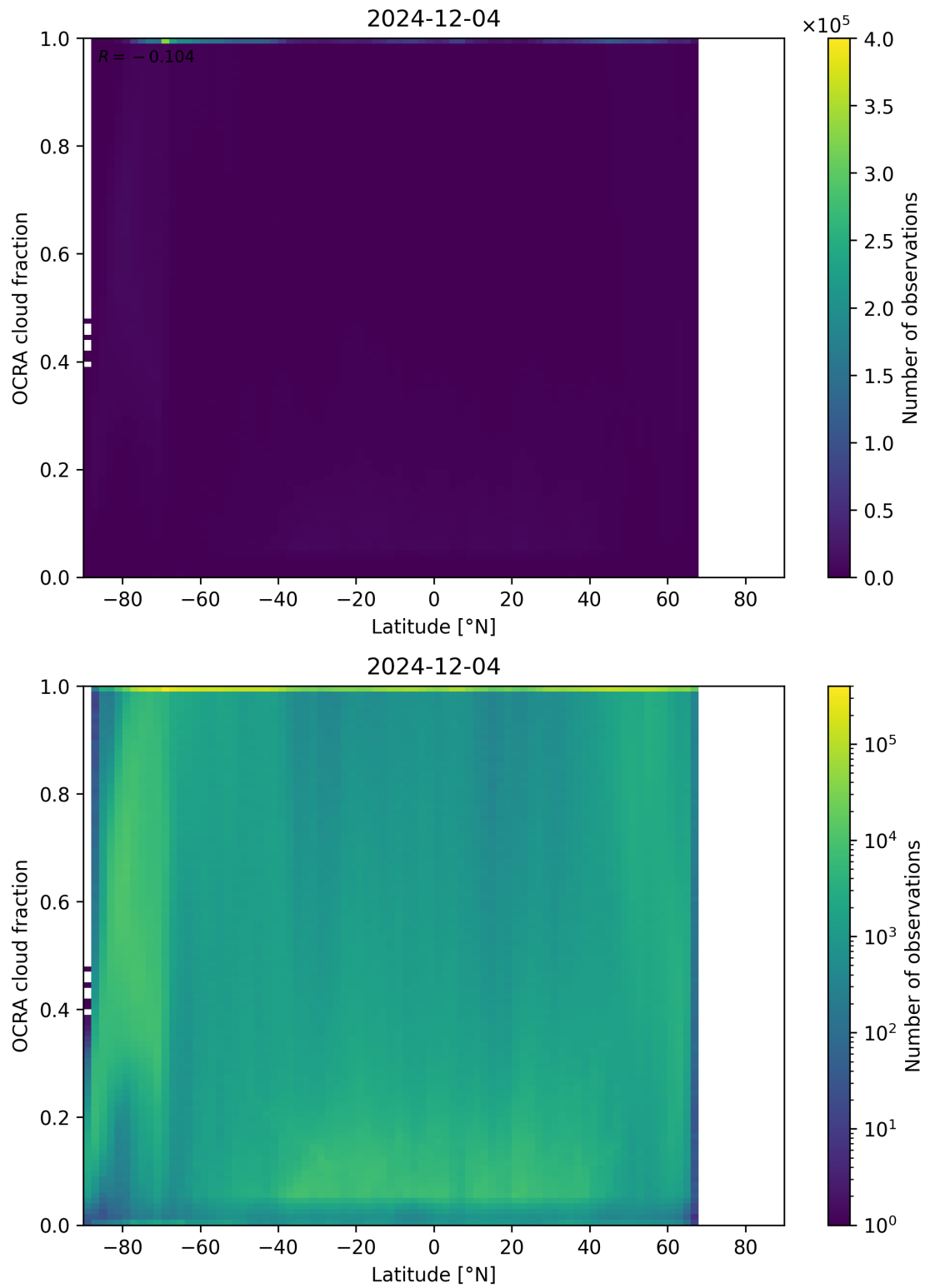
Figure 93: Scatter density plot of “Latitude” against “OCRA cloud fraction” for 2024-12-03 to 2024-12-05.
