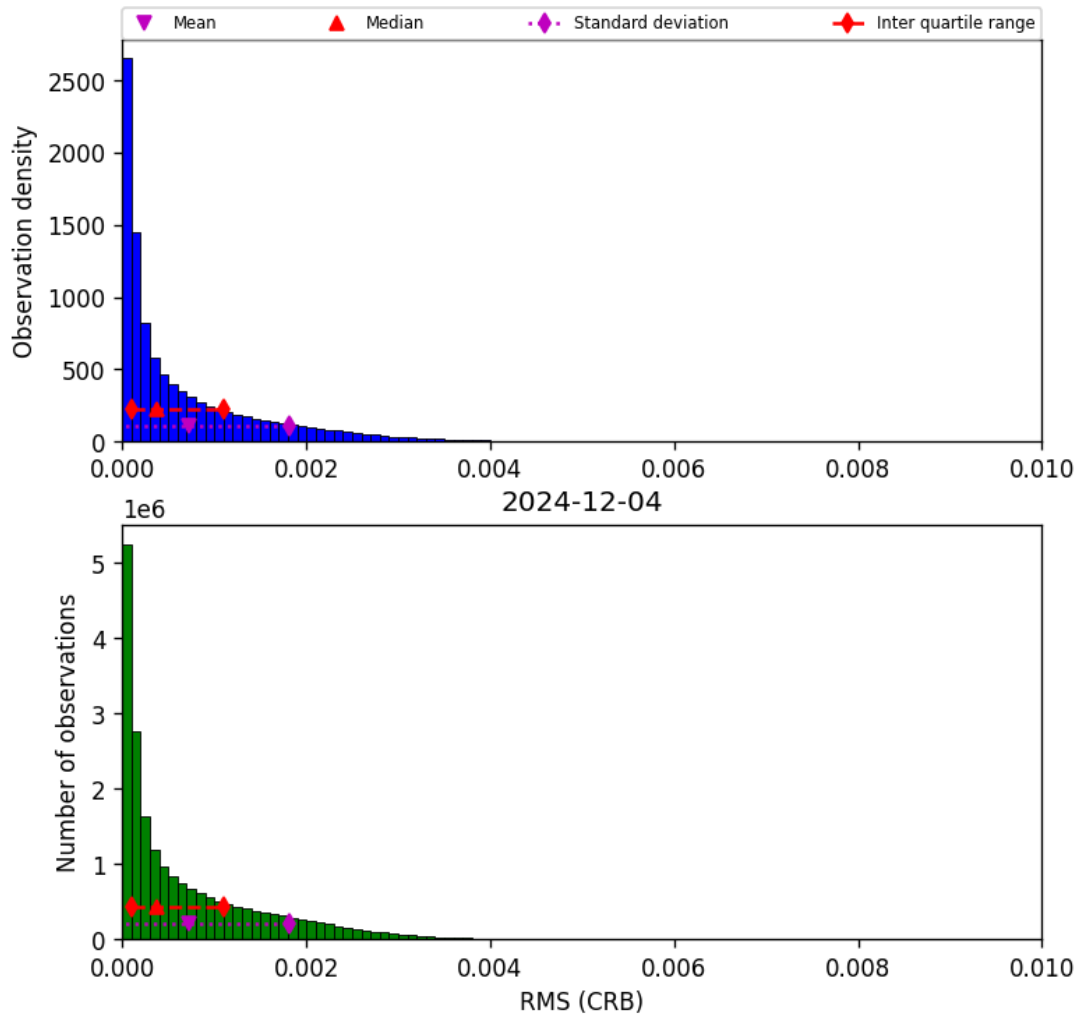
Figure 48: Histogram of “RMS (CRB)” for 2024-12-03 to 2024-12-05
