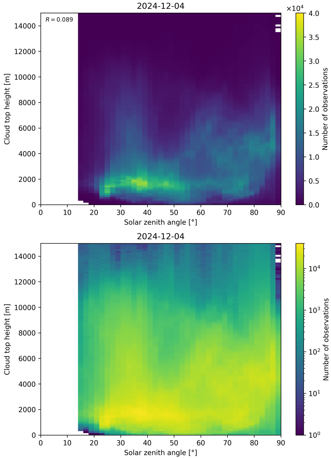
Figure 104: Scatter density plot of “Solar zenith angle” against “Cloud top height” for 2024-12-03 to 2024-12-05.
