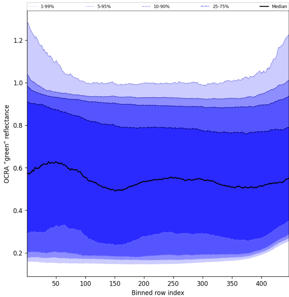
Figure 68: Along track statistics of "OCRA "green" reflectance" for 2024-12-03 to 2024-12-05
