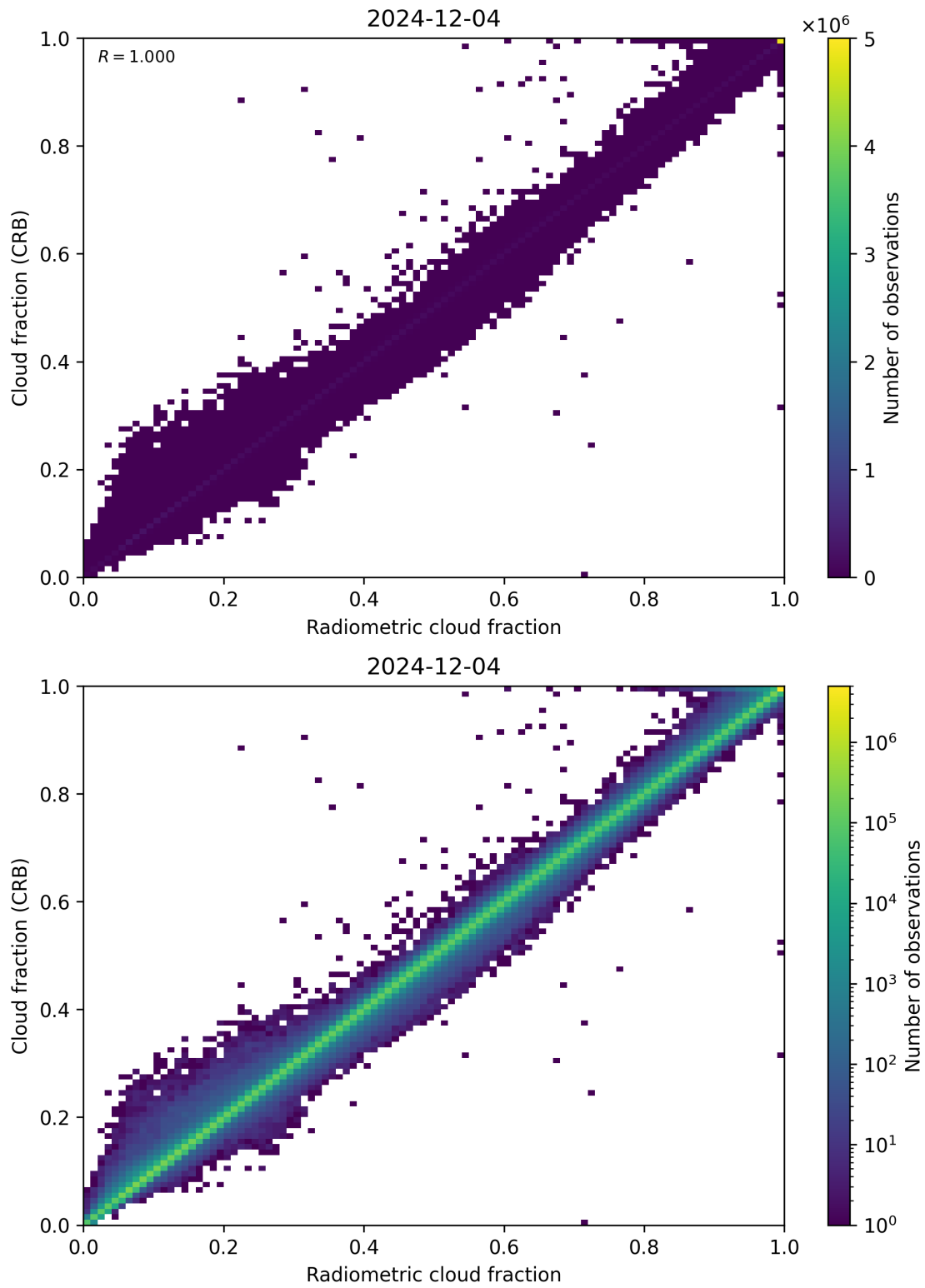
Figure 73: Scatter density plot of “Radiometric cloud fraction” against “Cloud fraction (CRB)” for 2024-12-03 to 2024-12-05.
