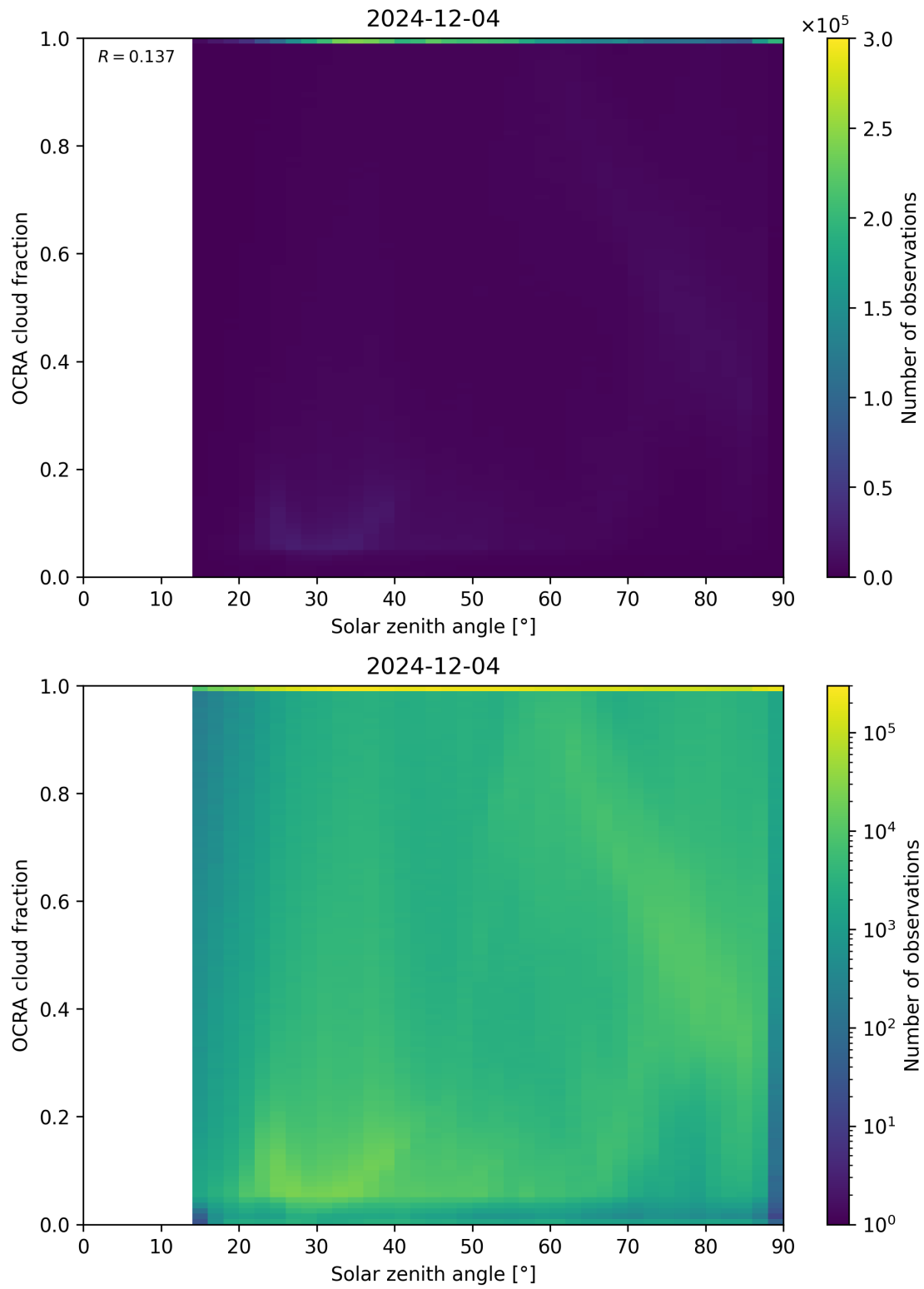
Figure 100: Scatter density plot of “Solar zenith angle” against “OCRA cloud fraction” for 2024-12-03 to 2024-12-05.
