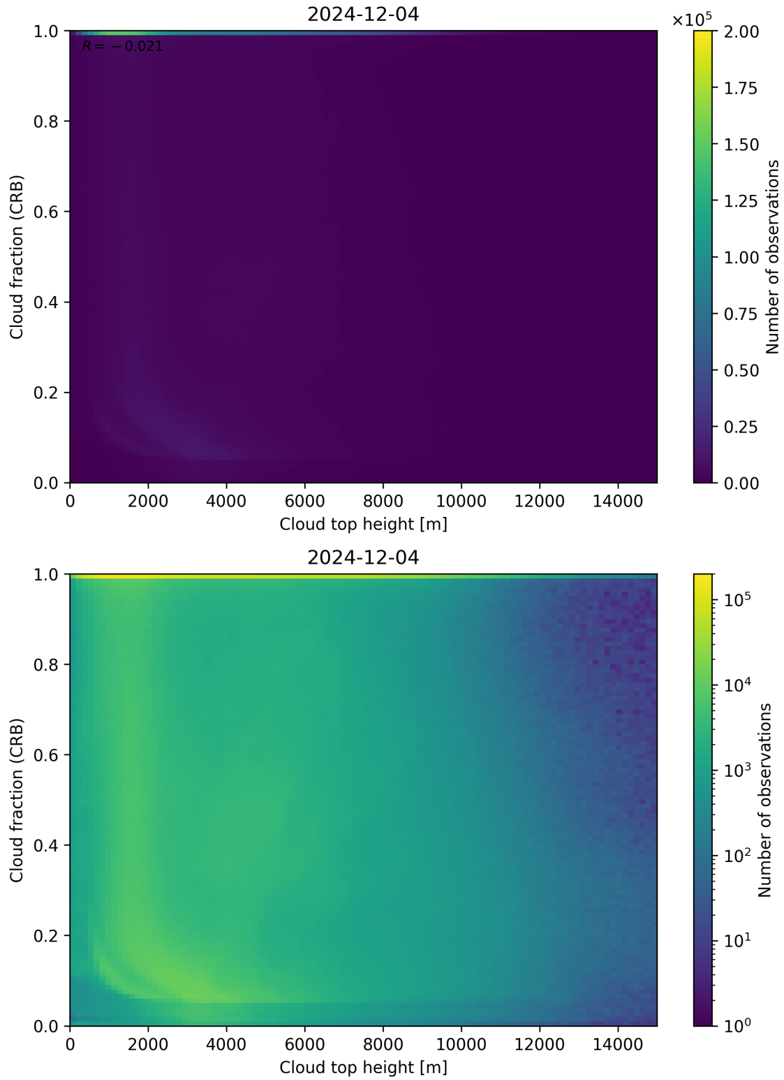
Figure 88: Scatter density plot of “Cloud top height” against “Cloud fraction (CRB)” for 2024-12-03 to 2024-12-05.
