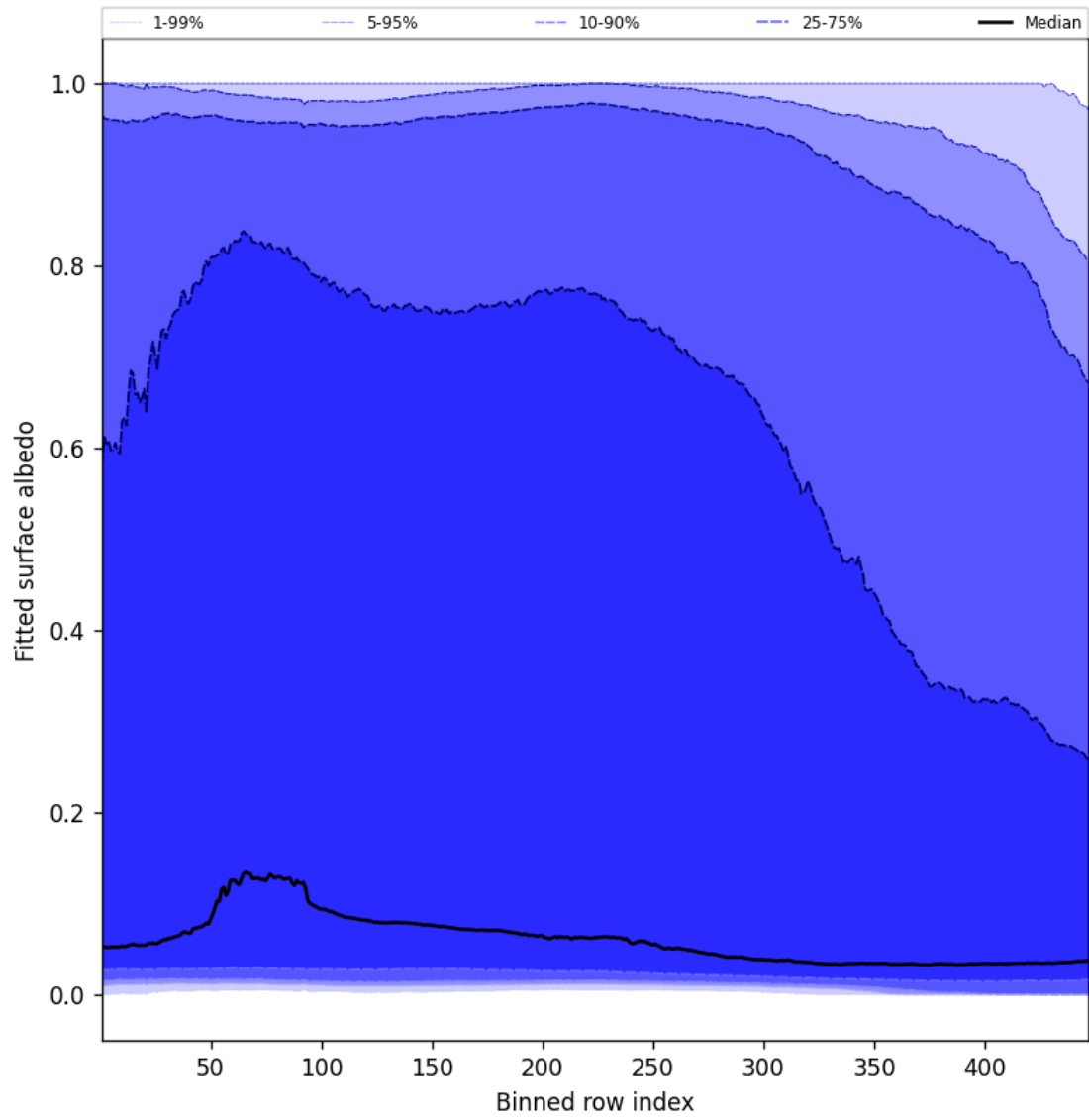
Figure 61: Along track statistics of “Fitted surface albedo” for 2024-12-03 to 2024-12-05
