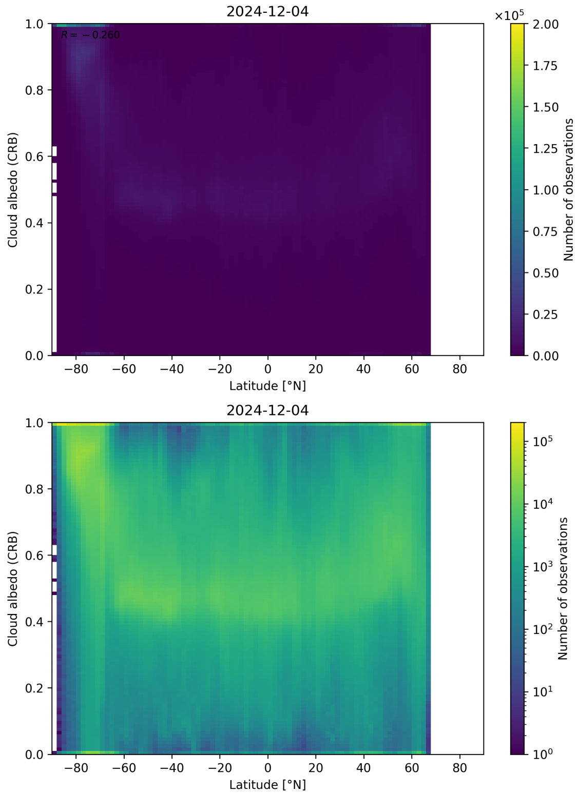
Figure 91: Scatter density plot of “Latitude” against “Cloud albedo (CRB)” for 2024-12-03 to 2024-12-05.
