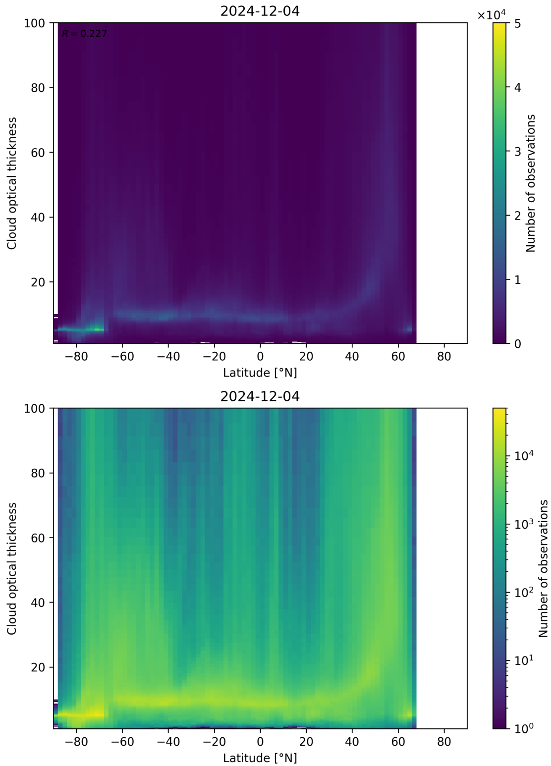
Figure 96: Scatter density plot of “Latitude” against “Cloud optical thickness” for 2024-12-03 to 2024-12-05.
