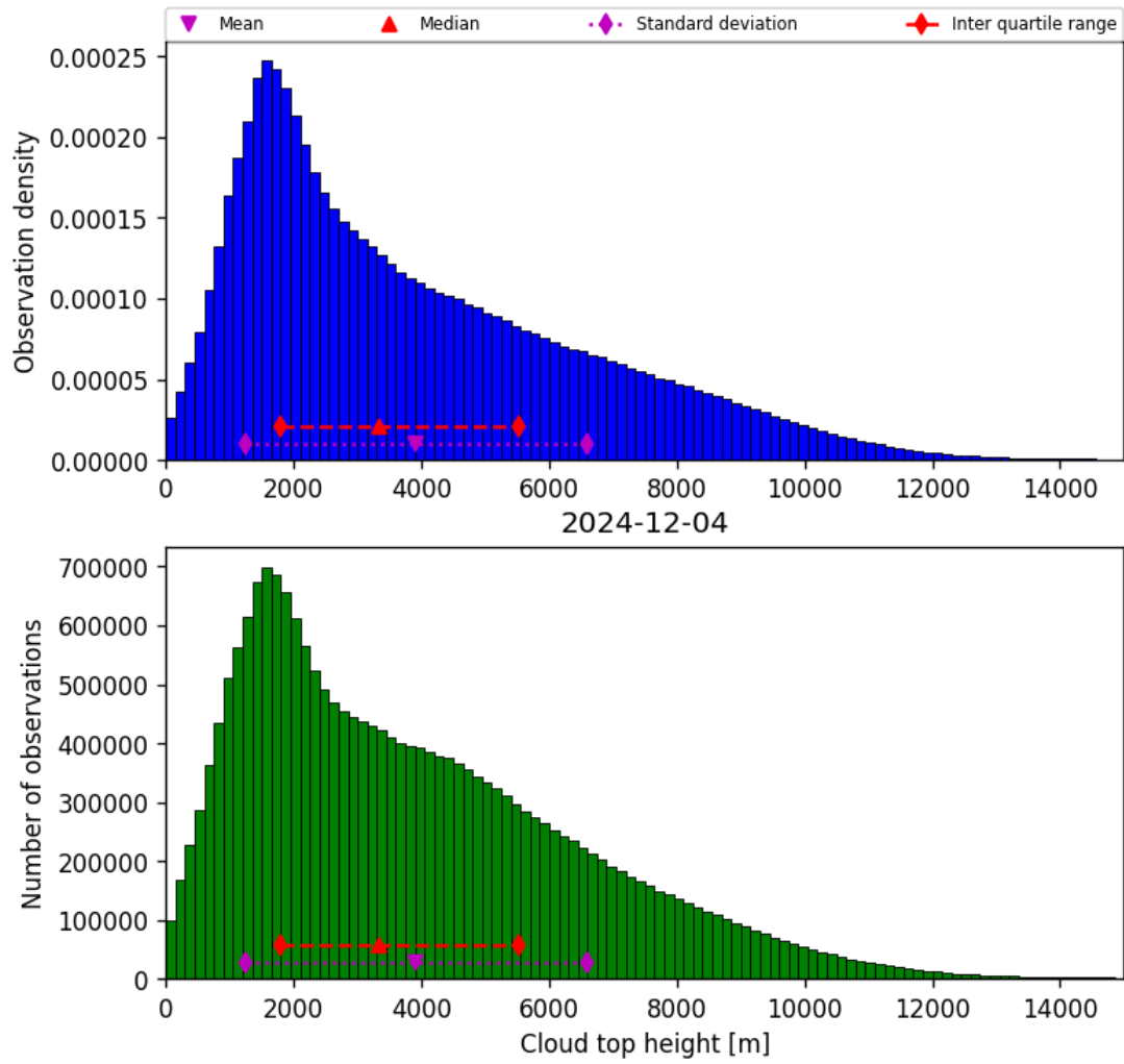
Figure 40: Histogram of “Cloud top height” for 2024-12-03 to 2024-12-05
