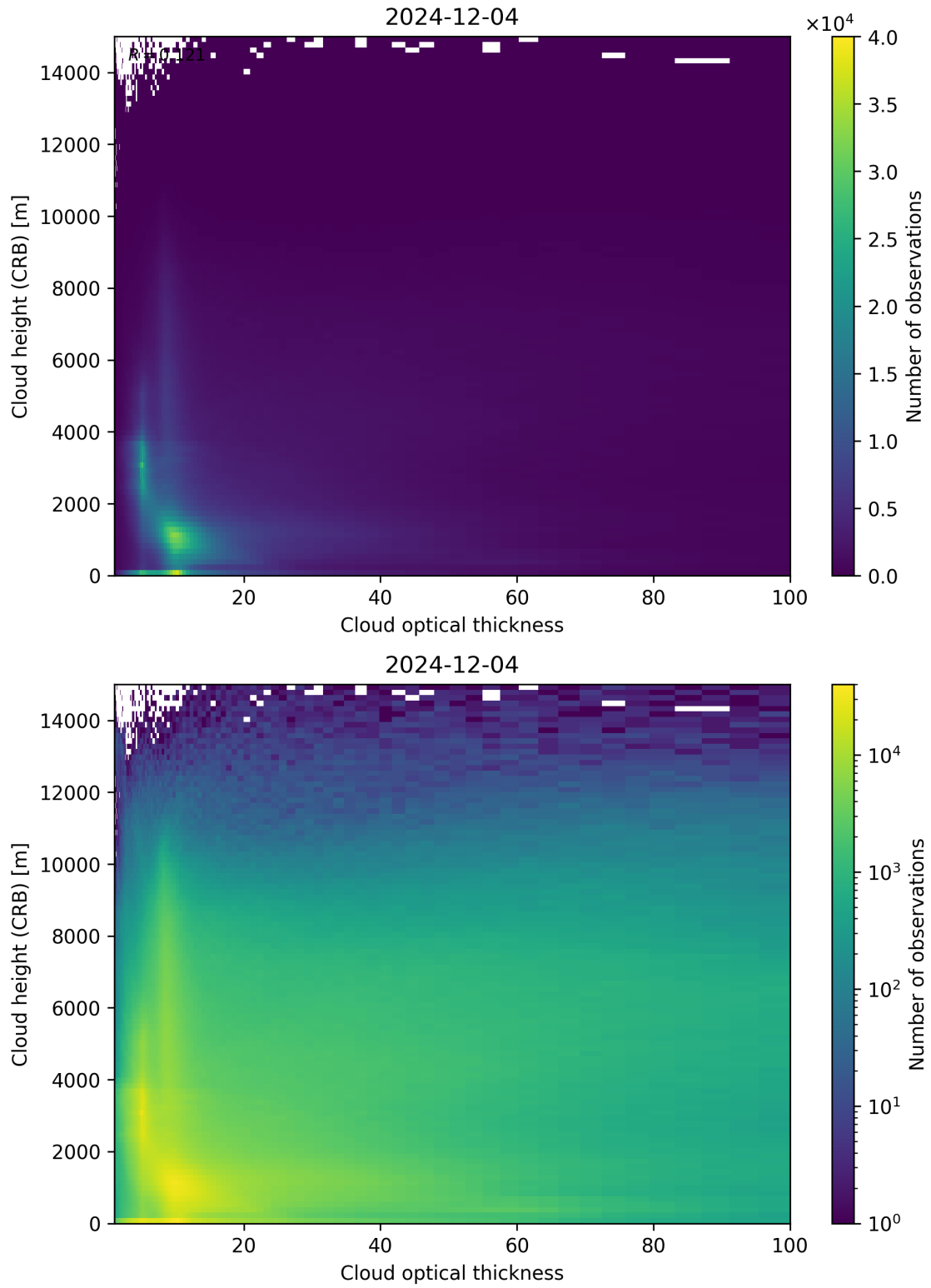
Figure 85: Scatter density plot of “Cloud optical thickness” against “Cloud height (CRB)” for 2024-12-03 to 2024-12-05.
