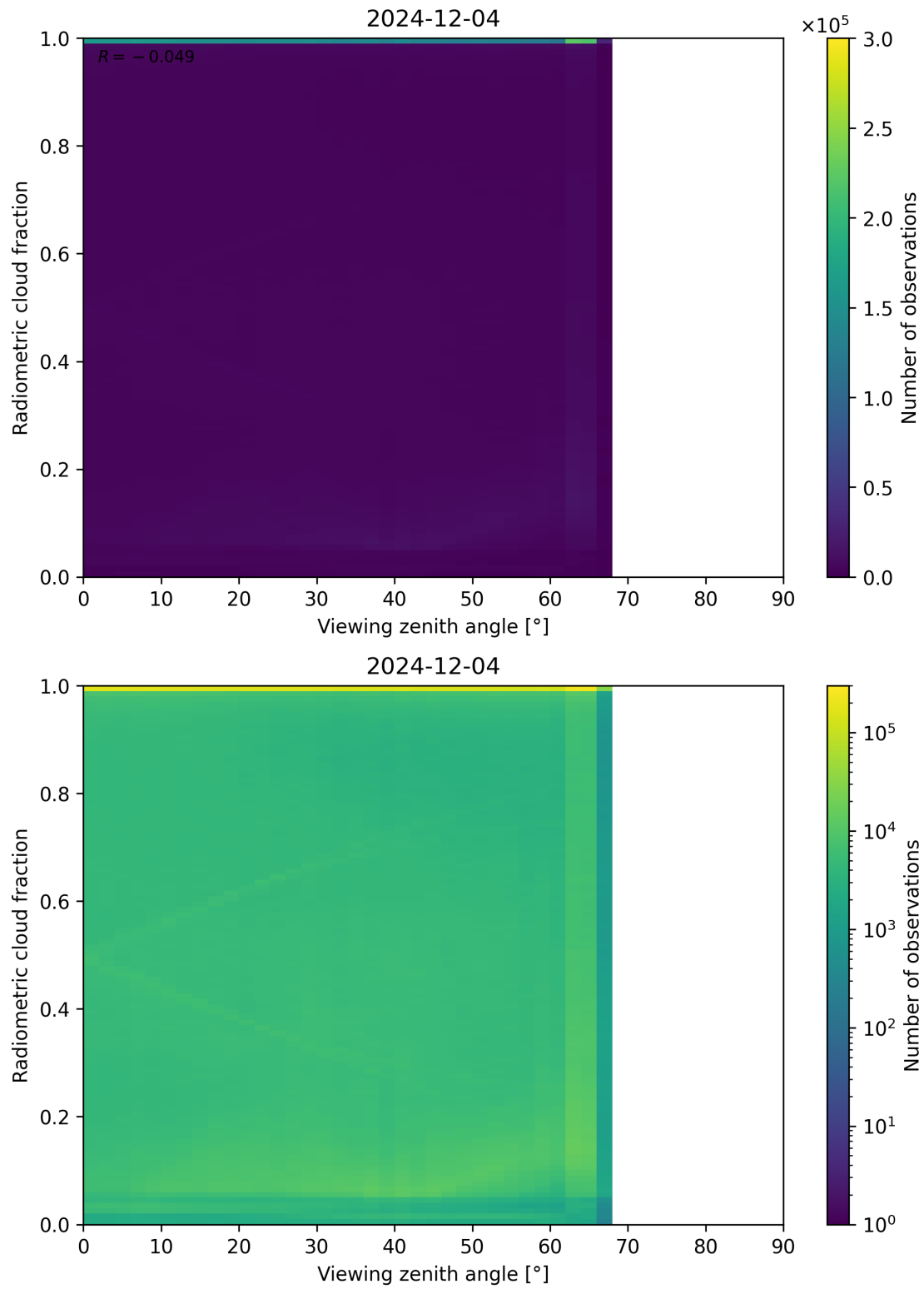
Figure 107: Scatter density plot of “Viewing zenith angle” against “Radiometric cloud fraction” for 2024-12-03 to 2024-12-05.
