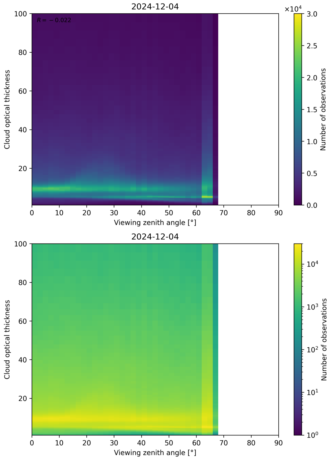
Figure 111: Scatter density plot of “Viewing zenith angle” against “Cloud optical thickness” for 2024-12-03 to 2024-12-05.
