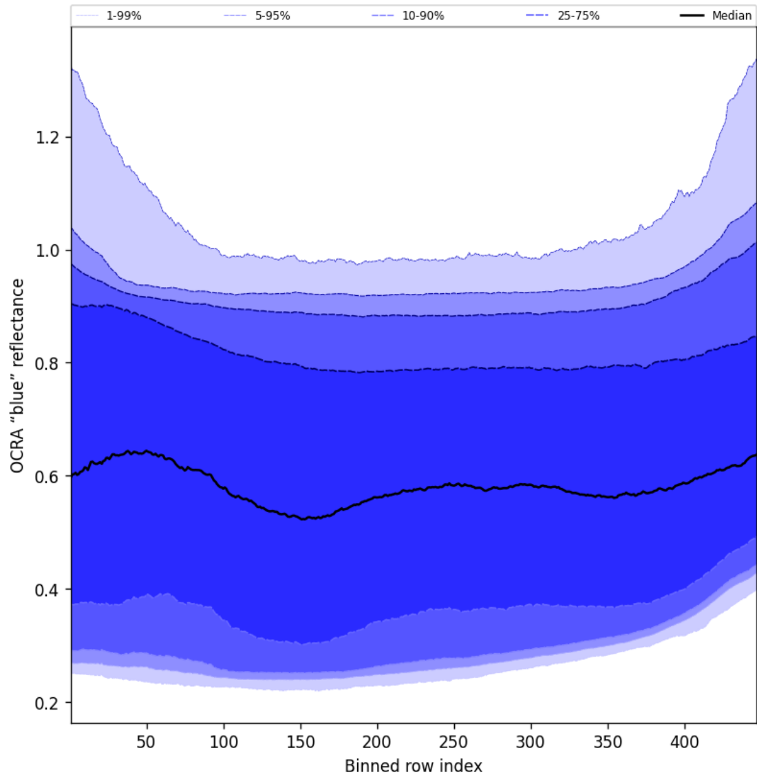
Figure 67: Along track statistics of “OCRA “blue” reflectance” for 2024-12-03 to 2024-12-05
