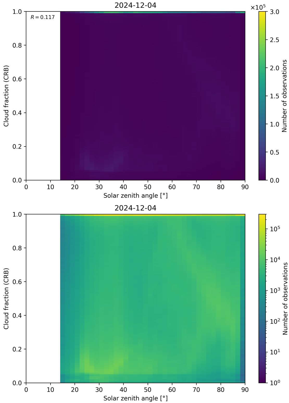
Figure 101: Scatter density plot of “Solar zenith angle” against “Cloud fraction (CRB)” for 2024-12-03 to 2024-12-05.
