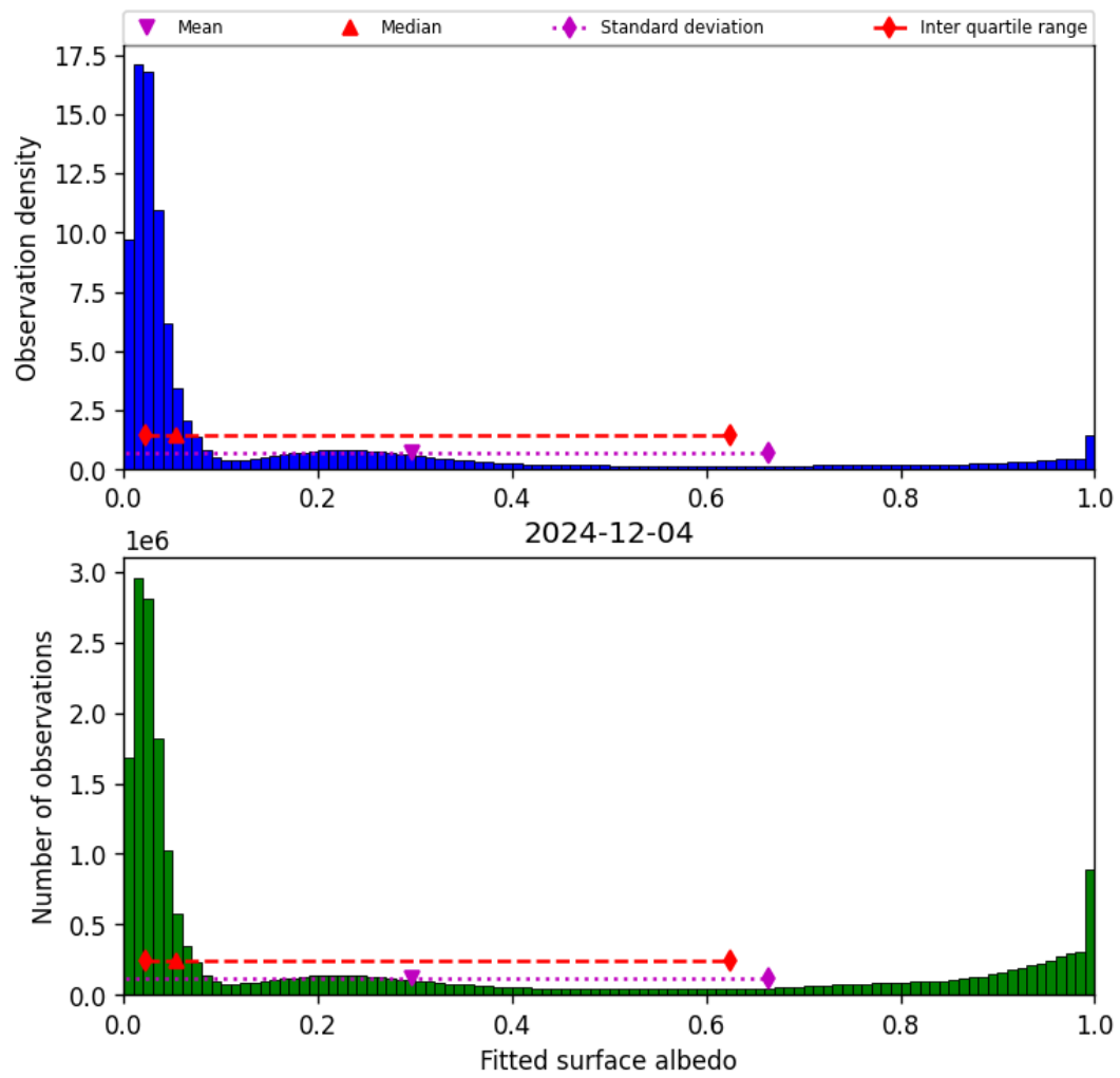
Figure 45: Histogram of “Fitted surface albedo” for 2024-12-03 to 2024-12-05
