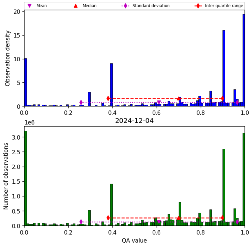
Figure 38: Histogram of “QA value” for 2024-12-03 to 2024-12-05
