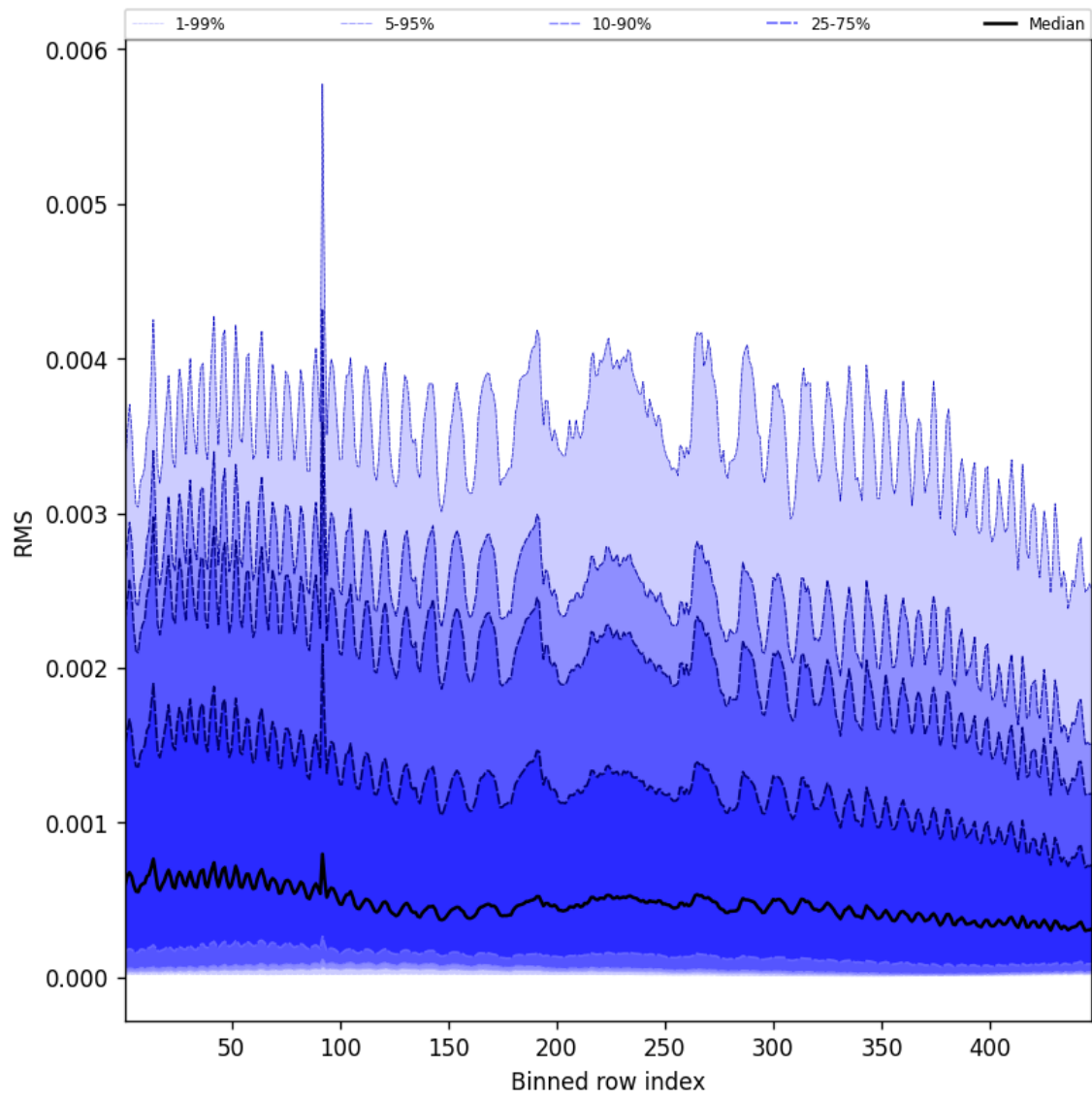
Figure 63: Along track statistics of “RMS” for 2024-12-03 to 2024-12-05
