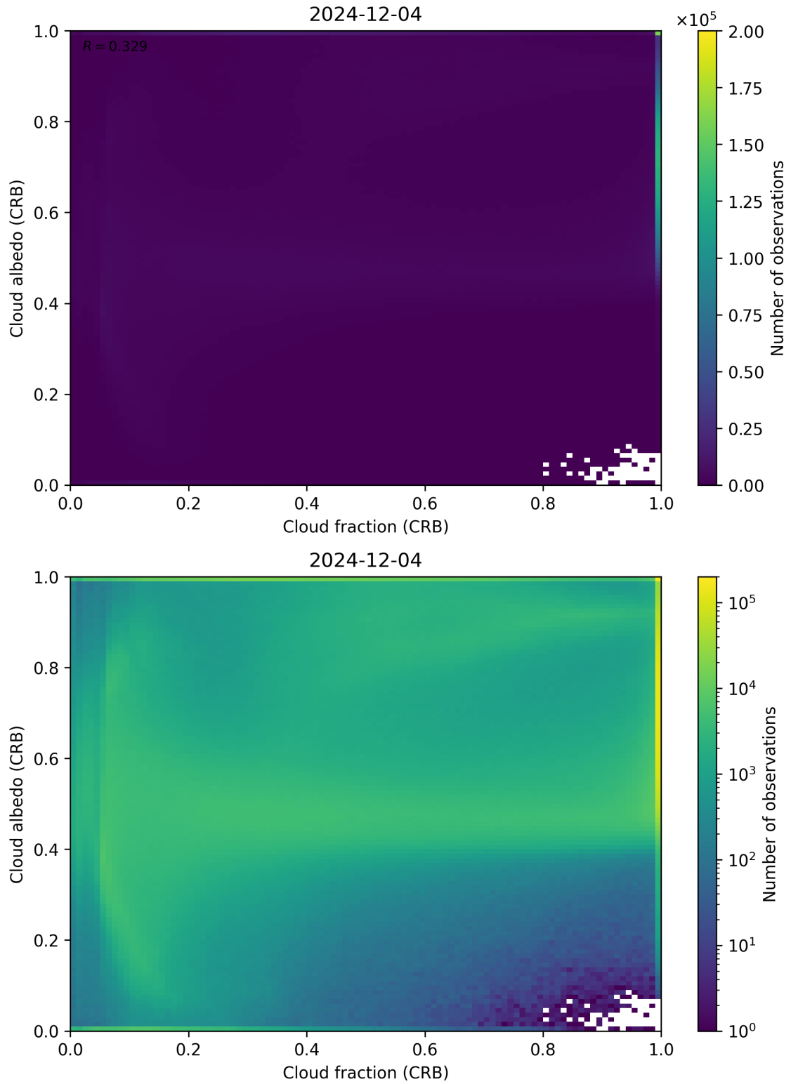
Figure 77: Scatter density plot of “Cloud fraction (CRB)” against “Cloud albedo (CRB)” for 2024-12-03 to 2024-12-05.
