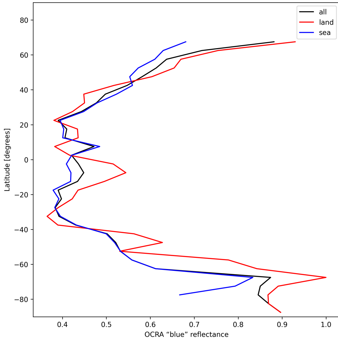
Figure 35: Zonal average of “OCRA “blue” reflectance” for 2024-12-03 to 2024-12-05.
