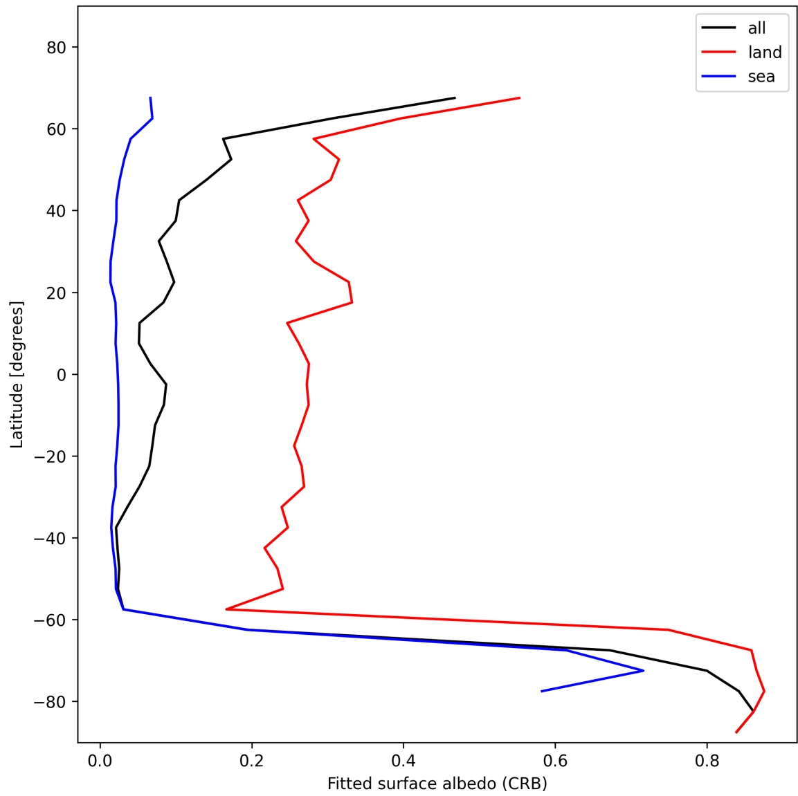
Figure 30: Zonal average of “Fitted surface albedo (CRB)” for 2024-12-03 to 2024-12-05.
