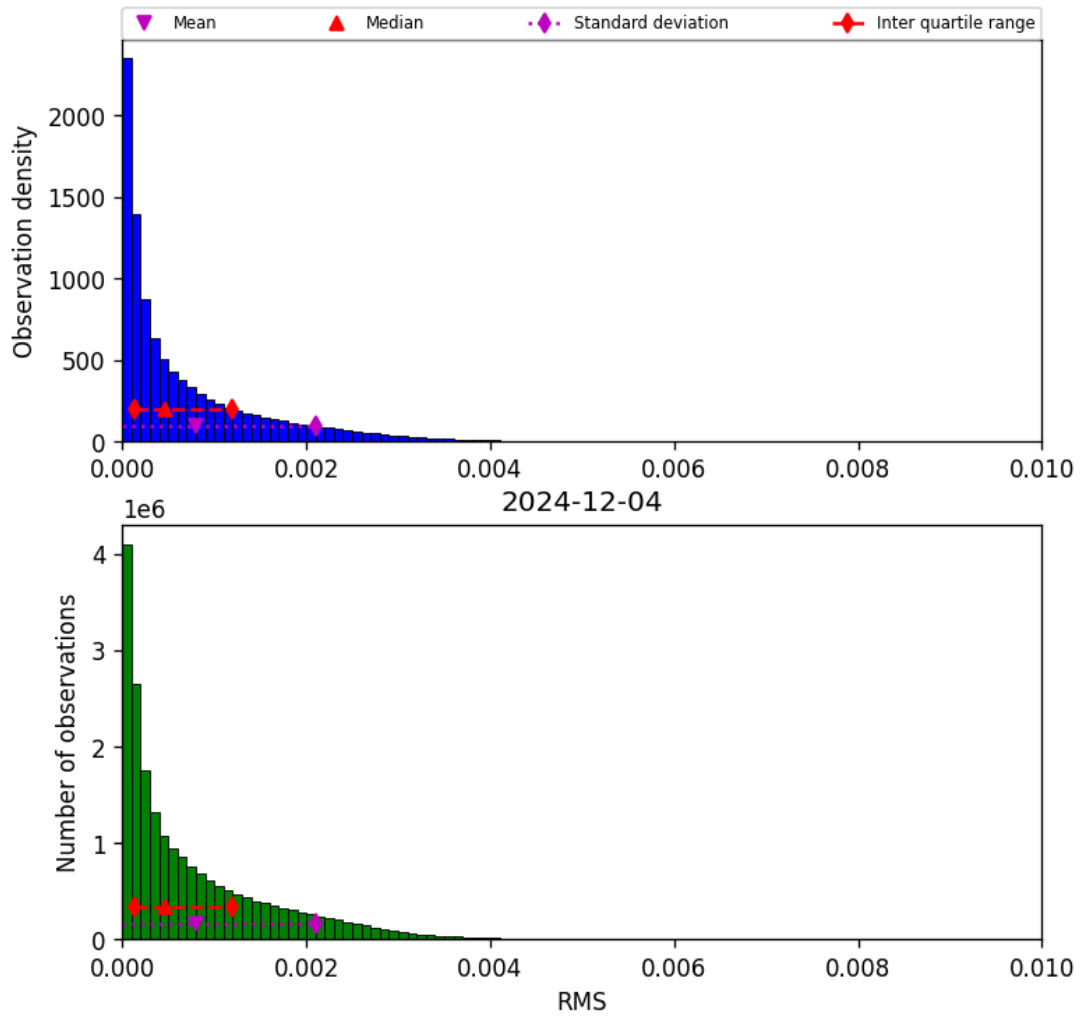
Figure 47: Histogram of “RMS” for 2024-12-03 to 2024-12-05
