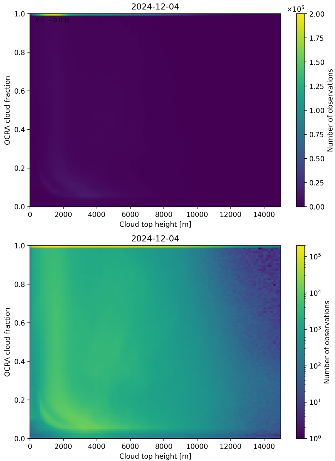
Figure 87: Scatter density plot of “Cloud top height” against “OCRA cloud fraction” for 2024-12-03 to 2024-12-05.
