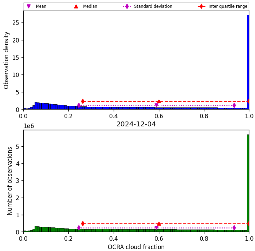
Figure 50: Histogram of “OCRA cloud fraction” for 2024-12-03 to 2024-12-05
