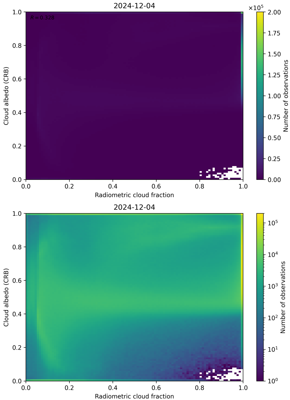
Figure 71: Scatter density plot of “Radiometric cloud fraction” against “Cloud albedo (CRB)” for 2024-12-03 to 2024-12-05.
