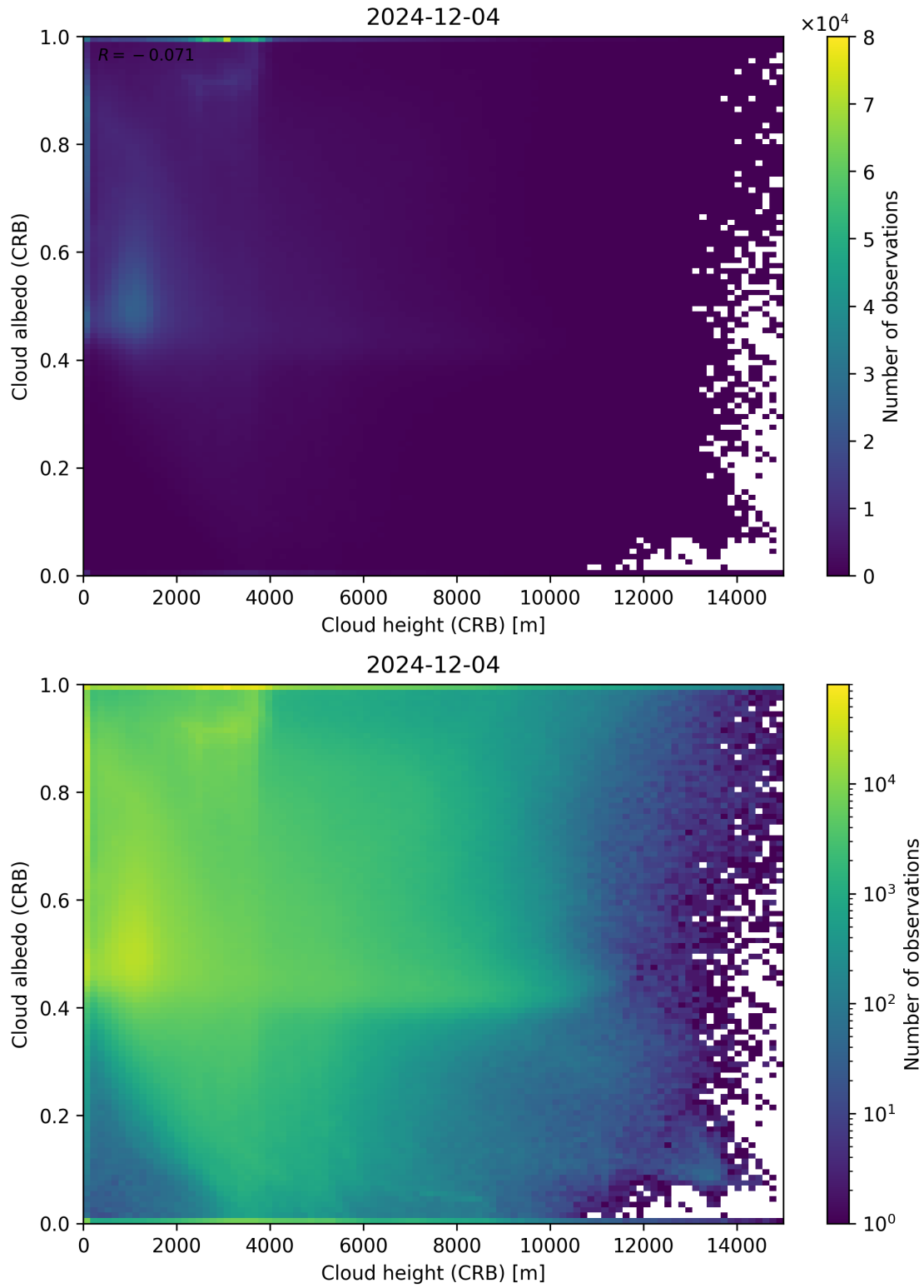
Figure 80: Scatter density plot of “Cloud height (CRB)” against “Cloud albedo (CRB)” for 2024-12-03 to 2024-12-05.
