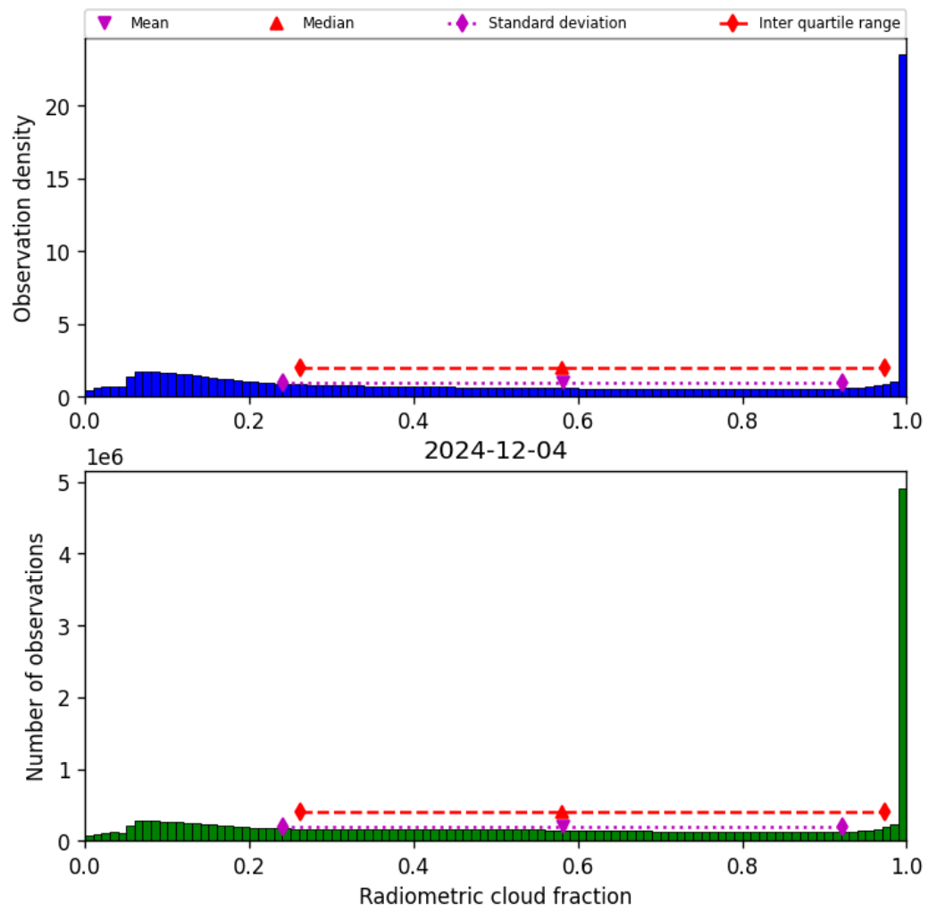
Figure 39: Histogram of “Radiometric cloud fraction” for 2024-12-03 to 2024-12-05
