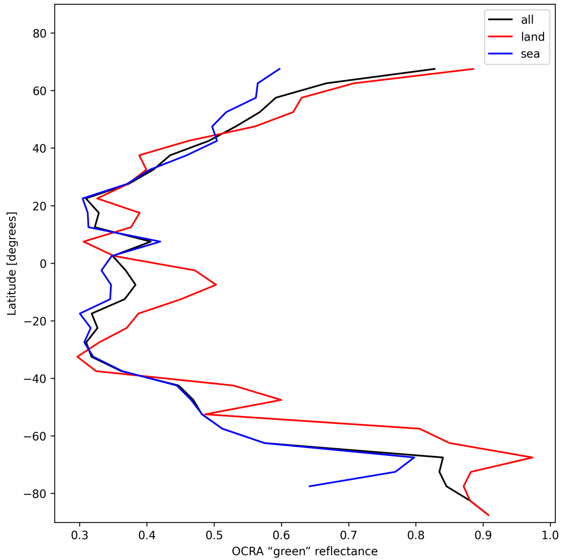
Figure 36: Zonal average of “OCRA “green” reflectance” for 2024-12-03 to 2024-12-05.
