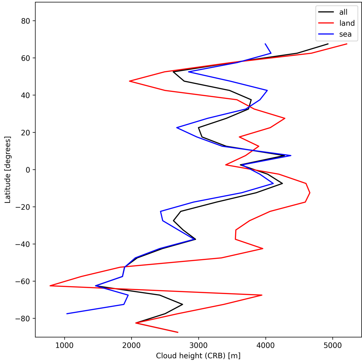
Figure 27: Zonal average of “Cloud height (CRB)” for 2024-12-03 to 2024-12-05.
