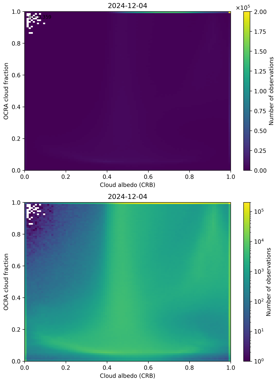
Figure 70: Scatter density plot of “Cloud albedo (CRB)” against “OCRA cloud fraction” for 2024-12-03 to 2024-12-05.
