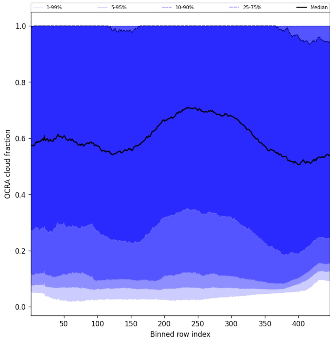
Figure 66: Along track statistics of “OCRA cloud fraction” for 2024-12-03 to 2024-12-05
