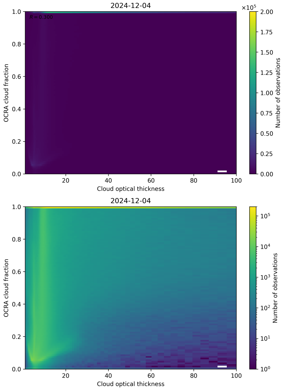
Figure 83: Scatter density plot of “Cloud optical thickness” against “OCRA cloud fraction” for 2024-12-03 to 2024-12-05.
