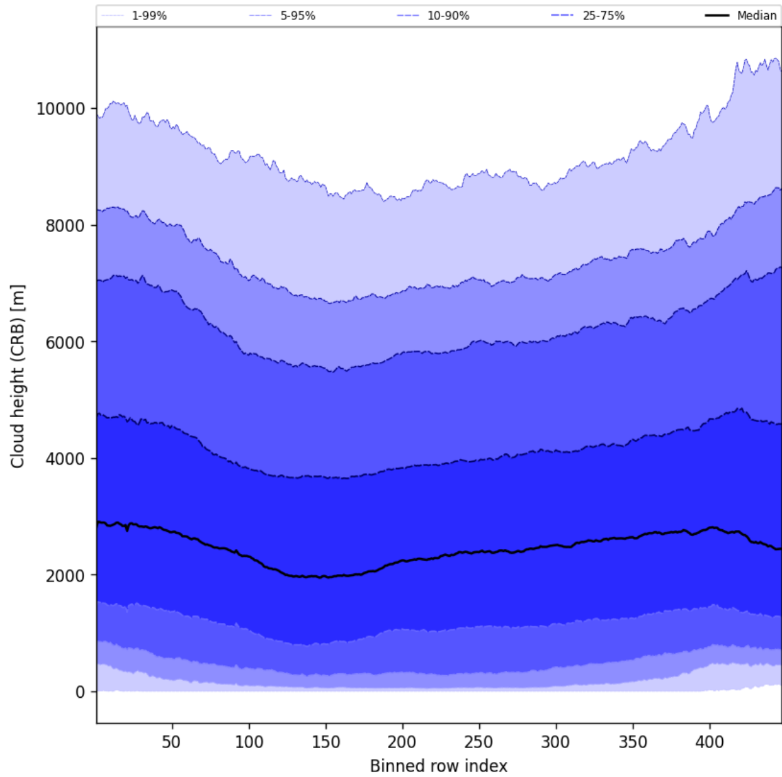
Figure 59: Along track statistics of “Cloud height (CRB)” for 2024-12-03 to 2024-12-05
