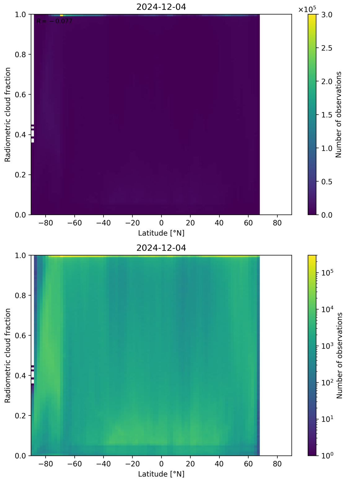
Figure 92: Scatter density plot of “Latitude” against “Radiometric cloud fraction” for 2024-12-03 to 2024-12-05.
