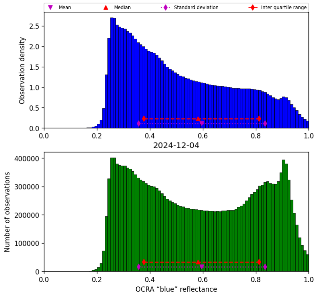
Figure 51: Histogram of “OCRA “blue” reflectance” for 2024-12-03 to 2024-12-05
