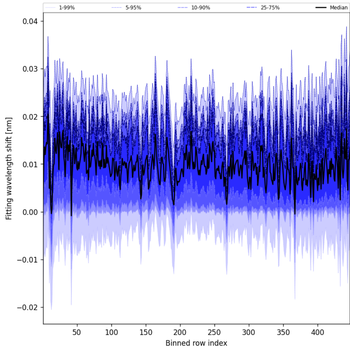
Figure 65: Along track statistics of “Fitting wavelength shift” for 2024-12-03 to 2024-12-05
