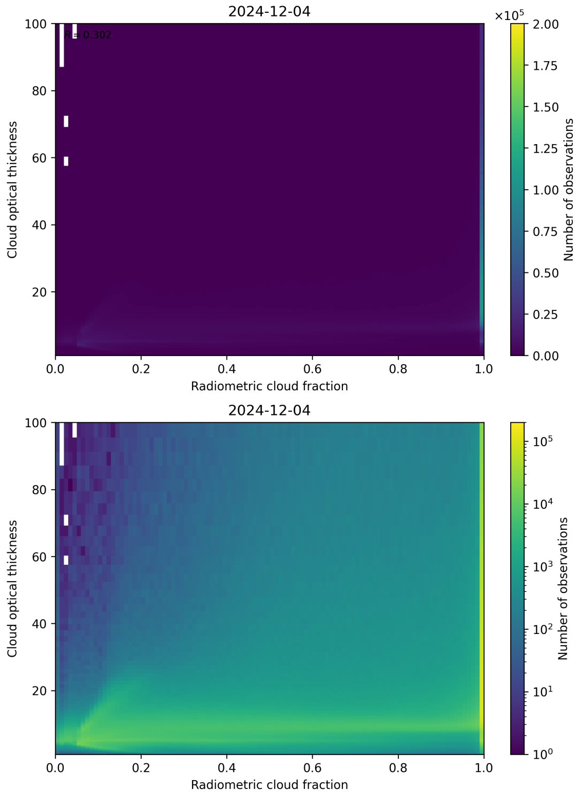
Figure 75: Scatter density plot of “Radiometric cloud fraction” against “Cloud optical thickness” for 2024-12-03 to 2024-12-05.
