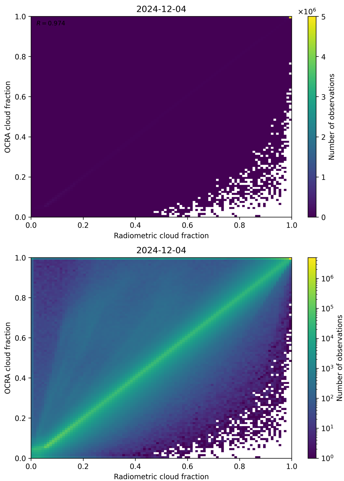
Figure 72: Scatter density plot of “Radiometric cloud fraction” against “OCRA cloud fraction” for 2024-12-03 to 2024-12-05.
