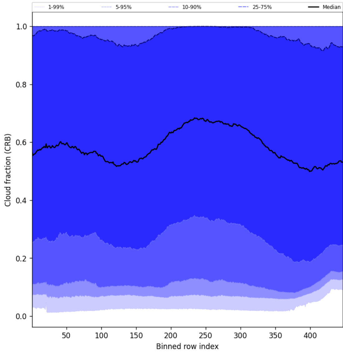
Figure 58: Along track statistics of “Cloud fraction (CRB)” for 2024-12-03 to 2024-12-05
