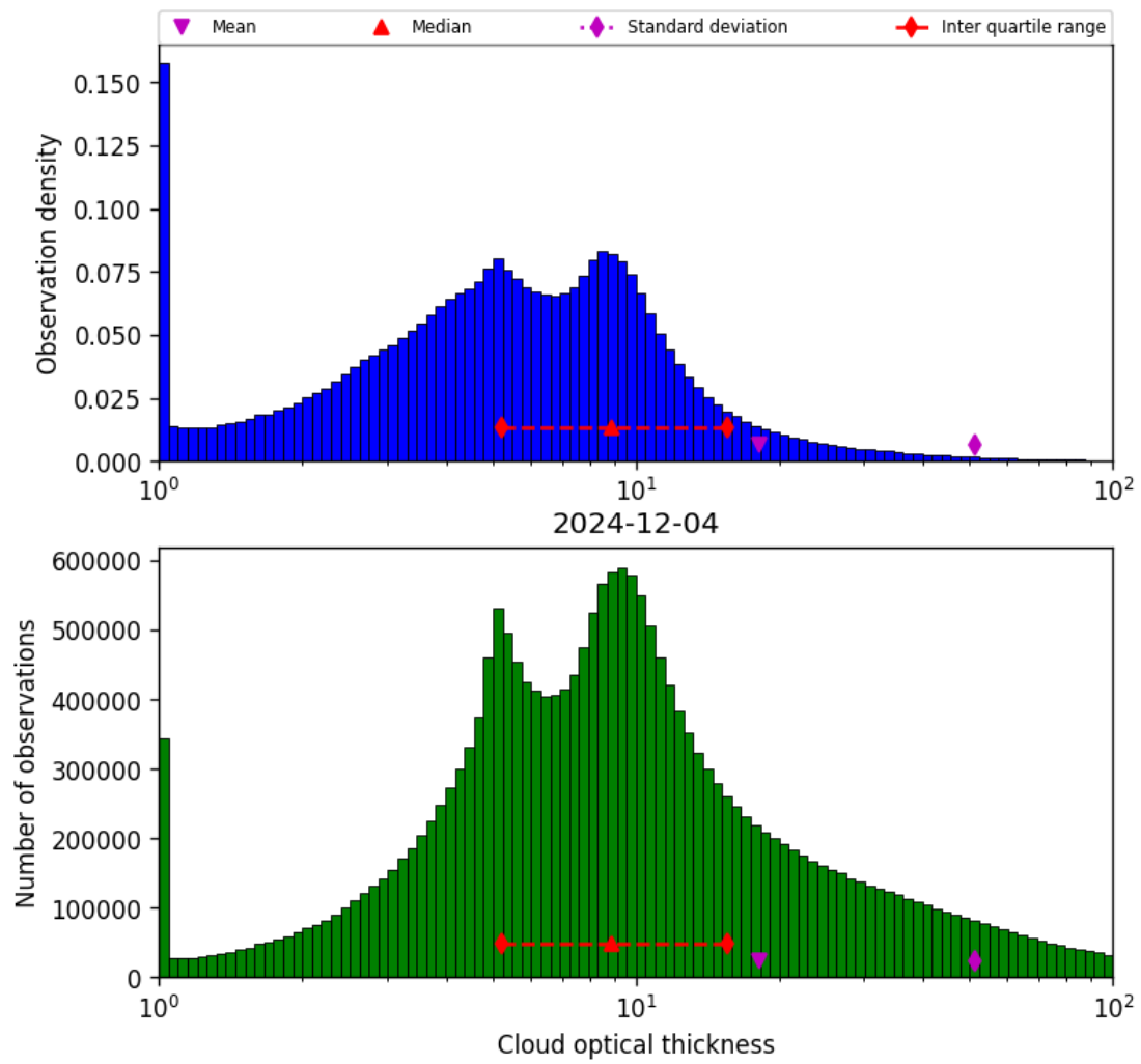
Figure 41: Histogram of “Cloud optical thickness” for 2024-12-03 to 2024-12-05
