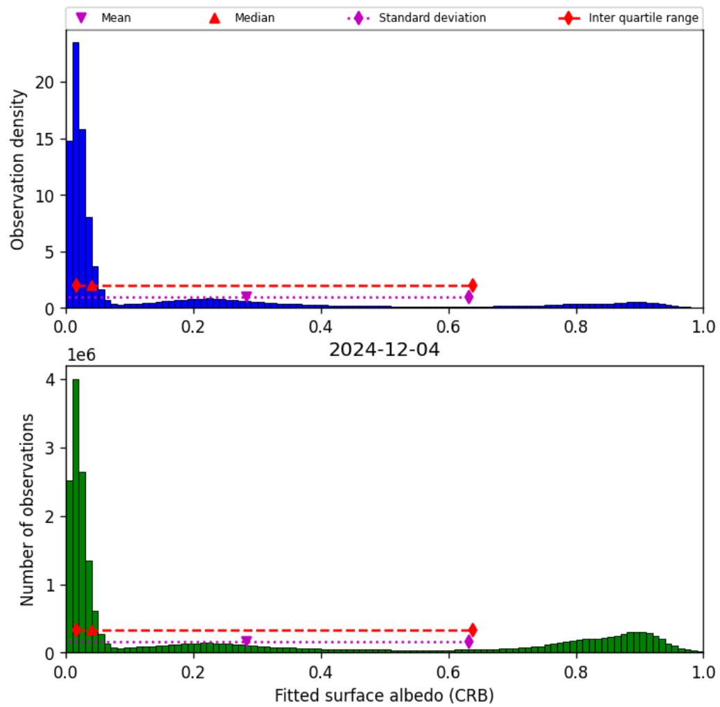
Figure 46: Histogram of “Fitted surface albedo (CRB)” for 2024-12-03 to 2024-12-05
