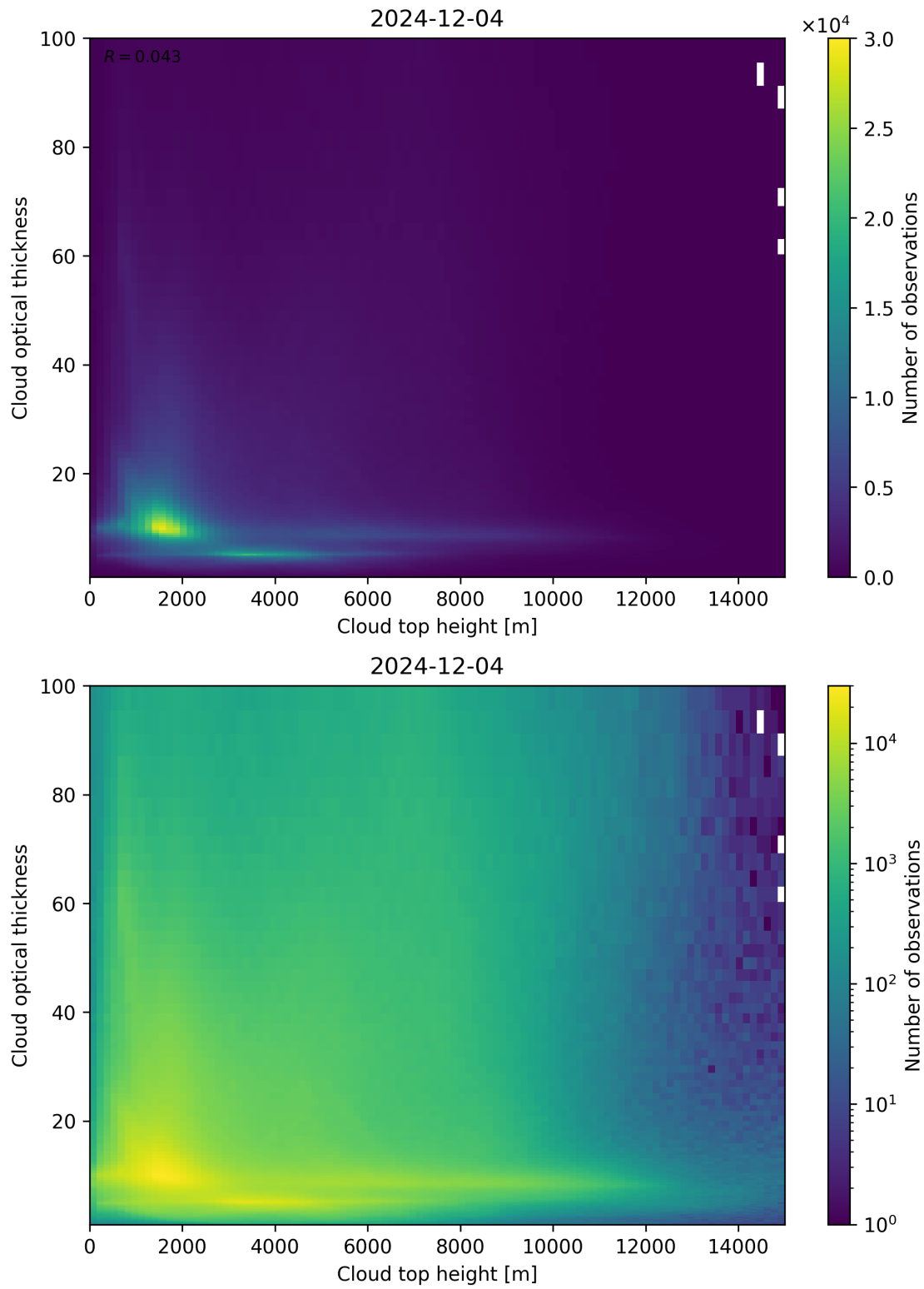
Figure 90: Scatter density plot of “Cloud top height” against “Cloud optical thickness” for 2024-12-03 to 2024-12-05.
