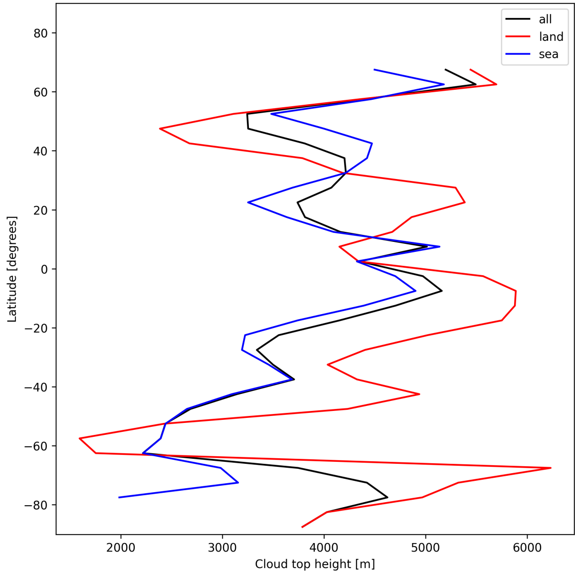
Figure 24: Zonal average of “Cloud top height” for 2024-12-03 to 2024-12-05.
