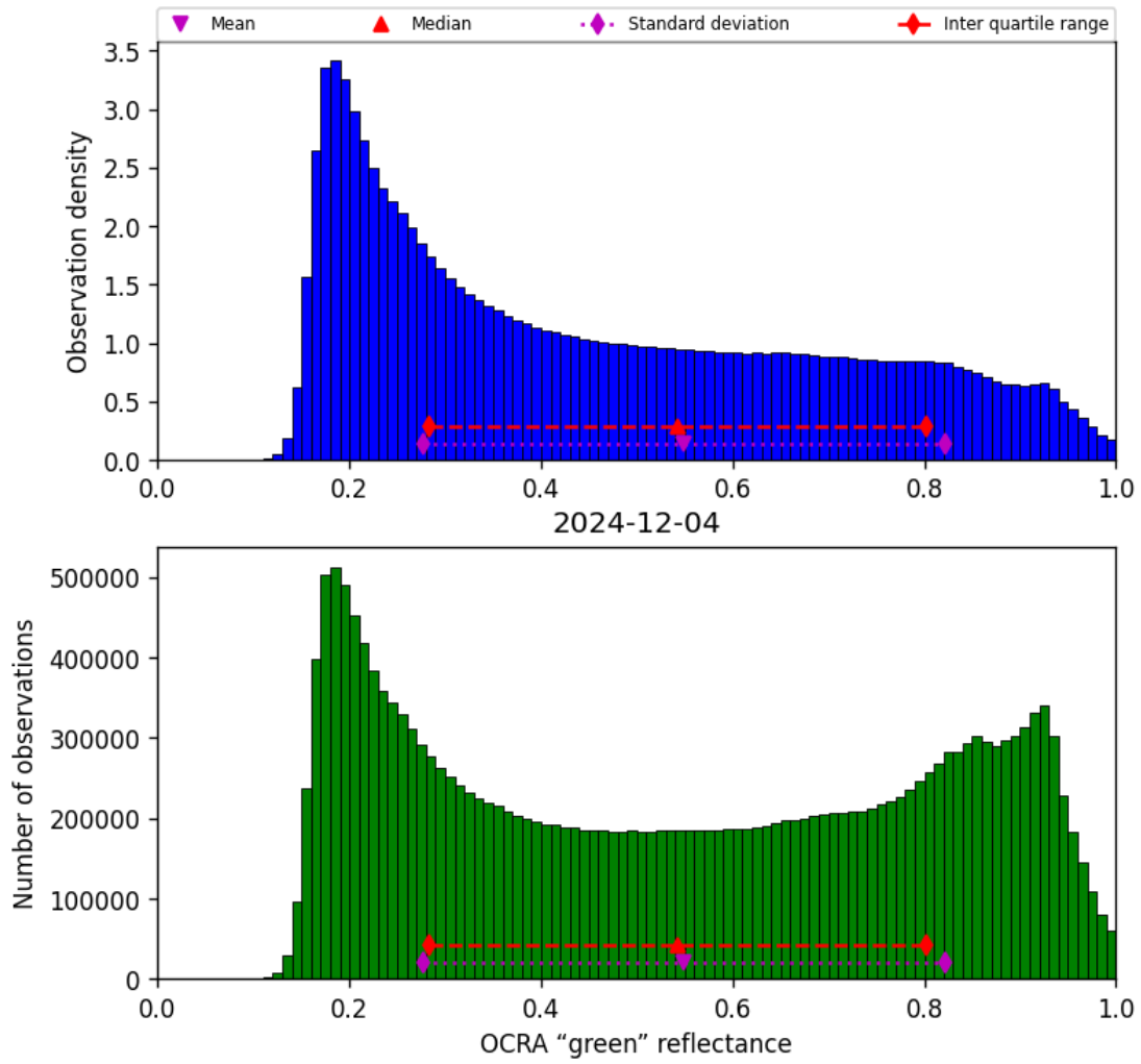
Figure 52: Histogram of “OCRA “green” reflectance” for 2024-12-03 to 2024-12-05
