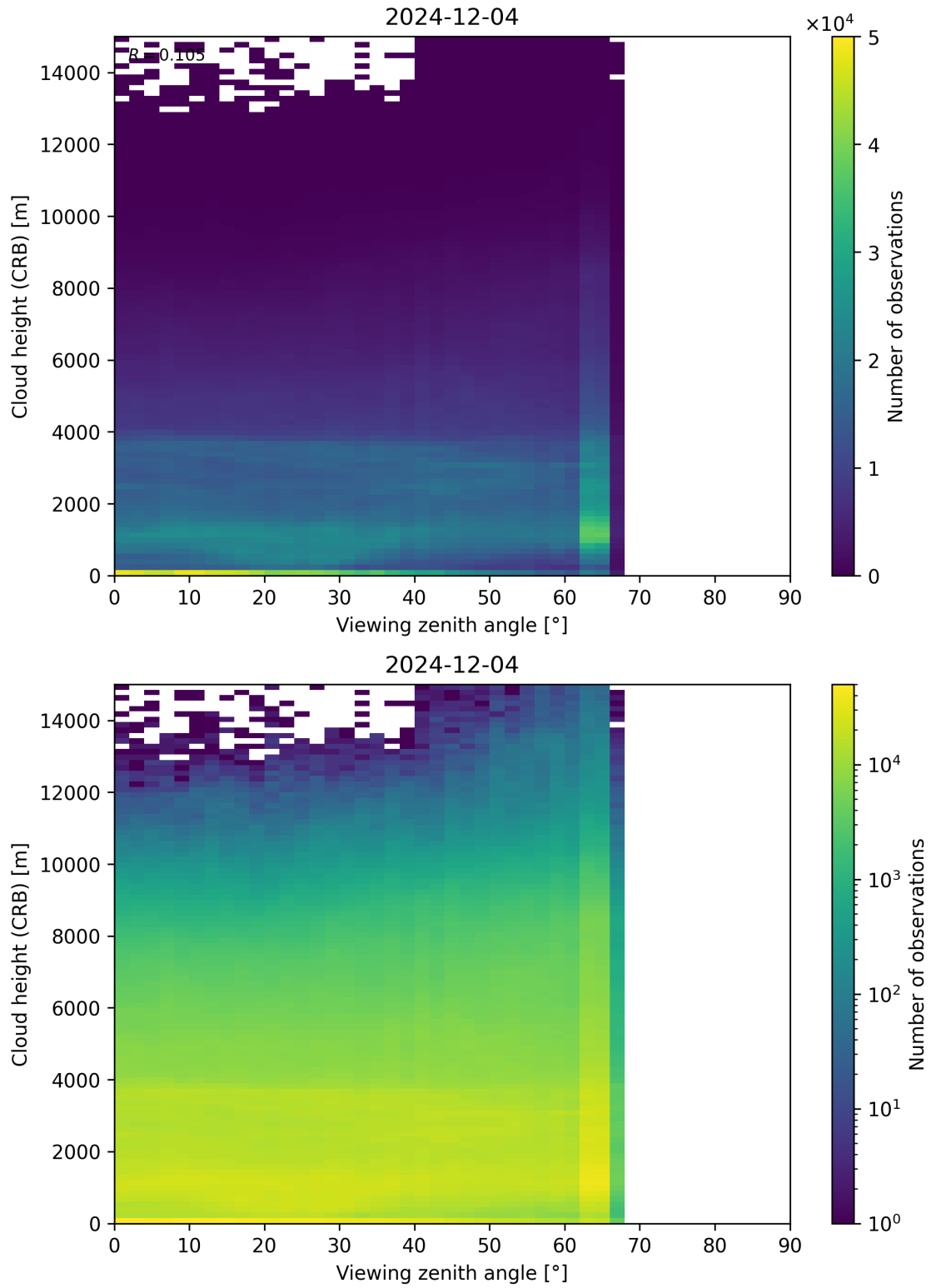
Figure 110: Scatter density plot of “Viewing zenith angle” against “Cloud height (CRB)” for 2024-12-03 to 2024-12-05.
