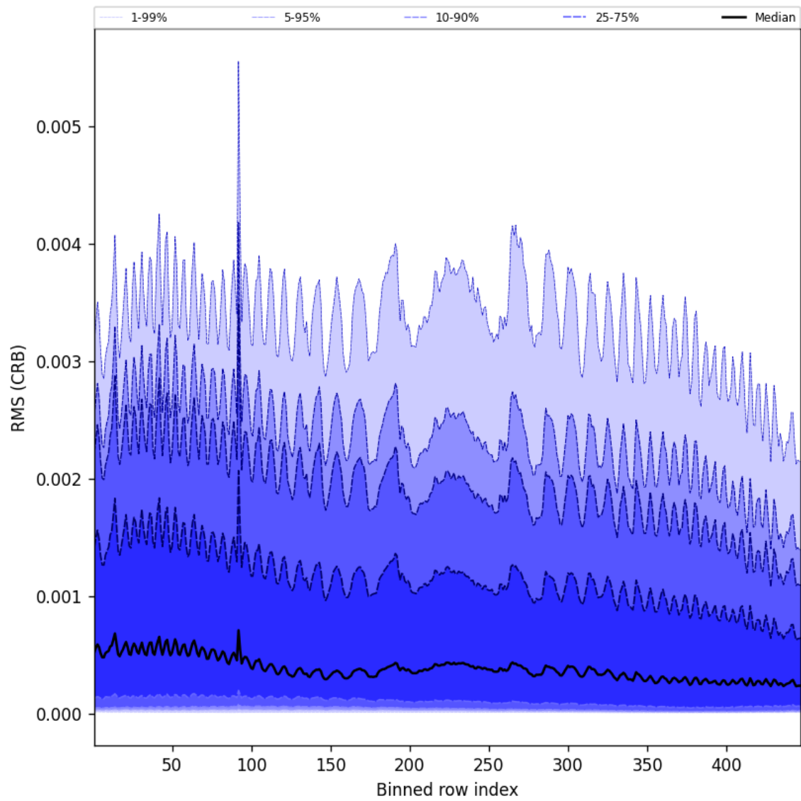
Figure 64: Along track statistics of “RMS (CRB)” for 2024-12-03 to 2024-12-05
