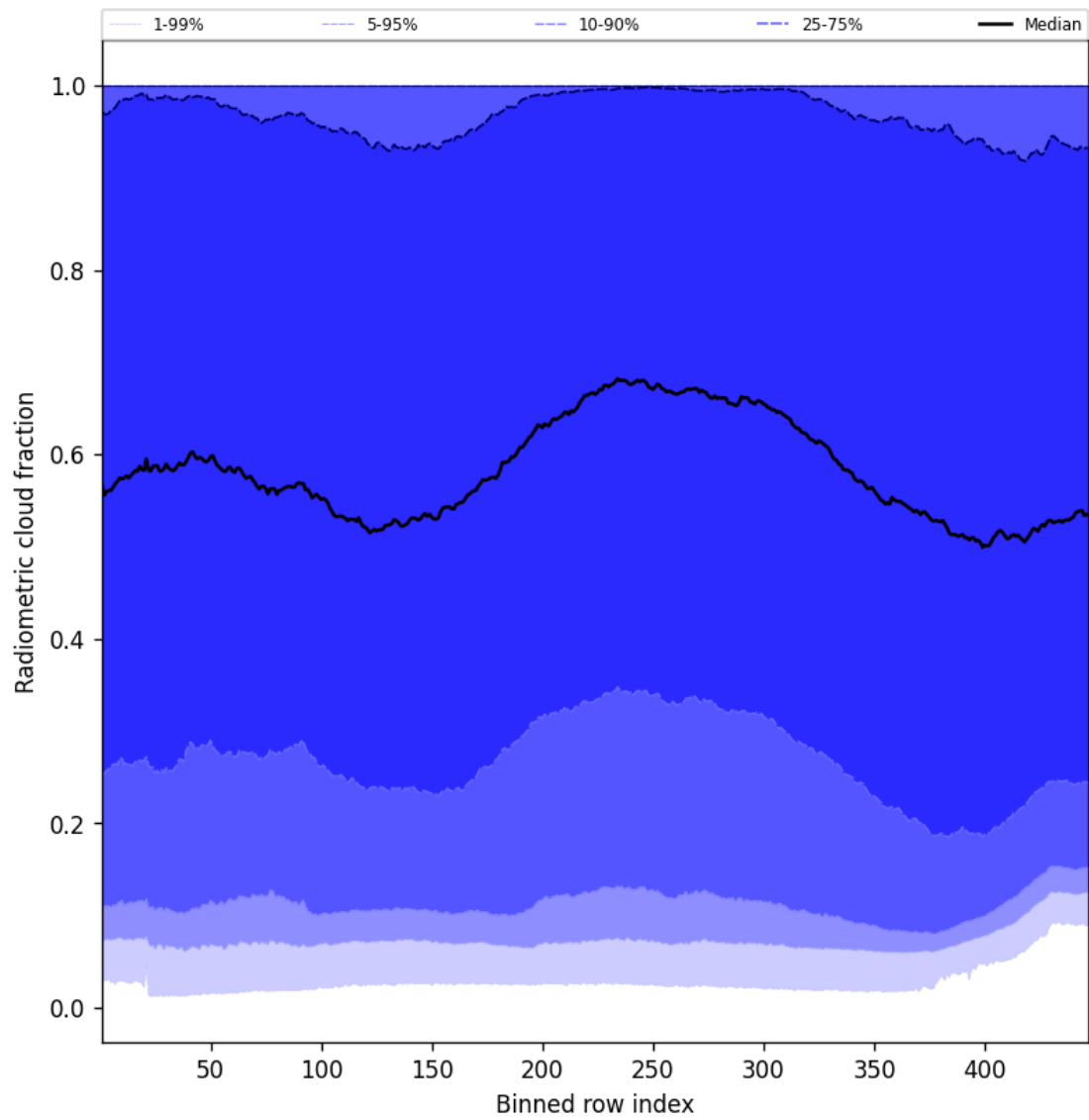
Figure 55: Along track statistics of “Radiometric cloud fraction” for 2024-12-03 to 2024-12-05
