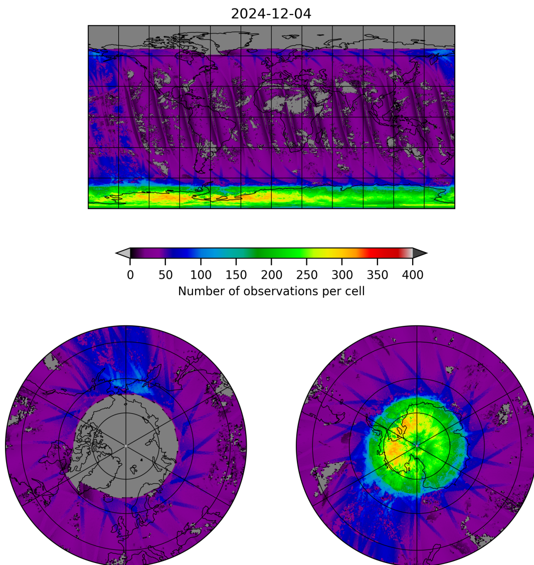
Figure 21: Map of the number of observations for 2024-12-03 to 2024-12-05
