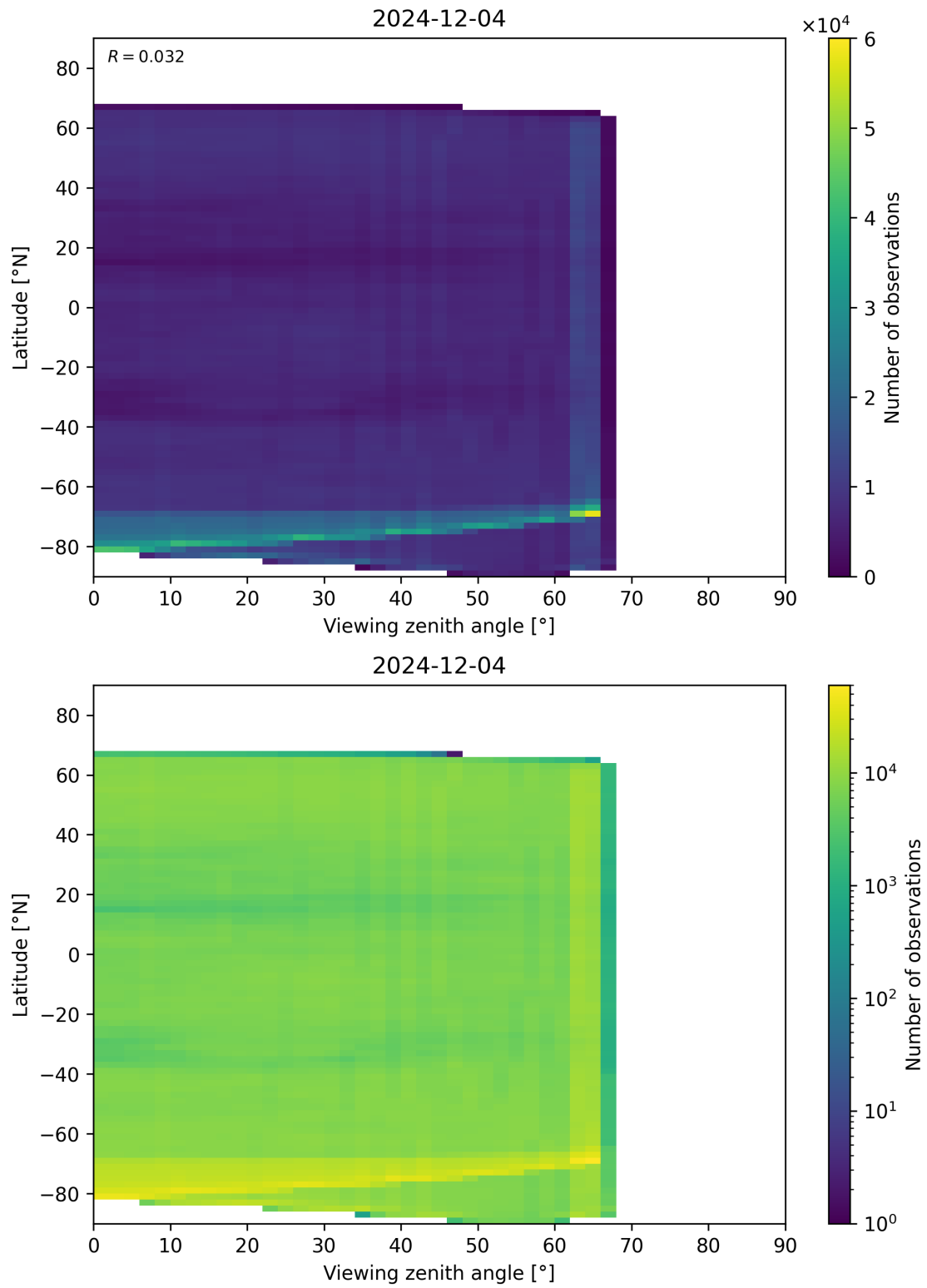
Figure 113: Scatter density plot of “Viewing zenith angle” against “Latitude” for 2024-12-03 to 2024-12-05.
