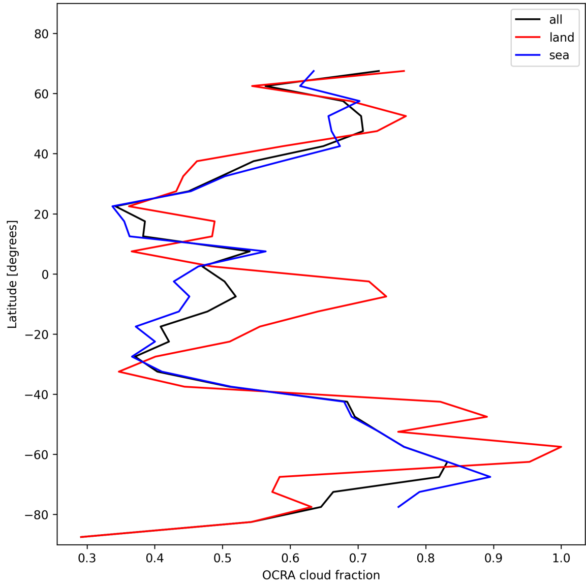
Figure 34: Zonal average of “OCRA cloud fraction” for 2024-12-03 to 2024-12-05.
