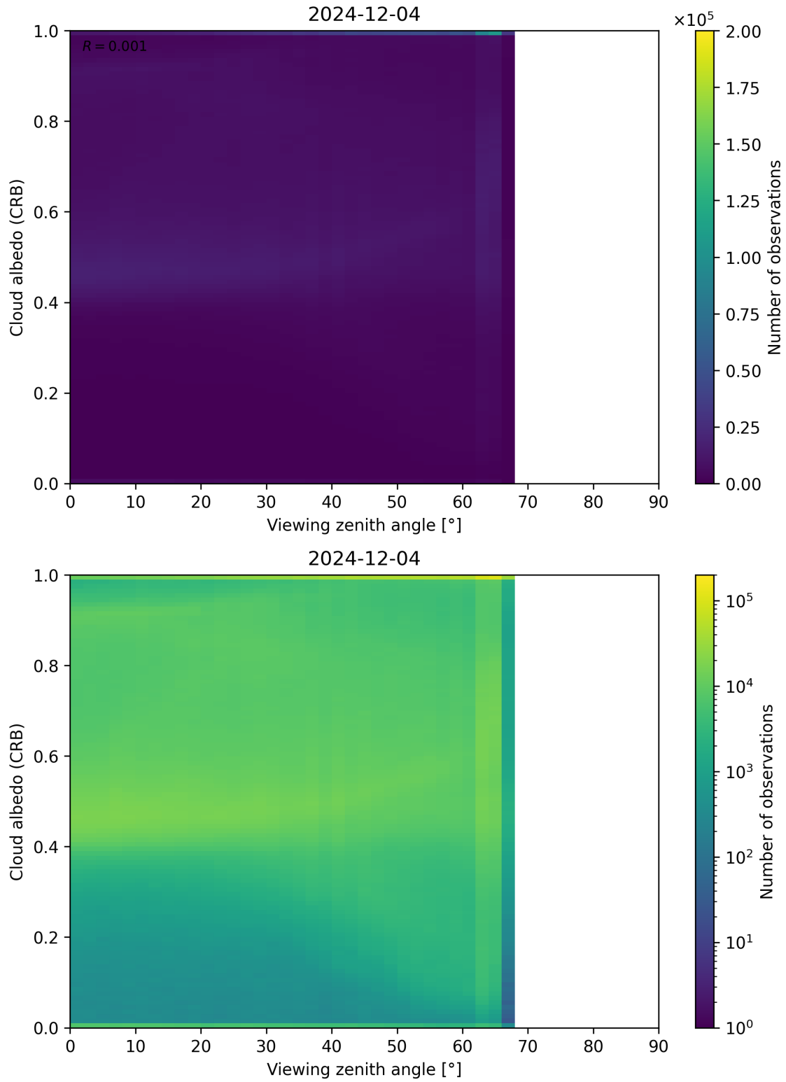
Figure 106: Scatter density plot of “Viewing zenith angle” against “Cloud albedo (CRB)” for 2024-12-03 to 2024-12-05.
