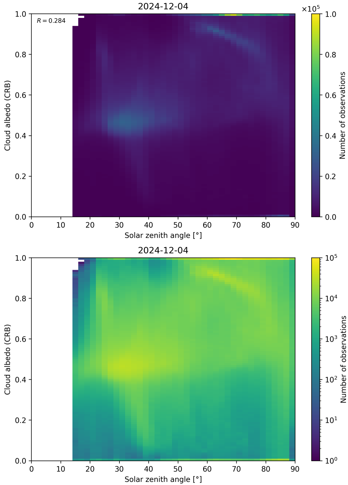
Figure 98: Scatter density plot of “Solar zenith angle” against “Cloud albedo (CRB)” for 2024-12-03 to 2024-12-05.
