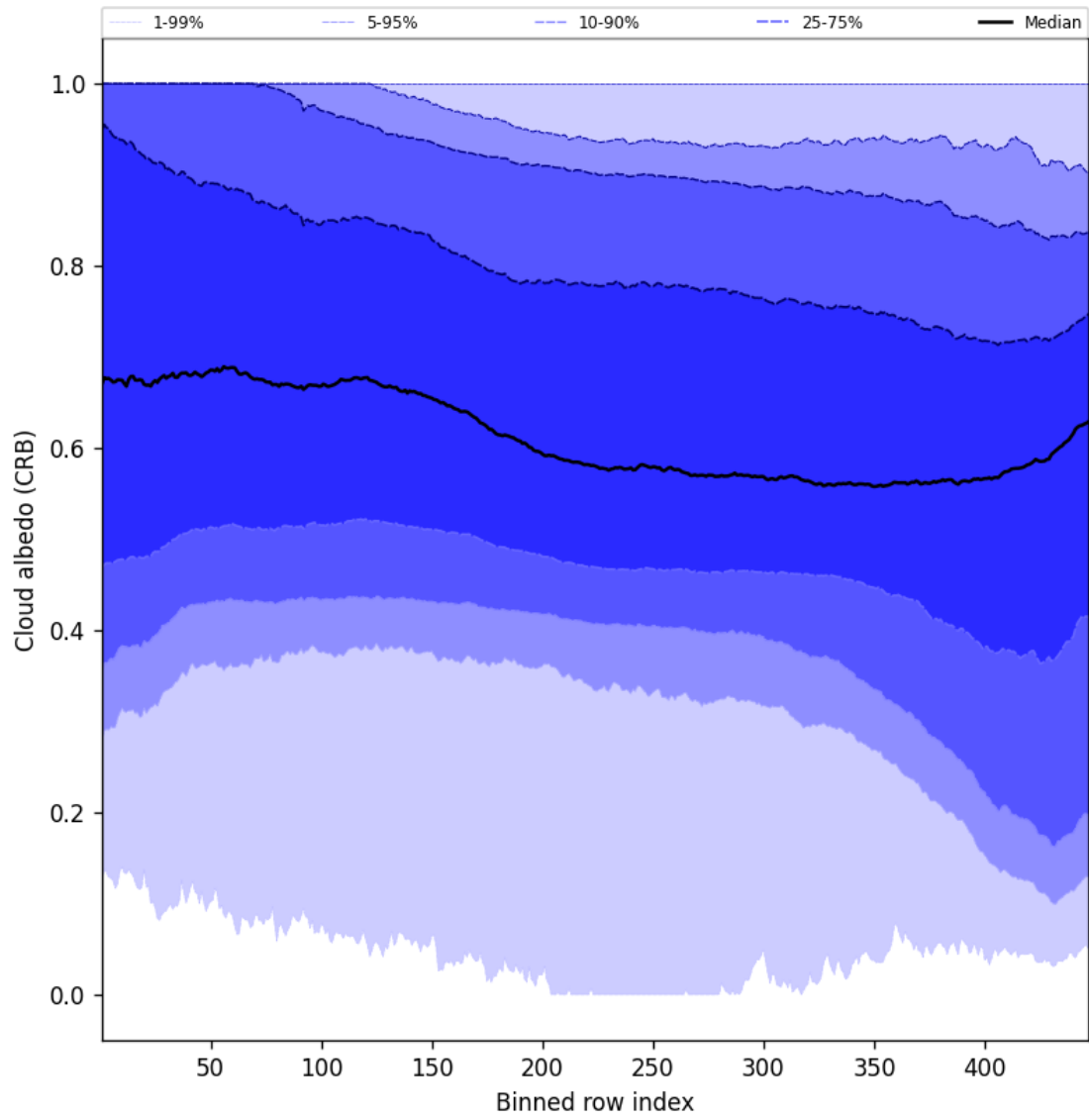
Figure 60: Along track statistics of “Cloud albedo (CRB)” for 2024-12-03 to 2024-12-05
