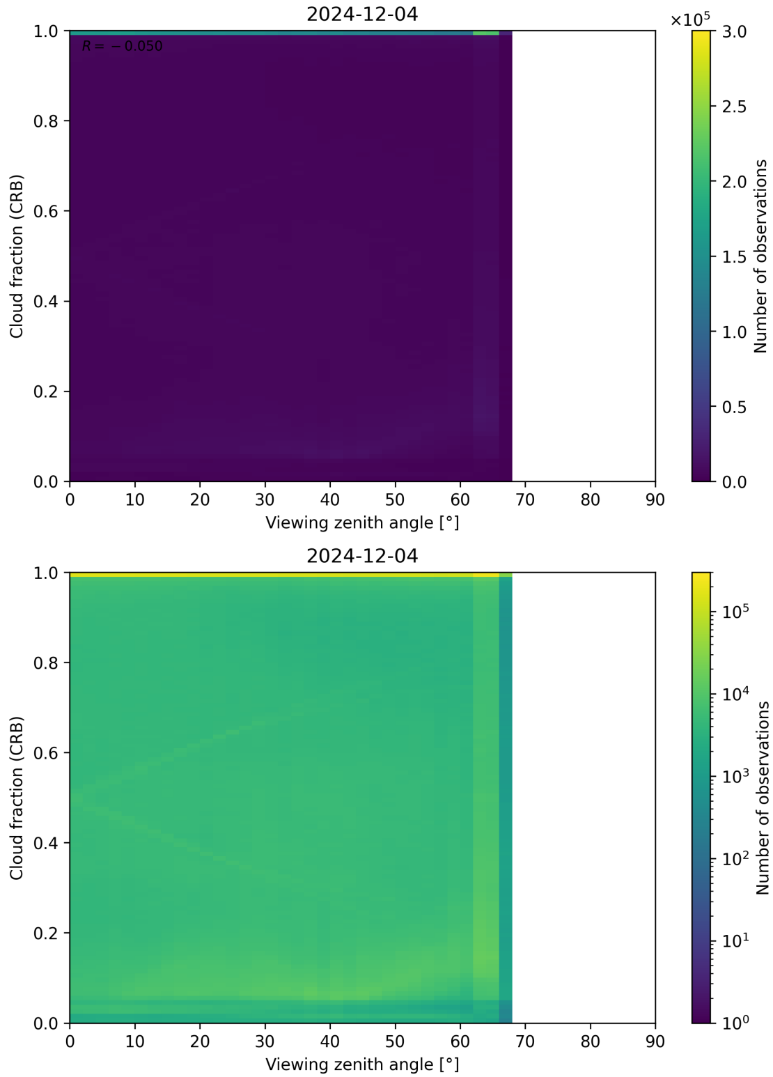
Figure 109: Scatter density plot of “Viewing zenith angle” against “Cloud fraction (CRB)” for 2024-12-03 to 2024-12-05.
