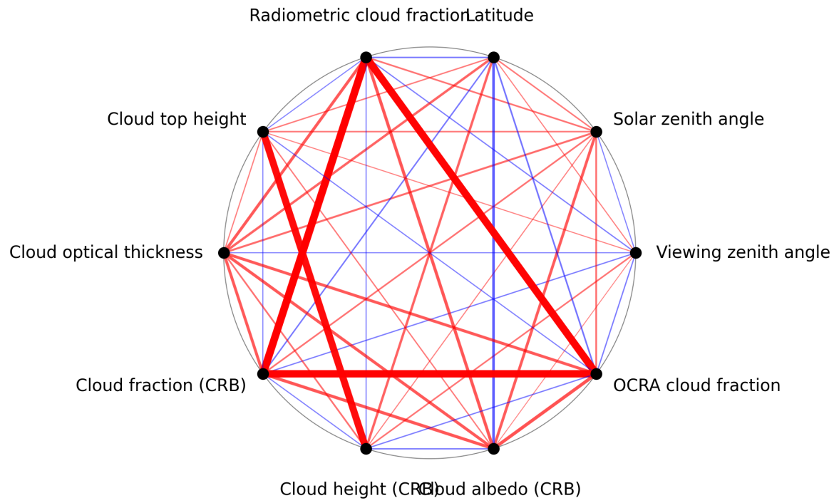
Figure 1: Map of correlation graph for 2024-12-03 to 2024-12-05.
