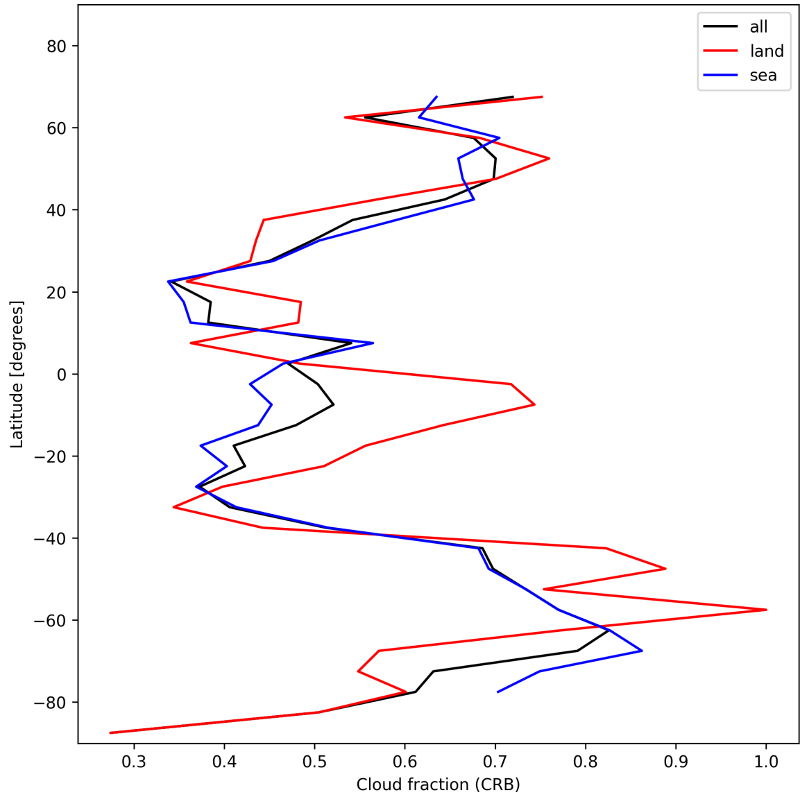
Figure 26: Zonal average of “Cloud fraction (CRB)” for 2024-12-03 to 2024-12-05.
