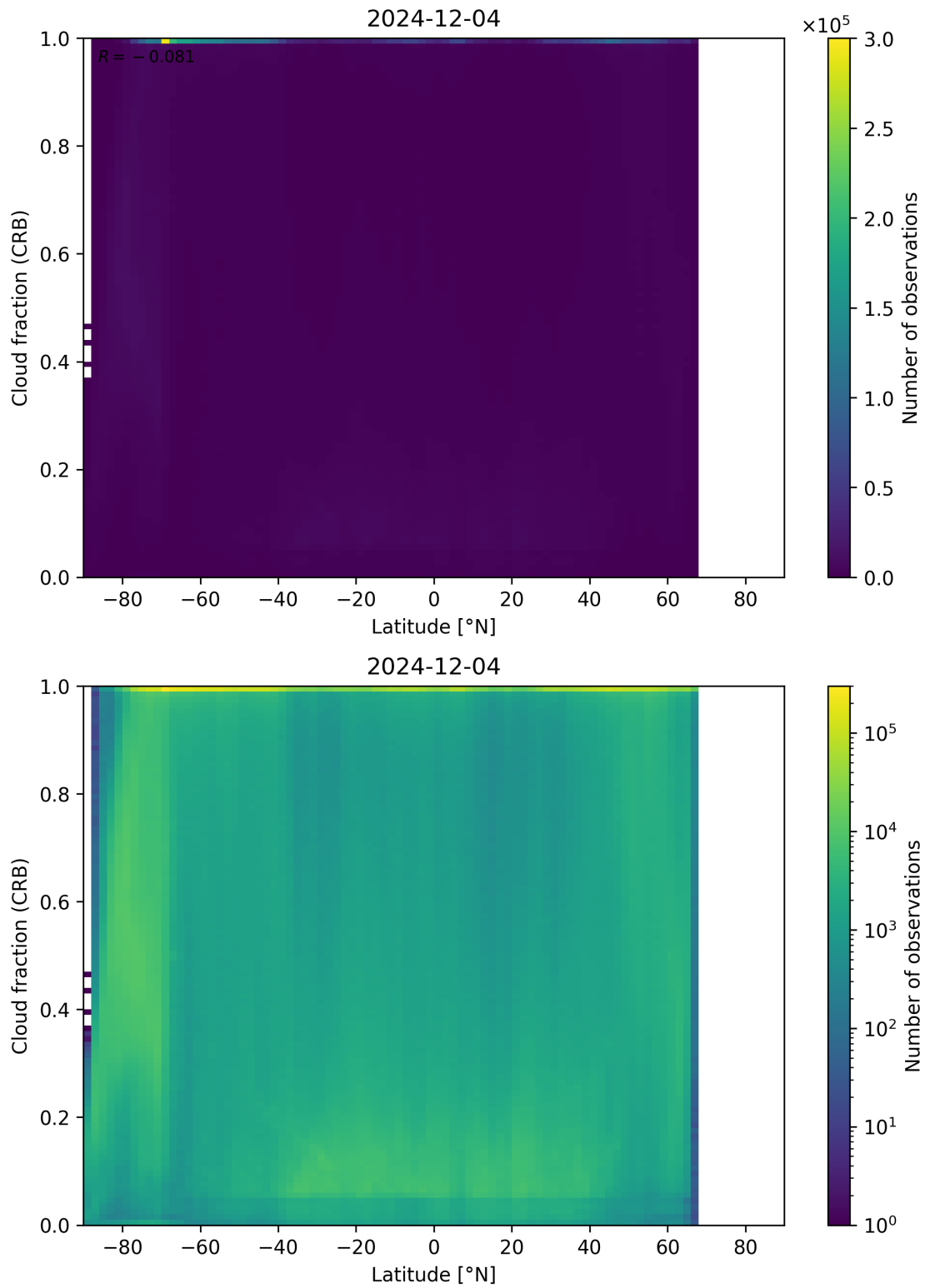
Figure 94: Scatter density plot of “Latitude” against “Cloud fraction (CRB)” for 2024-12-03 to 2024-12-05.
