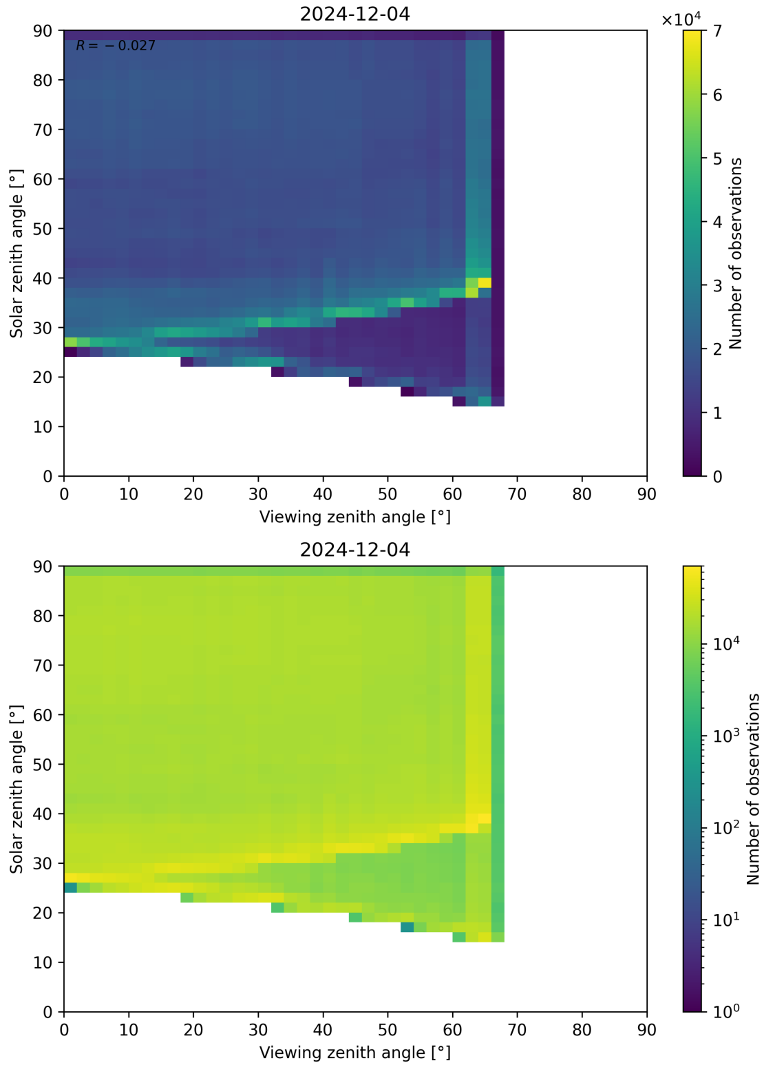
Figure 114: Scatter density plot of “Viewing zenith angle” against “Solar zenith angle” for 2024-12-03 to 2024-12-05.
