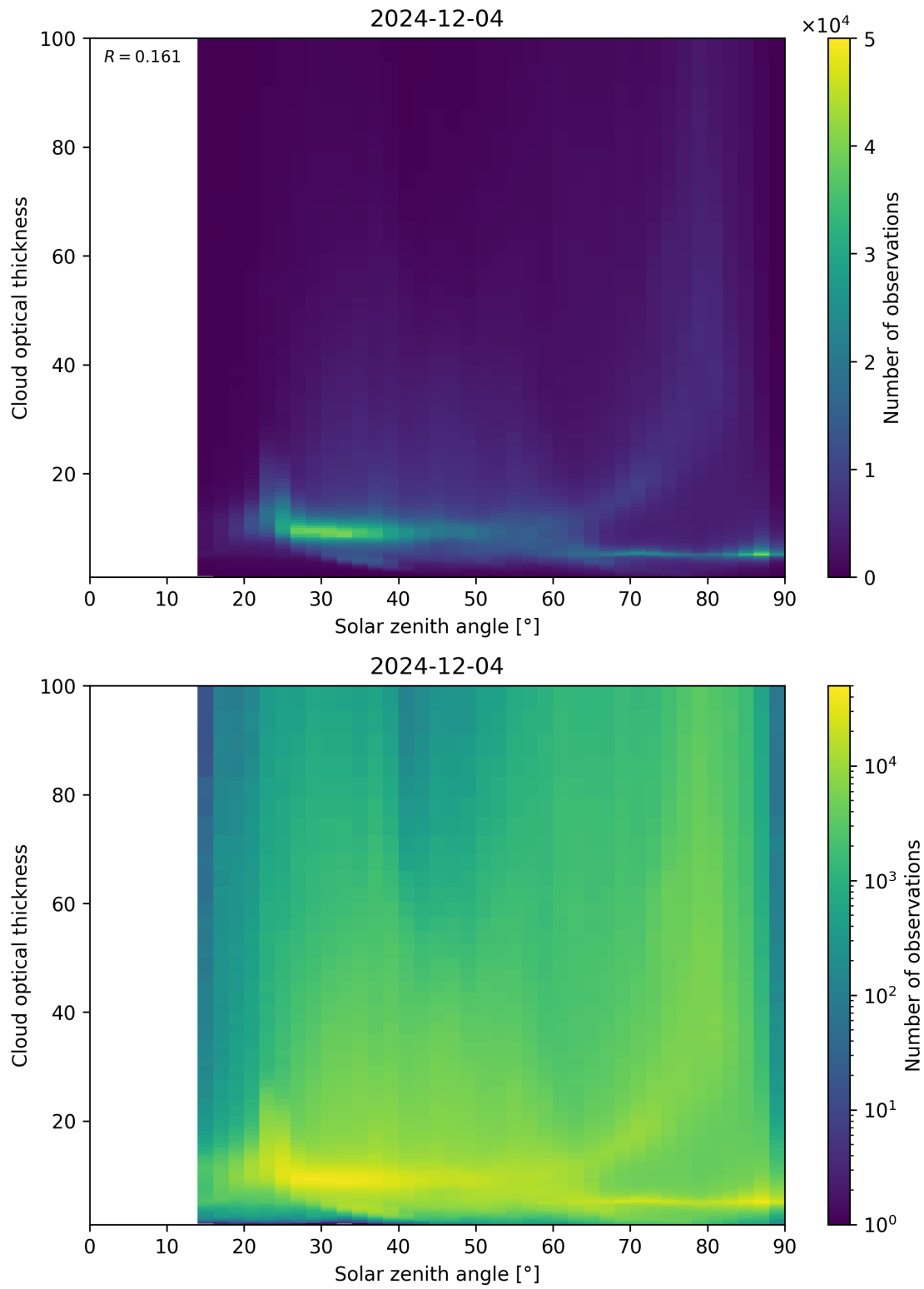
Figure 103: Scatter density plot of “Solar zenith angle” against “Cloud optical thickness” for 2024-12-03 to 2024-12-05.
