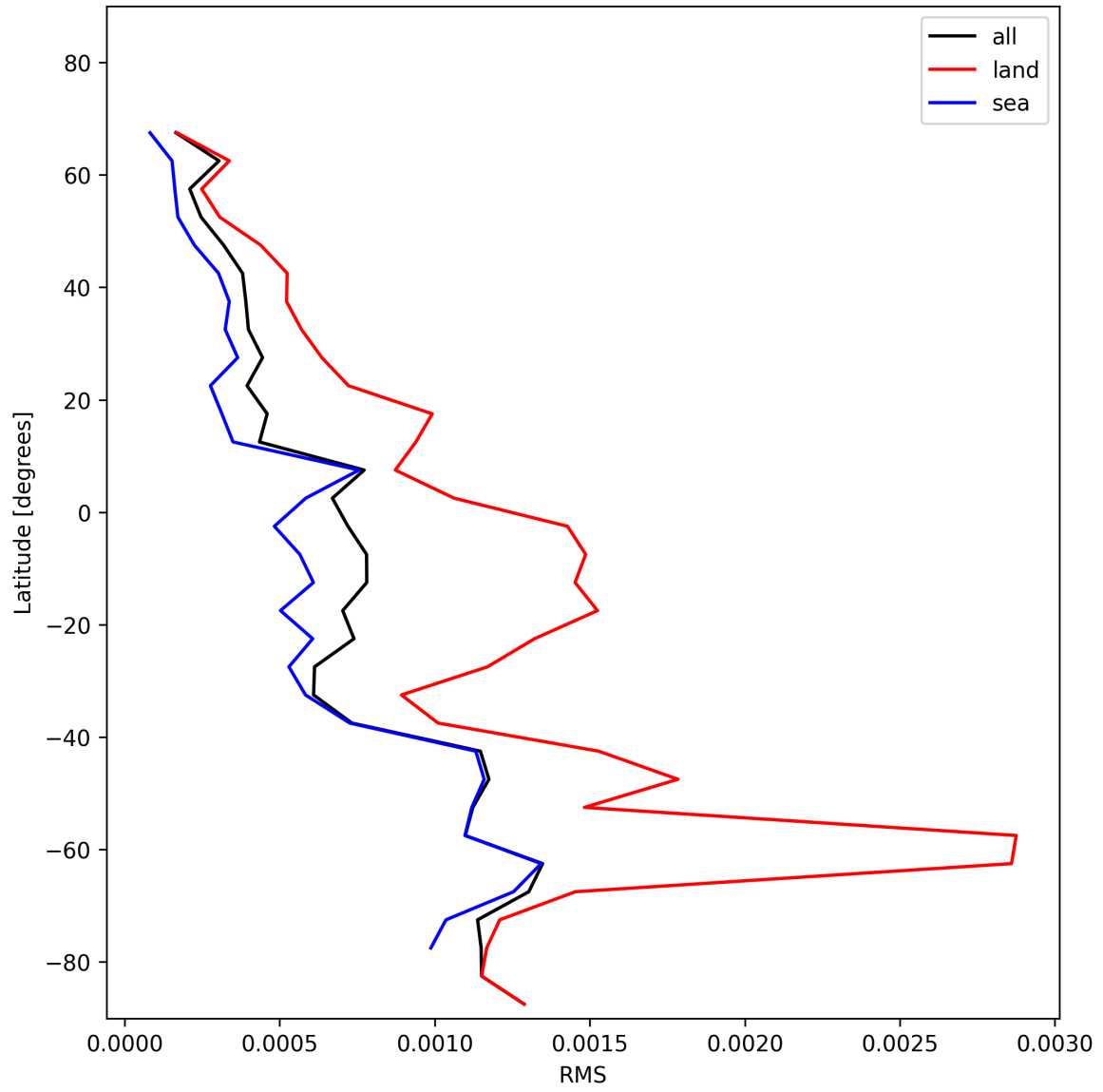
Figure 31: Zonal average of “RMS” for 2024-12-03 to 2024-12-05.
