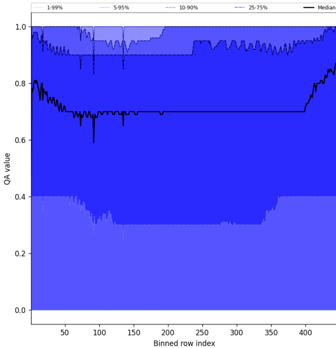
Figure 54: Along track statistics of “QA value” for 2024-12-03 to 2024-12-05
