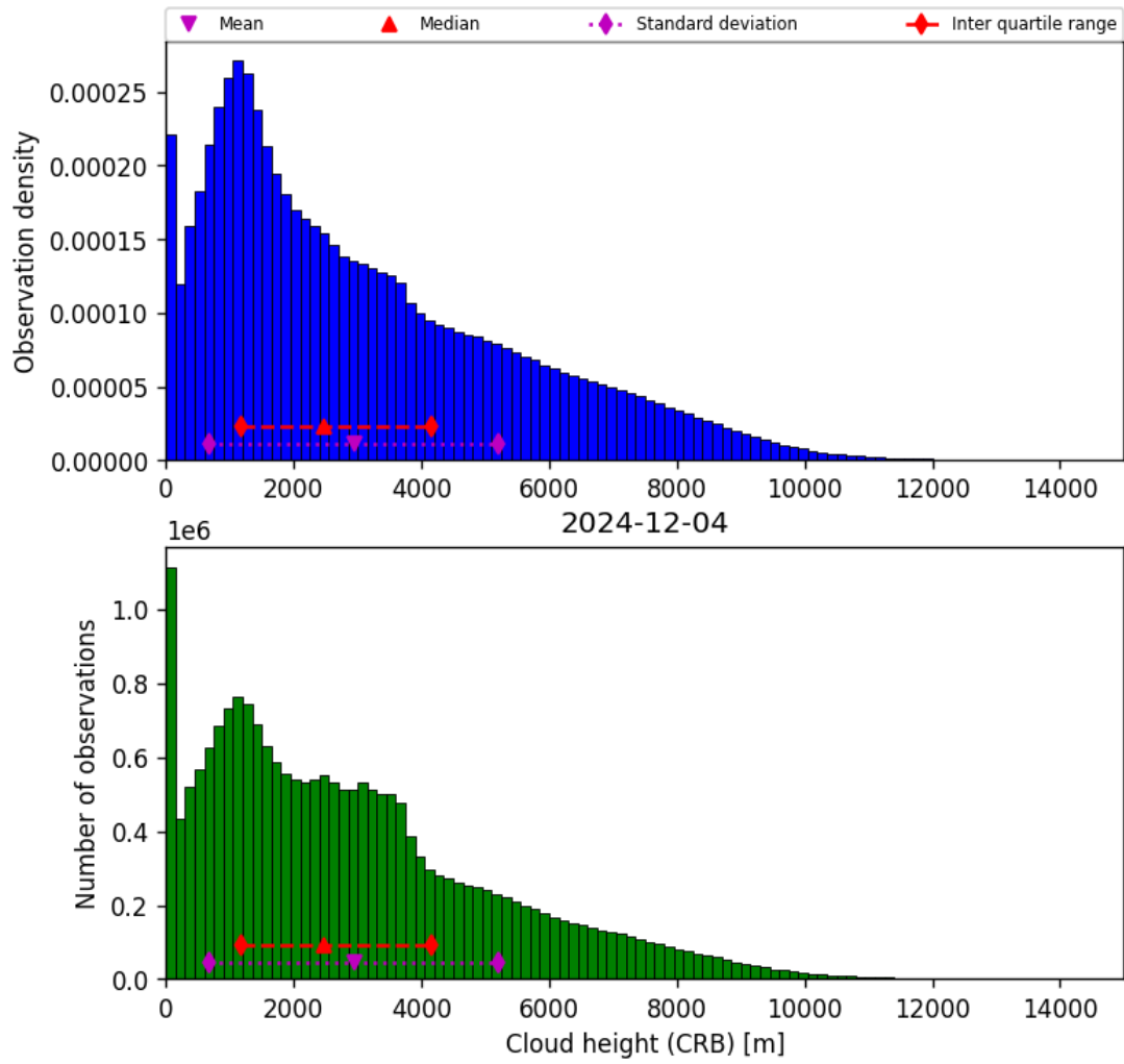
Figure 43: Histogram of “Cloud height (CRB)” for 2024-12-03 to 2024-12-05
