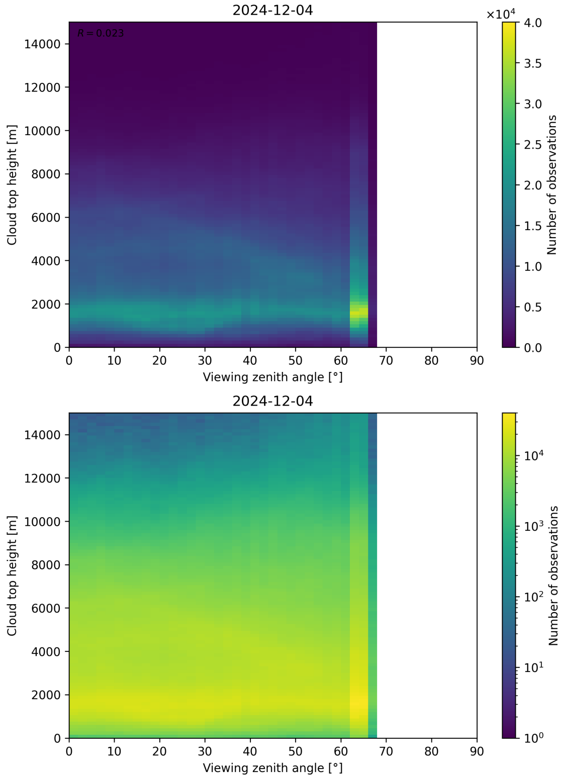
Figure 112: Scatter density plot of “Viewing zenith angle” against “Cloud top height” for 2024-12-03 to 2024-12-05.
