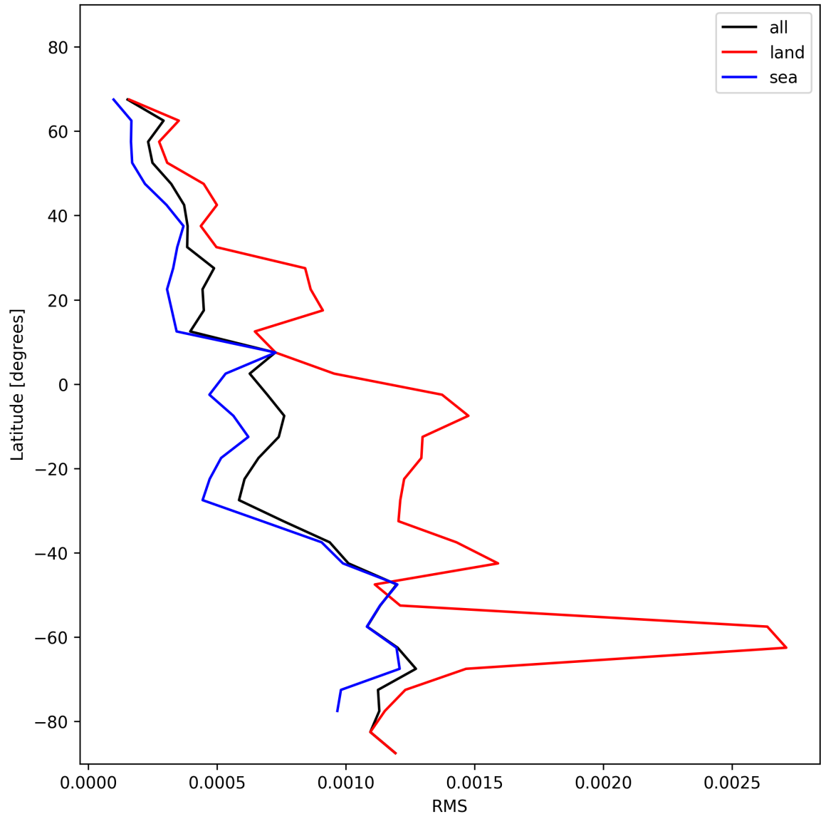
Figure 31: Zonal average of “RMS” for 2024-12-06 to 2024-12-07.
