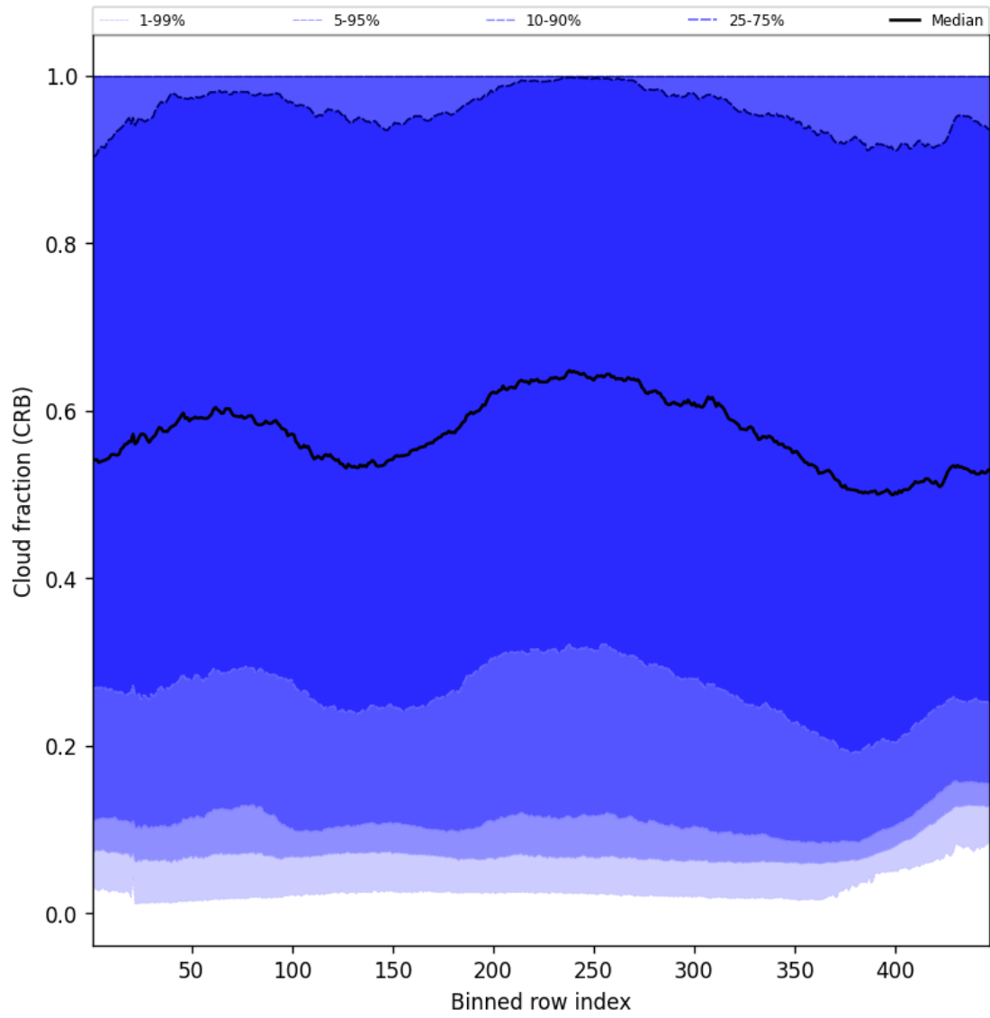
Figure 58: Along track statistics of “Cloud fraction (CRB)” for 2024-12-06 to 2024-12-07
