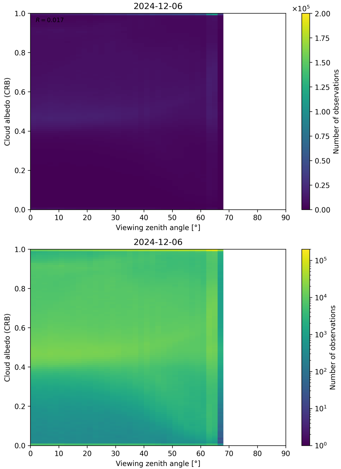
Figure 106: Scatter density plot of “Viewing zenith angle” against “Cloud albedo (CRB)” for 2024-12-06 to 2024-12-07.
