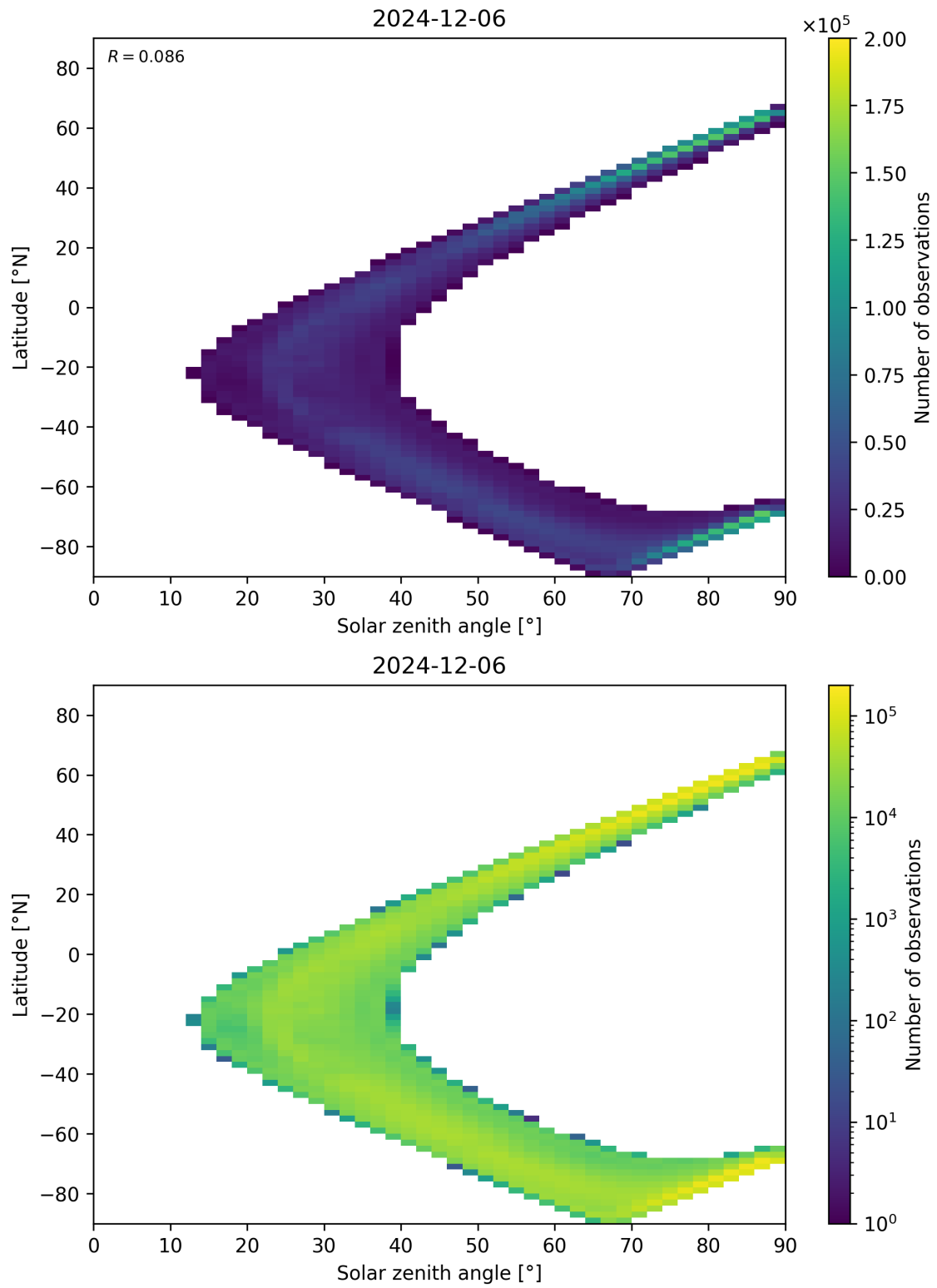
Figure 105: Scatter density plot of “Solar zenith angle” against “Latitude” for 2024-12-06 to 2024-12-07.
