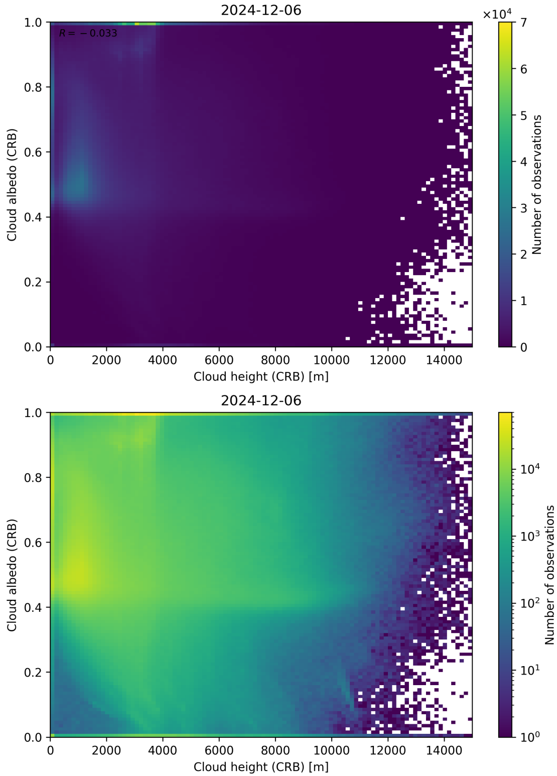
Figure 80: Scatter density plot of “Cloud height (CRB)” against “Cloud albedo (CRB)” for 2024-12-06 to 2024-12-07.
