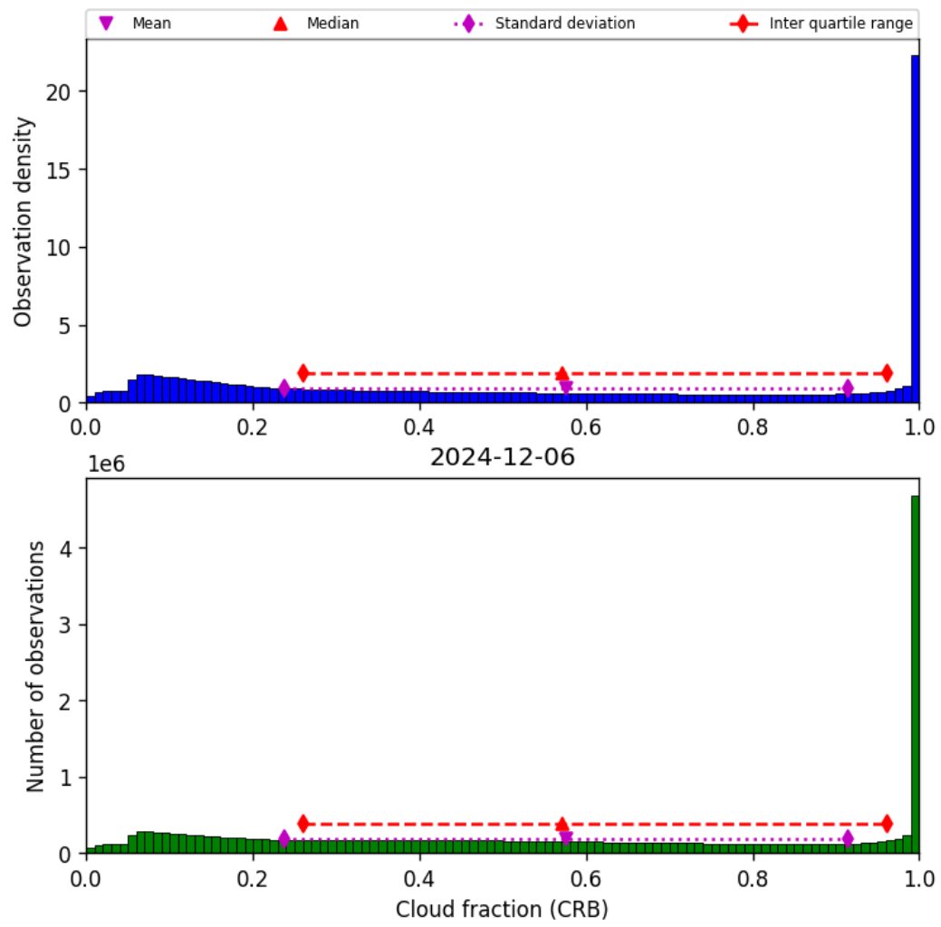
Figure 42: Histogram of “Cloud fraction (CRB)” for 2024-12-06 to 2024-12-07
