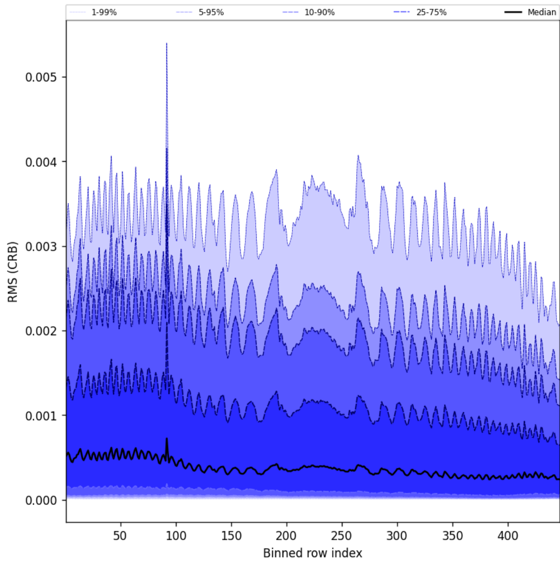
Figure 64: Along track statistics of “RMS (CRB)” for 2024-12-06 to 2024-12-07
