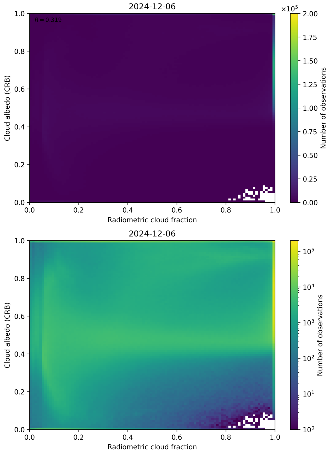
Figure 71: Scatter density plot of “Radiometric cloud fraction” against “Cloud albedo (CRB)” for 2024-12-06 to 2024-12-07.
