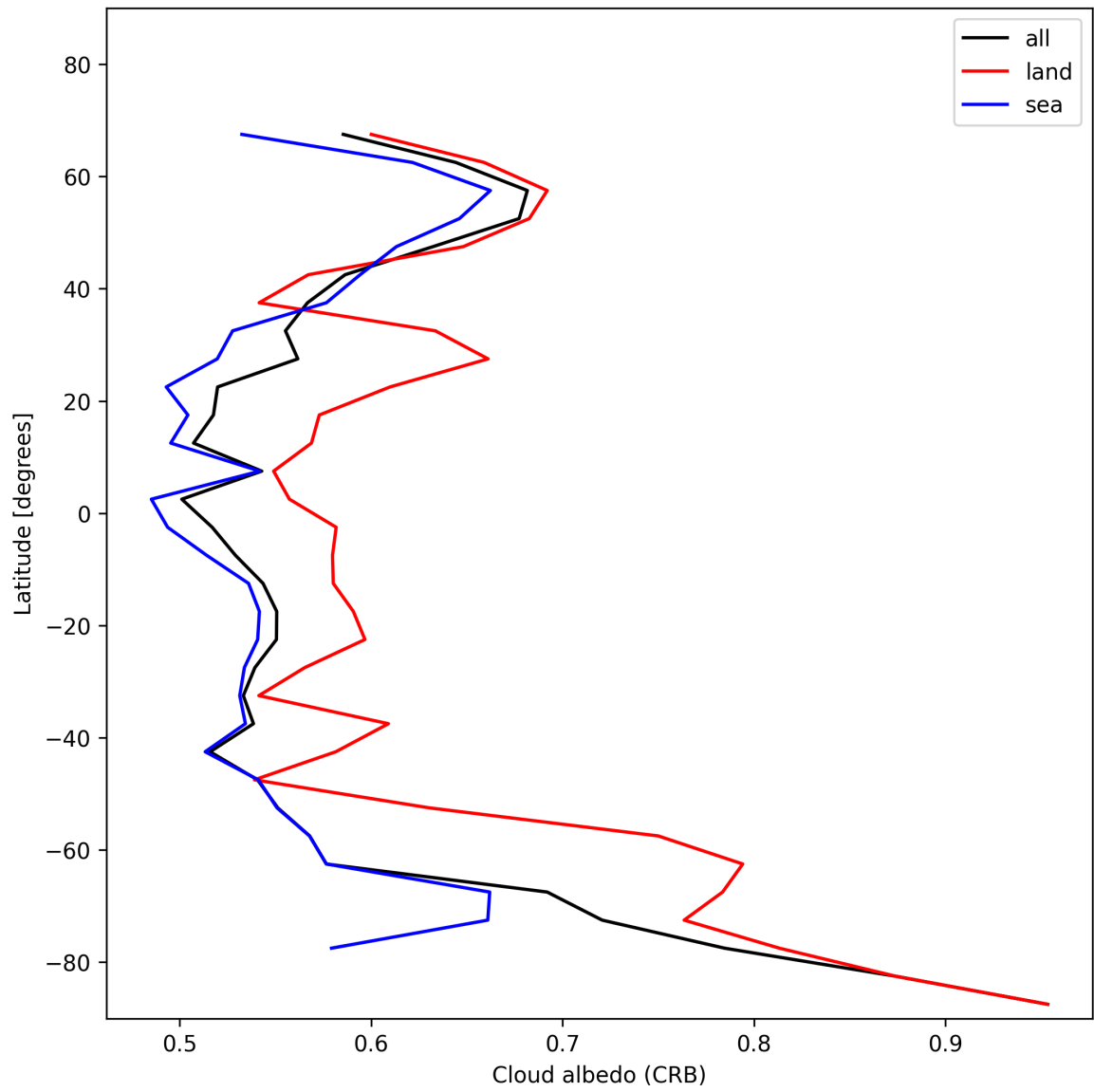
Figure 28: Zonal average of “Cloud albedo (CRB)” for 2024-12-06 to 2024-12-07.
