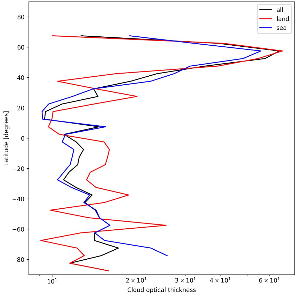
Figure 25: Zonal average of “Cloud optical thickness” for 2024-12-06 to 2024-12-07.
