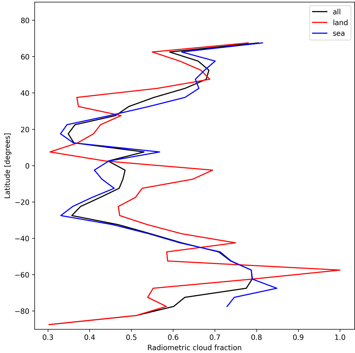
Figure 23: Zonal average of “Radiometric cloud fraction” for 2024-12-06 to 2024-12-07.
