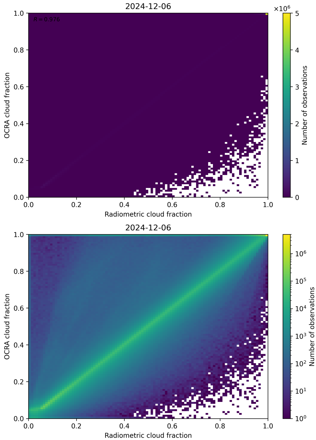
Figure 72: Scatter density plot of “Radiometric cloud fraction” against “OCRA cloud fraction” for 2024-12-06 to 2024-12-07.
