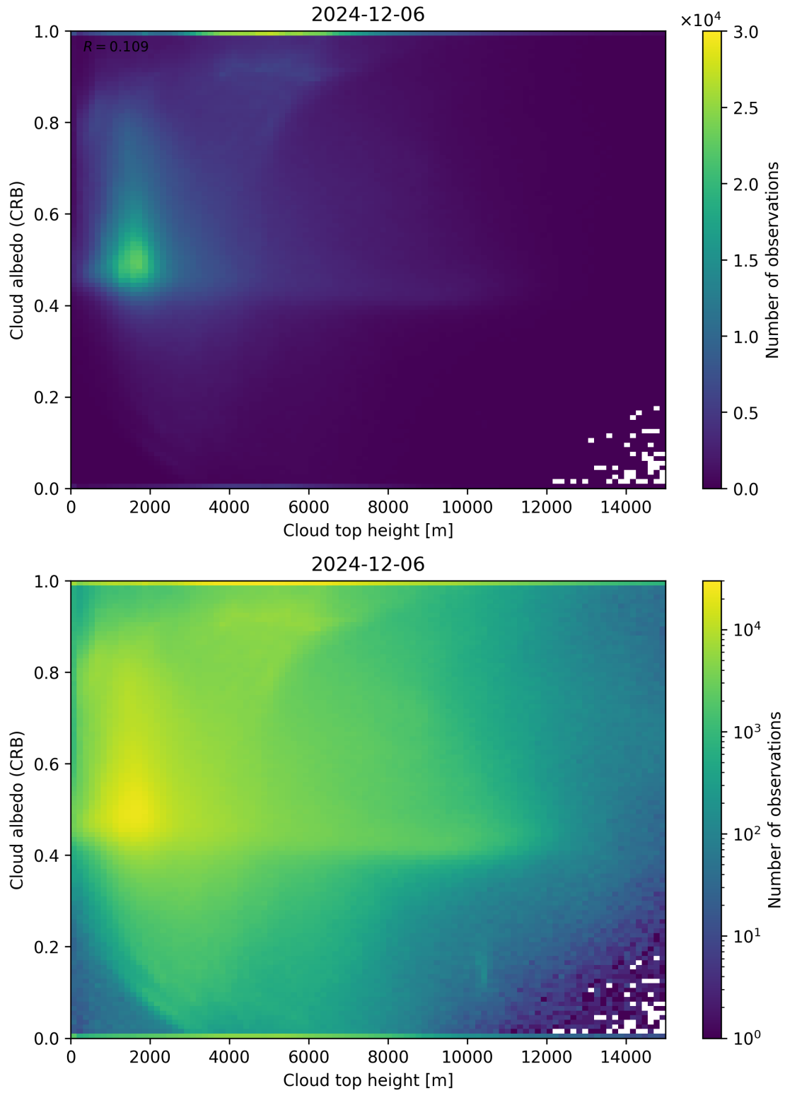
Figure 86: Scatter density plot of “Cloud top height” against “Cloud albedo (CRB)” for 2024-12-06 to 2024-12-07.
