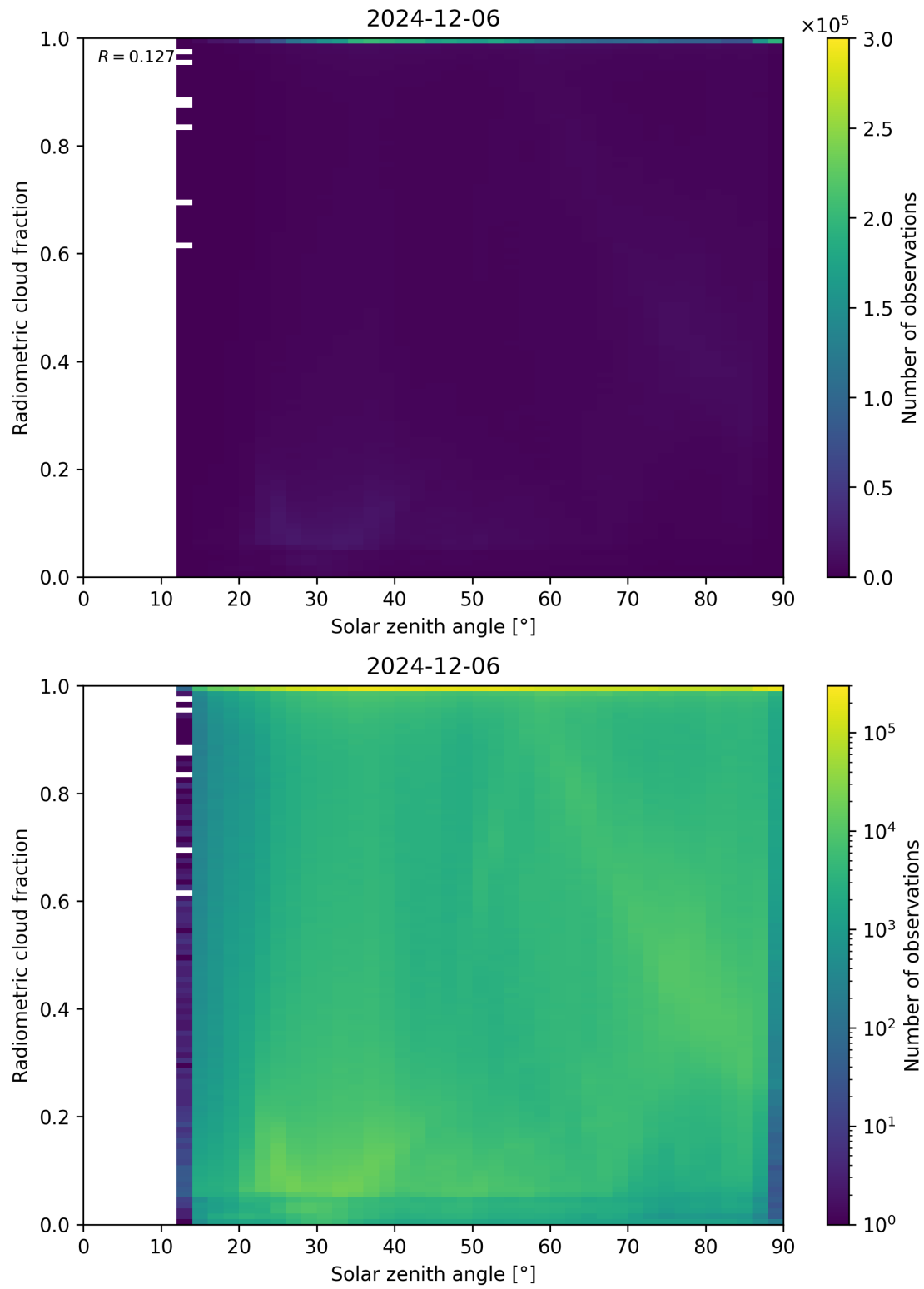
Figure 99: Scatter density plot of “Solar zenith angle” against “Radiometric cloud fraction” for 2024-12-06 to 2024-12-07.
