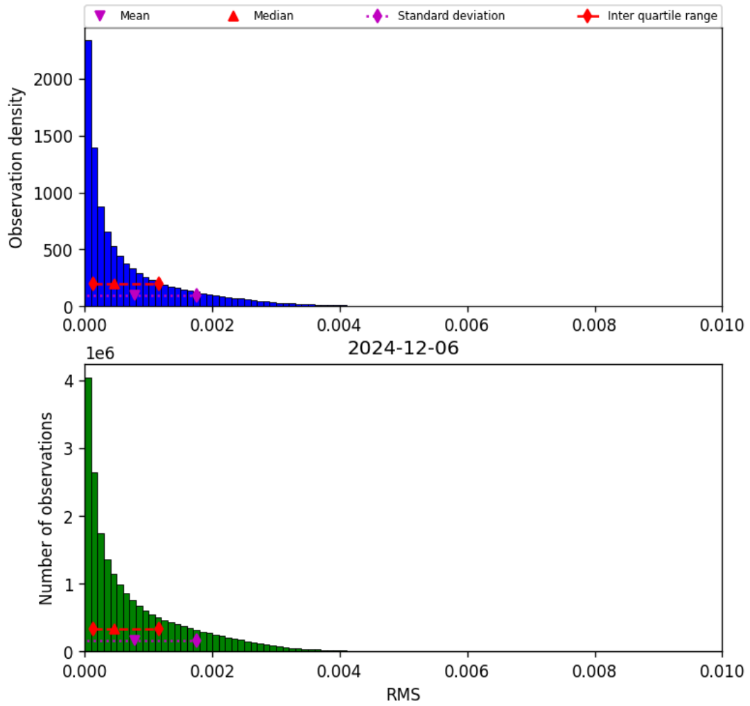
Figure 47: Histogram of “RMS” for 2024-12-06 to 2024-12-07
