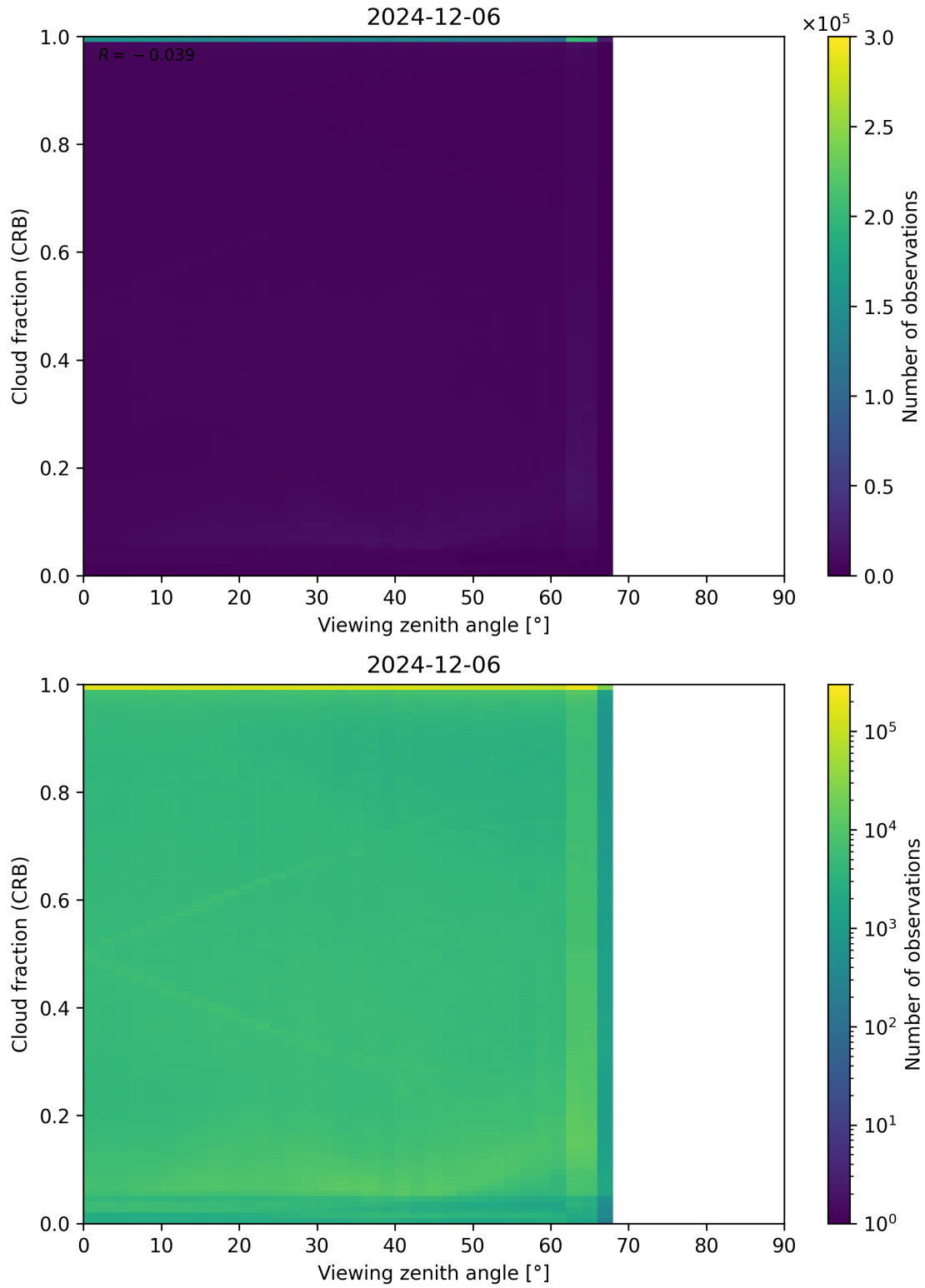
Figure 109: Scatter density plot of “Viewing zenith angle” against “Cloud fraction (CRB)” for 2024-12-06 to 2024-12-07.
