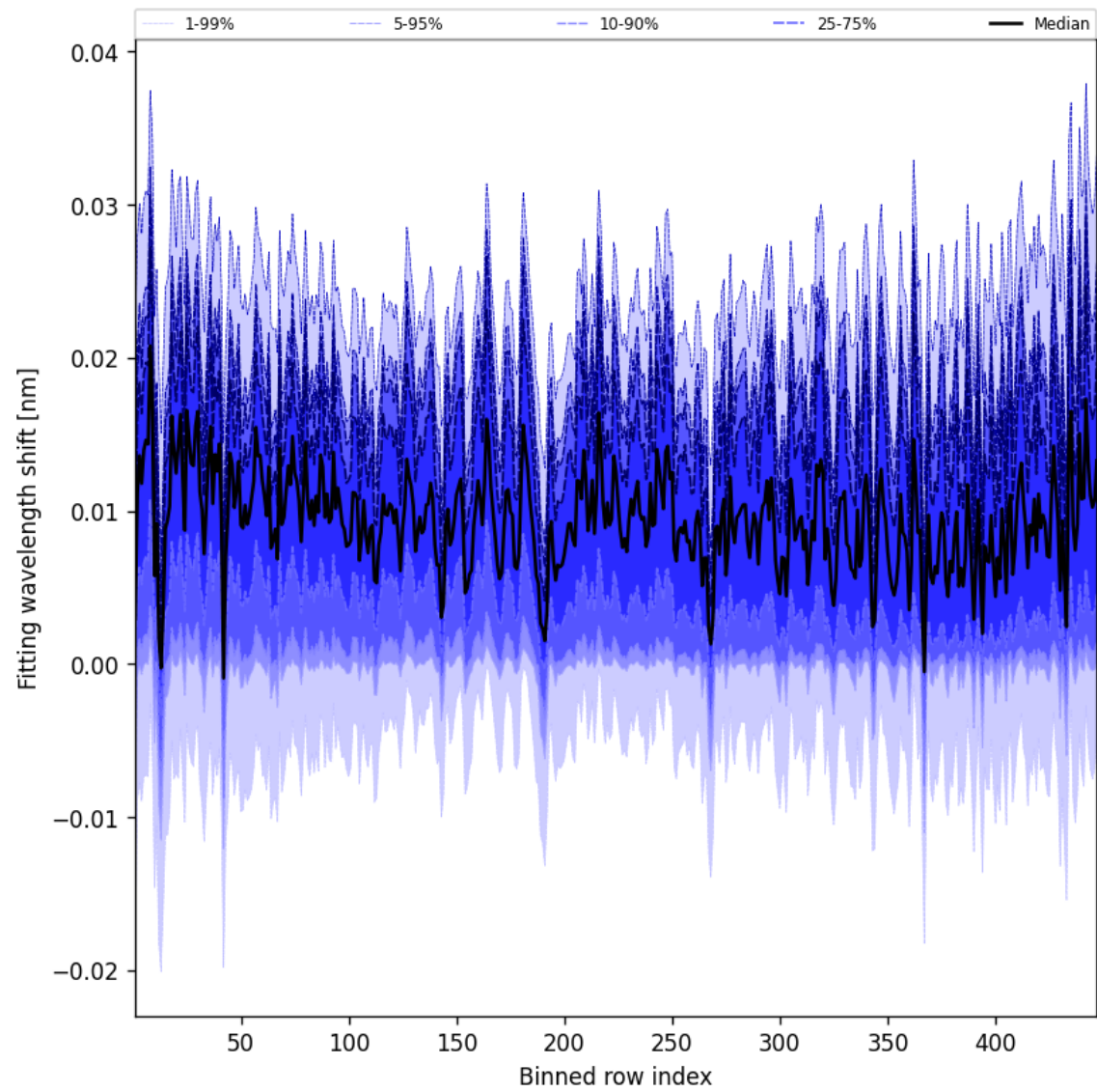
Figure 65: Along track statistics of “Fitting wavelength shift” for 2024-12-06 to 2024-12-07
