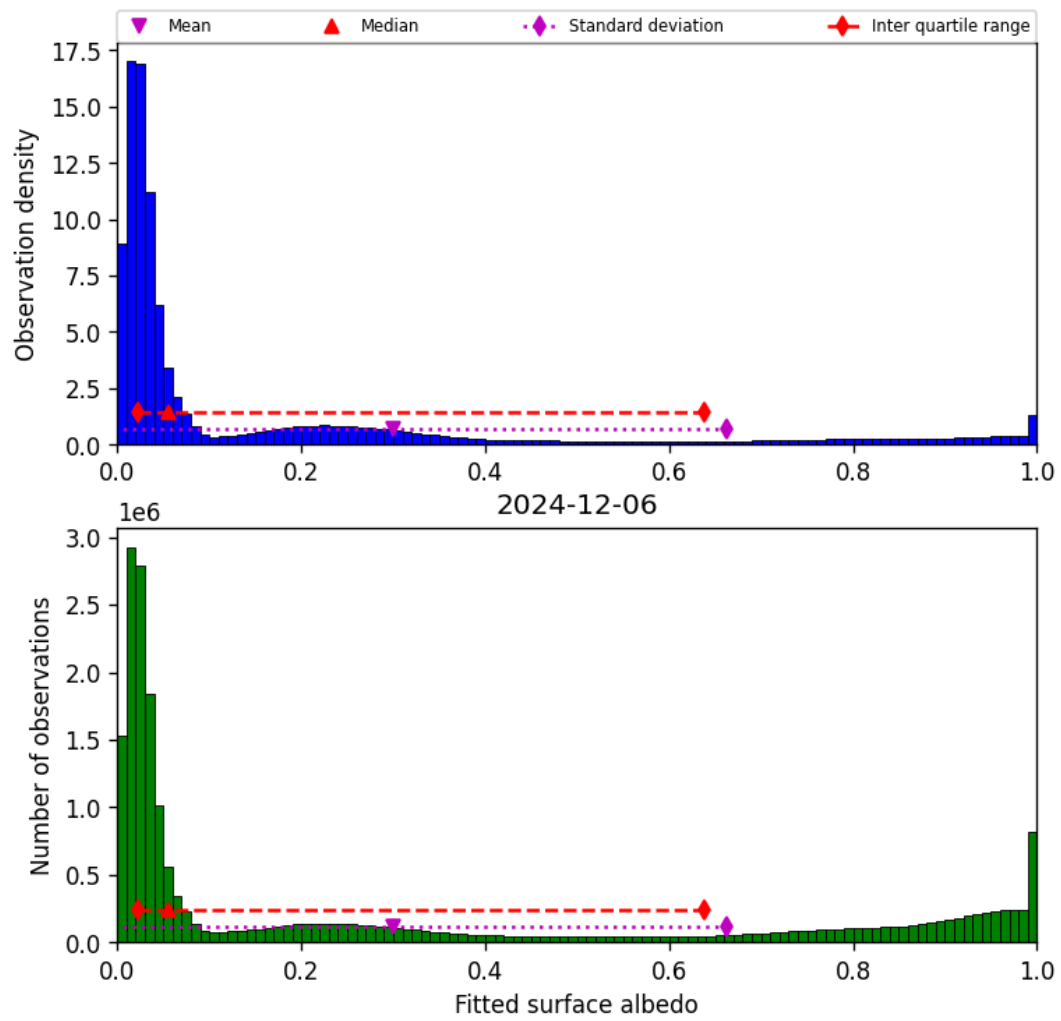
Figure 45: Histogram of “Fitted surface albedo” for 2024-12-06 to 2024-12-07
