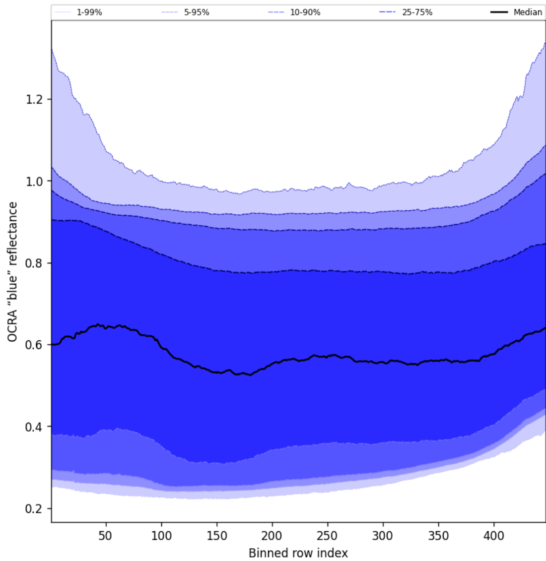
Figure 67: Along track statistics of “OCRA “blue” reflectance” for 2024-12-06 to 2024-12-07
