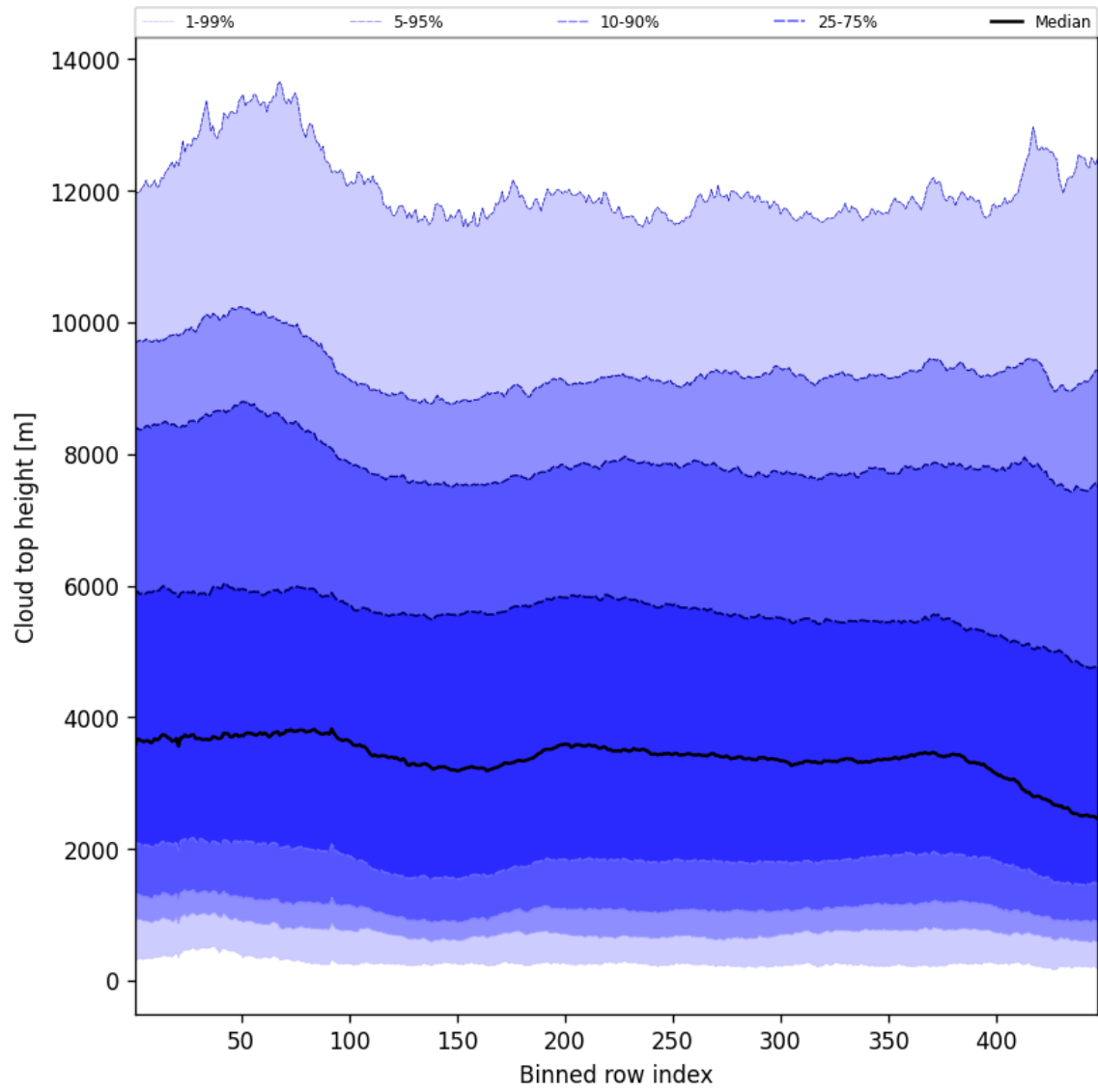
Figure 56: Along track statistics of “Cloud top height” for 2024-12-06 to 2024-12-07
