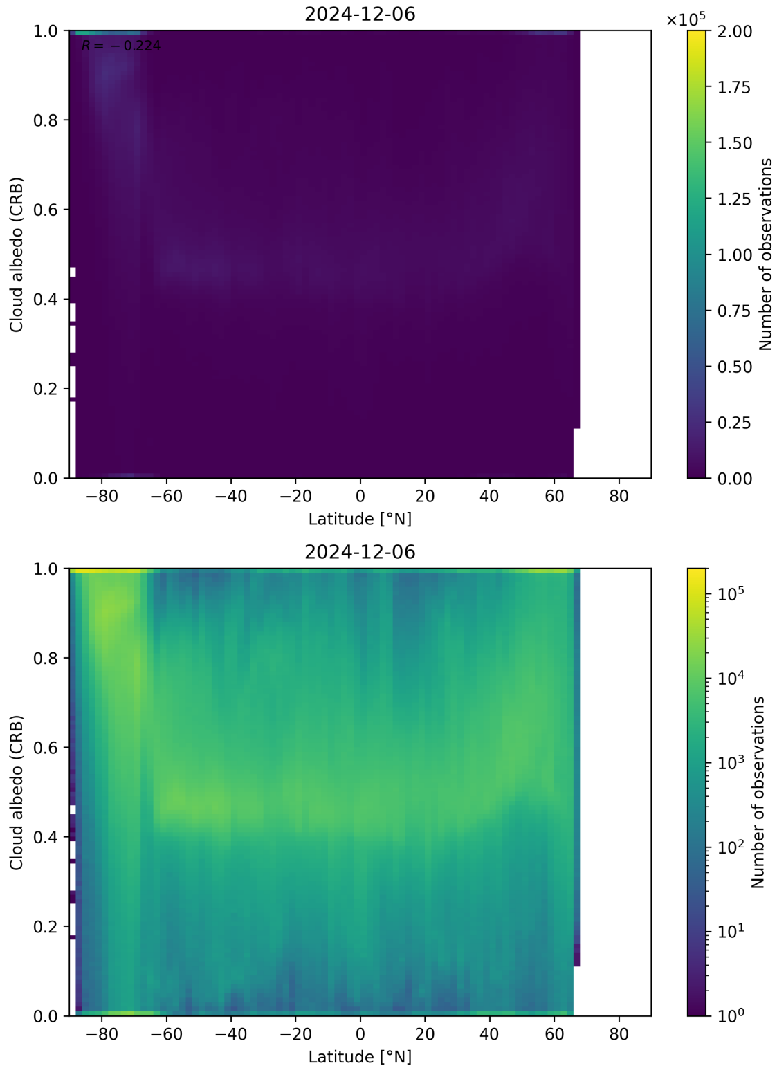
Figure 91: Scatter density plot of “Latitude” against “Cloud albedo (CRB)” for 2024-12-06 to 2024-12-07.
