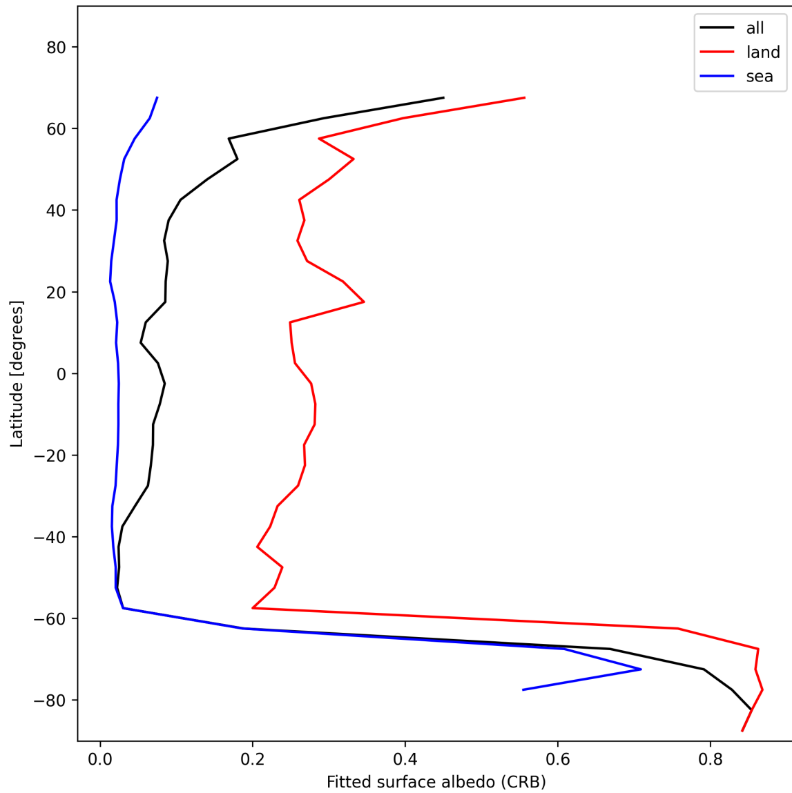
Figure 30: Zonal average of “Fitted surface albedo (CRB)” for 2024-12-06 to 2024-12-07.
