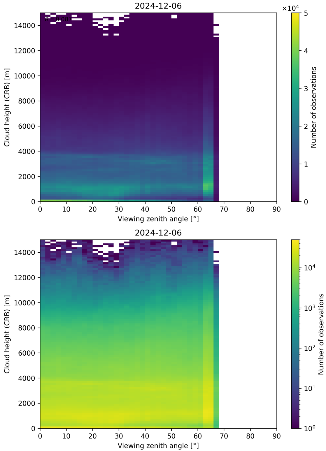
Figure 110: Scatter density plot of “Viewing zenith angle” against “Cloud height (CRB)” for 2024-12-06 to 2024-12-07.
