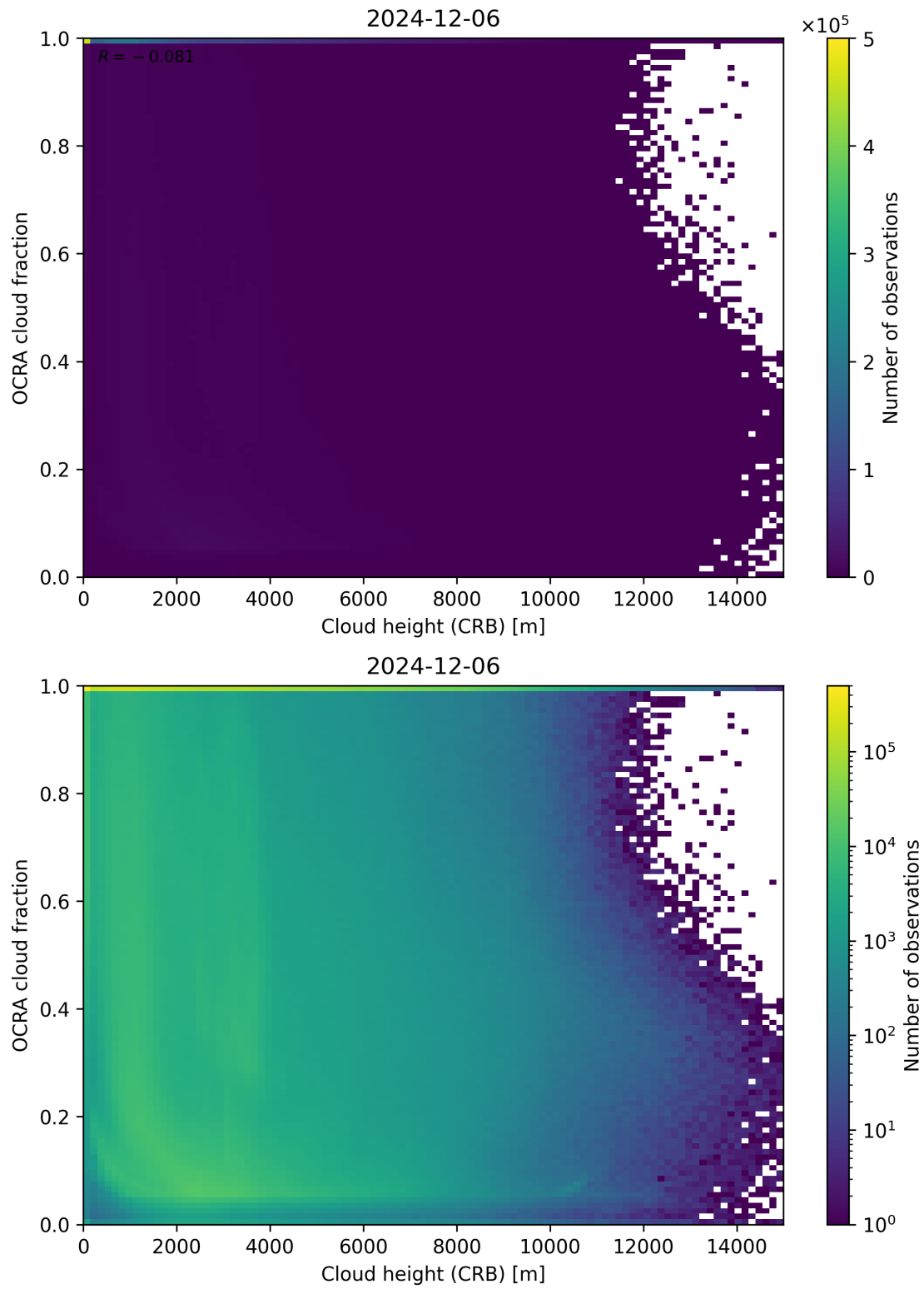
Figure 81: Scatter density plot of “Cloud height (CRB)” against “OCRA cloud fraction” for 2024-12-06 to 2024-12-07.
