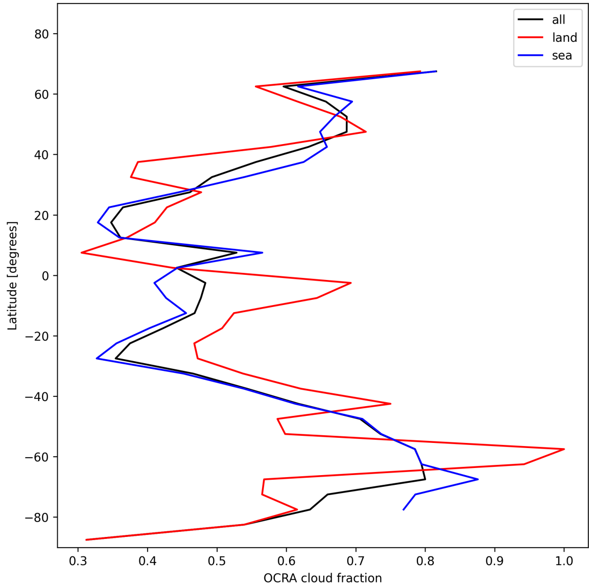
Figure 34: Zonal average of “OCRA cloud fraction” for 2024-12-06 to 2024-12-07.
