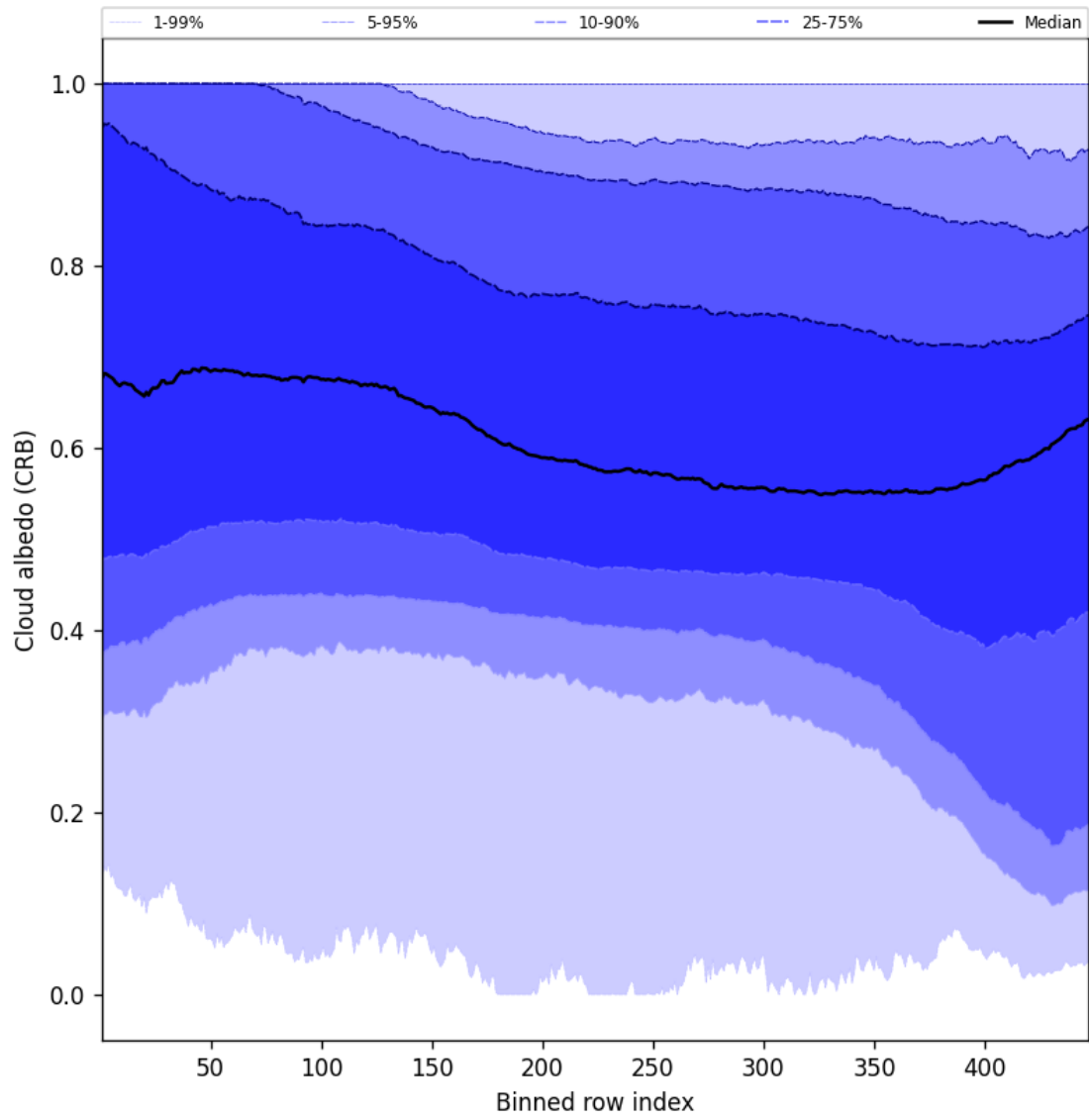
Figure 60: Along track statistics of “Cloud albedo (CRB)” for 2024-12-06 to 2024-12-07
