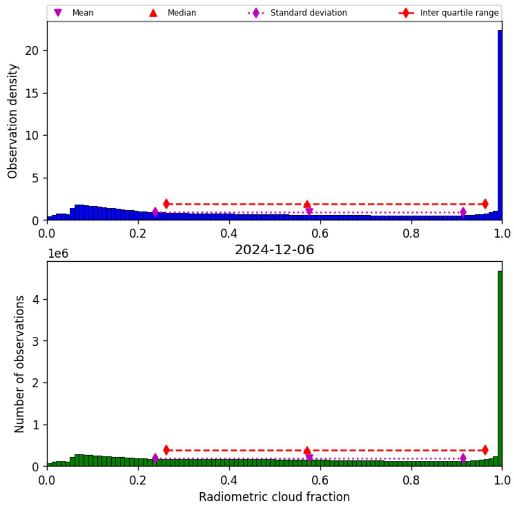
Figure 39: Histogram of “Radiometric cloud fraction” for 2024-12-06 to 2024-12-07
