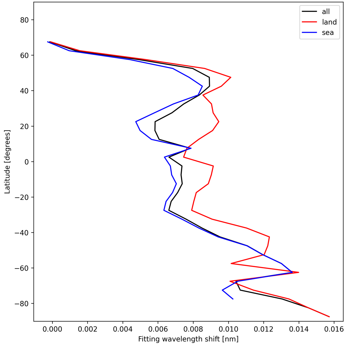
Figure 33: Zonal average of “Fitting wavelength shift” for 2024-12-06 to 2024-12-07.
