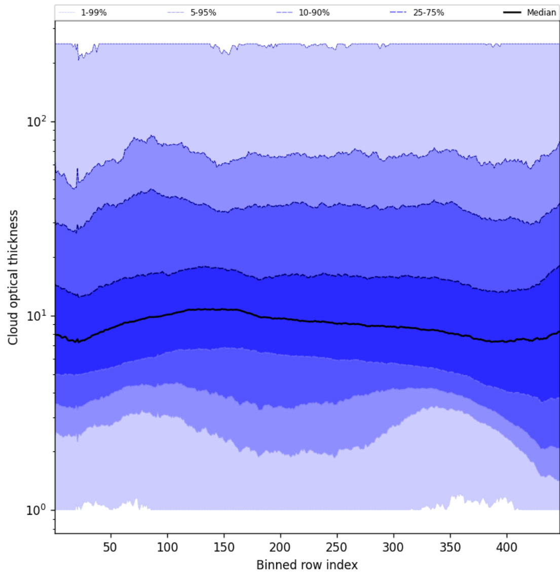
Figure 57: Along track statistics of “Cloud optical thickness” for 2024-12-06 to 2024-12-07
