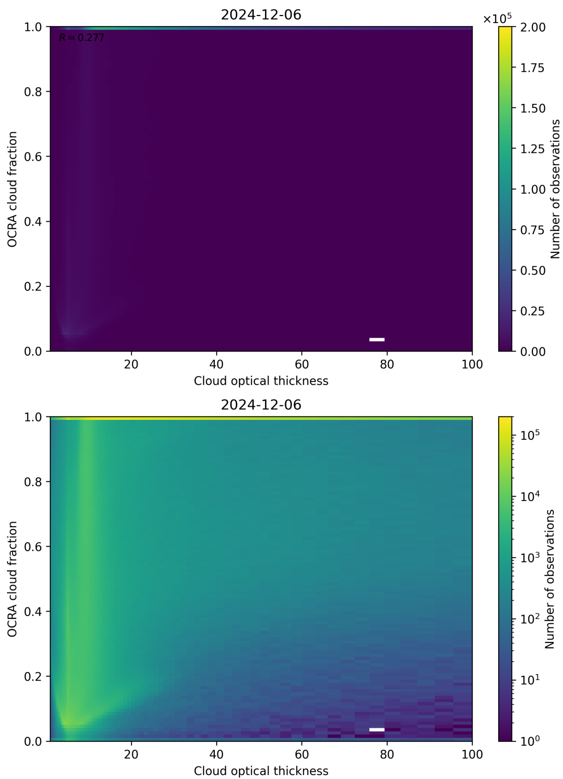
Figure 83: Scatter density plot of “Cloud optical thickness” against “OCRA cloud fraction” for 2024-12-06 to 2024-12-07.
