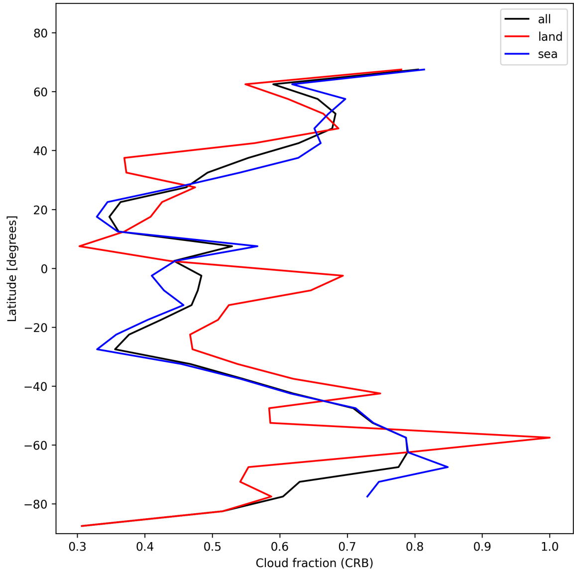
Figure 26: Zonal average of “Cloud fraction (CRB)” for 2024-12-06 to 2024-12-07.
