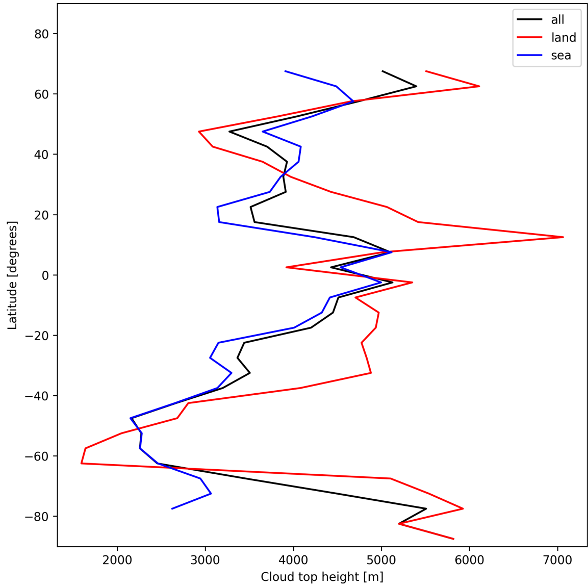
Figure 24: Zonal average of “Cloud top height” for 2024-12-06 to 2024-12-07.
