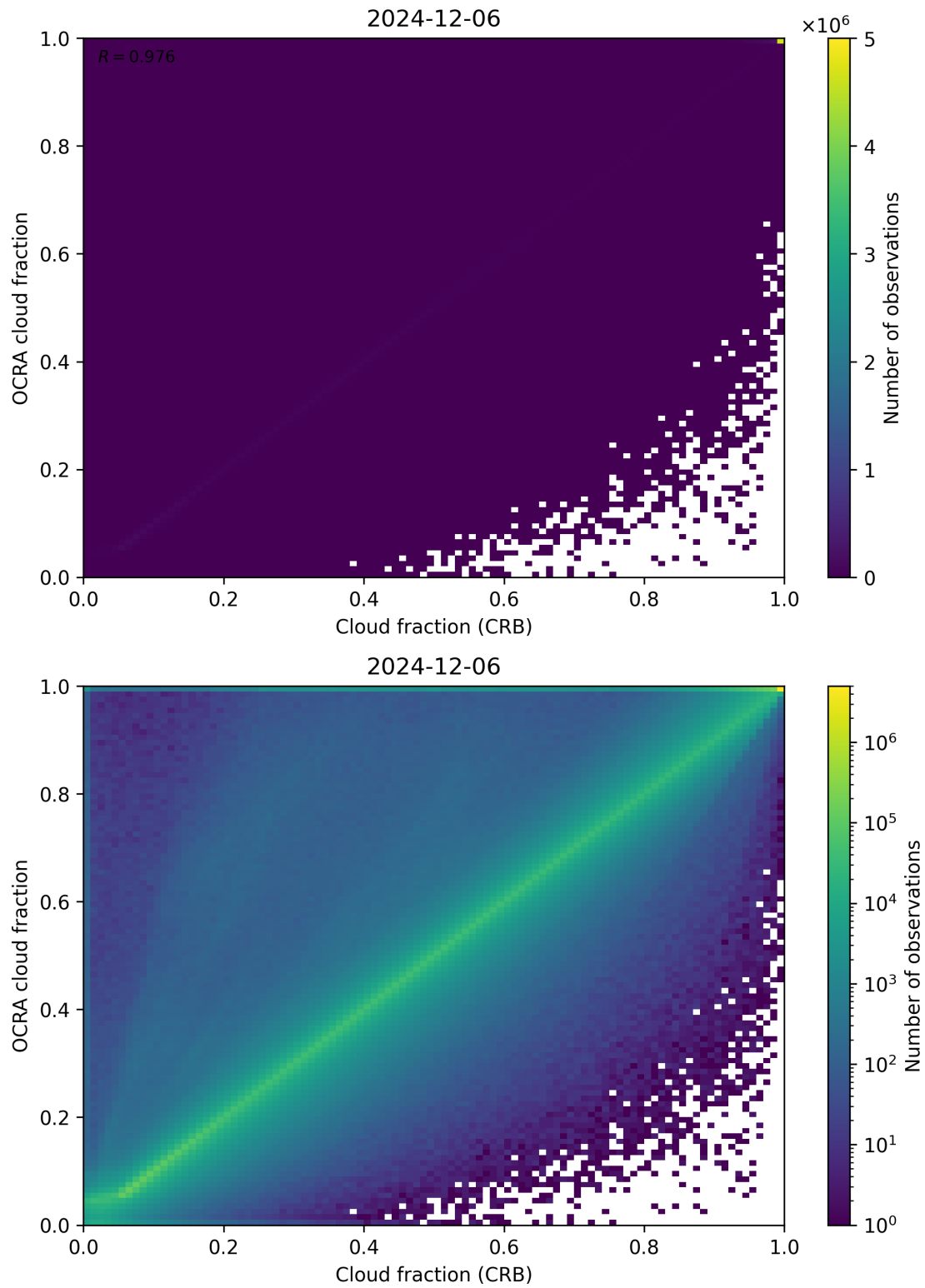
Figure 78: Scatter density plot of “Cloud fraction (CRB)” against “OCRA cloud fraction” for 2024-12-06 to 2024-12-07.
