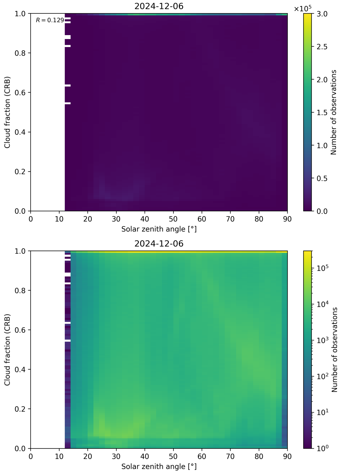
Figure 101: Scatter density plot of “Solar zenith angle” against “Cloud fraction (CRB)” for 2024-12-06 to 2024-12-07.
