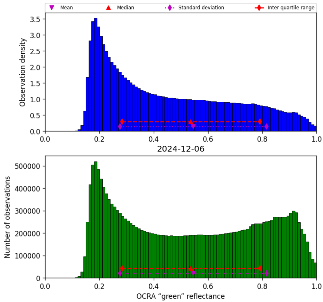
Figure 52: Histogram of “OCRA “green” reflectance” for 2024-12-06 to 2024-12-07
