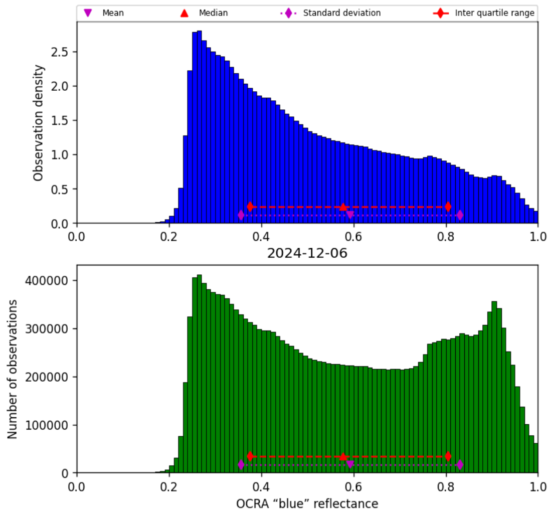
Figure 51: Histogram of “OCRA “blue” reflectance” for 2024-12-06 to 2024-12-07
