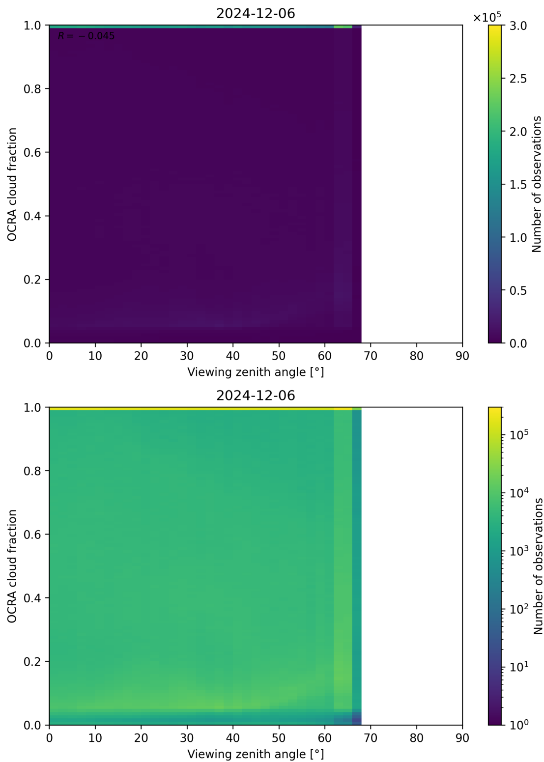
Figure 108: Scatter density plot of “Viewing zenith angle” against “OCRA cloud fraction” for 2024-12-06 to 2024-12-07.
