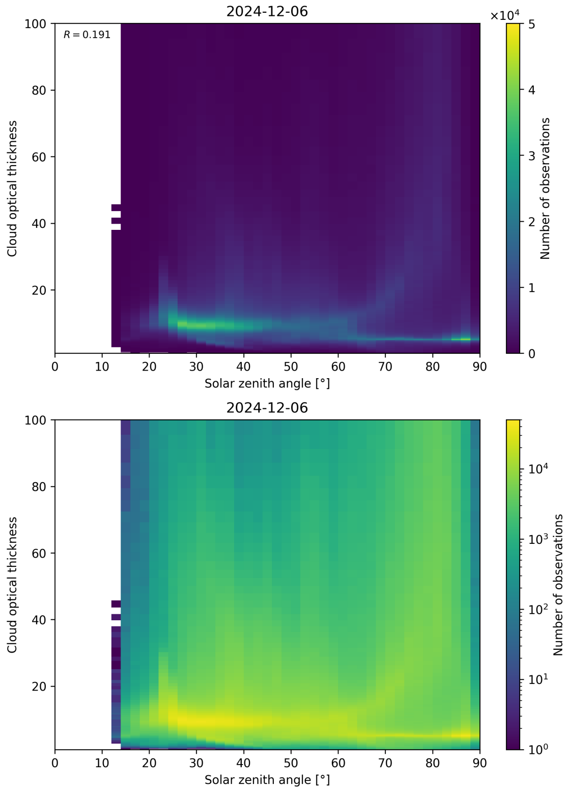
Figure 103: Scatter density plot of “Solar zenith angle” against “Cloud optical thickness” for 2024-12-06 to 2024-12-07.
