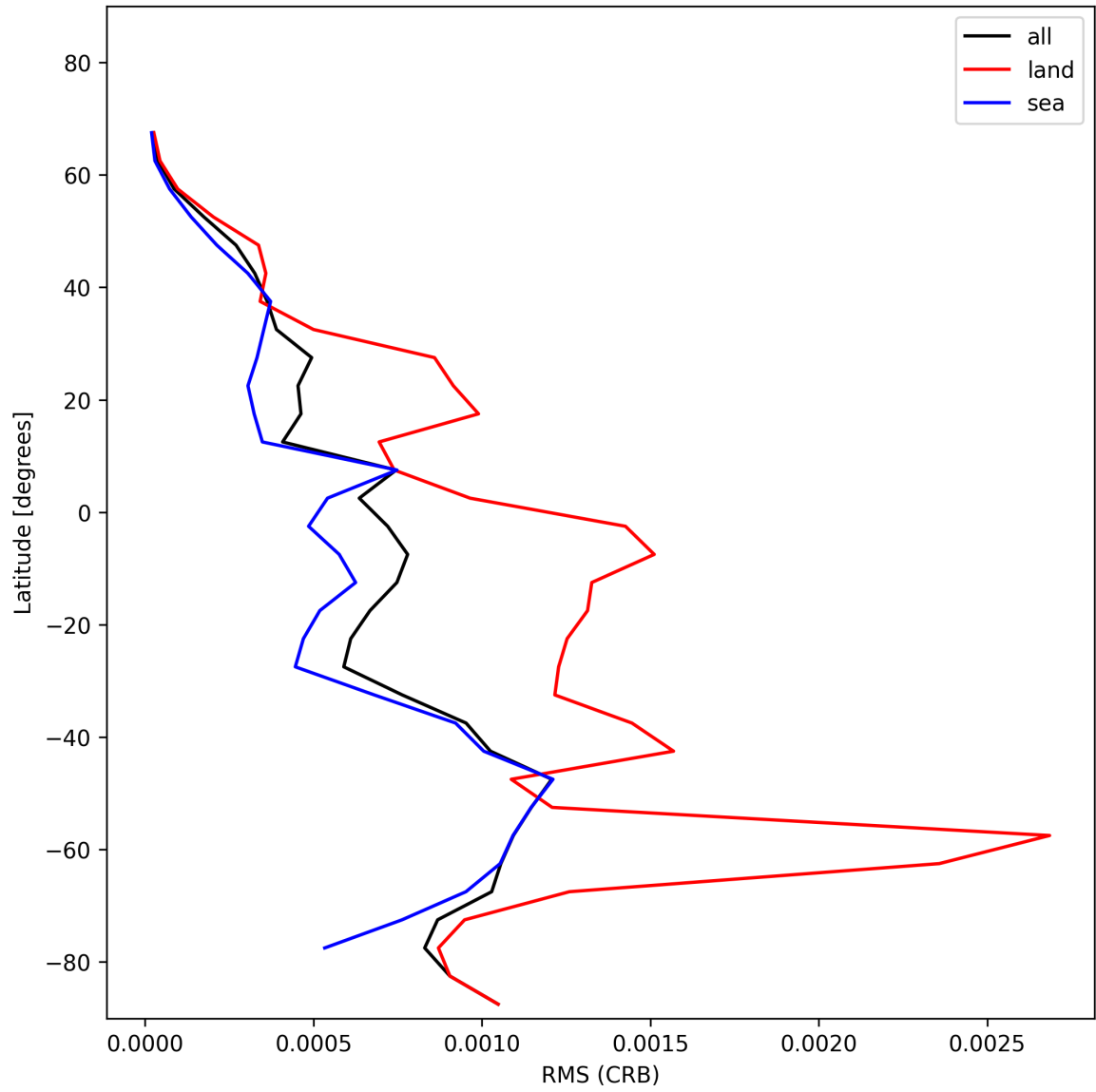
Figure 32: Zonal average of “RMS (CRB)” for 2024-12-06 to 2024-12-07.
