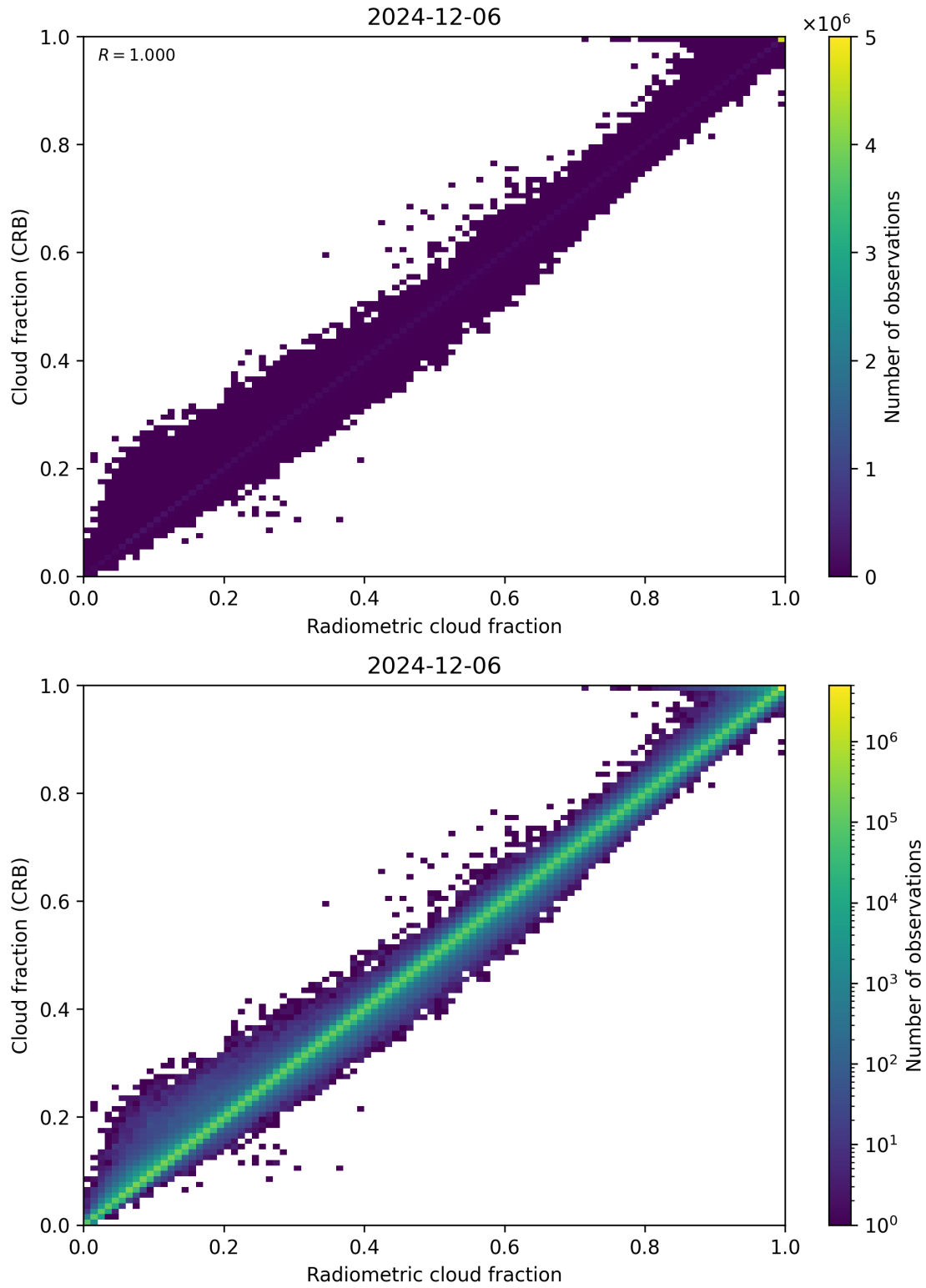
Figure 73: Scatter density plot of “Radiometric cloud fraction” against “Cloud fraction (CRB)” for 2024-12-06 to 2024-12-07.
