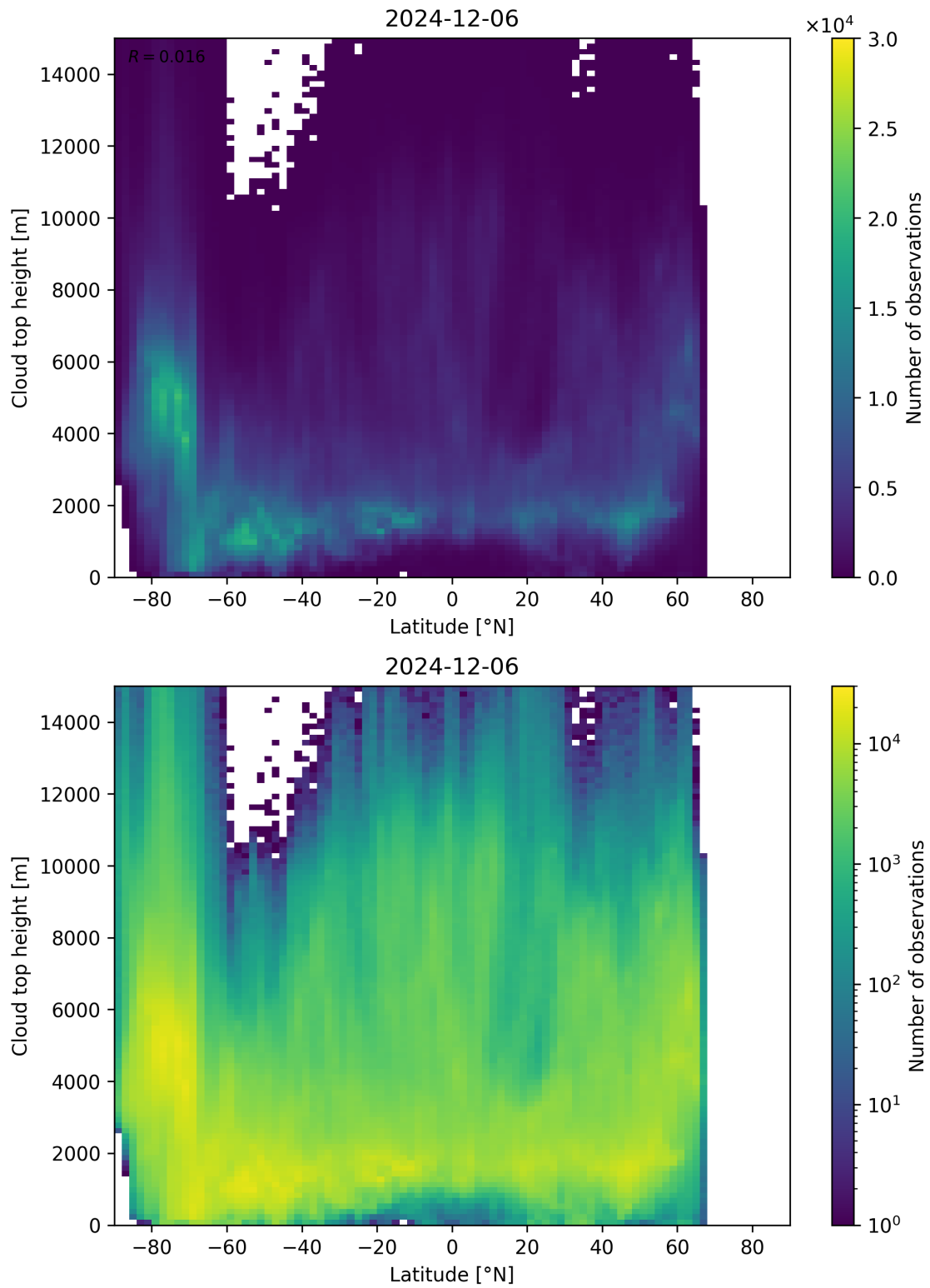
Figure 97: Scatter density plot of “Latitude” against “Cloud top height” for 2024-12-06 to 2024-12-07.
