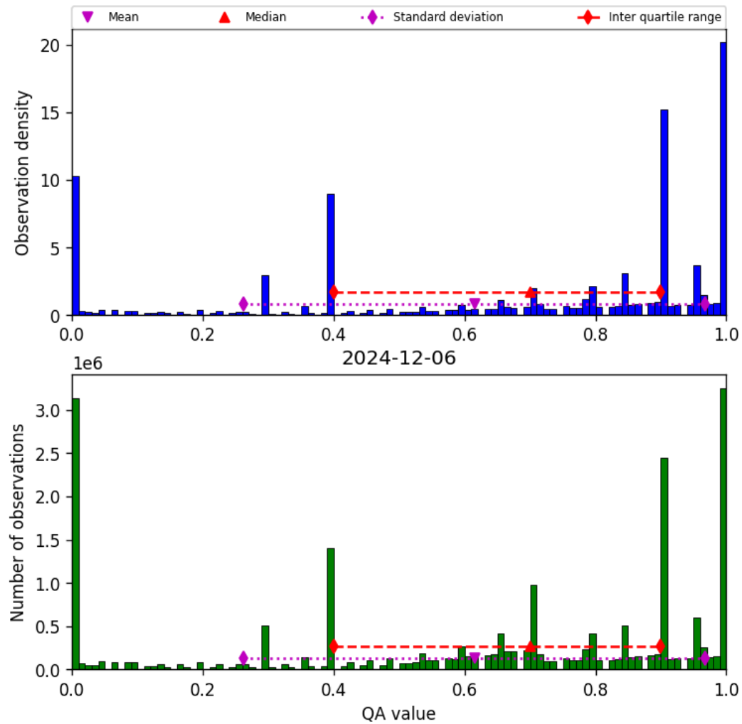
Figure 38: Histogram of “QA value” for 2024-12-06 to 2024-12-07
