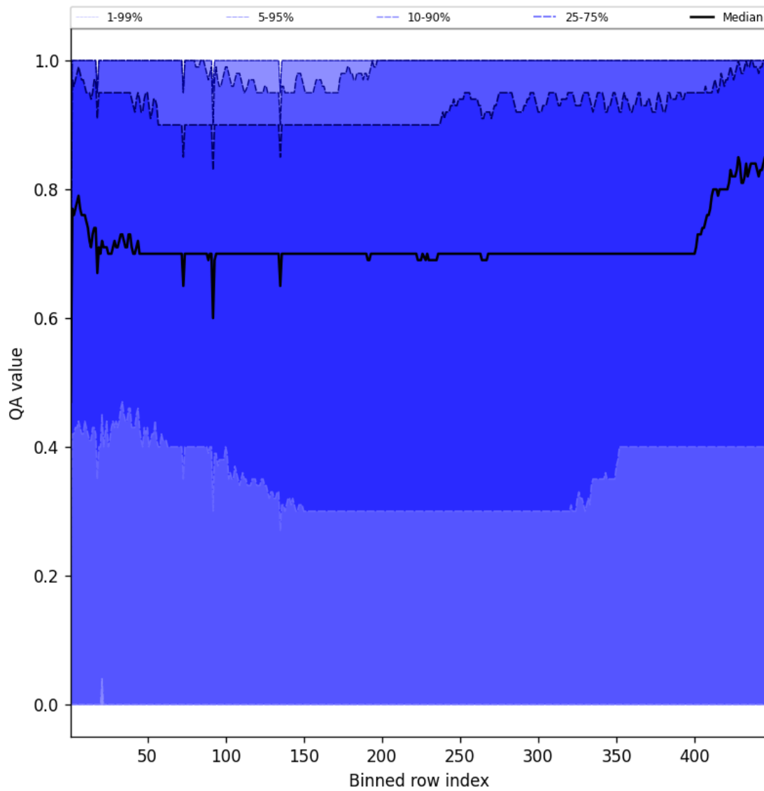
Figure 54: Along track statistics of “QA value” for 2024-12-06 to 2024-12-07
