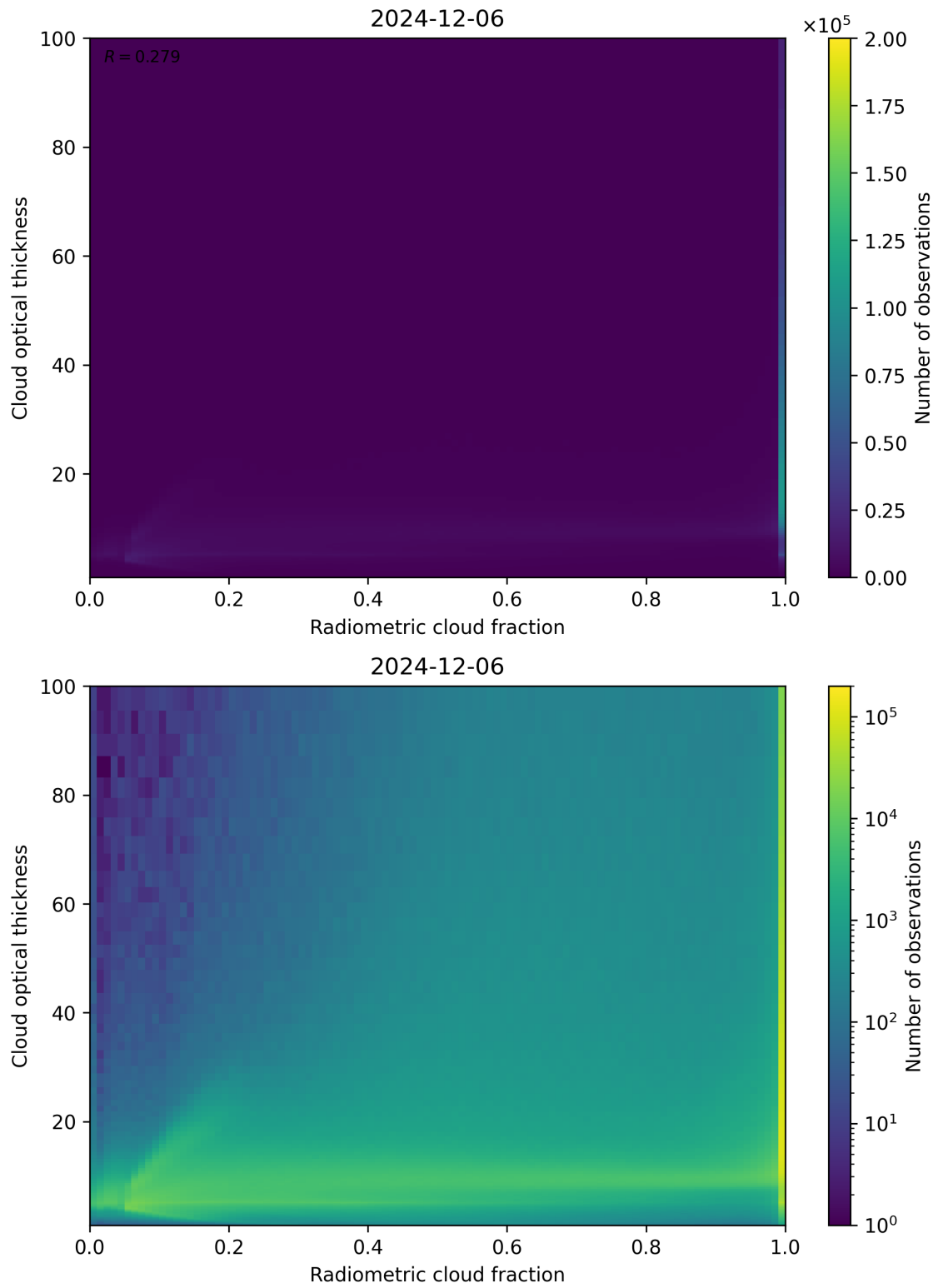
Figure 75: Scatter density plot of “Radiometric cloud fraction” against “Cloud optical thickness” for 2024-12-06 to 2024-12-07.
