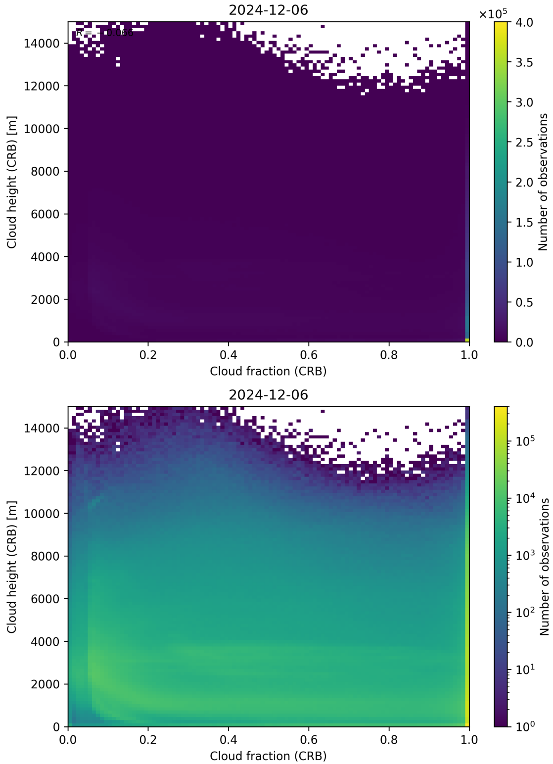
Figure 79: Scatter density plot of “Cloud fraction (CRB)” against “Cloud height (CRB)” for 2024-12-06 to 2024-12-07.
