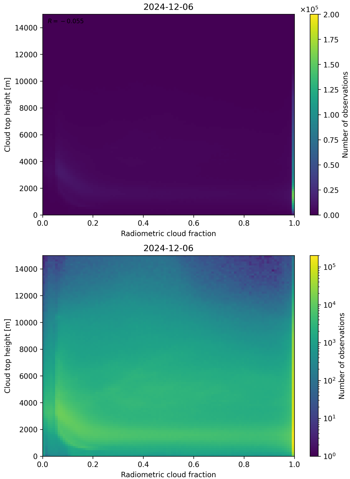
Figure 76: Scatter density plot of “Radiometric cloud fraction” against “Cloud top height” for 2024-12-06 to 2024-12-07.
