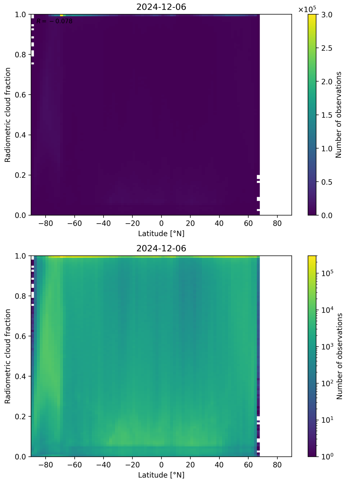
Figure 92: Scatter density plot of “Latitude” against “Radiometric cloud fraction” for 2024-12-06 to 2024-12-07.
