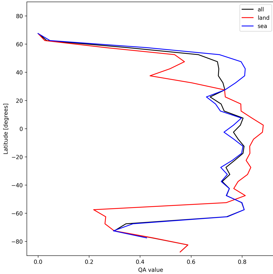
Figure 22: Zonal average of “QA value” for 2024-12-06 to 2024-12-07.
