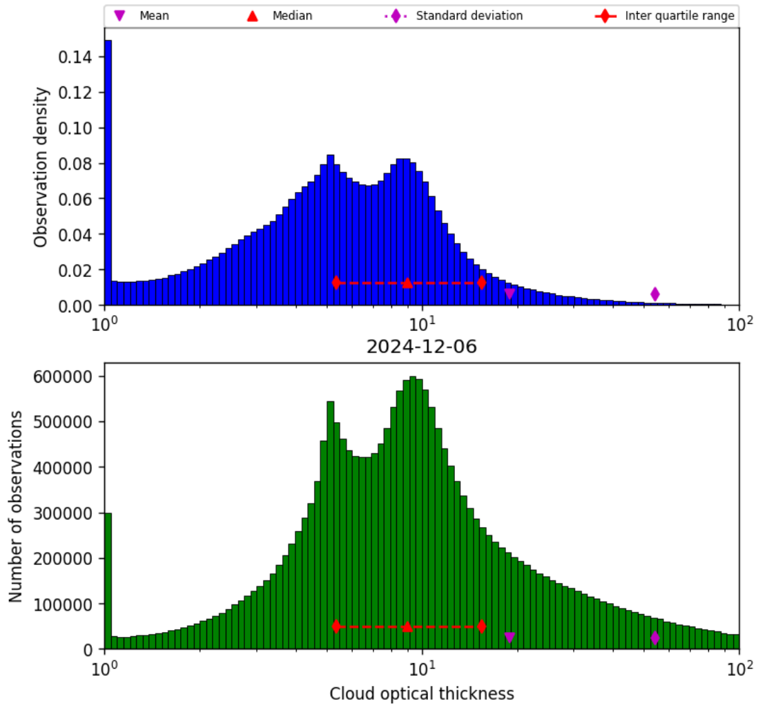
Figure 41: Histogram of “Cloud optical thickness” for 2024-12-06 to 2024-12-07
