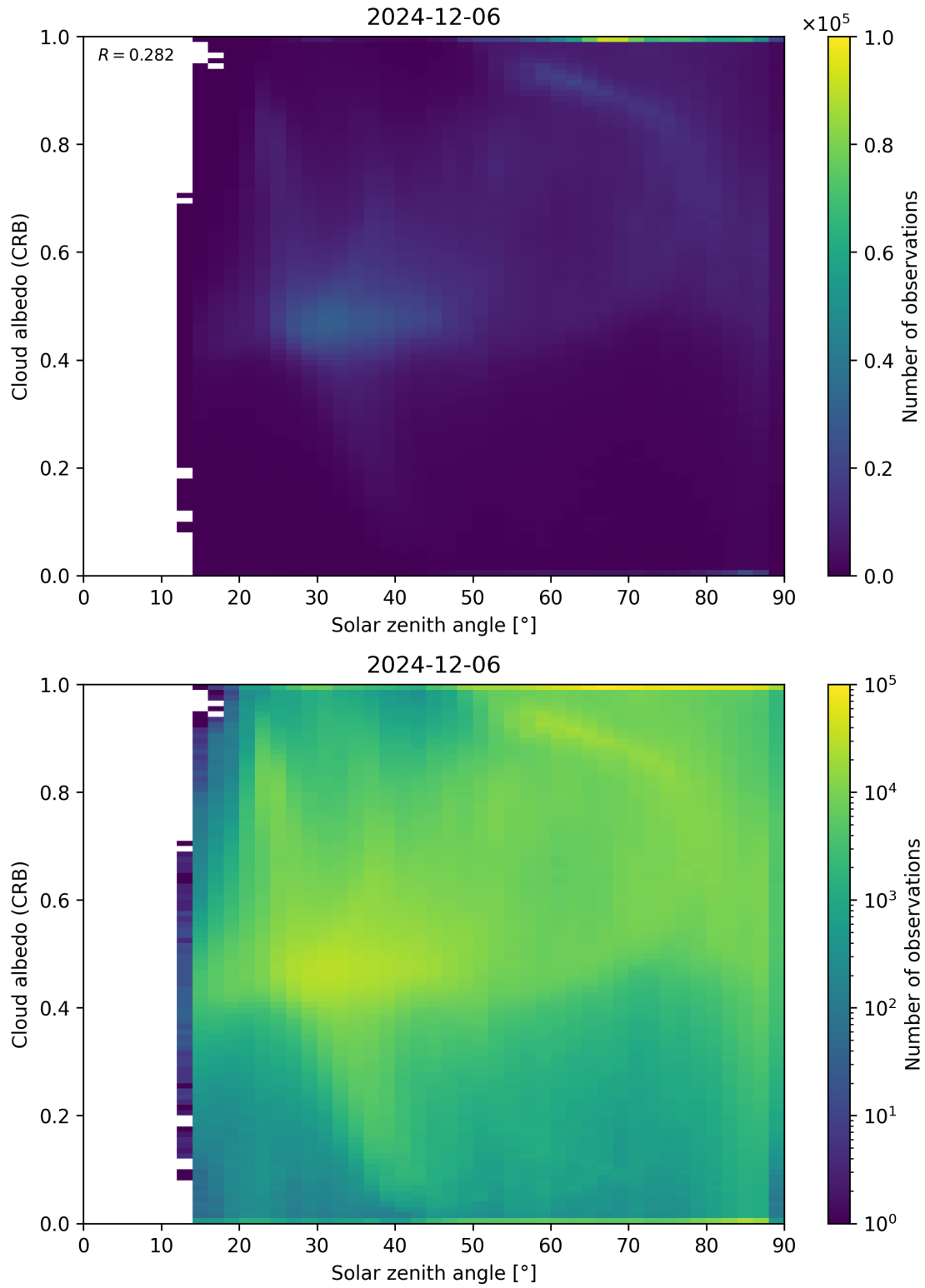
Figure 98: Scatter density plot of “Solar zenith angle” against “Cloud albedo (CRB)” for 2024-12-06 to 2024-12-07.
