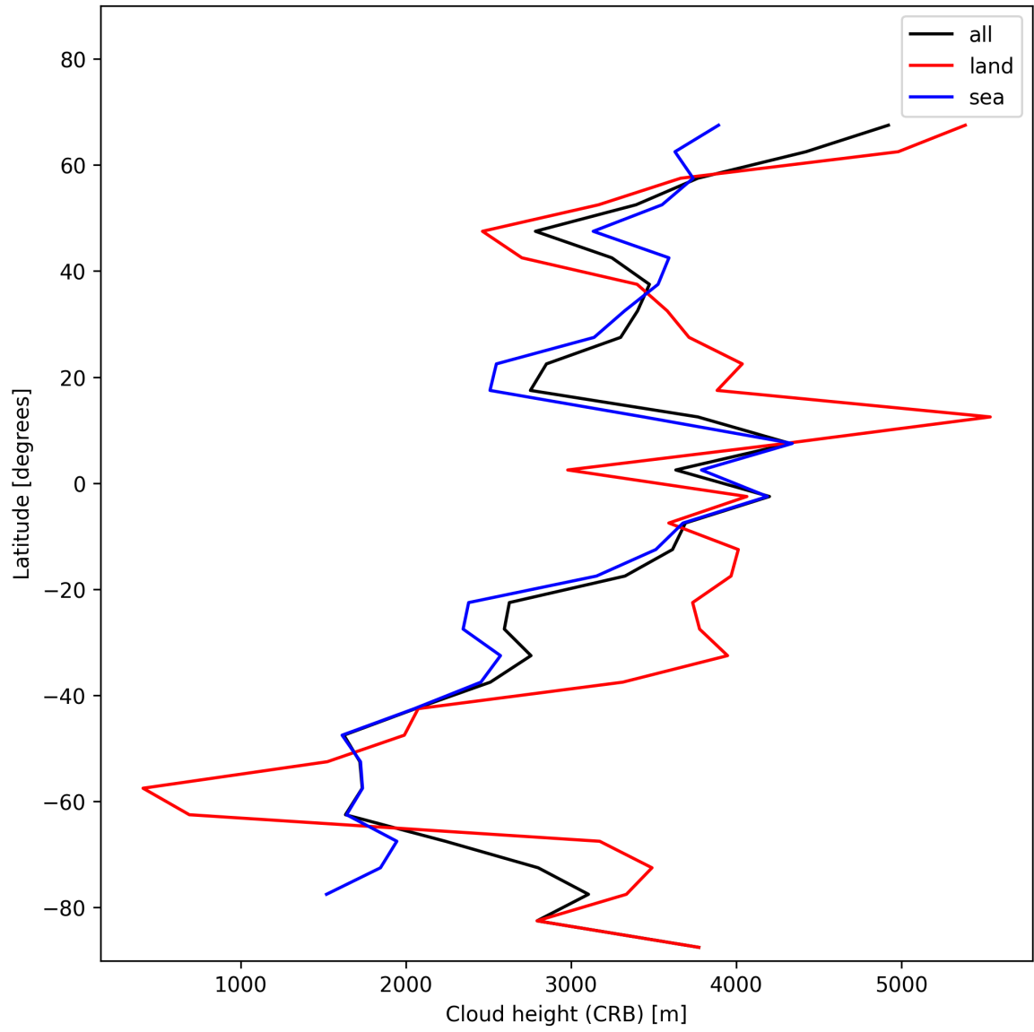
Figure 27: Zonal average of “Cloud height (CRB)” for 2024-12-06 to 2024-12-07.
