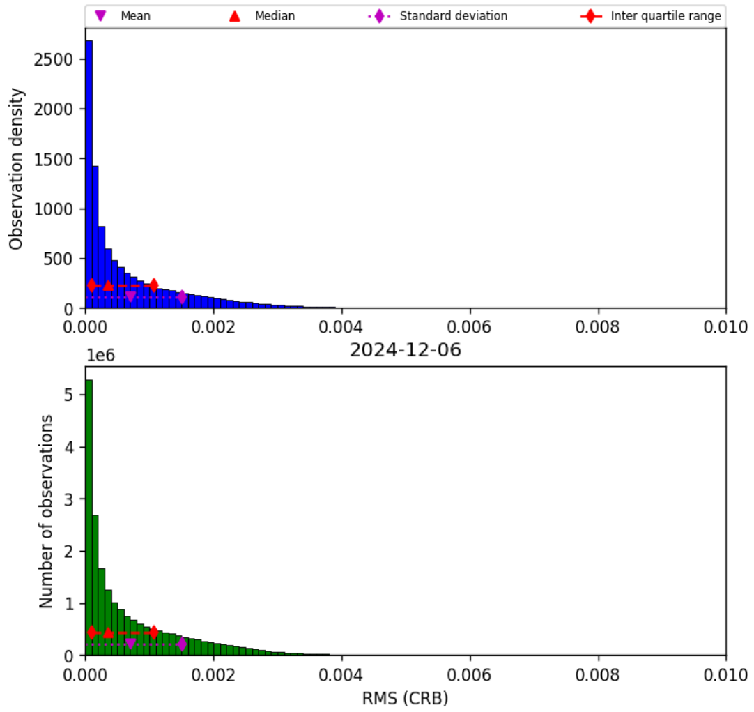
Figure 48: Histogram of “RMS (CRB)” for 2024-12-06 to 2024-12-07
