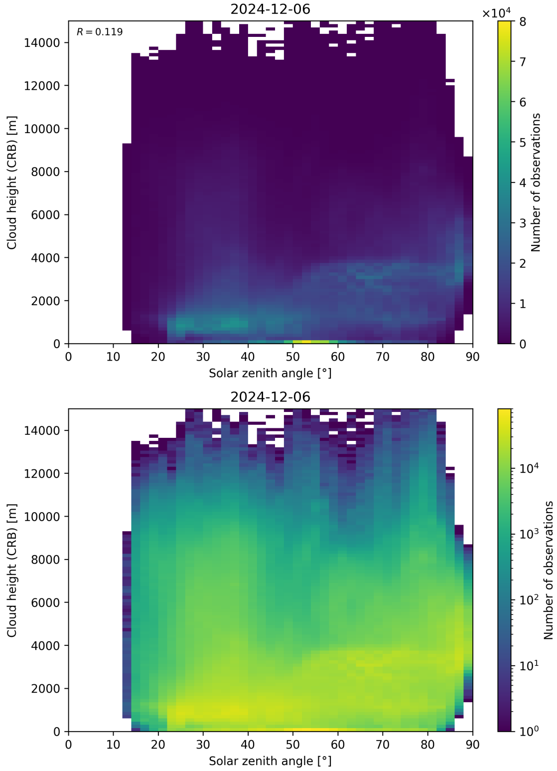
Figure 102: Scatter density plot of “Solar zenith angle” against “Cloud height (CRB)” for 2024-12-06 to 2024-12-07.
