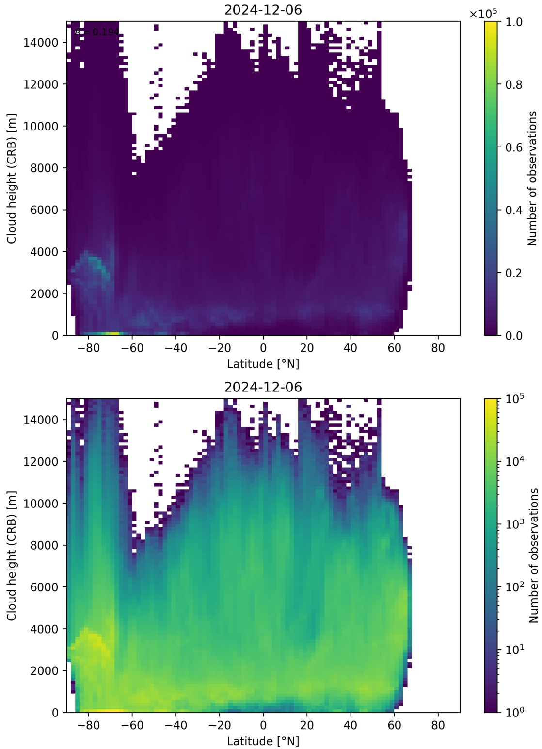
Figure 95: Scatter density plot of “Latitude” against “Cloud height (CRB)” for 2024-12-06 to 2024-12-07.
