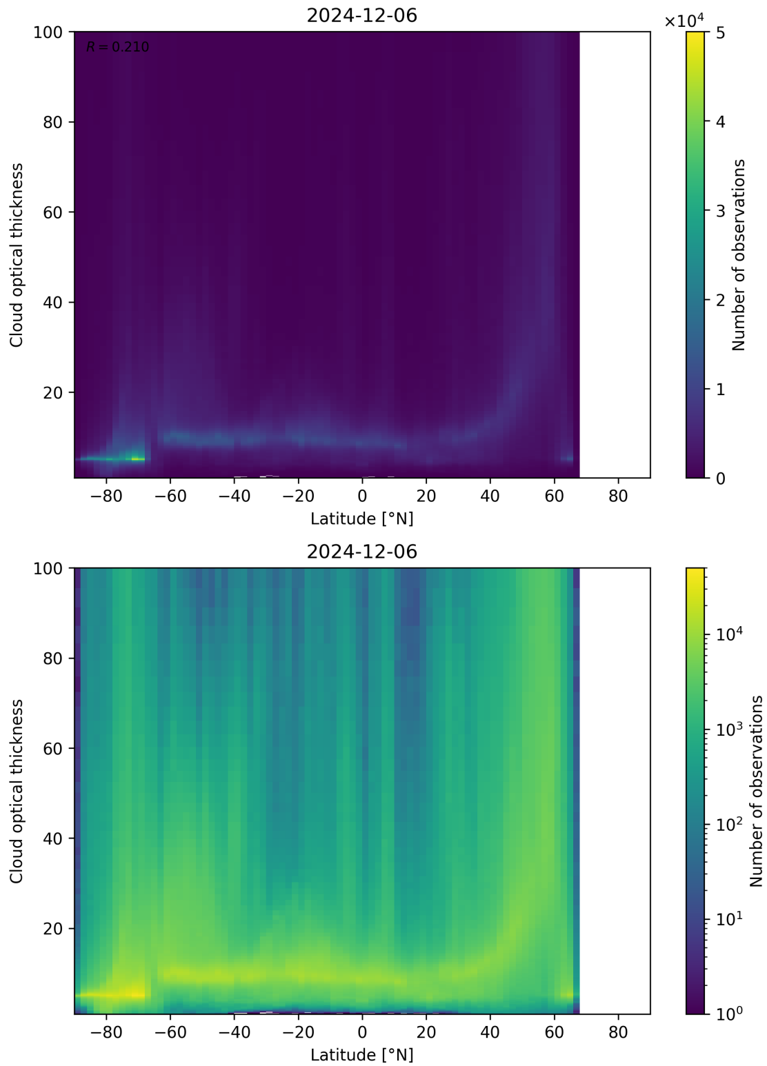
Figure 96: Scatter density plot of “Latitude” against “Cloud optical thickness” for 2024-12-06 to 2024-12-07.
