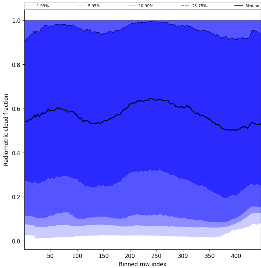
Figure 55: Along track statistics of “Radiometric cloud fraction” for 2024-12-06 to 2024-12-07
