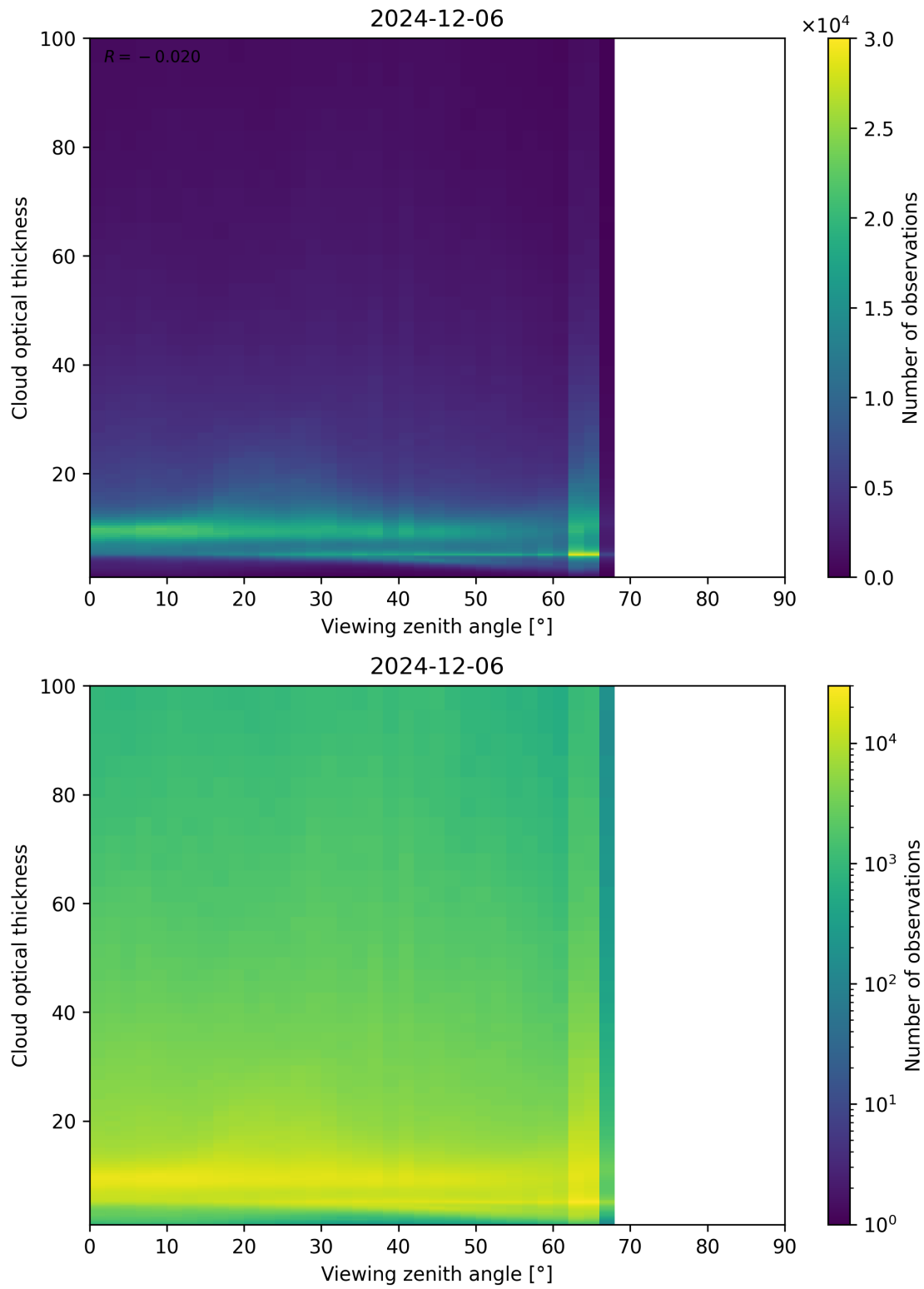
Figure 111: Scatter density plot of “Viewing zenith angle” against “Cloud optical thickness” for 2024-12-06 to 2024-12-07.
