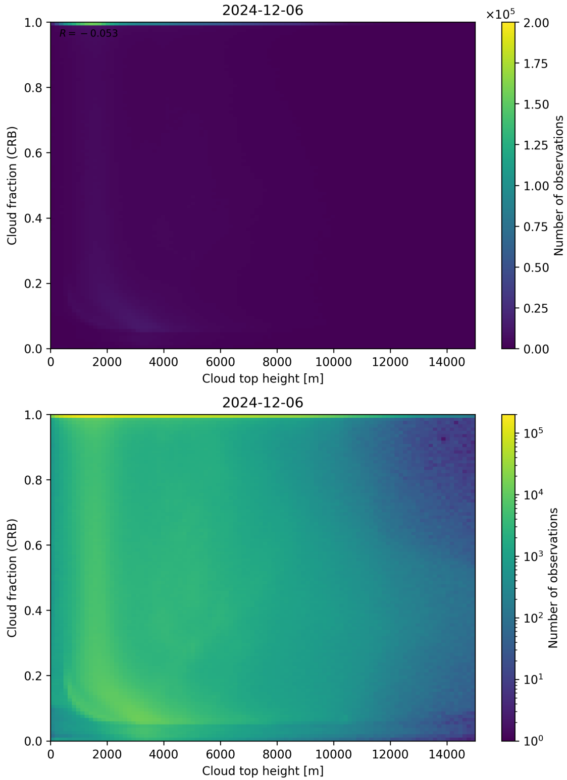
Figure 88: Scatter density plot of “Cloud top height” against “Cloud fraction (CRB)” for 2024-12-06 to 2024-12-07.
