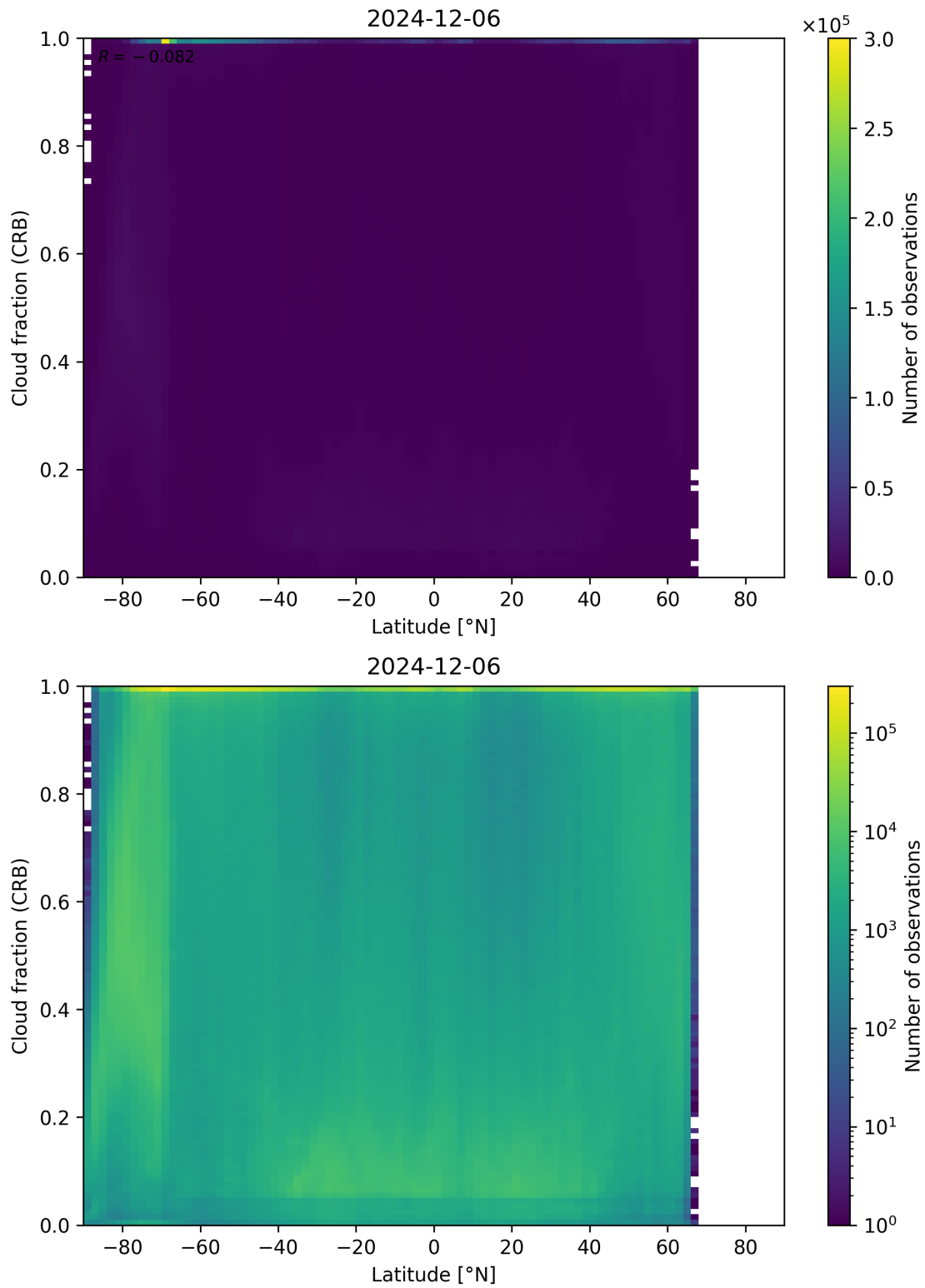
Figure 94: Scatter density plot of “Latitude” against “Cloud fraction (CRB)” for 2024-12-06 to 2024-12-07.
