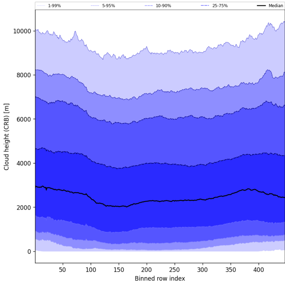
Figure 59: Along track statistics of “Cloud height (CRB)” for 2024-12-06 to 2024-12-07
