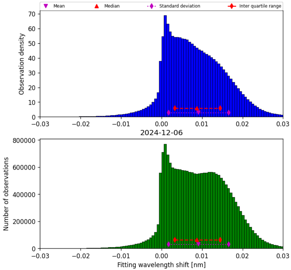
Figure 49: Histogram of “Fitting wavelength shift” for 2024-12-06 to 2024-12-07
