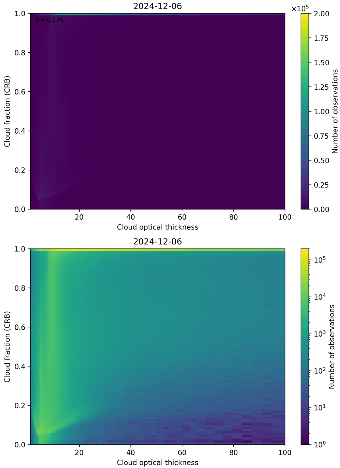
Figure 84: Scatter density plot of “Cloud optical thickness” against “Cloud fraction (CRB)” for 2024-12-06 to 2024-12-07.
