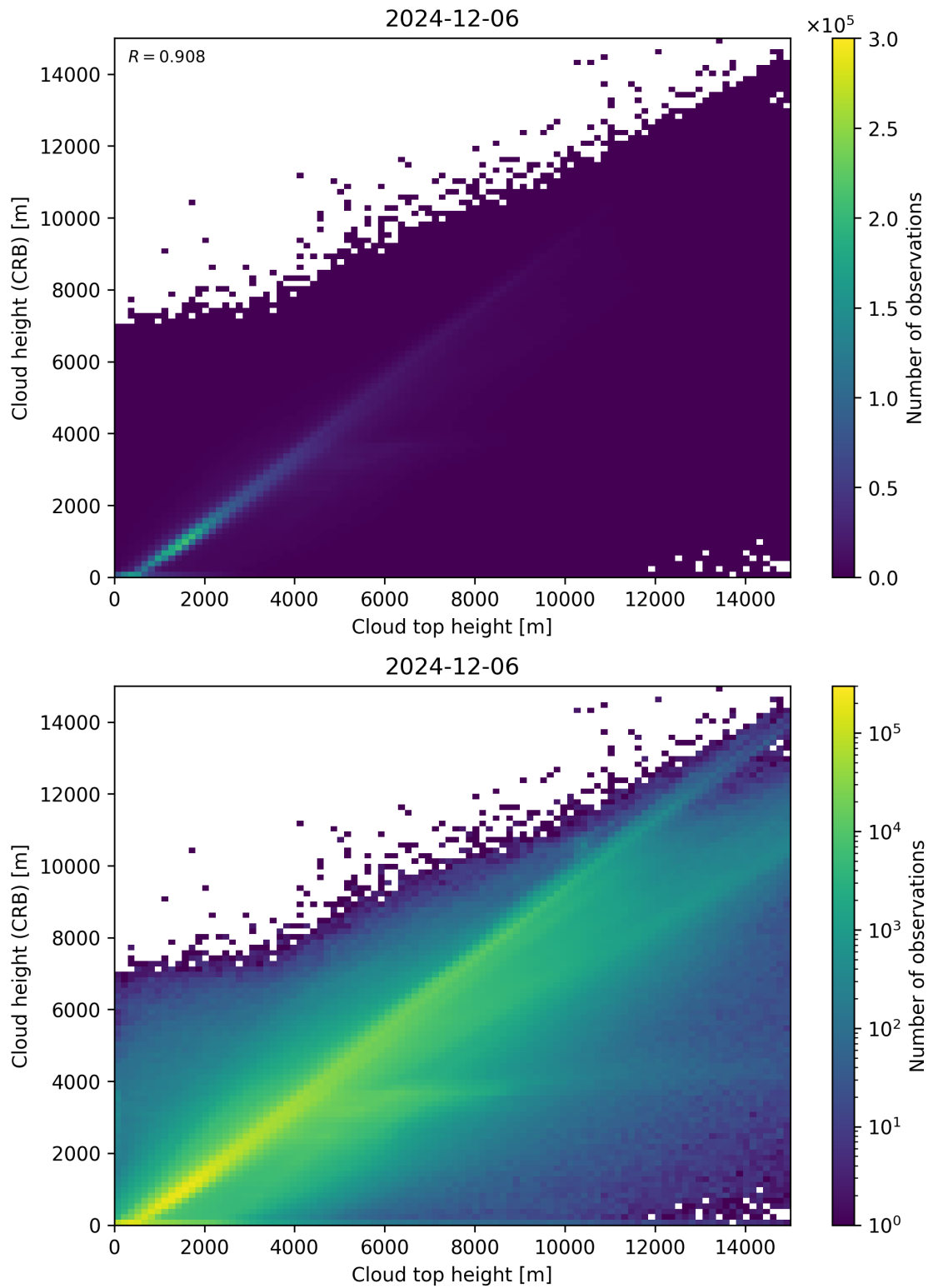
Figure 89: Scatter density plot of “Cloud top height” against “Cloud height (CRB)” for 2024-12-06 to 2024-12-07.
