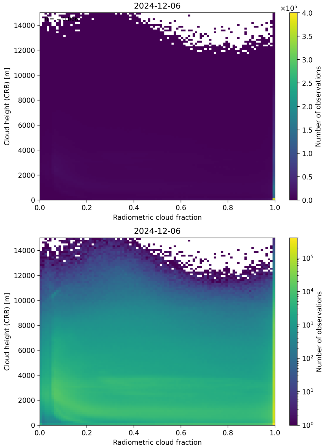
Figure 74: Scatter density plot of “Radiometric cloud fraction” against “Cloud height (CRB)” for 2024-12-06 to 2024-12-07.
