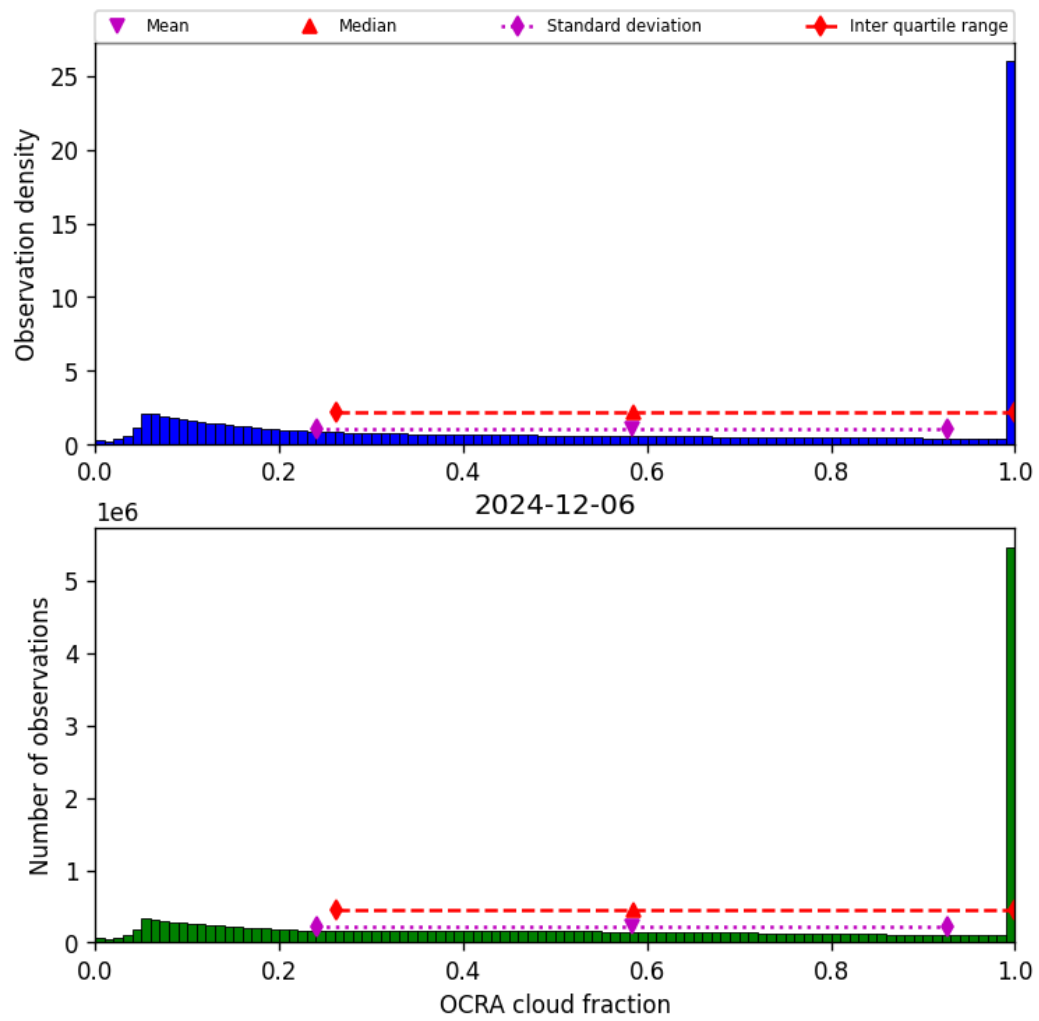
Figure 50: Histogram of “OCRA cloud fraction” for 2024-12-06 to 2024-12-07
