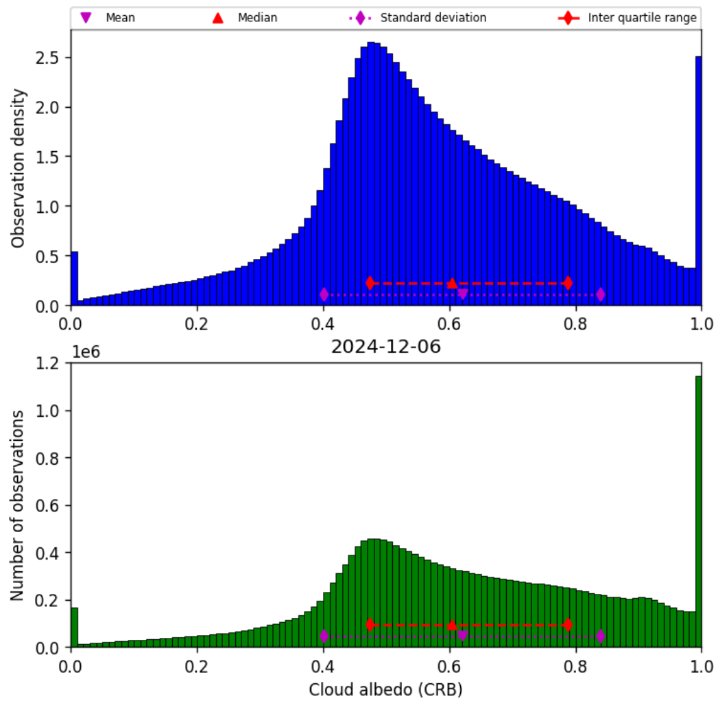
Figure 44: Histogram of “Cloud albedo (CRB)” for 2024-12-06 to 2024-12-07
