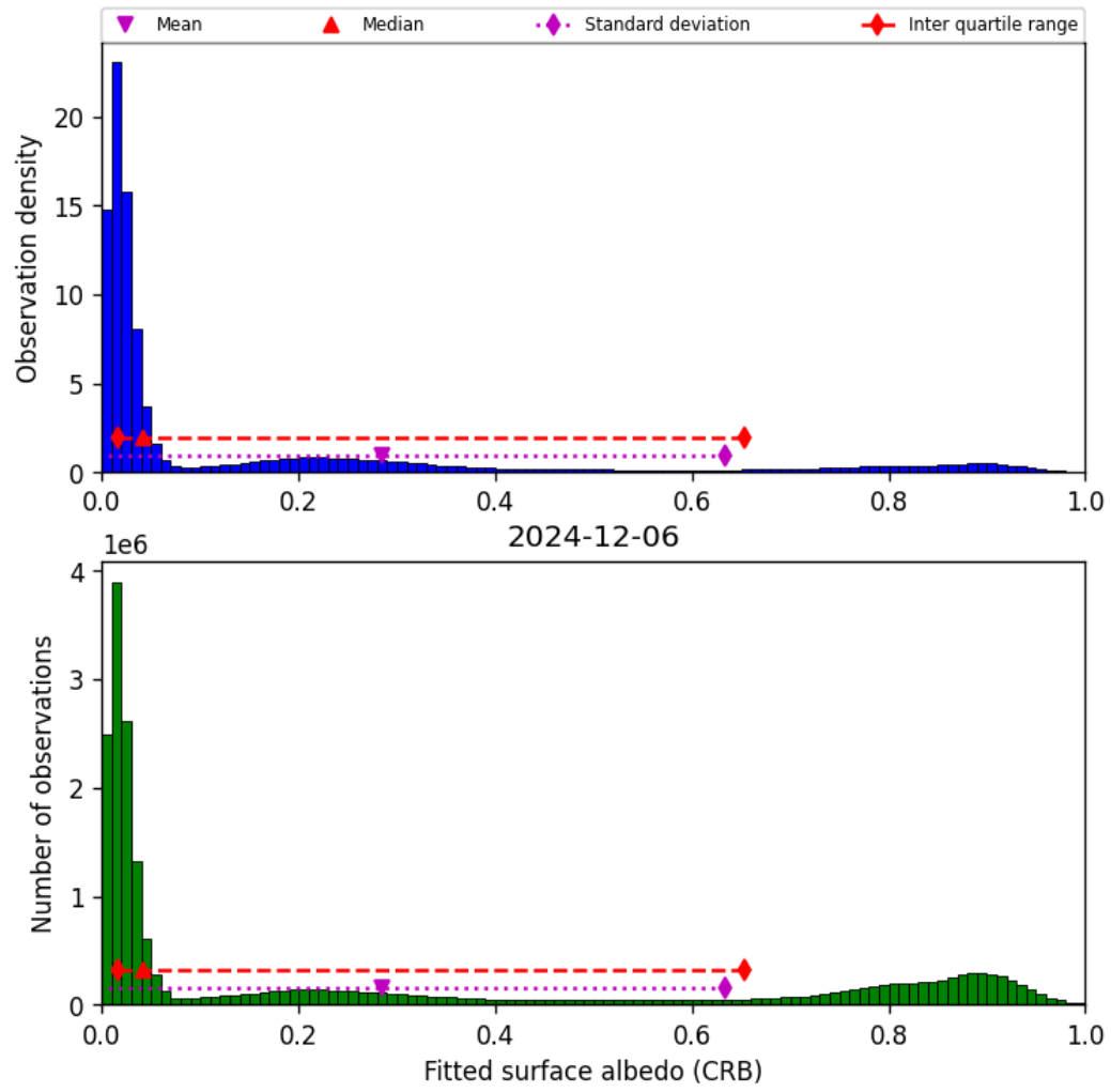
Figure 46: Histogram of “Fitted surface albedo (CRB)” for 2024-12-06 to 2024-12-07
