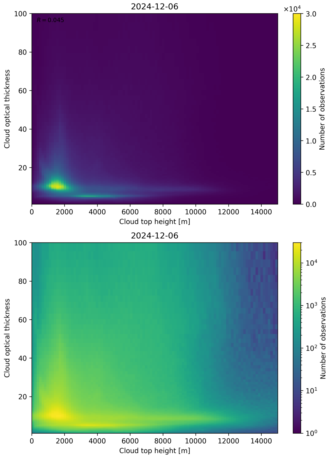
Figure 90: Scatter density plot of “Cloud top height” against “Cloud optical thickness” for 2024-12-06 to 2024-12-07.
