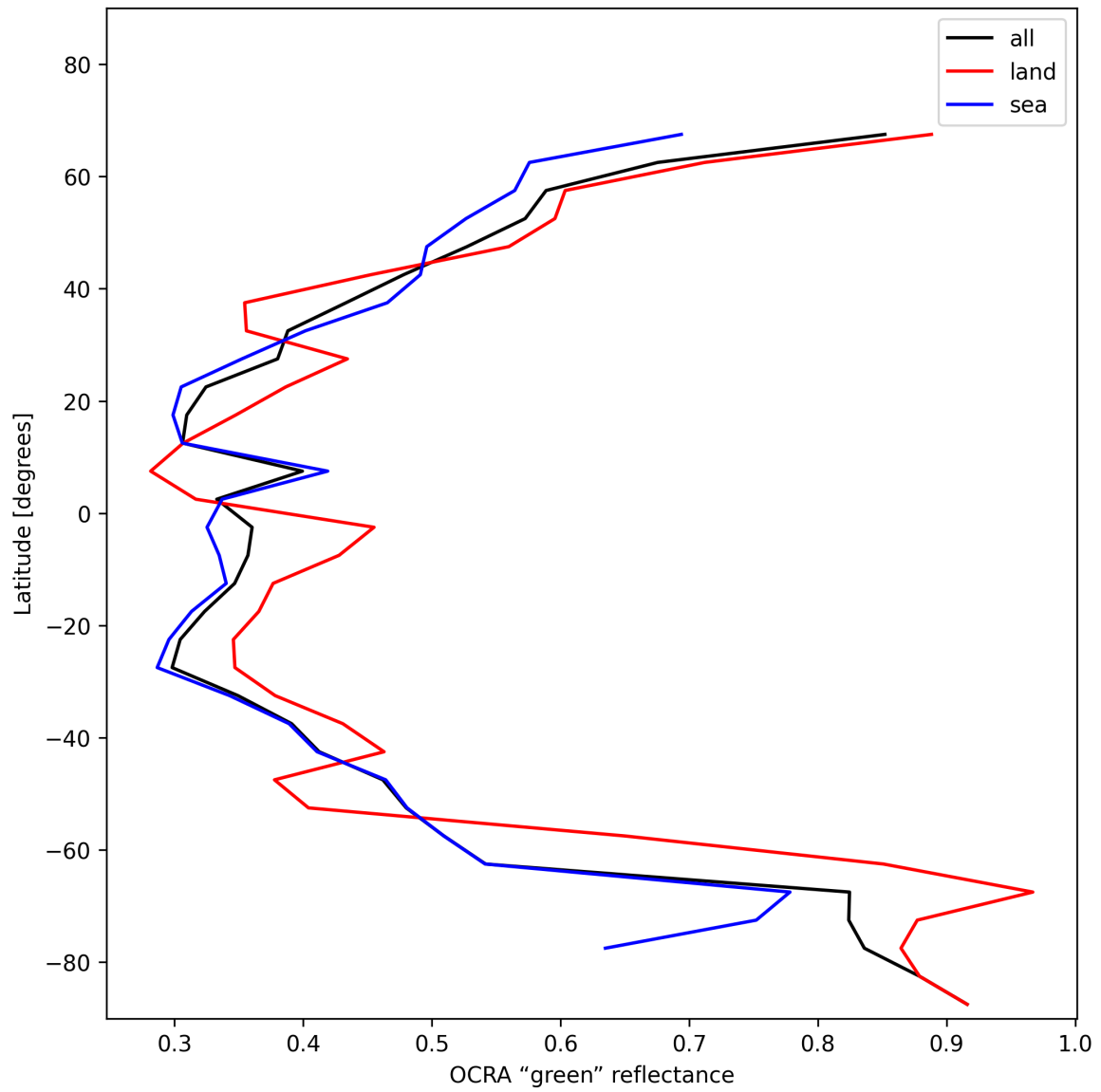
Figure 36: Zonal average of “OCRA “green” reflectance” for 2024-12-06 to 2024-12-07.
