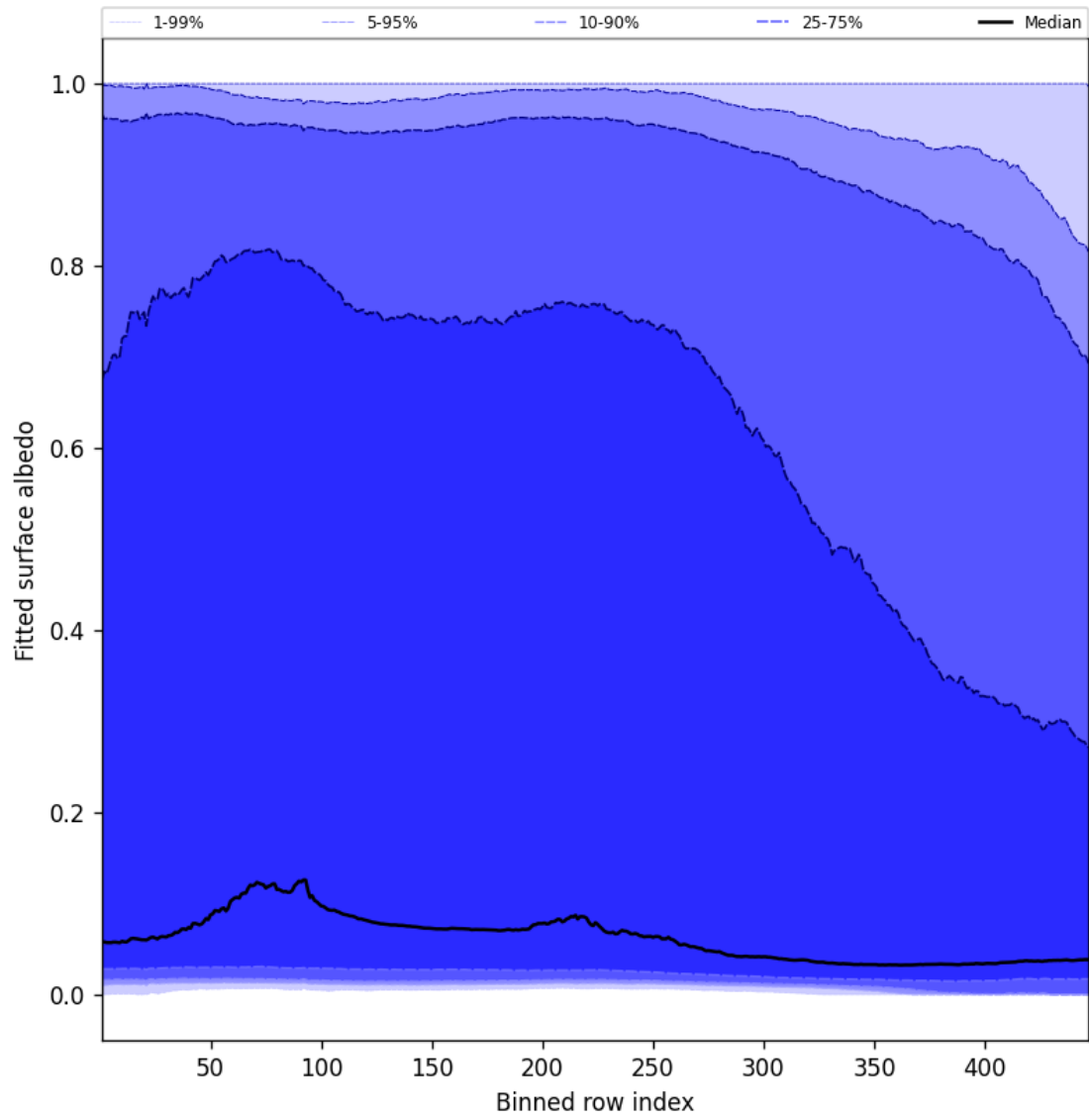
Figure 61: Along track statistics of “Fitted surface albedo” for 2024-12-06 to 2024-12-07
