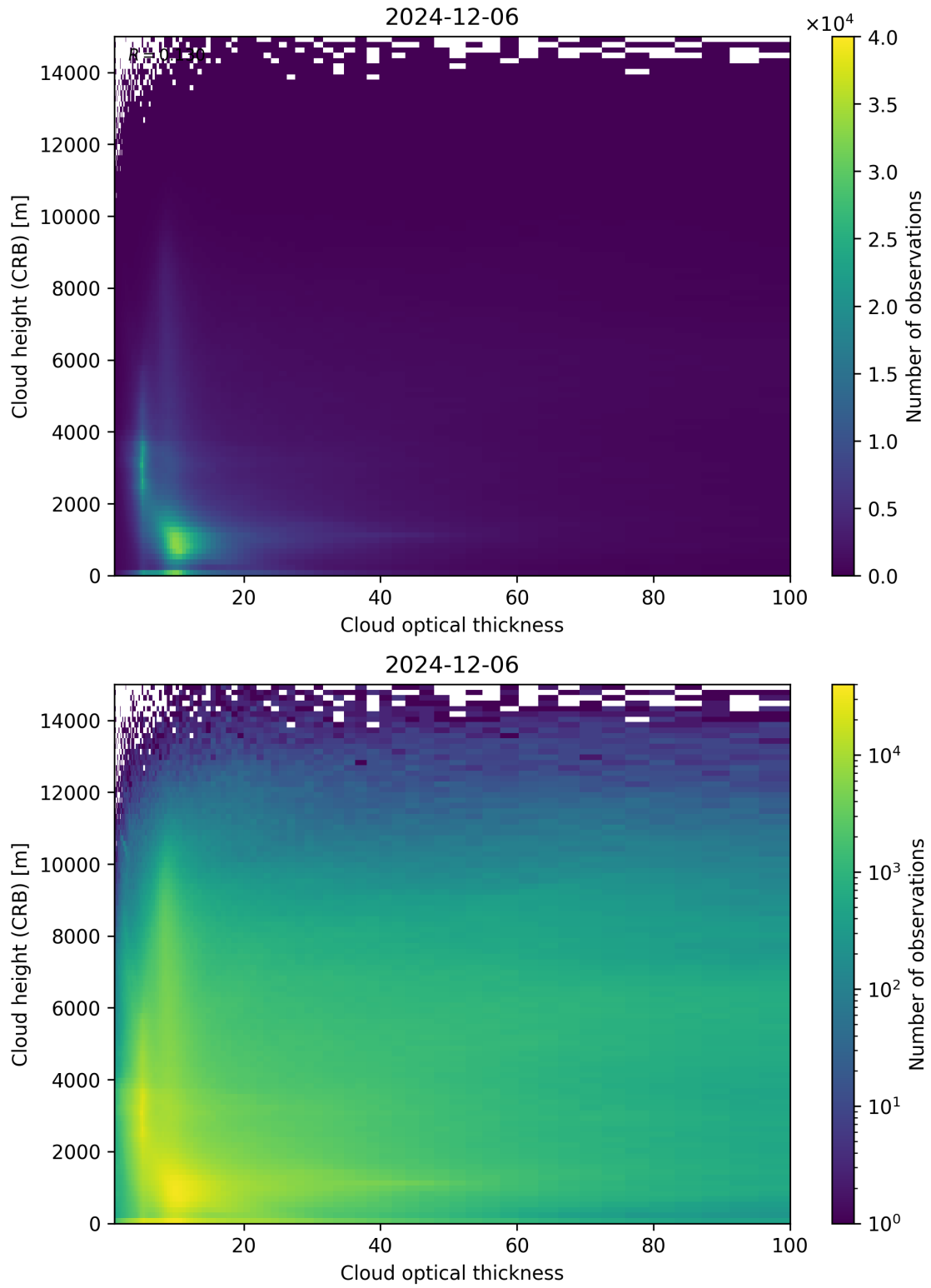
Figure 85: Scatter density plot of “Cloud optical thickness” against “Cloud height (CRB)” for 2024-12-06 to 2024-12-07.
