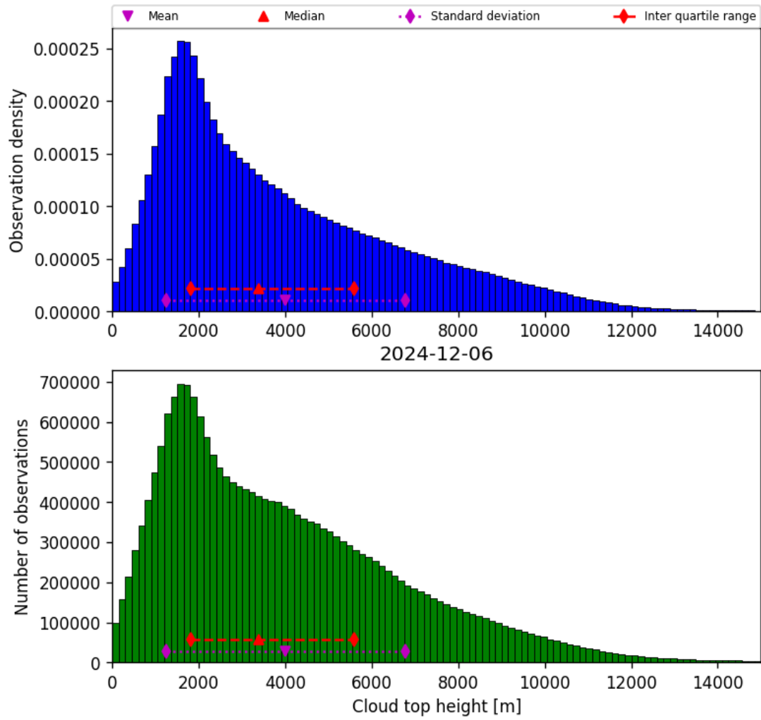
Figure 40: Histogram of “Cloud top height” for 2024-12-06 to 2024-12-07
