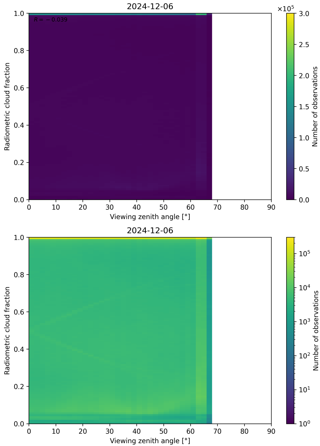
Figure 107: Scatter density plot of “Viewing zenith angle” against “Radiometric cloud fraction” for 2024-12-06 to 2024-12-07.
