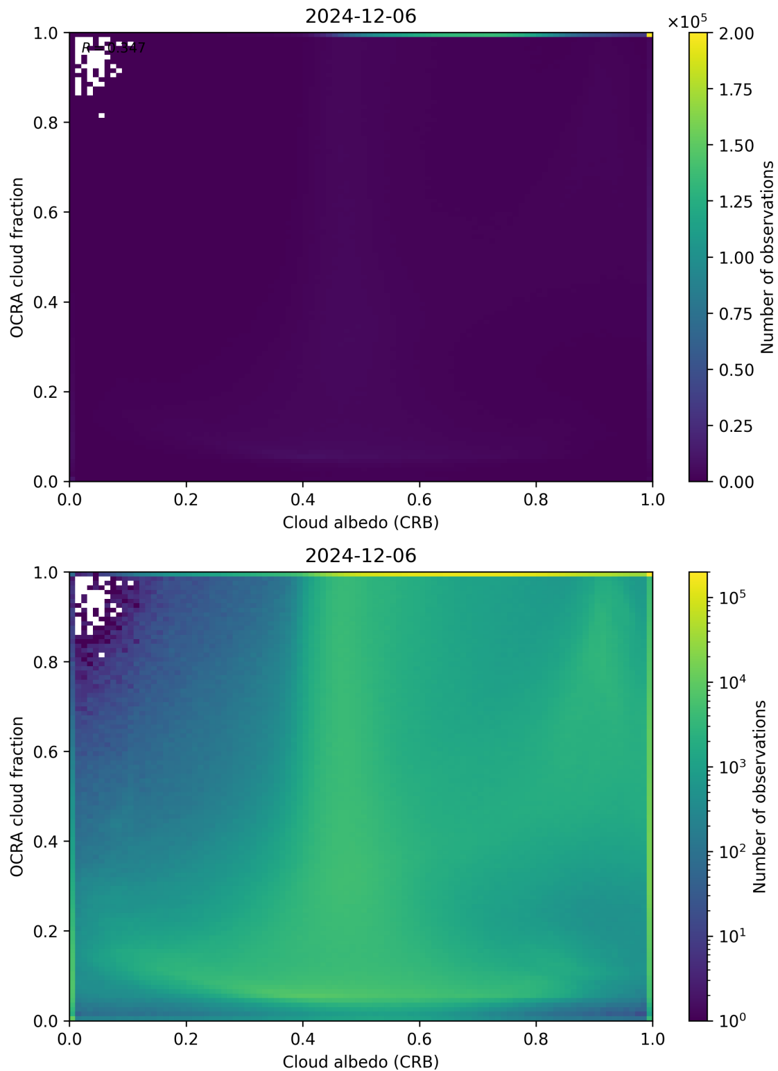
Figure 70: Scatter density plot of “Cloud albedo (CRB)” against “OCRA cloud fraction” for 2024-12-06 to 2024-12-07.
