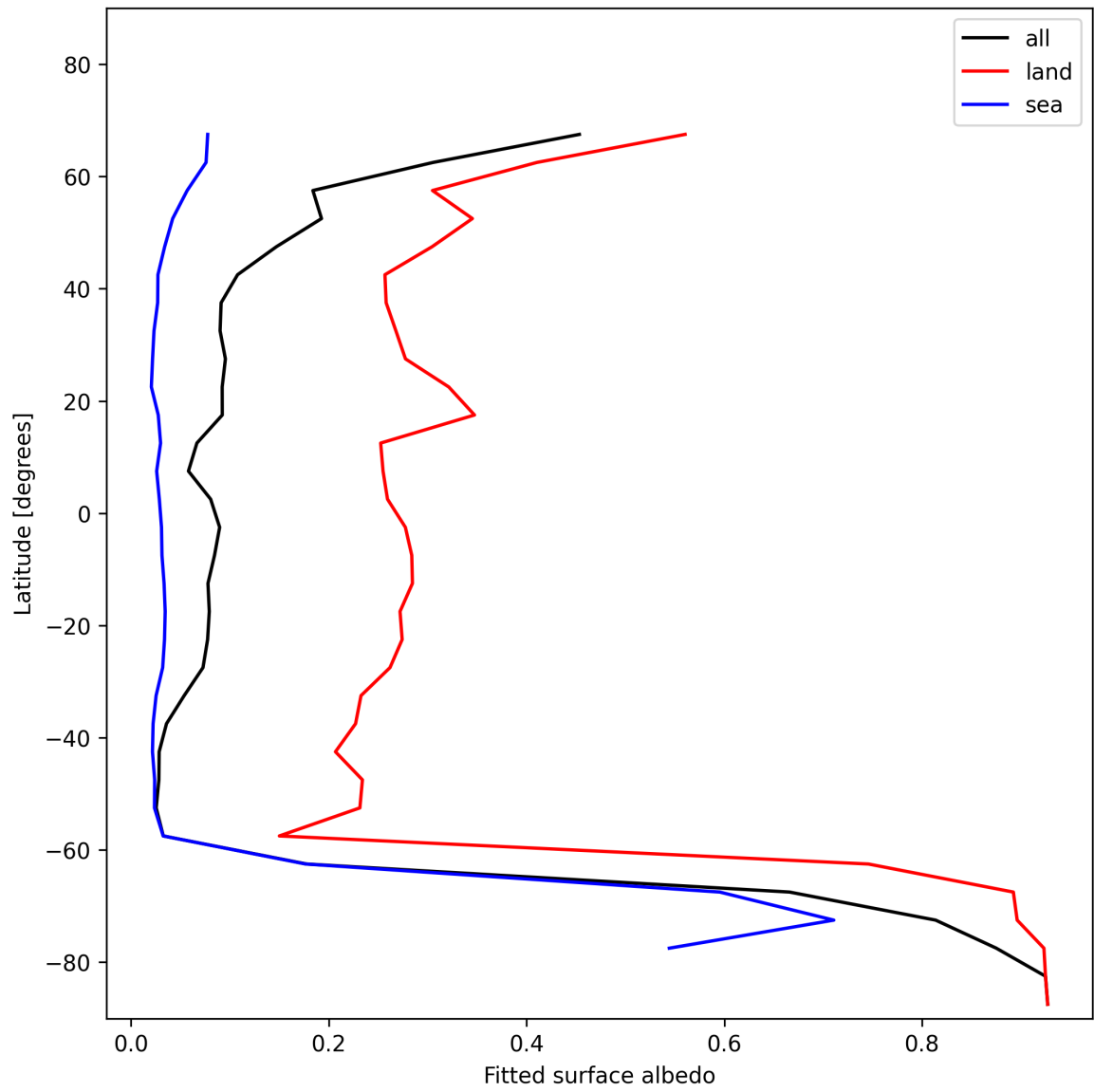
Figure 29: Zonal average of “Fitted surface albedo” for 2024-12-06 to 2024-12-07.
