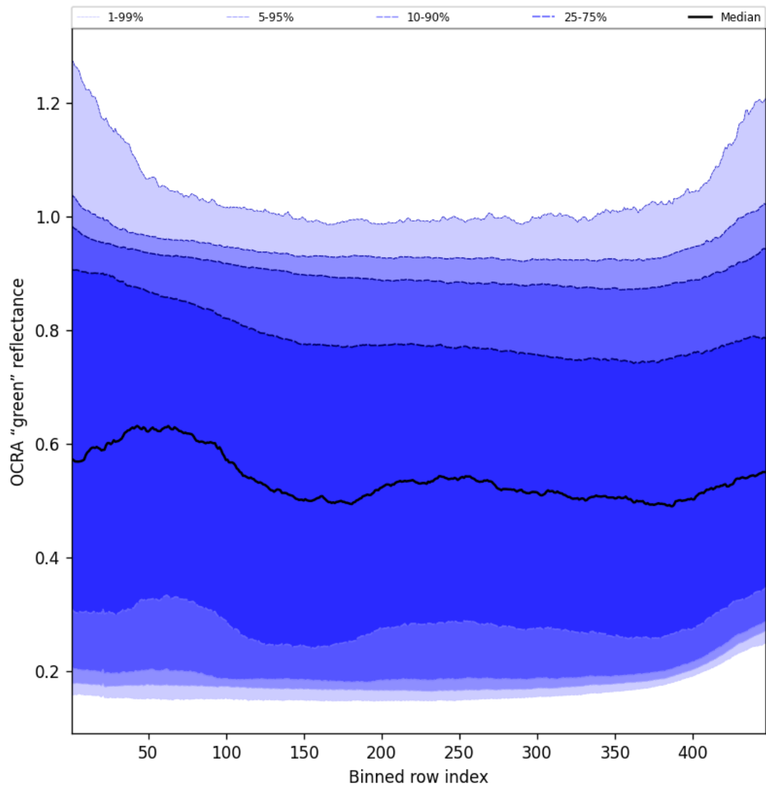
Figure 68: Along track statistics of "OCRA "green" reflectance" for 2024-12-06 to 2024-12-07
