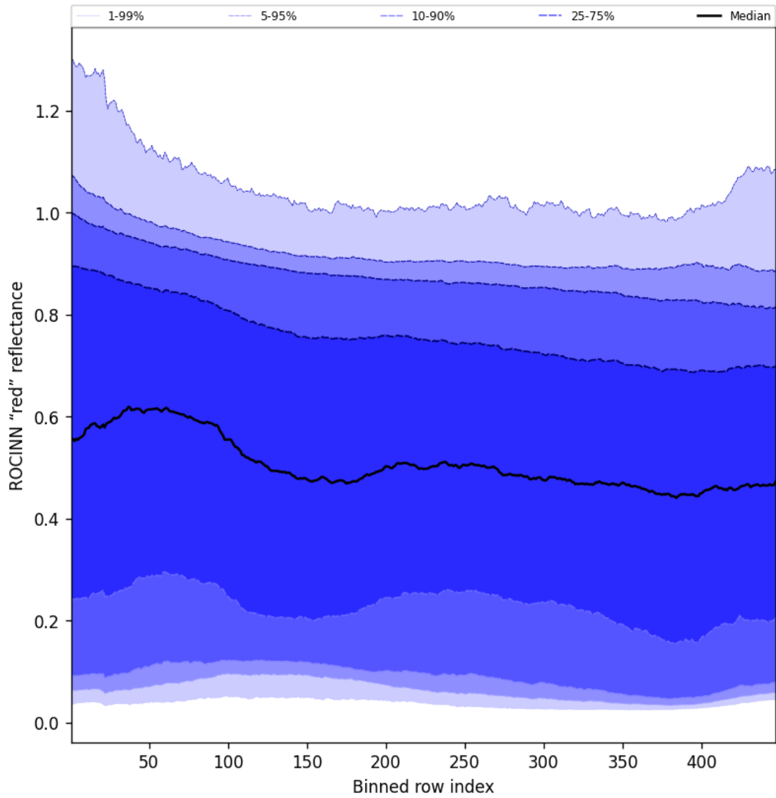
Figure 69: Along track statistics of “ROCINN “red” reflectance” for 2024-12-06 to 2024-12-07
