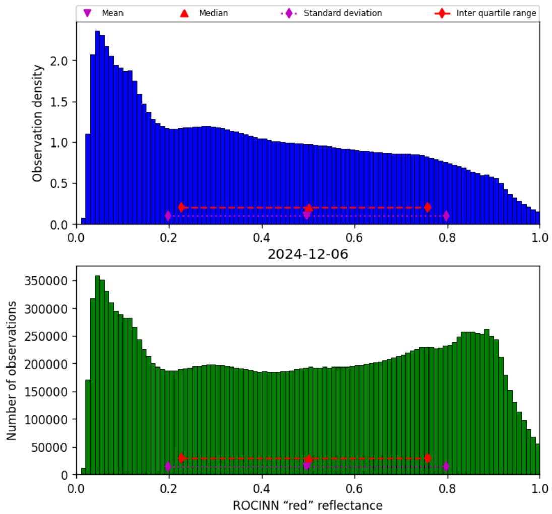
Figure 53: Histogram of “ROCINN “red” reflectance” for 2024-12-06 to 2024-12-07
