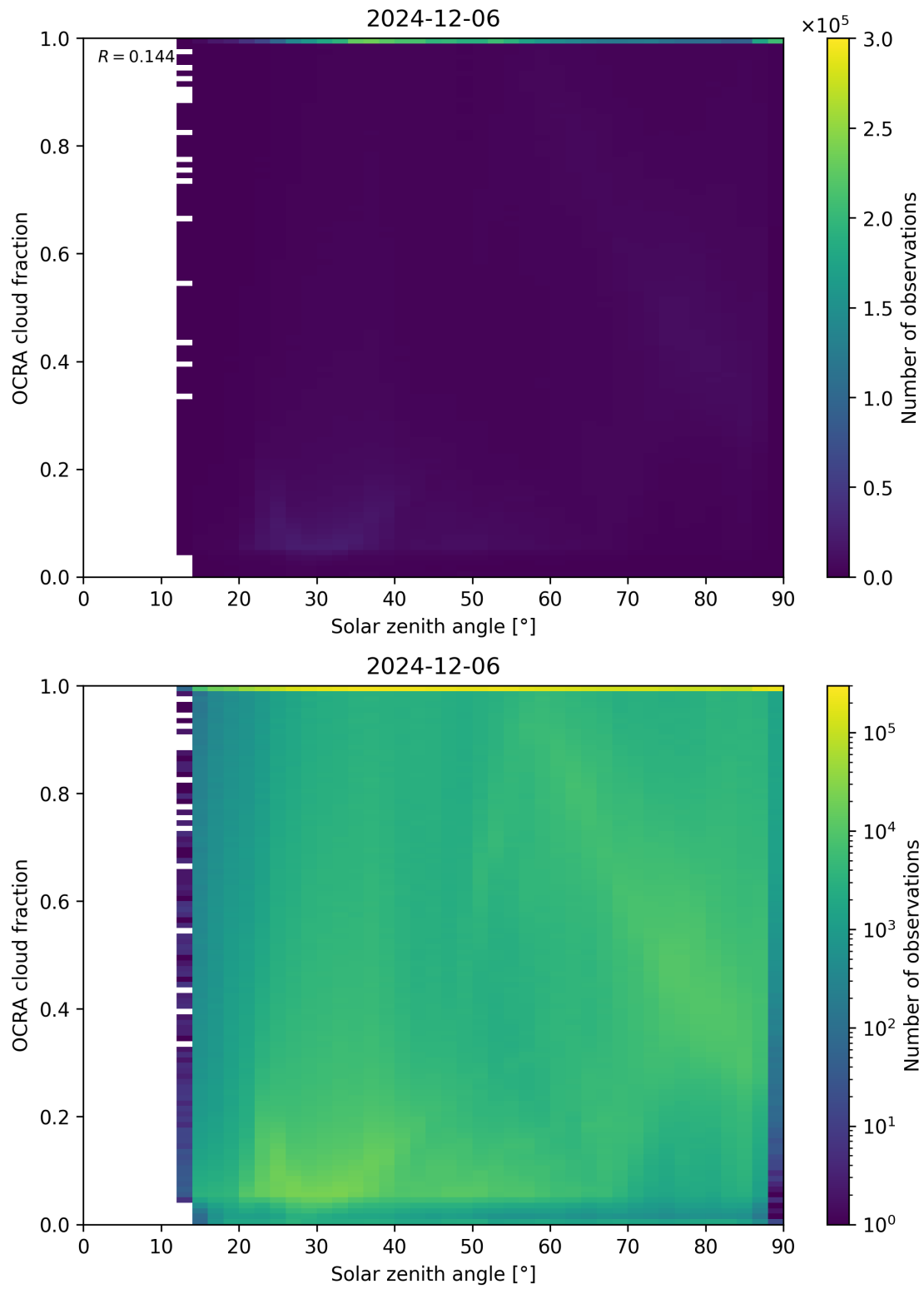
Figure 100: Scatter density plot of “Solar zenith angle” against “OCRA cloud fraction” for 2024-12-06 to 2024-12-07.
