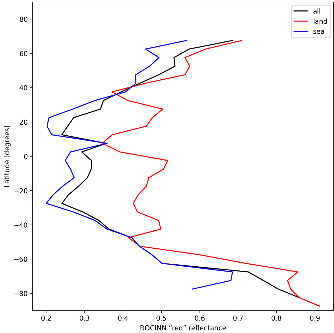
Figure 37: Zonal average of “ROCINN “red” reflectance” for 2024-12-06 to 2024-12-07.
