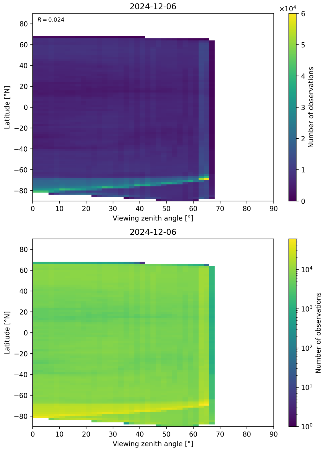
Figure 113: Scatter density plot of “Viewing zenith angle” against “Latitude” for 2024-12-06 to 2024-12-07.
