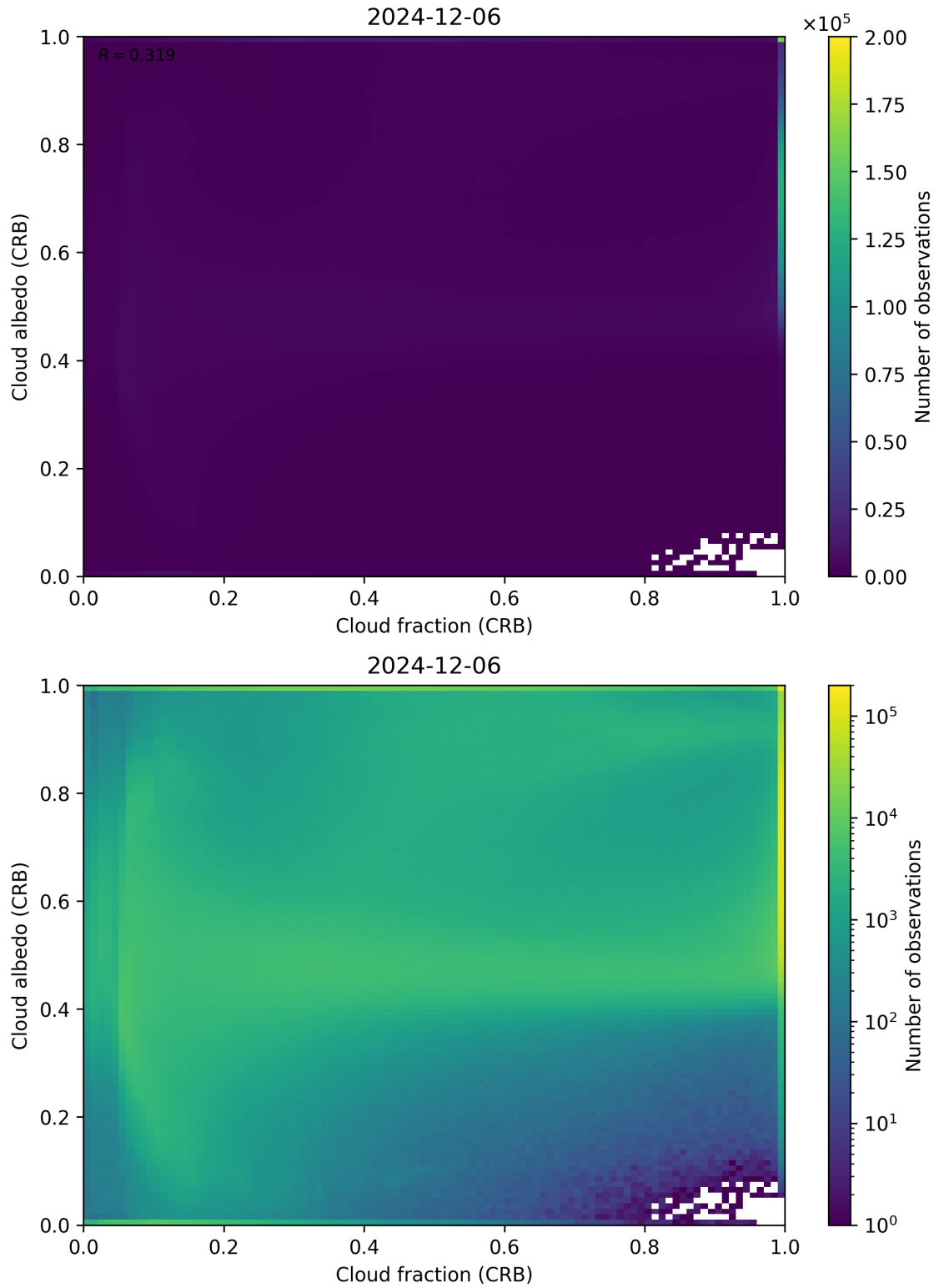
Figure 77: Scatter density plot of “Cloud fraction (CRB)” against “Cloud albedo (CRB)” for 2024-12-06 to 2024-12-07.
