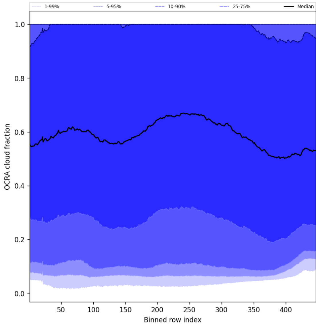
Figure 66: Along track statistics of “OCRA cloud fraction” for 2024-12-06 to 2024-12-07
