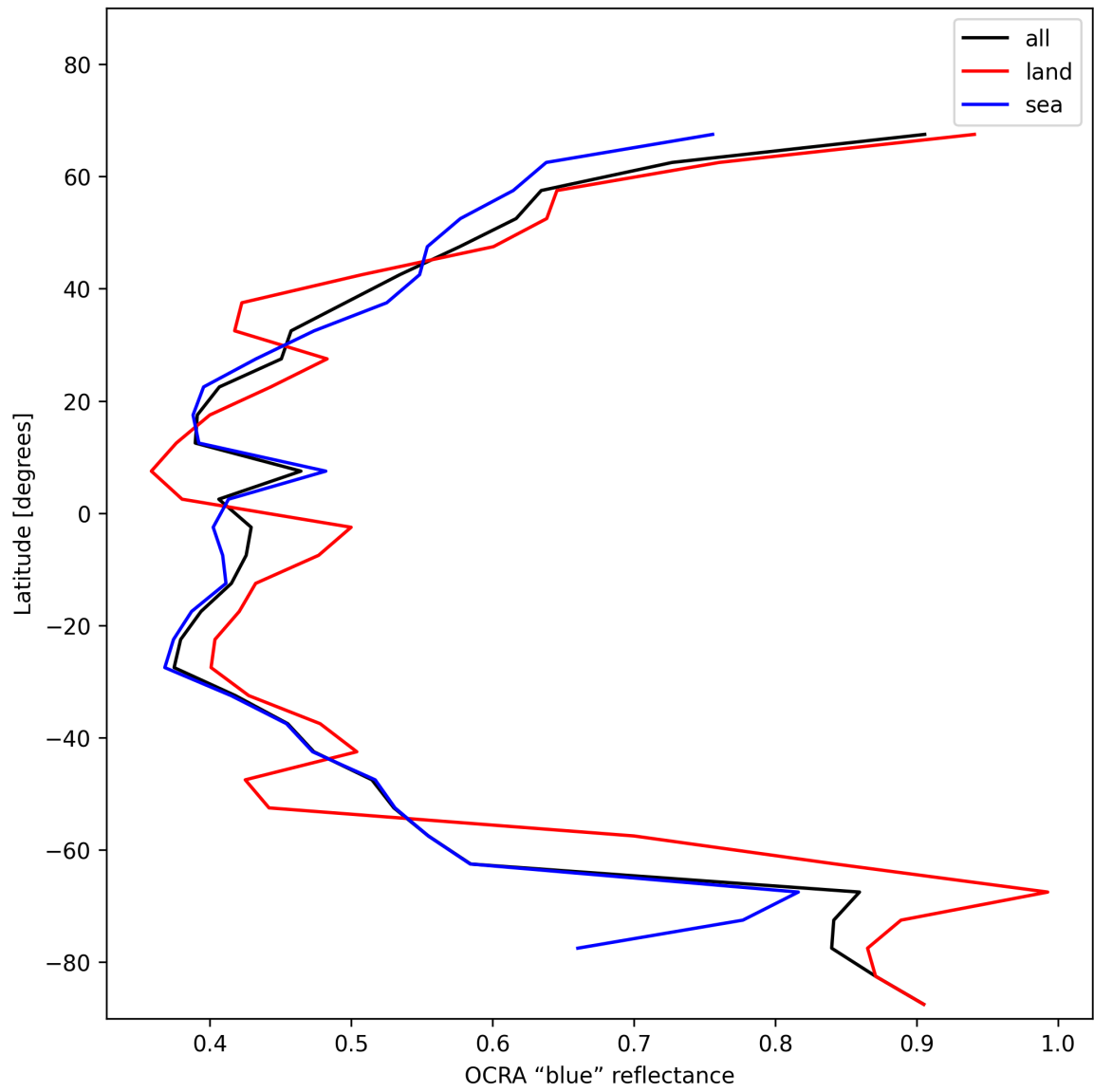
Figure 35: Zonal average of “OCRA “blue” reflectance” for 2024-12-06 to 2024-12-07.
