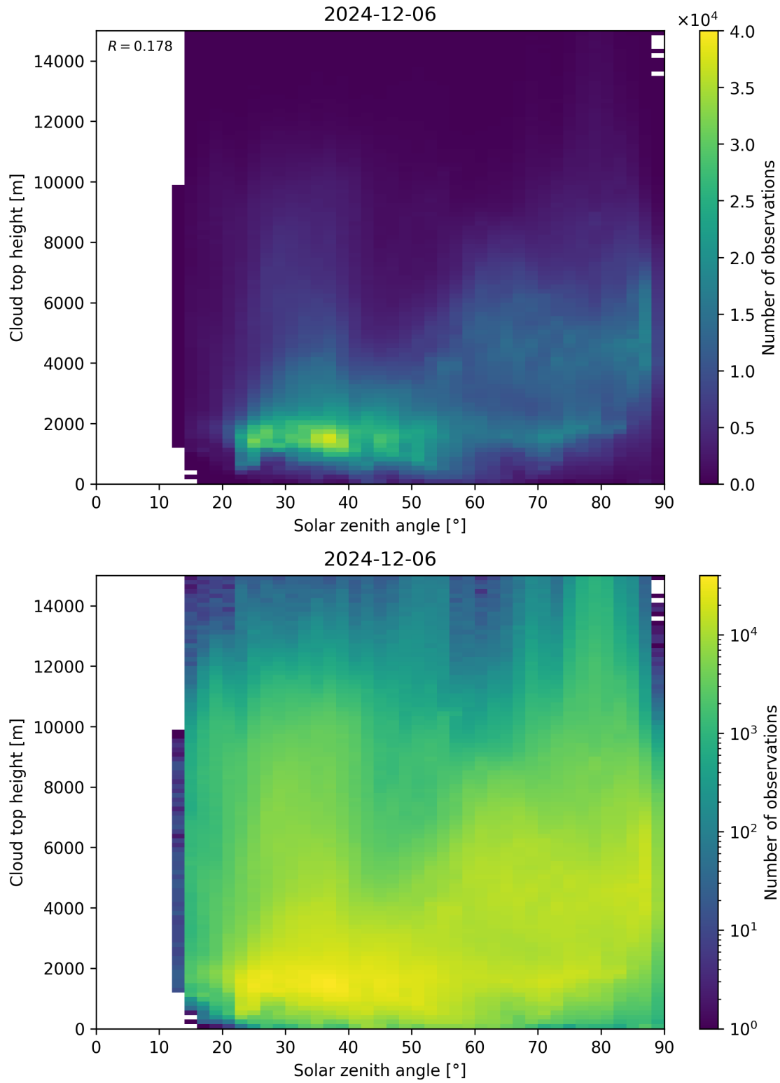
Figure 104: Scatter density plot of “Solar zenith angle” against “Cloud top height” for 2024-12-06 to 2024-12-07.
