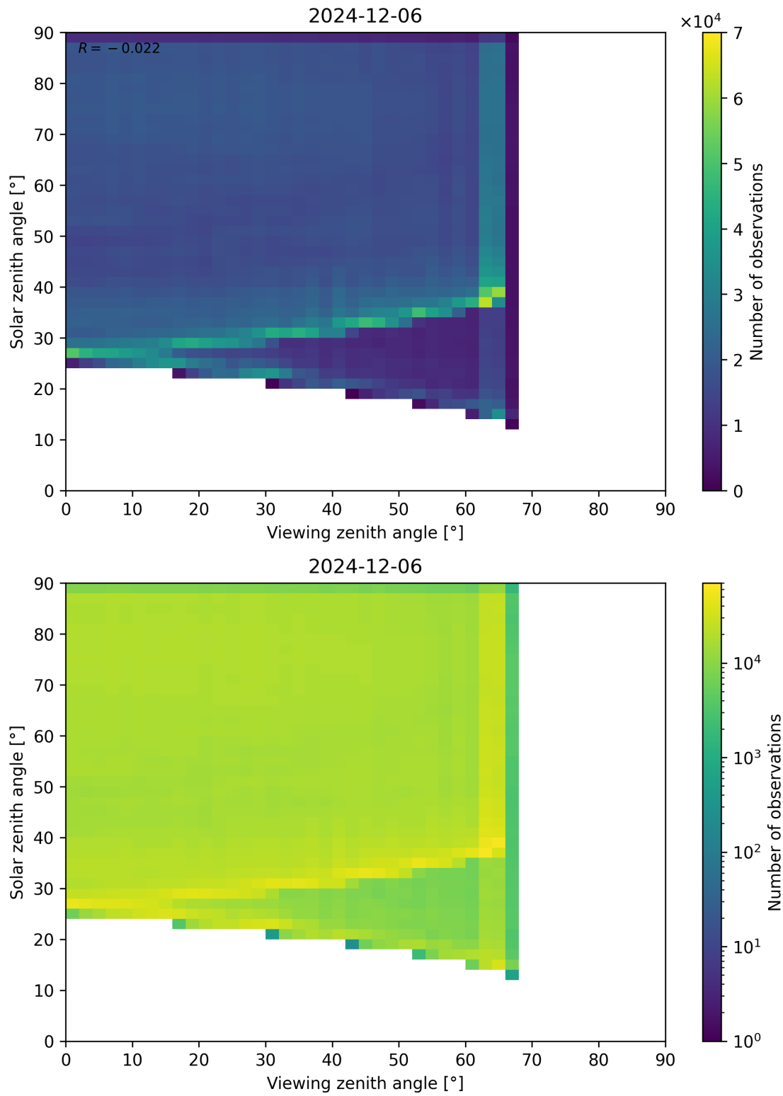
Figure 114: Scatter density plot of “Viewing zenith angle” against “Solar zenith angle” for 2024-12-06 to 2024-12-07.
