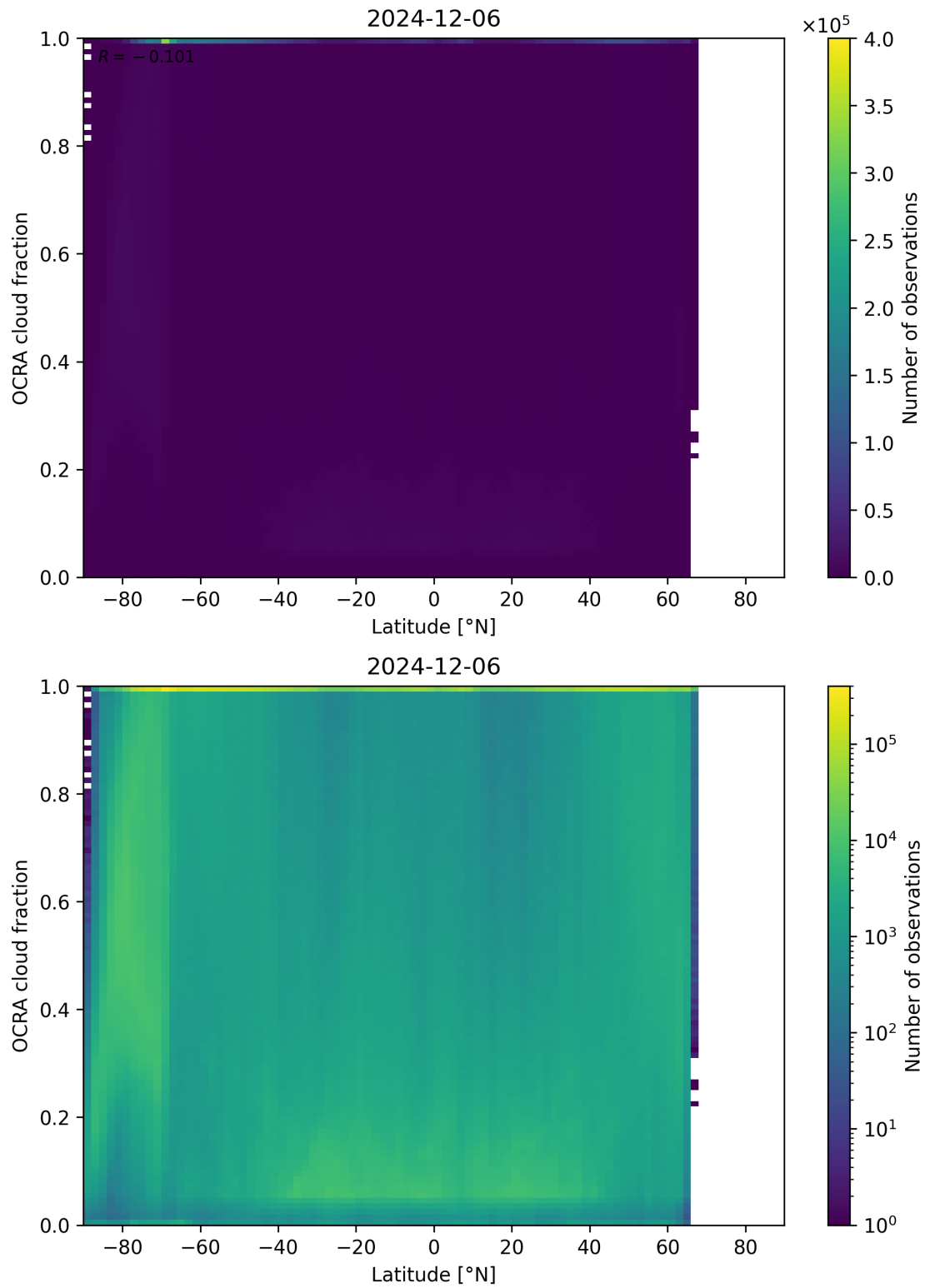
Figure 93: Scatter density plot of “Latitude” against “OCRA cloud fraction” for 2024-12-06 to 2024-12-07.
