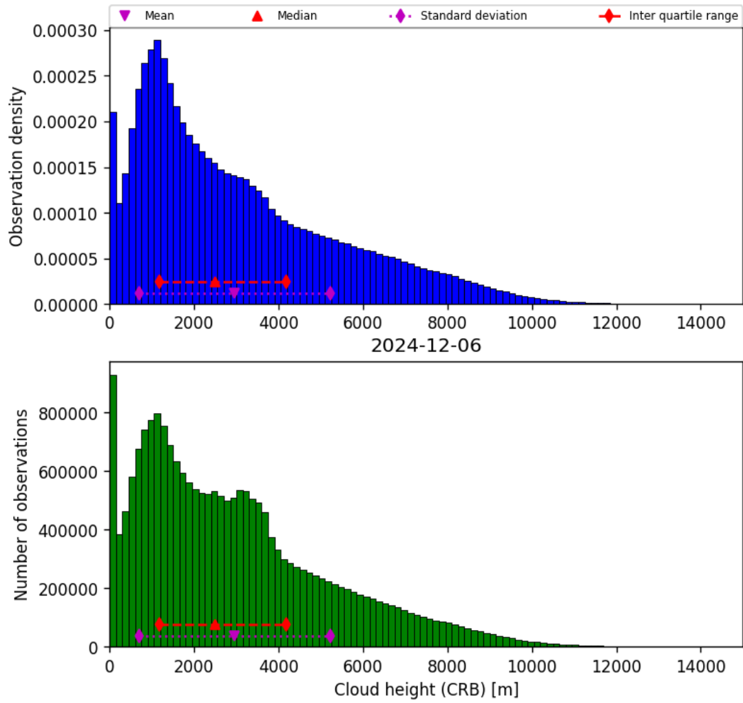
Figure 43: Histogram of “Cloud height (CRB)” for 2024-12-06 to 2024-12-07
