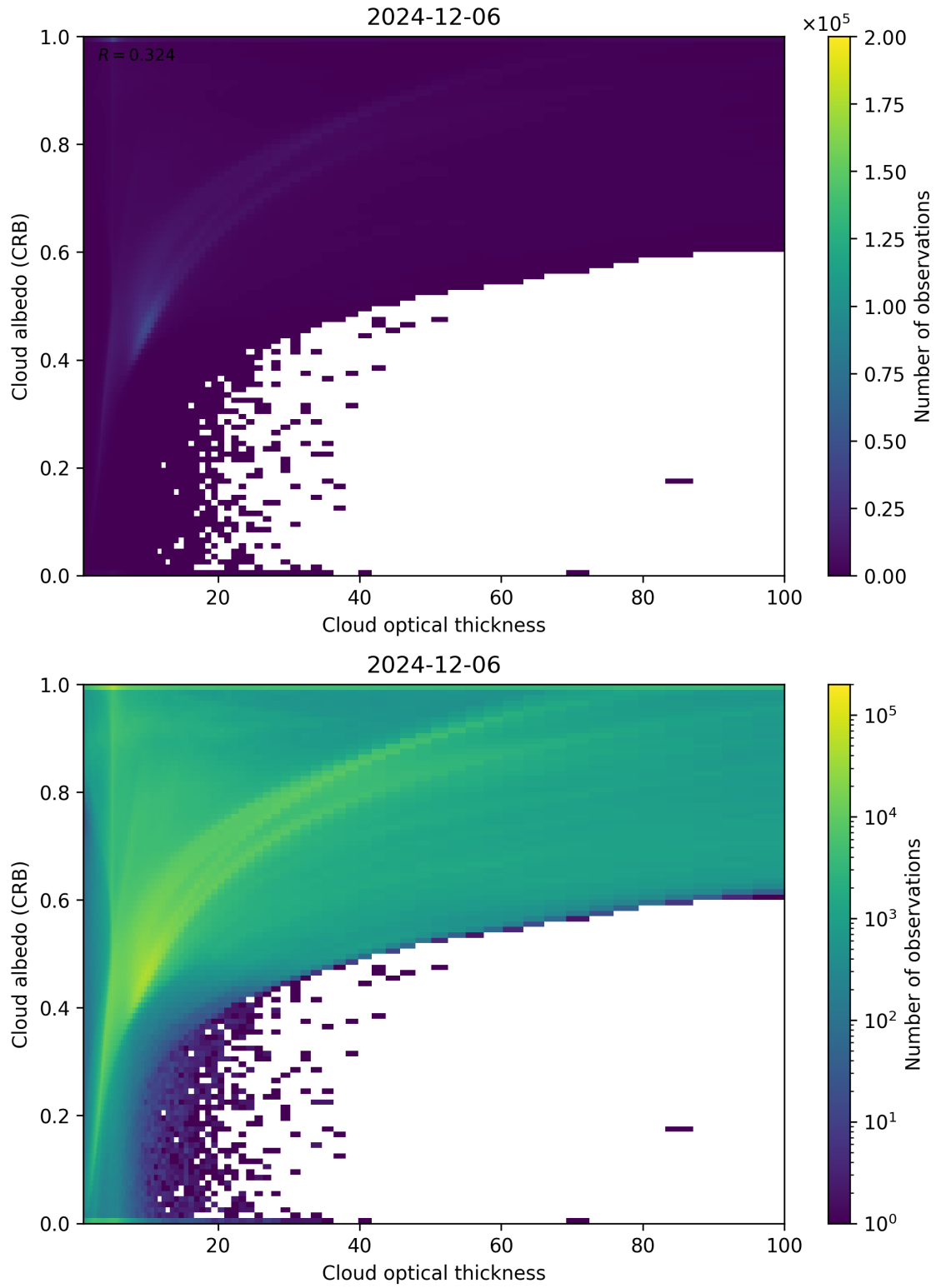
Figure 82: Scatter density plot of “Cloud optical thickness” against “Cloud albedo (CRB)” for 2024-12-06 to 2024-12-07.
