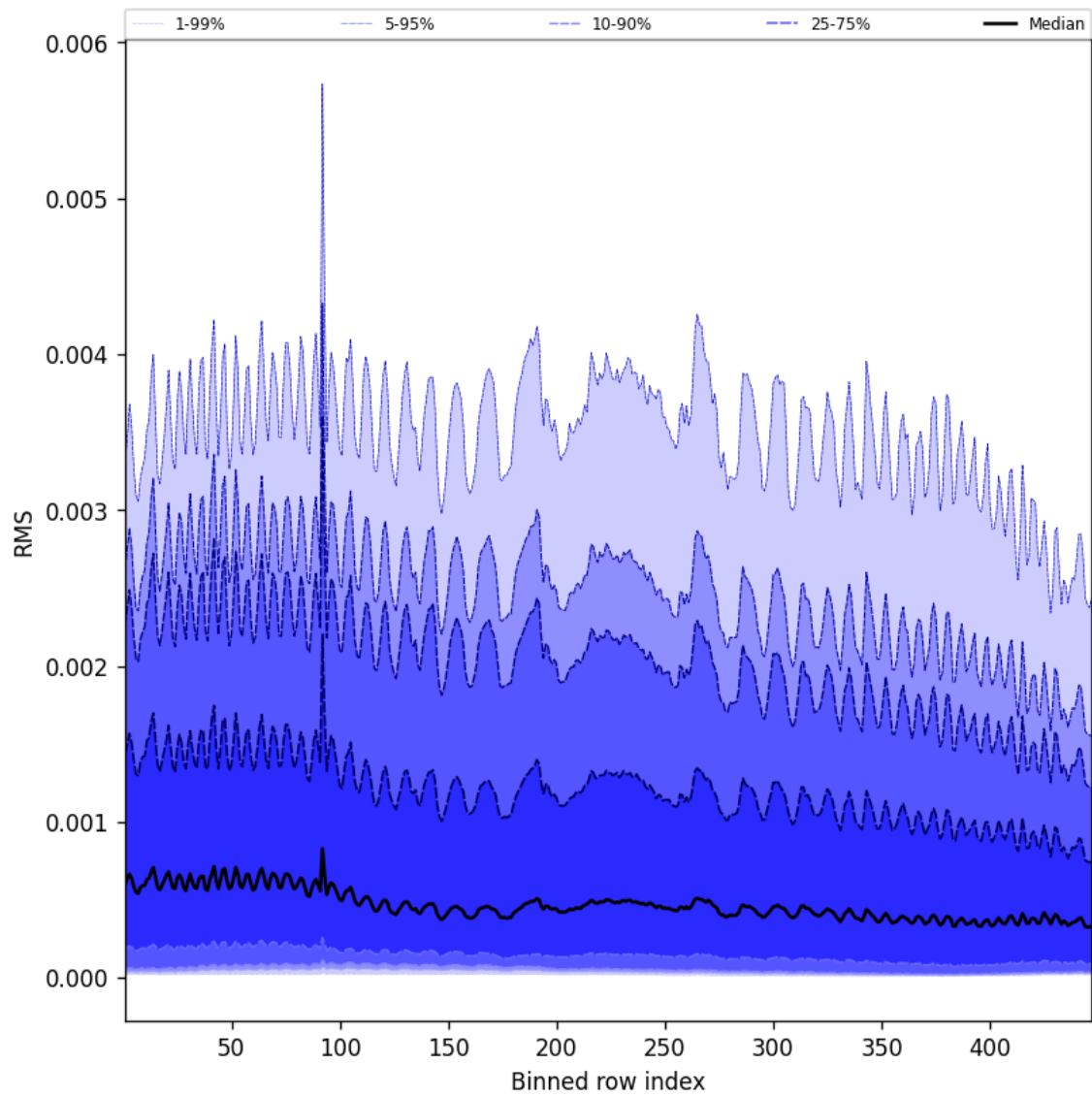
Figure 63: Along track statistics of “RMS” for 2024-12-06 to 2024-12-07
