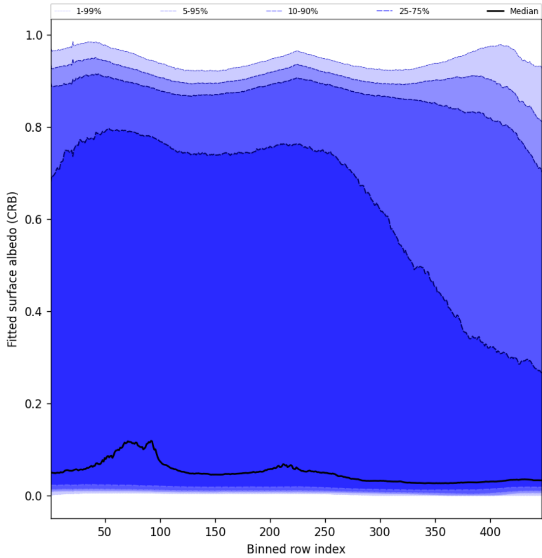
Figure 62: Along track statistics of “Fitted surface albedo (CRB)” for 2024-12-06 to 2024-12-07
