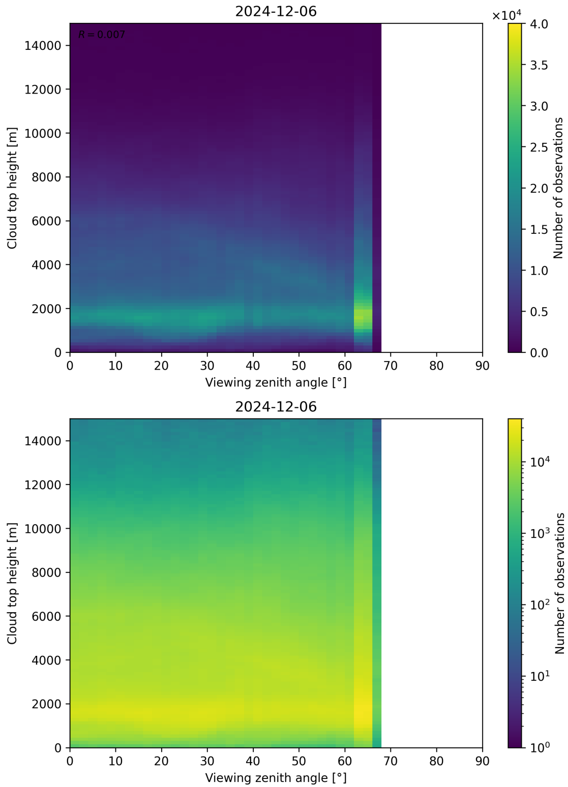
Figure 112: Scatter density plot of “Viewing zenith angle” against “Cloud top height” for 2024-12-06 to 2024-12-07.
