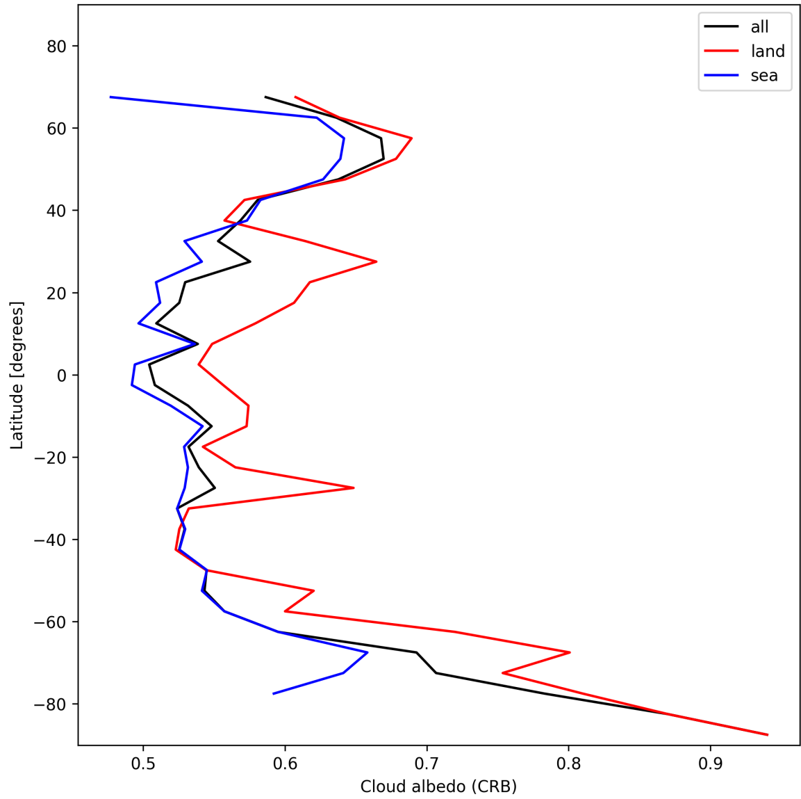
Figure 28: Zonal average of “Cloud albedo (CRB)” for 2024-12-06 to 2024-12-08.
