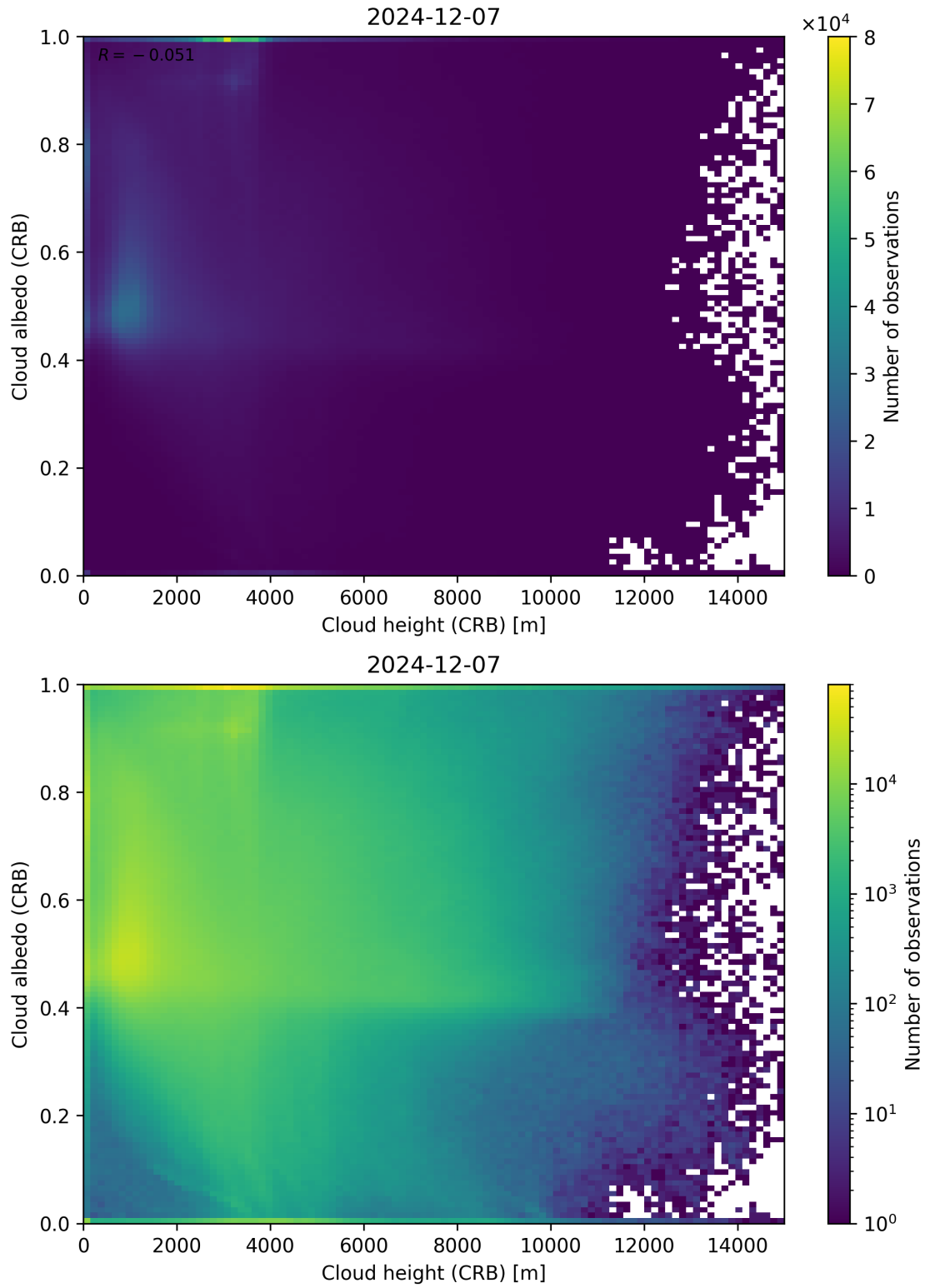
Figure 80: Scatter density plot of “Cloud height (CRB)” against “Cloud albedo (CRB)” for 2024-12-06 to 2024-12-08.
