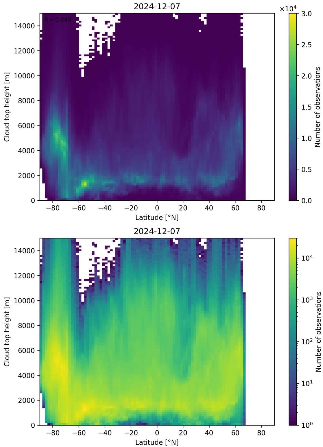
Figure 97: Scatter density plot of “Latitude” against “Cloud top height” for 2024-12-06 to 2024-12-08.
