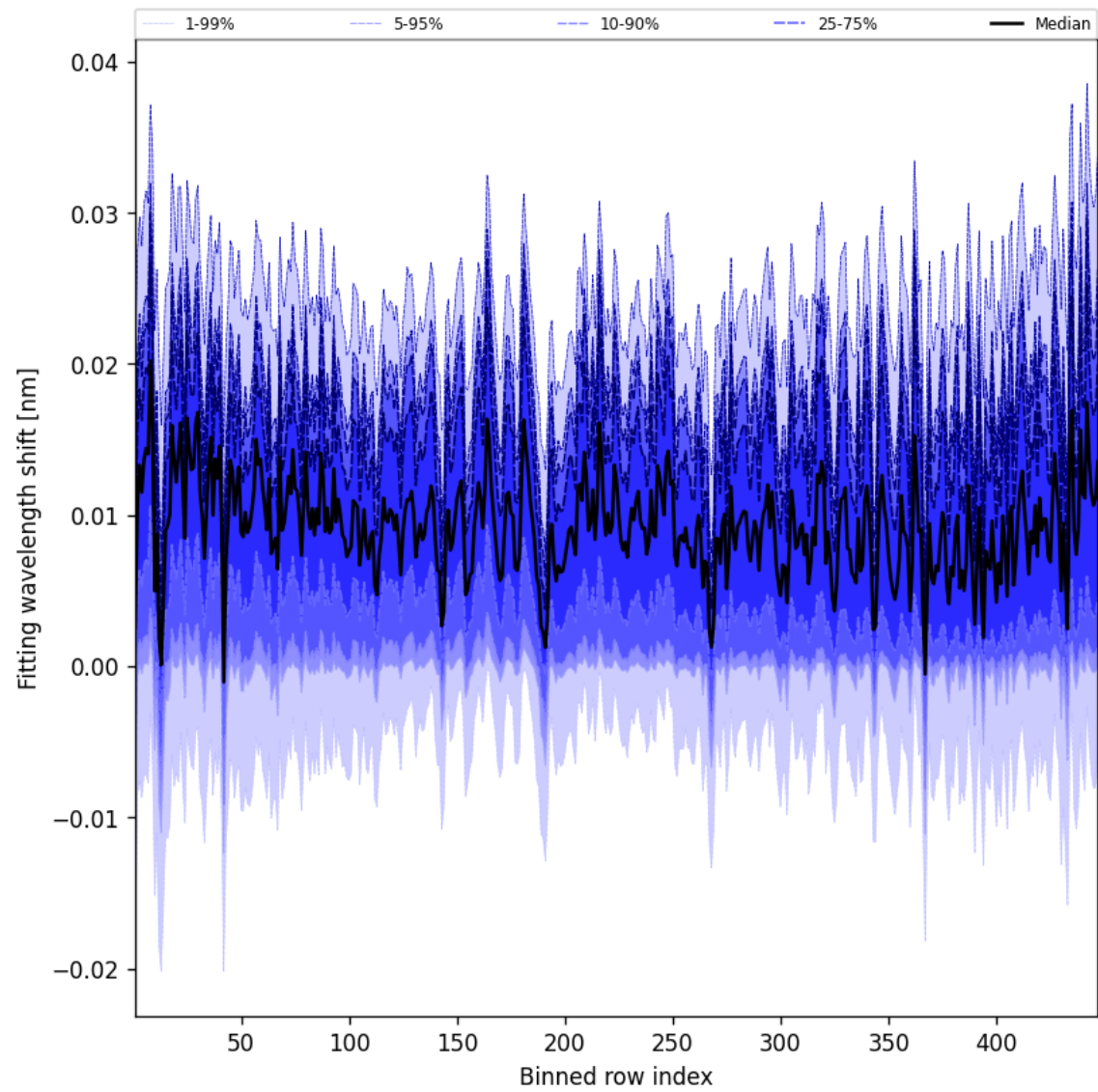
Figure 65: Along track statistics of “Fitting wavelength shift” for 2024-12-06 to 2024-12-08
