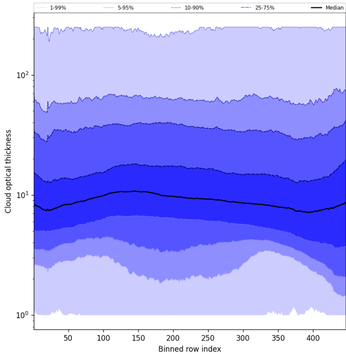
Figure 57: Along track statistics of “Cloud optical thickness” for 2024-12-06 to 2024-12-08
