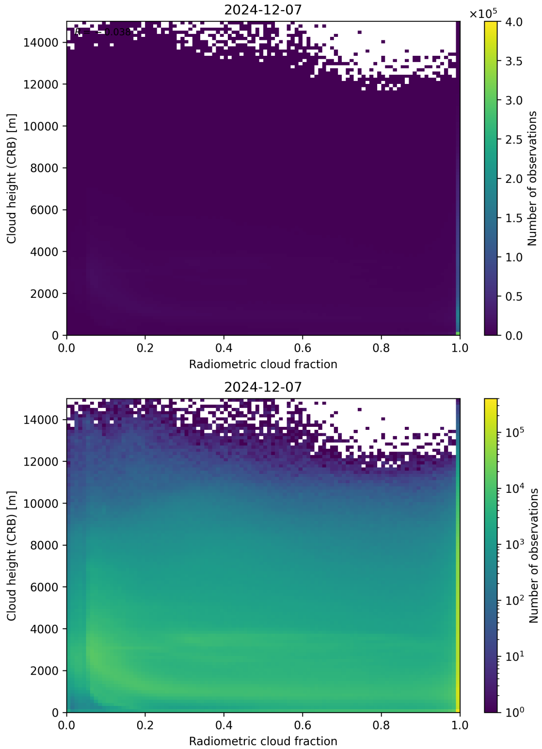
Figure 74: Scatter density plot of “Radiometric cloud fraction” against “Cloud height (CRB)” for 2024-12-06 to 2024-12-08.
