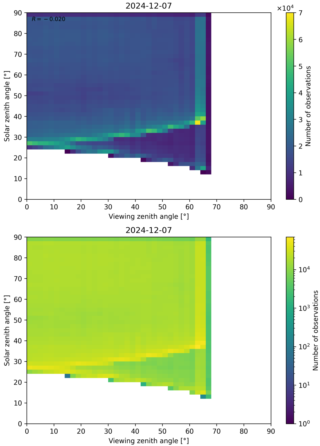
Figure 114: Scatter density plot of “Viewing zenith angle” against “Solar zenith angle” for 2024-12-06 to 2024-12-08.
