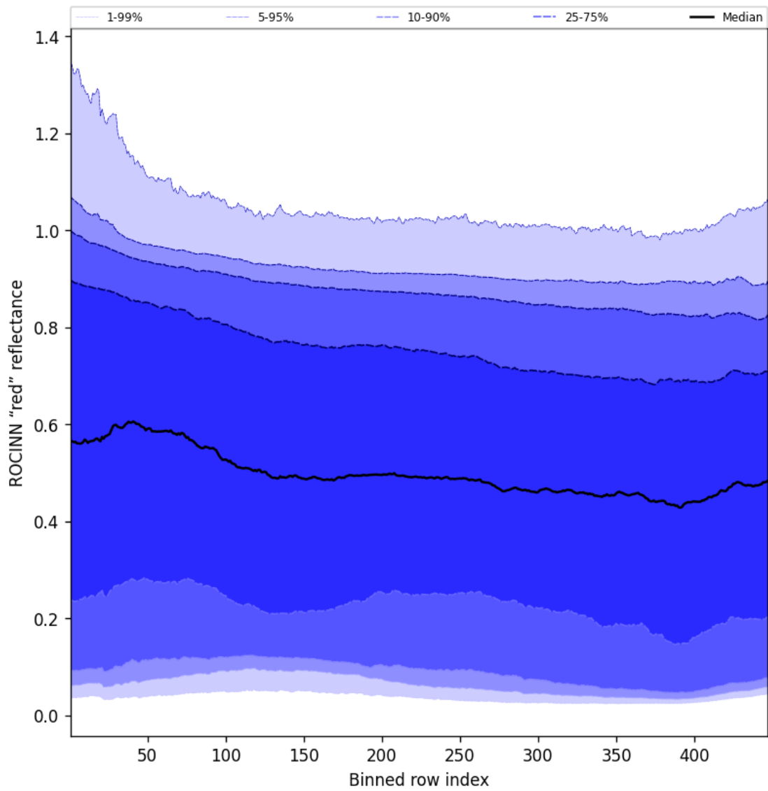
Figure 69: Along track statistics of “ROCINN “red” reflectance” for 2024-12-06 to 2024-12-08
