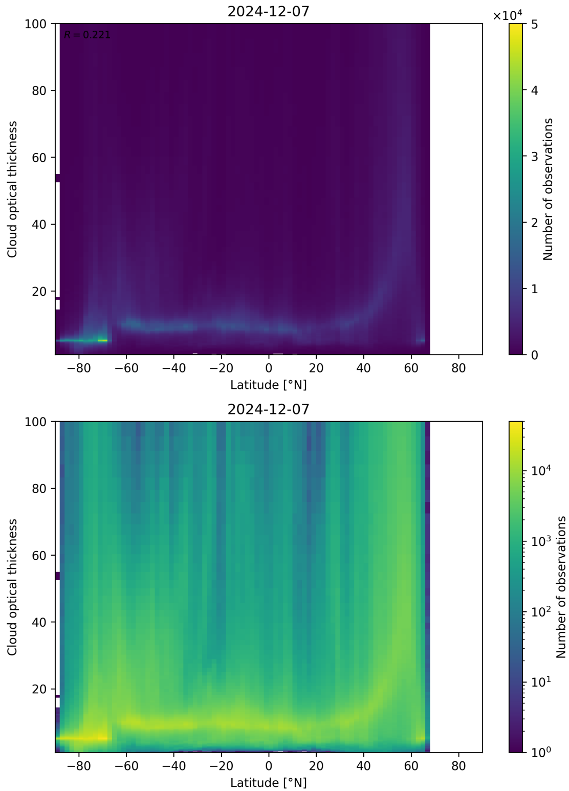
Figure 96: Scatter density plot of “Latitude” against “Cloud optical thickness” for 2024-12-06 to 2024-12-08.
