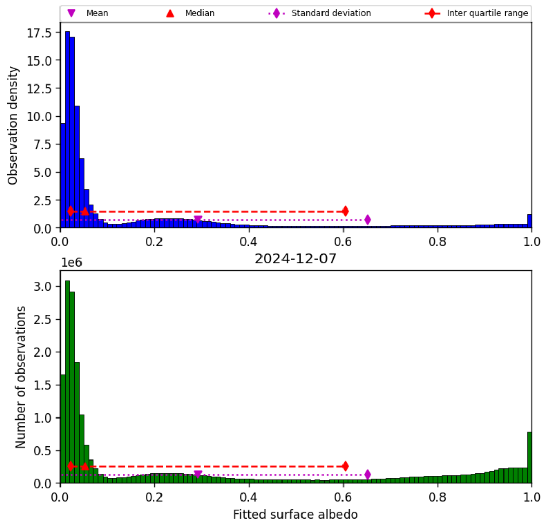
Figure 45: Histogram of “Fitted surface albedo” for 2024-12-06 to 2024-12-08
