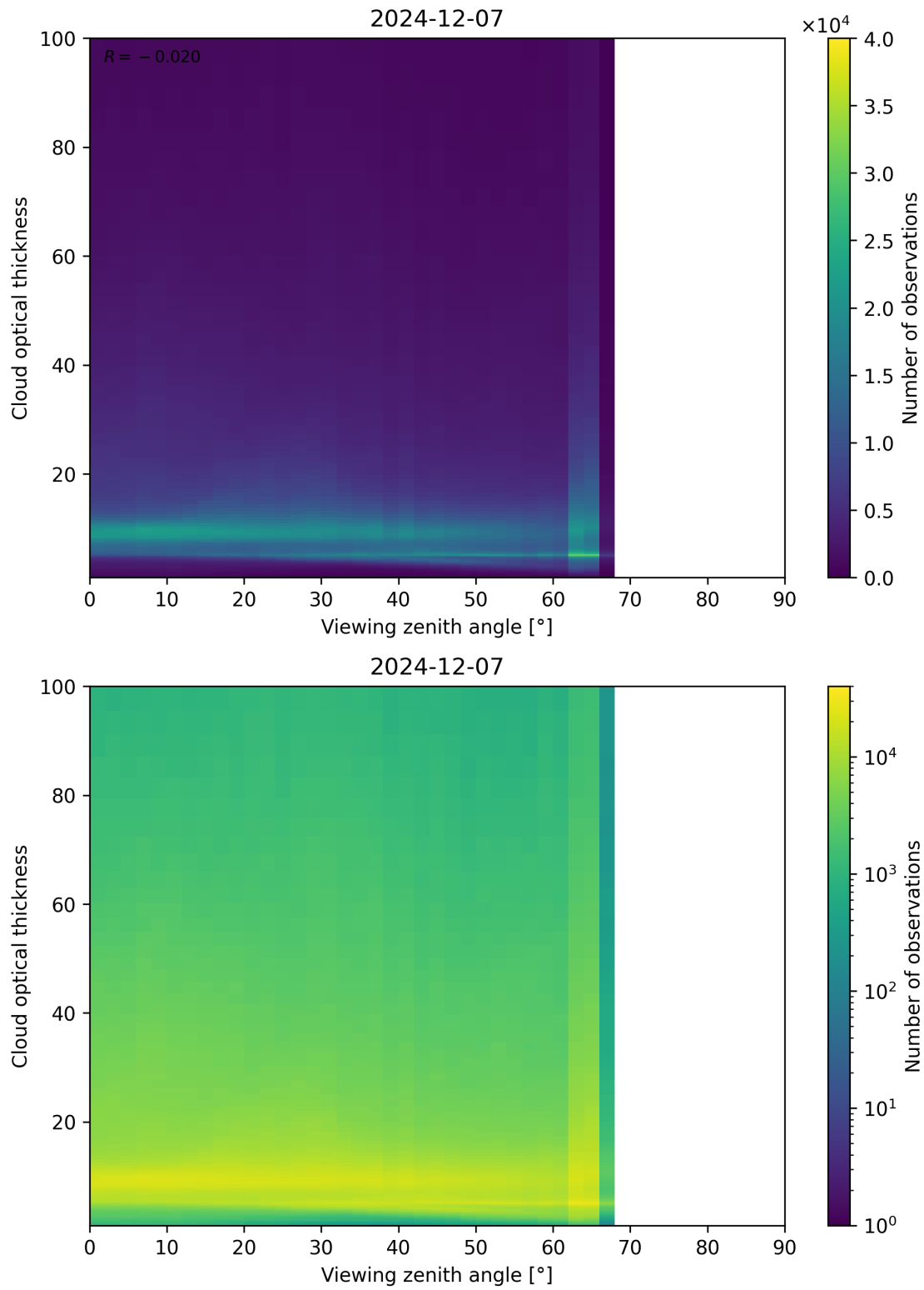
Figure 111: Scatter density plot of “Viewing zenith angle” against “Cloud optical thickness” for 2024-12-06 to 2024-12-08.
