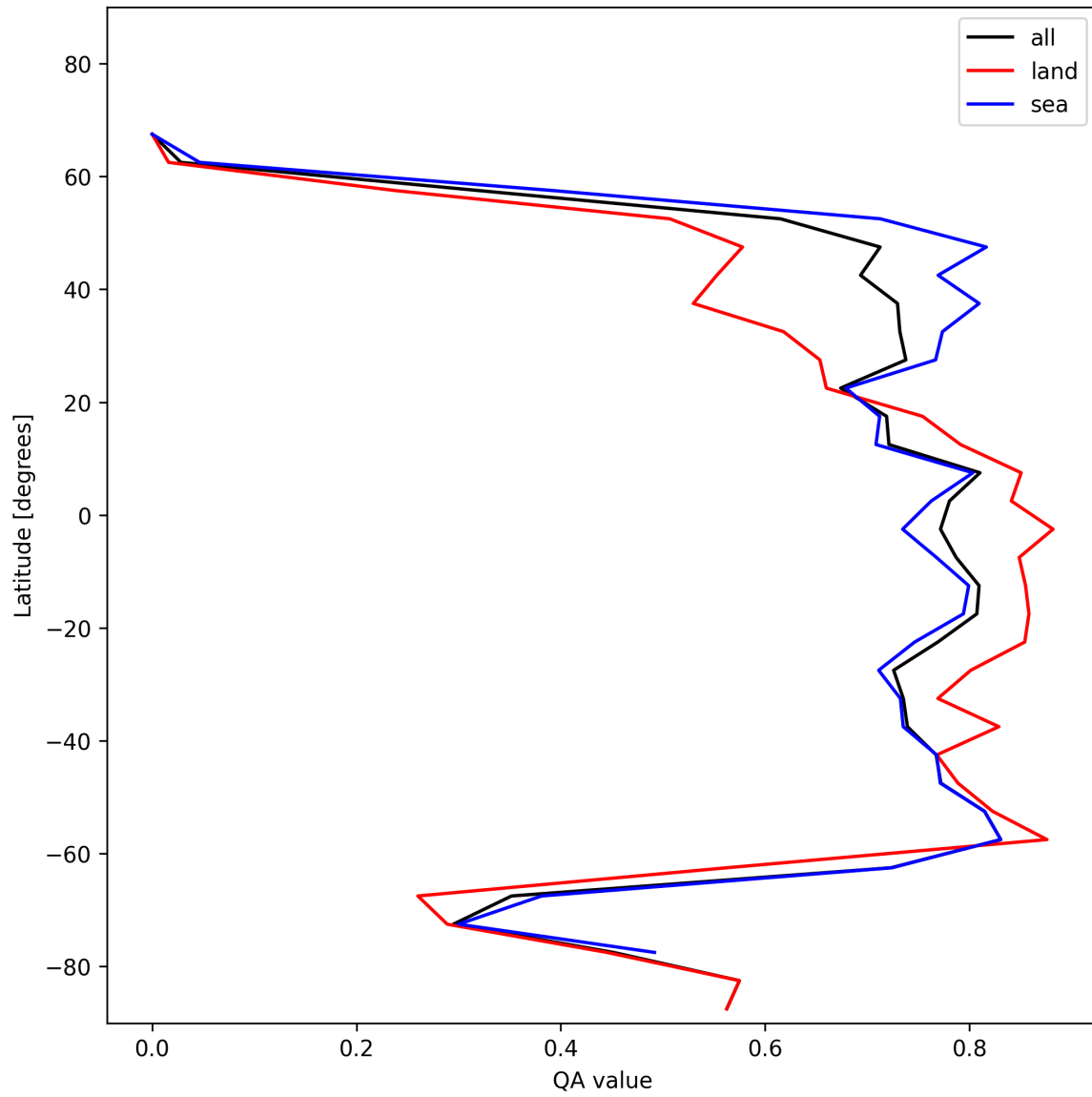
Figure 22: Zonal average of “QA value” for 2024-12-06 to 2024-12-08.
