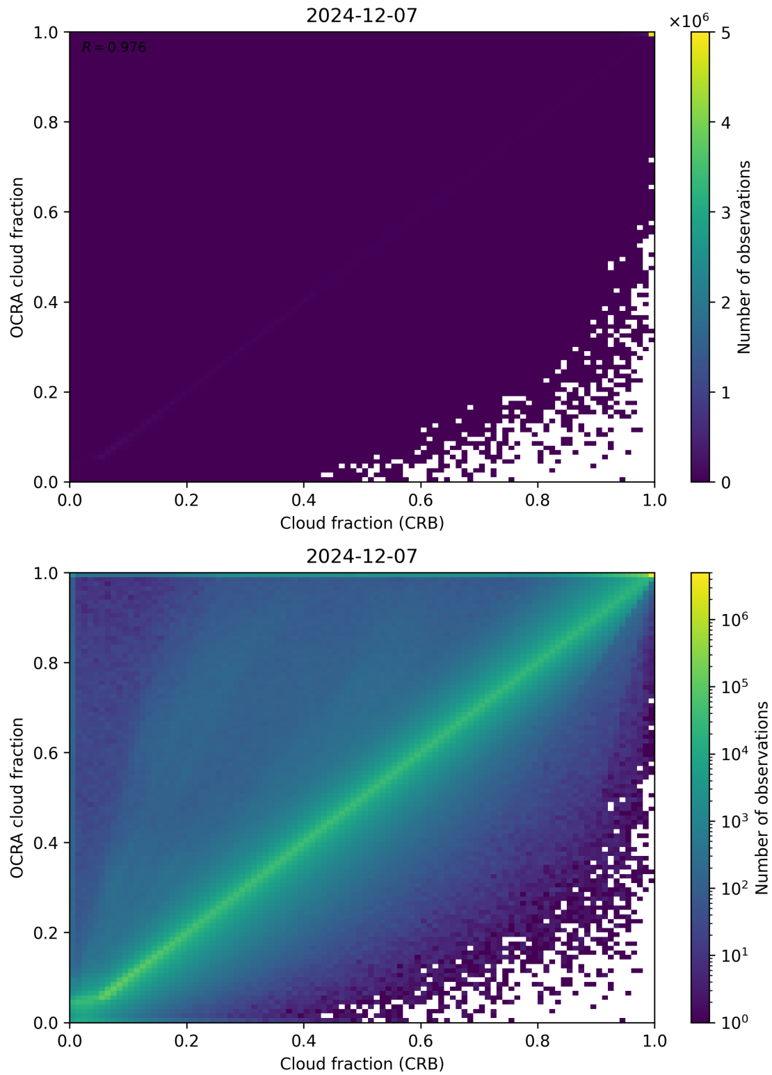
Figure 78: Scatter density plot of “Cloud fraction (CRB)” against “OCRA cloud fraction” for 2024-12-06 to 2024-12-08.
