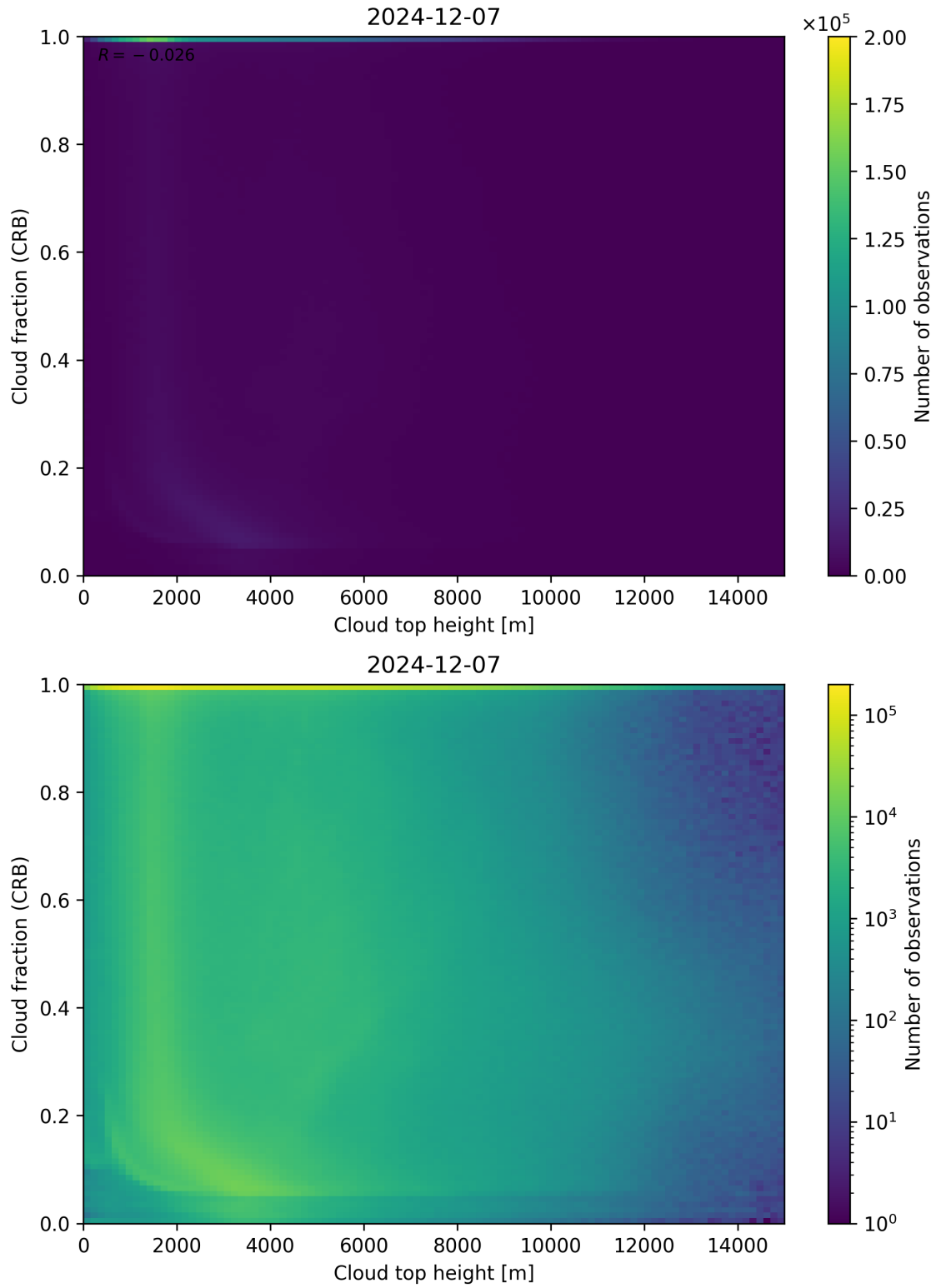
Figure 88: Scatter density plot of “Cloud top height” against “Cloud fraction (CRB)” for 2024-12-06 to 2024-12-08.
