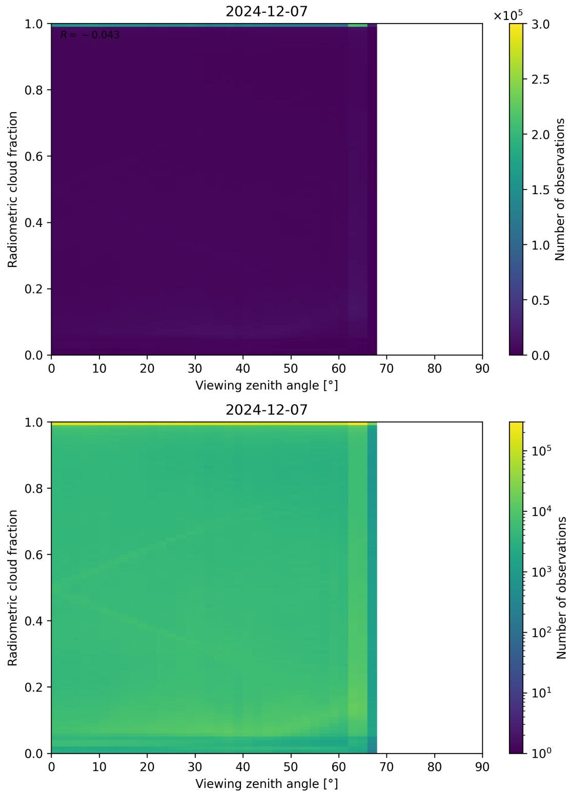
Figure 107: Scatter density plot of “Viewing zenith angle” against “Radiometric cloud fraction” for 2024-12-06 to 2024-12-08.
