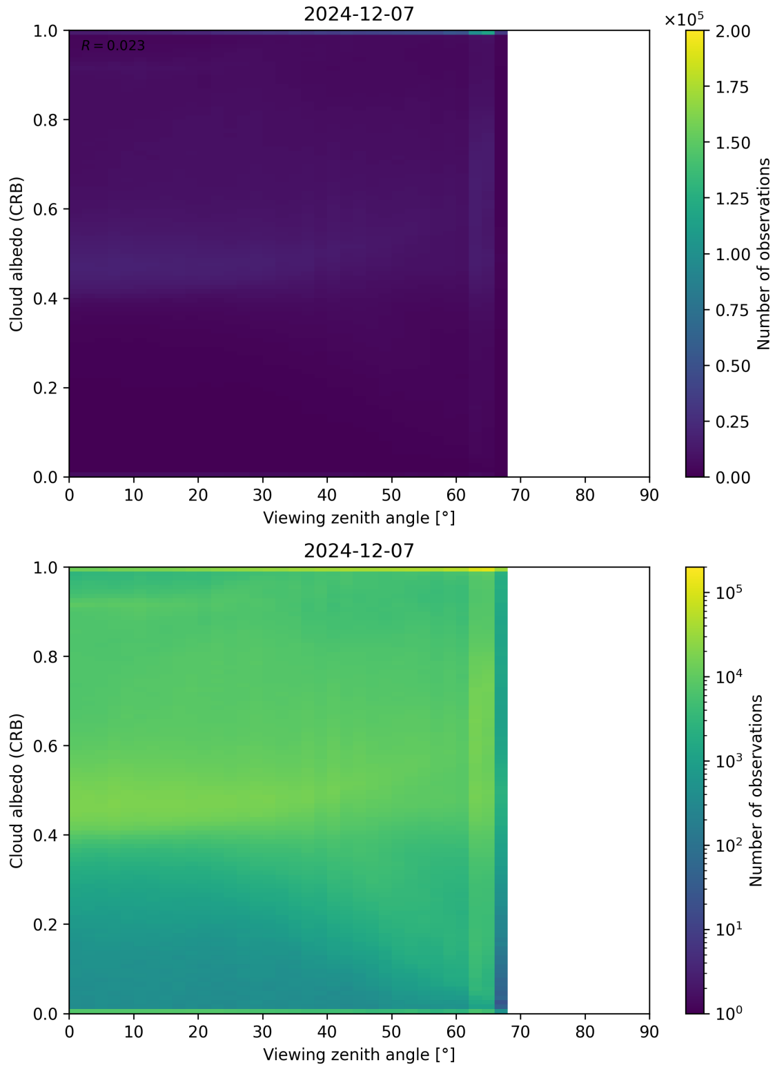
Figure 106: Scatter density plot of “Viewing zenith angle” against “Cloud albedo (CRB)” for 2024-12-06 to 2024-12-08.
