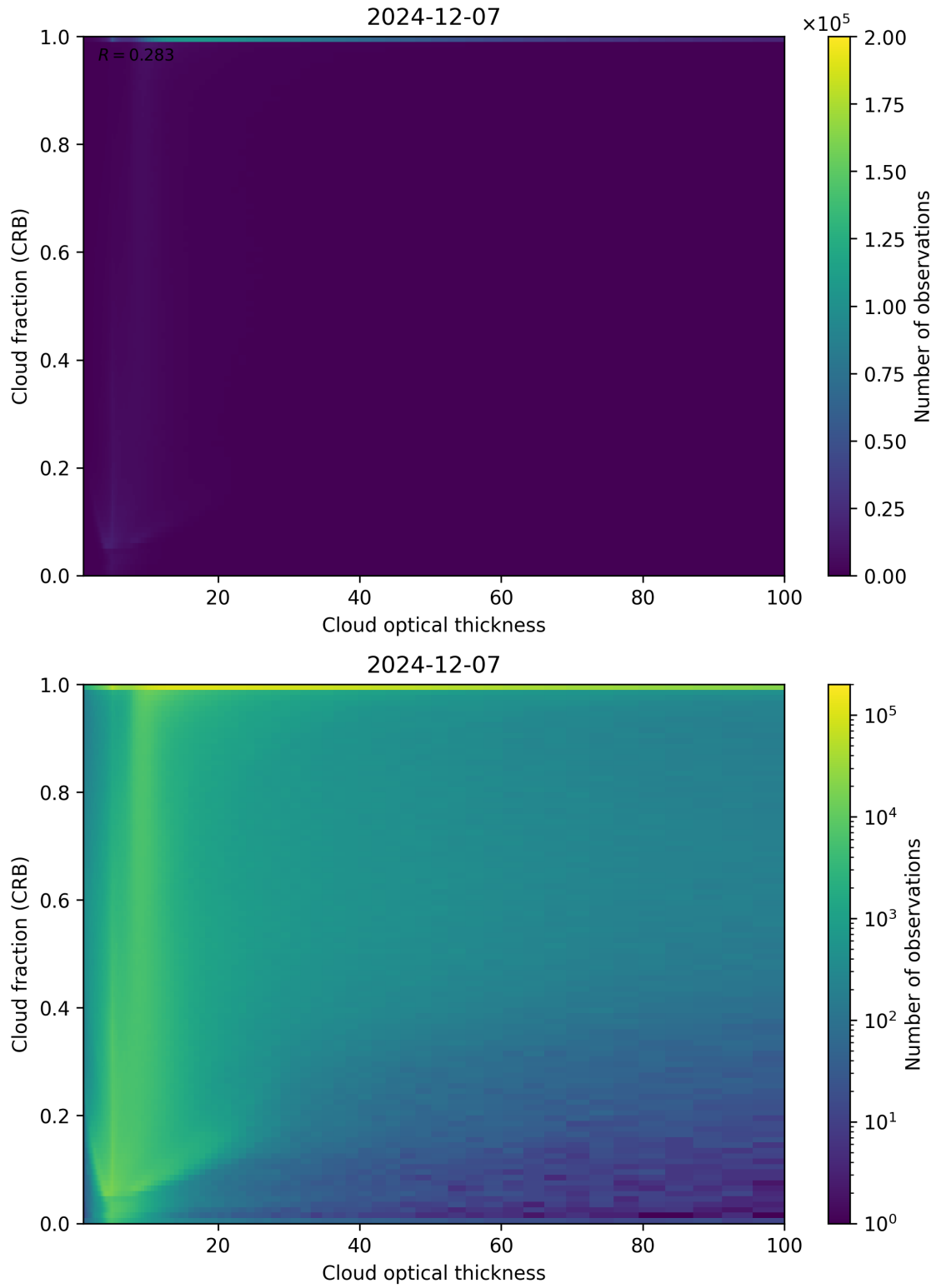
Figure 84: Scatter density plot of “Cloud optical thickness” against “Cloud fraction (CRB)” for 2024-12-06 to 2024-12-08.
