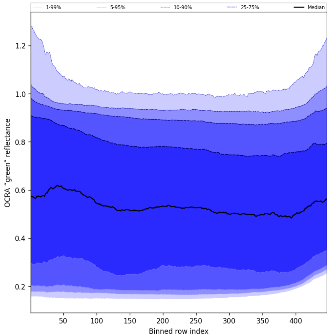
Figure 68: Along track statistics of "OCRA "green" reflectance" for 2024-12-06 to 2024-12-08
