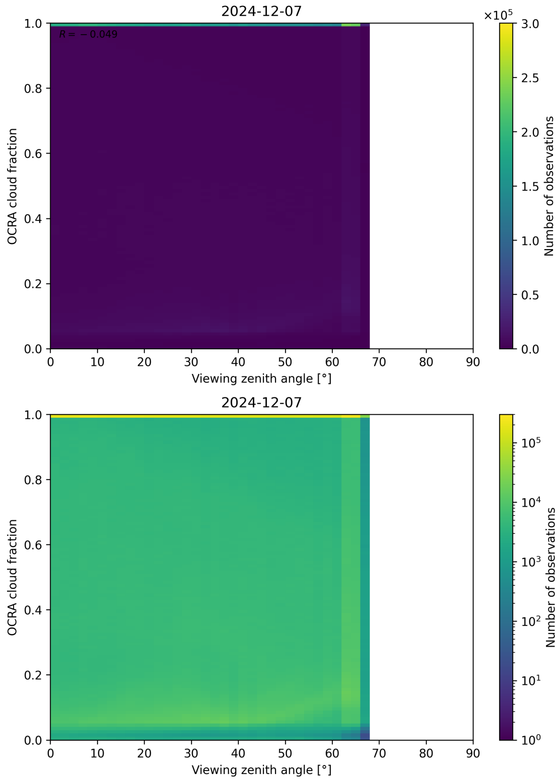
Figure 108: Scatter density plot of “Viewing zenith angle” against “OCRA cloud fraction” for 2024-12-06 to 2024-12-08.
