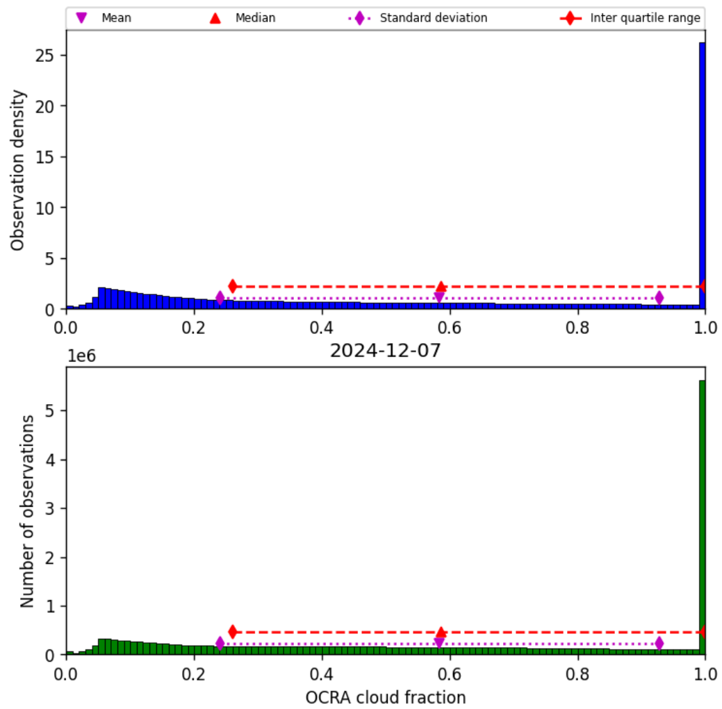
Figure 50: Histogram of “OCRA cloud fraction” for 2024-12-06 to 2024-12-08
