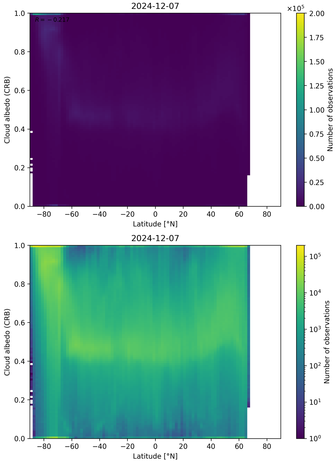
Figure 91: Scatter density plot of “Latitude” against “Cloud albedo (CRB)” for 2024-12-06 to 2024-12-08.
