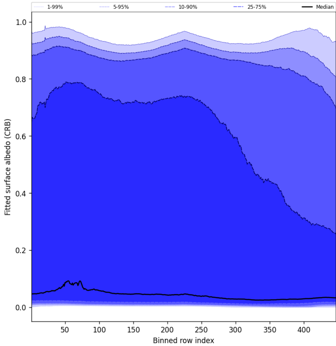
Figure 62: Along track statistics of “Fitted surface albedo (CRB)” for 2024-12-06 to 2024-12-08
