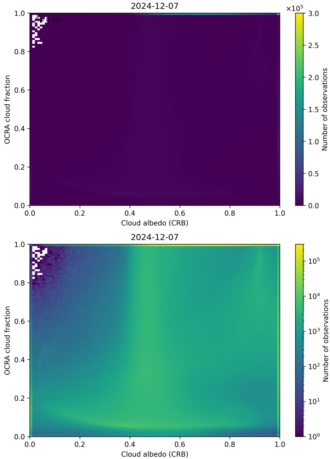
Figure 70: Scatter density plot of “Cloud albedo (CRB)” against “OCRA cloud fraction” for 2024-12-06 to 2024-12-08.
