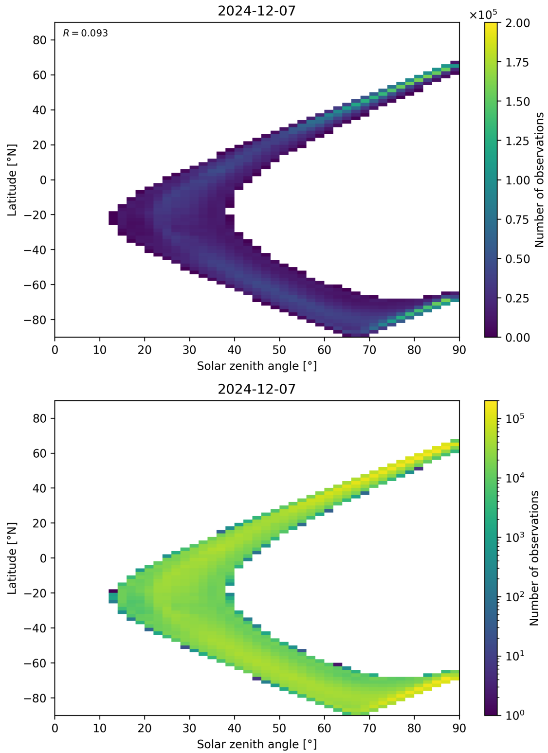
Figure 105: Scatter density plot of “Solar zenith angle” against “Latitude” for 2024-12-06 to 2024-12-08.
