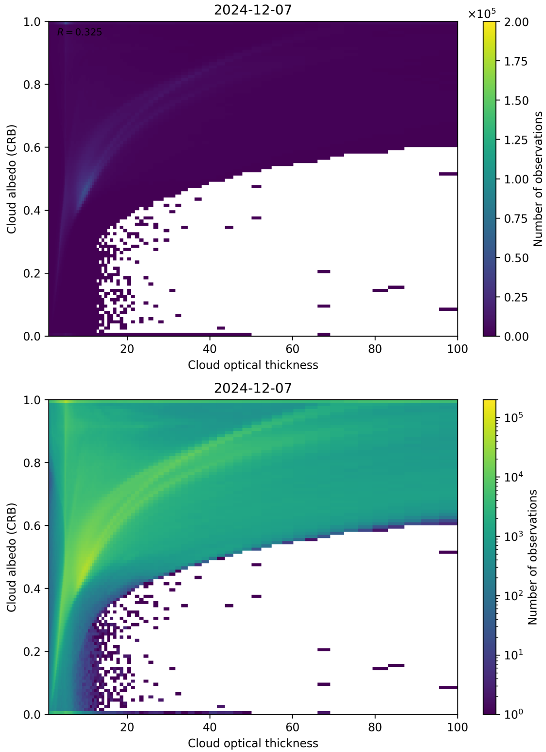
Figure 82: Scatter density plot of “Cloud optical thickness” against “Cloud albedo (CRB)” for 2024-12-06 to 2024-12-08.
