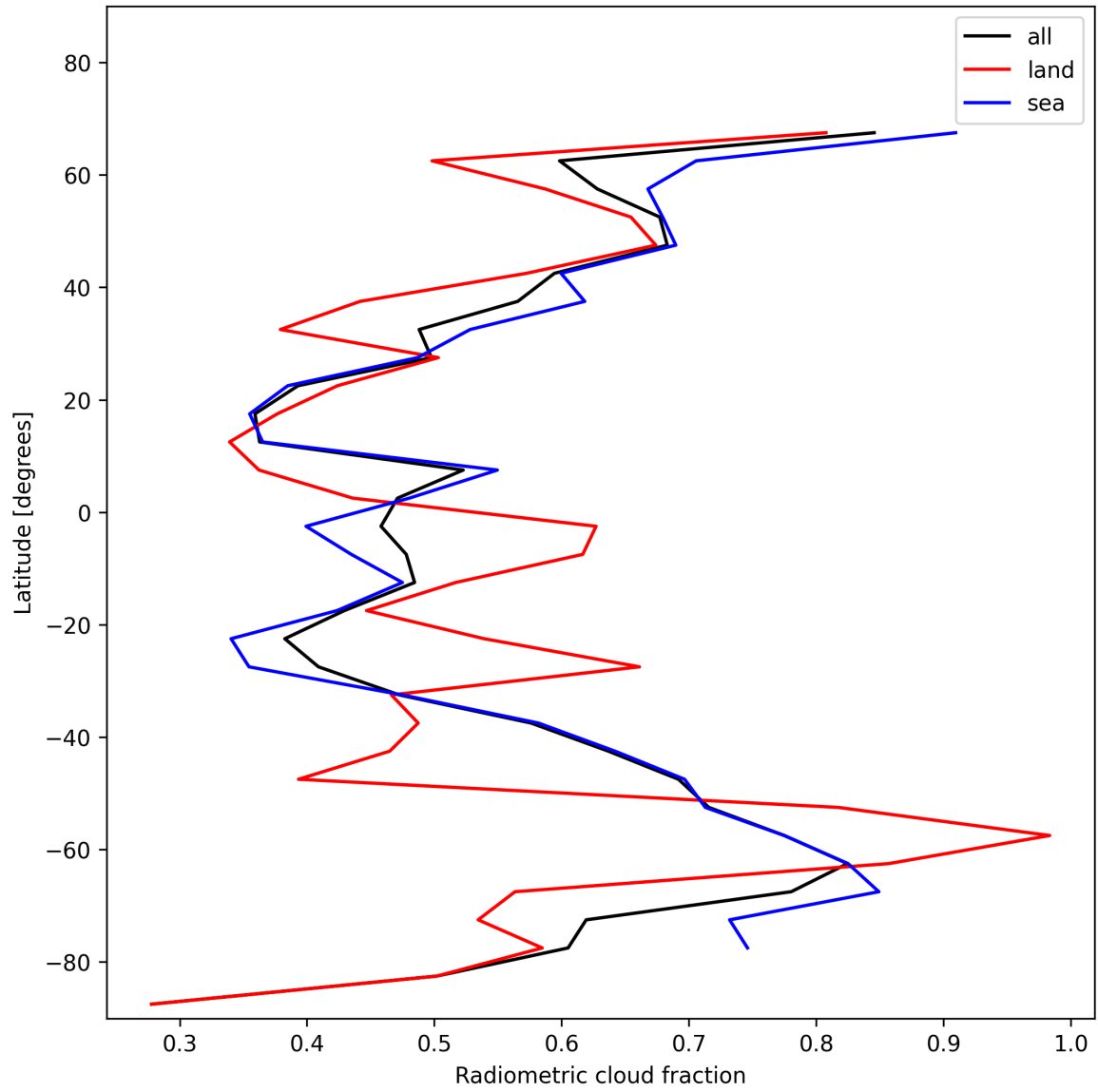
Figure 23: Zonal average of “Radiometric cloud fraction” for 2024-12-06 to 2024-12-08.
