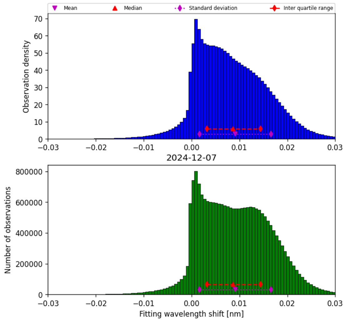
Figure 49: Histogram of “Fitting wavelength shift” for 2024-12-06 to 2024-12-08
