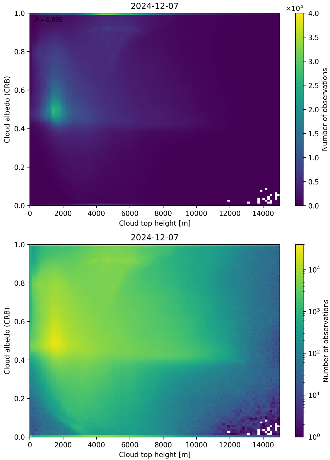
Figure 86: Scatter density plot of “Cloud top height” against “Cloud albedo (CRB)” for 2024-12-06 to 2024-12-08.
