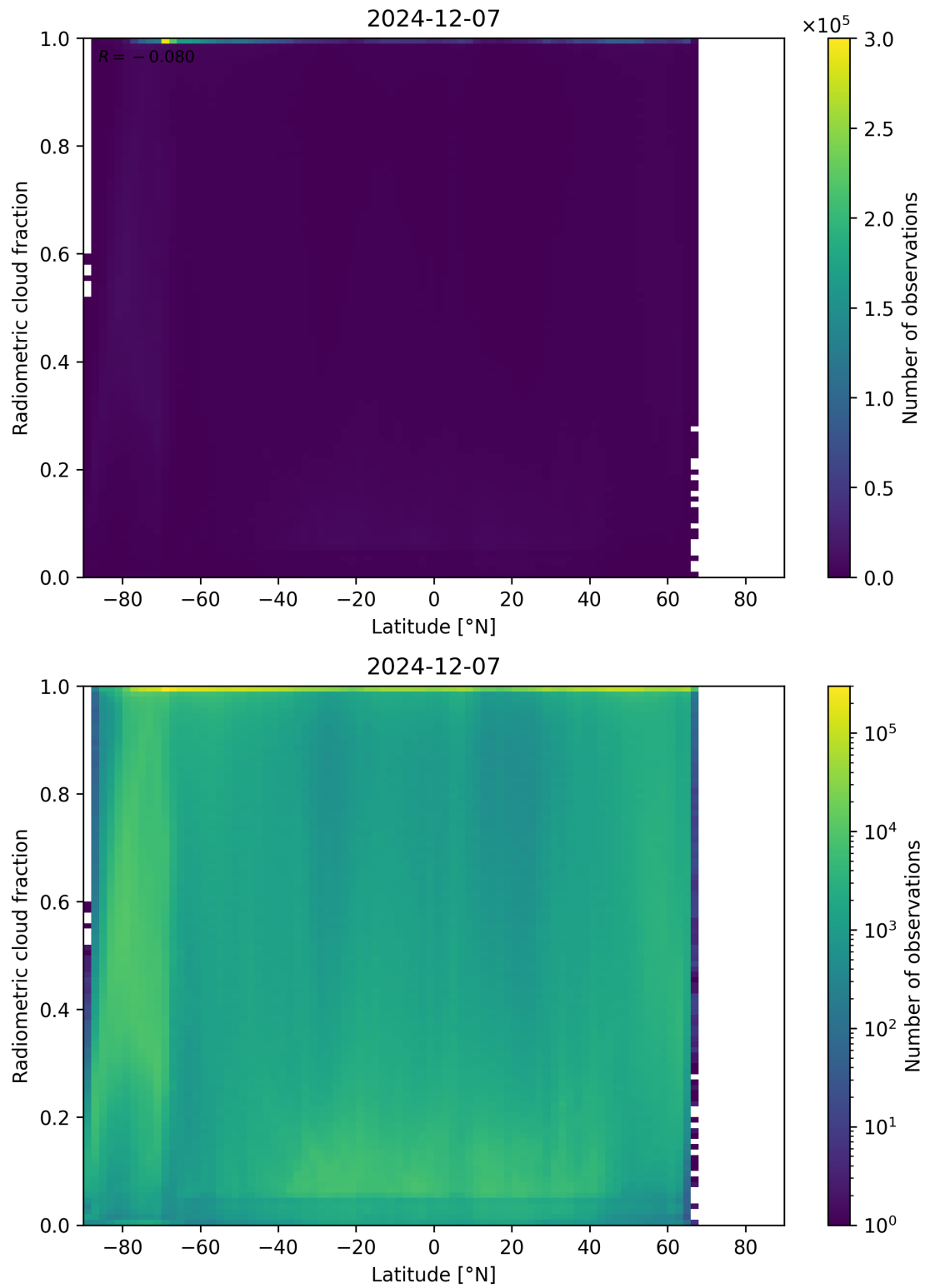
Figure 92: Scatter density plot of “Latitude” against “Radiometric cloud fraction” for 2024-12-06 to 2024-12-08.
