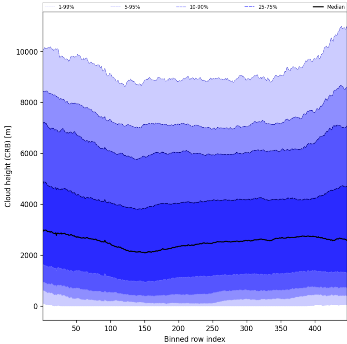
Figure 59: Along track statistics of “Cloud height (CRB)” for 2024-12-06 to 2024-12-08
