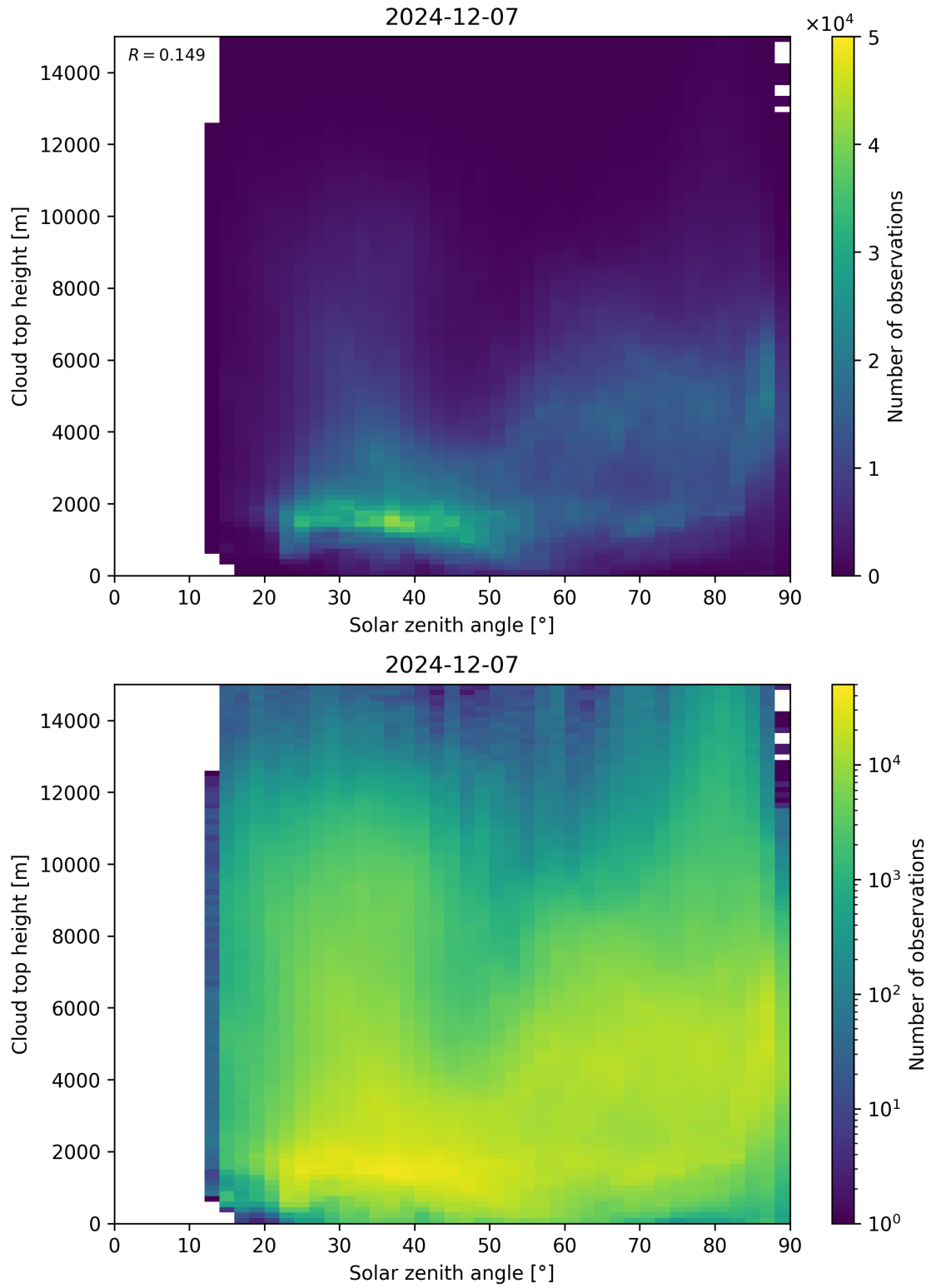
Figure 104: Scatter density plot of “Solar zenith angle” against “Cloud top height” for 2024-12-06 to 2024-12-08.
