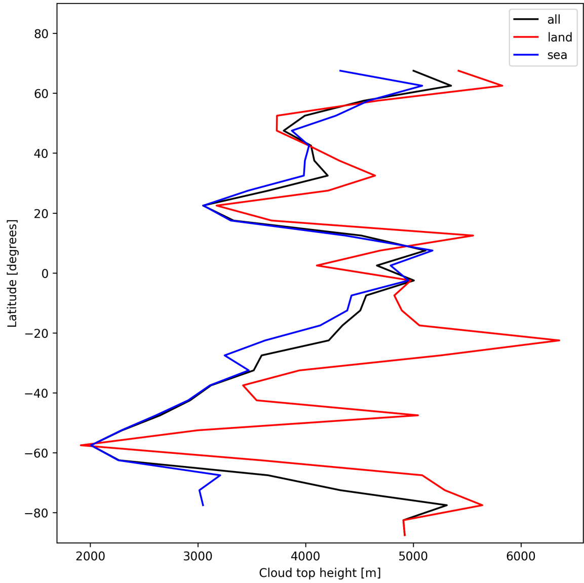
Figure 24: Zonal average of “Cloud top height” for 2024-12-06 to 2024-12-08.
