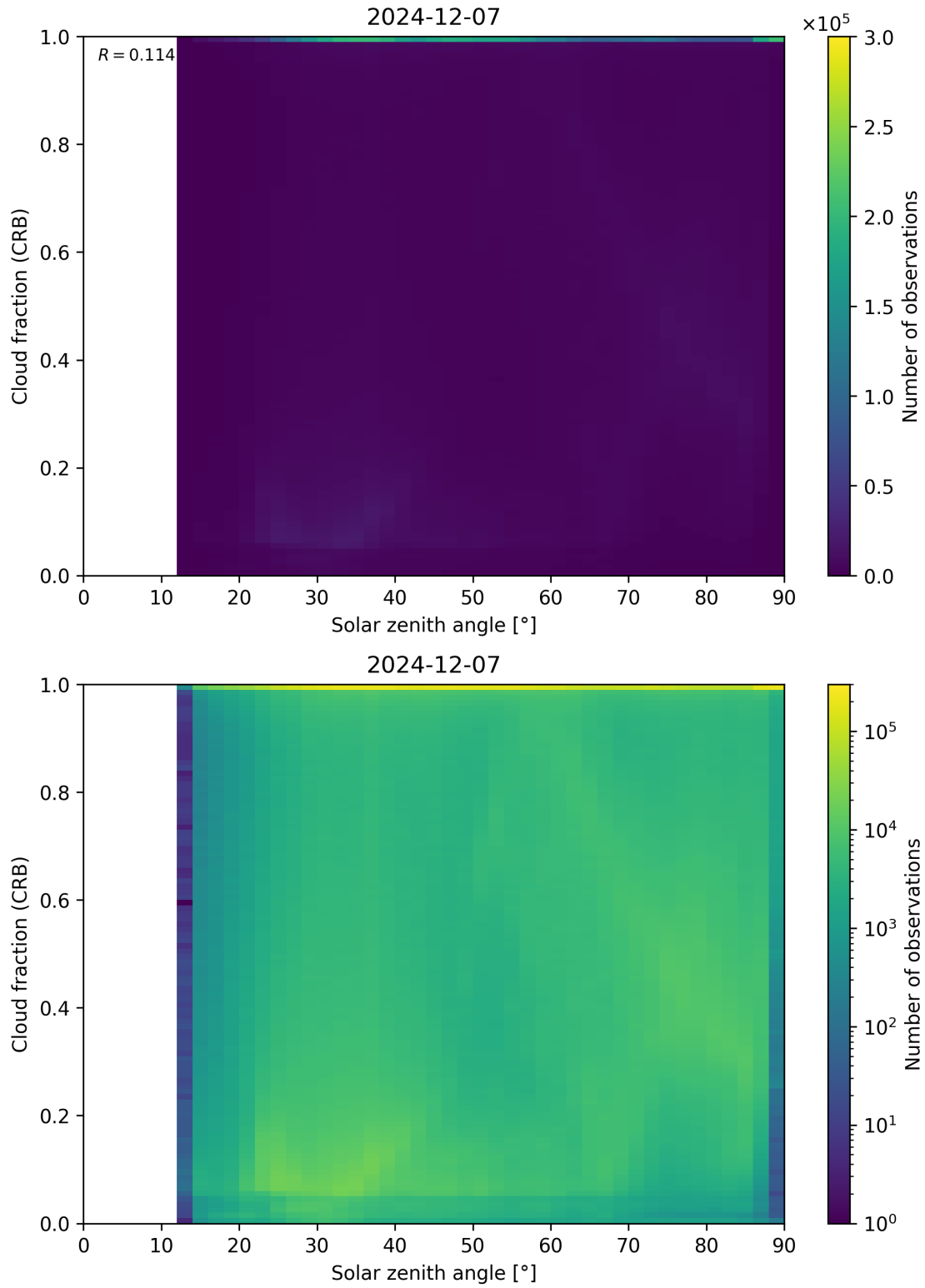
Figure 101: Scatter density plot of “Solar zenith angle” against “Cloud fraction (CRB)” for 2024-12-06 to 2024-12-08.
