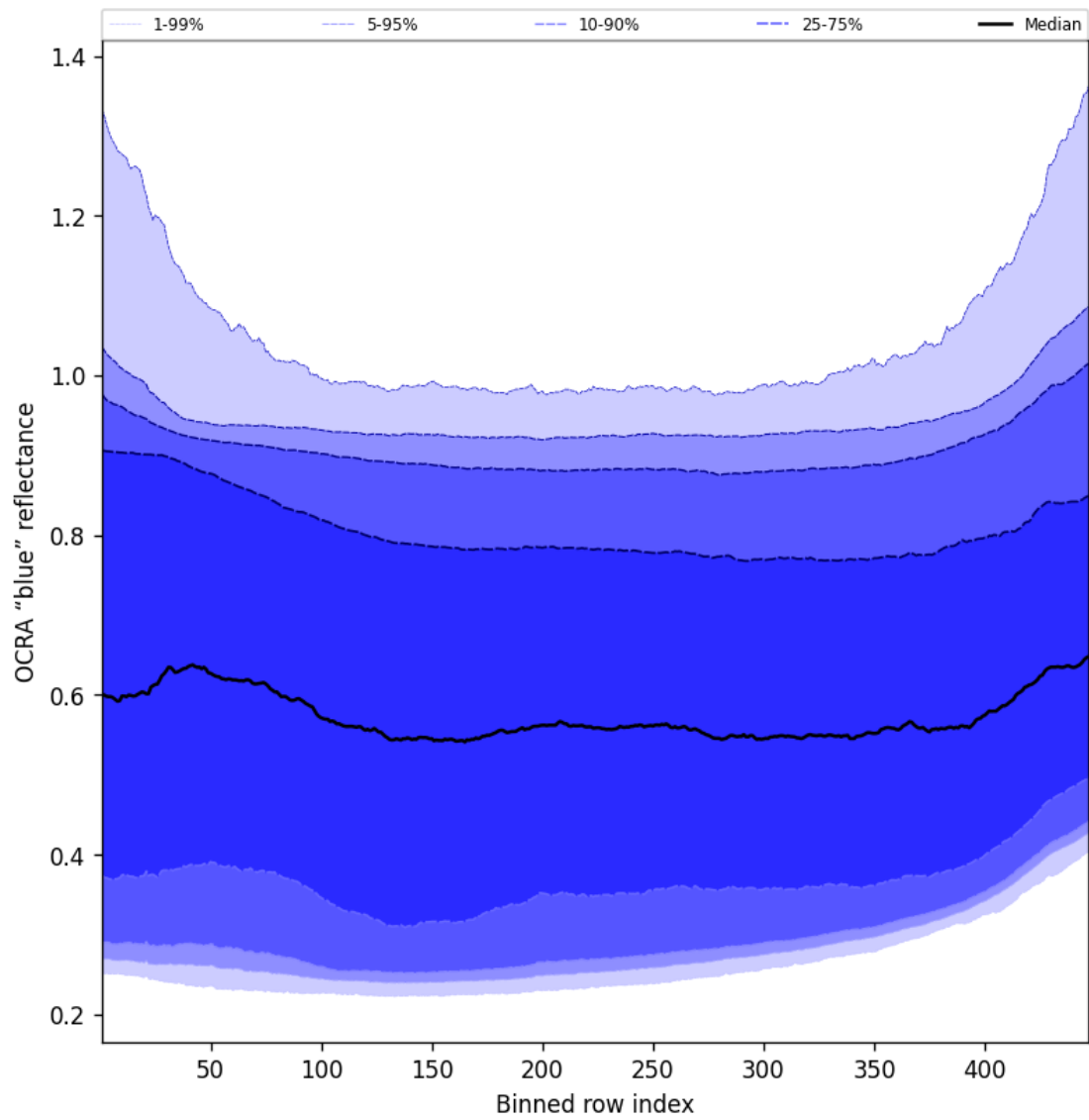
Figure 67: Along track statistics of "OCRA "blue" reflectance" for 2024-12-06 to 2024-12-08
