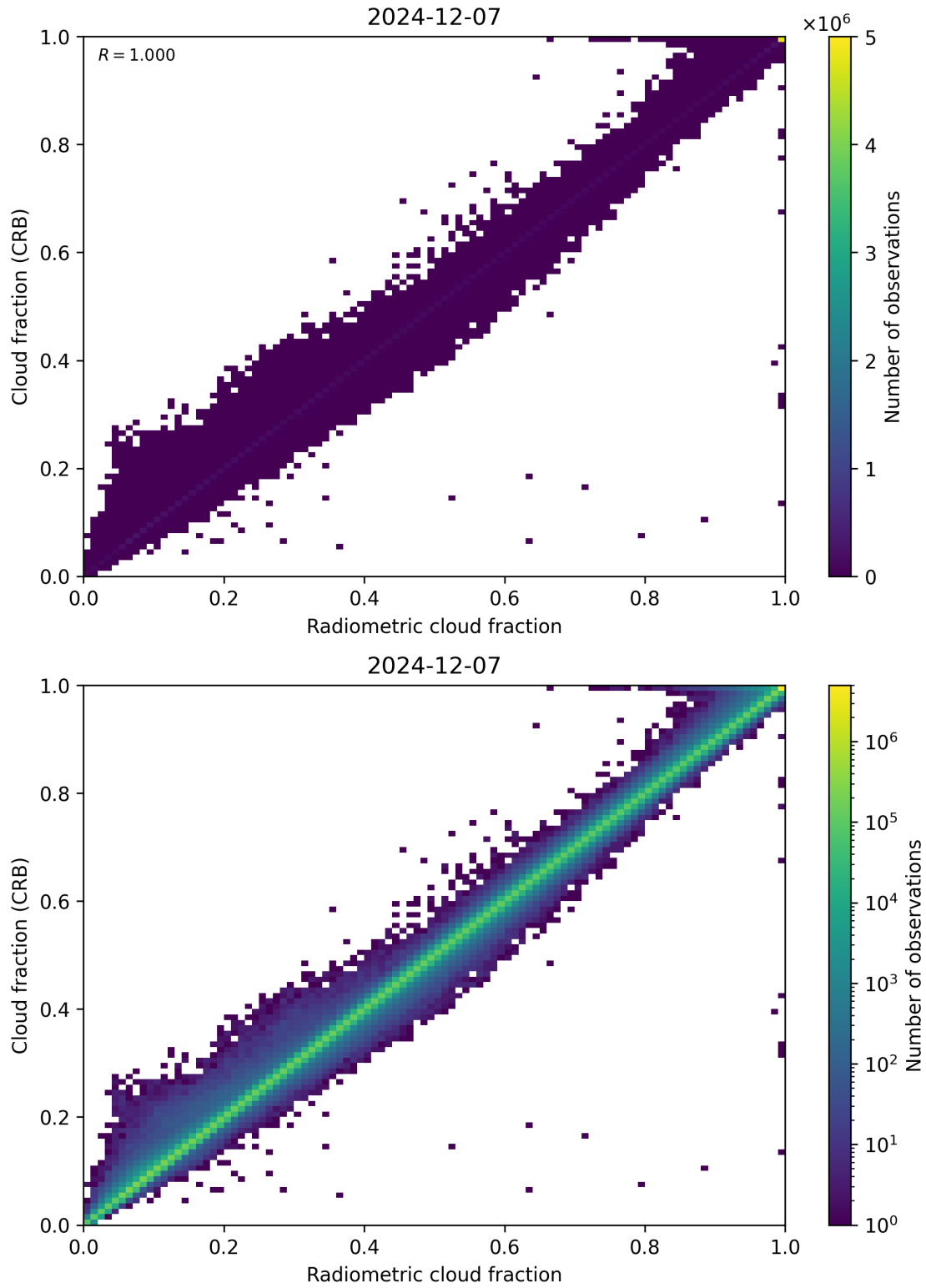
Figure 73: Scatter density plot of “Radiometric cloud fraction” against “Cloud fraction (CRB)” for 2024-12-06 to 2024-12-08.
