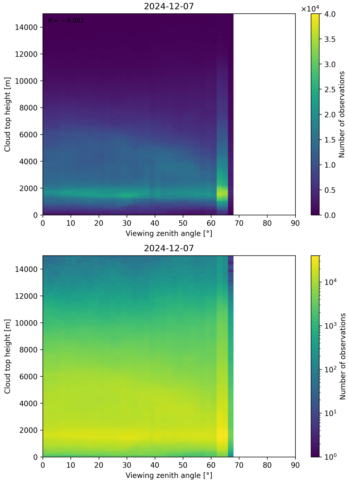
Figure 112: Scatter density plot of “Viewing zenith angle” against “Cloud top height” for 2024-12-06 to 2024-12-08.
