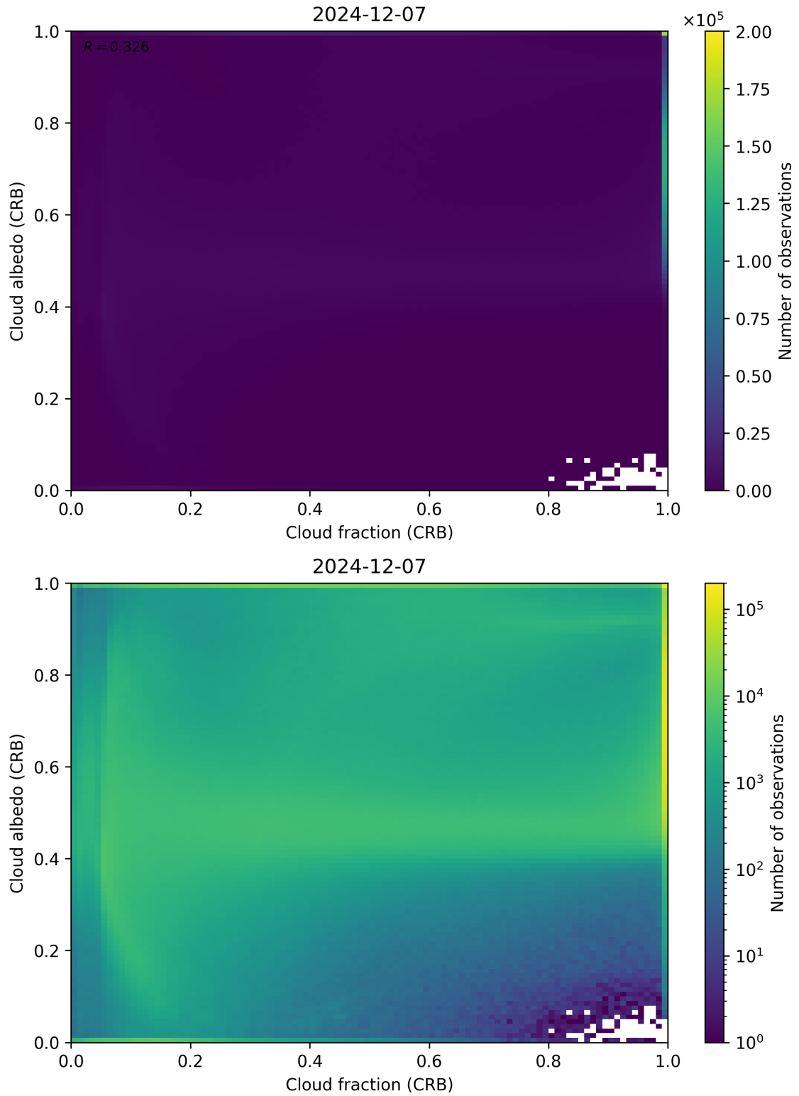
Figure 77: Scatter density plot of “Cloud fraction (CRB)” against “Cloud albedo (CRB)” for 2024-12-06 to 2024-12-08.
