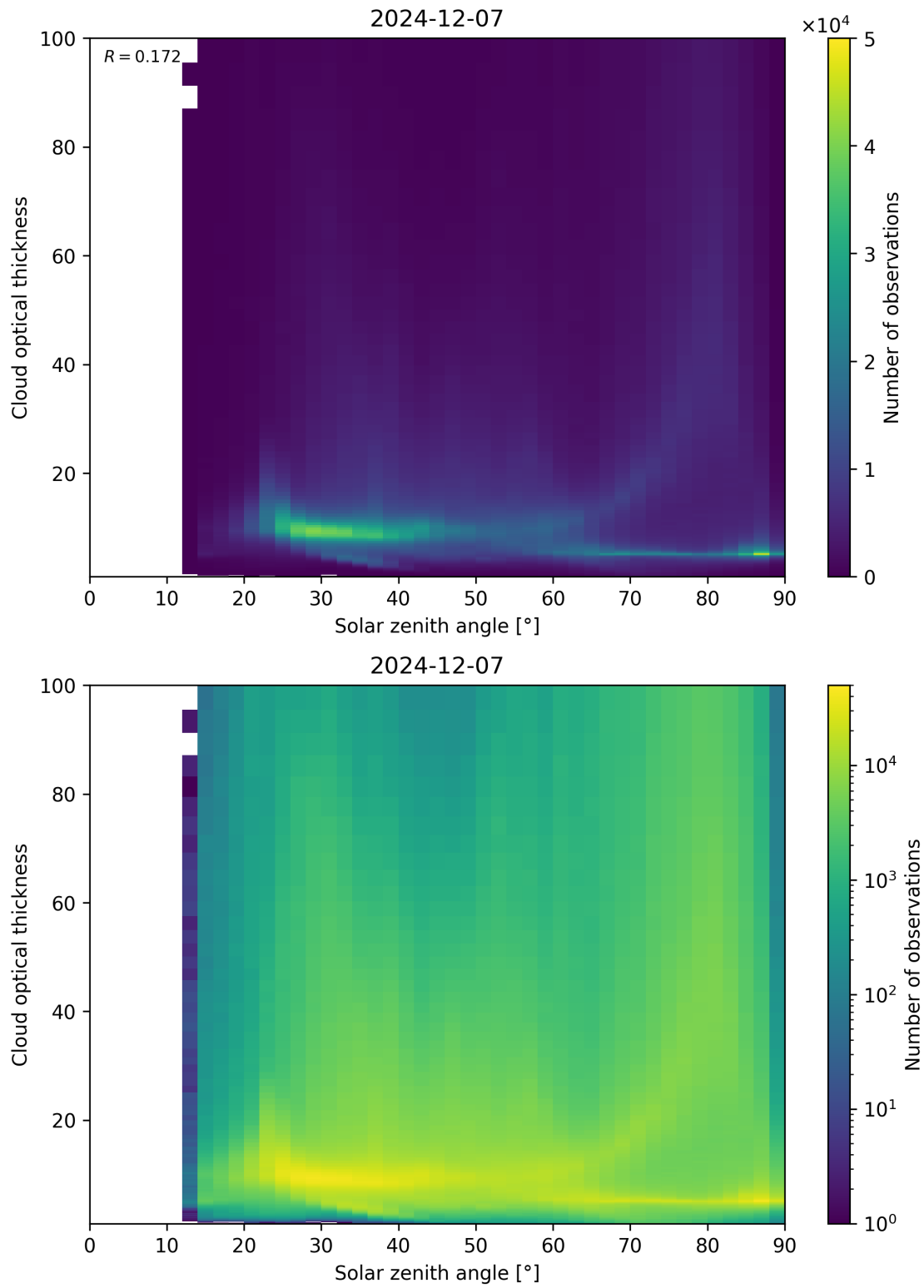
Figure 103: Scatter density plot of “Solar zenith angle” against “Cloud optical thickness” for 2024-12-06 to 2024-12-08.
