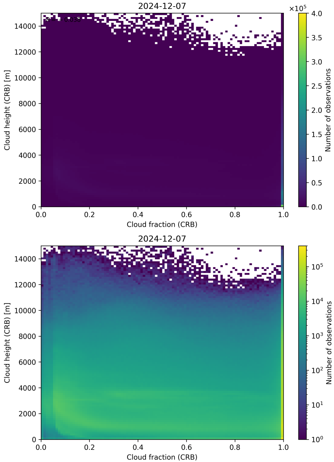
Figure 79: Scatter density plot of “Cloud fraction (CRB)” against “Cloud height (CRB)” for 2024-12-06 to 2024-12-08.
