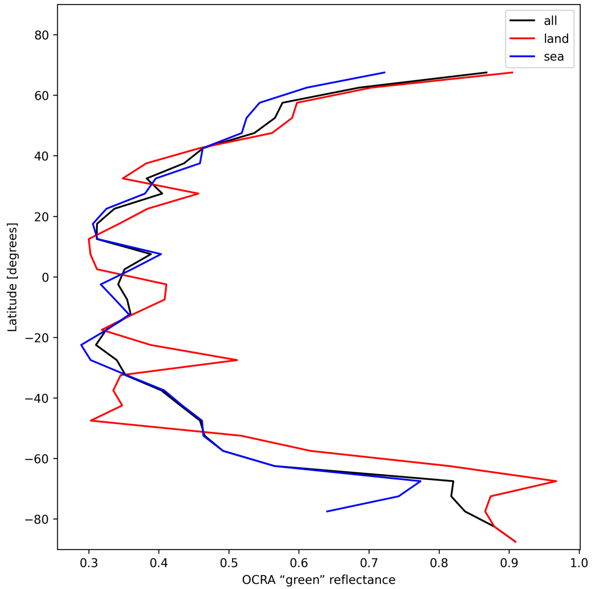
Figure 36: Zonal average of “OCRA “green” reflectance” for 2024-12-06 to 2024-12-08.
