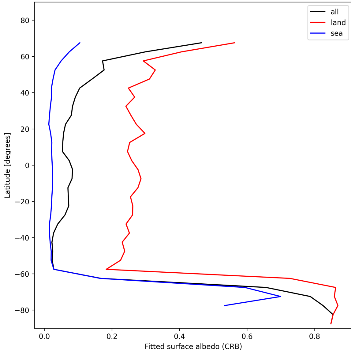
Figure 30: Zonal average of “Fitted surface albedo (CRB)” for 2024-12-06 to 2024-12-08.
