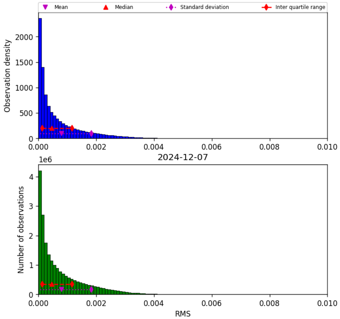
Figure 47: Histogram of “RMS” for 2024-12-06 to 2024-12-08
