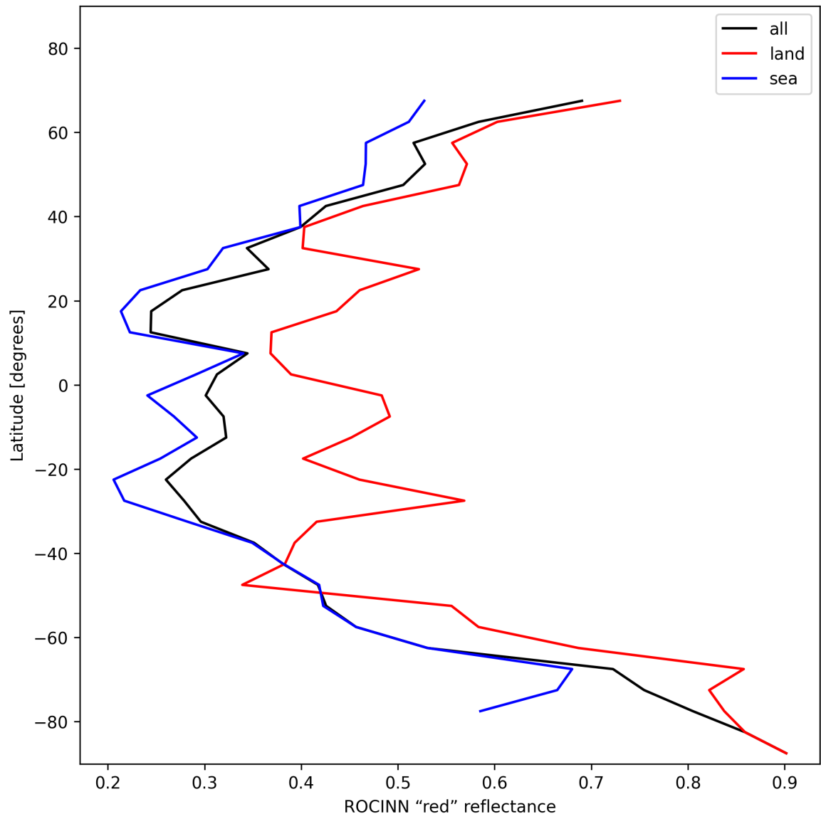
Figure 37: Zonal average of "ROCINN "red" reflectance" for 2024-12-06 to 2024-12-08.
