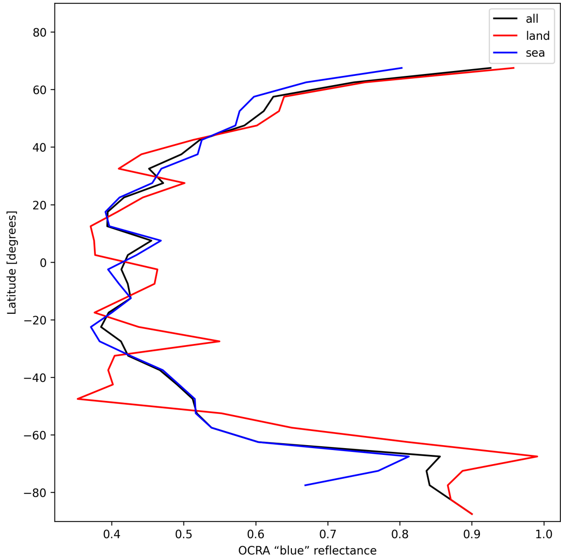
Figure 35: Zonal average of “OCRA “blue” reflectance” for 2024-12-06 to 2024-12-08.
