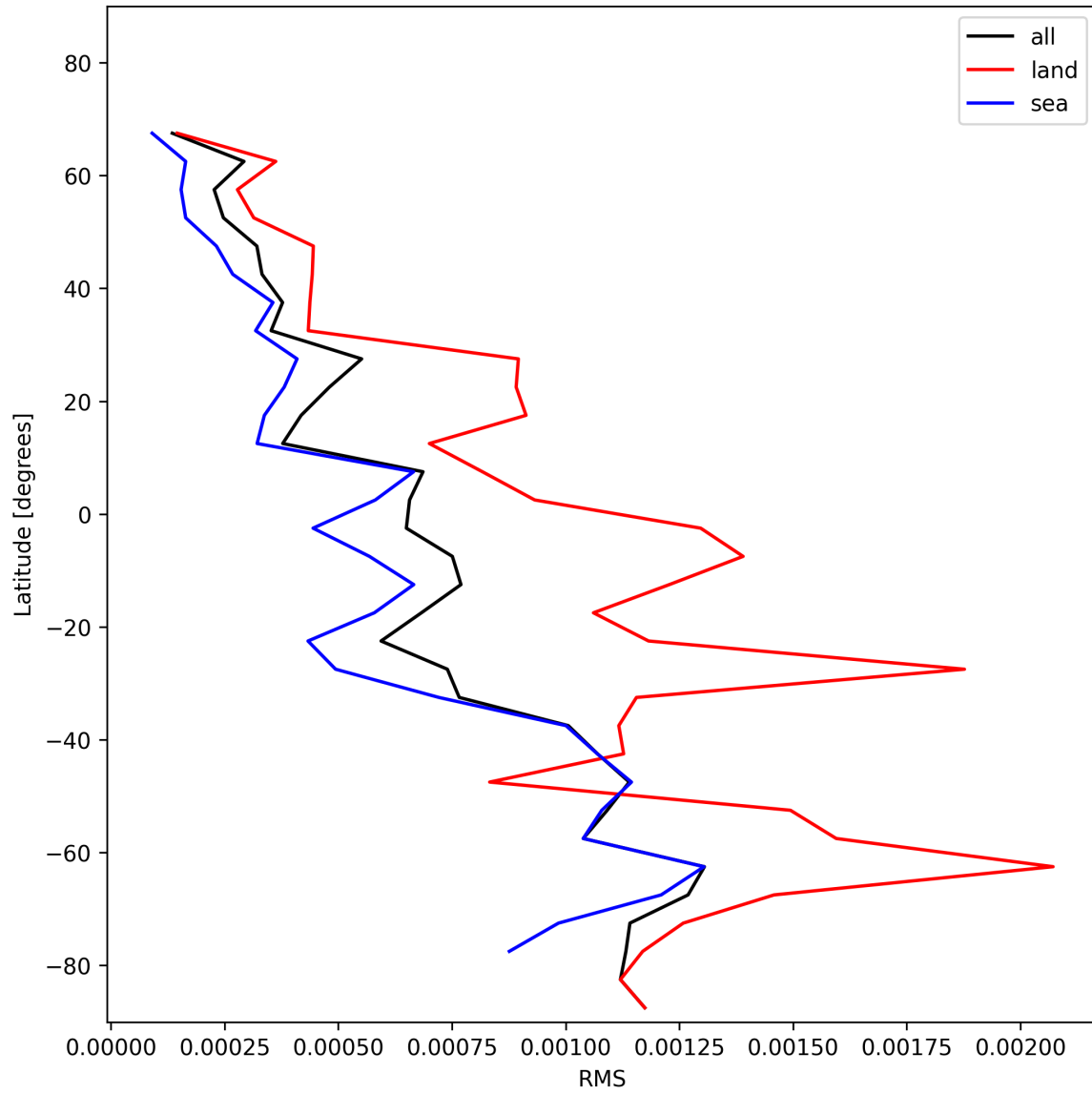
Figure 31: Zonal average of “RMS” for 2024-12-06 to 2024-12-08.
