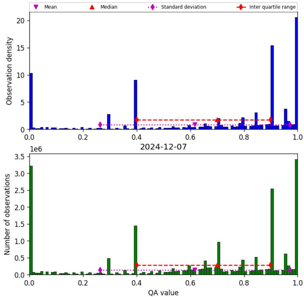
Figure 38: Histogram of “QA value” for 2024-12-06 to 2024-12-08
