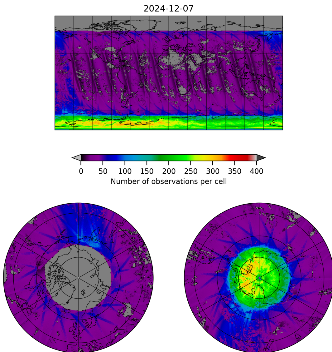
Figure 21: Map of the number of observations for 2024-12-06 to 2024-12-08
