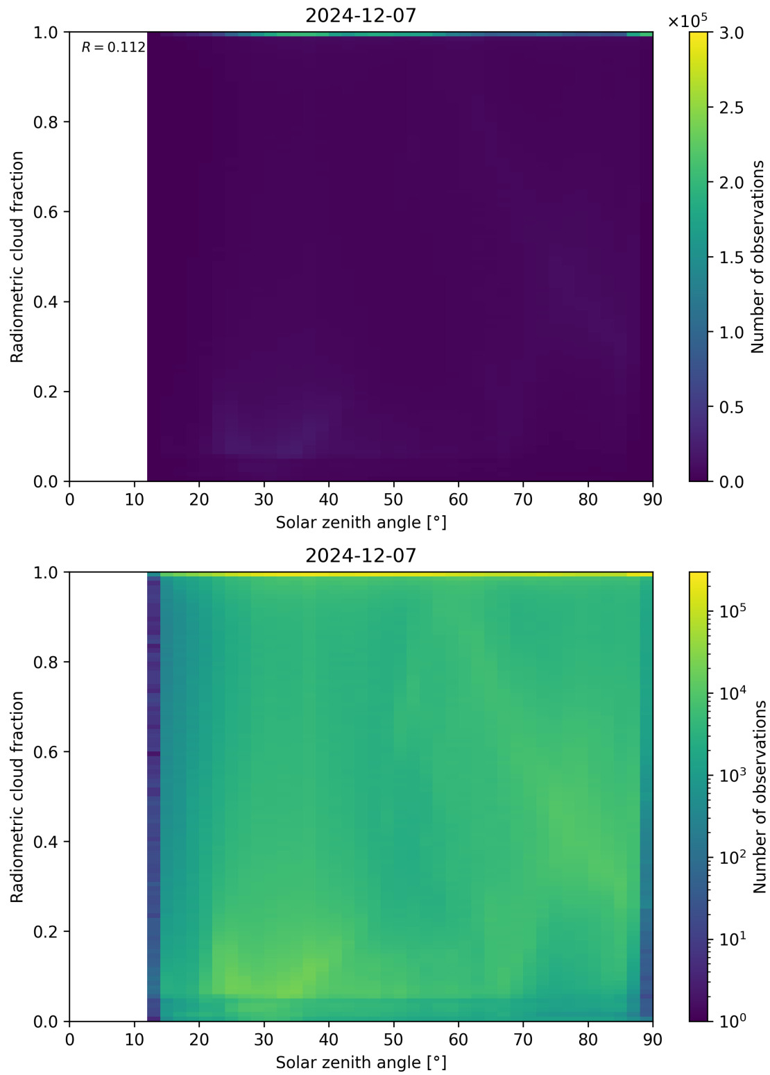
Figure 99: Scatter density plot of “Solar zenith angle” against “Radiometric cloud fraction” for 2024-12-06 to 2024-12-08.
