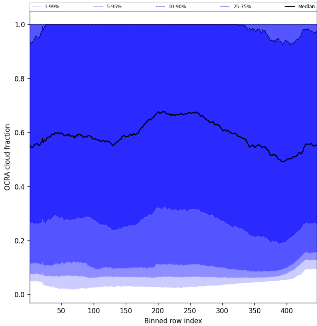
Figure 66: Along track statistics of “OCRA cloud fraction” for 2024-12-06 to 2024-12-08
