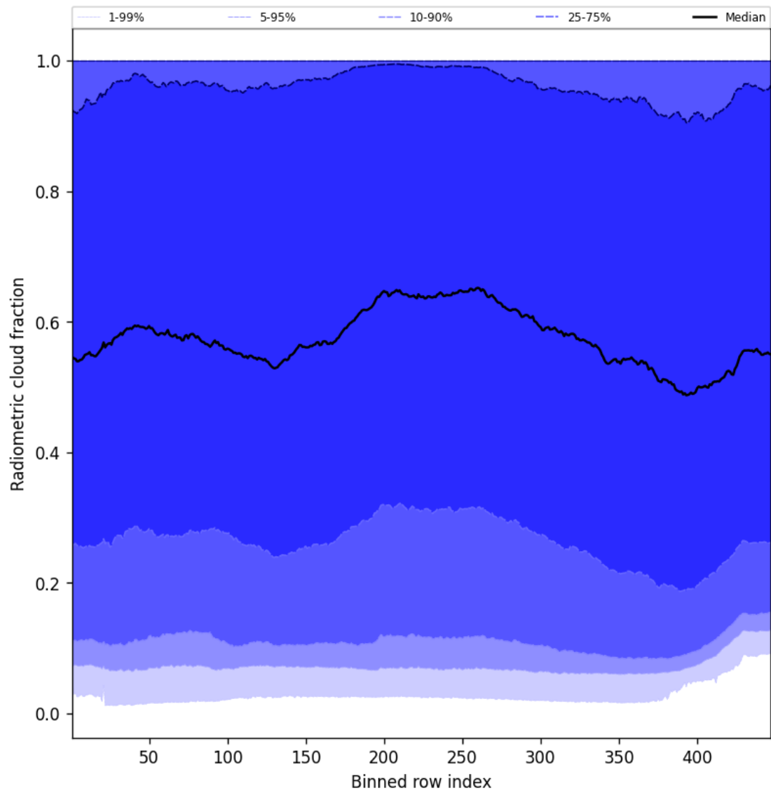
Figure 55: Along track statistics of “Radiometric cloud fraction” for 2024-12-06 to 2024-12-08
