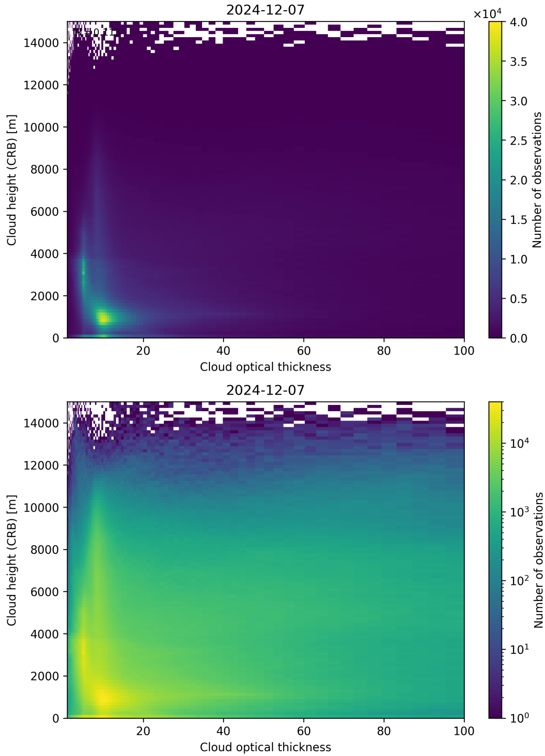
Figure 85: Scatter density plot of “Cloud optical thickness” against “Cloud height (CRB)” for 2024-12-06 to 2024-12-08.
