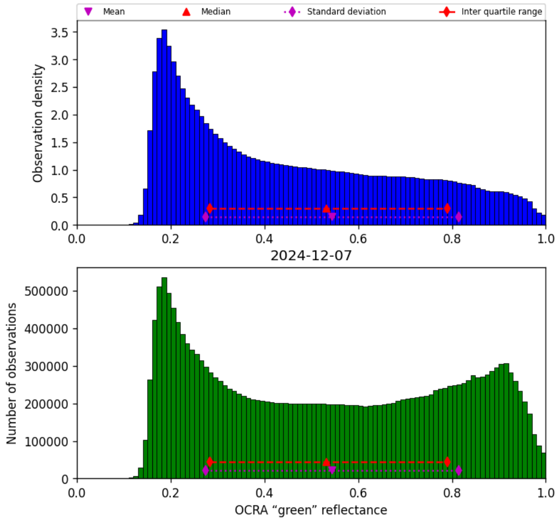
Figure 52: Histogram of “OCRA “green” reflectance” for 2024-12-06 to 2024-12-08
