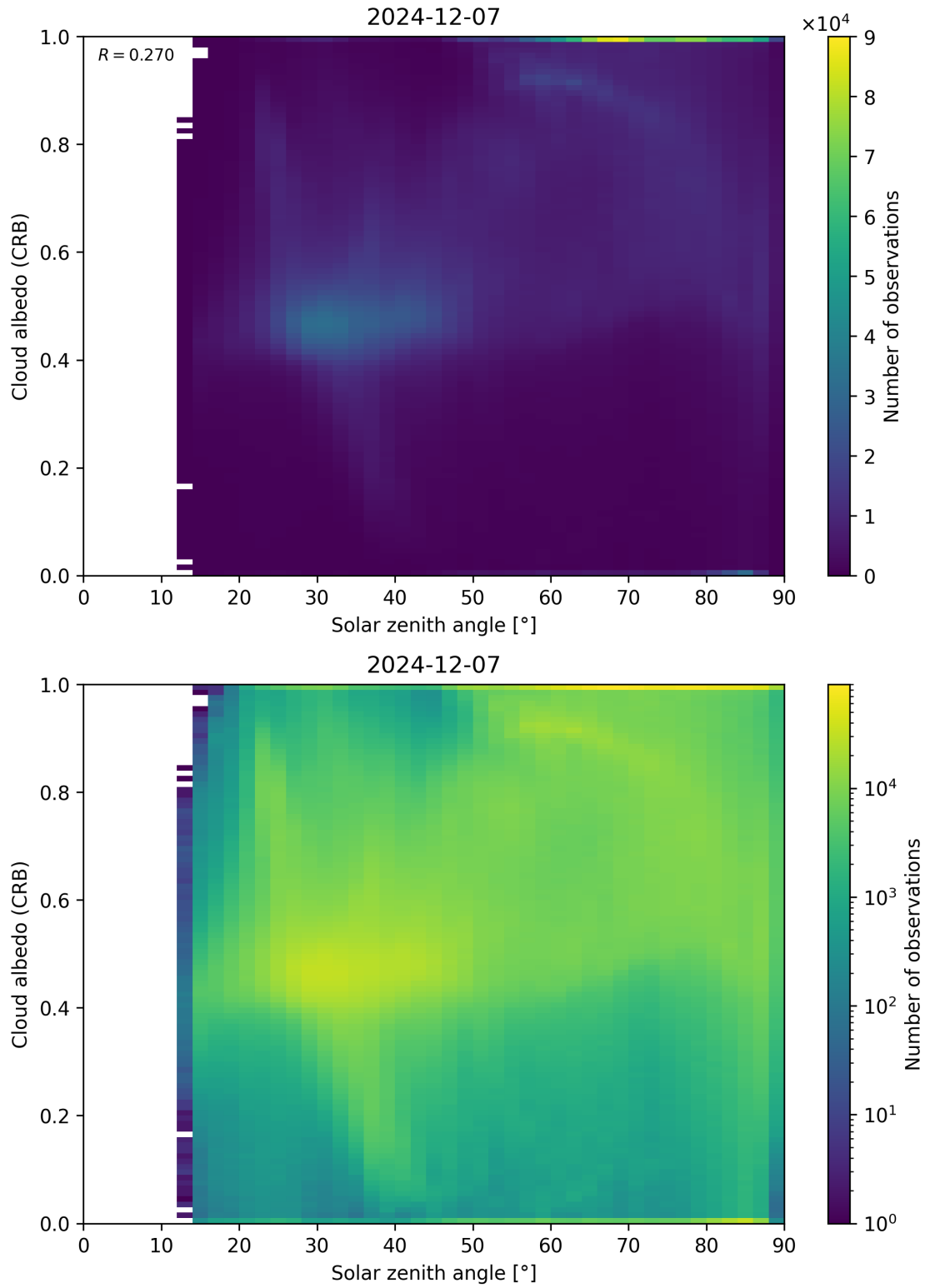
Figure 98: Scatter density plot of “Solar zenith angle” against “Cloud albedo (CRB)” for 2024-12-06 to 2024-12-08.
