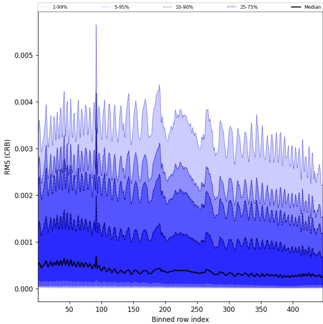
Figure 64: Along track statistics of “RMS (CRB)” for 2024-12-06 to 2024-12-08
