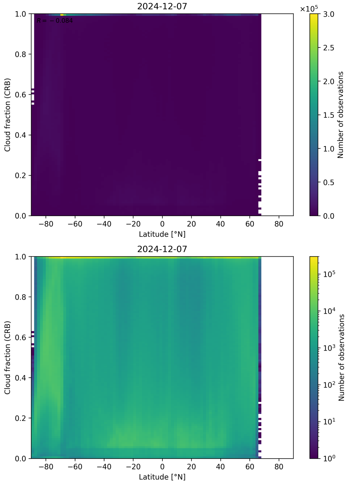
Figure 94: Scatter density plot of “Latitude” against “Cloud fraction (CRB)” for 2024-12-06 to 2024-12-08.
