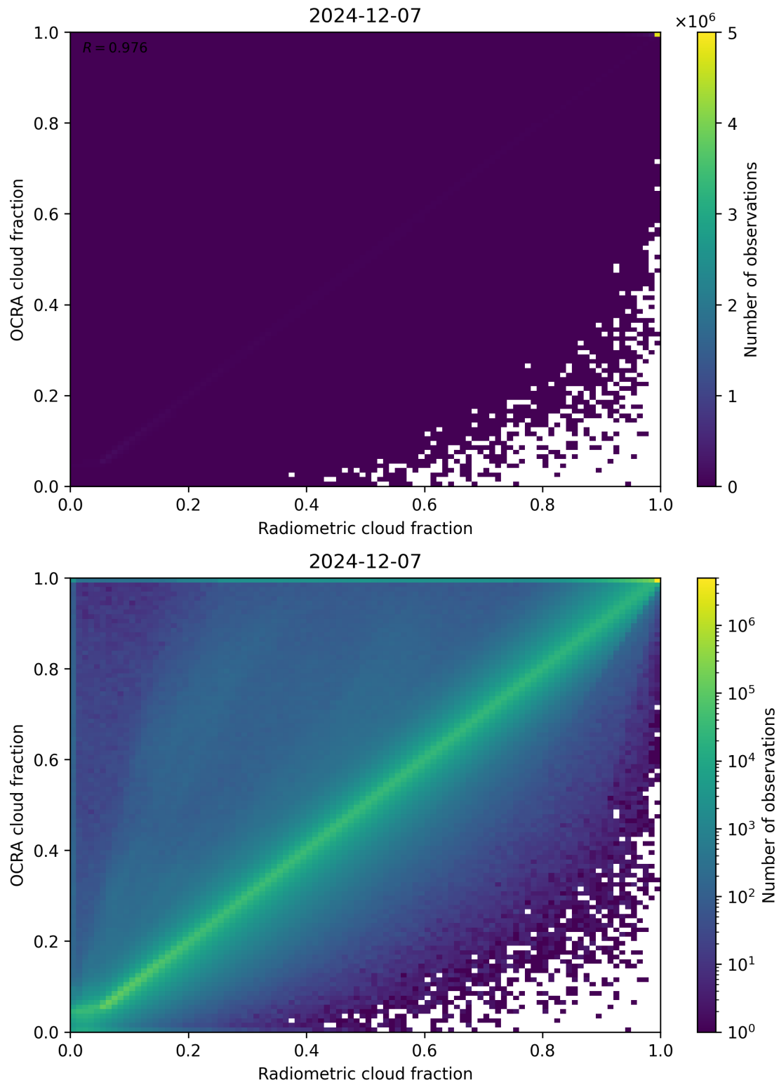
Figure 72: Scatter density plot of “Radiometric cloud fraction” against “OCRA cloud fraction” for 2024-12-06 to 2024-12-08.
