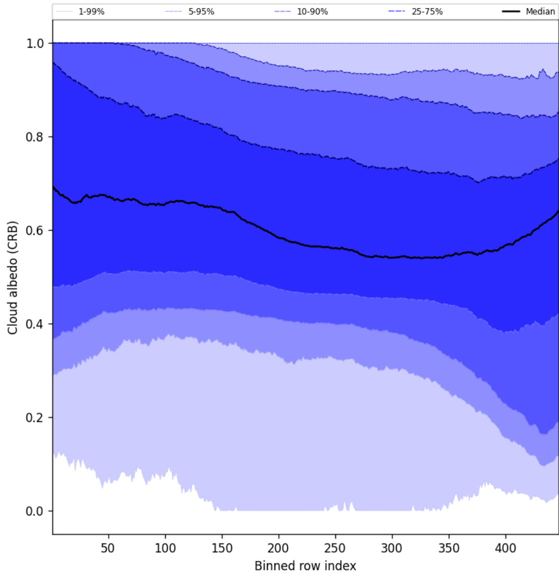
Figure 60: Along track statistics of “Cloud albedo (CRB)” for 2024-12-06 to 2024-12-08
