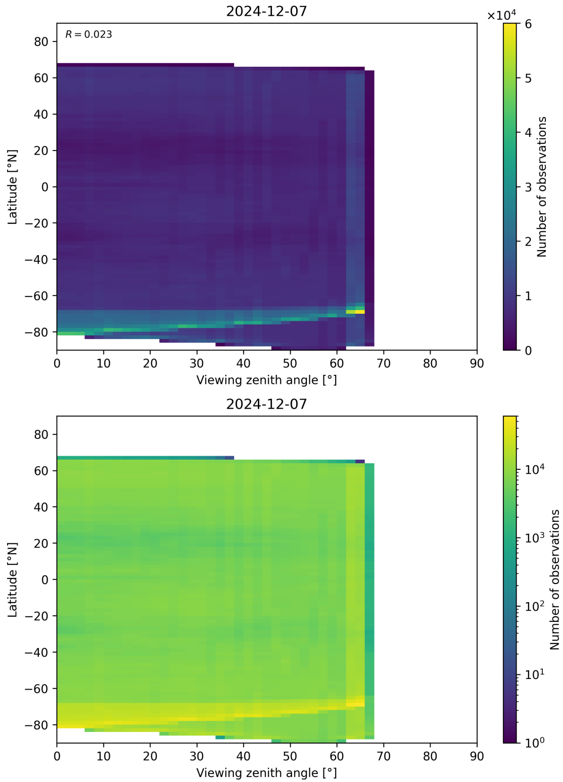
Figure 113: Scatter density plot of “Viewing zenith angle” against “Latitude” for 2024-12-06 to 2024-12-08.
