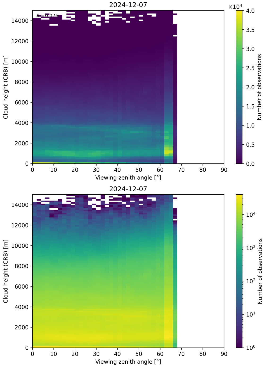
Figure 110: Scatter density plot of “Viewing zenith angle” against “Cloud height (CRB)” for 2024-12-06 to 2024-12-08.
