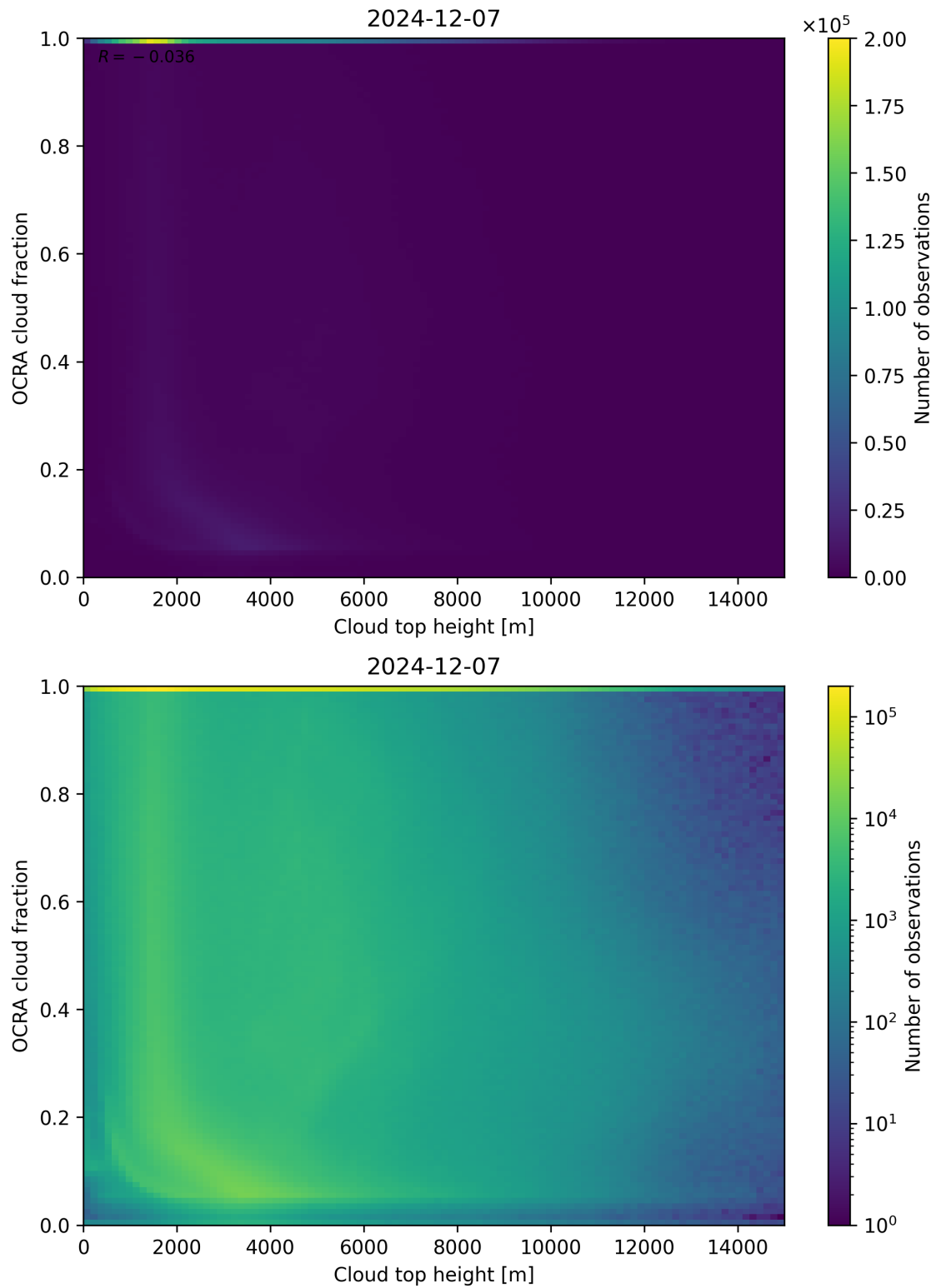
Figure 87: Scatter density plot of “Cloud top height” against “OCRA cloud fraction” for 2024-12-06 to 2024-12-08.
