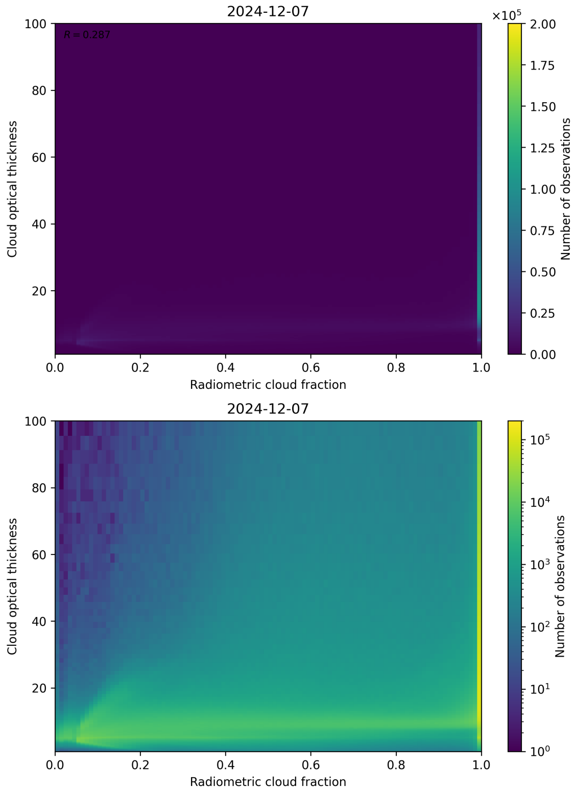
Figure 75: Scatter density plot of “Radiometric cloud fraction” against “Cloud optical thickness” for 2024-12-06 to 2024-12-08.
