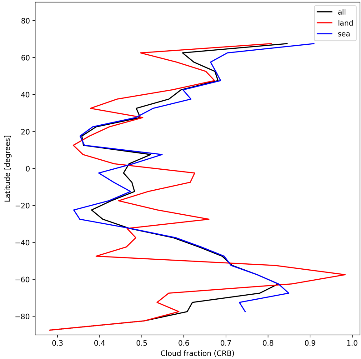
Figure 26: Zonal average of “Cloud fraction (CRB)” for 2024-12-06 to 2024-12-08.
