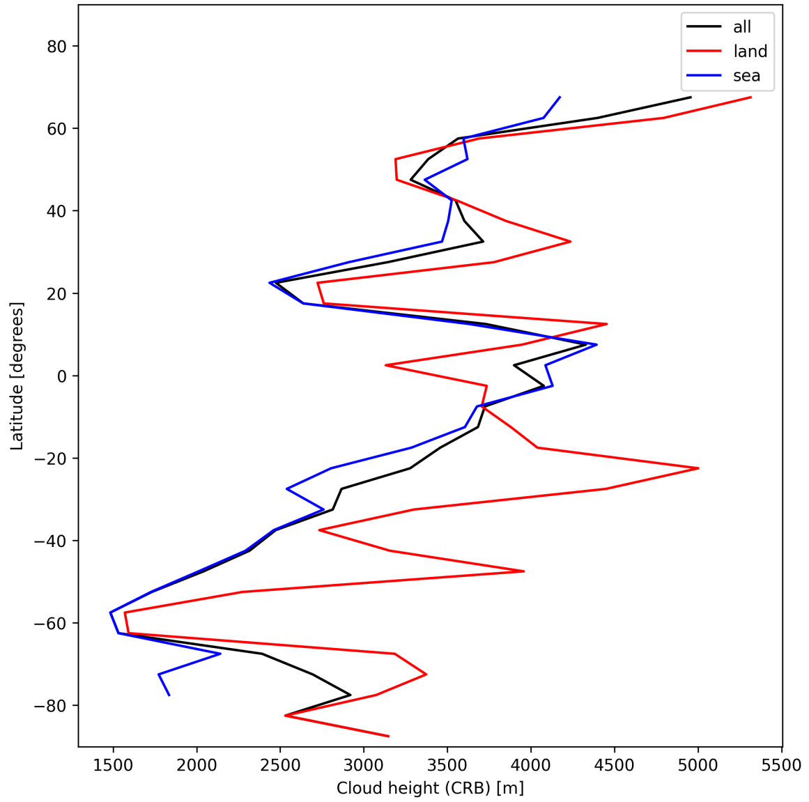
Figure 27: Zonal average of “Cloud height (CRB)” for 2024-12-06 to 2024-12-08.
