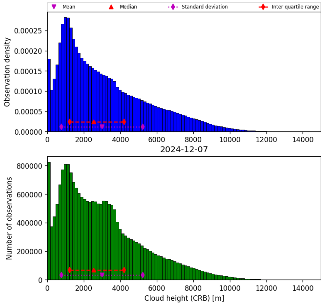
Figure 43: Histogram of “Cloud height (CRB)” for 2024-12-06 to 2024-12-08
