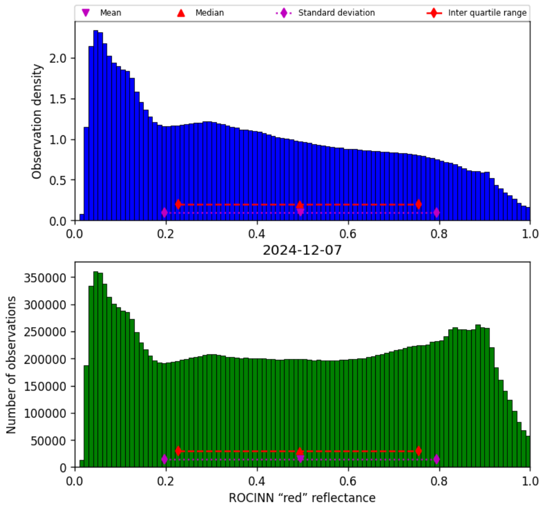
Figure 53: Histogram of “ROCINN “red” reflectance” for 2024-12-06 to 2024-12-08
