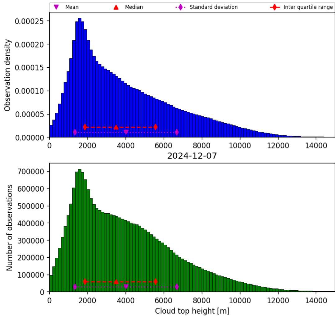
Figure 40: Histogram of “Cloud top height” for 2024-12-06 to 2024-12-08
