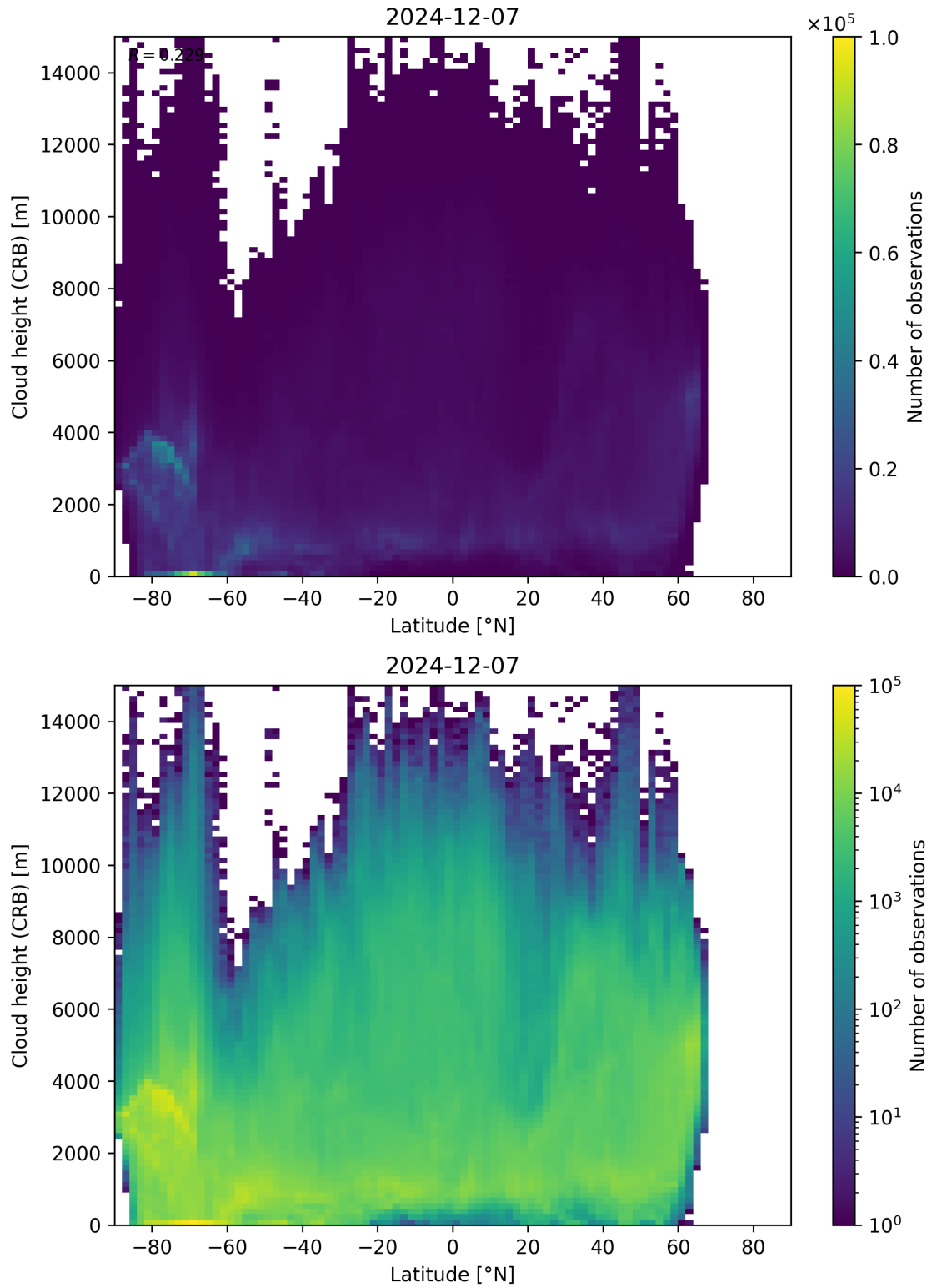
Figure 95: Scatter density plot of “Latitude” against “Cloud height (CRB)” for 2024-12-06 to 2024-12-08.
