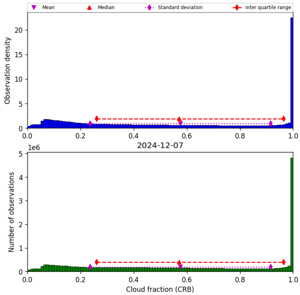
Figure 42: Histogram of “Cloud fraction (CRB)” for 2024-12-06 to 2024-12-08
