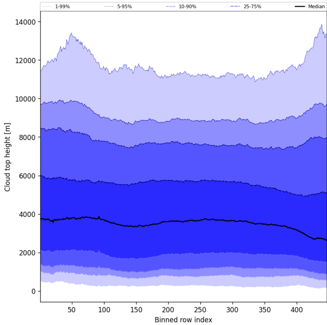
Figure 56: Along track statistics of “Cloud top height” for 2024-12-06 to 2024-12-08
