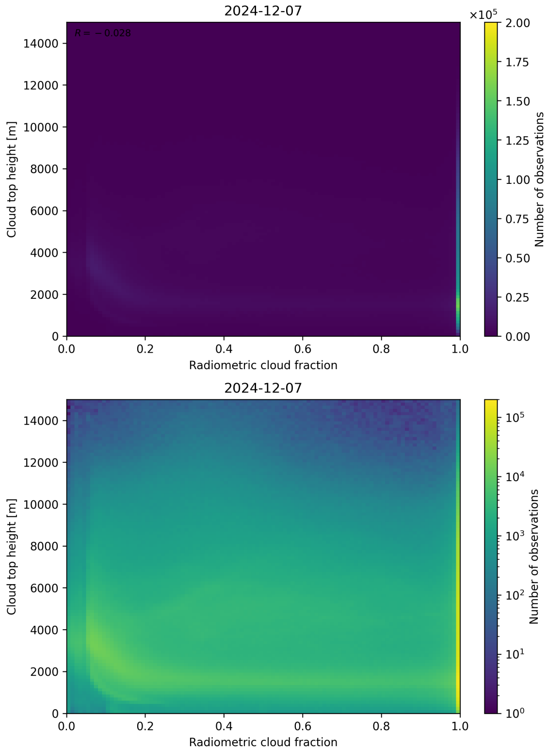
Figure 76: Scatter density plot of “Radiometric cloud fraction” against “Cloud top height” for 2024-12-06 to 2024-12-08.
