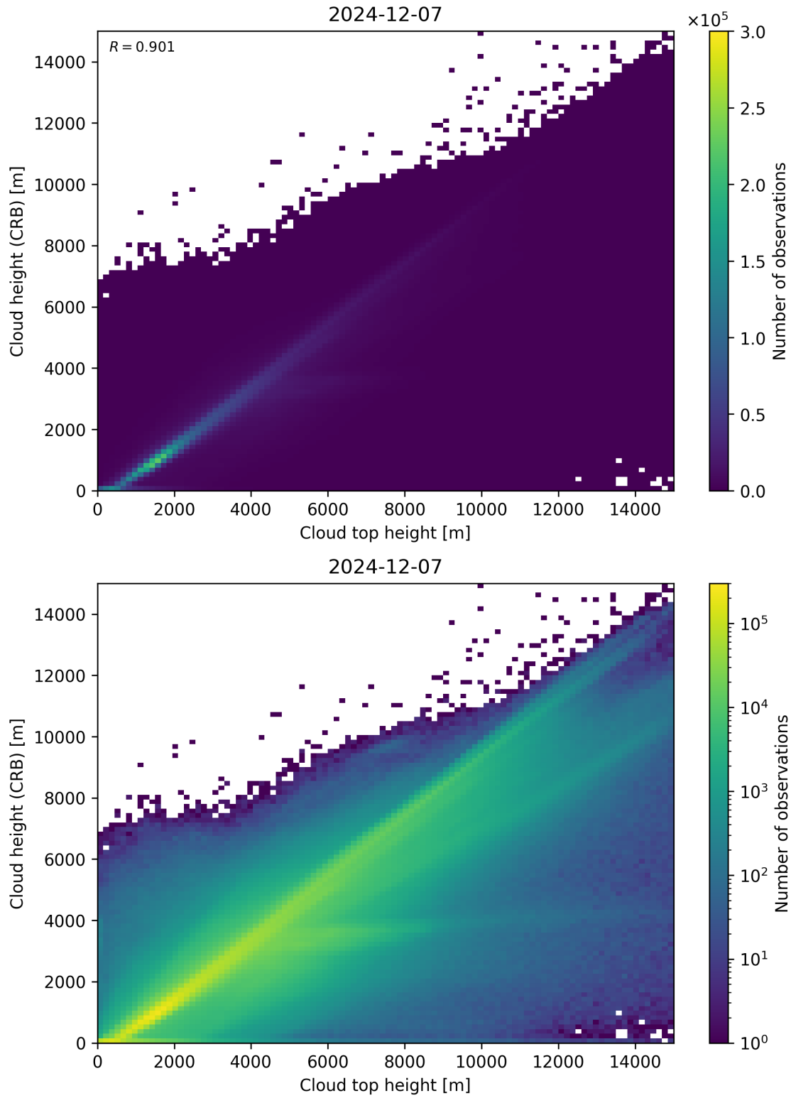
Figure 89: Scatter density plot of “Cloud top height” against “Cloud height (CRB)” for 2024-12-06 to 2024-12-08.
