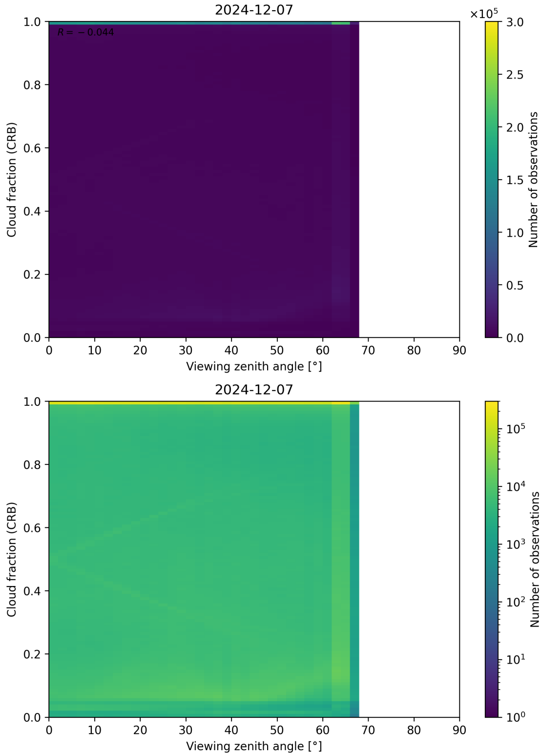
Figure 109: Scatter density plot of “Viewing zenith angle” against “Cloud fraction (CRB)” for 2024-12-06 to 2024-12-08.
