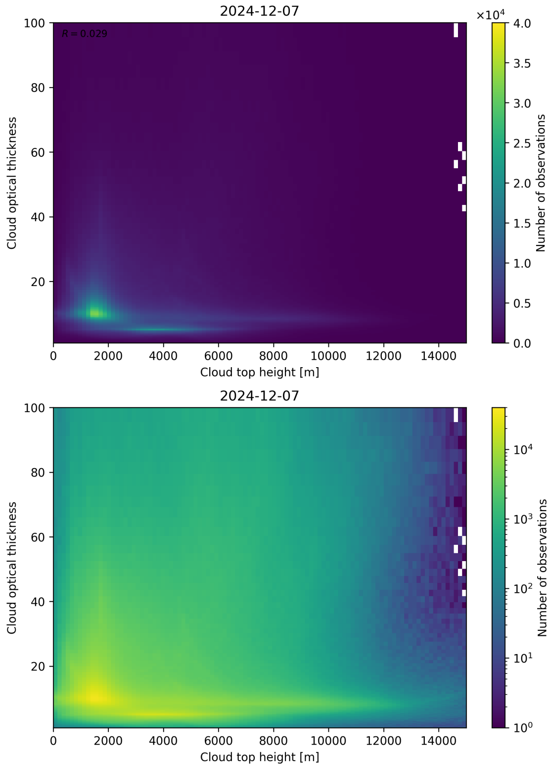
Figure 90: Scatter density plot of “Cloud top height” against “Cloud optical thickness” for 2024-12-06 to 2024-12-08.
