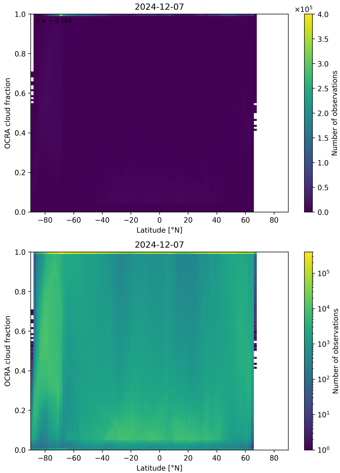
Figure 93: Scatter density plot of “Latitude” against “OCRA cloud fraction” for 2024-12-06 to 2024-12-08.
