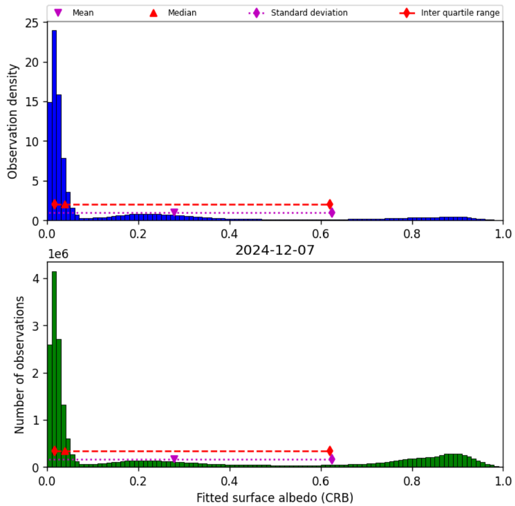
Figure 46: Histogram of “Fitted surface albedo (CRB)” for 2024-12-06 to 2024-12-08
