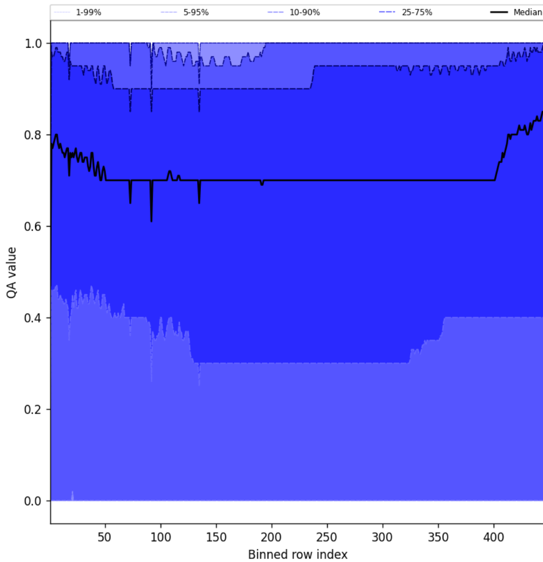
Figure 54: Along track statistics of “QA value” for 2024-12-06 to 2024-12-08
