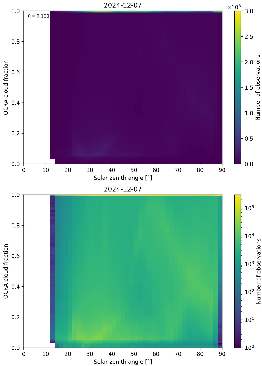
Figure 100: Scatter density plot of “Solar zenith angle” against “OCRA cloud fraction” for 2024-12-06 to 2024-12-08.
