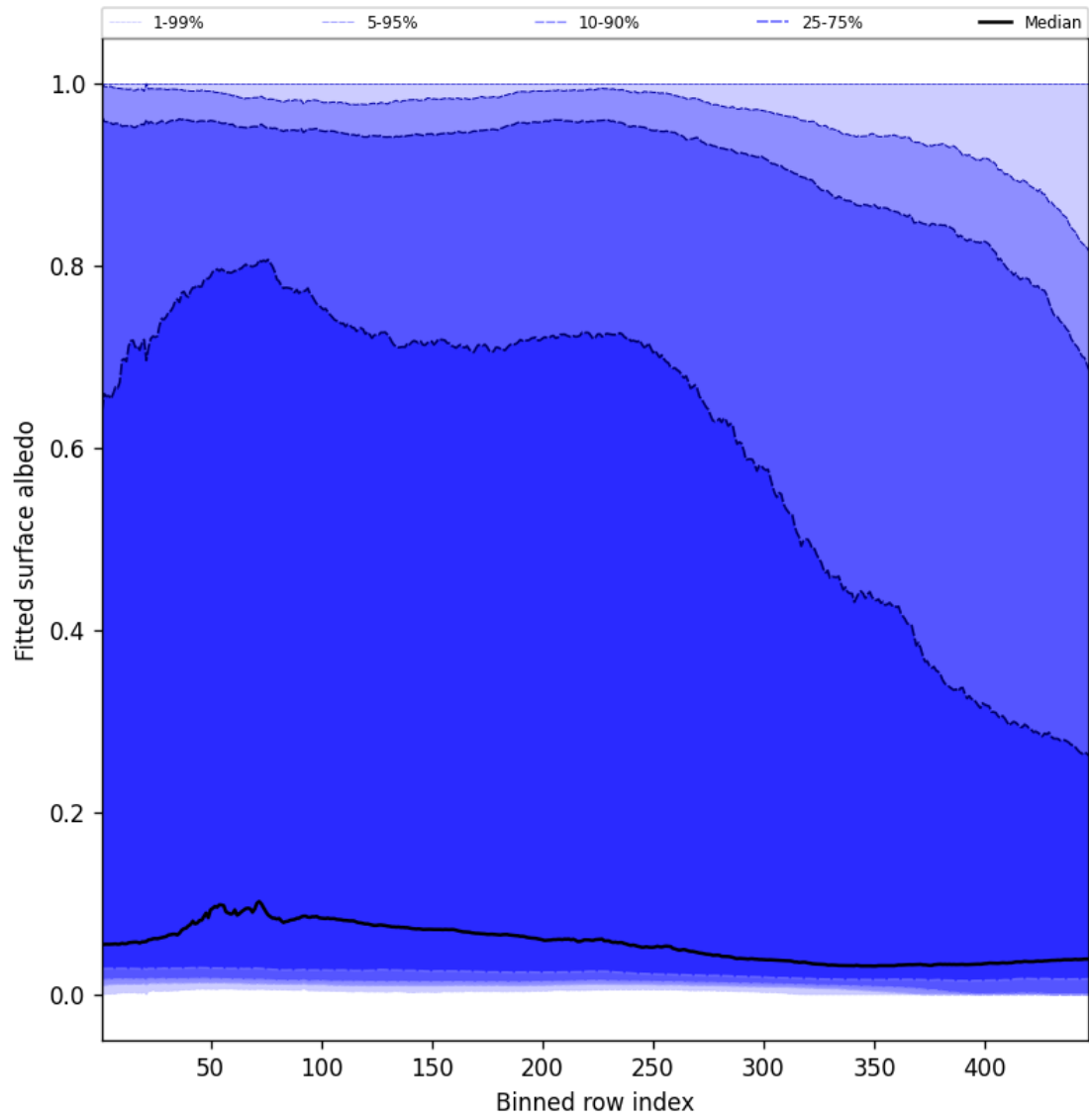
Figure 61: Along track statistics of “Fitted surface albedo” for 2024-12-06 to 2024-12-08
