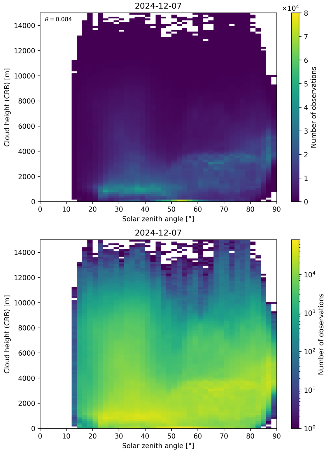
Figure 102: Scatter density plot of “Solar zenith angle” against “Cloud height (CRB)” for 2024-12-06 to 2024-12-08.
