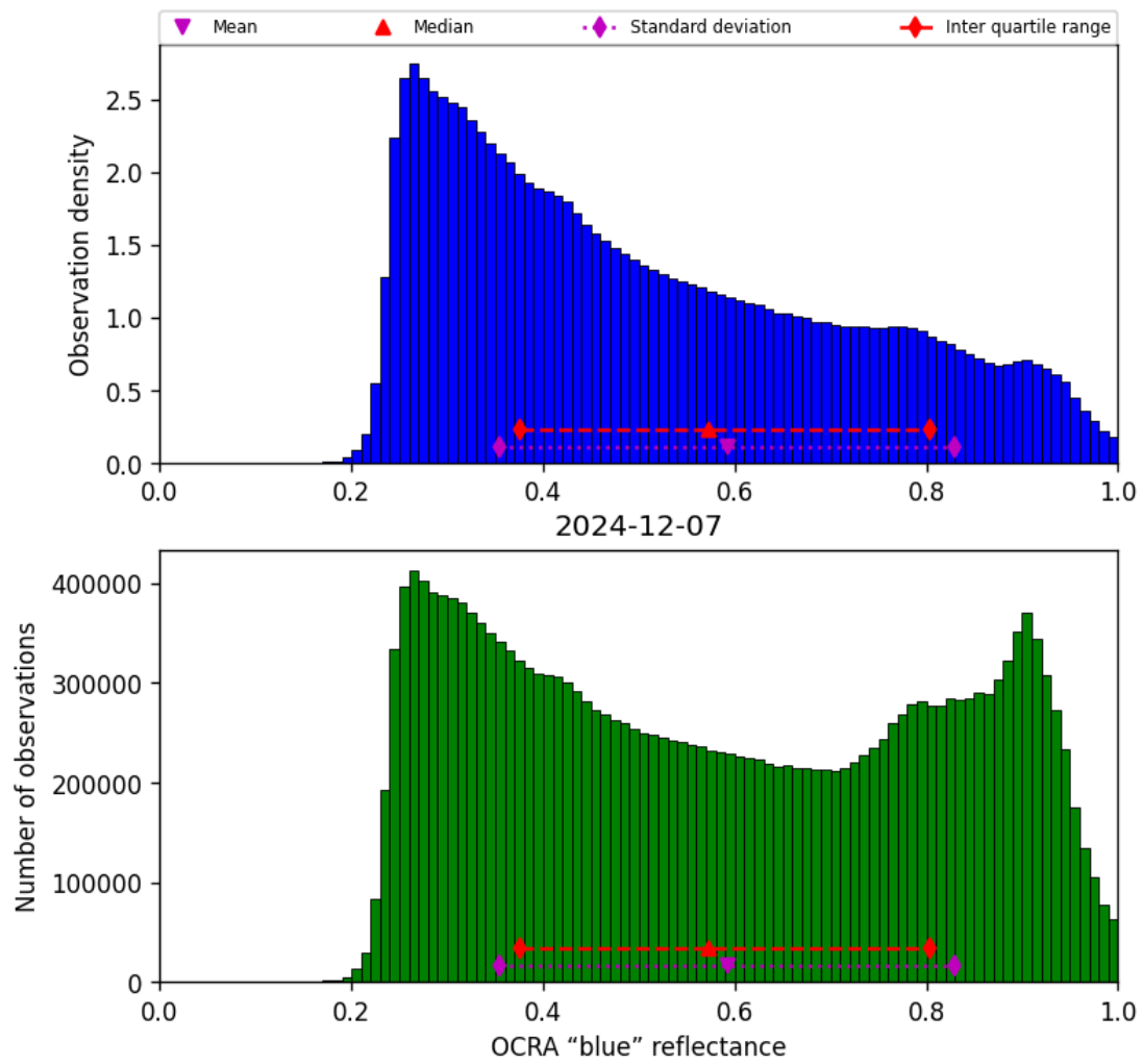
Figure 51: Histogram of “OCRA “blue” reflectance” for 2024-12-06 to 2024-12-08
