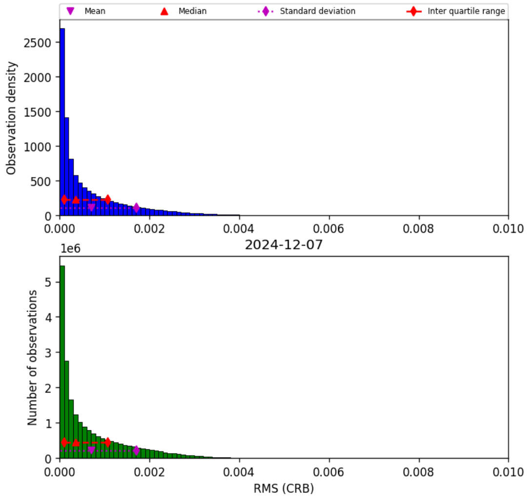
Figure 48: Histogram of “RMS (CRB)” for 2024-12-06 to 2024-12-08
