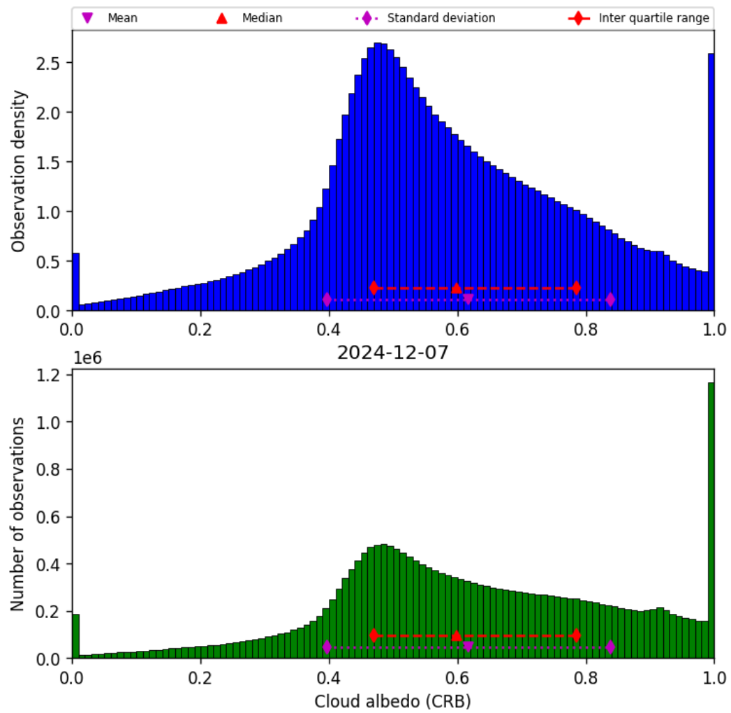
Figure 44: Histogram of “Cloud albedo (CRB)” for 2024-12-06 to 2024-12-08
