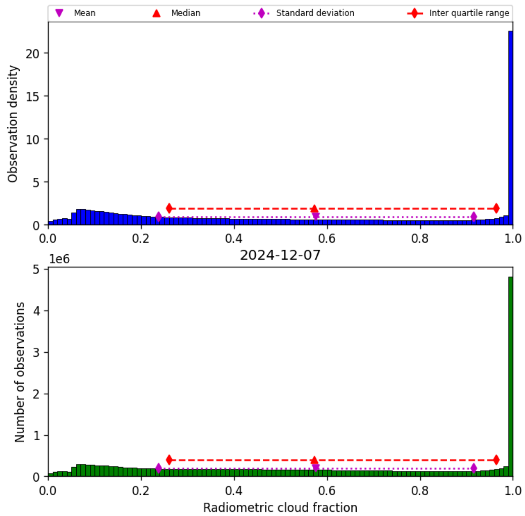
Figure 39: Histogram of “Radiometric cloud fraction” for 2024-12-06 to 2024-12-08
