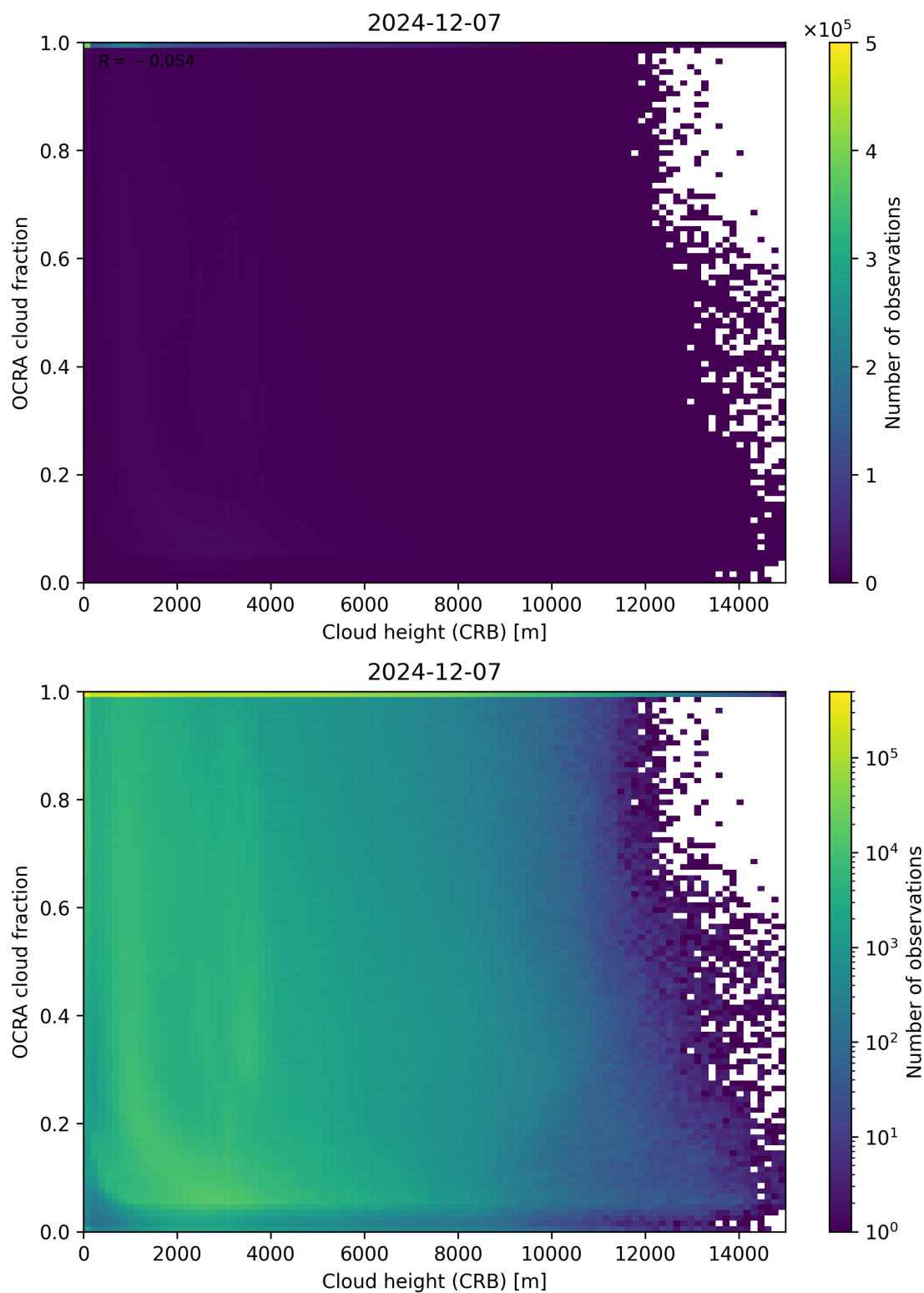
Figure 81: Scatter density plot of “Cloud height (CRB)” against “OCRA cloud fraction” for 2024-12-06 to 2024-12-08.
