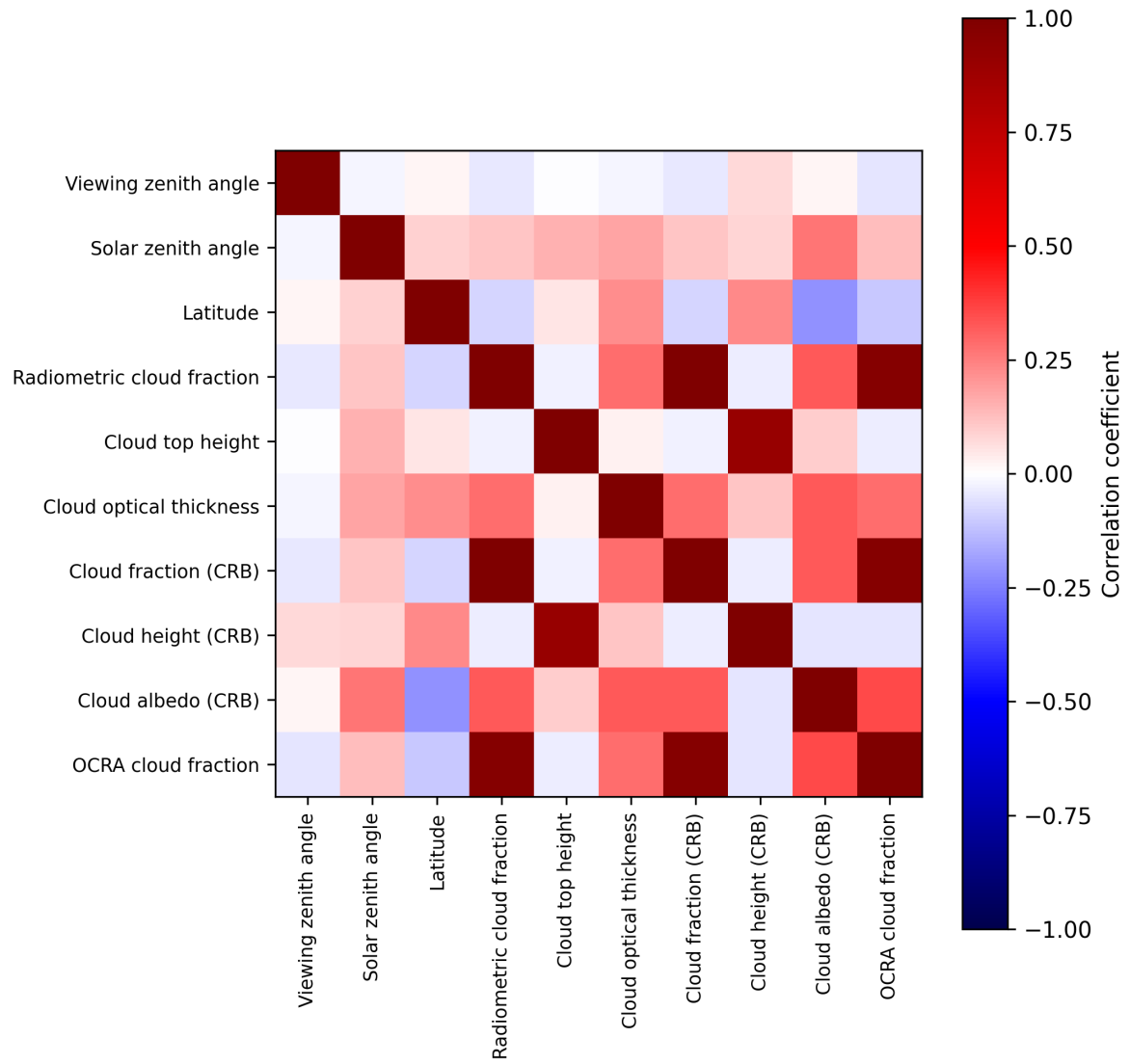
Figure 2: Map of correlation matrix for 2024-12-06 to 2024-12-08.
