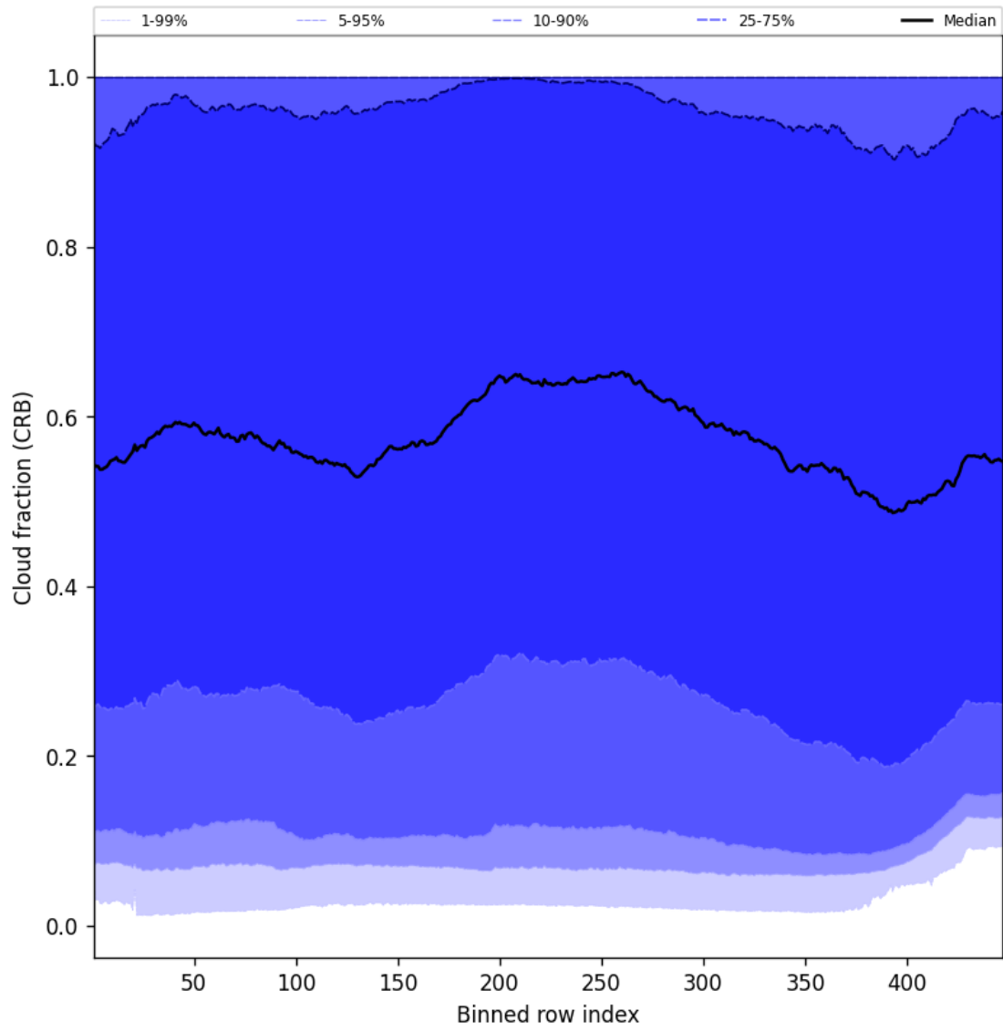
Figure 58: Along track statistics of “Cloud fraction (CRB)” for 2024-12-06 to 2024-12-08
