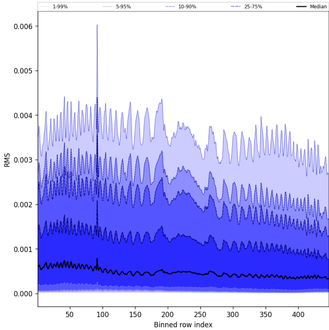
Figure 63: Along track statistics of “RMS” for 2024-12-06 to 2024-12-08
