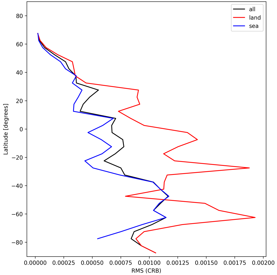
Figure 32: Zonal average of “RMS (CRB)” for 2024-12-06 to 2024-12-08.
