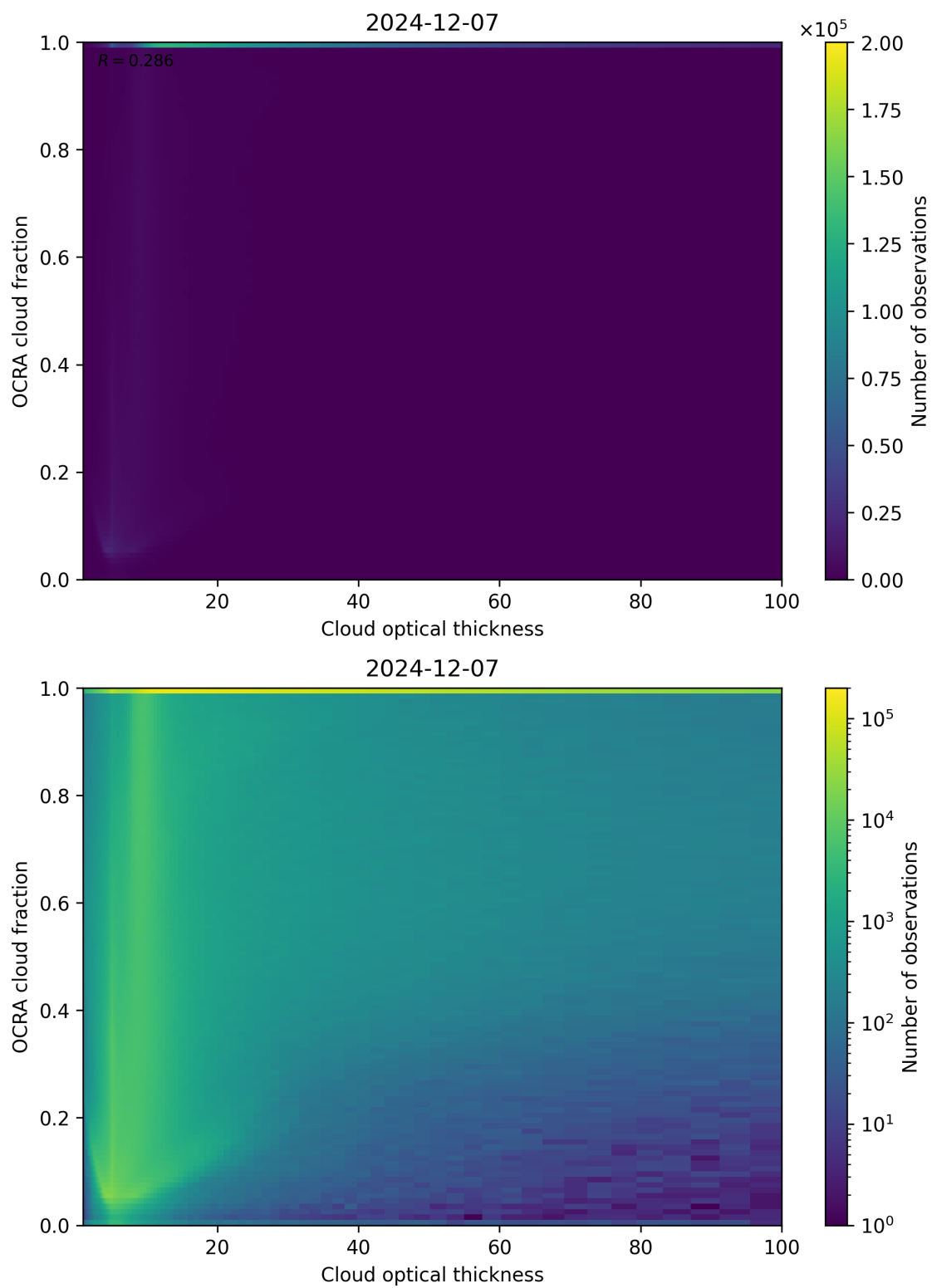
Figure 83: Scatter density plot of “Cloud optical thickness” against “OCRA cloud fraction” for 2024-12-06 to 2024-12-08.
