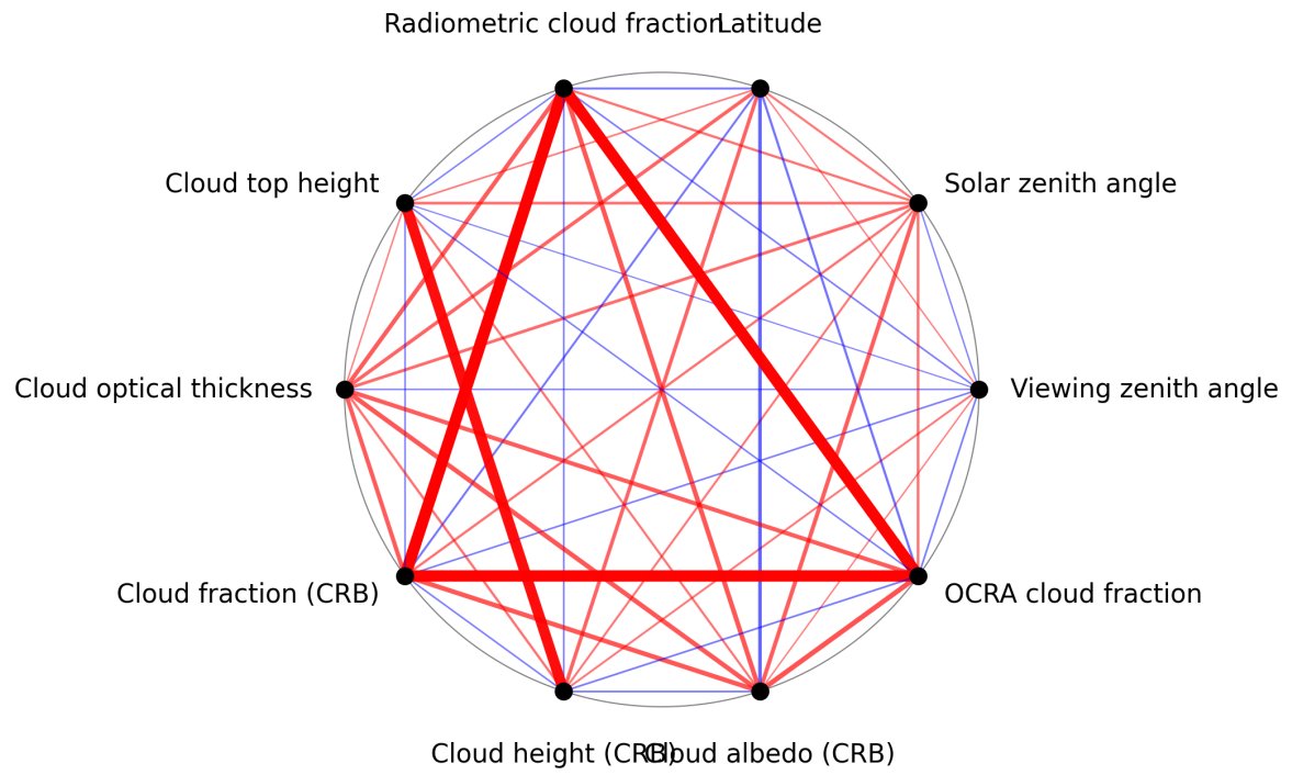
Figure 1: Map of correlation graph for 2024-12-06 to 2024-12-08.
