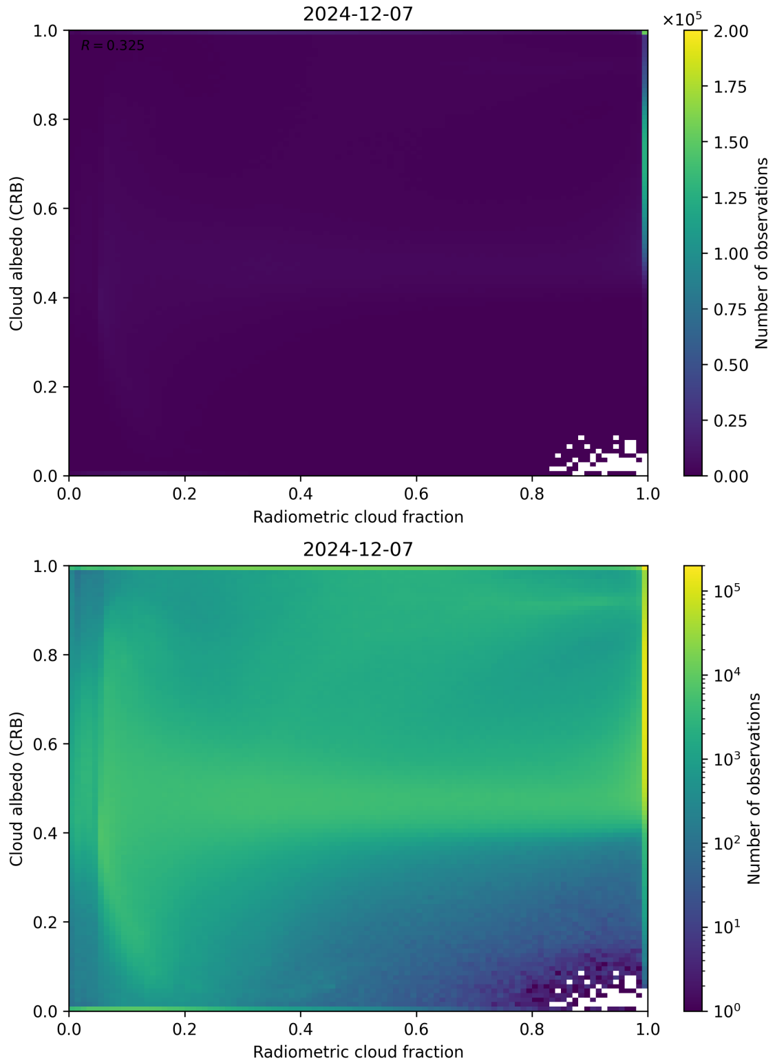
Figure 71: Scatter density plot of “Radiometric cloud fraction” against “Cloud albedo (CRB)” for 2024-12-06 to 2024-12-08.
