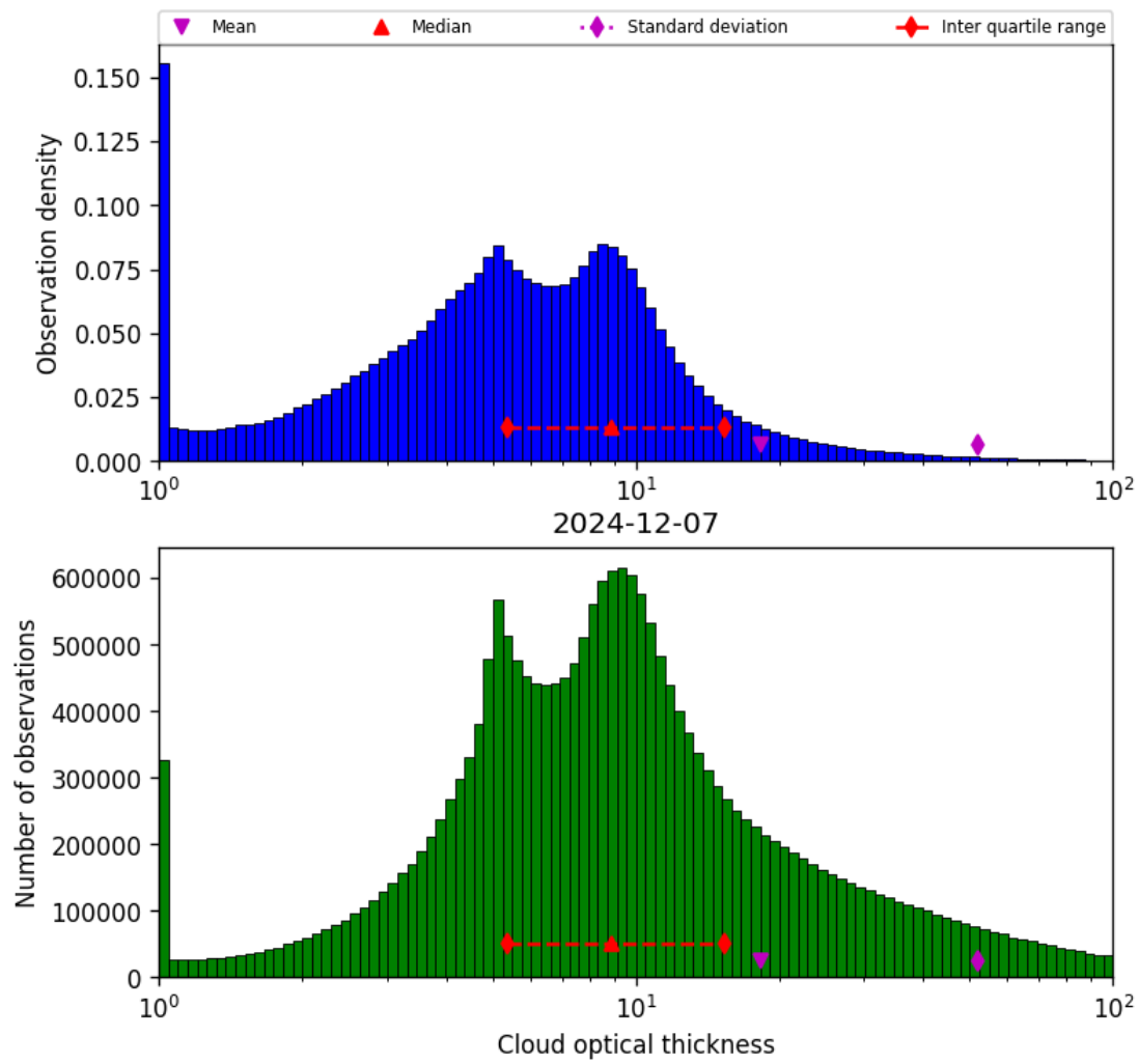
Figure 41: Histogram of “Cloud optical thickness” for 2024-12-06 to 2024-12-08
