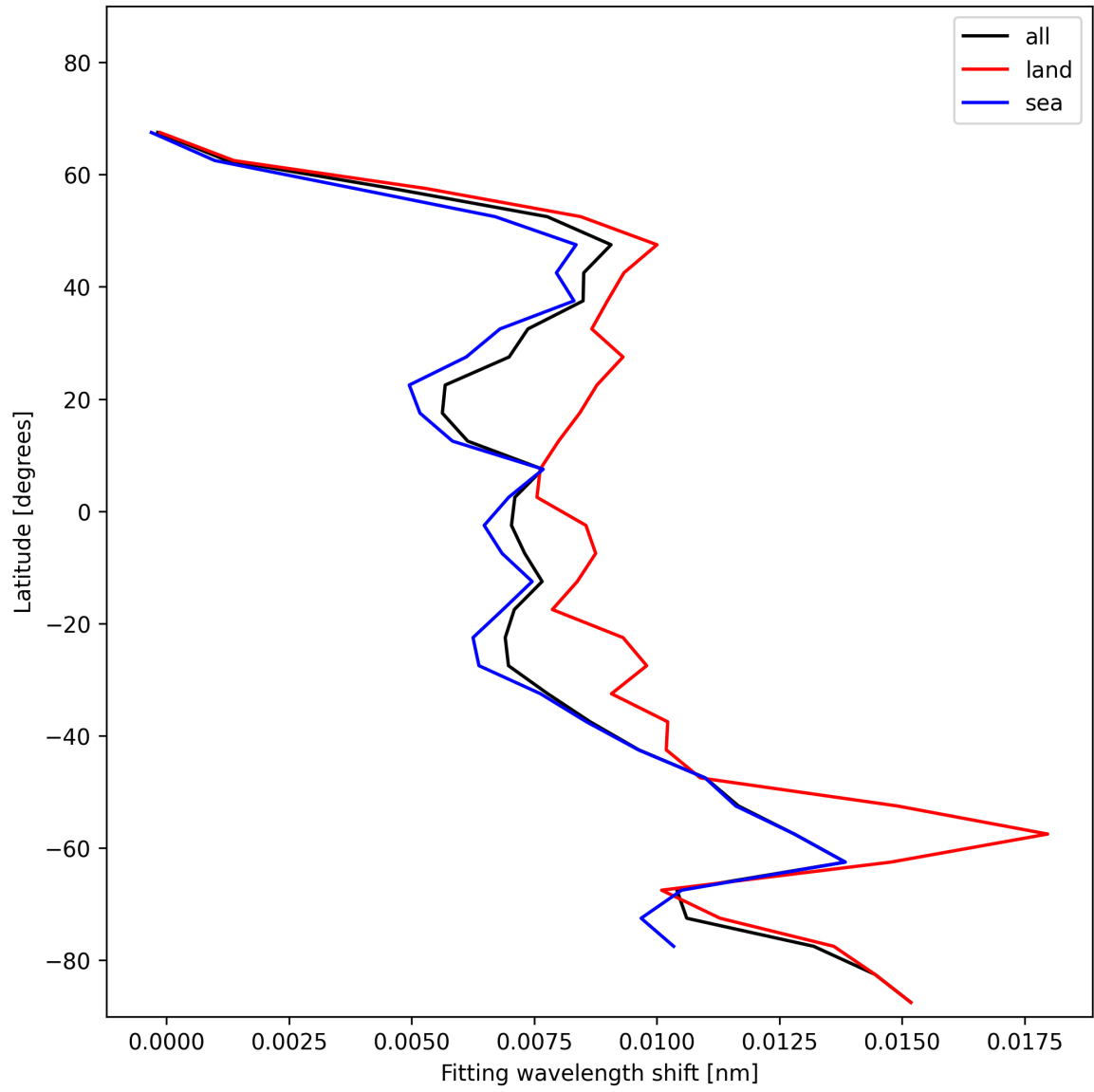
Figure 33: Zonal average of “Fitting wavelength shift” for 2024-12-06 to 2024-12-08.
