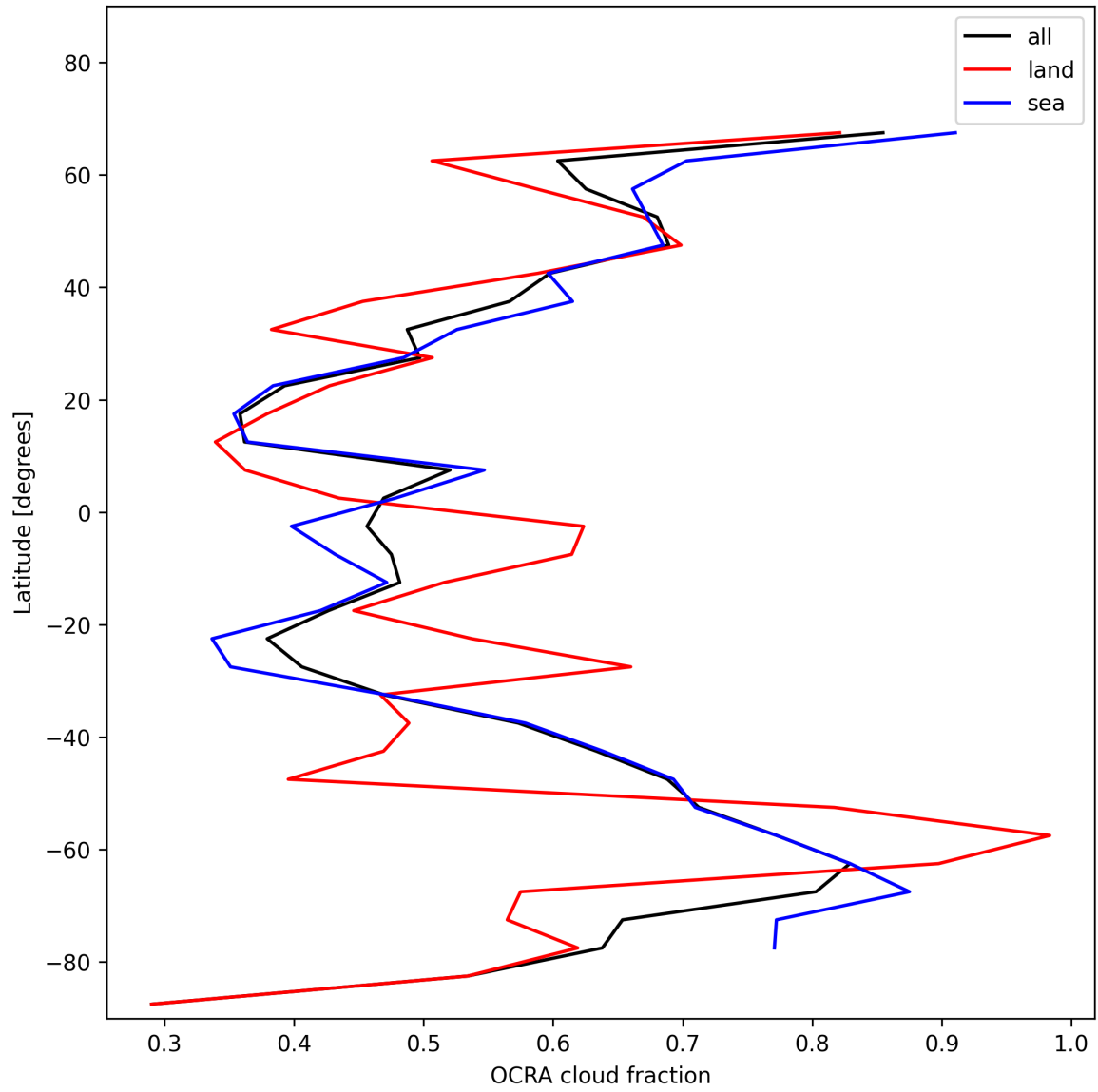
Figure 34: Zonal average of “OCRA cloud fraction” for 2024-12-06 to 2024-12-08.
