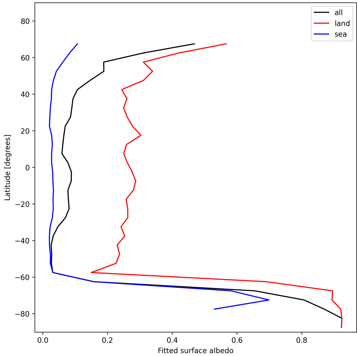
Figure 29: Zonal average of “Fitted surface albedo” for 2024-12-06 to 2024-12-08.
