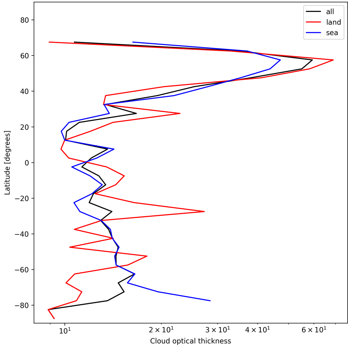
Figure 25: Zonal average of “Cloud optical thickness” for 2024-12-06 to 2024-12-08.
