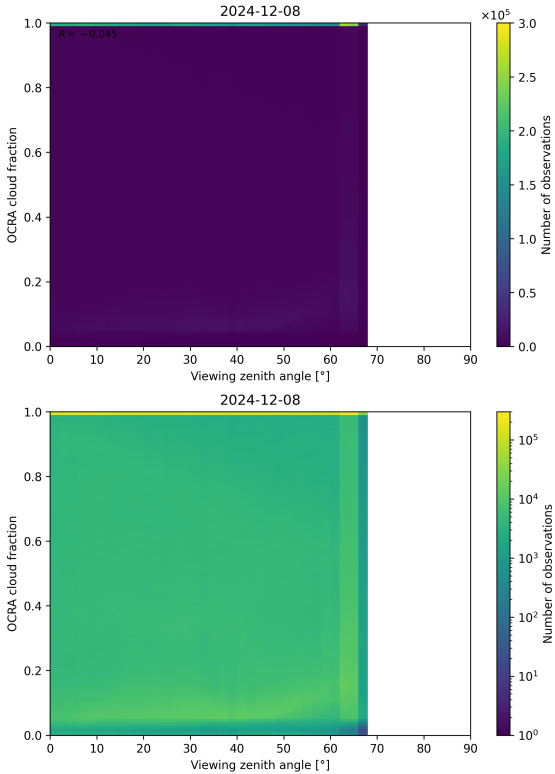
Figure 108: Scatter density plot of “Viewing zenith angle” against “OCRA cloud fraction” for 2024-12-07 to 2024-12-09.
