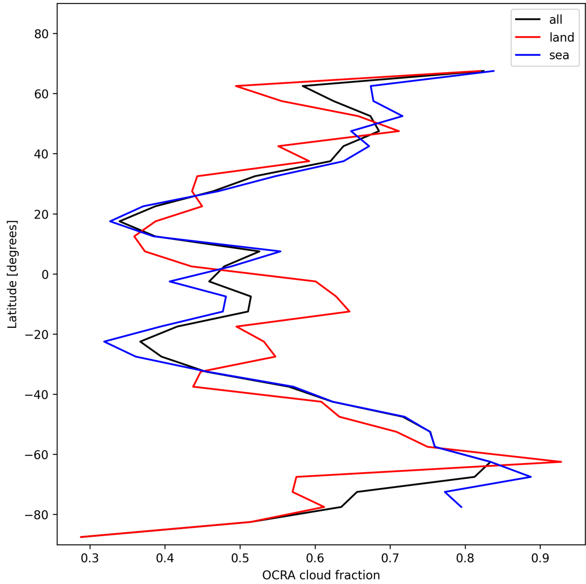
Figure 34: Zonal average of “OCRA cloud fraction” for 2024-12-07 to 2024-12-09.
