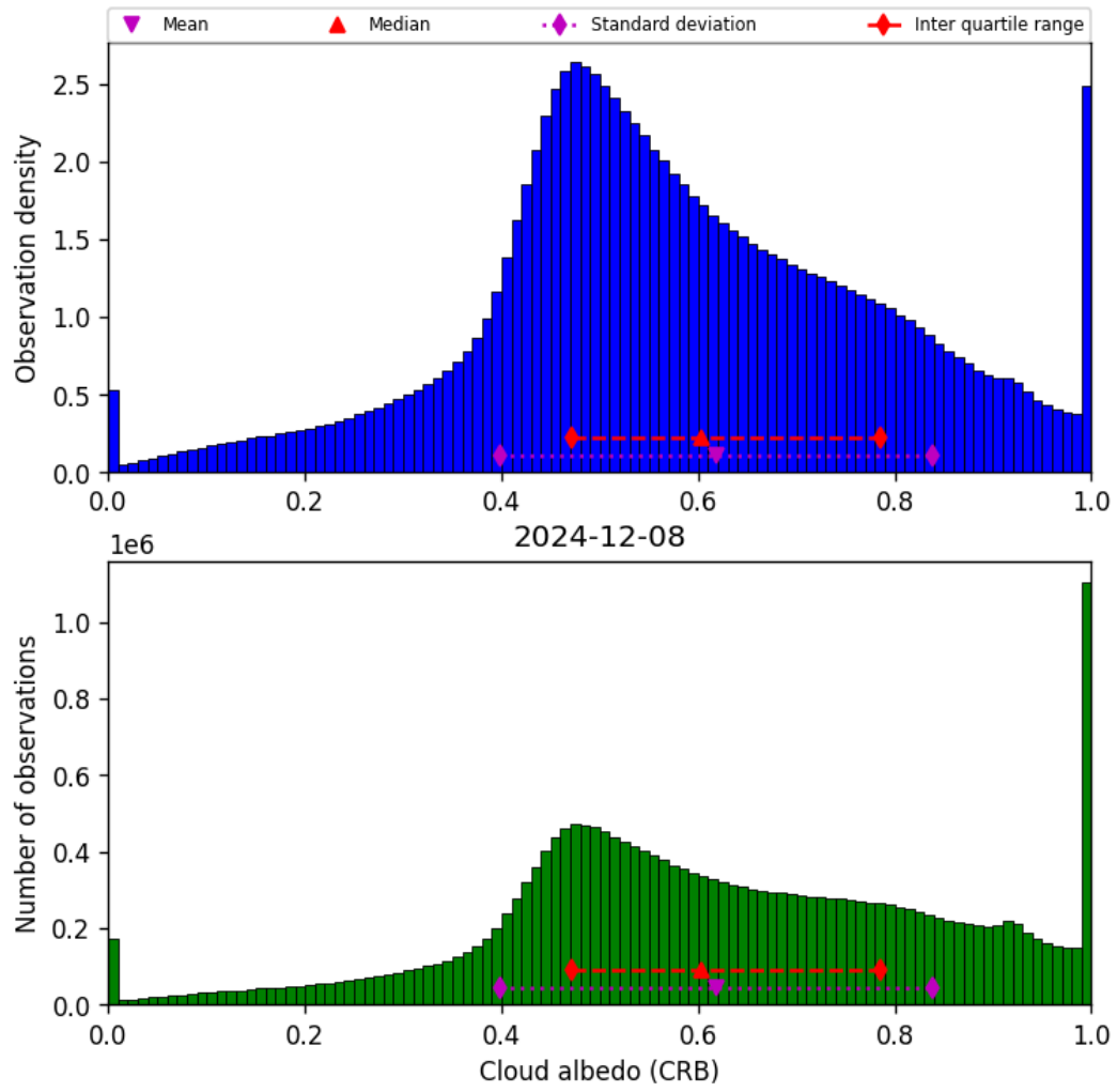
Figure 44: Histogram of “Cloud albedo (CRB)” for 2024-12-07 to 2024-12-09
