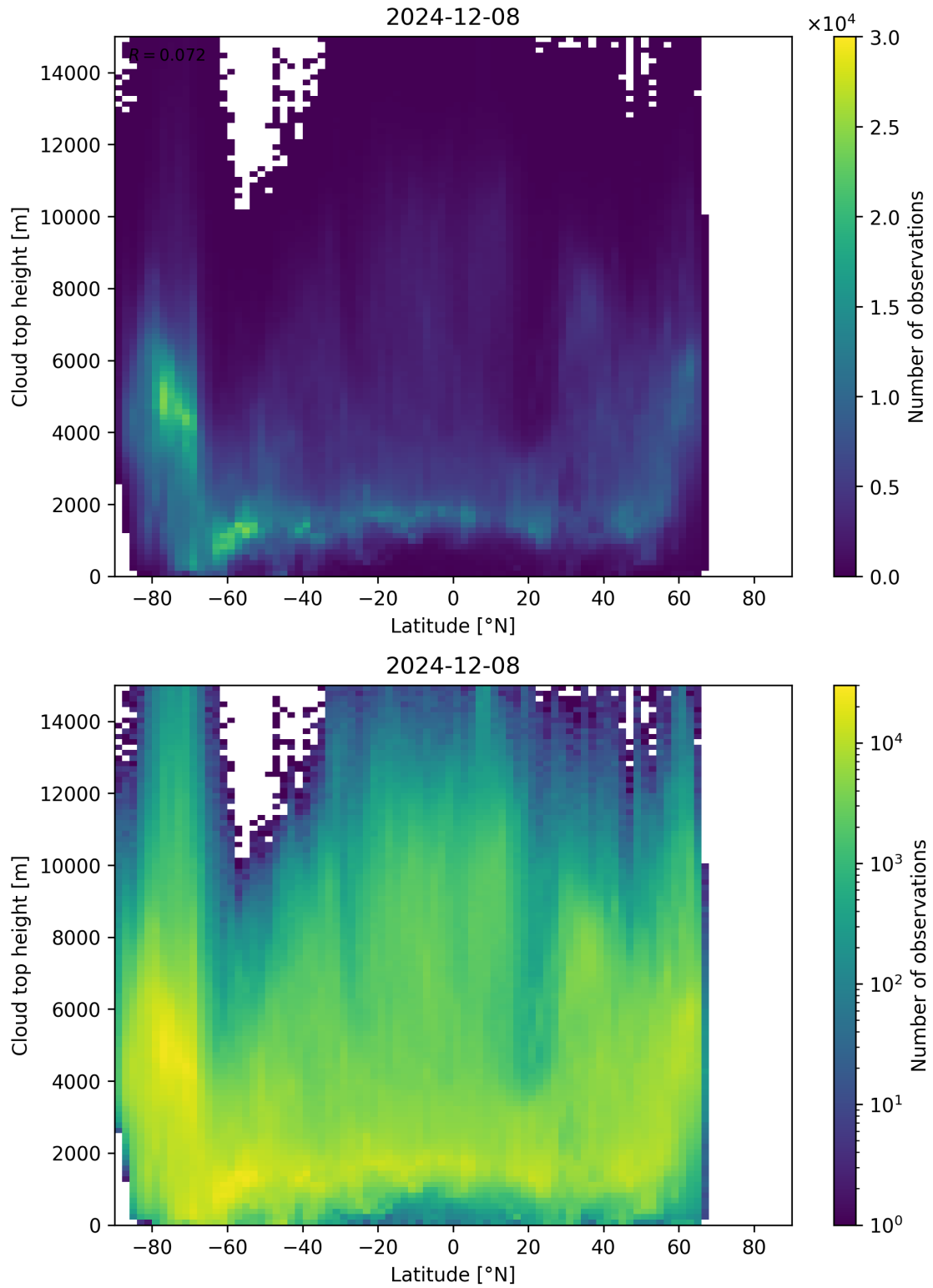
Figure 97: Scatter density plot of “Latitude” against “Cloud top height” for 2024-12-07 to 2024-12-09.
