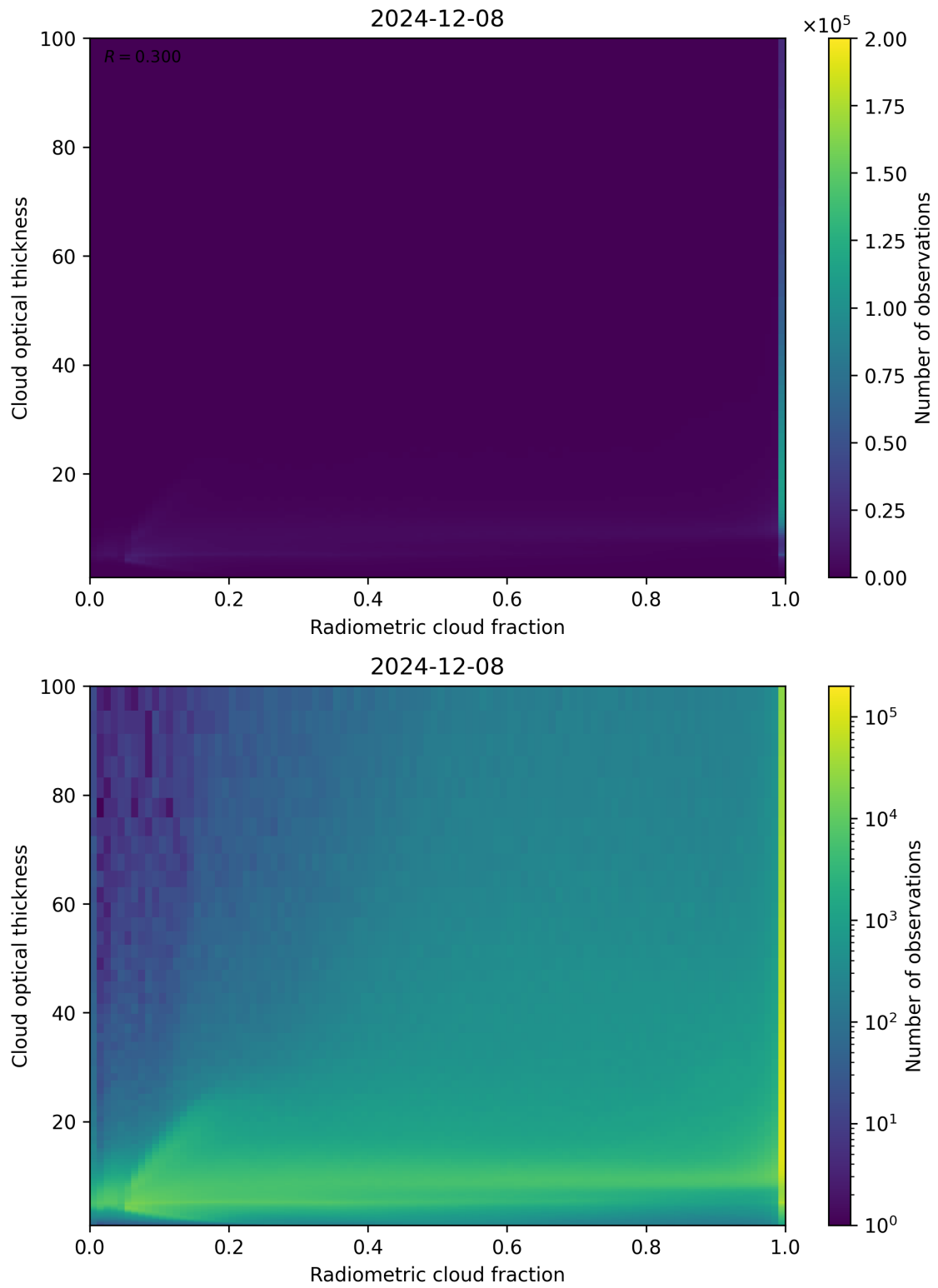
Figure 75: Scatter density plot of “Radiometric cloud fraction” against “Cloud optical thickness” for 2024-12-07 to 2024-12-09.
