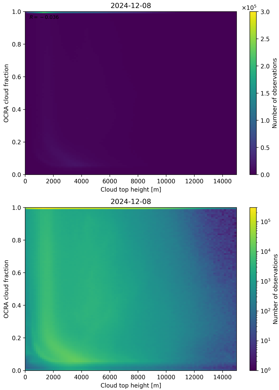
Figure 87: Scatter density plot of “Cloud top height” against “OCRA cloud fraction” for 2024-12-07 to 2024-12-09.
