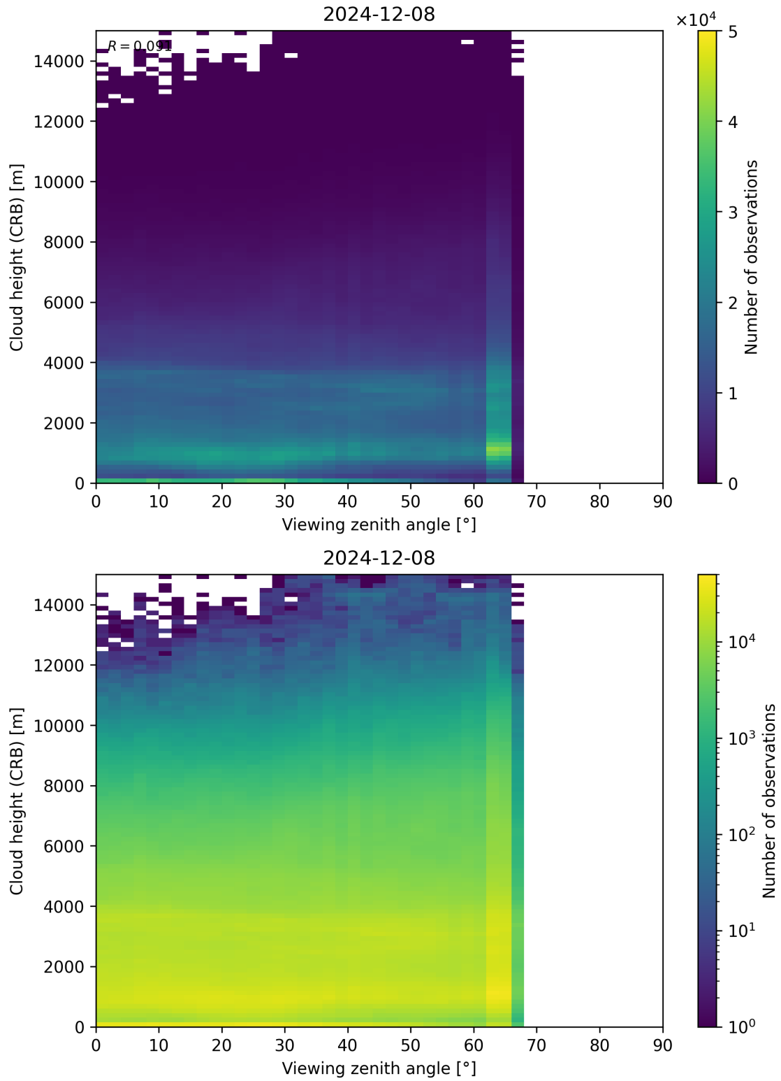
Figure 110: Scatter density plot of “Viewing zenith angle” against “Cloud height (CRB)” for 2024-12-07 to 2024-12-09.
