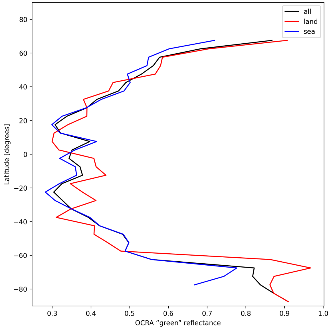
Figure 36: Zonal average of “OCRA “green” reflectance” for 2024-12-07 to 2024-12-09.
