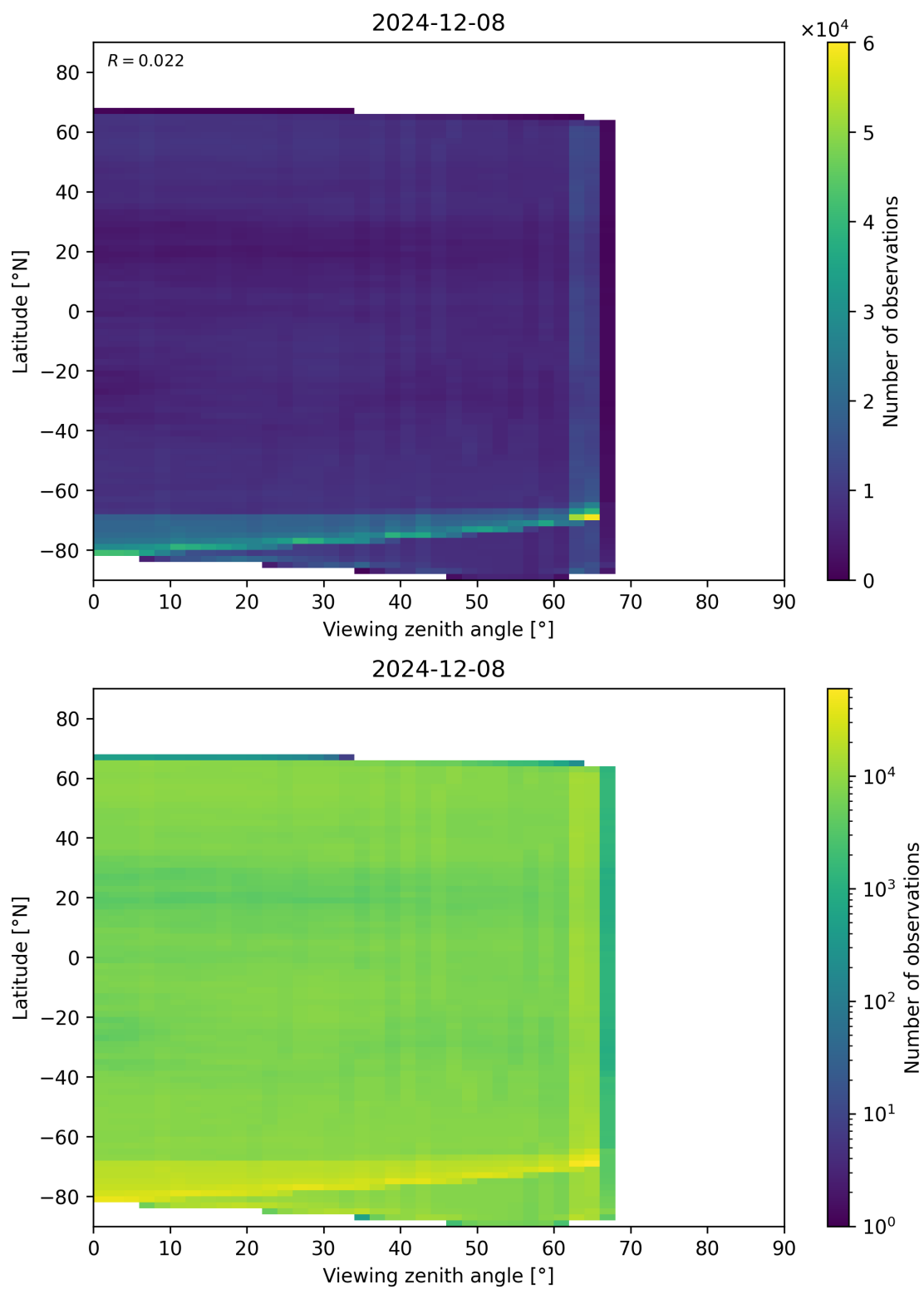
Figure 113: Scatter density plot of “Viewing zenith angle” against “Latitude” for 2024-12-07 to 2024-12-09.
