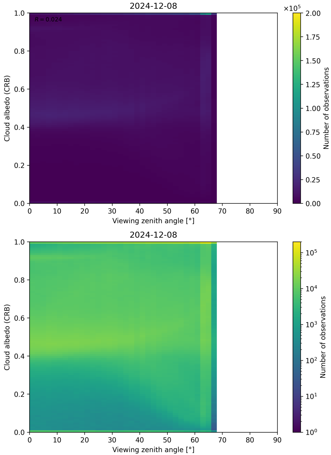
Figure 106: Scatter density plot of “Viewing zenith angle” against “Cloud albedo (CRB)” for 2024-12-07 to 2024-12-09.
