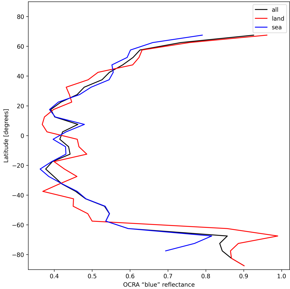
Figure 35: Zonal average of “OCRA “blue” reflectance” for 2024-12-07 to 2024-12-09.
