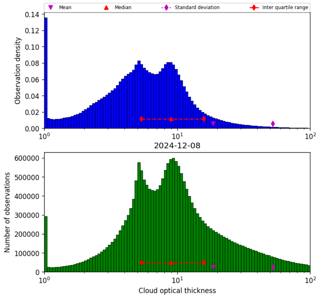
Figure 41: Histogram of “Cloud optical thickness” for 2024-12-07 to 2024-12-09
