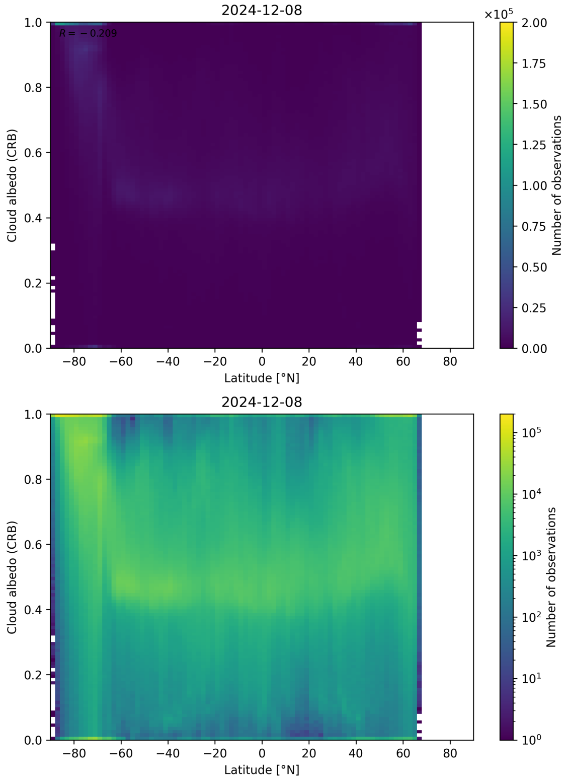
Figure 91: Scatter density plot of “Latitude” against “Cloud albedo (CRB)” for 2024-12-07 to 2024-12-09.
