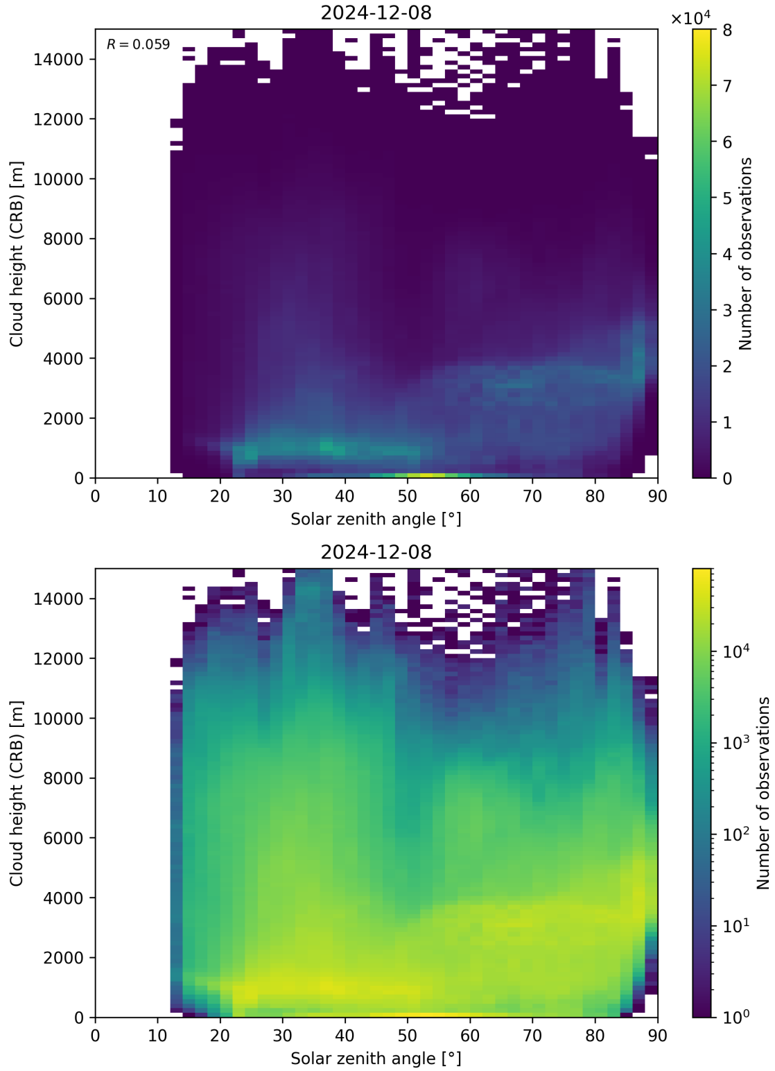
Figure 102: Scatter density plot of “Solar zenith angle” against “Cloud height (CRB)” for 2024-12-07 to 2024-12-09.
