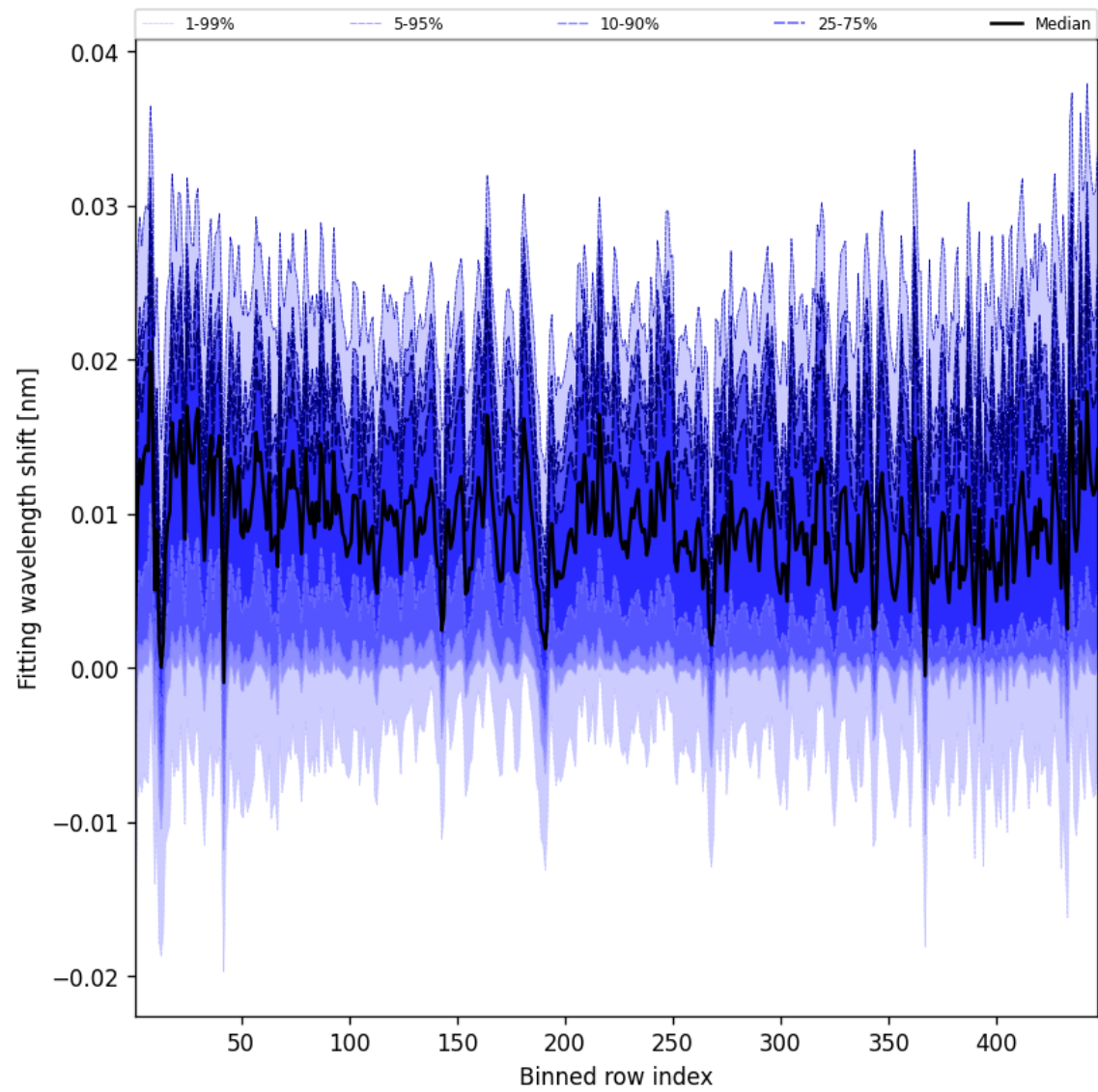
Figure 65: Along track statistics of “Fitting wavelength shift” for 2024-12-07 to 2024-12-09
