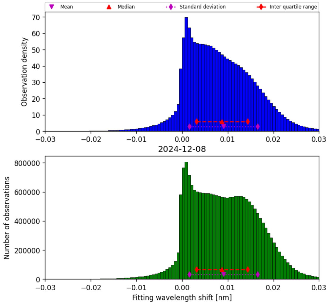
Figure 49: Histogram of “Fitting wavelength shift” for 2024-12-07 to 2024-12-09
