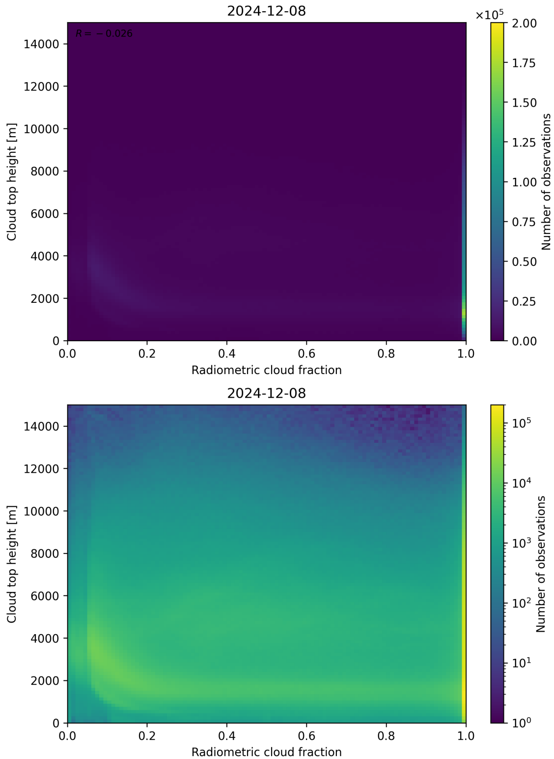
Figure 76: Scatter density plot of “Radiometric cloud fraction” against “Cloud top height” for 2024-12-07 to 2024-12-09.
