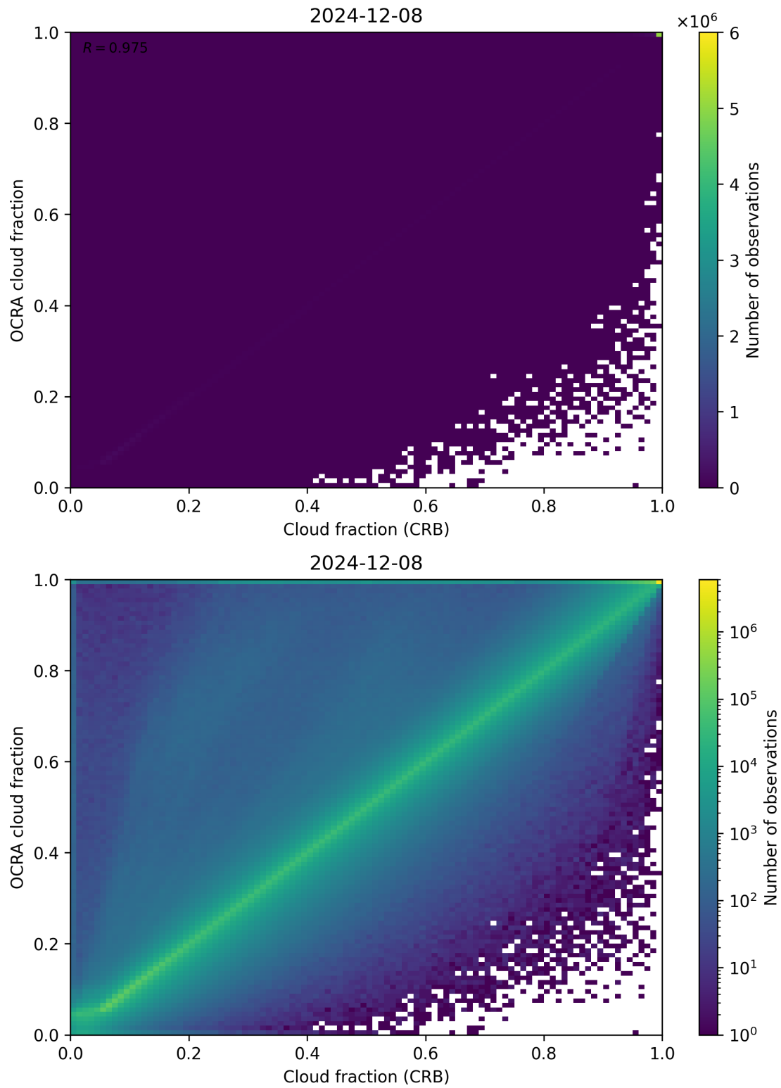
Figure 78: Scatter density plot of “Cloud fraction (CRB)” against “OCRA cloud fraction” for 2024-12-07 to 2024-12-09.
