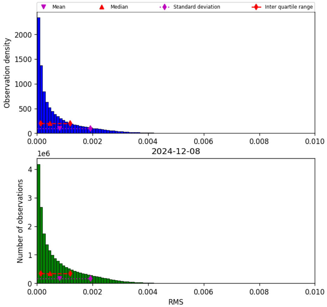
Figure 47: Histogram of “RMS” for 2024-12-07 to 2024-12-09
