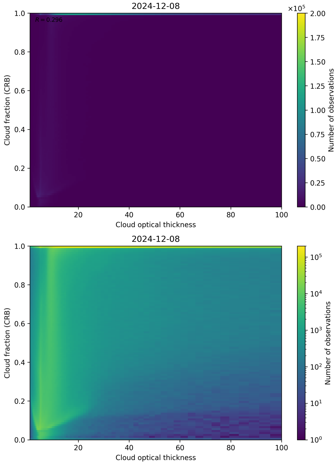
Figure 84: Scatter density plot of “Cloud optical thickness” against “Cloud fraction (CRB)” for 2024-12-07 to 2024-12-09.
