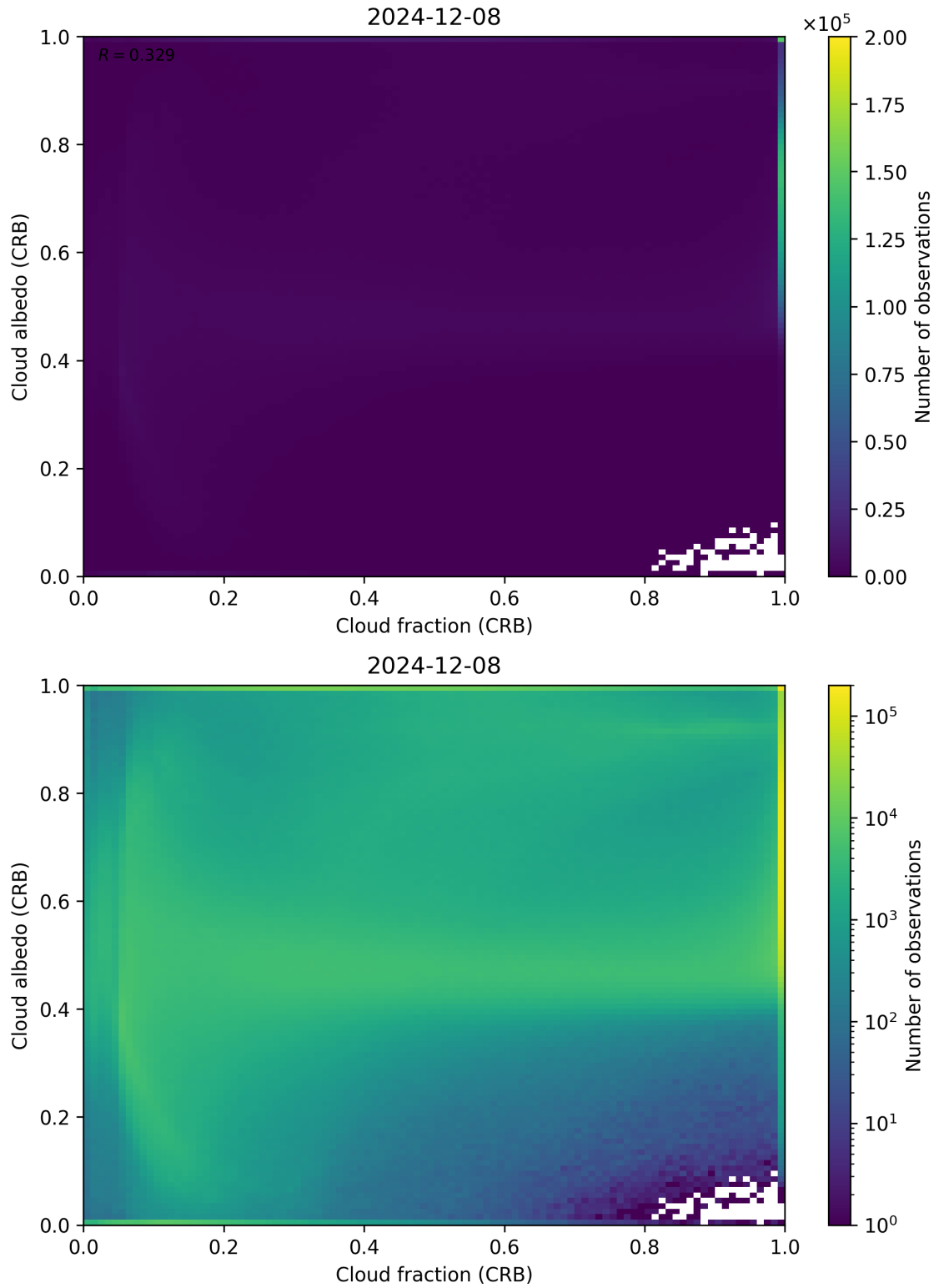
Figure 77: Scatter density plot of “Cloud fraction (CRB)” against “Cloud albedo (CRB)” for 2024-12-07 to 2024-12-09.
