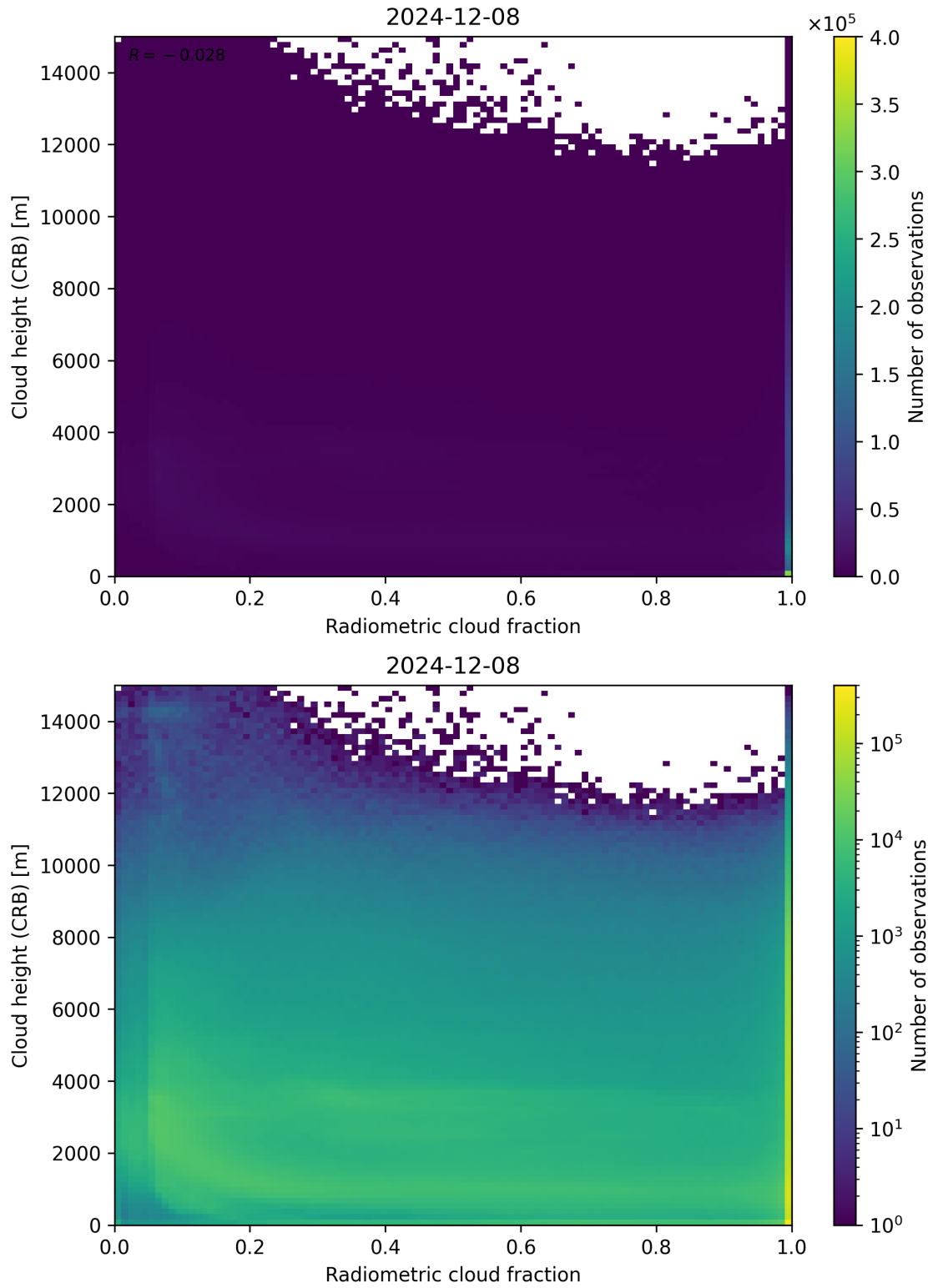
Figure 74: Scatter density plot of “Radiometric cloud fraction” against “Cloud height (CRB)” for 2024-12-07 to 2024-12-09.
