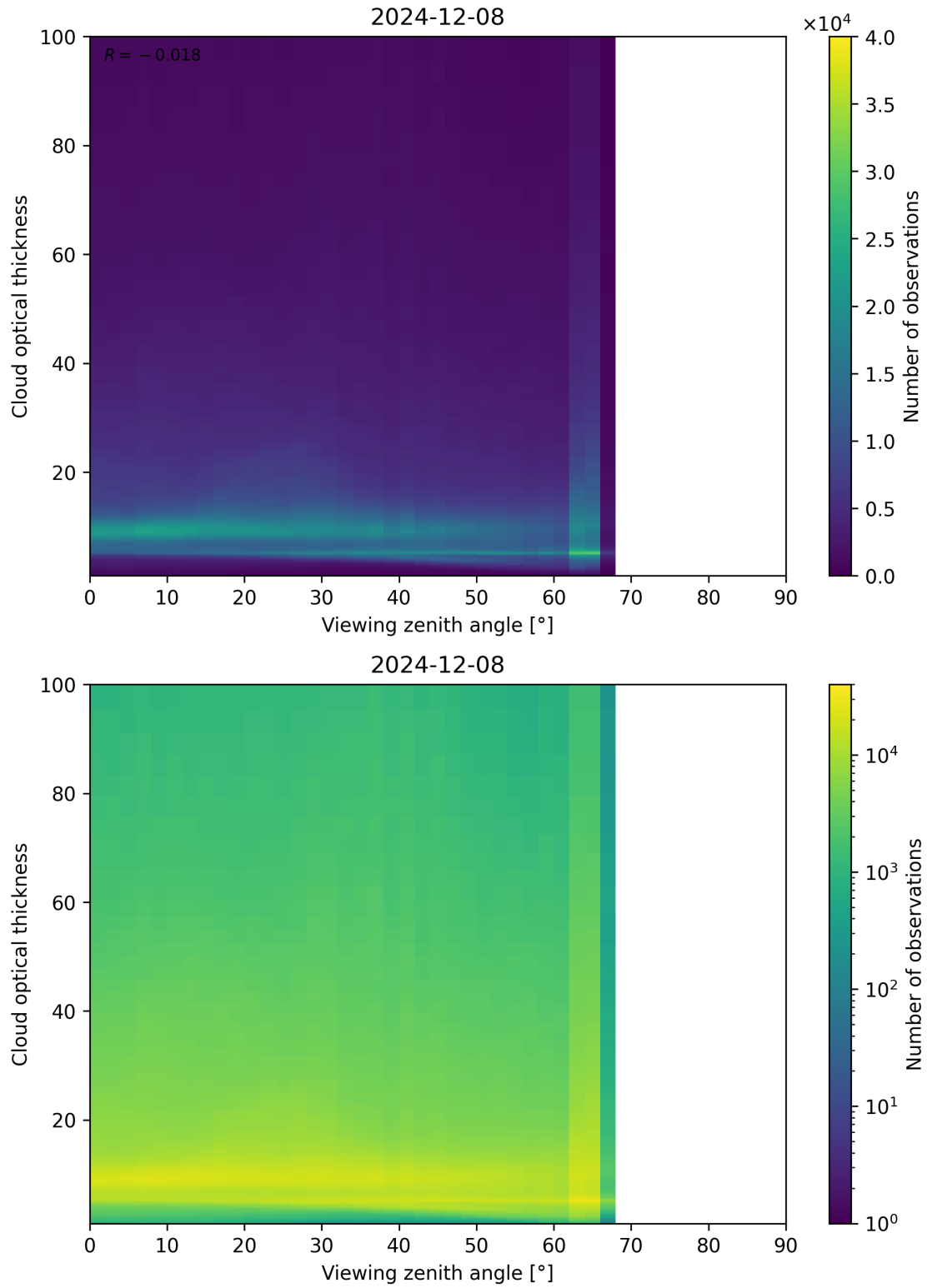
Figure 111: Scatter density plot of “Viewing zenith angle” against “Cloud optical thickness” for 2024-12-07 to 2024-12-09.
