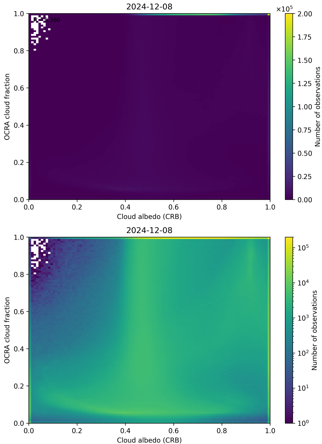
Figure 70: Scatter density plot of “Cloud albedo (CRB)” against “OCRA cloud fraction” for 2024-12-07 to 2024-12-09.
