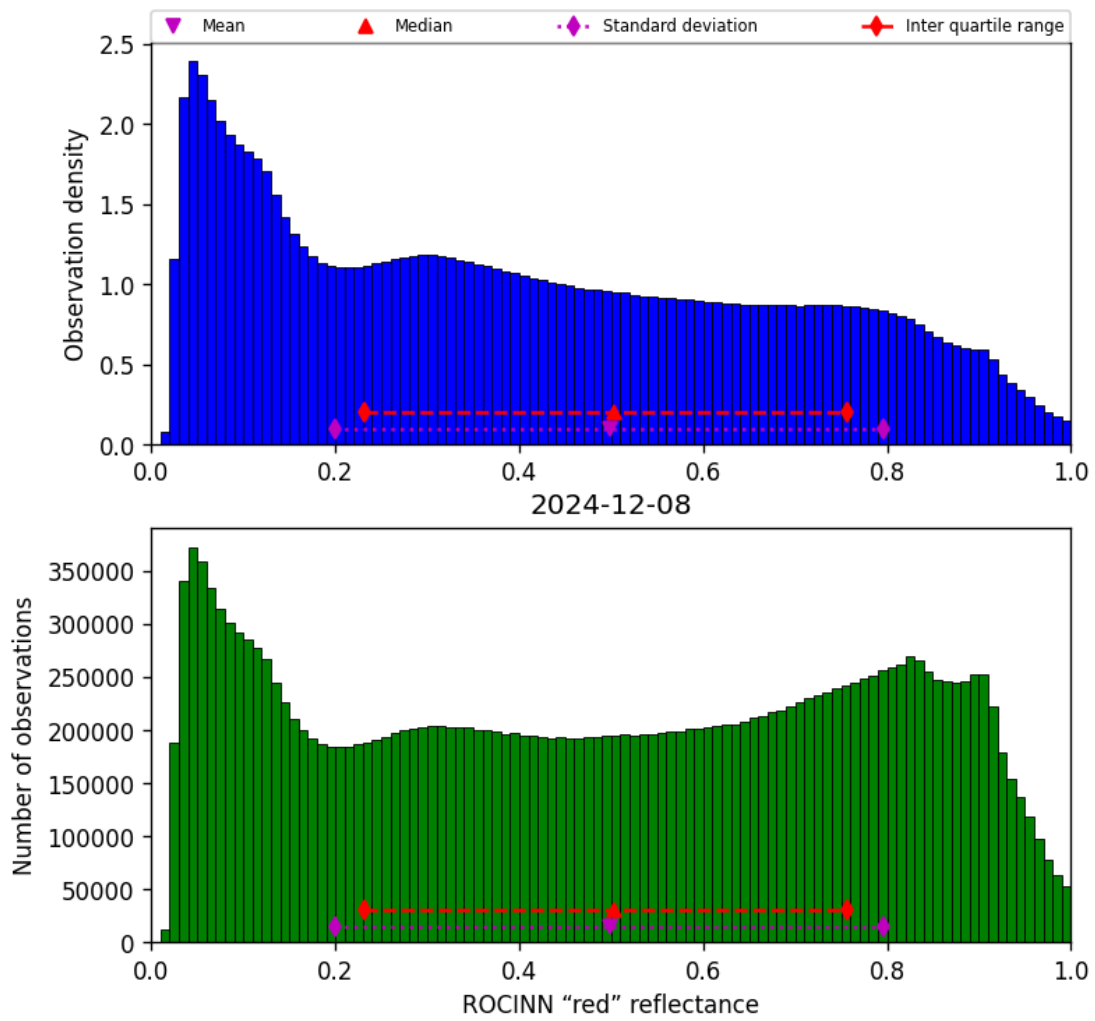
Figure 53: Histogram of “ROCINN “red” reflectance” for 2024-12-07 to 2024-12-09
