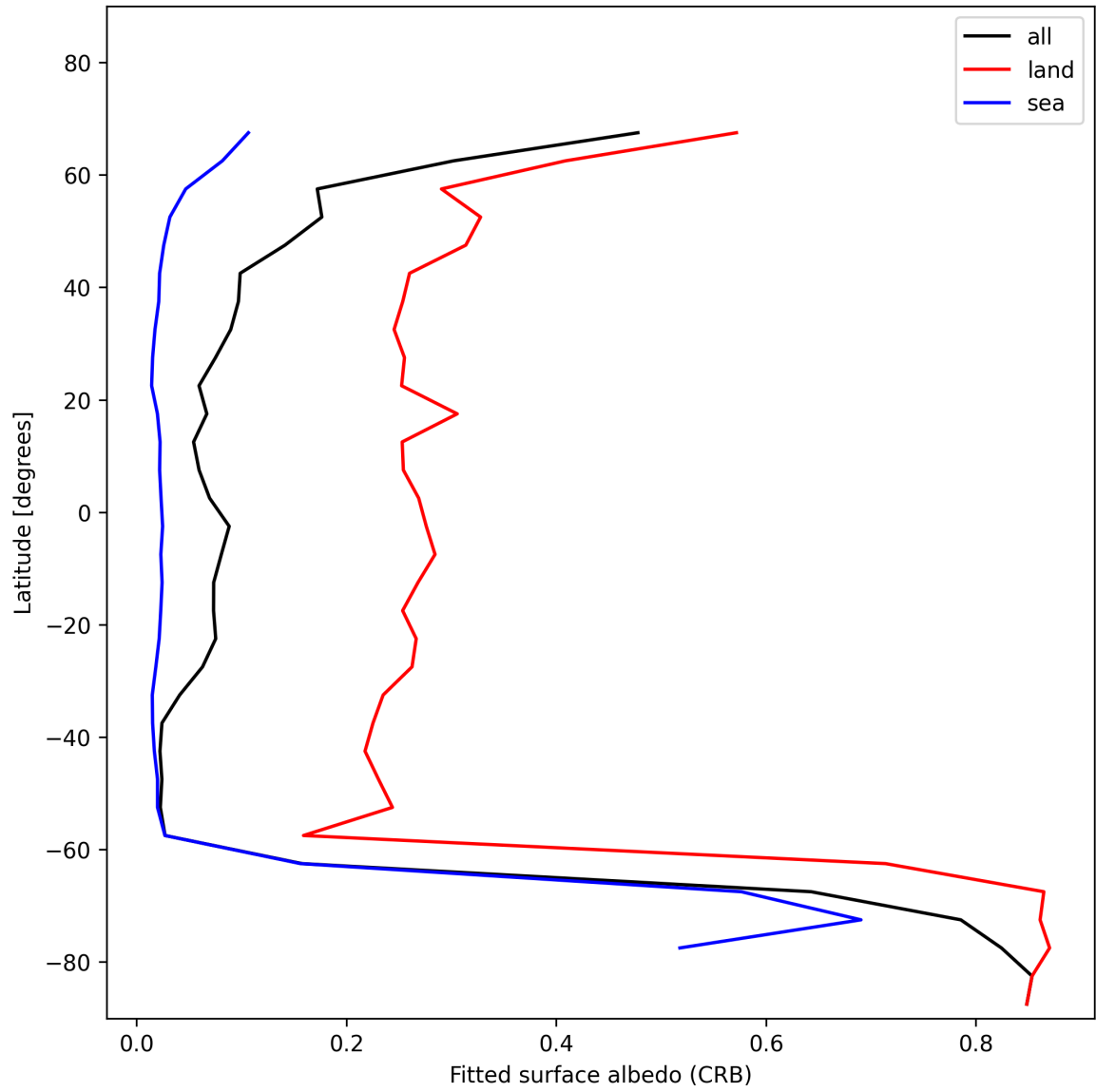
Figure 30: Zonal average of “Fitted surface albedo (CRB)” for 2024-12-07 to 2024-12-09.
