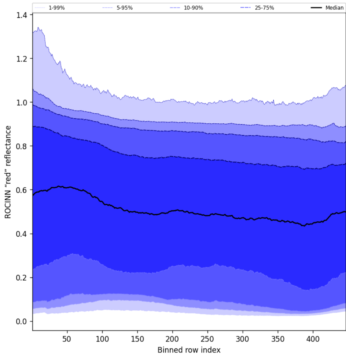
Figure 69: Along track statistics of “ROCINN “red” reflectance” for 2024-12-07 to 2024-12-09
