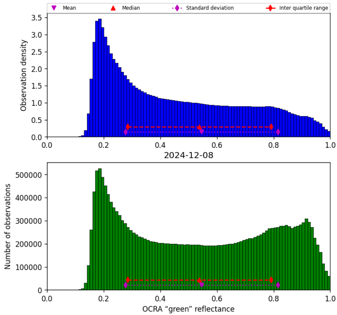
Figure 52: Histogram of “OCRA “green” reflectance” for 2024-12-07 to 2024-12-09
