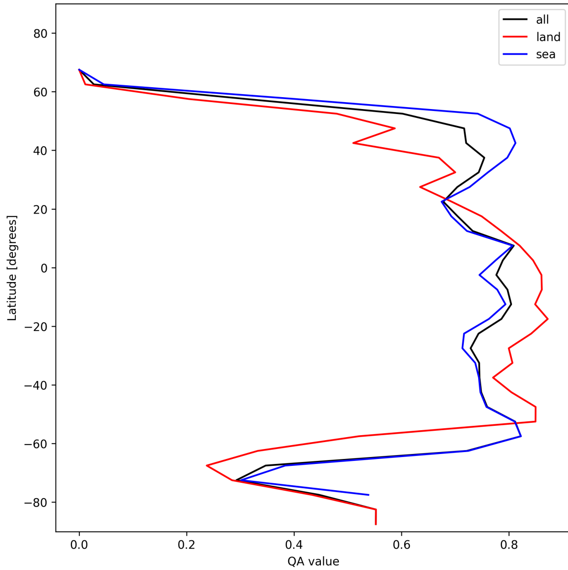
Figure 22: Zonal average of “QA value” for 2024-12-07 to 2024-12-09.
