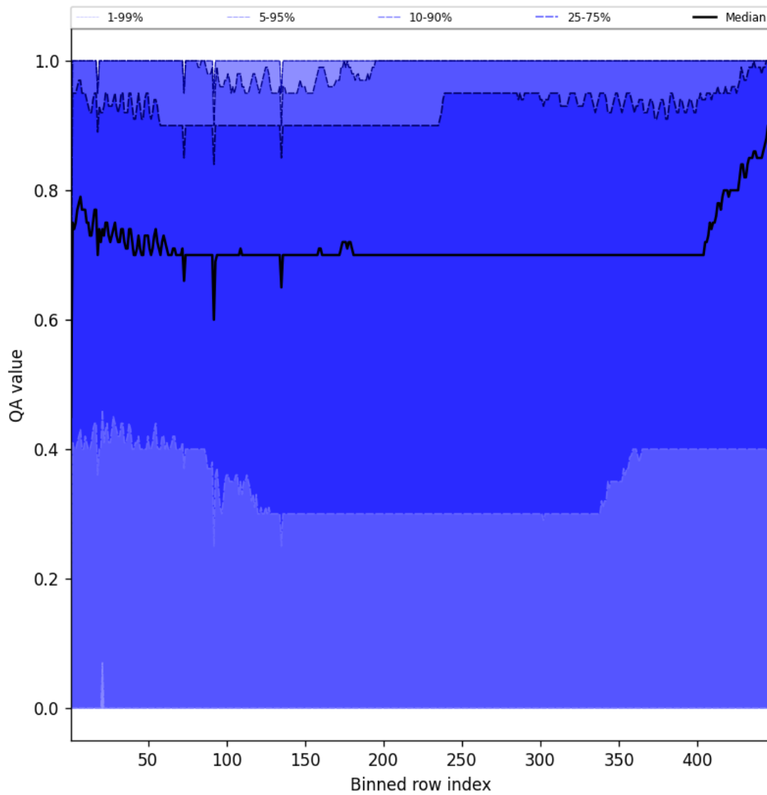
Figure 54: Along track statistics of “QA value” for 2024-12-07 to 2024-12-09
