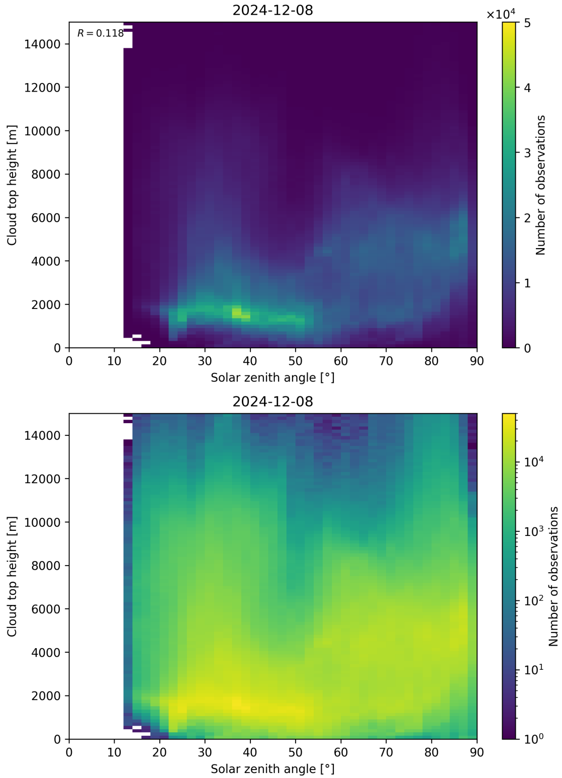
Figure 104: Scatter density plot of “Solar zenith angle” against “Cloud top height” for 2024-12-07 to 2024-12-09.
