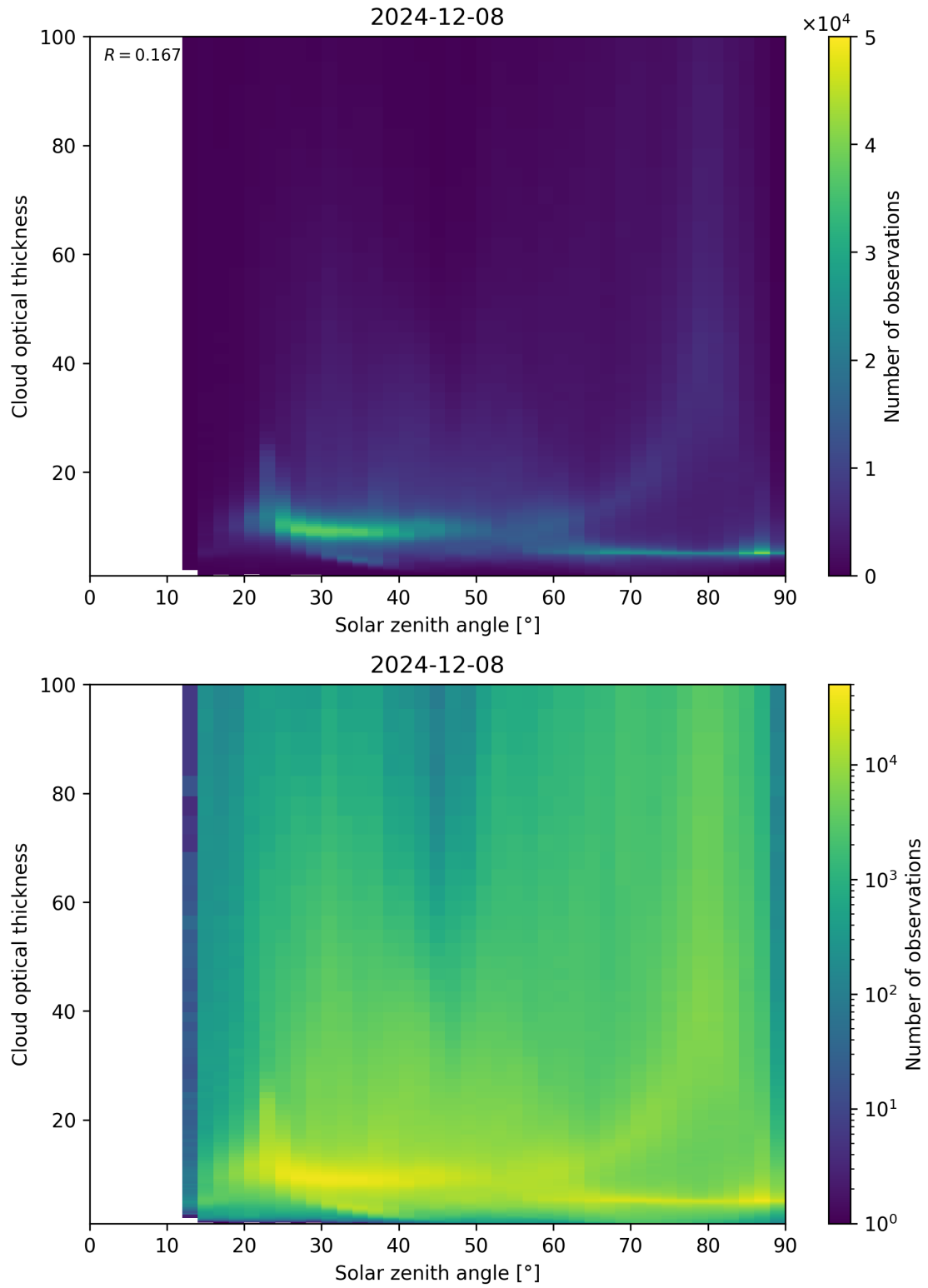
Figure 103: Scatter density plot of “Solar zenith angle” against “Cloud optical thickness” for 2024-12-07 to 2024-12-09.
