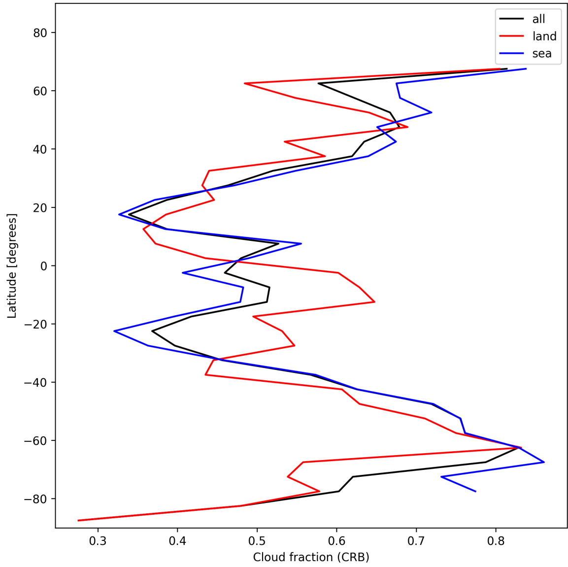
Figure 26: Zonal average of “Cloud fraction (CRB)” for 2024-12-07 to 2024-12-09.
