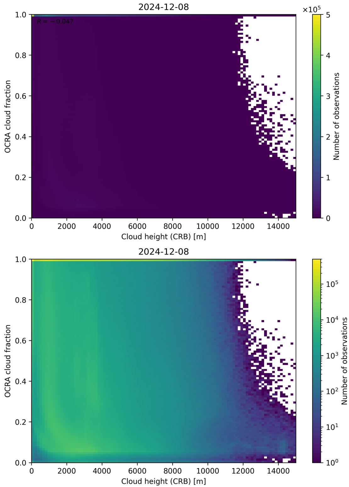
Figure 81: Scatter density plot of “Cloud height (CRB)” against “OCRA cloud fraction” for 2024-12-07 to 2024-12-09.
