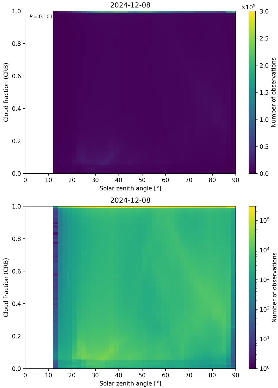
Figure 101: Scatter density plot of “Solar zenith angle” against “Cloud fraction (CRB)” for 2024-12-07 to 2024-12-09.
