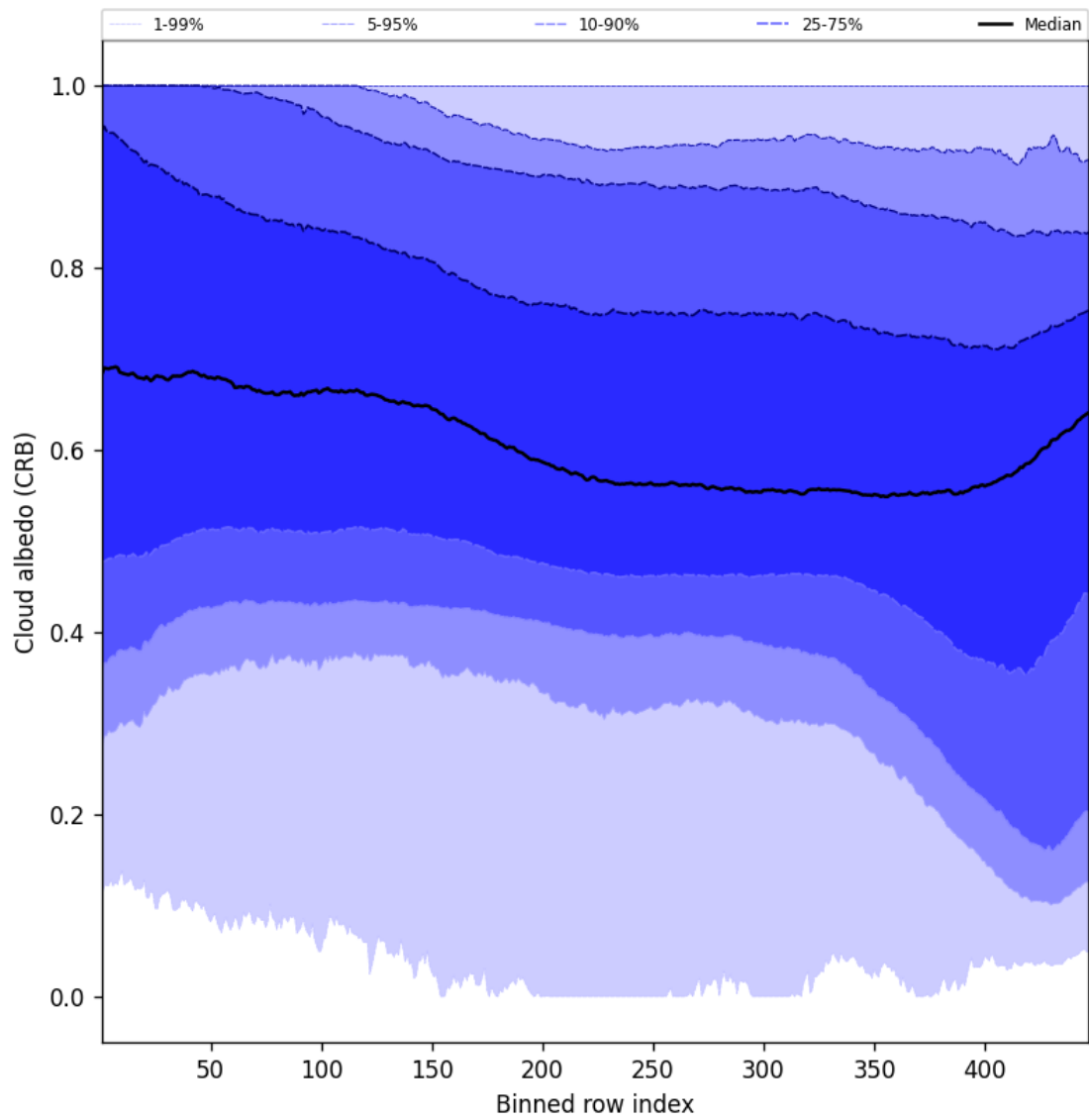
Figure 60: Along track statistics of “Cloud albedo (CRB)” for 2024-12-07 to 2024-12-09
