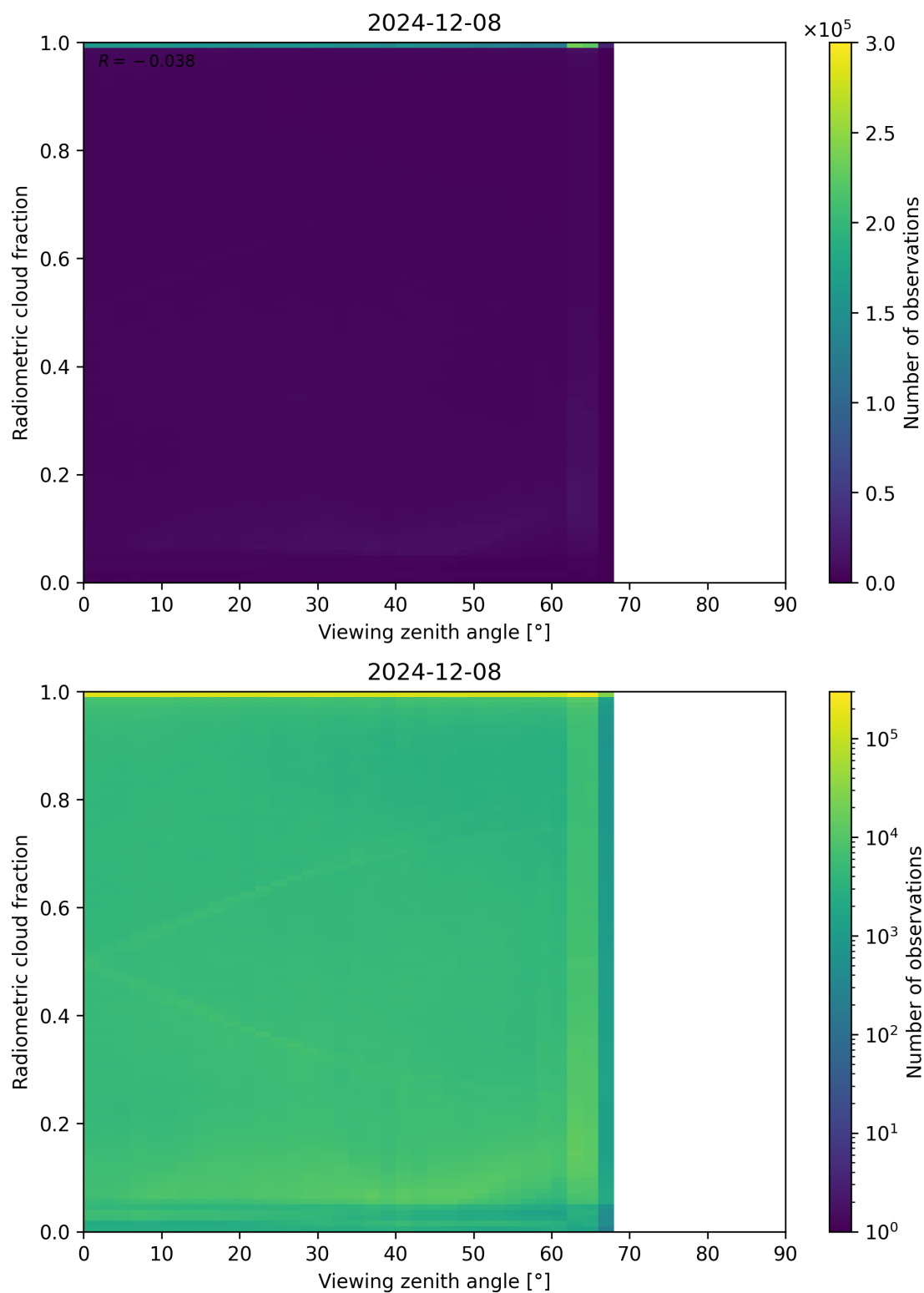
Figure 107: Scatter density plot of “Viewing zenith angle” against “Radiometric cloud fraction” for 2024-12-07 to 2024-12-09.
