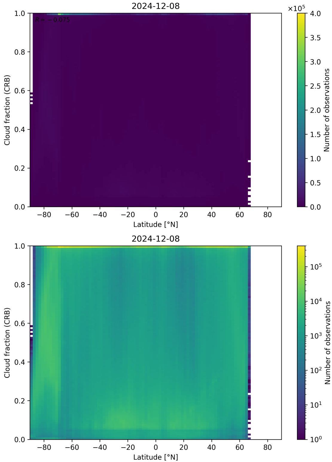
Figure 94: Scatter density plot of “Latitude” against “Cloud fraction (CRB)” for 2024-12-07 to 2024-12-09.
