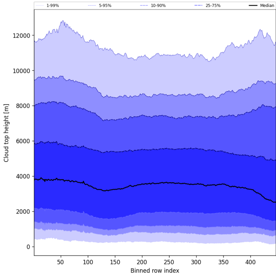
Figure 56: Along track statistics of “Cloud top height” for 2024-12-07 to 2024-12-09
