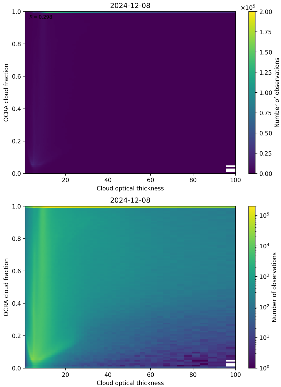
Figure 83: Scatter density plot of “Cloud optical thickness” against “OCRA cloud fraction” for 2024-12-07 to 2024-12-09.
