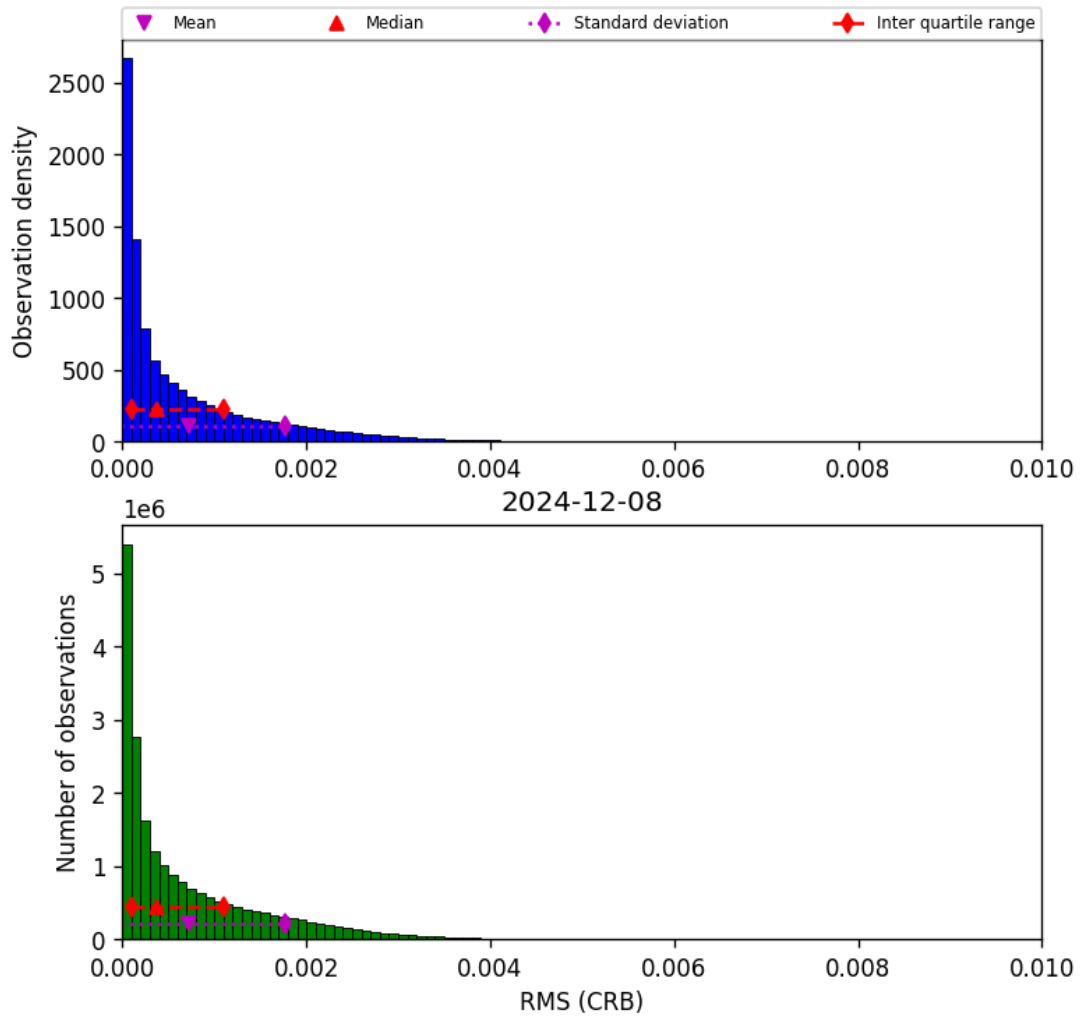
Figure 48: Histogram of “RMS (CRB)” for 2024-12-07 to 2024-12-09
