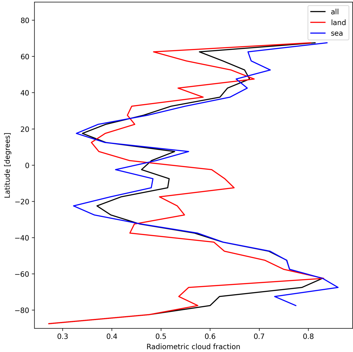
Figure 23: Zonal average of “Radiometric cloud fraction” for 2024-12-07 to 2024-12-09.
