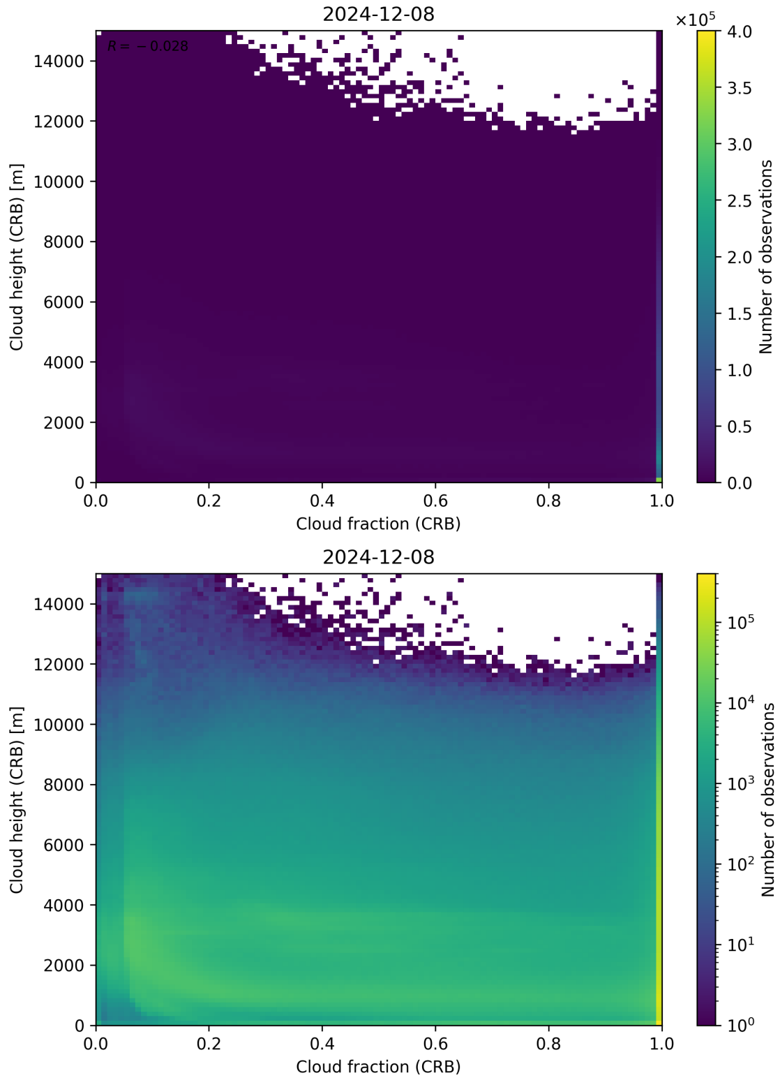
Figure 79: Scatter density plot of “Cloud fraction (CRB)” against “Cloud height (CRB)” for 2024-12-07 to 2024-12-09.
