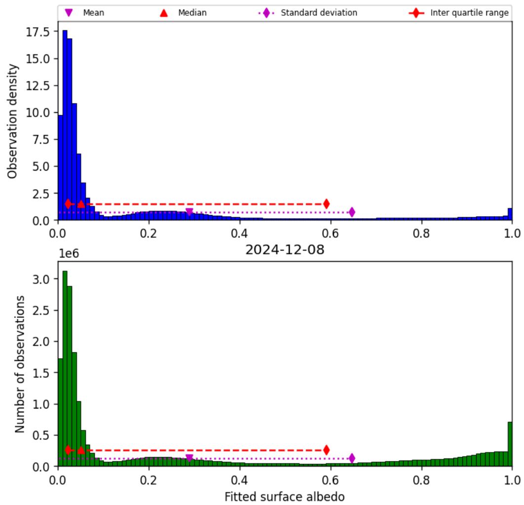
Figure 45: Histogram of “Fitted surface albedo” for 2024-12-07 to 2024-12-09
