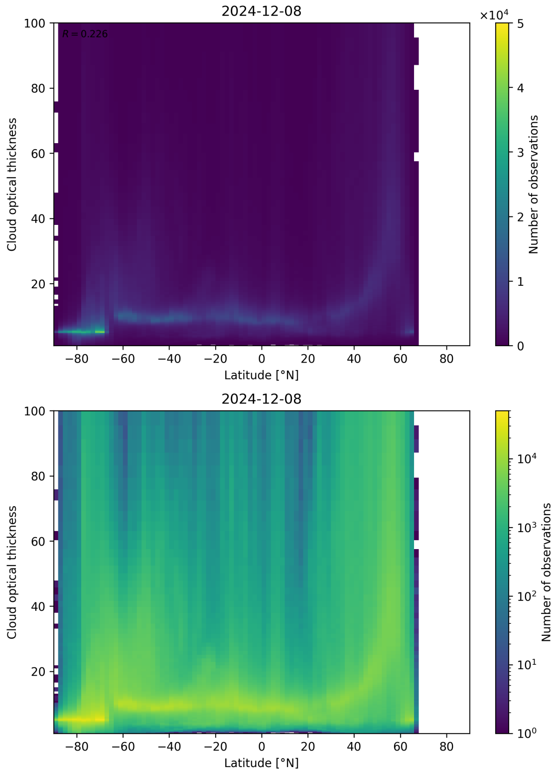
Figure 96: Scatter density plot of “Latitude” against “Cloud optical thickness” for 2024-12-07 to 2024-12-09.
