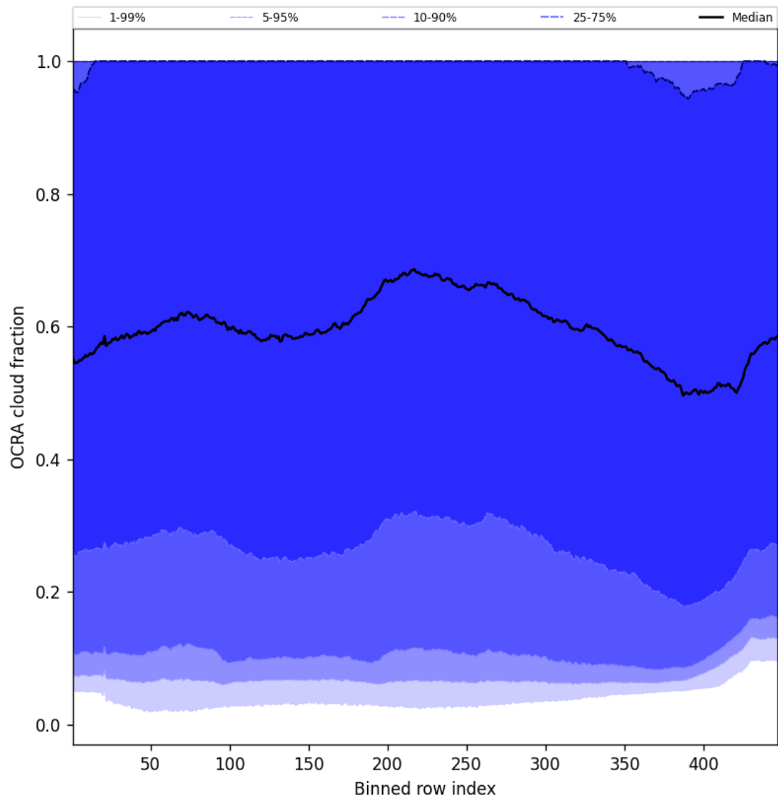
Figure 66: Along track statistics of “OCRA cloud fraction” for 2024-12-07 to 2024-12-09
