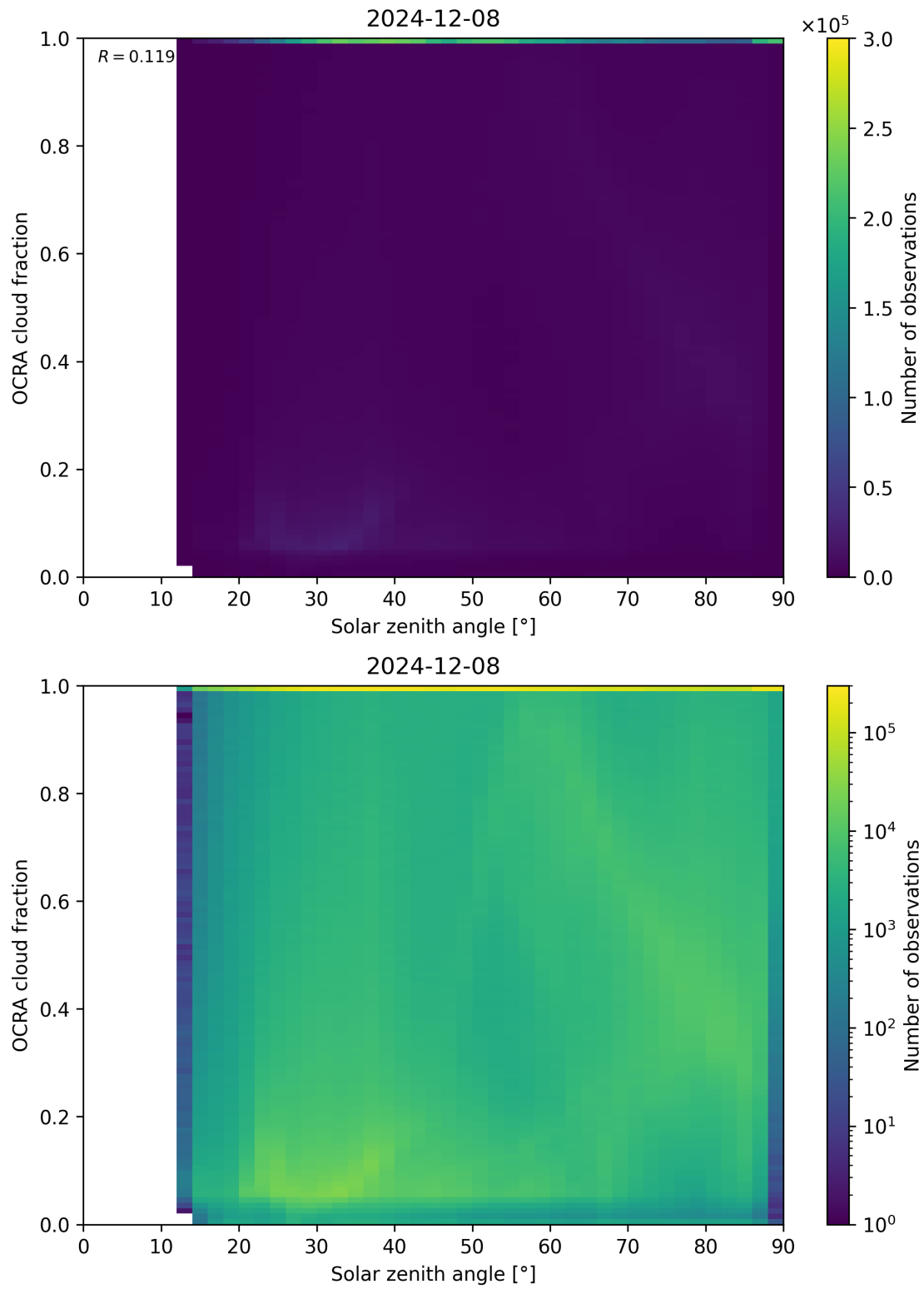
Figure 100: Scatter density plot of “Solar zenith angle” against “OCRA cloud fraction” for 2024-12-07 to 2024-12-09.
