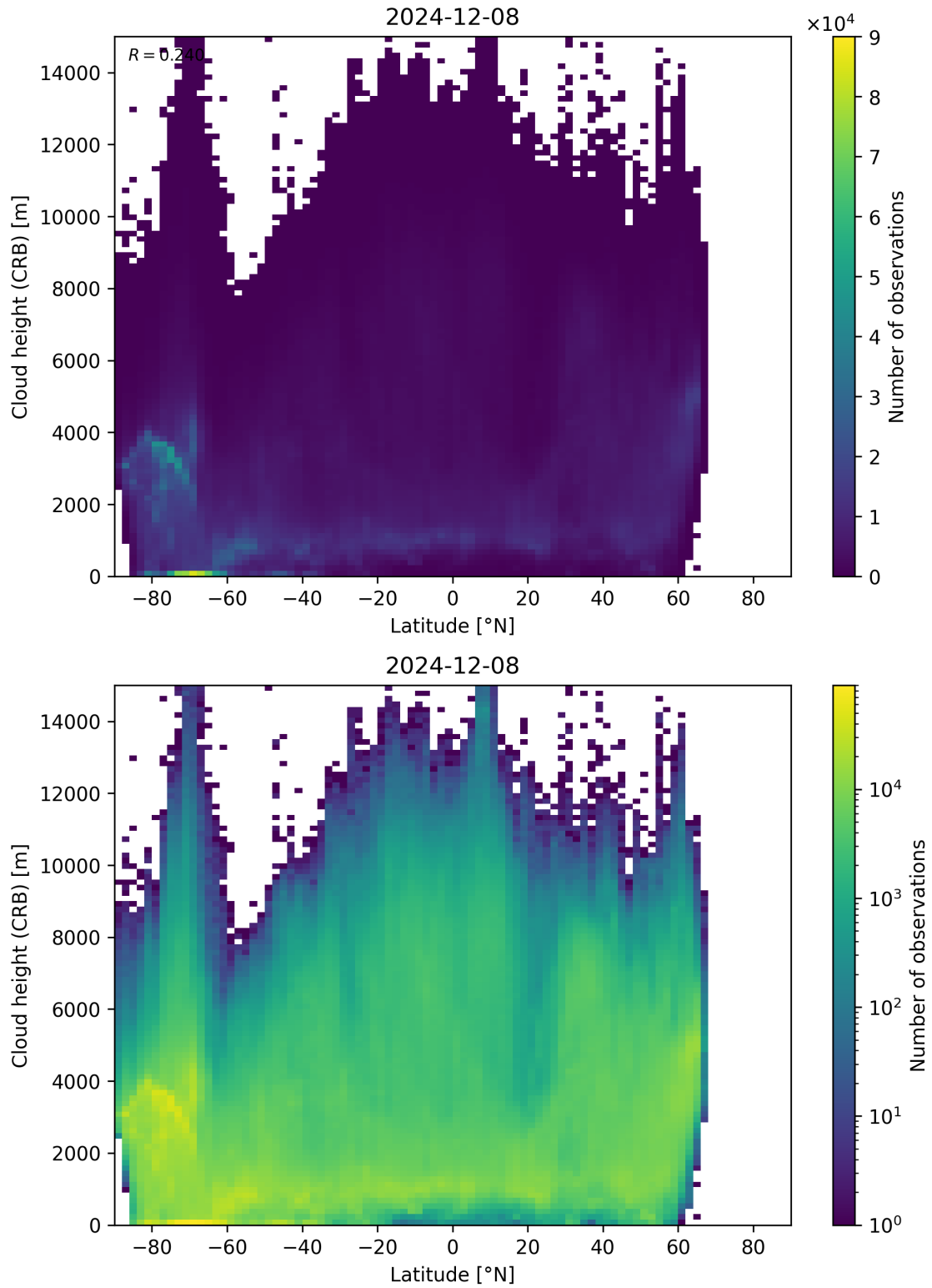
Figure 95: Scatter density plot of “Latitude” against “Cloud height (CRB)” for 2024-12-07 to 2024-12-09.
