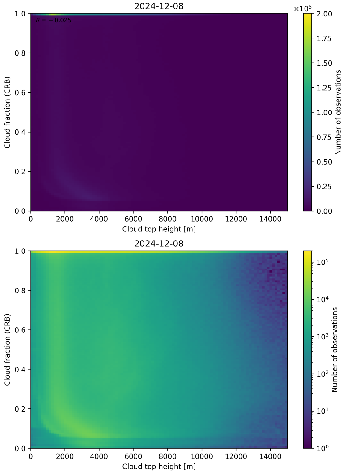
Figure 88: Scatter density plot of “Cloud top height” against “Cloud fraction (CRB)” for 2024-12-07 to 2024-12-09.
