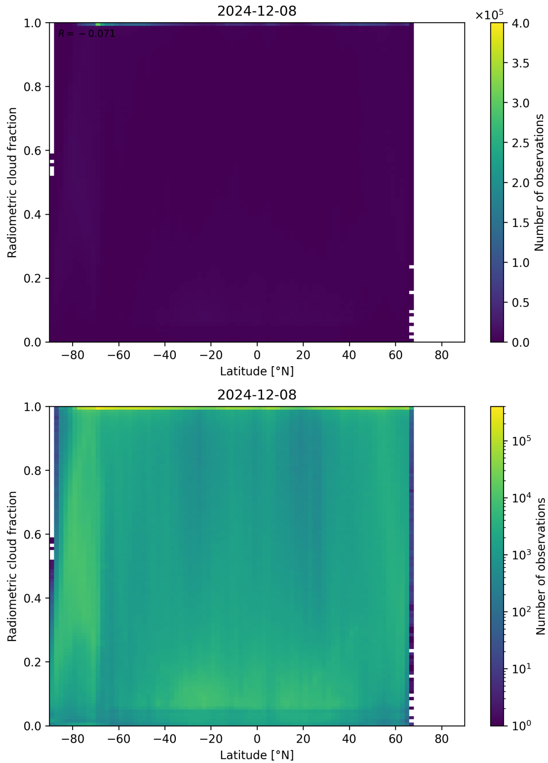
Figure 92: Scatter density plot of “Latitude” against “Radiometric cloud fraction” for 2024-12-07 to 2024-12-09.
