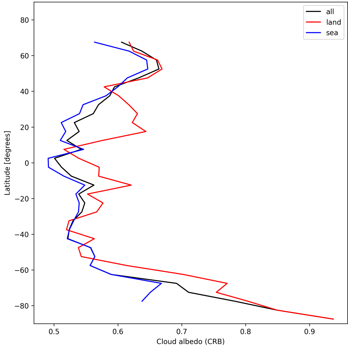
Figure 28: Zonal average of “Cloud albedo (CRB)” for 2024-12-07 to 2024-12-09.
