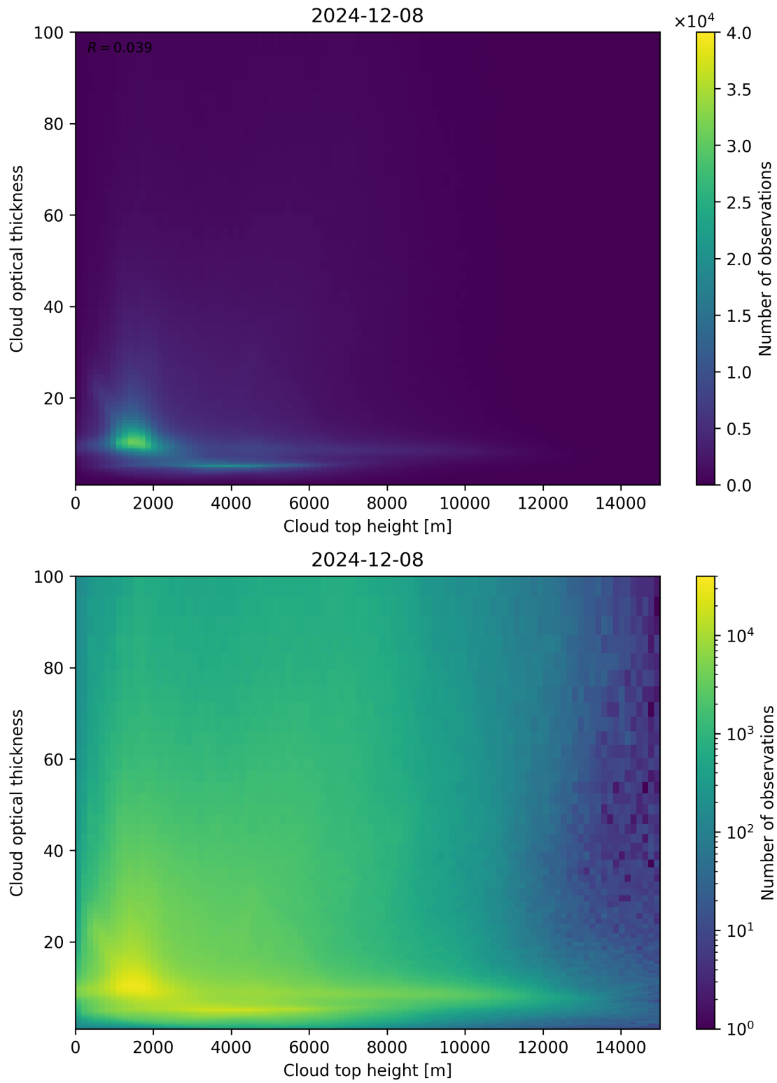
Figure 90: Scatter density plot of “Cloud top height” against “Cloud optical thickness” for 2024-12-07 to 2024-12-09.
