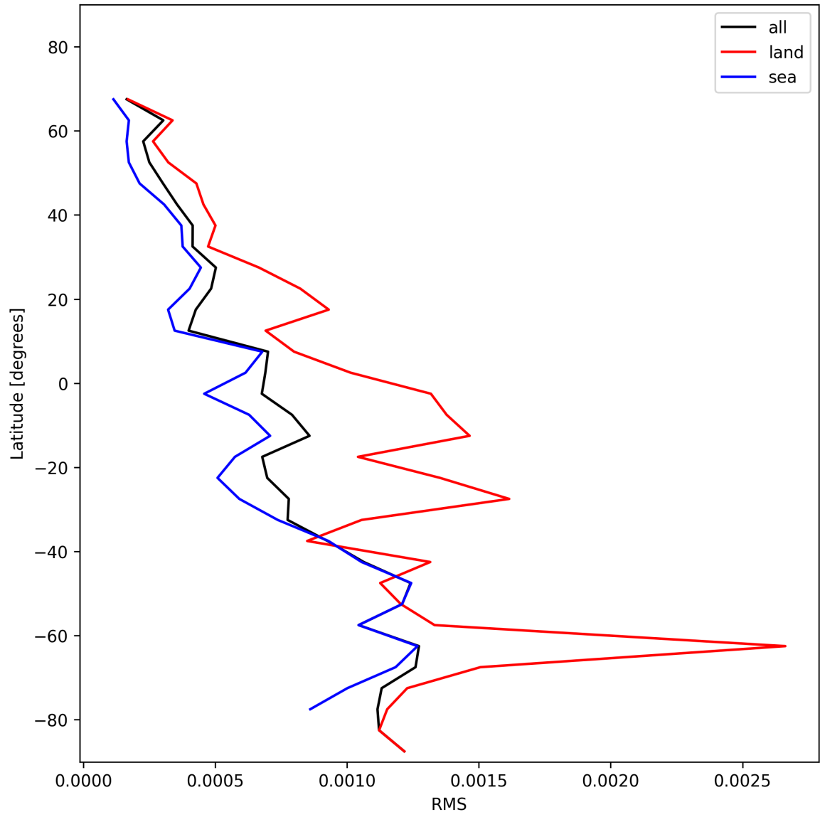
Figure 31: Zonal average of “RMS” for 2024-12-07 to 2024-12-09.
