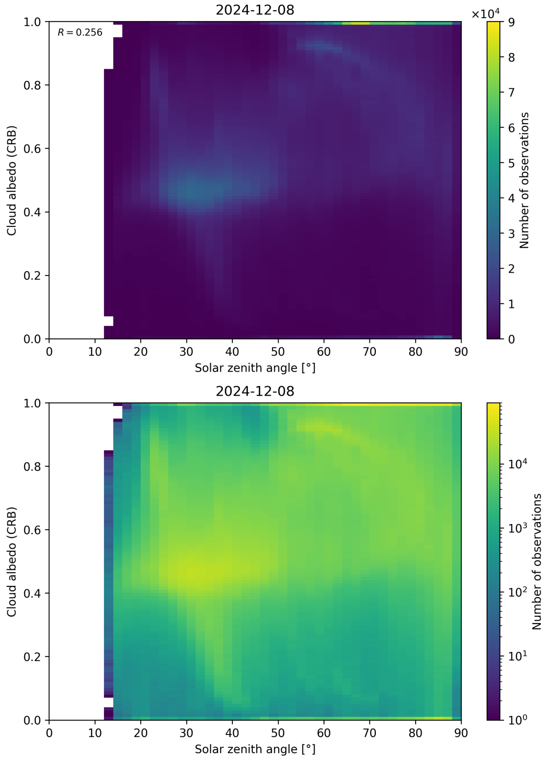
Figure 98: Scatter density plot of “Solar zenith angle” against “Cloud albedo (CRB)” for 2024-12-07 to 2024-12-09.
