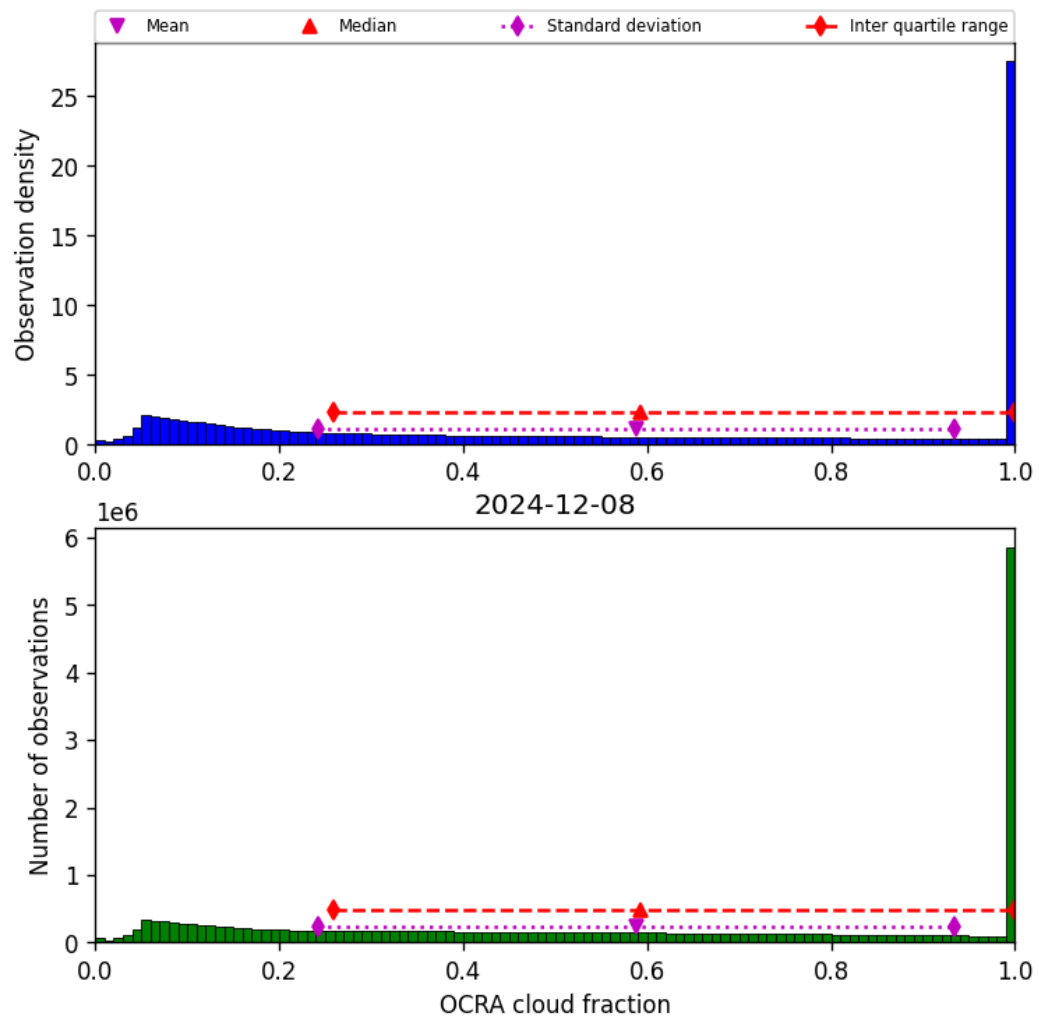
Figure 50: Histogram of “OCRA cloud fraction” for 2024-12-07 to 2024-12-09
