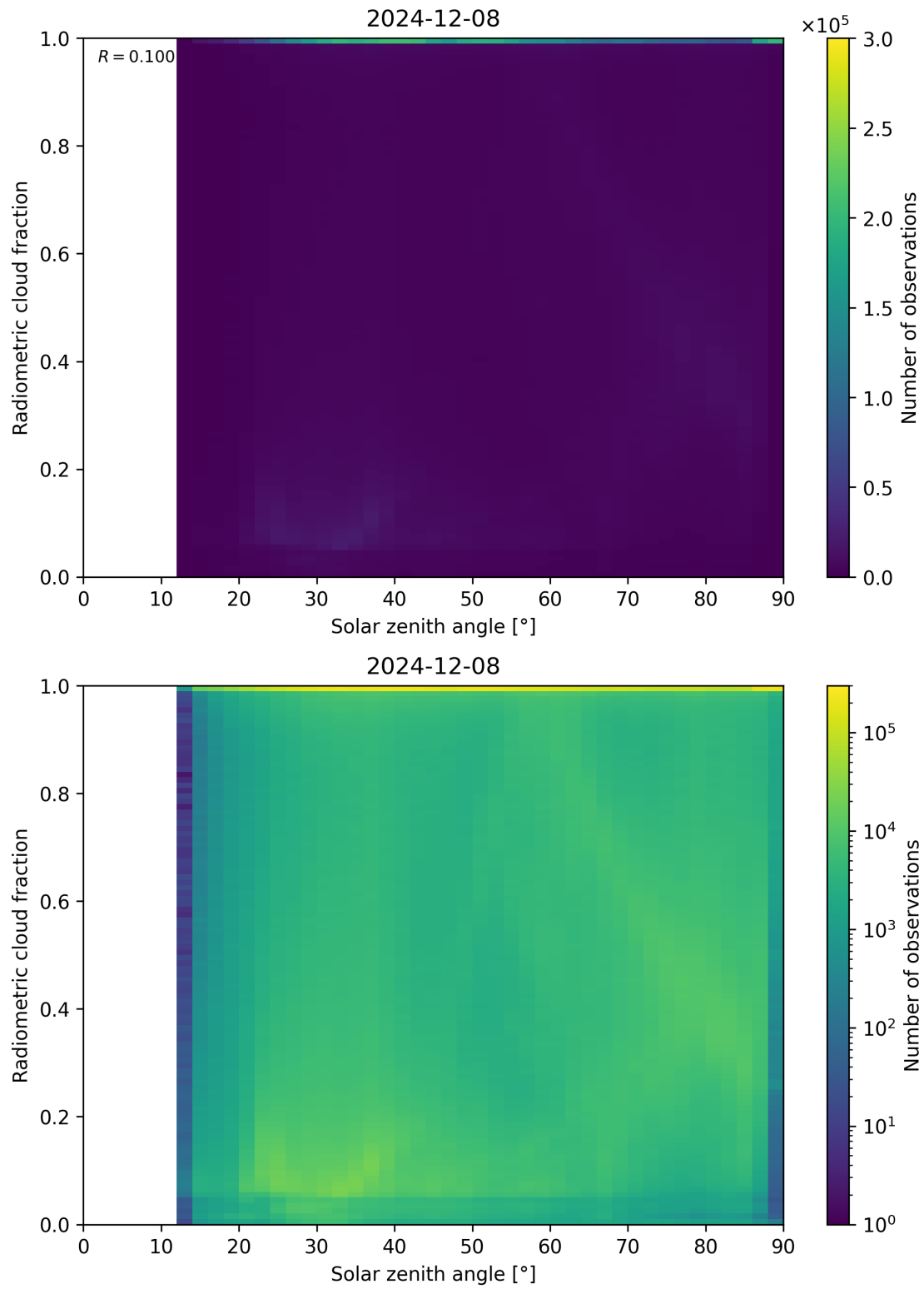
Figure 99: Scatter density plot of “Solar zenith angle” against “Radiometric cloud fraction” for 2024-12-07 to 2024-12-09.
