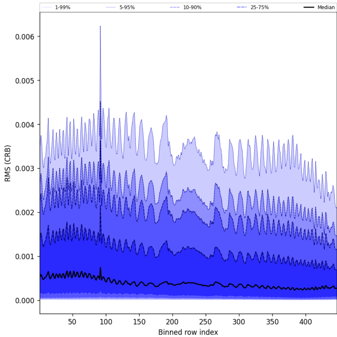
Figure 64: Along track statistics of “RMS (CRB)” for 2024-12-07 to 2024-12-09
