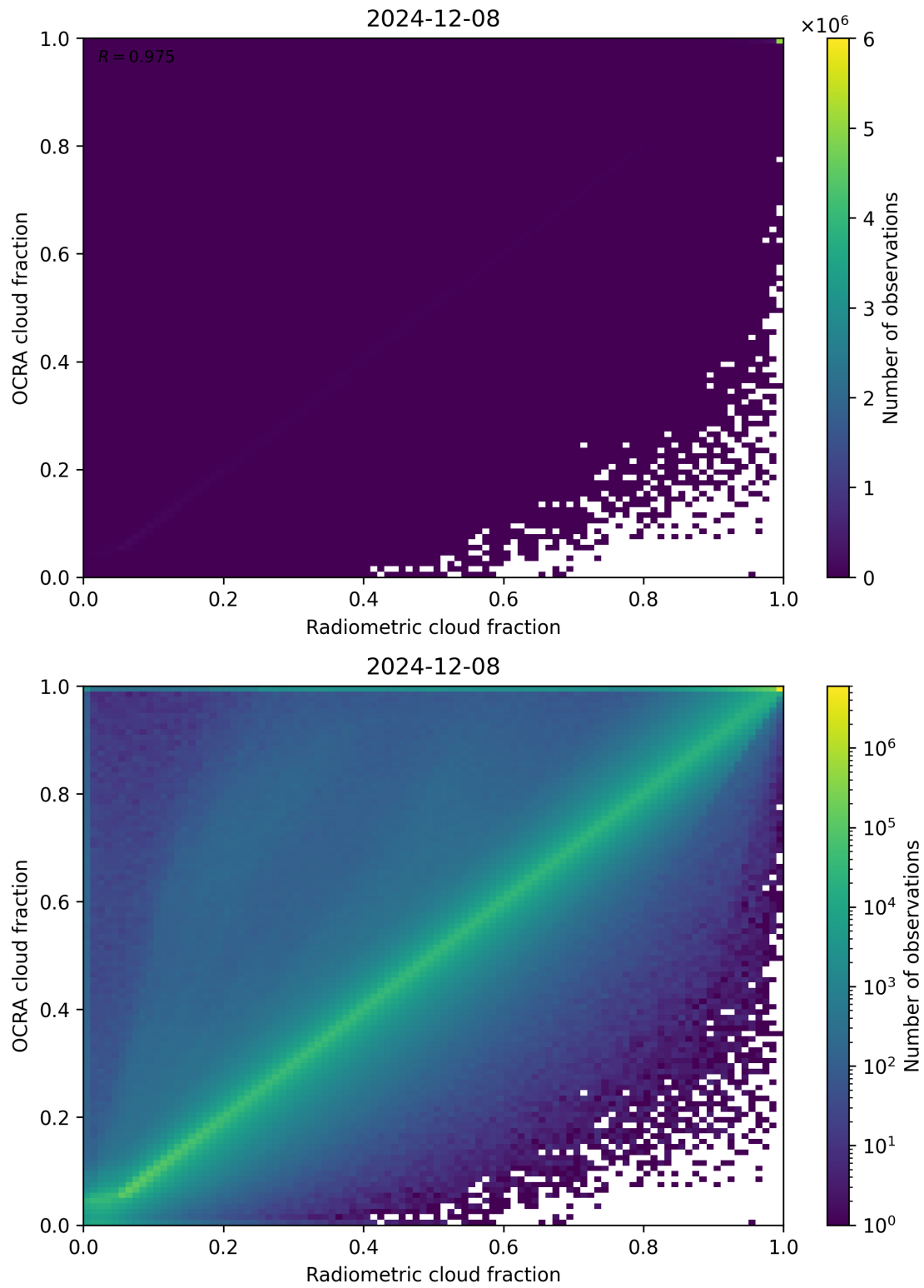
Figure 72: Scatter density plot of “Radiometric cloud fraction” against “OCRA cloud fraction” for 2024-12-07 to 2024-12-09.
