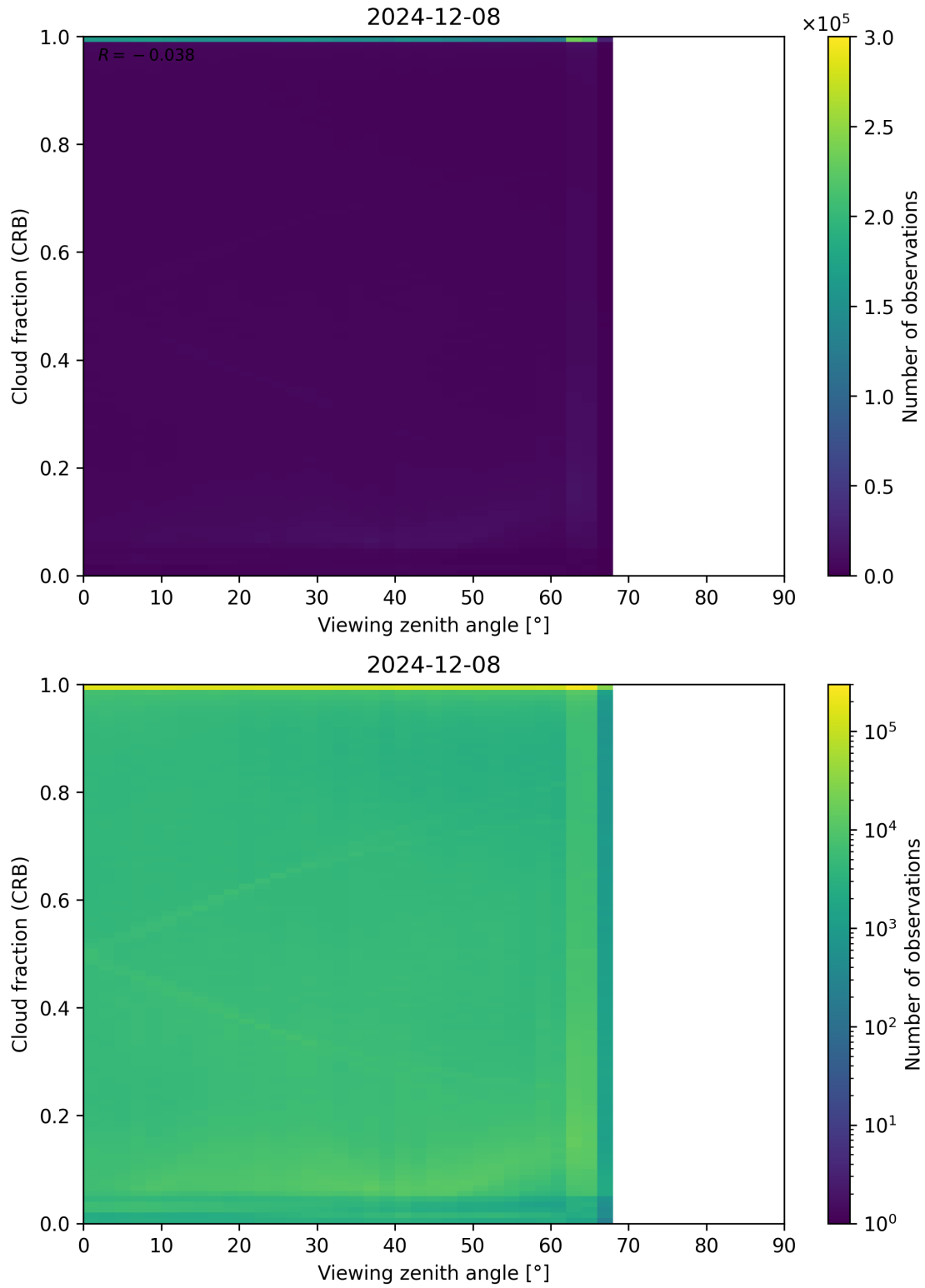
Figure 109: Scatter density plot of “Viewing zenith angle” against “Cloud fraction (CRB)” for 2024-12-07 to 2024-12-09.
