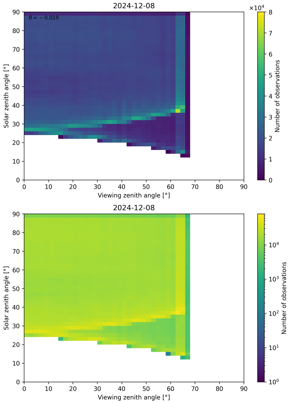
Figure 114: Scatter density plot of “Viewing zenith angle” against “Solar zenith angle” for 2024-12-07 to 2024-12-09.
