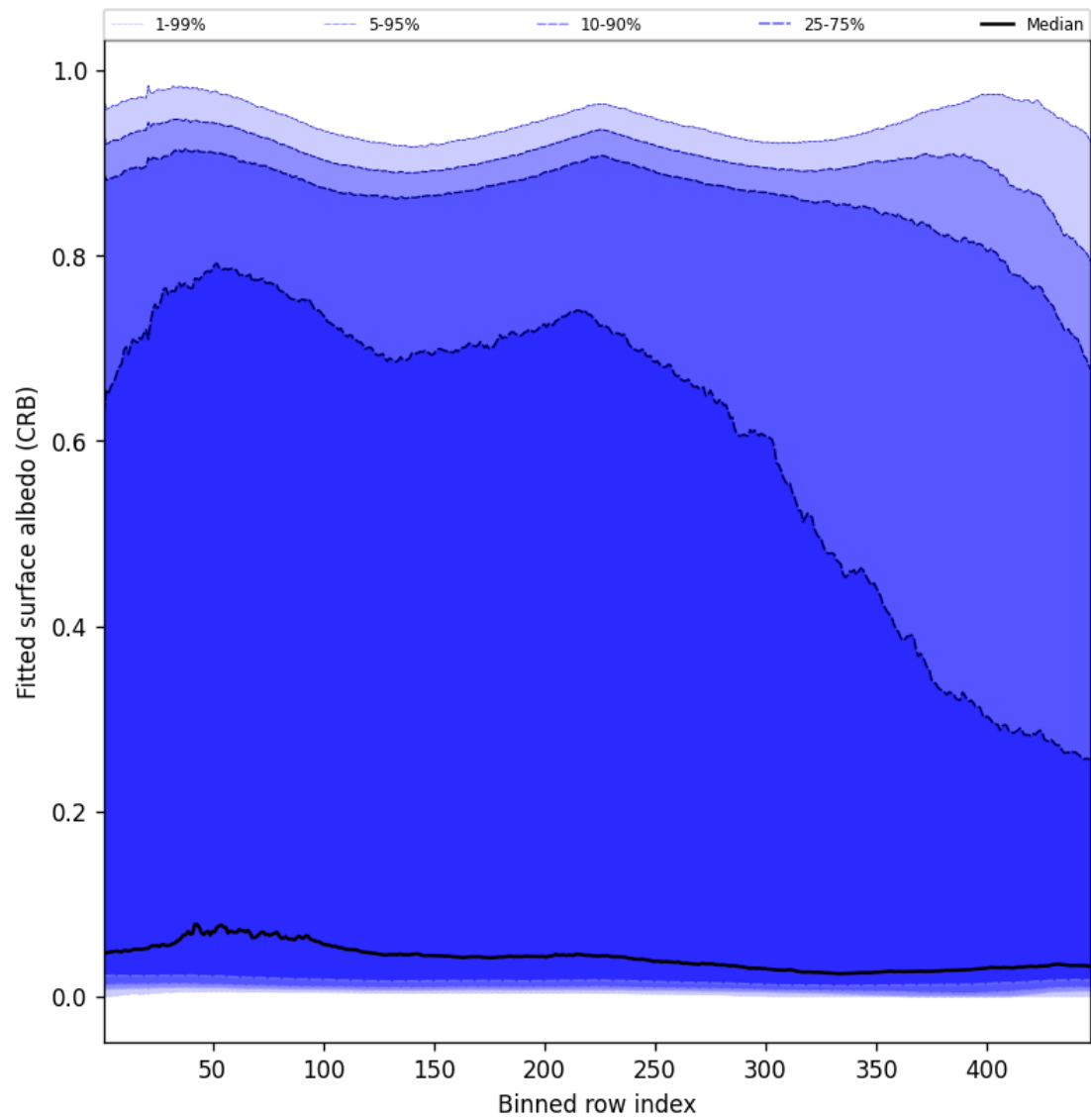
Figure 62: Along track statistics of “Fitted surface albedo (CRB)” for 2024-12-07 to 2024-12-09
