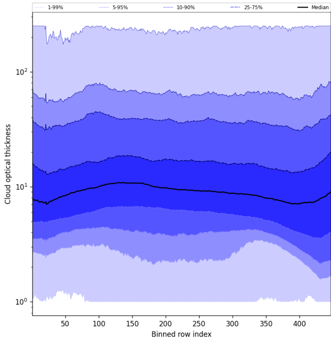
Figure 57: Along track statistics of “Cloud optical thickness” for 2024-12-07 to 2024-12-09
