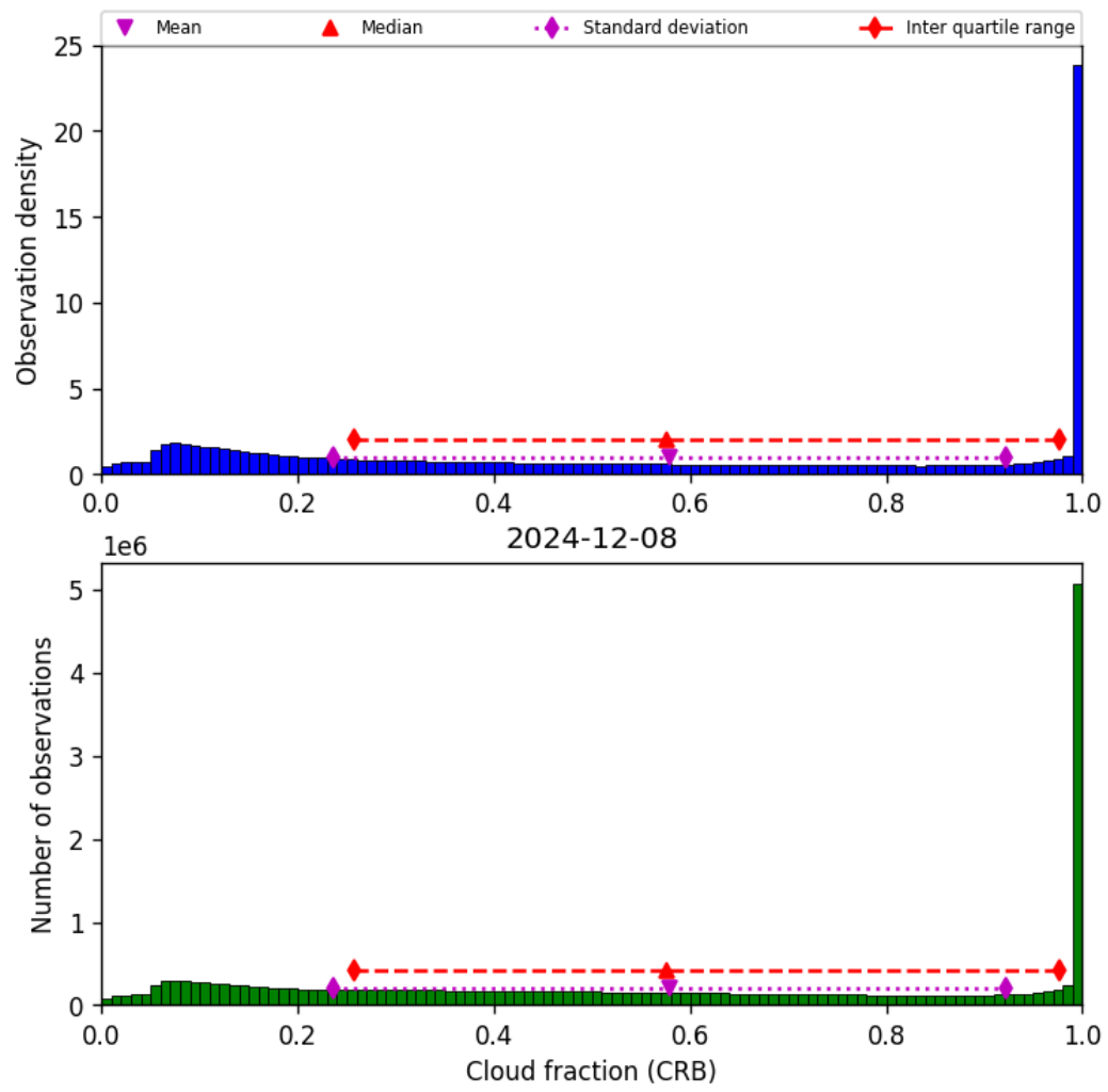
Figure 42: Histogram of “Cloud fraction (CRB)” for 2024-12-07 to 2024-12-09
