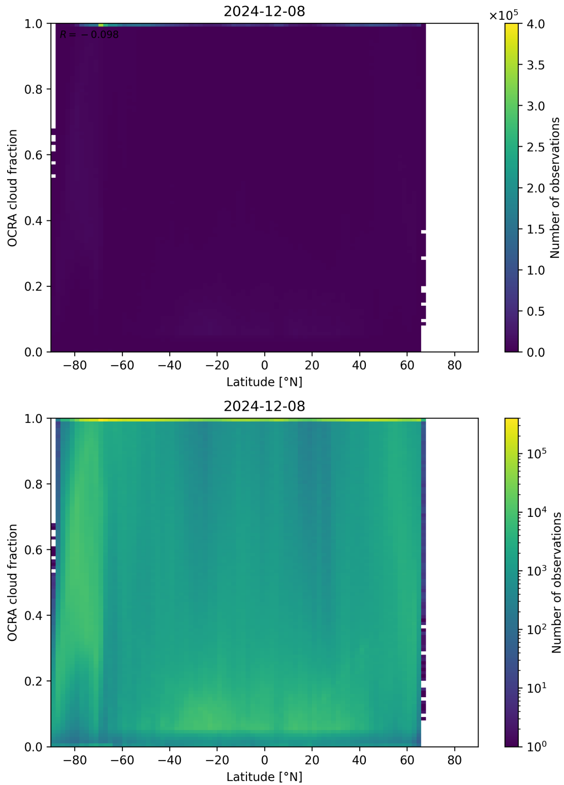
Figure 93: Scatter density plot of “Latitude” against “OCRA cloud fraction” for 2024-12-07 to 2024-12-09.
