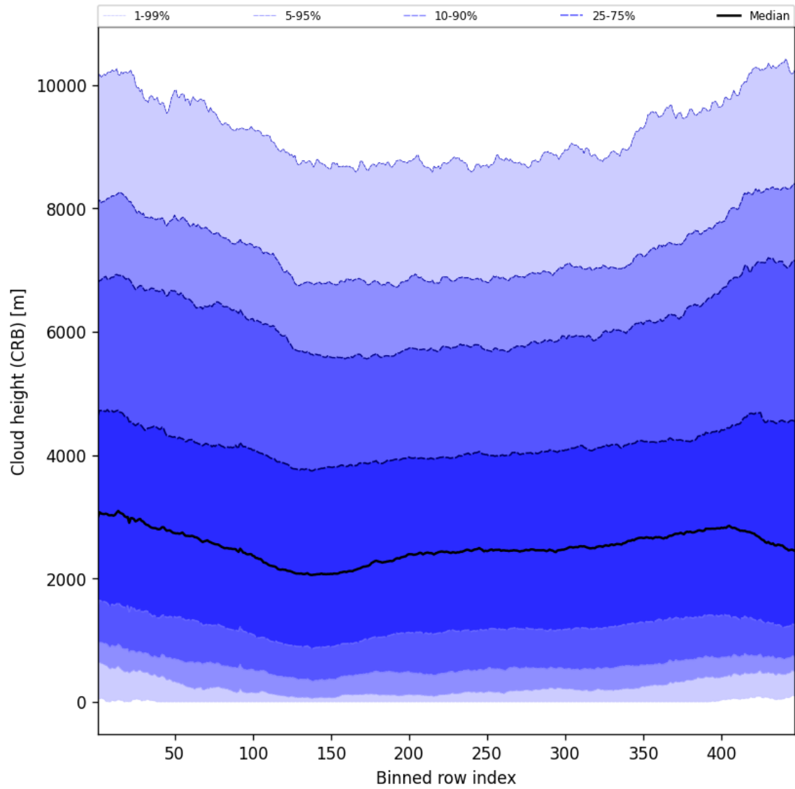
Figure 59: Along track statistics of “Cloud height (CRB)” for 2024-12-07 to 2024-12-09
