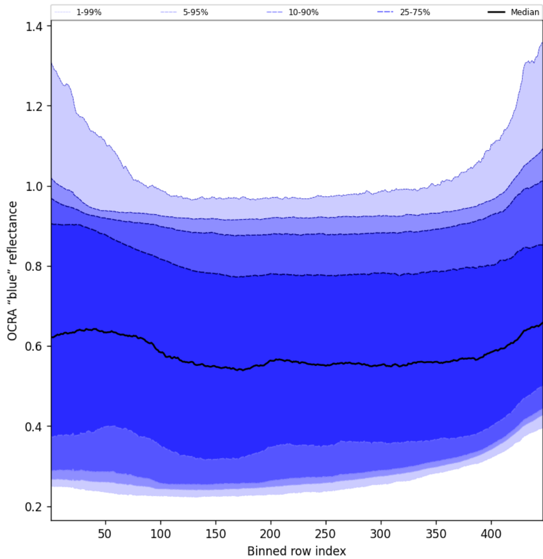
Figure 67: Along track statistics of “OCRA “blue” reflectance” for 2024-12-07 to 2024-12-09
