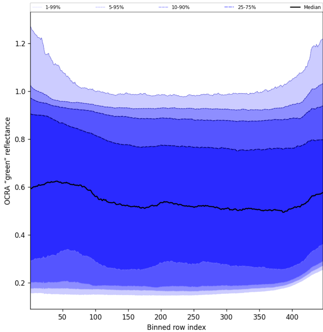
Figure 68: Along track statistics of “OCRA “green” reflectance” for 2024-12-07 to 2024-12-09
