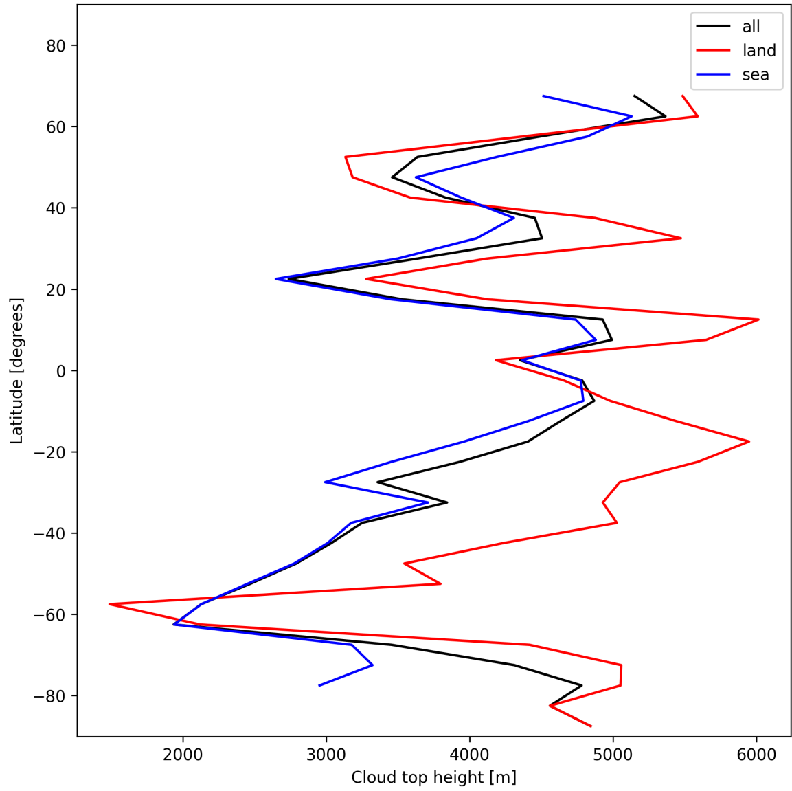
Figure 24: Zonal average of “Cloud top height” for 2024-12-07 to 2024-12-09.
