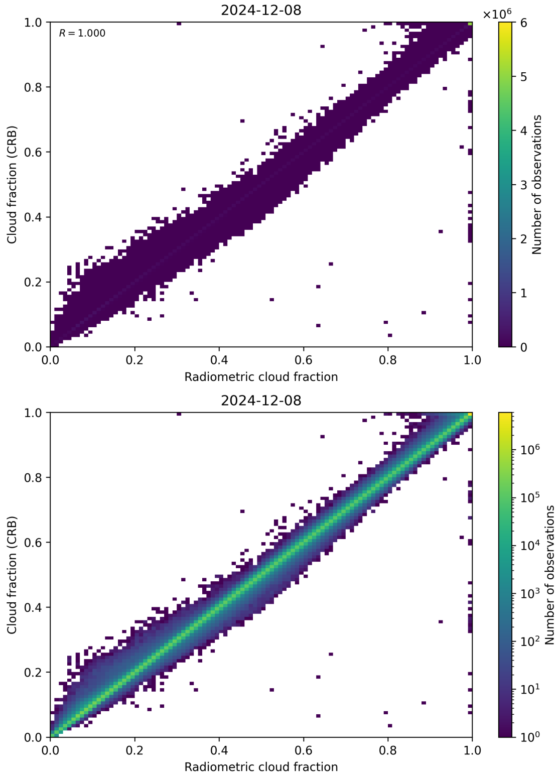
Figure 73: Scatter density plot of “Radiometric cloud fraction” against “Cloud fraction (CRB)” for 2024-12-07 to 2024-12-09.
