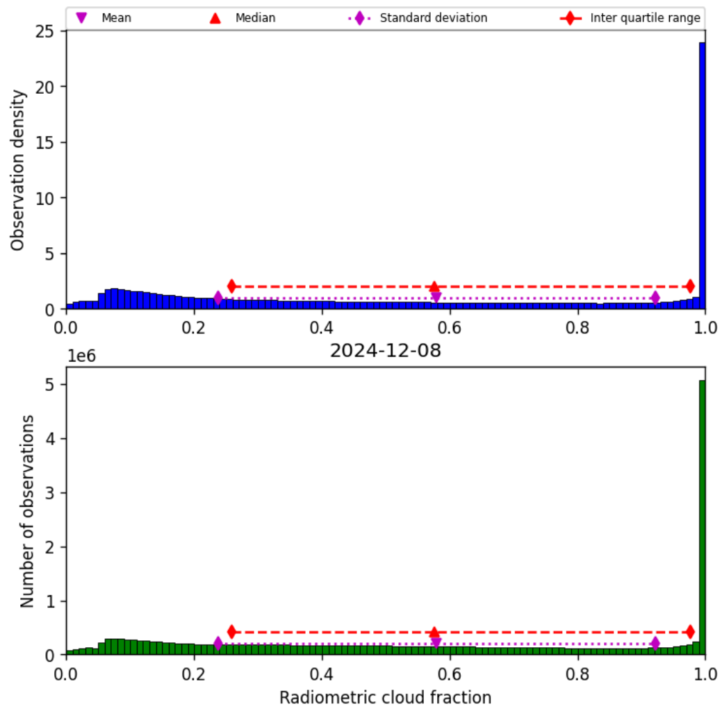
Figure 39: Histogram of “Radiometric cloud fraction” for 2024-12-07 to 2024-12-09
