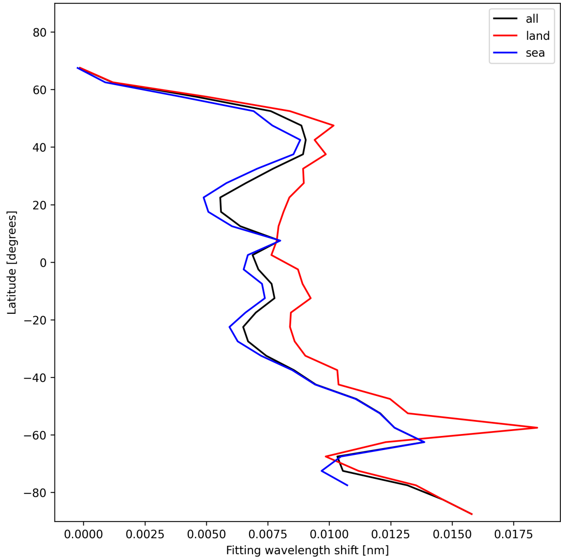
Figure 33: Zonal average of “Fitting wavelength shift” for 2024-12-07 to 2024-12-09.
