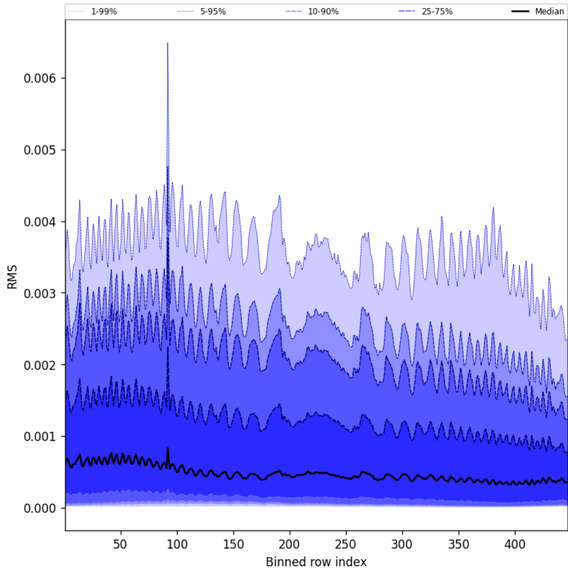
Figure 63: Along track statistics of “RMS” for 2024-12-07 to 2024-12-09
