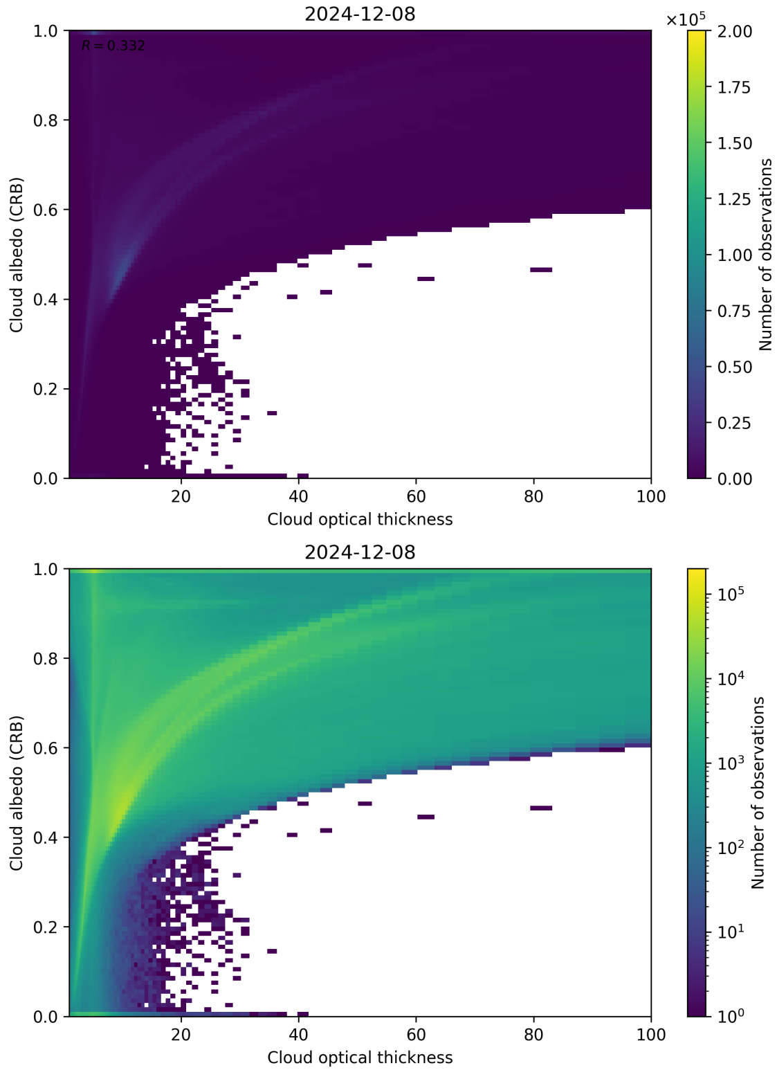
Figure 82: Scatter density plot of “Cloud optical thickness” against “Cloud albedo (CRB)” for 2024-12-07 to 2024-12-09.
