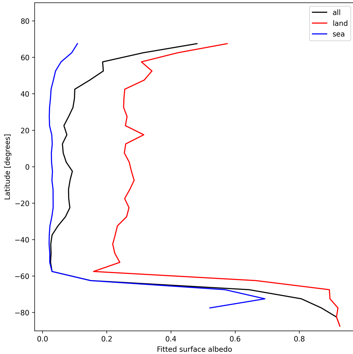
Figure 29: Zonal average of “Fitted surface albedo” for 2024-12-07 to 2024-12-09.
