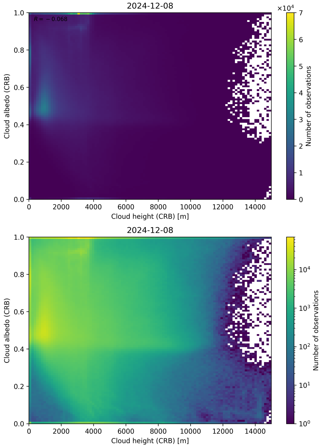
Figure 80: Scatter density plot of “Cloud height (CRB)” against “Cloud albedo (CRB)” for 2024-12-07 to 2024-12-09.
