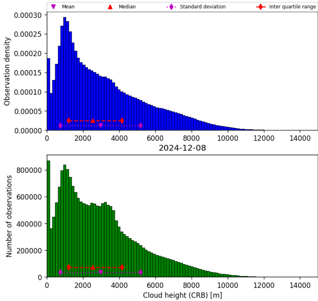
Figure 43: Histogram of “Cloud height (CRB)” for 2024-12-07 to 2024-12-09
