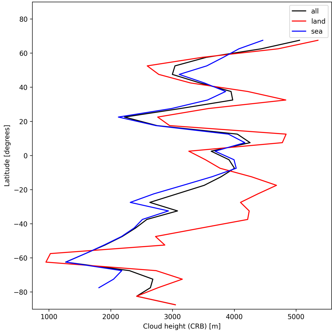
Figure 27: Zonal average of “Cloud height (CRB)” for 2024-12-07 to 2024-12-09.
