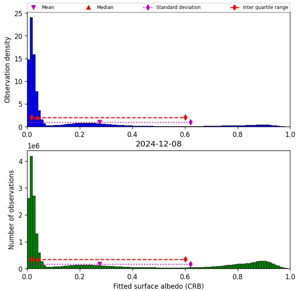
Figure 46: Histogram of “Fitted surface albedo (CRB)” for 2024-12-07 to 2024-12-09
