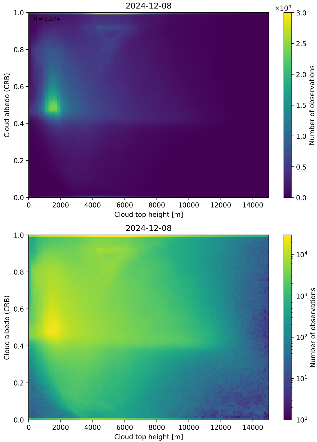
Figure 86: Scatter density plot of “Cloud top height” against “Cloud albedo (CRB)” for 2024-12-07 to 2024-12-09.
