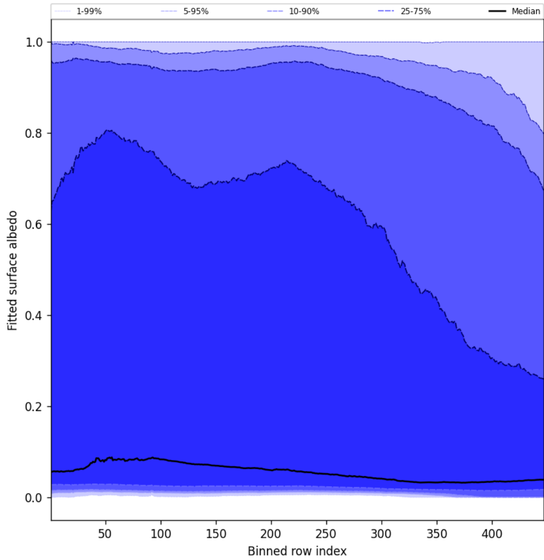
Figure 61: Along track statistics of “Fitted surface albedo” for 2024-12-07 to 2024-12-09
