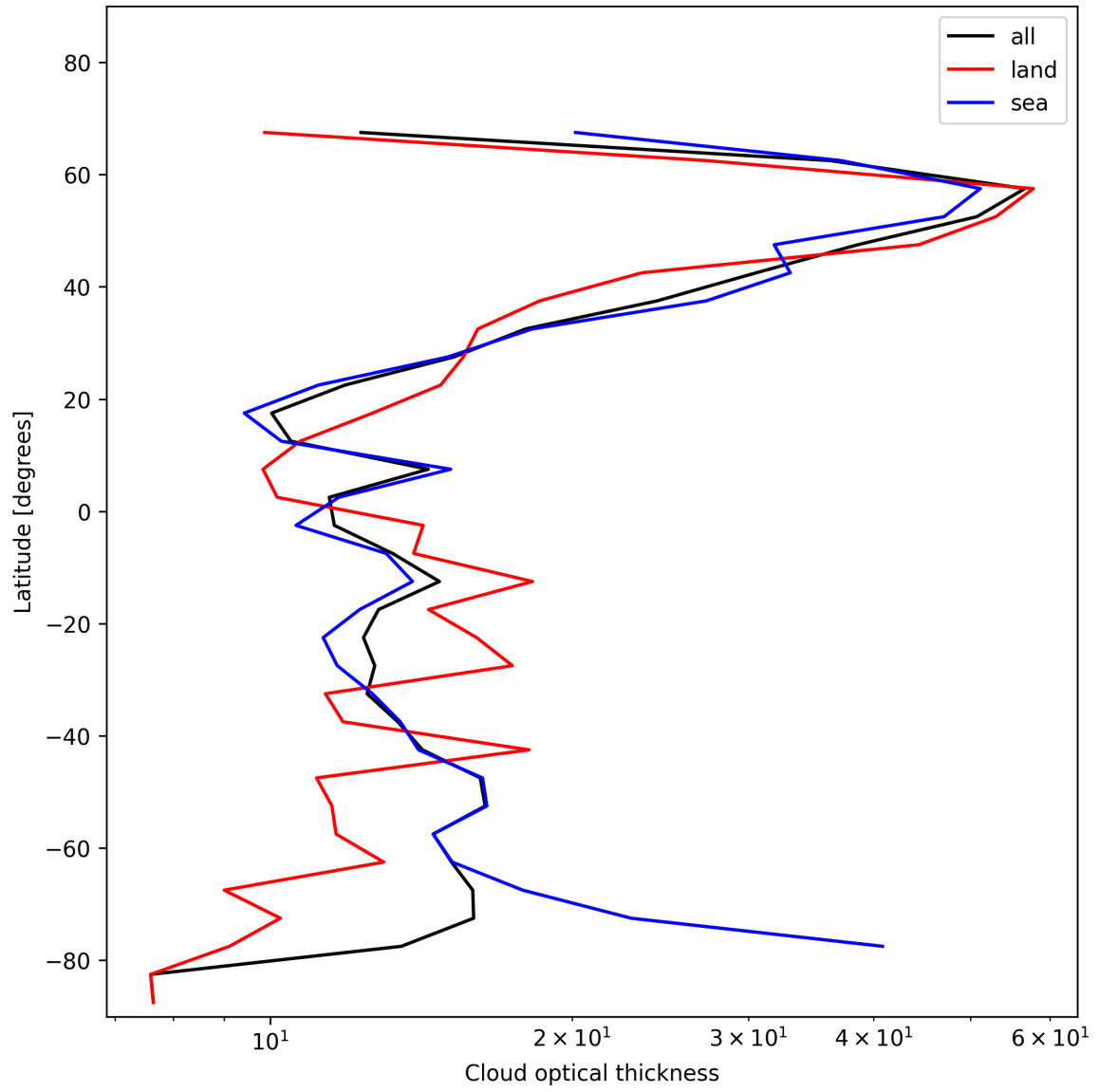
Figure 25: Zonal average of “Cloud optical thickness” for 2024-12-07 to 2024-12-09.
