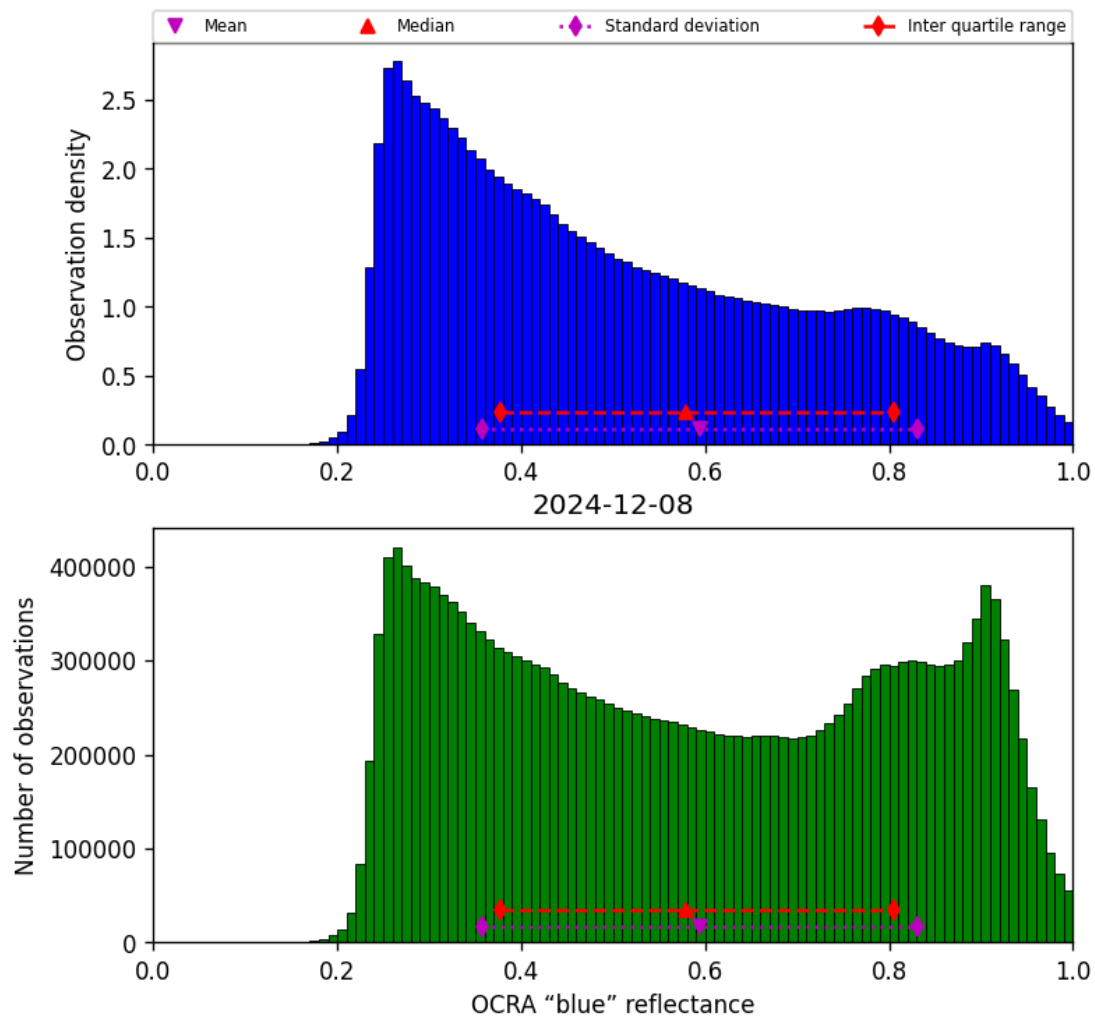
Figure 51: Histogram of “OCRA “blue” reflectance” for 2024-12-07 to 2024-12-09
