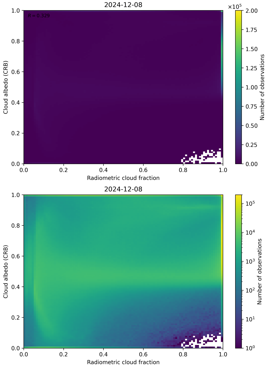
Figure 71: Scatter density plot of “Radiometric cloud fraction” against “Cloud albedo (CRB)” for 2024-12-07 to 2024-12-09.
