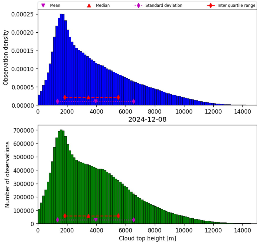
Figure 40: Histogram of “Cloud top height” for 2024-12-07 to 2024-12-09
