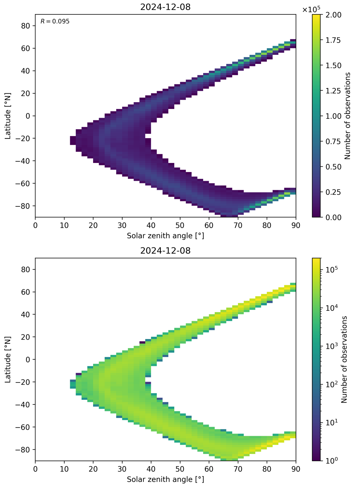
Figure 105: Scatter density plot of “Solar zenith angle” against “Latitude” for 2024-12-07 to 2024-12-09.
