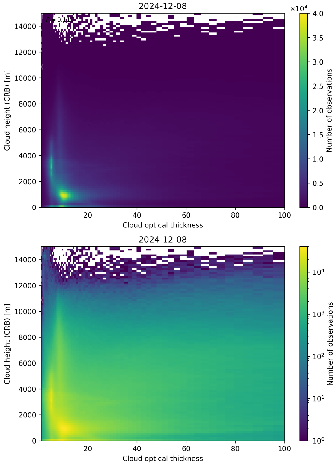
Figure 85: Scatter density plot of “Cloud optical thickness” against “Cloud height (CRB)” for 2024-12-07 to 2024-12-09.
