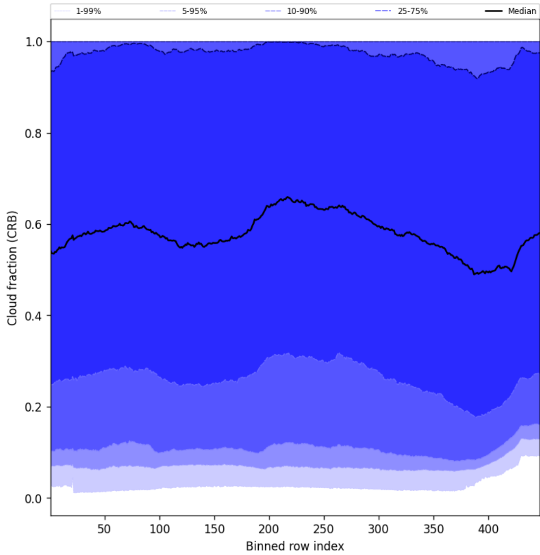
Figure 58: Along track statistics of “Cloud fraction (CRB)” for 2024-12-07 to 2024-12-09
