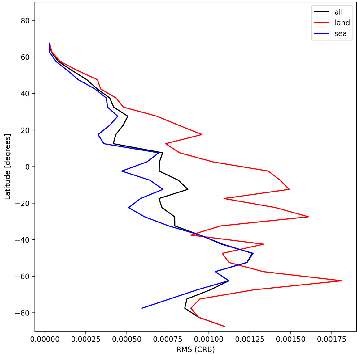
Figure 32: Zonal average of “RMS (CRB)” for 2024-12-07 to 2024-12-09.
