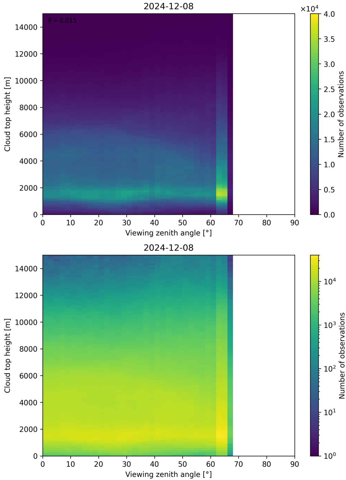
Figure 112: Scatter density plot of “Viewing zenith angle” against “Cloud top height” for 2024-12-07 to 2024-12-09.
