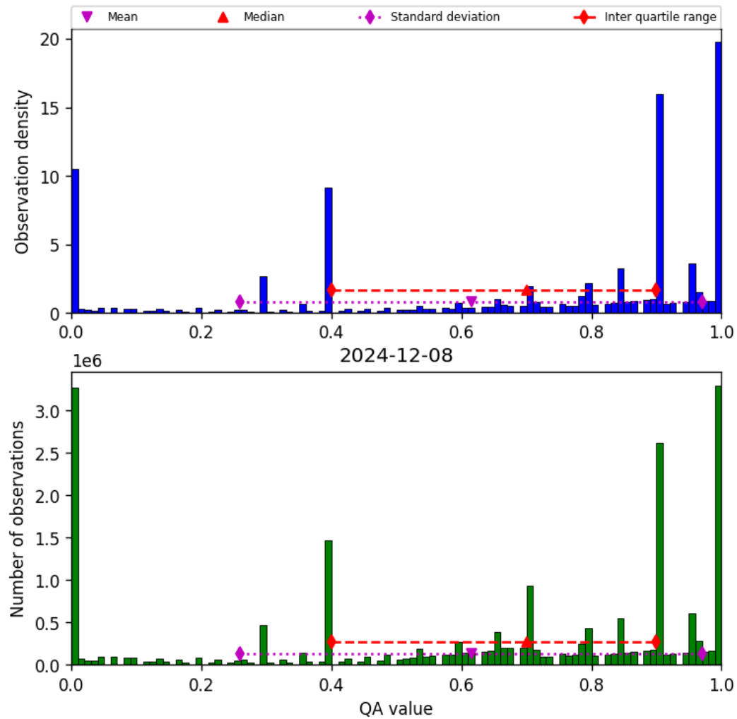
Figure 38: Histogram of “QA value” for 2024-12-07 to 2024-12-09
