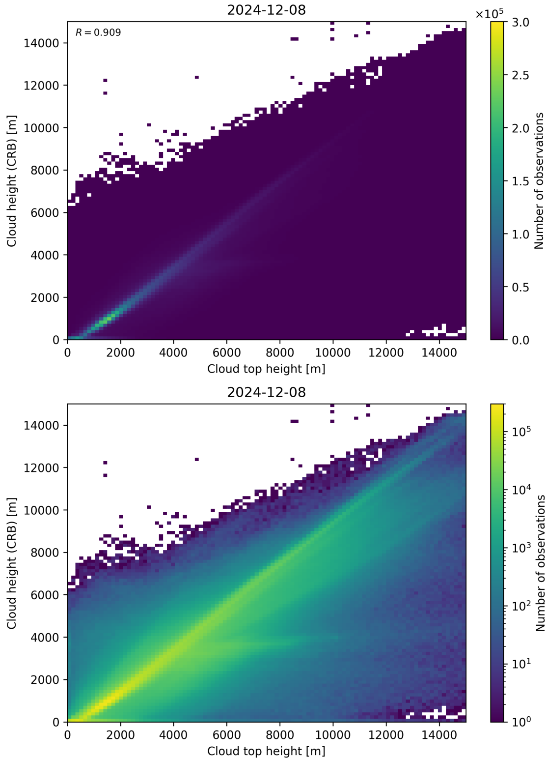
Figure 89: Scatter density plot of “Cloud top height” against “Cloud height (CRB)” for 2024-12-07 to 2024-12-09.
