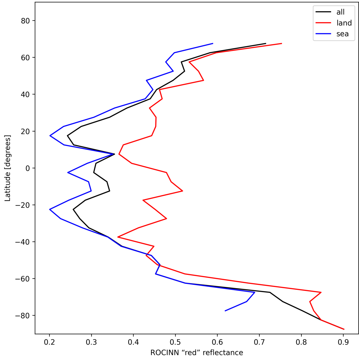
Figure 37: Zonal average of "ROCINN "red" reflectance" for 2024-12-07 to 2024-12-09.
