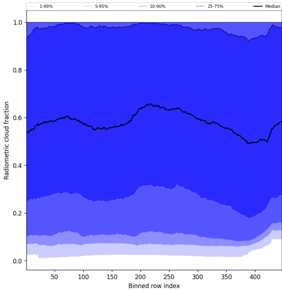
Figure 55: Along track statistics of “Radiometric cloud fraction” for 2024-12-07 to 2024-12-09
