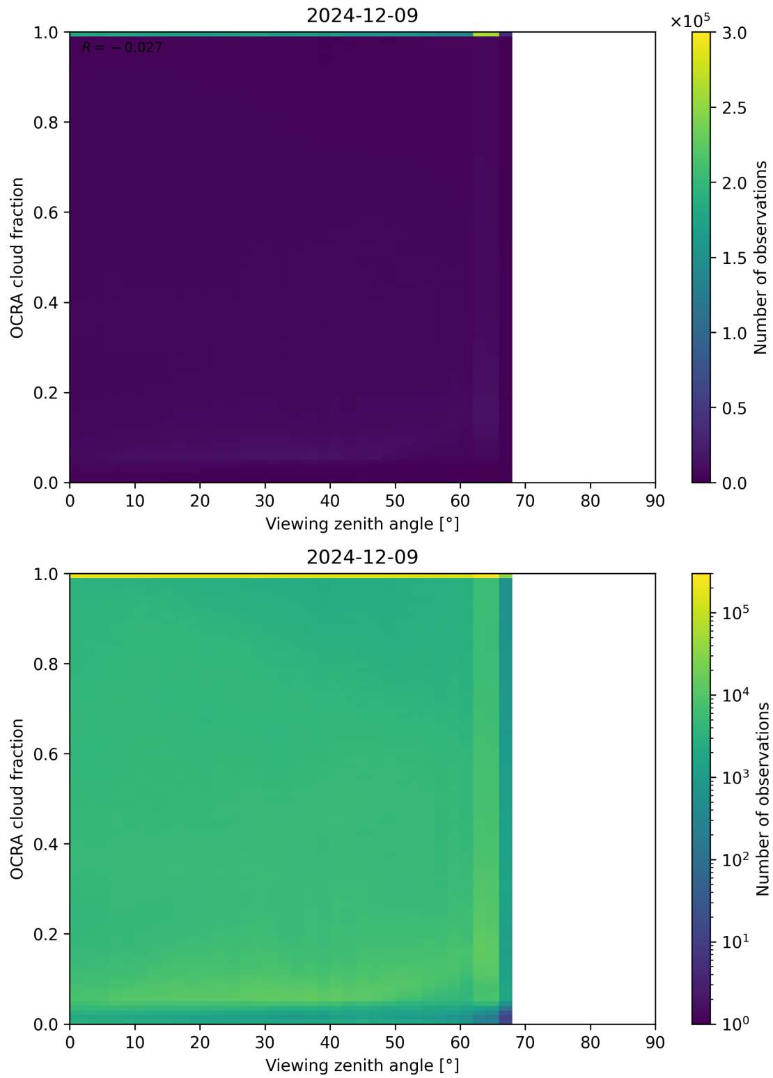
Figure 108: Scatter density plot of “Viewing zenith angle” against “OCRA cloud fraction” for 2024-12-08 to 2024-12-10.
