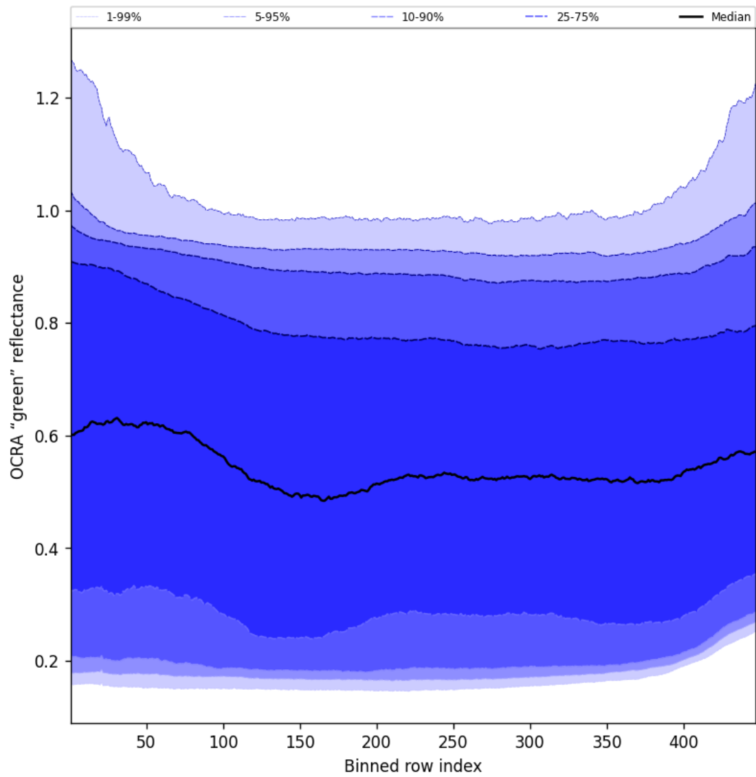
Figure 68: Along track statistics of “OCRA “green” reflectance” for 2024-12-08 to 2024-12-10
