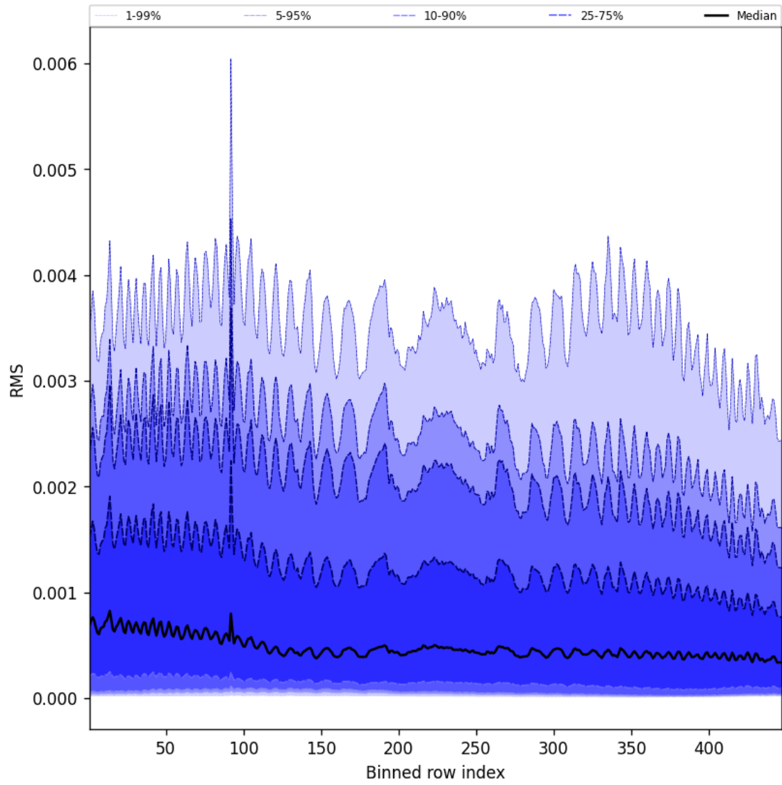
Figure 63: Along track statistics of “RMS” for 2024-12-08 to 2024-12-10
