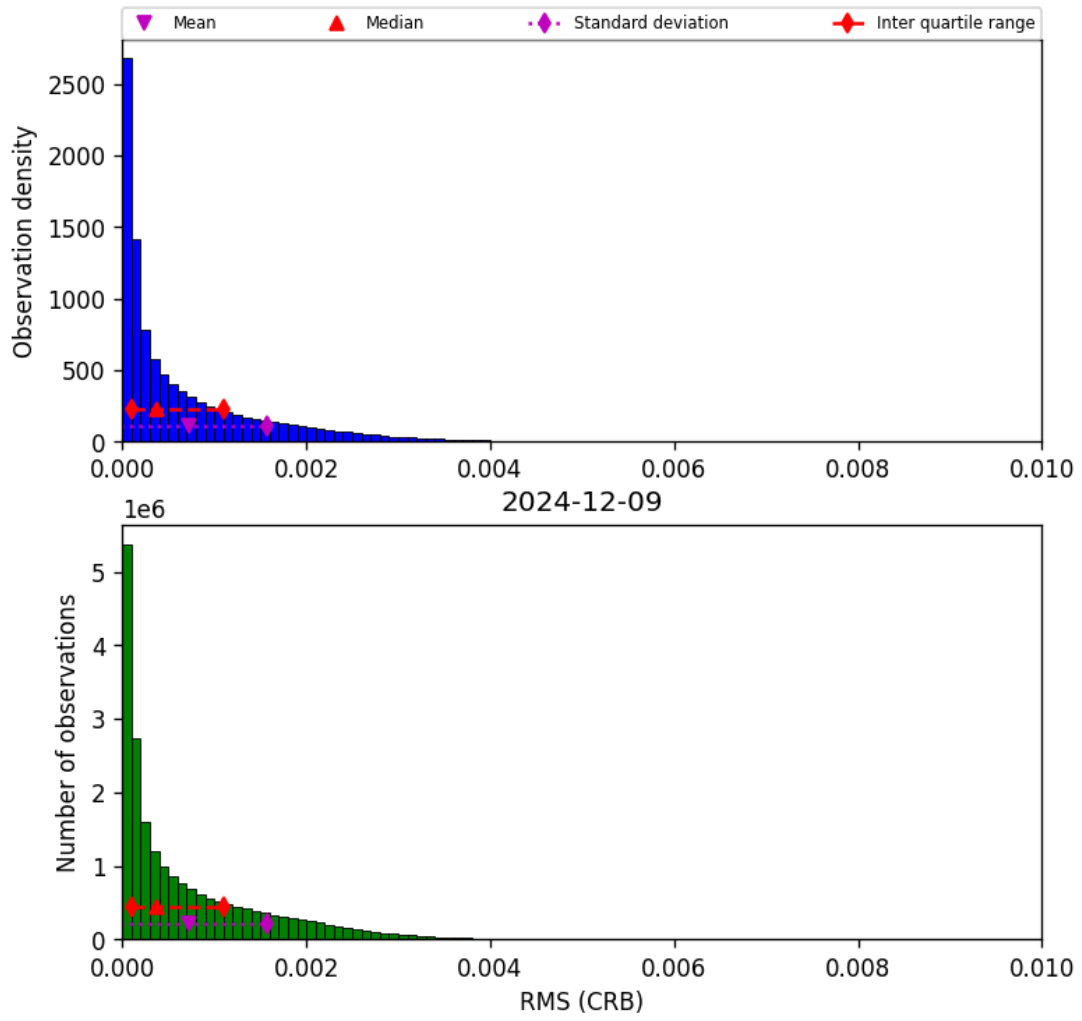
Figure 48: Histogram of “RMS (CRB)” for 2024-12-08 to 2024-12-10
