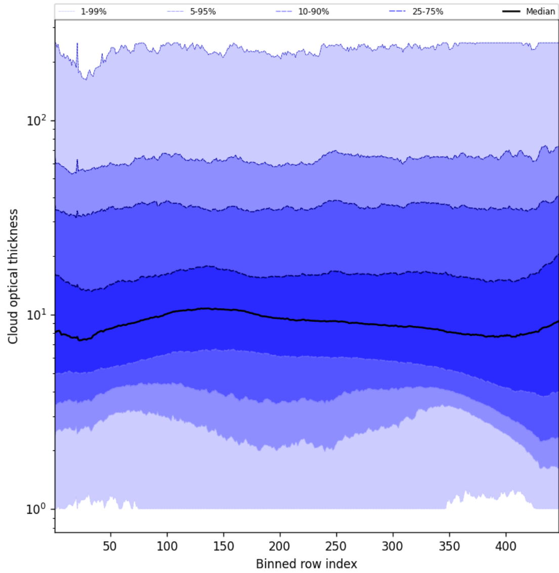
Figure 57: Along track statistics of “Cloud optical thickness” for 2024-12-08 to 2024-12-10
