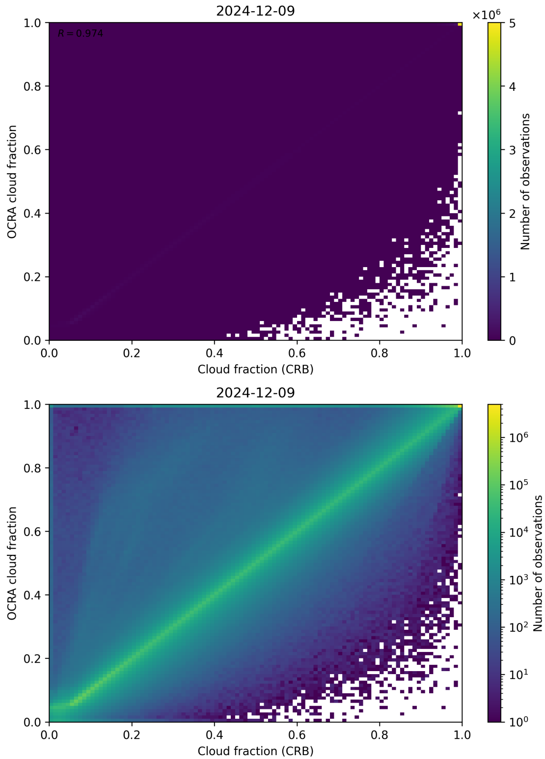
Figure 78: Scatter density plot of “Cloud fraction (CRB)” against “OCRA cloud fraction” for 2024-12-08 to 2024-12-10.
