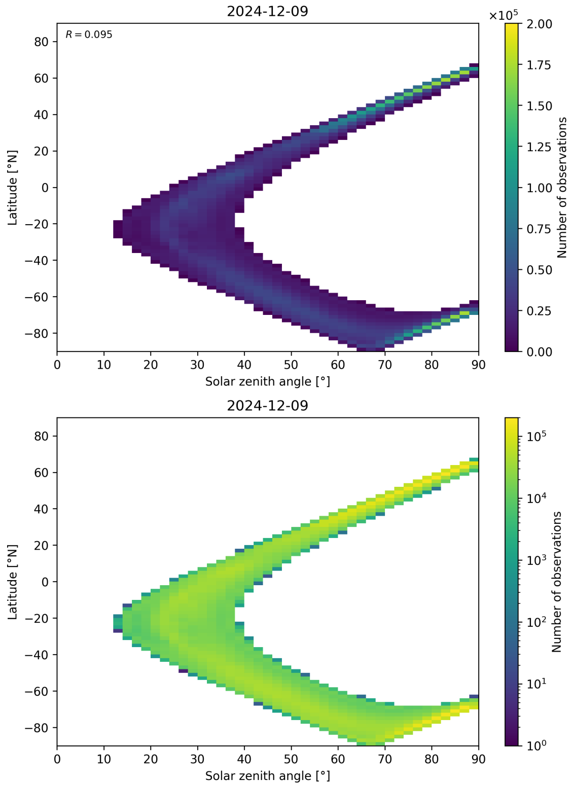
Figure 105: Scatter density plot of “Solar zenith angle” against “Latitude” for 2024-12-08 to 2024-12-10.
