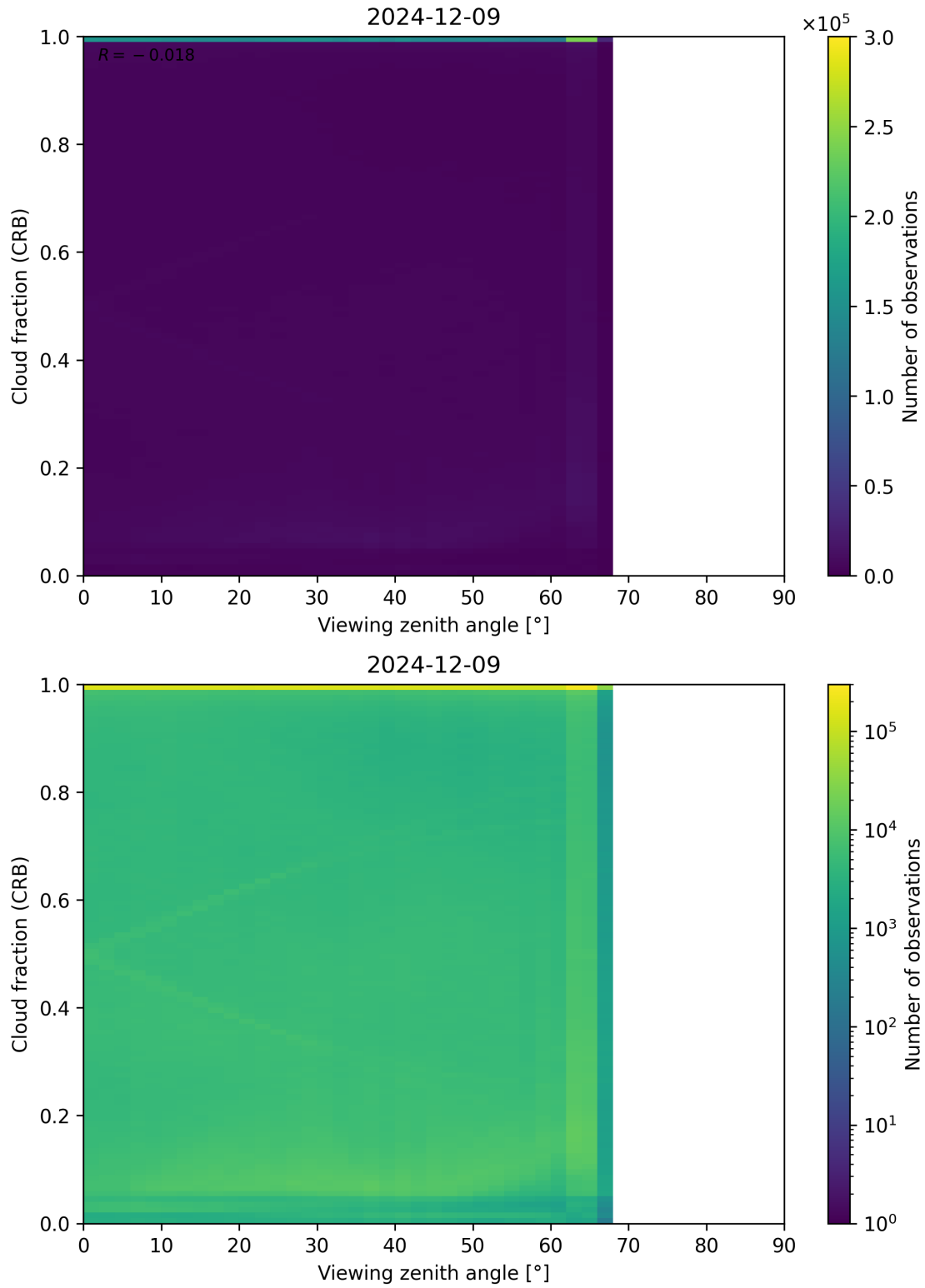
Figure 109: Scatter density plot of “Viewing zenith angle” against “Cloud fraction (CRB)” for 2024-12-08 to 2024-12-10.
