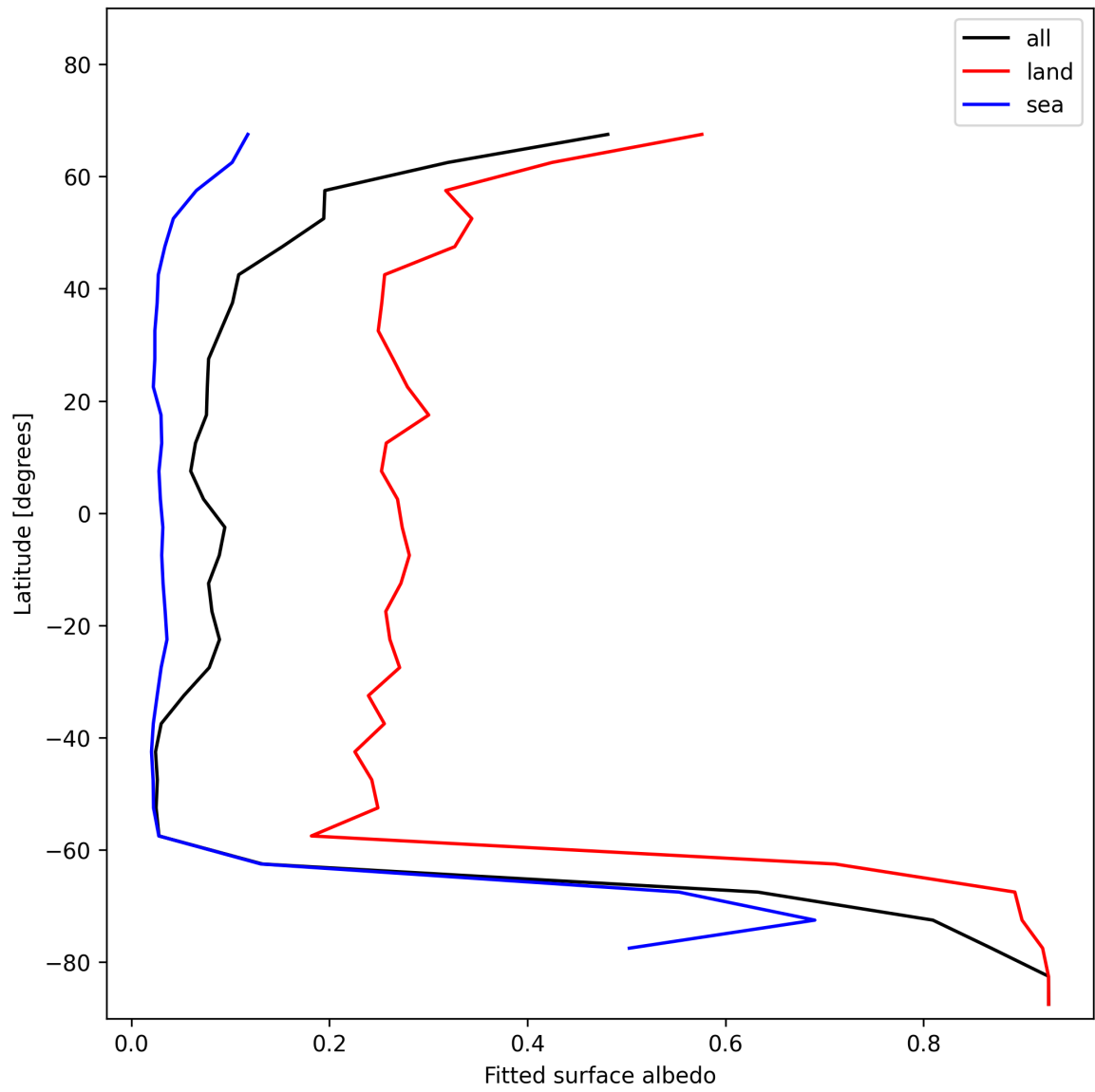
Figure 29: Zonal average of “Fitted surface albedo” for 2024-12-08 to 2024-12-10.
