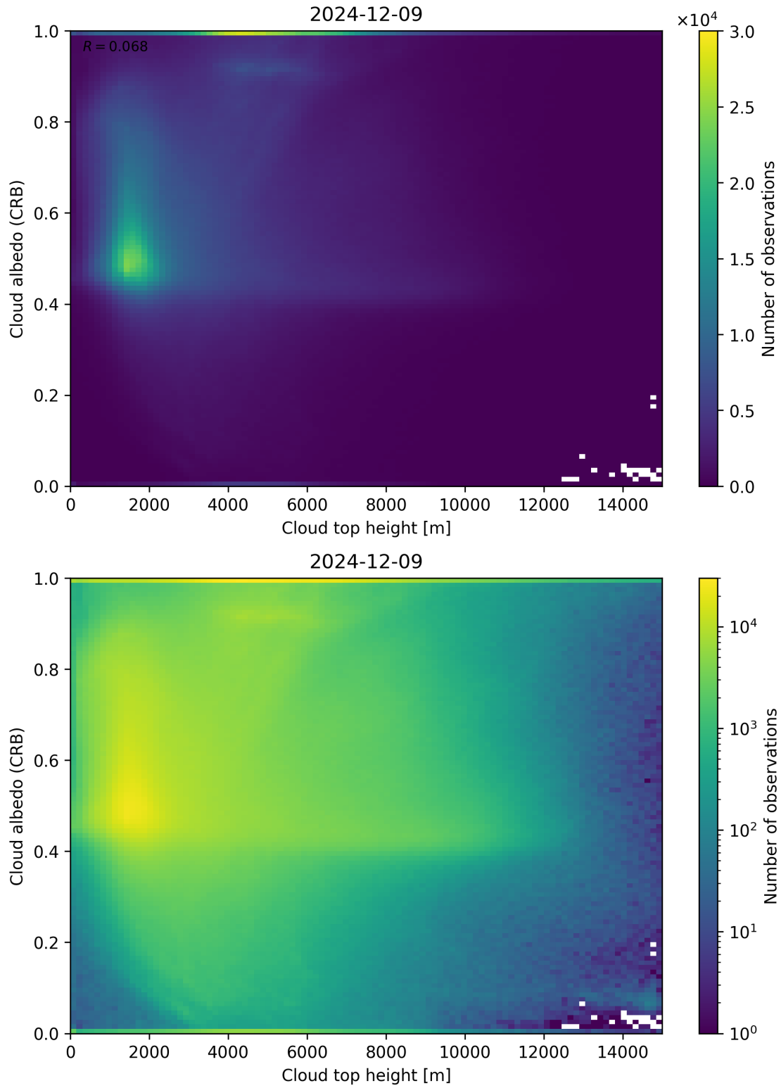
Figure 86: Scatter density plot of “Cloud top height” against “Cloud albedo (CRB)” for 2024-12-08 to 2024-12-10.
