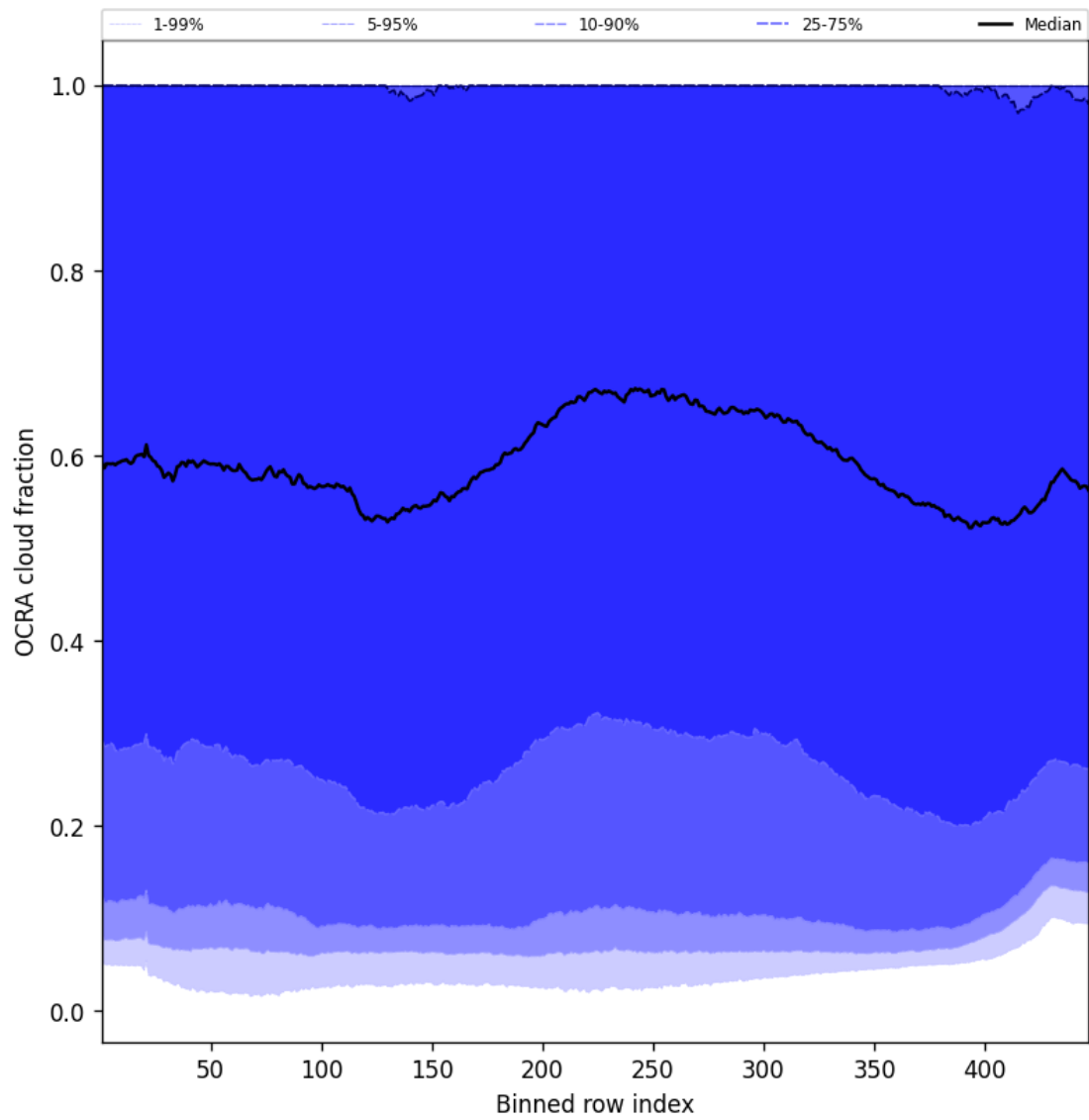
Figure 66: Along track statistics of “OCRA cloud fraction” for 2024-12-08 to 2024-12-10
