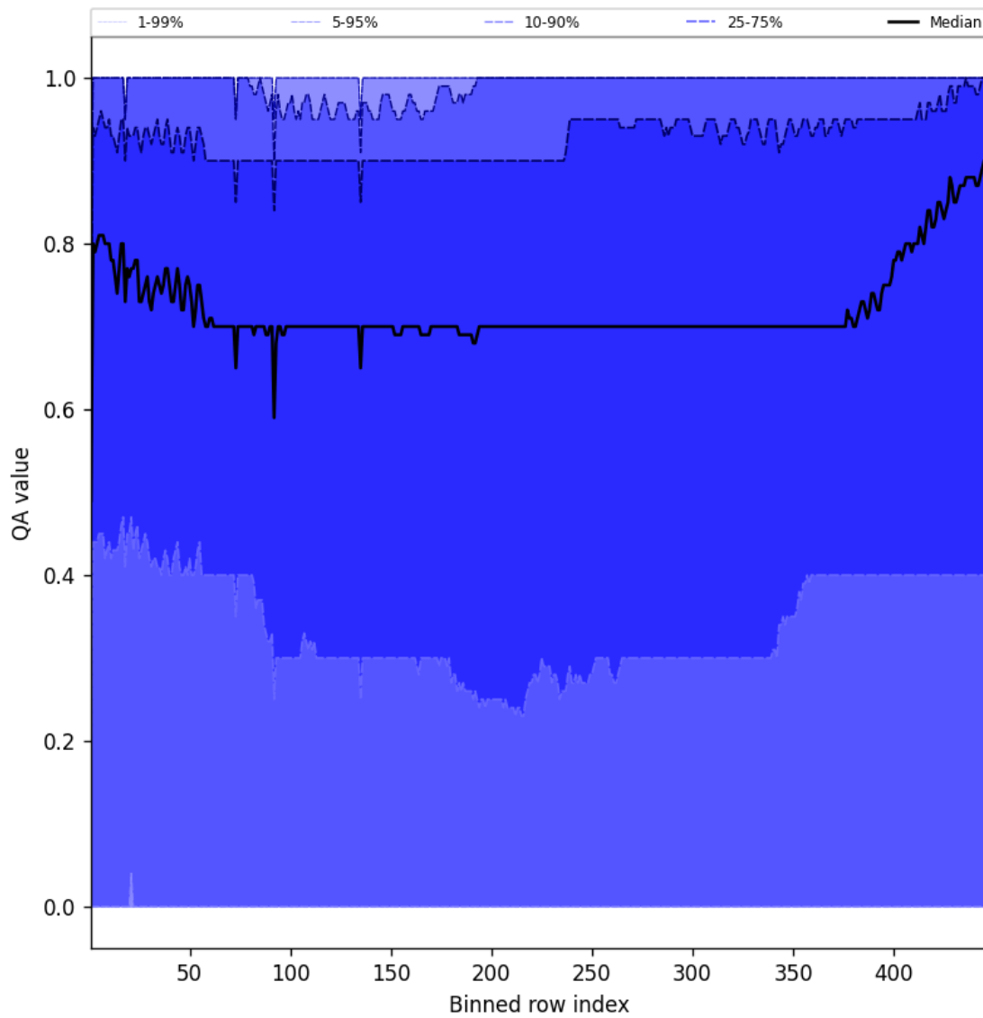
Figure 54: Along track statistics of “QA value” for 2024-12-08 to 2024-12-10
