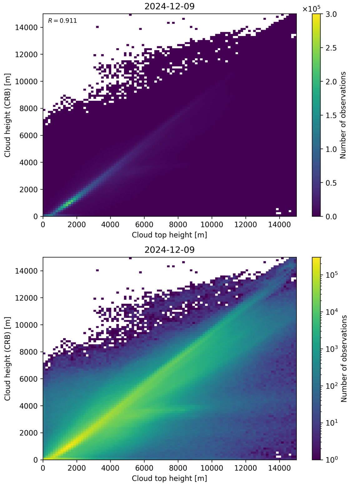
Figure 89: Scatter density plot of “Cloud top height” against “Cloud height (CRB)” for 2024-12-08 to 2024-12-10.
