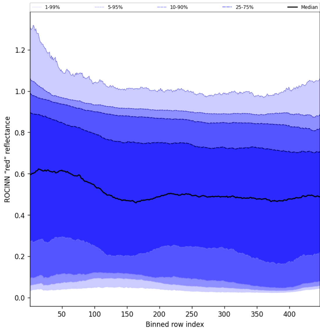
Figure 69: Along track statistics of "ROCINN "red" reflectance" for 2024-12-08 to 2024-12-10
