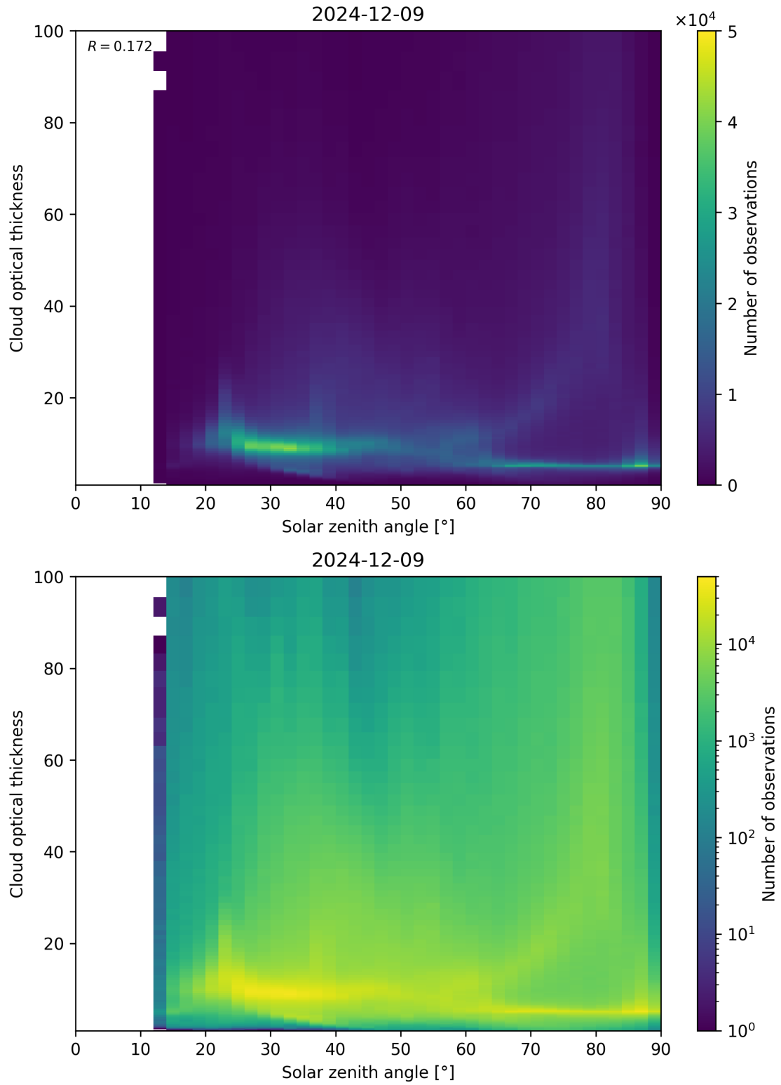
Figure 103: Scatter density plot of “Solar zenith angle” against “Cloud optical thickness” for 2024-12-08 to 2024-12-10.
