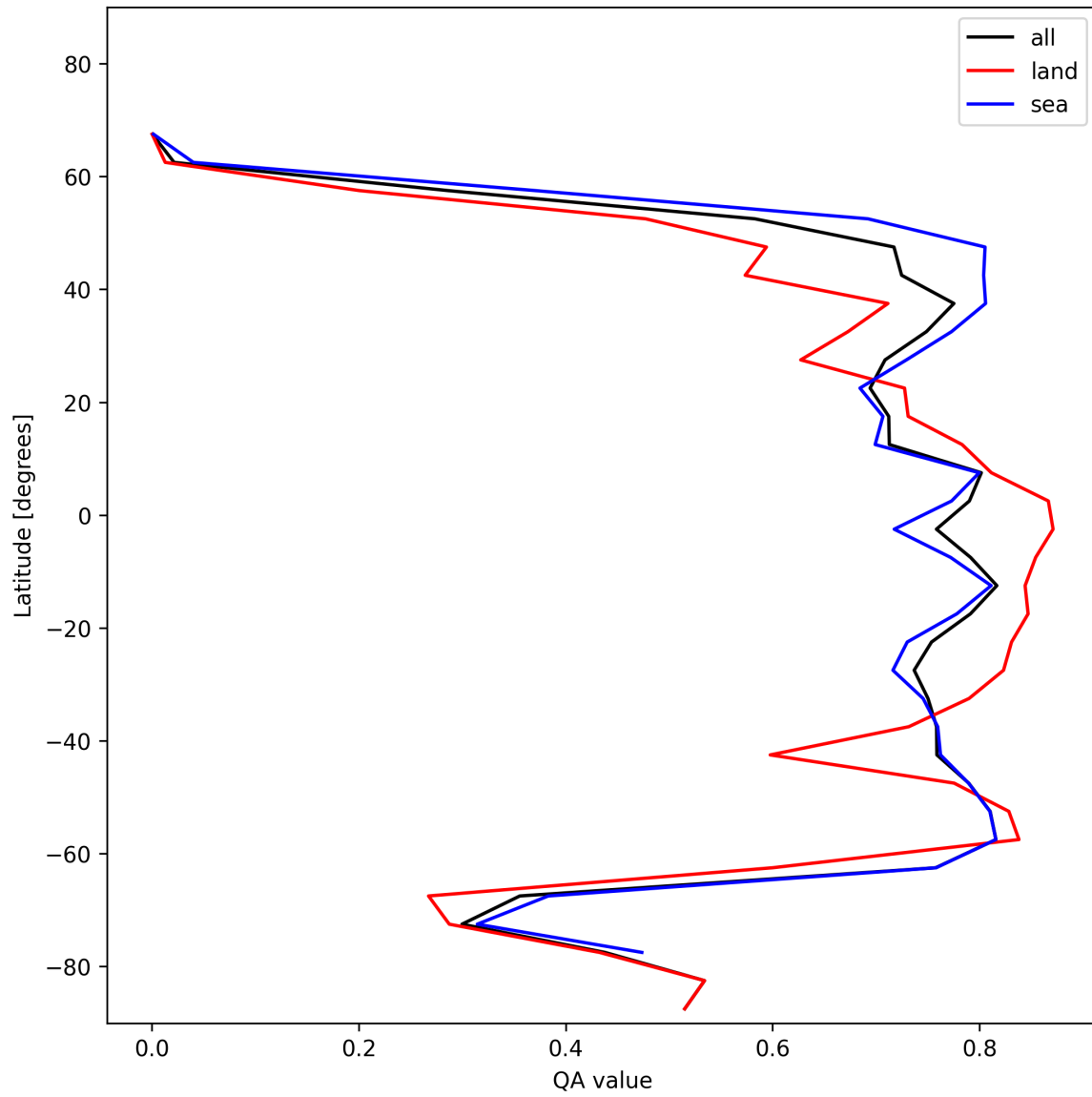
Figure 22: Zonal average of “QA value” for 2024-12-08 to 2024-12-10.
