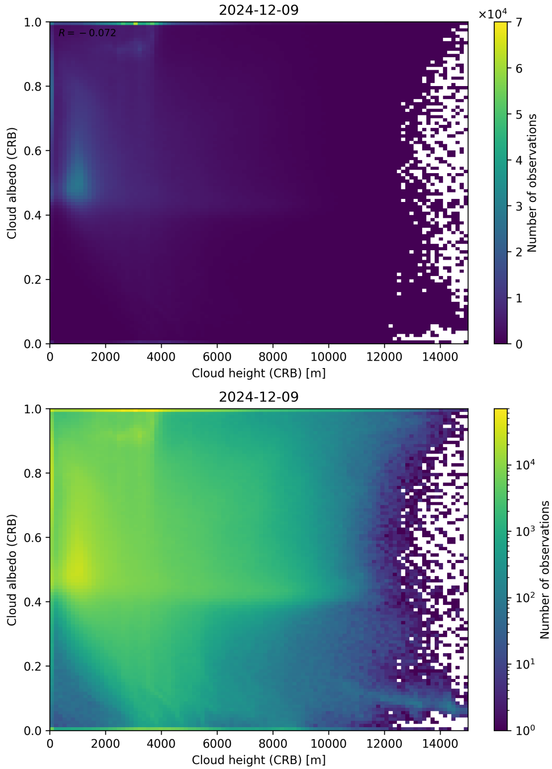
Figure 80: Scatter density plot of “Cloud height (CRB)” against “Cloud albedo (CRB)” for 2024-12-08 to 2024-12-10.
