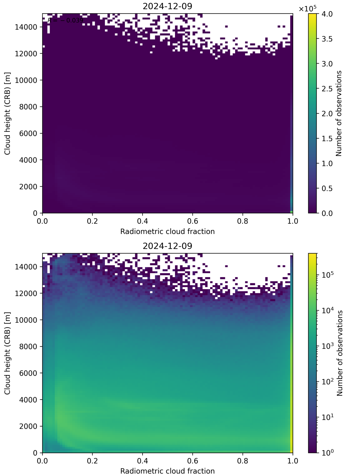
Figure 74: Scatter density plot of “Radiometric cloud fraction” against “Cloud height (CRB)” for 2024-12-08 to 2024-12-10.
