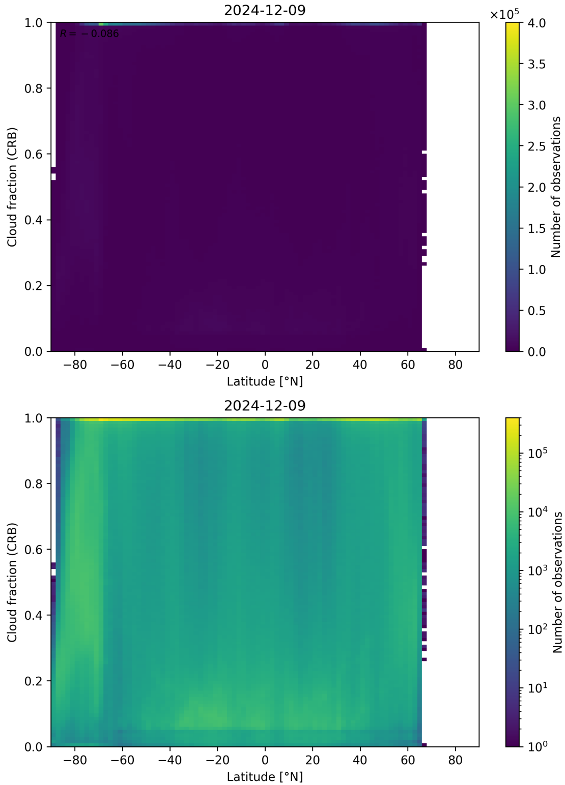
Figure 94: Scatter density plot of “Latitude” against “Cloud fraction (CRB)” for 2024-12-08 to 2024-12-10.
