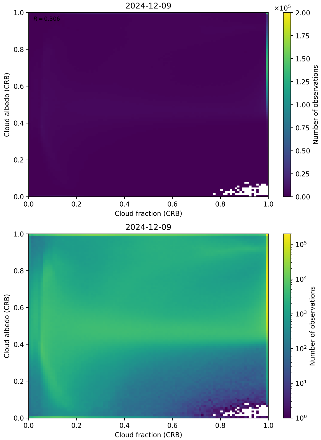
Figure 77: Scatter density plot of “Cloud fraction (CRB)” against “Cloud albedo (CRB)” for 2024-12-08 to 2024-12-10.
