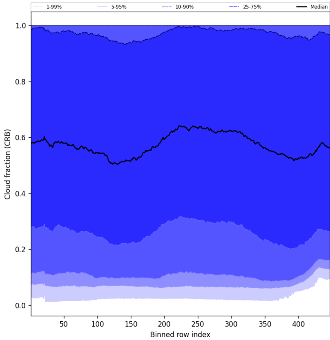
Figure 58: Along track statistics of “Cloud fraction (CRB)” for 2024-12-08 to 2024-12-10
