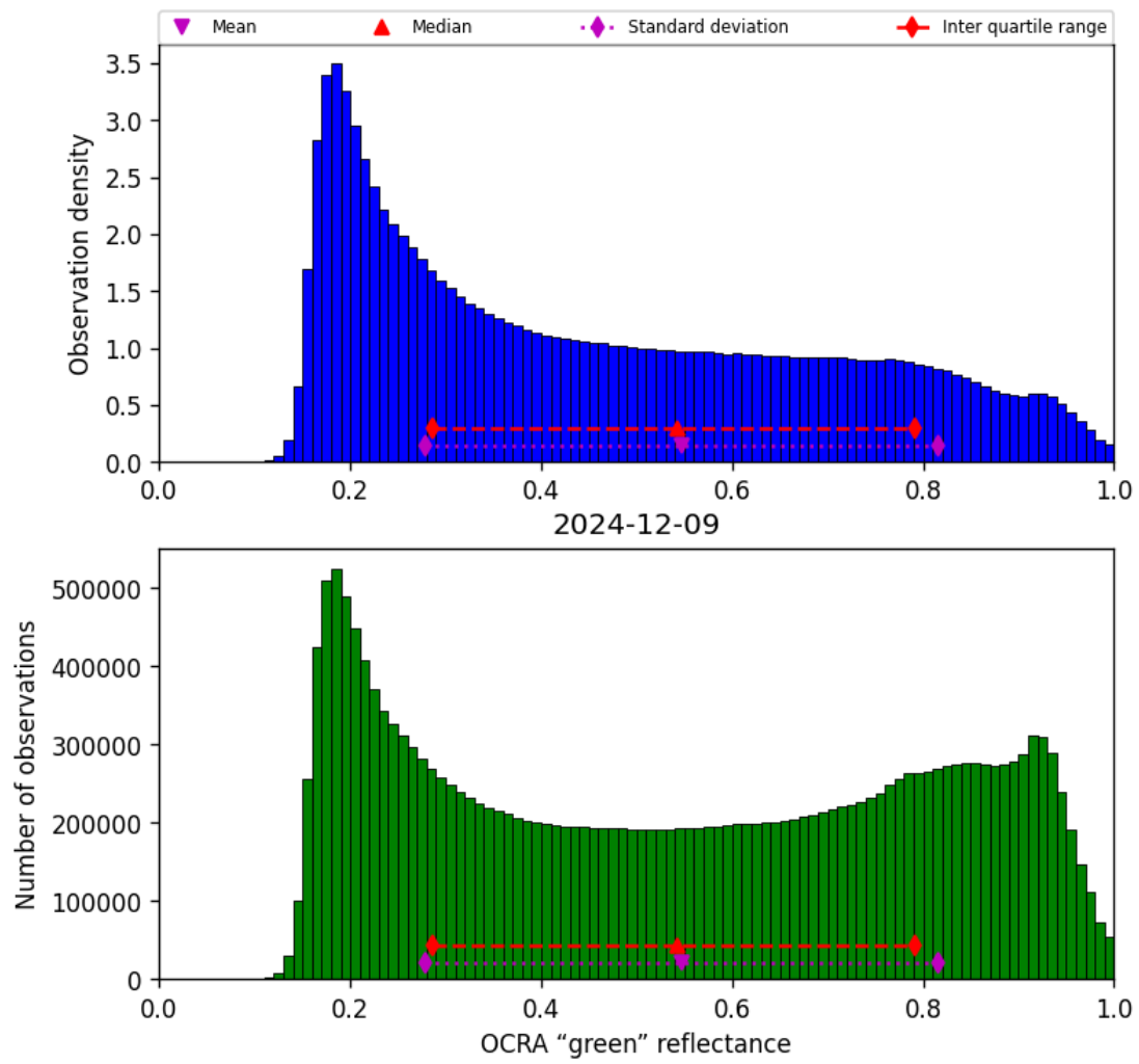
Figure 52: Histogram of “OCRA “green” reflectance” for 2024-12-08 to 2024-12-10
