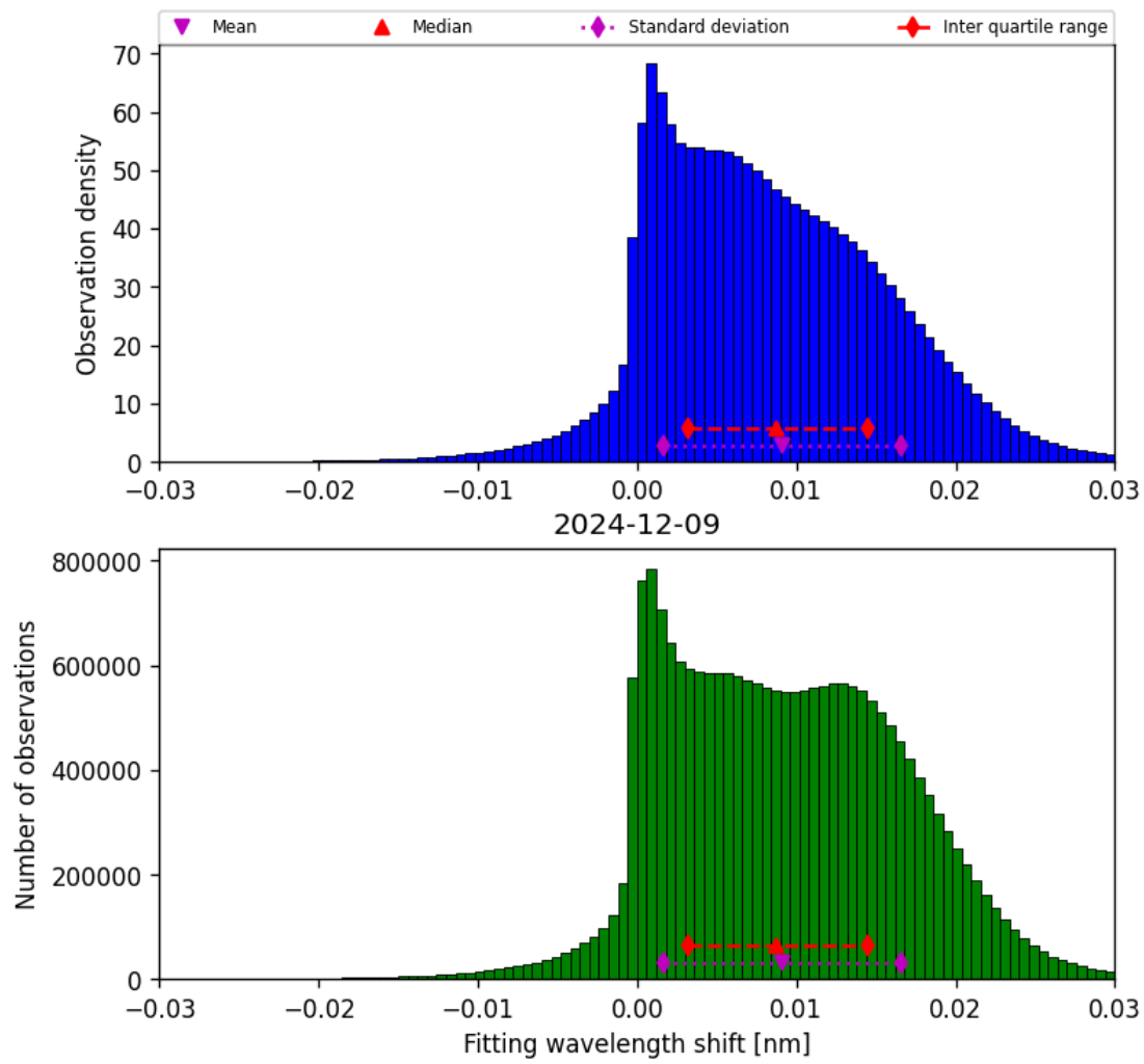
Figure 49: Histogram of “Fitting wavelength shift” for 2024-12-08 to 2024-12-10
