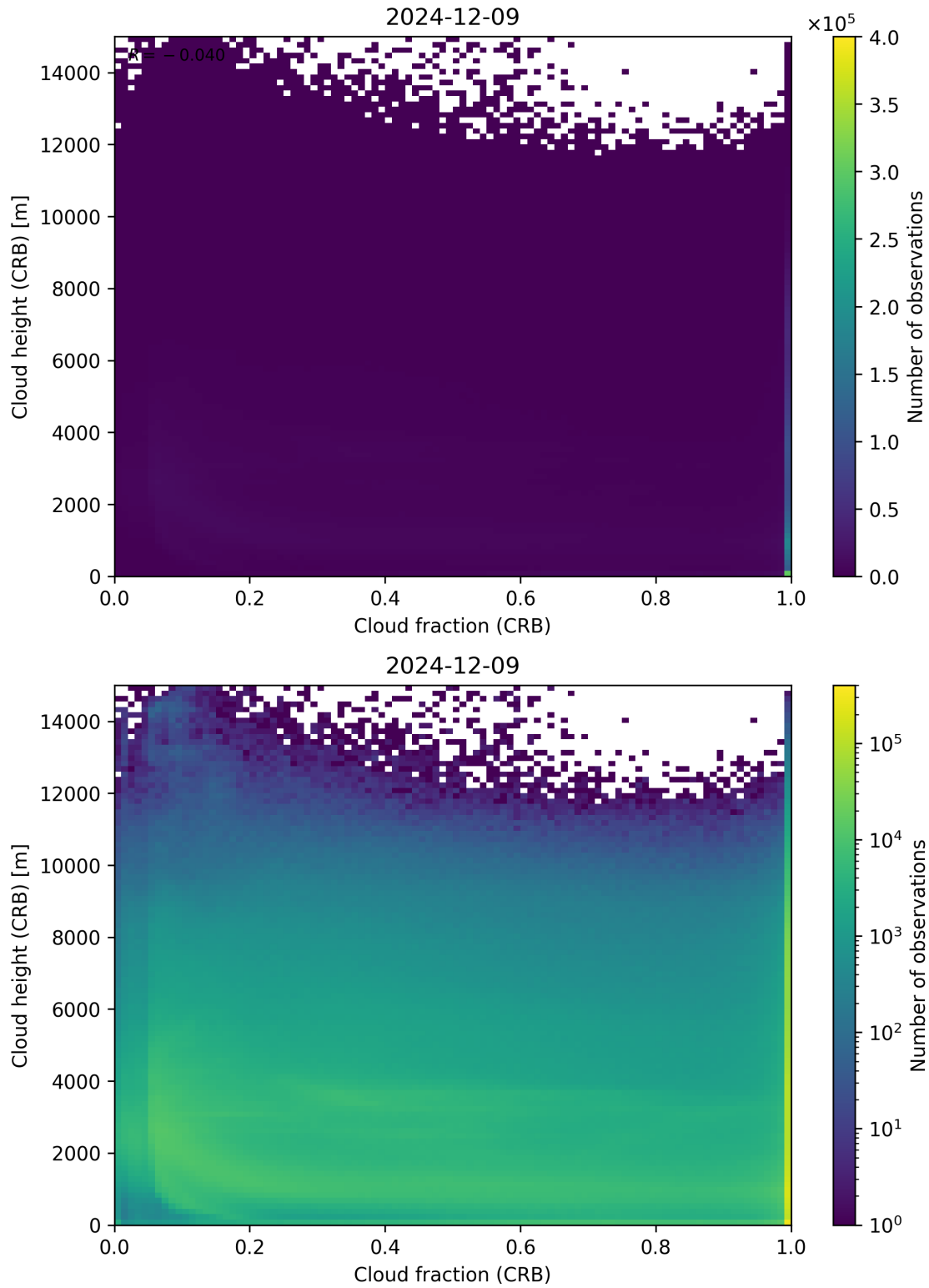
Figure 79: Scatter density plot of “Cloud fraction (CRB)” against “Cloud height (CRB)” for 2024-12-08 to 2024-12-10.
