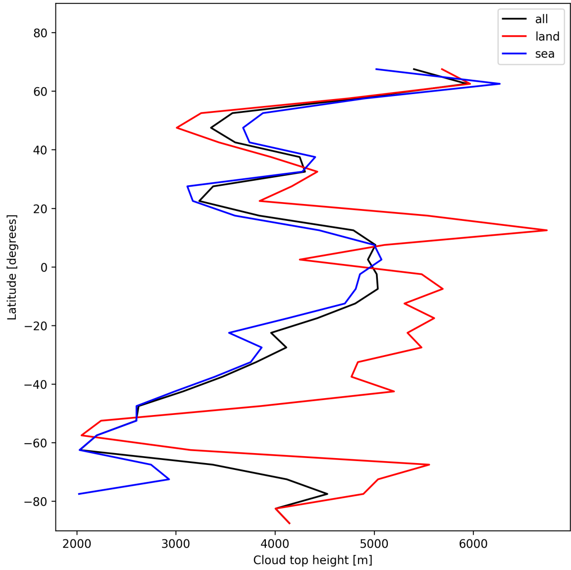
Figure 24: Zonal average of “Cloud top height” for 2024-12-09 to 2024-12-11.
