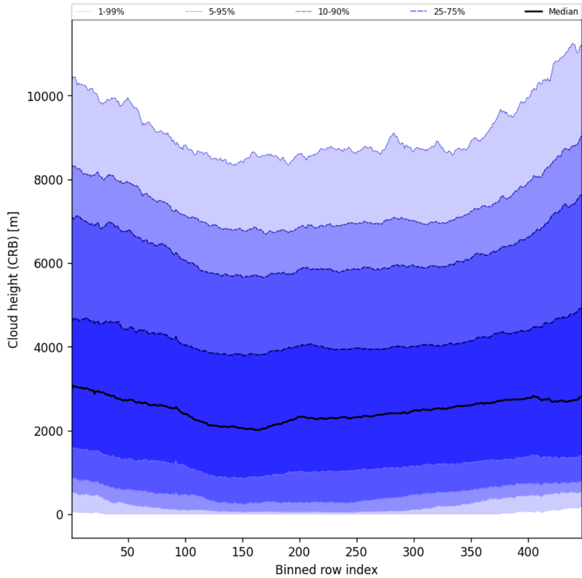
Figure 59: Along track statistics of “Cloud height (CRB)” for 2024-12-09 to 2024-12-11
