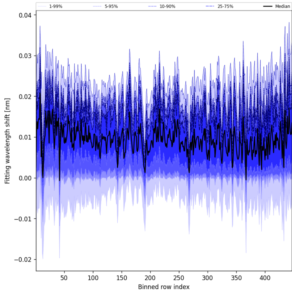
Figure 65: Along track statistics of “Fitting wavelength shift” for 2024-12-09 to 2024-12-11
