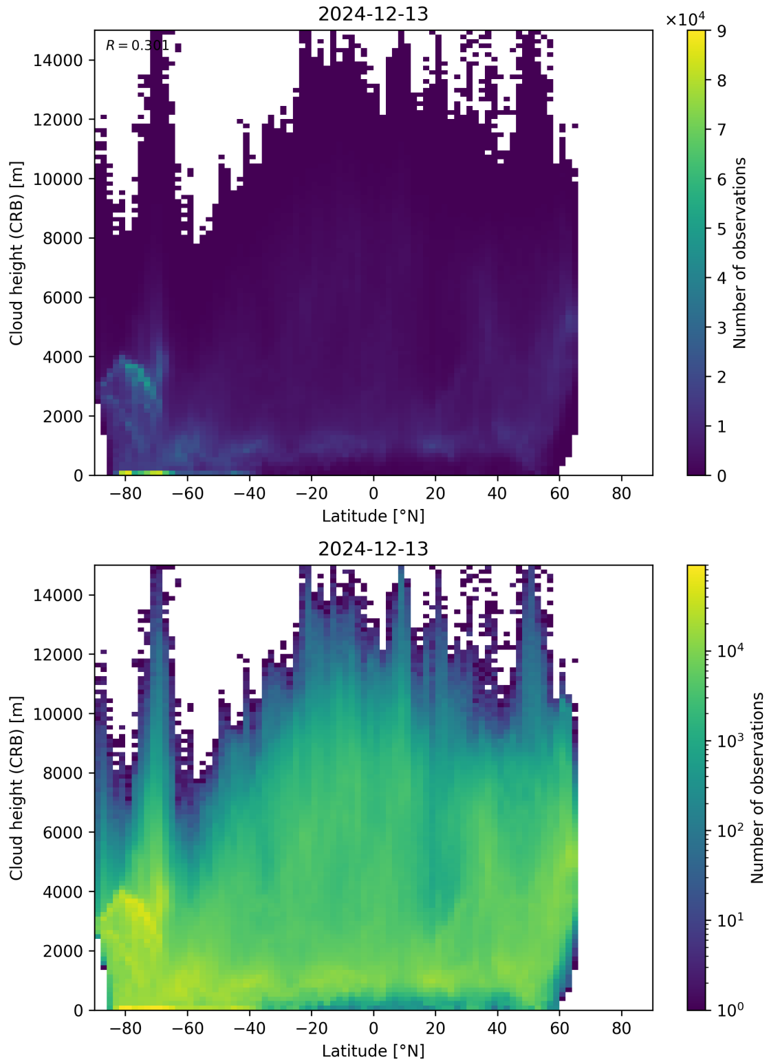
Figure 95: Scatter density plot of “Latitude” against “Cloud height (CRB)” for 2024-12-12 to 2024-12-14.
