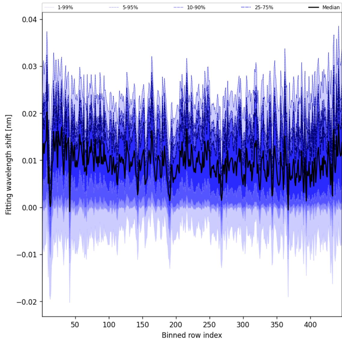
Figure 65: Along track statistics of “Fitting wavelength shift” for 2024-12-12 to 2024-12-14
