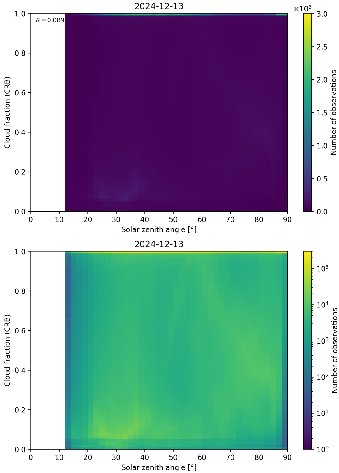
Figure 101: Scatter density plot of “Solar zenith angle” against “Cloud fraction (CRB)” for 2024-12-12 to 2024-12-14.
