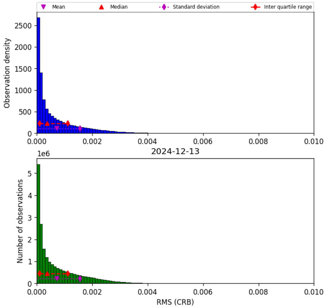
Figure 48: Histogram of “RMS (CRB)” for 2024-12-12 to 2024-12-14
