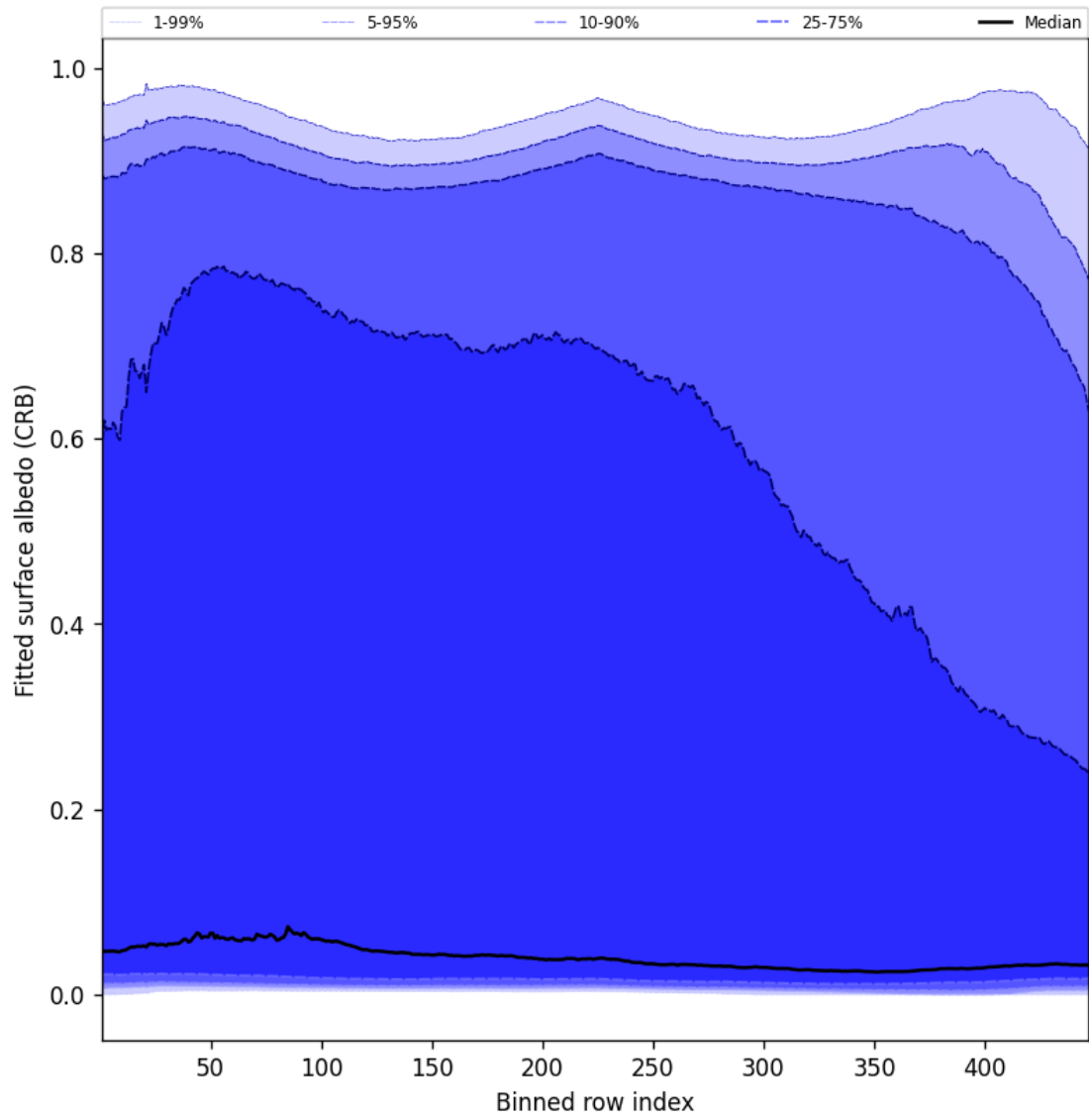
Figure 62: Along track statistics of “Fitted surface albedo (CRB)” for 2024-12-12 to 2024-12-14
