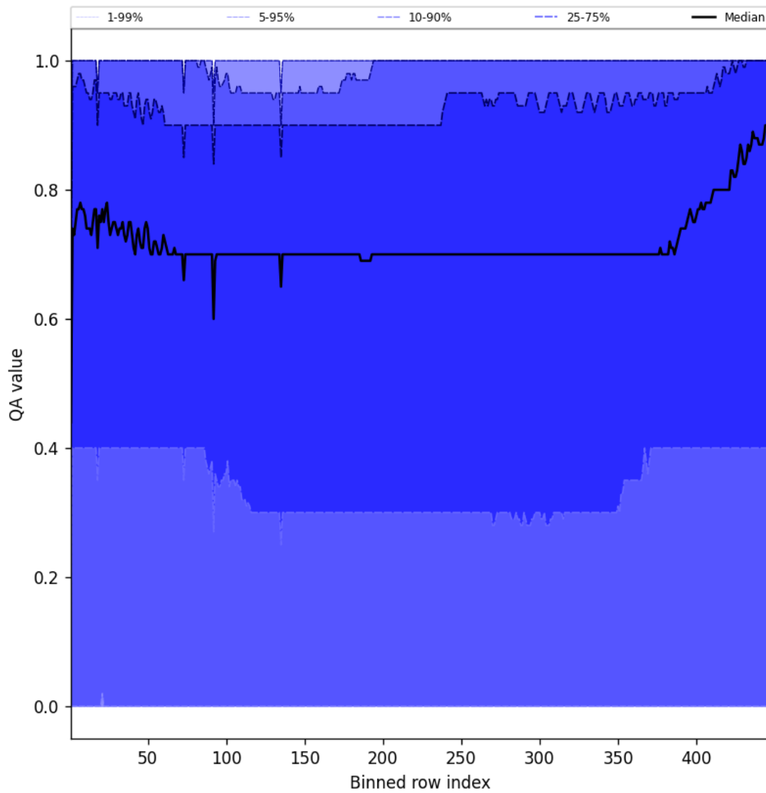
Figure 54: Along track statistics of “QA value” for 2024-12-12 to 2024-12-14
