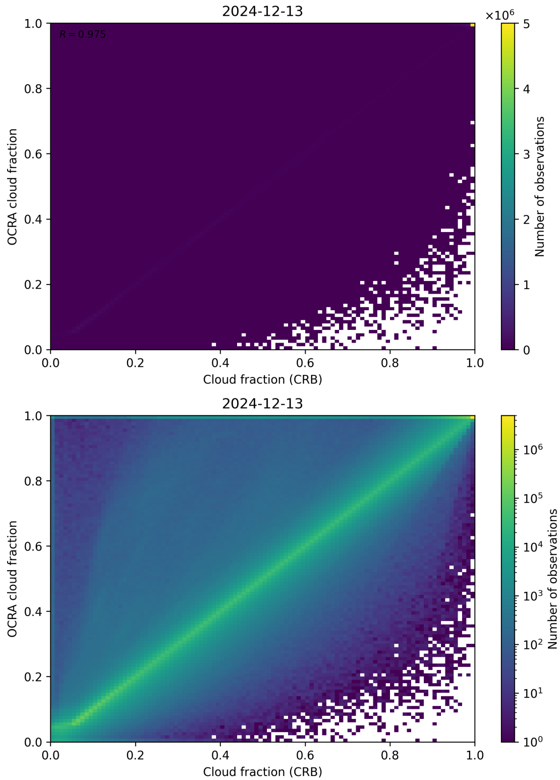
Figure 78: Scatter density plot of “Cloud fraction (CRB)” against “OCRA cloud fraction” for 2024-12-12 to 2024-12-14.
