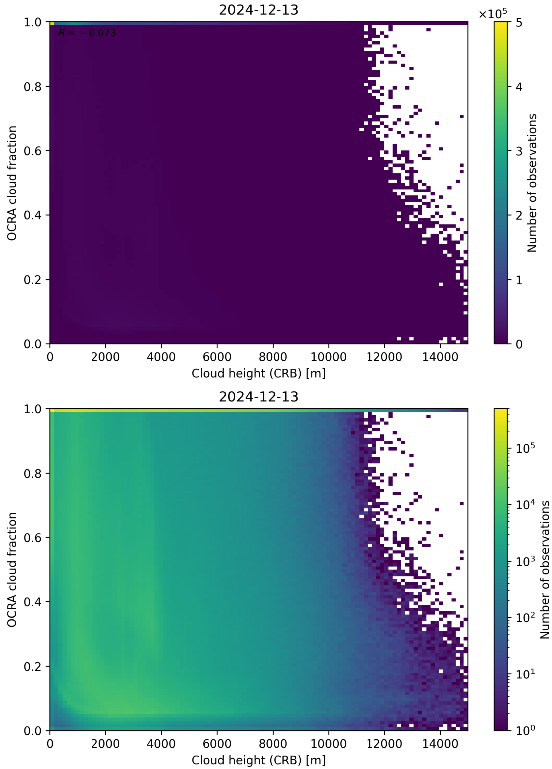
Figure 81: Scatter density plot of “Cloud height (CRB)” against “OCRA cloud fraction” for 2024-12-12 to 2024-12-14.
