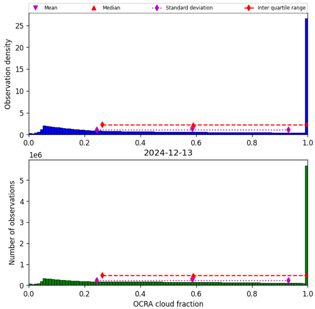
Figure 50: Histogram of “OCRA cloud fraction” for 2024-12-12 to 2024-12-14
