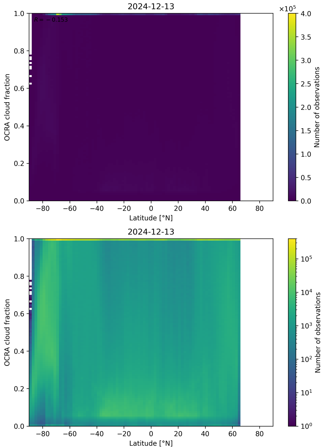
Figure 93: Scatter density plot of “Latitude” against “OCRA cloud fraction” for 2024-12-12 to 2024-12-14.
