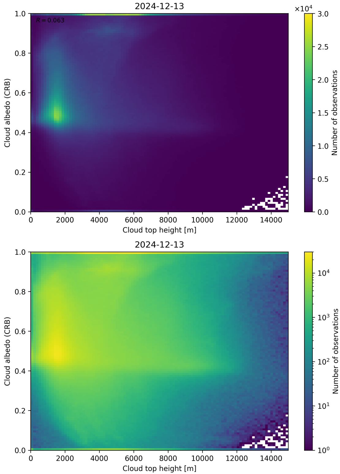
Figure 86: Scatter density plot of “Cloud top height” against “Cloud albedo (CRB)” for 2024-12-12 to 2024-12-14.
