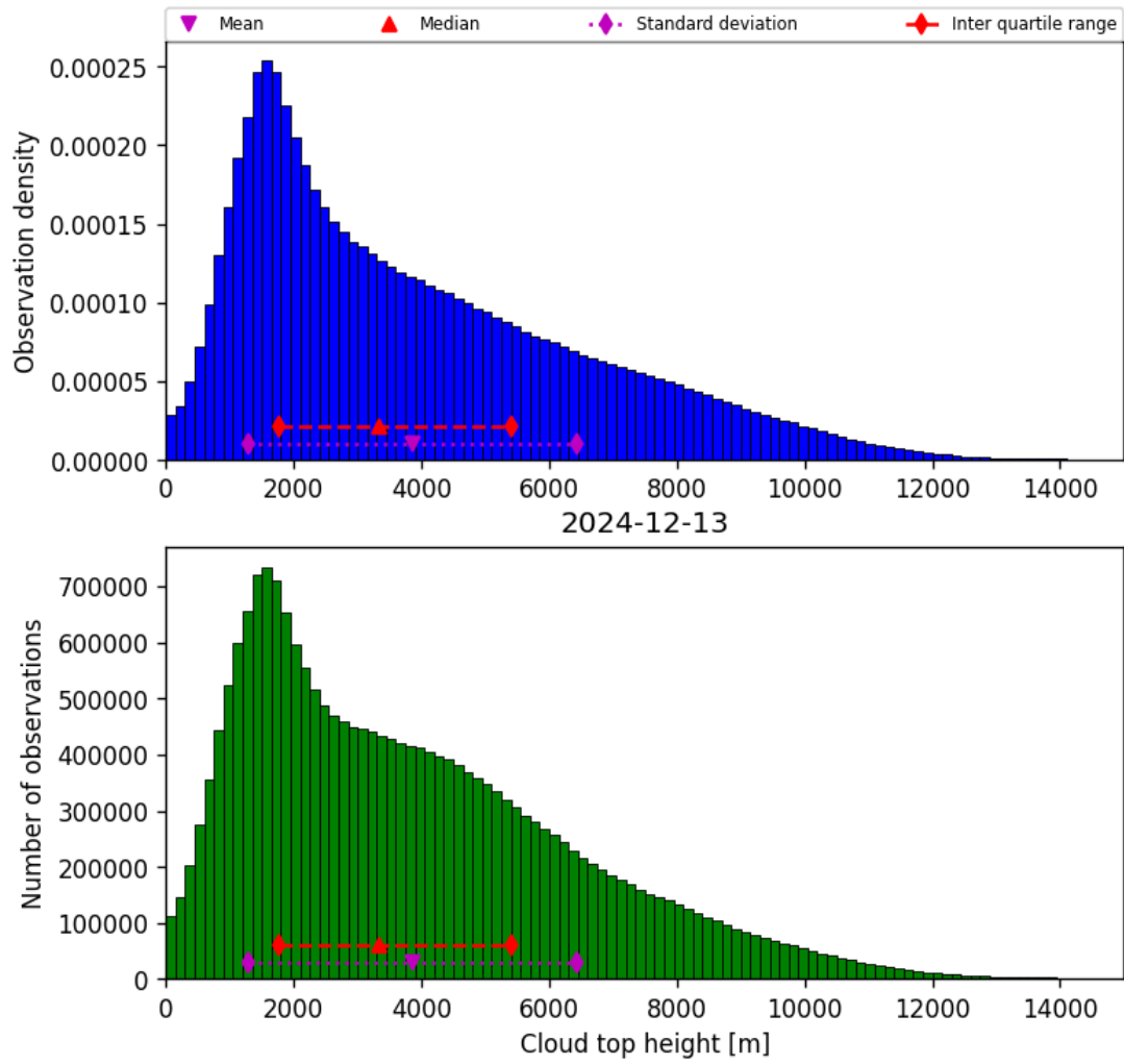
Figure 40: Histogram of “Cloud top height” for 2024-12-12 to 2024-12-14
