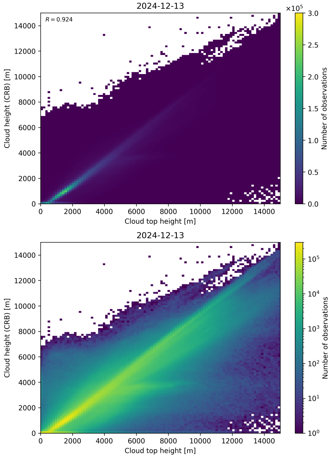
Figure 89: Scatter density plot of “Cloud top height” against “Cloud height (CRB)” for 2024-12-12 to 2024-12-14.
