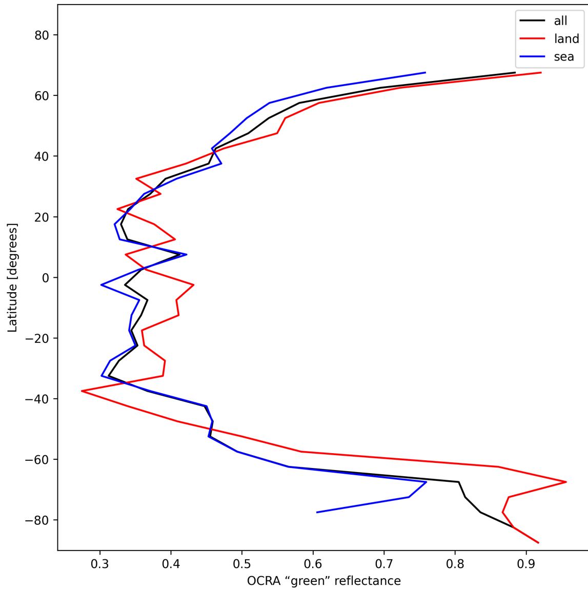
Figure 36: Zonal average of “OCRA “green” reflectance” for 2024-12-12 to 2024-12-14.
