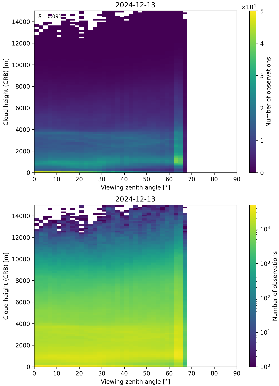
Figure 110: Scatter density plot of “Viewing zenith angle” against “Cloud height (CRB)” for 2024-12-12 to 2024-12-14.
