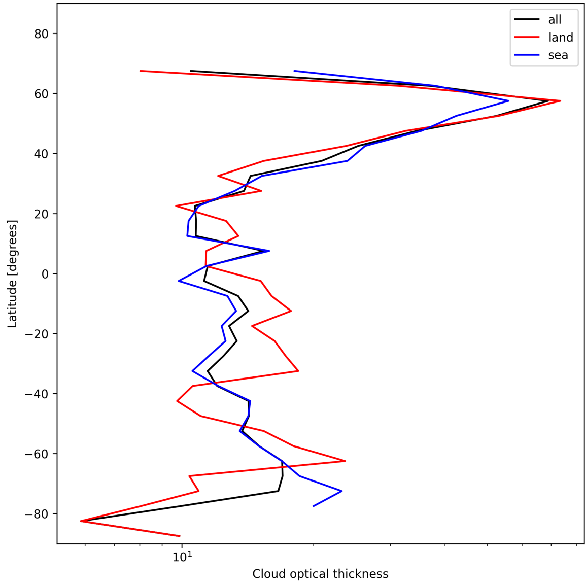
Figure 25: Zonal average of “Cloud optical thickness” for 2024-12-12 to 2024-12-14.
