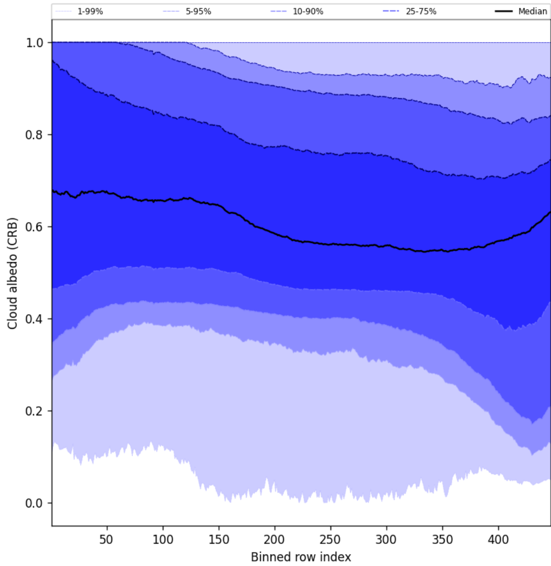
Figure 60: Along track statistics of “Cloud albedo (CRB)” for 2024-12-12 to 2024-12-14
