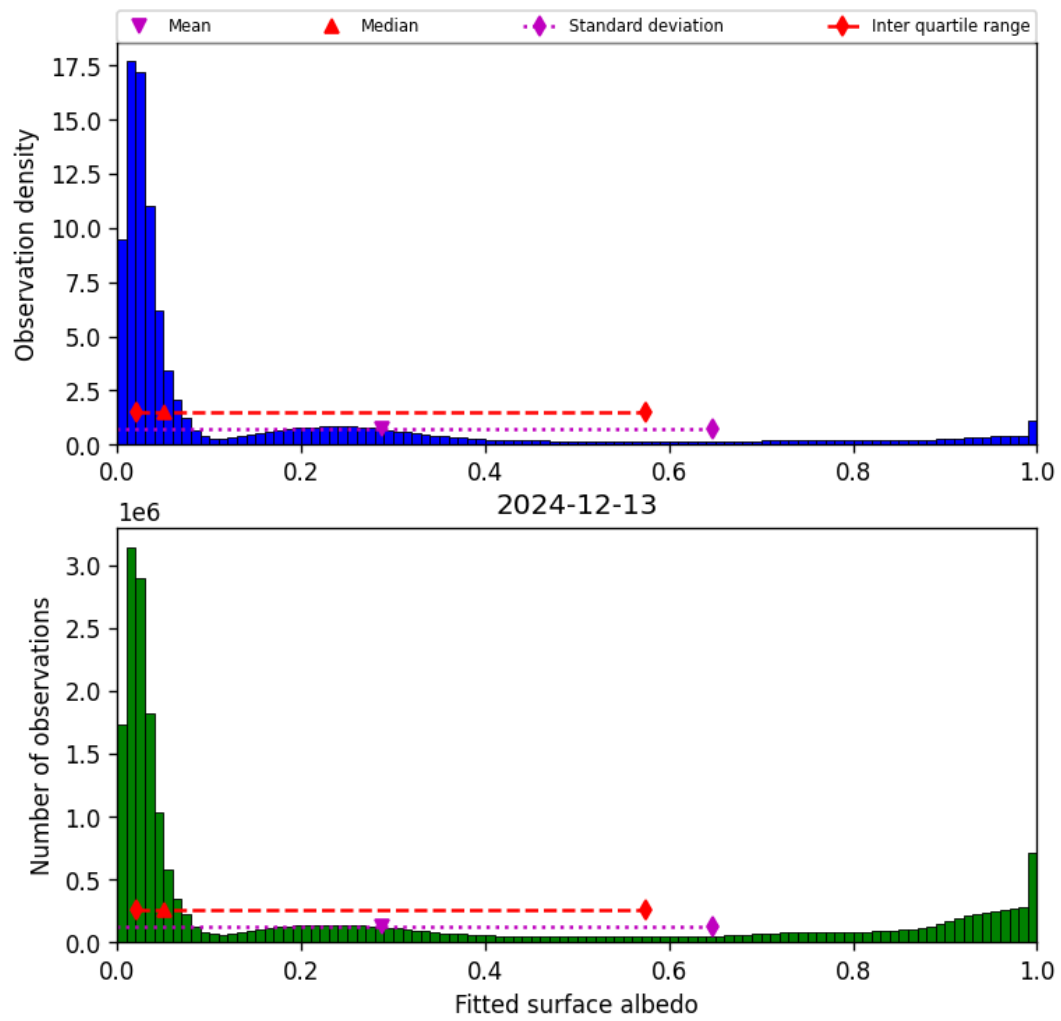
Figure 45: Histogram of “Fitted surface albedo” for 2024-12-12 to 2024-12-14
