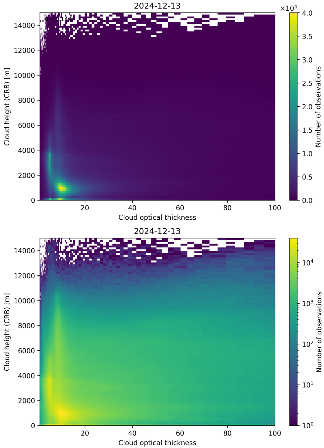
Figure 85: Scatter density plot of “Cloud optical thickness” against “Cloud height (CRB)” for 2024-12-12 to 2024-12-14.
