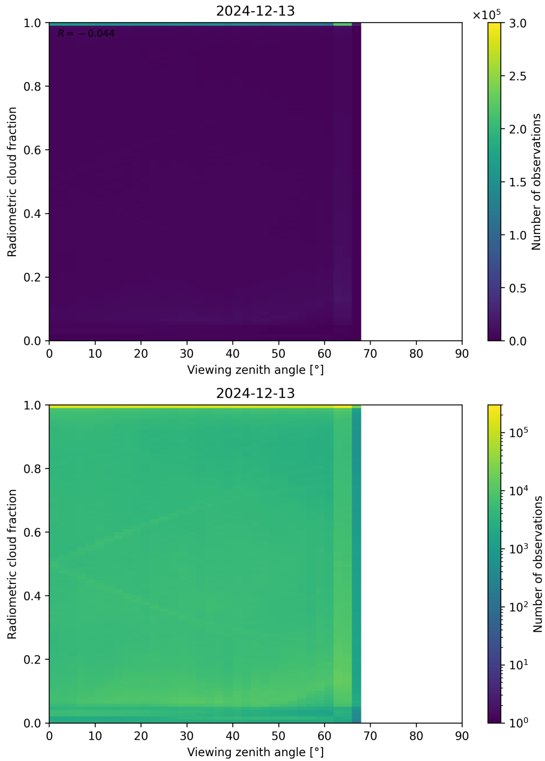
Figure 107: Scatter density plot of “Viewing zenith angle” against “Radiometric cloud fraction” for 2024-12-12 to 2024-12-14.
