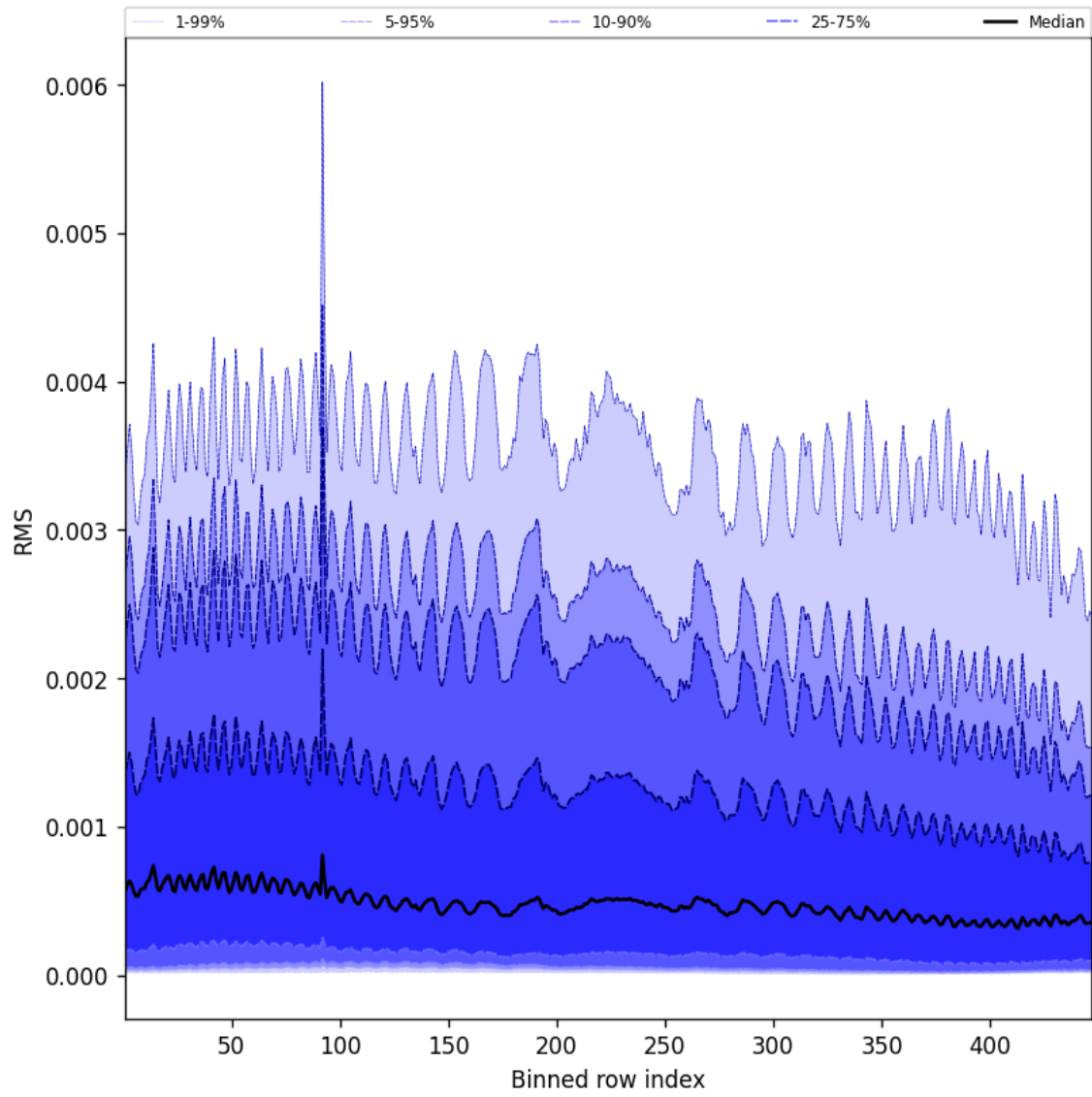
Figure 63: Along track statistics of “RMS” for 2024-12-12 to 2024-12-14
