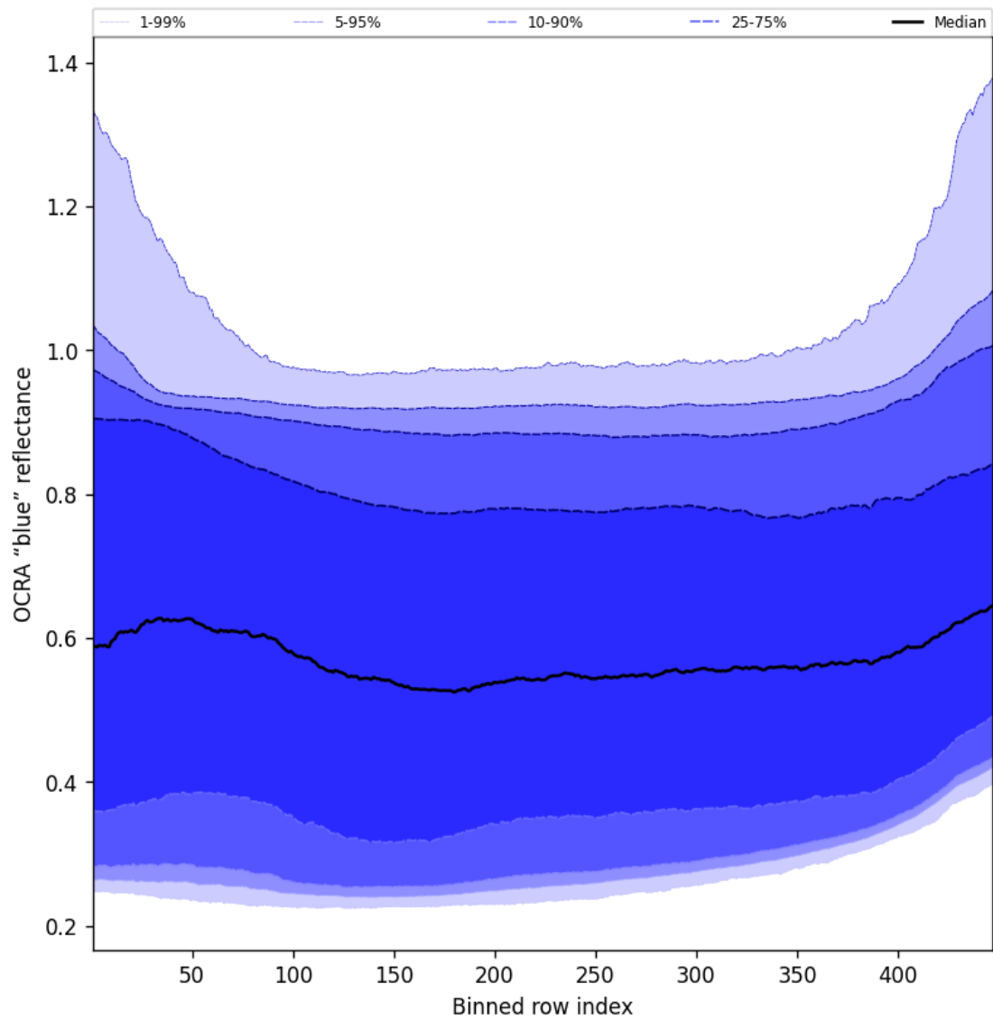
Figure 67: Along track statistics of “OCRA “blue” reflectance” for 2024-12-12 to 2024-12-14
