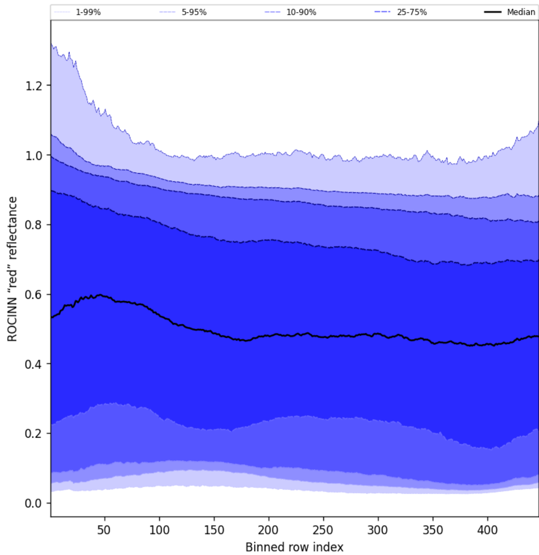
Figure 69: Along track statistics of “ROCINN “red” reflectance” for 2024-12-12 to 2024-12-14
