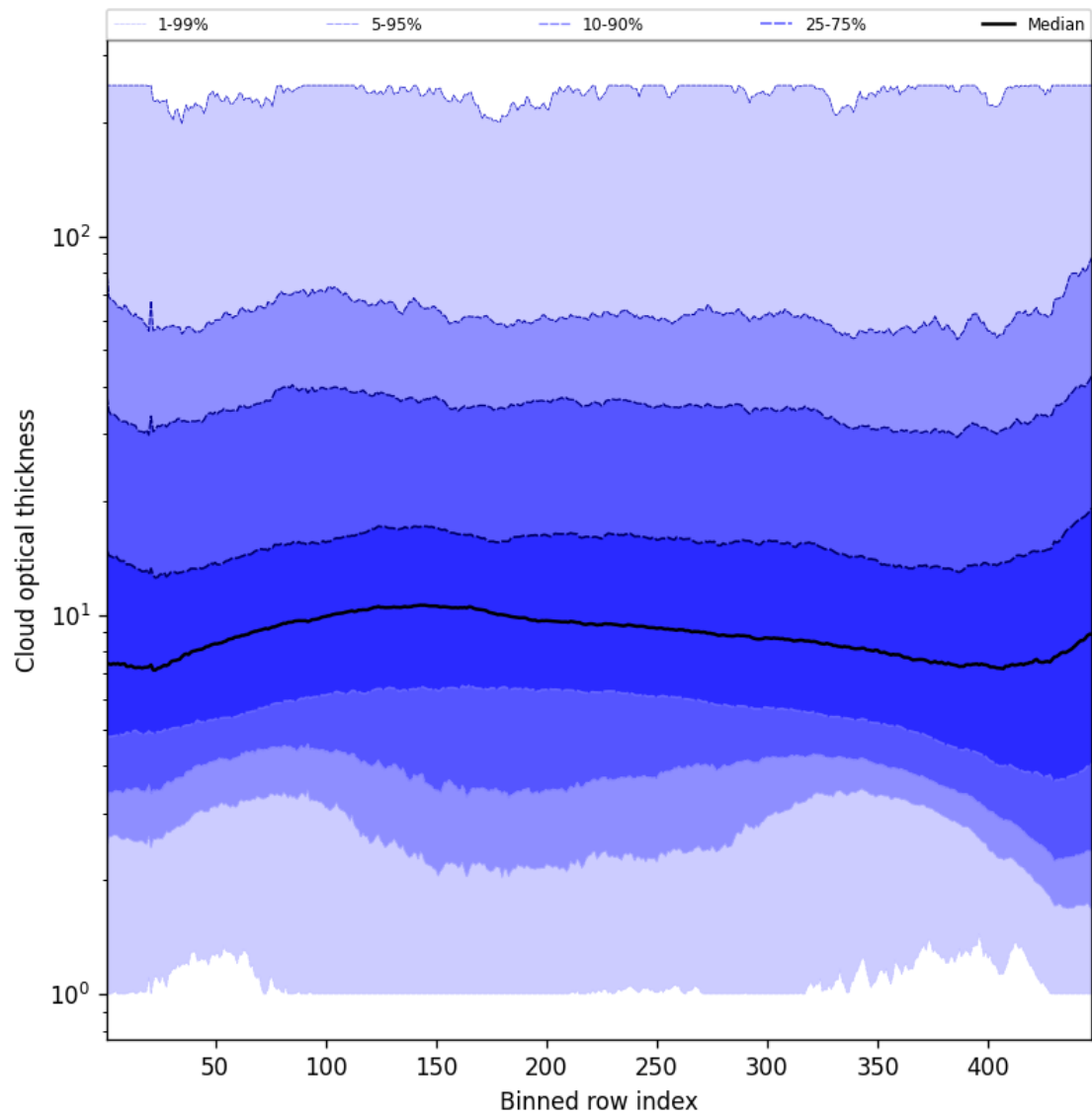
Figure 57: Along track statistics of “Cloud optical thickness” for 2024-12-12 to 2024-12-14
