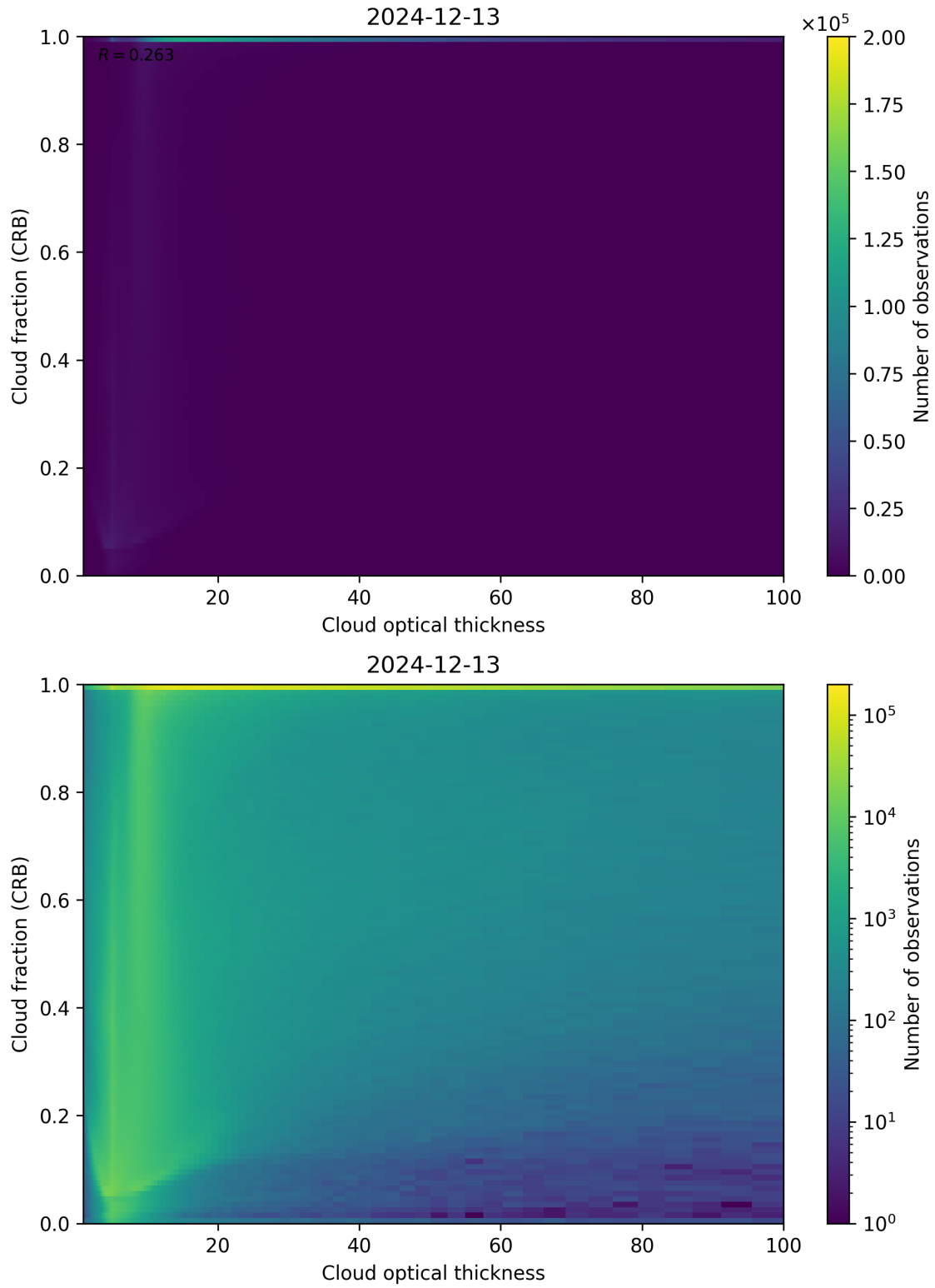
Figure 84: Scatter density plot of “Cloud optical thickness” against “Cloud fraction (CRB)” for 2024-12-12 to 2024-12-14.
