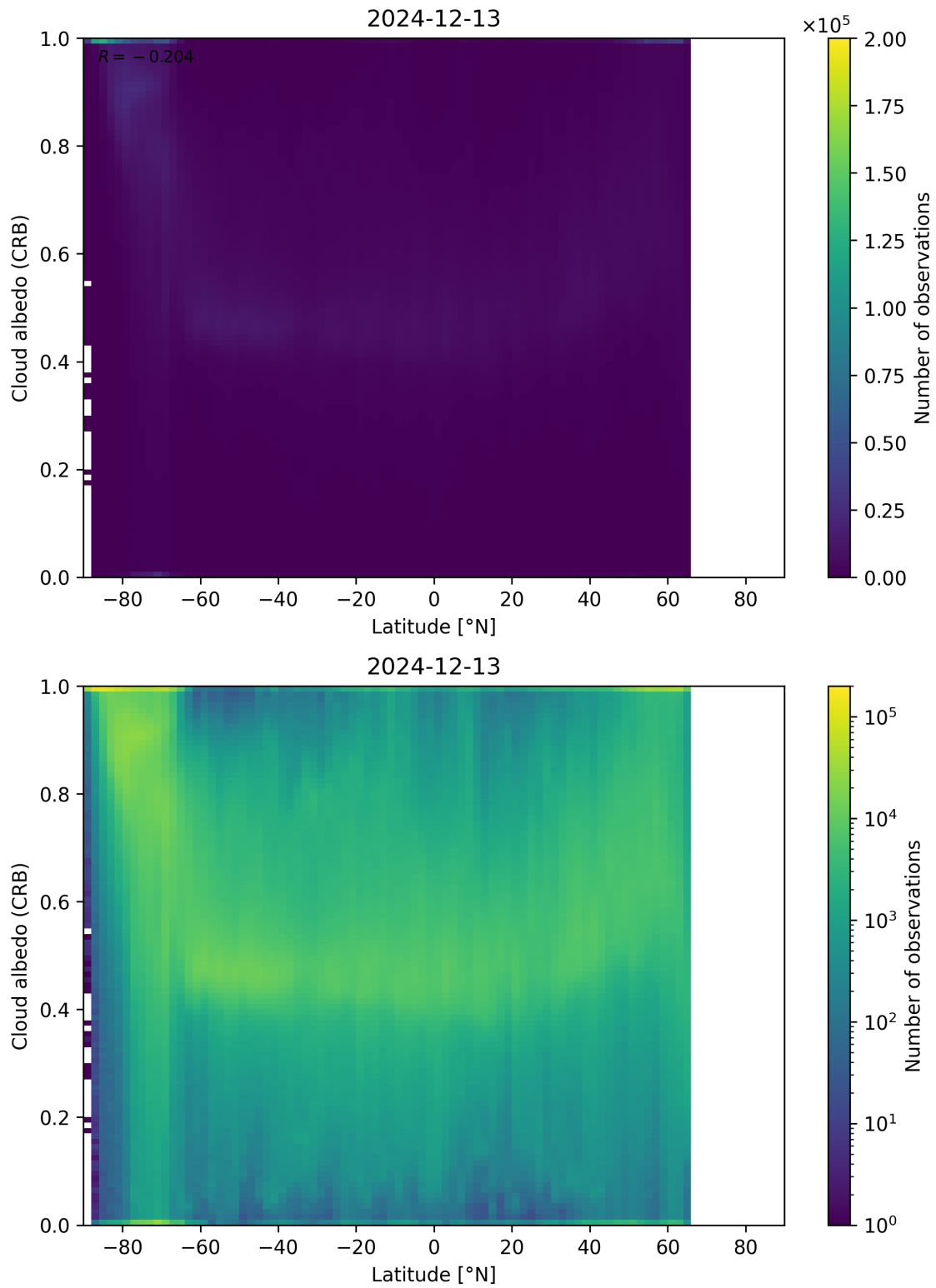
Figure 91: Scatter density plot of “Latitude” against “Cloud albedo (CRB)” for 2024-12-12 to 2024-12-14.
