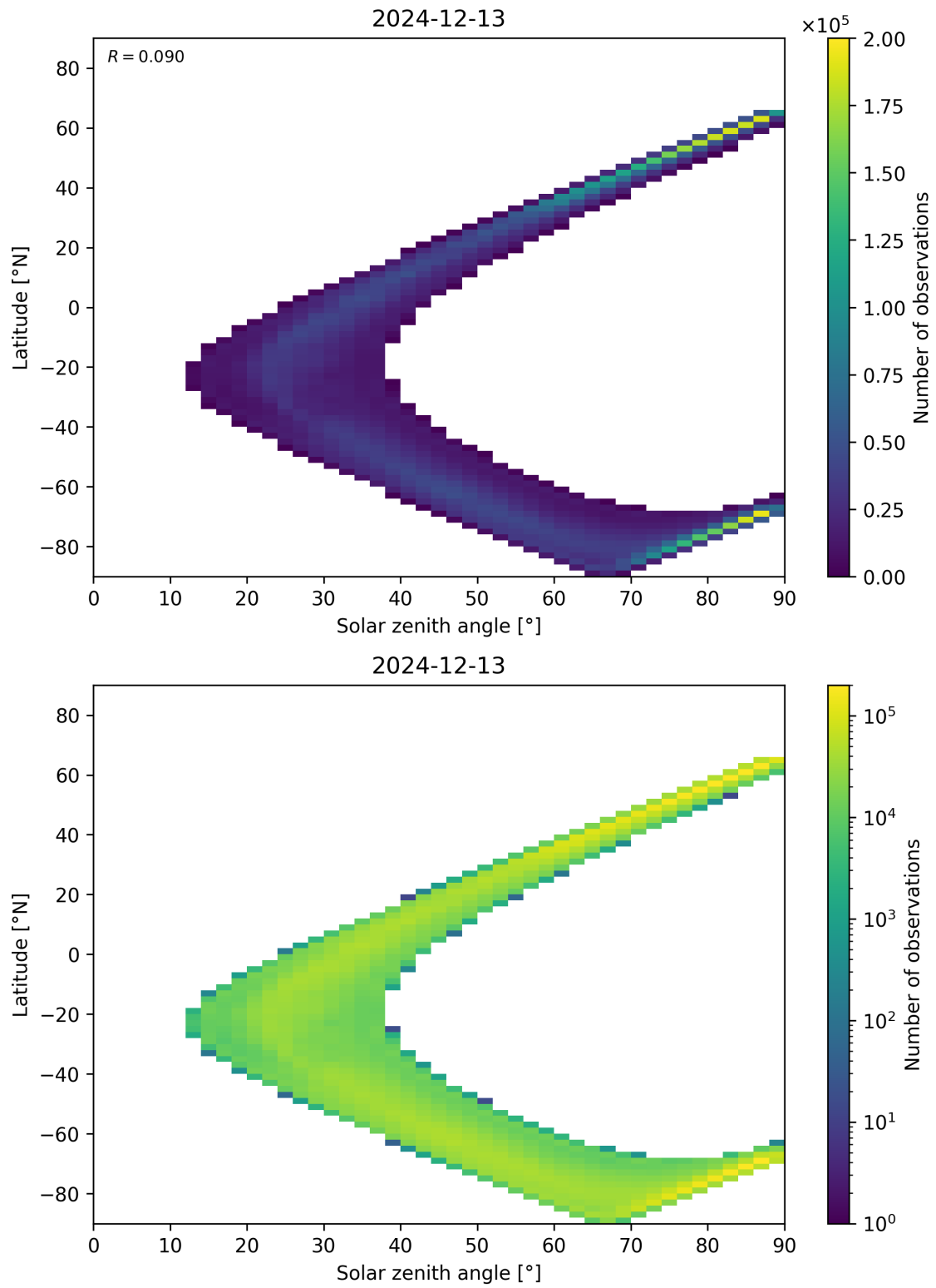
Figure 105: Scatter density plot of “Solar zenith angle” against “Latitude” for 2024-12-12 to 2024-12-14.
