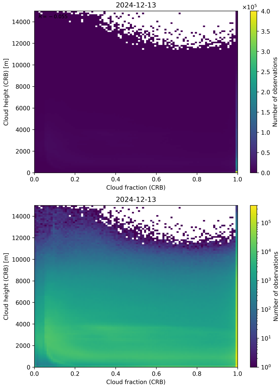
Figure 79: Scatter density plot of “Cloud fraction (CRB)” against “Cloud height (CRB)” for 2024-12-12 to 2024-12-14.
