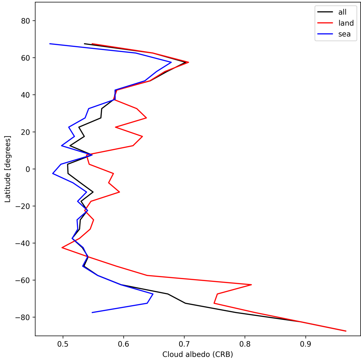
Figure 28: Zonal average of “Cloud albedo (CRB)” for 2024-12-12 to 2024-12-14.
