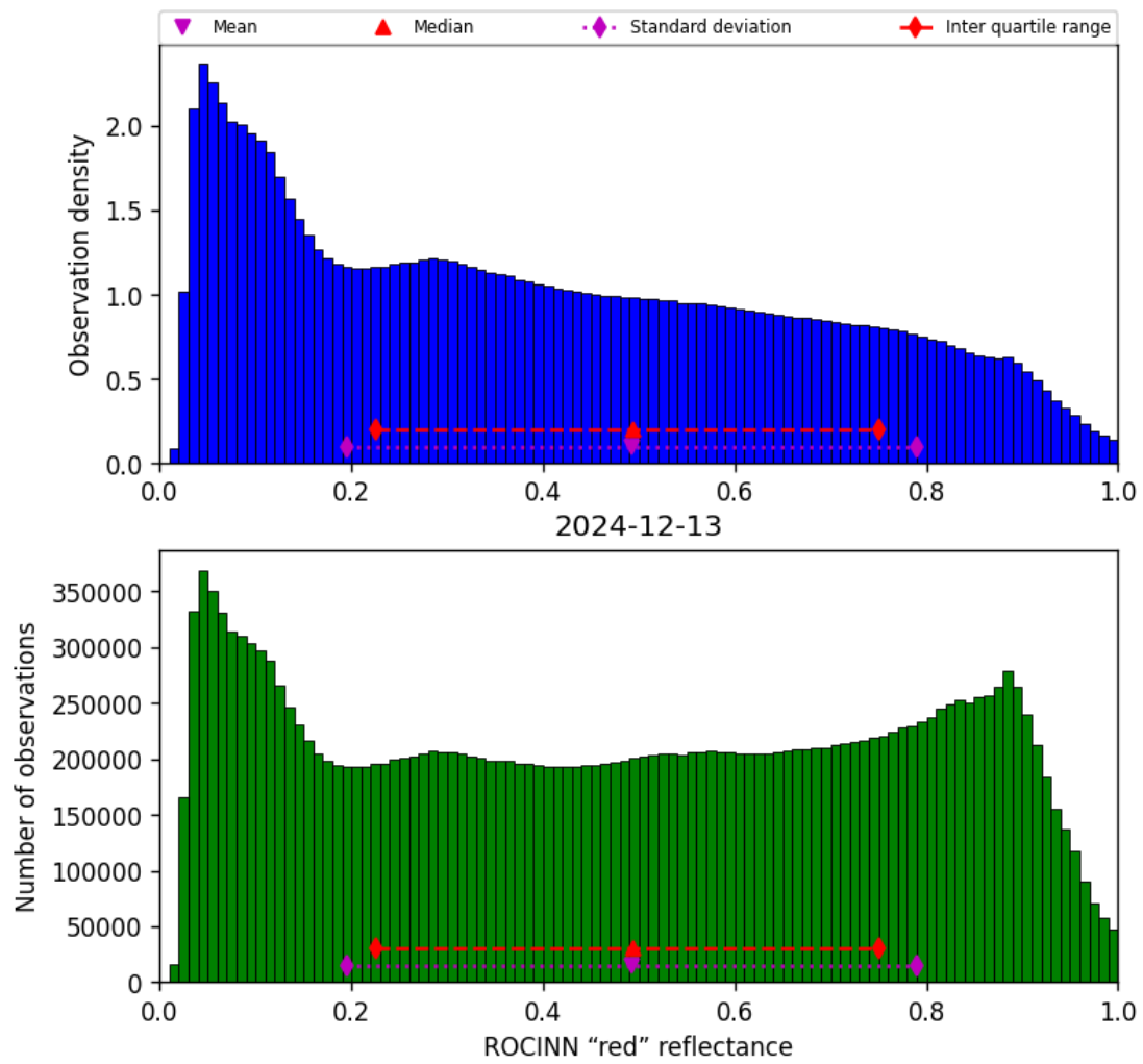
Figure 53: Histogram of “ROCINN “red” reflectance” for 2024-12-12 to 2024-12-14
