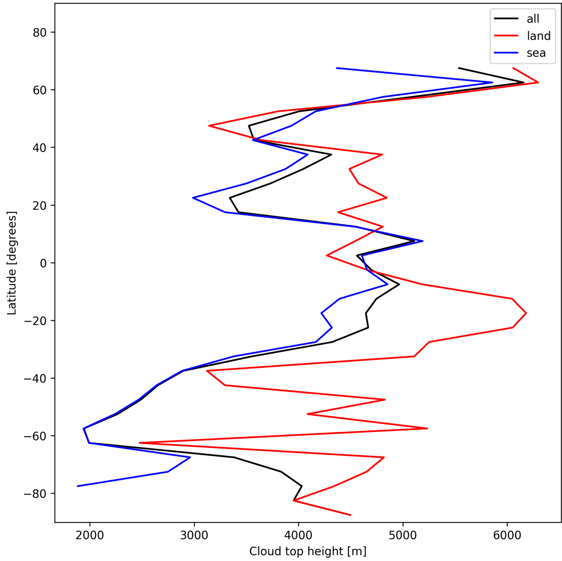
Figure 24: Zonal average of “Cloud top height” for 2024-12-12 to 2024-12-14.
