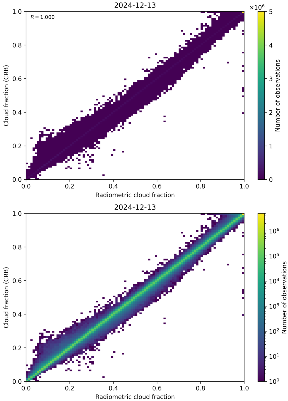
Figure 73: Scatter density plot of “Radiometric cloud fraction” against “Cloud fraction (CRB)” for 2024-12-12 to 2024-12-14.
