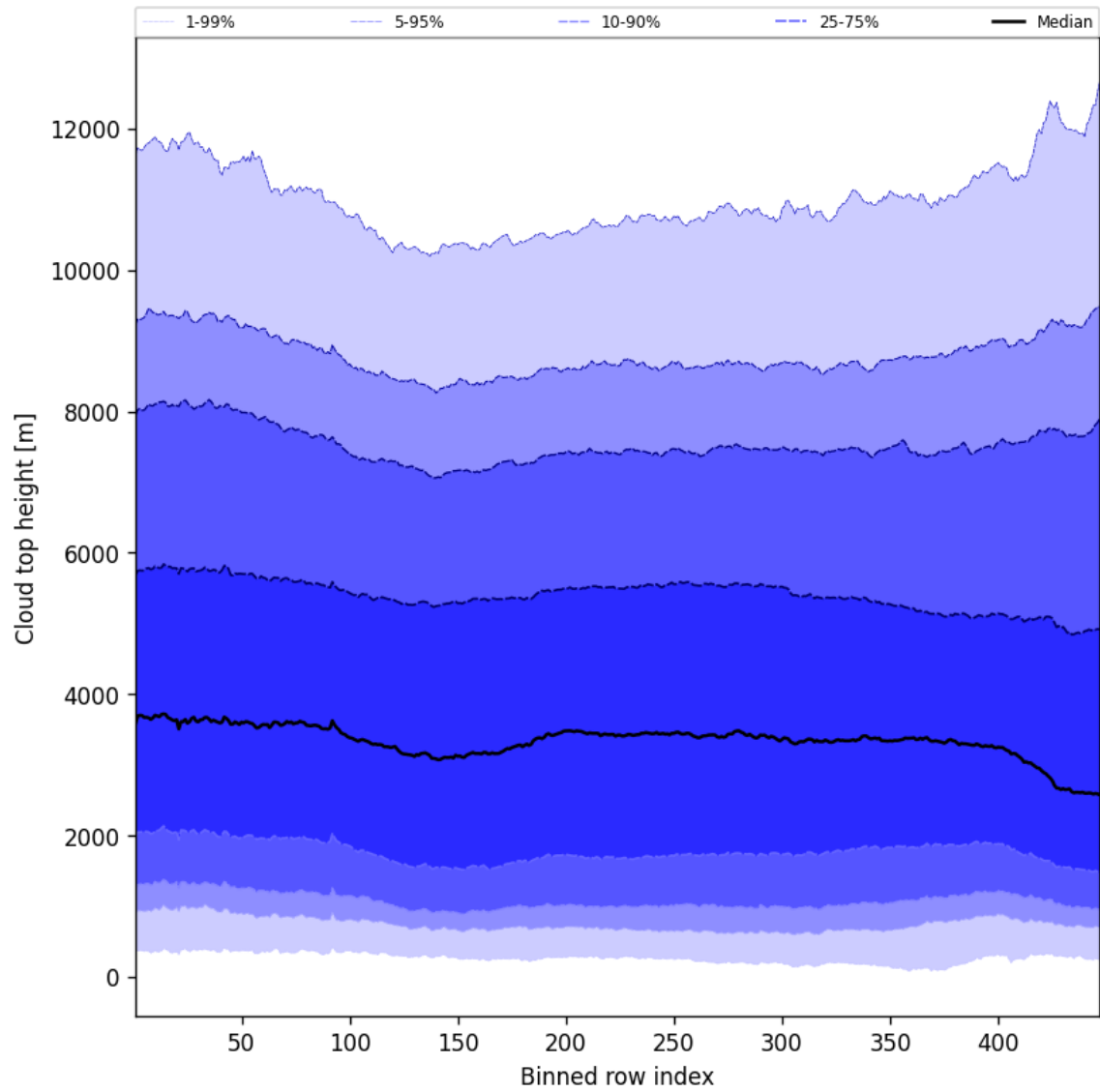
Figure 56: Along track statistics of “Cloud top height” for 2024-12-12 to 2024-12-14
