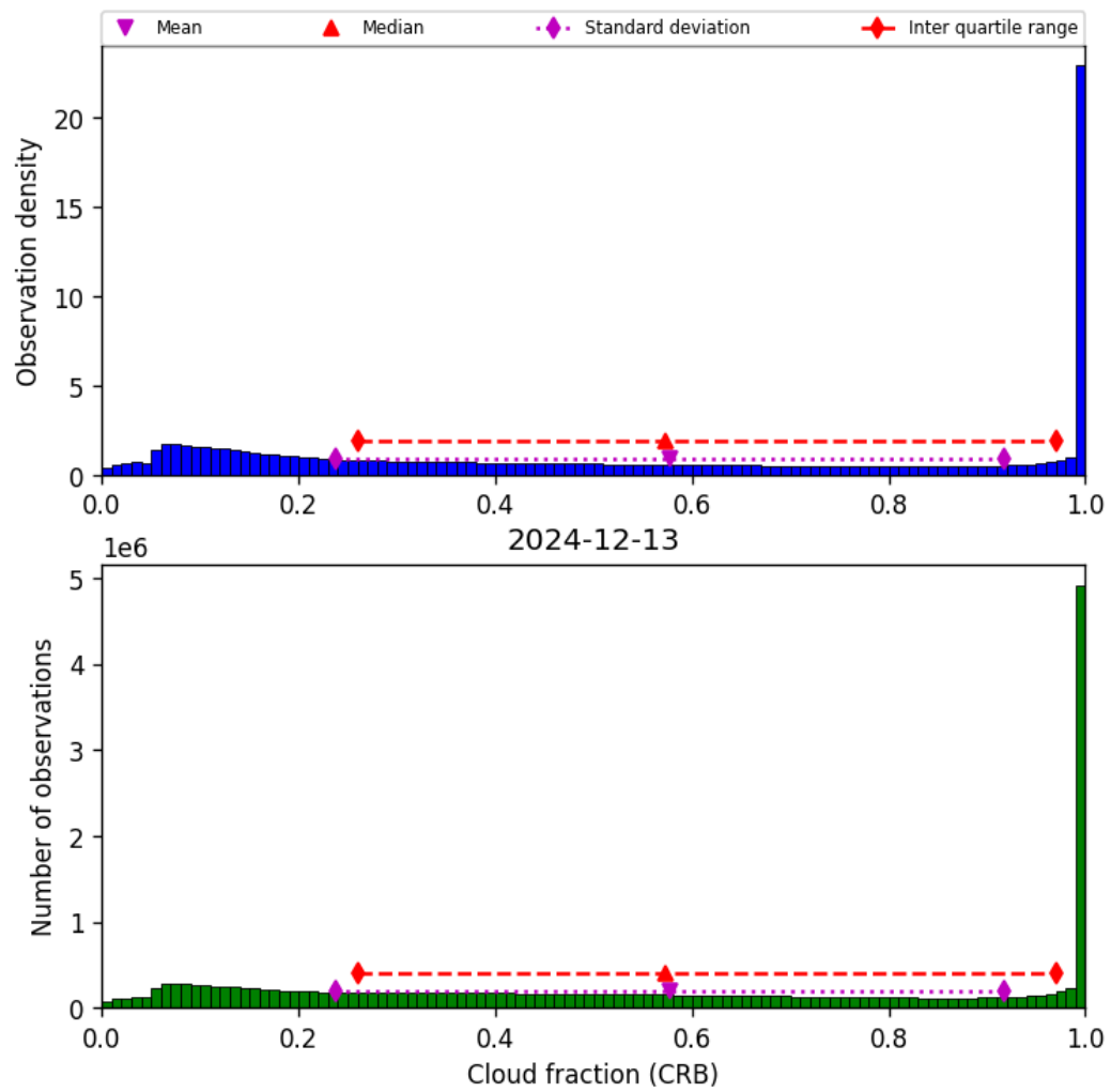
Figure 42: Histogram of “Cloud fraction (CRB)” for 2024-12-12 to 2024-12-14
