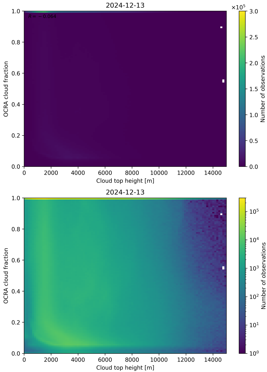
Figure 87: Scatter density plot of “Cloud top height” against “OCRA cloud fraction” for 2024-12-12 to 2024-12-14.
