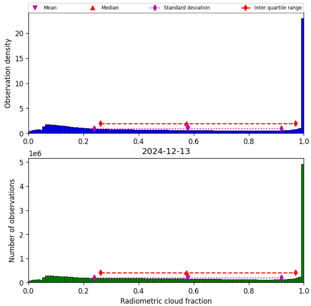
Figure 39: Histogram of "Radiometric cloud fraction" for 2024-12-12 to 2024-12-14
