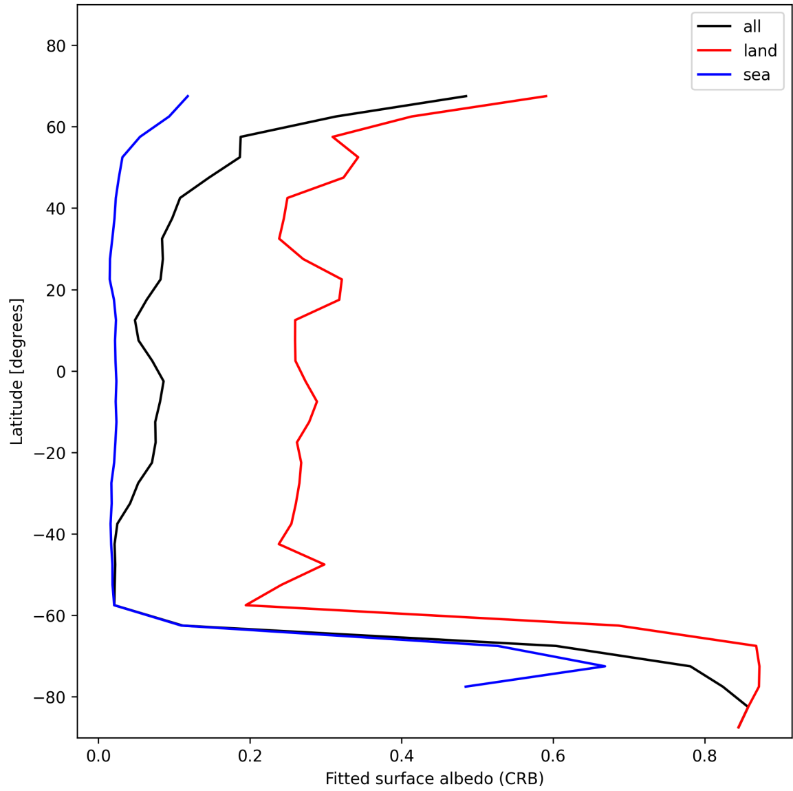
Figure 30: Zonal average of “Fitted surface albedo (CRB)” for 2024-12-12 to 2024-12-14.
