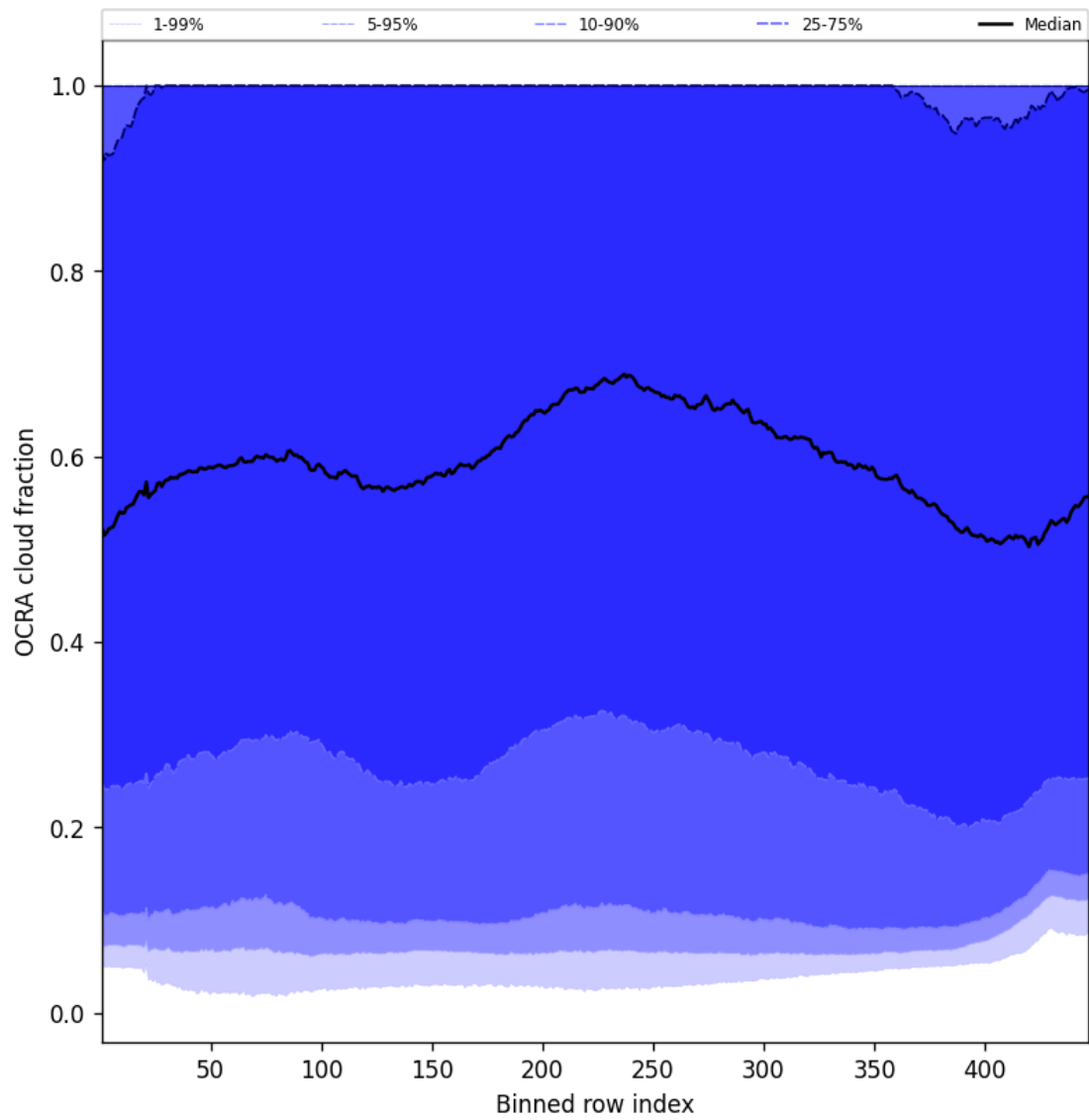
Figure 66: Along track statistics of “OCRA cloud fraction” for 2024-12-12 to 2024-12-14
