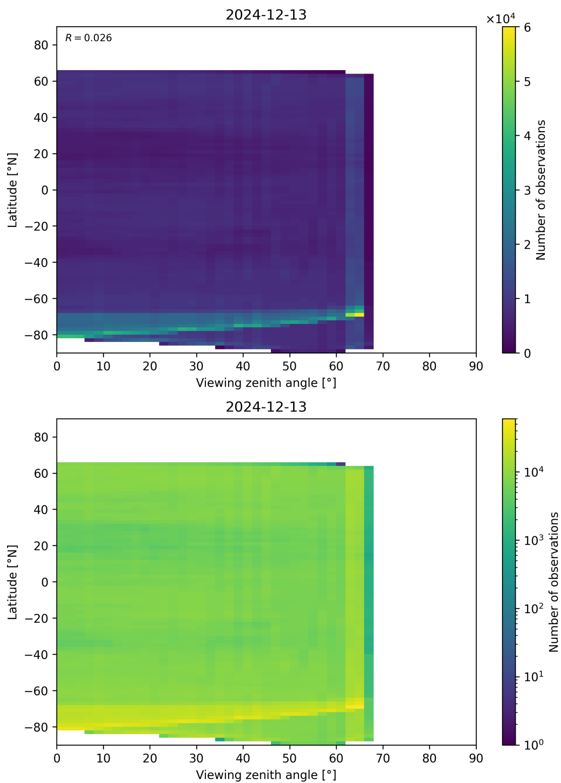
Figure 113: Scatter density plot of “Viewing zenith angle” against “Latitude” for 2024-12-12 to 2024-12-14.
