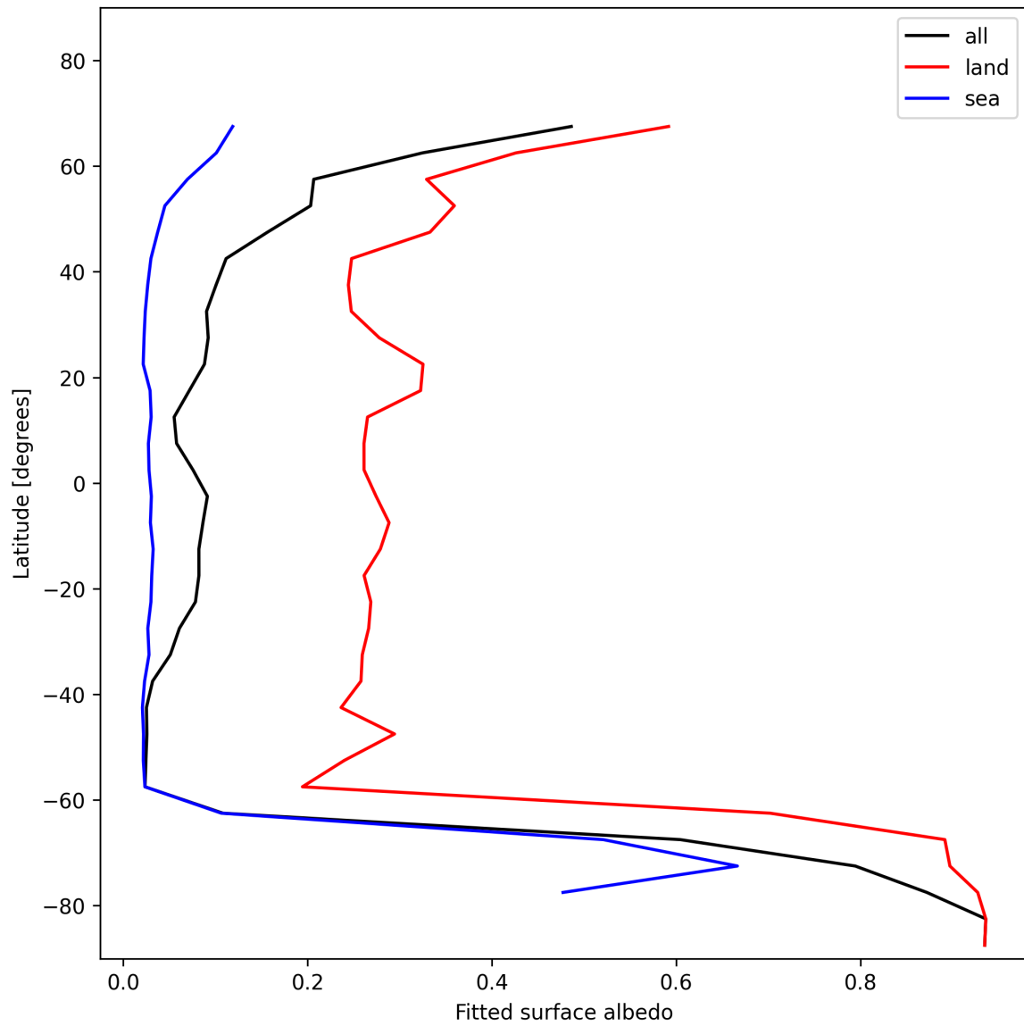
Figure 29: Zonal average of “Fitted surface albedo” for 2024-12-12 to 2024-12-14.
