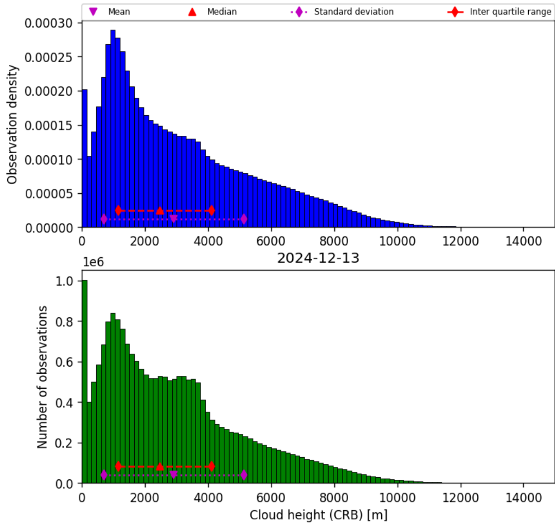
Figure 43: Histogram of “Cloud height (CRB)” for 2024-12-12 to 2024-12-14
