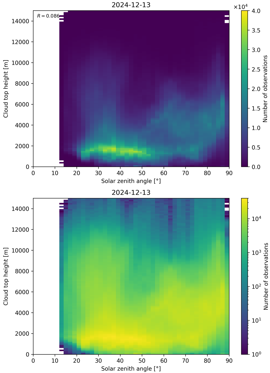
Figure 104: Scatter density plot of “Solar zenith angle” against “Cloud top height” for 2024-12-12 to 2024-12-14.
