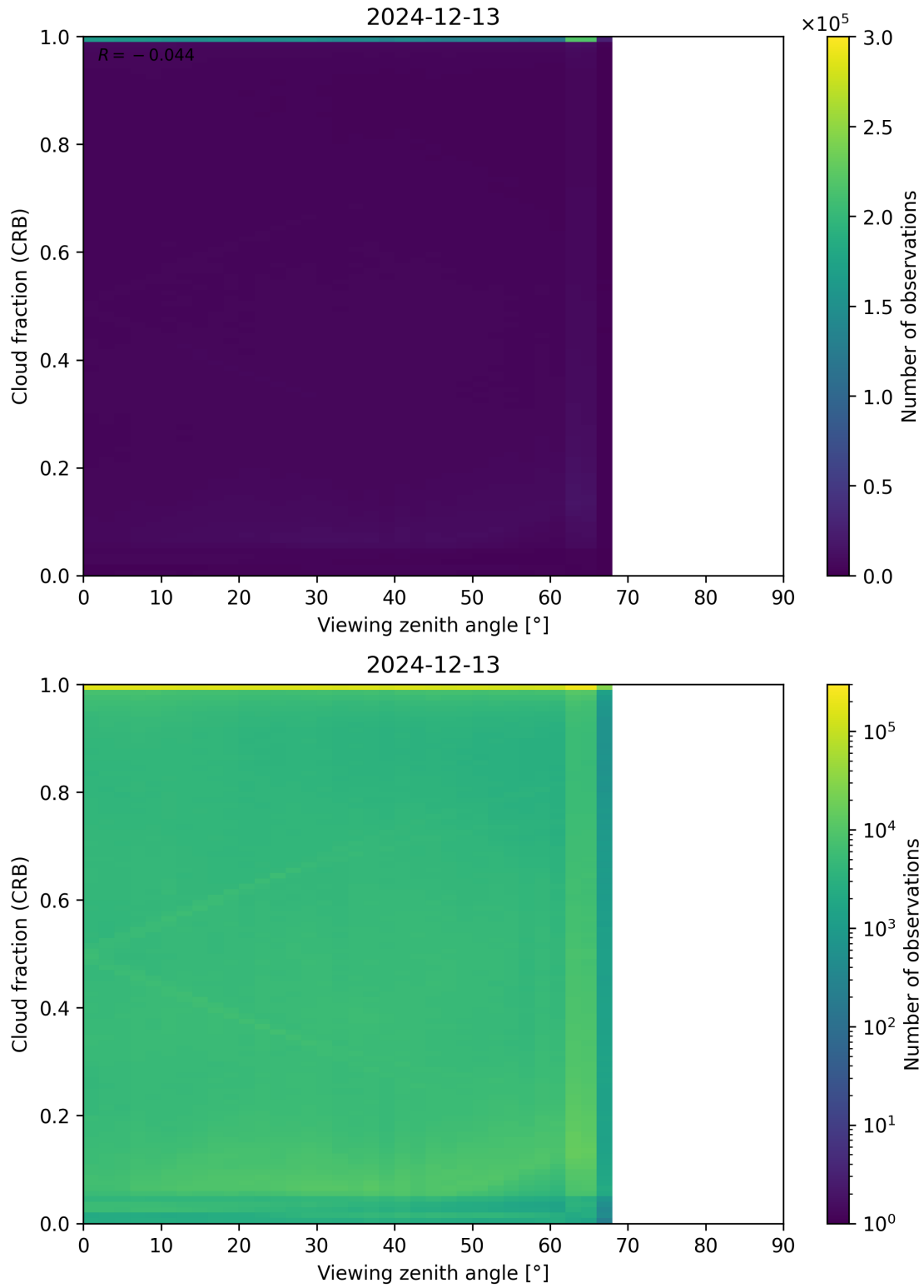
Figure 109: Scatter density plot of “Viewing zenith angle” against “Cloud fraction (CRB)” for 2024-12-12 to 2024-12-14.
