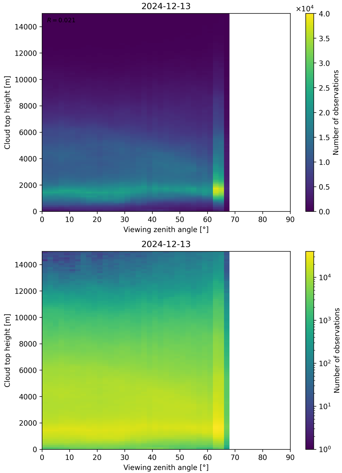
Figure 112: Scatter density plot of “Viewing zenith angle” against “Cloud top height” for 2024-12-12 to 2024-12-14.
