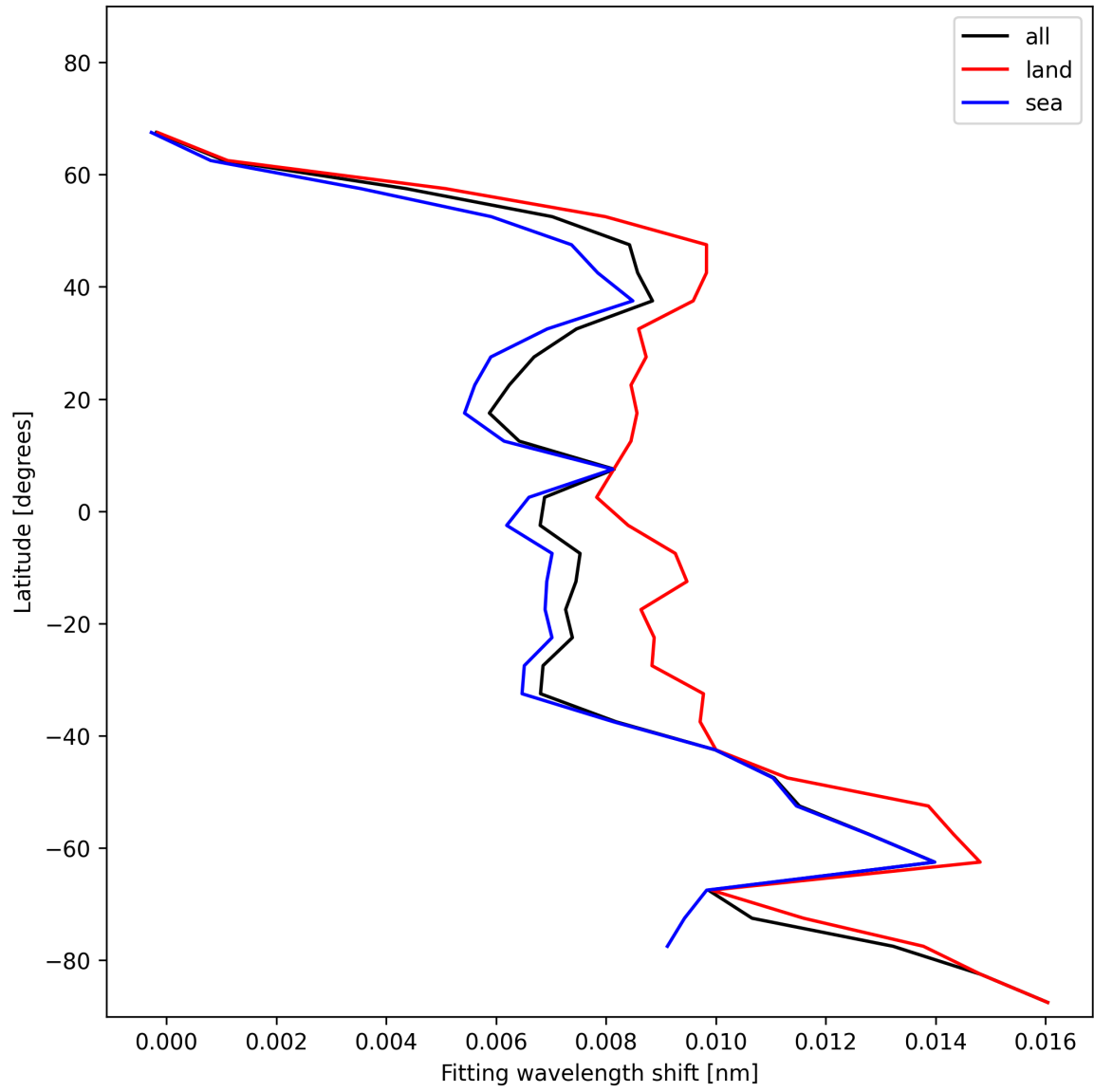
Figure 33: Zonal average of “Fitting wavelength shift” for 2024-12-12 to 2024-12-14.
