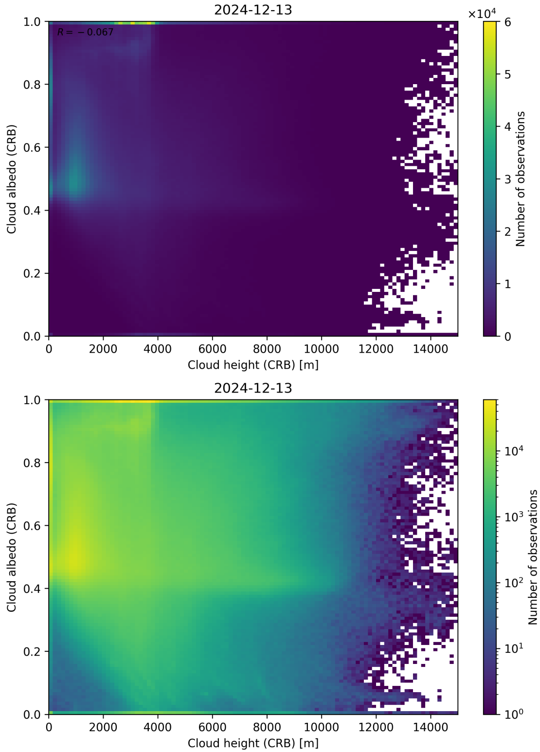
Figure 80: Scatter density plot of “Cloud height (CRB)” against “Cloud albedo (CRB)” for 2024-12-12 to 2024-12-14.
