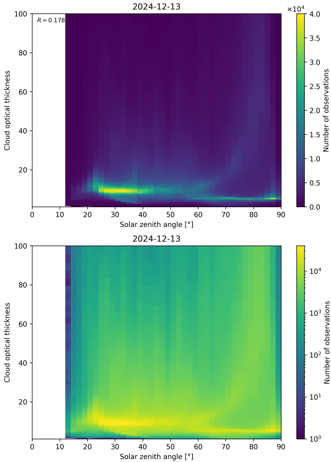
Figure 103: Scatter density plot of “Solar zenith angle” against “Cloud optical thickness” for 2024-12-12 to 2024-12-14.
