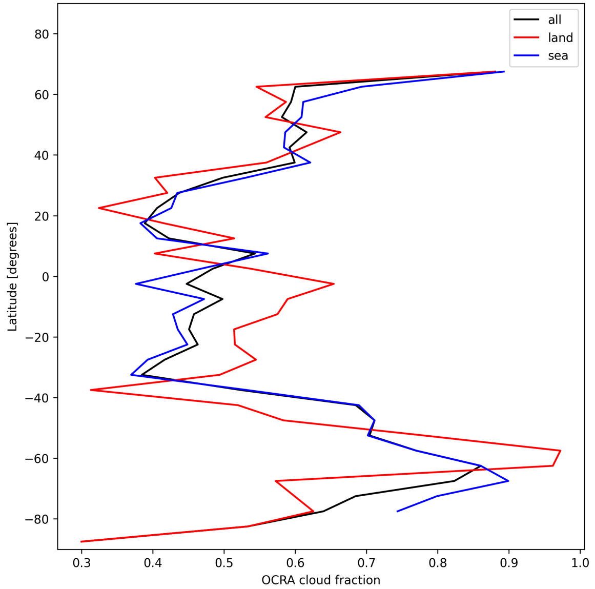
Figure 34: Zonal average of “OCRA cloud fraction” for 2024-12-12 to 2024-12-14.
