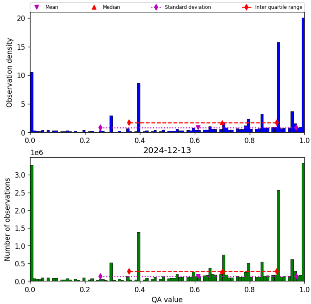
Figure 38: Histogram of “QA value” for 2024-12-12 to 2024-12-14
