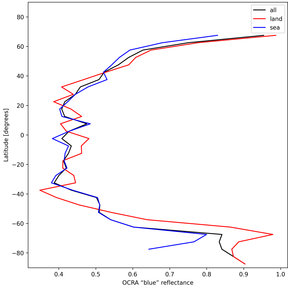
Figure 35: Zonal average of “OCRA “blue” reflectance” for 2024-12-12 to 2024-12-14.
