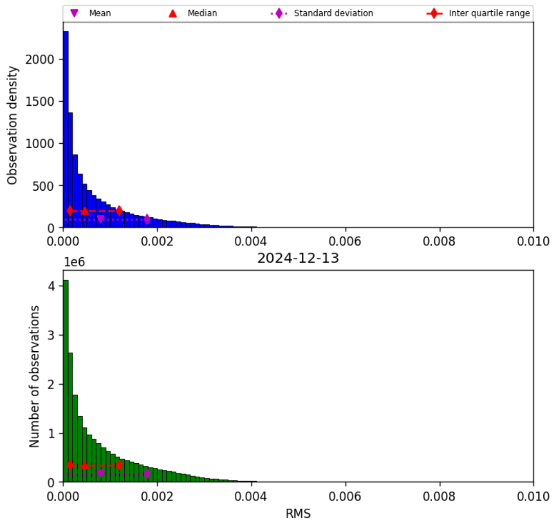
Figure 47: Histogram of “RMS” for 2024-12-12 to 2024-12-14
