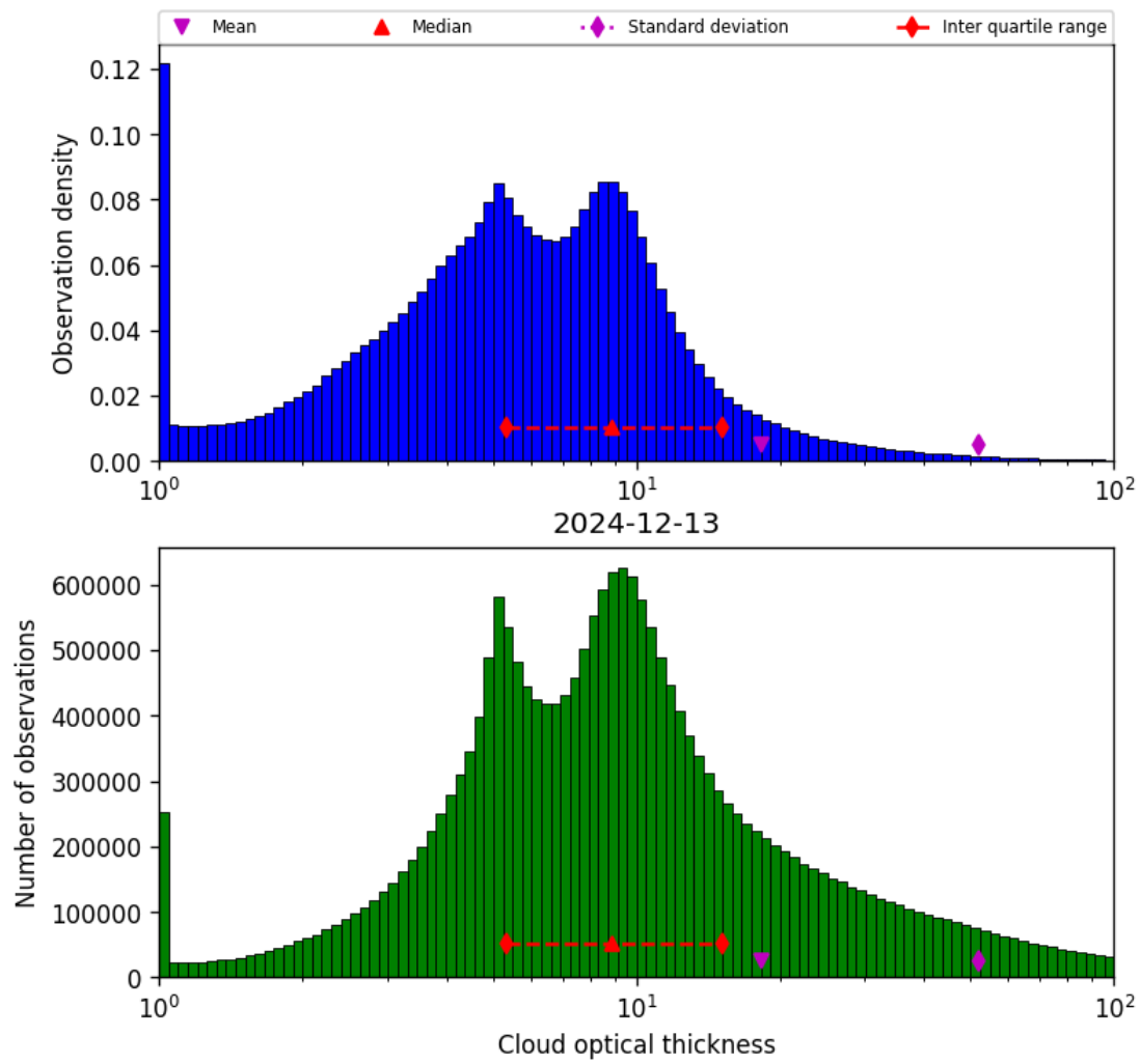
Figure 41: Histogram of “Cloud optical thickness” for 2024-12-12 to 2024-12-14
