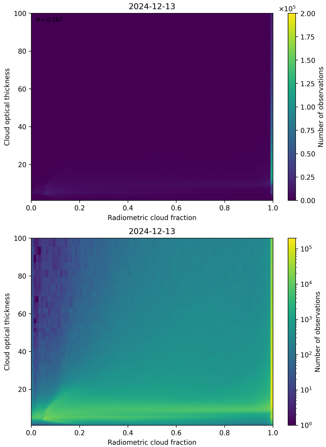
Figure 75: Scatter density plot of “Radiometric cloud fraction” against “Cloud optical thickness” for 2024-12-12 to 2024-12-14.
