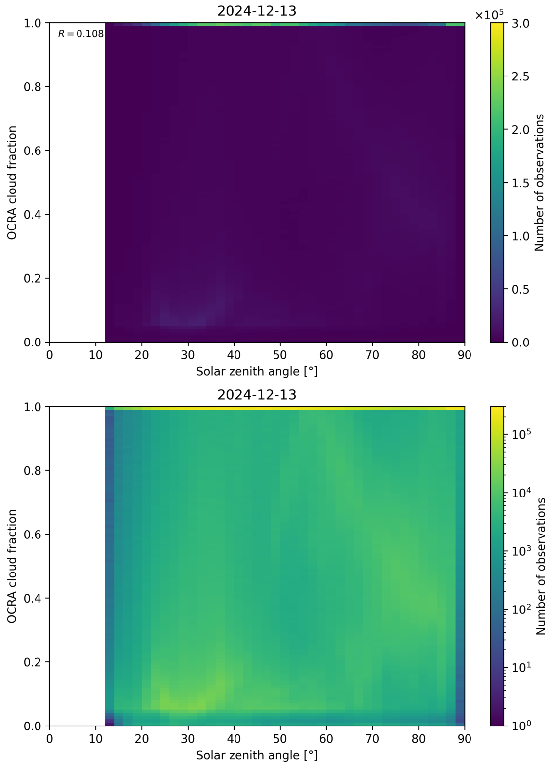
Figure 100: Scatter density plot of “Solar zenith angle” against “OCRA cloud fraction” for 2024-12-12 to 2024-12-14.
