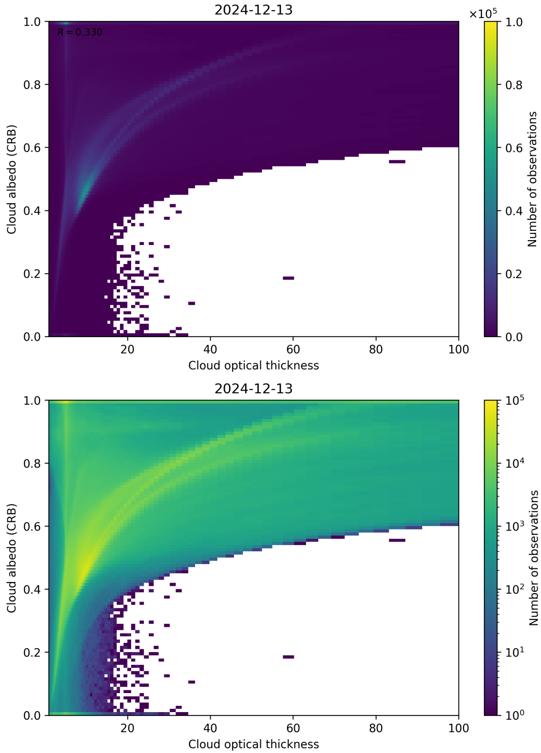
Figure 82: Scatter density plot of “Cloud optical thickness” against “Cloud albedo (CRB)” for 2024-12-12 to 2024-12-14.
