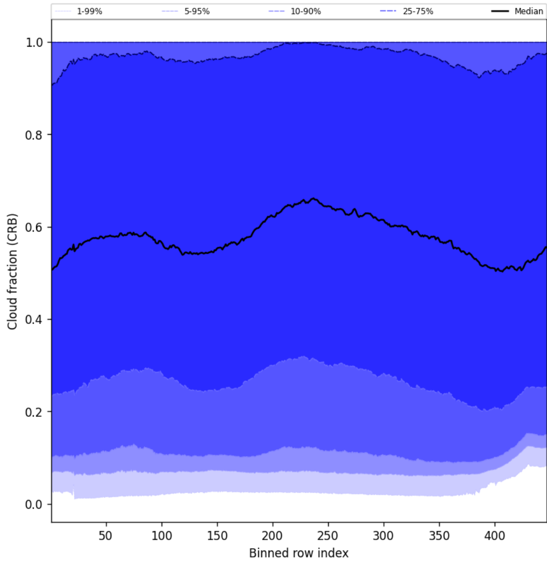
Figure 58: Along track statistics of “Cloud fraction (CRB)” for 2024-12-12 to 2024-12-14
