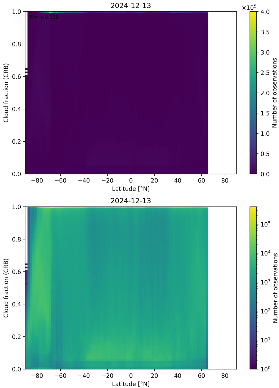
Figure 94: Scatter density plot of “Latitude” against “Cloud fraction (CRB)” for 2024-12-12 to 2024-12-14.
