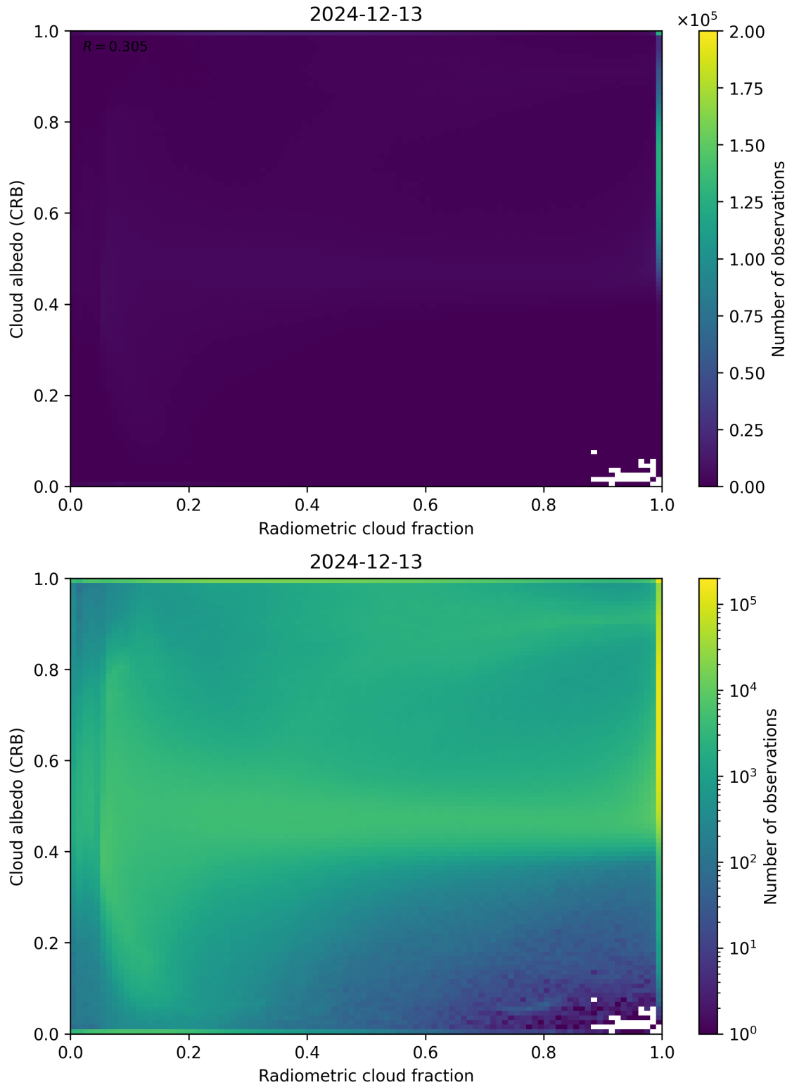
Figure 71: Scatter density plot of “Radiometric cloud fraction” against “Cloud albedo (CRB)” for 2024-12-12 to 2024-12-14.
