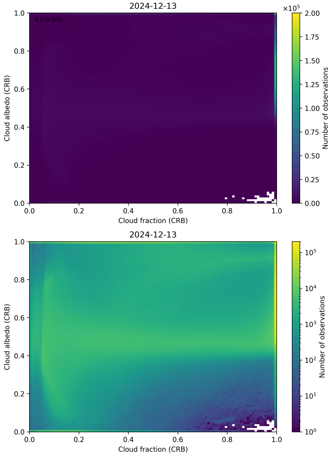
Figure 77: Scatter density plot of “Cloud fraction (CRB)” against “Cloud albedo (CRB)” for 2024-12-12 to 2024-12-14.
