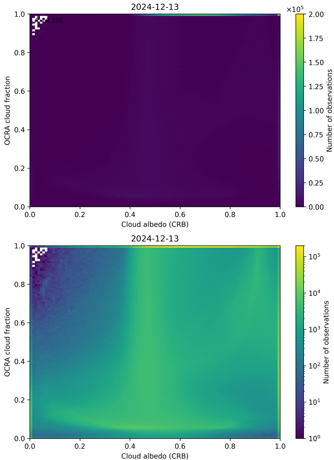
Figure 70: Scatter density plot of “Cloud albedo (CRB)” against “OCRA cloud fraction” for 2024-12-12 to 2024-12-14.
