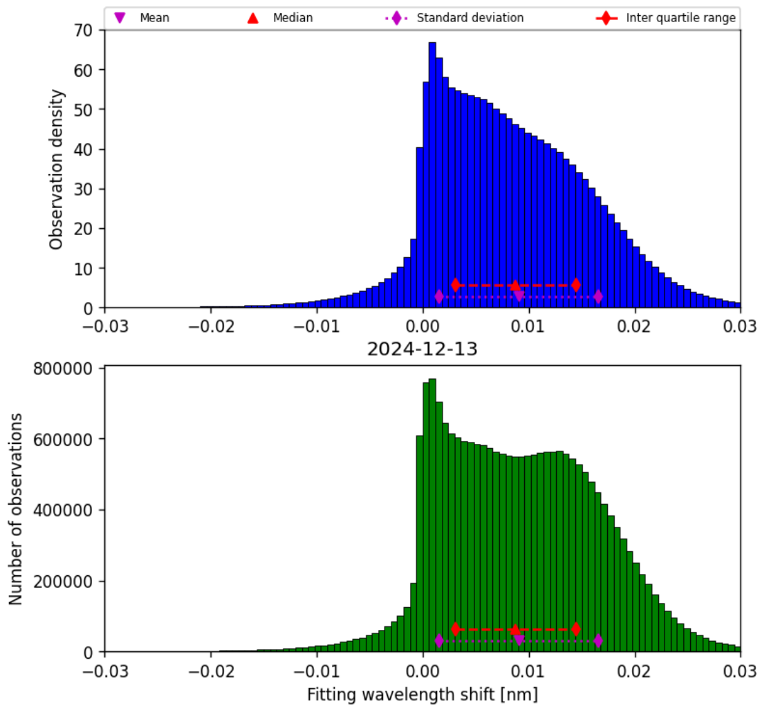
Figure 49: Histogram of “Fitting wavelength shift” for 2024-12-12 to 2024-12-14
