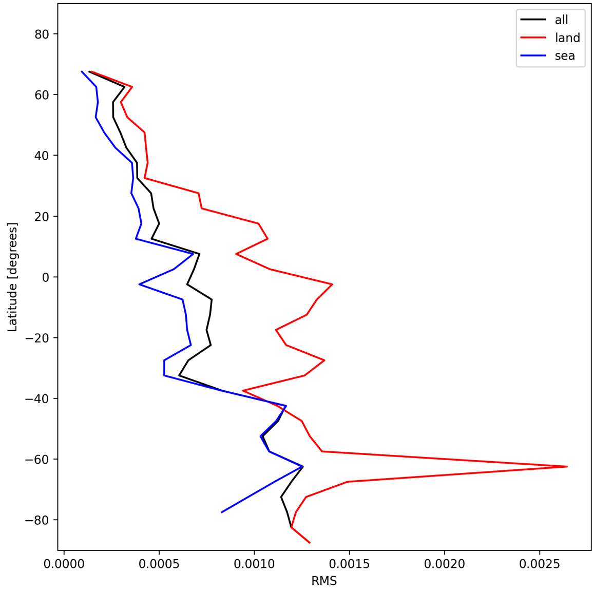
Figure 31: Zonal average of “RMS” for 2024-12-12 to 2024-12-14.
