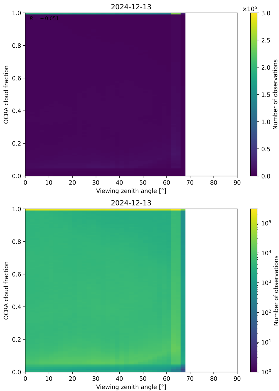
Figure 108: Scatter density plot of “Viewing zenith angle” against “OCRA cloud fraction” for 2024-12-12 to 2024-12-14.
