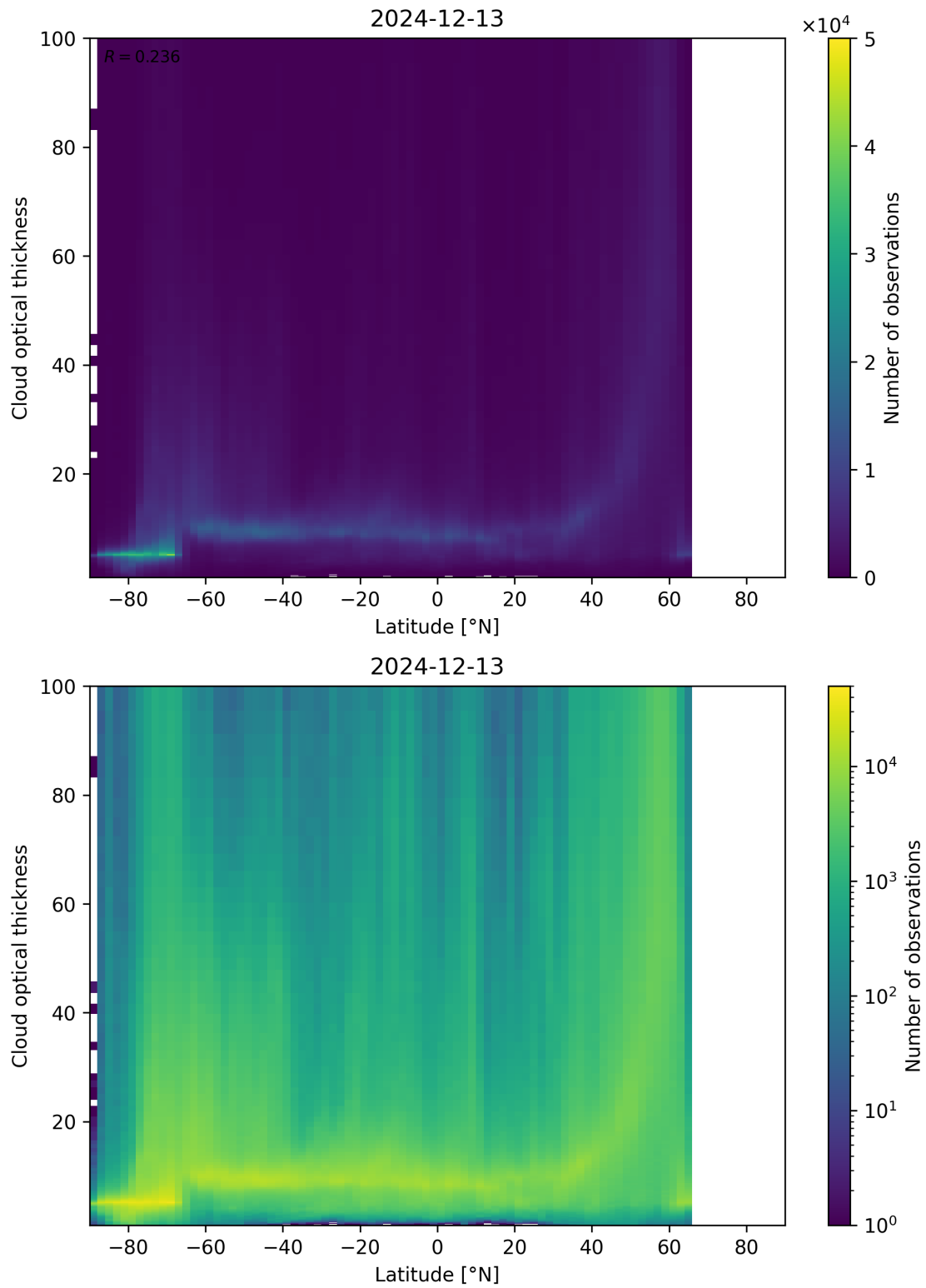
Figure 96: Scatter density plot of “Latitude” against “Cloud optical thickness” for 2024-12-12 to 2024-12-14.
