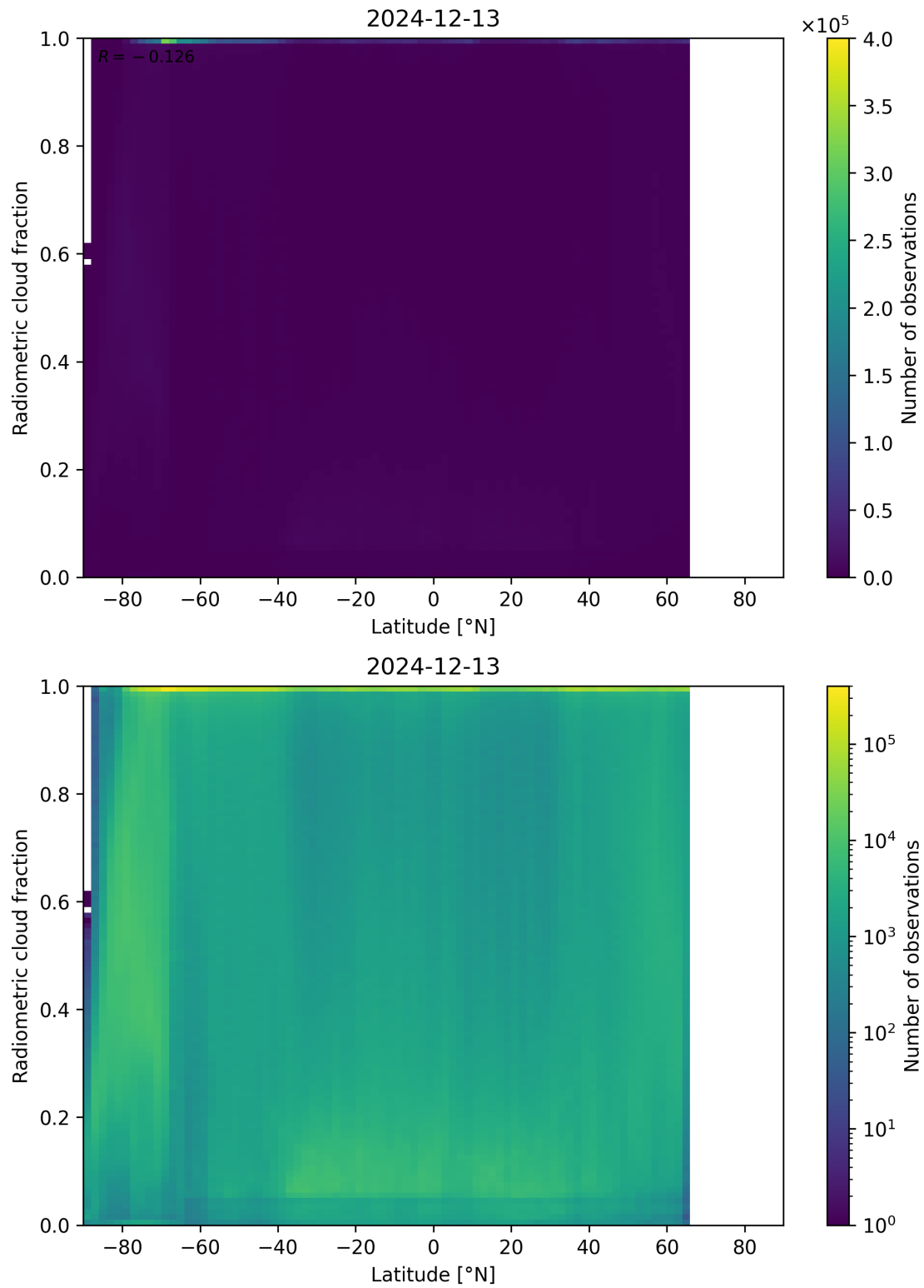
Figure 92: Scatter density plot of “Latitude” against “Radiometric cloud fraction” for 2024-12-12 to 2024-12-14.
