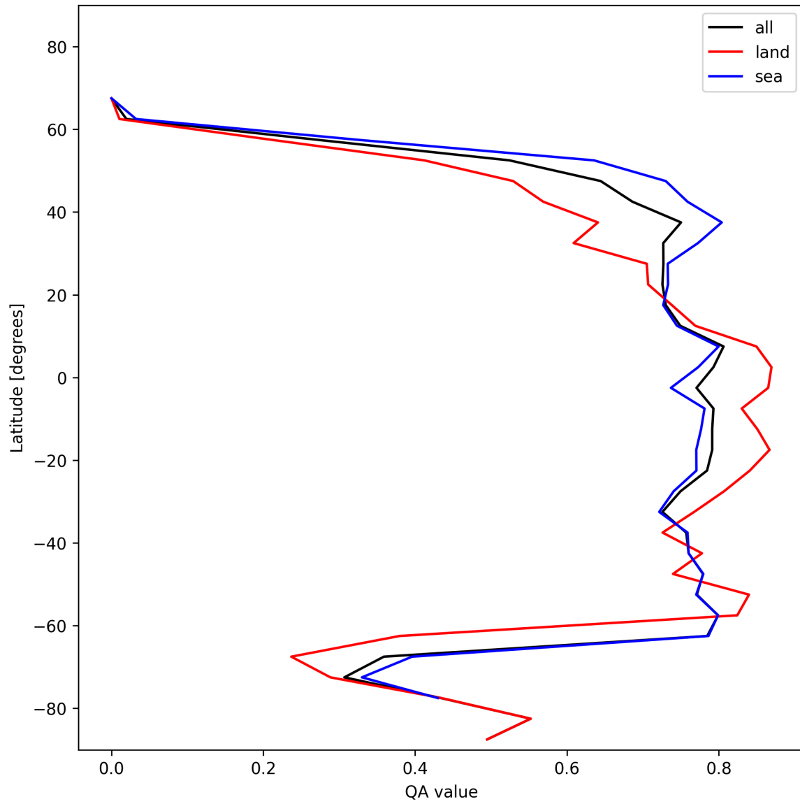
Figure 22: Zonal average of “QA value” for 2024-12-12 to 2024-12-14.
