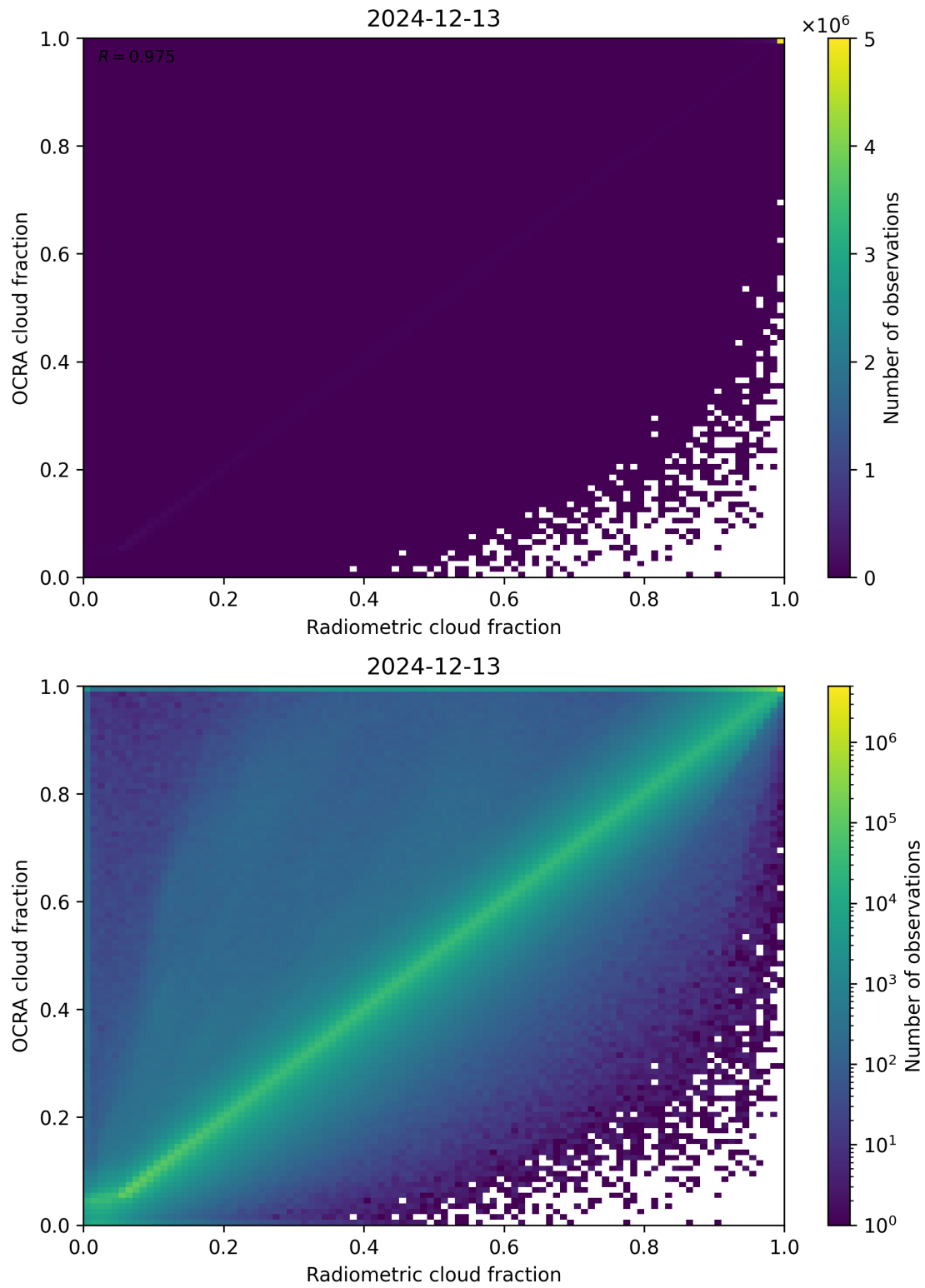
Figure 72: Scatter density plot of “Radiometric cloud fraction” against “OCRA cloud fraction” for 2024-12-12 to 2024-12-14.
