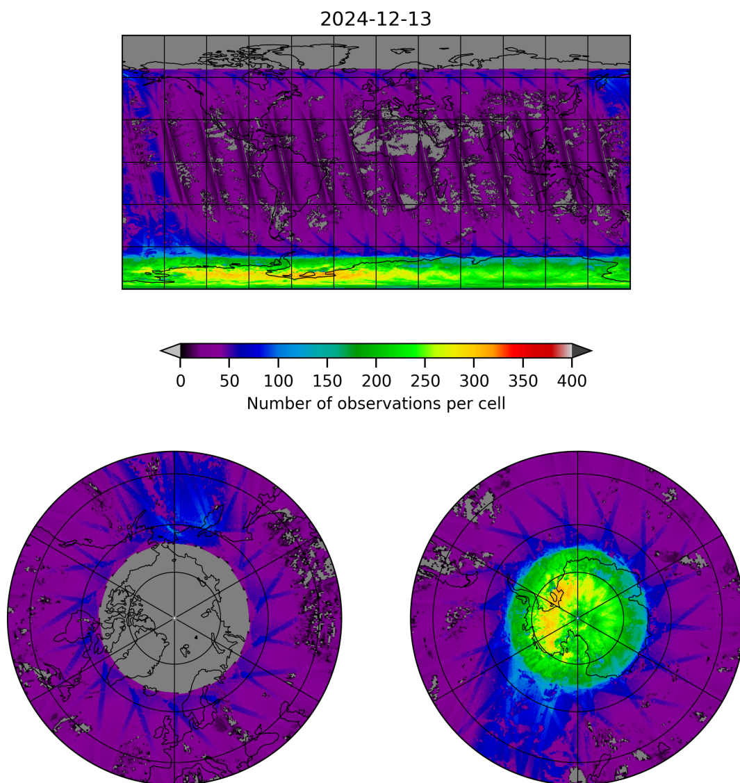
Figure 21: Map of the number of observations for 2024-12-12 to 2024-12-14
