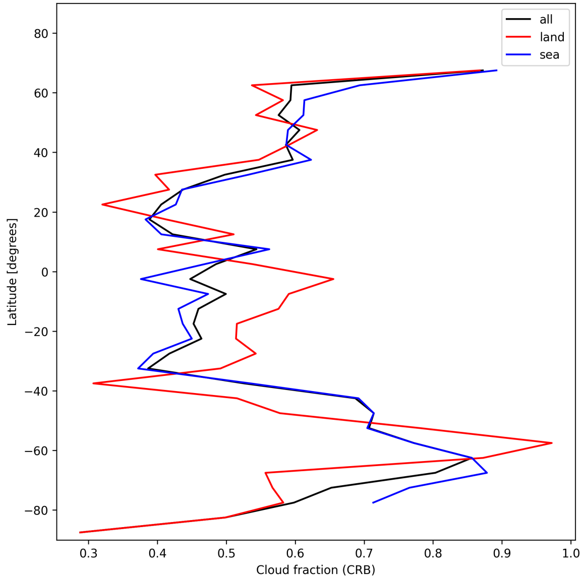
Figure 26: Zonal average of “Cloud fraction (CRB)” for 2024-12-12 to 2024-12-14.
