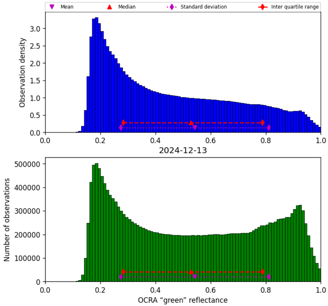
Figure 52: Histogram of “OCRA “green” reflectance” for 2024-12-12 to 2024-12-14
