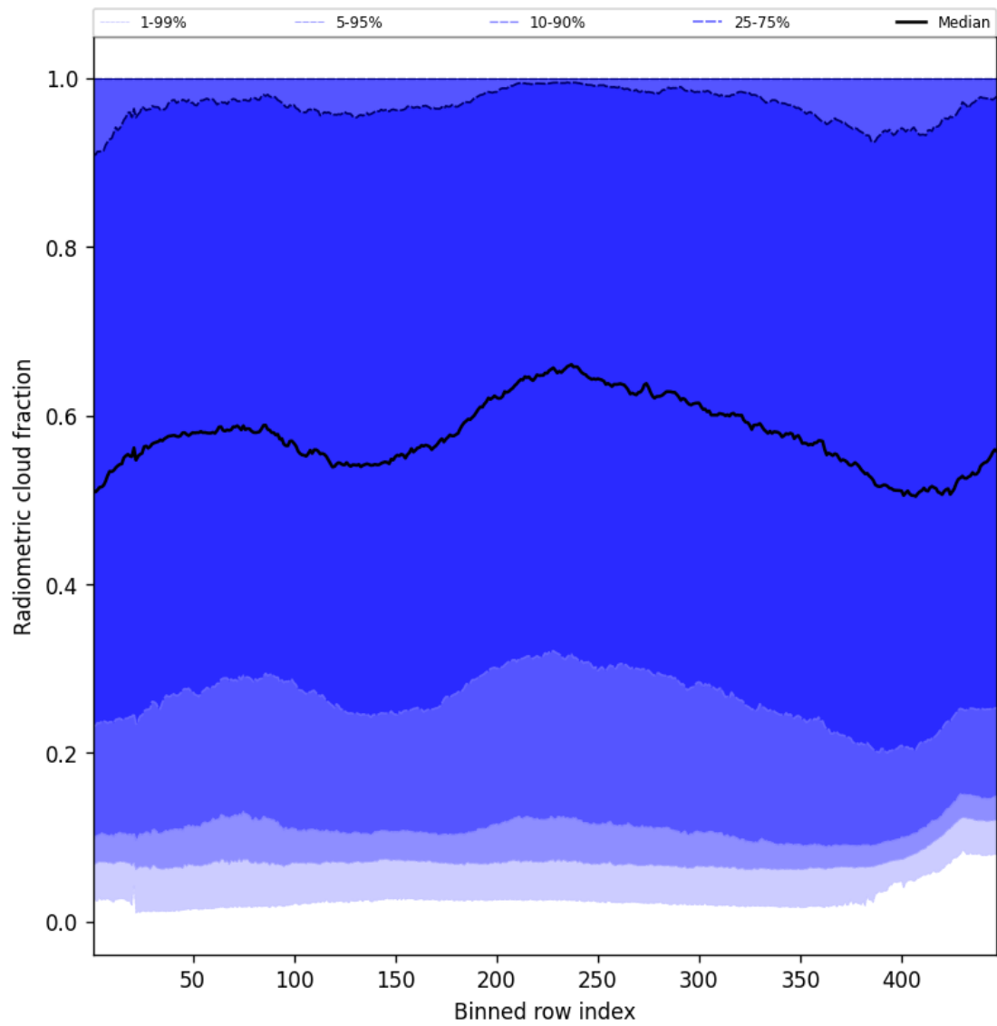
Figure 55: Along track statistics of “Radiometric cloud fraction” for 2024-12-12 to 2024-12-14
