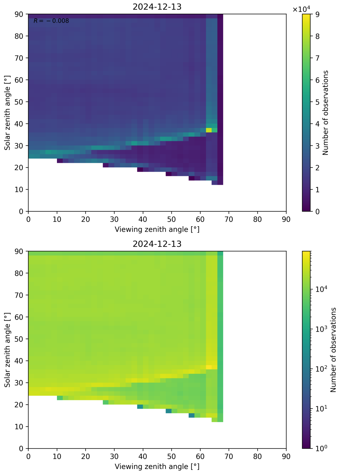
Figure 114: Scatter density plot of “Viewing zenith angle” against “Solar zenith angle” for 2024-12-12 to 2024-12-14.
