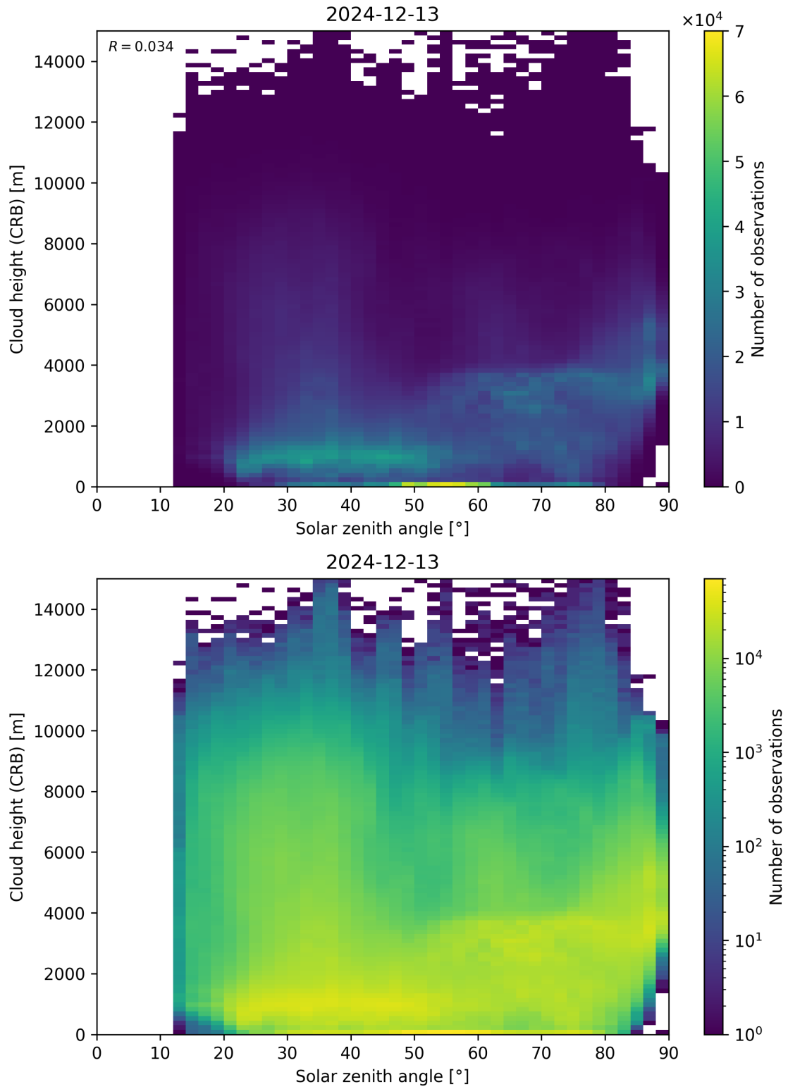
Figure 102: Scatter density plot of “Solar zenith angle” against “Cloud height (CRB)” for 2024-12-12 to 2024-12-14.
