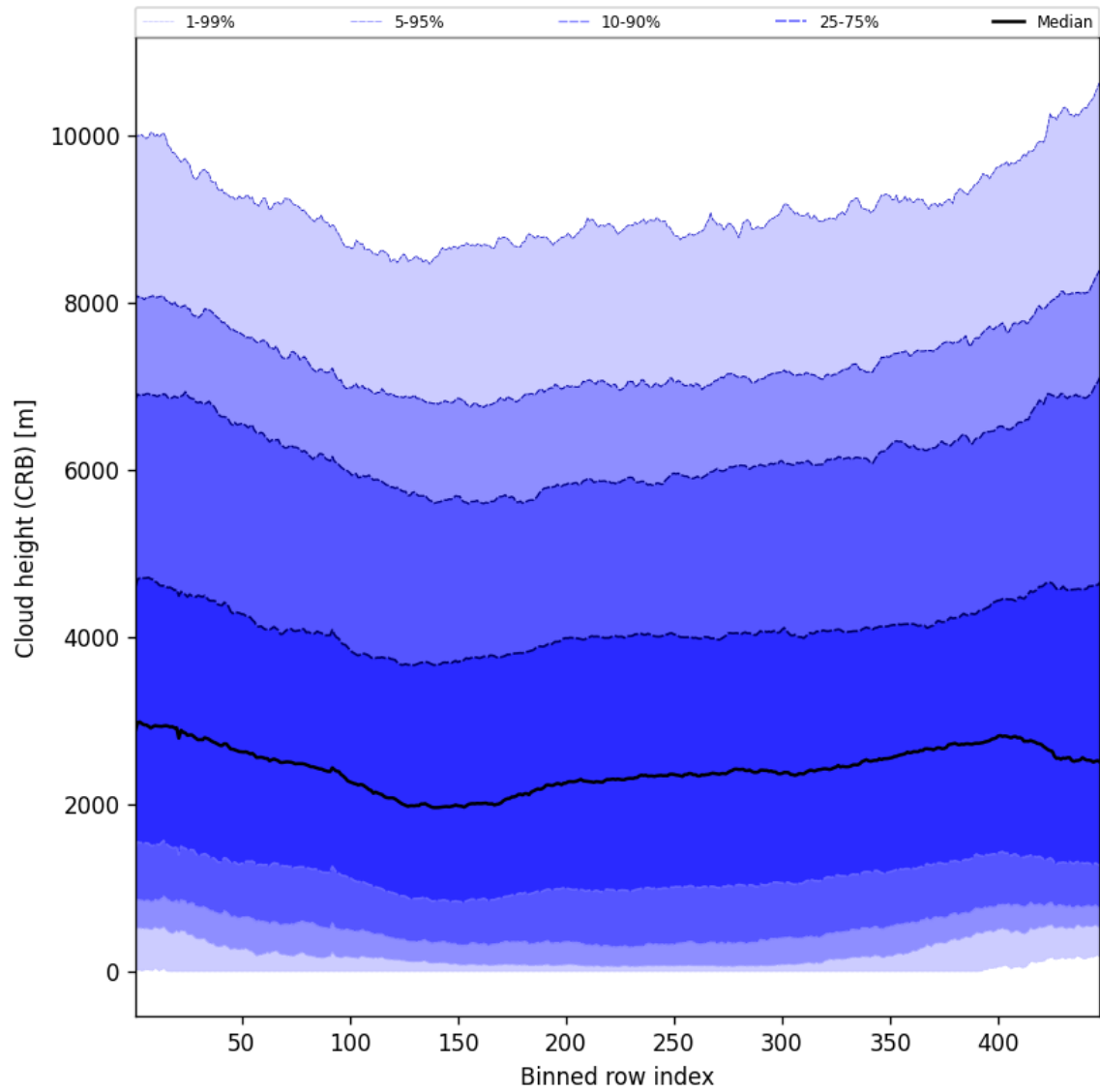
Figure 59: Along track statistics of “Cloud height (CRB)” for 2024-12-12 to 2024-12-14
