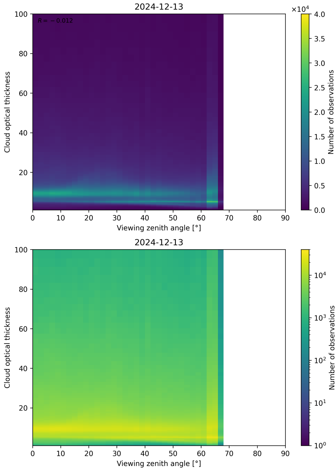
Figure 111: Scatter density plot of “Viewing zenith angle” against “Cloud optical thickness” for 2024-12-12 to 2024-12-14.
