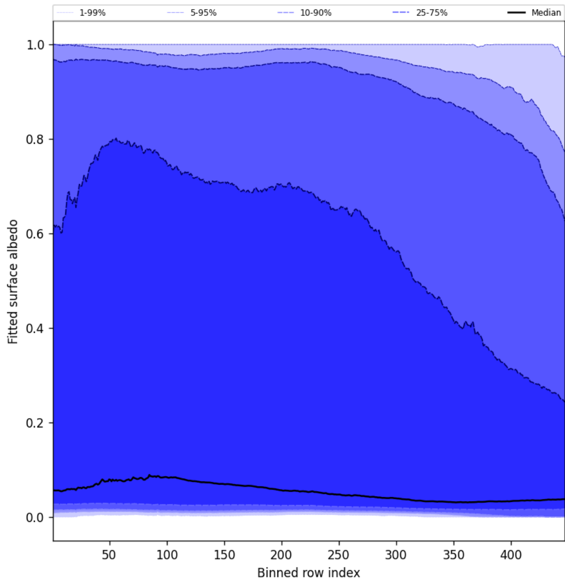
Figure 61: Along track statistics of “Fitted surface albedo” for 2024-12-12 to 2024-12-14
