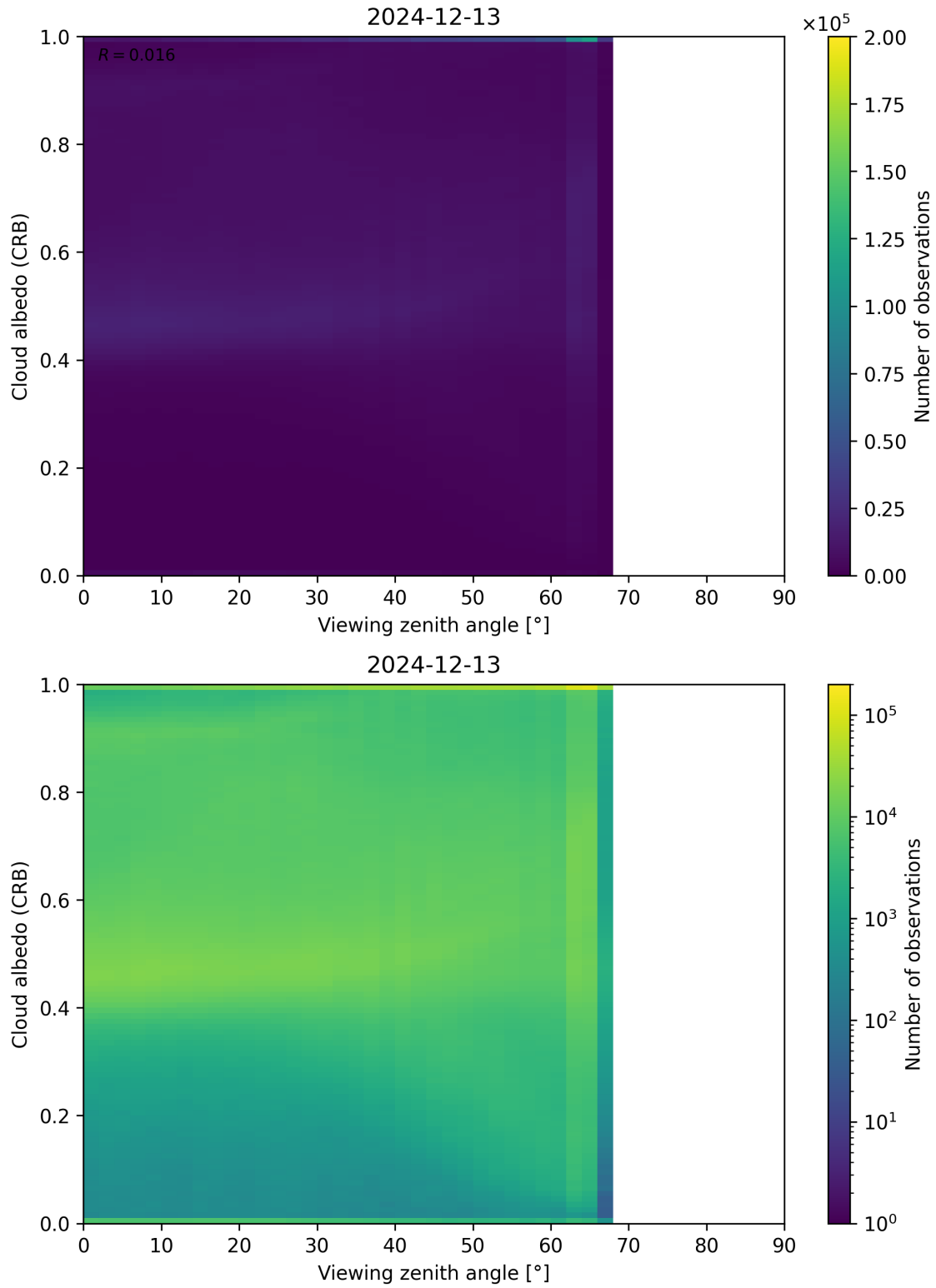
Figure 106: Scatter density plot of “Viewing zenith angle” against “Cloud albedo (CRB)” for 2024-12-12 to 2024-12-14.
