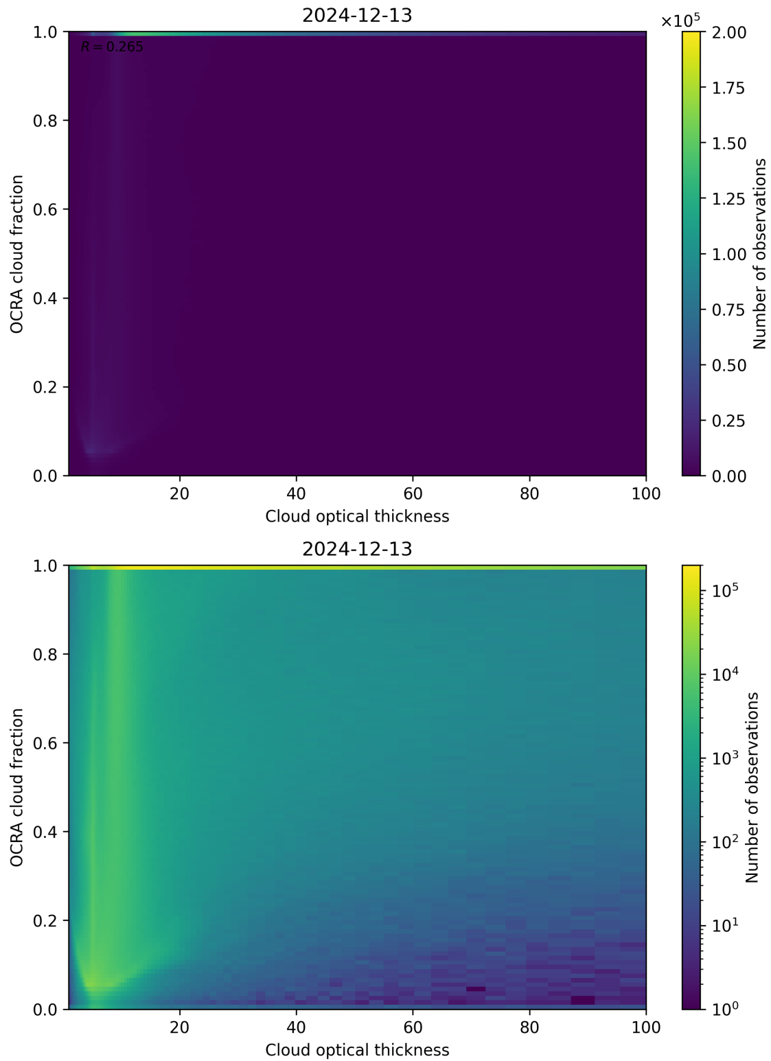
Figure 83: Scatter density plot of “Cloud optical thickness” against “OCRA cloud fraction” for 2024-12-12 to 2024-12-14.
