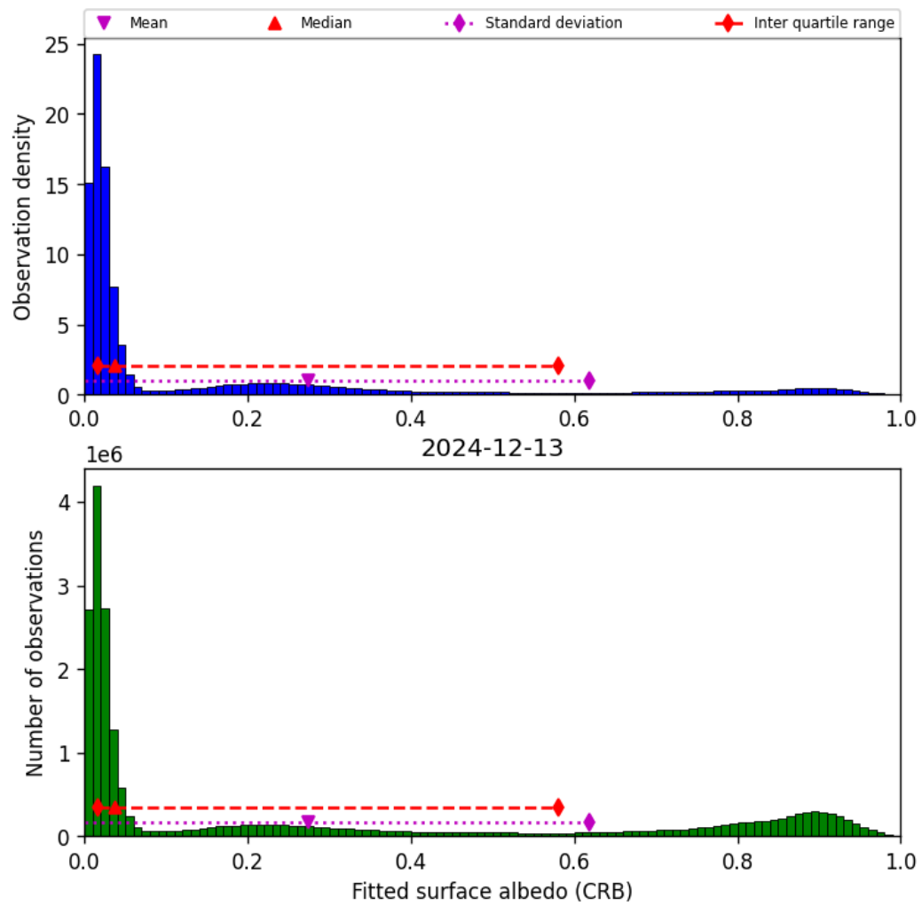
Figure 46: Histogram of “Fitted surface albedo (CRB)” for 2024-12-12 to 2024-12-14
