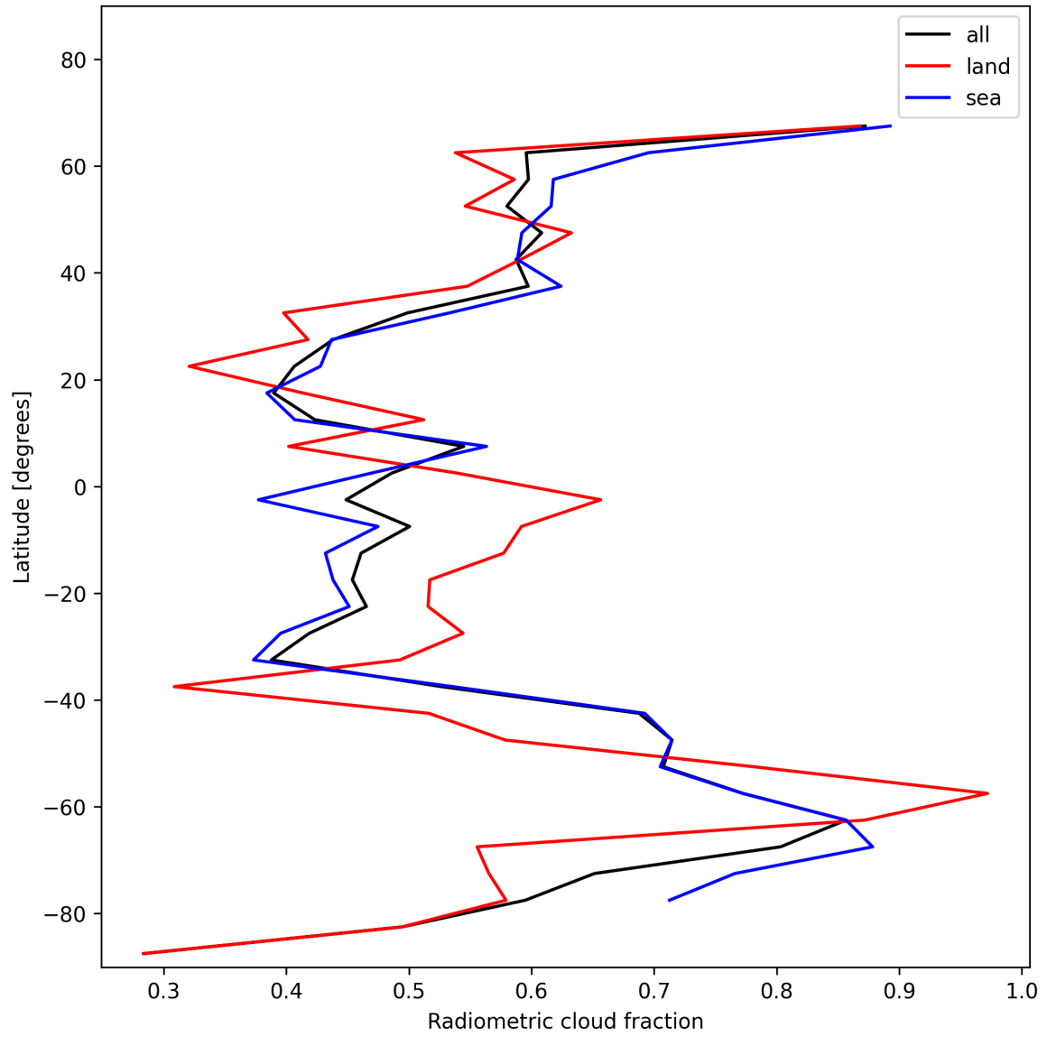
Figure 23: Zonal average of “Radiometric cloud fraction” for 2024-12-12 to 2024-12-14.
