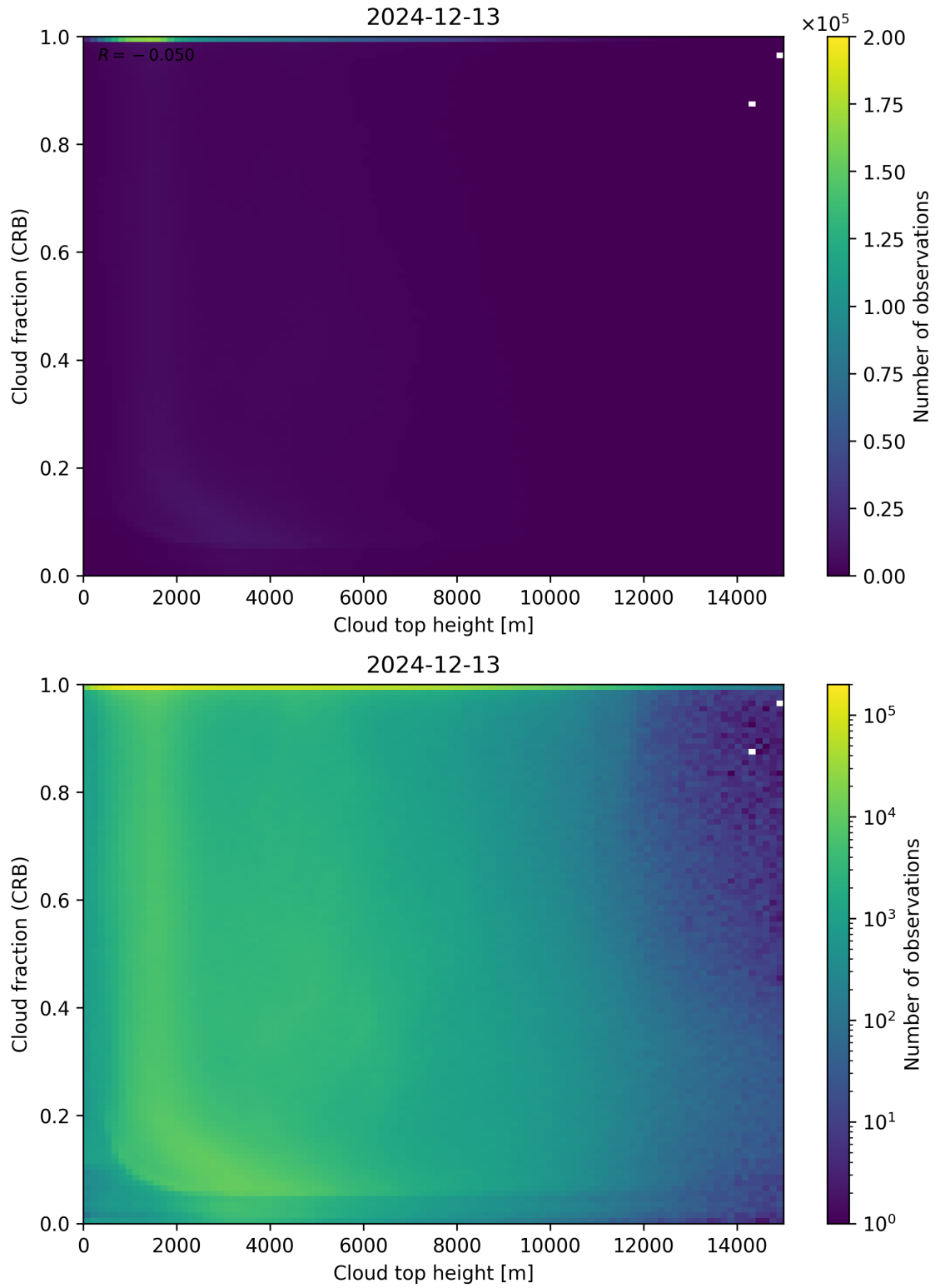
Figure 88: Scatter density plot of “Cloud top height” against “Cloud fraction (CRB)” for 2024-12-12 to 2024-12-14.
