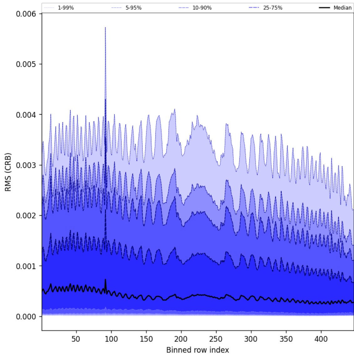
Figure 64: Along track statistics of “RMS (CRB)” for 2024-12-12 to 2024-12-14
