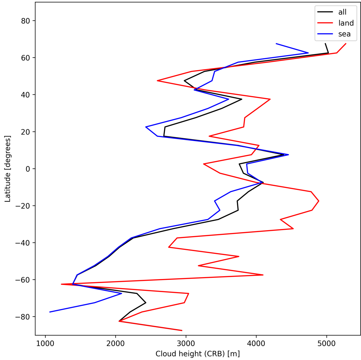
Figure 27: Zonal average of “Cloud height (CRB)” for 2024-12-12 to 2024-12-14.
