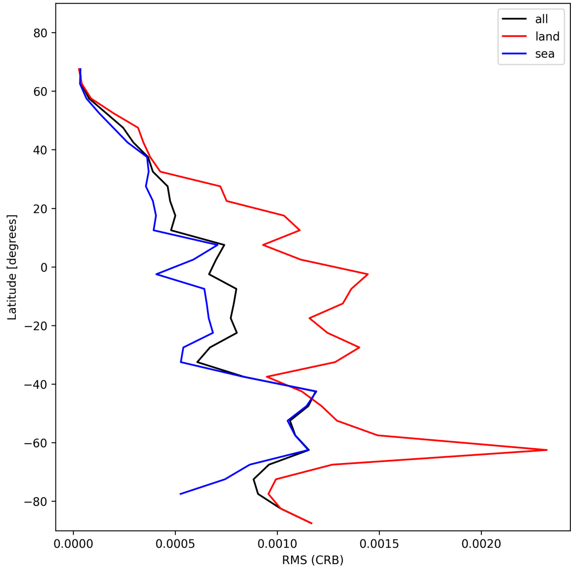
Figure 32: Zonal average of “RMS (CRB)” for 2024-12-12 to 2024-12-14.
