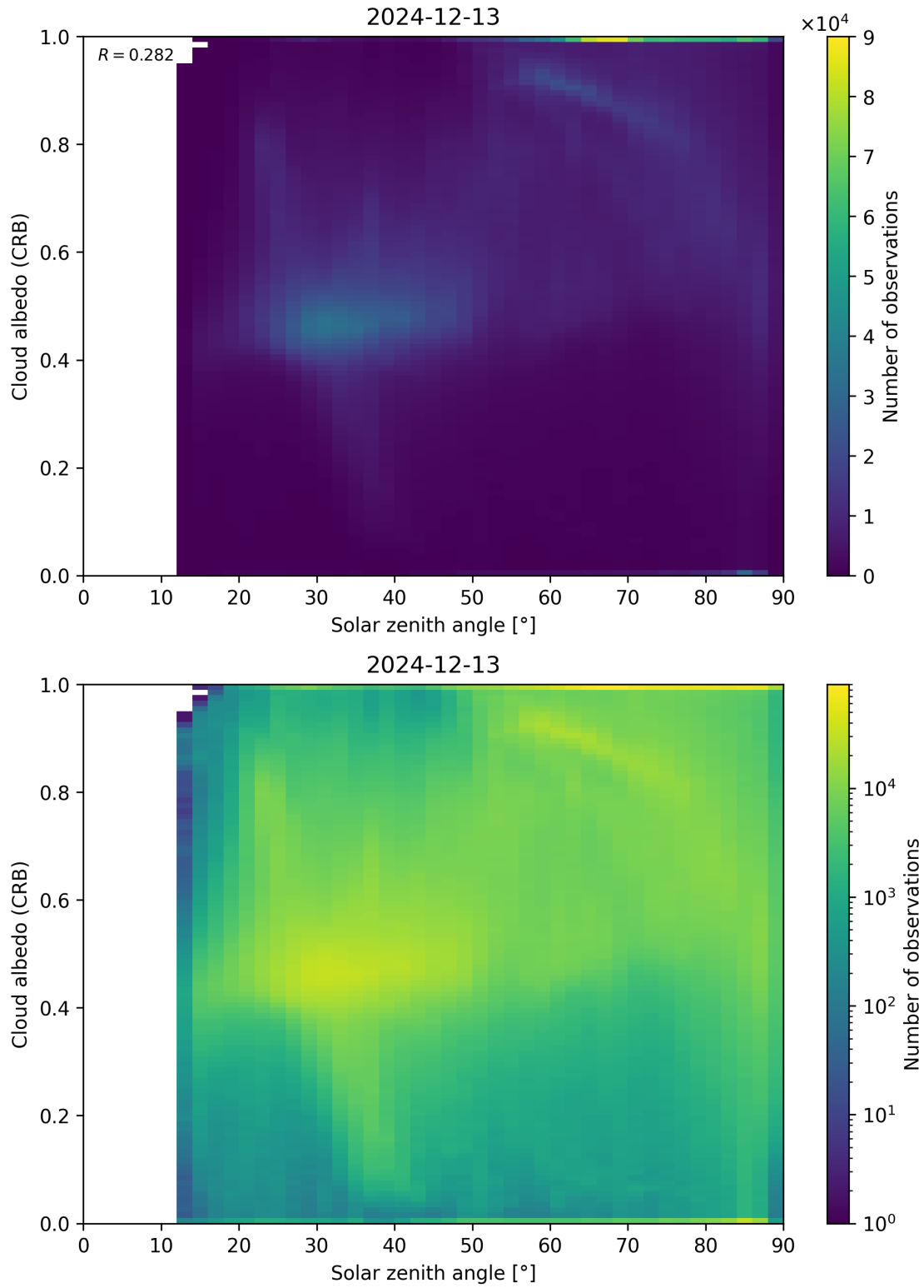
Figure 98: Scatter density plot of “Solar zenith angle” against “Cloud albedo (CRB)” for 2024-12-12 to 2024-12-14.
