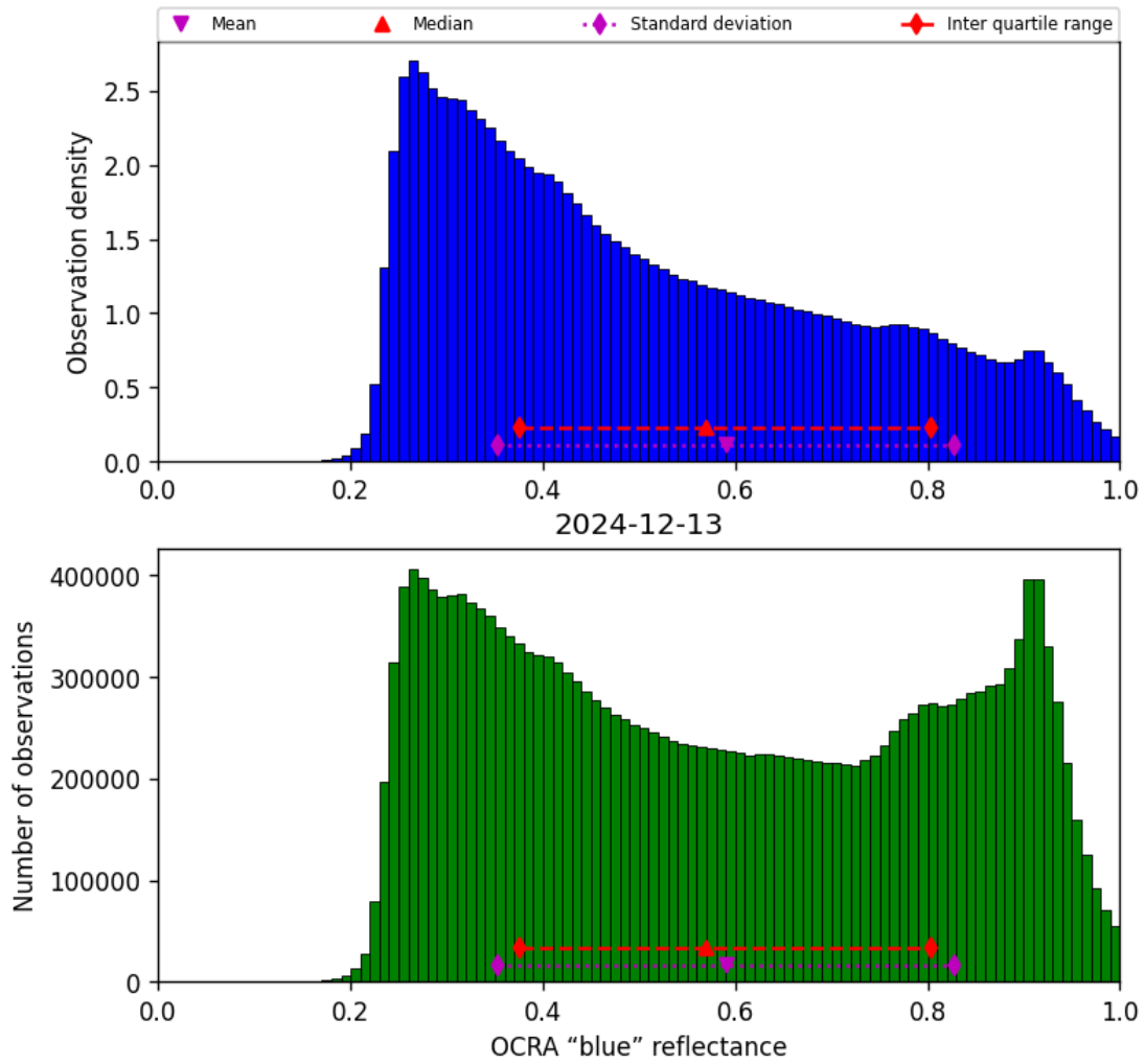
Figure 51: Histogram of “OCRA “blue” reflectance” for 2024-12-12 to 2024-12-14
