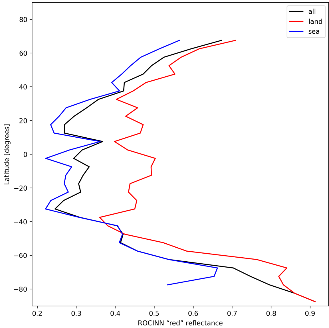
Figure 37: Zonal average of “ROCINN “red” reflectance” for 2024-12-12 to 2024-12-14.
