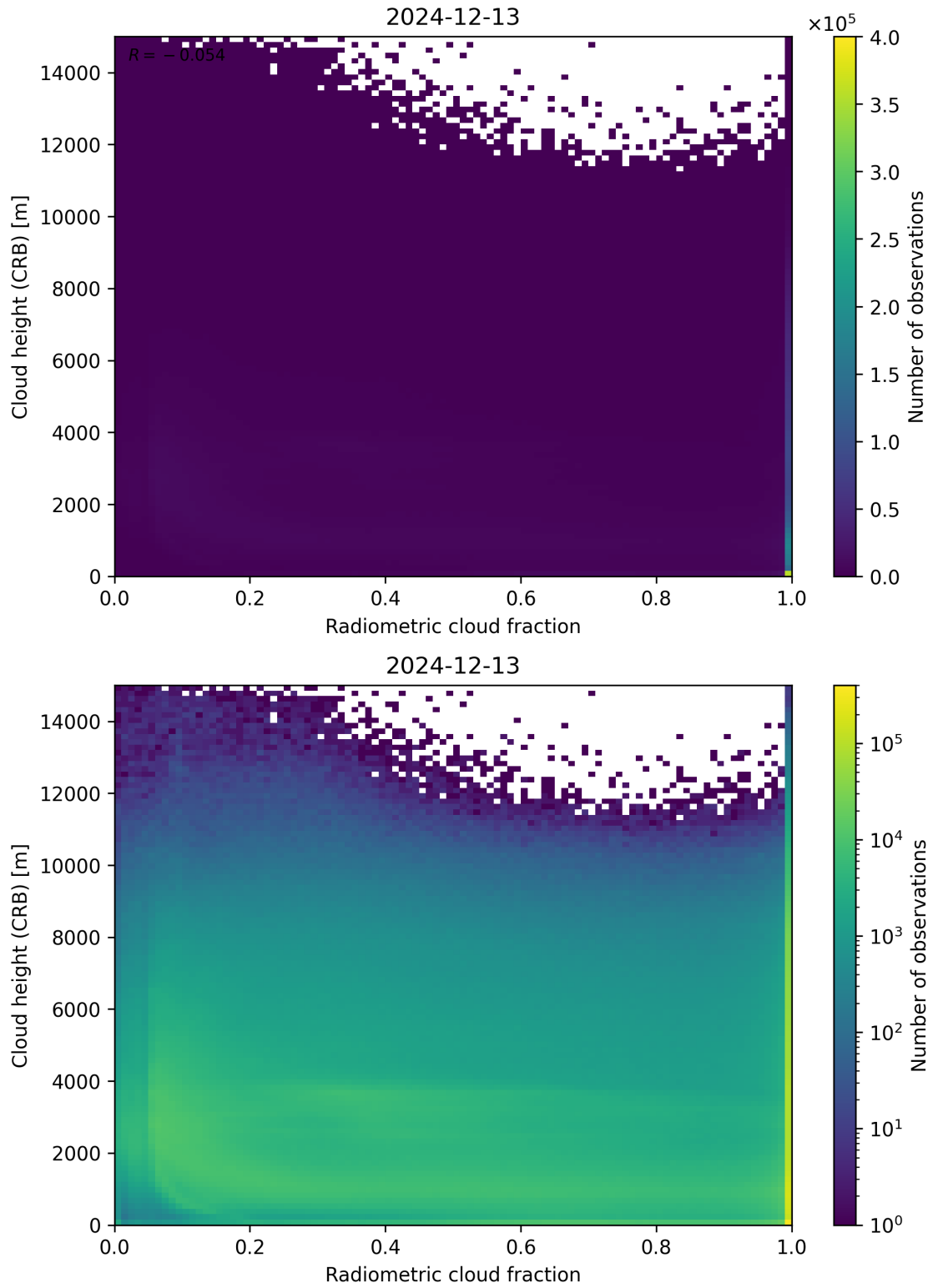
Figure 74: Scatter density plot of “Radiometric cloud fraction” against “Cloud height (CRB)” for 2024-12-12 to 2024-12-14.
