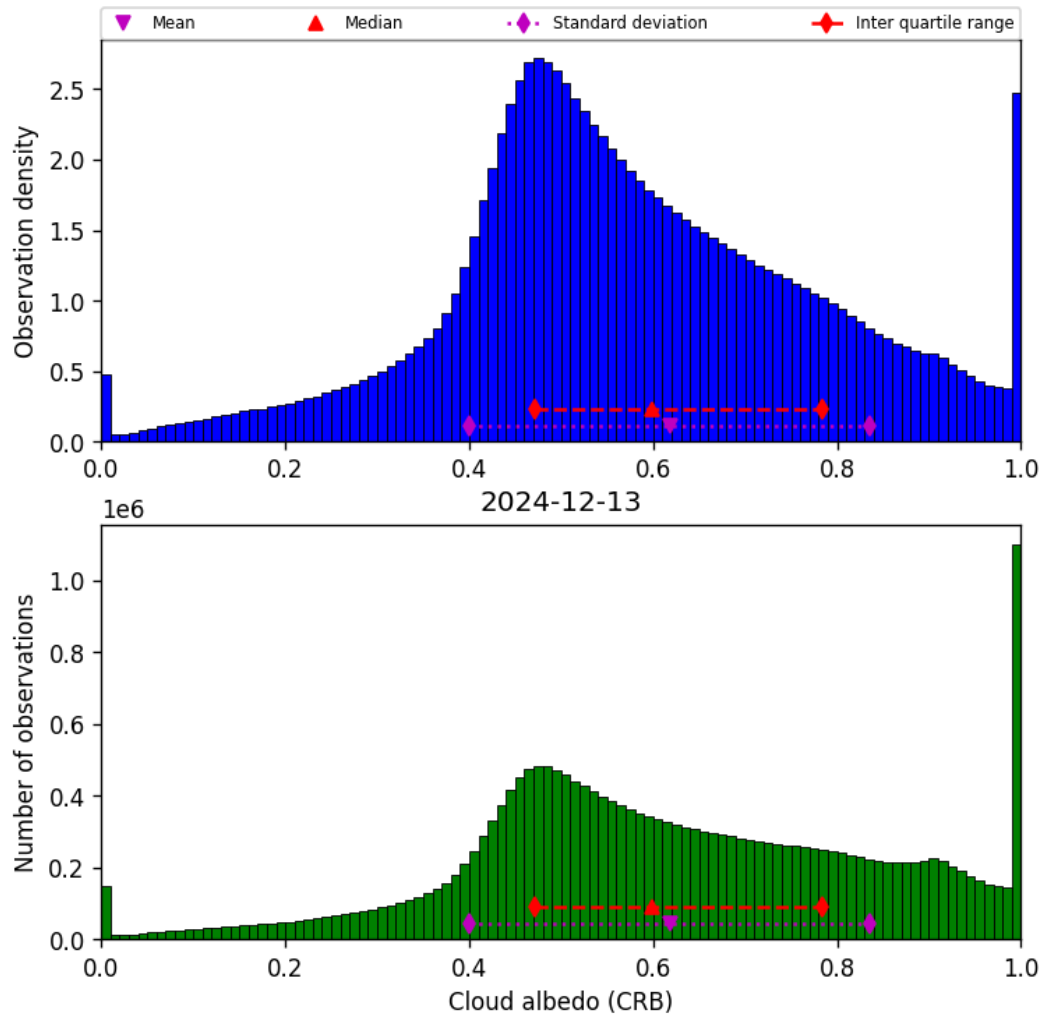
Figure 44: Histogram of “Cloud albedo (CRB)” for 2024-12-12 to 2024-12-14
