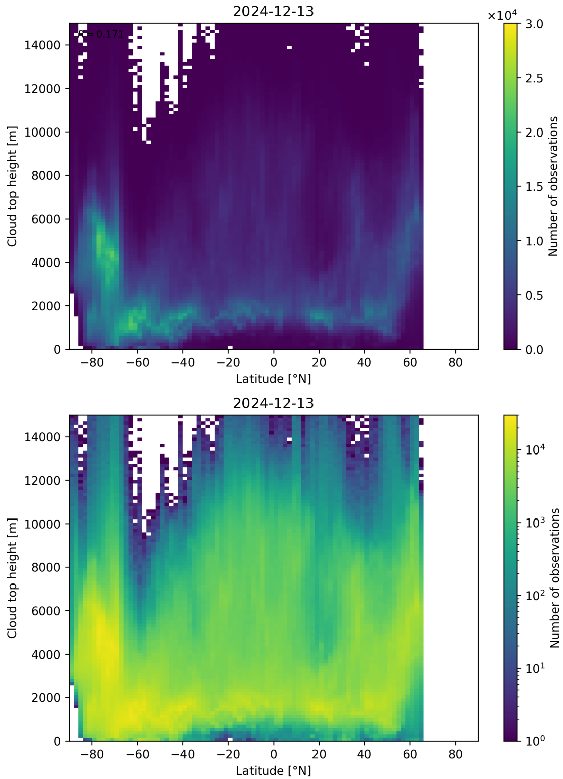
Figure 97: Scatter density plot of “Latitude” against “Cloud top height” for 2024-12-12 to 2024-12-14.
