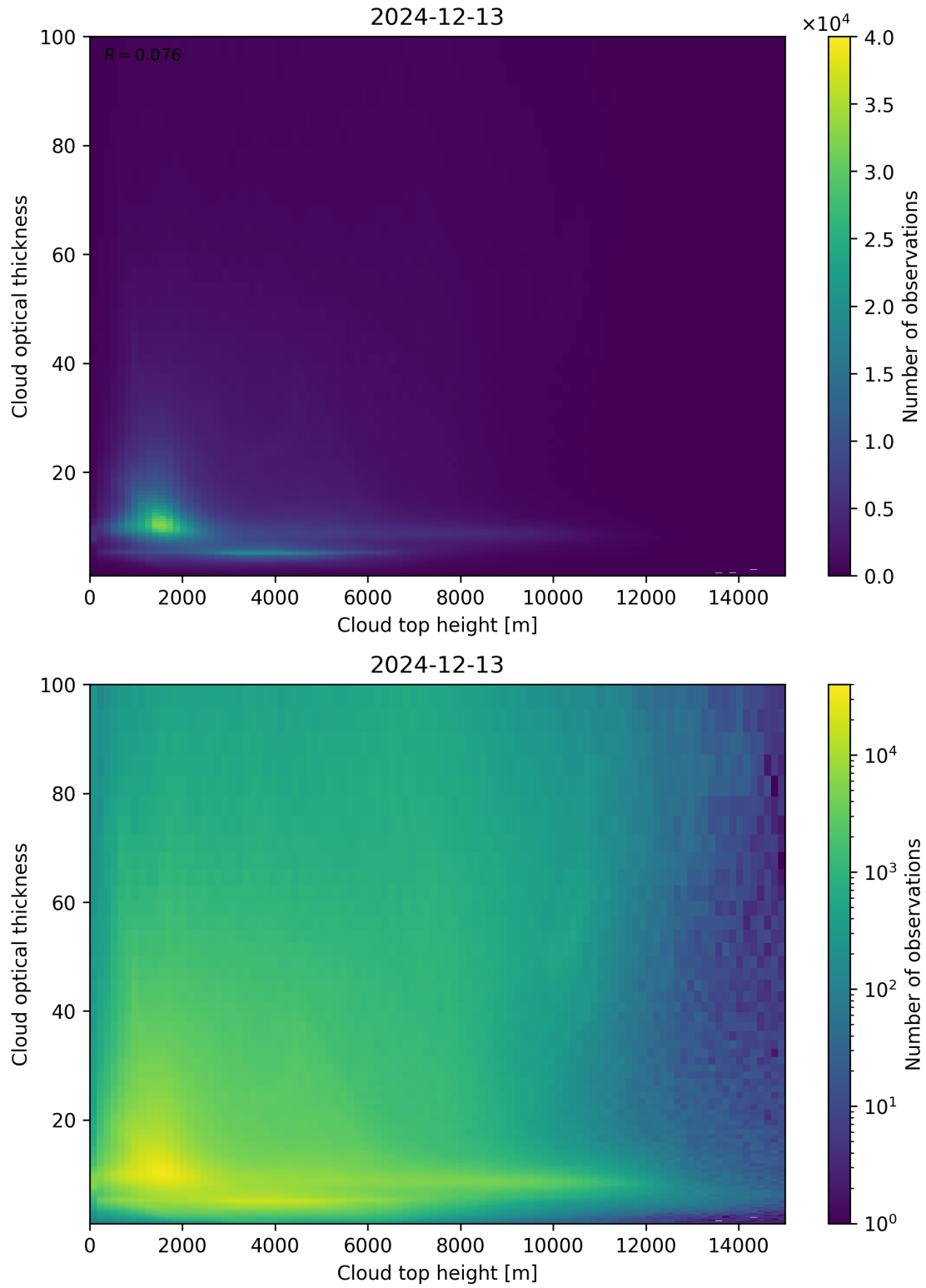
Figure 90: Scatter density plot of “Cloud top height” against “Cloud optical thickness” for 2024-12-12 to 2024-12-14.
