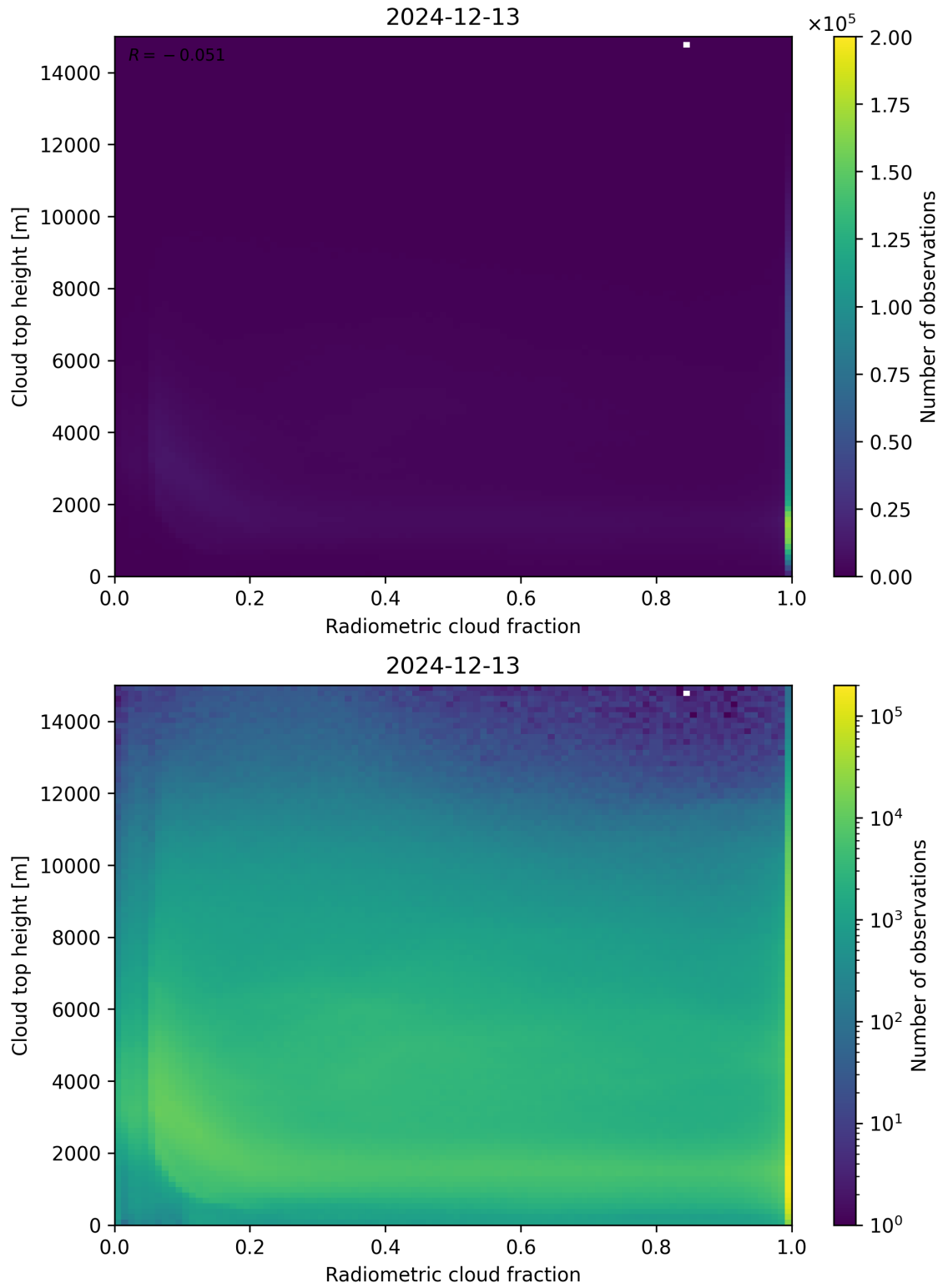
Figure 76: Scatter density plot of “Radiometric cloud fraction” against “Cloud top height” for 2024-12-12 to 2024-12-14.
