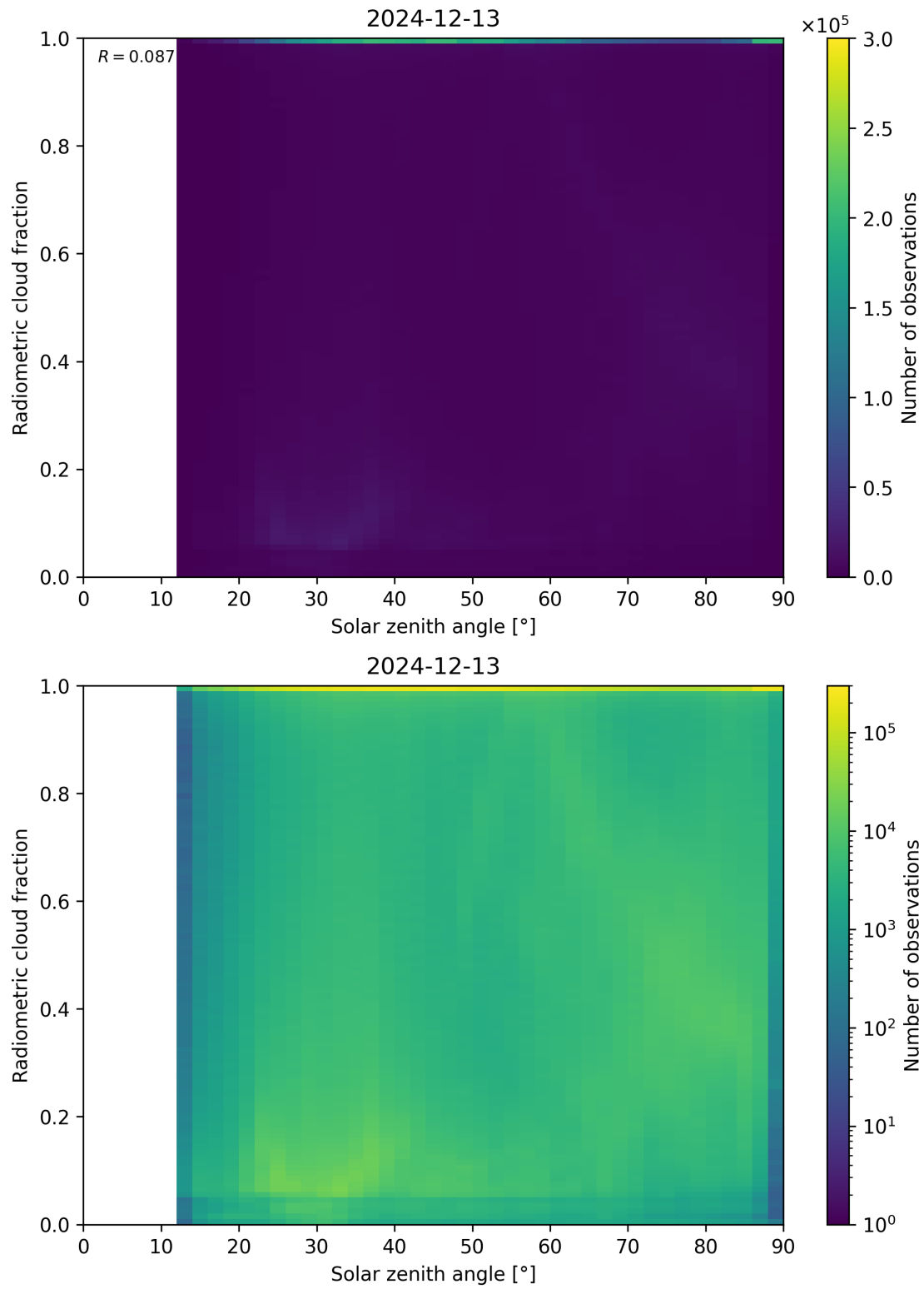
Figure 99: Scatter density plot of “Solar zenith angle” against “Radiometric cloud fraction” for 2024-12-12 to 2024-12-14.
