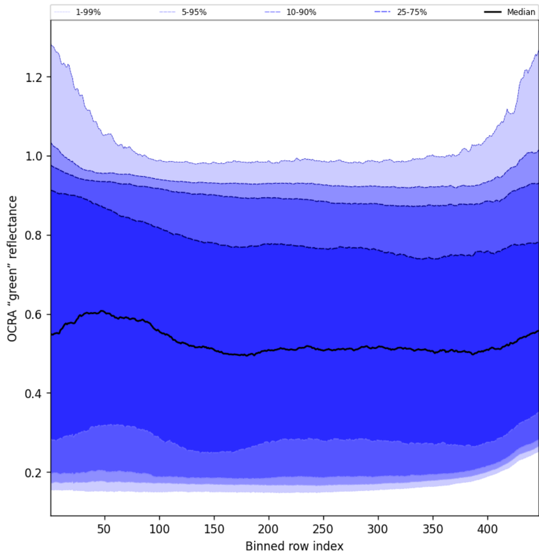
Figure 68: Along track statistics of "OCRA "green" reflectance" for 2024-12-12 to 2024-12-14
