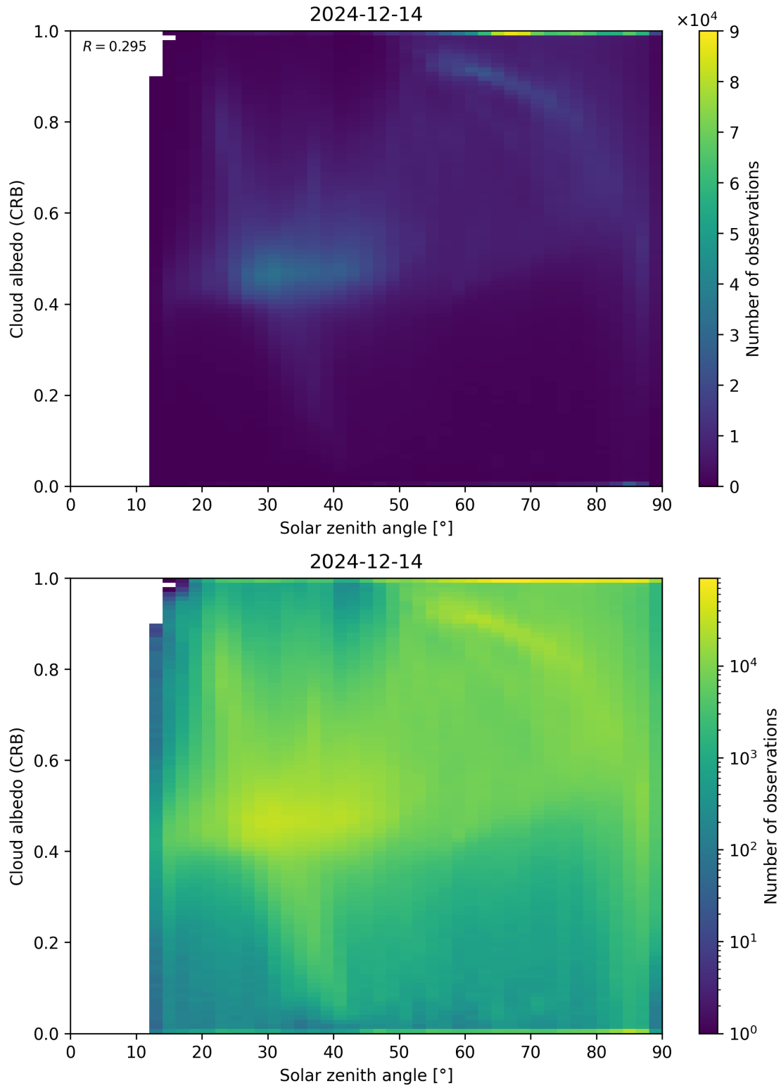
Figure 98: Scatter density plot of “Solar zenith angle” against “Cloud albedo (CRB)” for 2024-12-13 to 2024-12-15.
