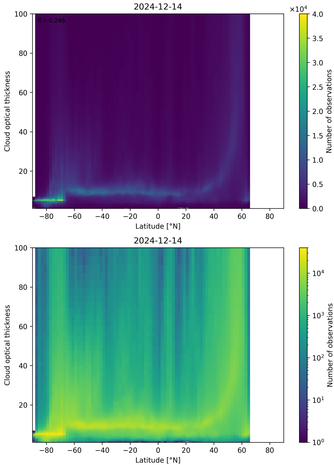
Figure 96: Scatter density plot of “Latitude” against “Cloud optical thickness” for 2024-12-13 to 2024-12-15.
