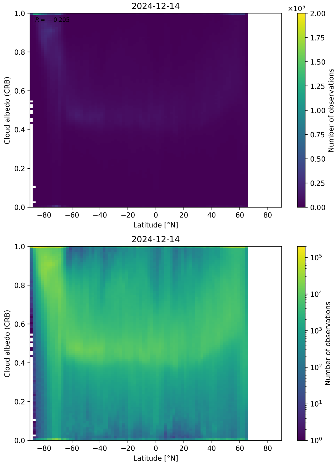
Figure 91: Scatter density plot of “Latitude” against “Cloud albedo (CRB)” for 2024-12-13 to 2024-12-15.
