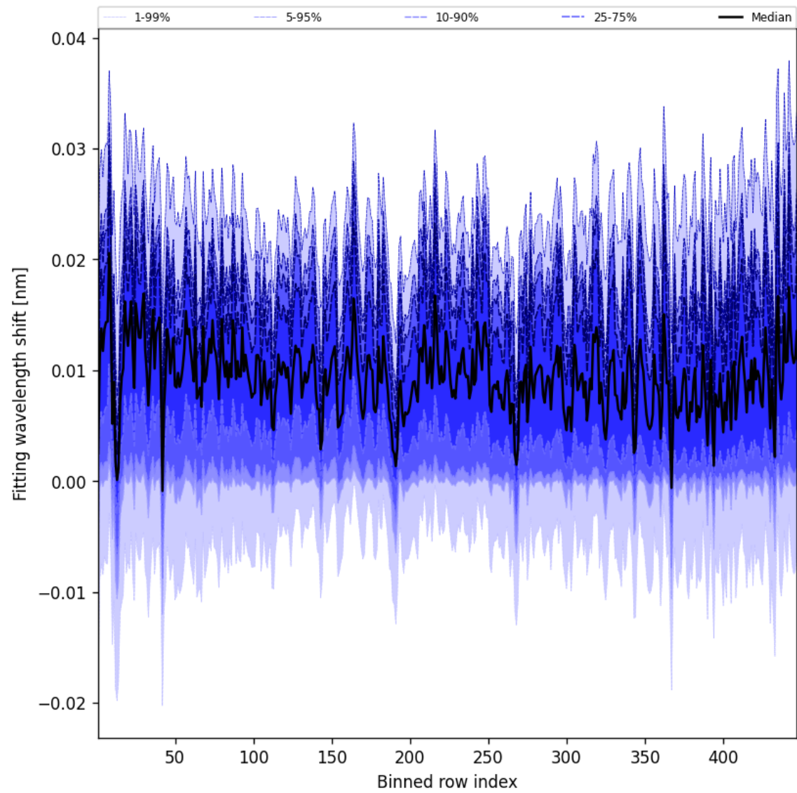
Figure 65: Along track statistics of “Fitting wavelength shift” for 2024-12-13 to 2024-12-15
