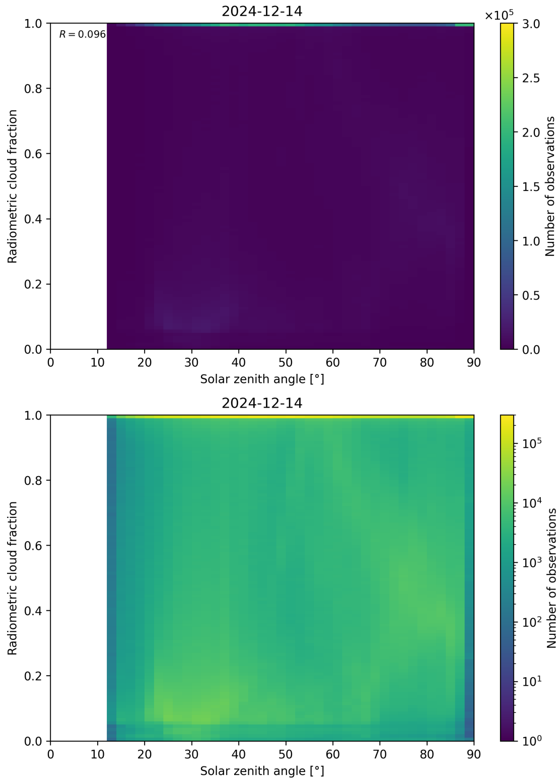
Figure 99: Scatter density plot of “Solar zenith angle” against “Radiometric cloud fraction” for 2024-12-13 to 2024-12-15.
