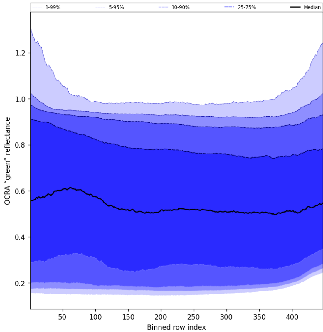
Figure 68: Along track statistics of “OCRA “green” reflectance” for 2024-12-13 to 2024-12-15
