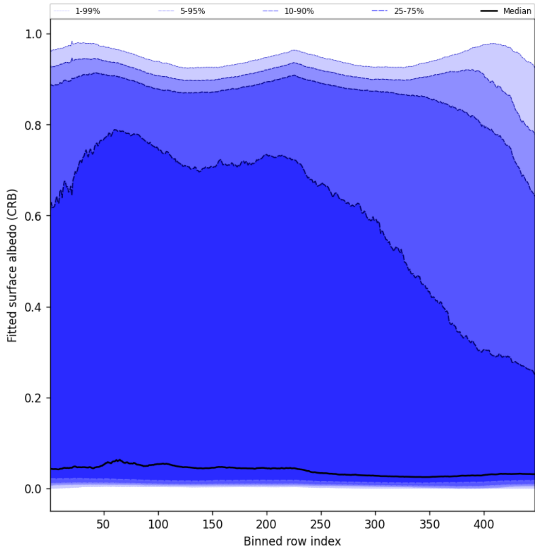
Figure 62: Along track statistics of “Fitted surface albedo (CRB)” for 2024-12-13 to 2024-12-15
