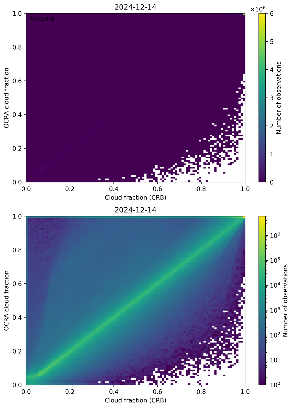
Figure 78: Scatter density plot of “Cloud fraction (CRB)” against “OCRA cloud fraction” for 2024-12-13 to 2024-12-15.
