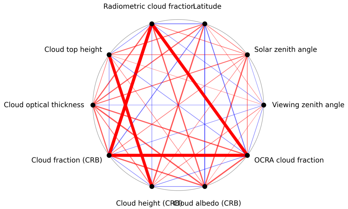
Figure 1: Map of correlation graph for 2024-12-13 to 2024-12-15.
