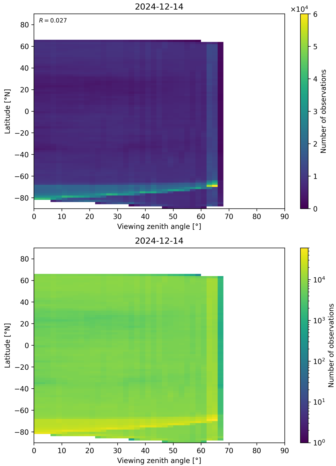
Figure 113: Scatter density plot of “Viewing zenith angle” against “Latitude” for 2024-12-13 to 2024-12-15.
