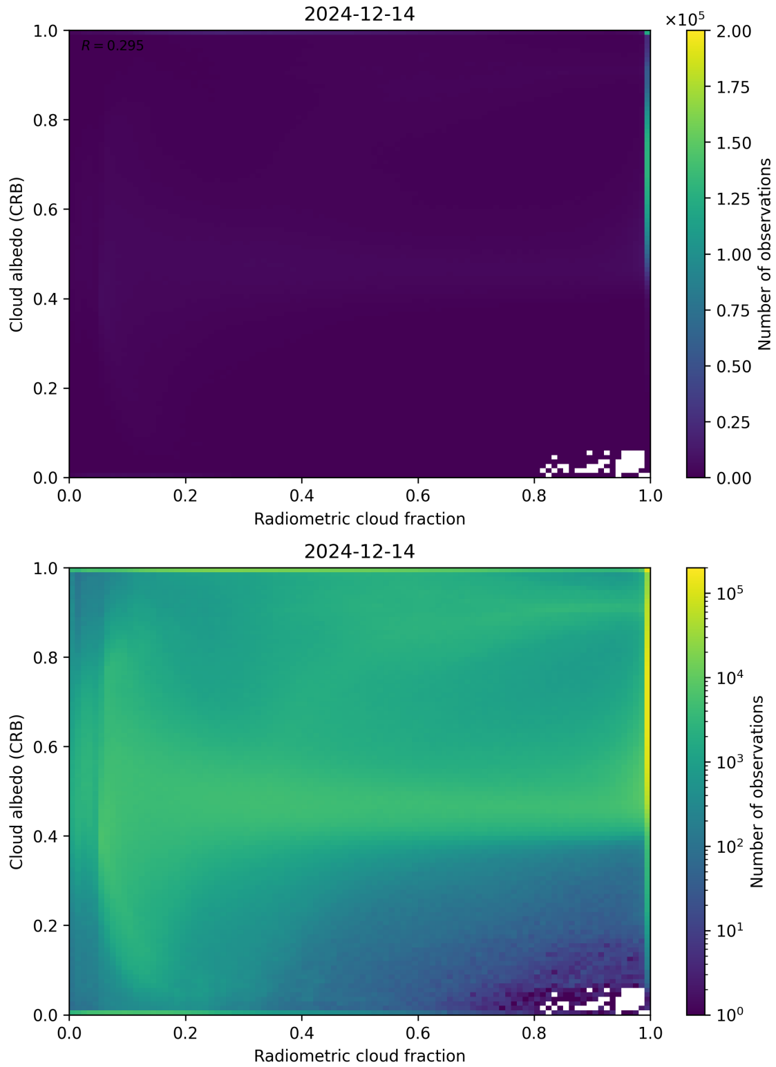
Figure 71: Scatter density plot of “Radiometric cloud fraction” against “Cloud albedo (CRB)” for 2024-12-13 to 2024-12-15.
