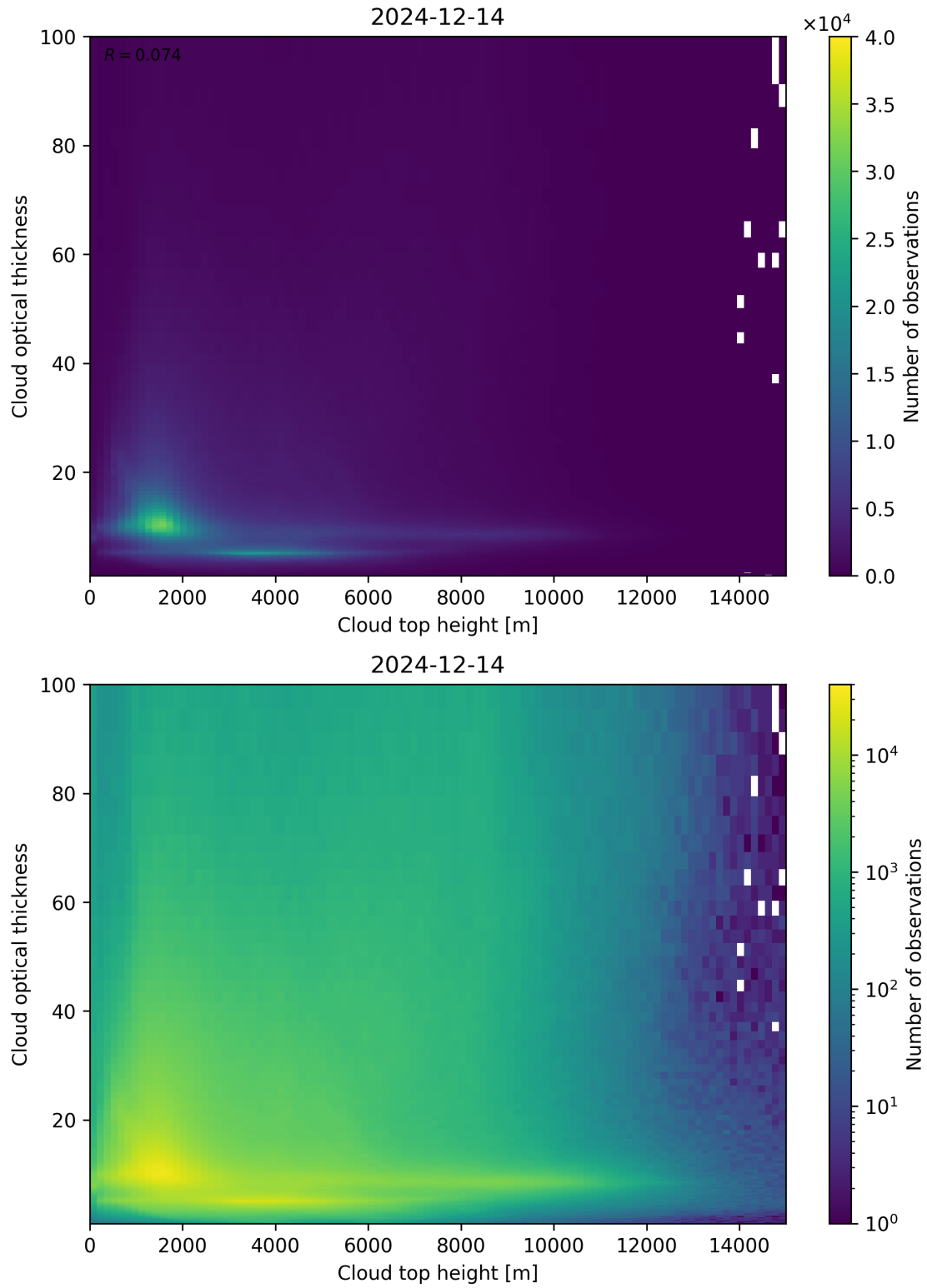
Figure 90: Scatter density plot of “Cloud top height” against “Cloud optical thickness” for 2024-12-13 to 2024-12-15.
