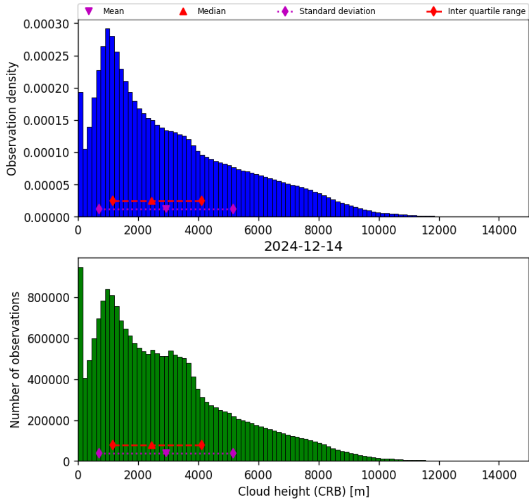
Figure 43: Histogram of “Cloud height (CRB)” for 2024-12-13 to 2024-12-15
