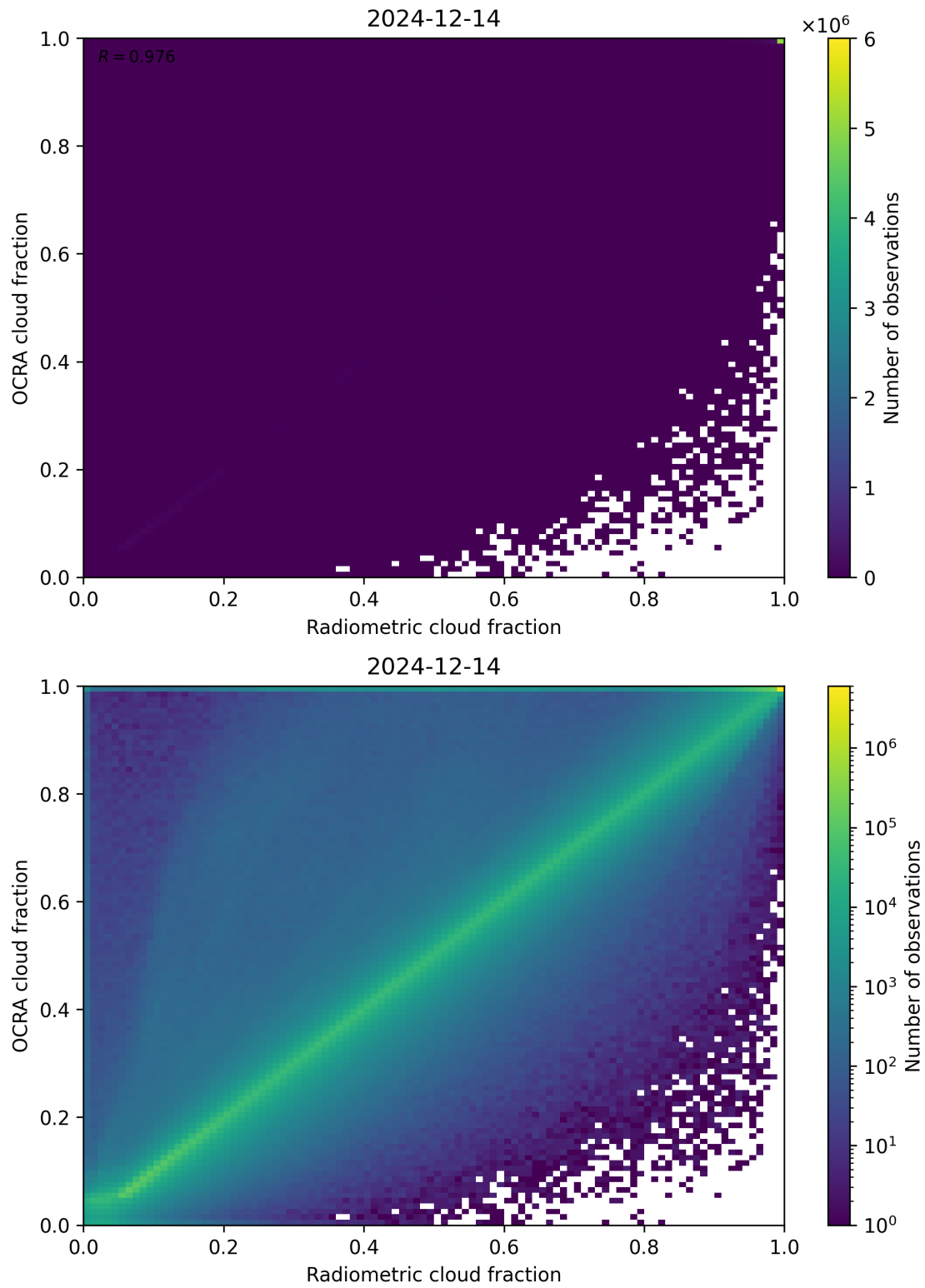
Figure 72: Scatter density plot of “Radiometric cloud fraction” against “OCRA cloud fraction” for 2024-12-13 to 2024-12-15.
