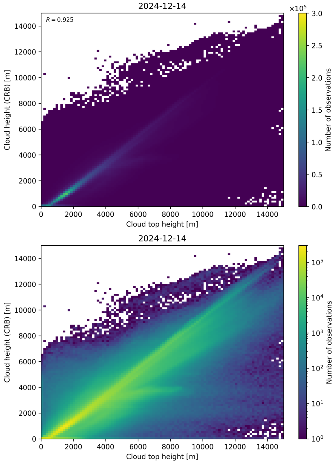
Figure 89: Scatter density plot of “Cloud top height” against “Cloud height (CRB)” for 2024-12-13 to 2024-12-15.
