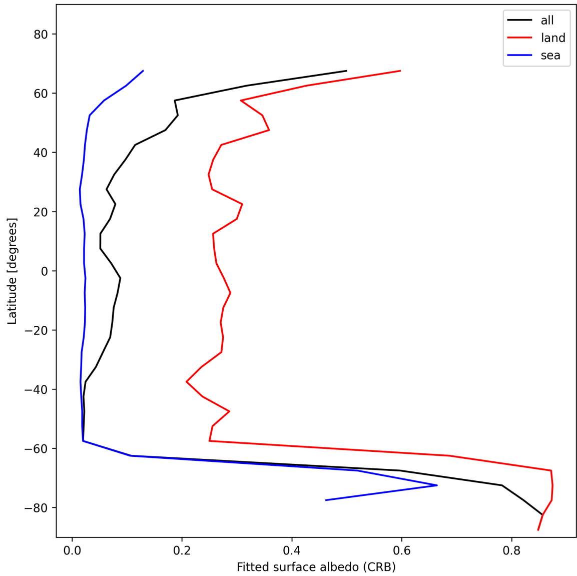
Figure 30: Zonal average of “Fitted surface albedo (CRB)” for 2024-12-13 to 2024-12-15.
