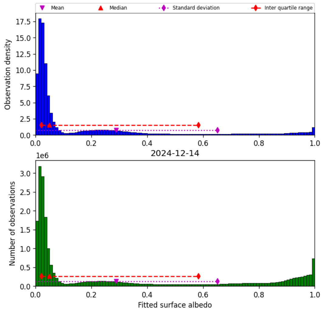
Figure 45: Histogram of “Fitted surface albedo” for 2024-12-13 to 2024-12-15
