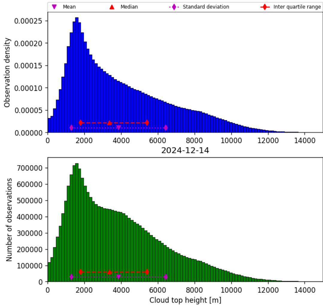
Figure 40: Histogram of “Cloud top height” for 2024-12-13 to 2024-12-15
