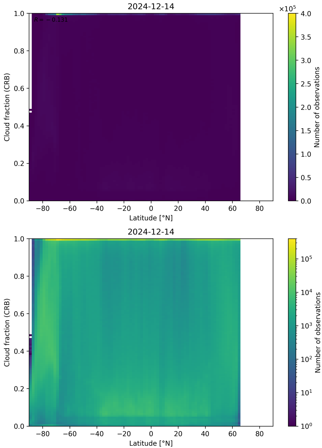
Figure 94: Scatter density plot of “Latitude” against “Cloud fraction (CRB)” for 2024-12-13 to 2024-12-15.
