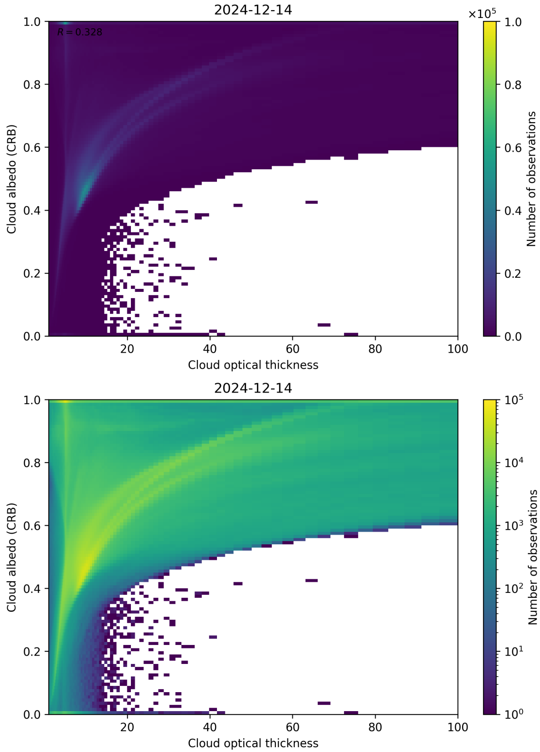
Figure 82: Scatter density plot of “Cloud optical thickness” against “Cloud albedo (CRB)” for 2024-12-13 to 2024-12-15.
