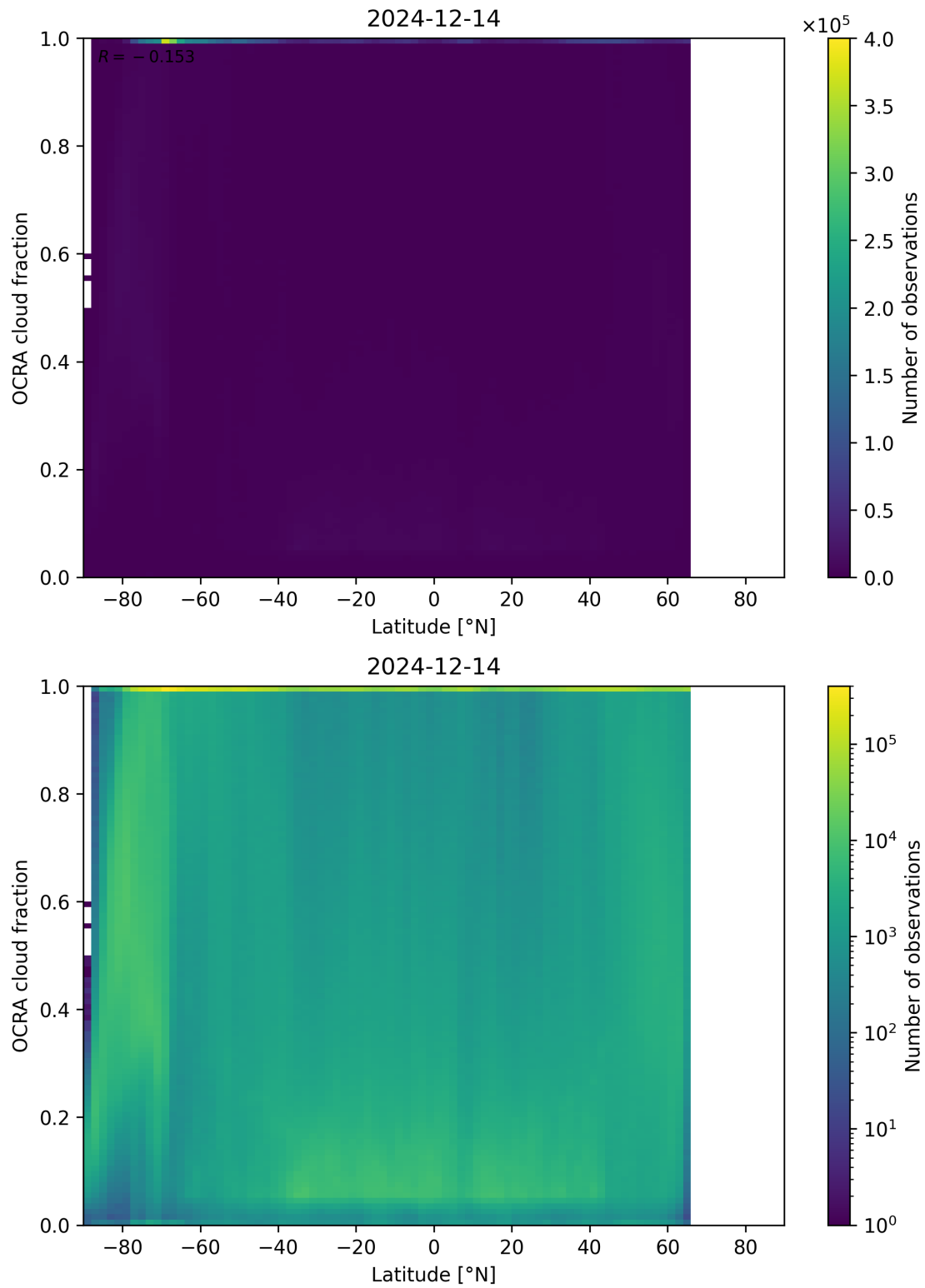
Figure 93: Scatter density plot of “Latitude” against “OCRA cloud fraction” for 2024-12-13 to 2024-12-15.
