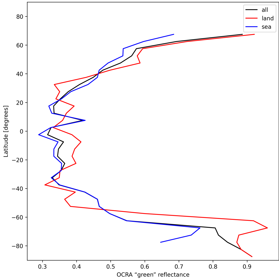
Figure 36: Zonal average of “OCRA “green” reflectance” for 2024-12-13 to 2024-12-15.
