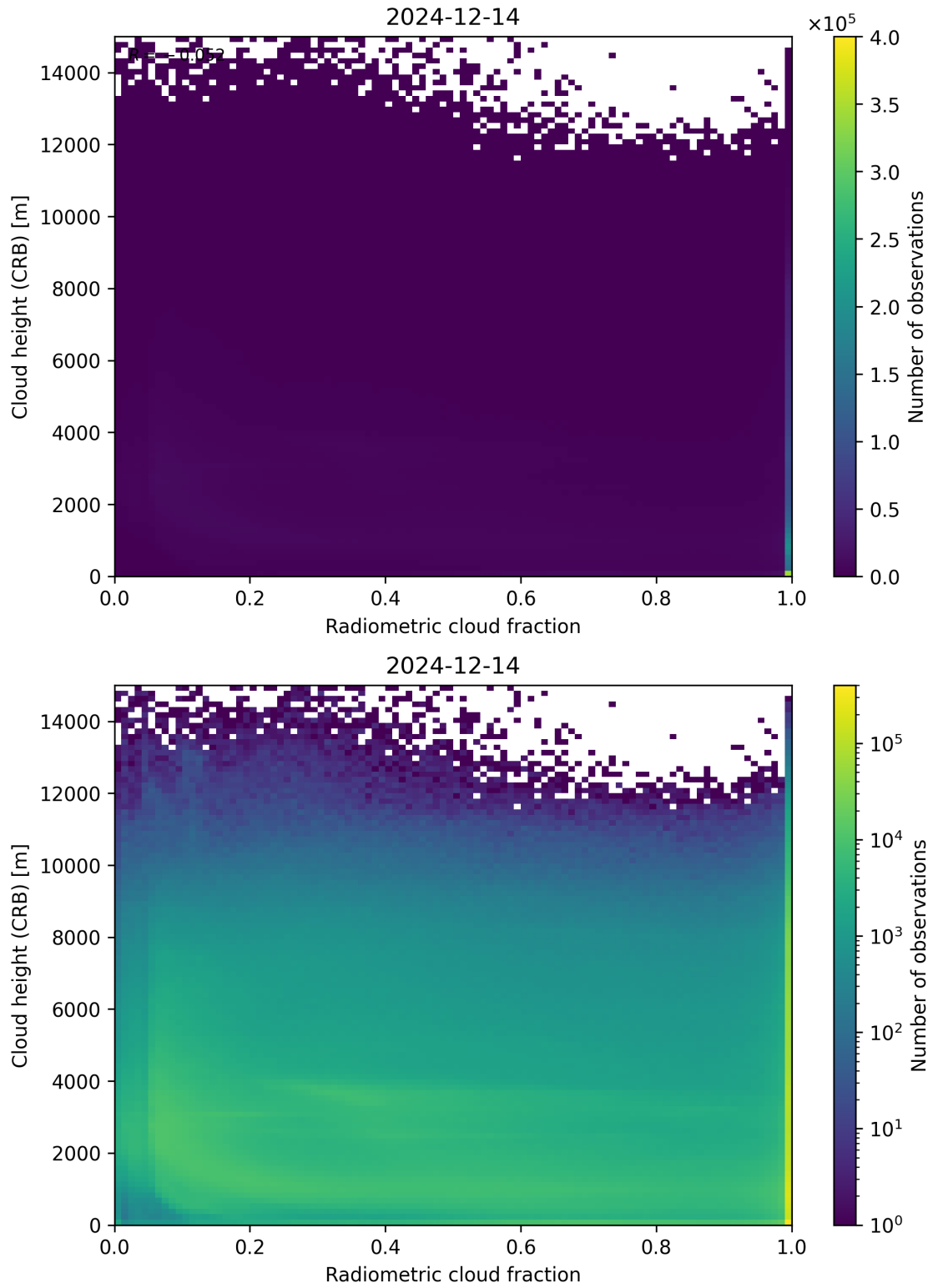
Figure 74: Scatter density plot of “Radiometric cloud fraction” against “Cloud height (CRB)” for 2024-12-13 to 2024-12-15.
