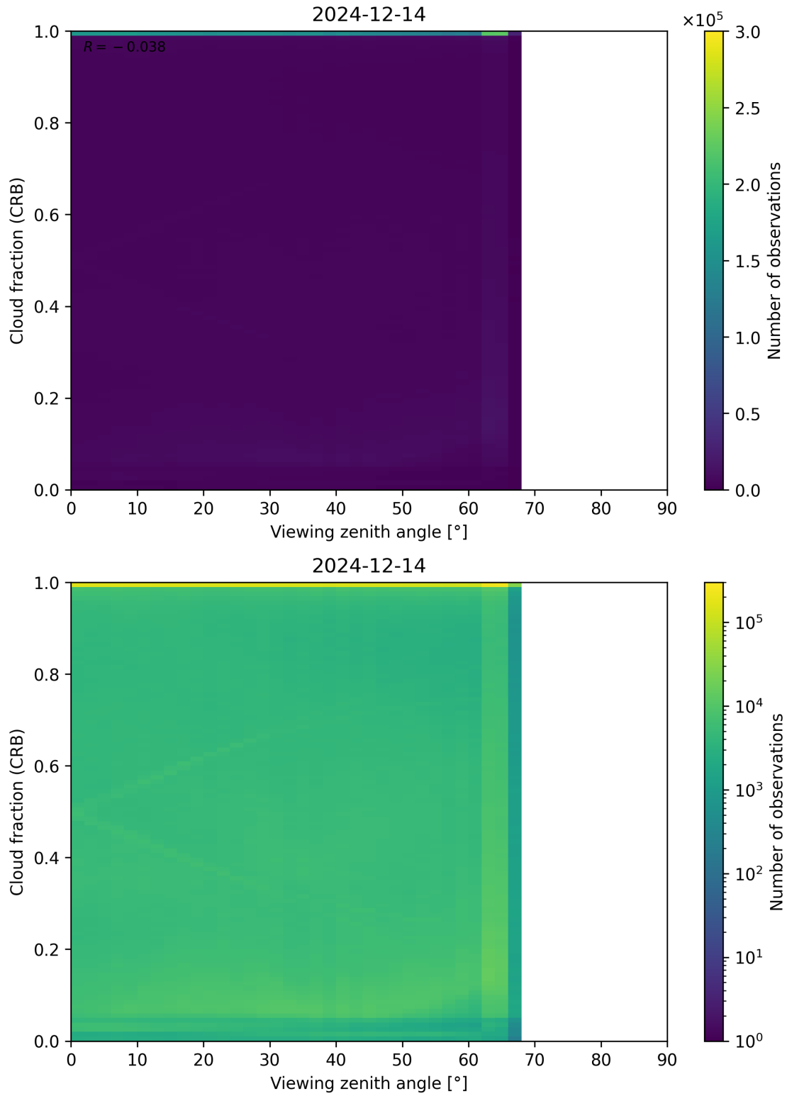
Figure 109: Scatter density plot of “Viewing zenith angle” against “Cloud fraction (CRB)” for 2024-12-13 to 2024-12-15.
