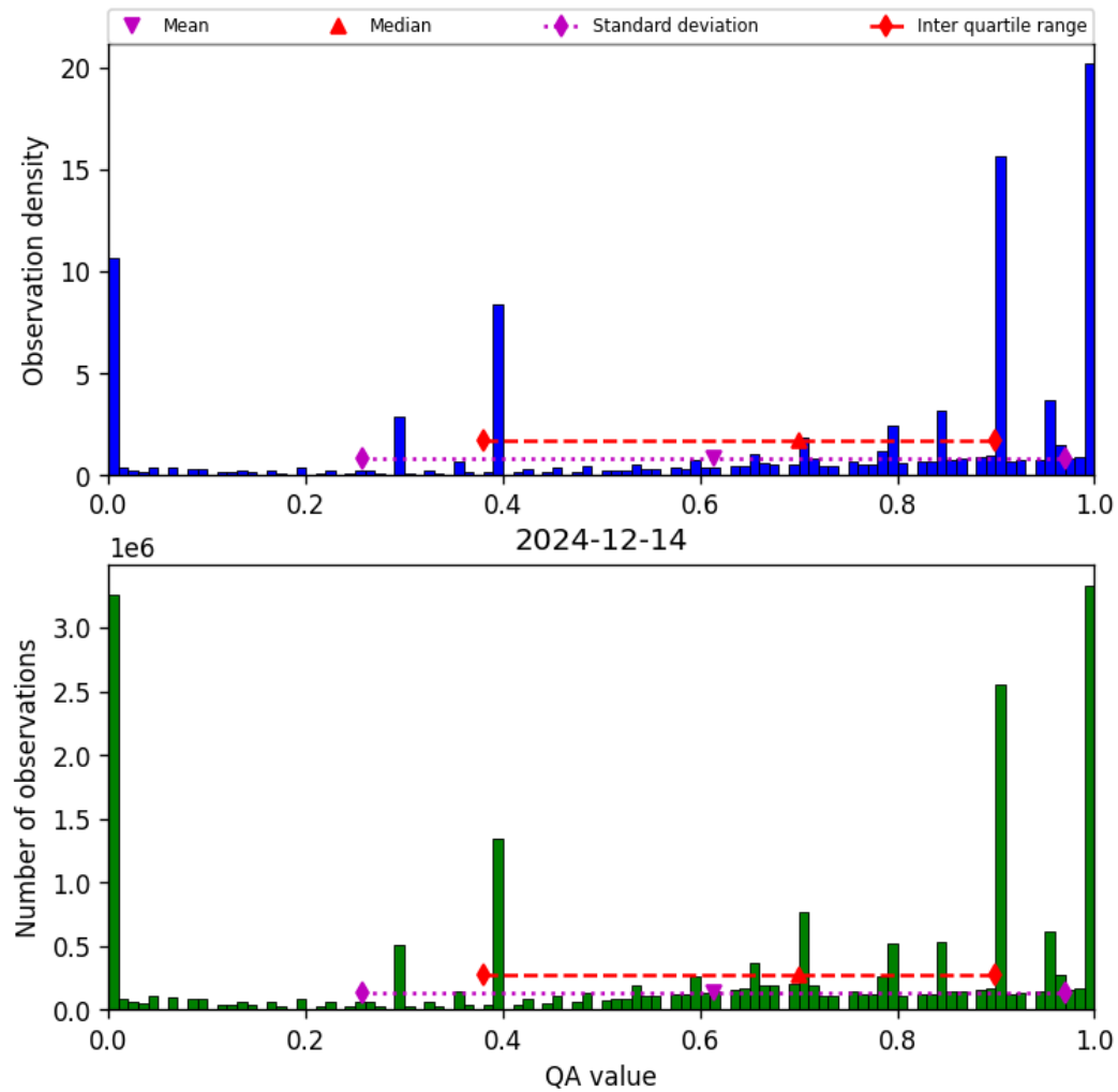
Figure 38: Histogram of “QA value” for 2024-12-13 to 2024-12-15
