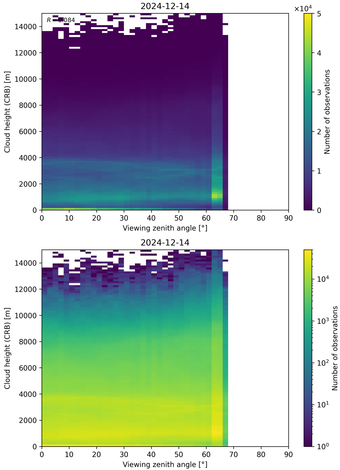
Figure 110: Scatter density plot of “Viewing zenith angle” against “Cloud height (CRB)” for 2024-12-13 to 2024-12-15.
