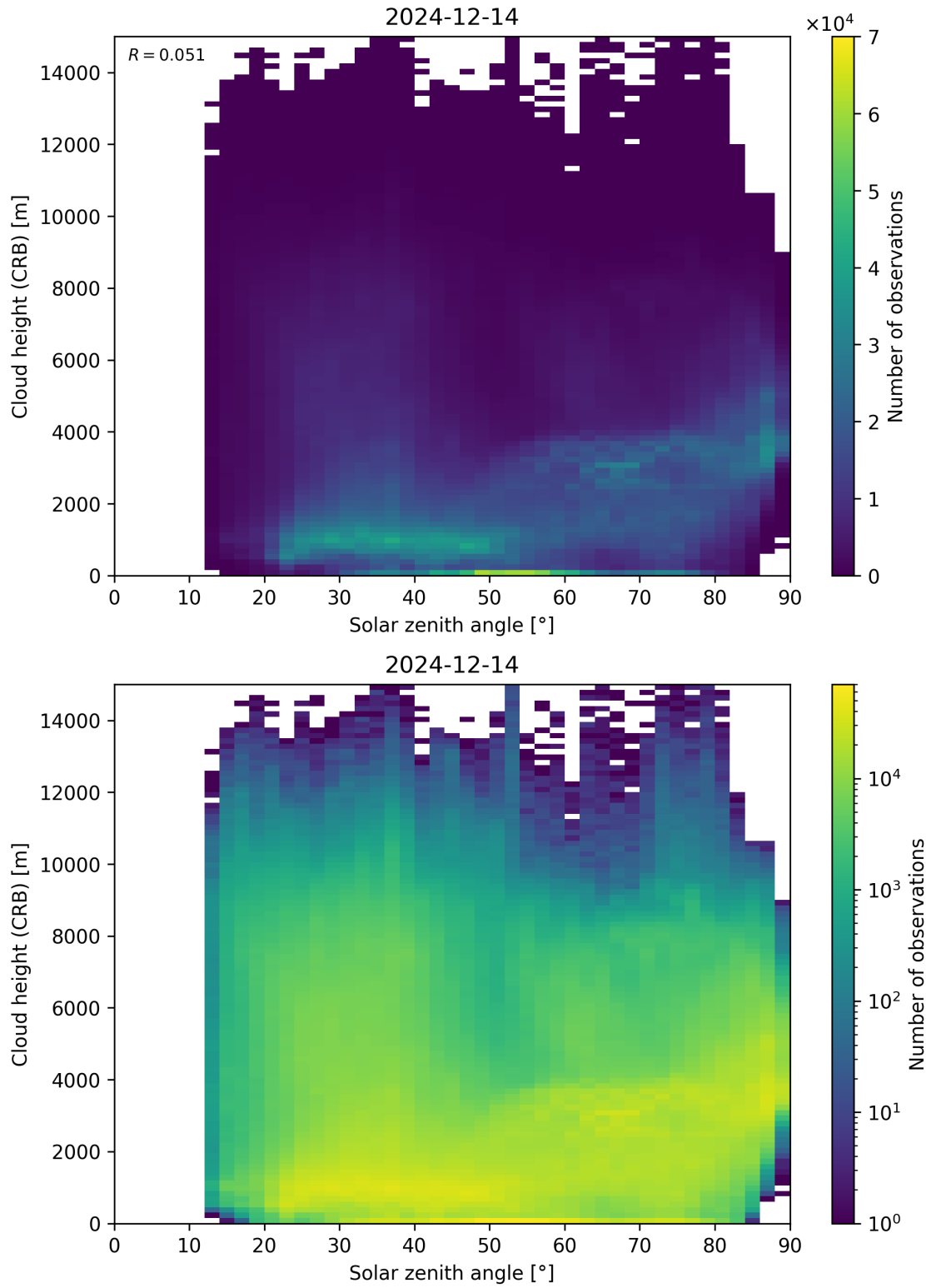
Figure 102: Scatter density plot of “Solar zenith angle” against “Cloud height (CRB)” for 2024-12-13 to 2024-12-15.
