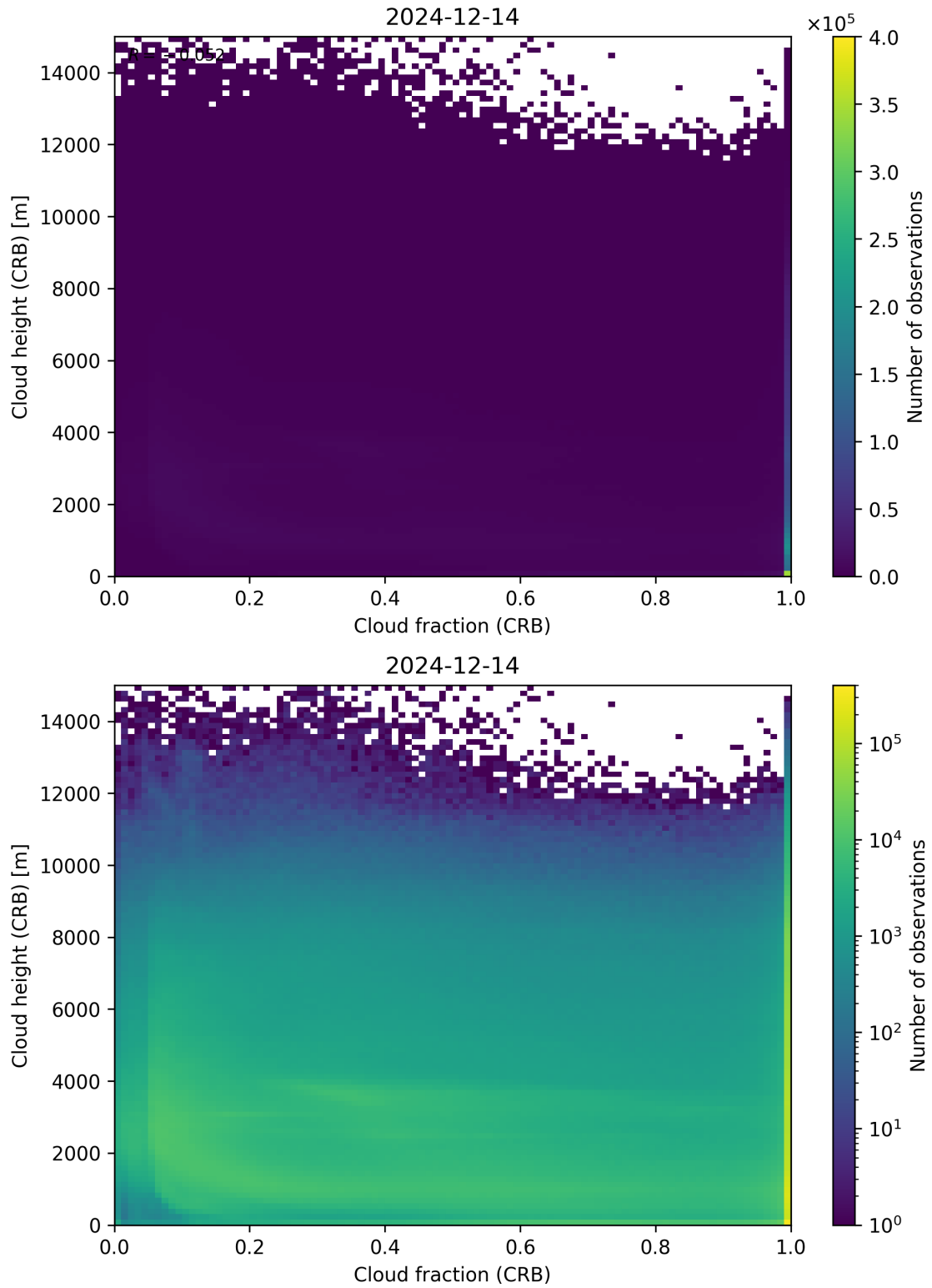
Figure 79: Scatter density plot of “Cloud fraction (CRB)” against “Cloud height (CRB)” for 2024-12-13 to 2024-12-15.
