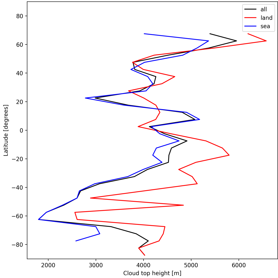
Figure 24: Zonal average of “Cloud top height” for 2024-12-13 to 2024-12-15.
