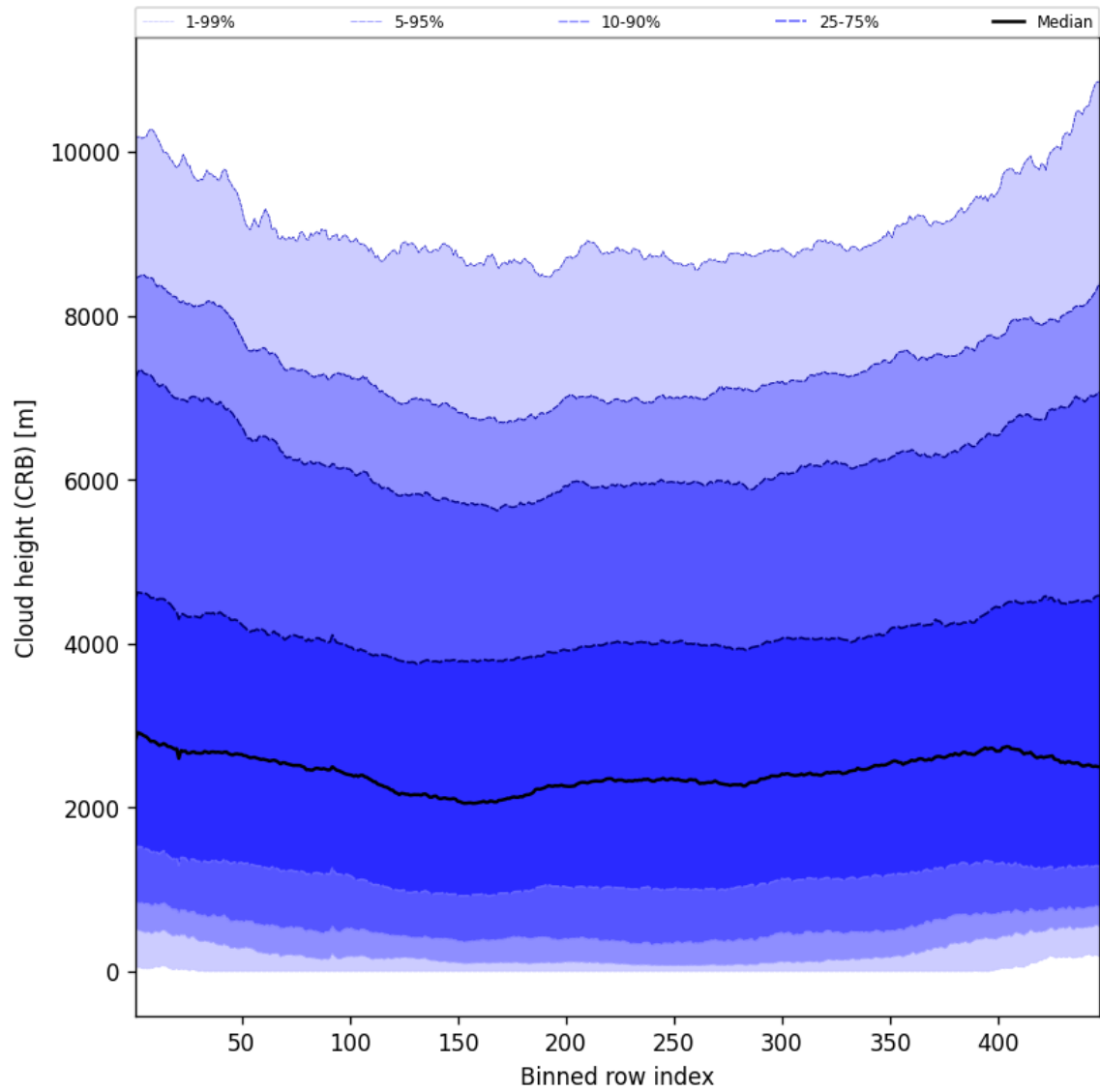
Figure 59: Along track statistics of “Cloud height (CRB)” for 2024-12-13 to 2024-12-15
