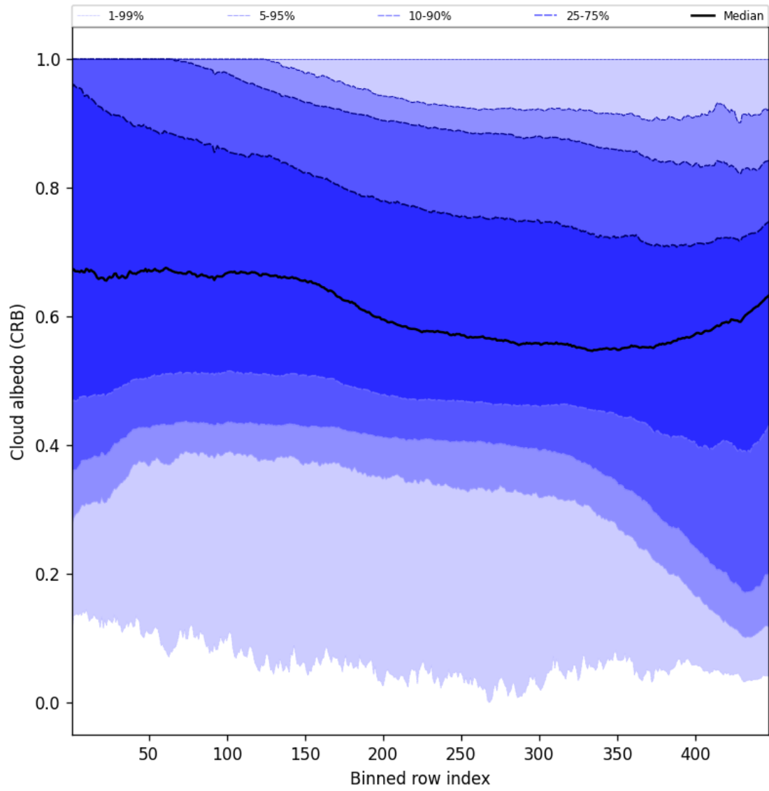
Figure 60: Along track statistics of “Cloud albedo (CRB)” for 2024-12-13 to 2024-12-15
