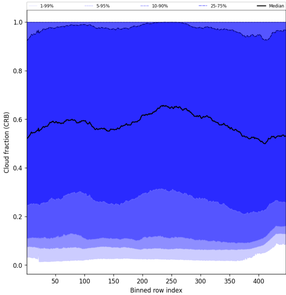
Figure 58: Along track statistics of “Cloud fraction (CRB)” for 2024-12-13 to 2024-12-15
