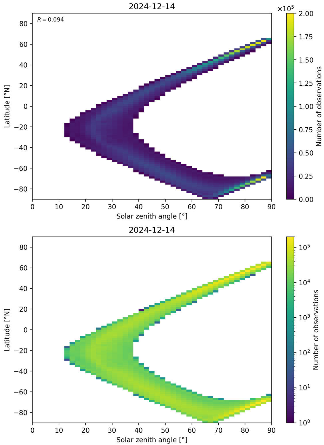
Figure 105: Scatter density plot of “Solar zenith angle” against “Latitude” for 2024-12-13 to 2024-12-15.
