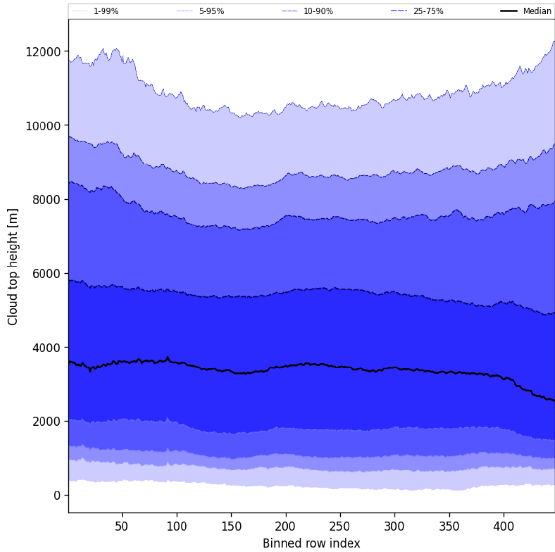
Figure 56: Along track statistics of “Cloud top height” for 2024-12-13 to 2024-12-15
