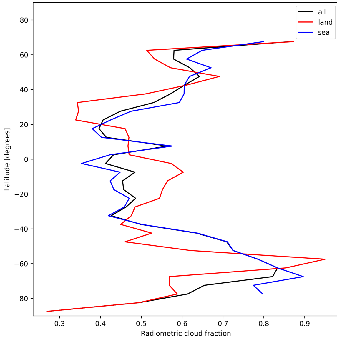
Figure 23: Zonal average of “Radiometric cloud fraction” for 2024-12-13 to 2024-12-15.
