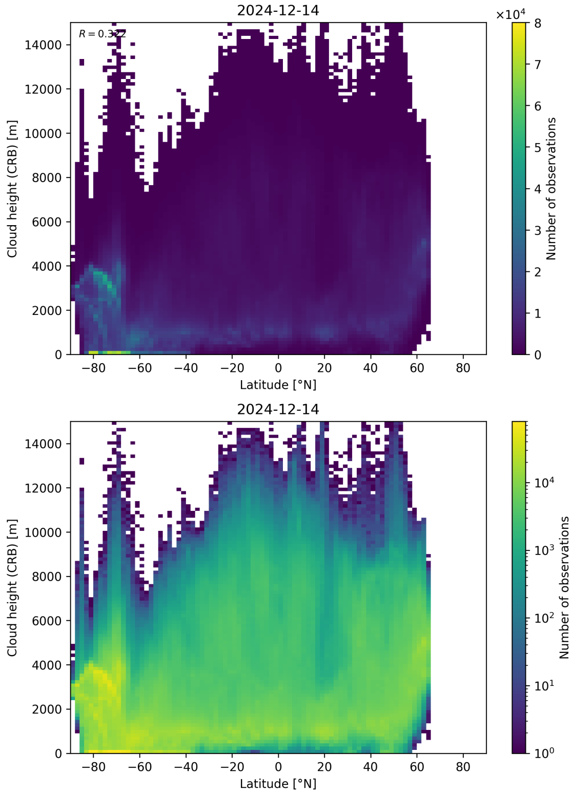
Figure 95: Scatter density plot of “Latitude” against “Cloud height (CRB)” for 2024-12-13 to 2024-12-15.
