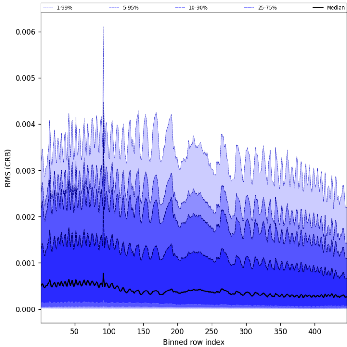
Figure 64: Along track statistics of “RMS (CRB)” for 2024-12-13 to 2024-12-15
