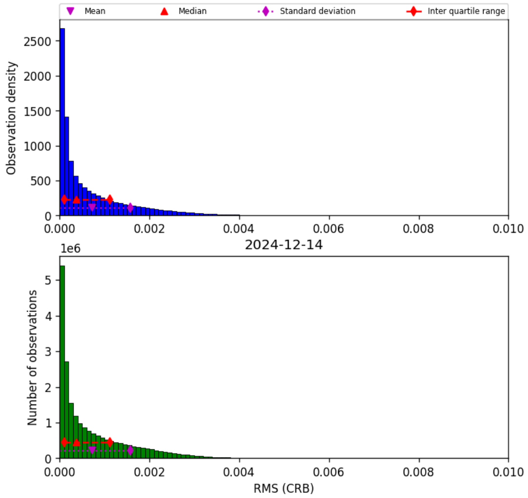
Figure 48: Histogram of “RMS (CRB)” for 2024-12-13 to 2024-12-15
