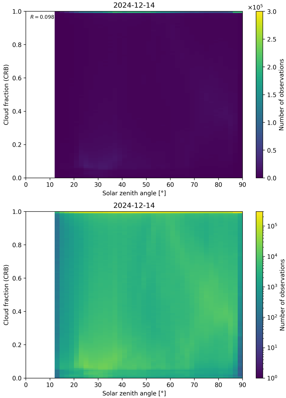
Figure 101: Scatter density plot of “Solar zenith angle” against “Cloud fraction (CRB)” for 2024-12-13 to 2024-12-15.
