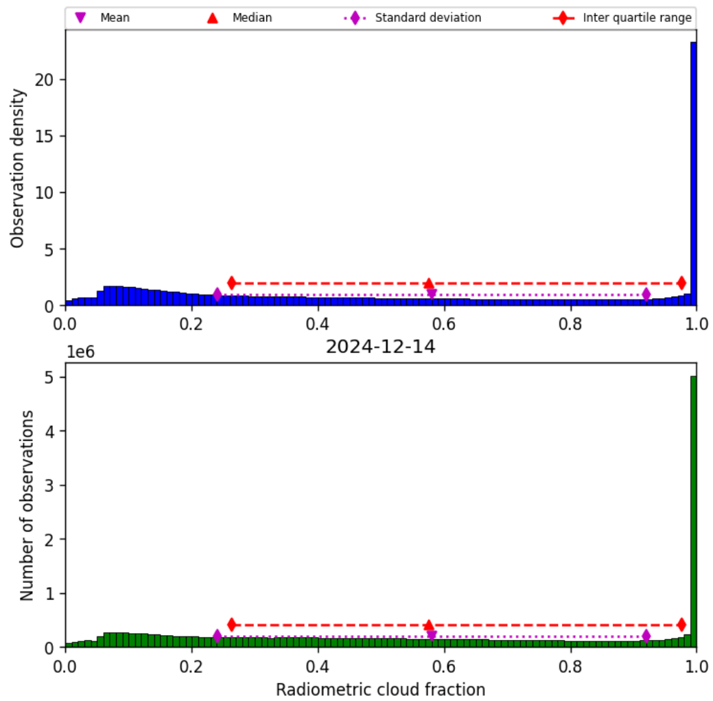
Figure 39: Histogram of “Radiometric cloud fraction” for 2024-12-13 to 2024-12-15
