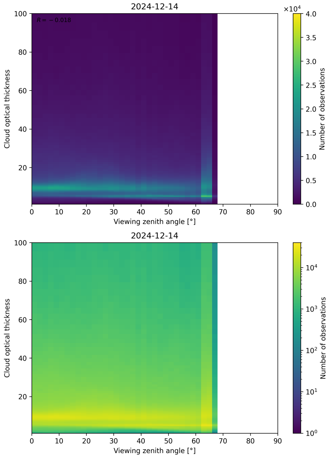
Figure 111: Scatter density plot of “Viewing zenith angle” against “Cloud optical thickness” for 2024-12-13 to 2024-12-15.
