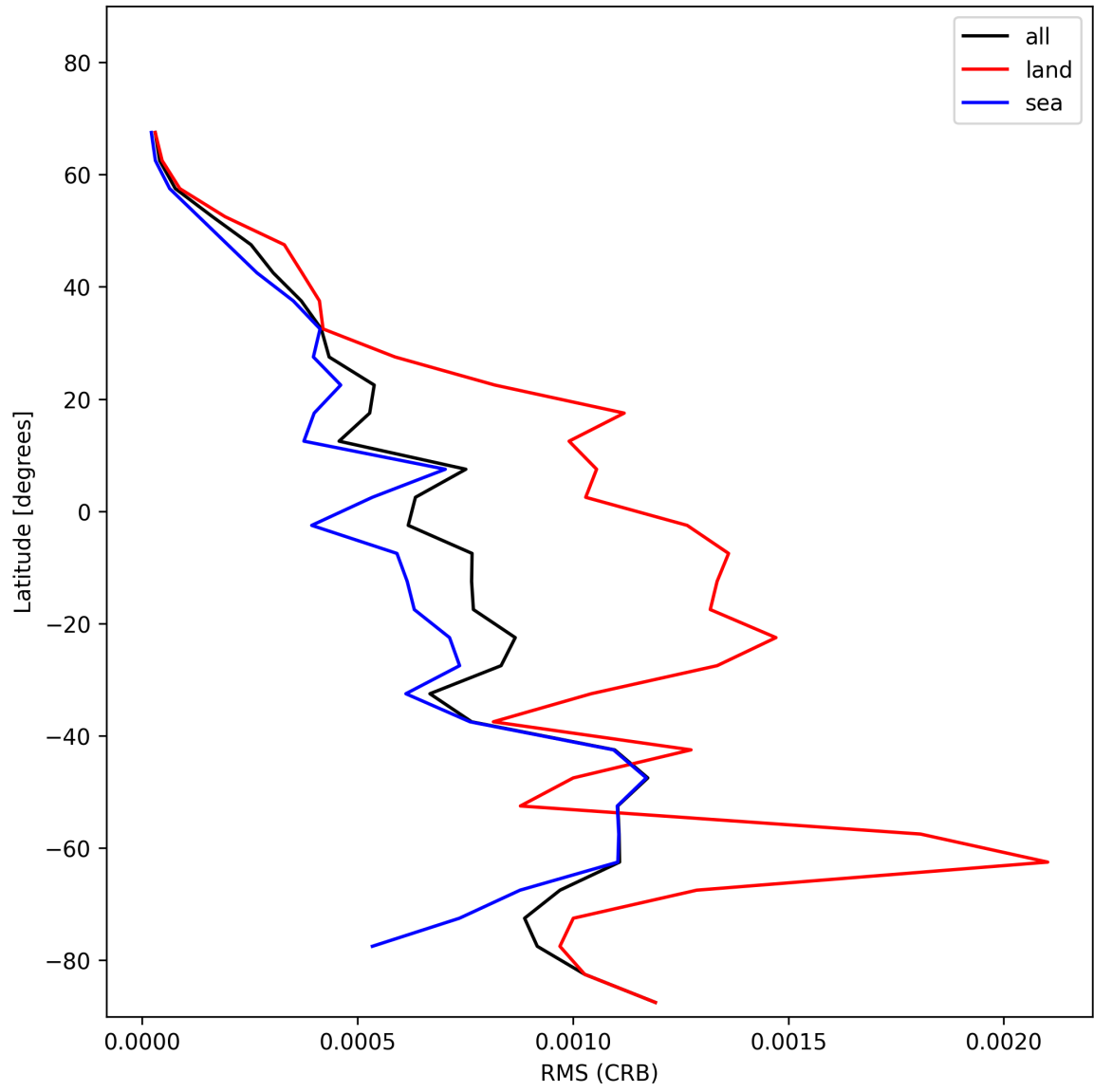
Figure 32: Zonal average of “RMS (CRB)” for 2024-12-13 to 2024-12-15.
