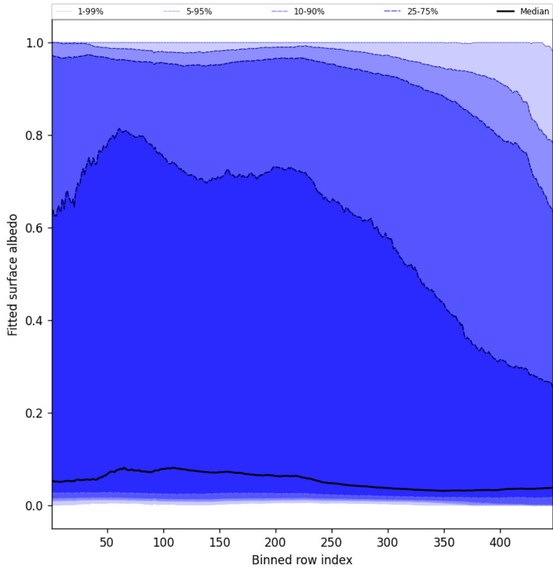
Figure 61: Along track statistics of “Fitted surface albedo” for 2024-12-13 to 2024-12-15
