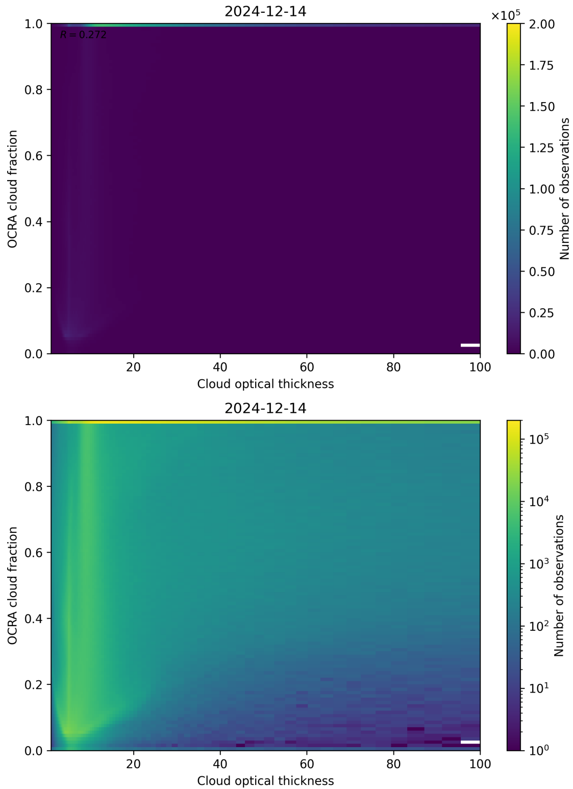
Figure 83: Scatter density plot of “Cloud optical thickness” against “OCRA cloud fraction” for 2024-12-13 to 2024-12-15.
