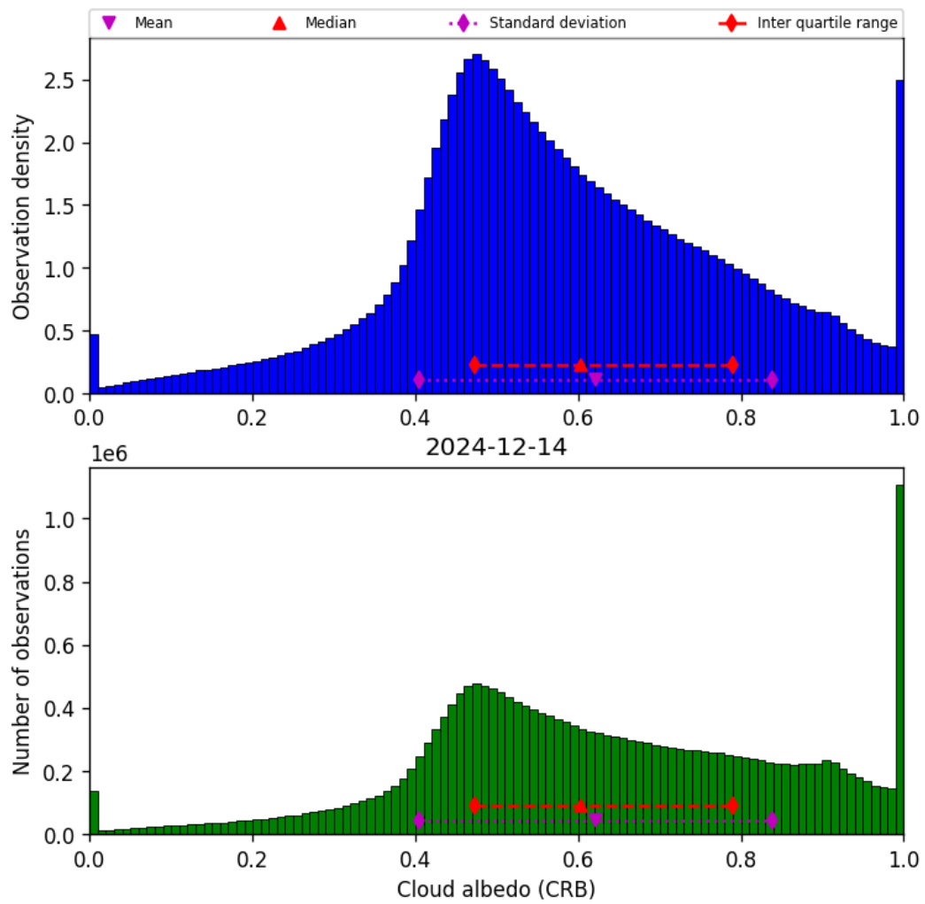
Figure 44: Histogram of “Cloud albedo (CRB)” for 2024-12-13 to 2024-12-15
