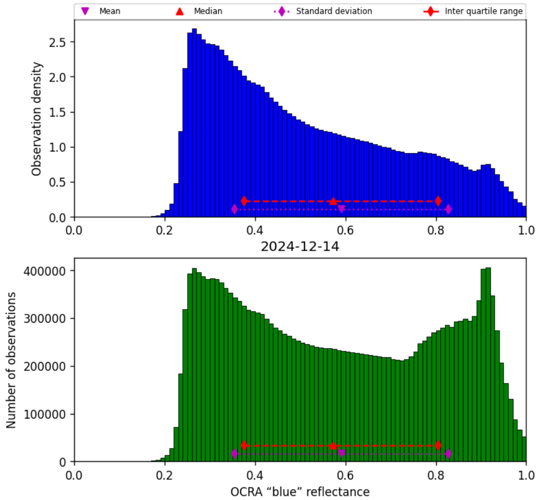
Figure 51: Histogram of “OCRA “blue” reflectance” for 2024-12-13 to 2024-12-15
