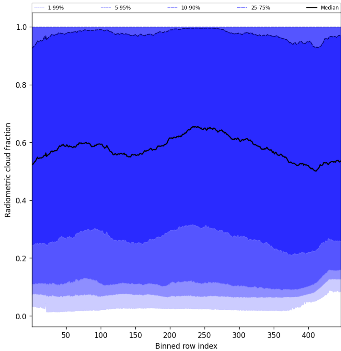
Figure 55: Along track statistics of “Radiometric cloud fraction” for 2024-12-13 to 2024-12-15
