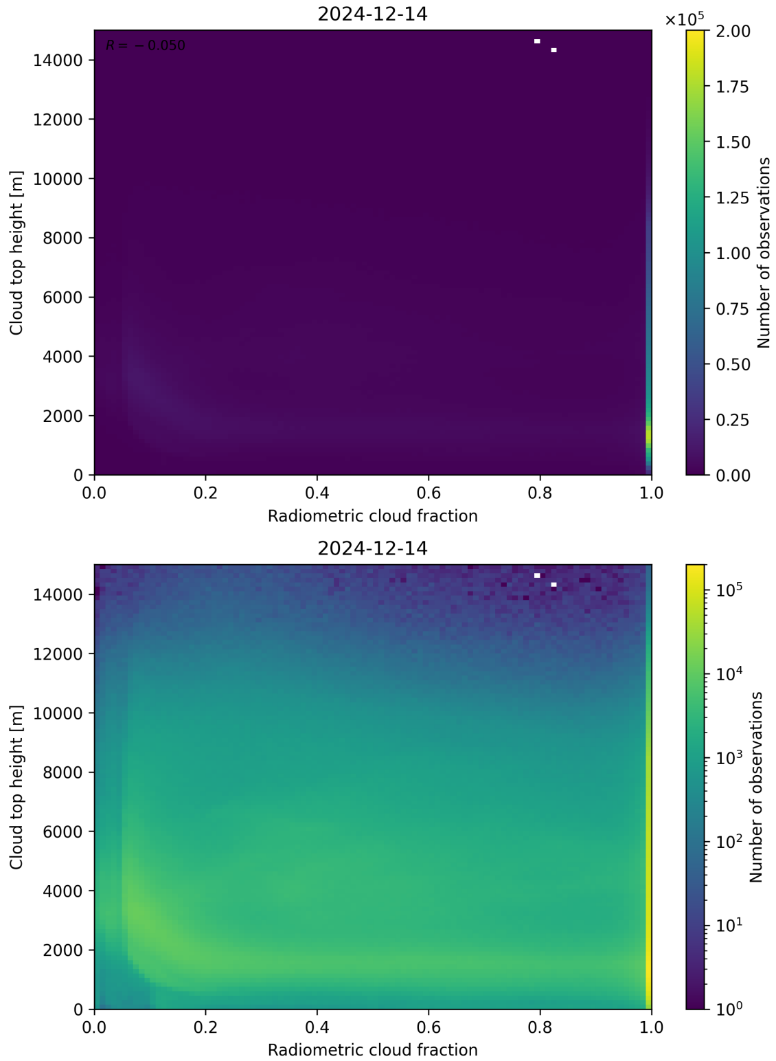
Figure 76: Scatter density plot of “Radiometric cloud fraction” against “Cloud top height” for 2024-12-13 to 2024-12-15.
