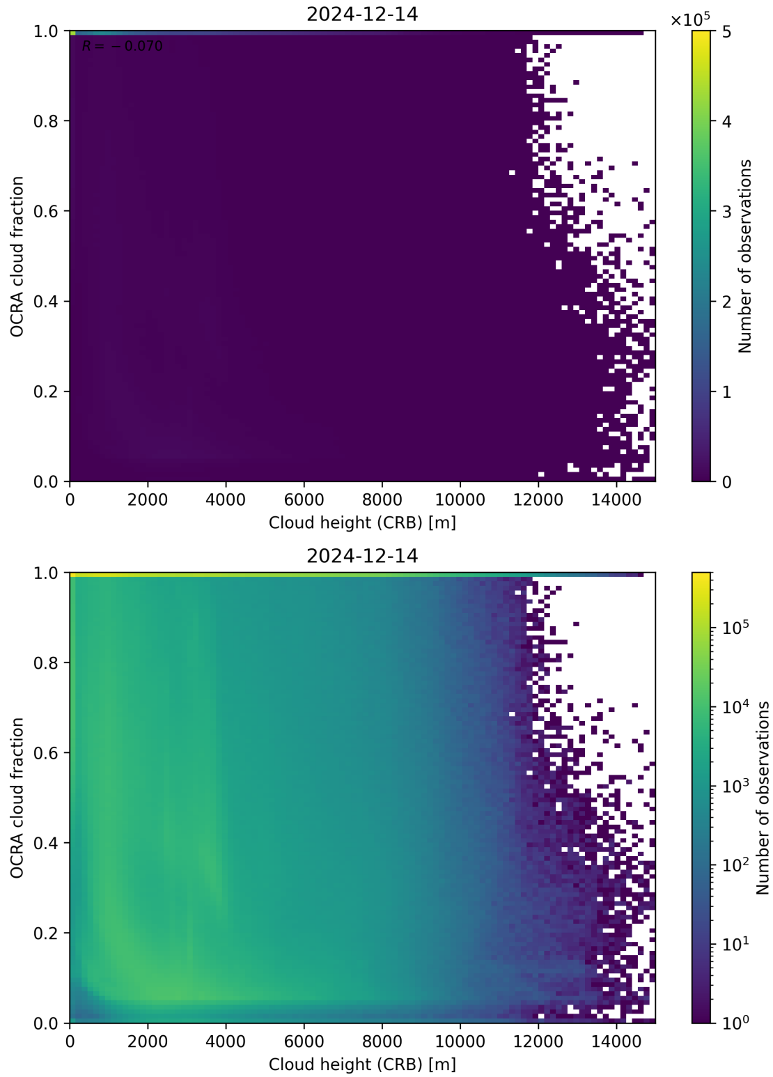
Figure 81: Scatter density plot of “Cloud height (CRB)” against “OCRA cloud fraction” for 2024-12-13 to 2024-12-15.
