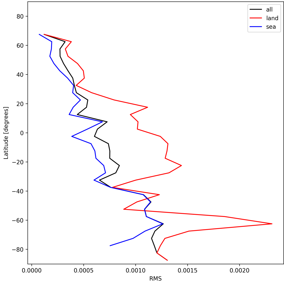
Figure 31: Zonal average of “RMS” for 2024-12-13 to 2024-12-15.
