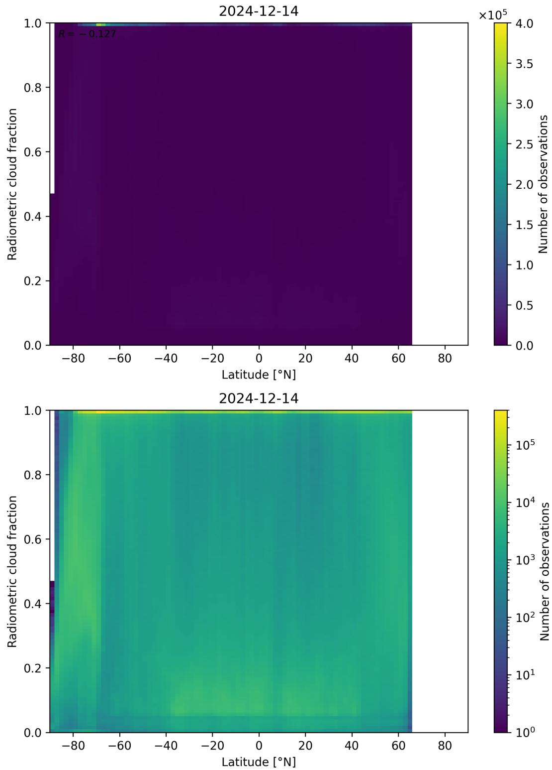
Figure 92: Scatter density plot of “Latitude” against “Radiometric cloud fraction” for 2024-12-13 to 2024-12-15.
