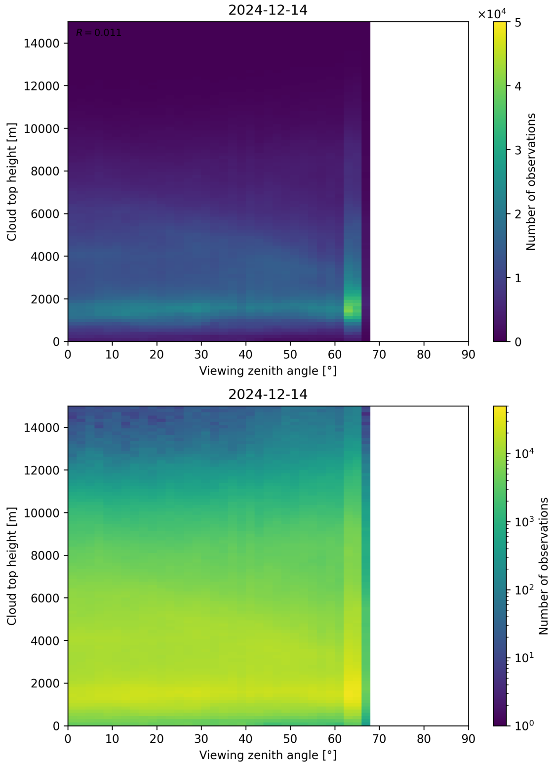
Figure 112: Scatter density plot of “Viewing zenith angle” against “Cloud top height” for 2024-12-13 to 2024-12-15.
