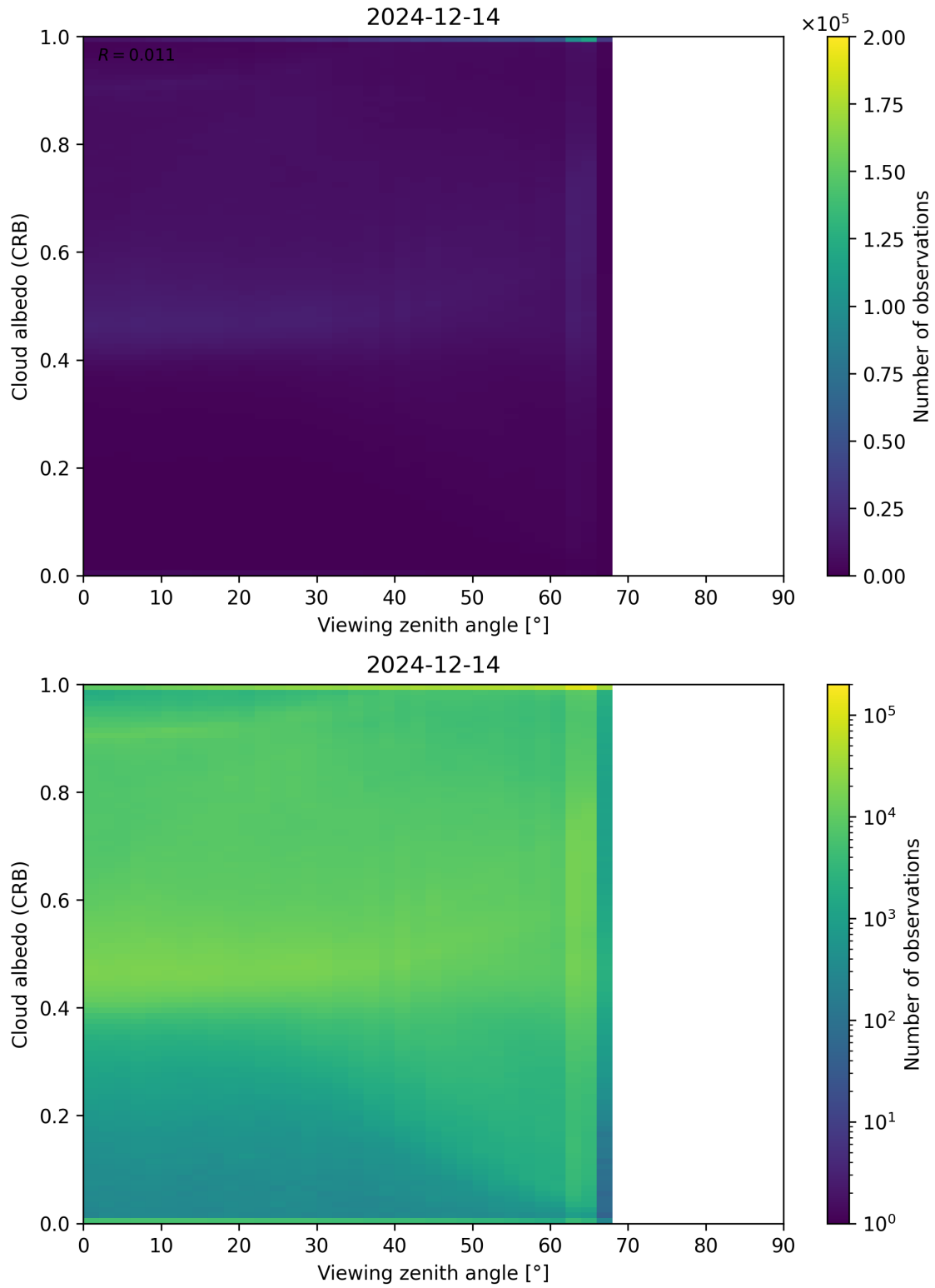
Figure 106: Scatter density plot of “Viewing zenith angle” against “Cloud albedo (CRB)” for 2024-12-13 to 2024-12-15.
