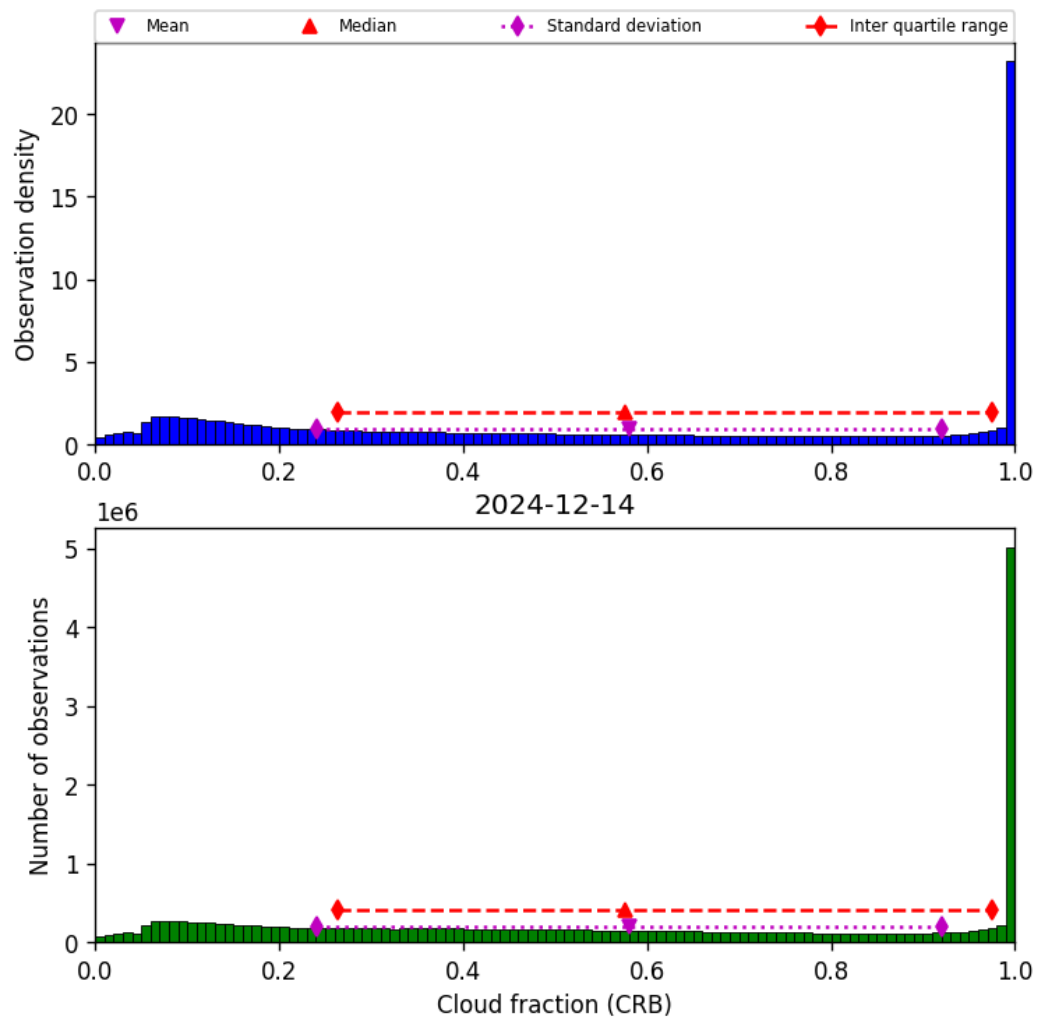
Figure 42: Histogram of “Cloud fraction (CRB)” for 2024-12-13 to 2024-12-15
