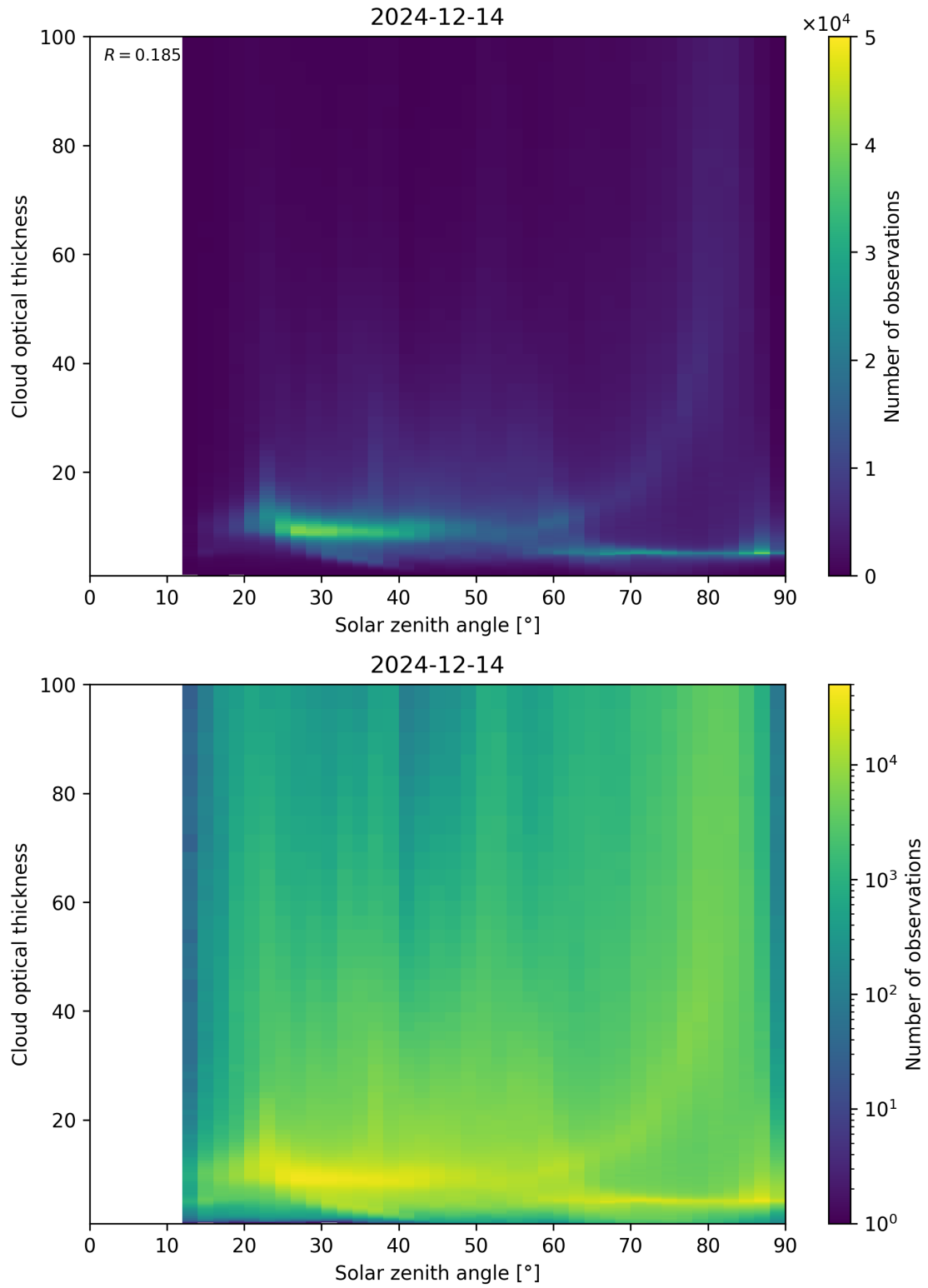
Figure 103: Scatter density plot of “Solar zenith angle” against “Cloud optical thickness” for 2024-12-13 to 2024-12-15.
