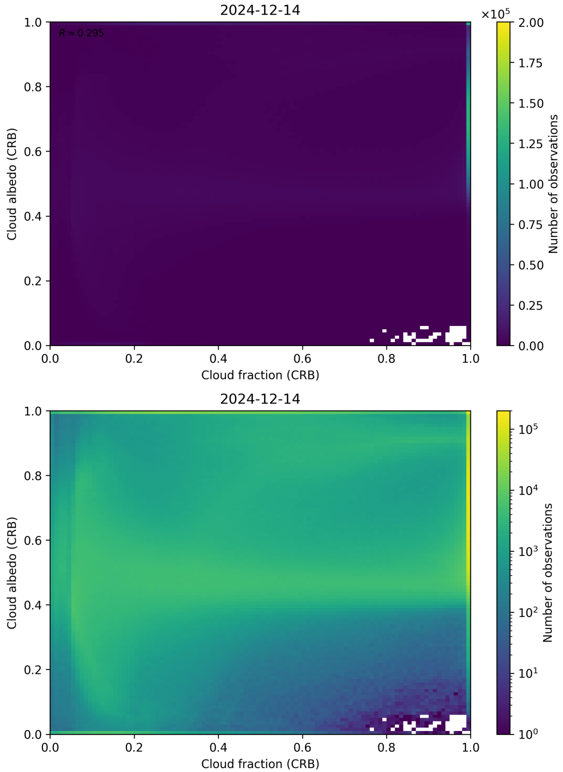
Figure 77: Scatter density plot of “Cloud fraction (CRB)” against “Cloud albedo (CRB)” for 2024-12-13 to 2024-12-15.
