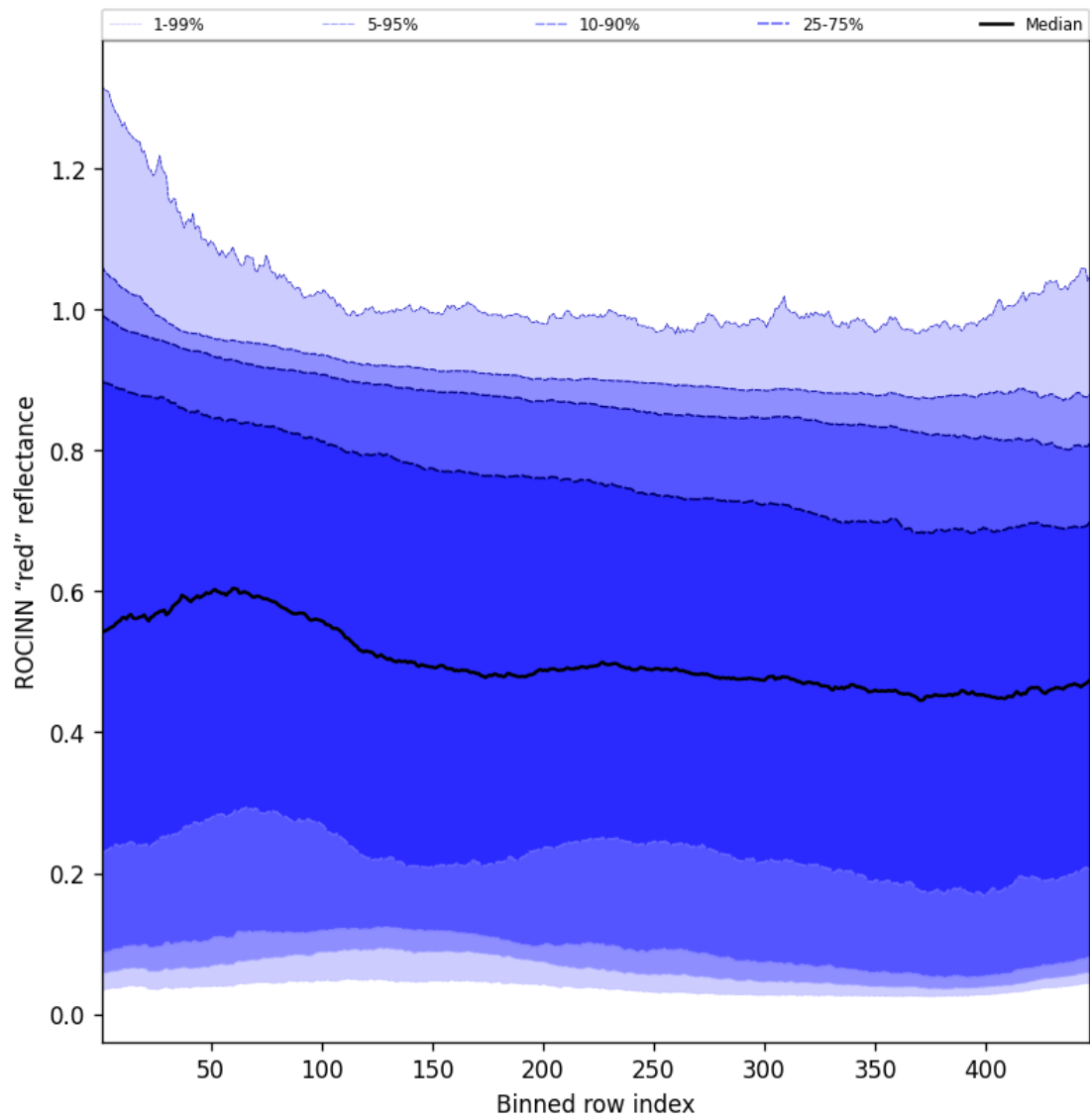
Figure 69: Along track statistics of "ROCINN "red" reflectance" for 2024-12-13 to 2024-12-15
