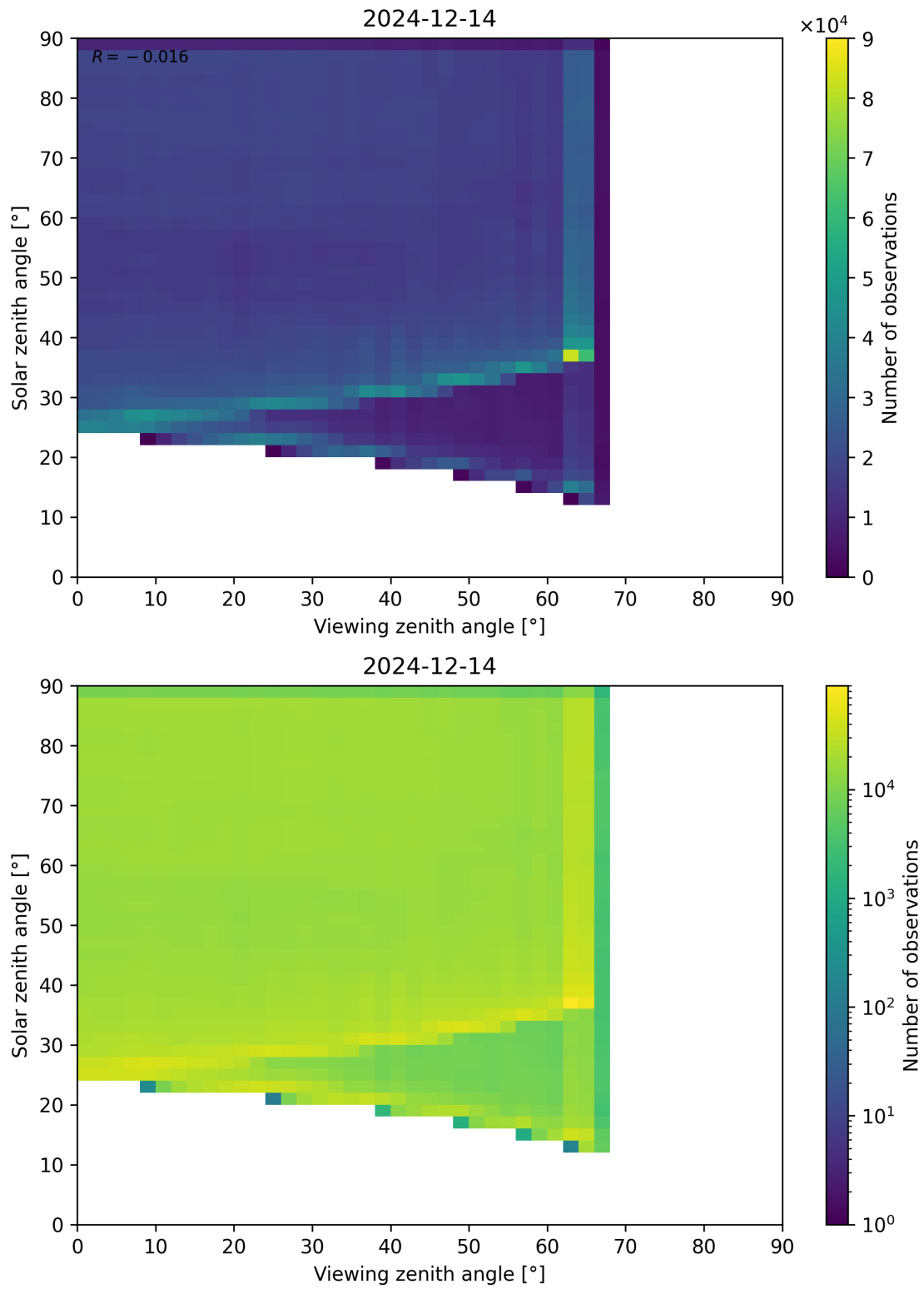
Figure 114: Scatter density plot of “Viewing zenith angle” against “Solar zenith angle” for 2024-12-13 to 2024-12-15.
