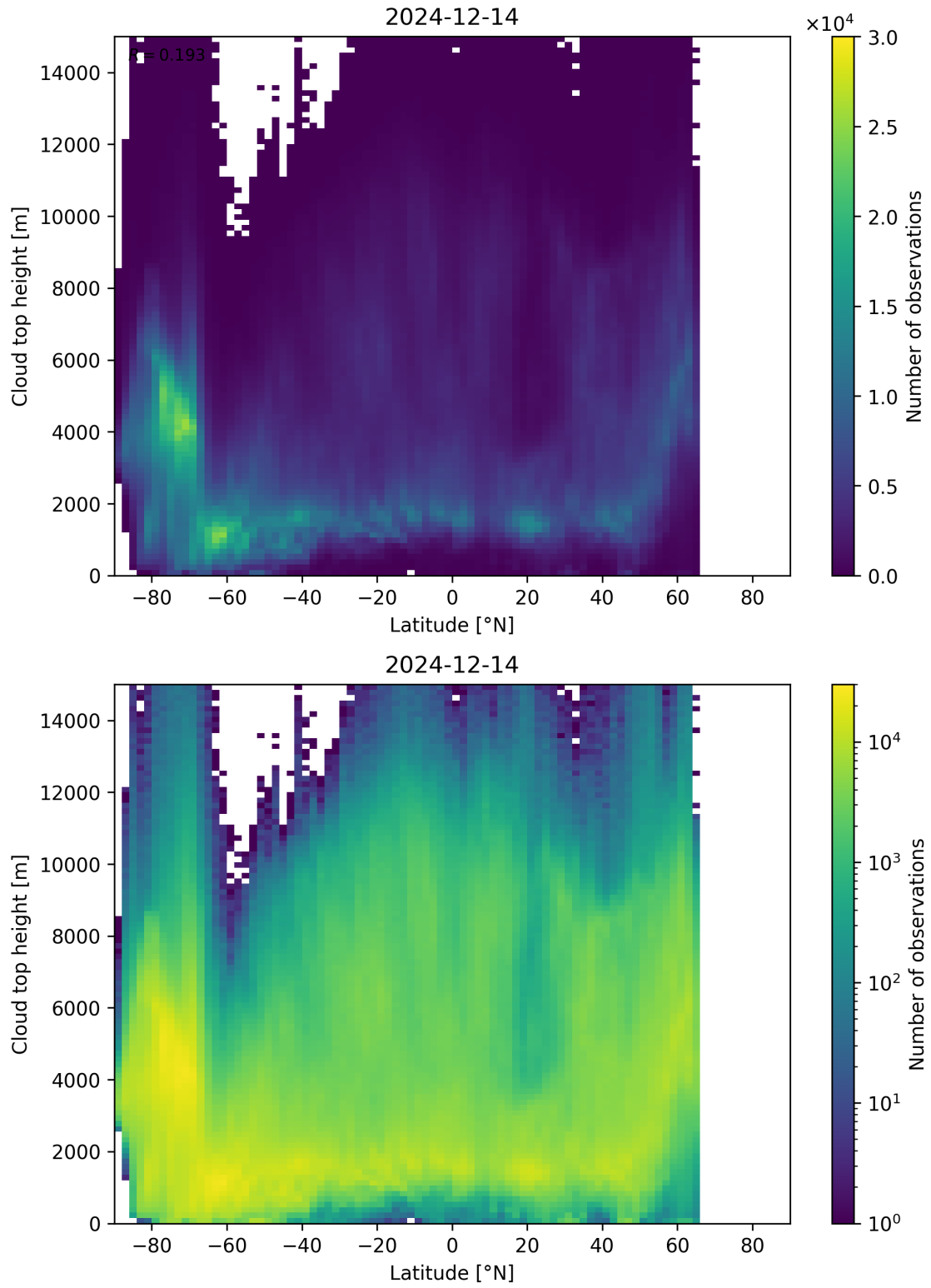
Figure 97: Scatter density plot of “Latitude” against “Cloud top height” for 2024-12-13 to 2024-12-15.
