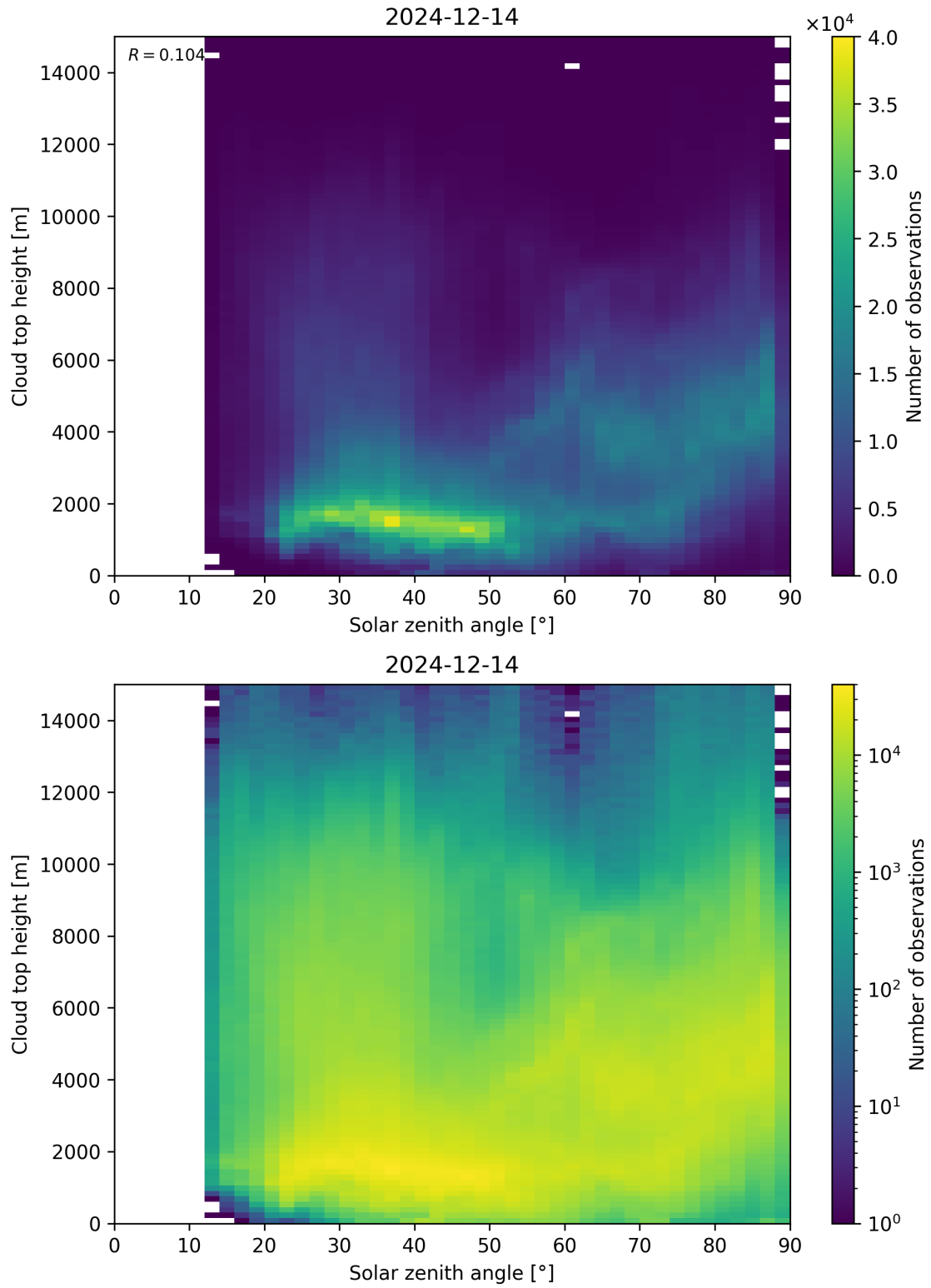
Figure 104: Scatter density plot of “Solar zenith angle” against “Cloud top height” for 2024-12-13 to 2024-12-15.
