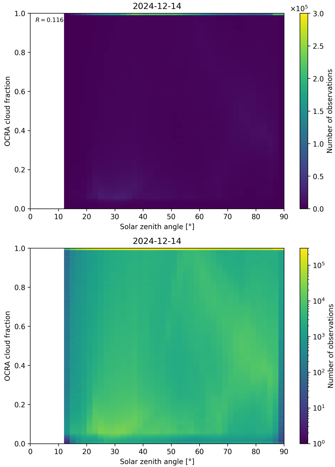
Figure 100: Scatter density plot of “Solar zenith angle” against “OCRA cloud fraction” for 2024-12-13 to 2024-12-15.
