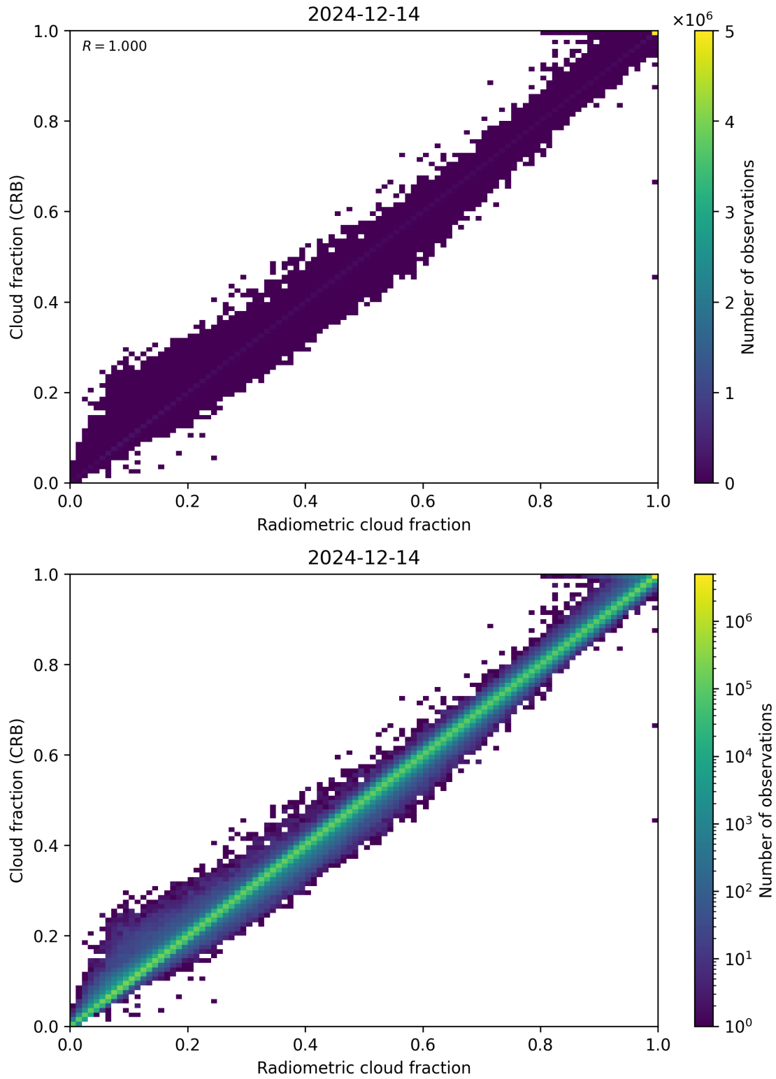
Figure 73: Scatter density plot of “Radiometric cloud fraction” against “Cloud fraction (CRB)” for 2024-12-13 to 2024-12-15.
