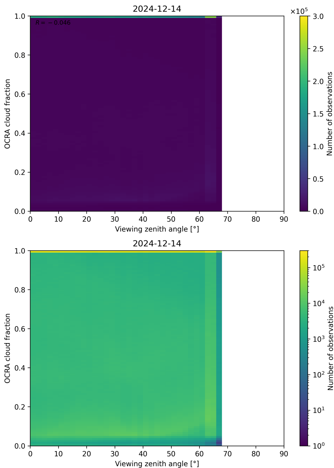
Figure 108: Scatter density plot of “Viewing zenith angle” against “OCRA cloud fraction” for 2024-12-13 to 2024-12-15.
