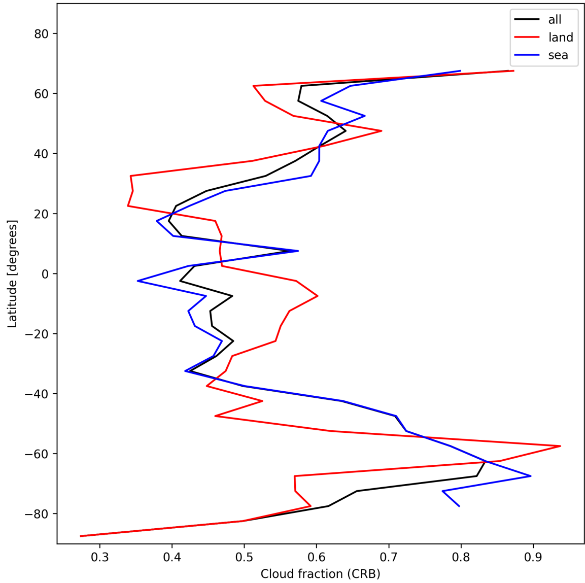
Figure 26: Zonal average of “Cloud fraction (CRB)” for 2024-12-13 to 2024-12-15.
