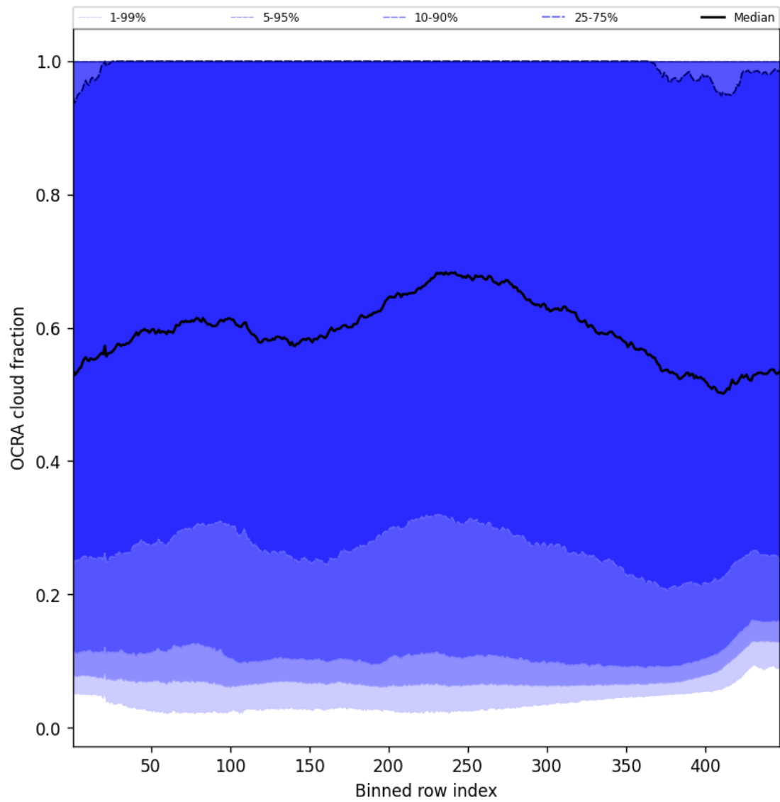
Figure 66: Along track statistics of “OCRA cloud fraction” for 2024-12-13 to 2024-12-15
