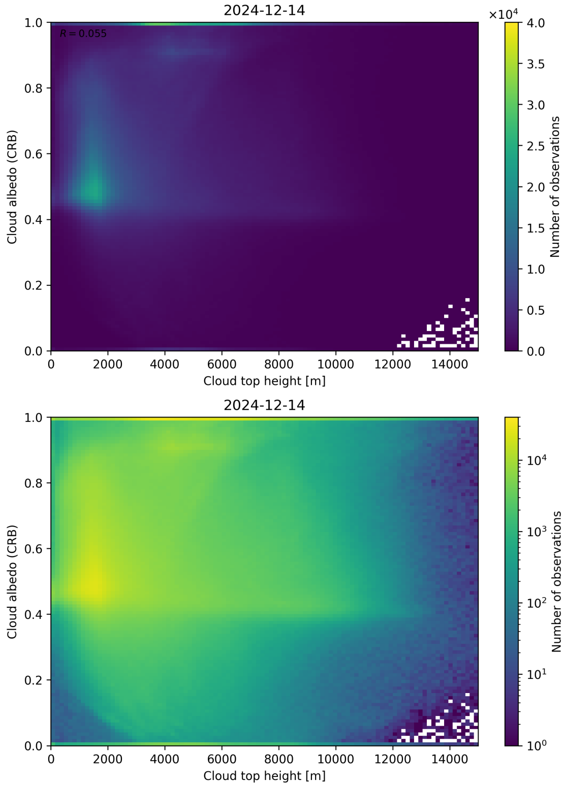
Figure 86: Scatter density plot of “Cloud top height” against “Cloud albedo (CRB)” for 2024-12-13 to 2024-12-15.
