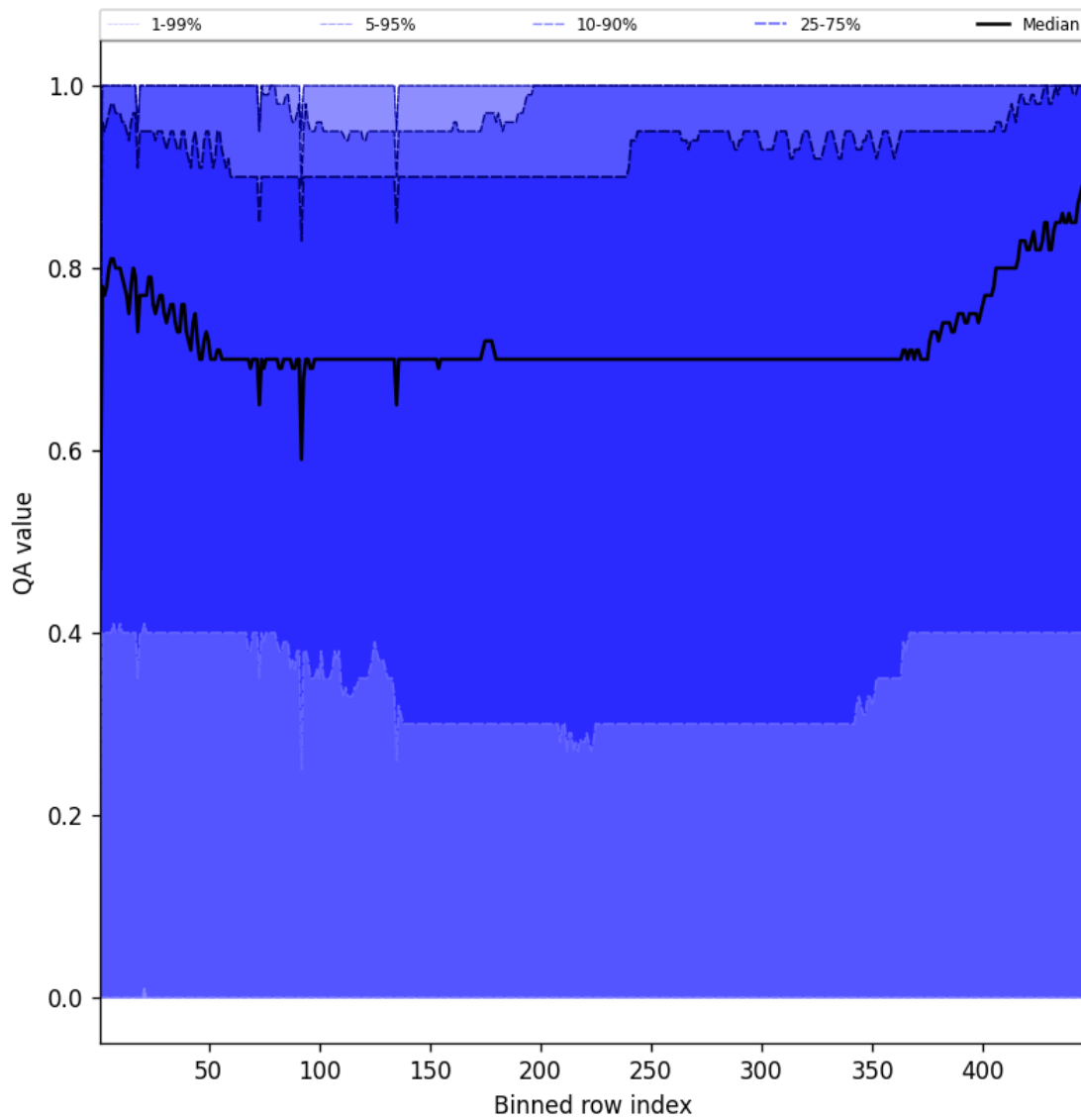
Figure 54: Along track statistics of “QA value” for 2024-12-13 to 2024-12-15
