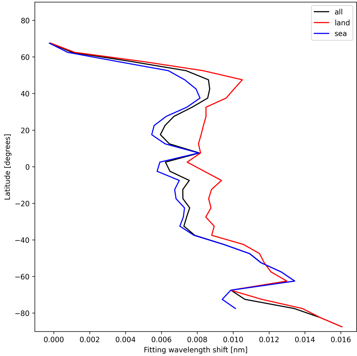
Figure 33: Zonal average of “Fitting wavelength shift” for 2024-12-13 to 2024-12-15.
