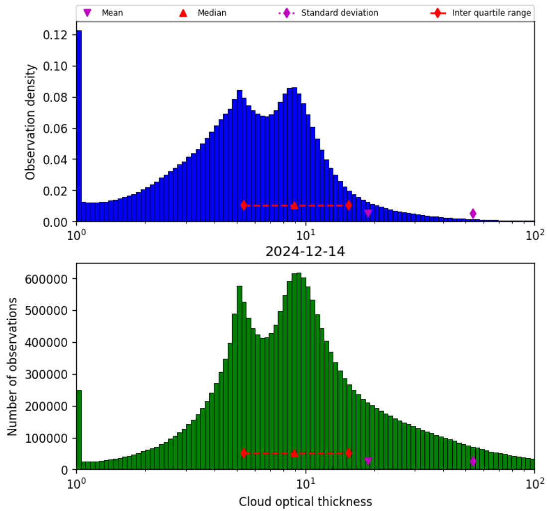
Figure 41: Histogram of “Cloud optical thickness” for 2024-12-13 to 2024-12-15
