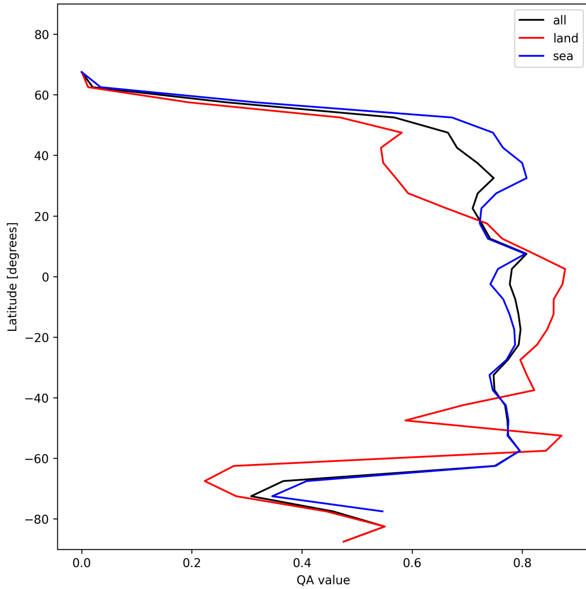
Figure 22: Zonal average of “QA value” for 2024-12-13 to 2024-12-15.
