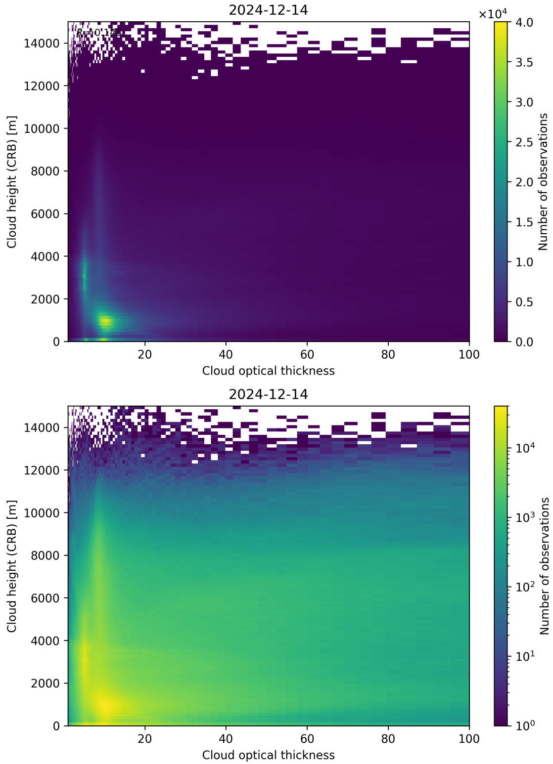
Figure 85: Scatter density plot of “Cloud optical thickness” against “Cloud height (CRB)” for 2024-12-13 to 2024-12-15.
