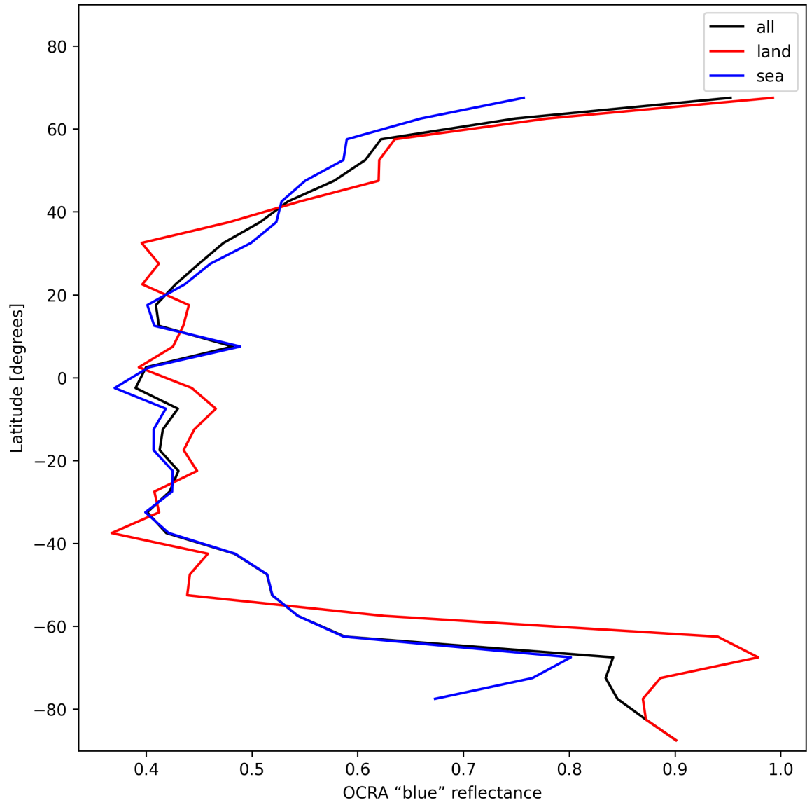
Figure 35: Zonal average of “OCRA “blue” reflectance” for 2024-12-13 to 2024-12-15.
