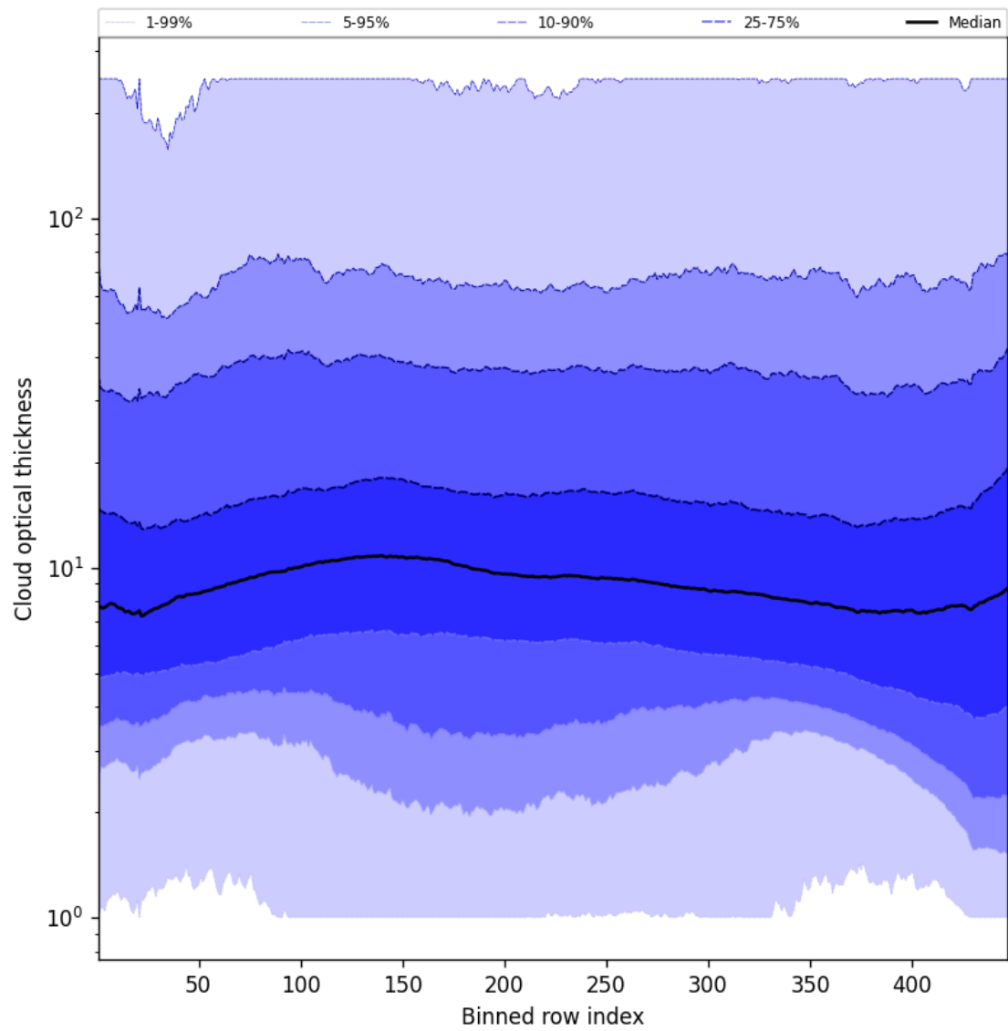
Figure 57: Along track statistics of “Cloud optical thickness” for 2024-12-13 to 2024-12-15
