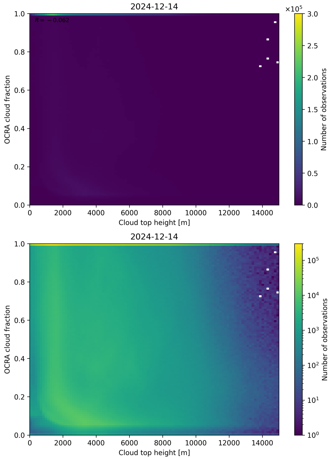
Figure 87: Scatter density plot of “Cloud top height” against “OCRA cloud fraction” for 2024-12-13 to 2024-12-15.
