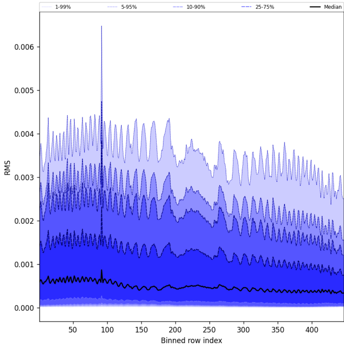
Figure 63: Along track statistics of “RMS” for 2024-12-13 to 2024-12-15
