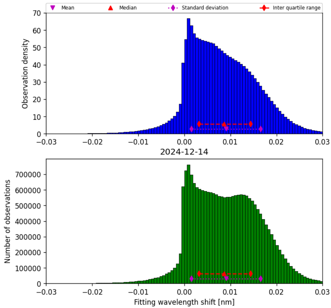
Figure 49: Histogram of “Fitting wavelength shift” for 2024-12-13 to 2024-12-15
