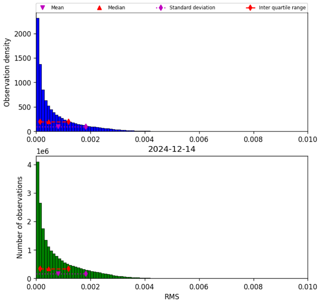
Figure 47: Histogram of “RMS” for 2024-12-13 to 2024-12-15
