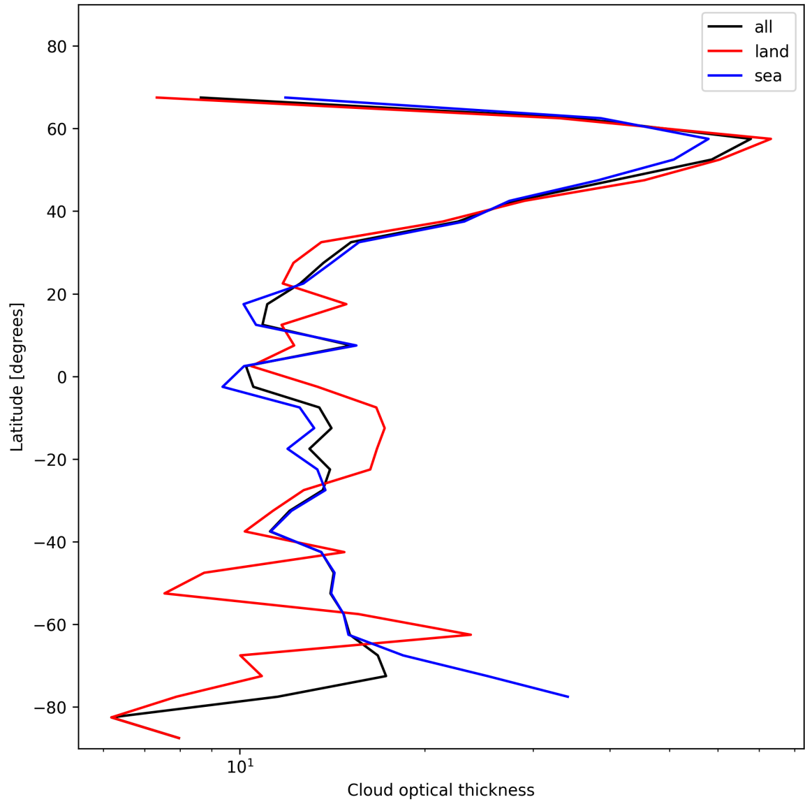
Figure 25: Zonal average of “Cloud optical thickness” for 2024-12-13 to 2024-12-15.
