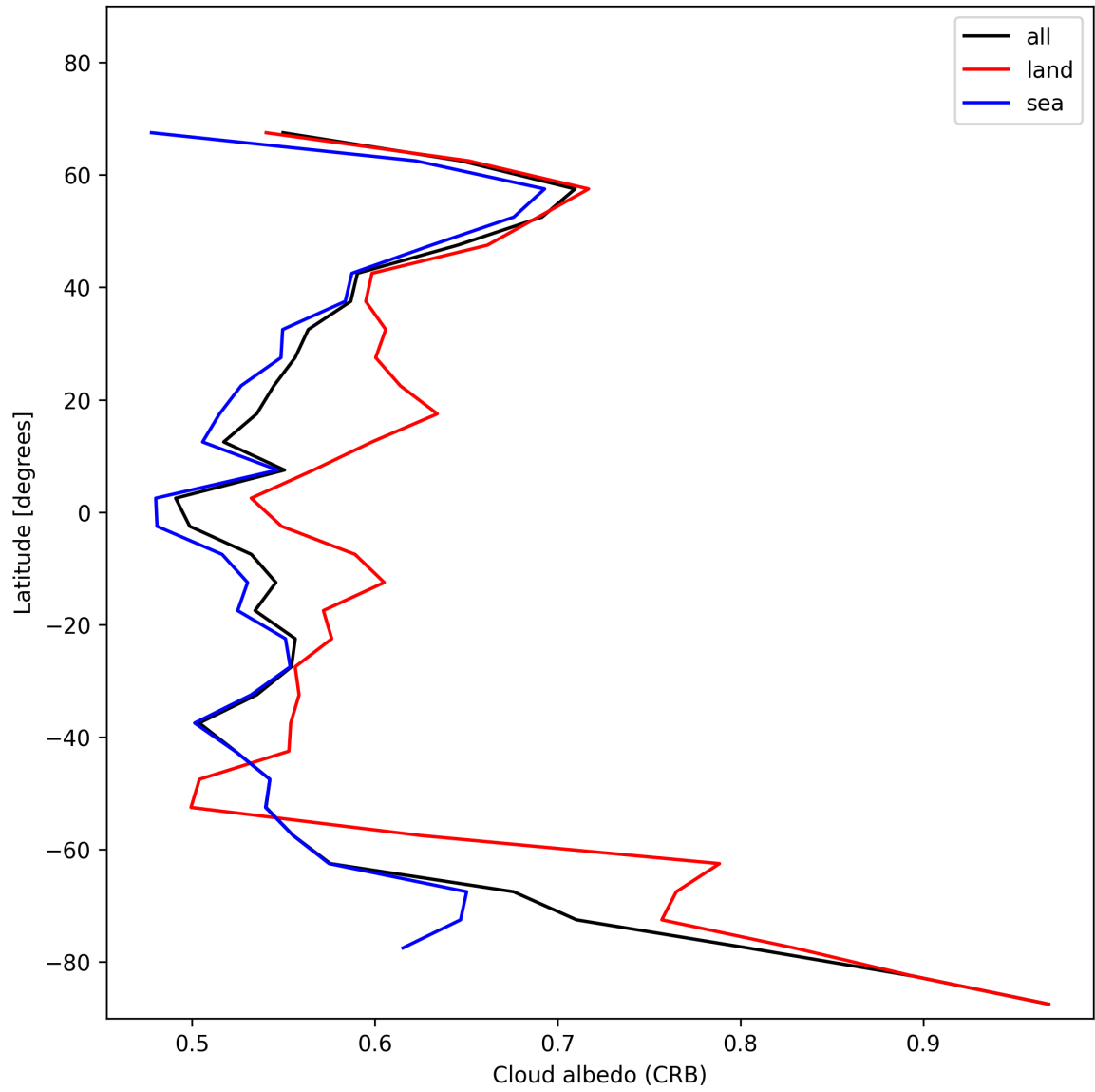
Figure 28: Zonal average of “Cloud albedo (CRB)” for 2024-12-13 to 2024-12-15.
