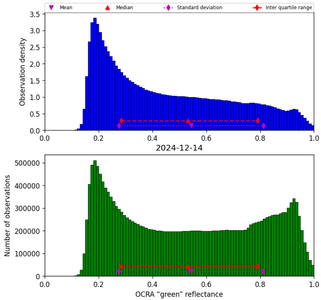
Figure 52: Histogram of “OCRA “green” reflectance” for 2024-12-13 to 2024-12-15
