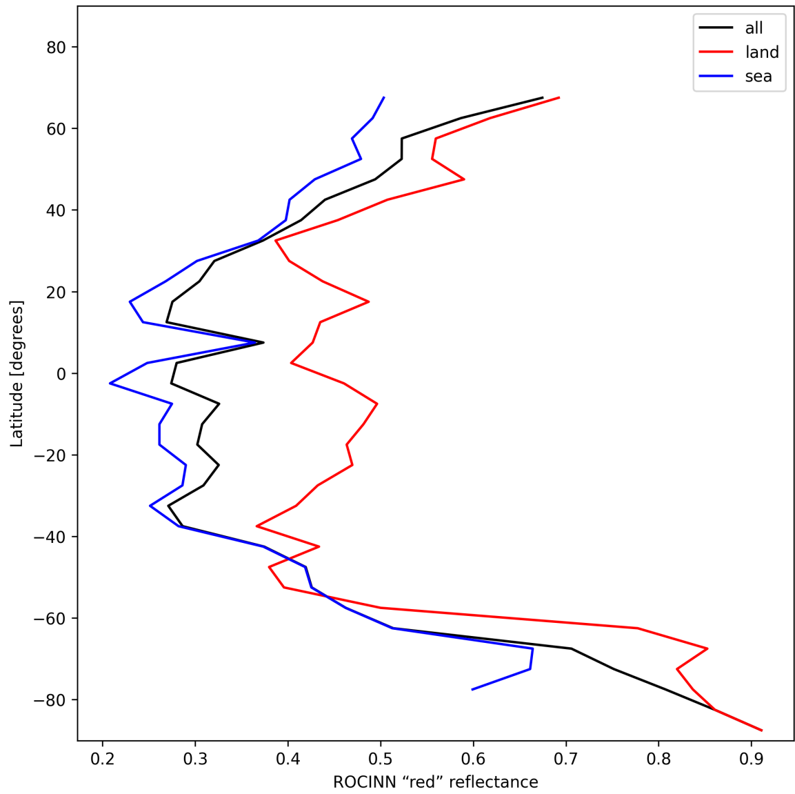
Figure 37: Zonal average of "ROCINN "red" reflectance" for 2024-12-13 to 2024-12-15.
