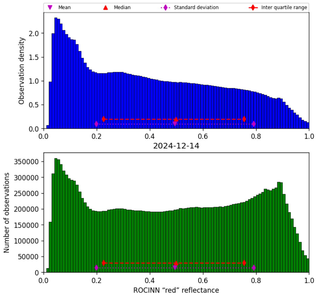
Figure 53: Histogram of “ROCINN “red” reflectance” for 2024-12-13 to 2024-12-15
