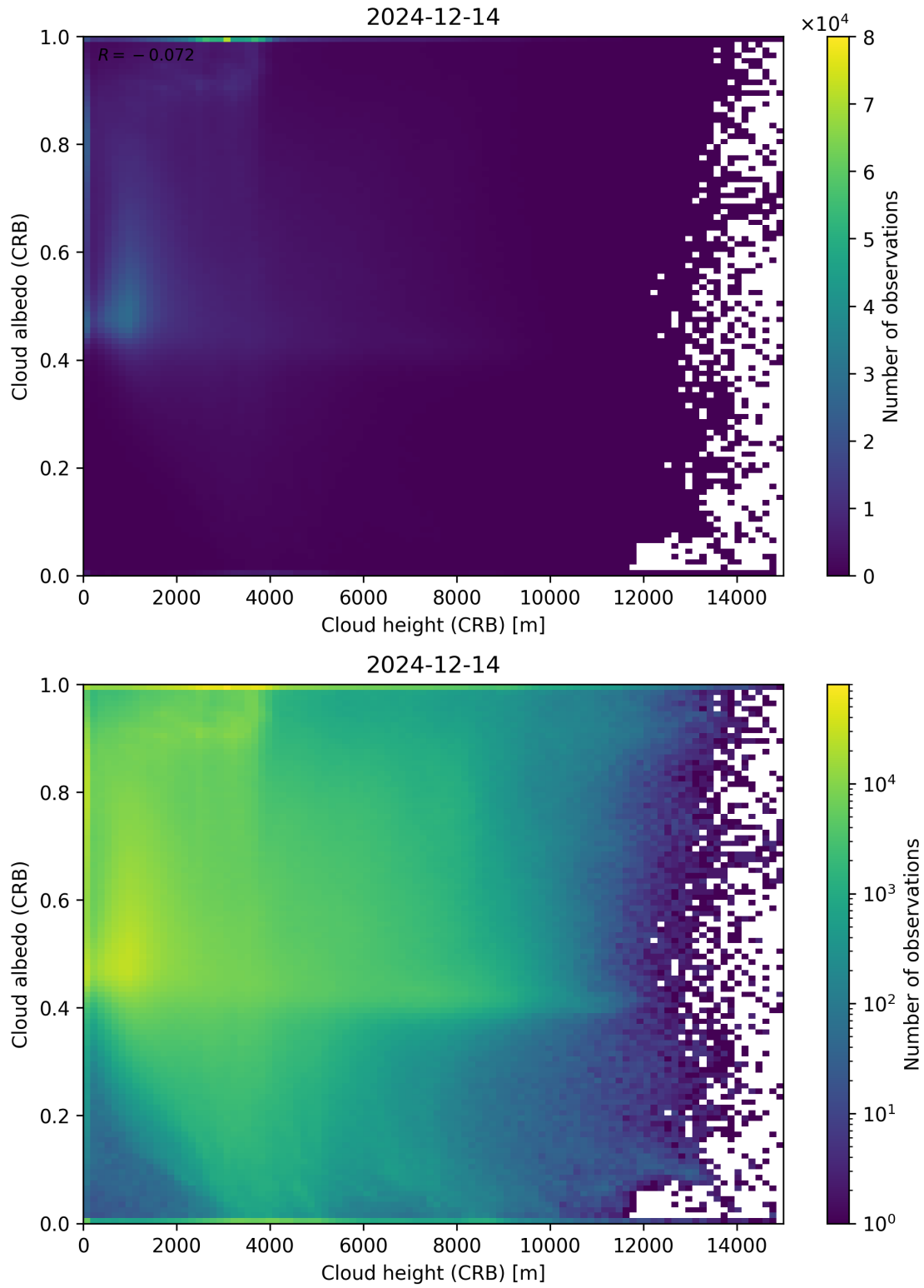
Figure 80: Scatter density plot of “Cloud height (CRB)” against “Cloud albedo (CRB)” for 2024-12-13 to 2024-12-15.
