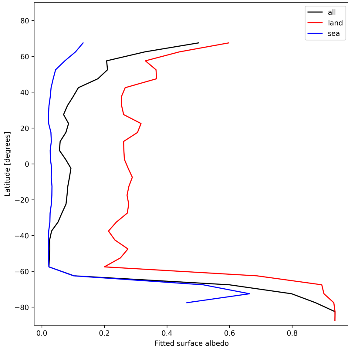
Figure 29: Zonal average of “Fitted surface albedo” for 2024-12-13 to 2024-12-15.
