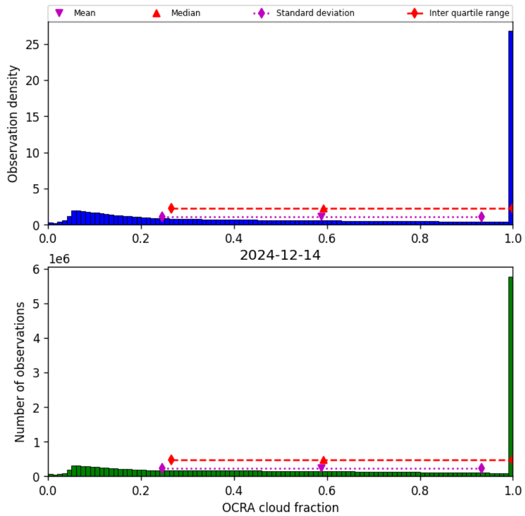
Figure 50: Histogram of “OCRA cloud fraction” for 2024-12-13 to 2024-12-15
