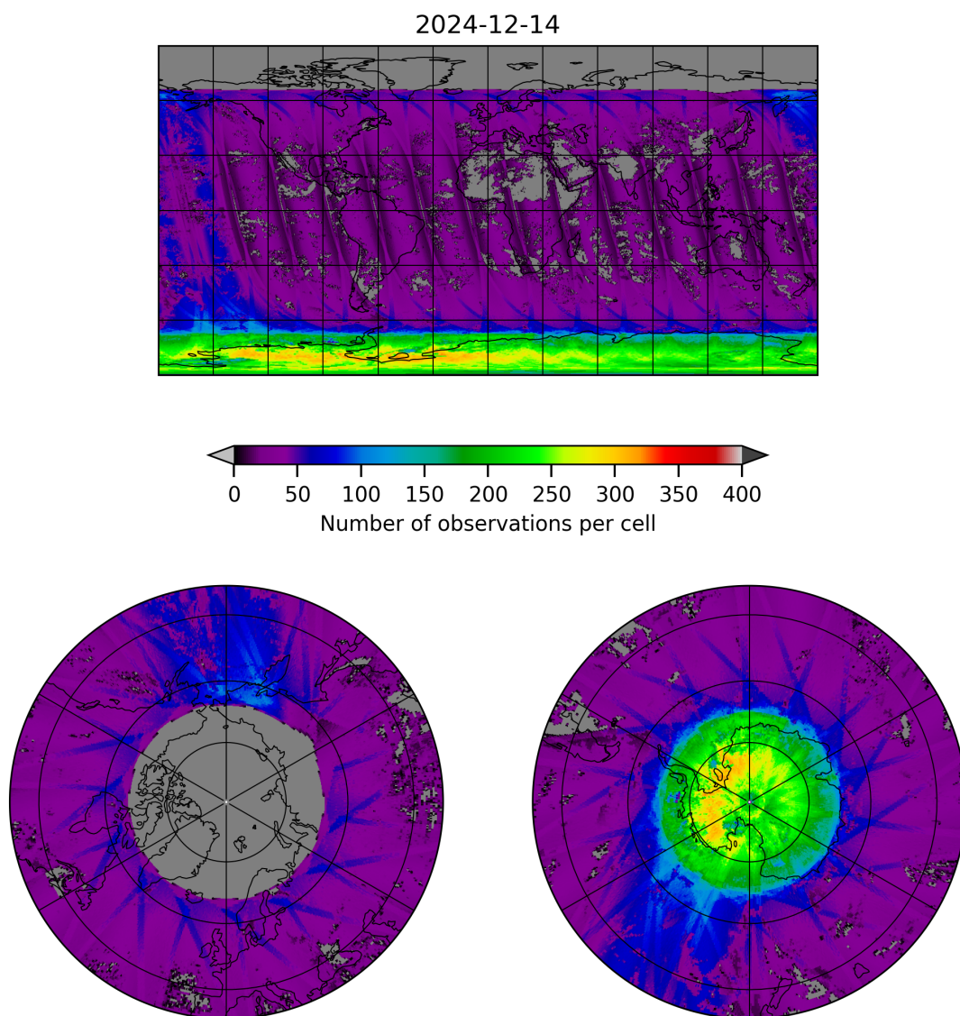
Figure 21: Map of the number of observations for 2024-12-13 to 2024-12-15
