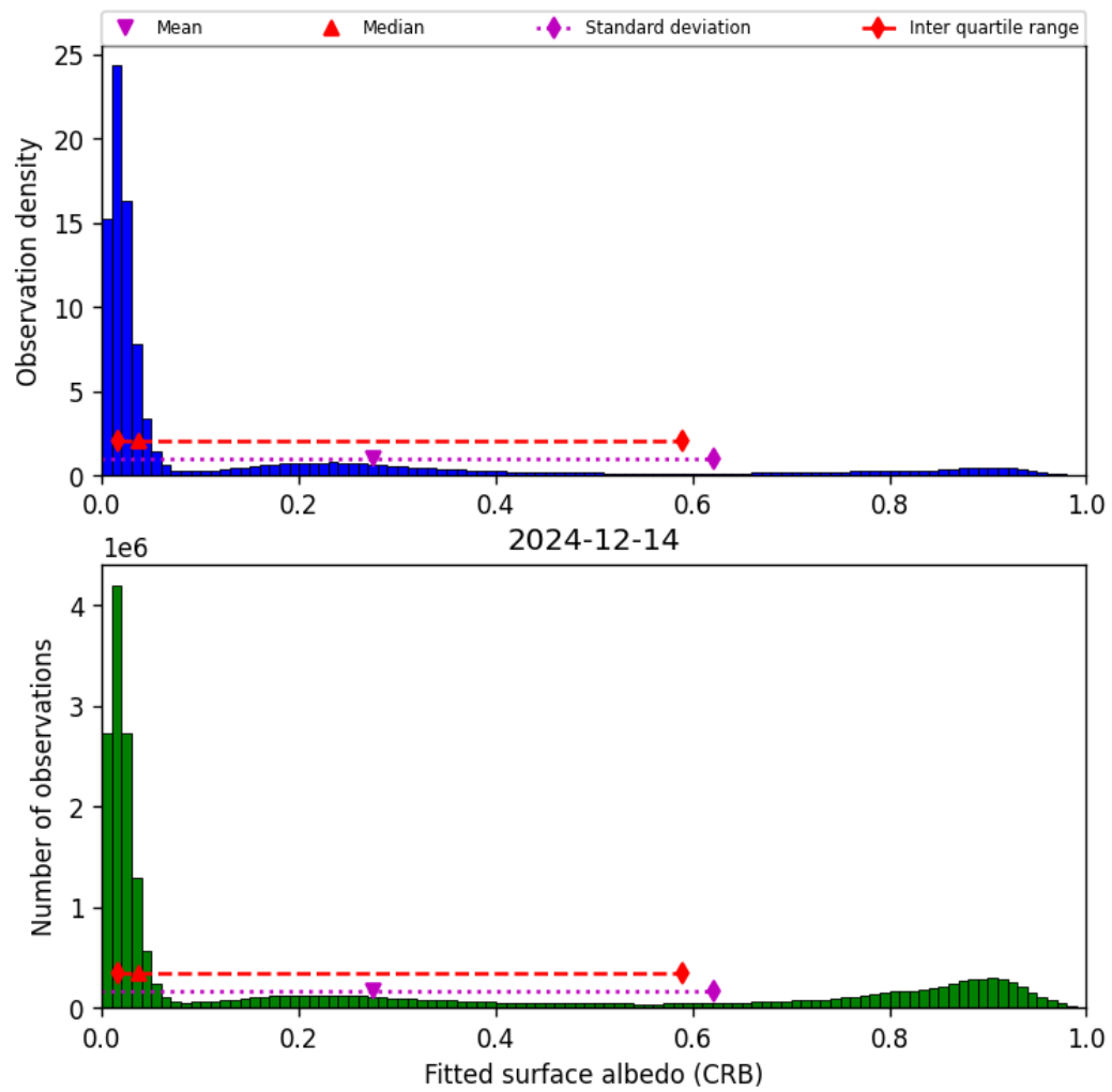
Figure 46: Histogram of “Fitted surface albedo (CRB)” for 2024-12-13 to 2024-12-15
