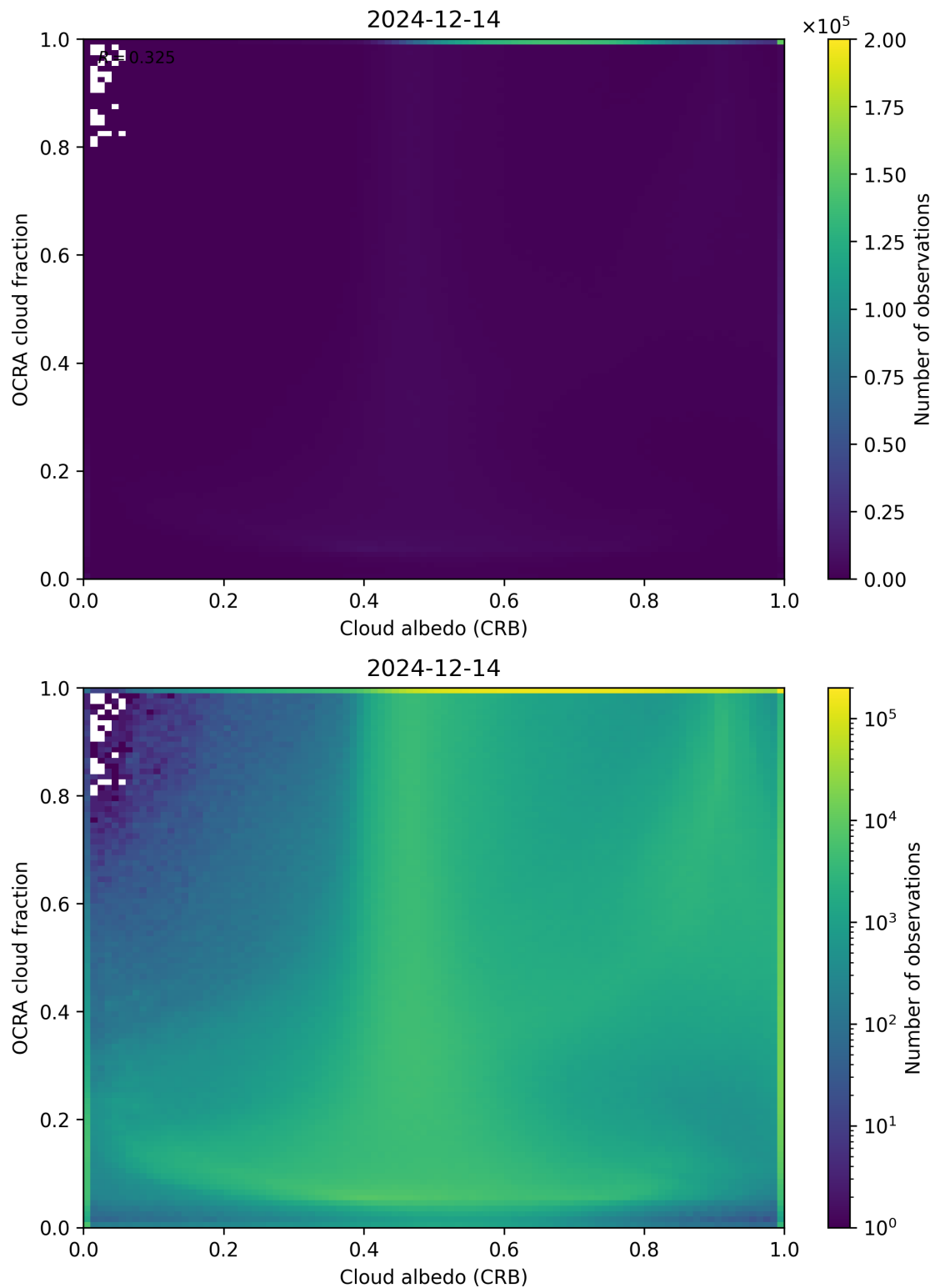
Figure 70: Scatter density plot of “Cloud albedo (CRB)” against “OCRA cloud fraction” for 2024-12-13 to 2024-12-15.
