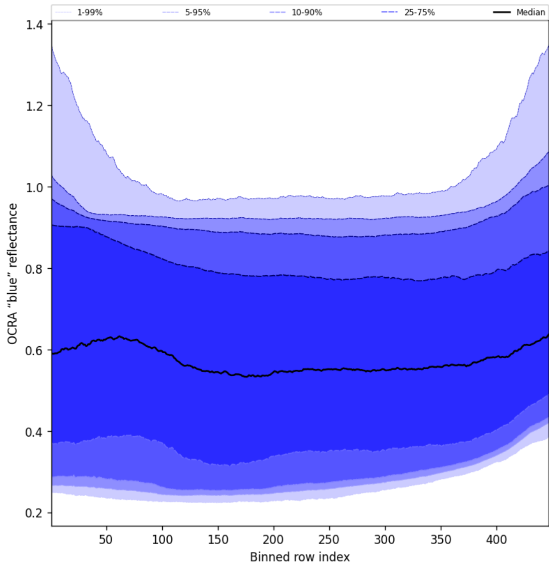
Figure 67: Along track statistics of “OCRA “blue” reflectance” for 2024-12-13 to 2024-12-15
