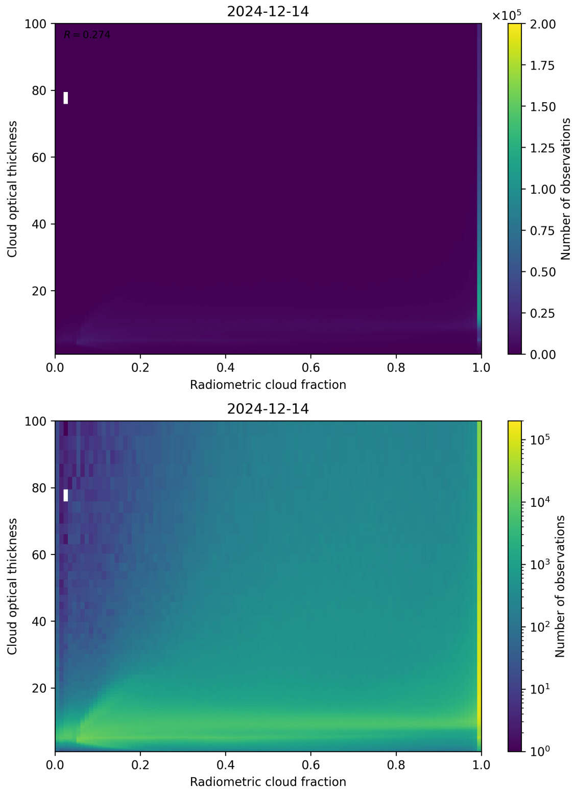
Figure 75: Scatter density plot of “Radiometric cloud fraction” against “Cloud optical thickness” for 2024-12-13 to 2024-12-15.
