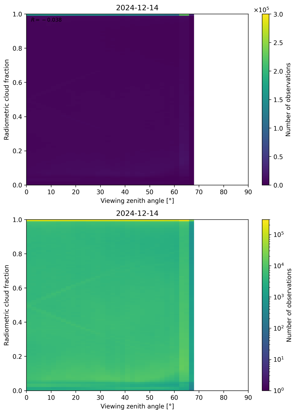
Figure 107: Scatter density plot of “Viewing zenith angle” against “Radiometric cloud fraction” for 2024-12-13 to 2024-12-15.
