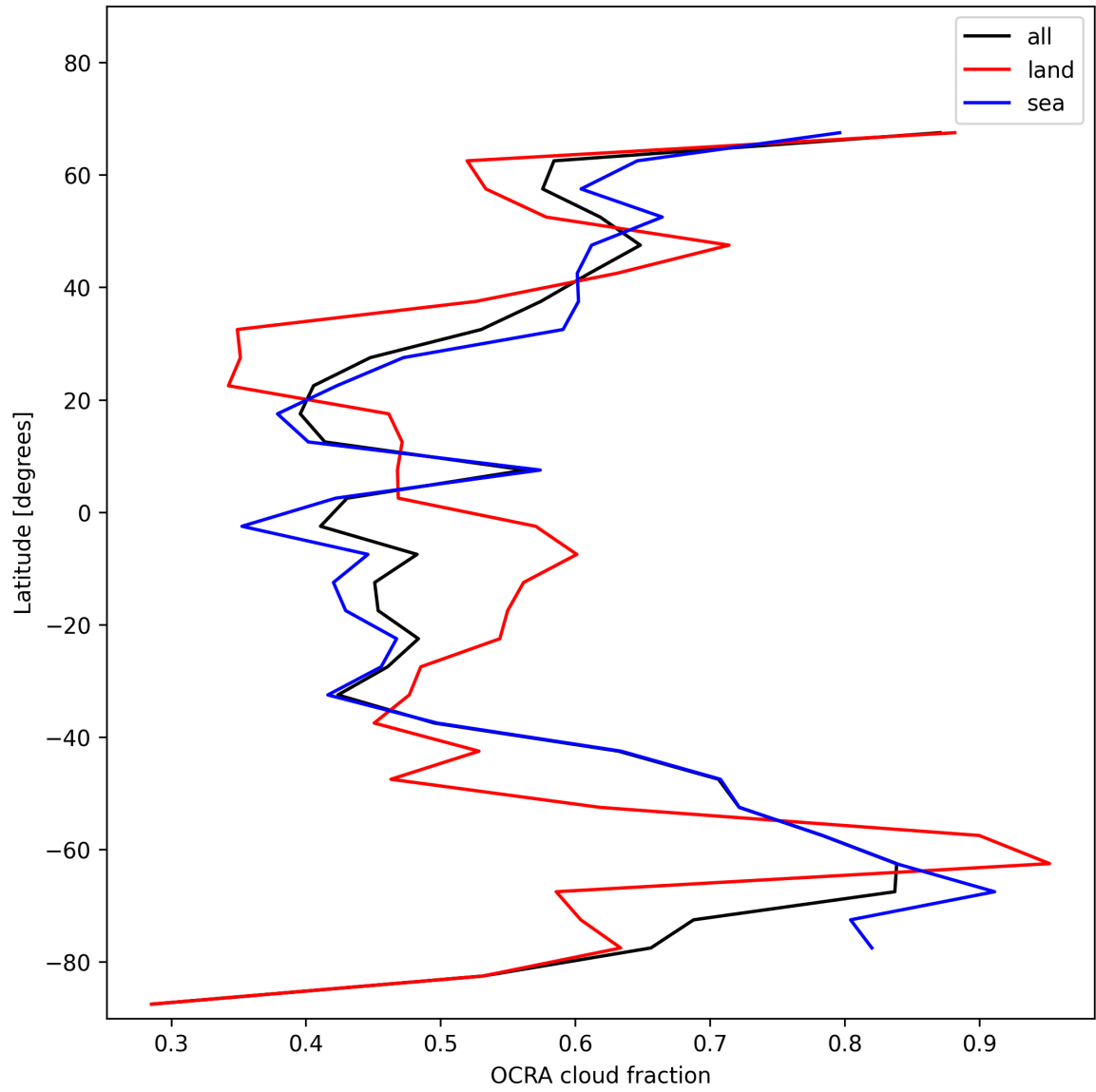
Figure 34: Zonal average of “OCRA cloud fraction” for 2024-12-13 to 2024-12-15.
