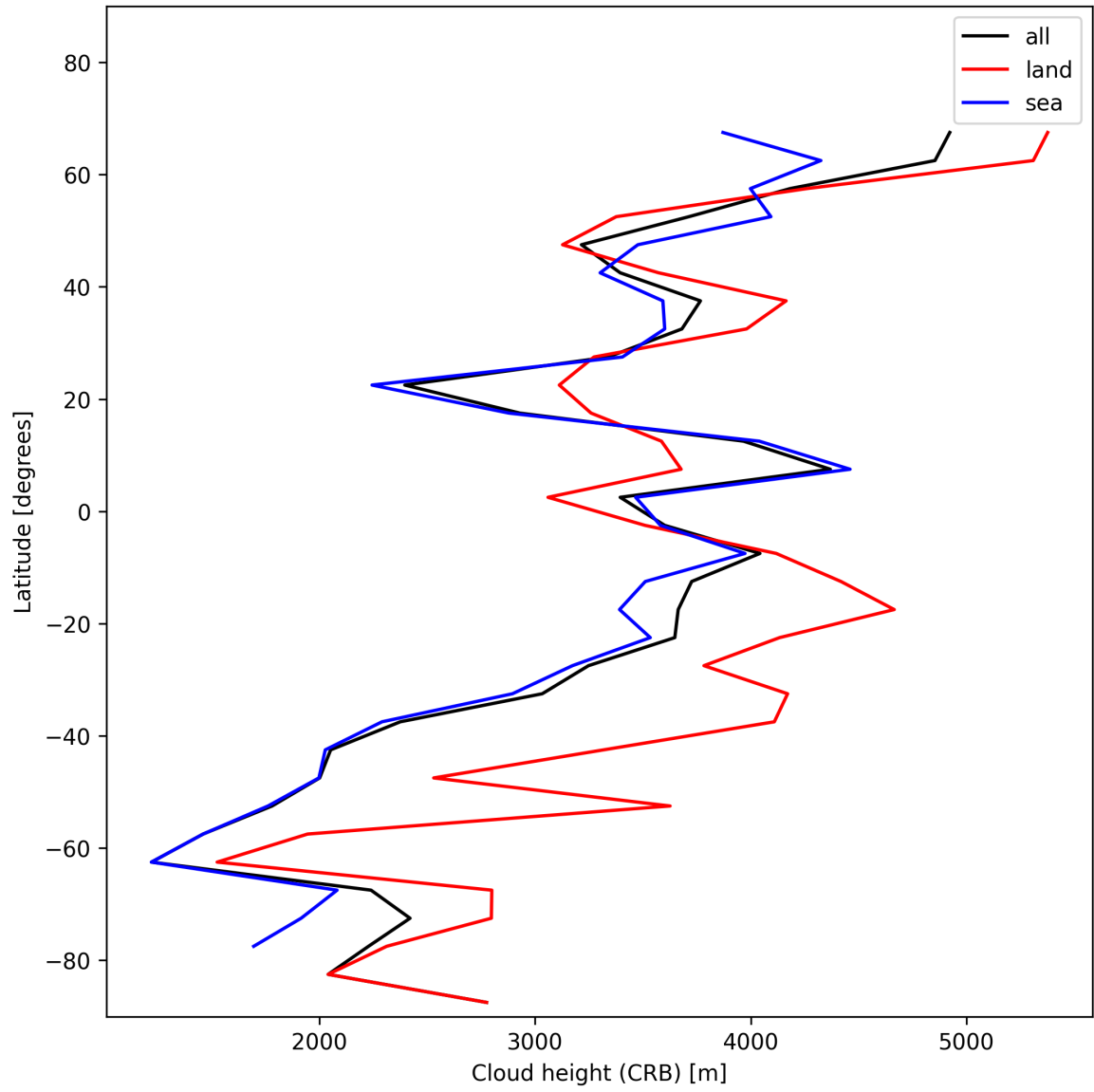
Figure 27: Zonal average of “Cloud height (CRB)” for 2024-12-13 to 2024-12-15.
