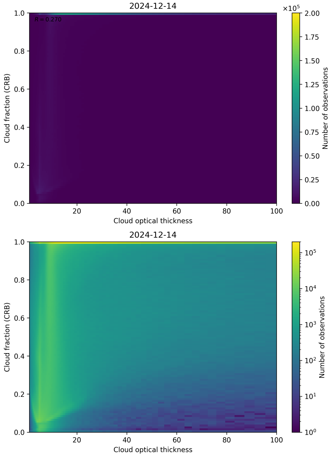
Figure 84: Scatter density plot of “Cloud optical thickness” against “Cloud fraction (CRB)” for 2024-12-13 to 2024-12-15.
