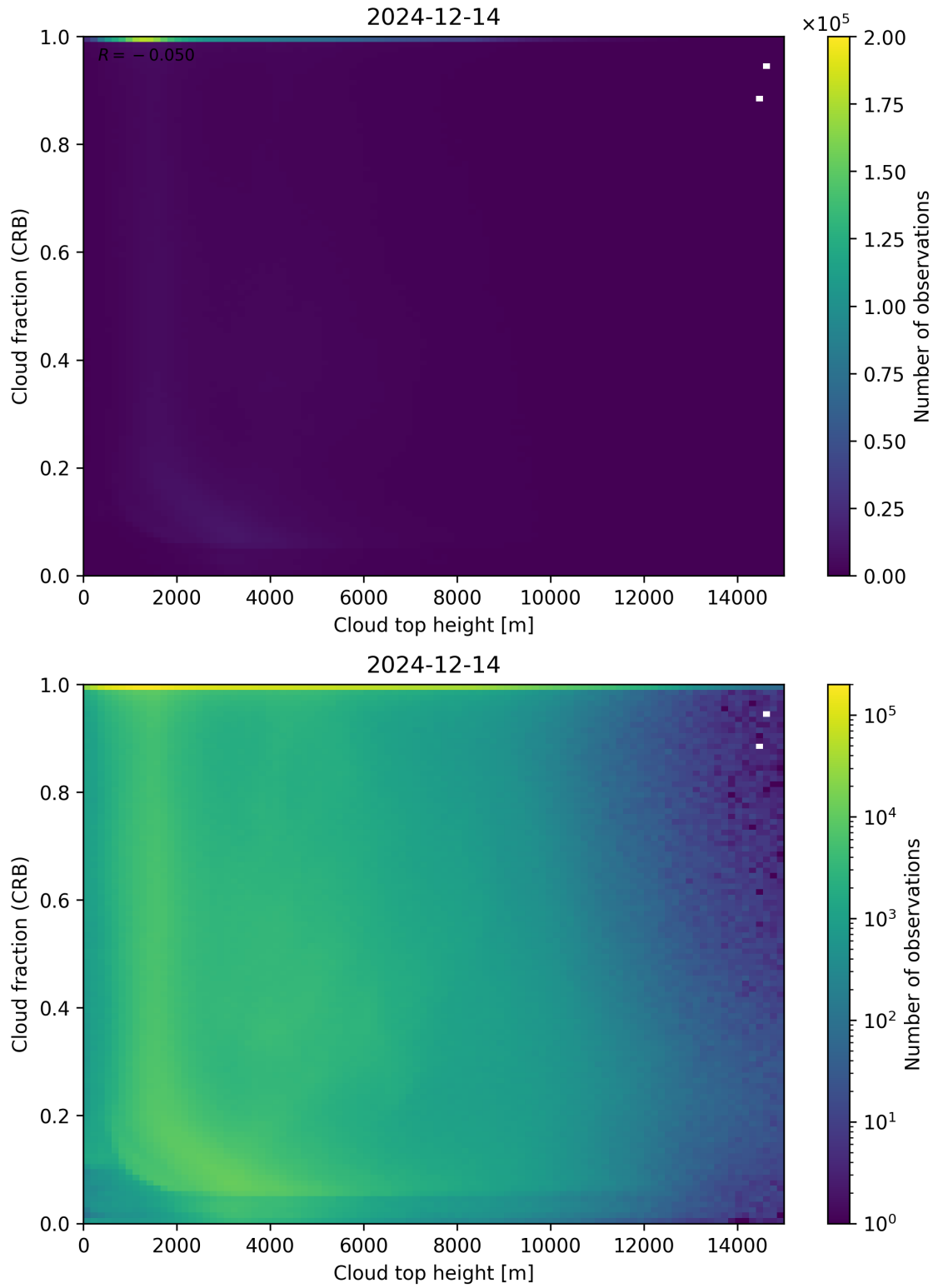
Figure 88: Scatter density plot of “Cloud top height” against “Cloud fraction (CRB)” for 2024-12-13 to 2024-12-15.
