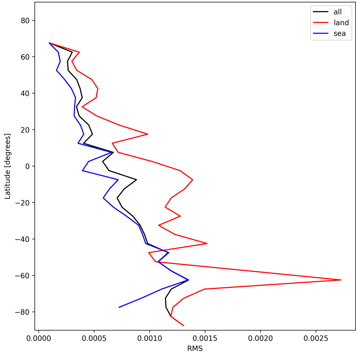
Figure 31: Zonal average of “RMS” for 2024-12-16 to 2024-12-17.
