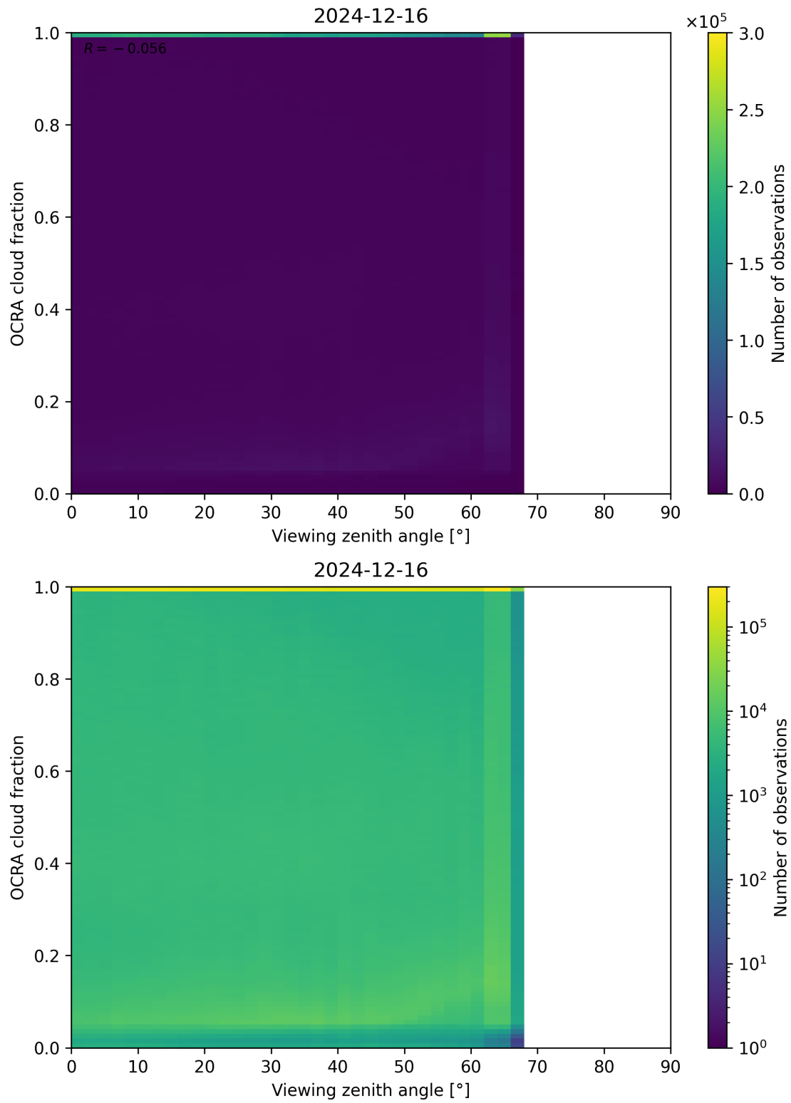
Figure 108: Scatter density plot of “Viewing zenith angle” against “OCRA cloud fraction” for 2024-12-16 to 2024-12-17.
