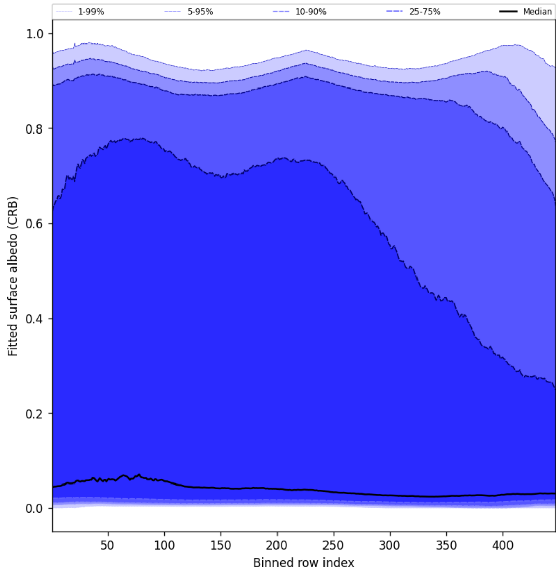
Figure 62: Along track statistics of “Fitted surface albedo (CRB)” for 2024-12-16 to 2024-12-17
