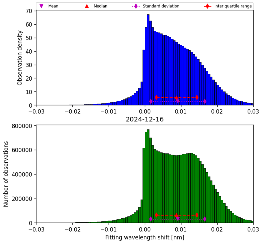
Figure 49: Histogram of “Fitting wavelength shift” for 2024-12-16 to 2024-12-17
