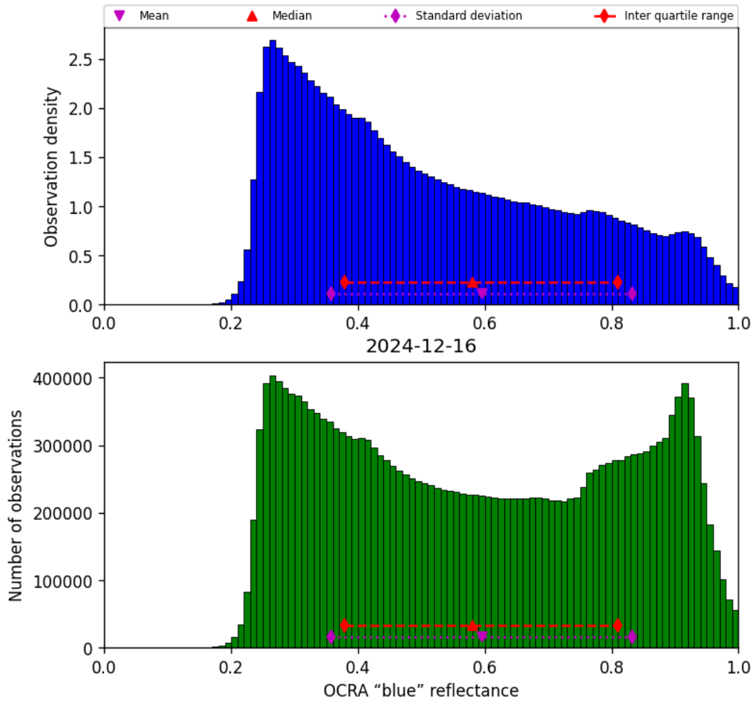
Figure 51: Histogram of “OCRA “blue” reflectance” for 2024-12-16 to 2024-12-17
