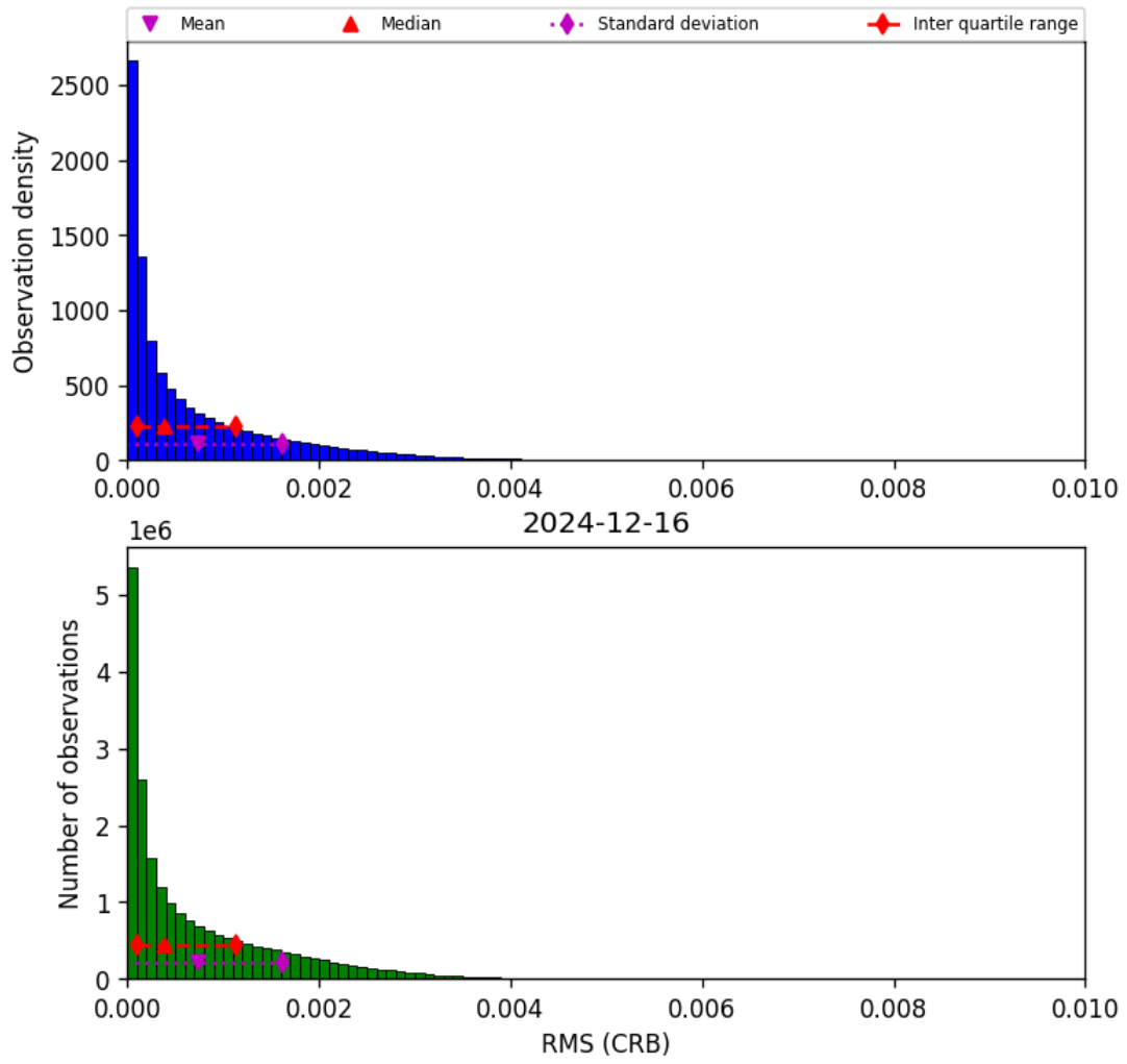
Figure 48: Histogram of “RMS (CRB)” for 2024-12-16 to 2024-12-17
