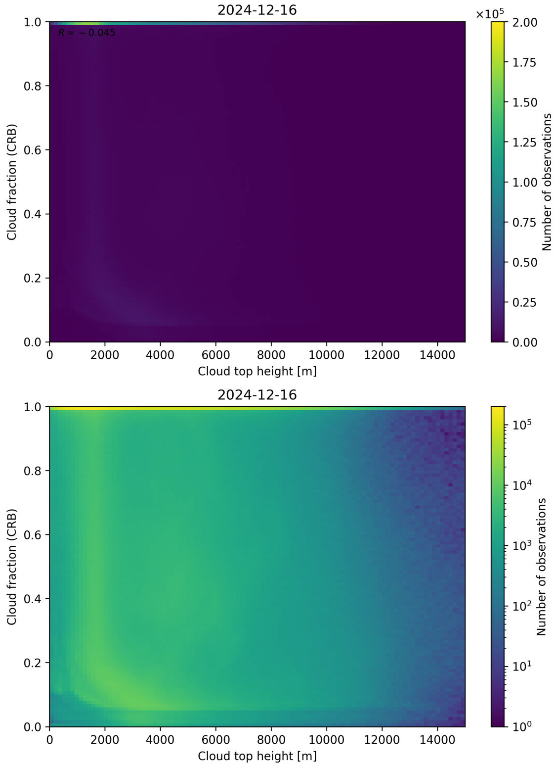
Figure 88: Scatter density plot of “Cloud top height” against “Cloud fraction (CRB)” for 2024-12-16 to 2024-12-17.
