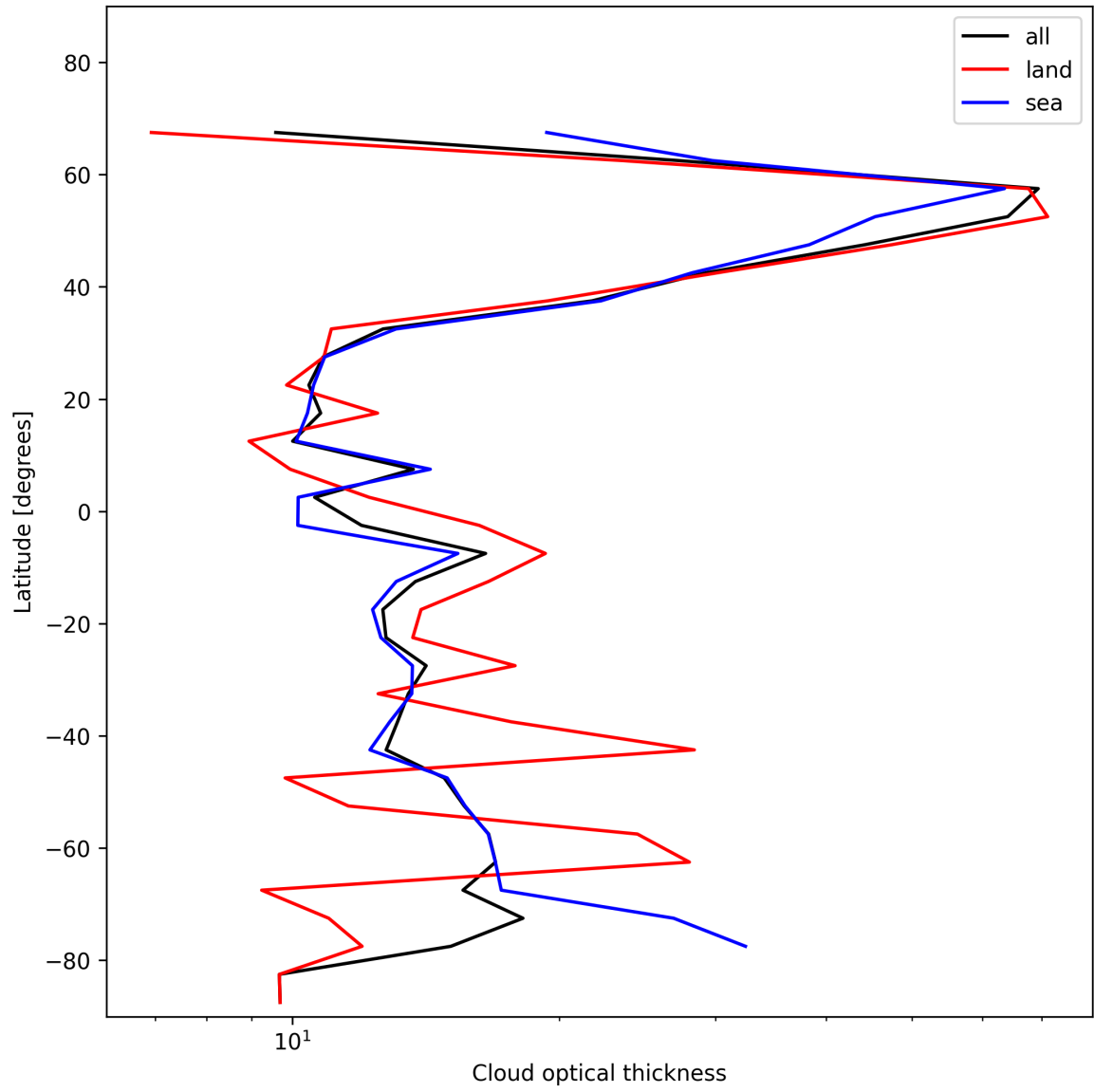
Figure 25: Zonal average of “Cloud optical thickness” for 2024-12-16 to 2024-12-17.
