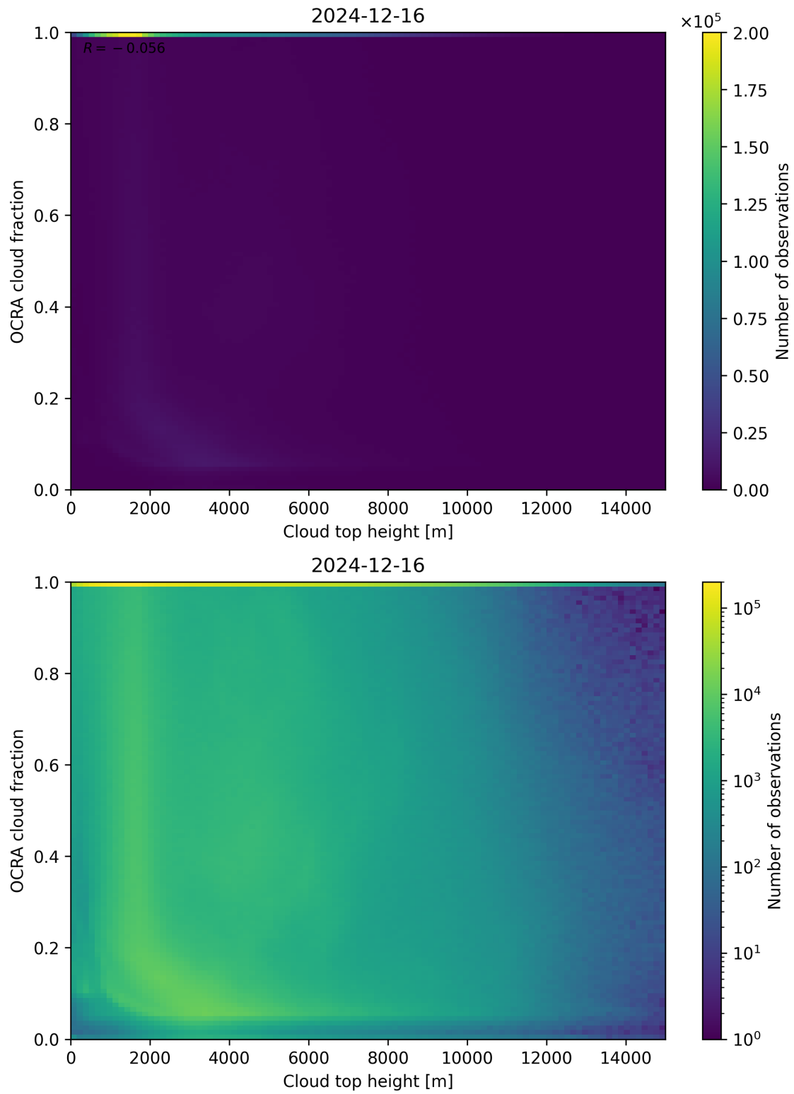
Figure 87: Scatter density plot of “Cloud top height” against “OCRA cloud fraction” for 2024-12-16 to 2024-12-17.
