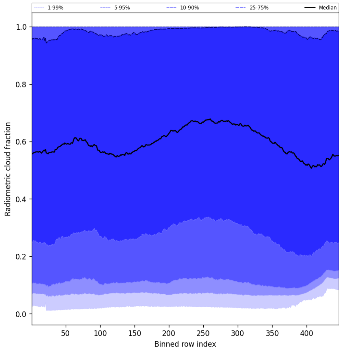
Figure 55: Along track statistics of “Radiometric cloud fraction” for 2024-12-16 to 2024-12-17
