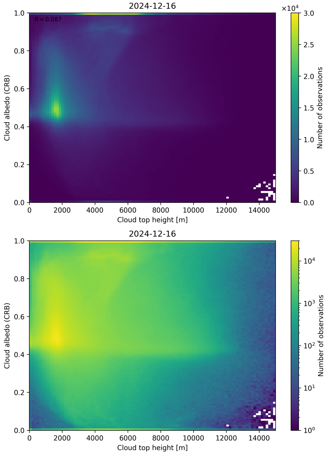
Figure 86: Scatter density plot of “Cloud top height” against “Cloud albedo (CRB)” for 2024-12-16 to 2024-12-17.
