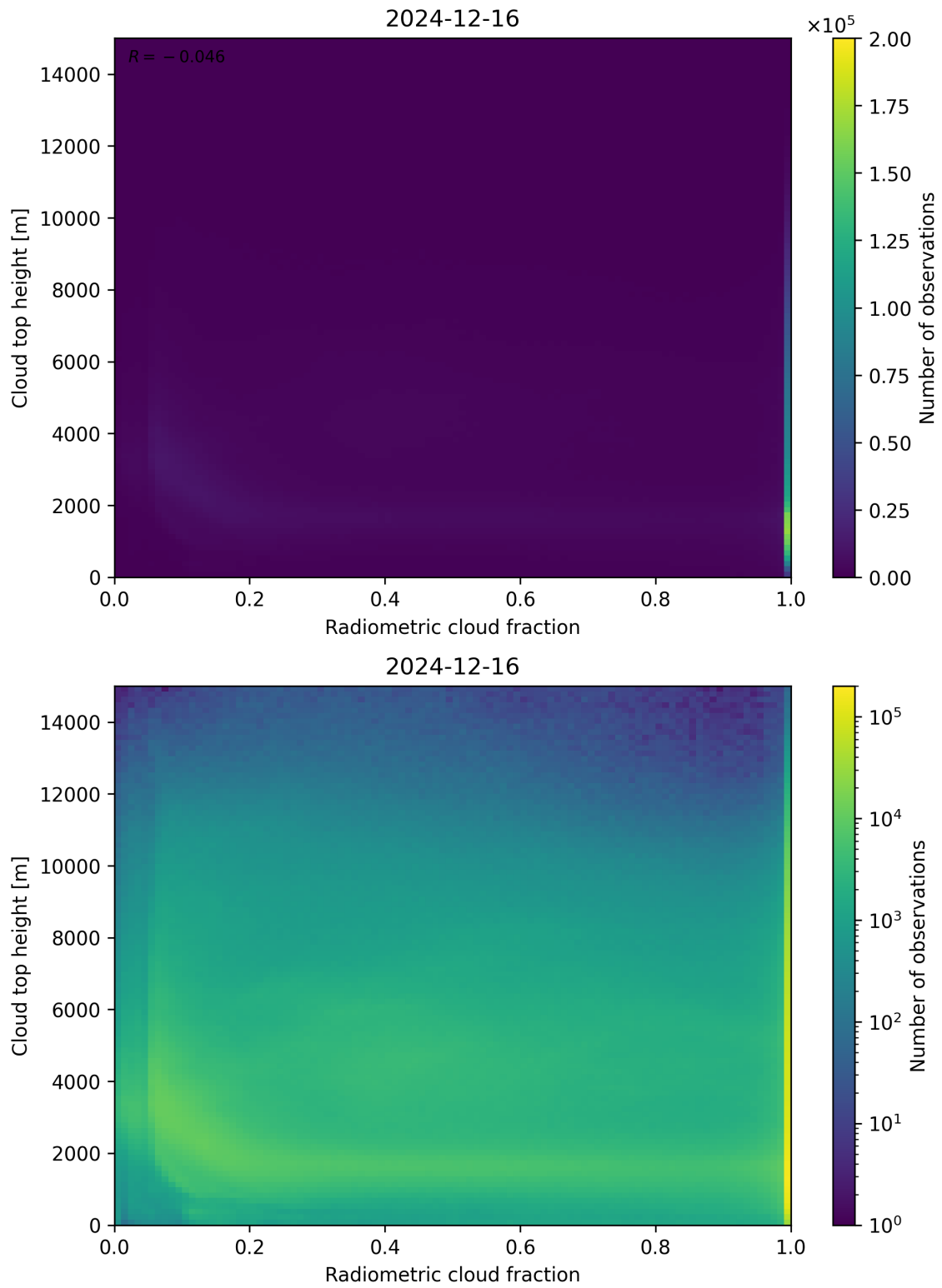
Figure 76: Scatter density plot of “Radiometric cloud fraction” against “Cloud top height” for 2024-12-16 to 2024-12-17.
