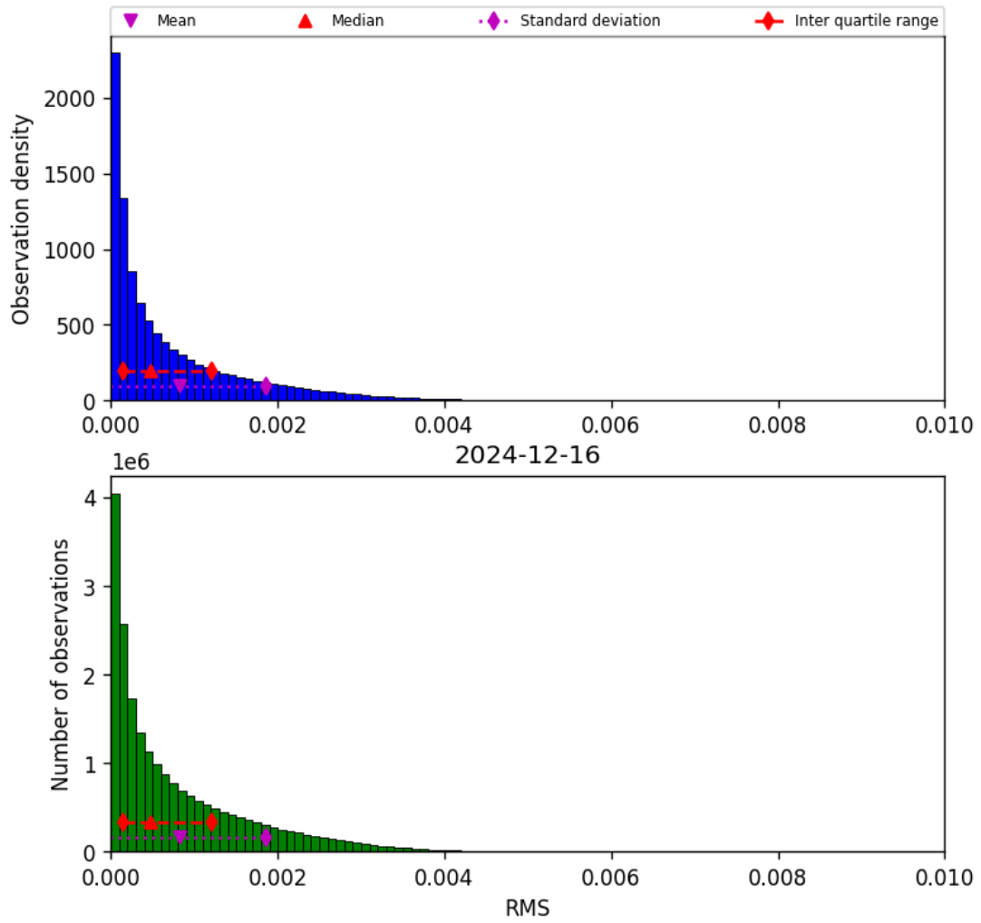
Figure 47: Histogram of “RMS” for 2024-12-16 to 2024-12-17
