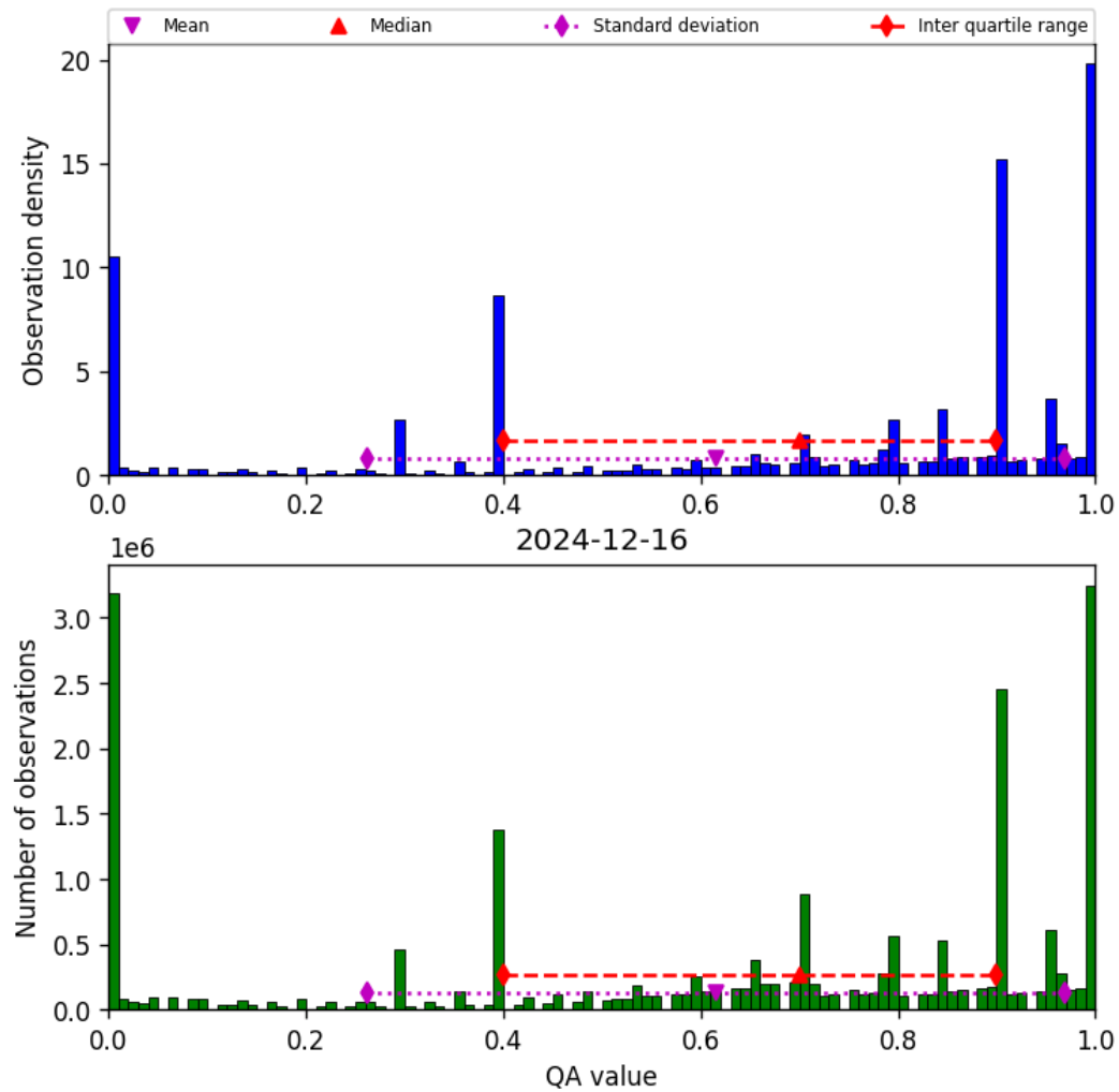
Figure 38: Histogram of “QA value” for 2024-12-16 to 2024-12-17
