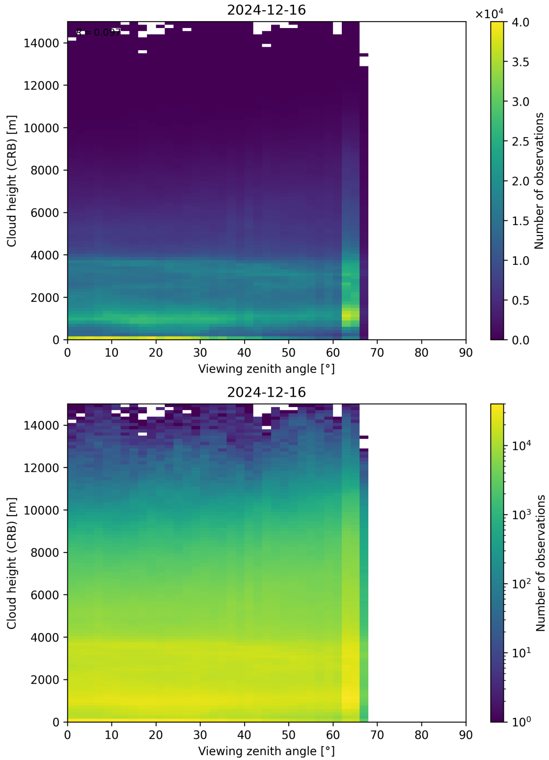
Figure 110: Scatter density plot of “Viewing zenith angle” against “Cloud height (CRB)” for 2024-12-16 to 2024-12-17.
