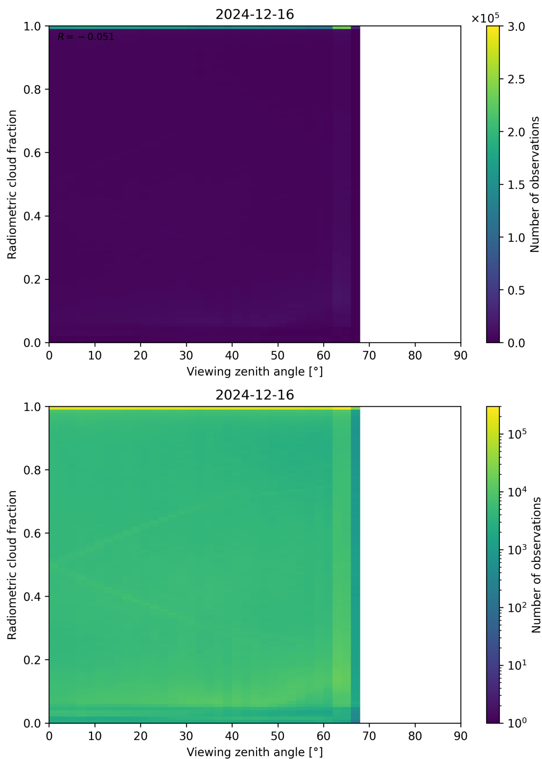
Figure 107: Scatter density plot of “Viewing zenith angle” against “Radiometric cloud fraction” for 2024-12-16 to 2024-12-17.
