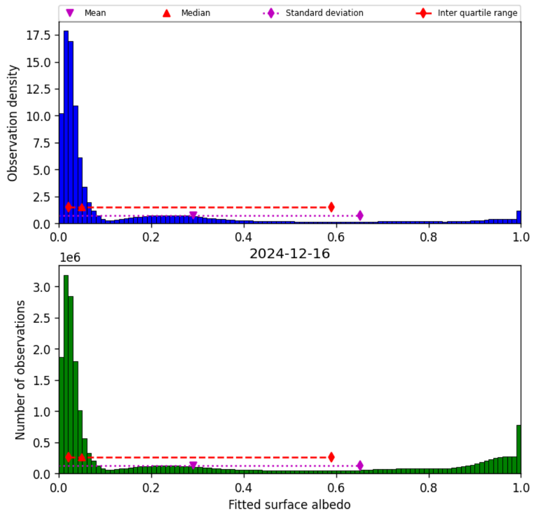
Figure 45: Histogram of “Fitted surface albedo” for 2024-12-16 to 2024-12-17
