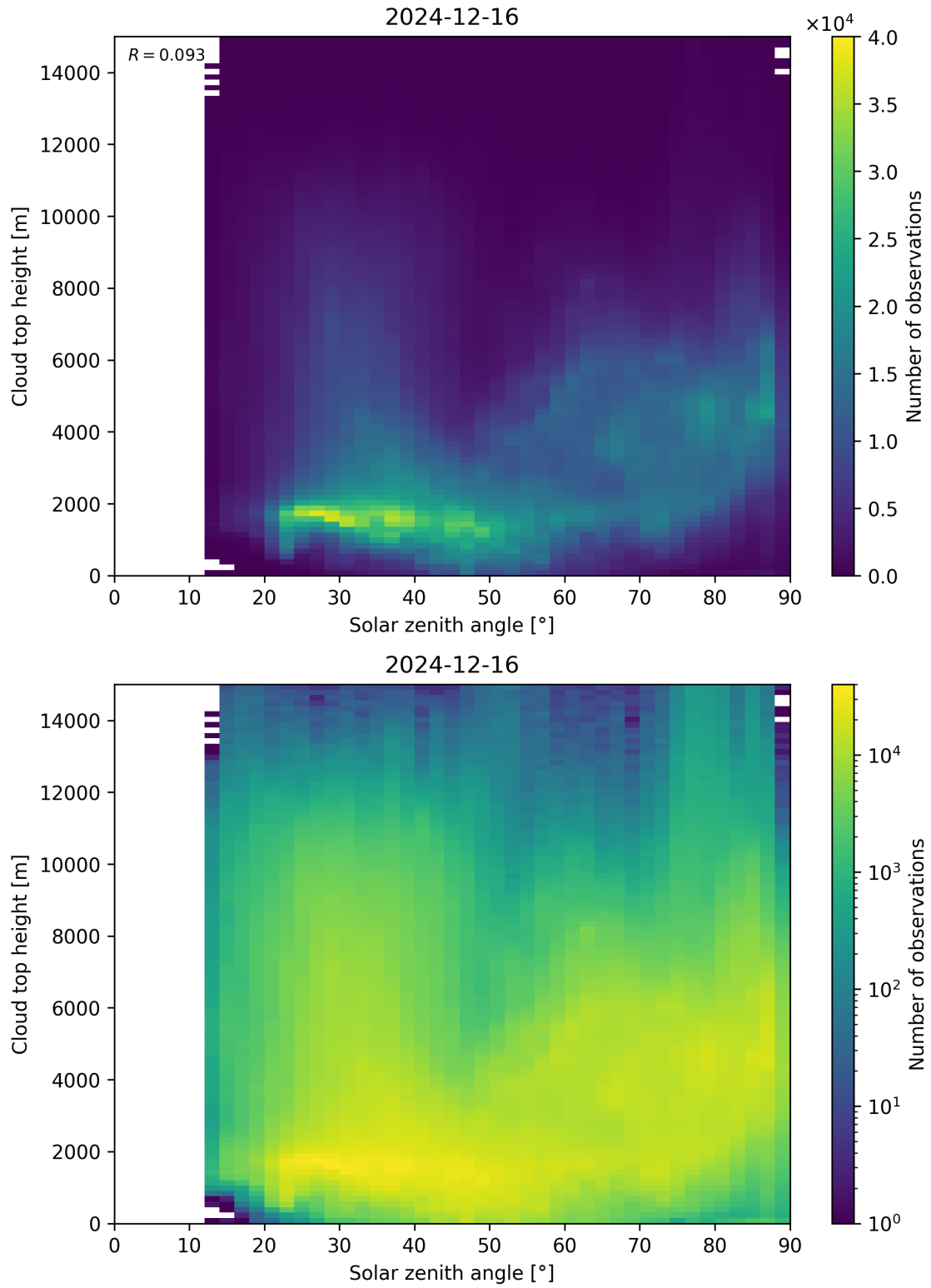
Figure 104: Scatter density plot of “Solar zenith angle” against “Cloud top height” for 2024-12-16 to 2024-12-17.
