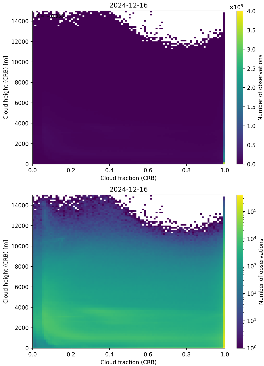
Figure 79: Scatter density plot of “Cloud fraction (CRB)” against “Cloud height (CRB)” for 2024-12-16 to 2024-12-17.
