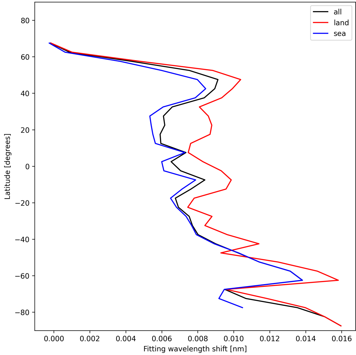
Figure 33: Zonal average of “Fitting wavelength shift” for 2024-12-16 to 2024-12-17.
