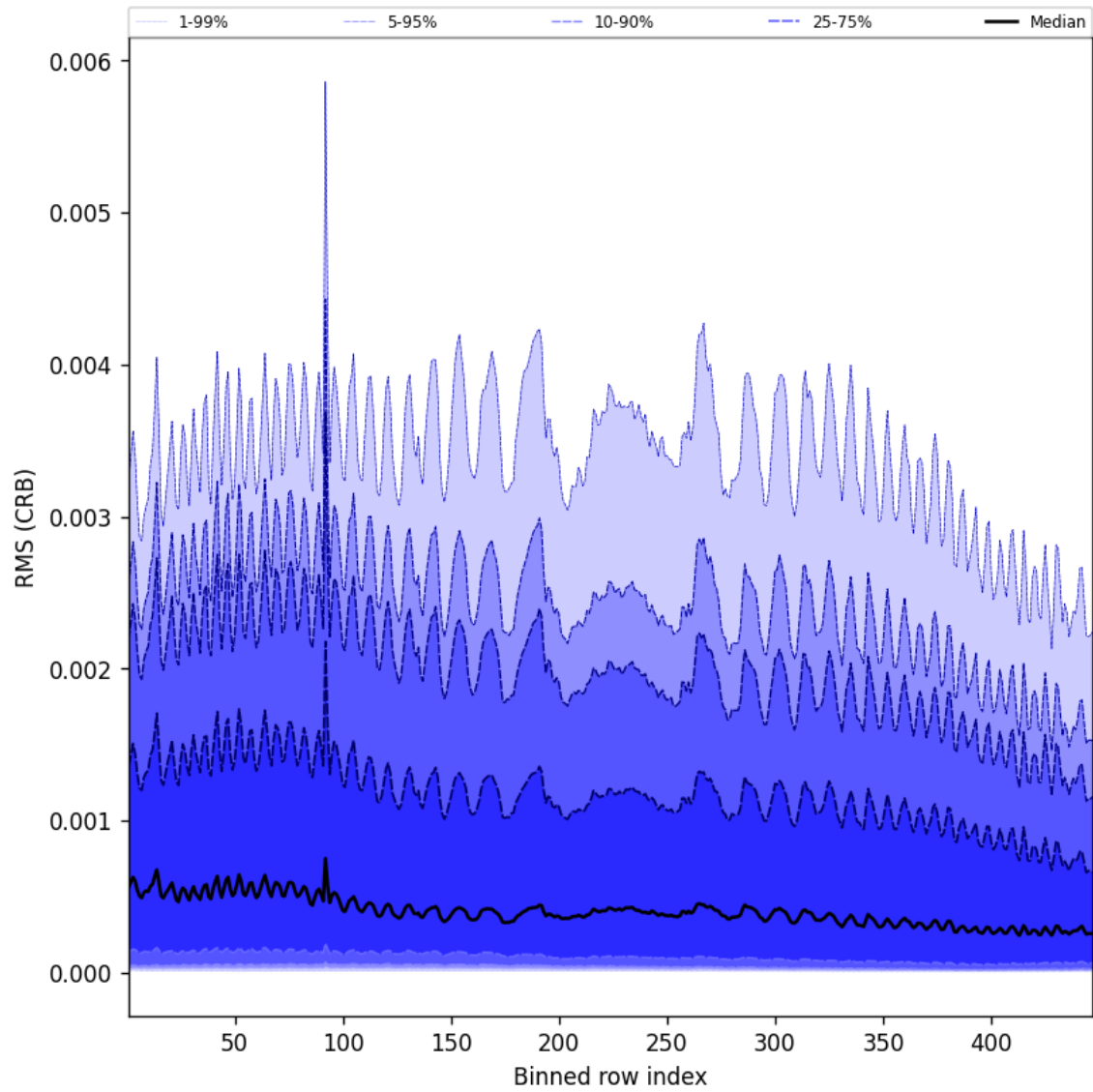
Figure 64: Along track statistics of “RMS (CRB)” for 2024-12-16 to 2024-12-17
