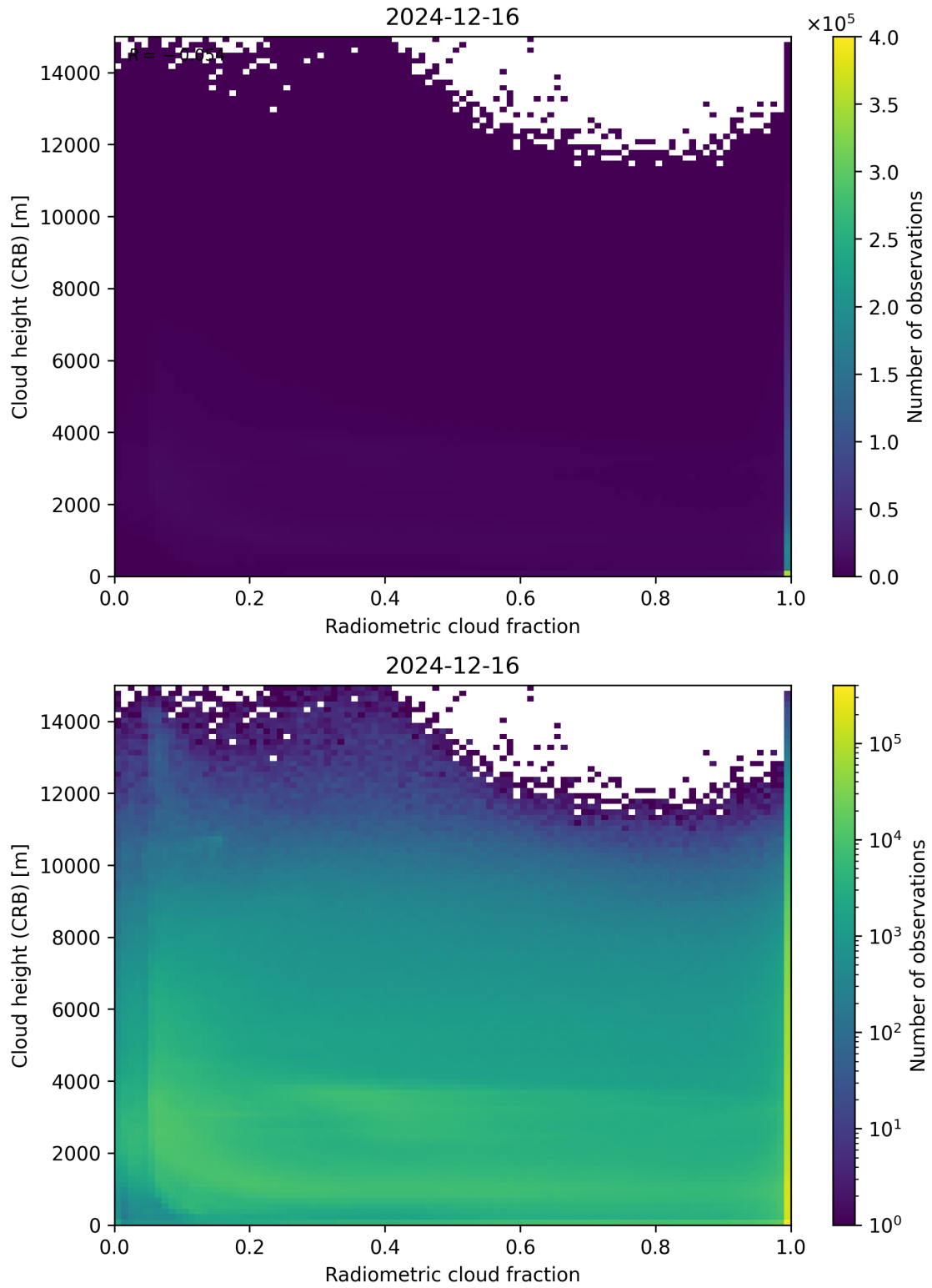
Figure 74: Scatter density plot of “Radiometric cloud fraction” against “Cloud height (CRB)” for 2024-12-16 to 2024-12-17.
