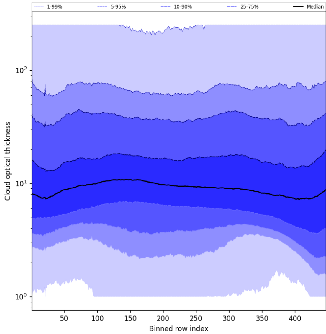
Figure 57: Along track statistics of “Cloud optical thickness” for 2024-12-16 to 2024-12-17
