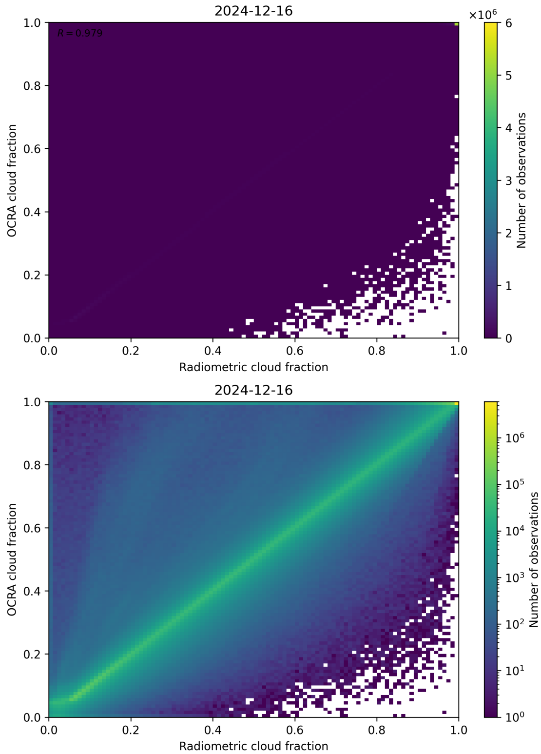
Figure 72: Scatter density plot of “Radiometric cloud fraction” against “OCRA cloud fraction” for 2024-12-16 to 2024-12-17.
