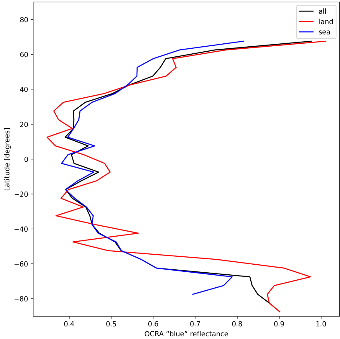
Figure 35: Zonal average of “OCRA “blue” reflectance” for 2024-12-16 to 2024-12-17.
