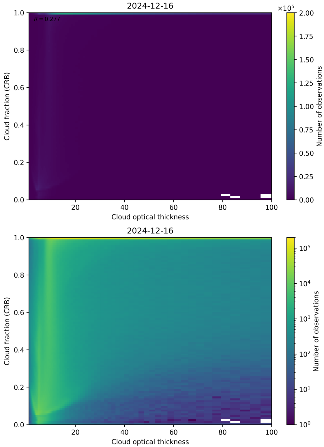
Figure 84: Scatter density plot of “Cloud optical thickness” against “Cloud fraction (CRB)” for 2024-12-16 to 2024-12-17.
