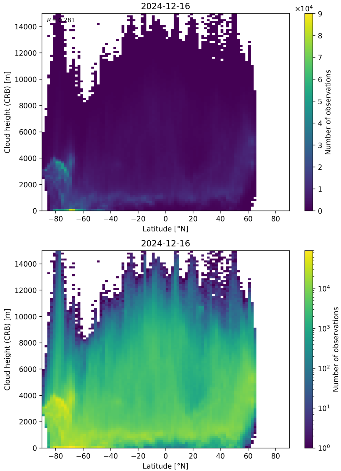
Figure 95: Scatter density plot of “Latitude” against “Cloud height (CRB)” for 2024-12-16 to 2024-12-17.
