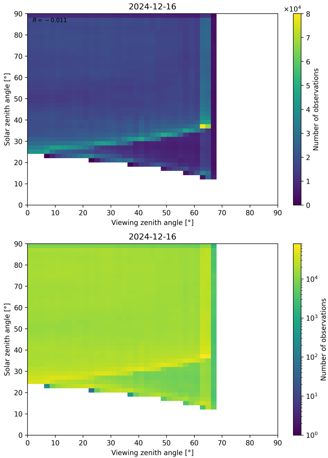
Figure 114: Scatter density plot of “Viewing zenith angle” against “Solar zenith angle” for 2024-12-16 to 2024-12-17.
