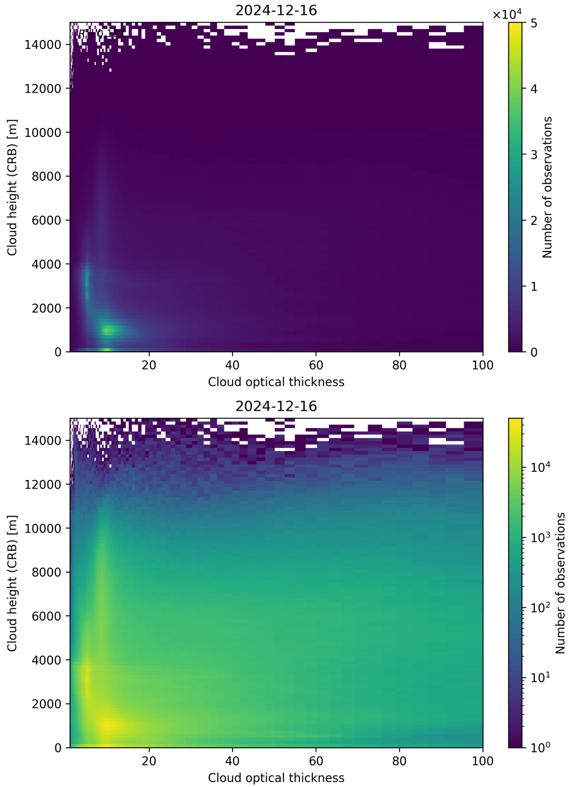
Figure 85: Scatter density plot of “Cloud optical thickness” against “Cloud height (CRB)” for 2024-12-16 to 2024-12-17.
