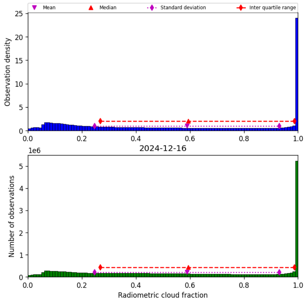
Figure 39: Histogram of “Radiometric cloud fraction” for 2024-12-16 to 2024-12-17
