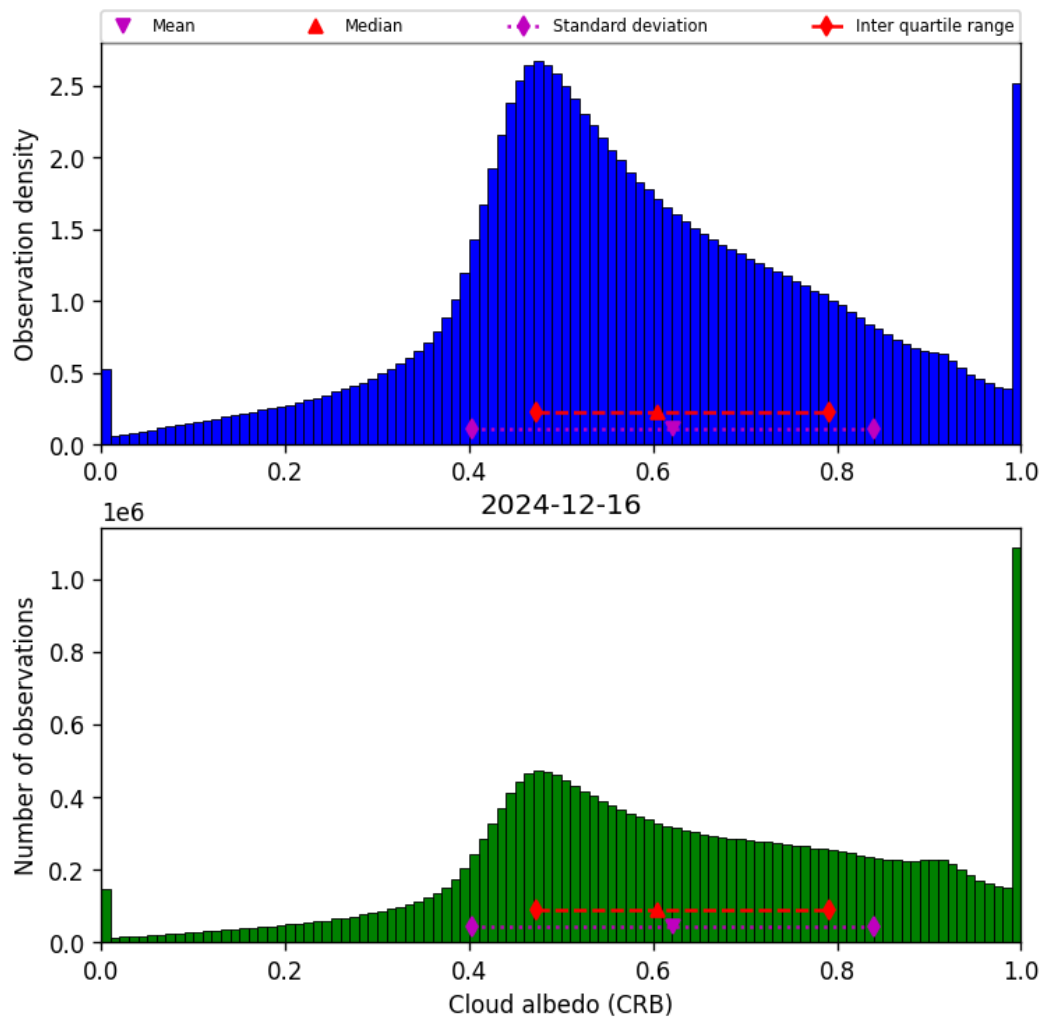
Figure 44: Histogram of “Cloud albedo (CRB)” for 2024-12-16 to 2024-12-17
