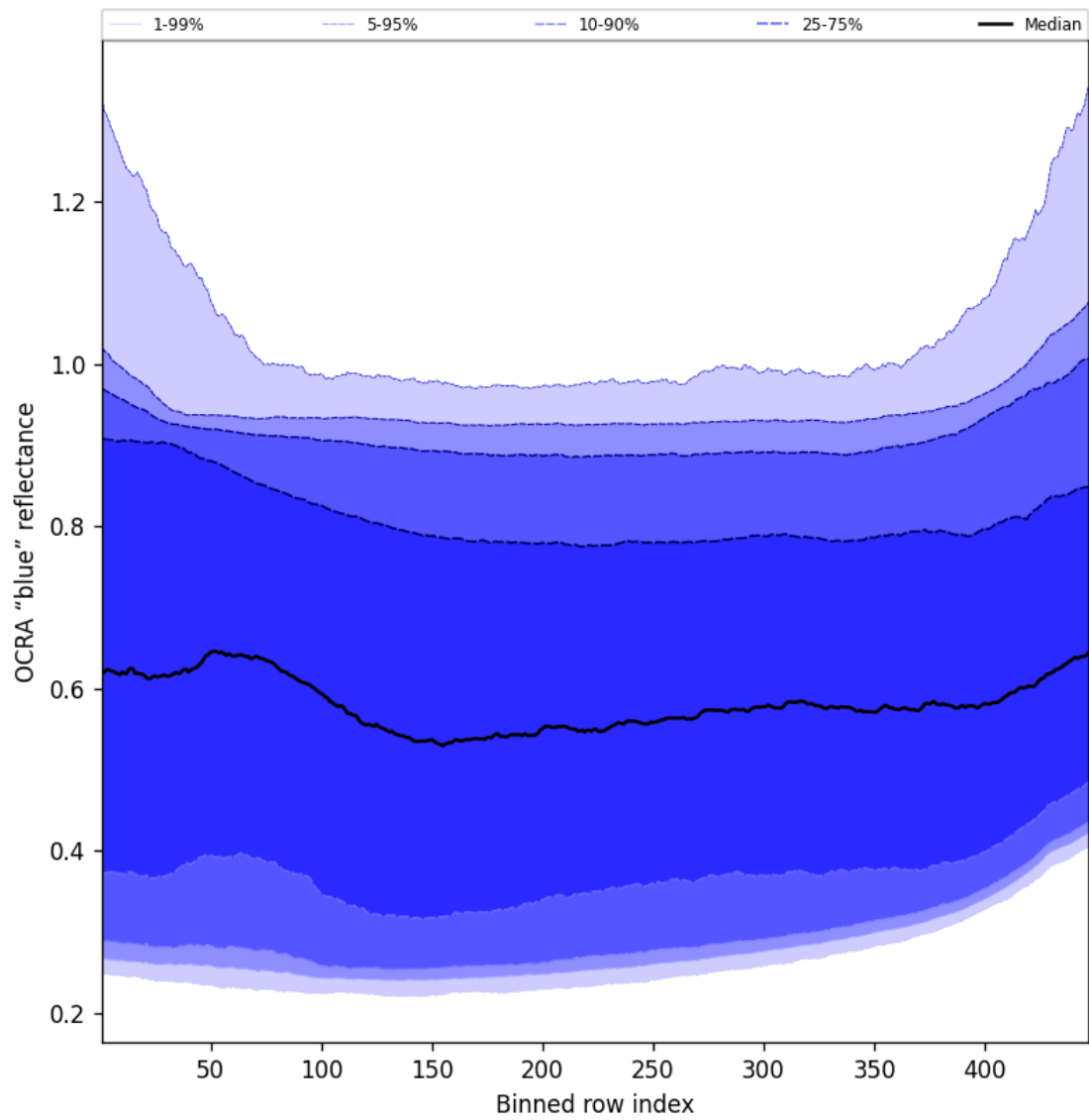
Figure 67: Along track statistics of “OCRA “blue” reflectance” for 2024-12-16 to 2024-12-17
