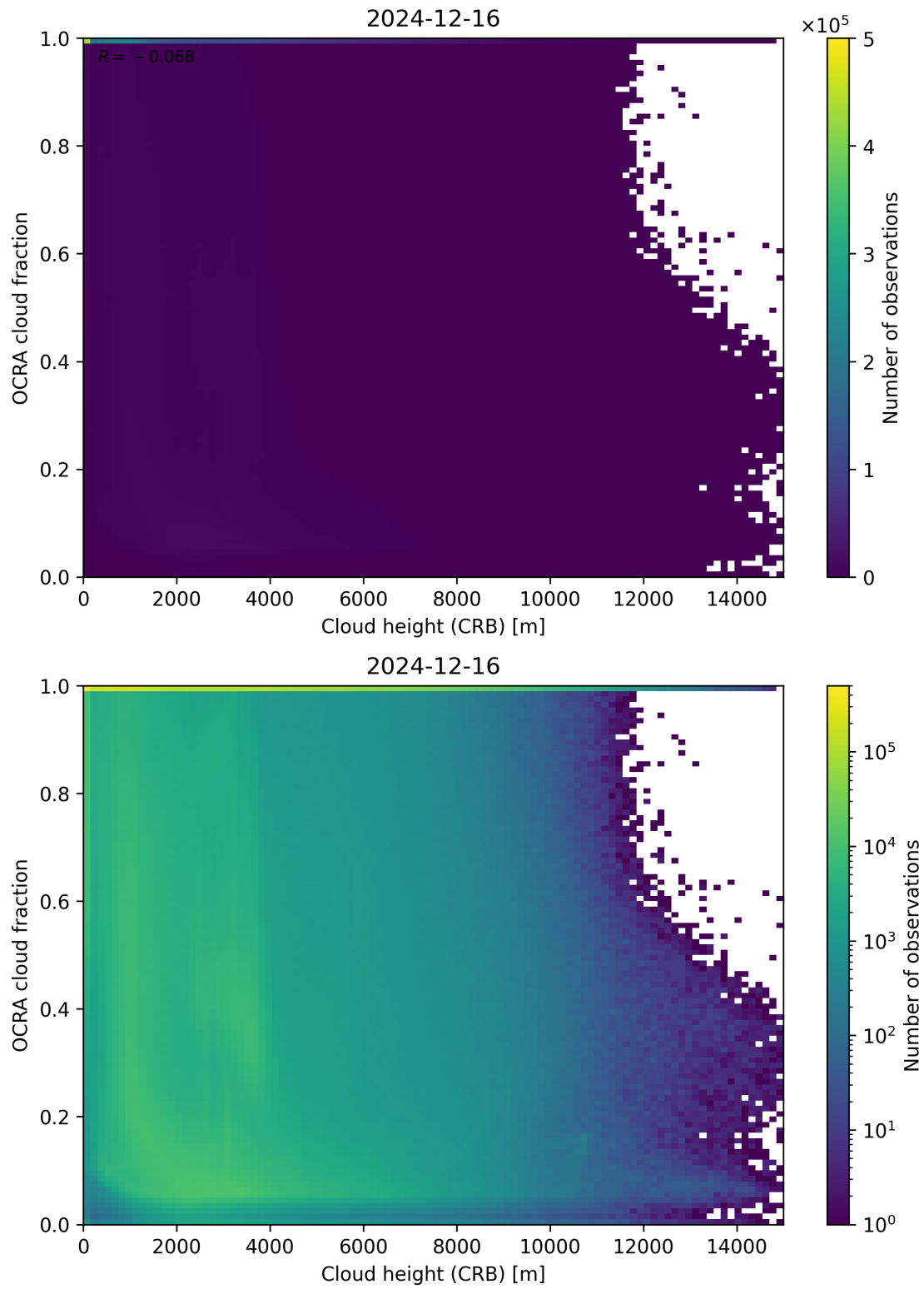
Figure 81: Scatter density plot of “Cloud height (CRB)” against “OCRA cloud fraction” for 2024-12-16 to 2024-12-17.
