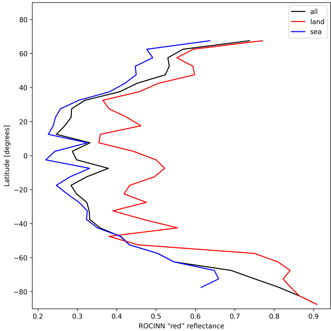
Figure 37: Zonal average of “ROCINN “red” reflectance” for 2024-12-16 to 2024-12-17.
