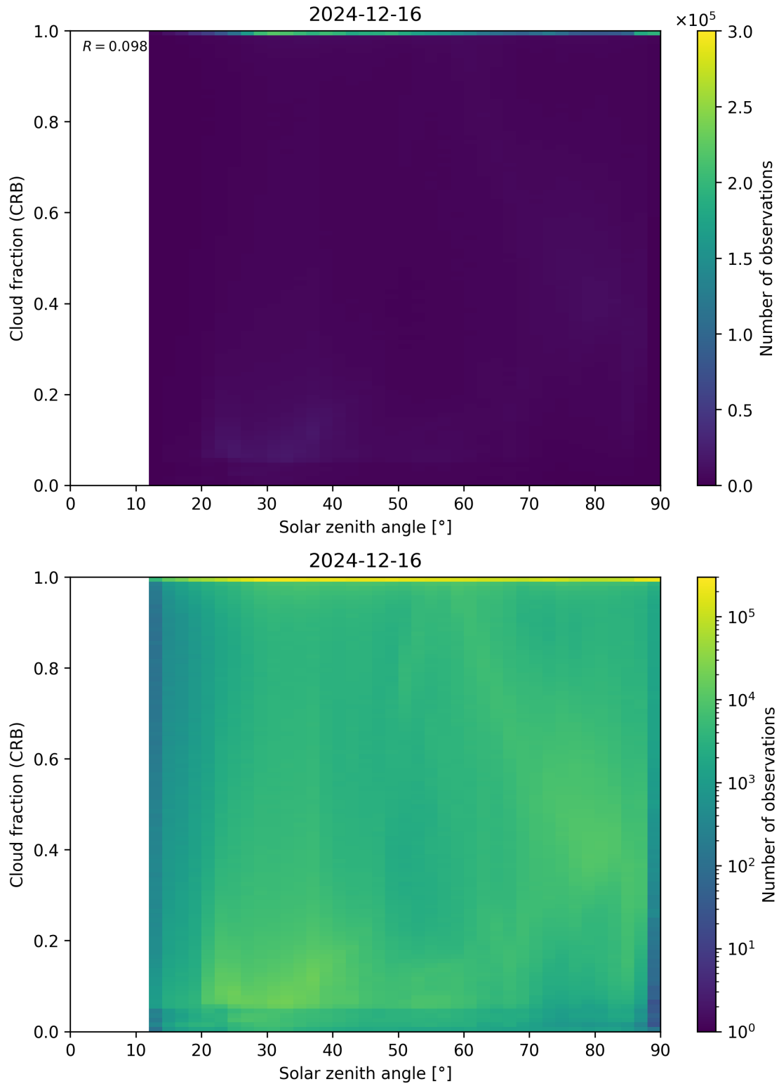
Figure 101: Scatter density plot of “Solar zenith angle” against “Cloud fraction (CRB)” for 2024-12-16 to 2024-12-17.
