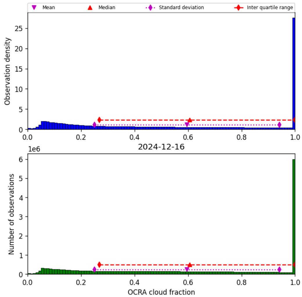
Figure 50: Histogram of “OCRA cloud fraction” for 2024-12-16 to 2024-12-17
