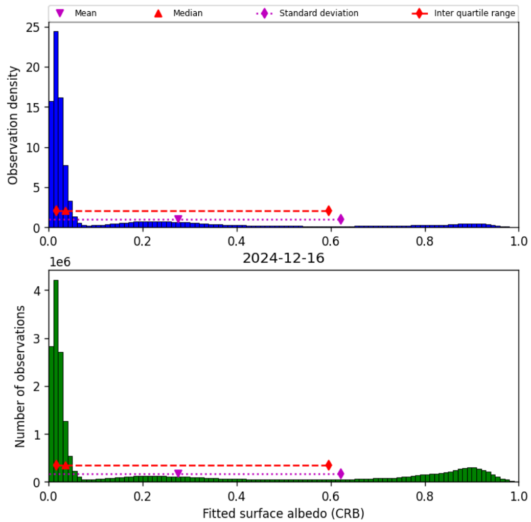
Figure 46: Histogram of “Fitted surface albedo (CRB)” for 2024-12-16 to 2024-12-17
