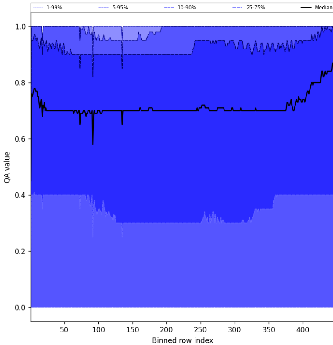
Figure 54: Along track statistics of “QA value” for 2024-12-16 to 2024-12-17
