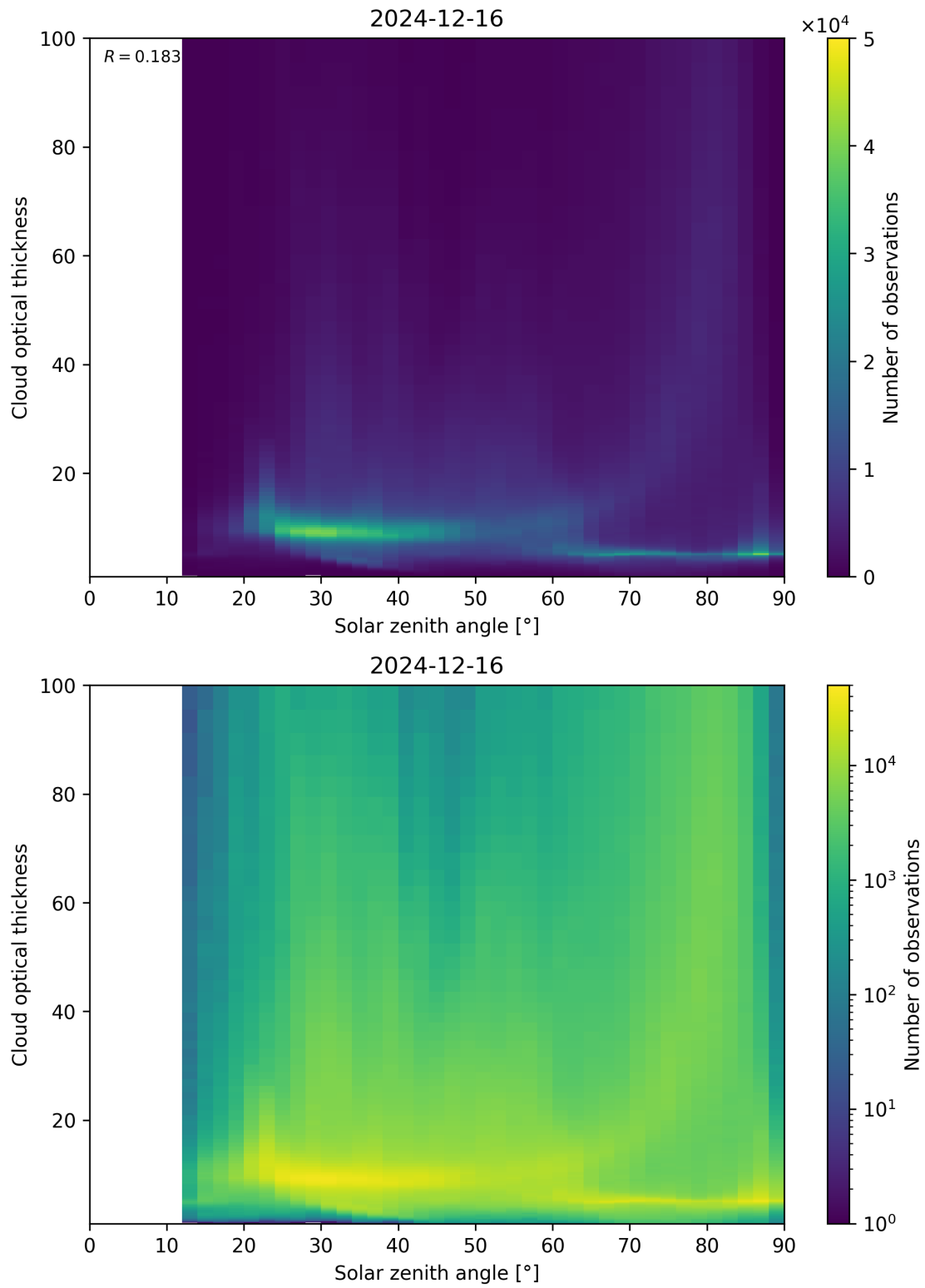
Figure 103: Scatter density plot of “Solar zenith angle” against “Cloud optical thickness” for 2024-12-16 to 2024-12-17.
