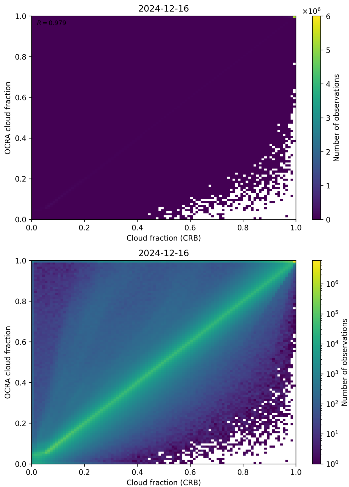
Figure 78: Scatter density plot of “Cloud fraction (CRB)” against “OCRA cloud fraction” for 2024-12-16 to 2024-12-17.
