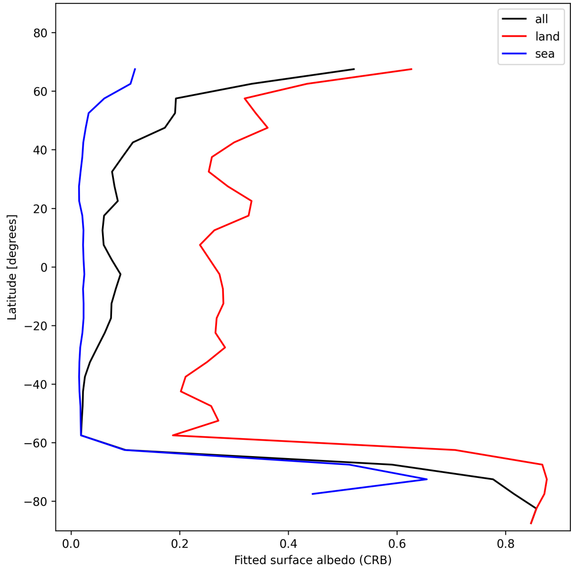
Figure 30: Zonal average of “Fitted surface albedo (CRB)” for 2024-12-16 to 2024-12-17.
