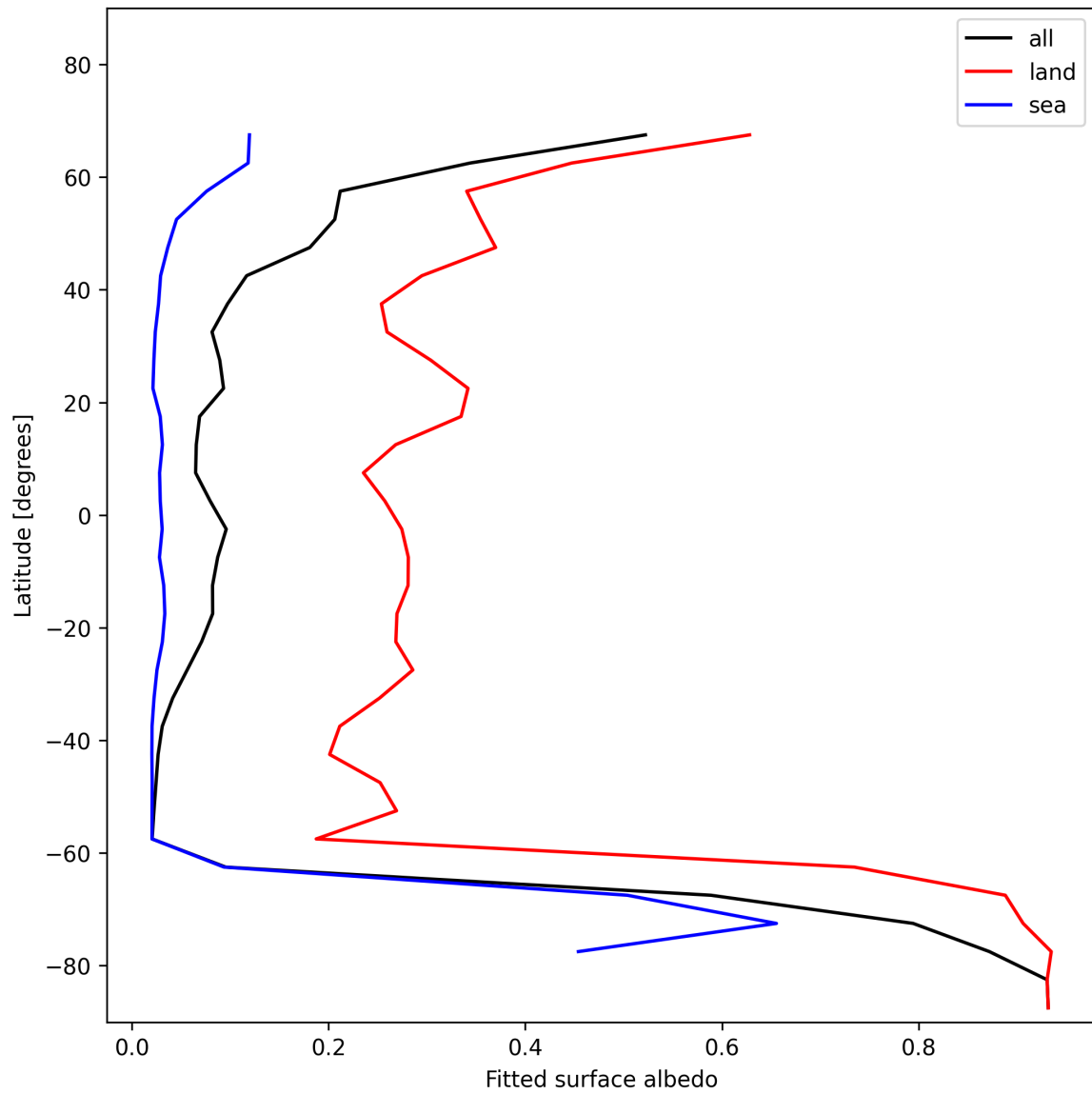
Figure 29: Zonal average of “Fitted surface albedo” for 2024-12-16 to 2024-12-17.
