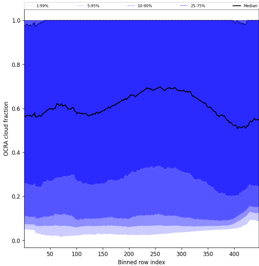
Figure 66: Along track statistics of “OCRA cloud fraction” for 2024-12-16 to 2024-12-17
