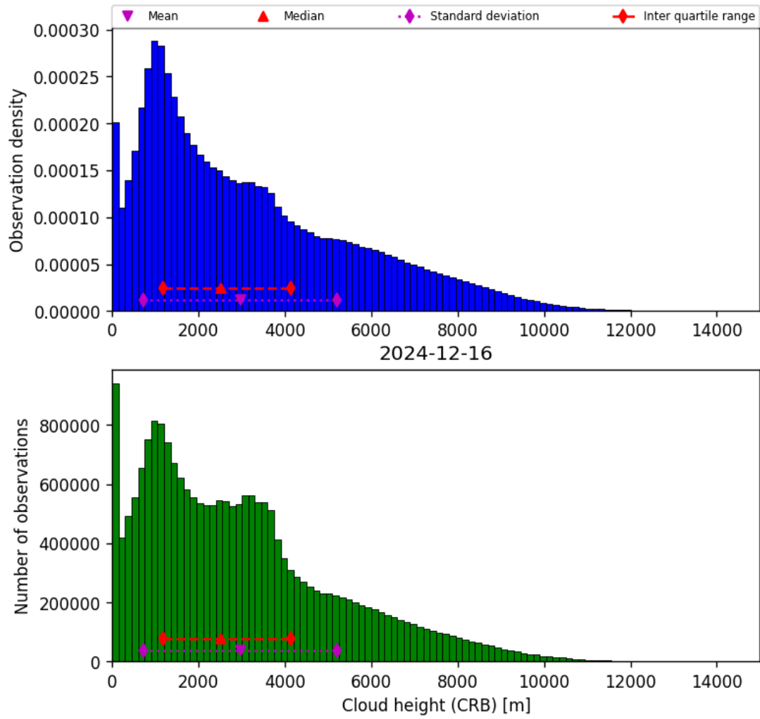
Figure 43: Histogram of “Cloud height (CRB)” for 2024-12-16 to 2024-12-17
