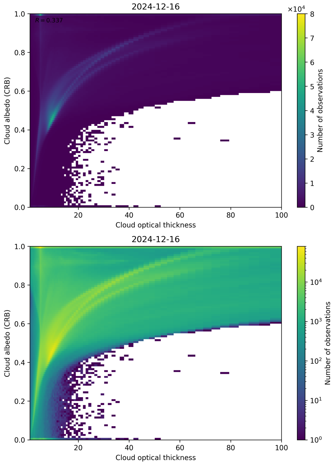
Figure 82: Scatter density plot of “Cloud optical thickness” against “Cloud albedo (CRB)” for 2024-12-16 to 2024-12-17.
