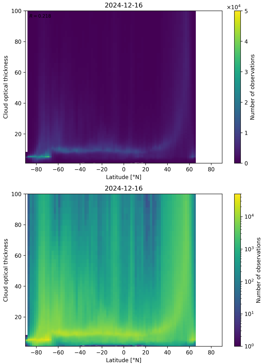
Figure 96: Scatter density plot of “Latitude” against “Cloud optical thickness” for 2024-12-16 to 2024-12-17.
