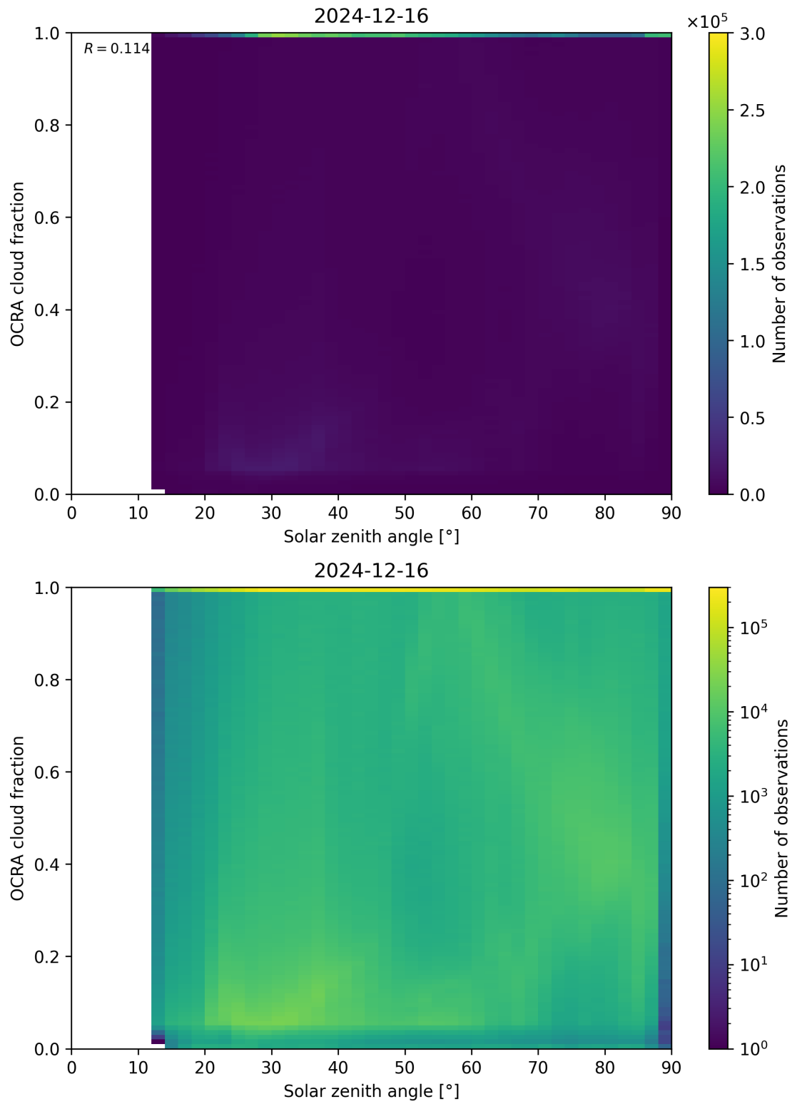
Figure 100: Scatter density plot of “Solar zenith angle” against “OCRA cloud fraction” for 2024-12-16 to 2024-12-17.
