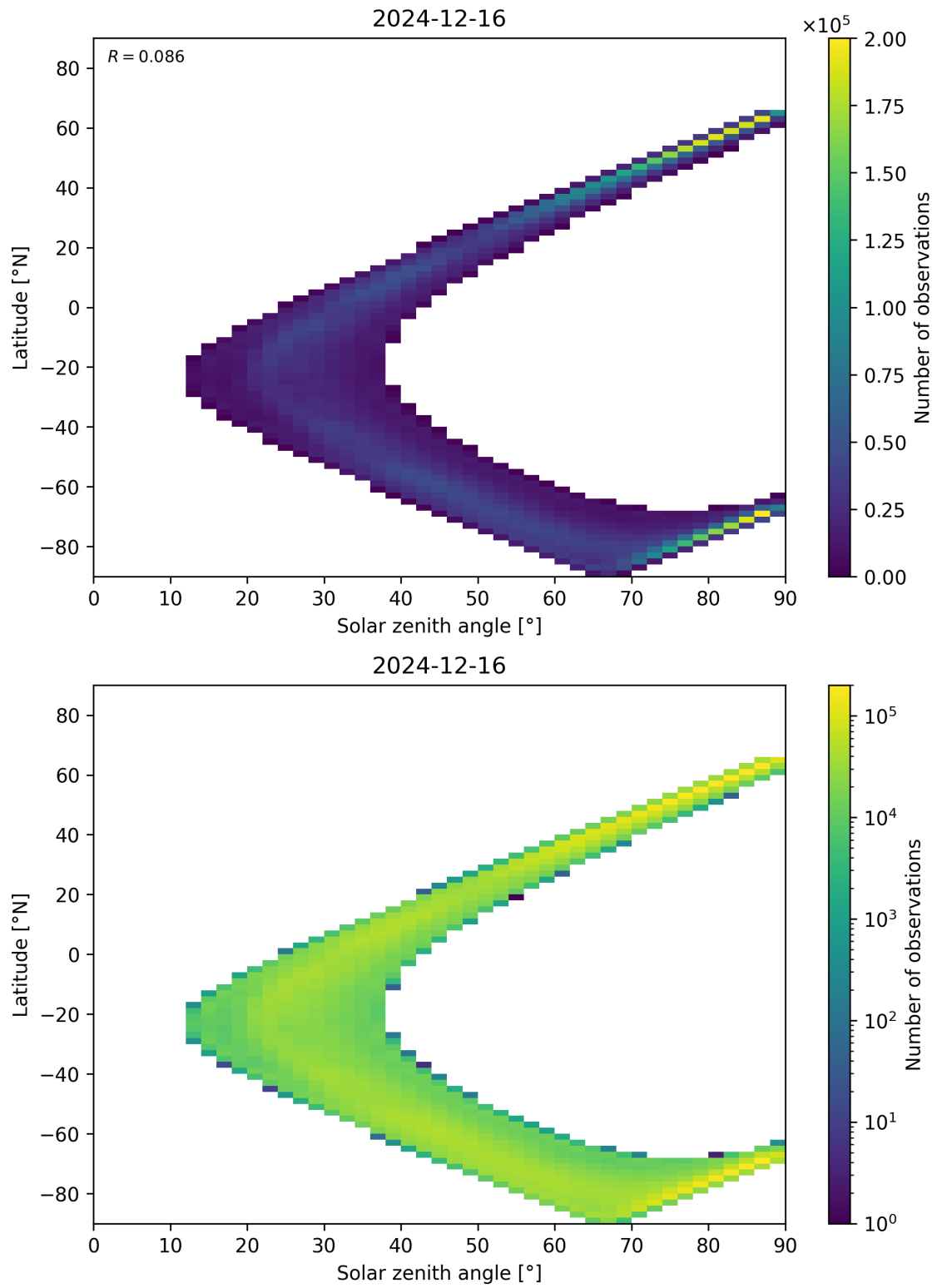
Figure 105: Scatter density plot of “Solar zenith angle” against “Latitude” for 2024-12-16 to 2024-12-17.
