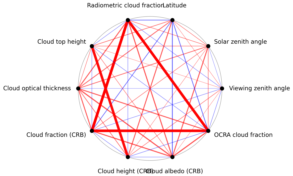
Figure 1: Map of correlation graph for 2024-12-16 to 2024-12-17.
