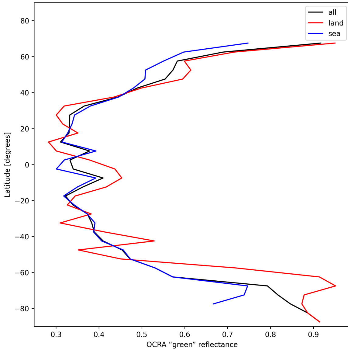
Figure 36: Zonal average of “OCRA “green” reflectance” for 2024-12-16 to 2024-12-17.
