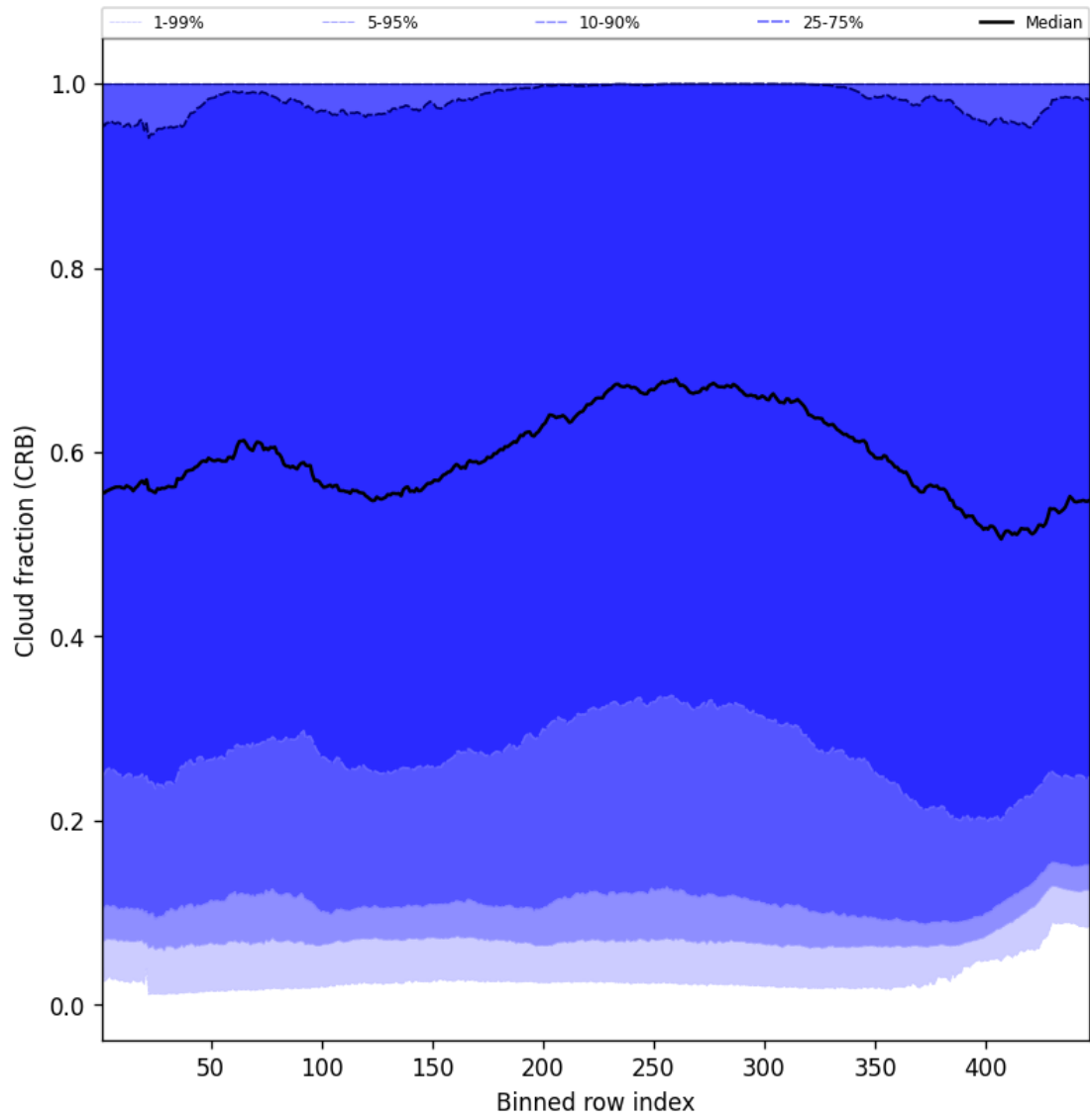
Figure 58: Along track statistics of “Cloud fraction (CRB)” for 2024-12-16 to 2024-12-17
