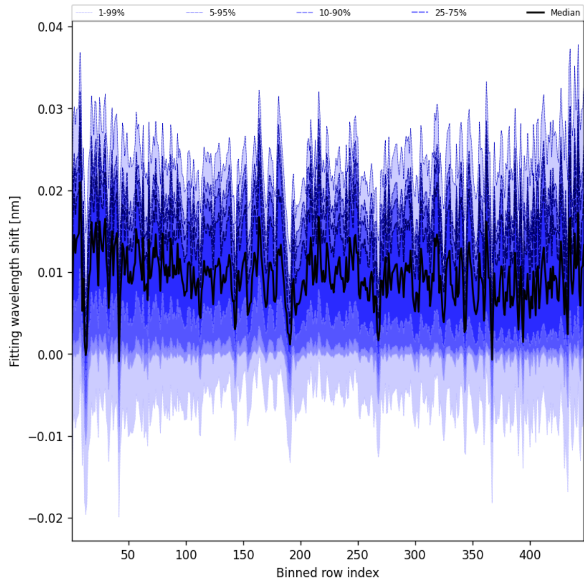
Figure 65: Along track statistics of “Fitting wavelength shift” for 2024-12-16 to 2024-12-17
