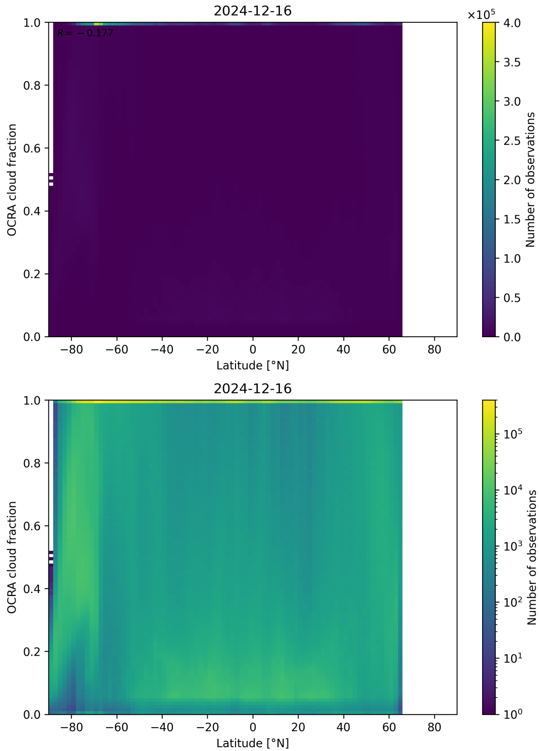
Figure 93: Scatter density plot of “Latitude” against “OCRA cloud fraction” for 2024-12-16 to 2024-12-17.
