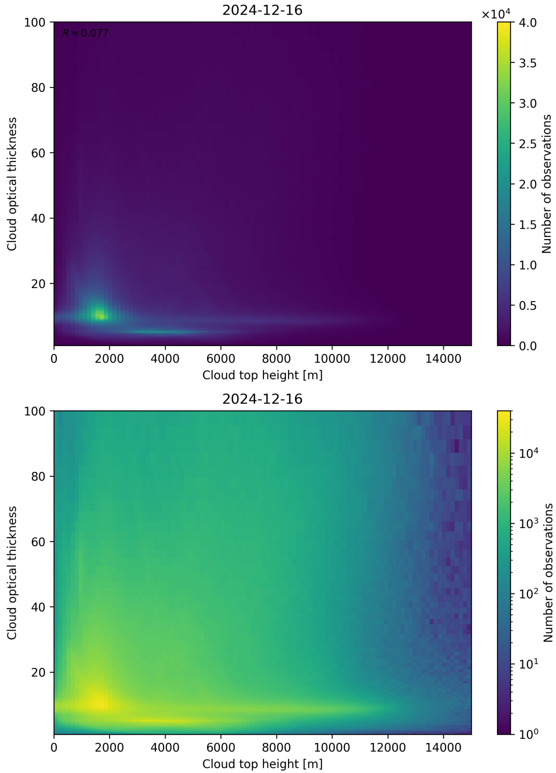
Figure 90: Scatter density plot of “Cloud top height” against “Cloud optical thickness” for 2024-12-16 to 2024-12-17.
