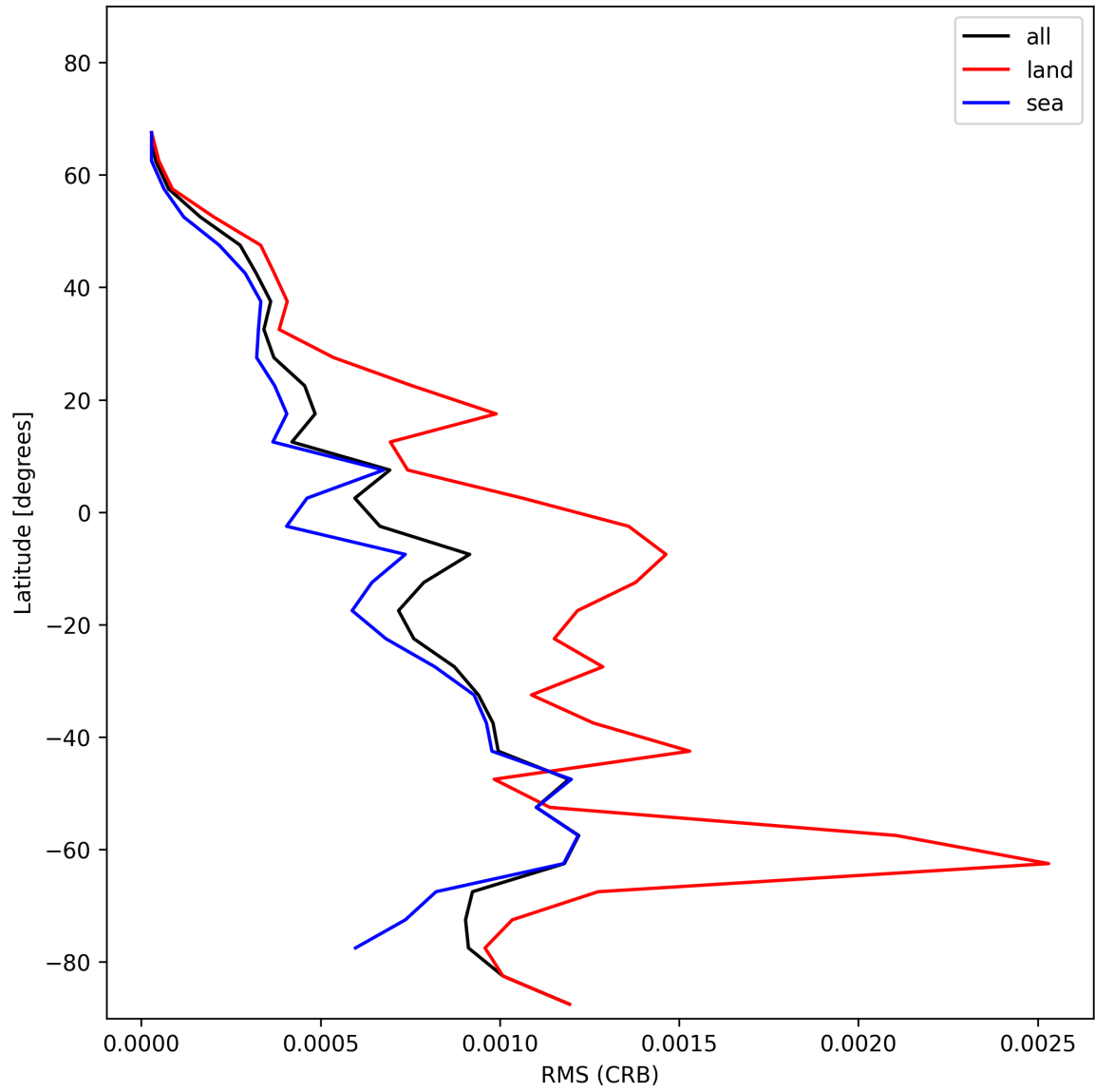
Figure 32: Zonal average of “RMS (CRB)” for 2024-12-16 to 2024-12-17.
