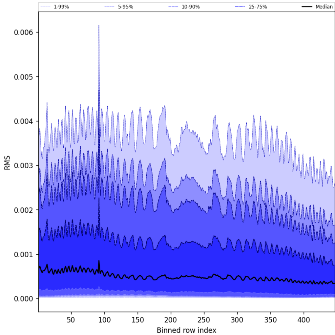
Figure 63: Along track statistics of “RMS” for 2024-12-16 to 2024-12-17
