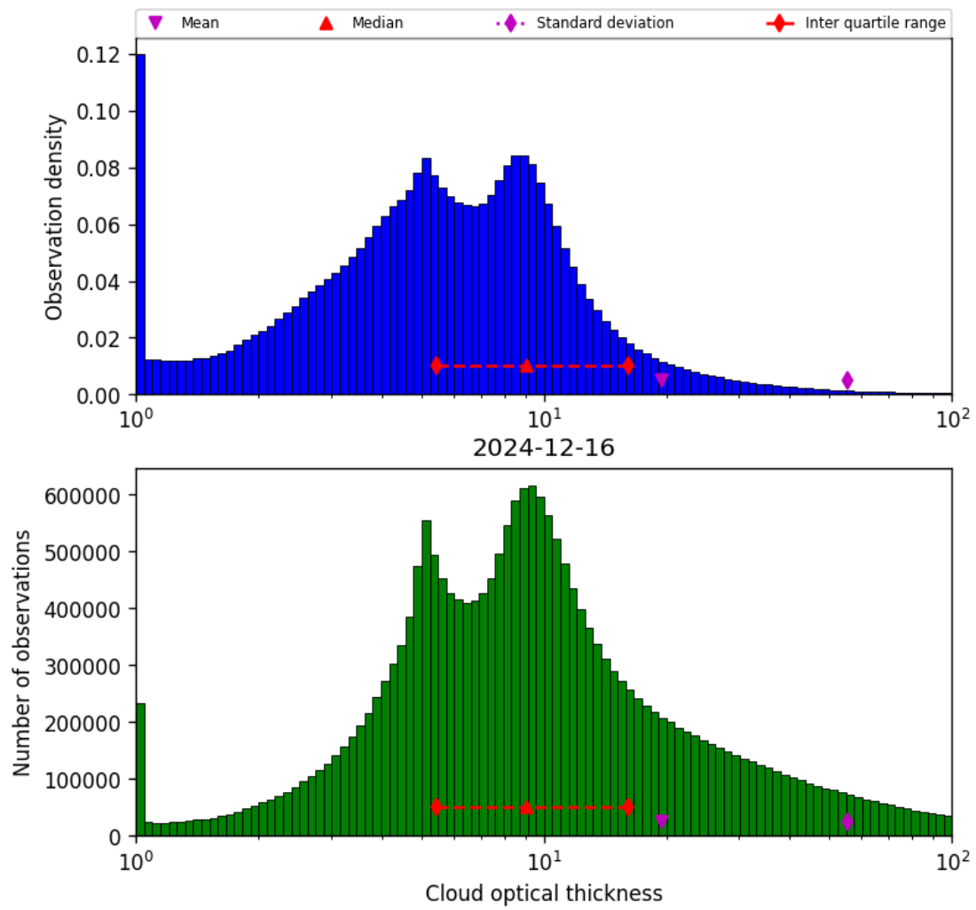
Figure 41: Histogram of “Cloud optical thickness” for 2024-12-16 to 2024-12-17
