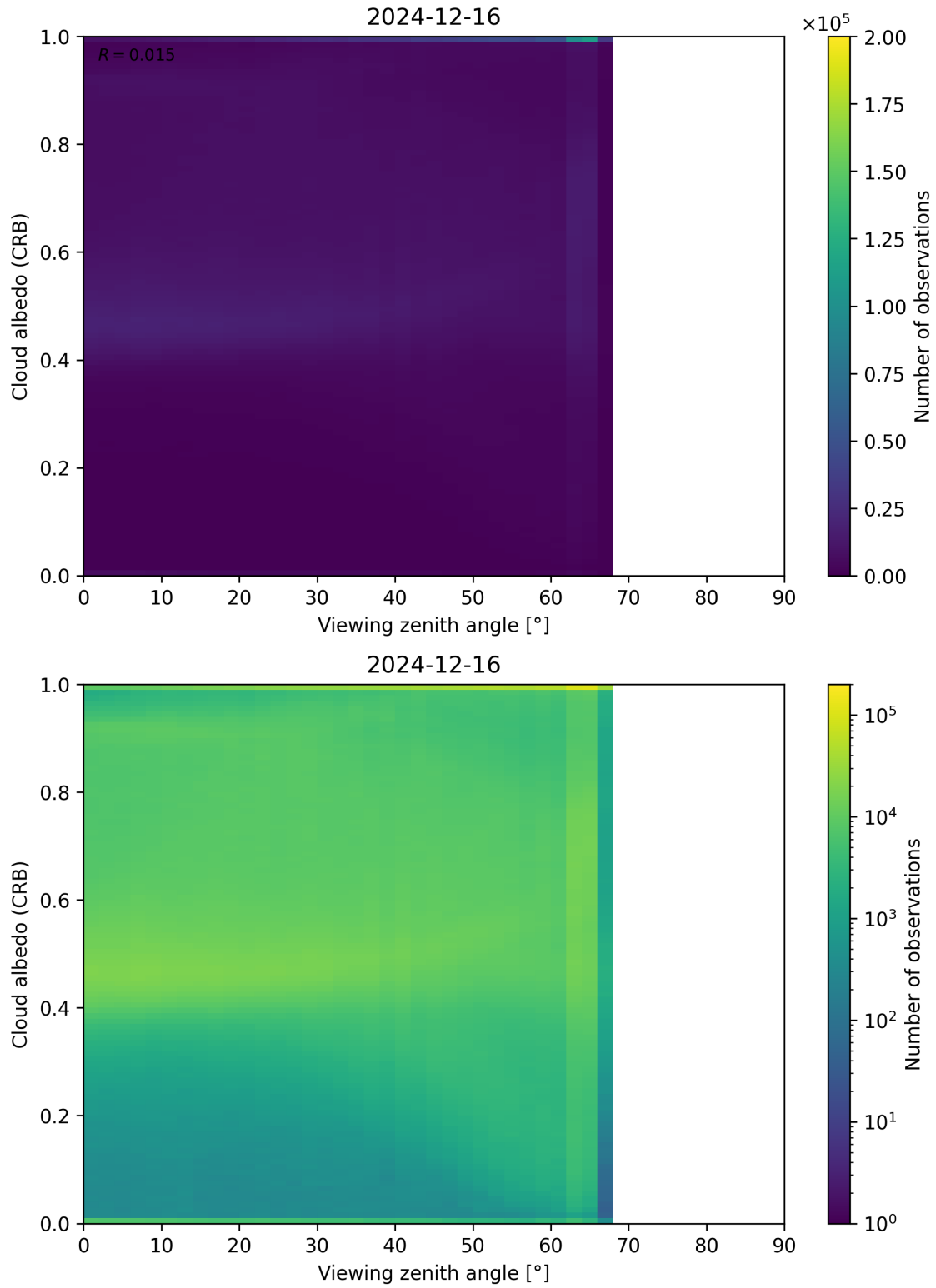
Figure 106: Scatter density plot of “Viewing zenith angle” against “Cloud albedo (CRB)” for 2024-12-16 to 2024-12-17.
