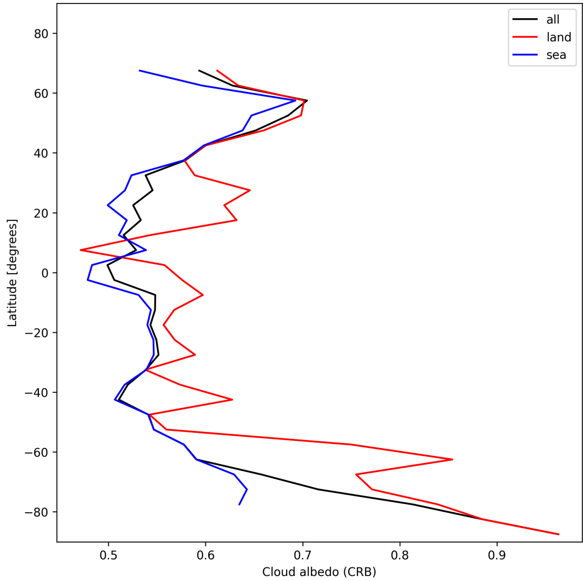
Figure 28: Zonal average of “Cloud albedo (CRB)” for 2024-12-16 to 2024-12-17.
