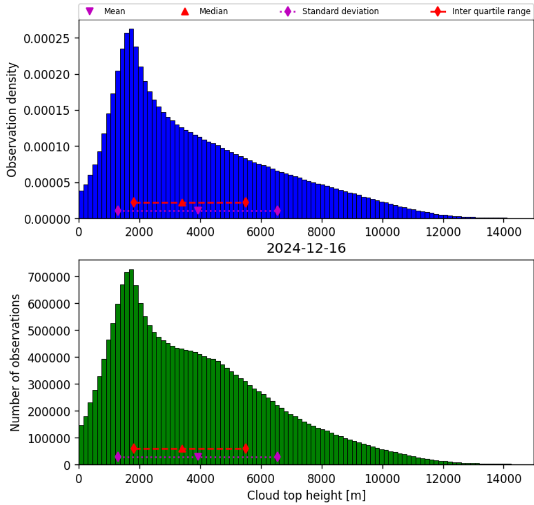
Figure 40: Histogram of “Cloud top height” for 2024-12-16 to 2024-12-17
