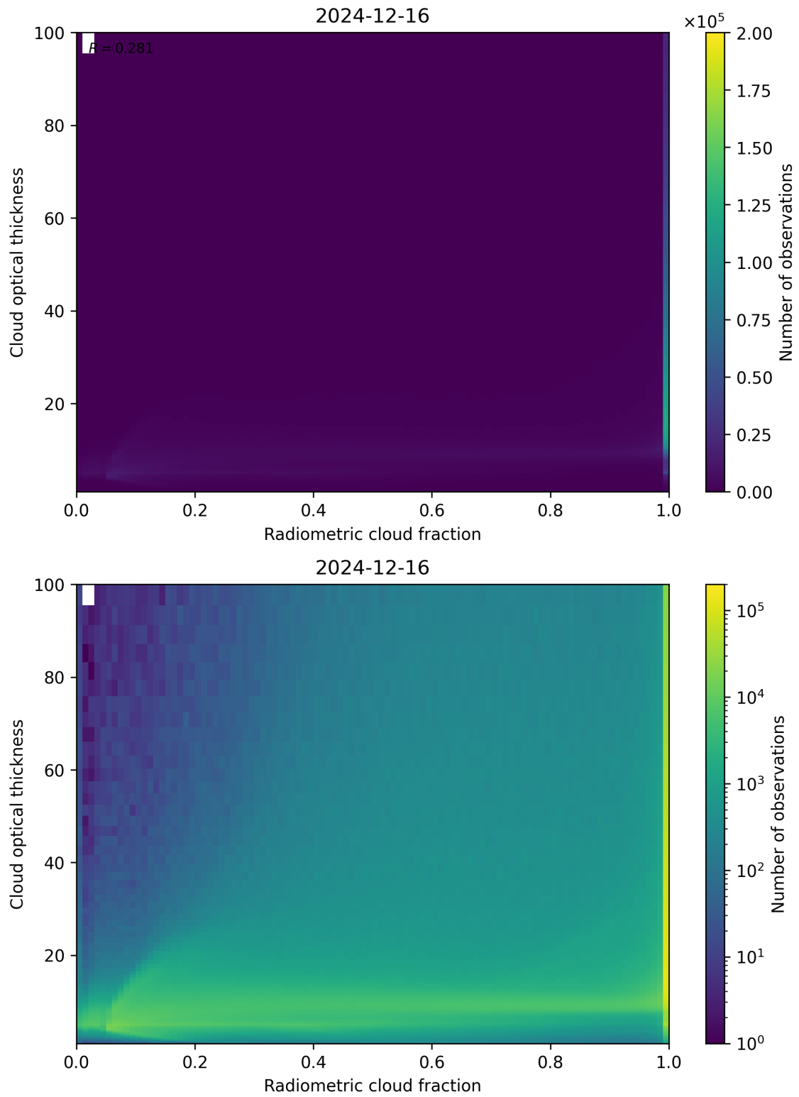
Figure 75: Scatter density plot of “Radiometric cloud fraction” against “Cloud optical thickness” for 2024-12-16 to 2024-12-17.
