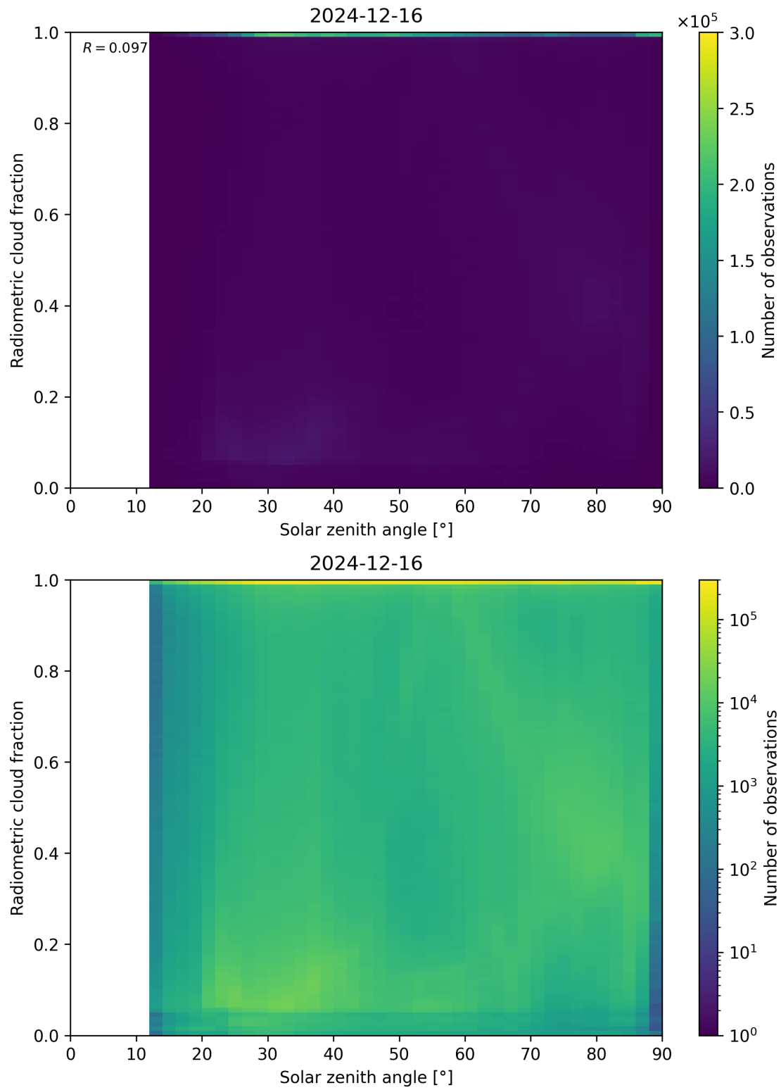
Figure 99: Scatter density plot of “Solar zenith angle” against “Radiometric cloud fraction” for 2024-12-16 to 2024-12-17.
