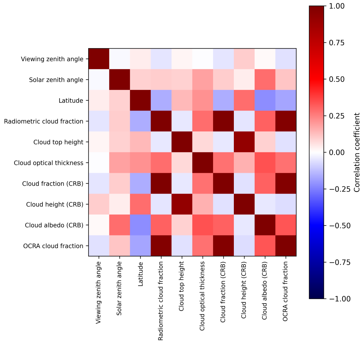
Figure 2: Map of correlation matrix for 2024-12-16 to 2024-12-17.
