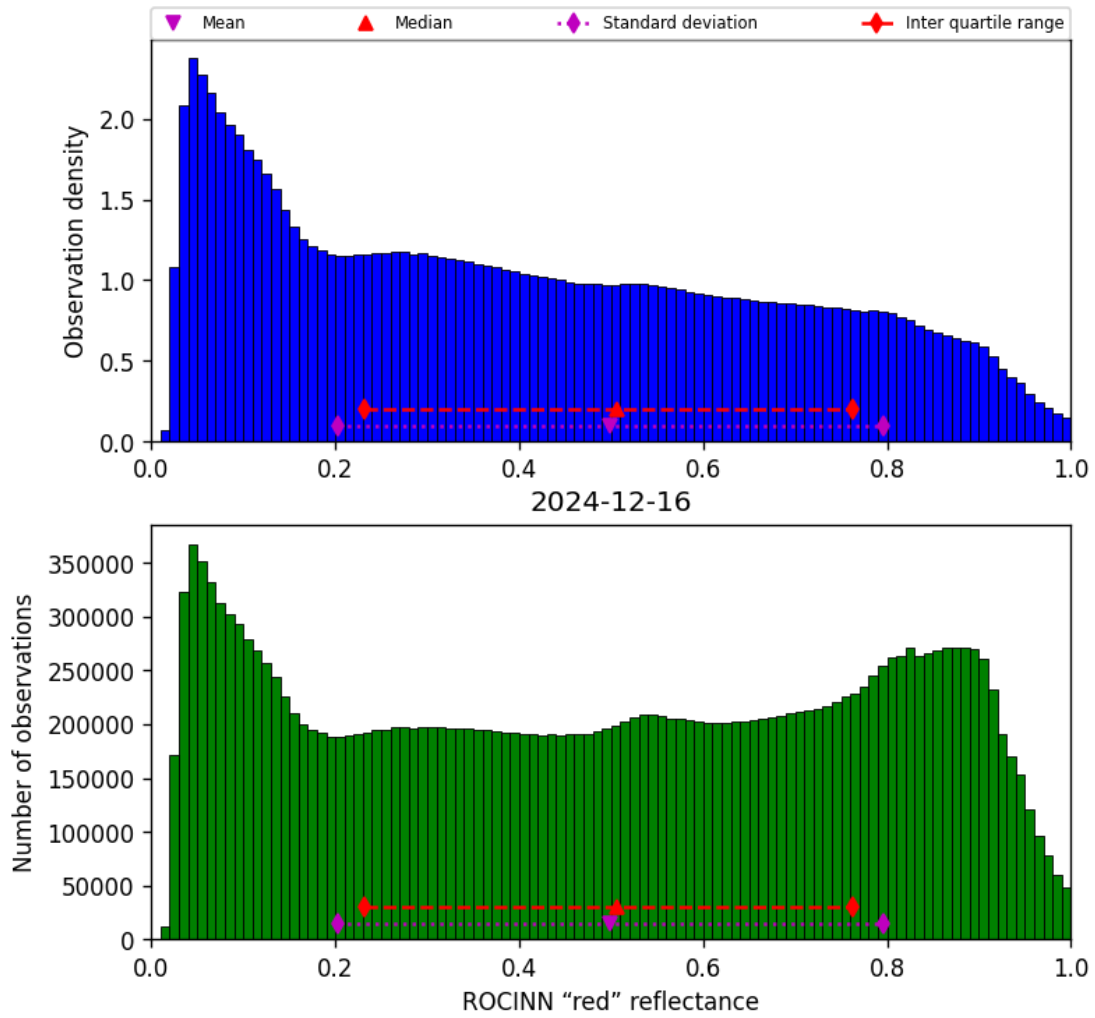
Figure 53: Histogram of “ROCINN “red” reflectance” for 2024-12-16 to 2024-12-17
