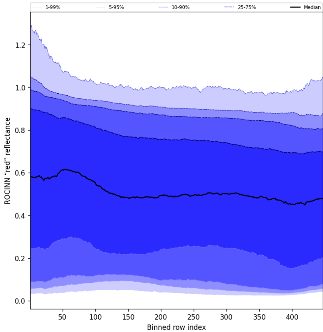
Figure 69: Along track statistics of “ROCINN “red” reflectance” for 2024-12-16 to 2024-12-17
