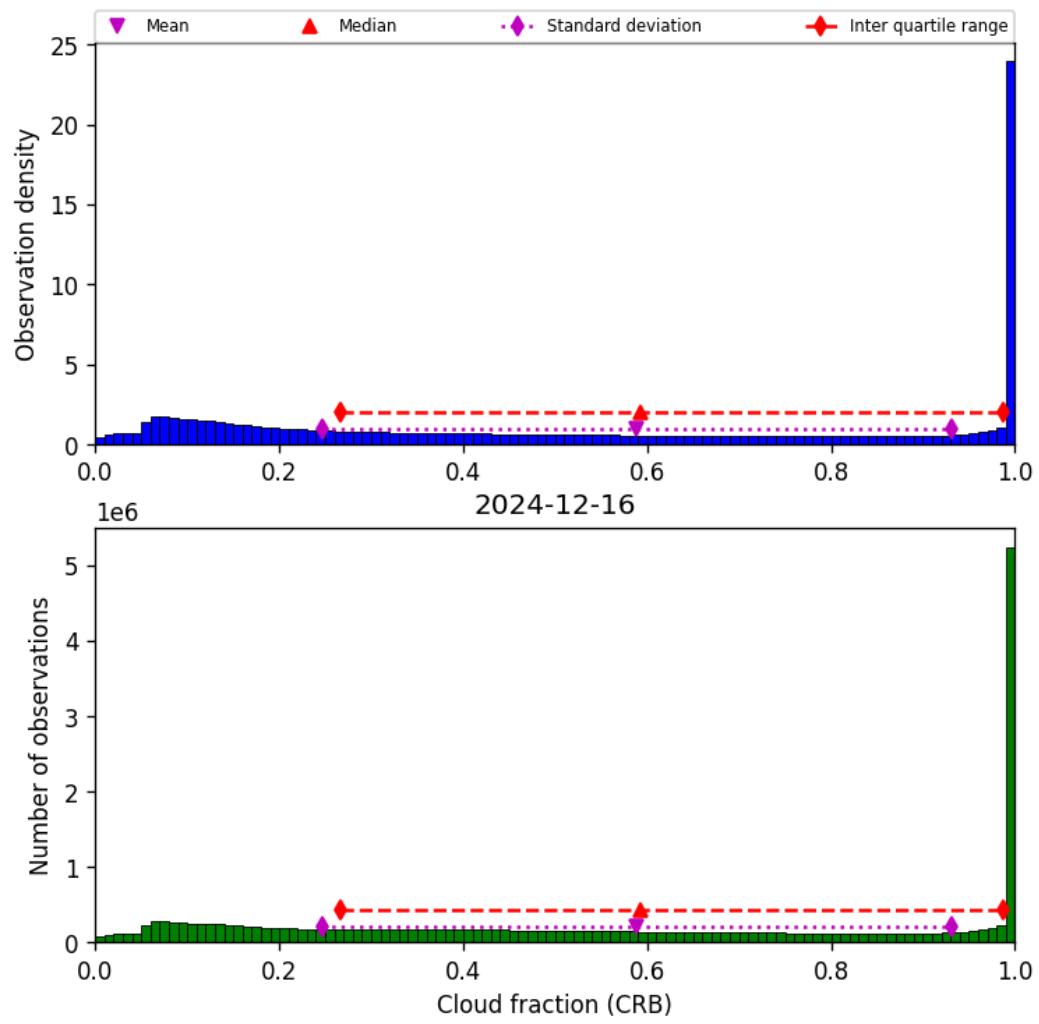
Figure 42: Histogram of “Cloud fraction (CRB)” for 2024-12-16 to 2024-12-17
