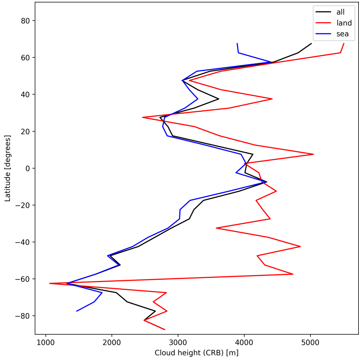
Figure 27: Zonal average of “Cloud height (CRB)” for 2024-12-16 to 2024-12-17.
