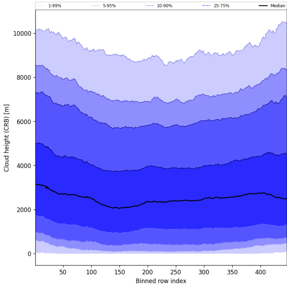
Figure 59: Along track statistics of “Cloud height (CRB)” for 2024-12-16 to 2024-12-17
