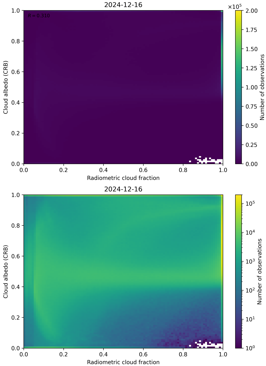
Figure 71: Scatter density plot of “Radiometric cloud fraction” against “Cloud albedo (CRB)” for 2024-12-16 to 2024-12-17.
