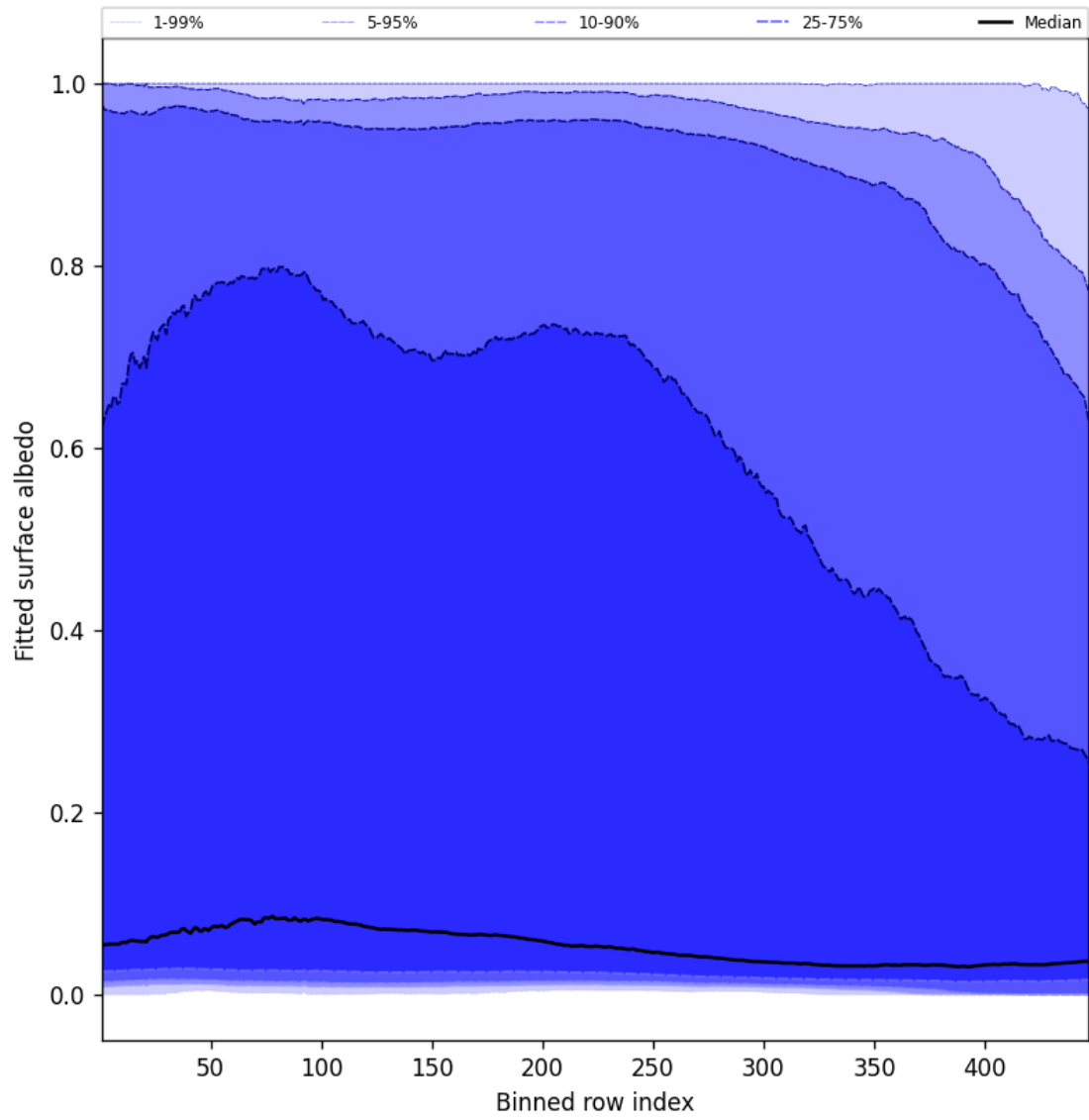
Figure 61: Along track statistics of “Fitted surface albedo” for 2024-12-16 to 2024-12-17
