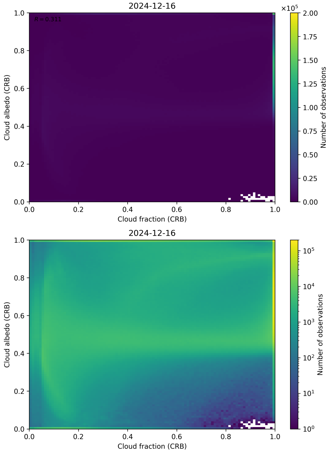
Figure 77: Scatter density plot of “Cloud fraction (CRB)” against “Cloud albedo (CRB)” for 2024-12-16 to 2024-12-17.
