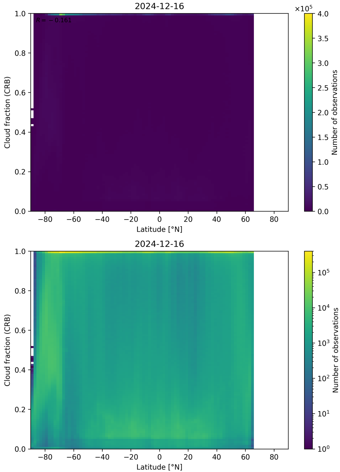
Figure 94: Scatter density plot of “Latitude” against “Cloud fraction (CRB)” for 2024-12-16 to 2024-12-17.
