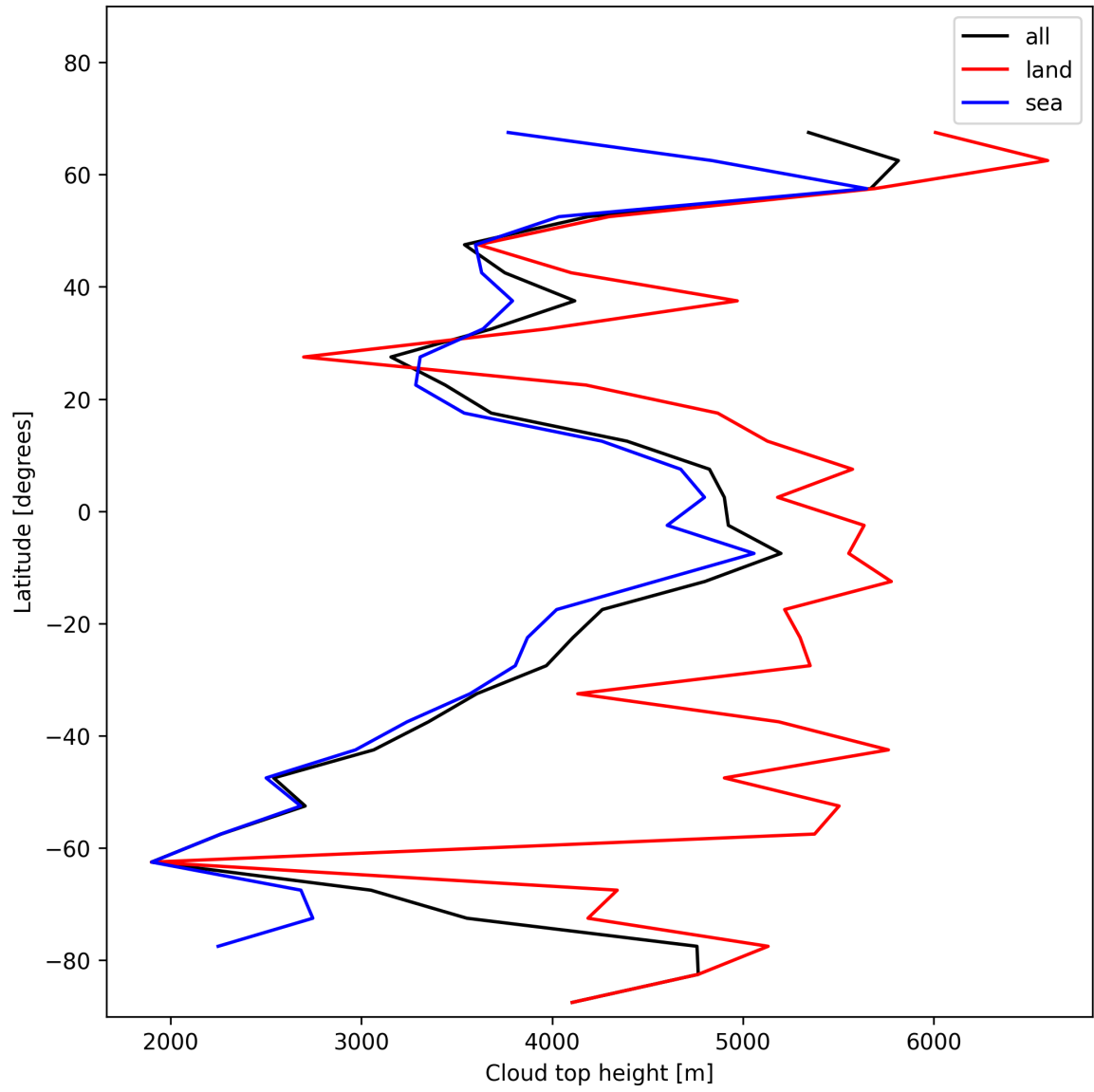
Figure 24: Zonal average of “Cloud top height” for 2024-12-16 to 2024-12-17.
