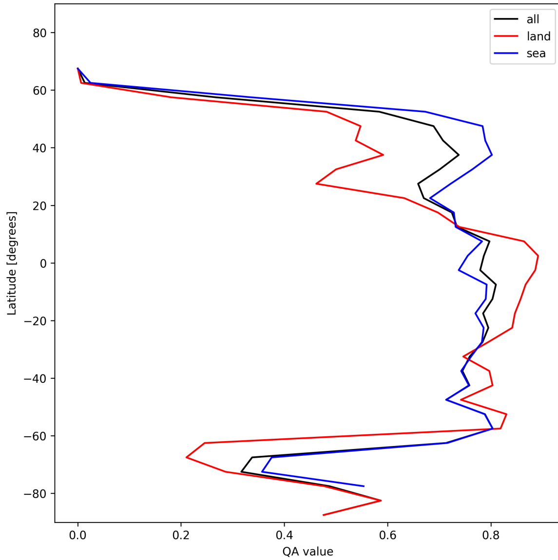
Figure 22: Zonal average of “QA value” for 2024-12-16 to 2024-12-17.
