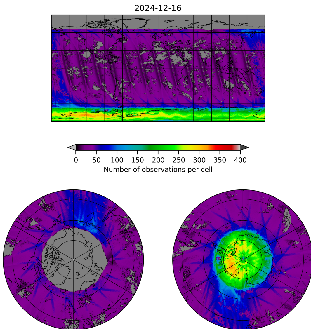
Figure 21: Map of the number of observations for 2024-12-16 to 2024-12-17
