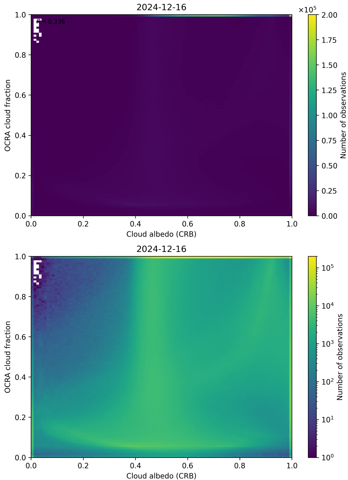
Figure 70: Scatter density plot of “Cloud albedo (CRB)” against “OCRA cloud fraction” for 2024-12-16 to 2024-12-17.
