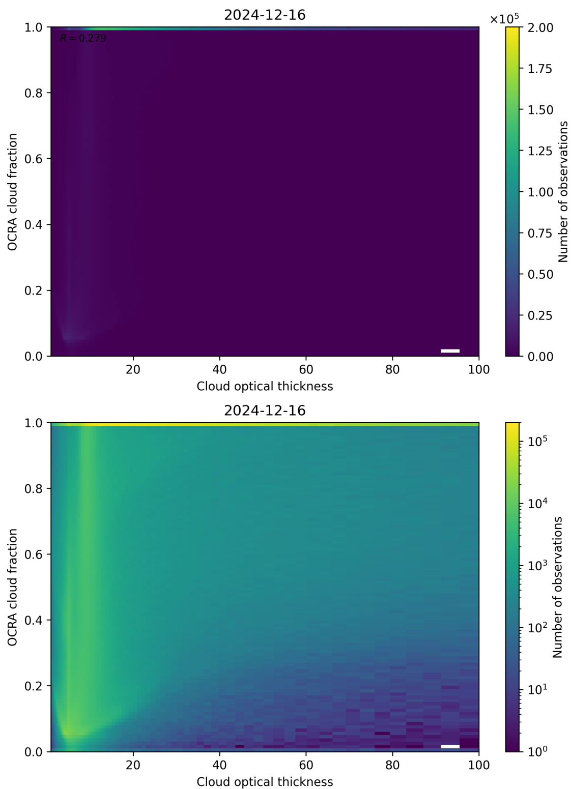
Figure 83: Scatter density plot of “Cloud optical thickness” against “OCRA cloud fraction” for 2024-12-16 to 2024-12-17.
