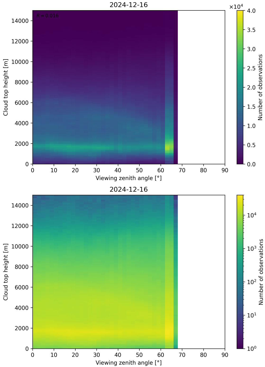
Figure 112: Scatter density plot of “Viewing zenith angle” against “Cloud top height” for 2024-12-16 to 2024-12-17.
