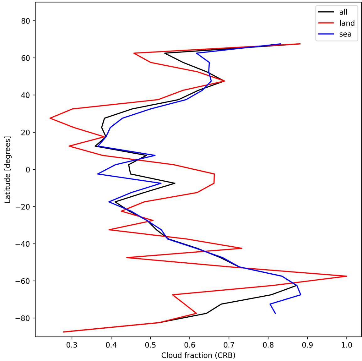
Figure 26: Zonal average of “Cloud fraction (CRB)” for 2024-12-16 to 2024-12-17.
