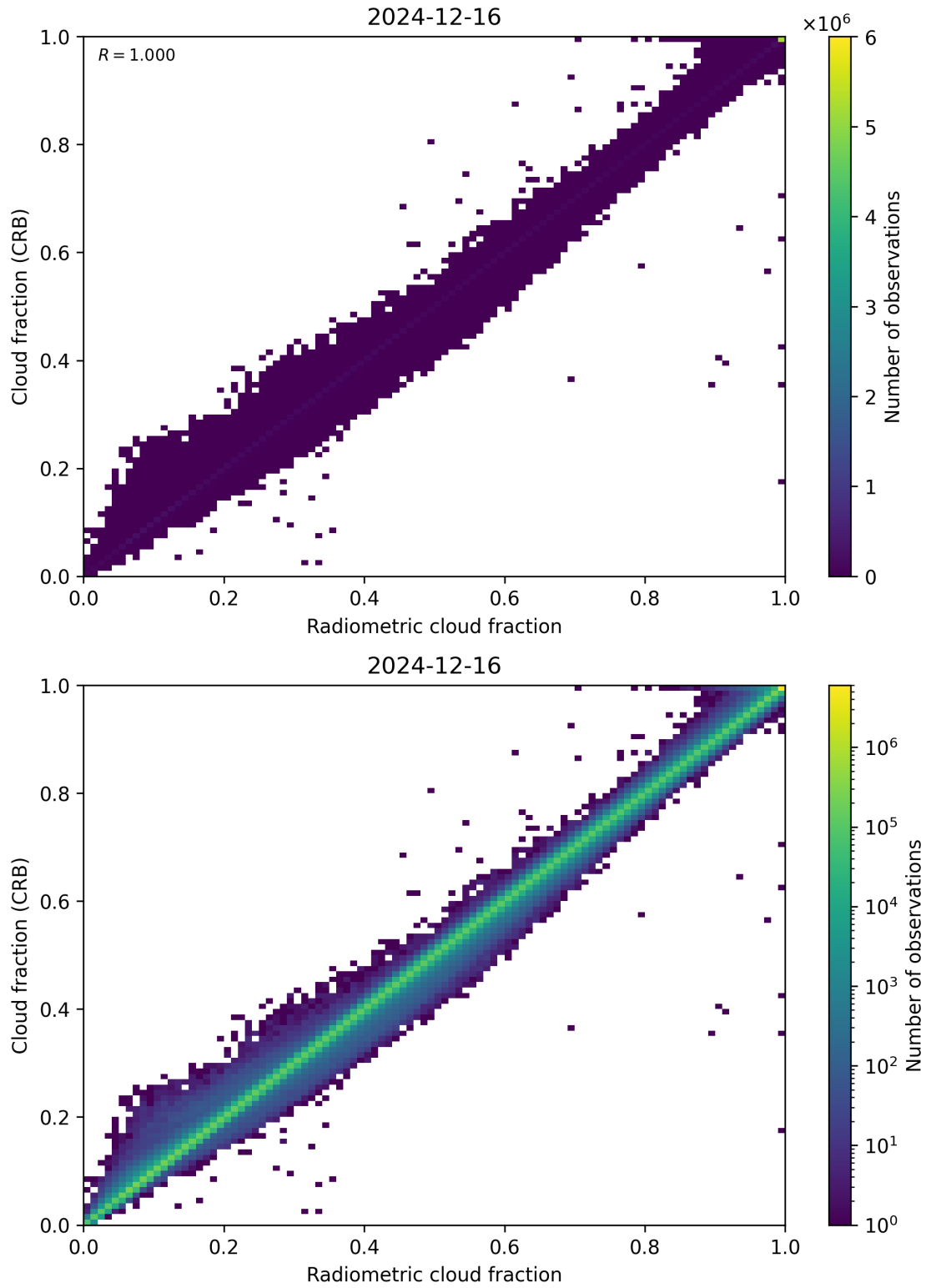
Figure 73: Scatter density plot of “Radiometric cloud fraction” against “Cloud fraction (CRB)” for 2024-12-16 to 2024-12-17.
