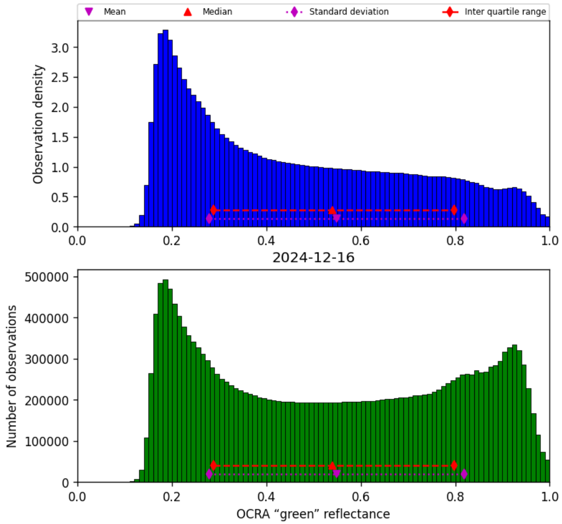
Figure 52: Histogram of “OCRA “green” reflectance” for 2024-12-16 to 2024-12-17
