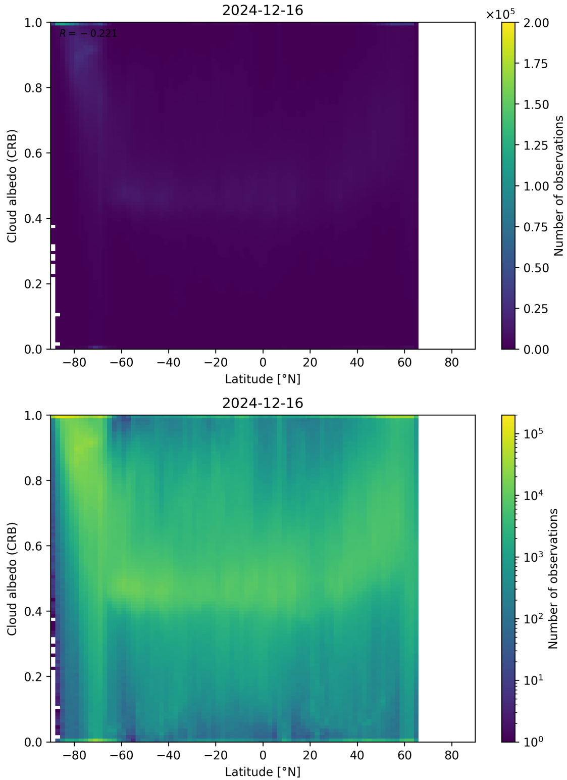
Figure 91: Scatter density plot of “Latitude” against “Cloud albedo (CRB)” for 2024-12-16 to 2024-12-17.
