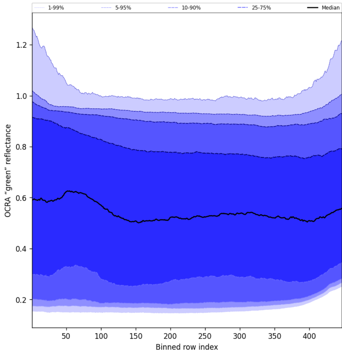
Figure 68: Along track statistics of “OCRA “green” reflectance” for 2024-12-16 to 2024-12-17
