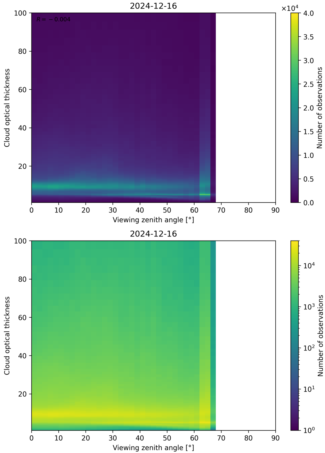
Figure 111: Scatter density plot of “Viewing zenith angle” against “Cloud optical thickness” for 2024-12-16 to 2024-12-17.
