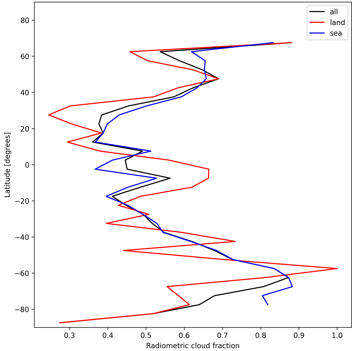
Figure 23: Zonal average of “Radiometric cloud fraction” for 2024-12-16 to 2024-12-17.
