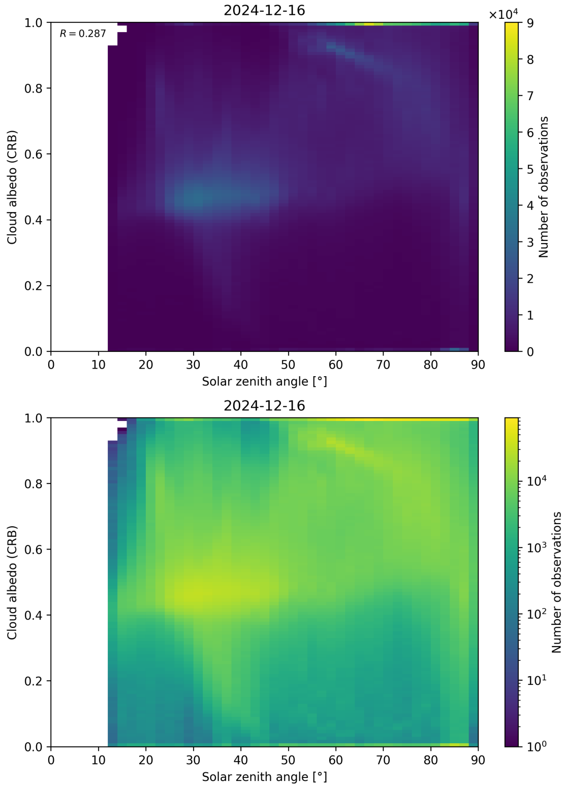
Figure 98: Scatter density plot of “Solar zenith angle” against “Cloud albedo (CRB)” for 2024-12-16 to 2024-12-17.
