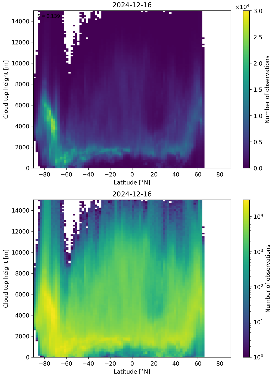
Figure 97: Scatter density plot of “Latitude” against “Cloud top height” for 2024-12-16 to 2024-12-17.
