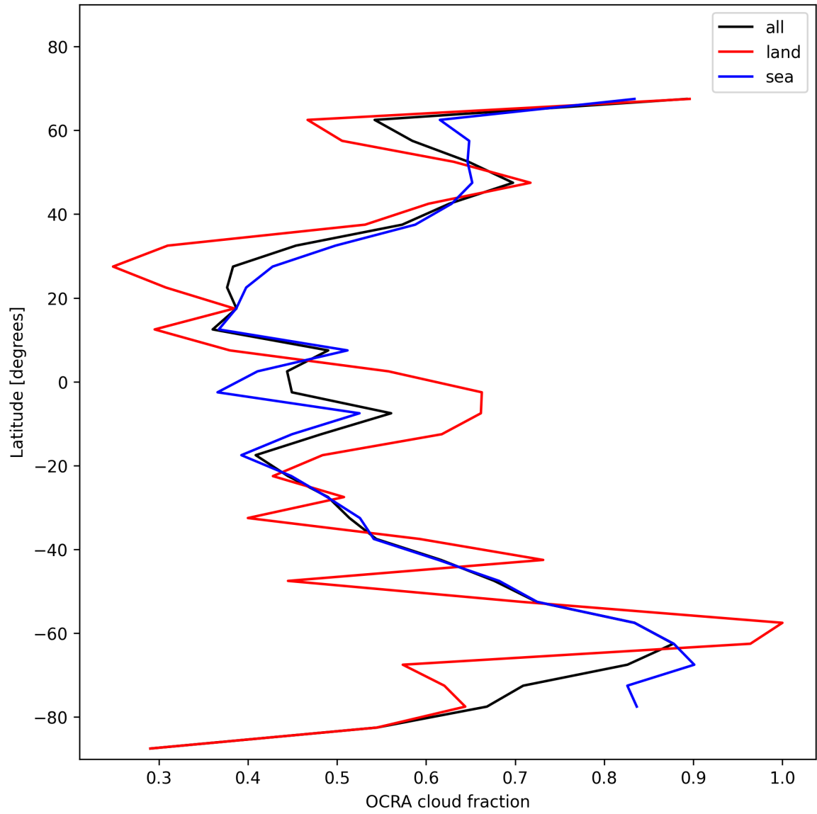
Figure 34: Zonal average of “OCRA cloud fraction” for 2024-12-16 to 2024-12-17.
