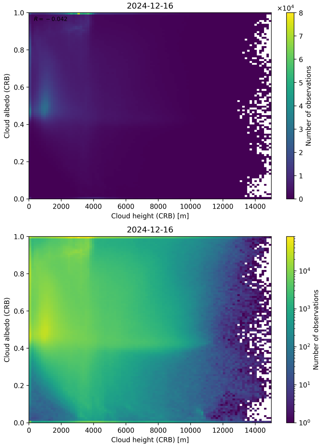
Figure 80: Scatter density plot of “Cloud height (CRB)” against “Cloud albedo (CRB)” for 2024-12-16 to 2024-12-17.
