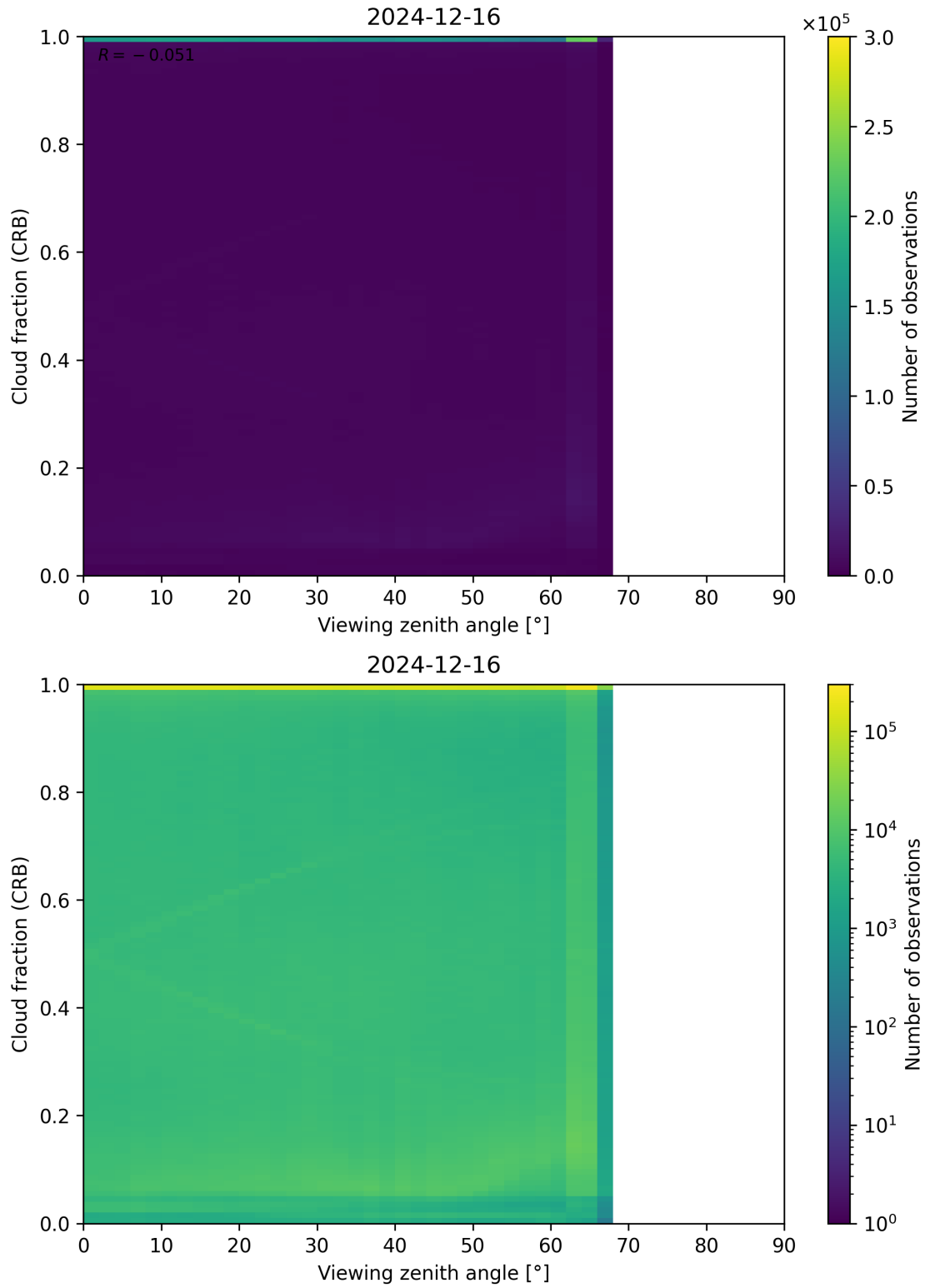
Figure 109: Scatter density plot of “Viewing zenith angle” against “Cloud fraction (CRB)” for 2024-12-16 to 2024-12-17.
