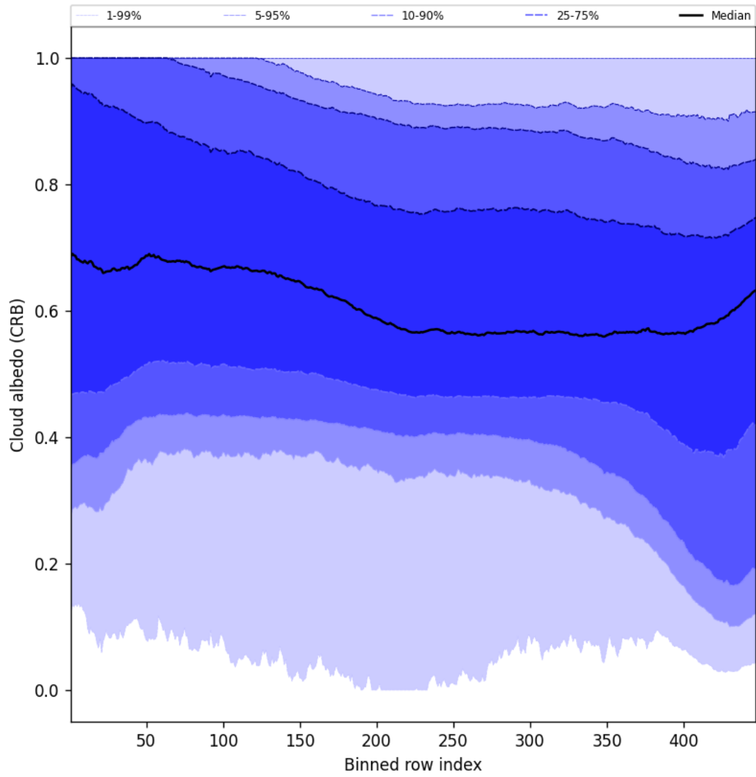
Figure 60: Along track statistics of “Cloud albedo (CRB)” for 2024-12-16 to 2024-12-17
