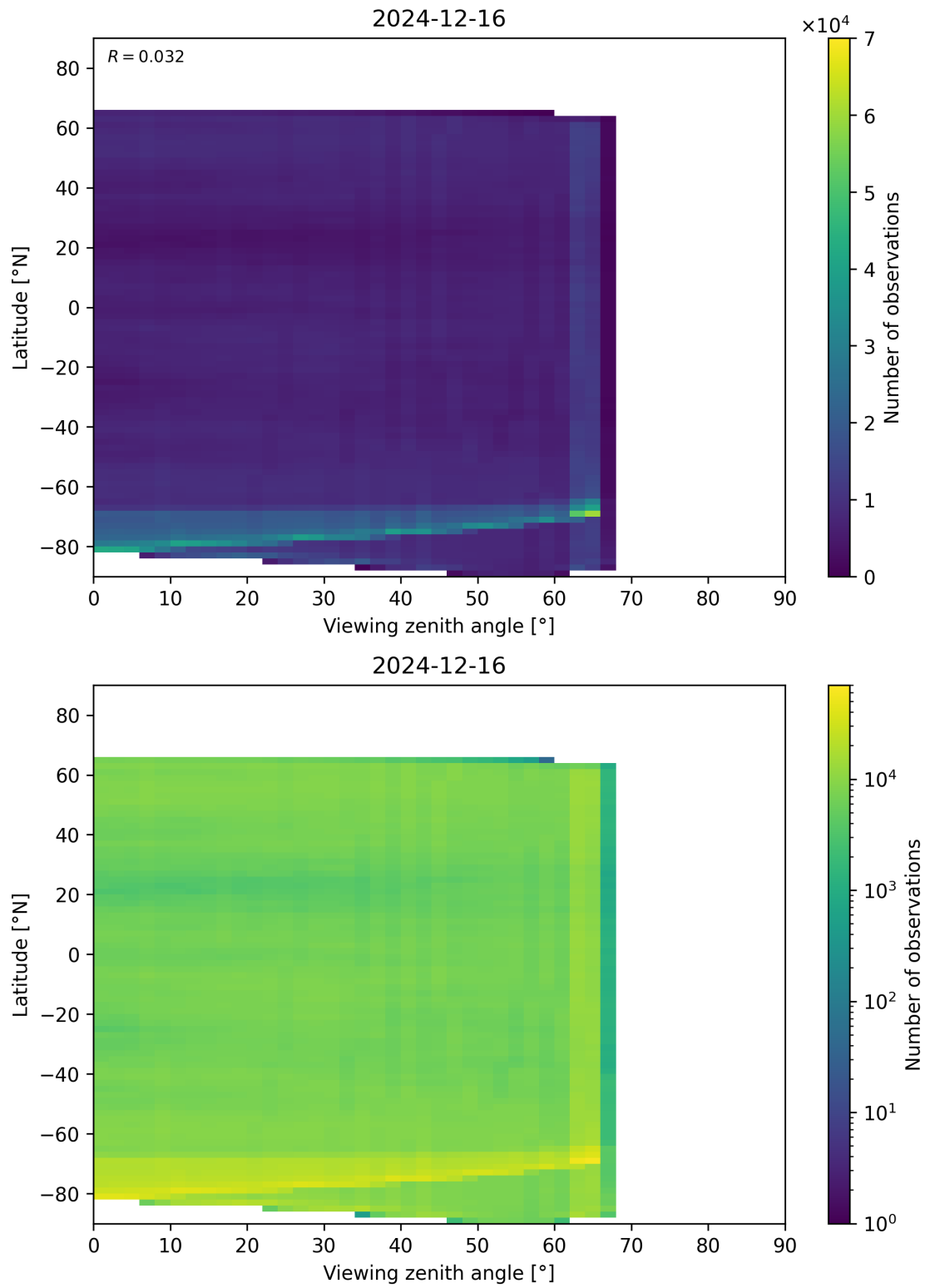
Figure 113: Scatter density plot of “Viewing zenith angle” against “Latitude” for 2024-12-16 to 2024-12-17.
