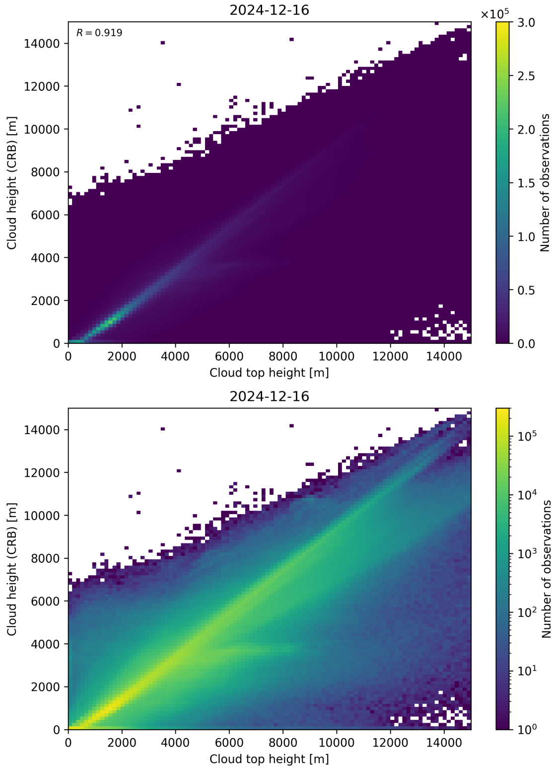
Figure 89: Scatter density plot of “Cloud top height” against “Cloud height (CRB)” for 2024-12-16 to 2024-12-17.
