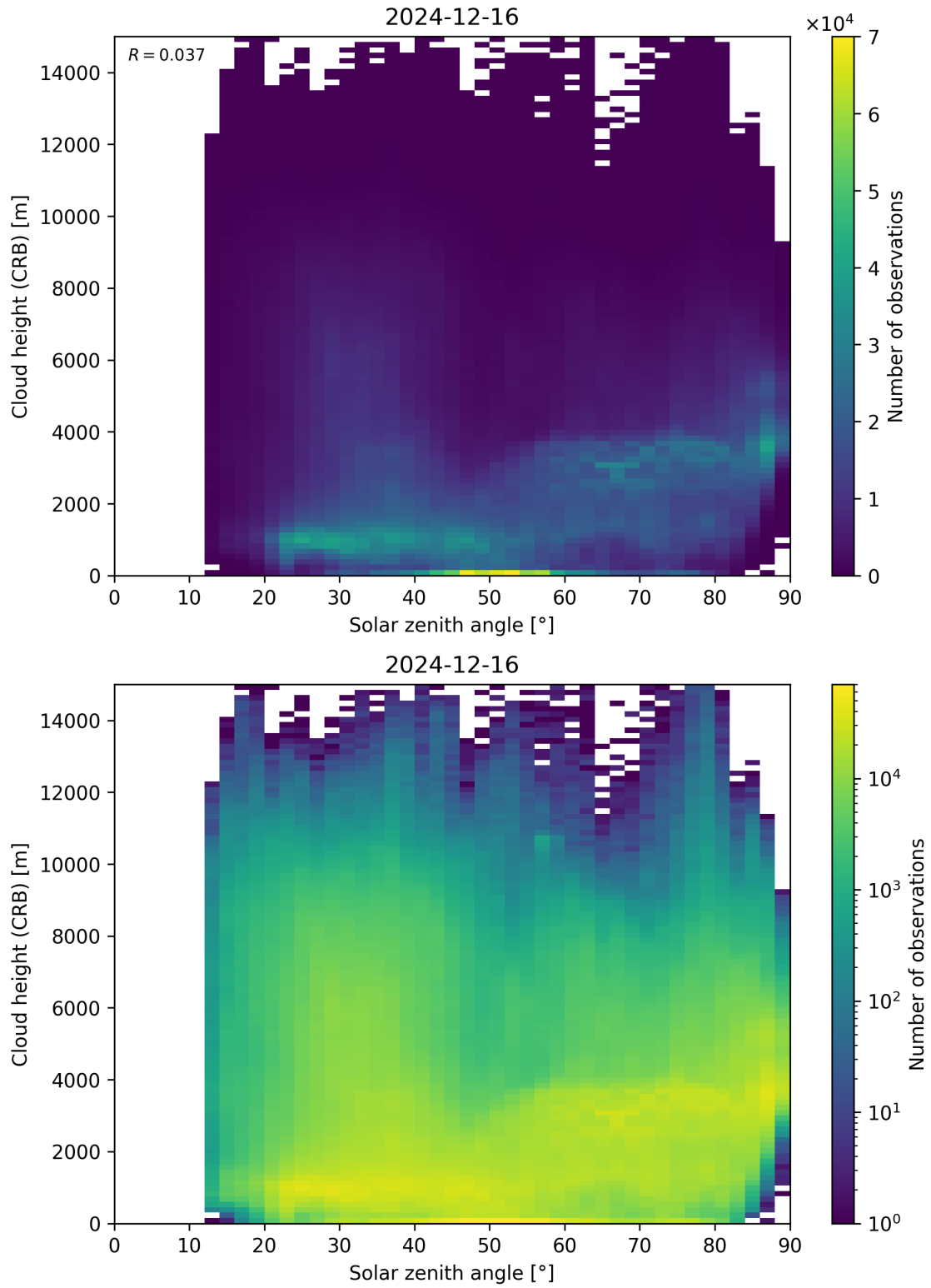
Figure 102: Scatter density plot of “Solar zenith angle” against “Cloud height (CRB)” for 2024-12-16 to 2024-12-17.
