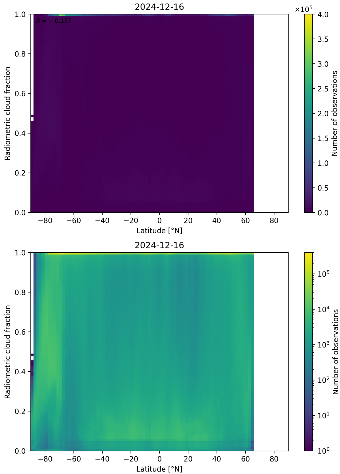
Figure 92: Scatter density plot of “Latitude” against “Radiometric cloud fraction” for 2024-12-16 to 2024-12-17.
