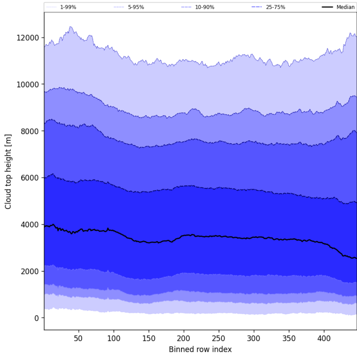
Figure 56: Along track statistics of “Cloud top height” for 2024-12-16 to 2024-12-17
