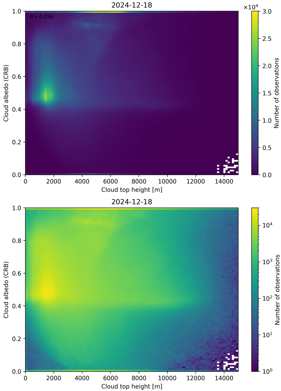
Figure 86: Scatter density plot of “Cloud top height” against “Cloud albedo (CRB)” for 2024-12-17 to 2024-12-19.
