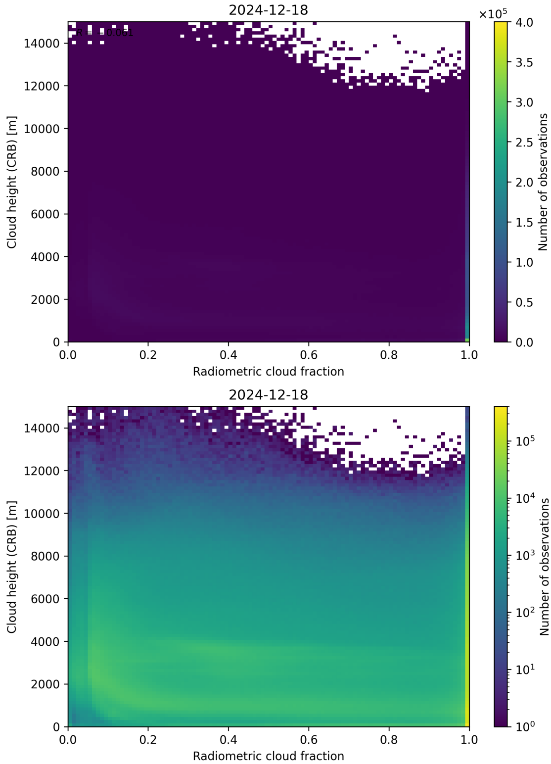
Figure 74: Scatter density plot of “Radiometric cloud fraction” against “Cloud height (CRB)” for 2024-12-17 to 2024-12-19.
