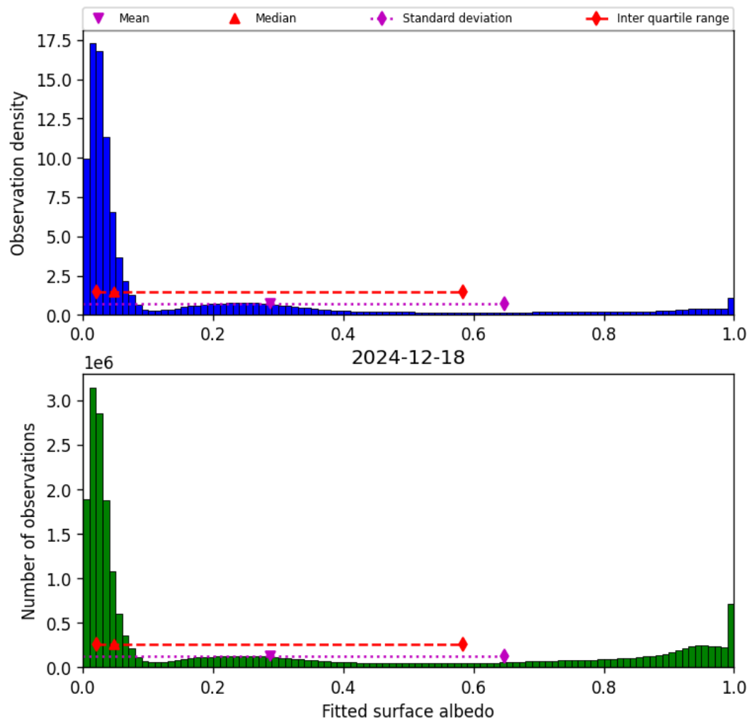
Figure 45: Histogram of “Fitted surface albedo” for 2024-12-17 to 2024-12-19
