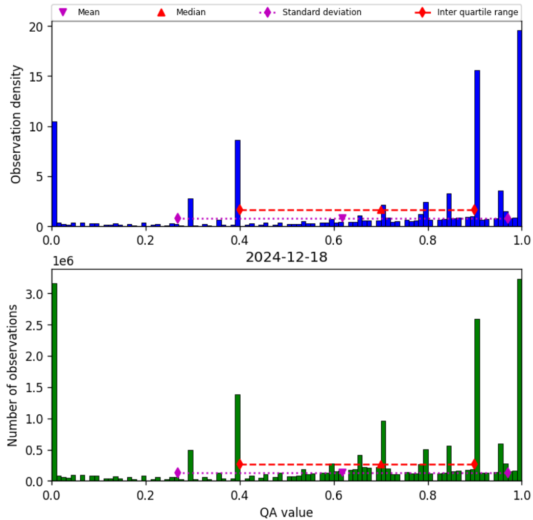
Figure 38: Histogram of “QA value” for 2024-12-17 to 2024-12-19
