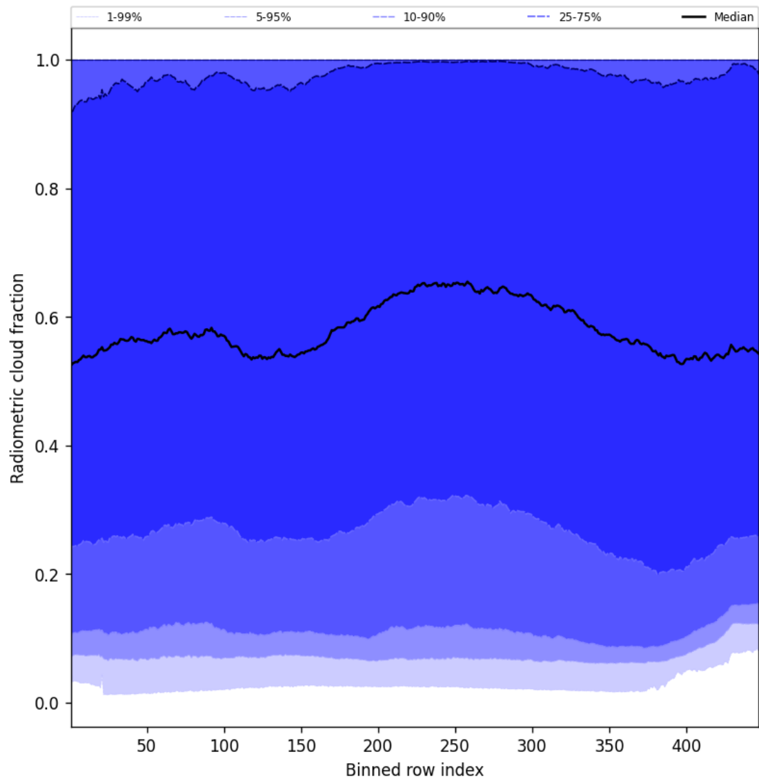
Figure 55: Along track statistics of “Radiometric cloud fraction” for 2024-12-17 to 2024-12-19
