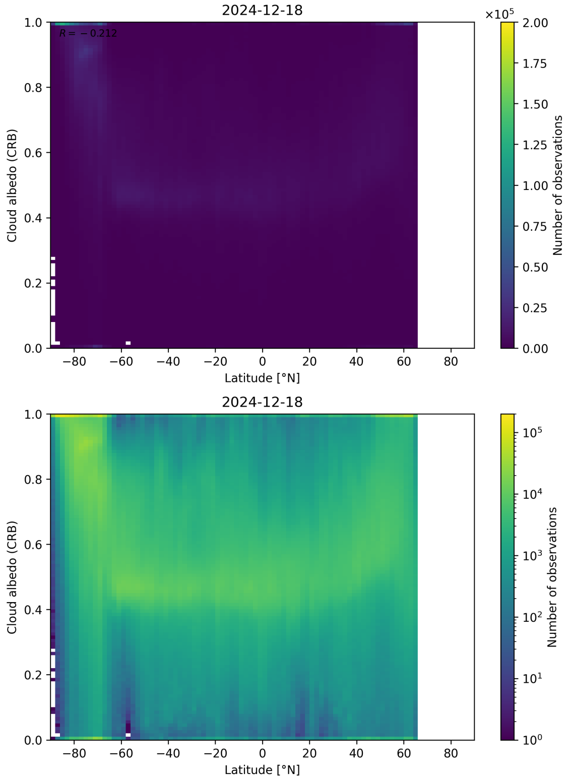
Figure 91: Scatter density plot of “Latitude” against “Cloud albedo (CRB)” for 2024-12-17 to 2024-12-19.
