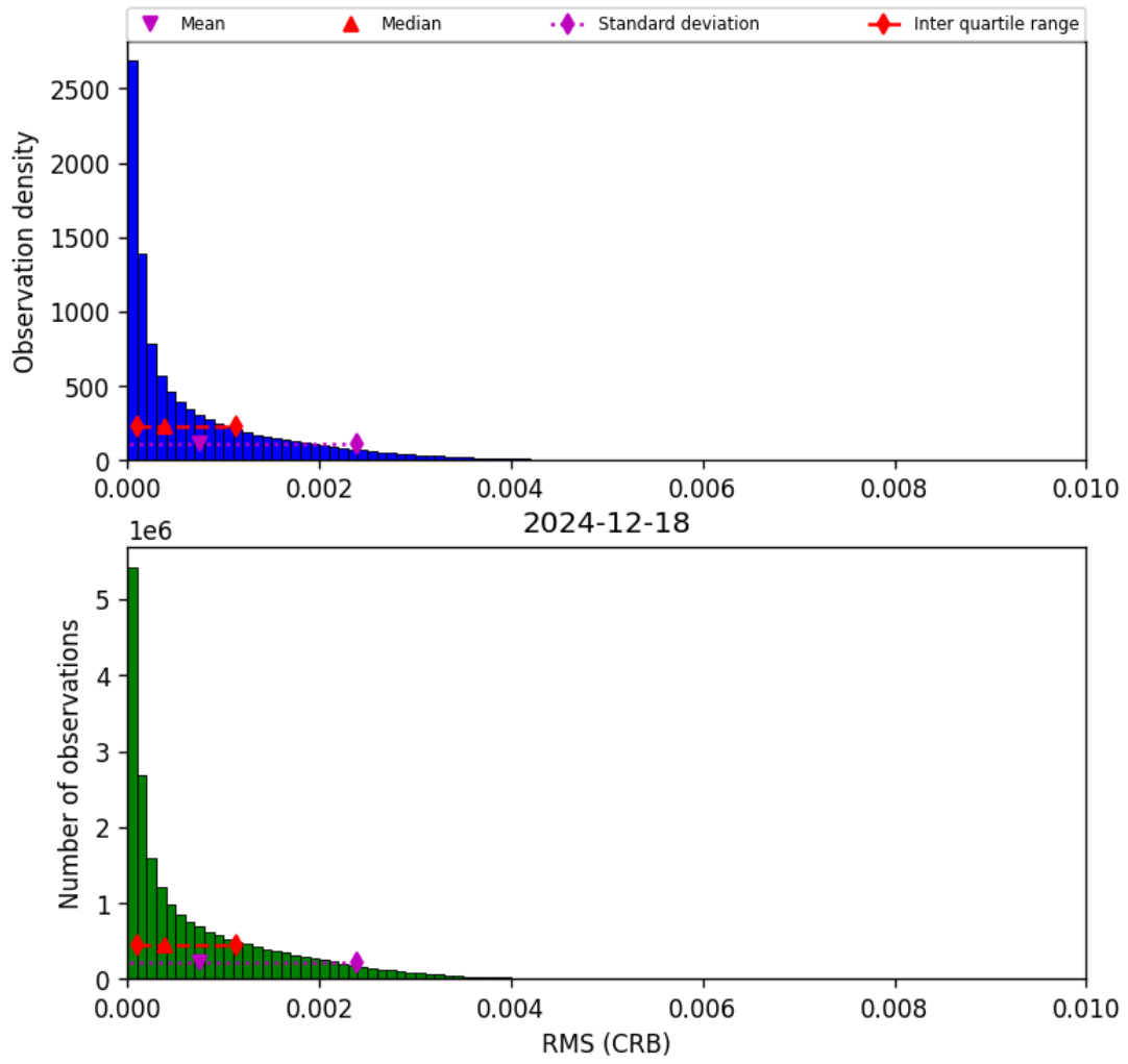
Figure 48: Histogram of “RMS (CRB)” for 2024-12-17 to 2024-12-19
