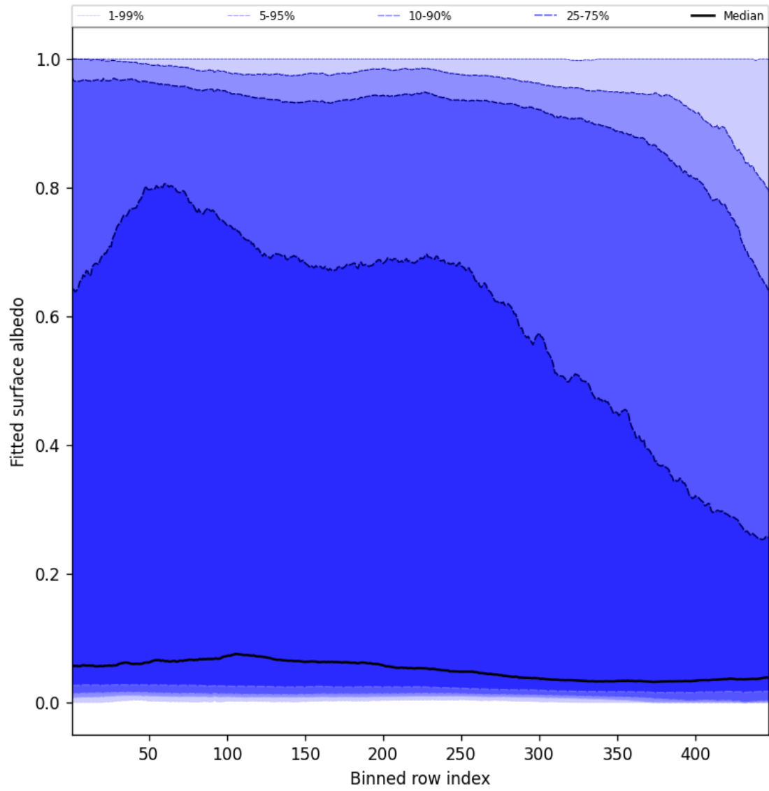
Figure 61: Along track statistics of “Fitted surface albedo” for 2024-12-17 to 2024-12-19
