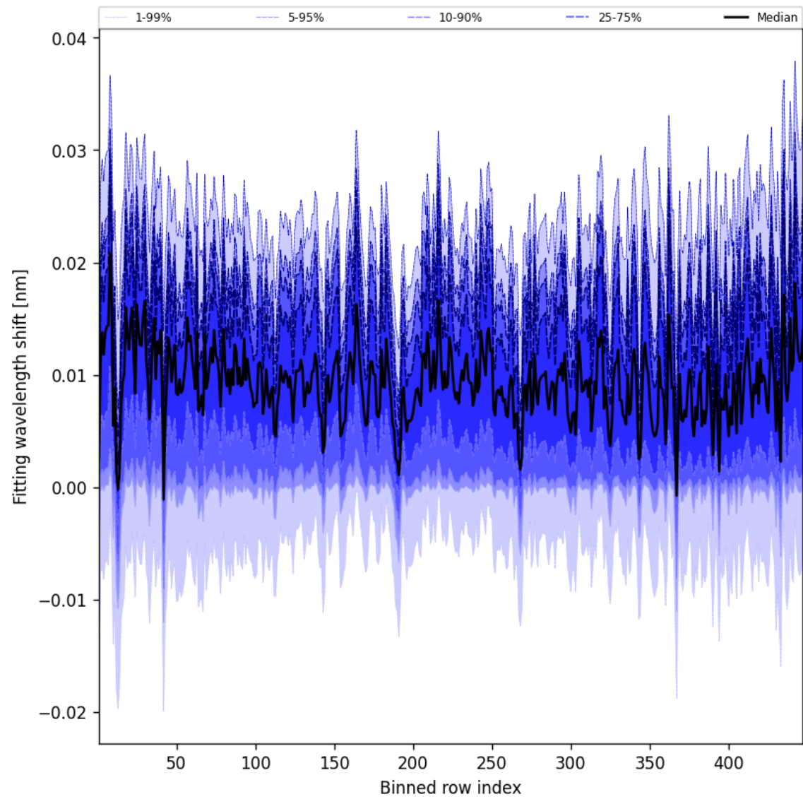
Figure 65: Along track statistics of “Fitting wavelength shift” for 2024-12-17 to 2024-12-19
