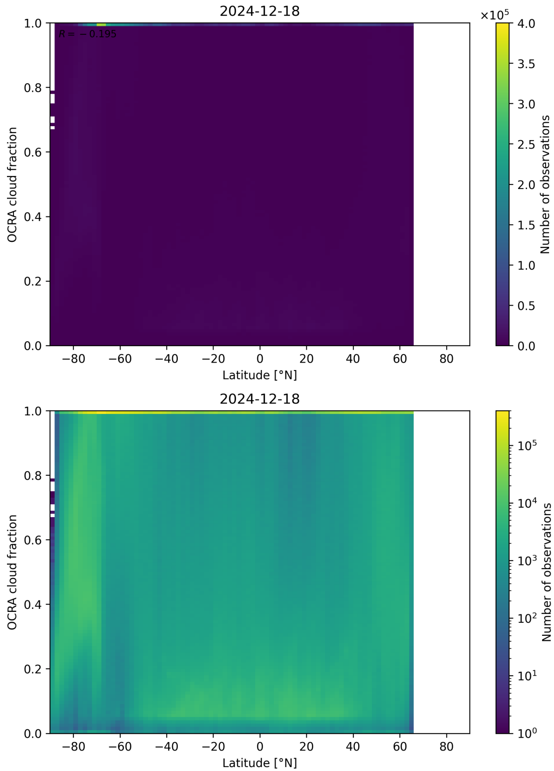
Figure 93: Scatter density plot of “Latitude” against “OCRA cloud fraction” for 2024-12-17 to 2024-12-19.
