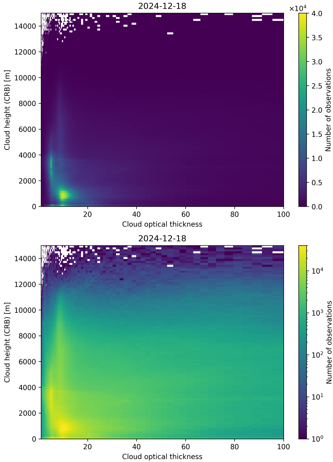
Figure 85: Scatter density plot of “Cloud optical thickness” against “Cloud height (CRB)” for 2024-12-17 to 2024-12-19.
