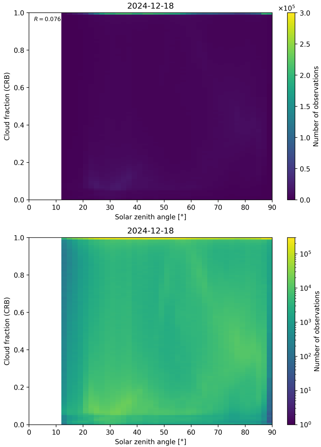
Figure 101: Scatter density plot of “Solar zenith angle” against “Cloud fraction (CRB)” for 2024-12-17 to 2024-12-19.
