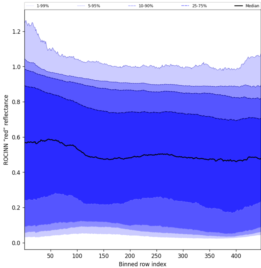
Figure 69: Along track statistics of “ROCINN “red” reflectance” for 2024-12-17 to 2024-12-19
