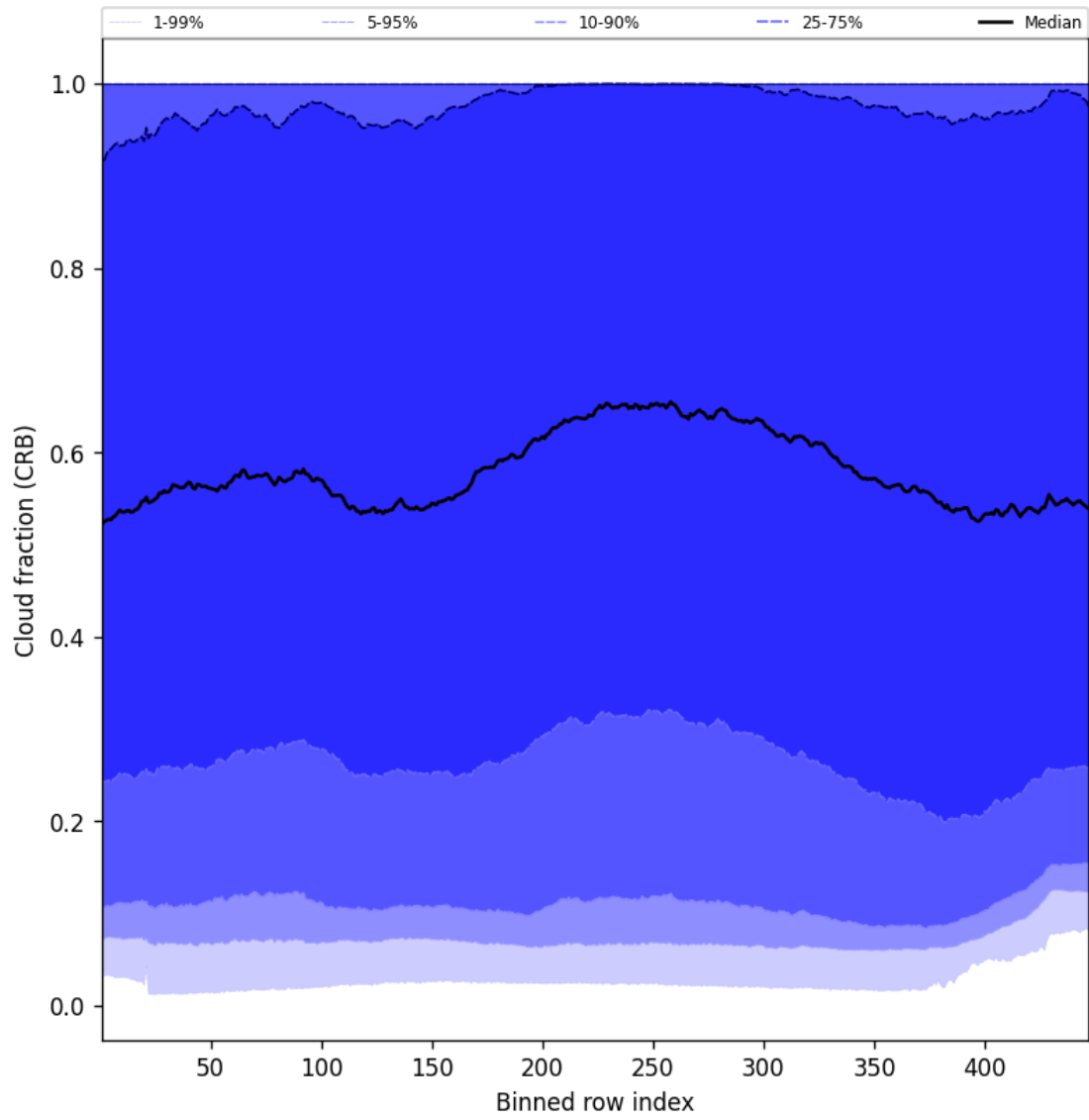
Figure 58: Along track statistics of “Cloud fraction (CRB)” for 2024-12-17 to 2024-12-19
