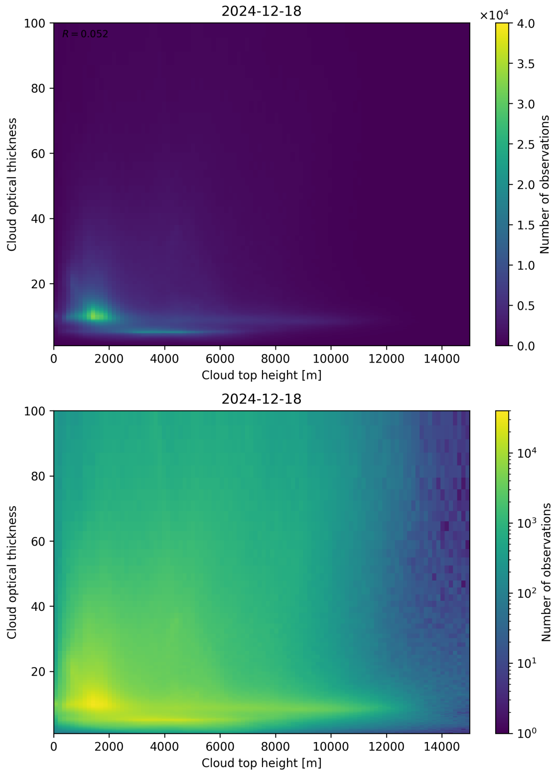
Figure 90: Scatter density plot of “Cloud top height” against “Cloud optical thickness” for 2024-12-17 to 2024-12-19.
