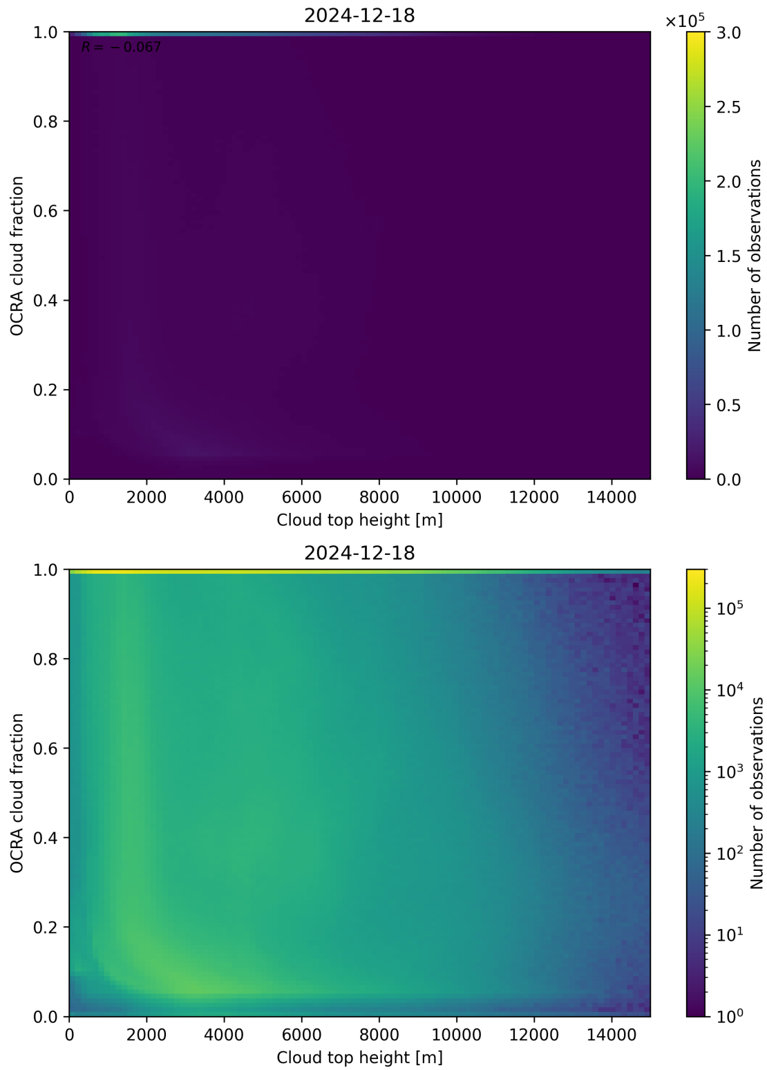
Figure 87: Scatter density plot of “Cloud top height” against “OCRA cloud fraction” for 2024-12-17 to 2024-12-19.
