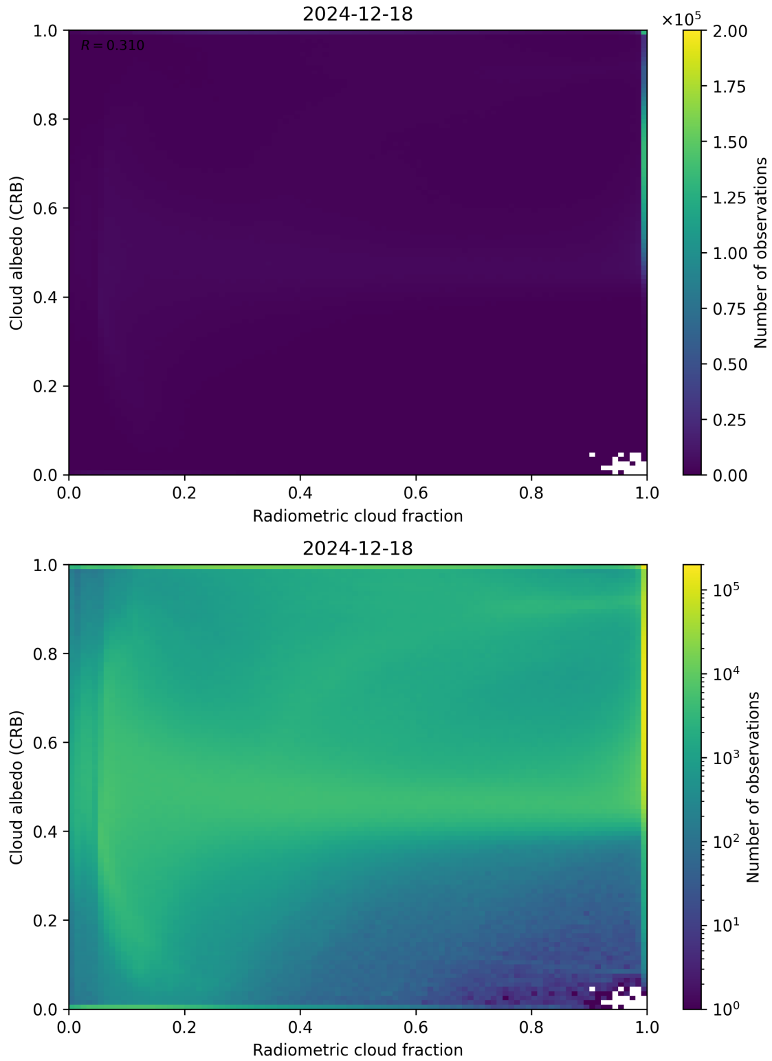
Figure 71: Scatter density plot of “Radiometric cloud fraction” against “Cloud albedo (CRB)” for 2024-12-17 to 2024-12-19.
