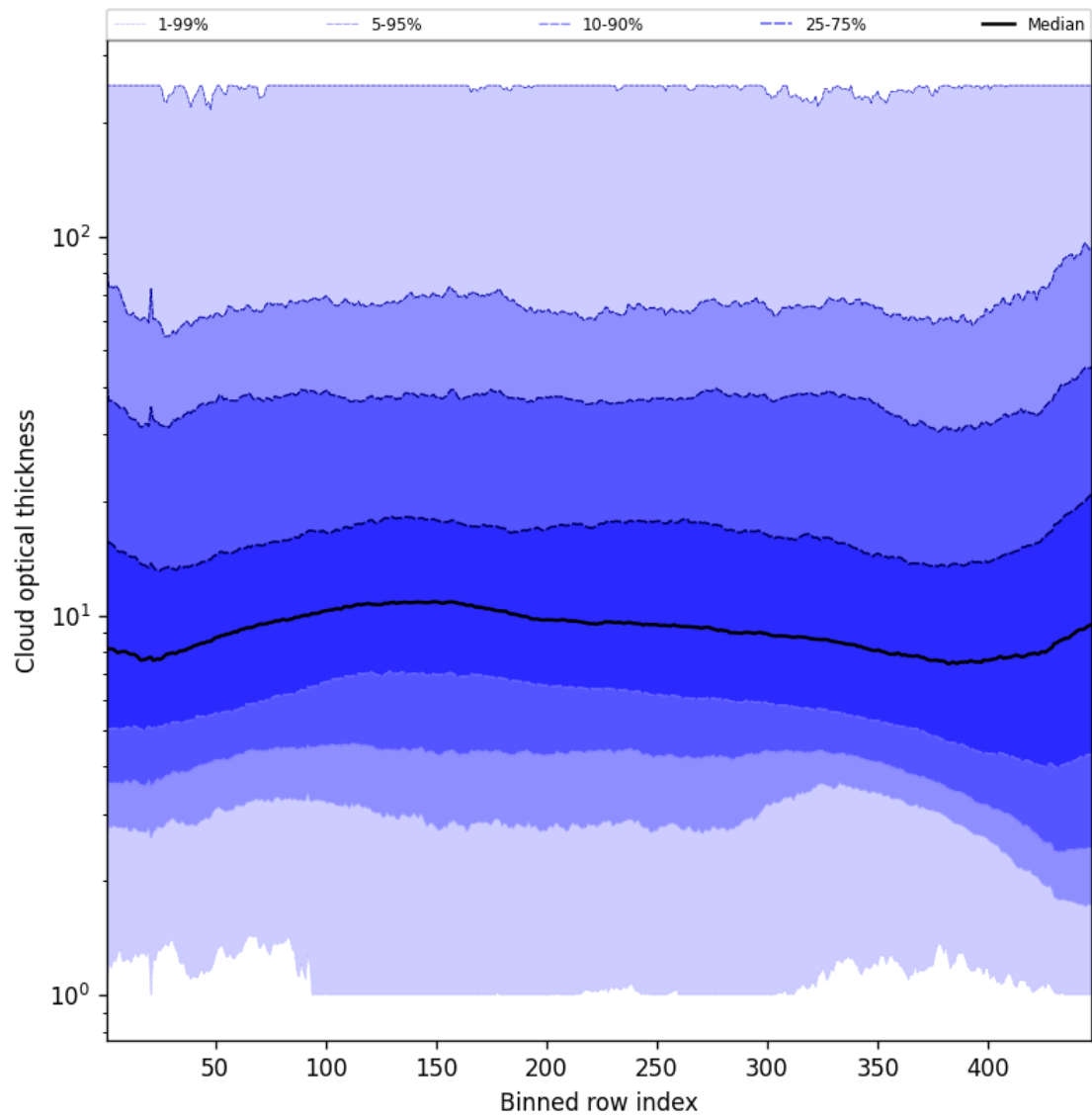
Figure 57: Along track statistics of “Cloud optical thickness” for 2024-12-17 to 2024-12-19
