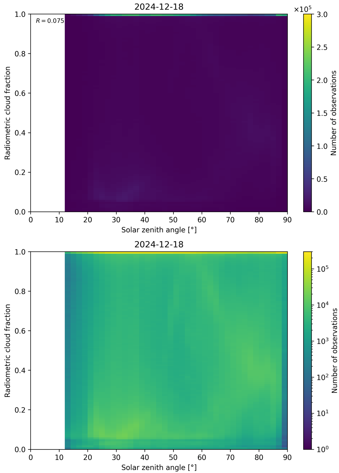
Figure 99: Scatter density plot of “Solar zenith angle” against “Radiometric cloud fraction” for 2024-12-17 to 2024-12-19.
