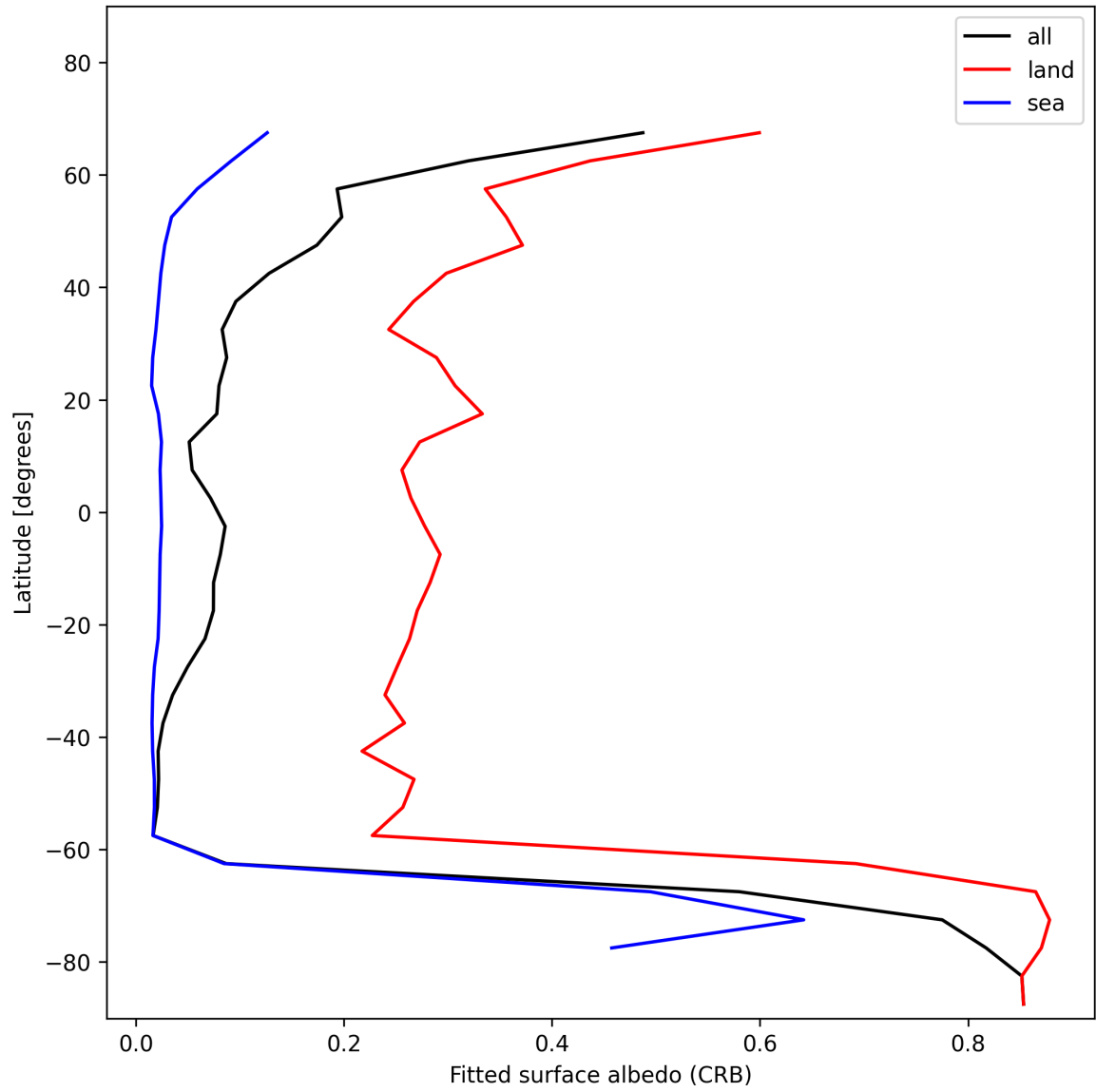
Figure 30: Zonal average of “Fitted surface albedo (CRB)” for 2024-12-17 to 2024-12-19.
