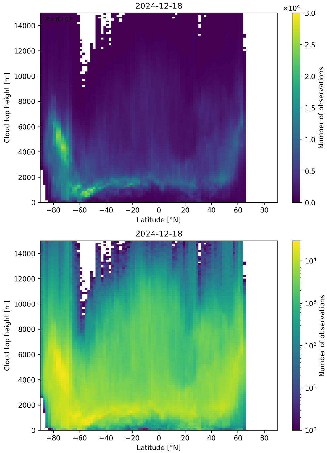
Figure 97: Scatter density plot of “Latitude” against “Cloud top height” for 2024-12-17 to 2024-12-19.
