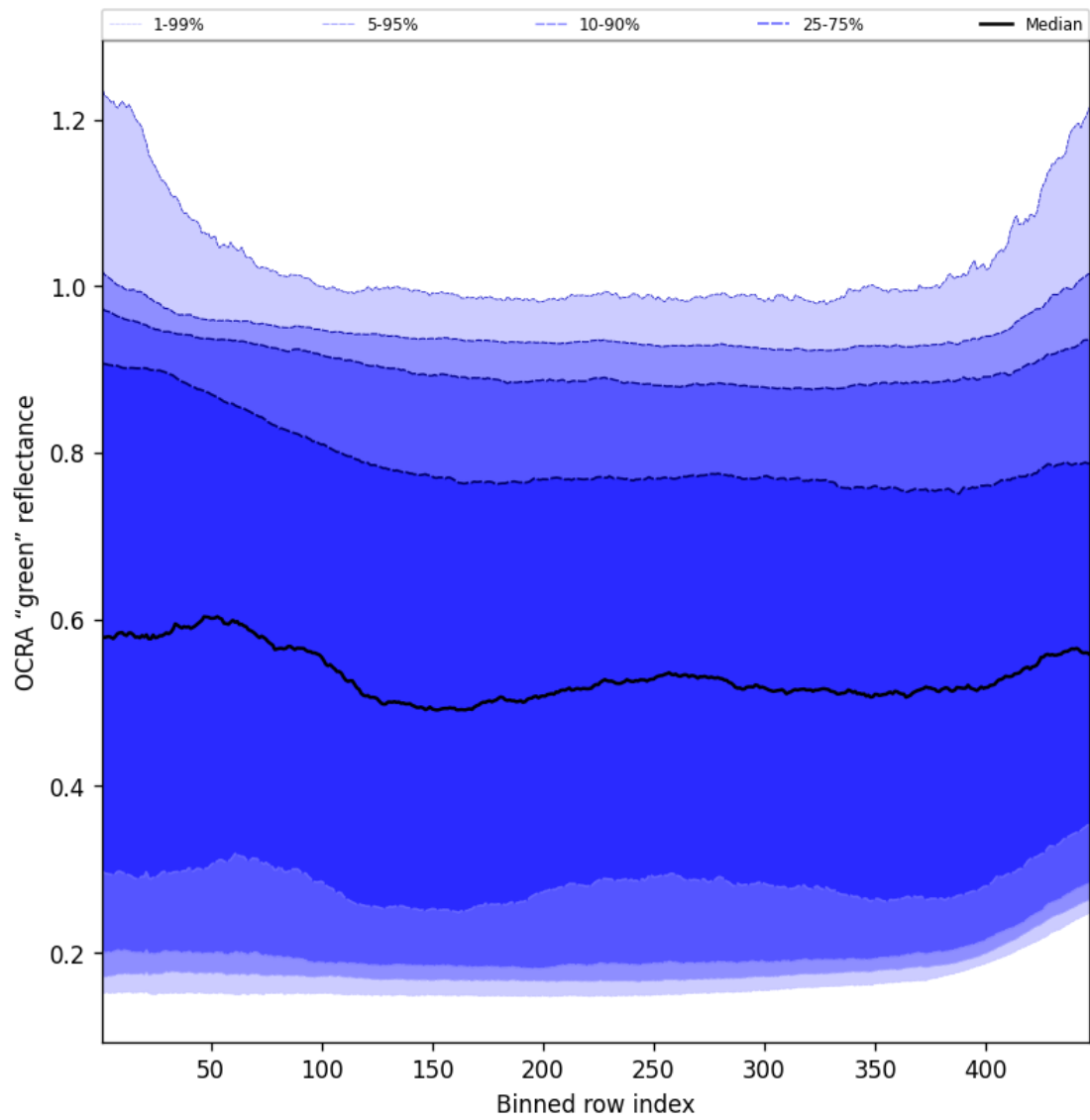
Figure 68: Along track statistics of "OCRA "green" reflectance" for 2024-12-17 to 2024-12-19
