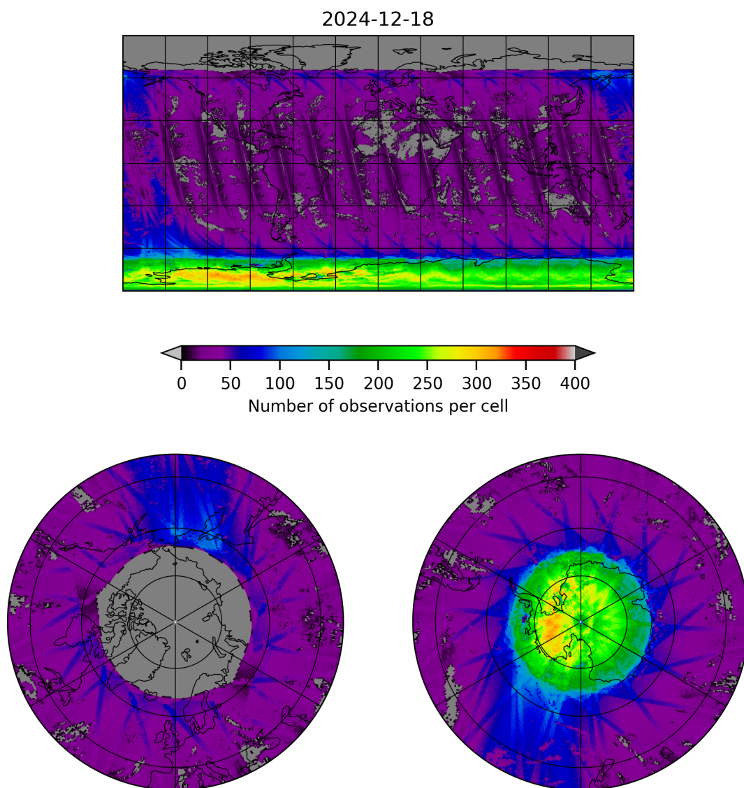
Figure 21: Map of the number of observations for 2024-12-17 to 2024-12-19
