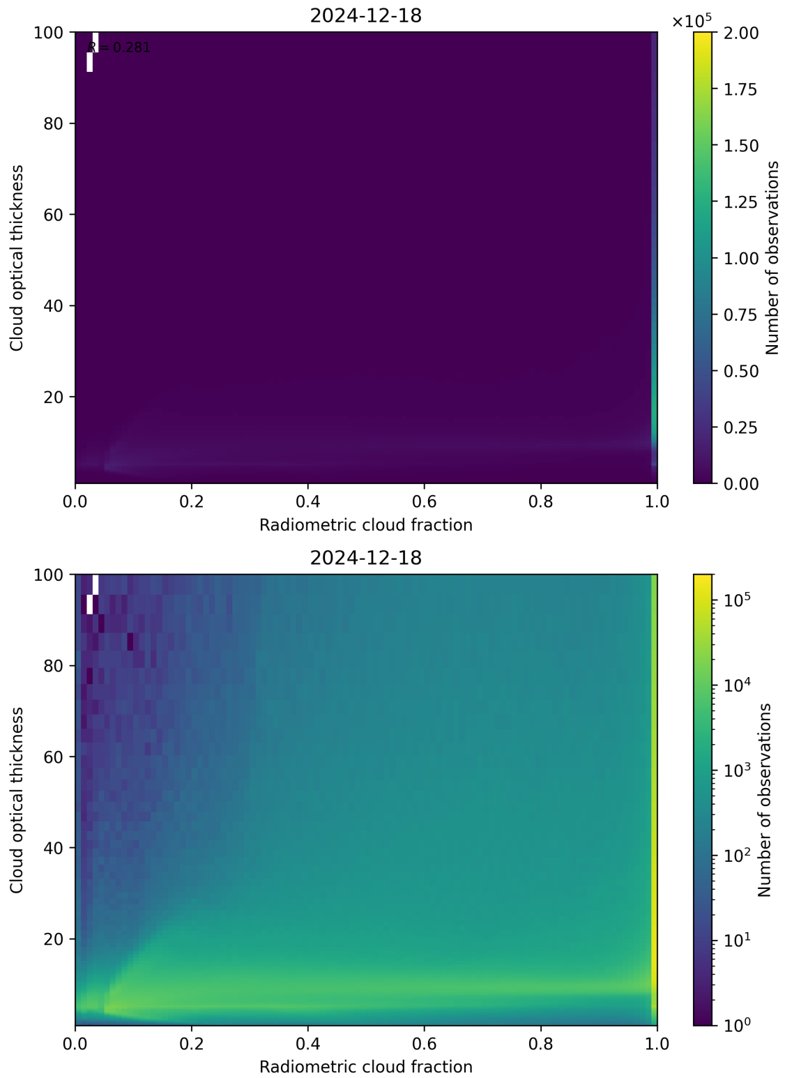
Figure 75: Scatter density plot of “Radiometric cloud fraction” against “Cloud optical thickness” for 2024-12-17 to 2024-12-19.
