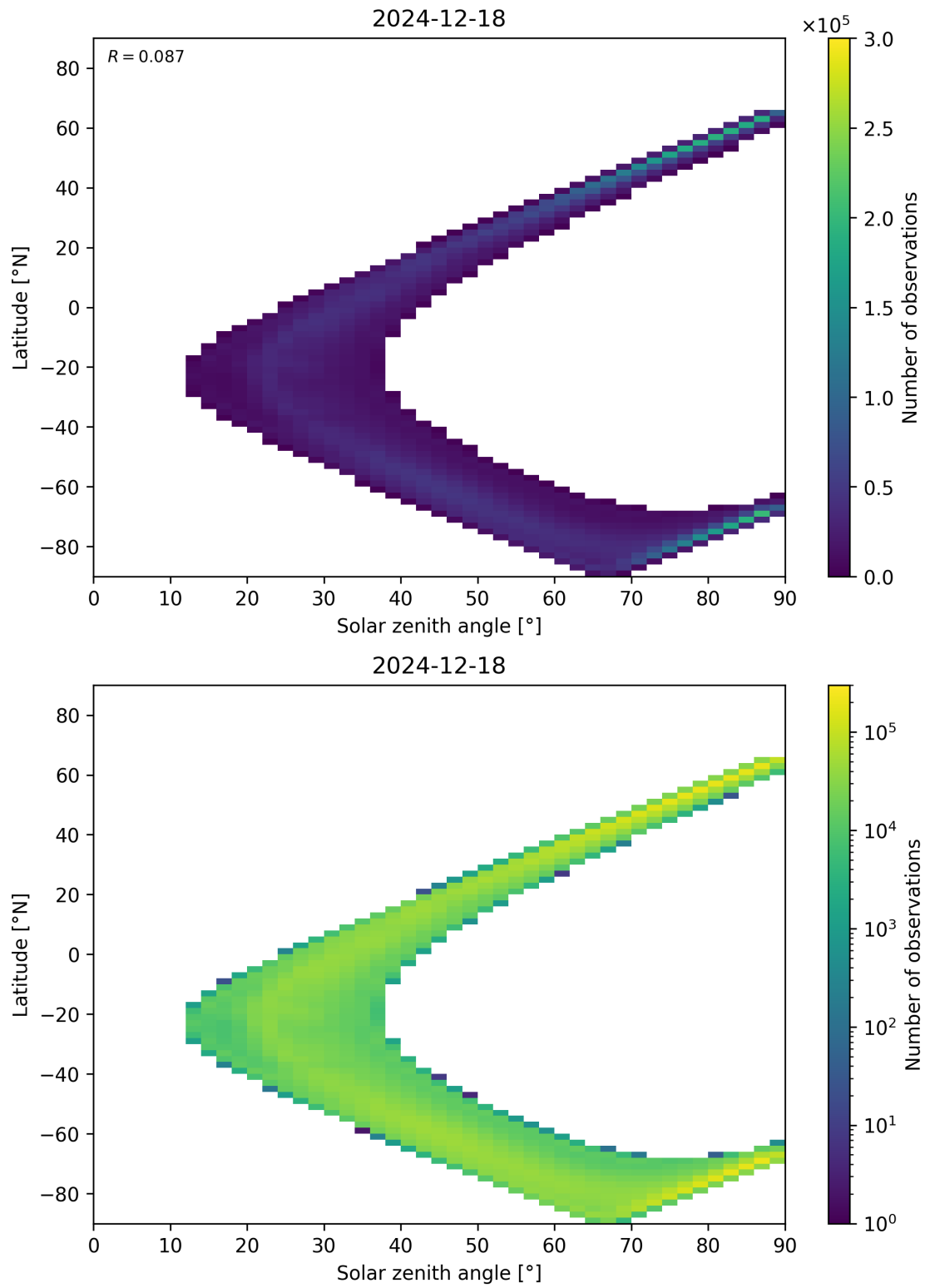
Figure 105: Scatter density plot of “Solar zenith angle” against “Latitude” for 2024-12-17 to 2024-12-19.
