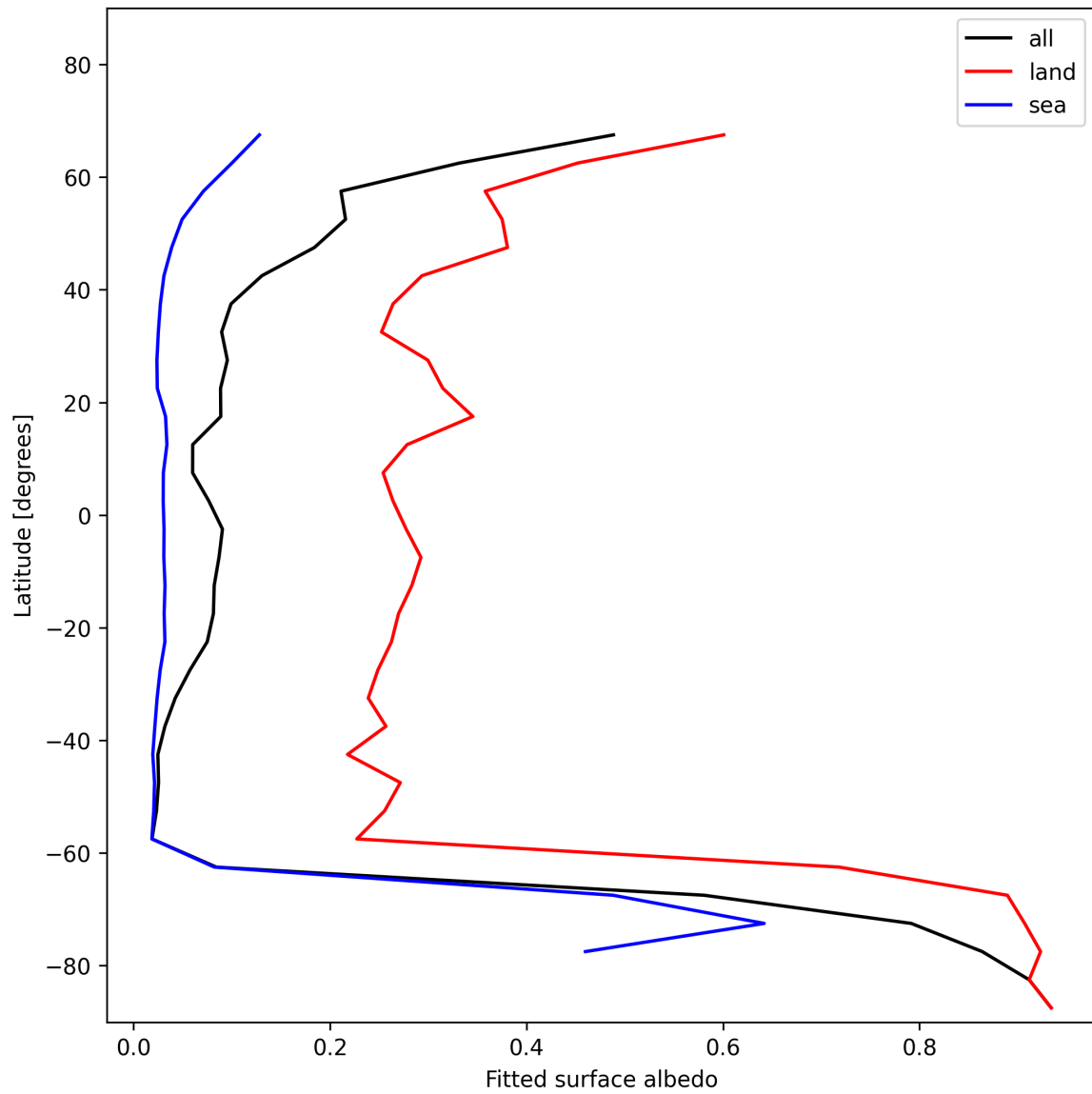
Figure 29: Zonal average of “Fitted surface albedo” for 2024-12-17 to 2024-12-19.
