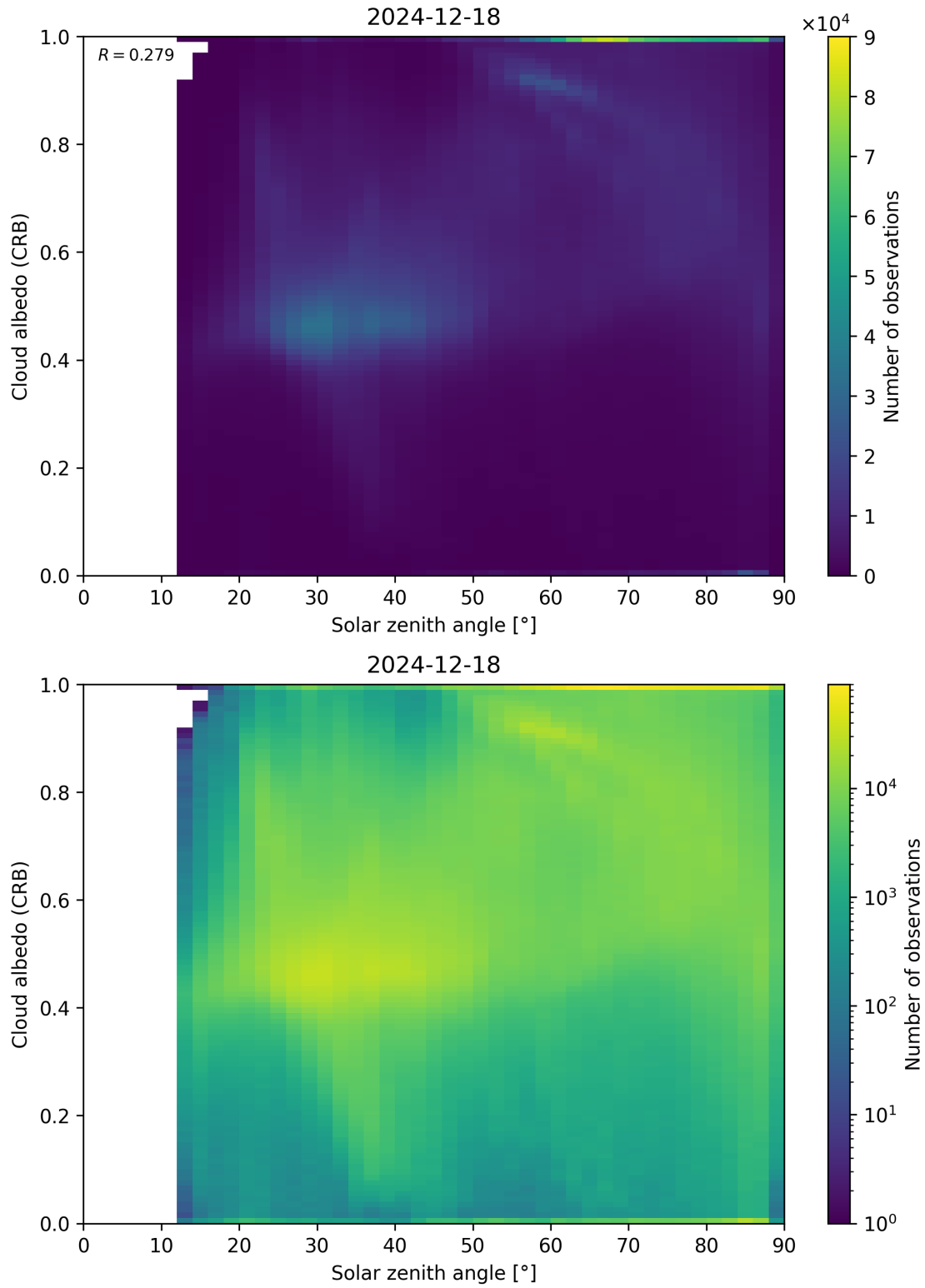
Figure 98: Scatter density plot of “Solar zenith angle” against “Cloud albedo (CRB)” for 2024-12-17 to 2024-12-19.
