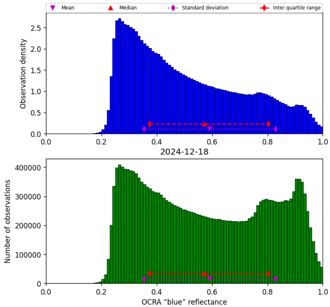
Figure 51: Histogram of "OCRA "blue" reflectance" for 2024-12-17 to 2024-12-19
