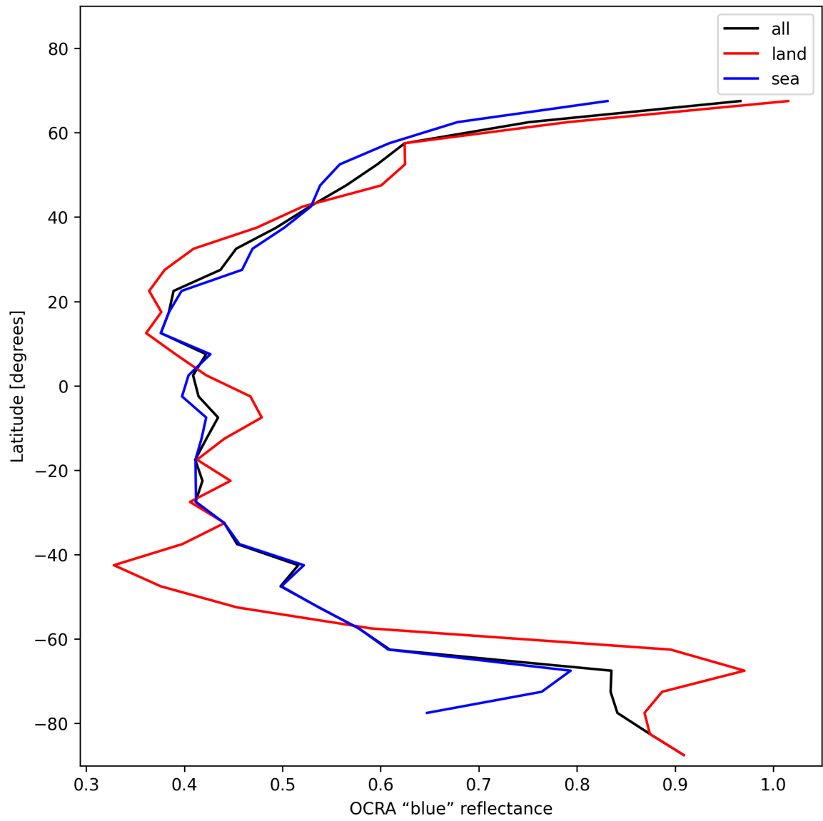
Figure 35: Zonal average of "OCRA "blue" reflectance" for 2024-12-17 to 2024-12-19.
