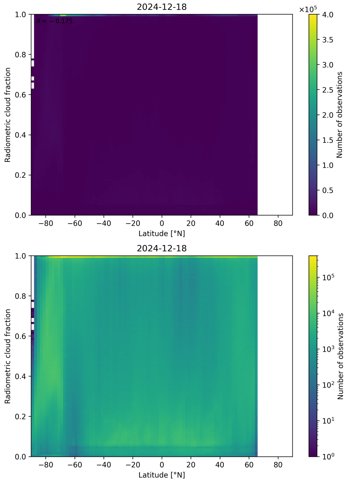
Figure 92: Scatter density plot of “Latitude” against “Radiometric cloud fraction” for 2024-12-17 to 2024-12-19.
