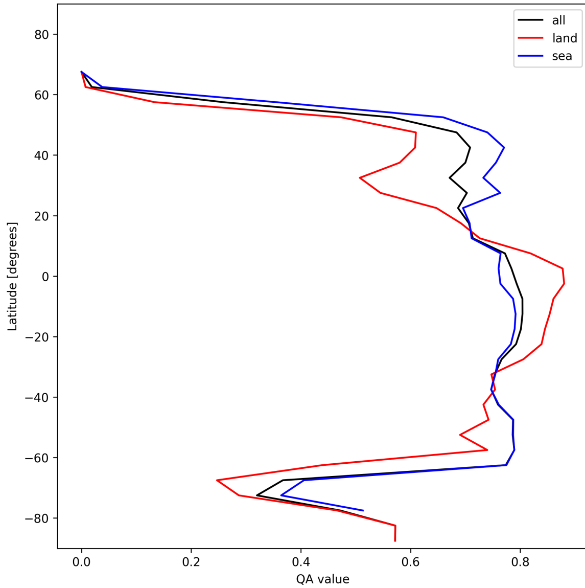
Figure 22: Zonal average of “QA value” for 2024-12-17 to 2024-12-19.
