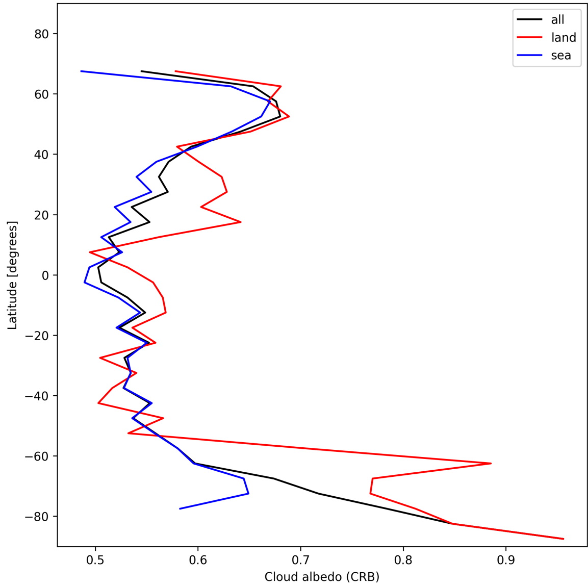
Figure 28: Zonal average of “Cloud albedo (CRB)” for 2024-12-17 to 2024-12-19.
