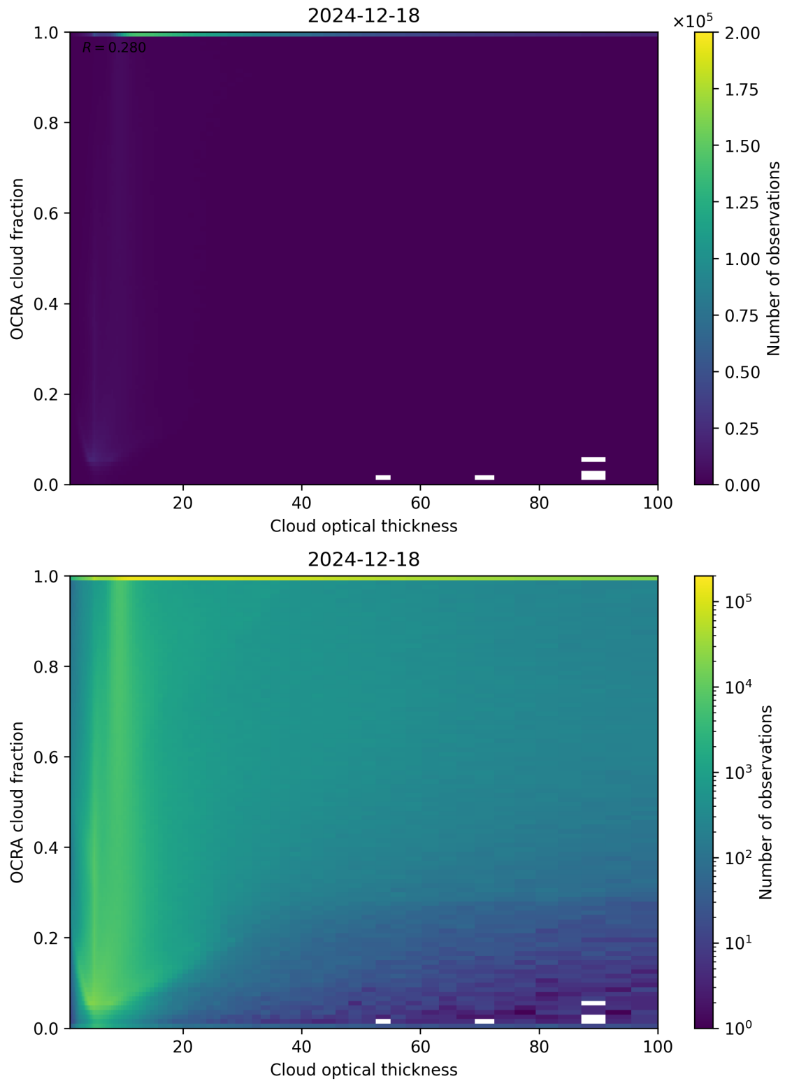
Figure 83: Scatter density plot of “Cloud optical thickness” against “OCRA cloud fraction” for 2024-12-17 to 2024-12-19.
