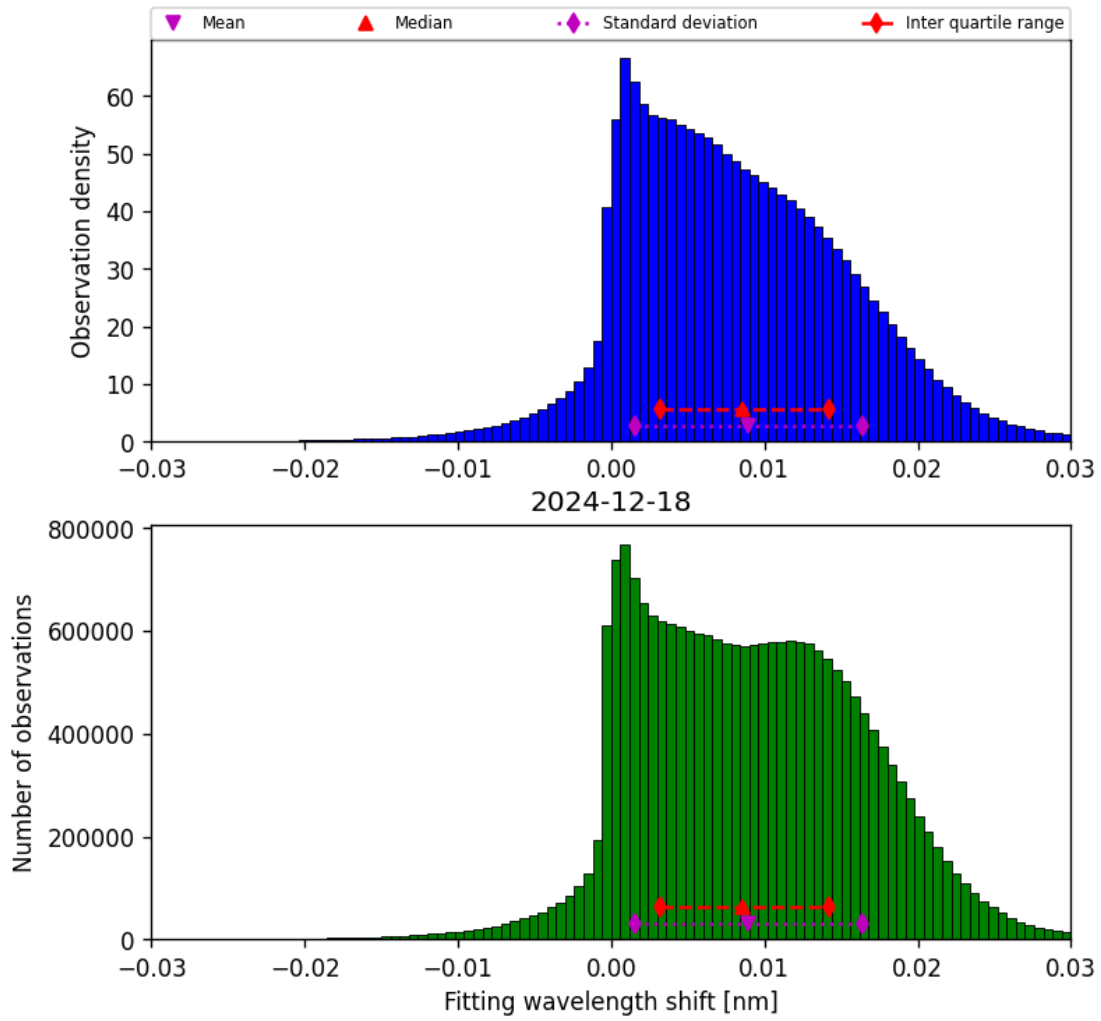
Figure 49: Histogram of “Fitting wavelength shift” for 2024-12-17 to 2024-12-19
