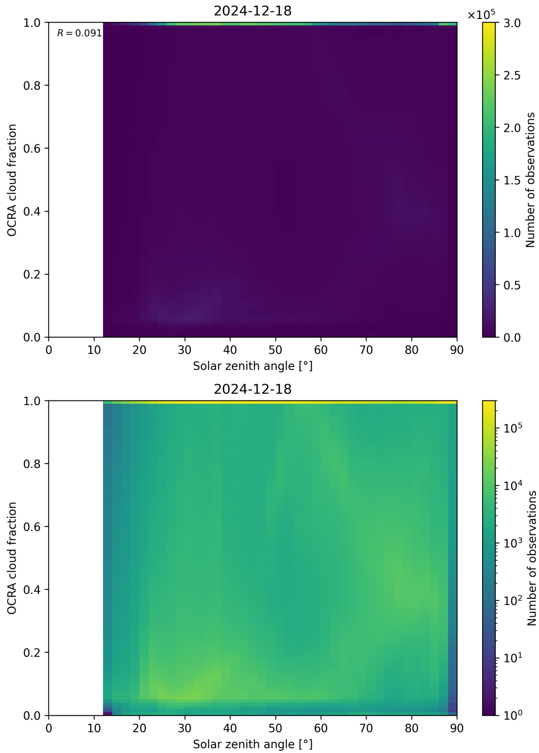
Figure 100: Scatter density plot of “Solar zenith angle” against “OCRA cloud fraction” for 2024-12-17 to 2024-12-19.
