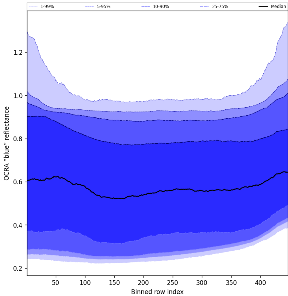
Figure 67: Along track statistics of "OCRA "blue" reflectance" for 2024-12-17 to 2024-12-19
