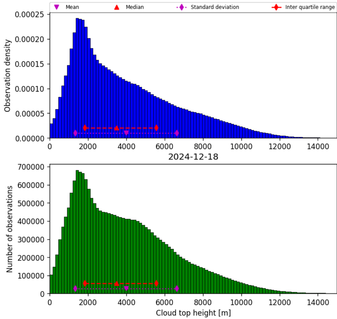
Figure 40: Histogram of “Cloud top height” for 2024-12-17 to 2024-12-19
