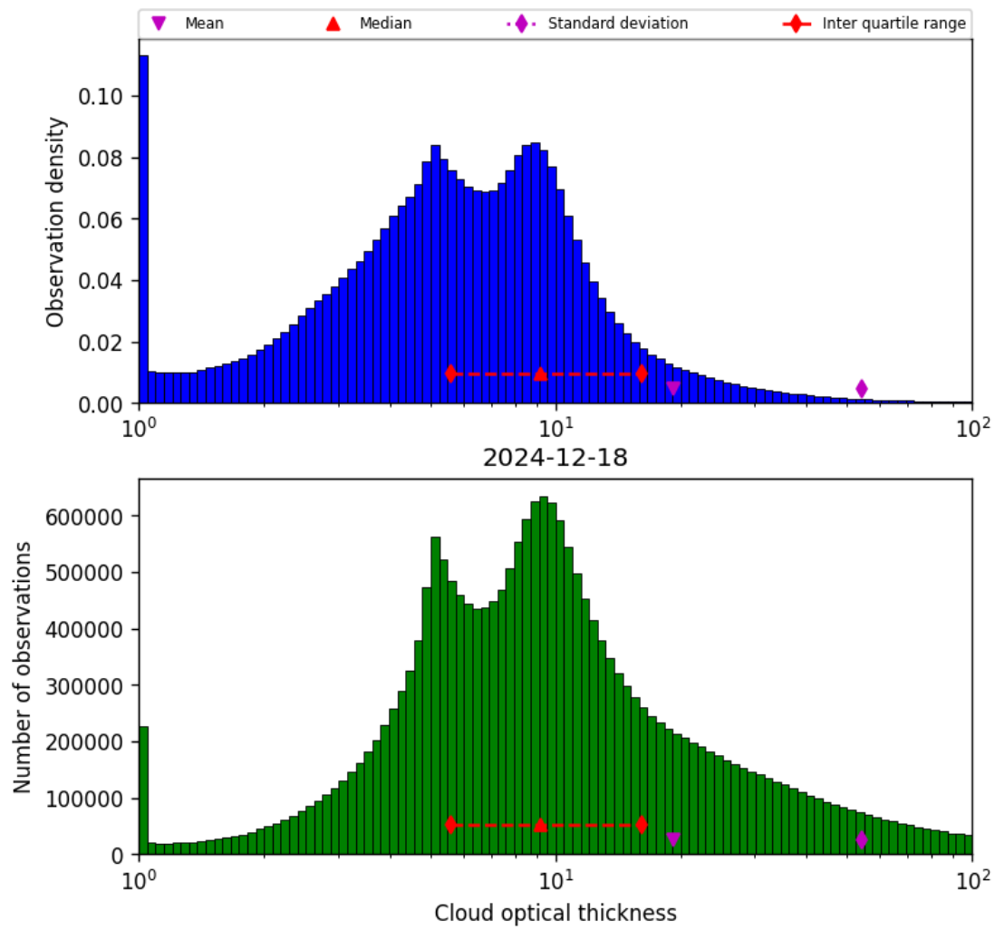
Figure 41: Histogram of “Cloud optical thickness” for 2024-12-17 to 2024-12-19
