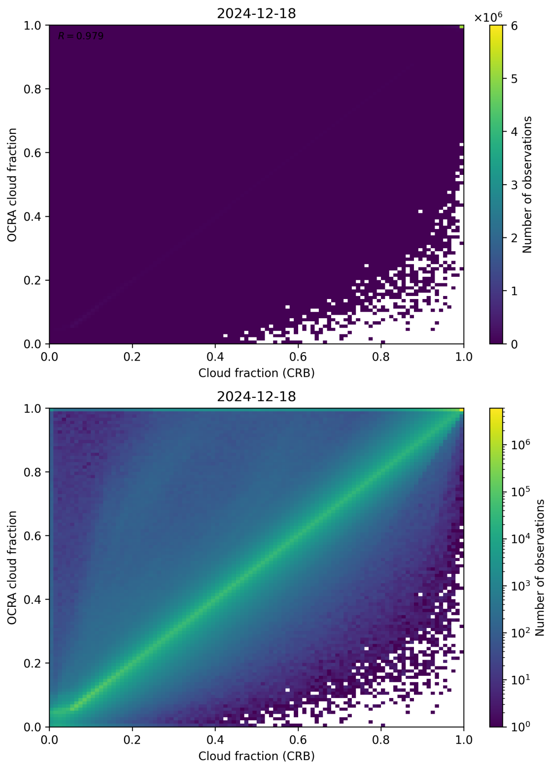
Figure 78: Scatter density plot of “Cloud fraction (CRB)” against “OCRA cloud fraction” for 2024-12-17 to 2024-12-19.
