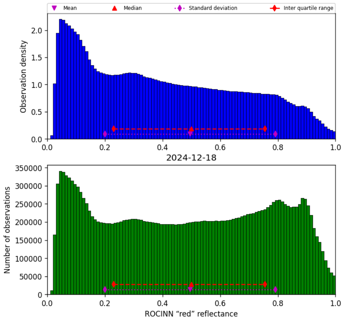
Figure 53: Histogram of “ROCINN “red” reflectance” for 2024-12-17 to 2024-12-19
