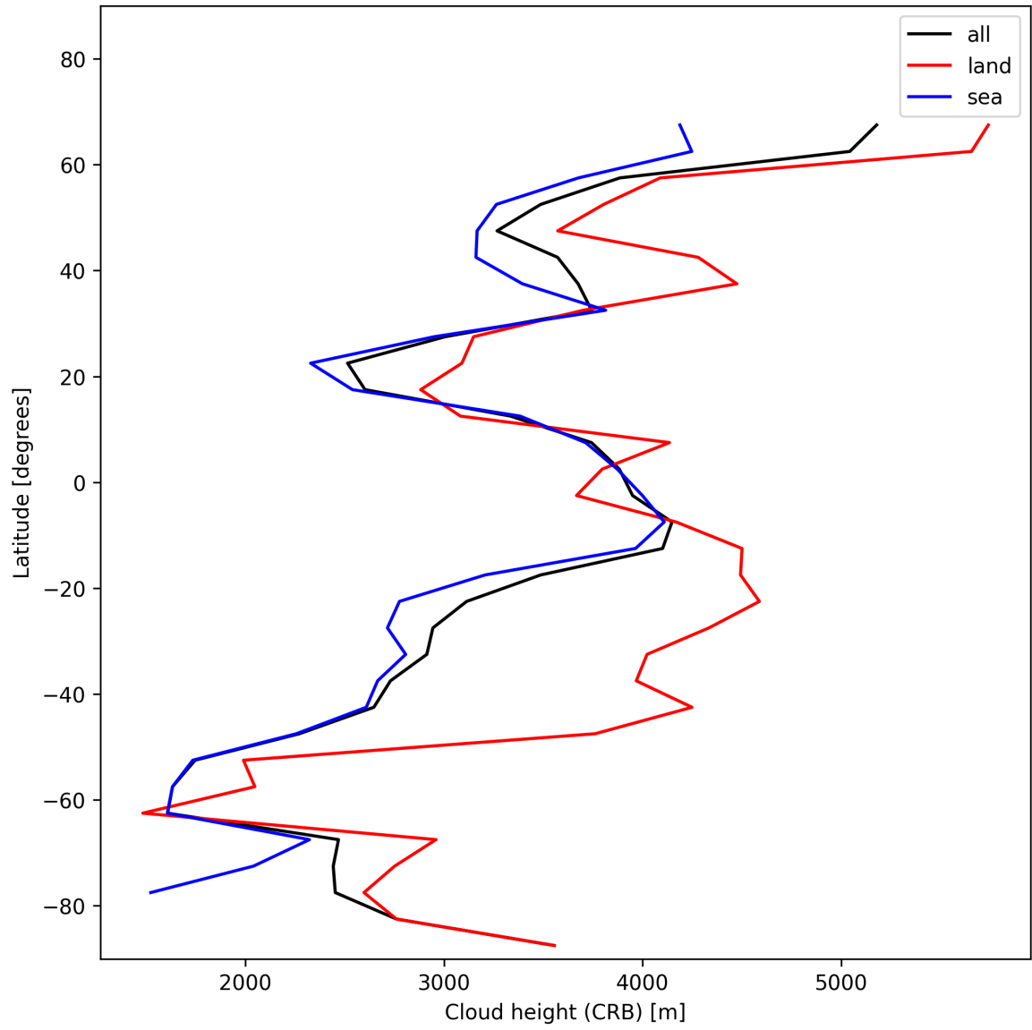
Figure 27: Zonal average of “Cloud height (CRB)” for 2024-12-17 to 2024-12-19.
