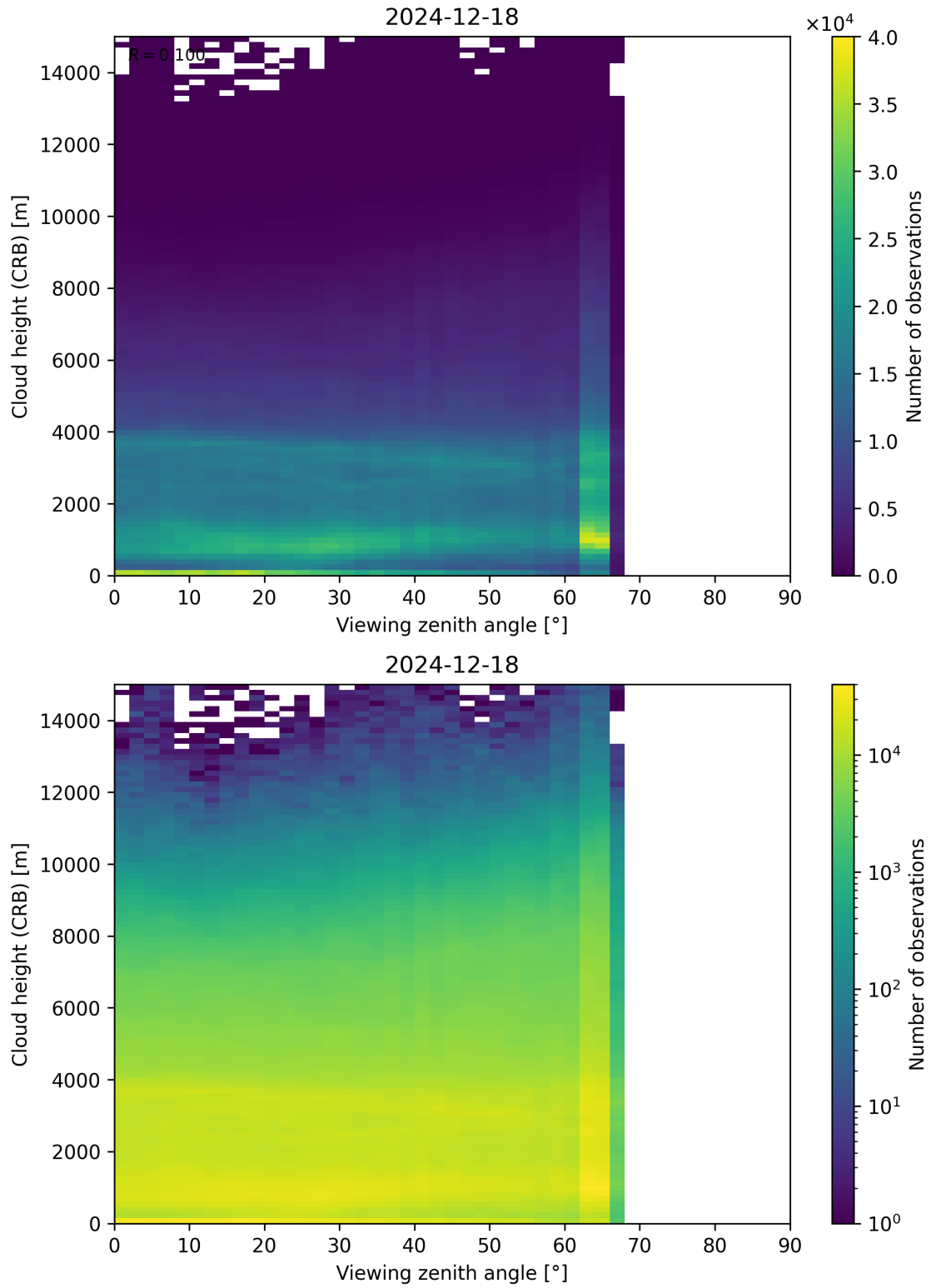
Figure 110: Scatter density plot of “Viewing zenith angle” against “Cloud height (CRB)” for 2024-12-17 to 2024-12-19.
