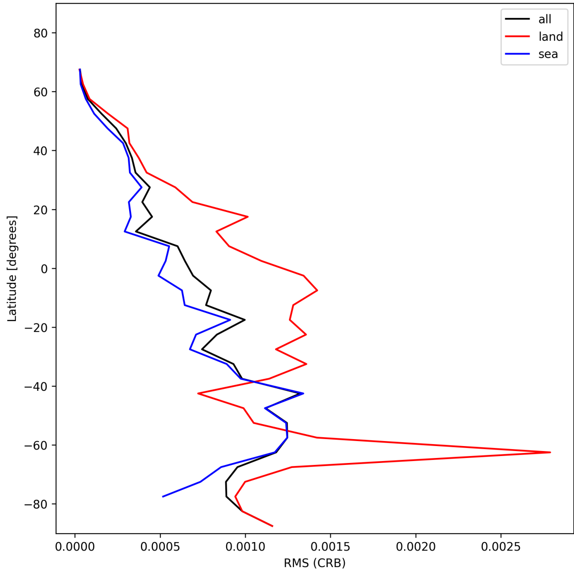
Figure 32: Zonal average of “RMS (CRB)” for 2024-12-17 to 2024-12-19.
