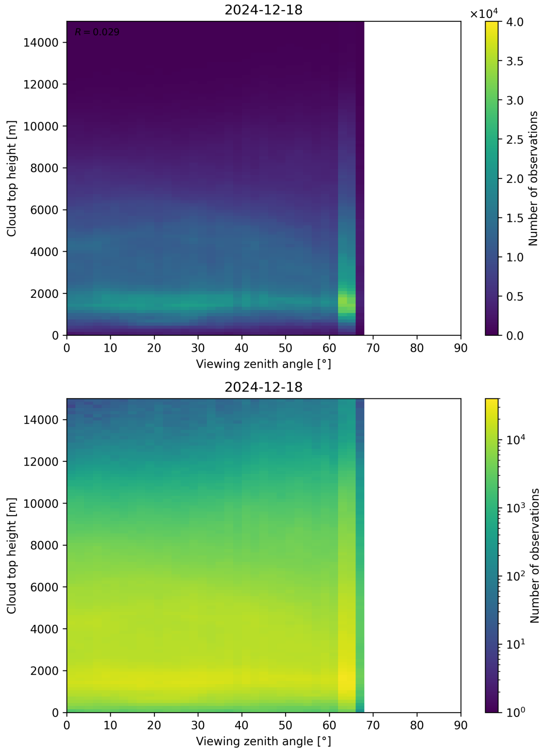
Figure 112: Scatter density plot of “Viewing zenith angle” against “Cloud top height” for 2024-12-17 to 2024-12-19.
