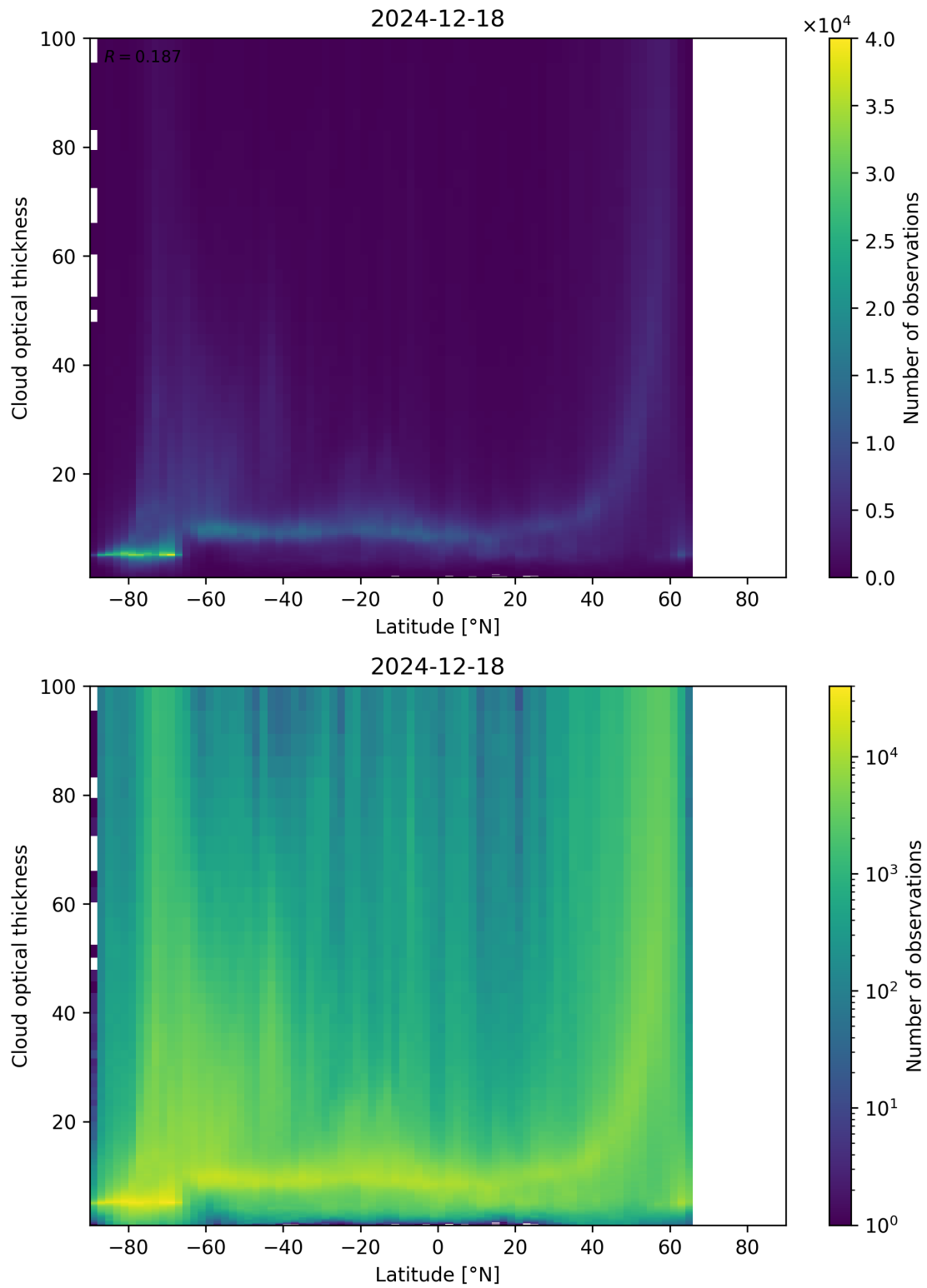
Figure 96: Scatter density plot of “Latitude” against “Cloud optical thickness” for 2024-12-17 to 2024-12-19.
