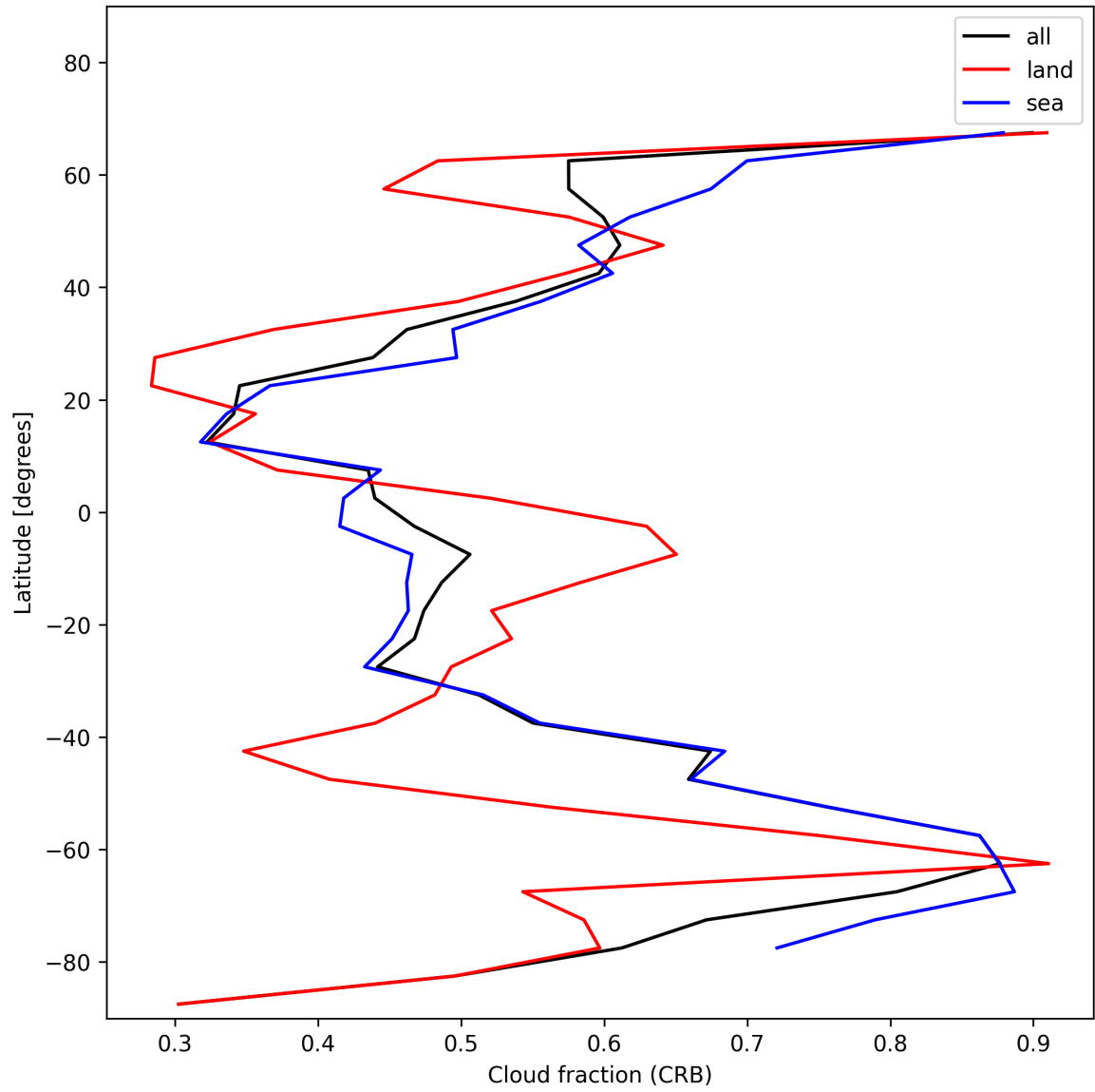
Figure 26: Zonal average of “Cloud fraction (CRB)” for 2024-12-17 to 2024-12-19.
