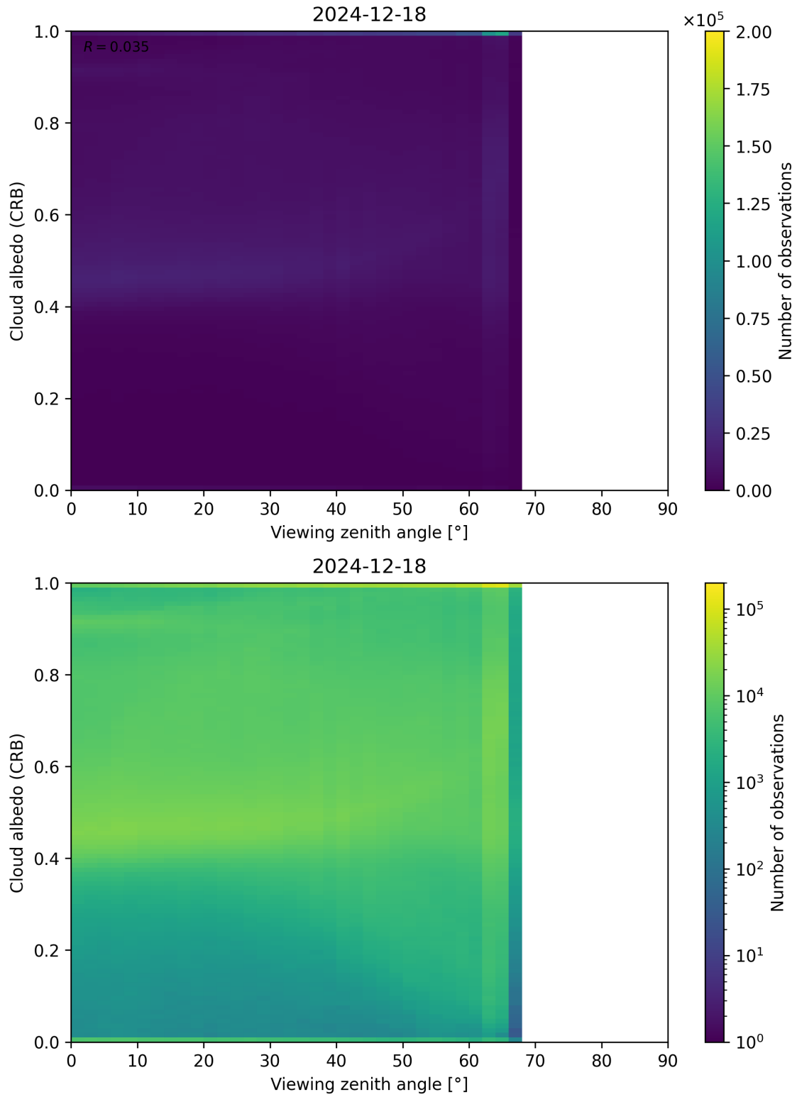
Figure 106: Scatter density plot of “Viewing zenith angle” against “Cloud albedo (CRB)” for 2024-12-17 to 2024-12-19.
