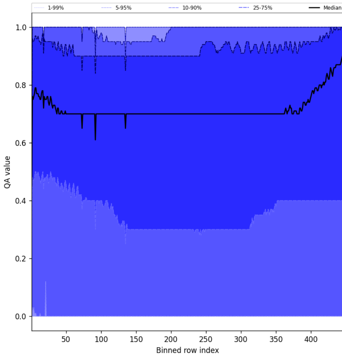
Figure 54: Along track statistics of “QA value” for 2024-12-17 to 2024-12-19
