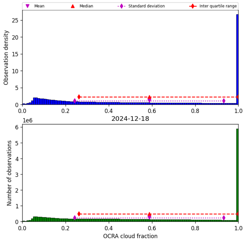
Figure 50: Histogram of “OCRA cloud fraction” for 2024-12-17 to 2024-12-19
