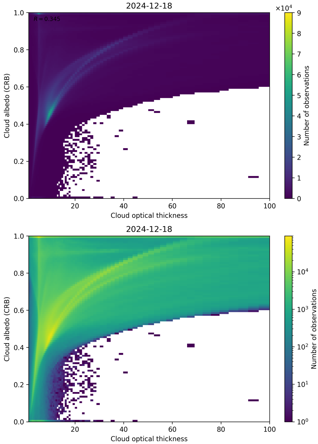
Figure 82: Scatter density plot of “Cloud optical thickness” against “Cloud albedo (CRB)” for 2024-12-17 to 2024-12-19.
