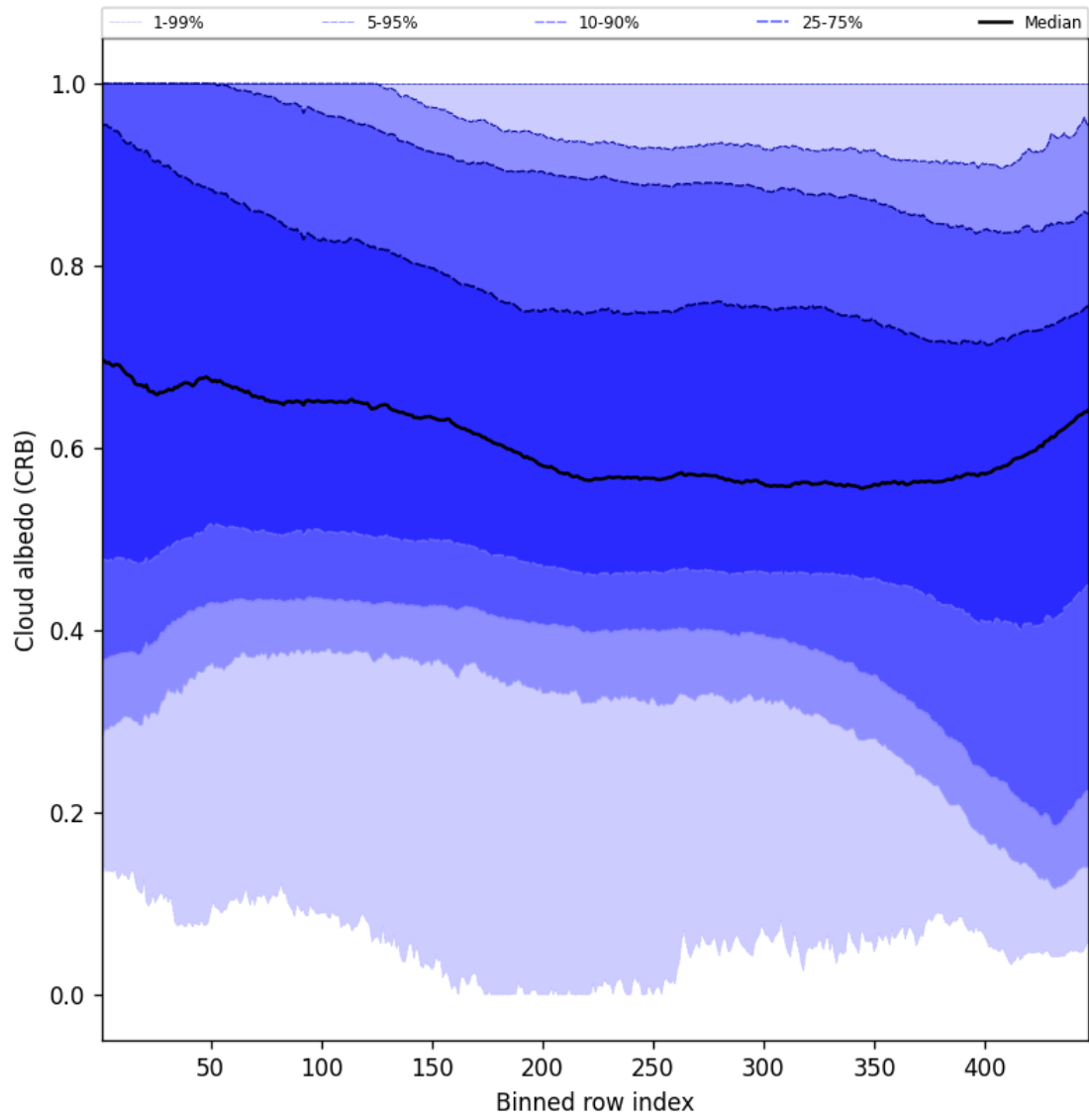
Figure 60: Along track statistics of “Cloud albedo (CRB)” for 2024-12-17 to 2024-12-19
