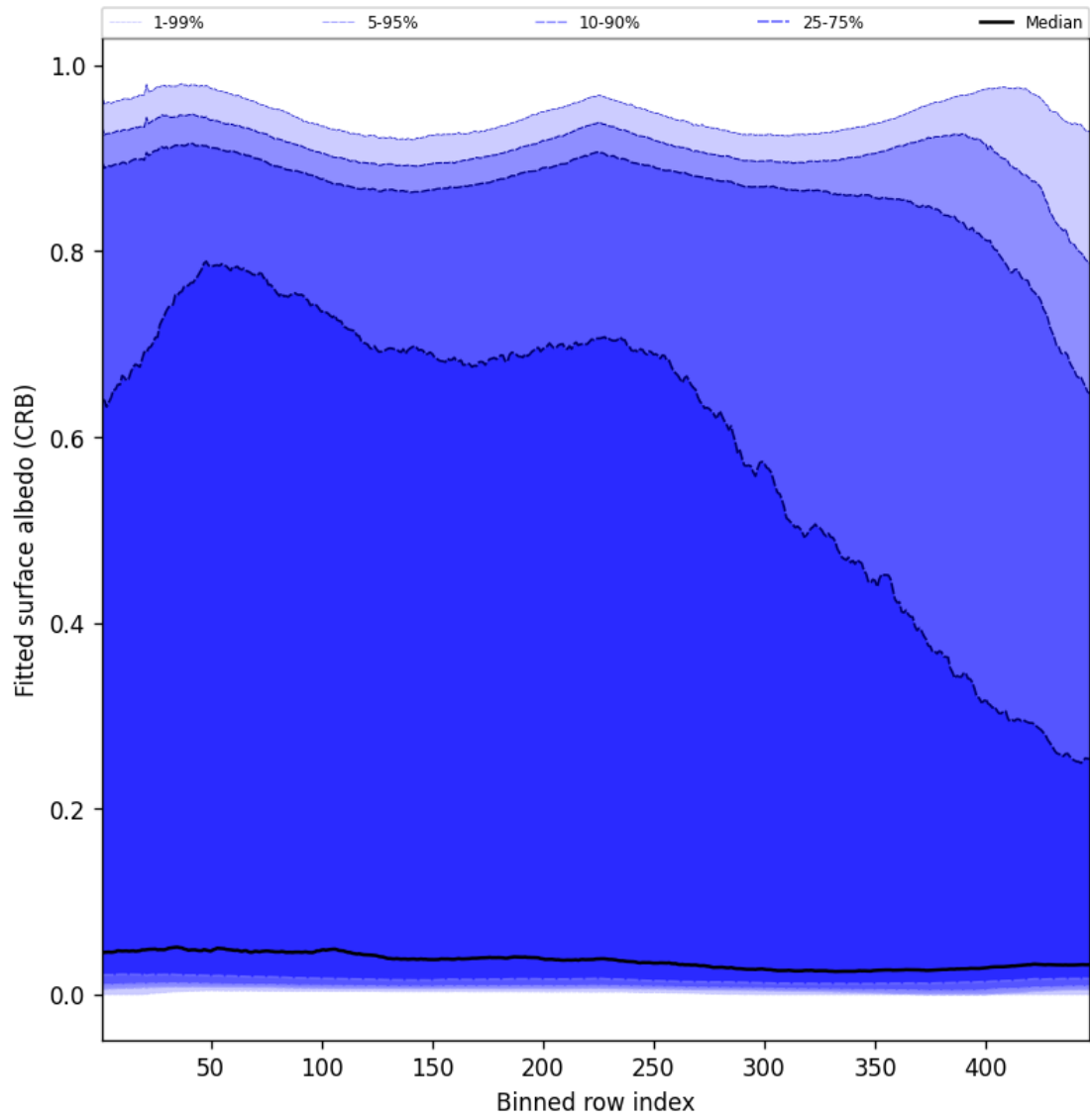
Figure 62: Along track statistics of “Fitted surface albedo (CRB)” for 2024-12-17 to 2024-12-19
