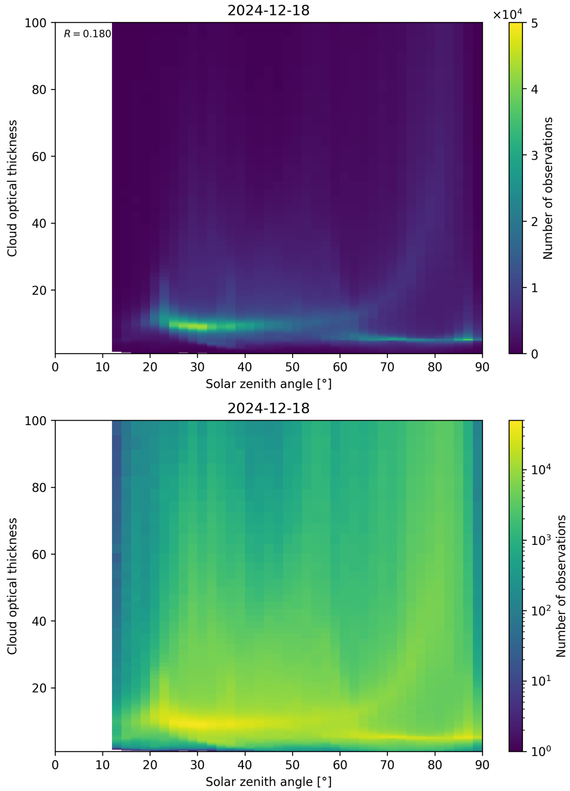
Figure 103: Scatter density plot of “Solar zenith angle” against “Cloud optical thickness” for 2024-12-17 to 2024-12-19.
