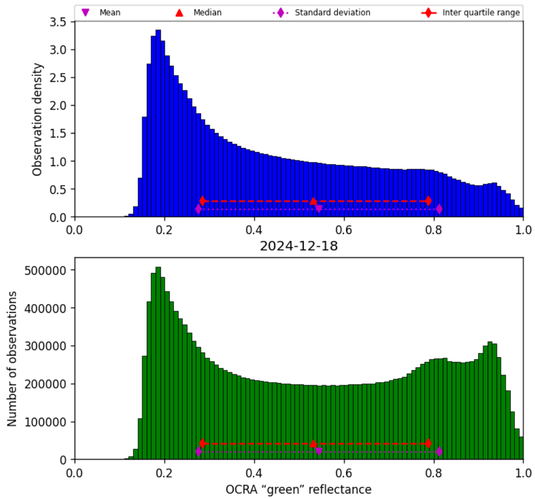
Figure 52: Histogram of “OCRA “green” reflectance” for 2024-12-17 to 2024-12-19
