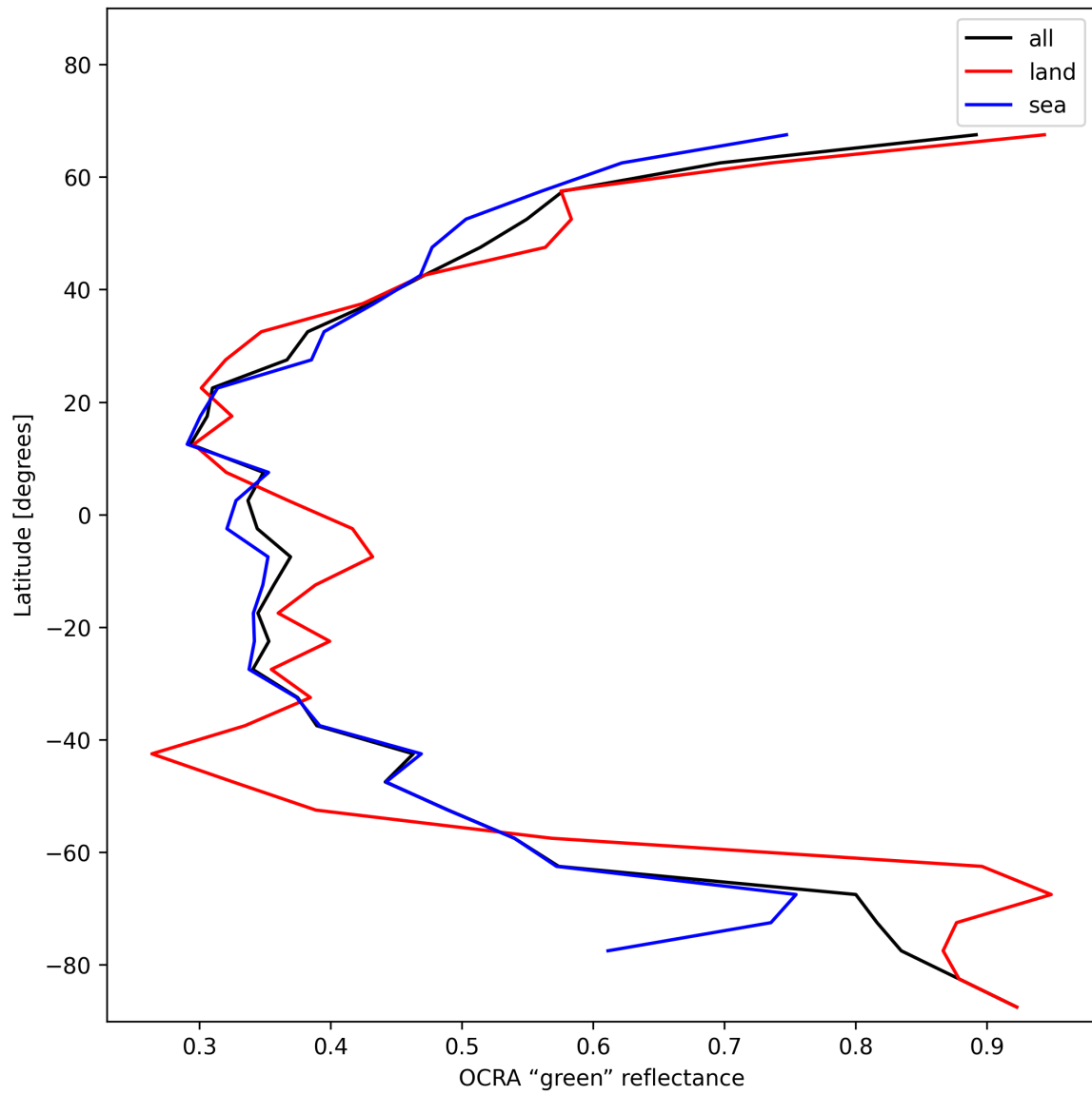
Figure 36: Zonal average of “OCRA “green” reflectance” for 2024-12-17 to 2024-12-19.
