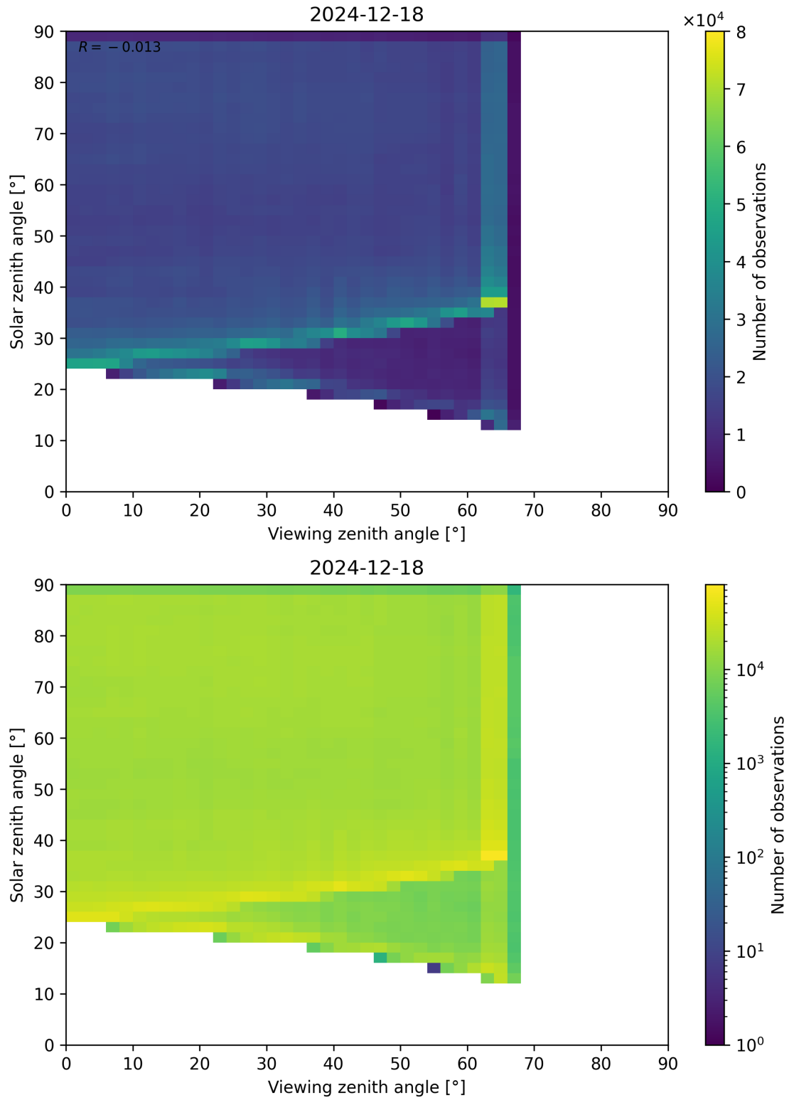
Figure 114: Scatter density plot of “Viewing zenith angle” against “Solar zenith angle” for 2024-12-17 to 2024-12-19.
