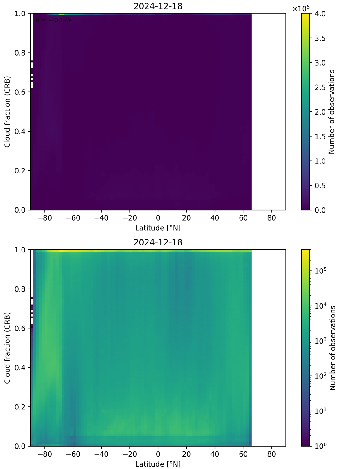
Figure 94: Scatter density plot of “Latitude” against “Cloud fraction (CRB)” for 2024-12-17 to 2024-12-19.
