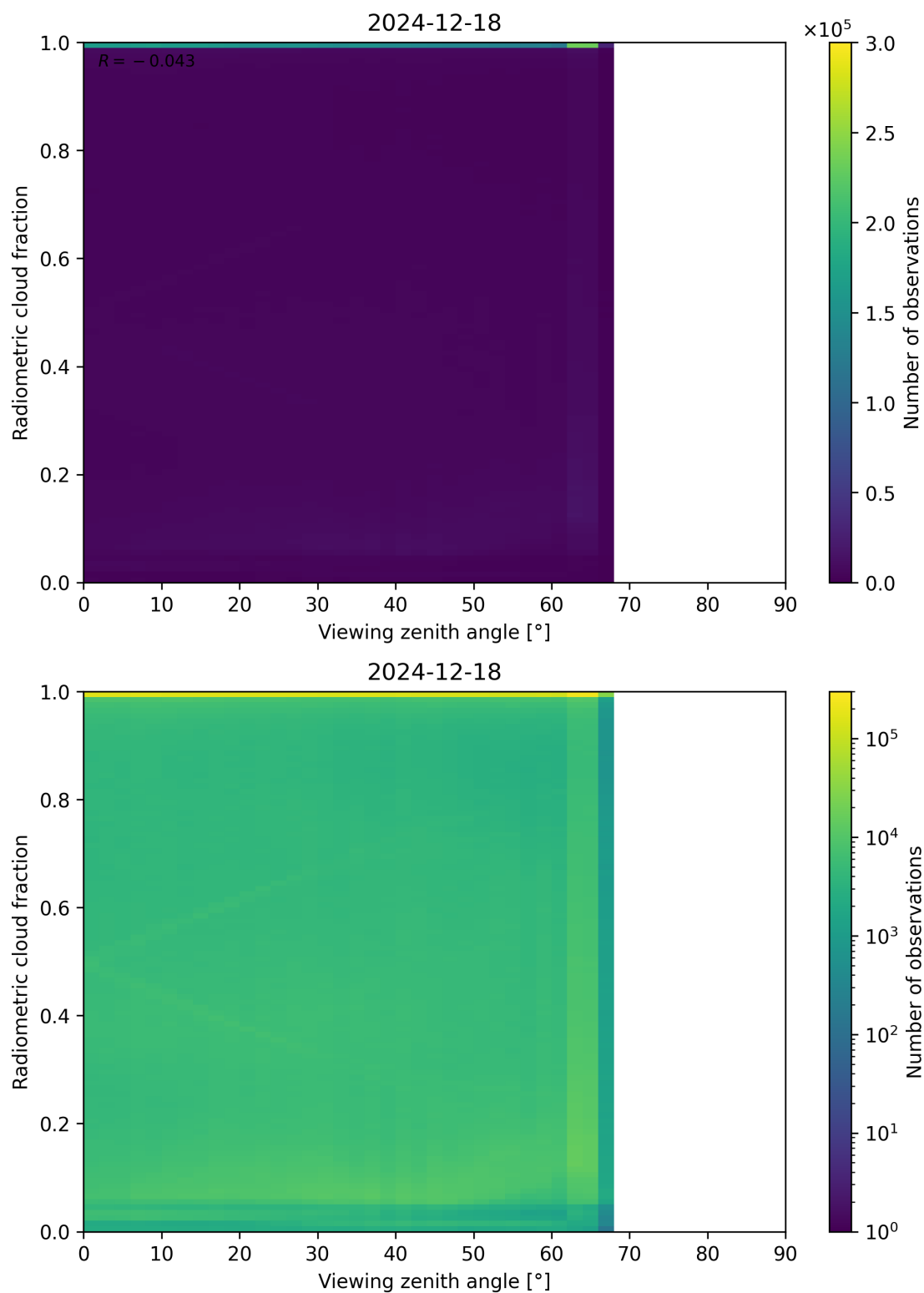
Figure 107: Scatter density plot of “Viewing zenith angle” against “Radiometric cloud fraction” for 2024-12-17 to 2024-12-19.
