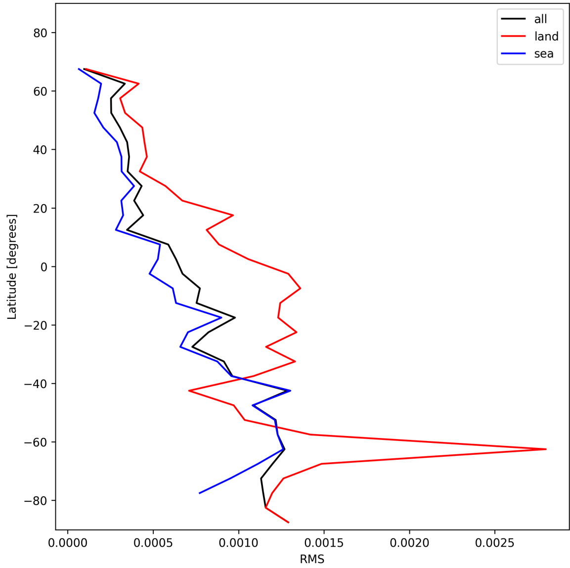
Figure 31: Zonal average of “RMS” for 2024-12-17 to 2024-12-19.
