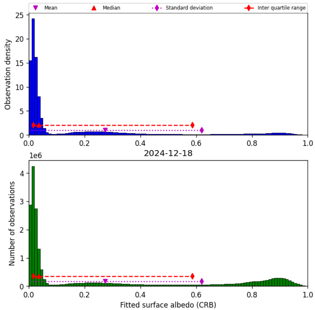
Figure 46: Histogram of “Fitted surface albedo (CRB)” for 2024-12-17 to 2024-12-19
