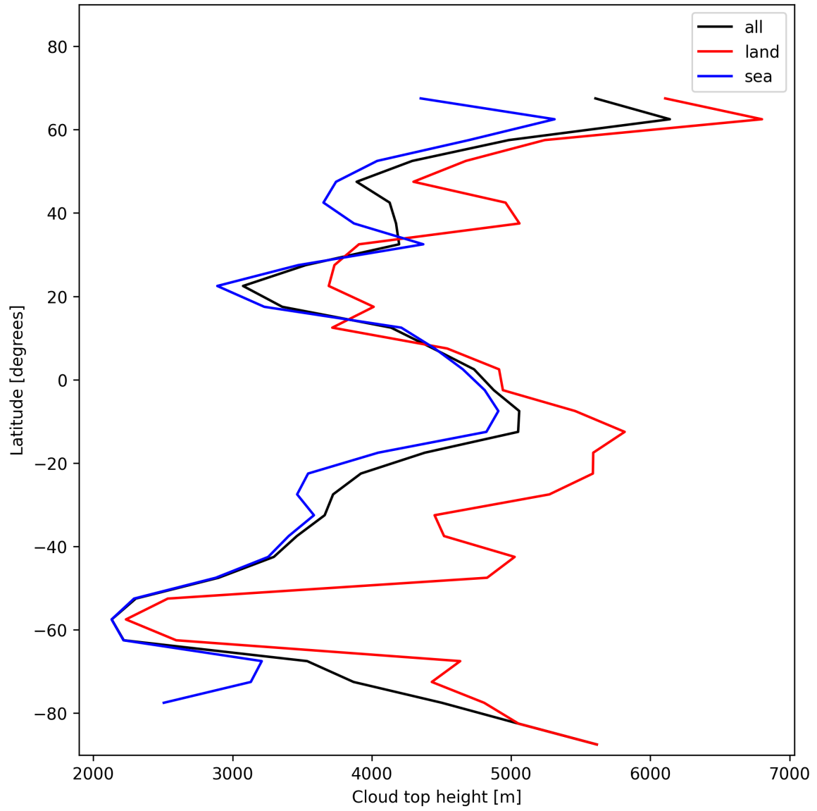
Figure 24: Zonal average of “Cloud top height” for 2024-12-17 to 2024-12-19.
