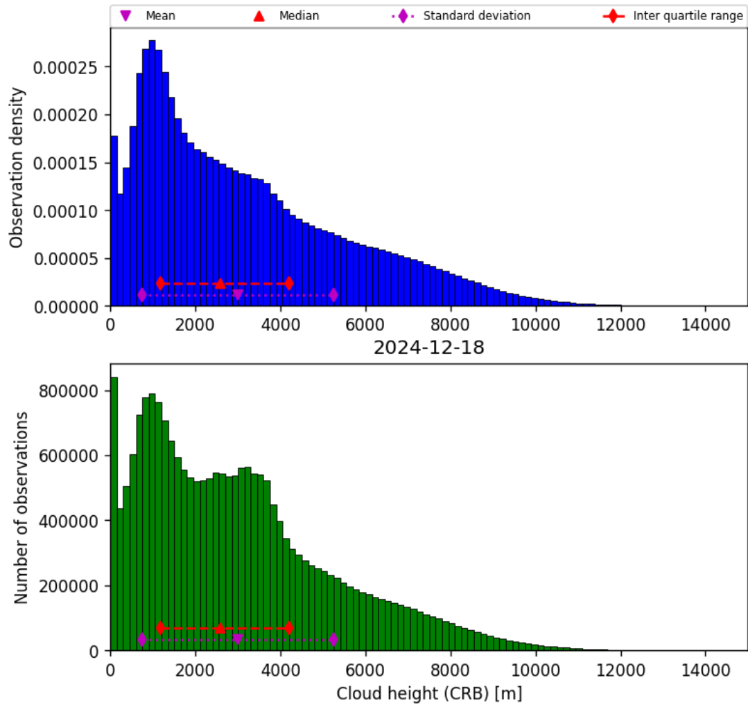
Figure 43: Histogram of “Cloud height (CRB)” for 2024-12-17 to 2024-12-19
