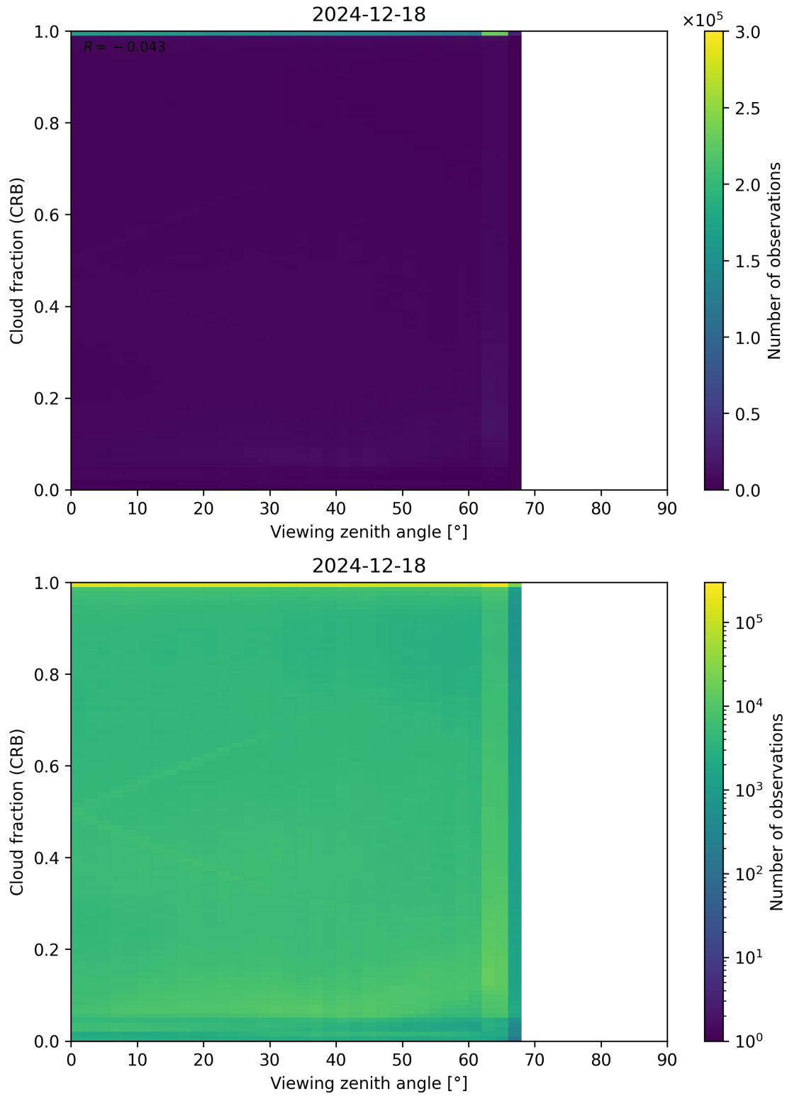
Figure 109: Scatter density plot of “Viewing zenith angle” against “Cloud fraction (CRB)” for 2024-12-17 to 2024-12-19.
