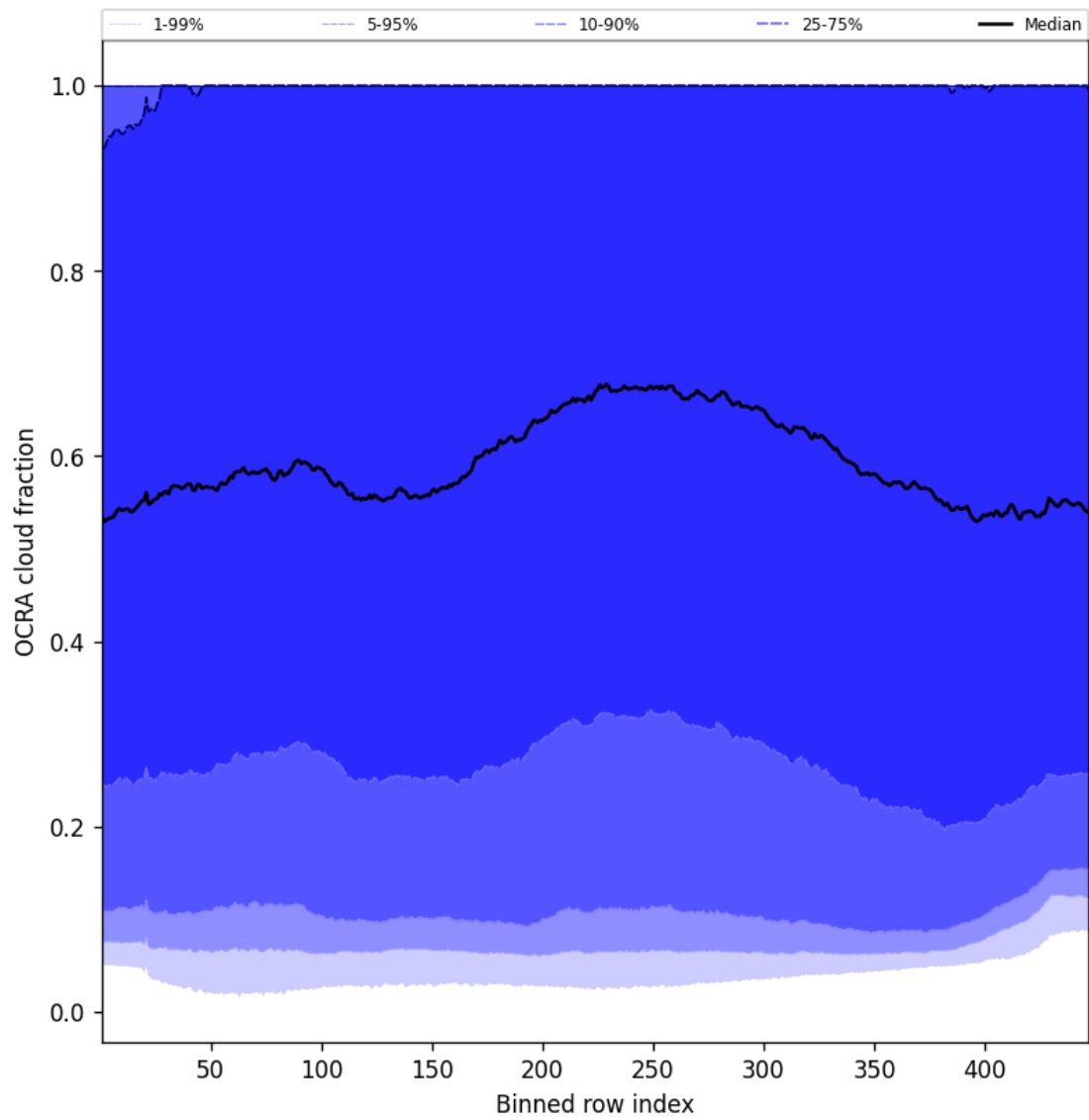
Figure 66: Along track statistics of “OCRA cloud fraction” for 2024-12-17 to 2024-12-19
