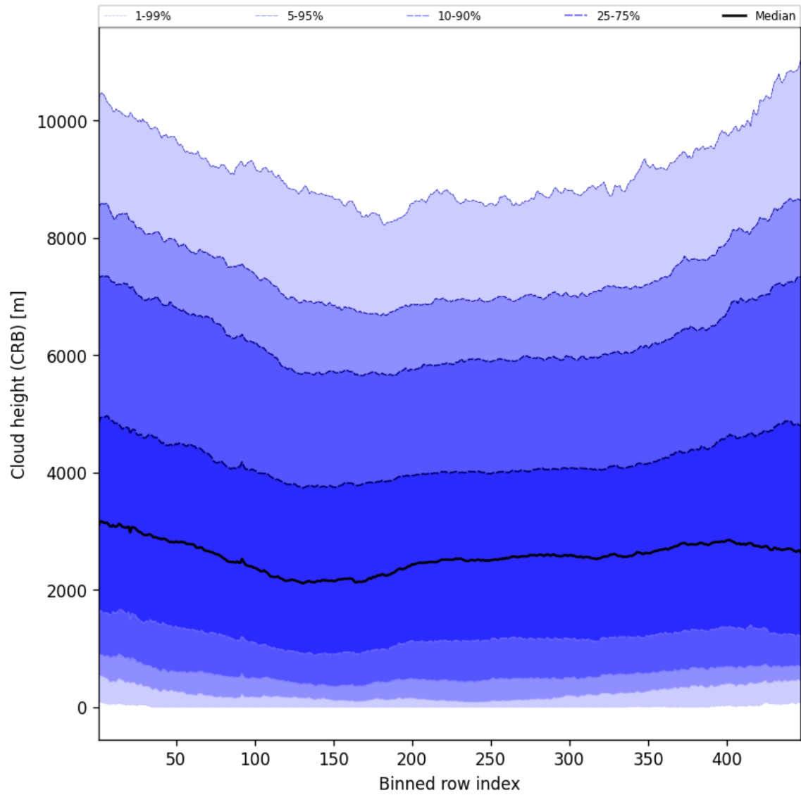
Figure 59: Along track statistics of “Cloud height (CRB)” for 2024-12-17 to 2024-12-19
