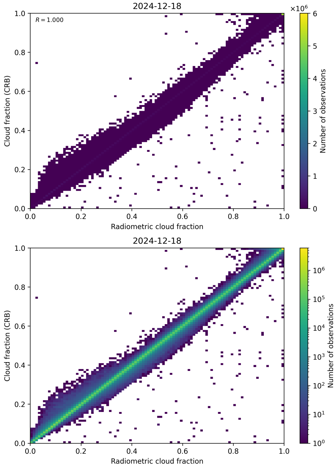
Figure 73: Scatter density plot of “Radiometric cloud fraction” against “Cloud fraction (CRB)” for 2024-12-17 to 2024-12-19.
