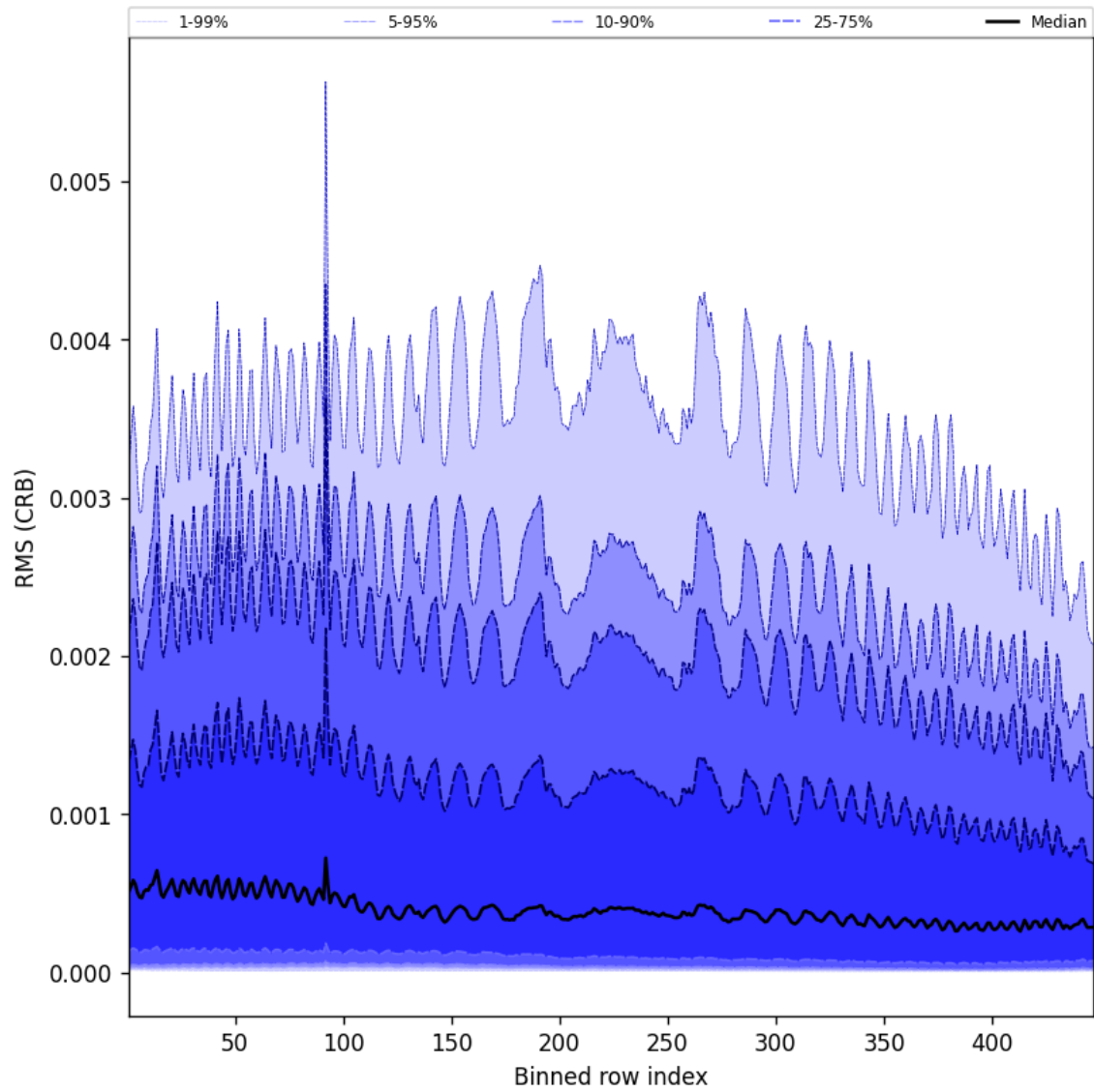
Figure 64: Along track statistics of “RMS (CRB)” for 2024-12-17 to 2024-12-19
