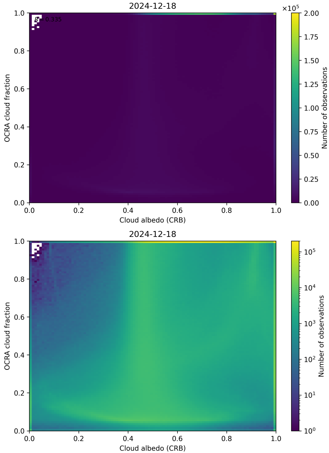
Figure 70: Scatter density plot of “Cloud albedo (CRB)” against “OCRA cloud fraction” for 2024-12-17 to 2024-12-19.
