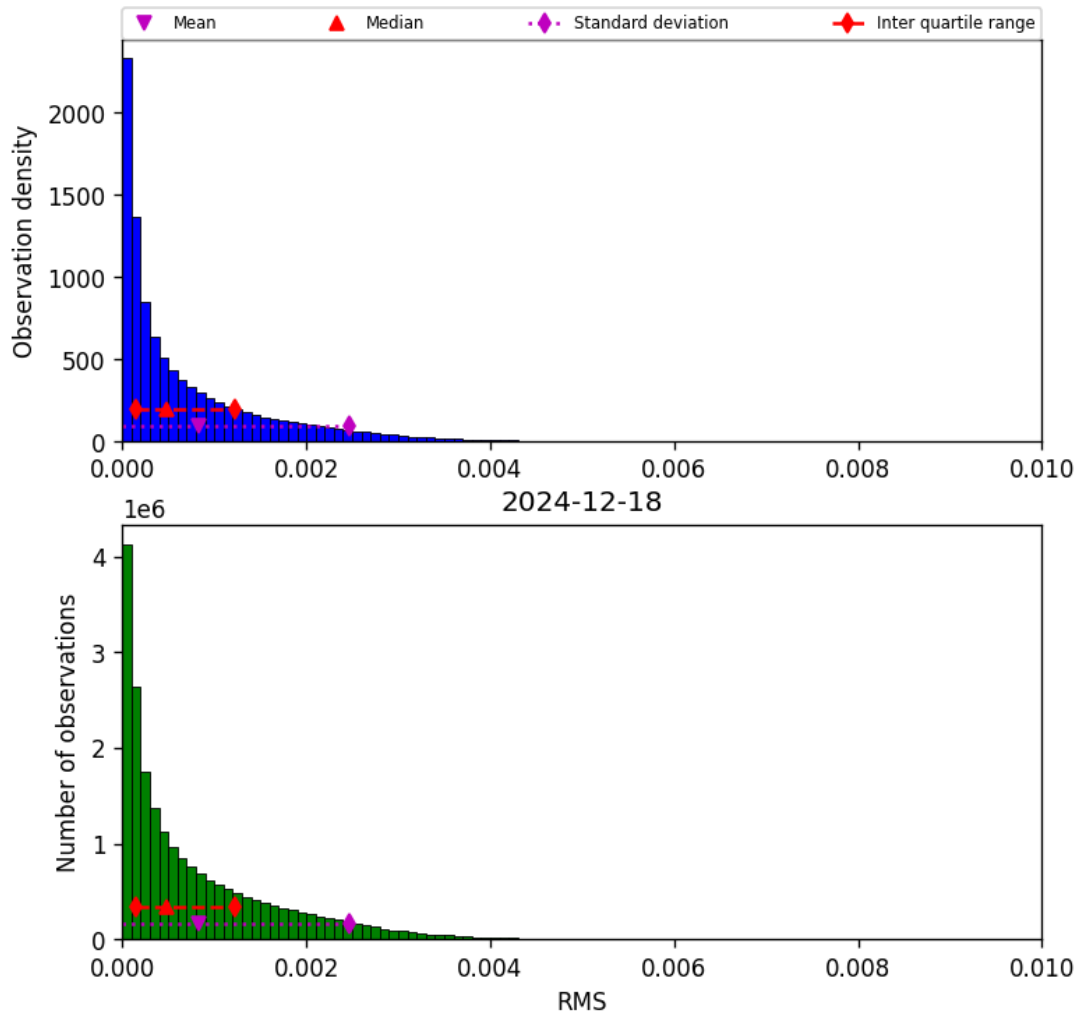
Figure 47: Histogram of “RMS” for 2024-12-17 to 2024-12-19
