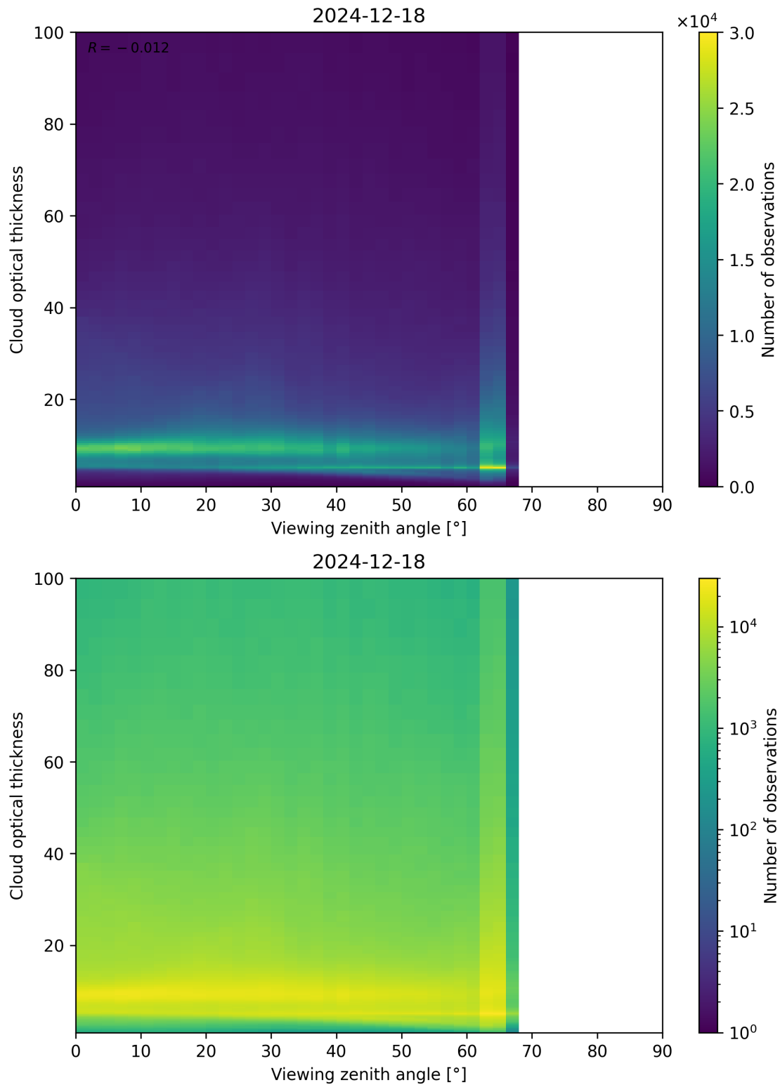
Figure 111: Scatter density plot of “Viewing zenith angle” against “Cloud optical thickness” for 2024-12-17 to 2024-12-19.
