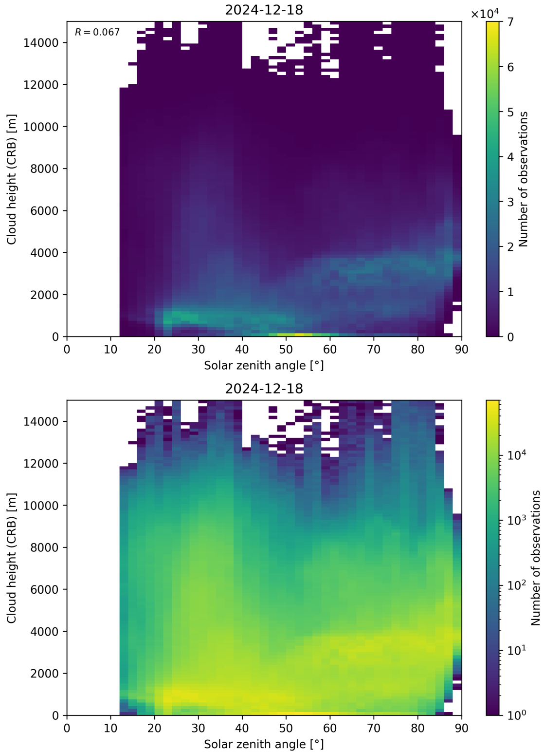
Figure 102: Scatter density plot of “Solar zenith angle” against “Cloud height (CRB)” for 2024-12-17 to 2024-12-19.
