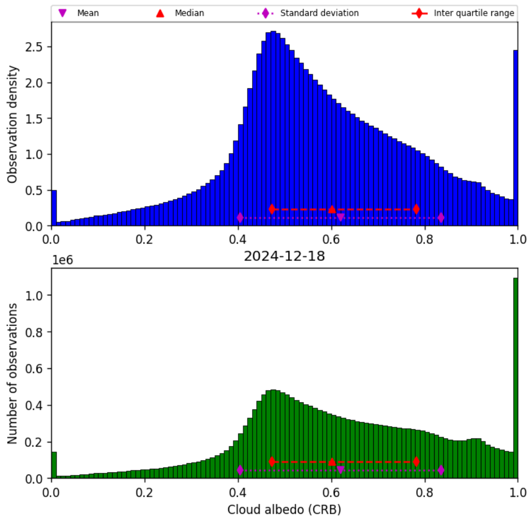
Figure 44: Histogram of “Cloud albedo (CRB)” for 2024-12-17 to 2024-12-19
