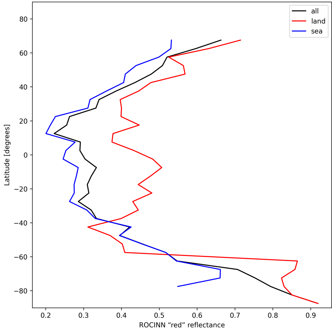
Figure 37: Zonal average of “ROCINN “red” reflectance” for 2024-12-17 to 2024-12-19.
