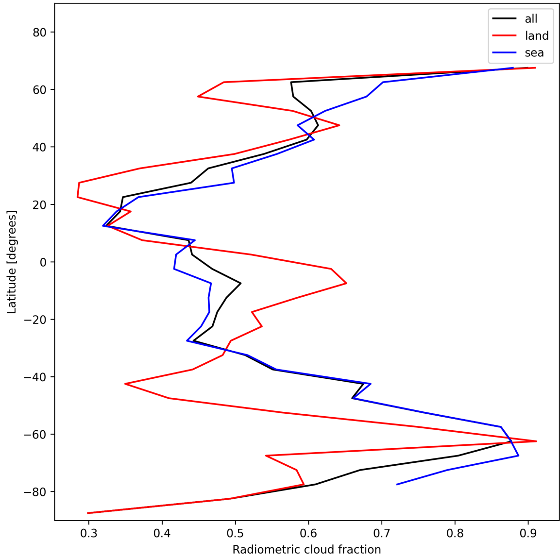
Figure 23: Zonal average of “Radiometric cloud fraction” for 2024-12-17 to 2024-12-19.
