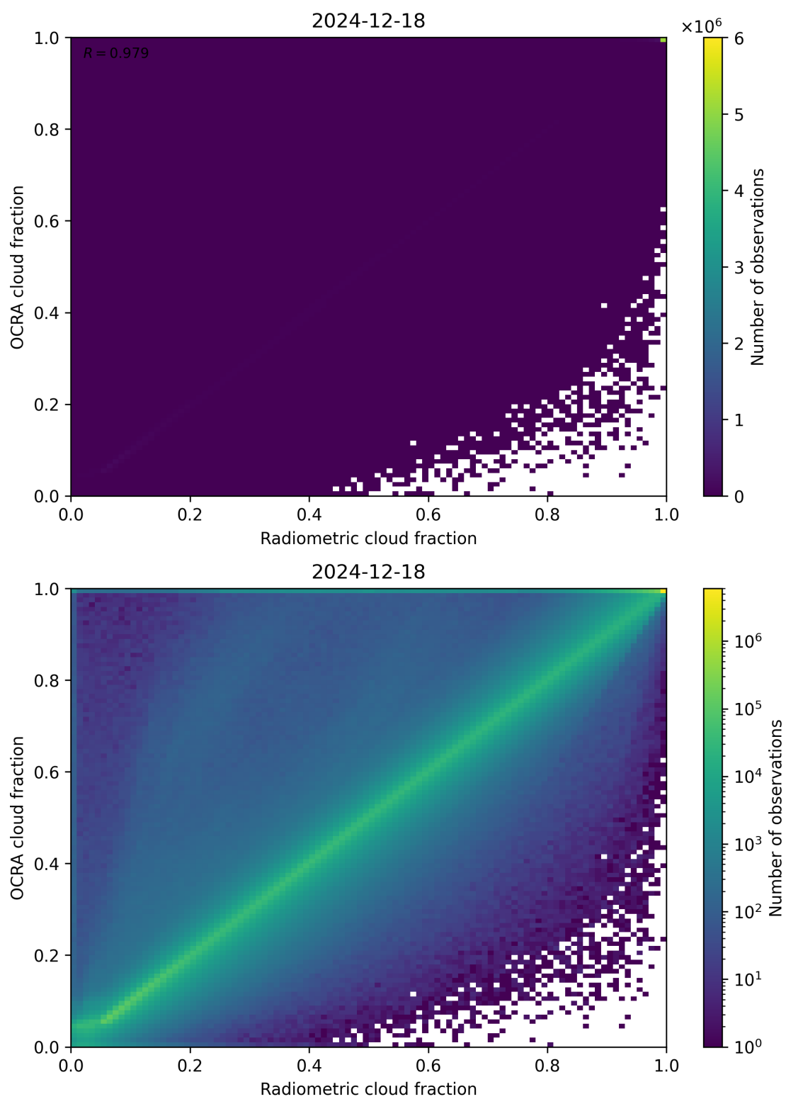
Figure 72: Scatter density plot of “Radiometric cloud fraction” against “OCRA cloud fraction” for 2024-12-17 to 2024-12-19.
