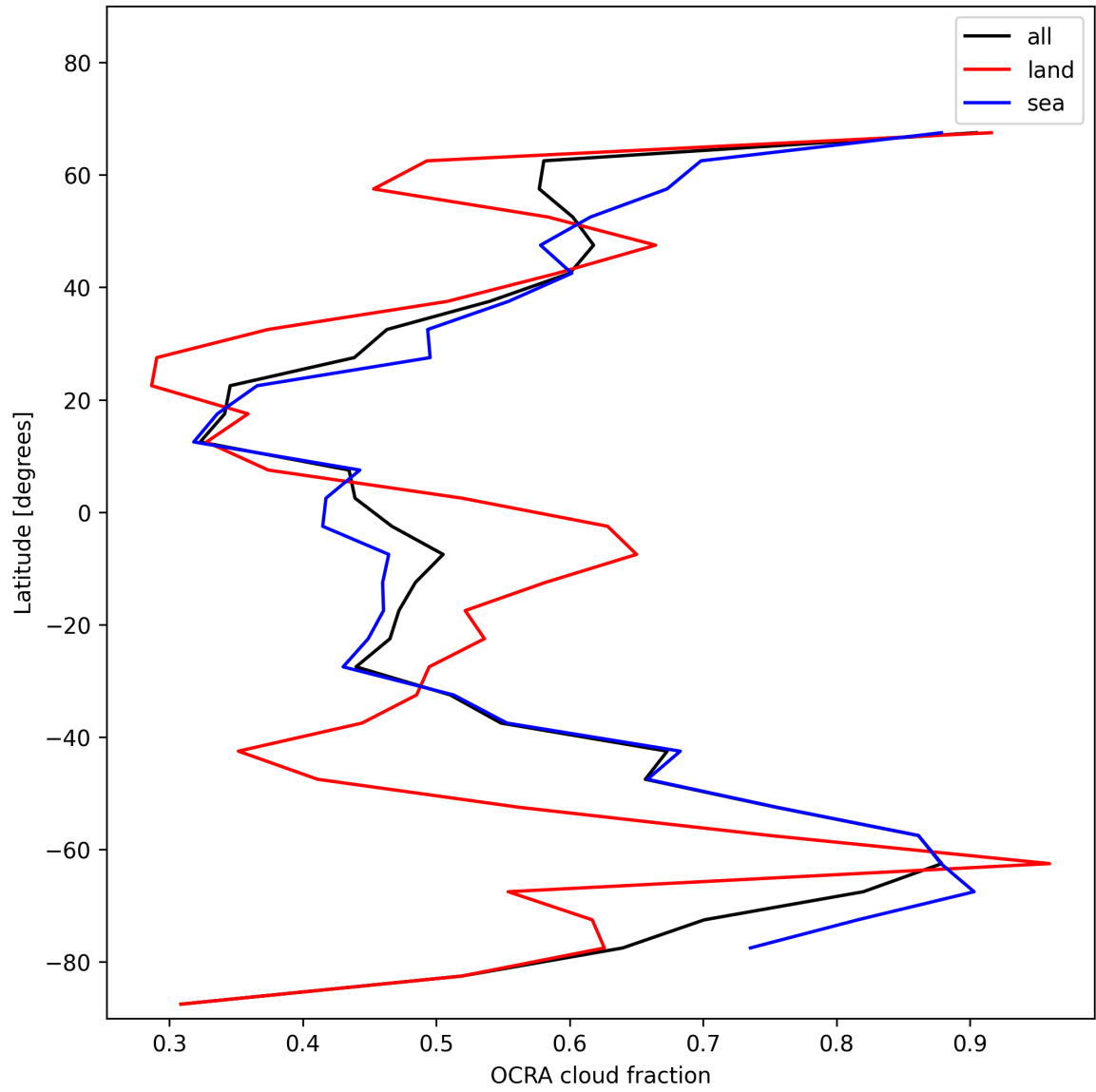
Figure 34: Zonal average of “OCRA cloud fraction” for 2024-12-17 to 2024-12-19.
