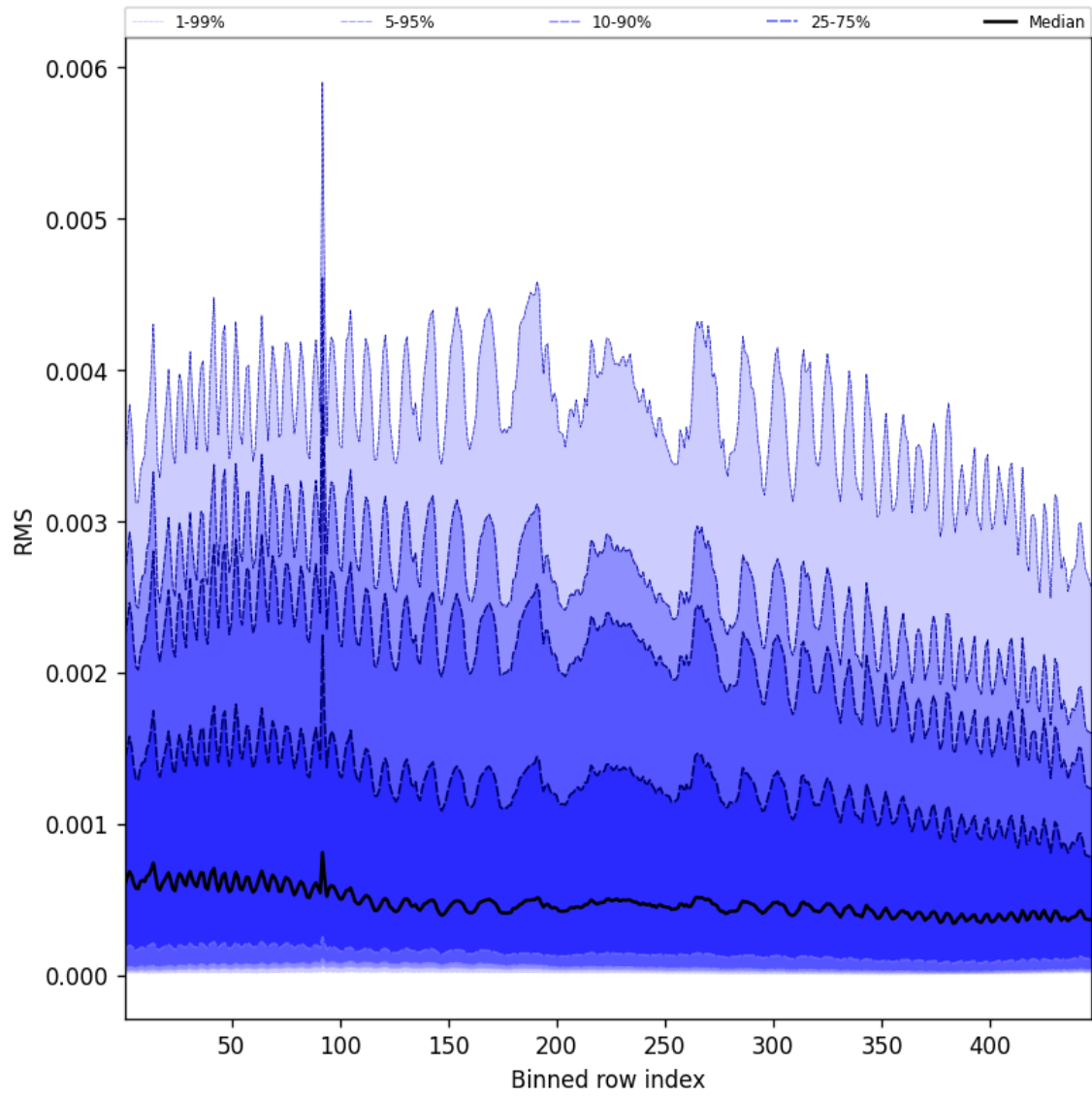
Figure 63: Along track statistics of “RMS” for 2024-12-17 to 2024-12-19
