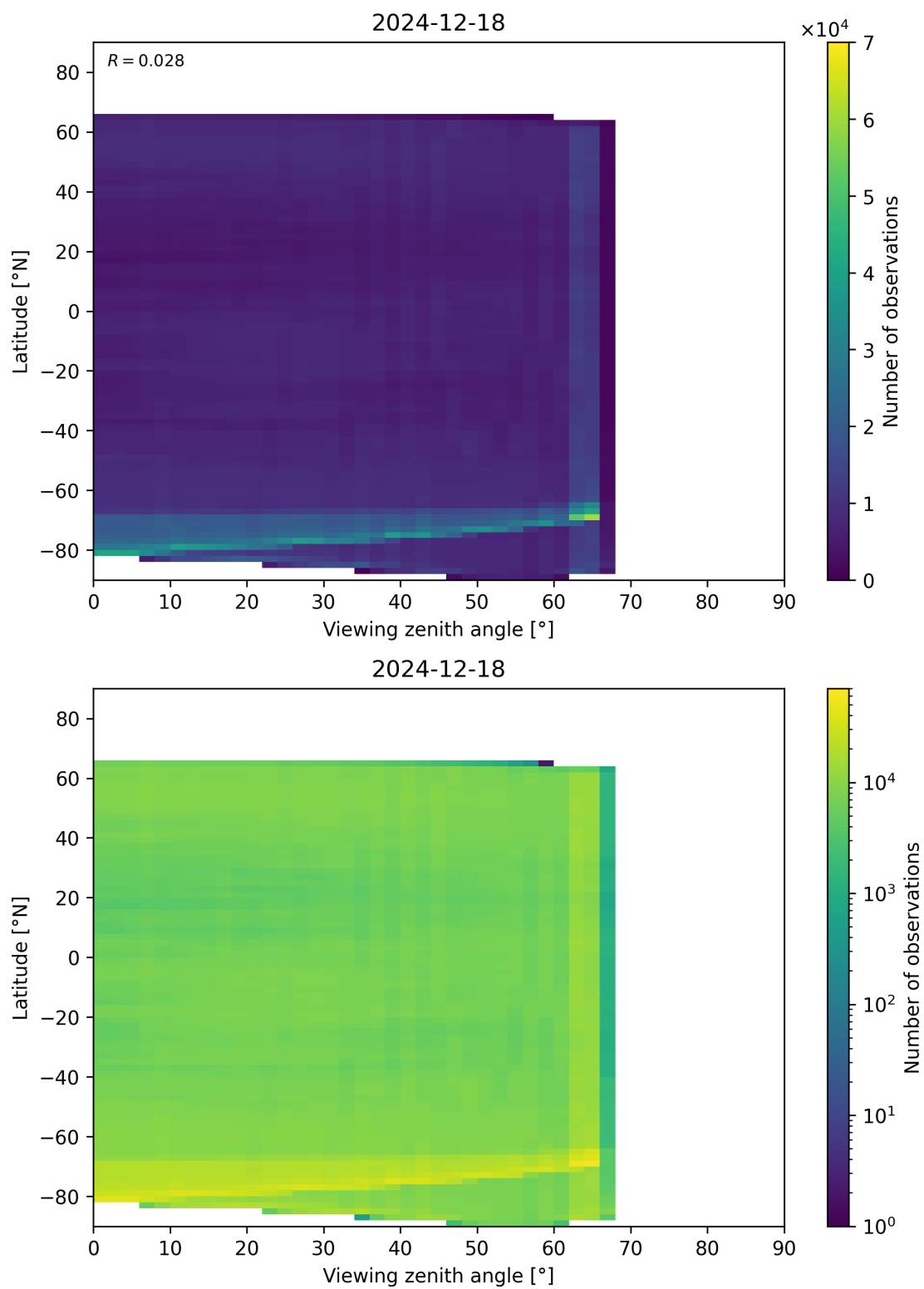
Figure 113: Scatter density plot of “Viewing zenith angle” against “Latitude” for 2024-12-17 to 2024-12-19.
