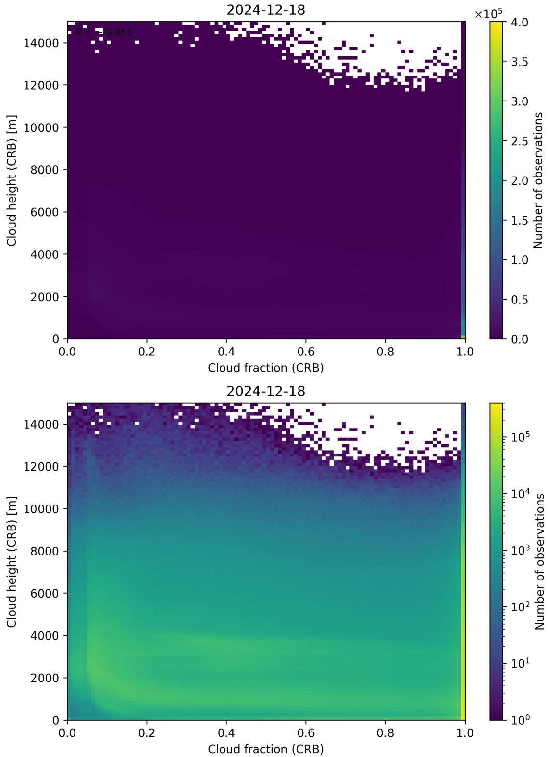
Figure 79: Scatter density plot of “Cloud fraction (CRB)” against “Cloud height (CRB)” for 2024-12-17 to 2024-12-19.
