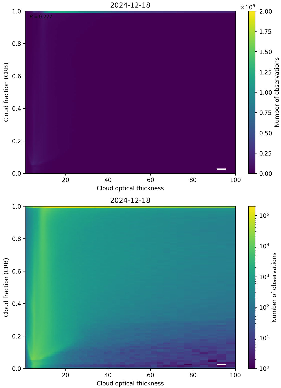
Figure 84: Scatter density plot of “Cloud optical thickness” against “Cloud fraction (CRB)” for 2024-12-17 to 2024-12-19.
