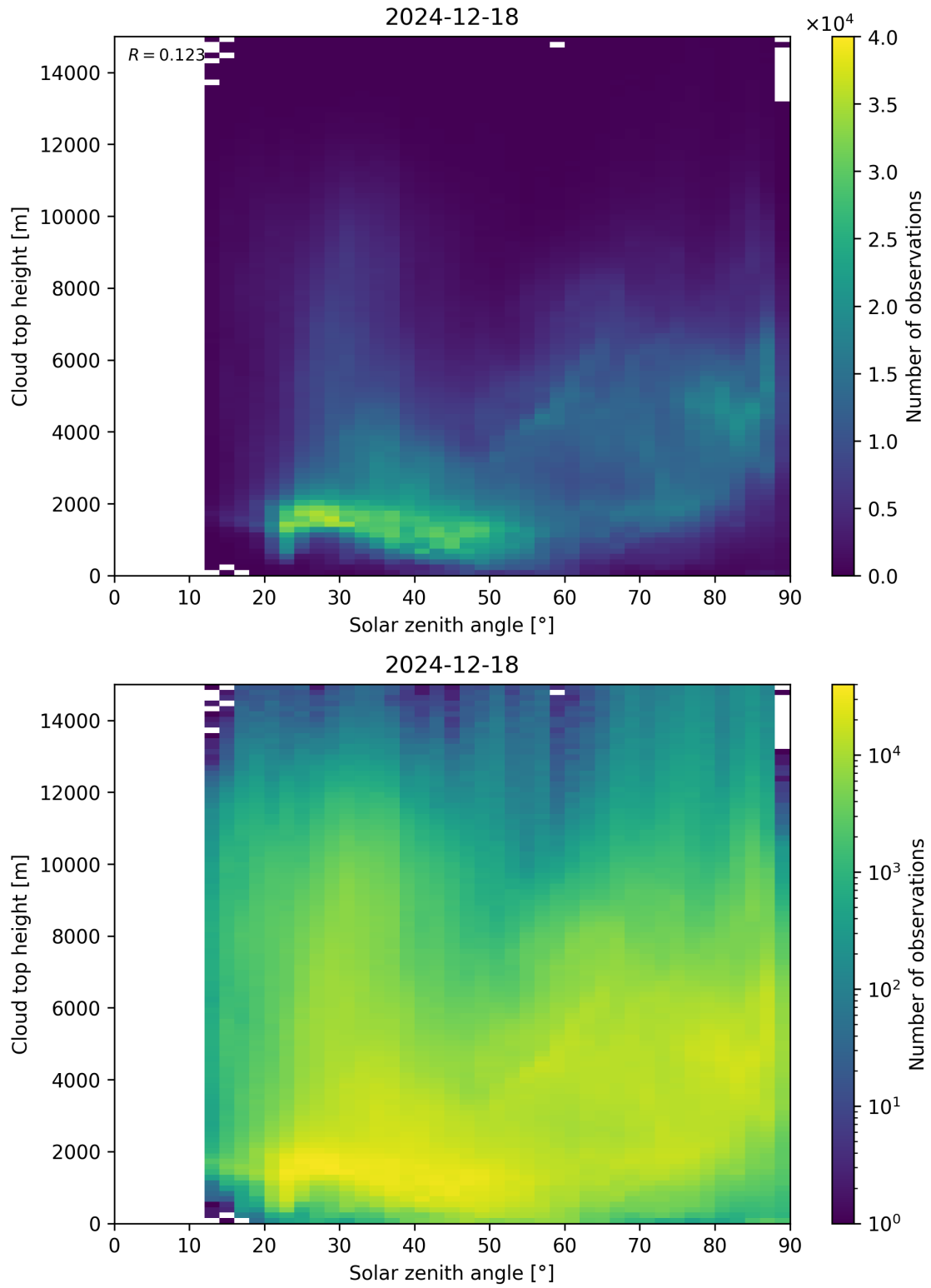
Figure 104: Scatter density plot of “Solar zenith angle” against “Cloud top height” for 2024-12-17 to 2024-12-19.
