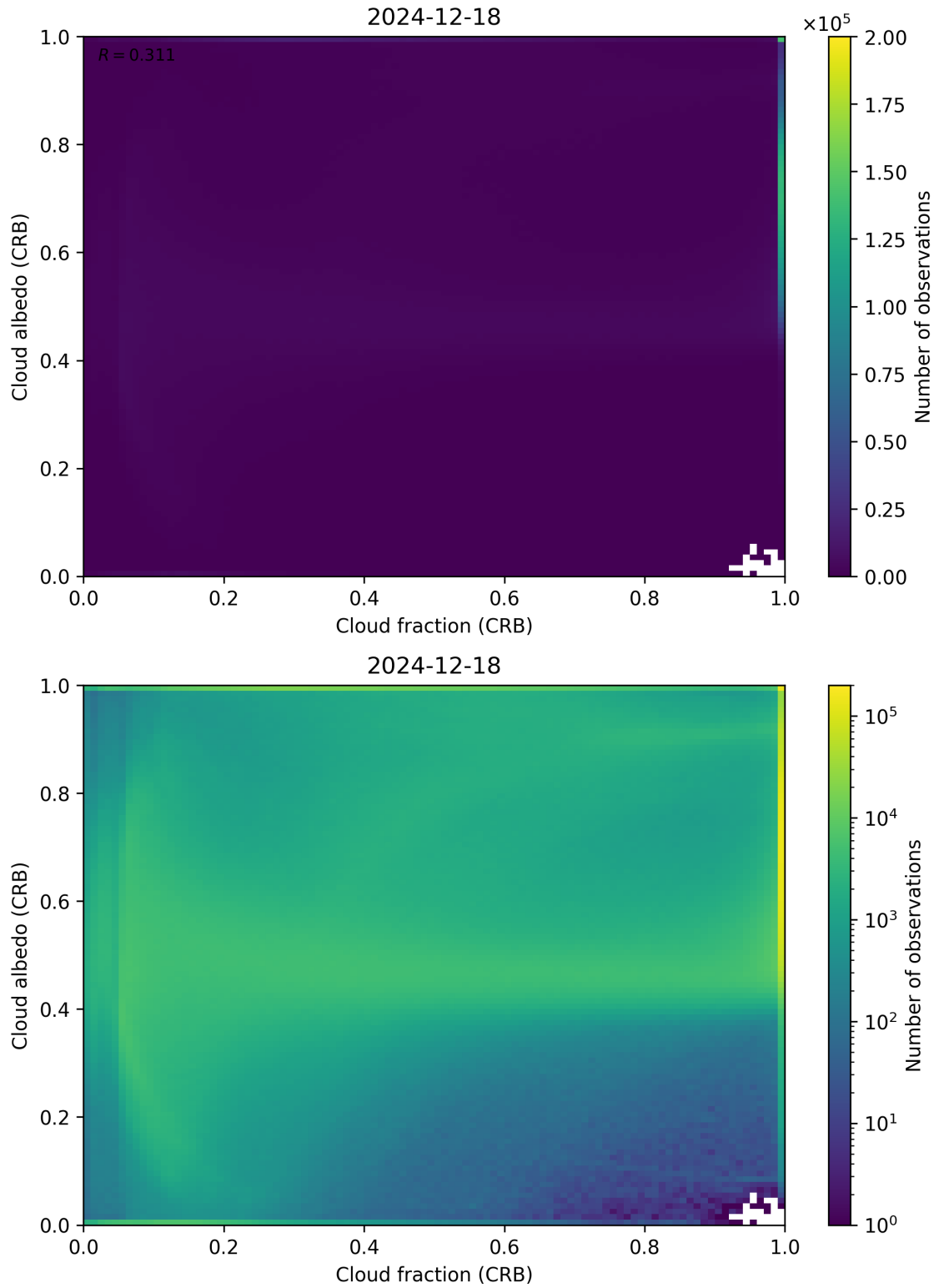
Figure 77: Scatter density plot of “Cloud fraction (CRB)” against “Cloud albedo (CRB)” for 2024-12-17 to 2024-12-19.
