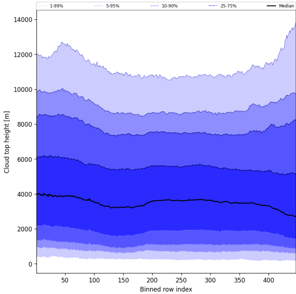
Figure 56: Along track statistics of “Cloud top height” for 2024-12-17 to 2024-12-19
