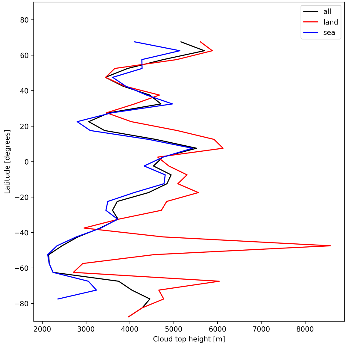
Figure 24: Zonal average of “Cloud top height” for 2024-12-23 to 2024-12-25.
