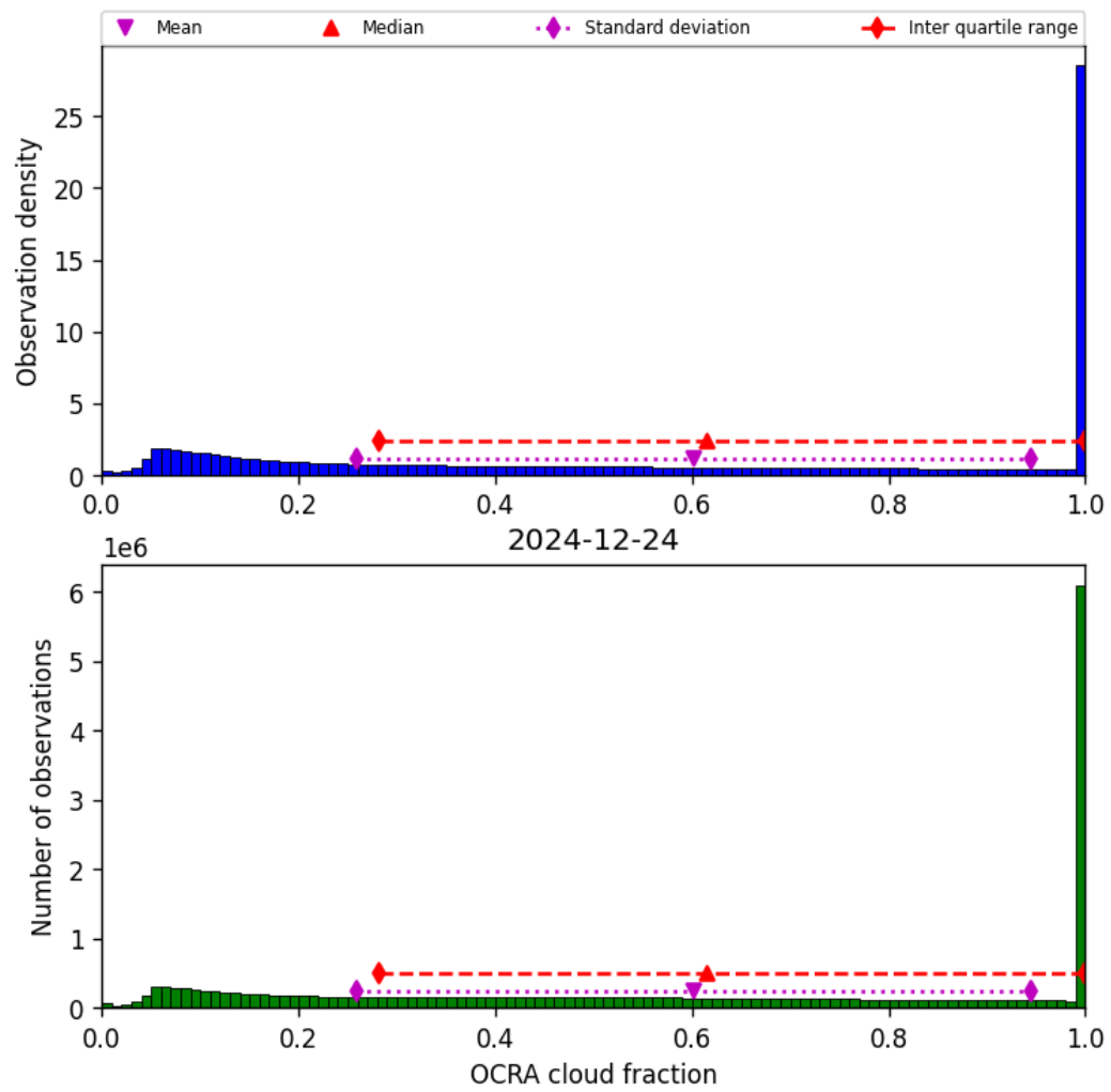
Figure 50: Histogram of “OCRA cloud fraction” for 2024-12-23 to 2024-12-25
