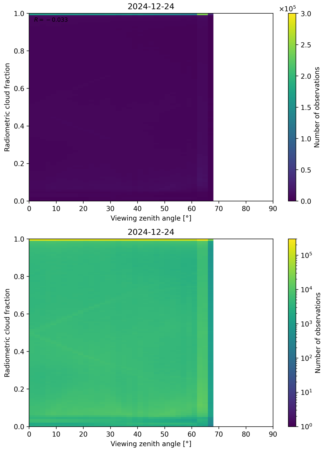
Figure 107: Scatter density plot of “Viewing zenith angle” against “Radiometric cloud fraction” for 2024-12-23 to 2024-12-25.
