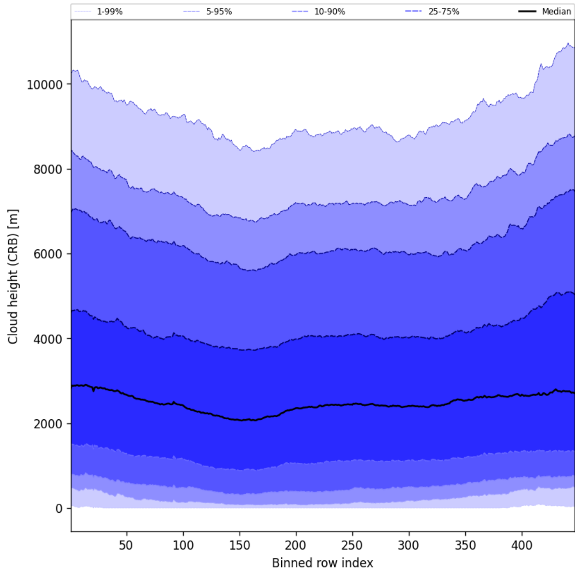
Figure 59: Along track statistics of “Cloud height (CRB)” for 2024-12-23 to 2024-12-25
