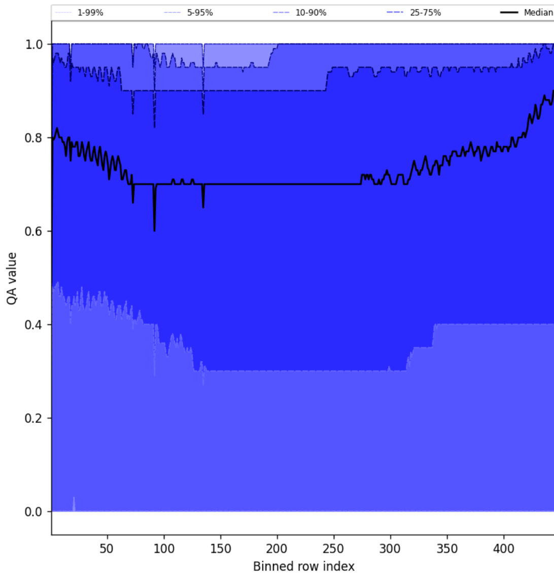
Figure 54: Along track statistics of “QA value” for 2024-12-23 to 2024-12-25
