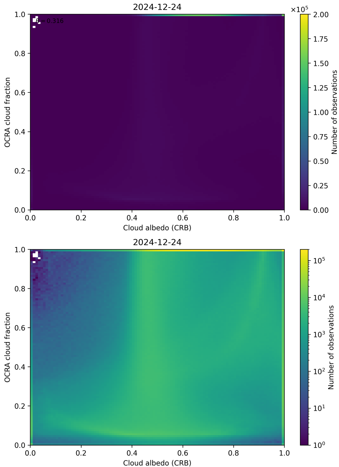
Figure 70: Scatter density plot of “Cloud albedo (CRB)” against “OCRA cloud fraction” for 2024-12-23 to 2024-12-25.
