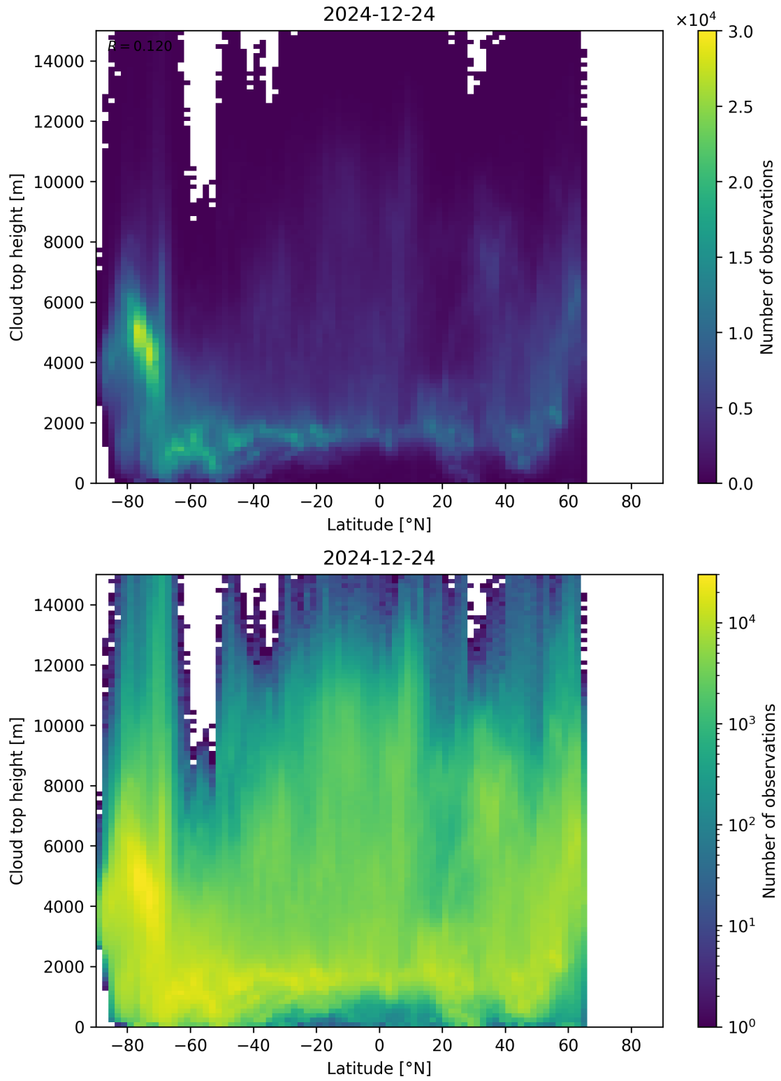
Figure 97: Scatter density plot of “Latitude” against “Cloud top height” for 2024-12-23 to 2024-12-25.
