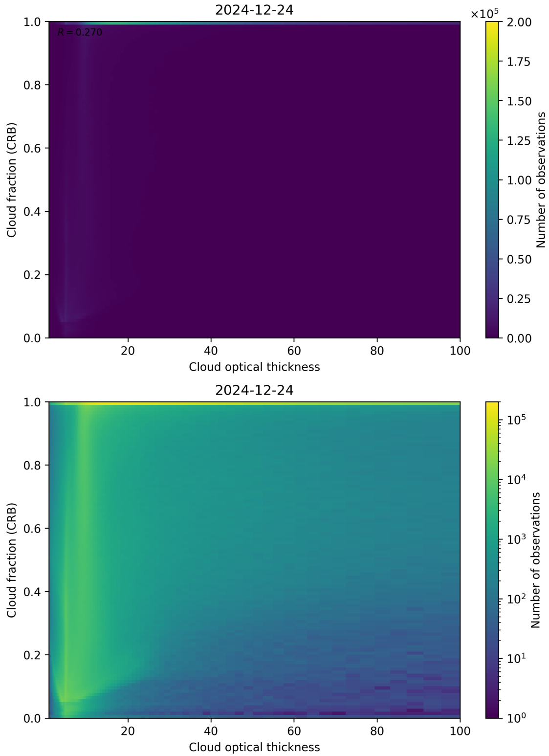
Figure 84: Scatter density plot of “Cloud optical thickness” against “Cloud fraction (CRB)” for 2024-12-23 to 2024-12-25.
