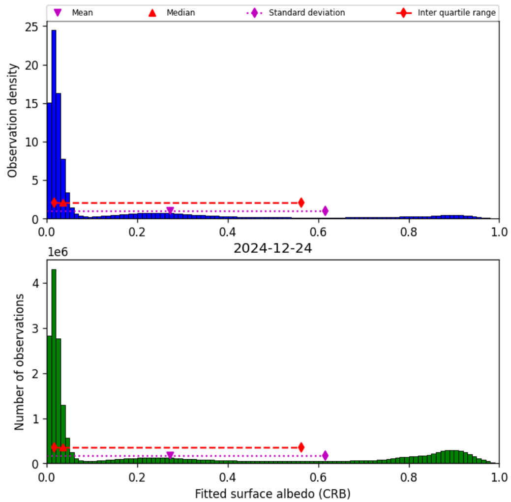
Figure 46: Histogram of “Fitted surface albedo (CRB)” for 2024-12-23 to 2024-12-25
