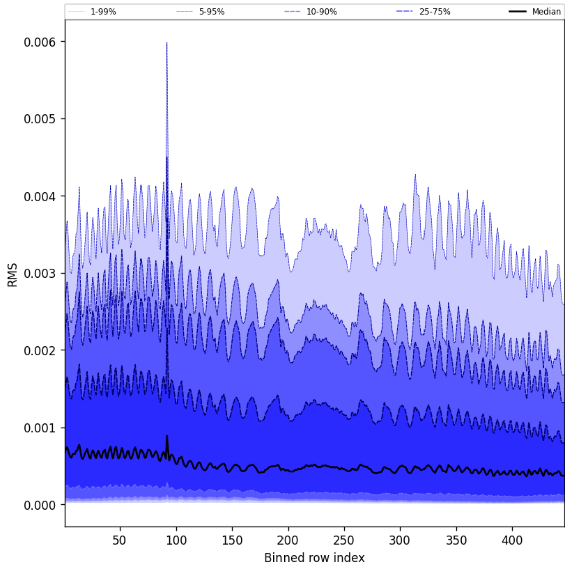
Figure 63: Along track statistics of “RMS” for 2024-12-23 to 2024-12-25
