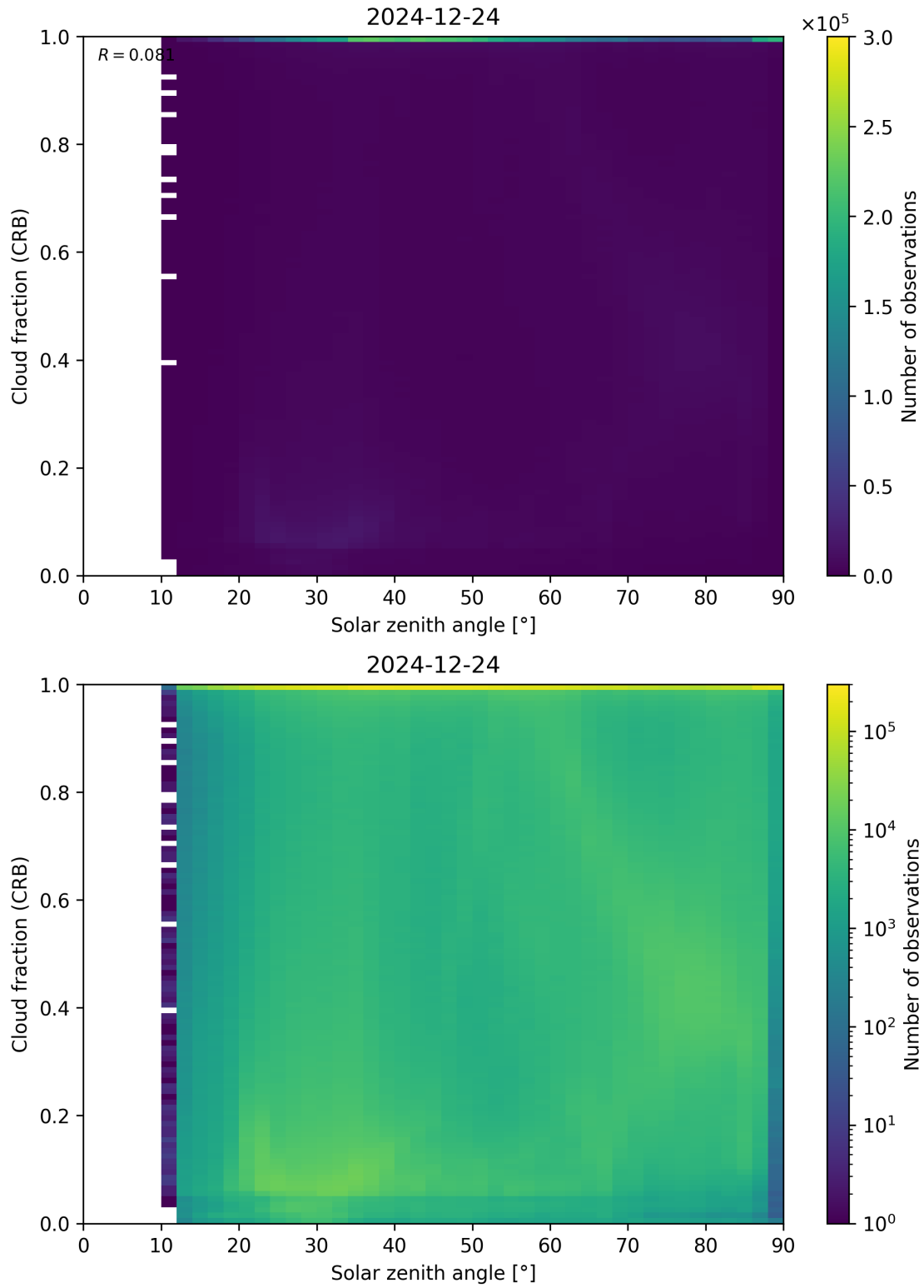
Figure 101: Scatter density plot of “Solar zenith angle” against “Cloud fraction (CRB)” for 2024-12-23 to 2024-12-25.
