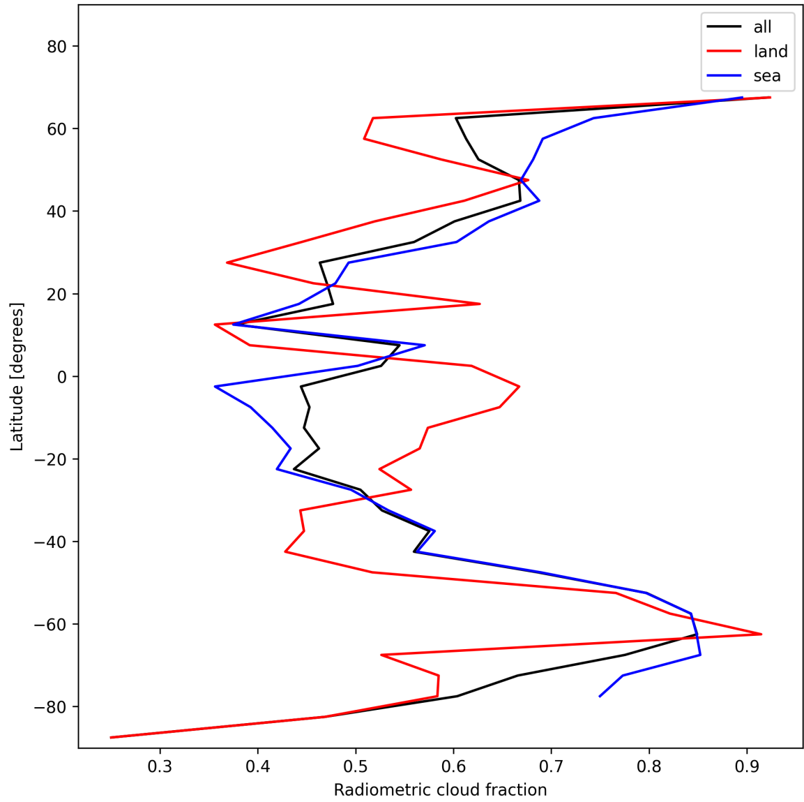
Figure 23: Zonal average of “Radiometric cloud fraction” for 2024-12-23 to 2024-12-25.
