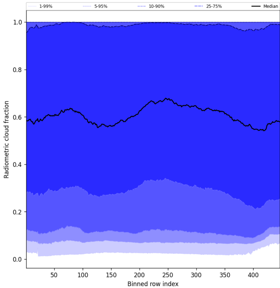
Figure 55: Along track statistics of “Radiometric cloud fraction” for 2024-12-23 to 2024-12-25
