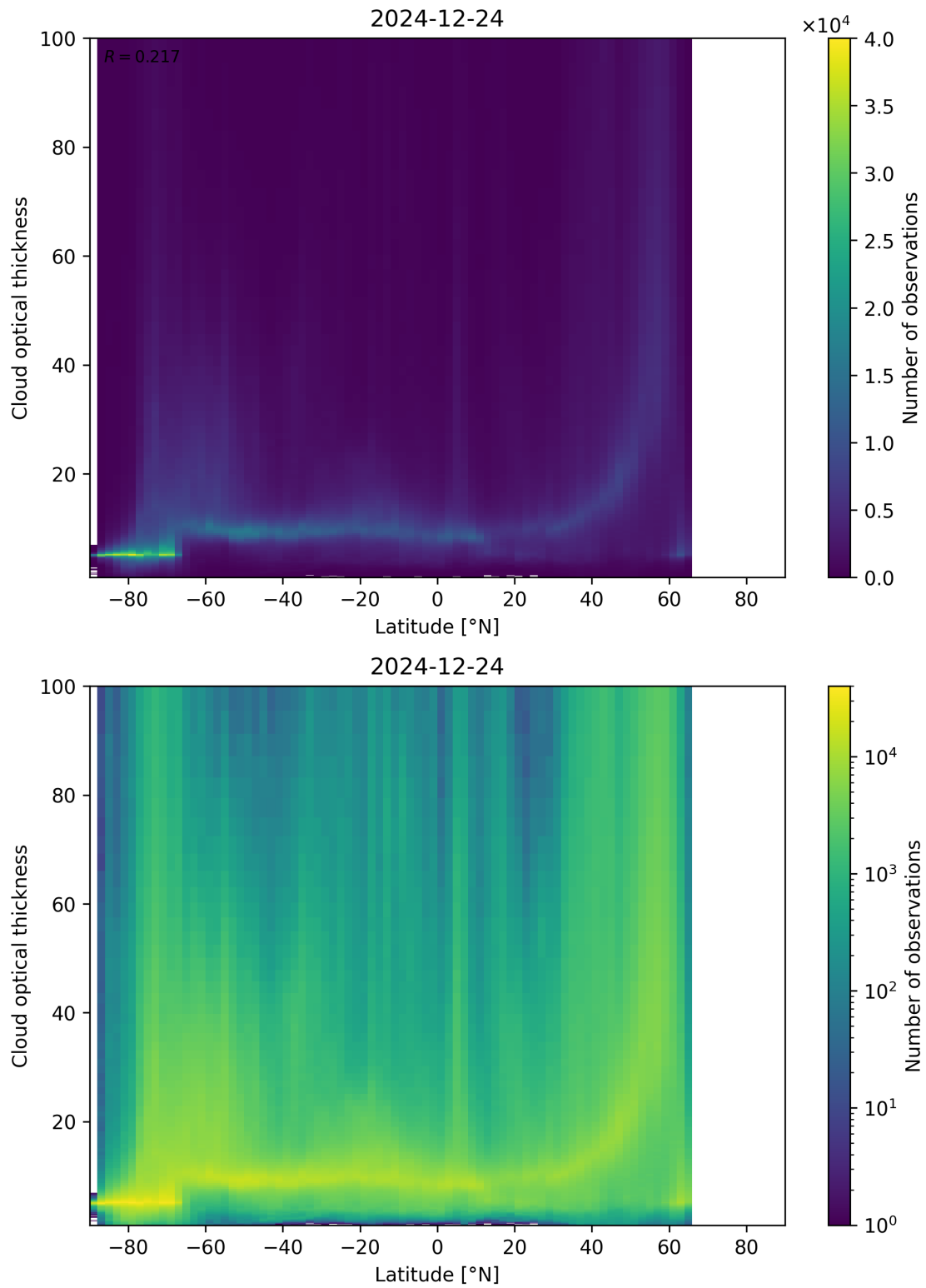
Figure 96: Scatter density plot of “Latitude” against “Cloud optical thickness” for 2024-12-23 to 2024-12-25.
