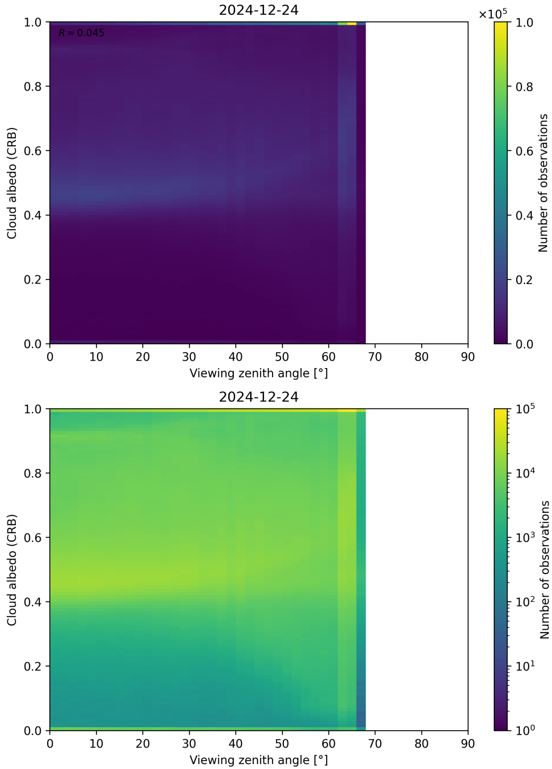
Figure 106: Scatter density plot of “Viewing zenith angle” against “Cloud albedo (CRB)” for 2024-12-23 to 2024-12-25.
