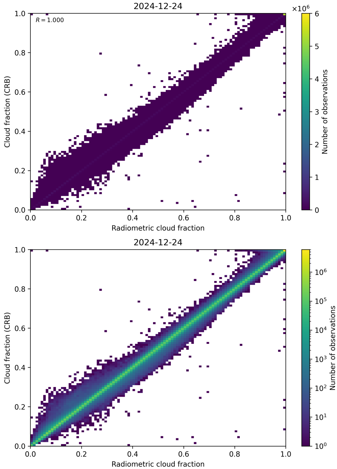
Figure 73: Scatter density plot of “Radiometric cloud fraction” against “Cloud fraction (CRB)” for 2024-12-23 to 2024-12-25.
