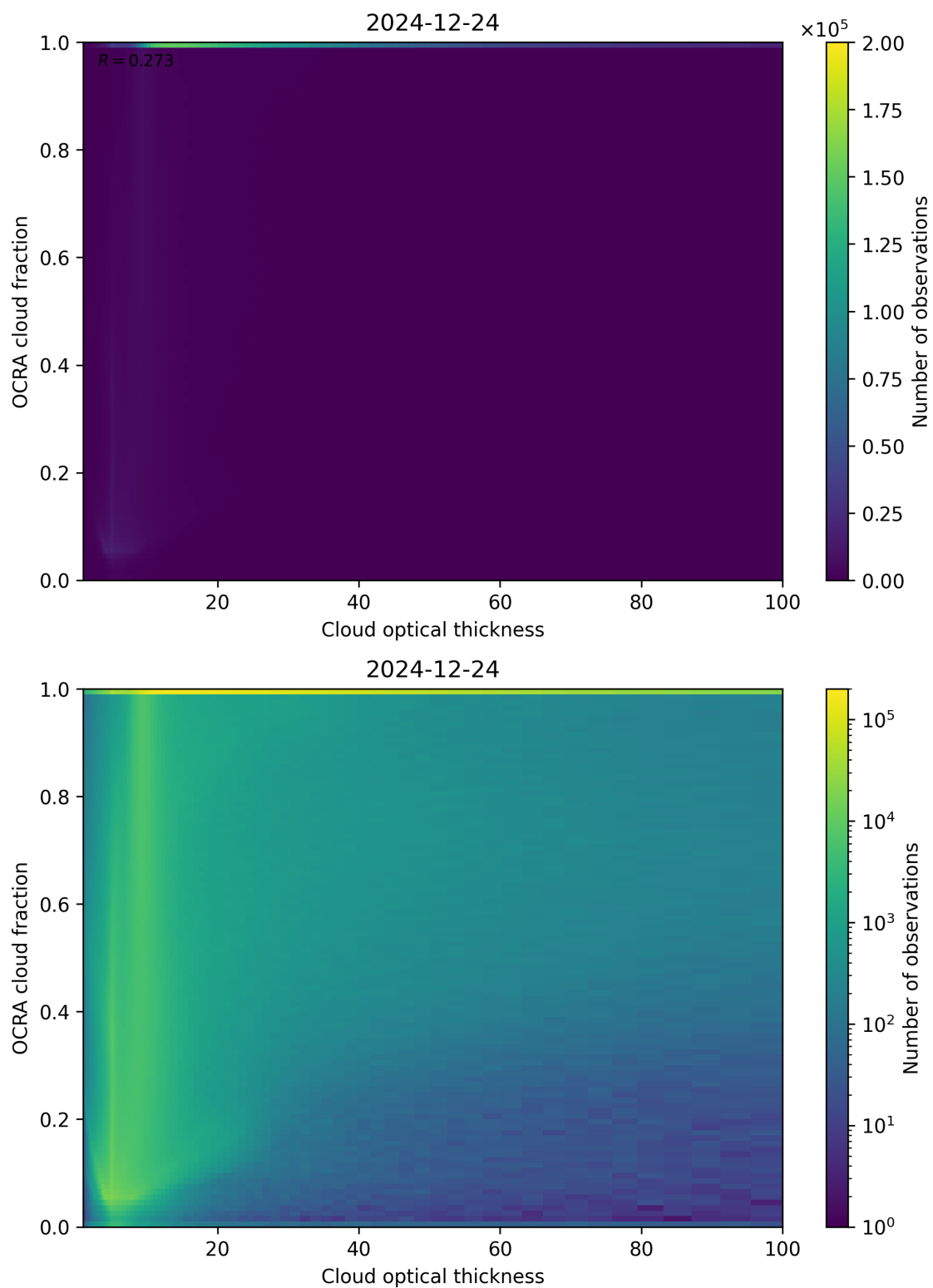
Figure 83: Scatter density plot of “Cloud optical thickness” against “OCRA cloud fraction” for 2024-12-23 to 2024-12-25.
