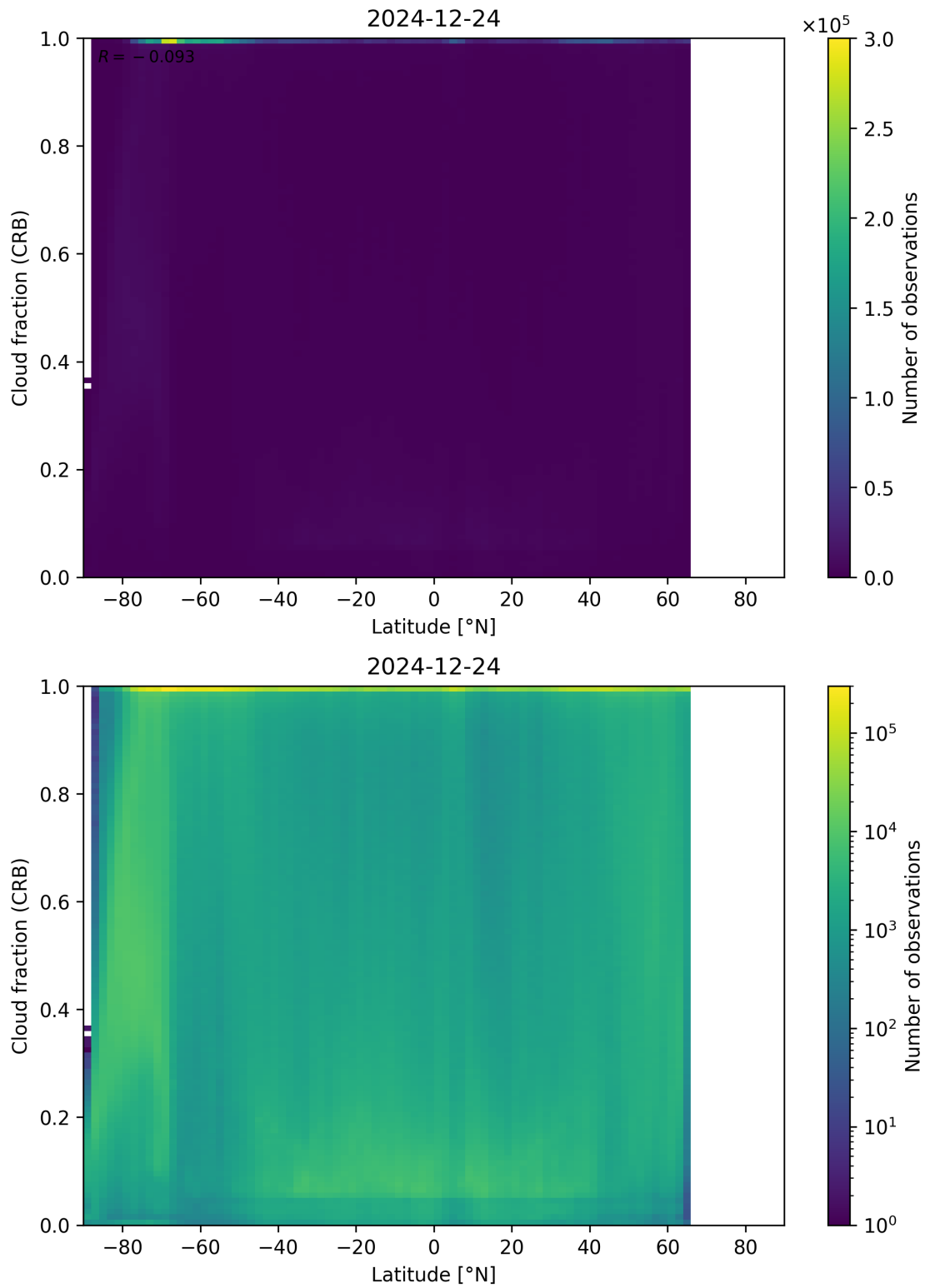
Figure 94: Scatter density plot of “Latitude” against “Cloud fraction (CRB)” for 2024-12-23 to 2024-12-25.
