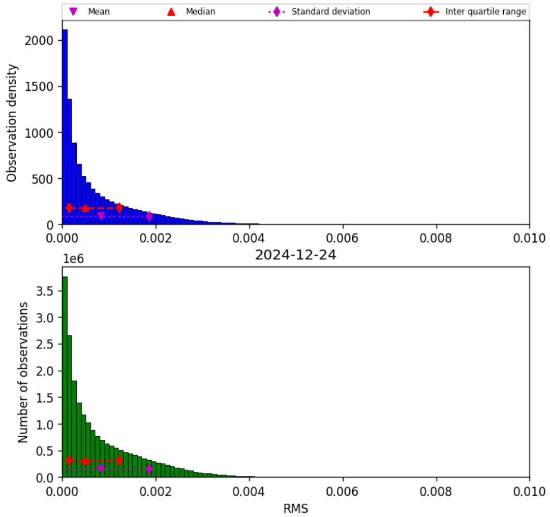
Figure 47: Histogram of “RMS” for 2024-12-23 to 2024-12-25
