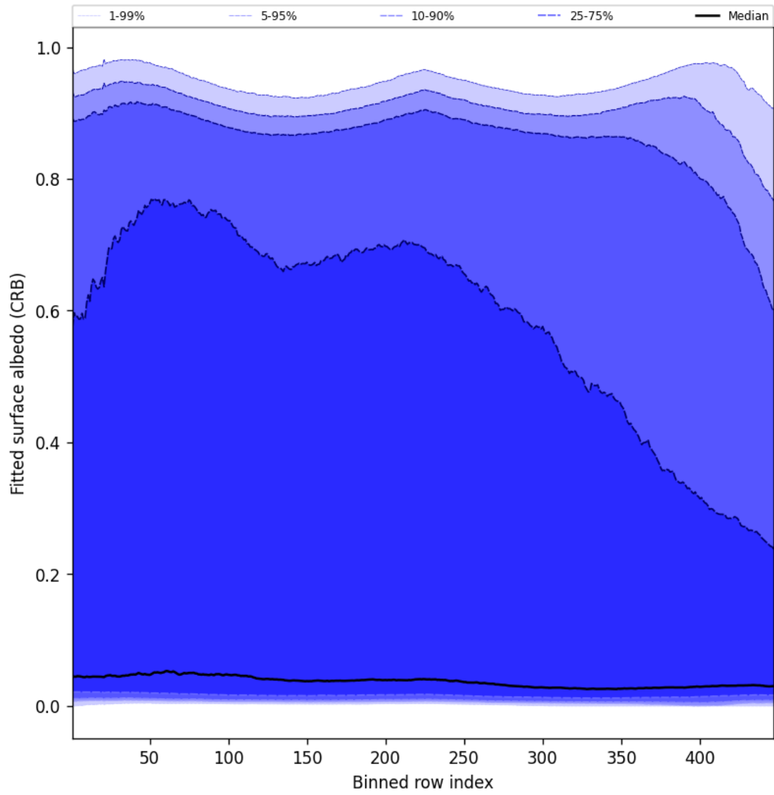
Figure 62: Along track statistics of “Fitted surface albedo (CRB)” for 2024-12-23 to 2024-12-25
