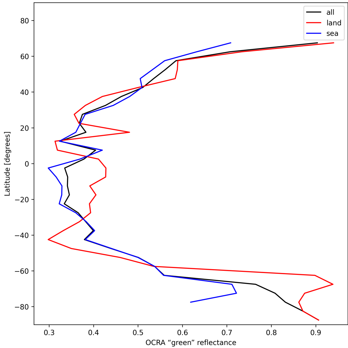
Figure 36: Zonal average of “OCRA “green” reflectance” for 2024-12-23 to 2024-12-25.
