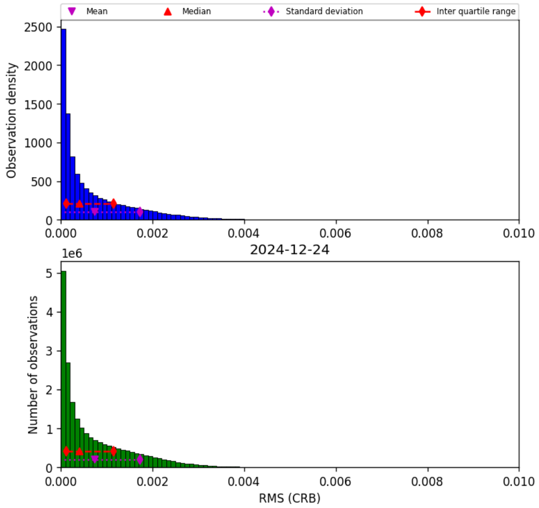
Figure 48: Histogram of “RMS (CRB)” for 2024-12-23 to 2024-12-25
