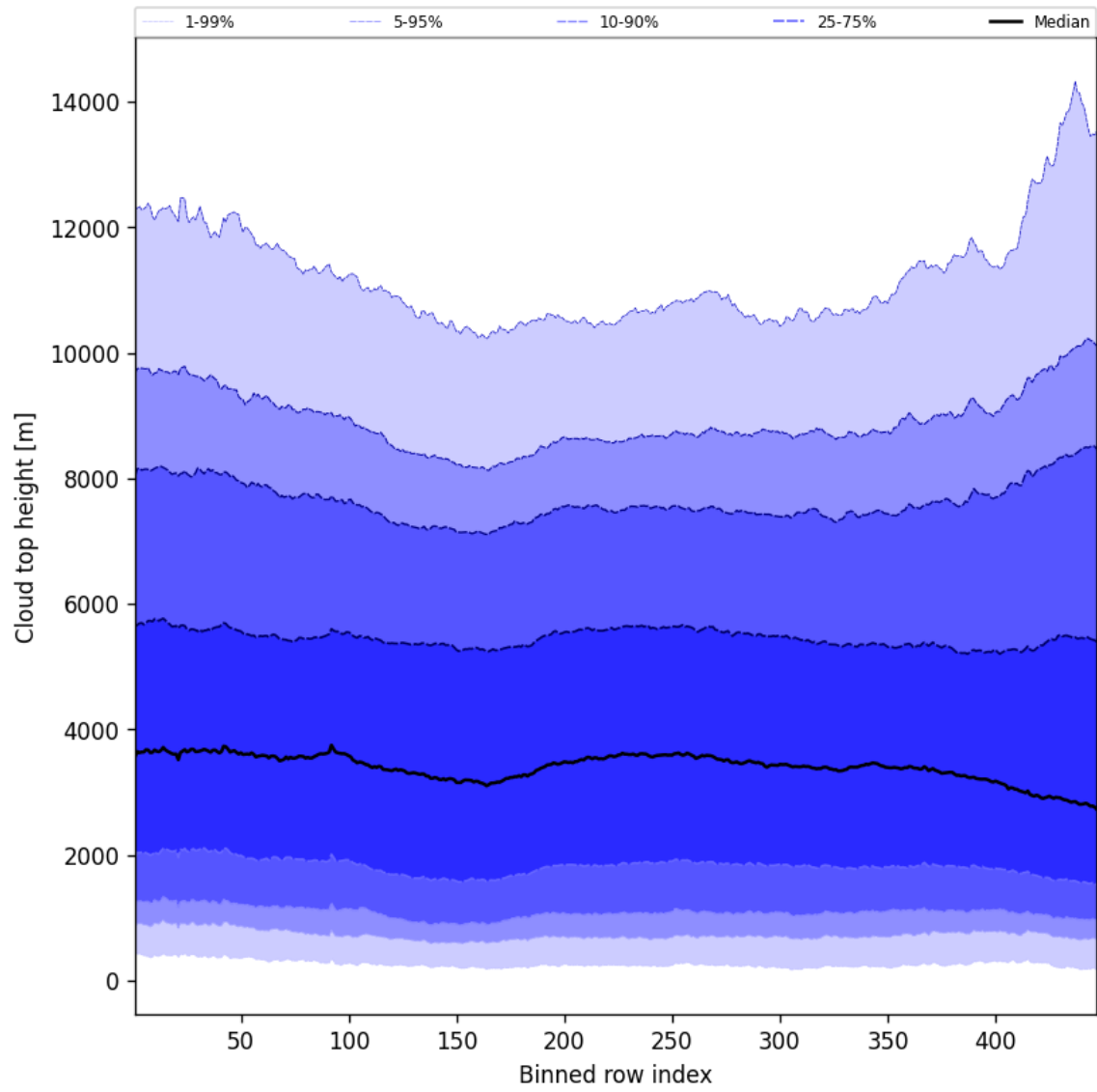
Figure 56: Along track statistics of “Cloud top height” for 2024-12-23 to 2024-12-25
