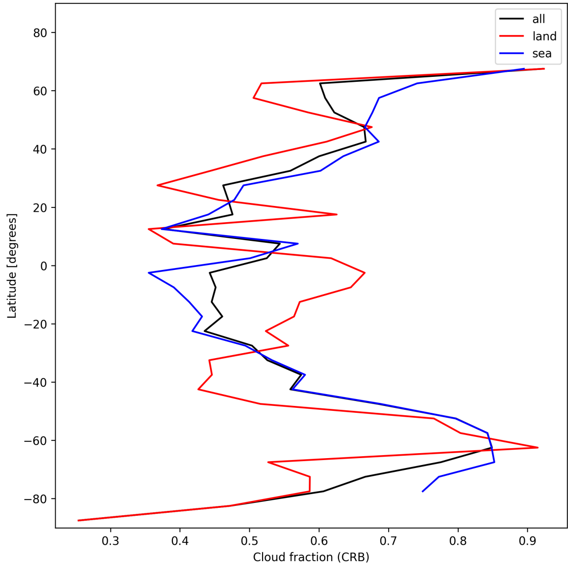
Figure 26: Zonal average of “Cloud fraction (CRB)” for 2024-12-23 to 2024-12-25.
