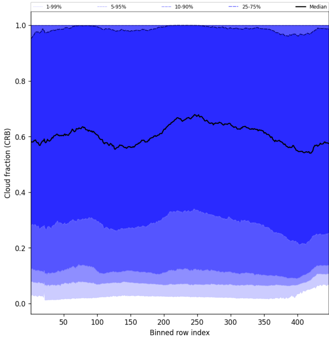
Figure 58: Along track statistics of “Cloud fraction (CRB)” for 2024-12-23 to 2024-12-25
