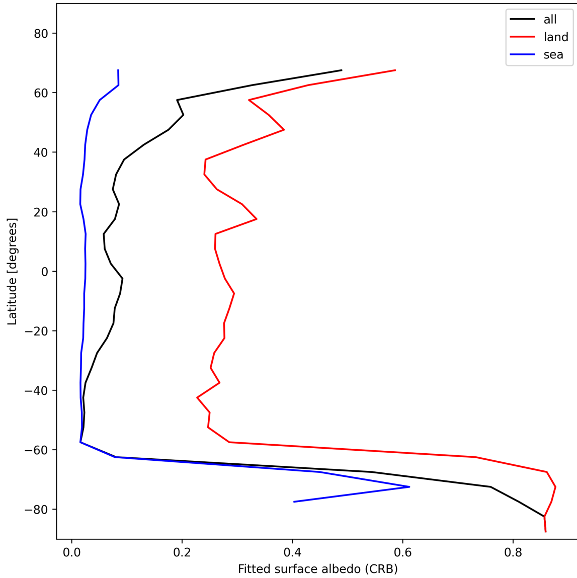
Figure 30: Zonal average of “Fitted surface albedo (CRB)” for 2024-12-23 to 2024-12-25.
