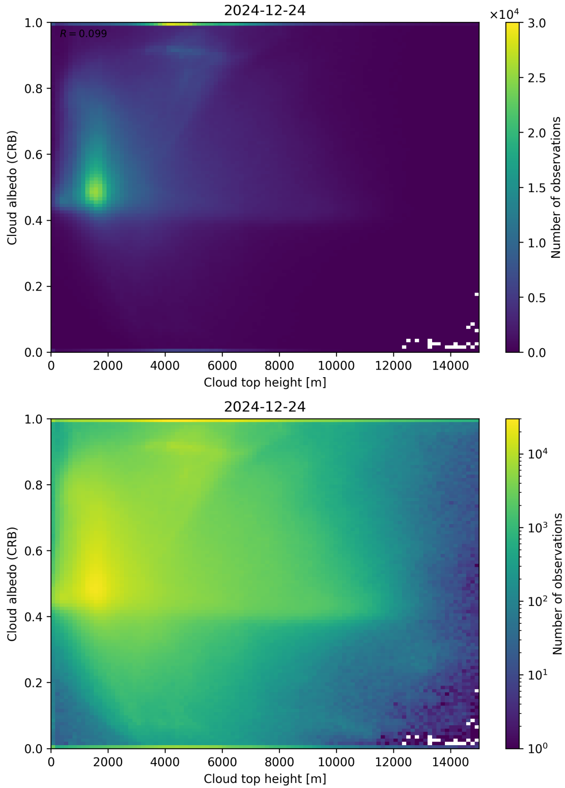
Figure 86: Scatter density plot of “Cloud top height” against “Cloud albedo (CRB)” for 2024-12-23 to 2024-12-25.
