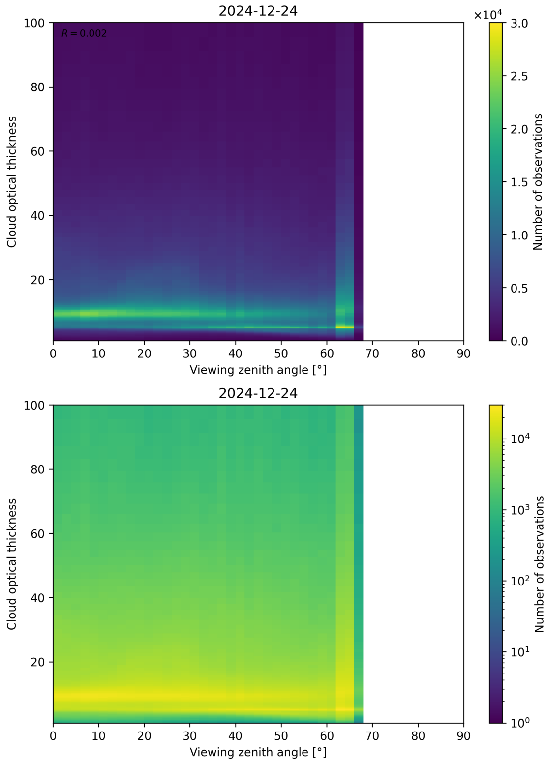
Figure 111: Scatter density plot of “Viewing zenith angle” against “Cloud optical thickness” for 2024-12-23 to 2024-12-25.
