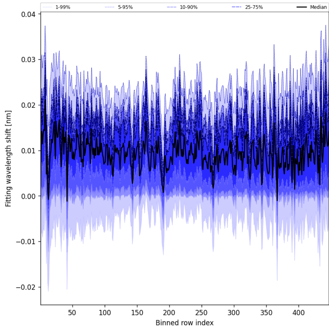
Figure 65: Along track statistics of “Fitting wavelength shift” for 2024-12-23 to 2024-12-25
