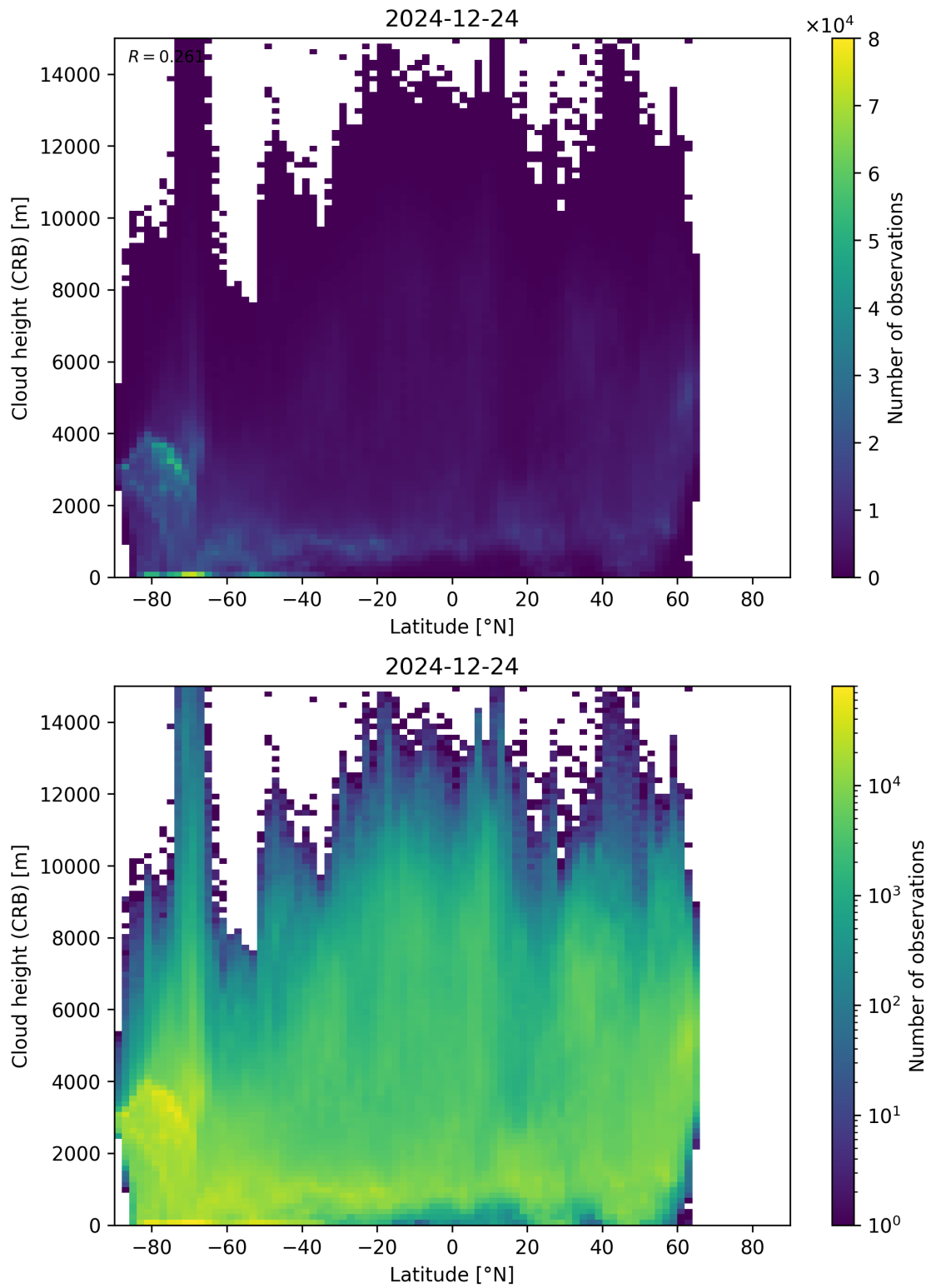
Figure 95: Scatter density plot of “Latitude” against “Cloud height (CRB)” for 2024-12-23 to 2024-12-25.
