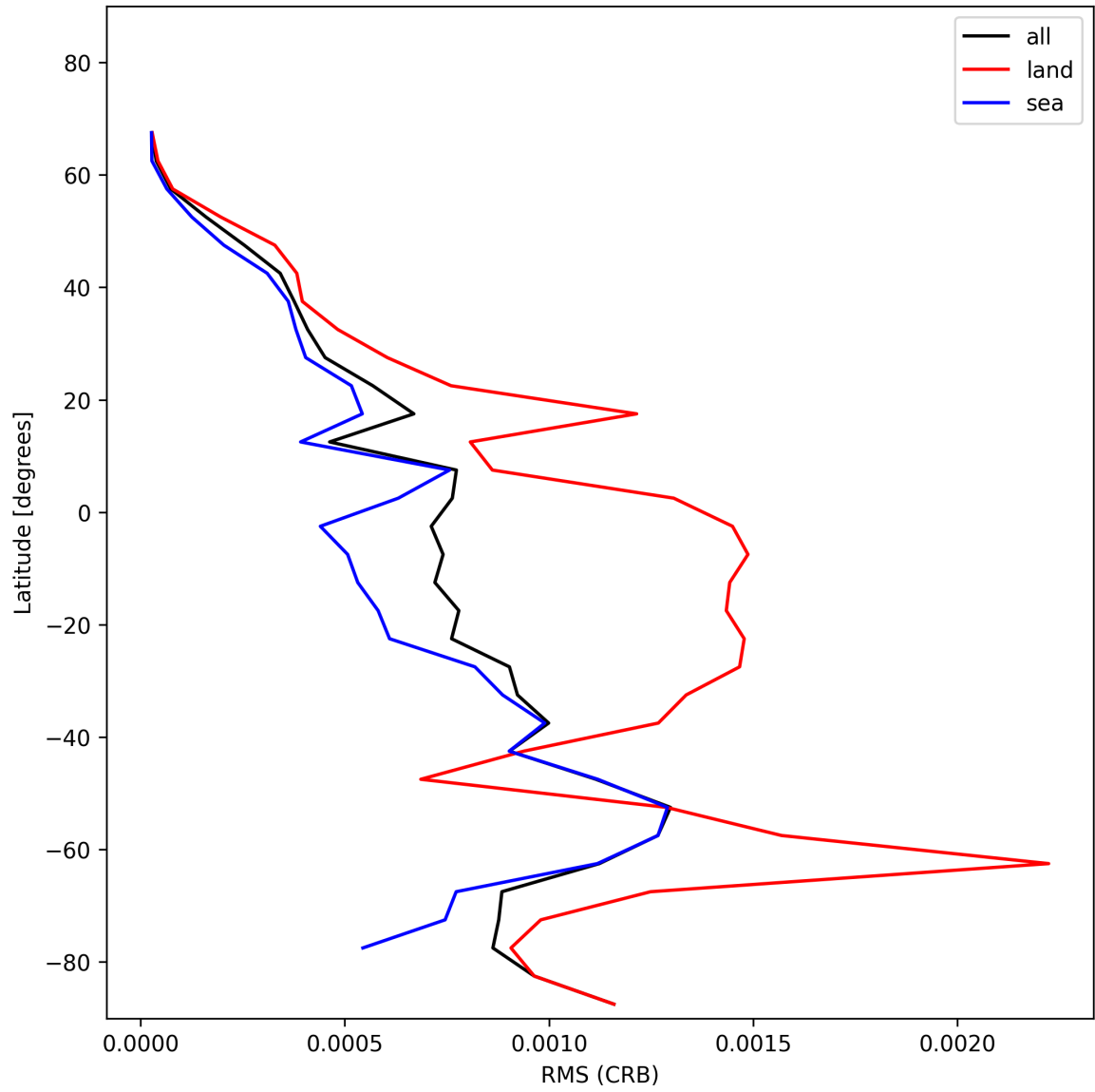
Figure 32: Zonal average of “RMS (CRB)” for 2024-12-23 to 2024-12-25.
