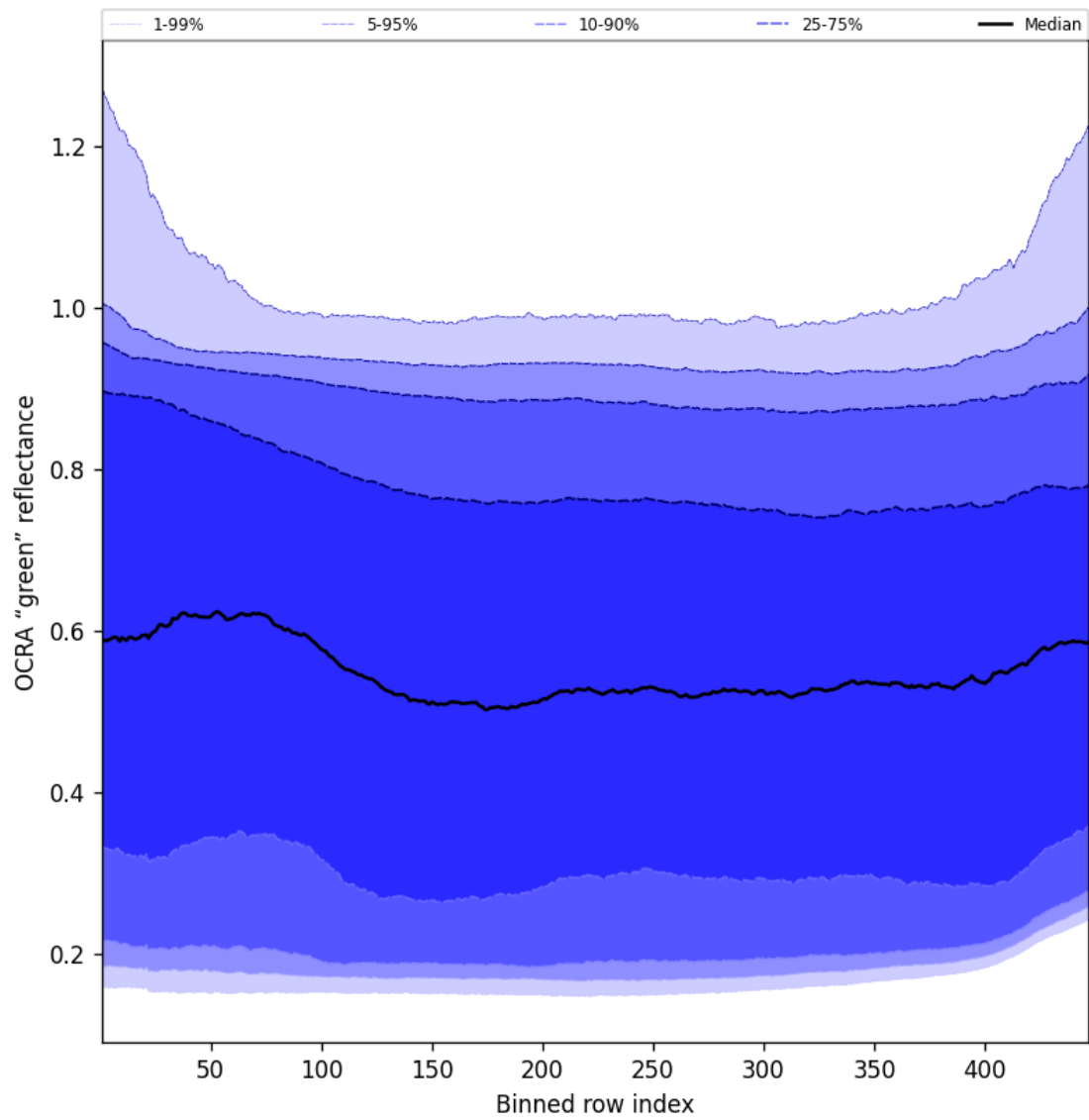
Figure 68: Along track statistics of “OCRA “green” reflectance” for 2024-12-23 to 2024-12-25
