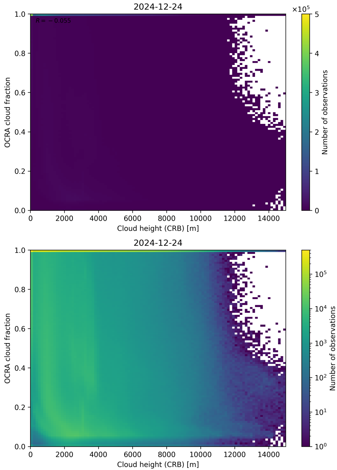
Figure 81: Scatter density plot of “Cloud height (CRB)” against “OCRA cloud fraction” for 2024-12-23 to 2024-12-25.
