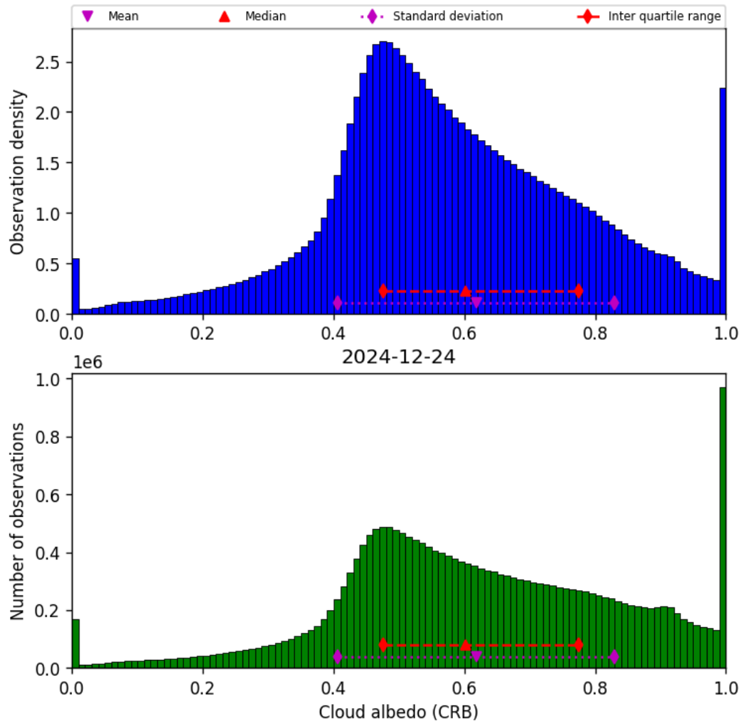
Figure 44: Histogram of “Cloud albedo (CRB)” for 2024-12-23 to 2024-12-25
