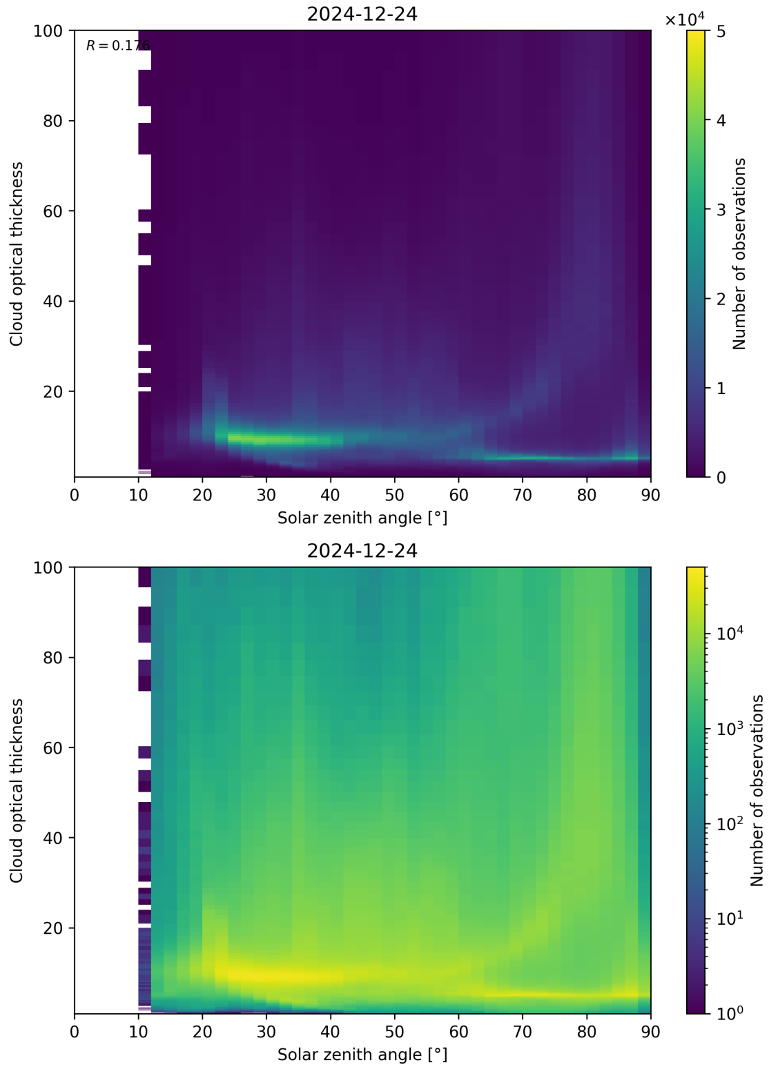
Figure 103: Scatter density plot of “Solar zenith angle” against “Cloud optical thickness” for 2024-12-23 to 2024-12-25.
