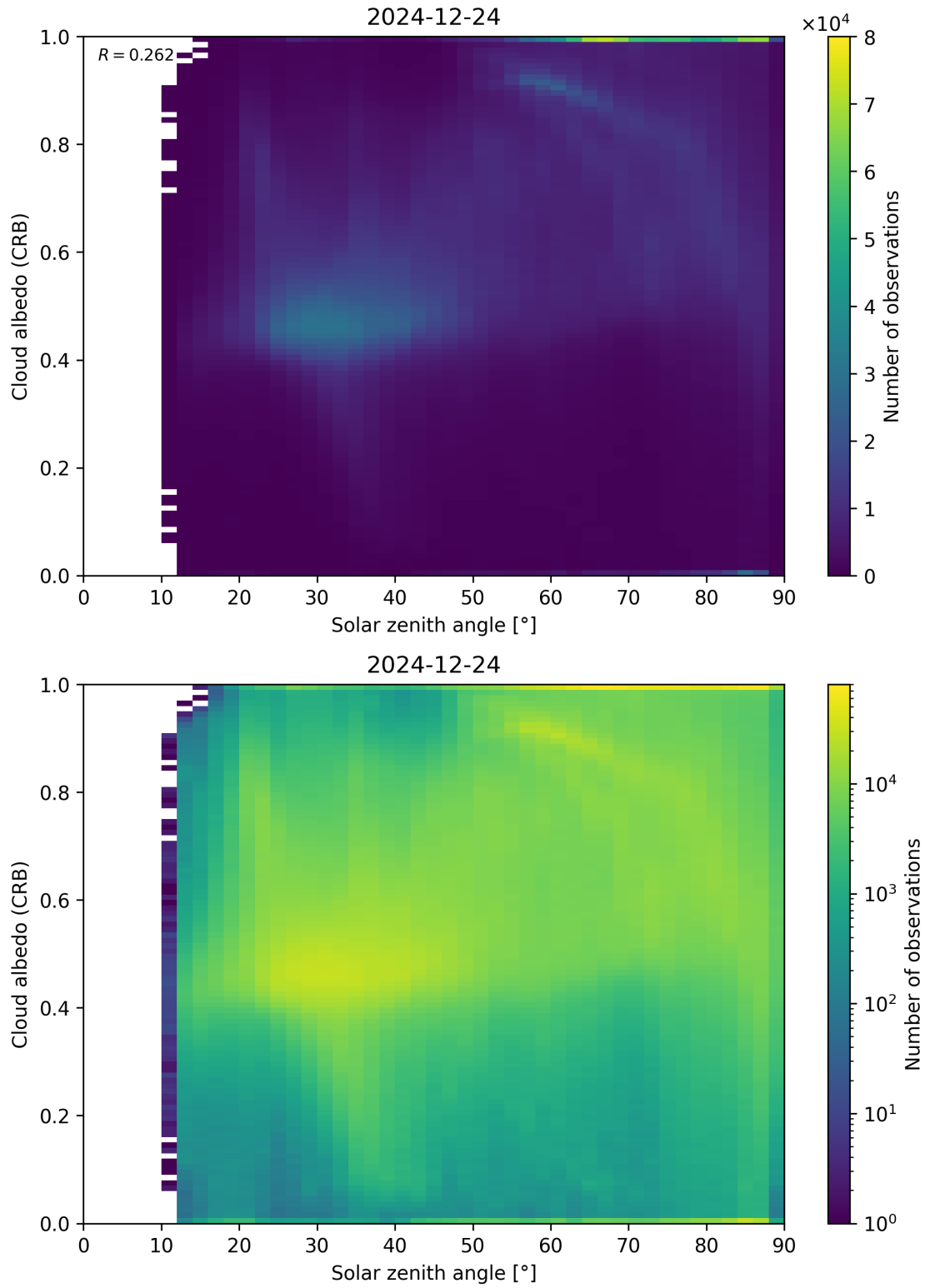
Figure 98: Scatter density plot of “Solar zenith angle” against “Cloud albedo (CRB)” for 2024-12-23 to 2024-12-25.
