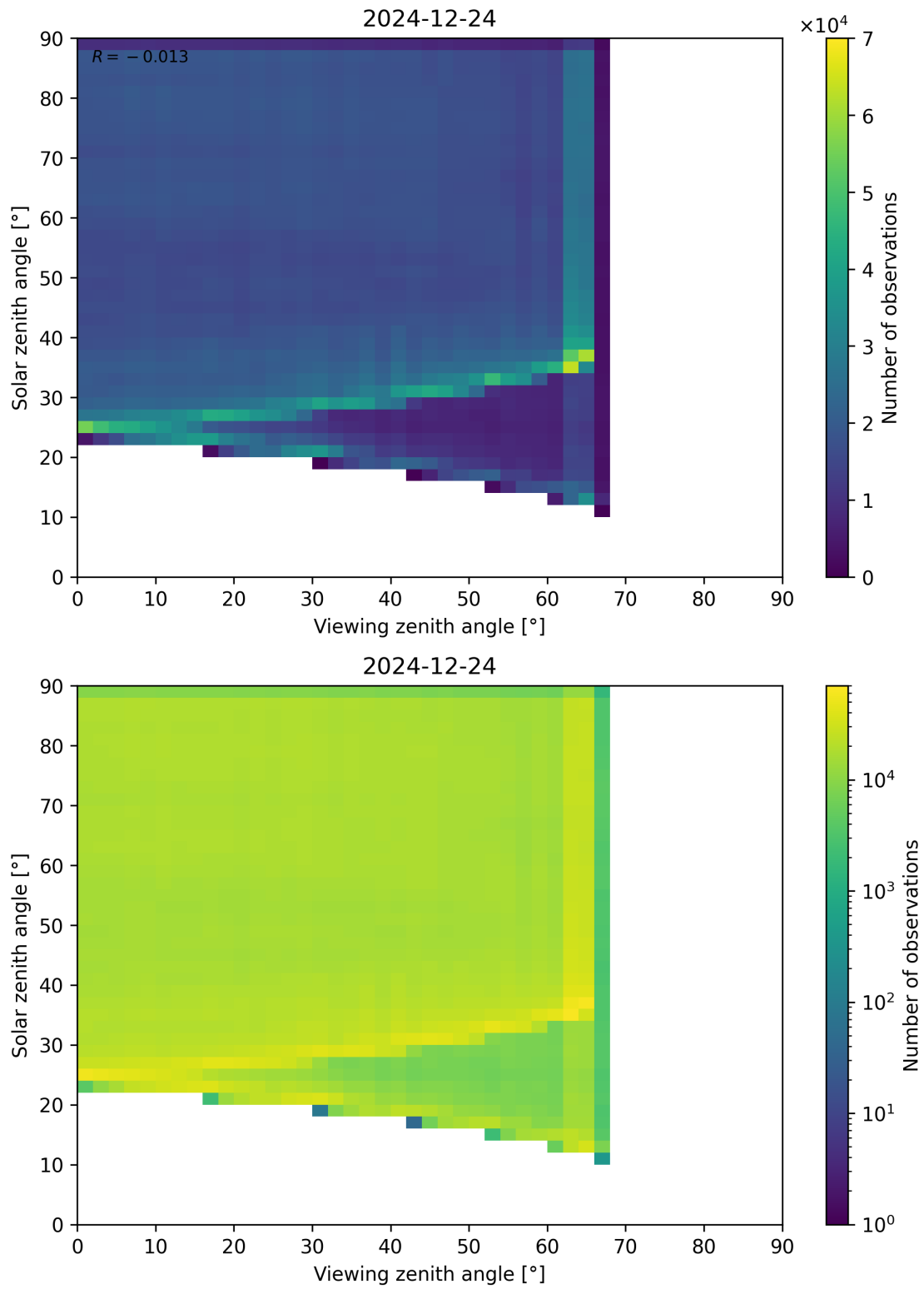
Figure 114: Scatter density plot of “Viewing zenith angle” against “Solar zenith angle” for 2024-12-23 to 2024-12-25.
