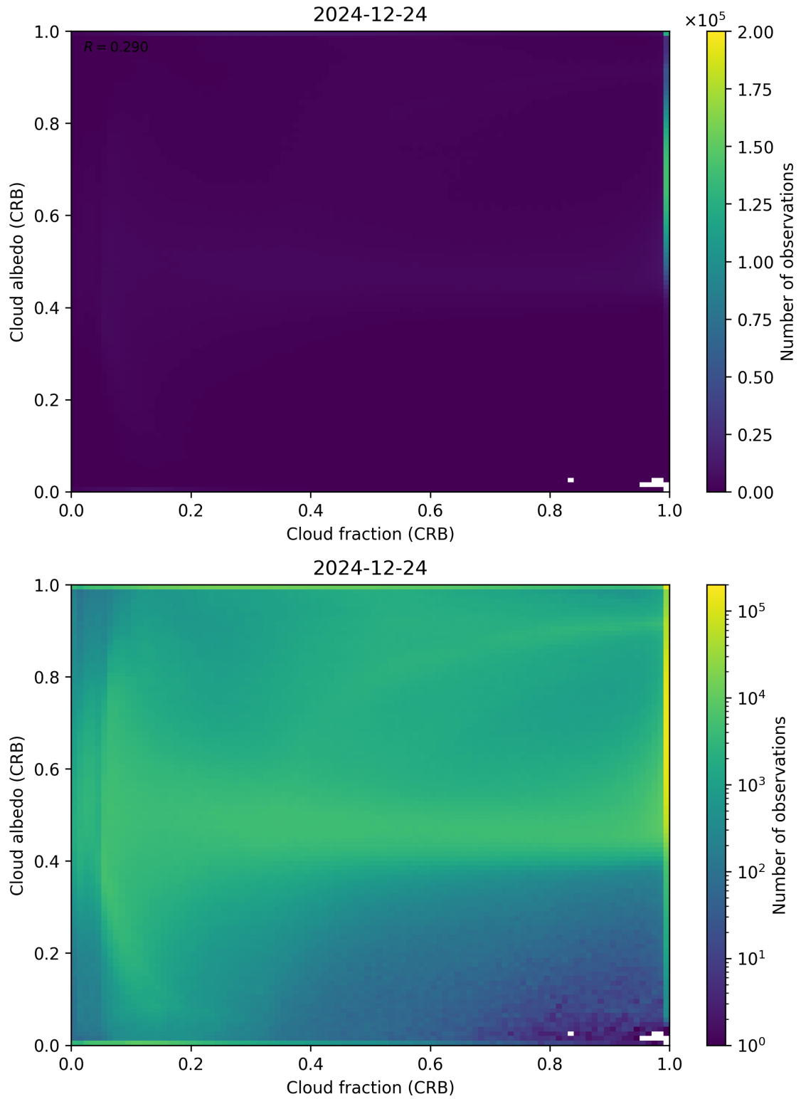
Figure 77: Scatter density plot of “Cloud fraction (CRB)” against “Cloud albedo (CRB)” for 2024-12-23 to 2024-12-25.
