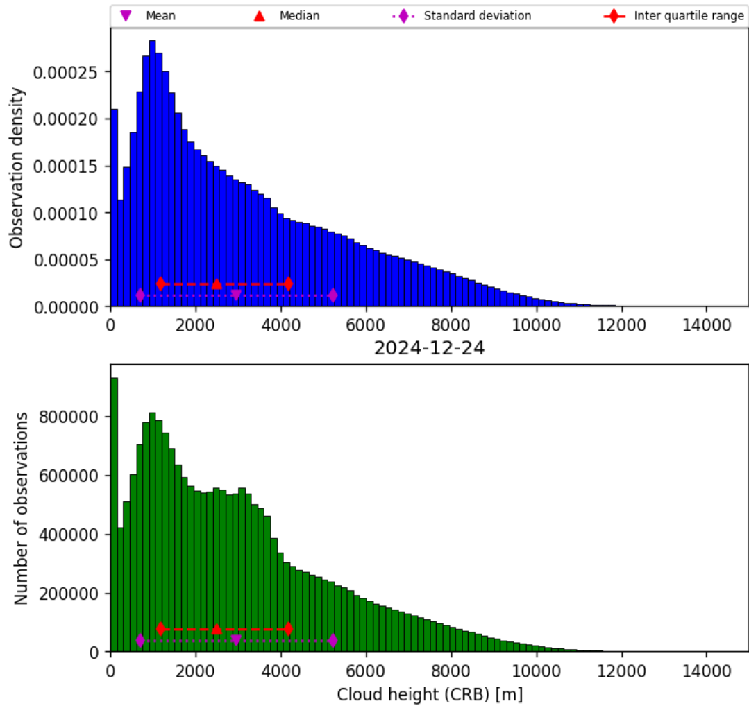
Figure 43: Histogram of “Cloud height (CRB)” for 2024-12-23 to 2024-12-25
