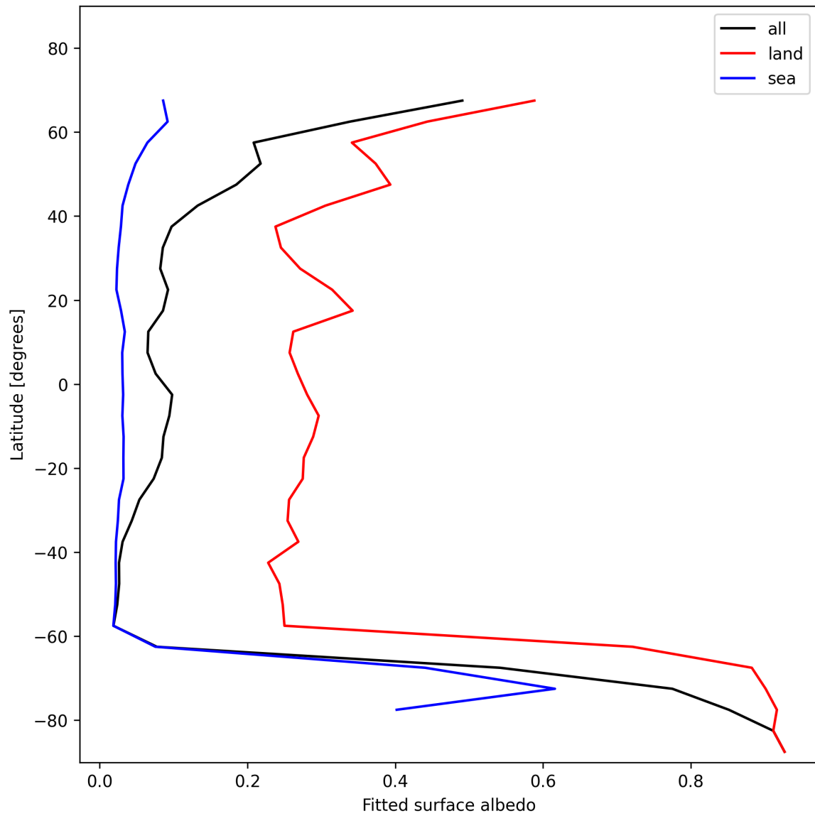
Figure 29: Zonal average of “Fitted surface albedo” for 2024-12-23 to 2024-12-25.
