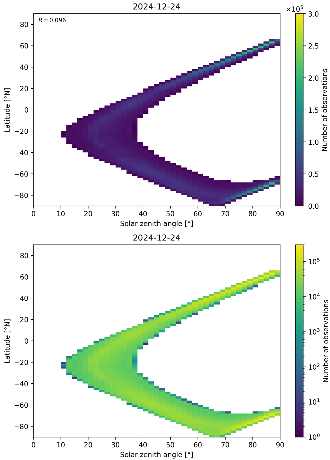
Figure 105: Scatter density plot of “Solar zenith angle” against “Latitude” for 2024-12-23 to 2024-12-25.
