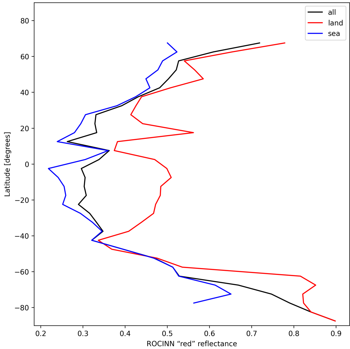
Figure 37: Zonal average of “ROCINN “red” reflectance” for 2024-12-23 to 2024-12-25.
