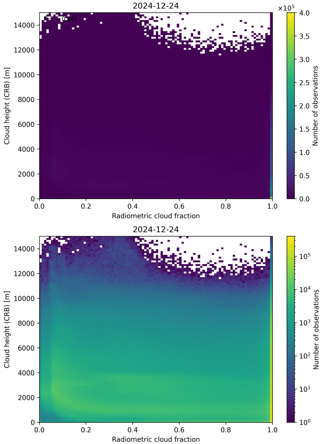
Figure 74: Scatter density plot of “Radiometric cloud fraction” against “Cloud height (CRB)” for 2024-12-23 to 2024-12-25.
