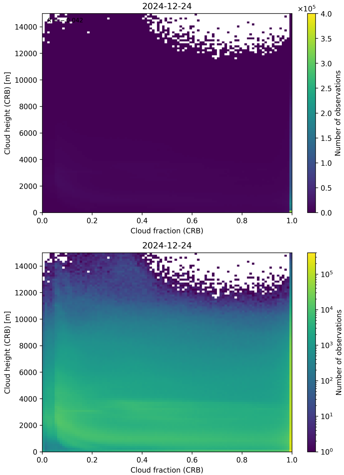
Figure 79: Scatter density plot of “Cloud fraction (CRB)” against “Cloud height (CRB)” for 2024-12-23 to 2024-12-25.
