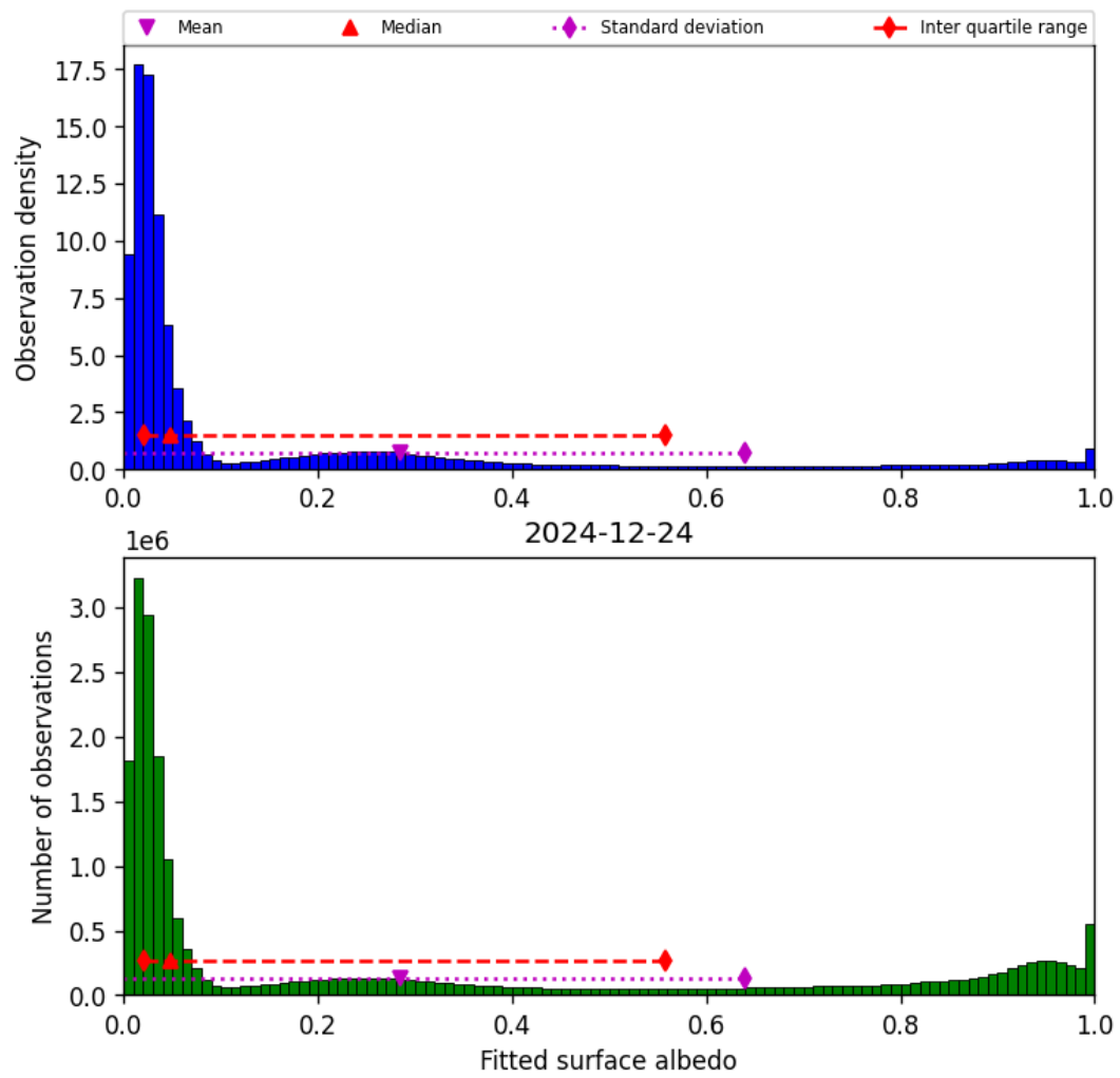
Figure 45: Histogram of “Fitted surface albedo” for 2024-12-23 to 2024-12-25
