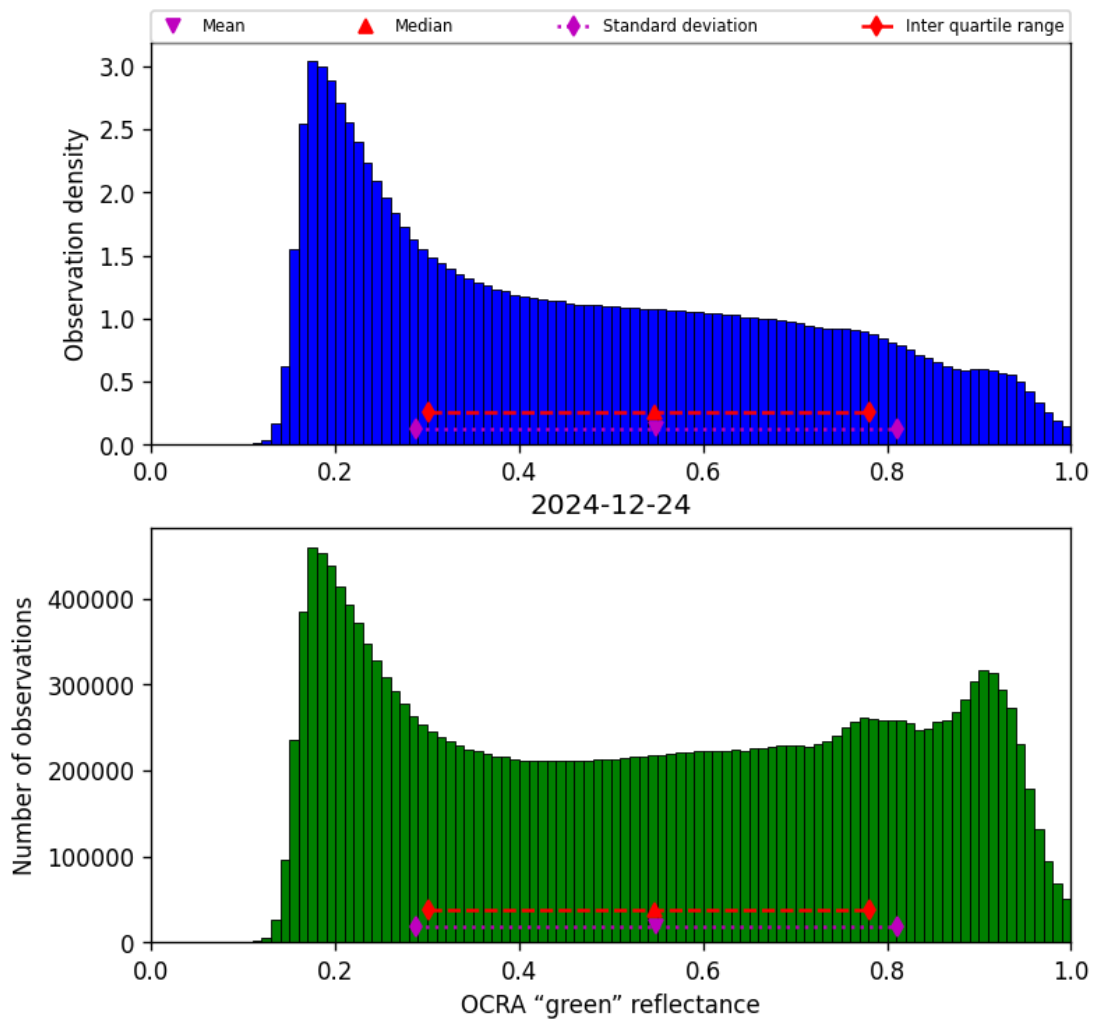
Figure 52: Histogram of “OCRA “green” reflectance” for 2024-12-23 to 2024-12-25
