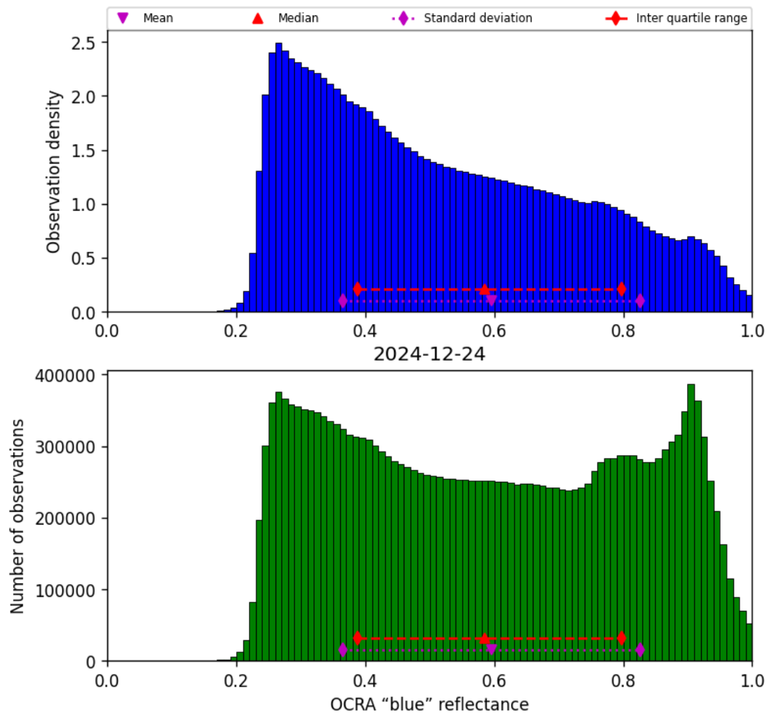
Figure 51: Histogram of “OCRA “blue” reflectance” for 2024-12-23 to 2024-12-25
