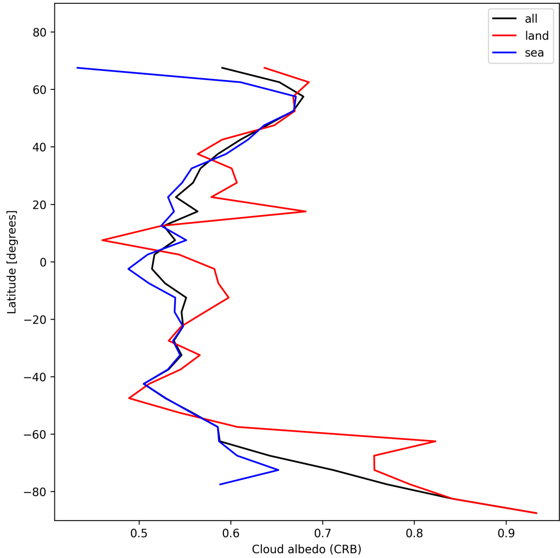
Figure 28: Zonal average of “Cloud albedo (CRB)” for 2024-12-23 to 2024-12-25.
