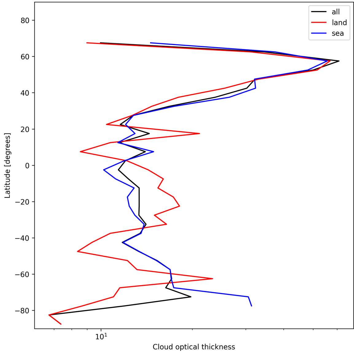
Figure 25: Zonal average of “Cloud optical thickness” for 2024-12-23 to 2024-12-25.
