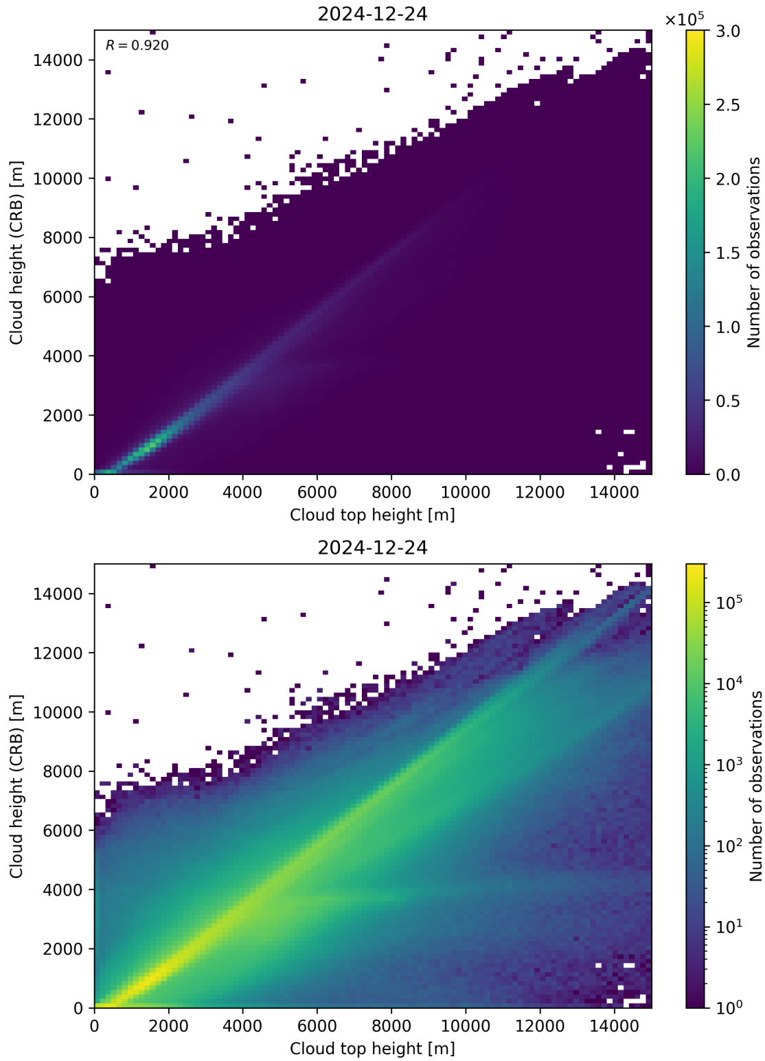
Figure 89: Scatter density plot of “Cloud top height” against “Cloud height (CRB)” for 2024-12-23 to 2024-12-25.
