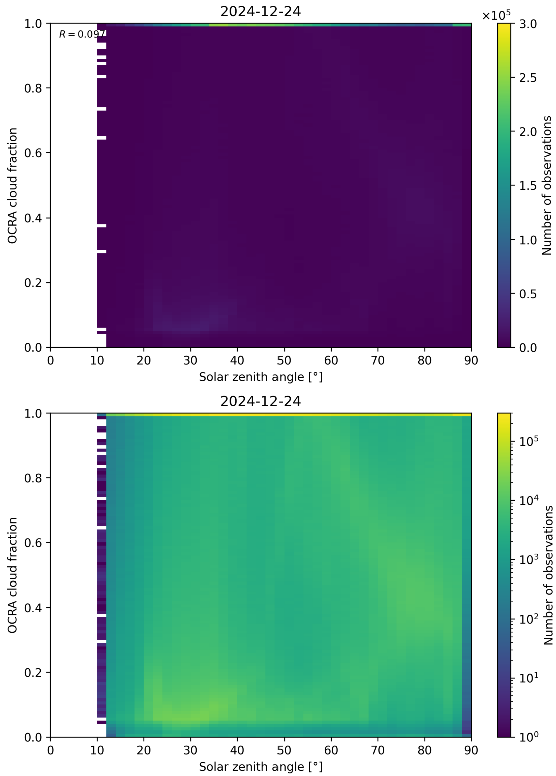
Figure 100: Scatter density plot of “Solar zenith angle” against “OCRA cloud fraction” for 2024-12-23 to 2024-12-25.
