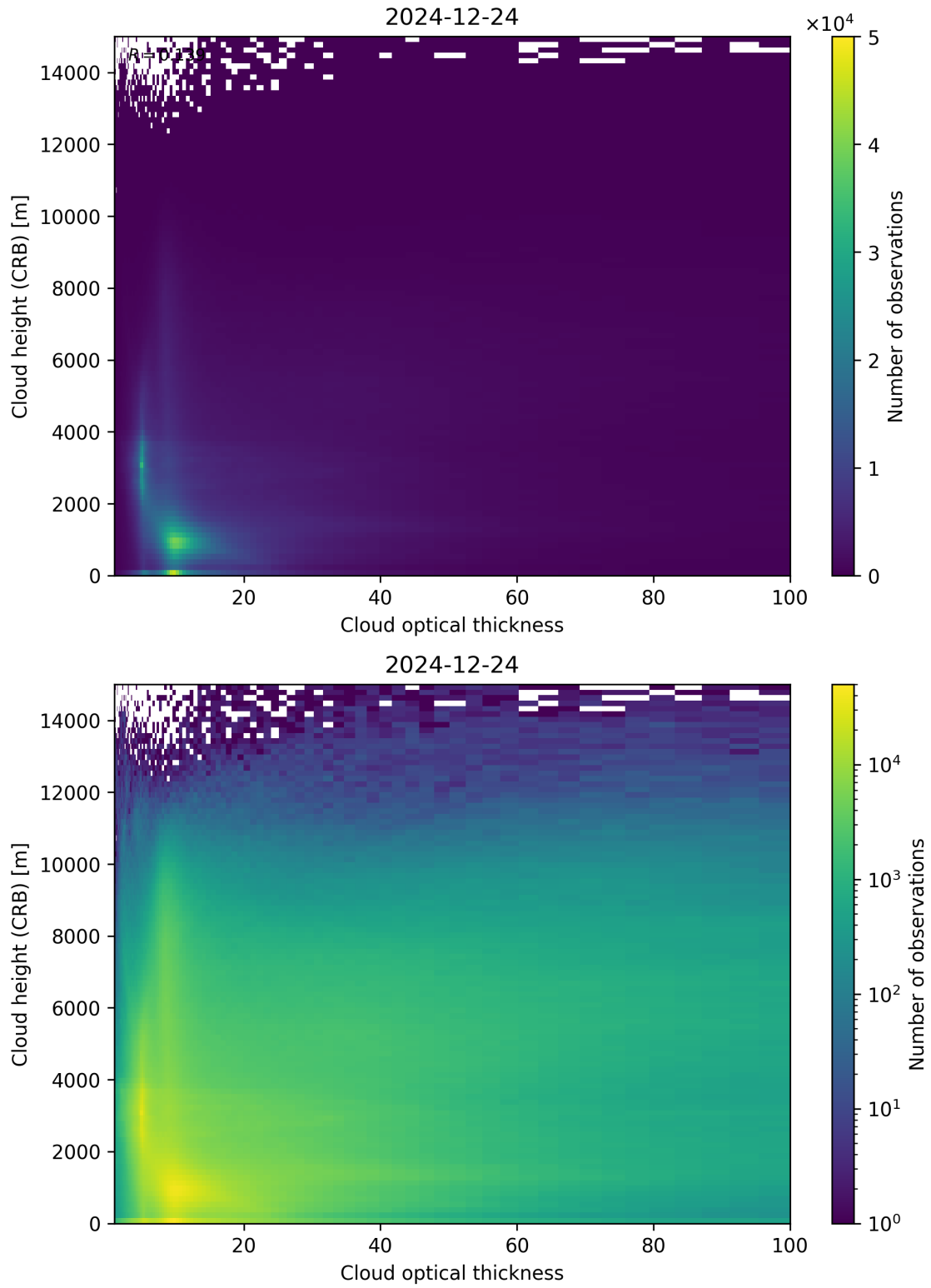
Figure 85: Scatter density plot of “Cloud optical thickness” against “Cloud height (CRB)” for 2024-12-23 to 2024-12-25.
