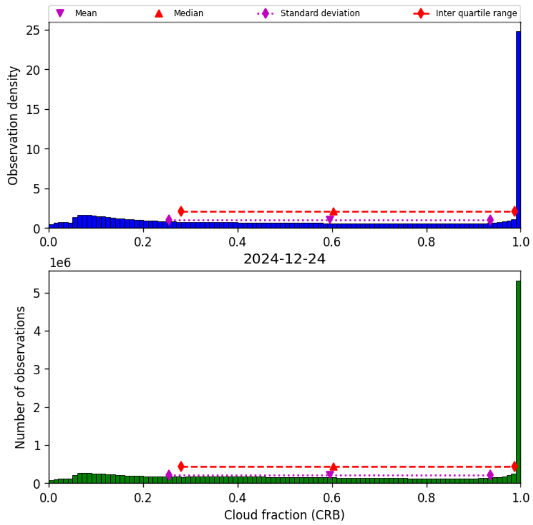
Figure 42: Histogram of “Cloud fraction (CRB)” for 2024-12-23 to 2024-12-25
