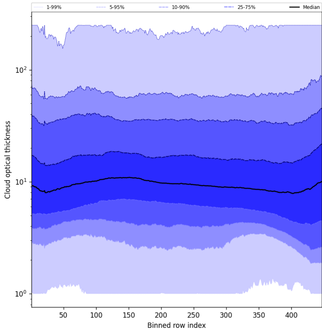
Figure 57: Along track statistics of “Cloud optical thickness” for 2024-12-23 to 2024-12-25
