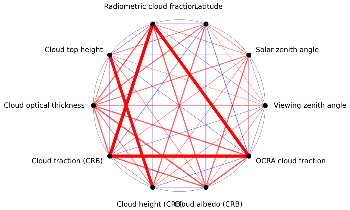
Figure 1: Map of correlation graph for 2024-12-23 to 2024-12-25.
