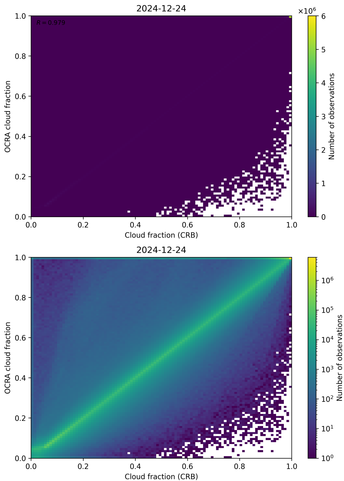
Figure 78: Scatter density plot of “Cloud fraction (CRB)” against “OCRA cloud fraction” for 2024-12-23 to 2024-12-25.
