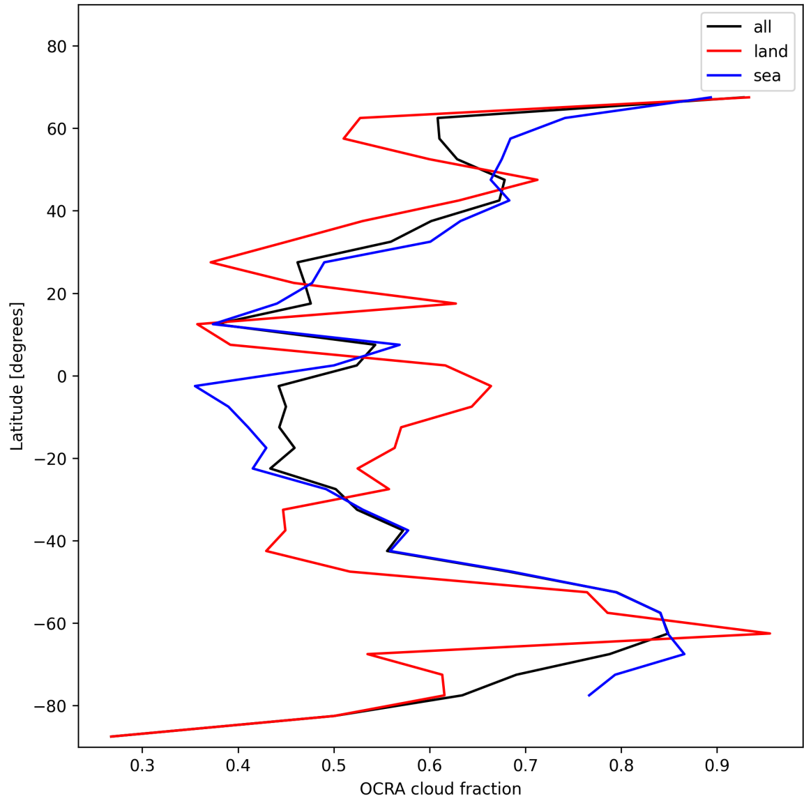
Figure 34: Zonal average of “OCRA cloud fraction” for 2024-12-23 to 2024-12-25.
