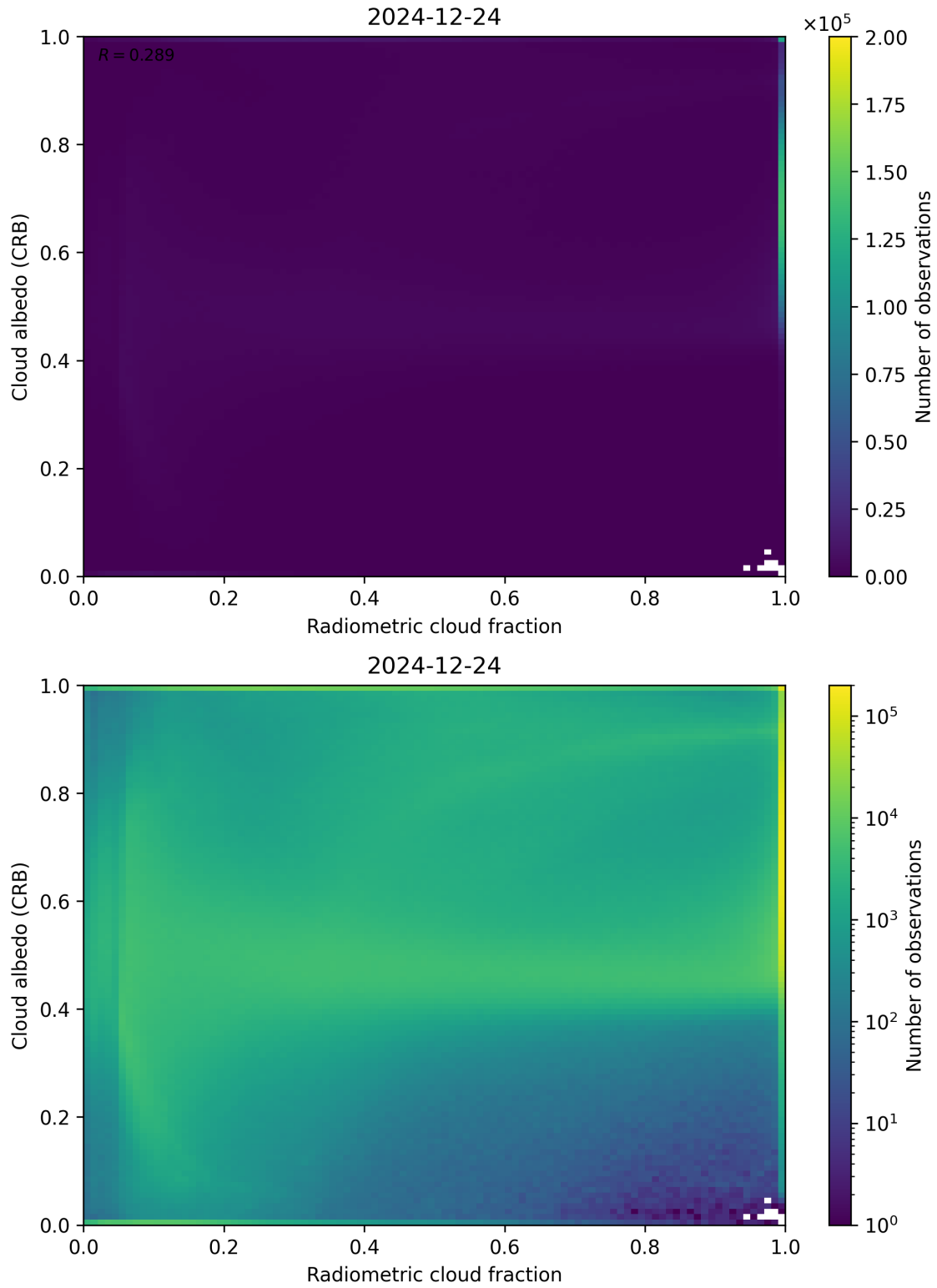
Figure 71: Scatter density plot of “Radiometric cloud fraction” against “Cloud albedo (CRB)” for 2024-12-23 to 2024-12-25.
