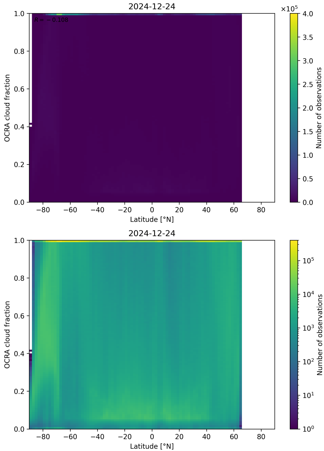
Figure 93: Scatter density plot of “Latitude” against “OCRA cloud fraction” for 2024-12-23 to 2024-12-25.
