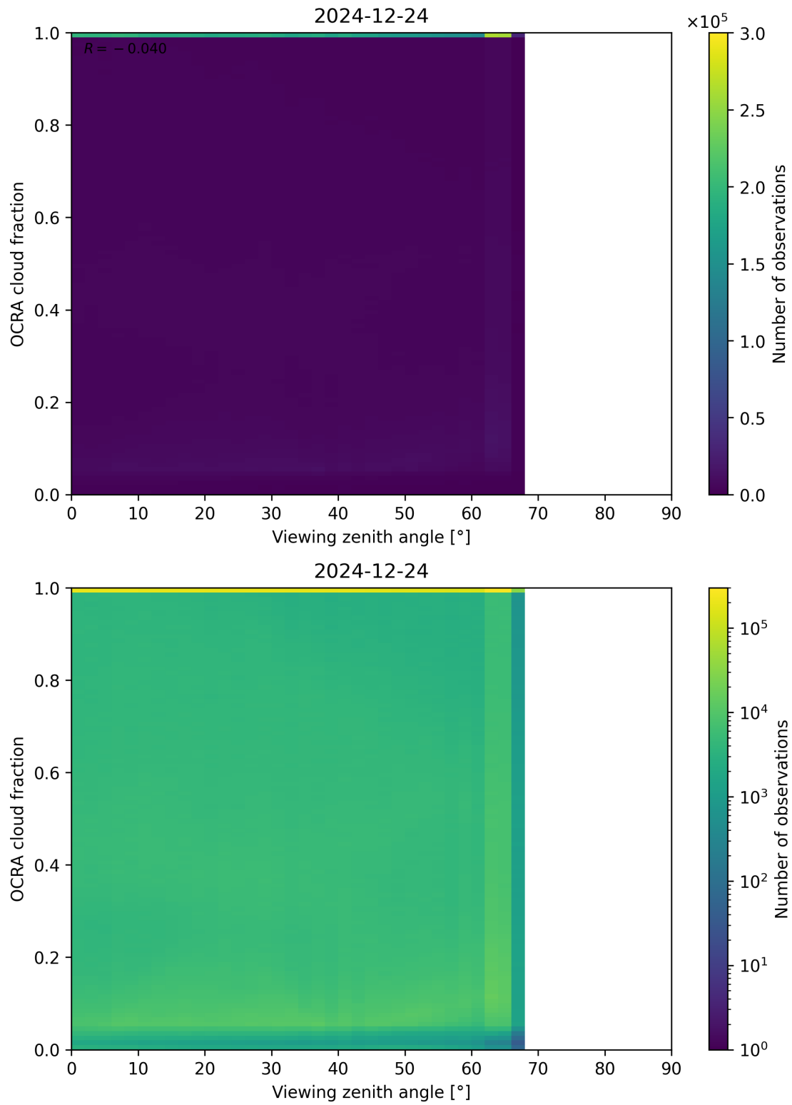
Figure 108: Scatter density plot of “Viewing zenith angle” against “OCRA cloud fraction” for 2024-12-23 to 2024-12-25.
