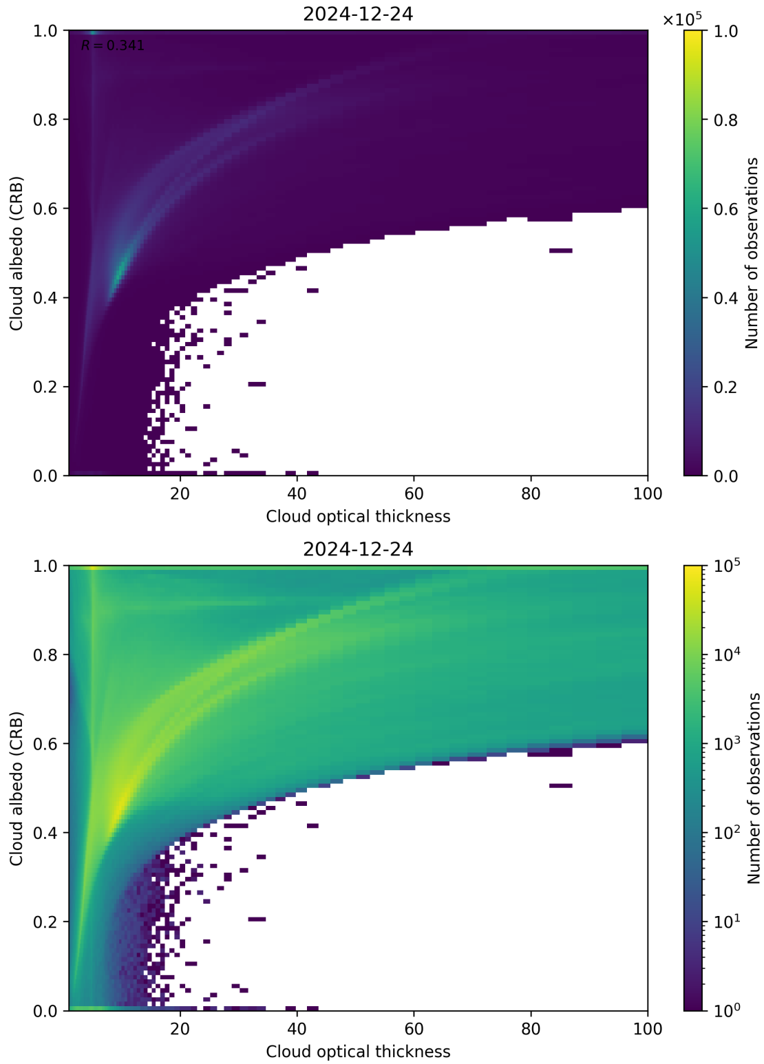
Figure 82: Scatter density plot of “Cloud optical thickness” against “Cloud albedo (CRB)” for 2024-12-23 to 2024-12-25.
