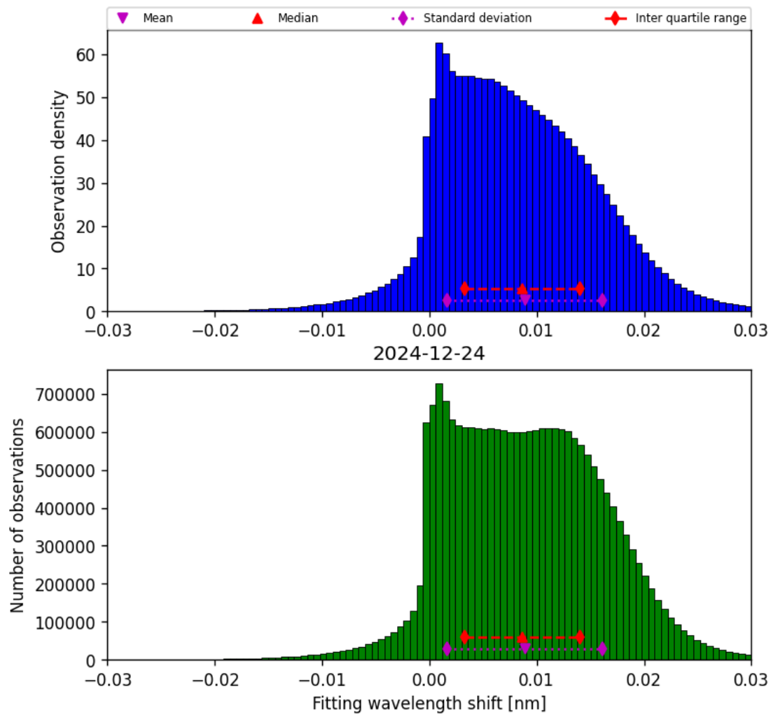
Figure 49: Histogram of “Fitting wavelength shift” for 2024-12-23 to 2024-12-25
