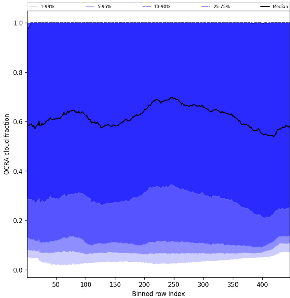
Figure 66: Along track statistics of “OCRA cloud fraction” for 2024-12-23 to 2024-12-25
