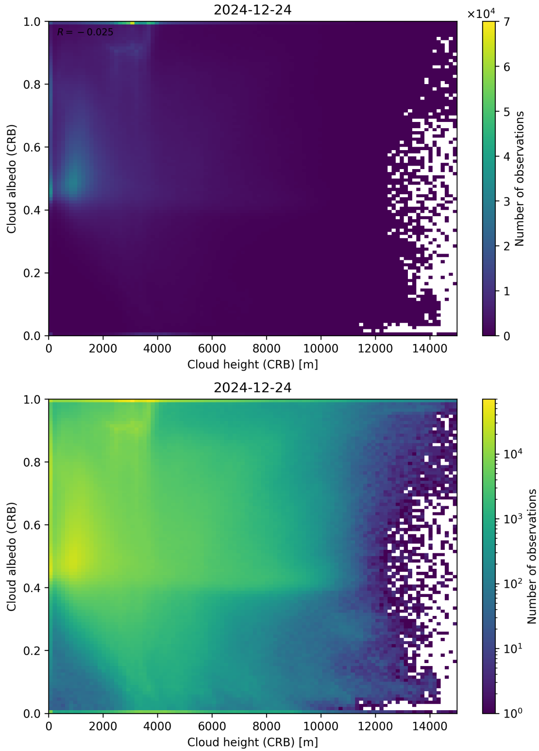
Figure 80: Scatter density plot of “Cloud height (CRB)” against “Cloud albedo (CRB)” for 2024-12-23 to 2024-12-25.
