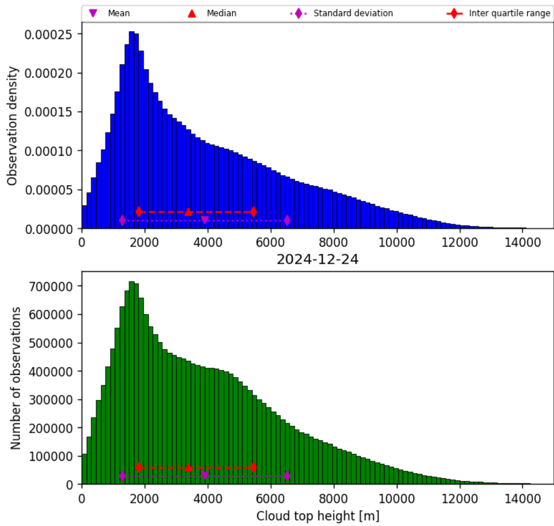
Figure 40: Histogram of “Cloud top height” for 2024-12-23 to 2024-12-25
