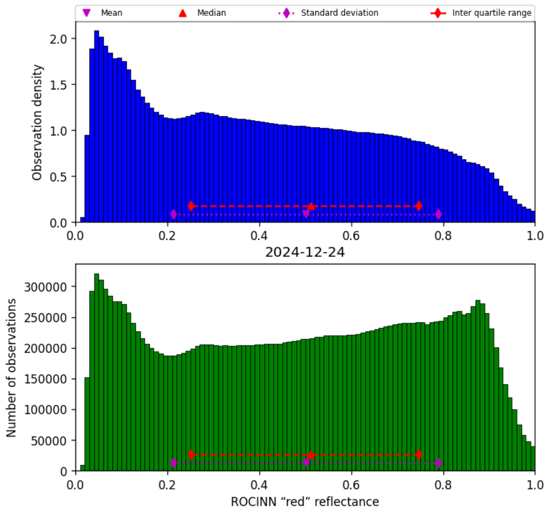
Figure 53: Histogram of “ROCINN “red” reflectance” for 2024-12-23 to 2024-12-25
