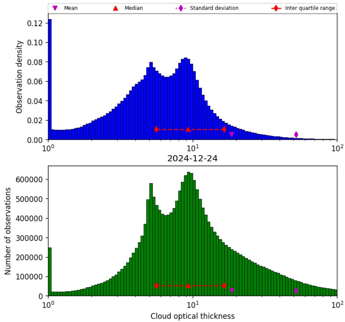
Figure 41: Histogram of “Cloud optical thickness” for 2024-12-23 to 2024-12-25
