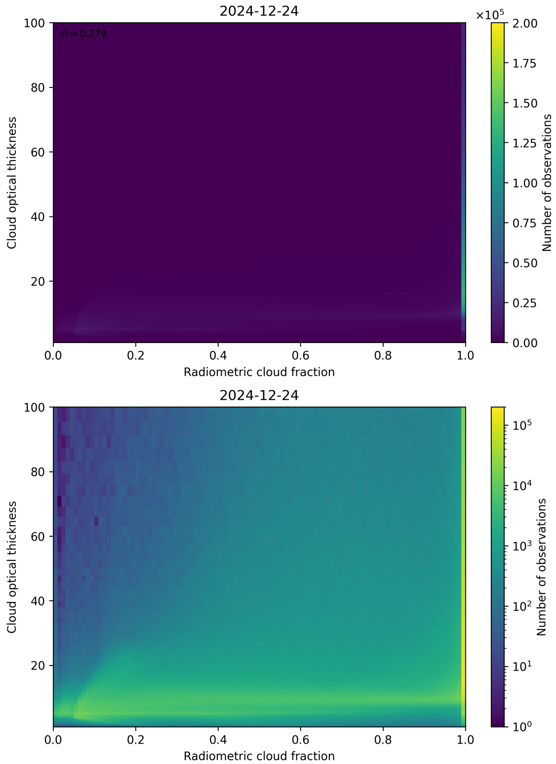
Figure 75: Scatter density plot of “Radiometric cloud fraction” against “Cloud optical thickness” for 2024-12-23 to 2024-12-25.
