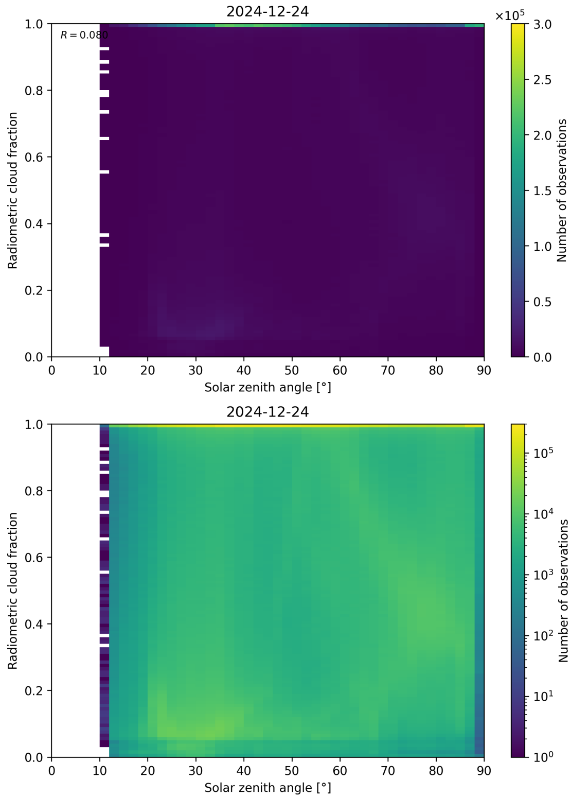
Figure 99: Scatter density plot of “Solar zenith angle” against “Radiometric cloud fraction” for 2024-12-23 to 2024-12-25.
