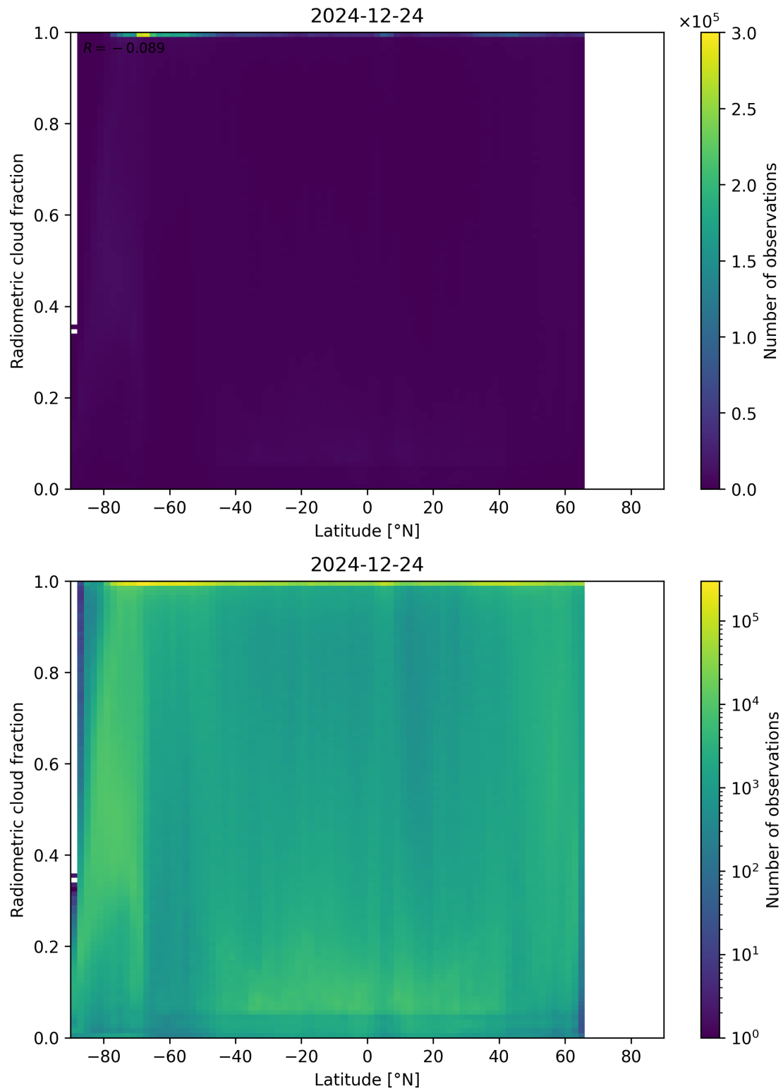
Figure 92: Scatter density plot of “Latitude” against “Radiometric cloud fraction” for 2024-12-23 to 2024-12-25.
