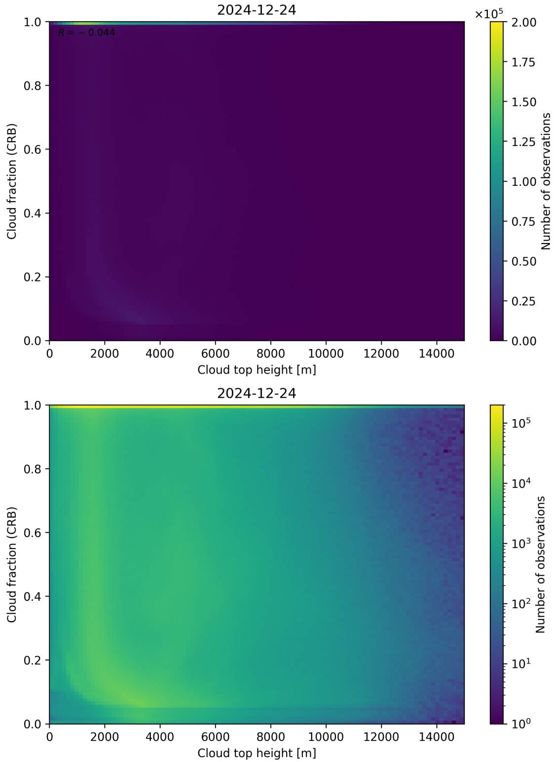
Figure 88: Scatter density plot of “Cloud top height” against “Cloud fraction (CRB)” for 2024-12-23 to 2024-12-25.
