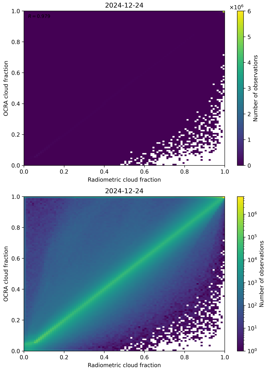
Figure 72: Scatter density plot of “Radiometric cloud fraction” against “OCRA cloud fraction” for 2024-12-23 to 2024-12-25.
