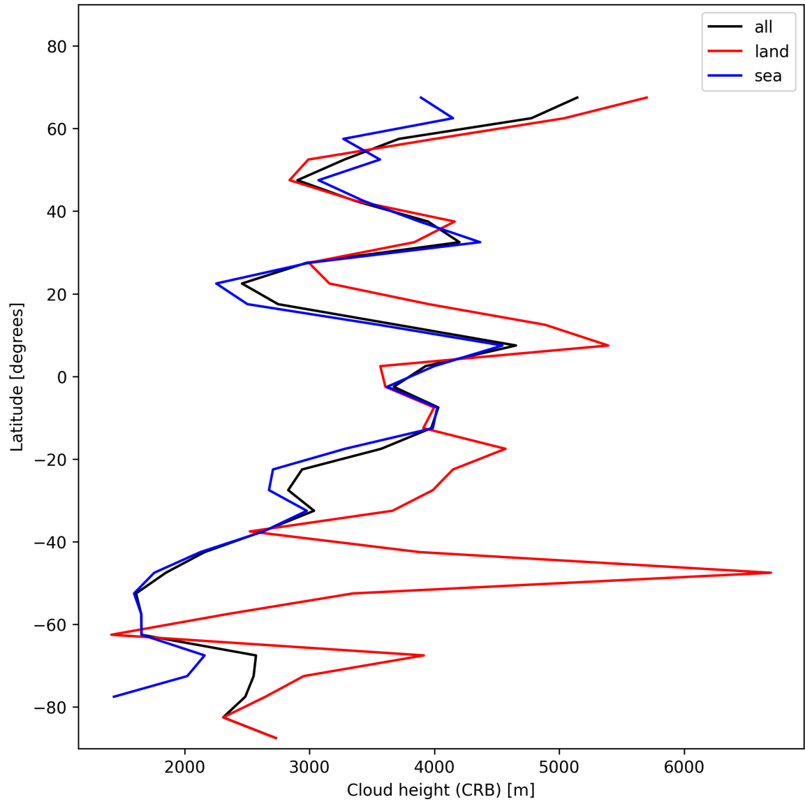
Figure 27: Zonal average of “Cloud height (CRB)” for 2024-12-23 to 2024-12-25.
