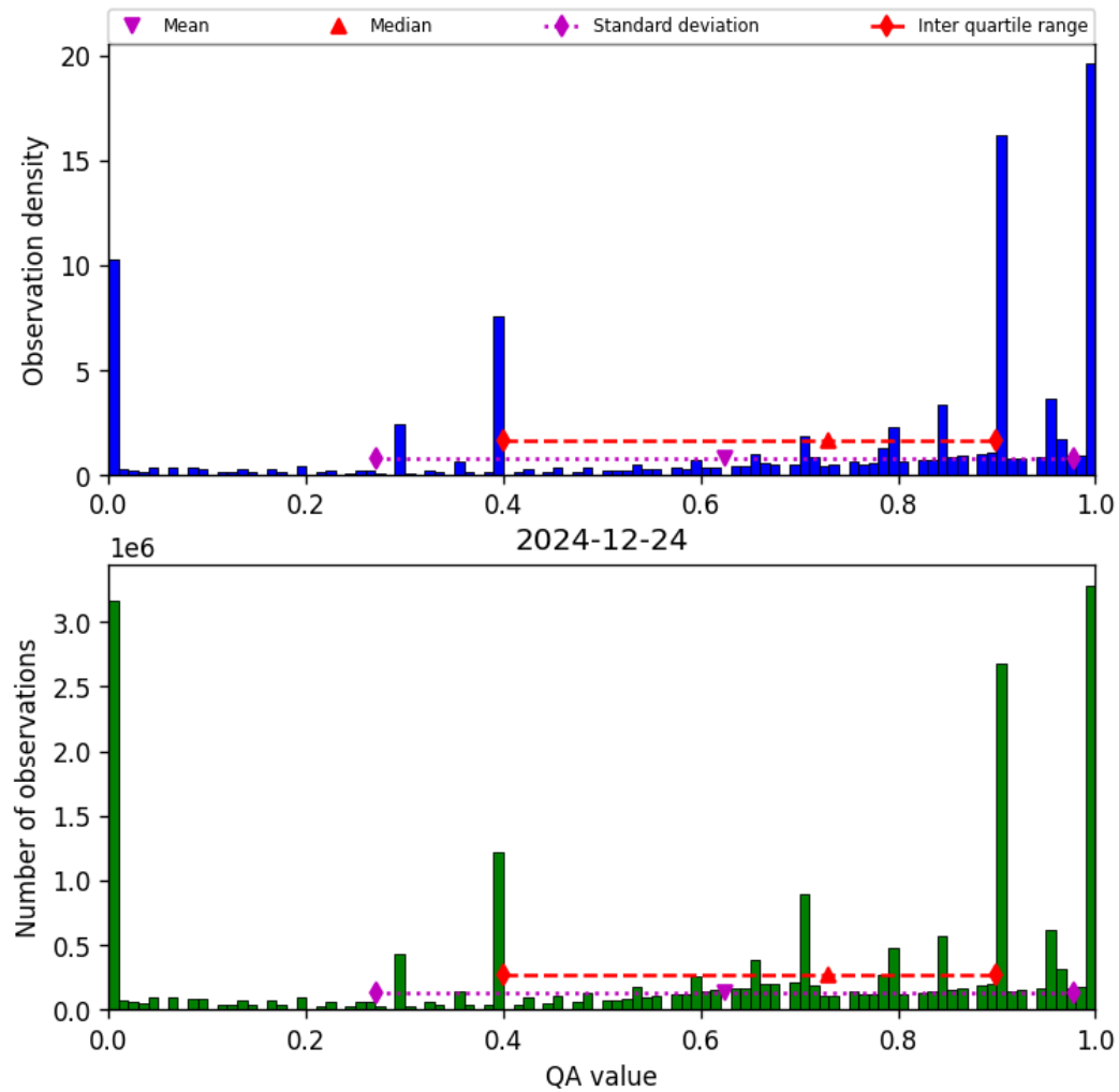
Figure 38: Histogram of “QA value” for 2024-12-23 to 2024-12-25
