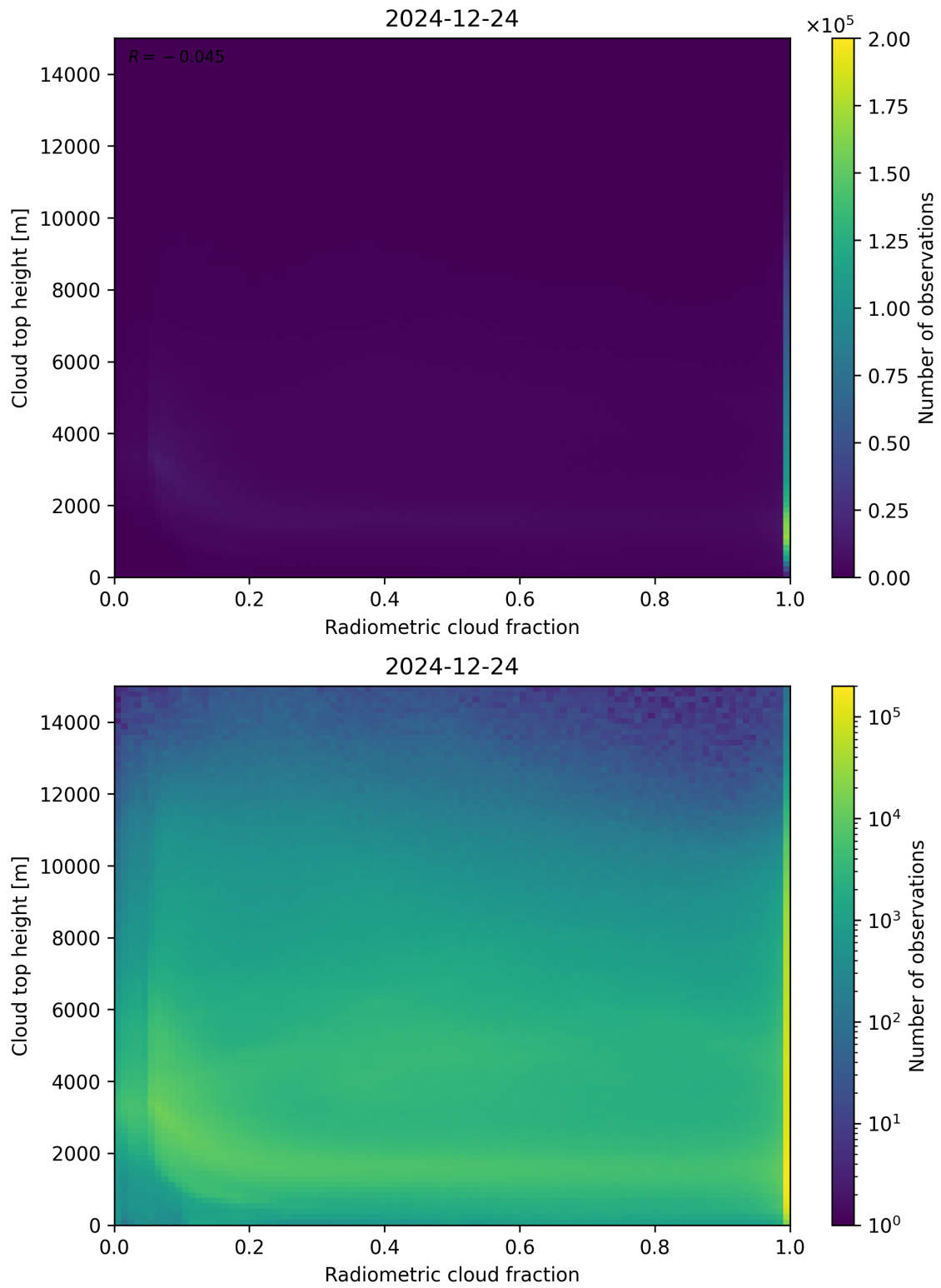
Figure 76: Scatter density plot of “Radiometric cloud fraction” against “Cloud top height” for 2024-12-23 to 2024-12-25.
