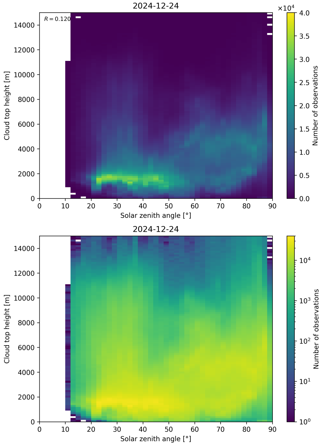
Figure 104: Scatter density plot of “Solar zenith angle” against “Cloud top height” for 2024-12-23 to 2024-12-25.
