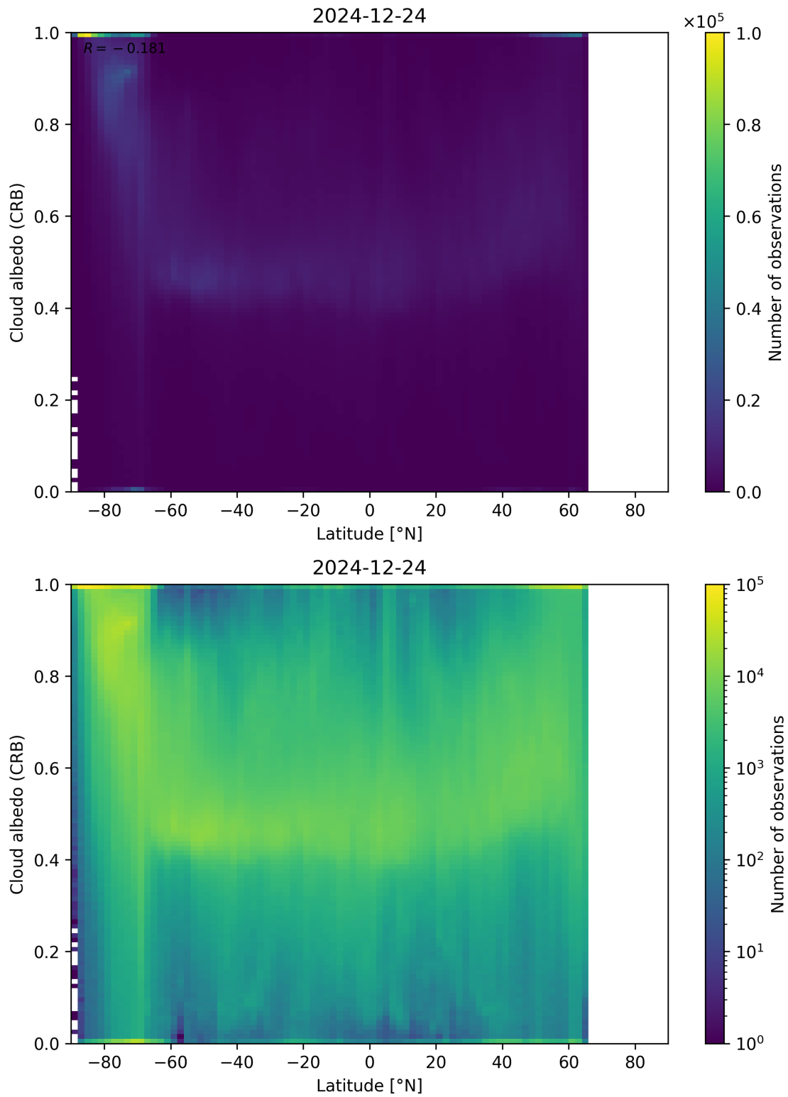
Figure 91: Scatter density plot of “Latitude” against “Cloud albedo (CRB)” for 2024-12-23 to 2024-12-25.
