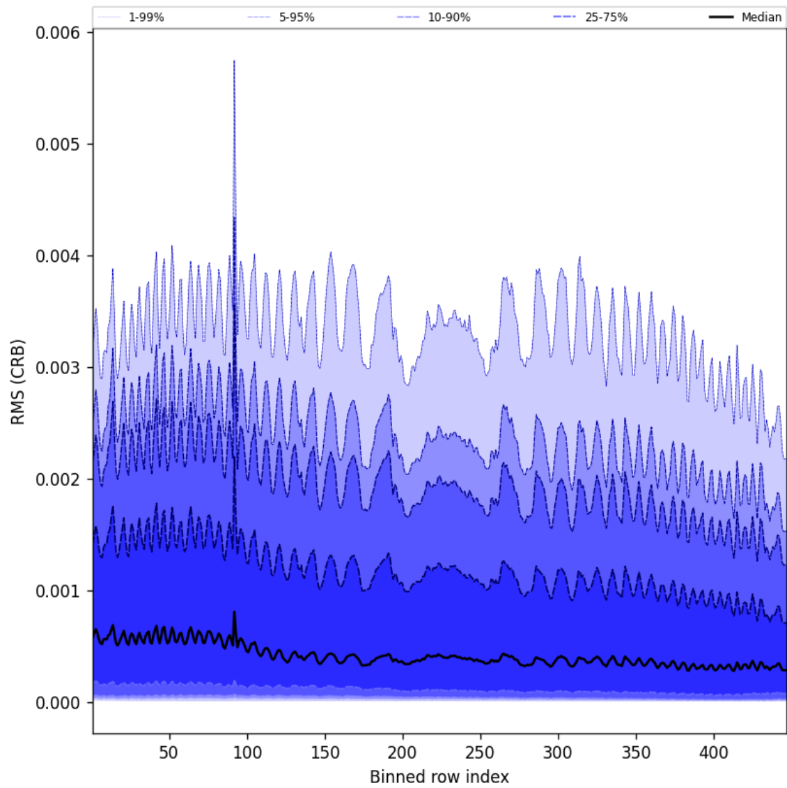
Figure 64: Along track statistics of “RMS (CRB)” for 2024-12-23 to 2024-12-25
