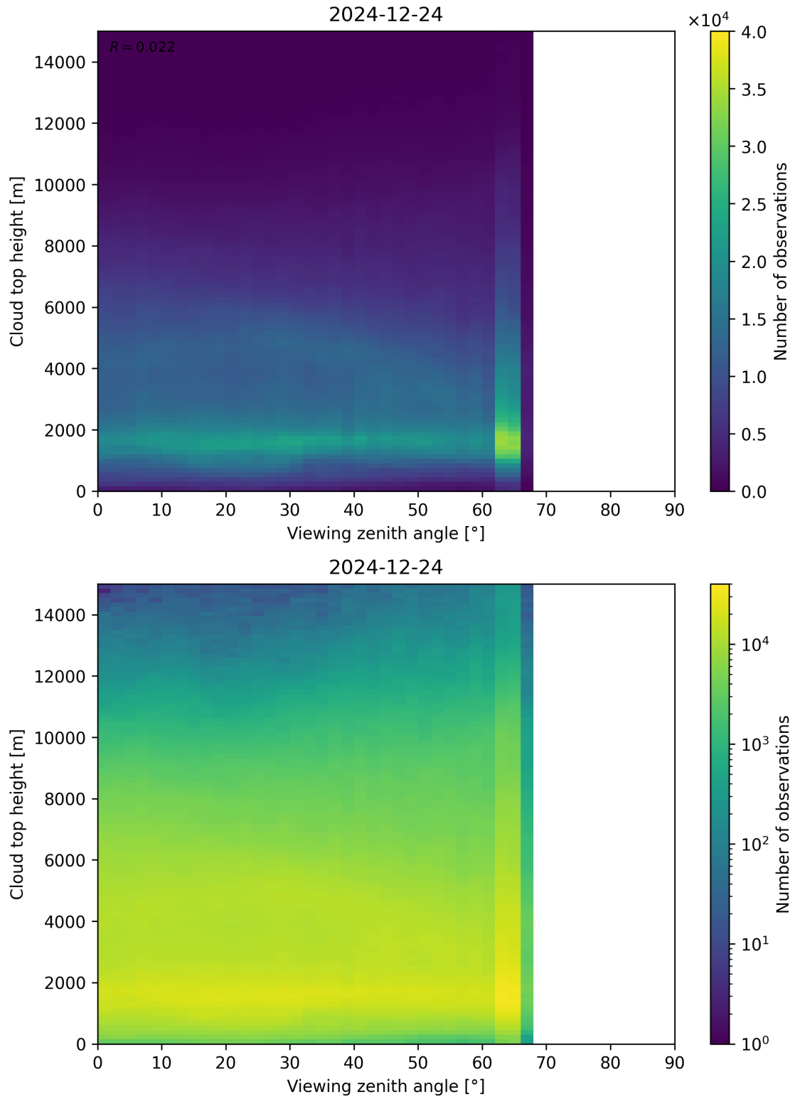
Figure 112: Scatter density plot of “Viewing zenith angle” against “Cloud top height” for 2024-12-23 to 2024-12-25.
