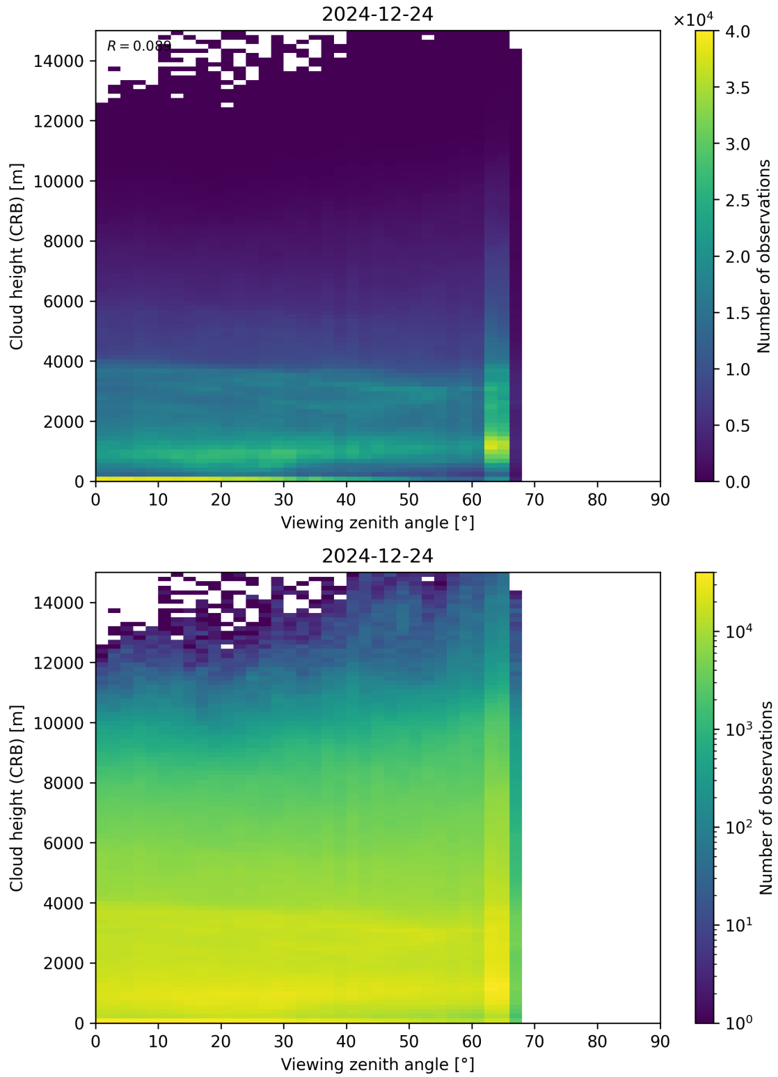
Figure 110: Scatter density plot of “Viewing zenith angle” against “Cloud height (CRB)” for 2024-12-23 to 2024-12-25.
