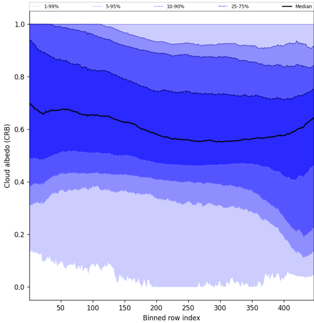
Figure 60: Along track statistics of “Cloud albedo (CRB)” for 2024-12-23 to 2024-12-25
