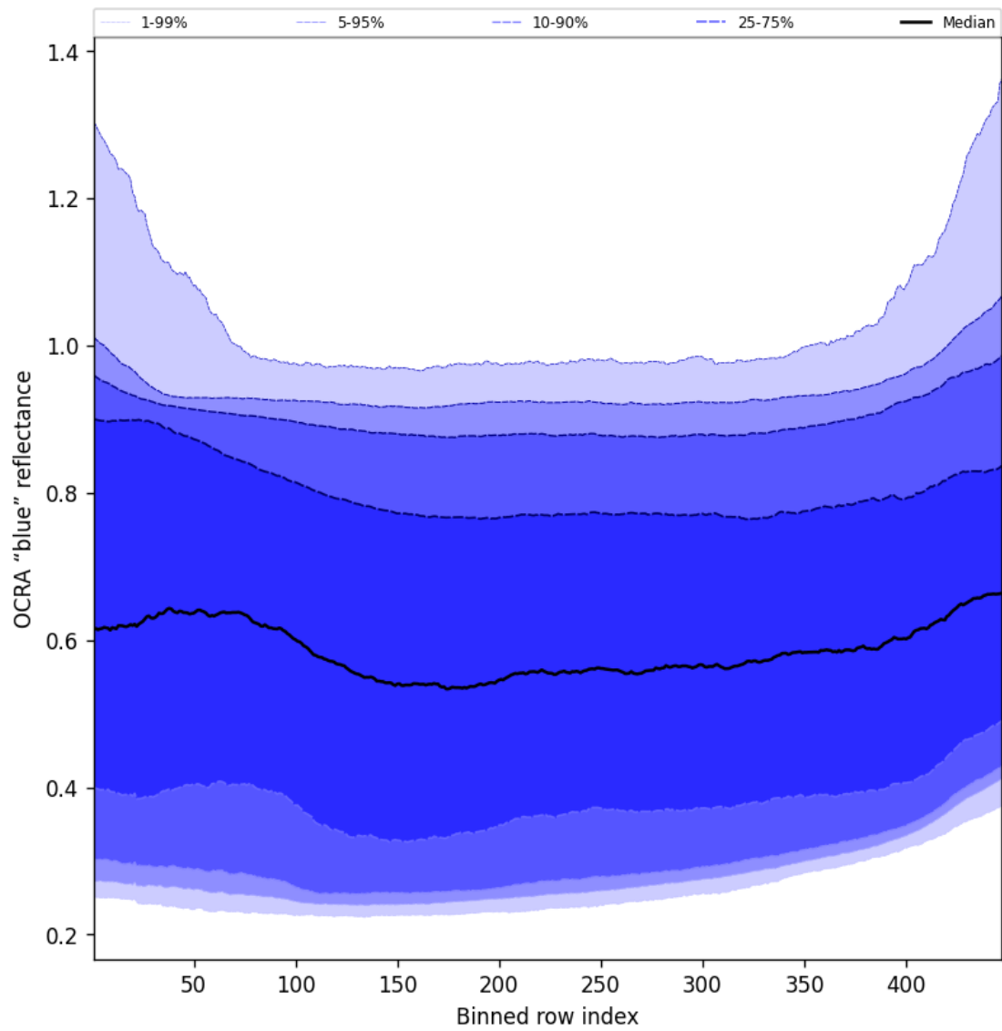
Figure 67: Along track statistics of “OCRA “blue” reflectance” for 2024-12-23 to 2024-12-25
