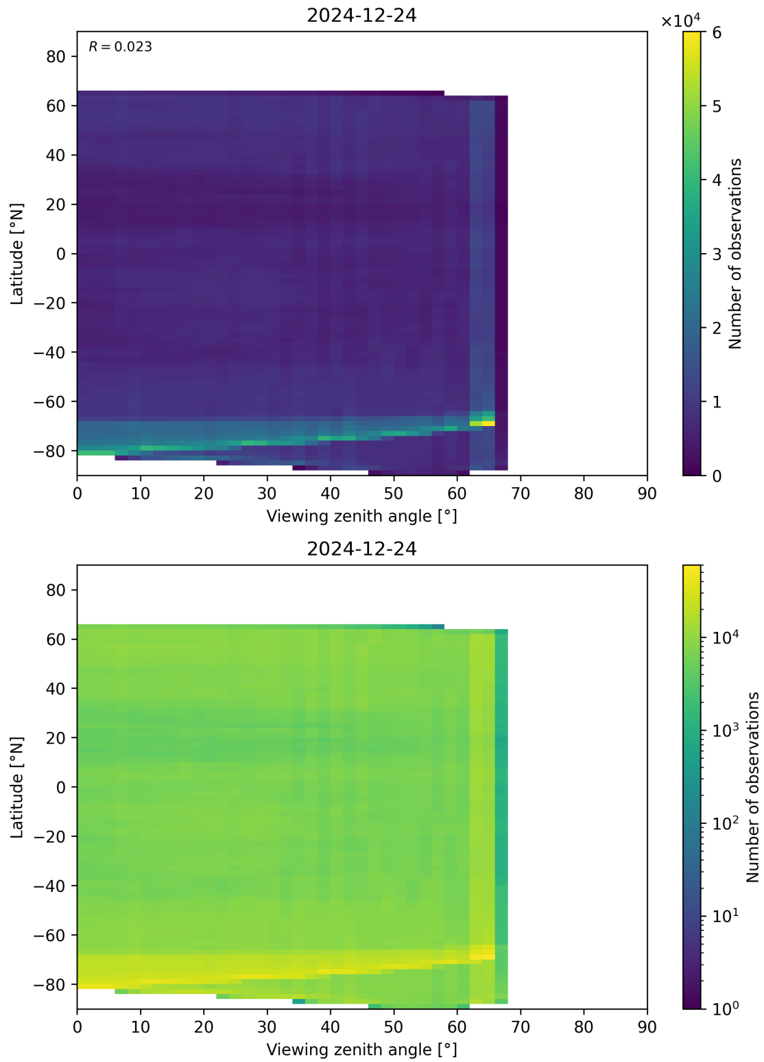
Figure 113: Scatter density plot of “Viewing zenith angle” against “Latitude” for 2024-12-23 to 2024-12-25.
