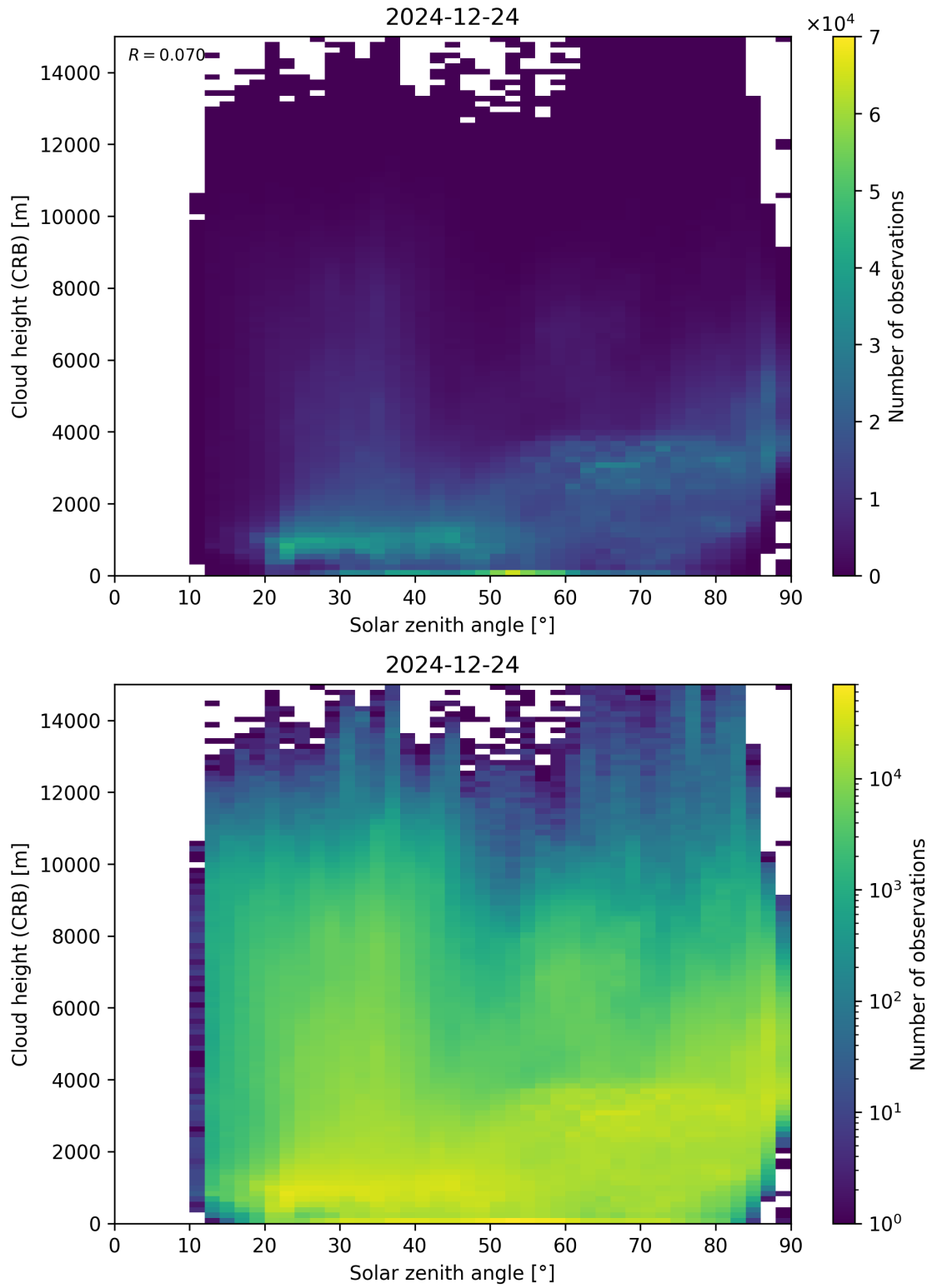
Figure 102: Scatter density plot of “Solar zenith angle” against “Cloud height (CRB)” for 2024-12-23 to 2024-12-25.
