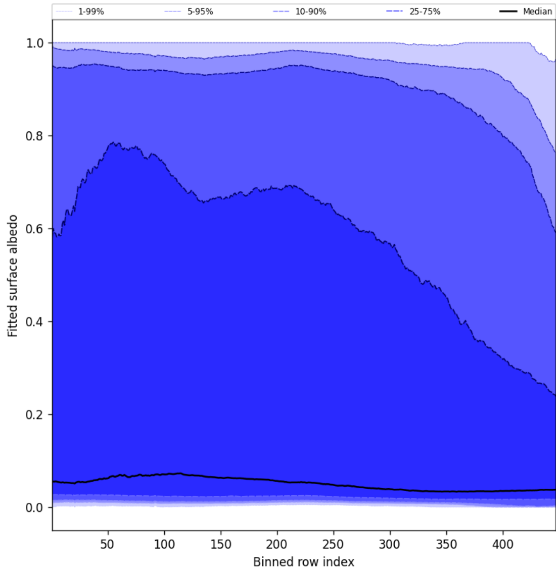
Figure 61: Along track statistics of “Fitted surface albedo” for 2024-12-23 to 2024-12-25
