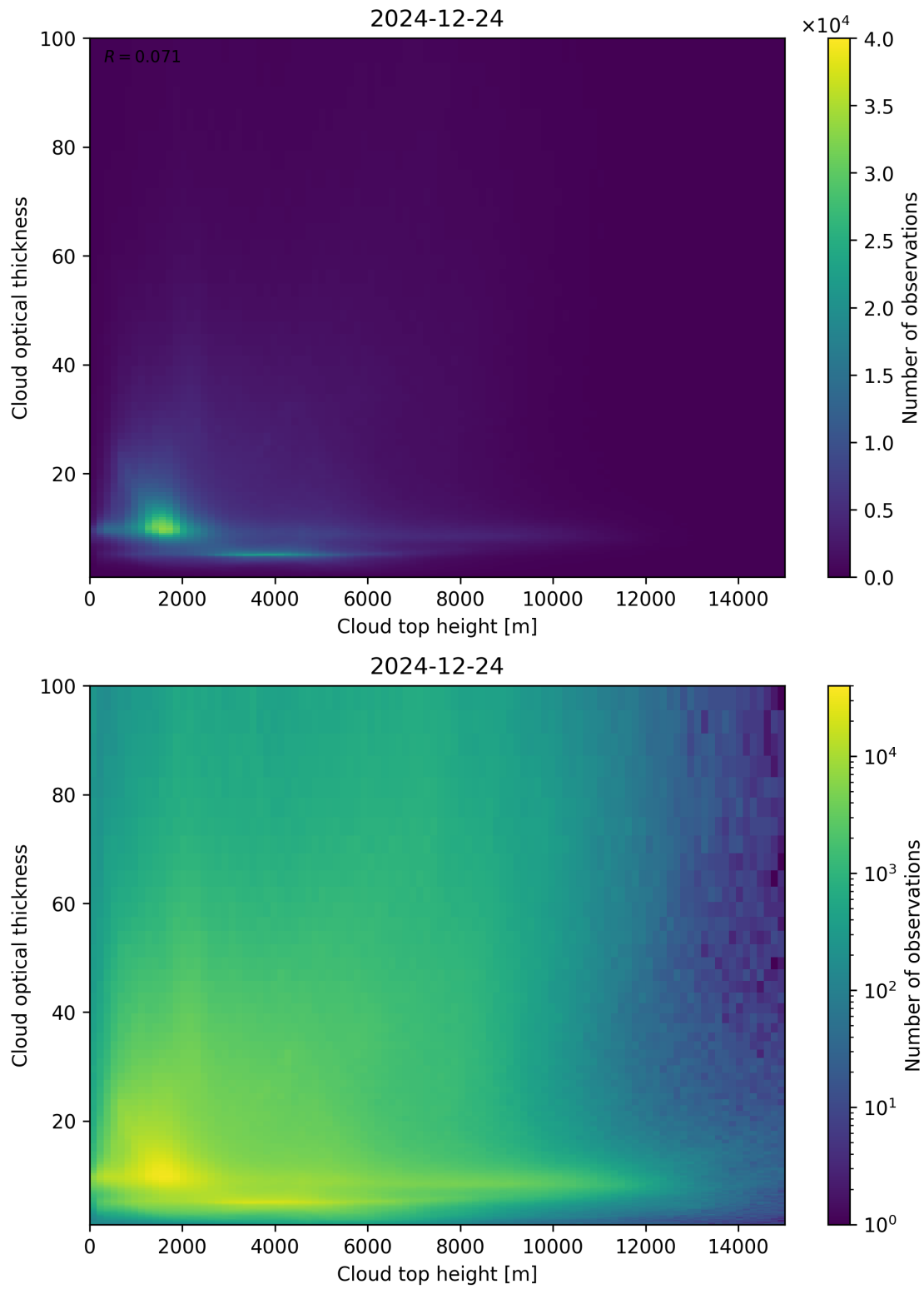
Figure 90: Scatter density plot of “Cloud top height” against “Cloud optical thickness” for 2024-12-23 to 2024-12-25.
