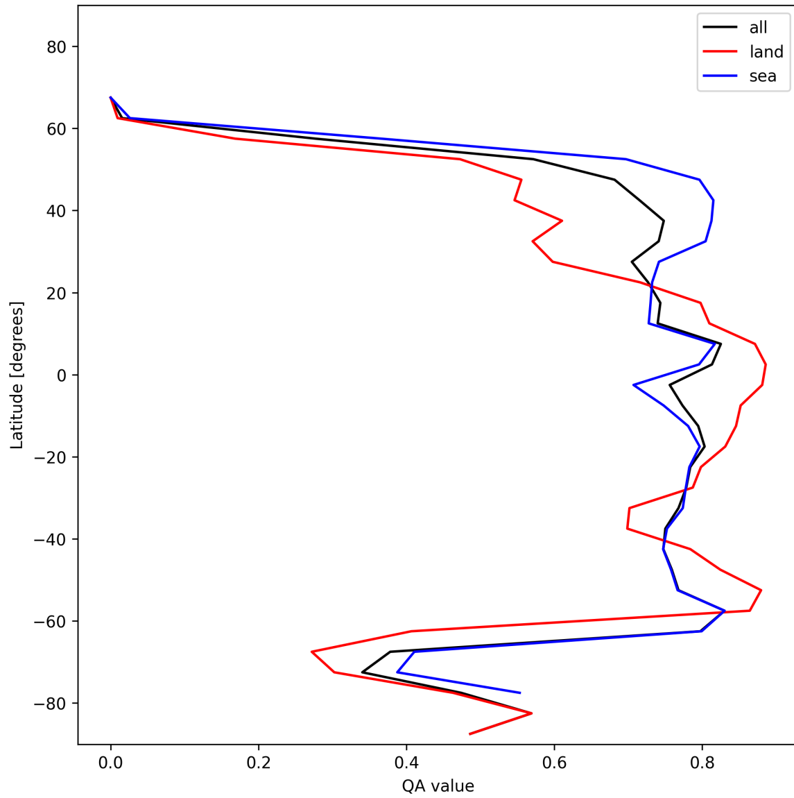
Figure 22: Zonal average of “QA value” for 2024-12-23 to 2024-12-25.
