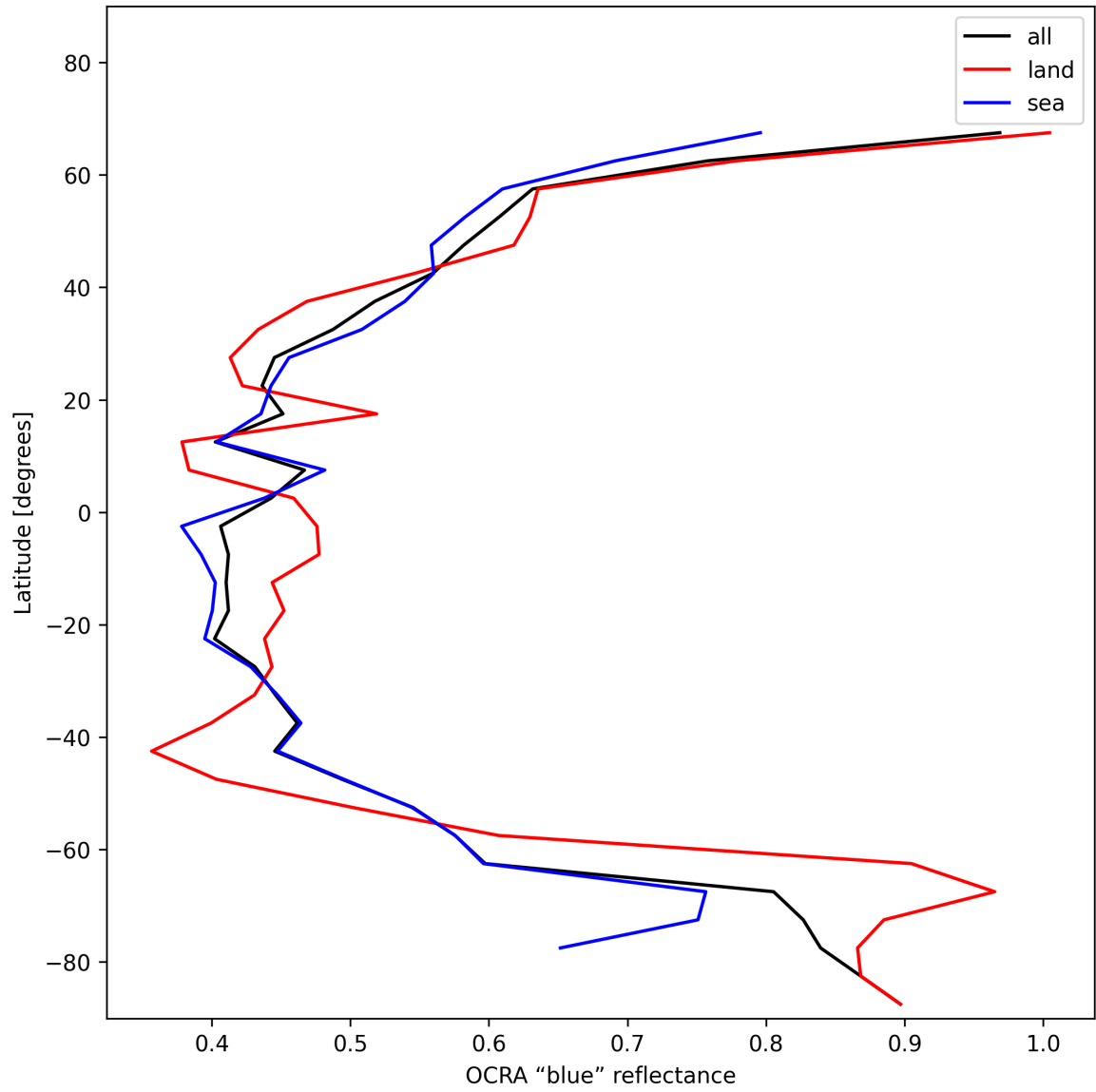
Figure 35: Zonal average of "OCRA "blue" reflectance" for 2024-12-23 to 2024-12-25.
