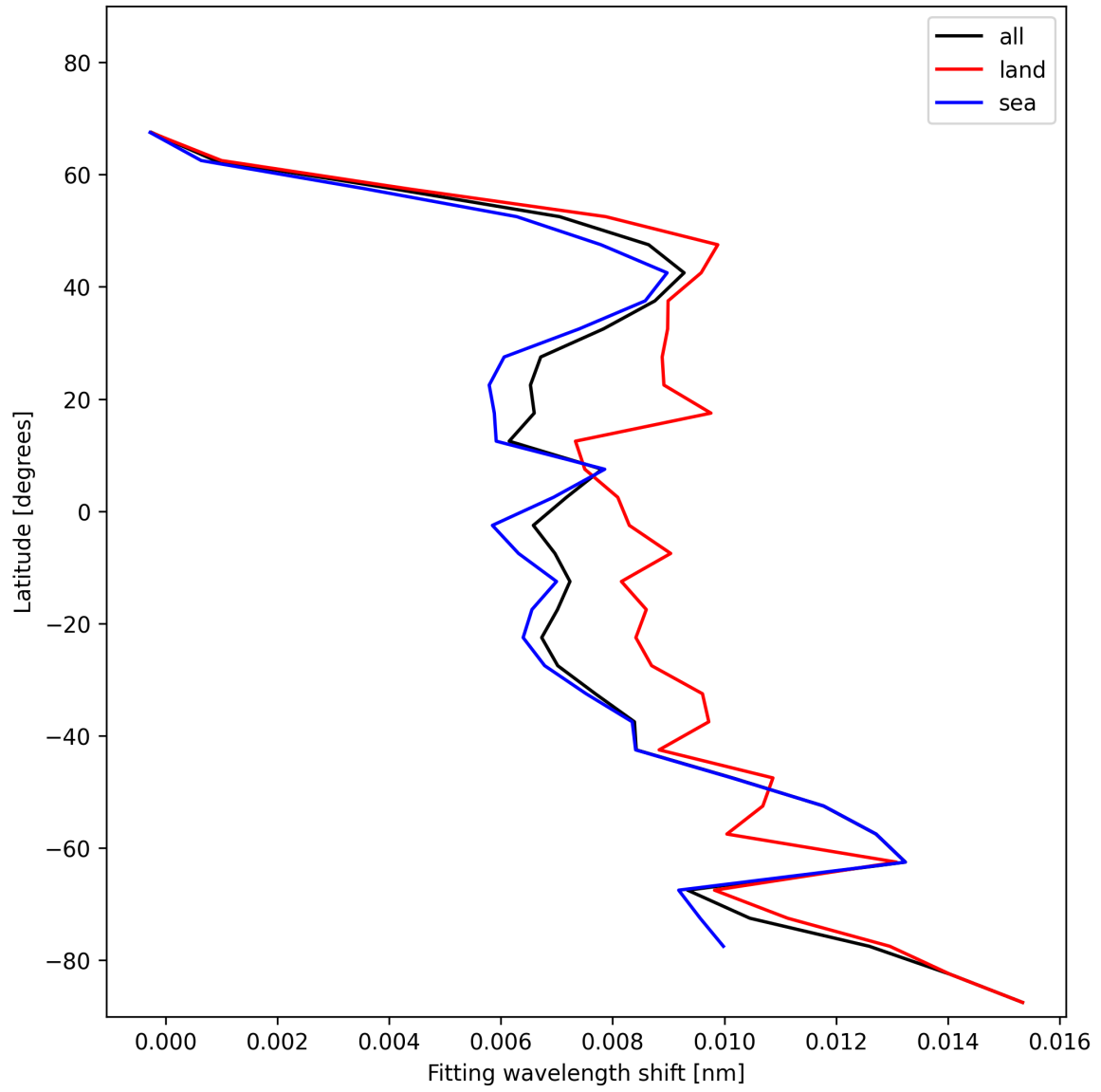
Figure 33: Zonal average of “Fitting wavelength shift” for 2024-12-23 to 2024-12-25.
