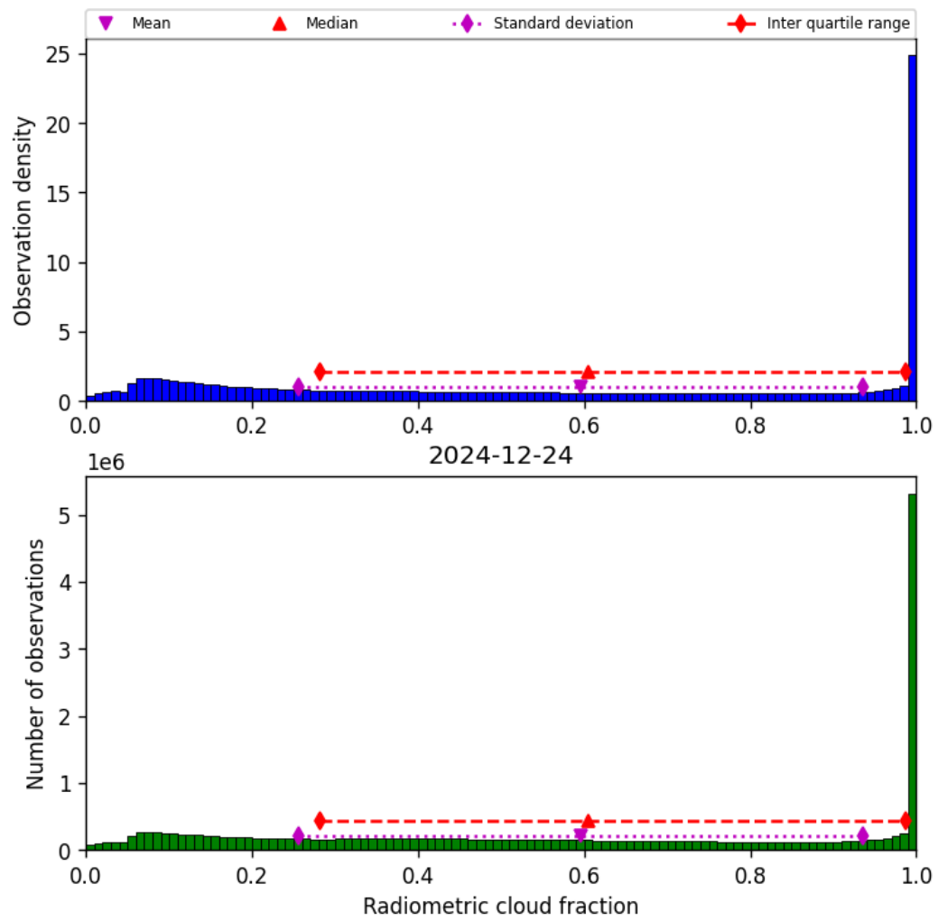
Figure 39: Histogram of “Radiometric cloud fraction” for 2024-12-23 to 2024-12-25
