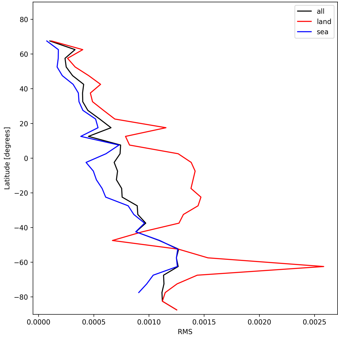
Figure 31: Zonal average of “RMS” for 2024-12-23 to 2024-12-25.
