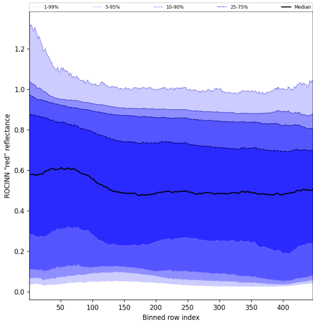
Figure 69: Along track statistics of “ROCINN “red” reflectance” for 2024-12-23 to 2024-12-25
