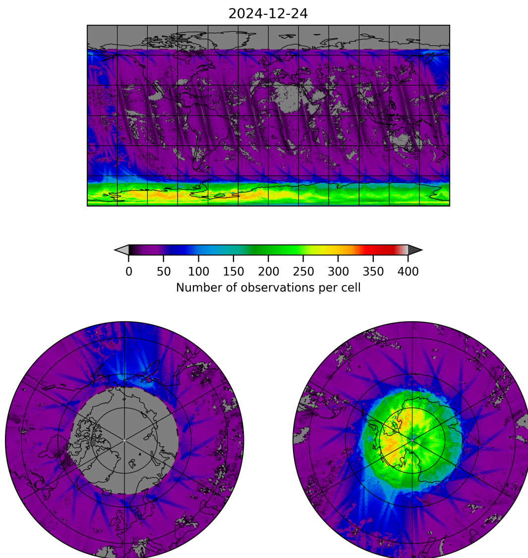
Figure 21: Map of the number of observations for 2024-12-23 to 2024-12-25
