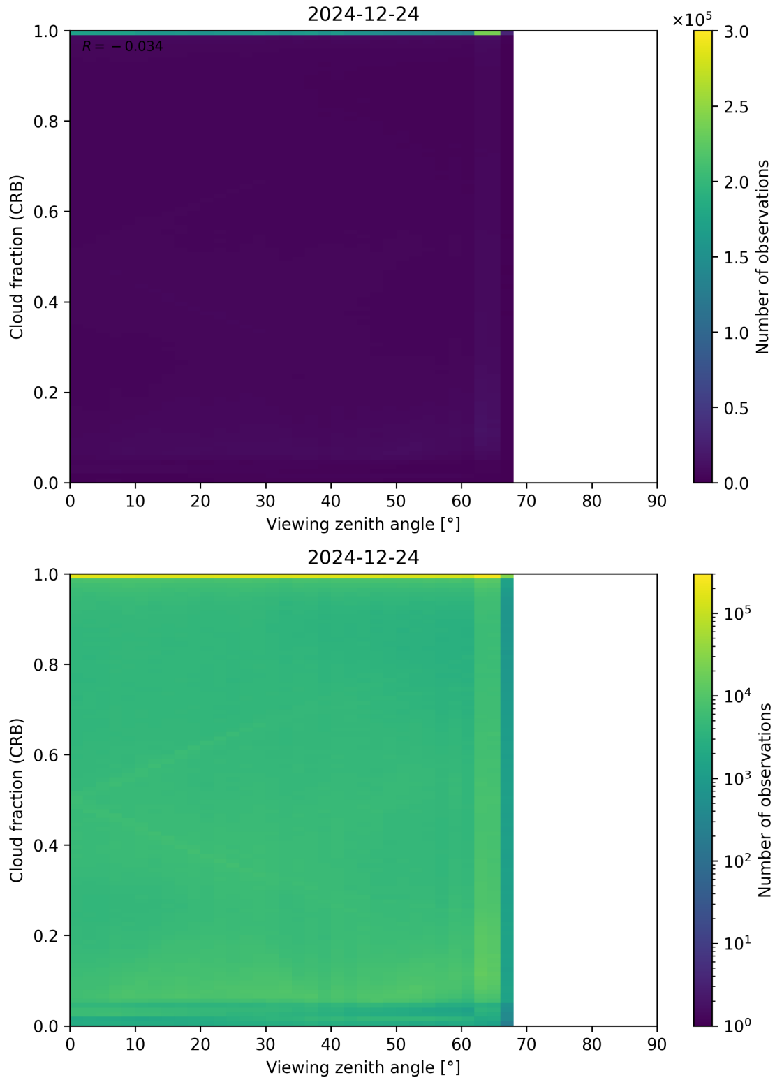
Figure 109: Scatter density plot of “Viewing zenith angle” against “Cloud fraction (CRB)” for 2024-12-23 to 2024-12-25.
