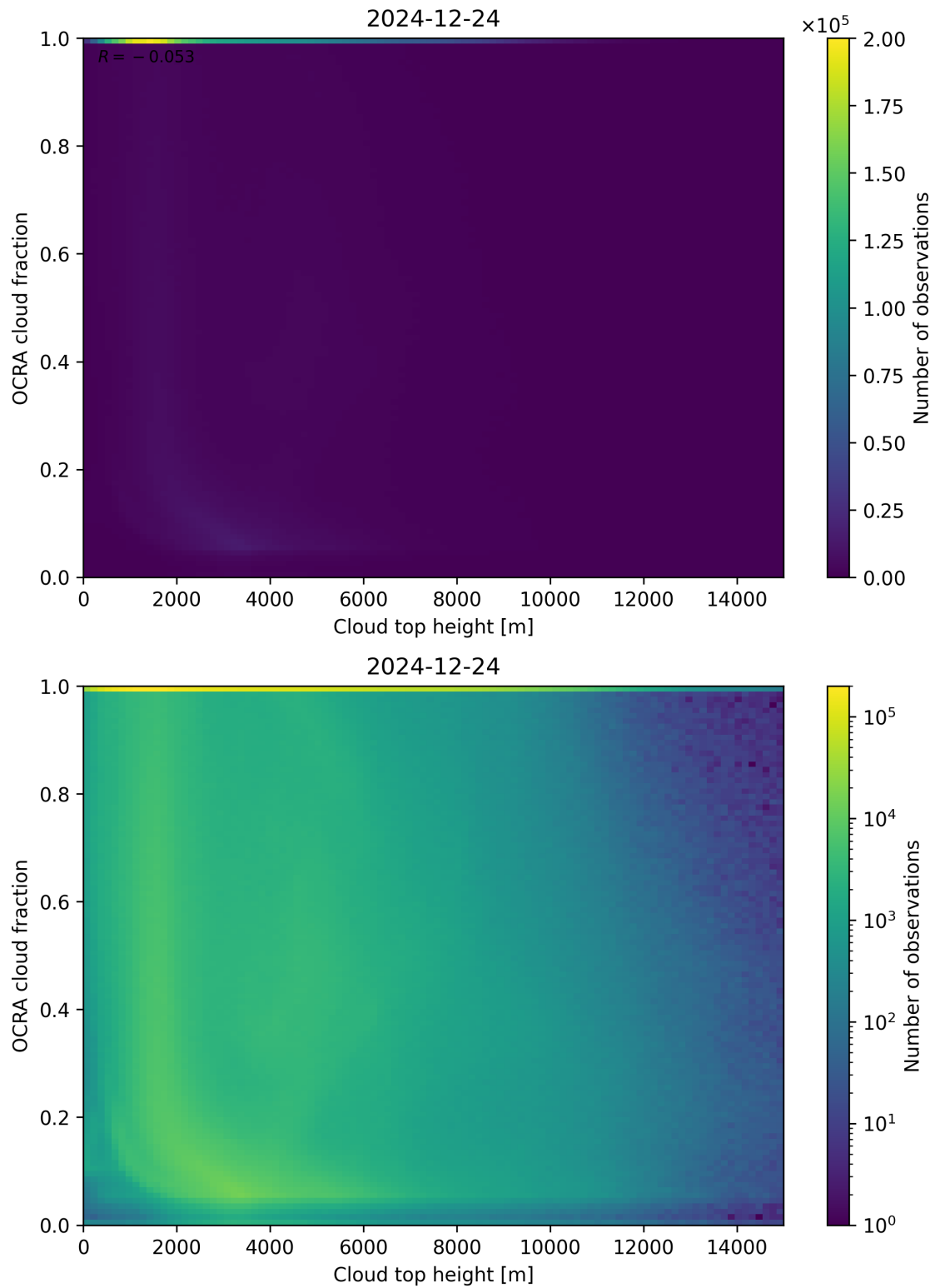
Figure 87: Scatter density plot of “Cloud top height” against “OCRA cloud fraction” for 2024-12-23 to 2024-12-25.
