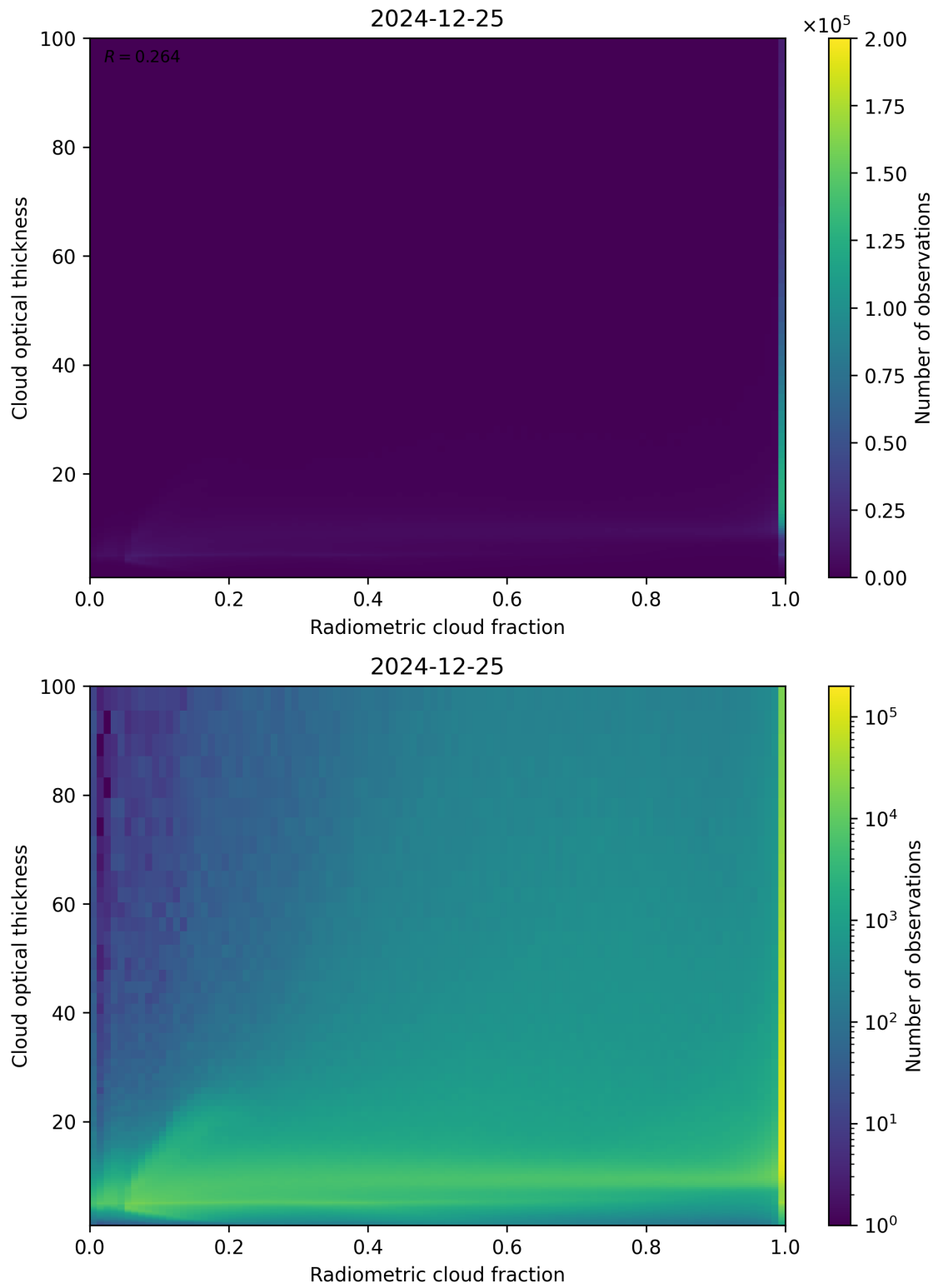
Figure 75: Scatter density plot of “Radiometric cloud fraction” against “Cloud optical thickness” for 2024-12-24 to 2024-12-26.
