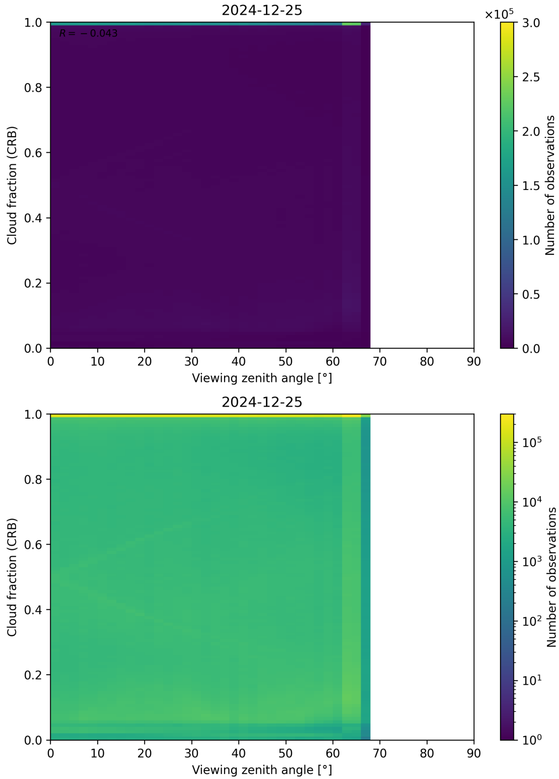
Figure 109: Scatter density plot of “Viewing zenith angle” against “Cloud fraction (CRB)” for 2024-12-24 to 2024-12-26.
