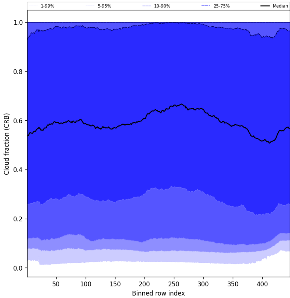
Figure 58: Along track statistics of “Cloud fraction (CRB)” for 2024-12-24 to 2024-12-26
