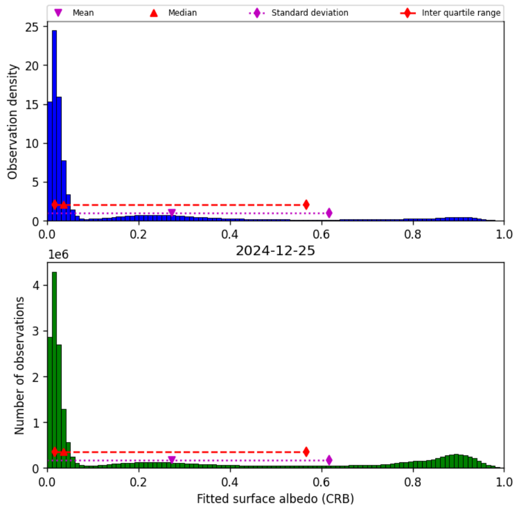
Figure 46: Histogram of “Fitted surface albedo (CRB)” for 2024-12-24 to 2024-12-26
