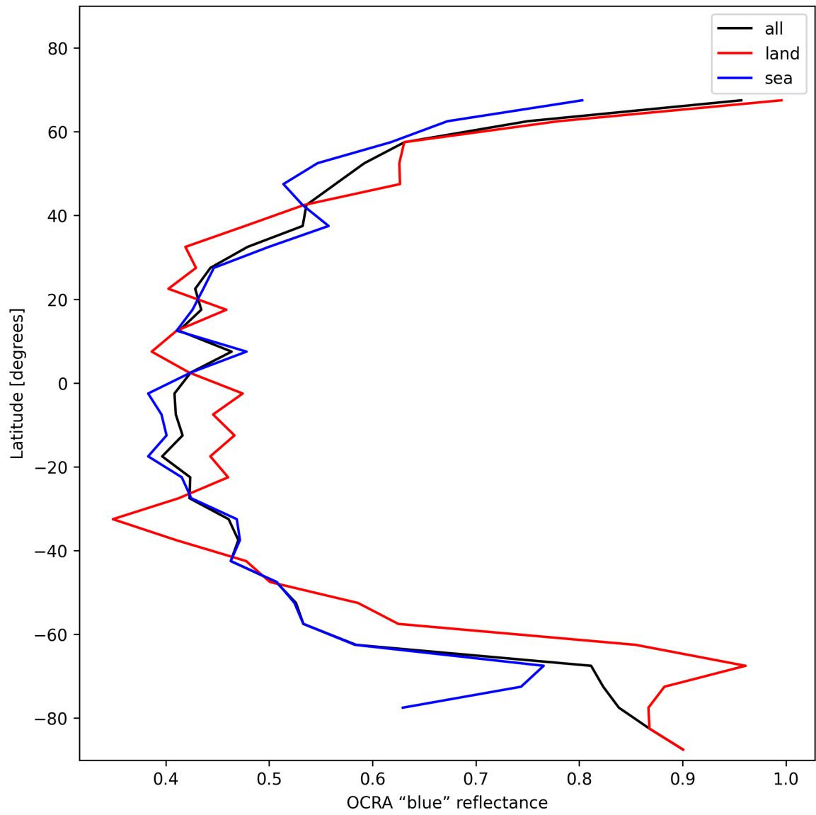
Figure 35: Zonal average of “OCRA “blue” reflectance” for 2024-12-24 to 2024-12-26.
