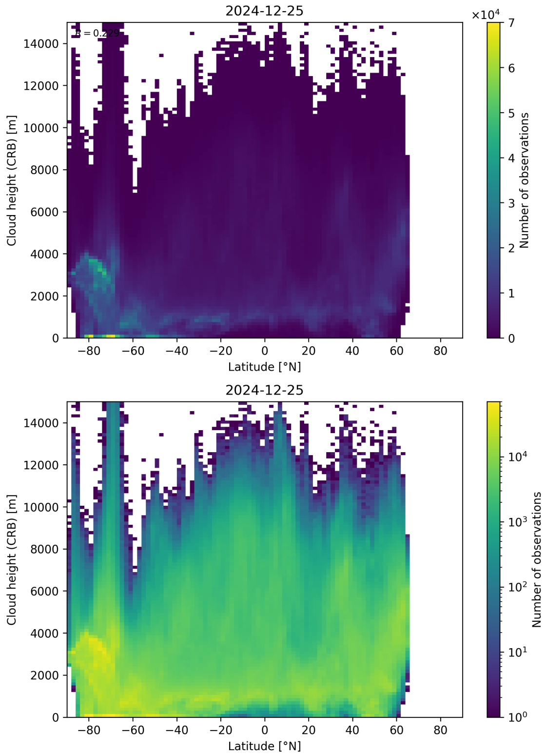
Figure 95: Scatter density plot of “Latitude” against “Cloud height (CRB)” for 2024-12-24 to 2024-12-26.
