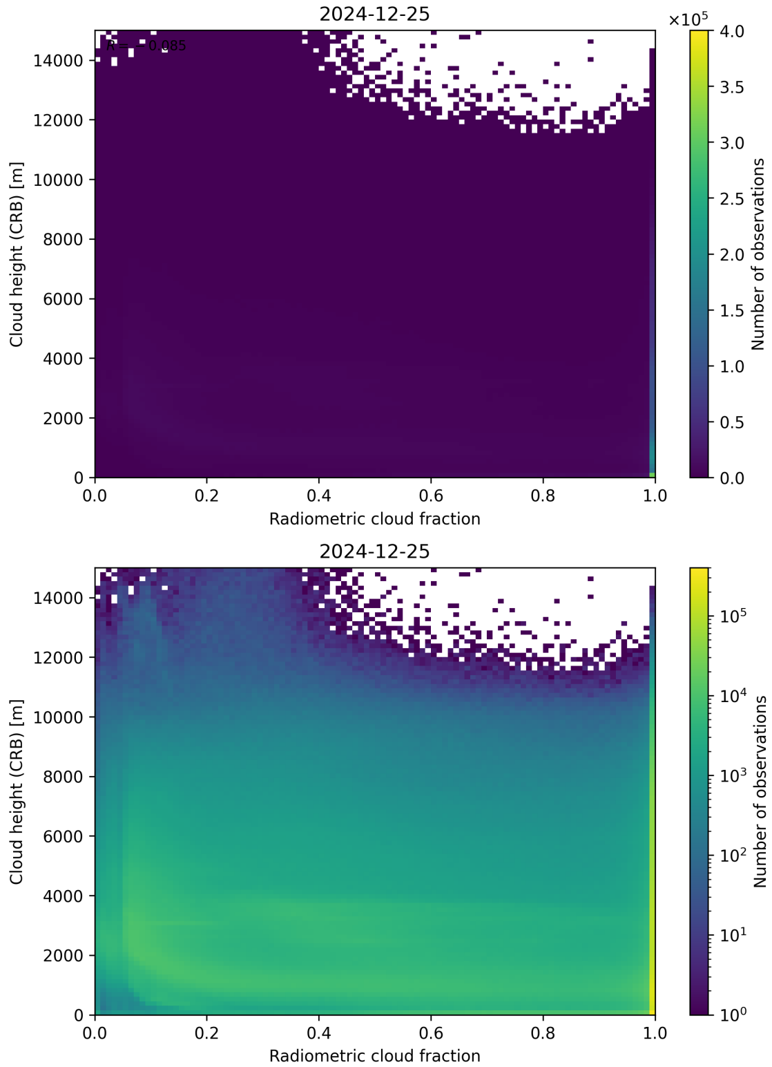
Figure 74: Scatter density plot of “Radiometric cloud fraction” against “Cloud height (CRB)” for 2024-12-24 to 2024-12-26.
