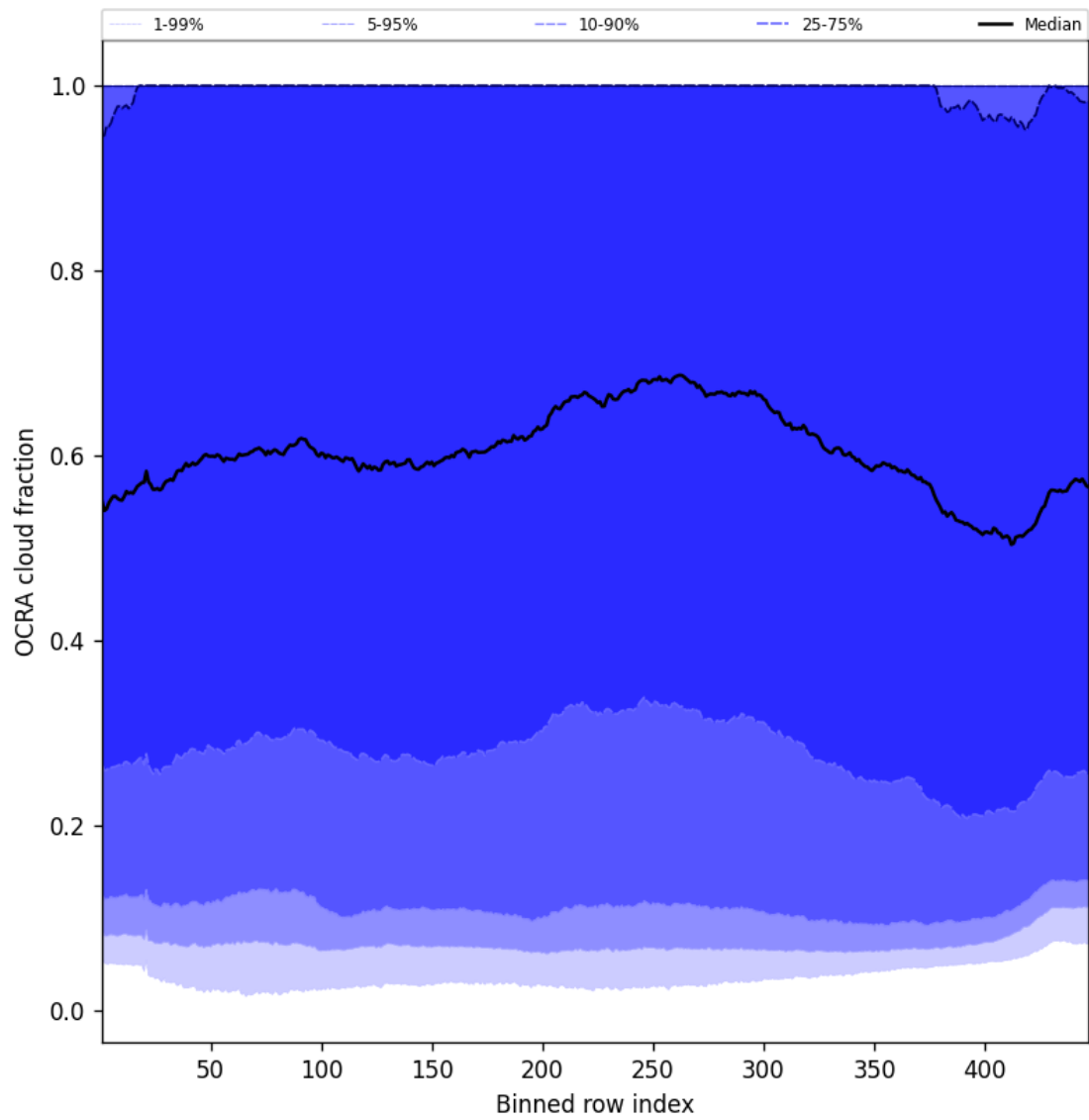
Figure 66: Along track statistics of “OCRA cloud fraction” for 2024-12-24 to 2024-12-26
