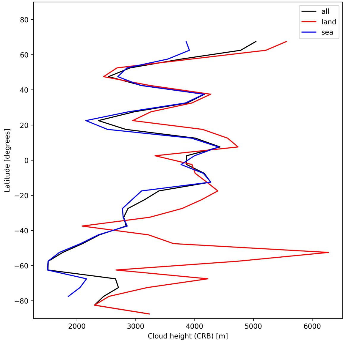
Figure 27: Zonal average of “Cloud height (CRB)” for 2024-12-24 to 2024-12-26.
