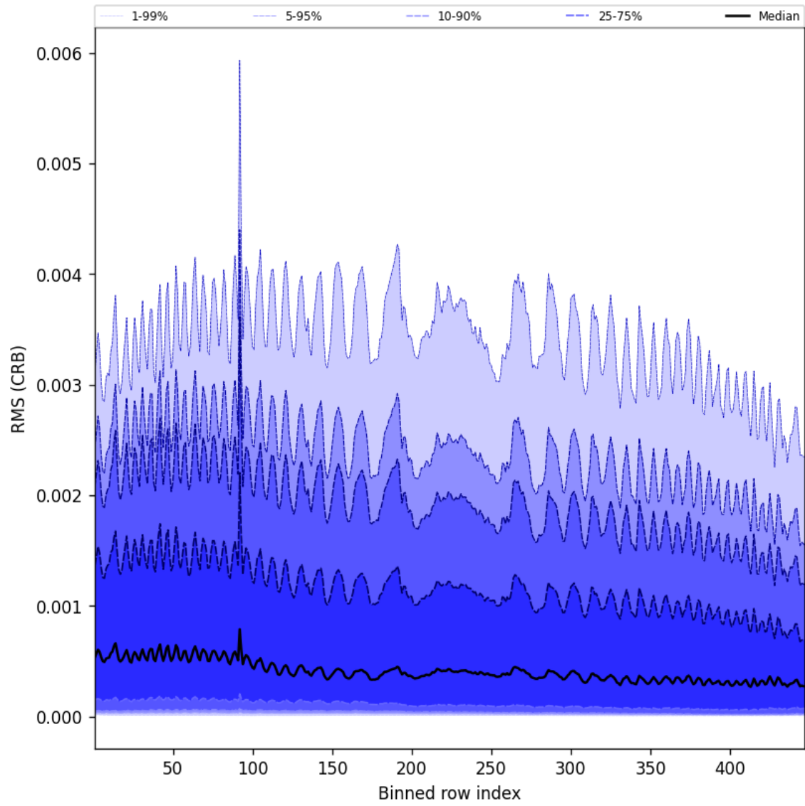
Figure 64: Along track statistics of “RMS (CRB)” for 2024-12-24 to 2024-12-26
