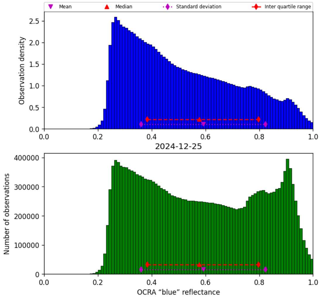
Figure 51: Histogram of “OCRA “blue” reflectance” for 2024-12-24 to 2024-12-26
