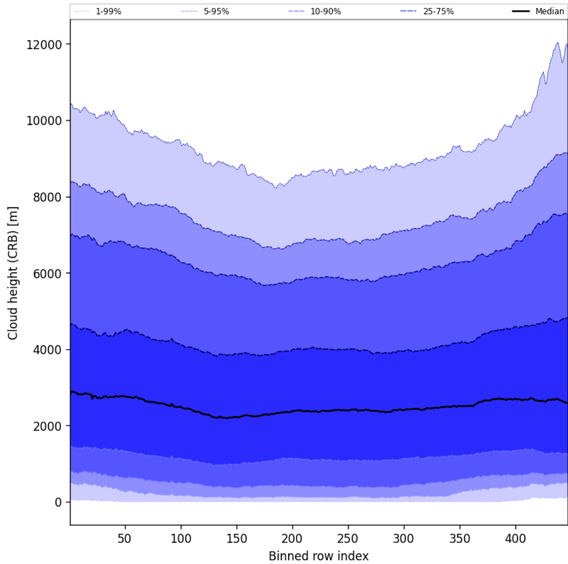
Figure 59: Along track statistics of “Cloud height (CRB)” for 2024-12-24 to 2024-12-26
