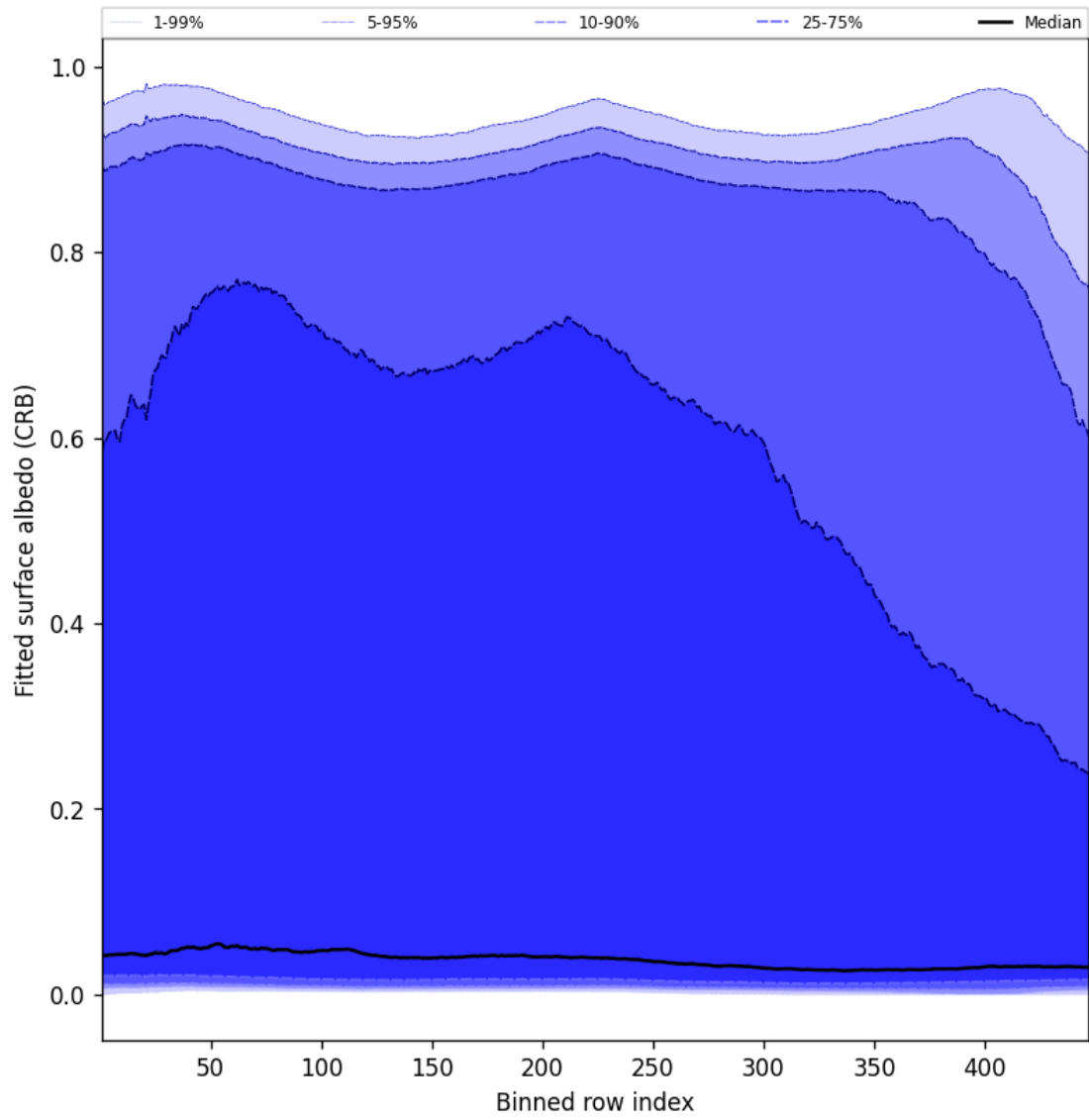
Figure 62: Along track statistics of “Fitted surface albedo (CRB)” for 2024-12-24 to 2024-12-26
