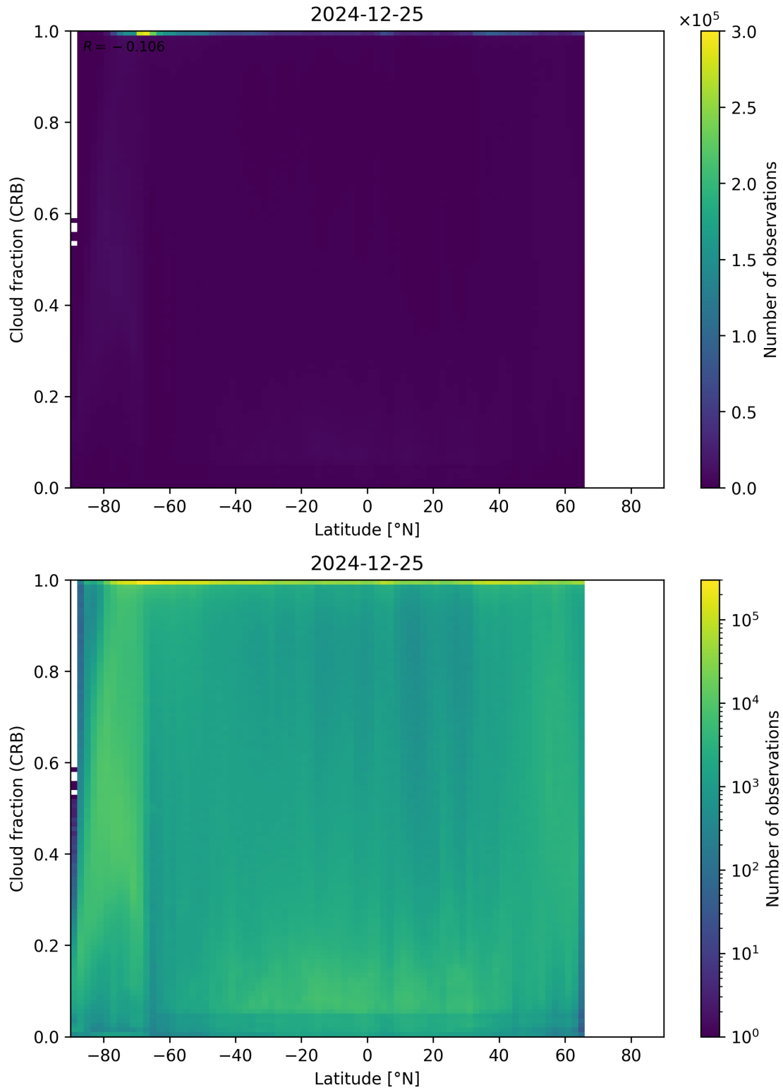
Figure 94: Scatter density plot of “Latitude” against “Cloud fraction (CRB)” for 2024-12-24 to 2024-12-26.
