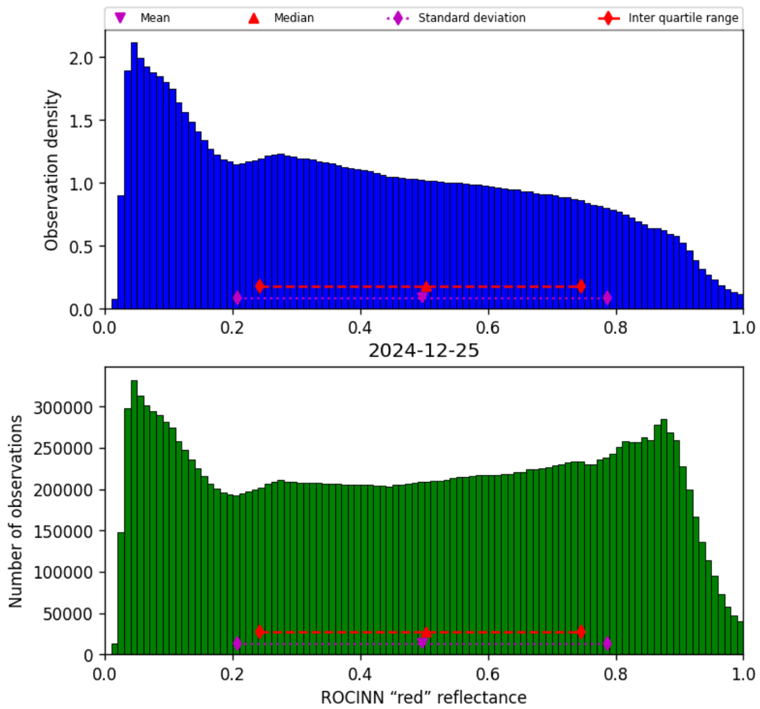
Figure 53: Histogram of “ROCINN “red” reflectance” for 2024-12-24 to 2024-12-26
