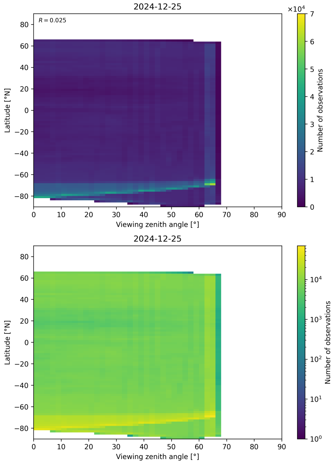
Figure 113: Scatter density plot of “Viewing zenith angle” against “Latitude” for 2024-12-24 to 2024-12-26.
