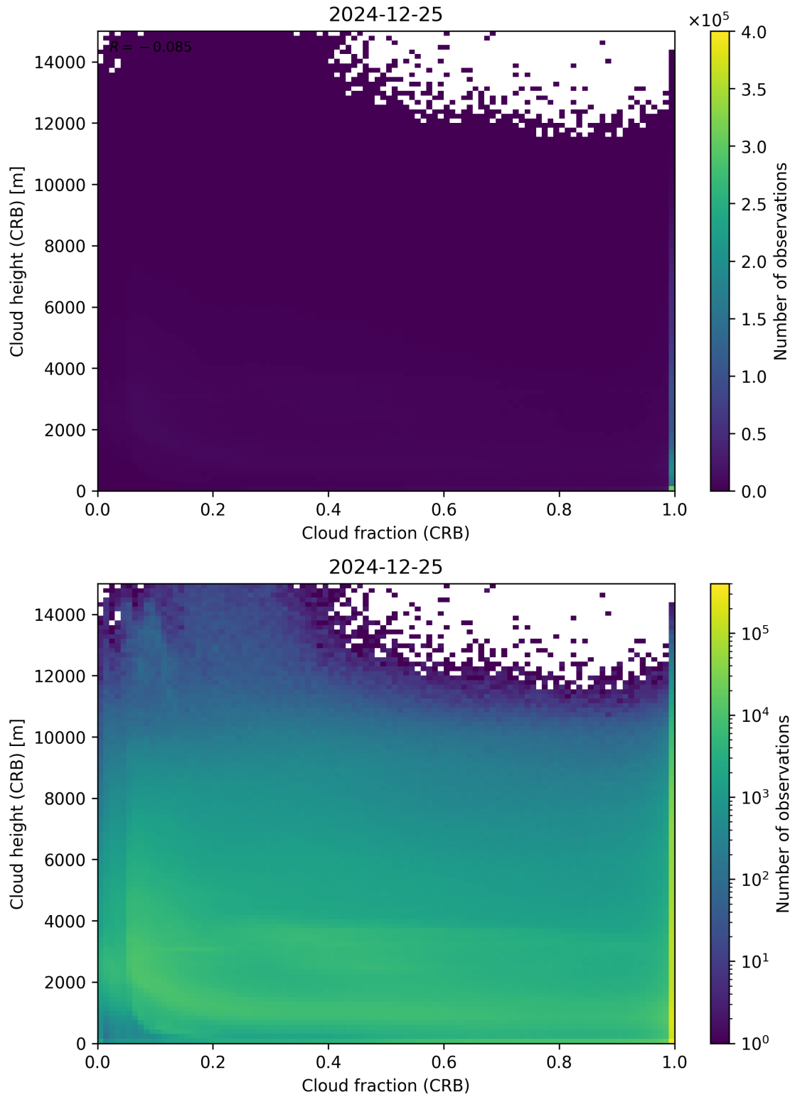
Figure 79: Scatter density plot of “Cloud fraction (CRB)” against “Cloud height (CRB)” for 2024-12-24 to 2024-12-26.
