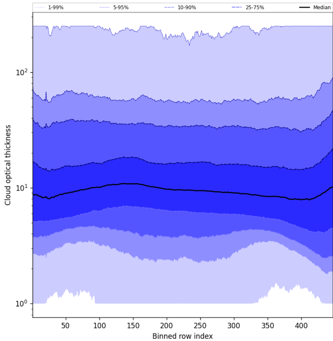
Figure 57: Along track statistics of “Cloud optical thickness” for 2024-12-24 to 2024-12-26
