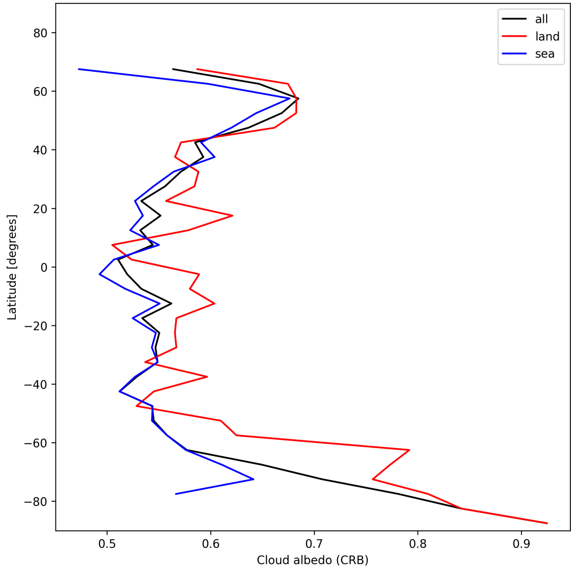
Figure 28: Zonal average of “Cloud albedo (CRB)” for 2024-12-24 to 2024-12-26.
