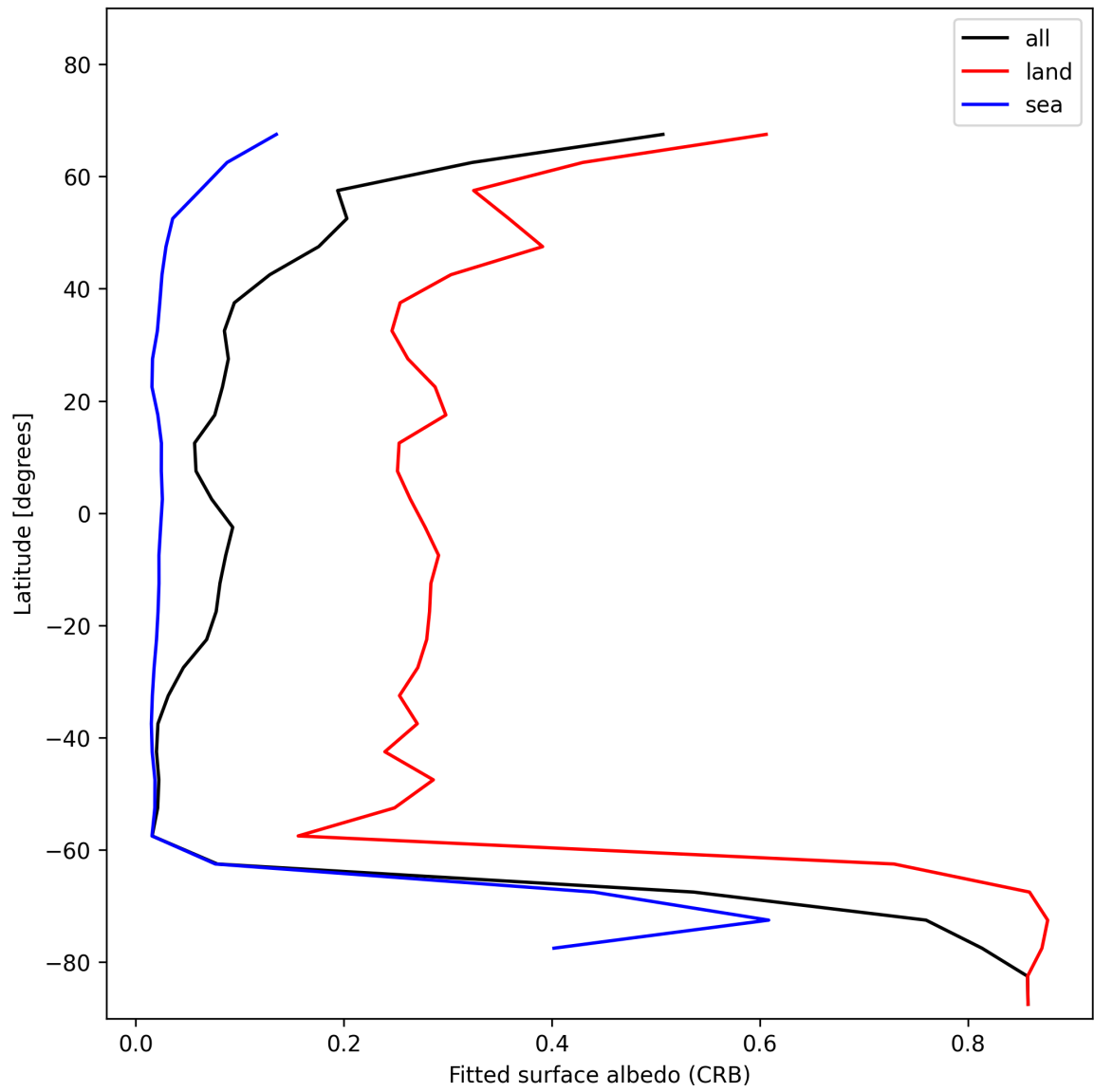
Figure 30: Zonal average of “Fitted surface albedo (CRB)” for 2024-12-24 to 2024-12-26.
