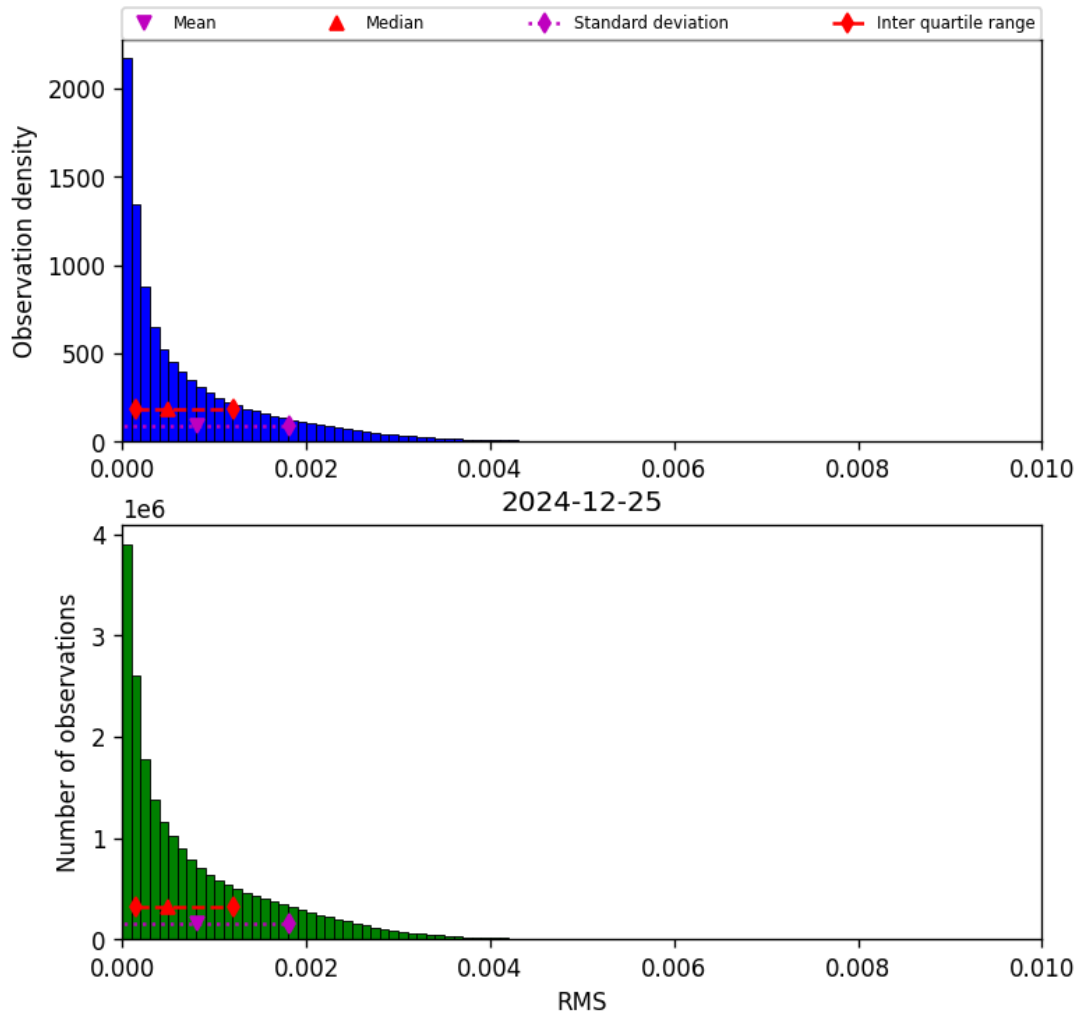
Figure 47: Histogram of “RMS” for 2024-12-24 to 2024-12-26
