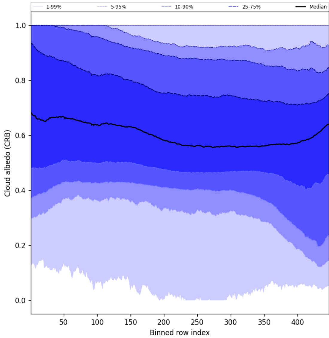
Figure 60: Along track statistics of “Cloud albedo (CRB)” for 2024-12-24 to 2024-12-26
