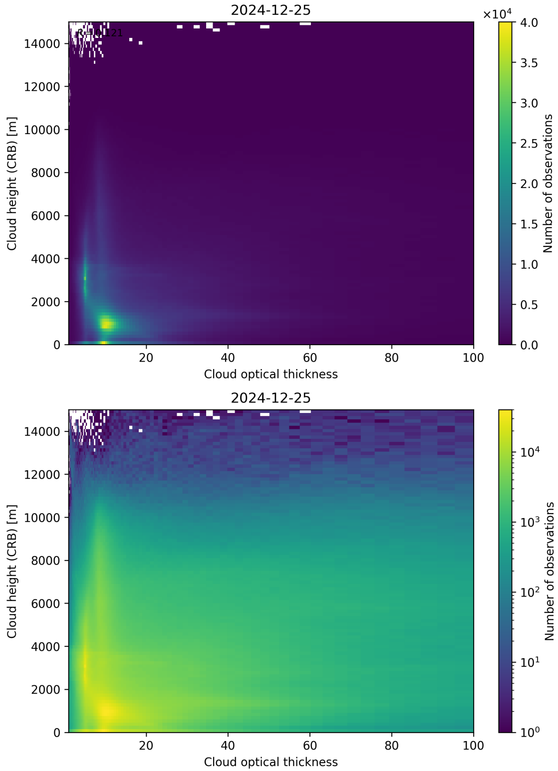
Figure 85: Scatter density plot of “Cloud optical thickness” against “Cloud height (CRB)” for 2024-12-24 to 2024-12-26.
