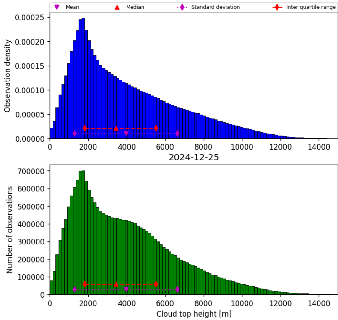
Figure 40: Histogram of “Cloud top height” for 2024-12-24 to 2024-12-26
