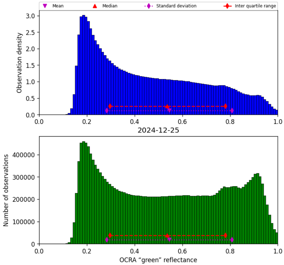
Figure 52: Histogram of “OCRA “green” reflectance” for 2024-12-24 to 2024-12-26
