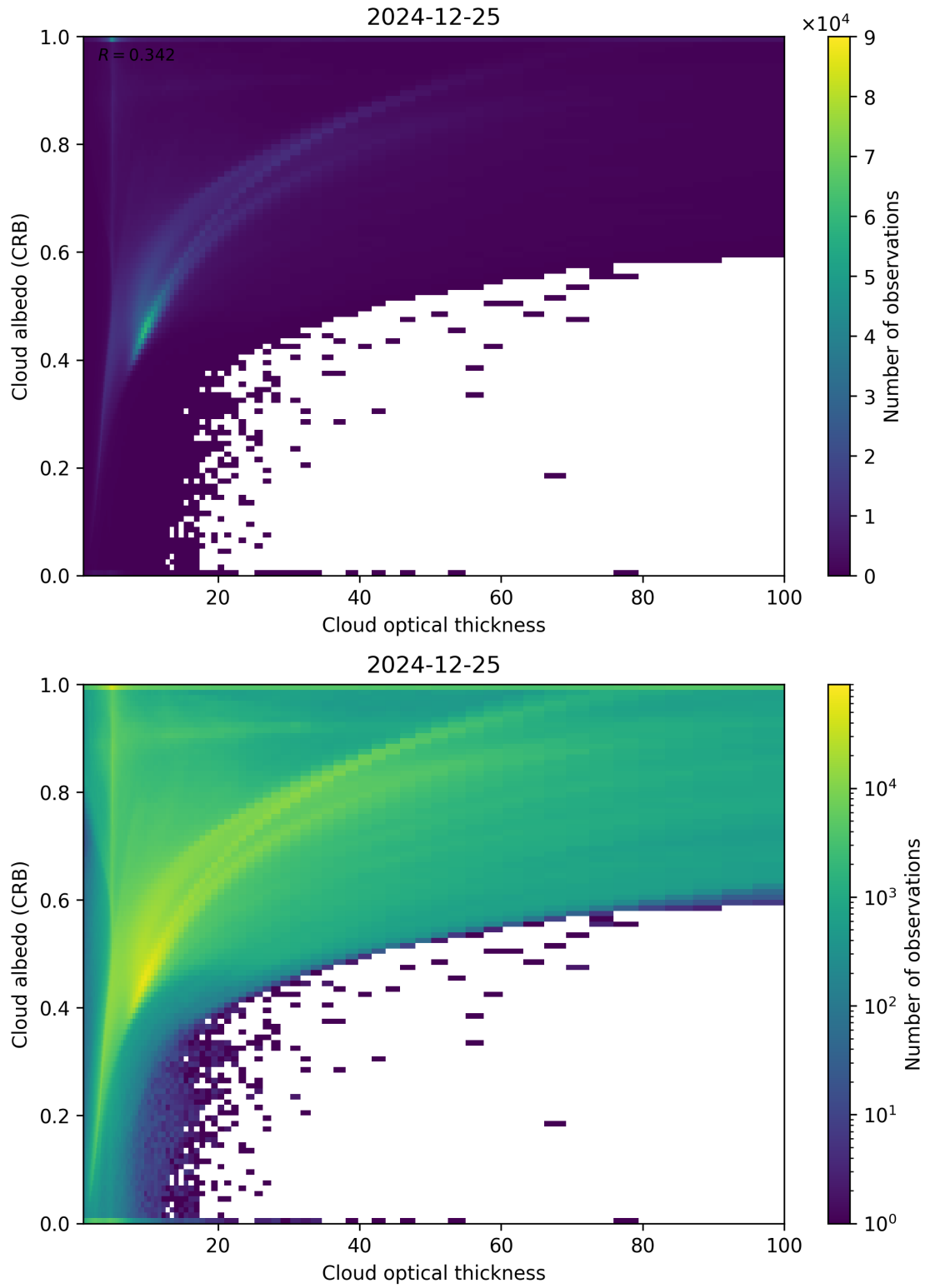
Figure 82: Scatter density plot of “Cloud optical thickness” against “Cloud albedo (CRB)” for 2024-12-24 to 2024-12-26.
