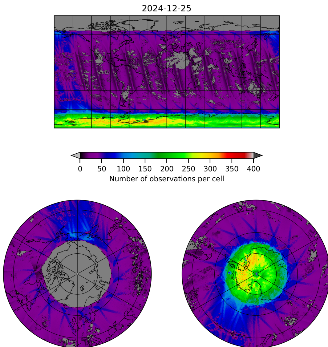
Figure 21: Map of the number of observations for 2024-12-24 to 2024-12-26
