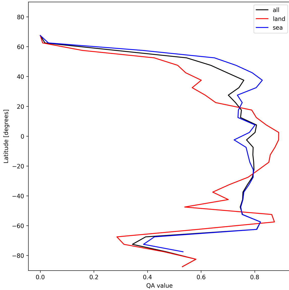
Figure 22: Zonal average of “QA value” for 2024-12-24 to 2024-12-26.
