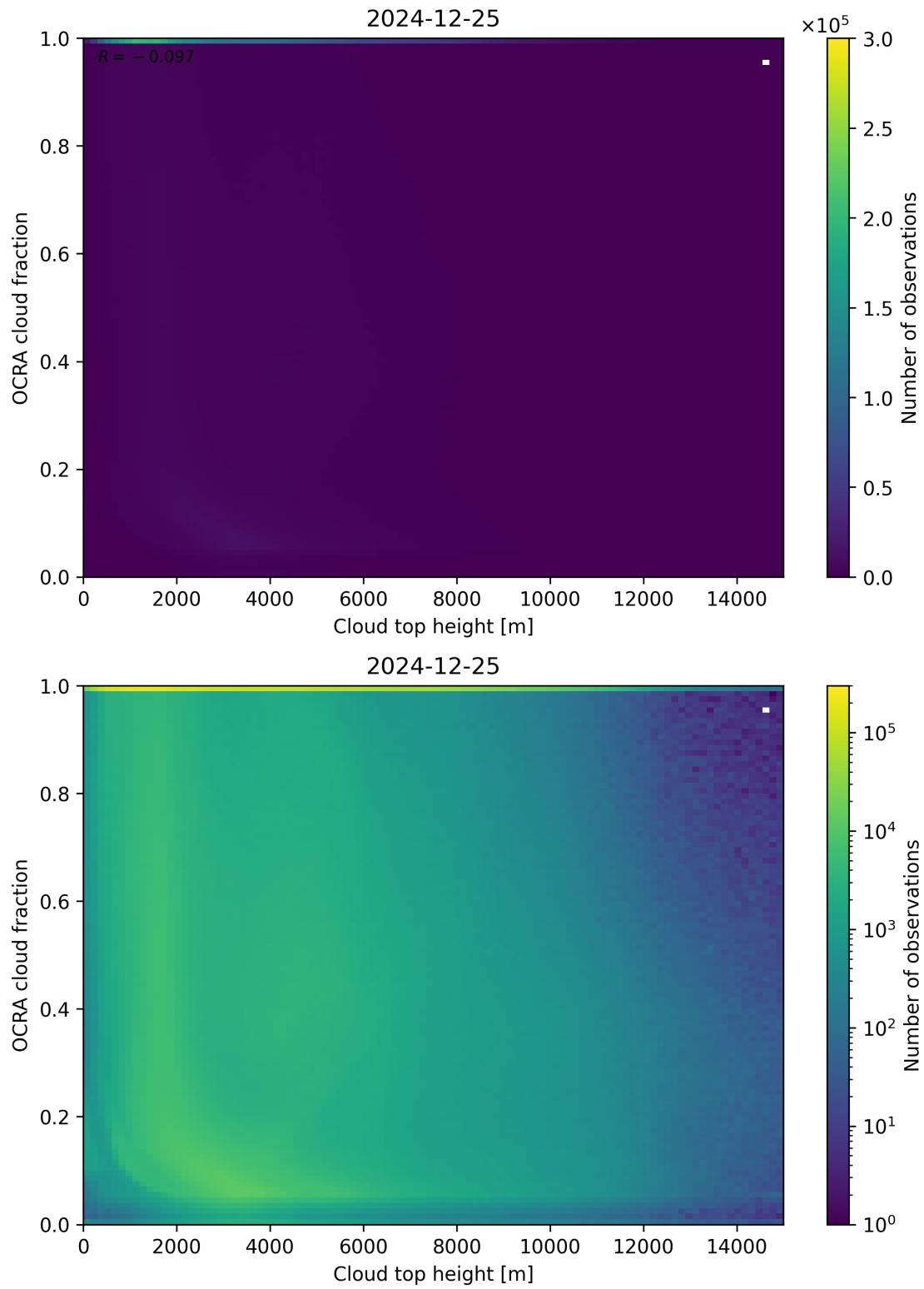
Figure 87: Scatter density plot of “Cloud top height” against “OCRA cloud fraction” for 2024-12-24 to 2024-12-26.
