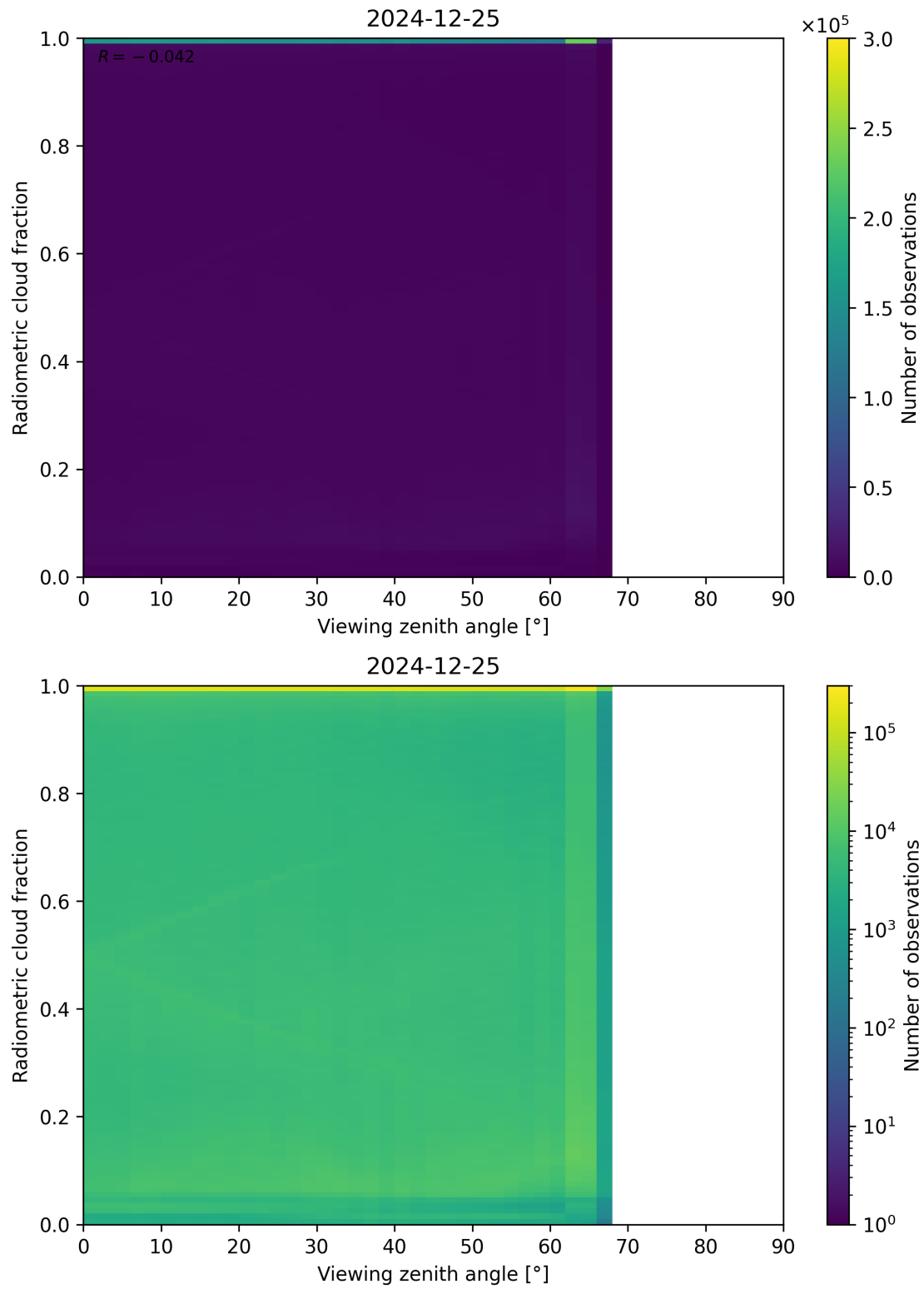
Figure 107: Scatter density plot of “Viewing zenith angle” against “Radiometric cloud fraction” for 2024-12-24 to 2024-12-26.
