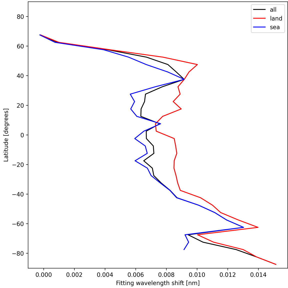
Figure 33: Zonal average of “Fitting wavelength shift” for 2024-12-24 to 2024-12-26.
