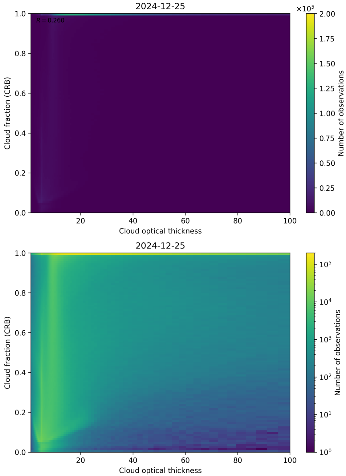
Figure 84: Scatter density plot of “Cloud optical thickness” against “Cloud fraction (CRB)” for 2024-12-24 to 2024-12-26.
