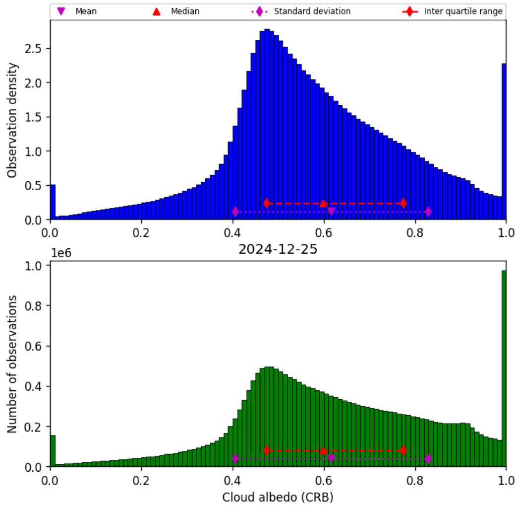
Figure 44: Histogram of “Cloud albedo (CRB)” for 2024-12-24 to 2024-12-26
