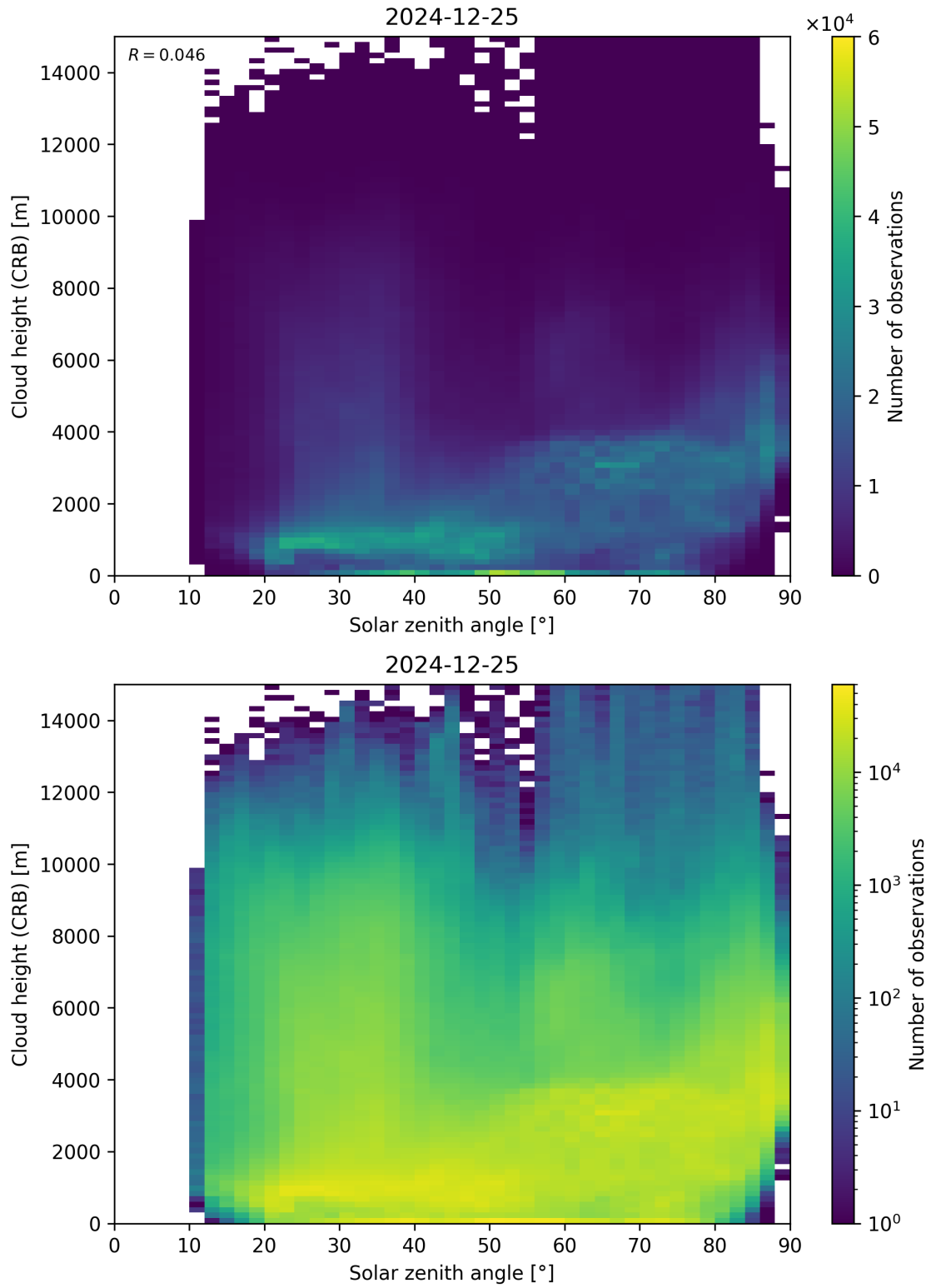
Figure 102: Scatter density plot of “Solar zenith angle” against “Cloud height (CRB)” for 2024-12-24 to 2024-12-26.
