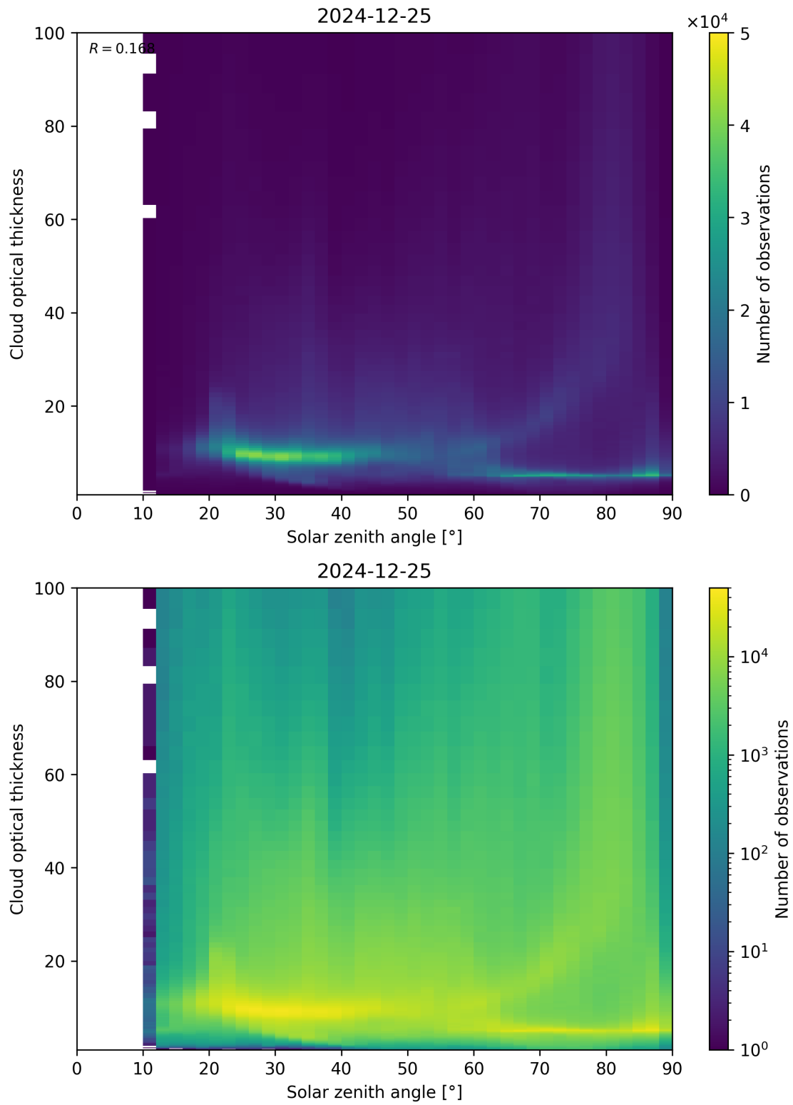
Figure 103: Scatter density plot of “Solar zenith angle” against “Cloud optical thickness” for 2024-12-24 to 2024-12-26.
