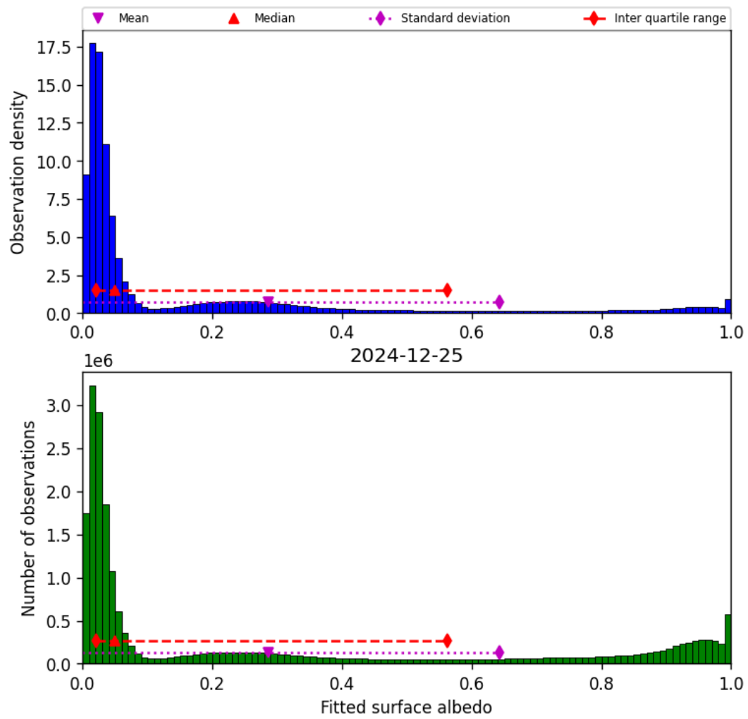
Figure 45: Histogram of “Fitted surface albedo” for 2024-12-24 to 2024-12-26
