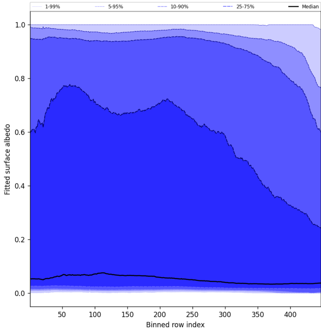
Figure 61: Along track statistics of “Fitted surface albedo” for 2024-12-24 to 2024-12-26
