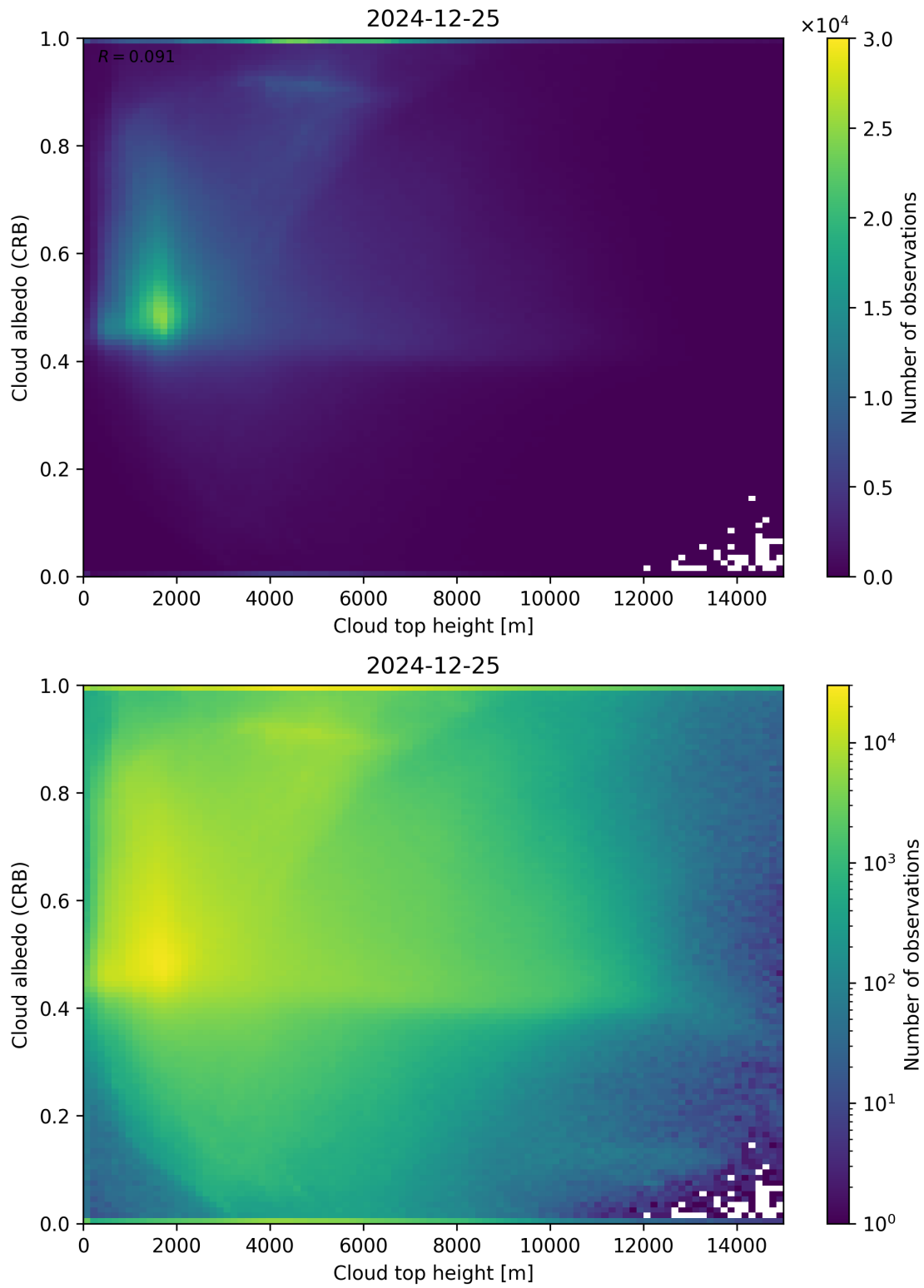
Figure 86: Scatter density plot of “Cloud top height” against “Cloud albedo (CRB)” for 2024-12-24 to 2024-12-26.
