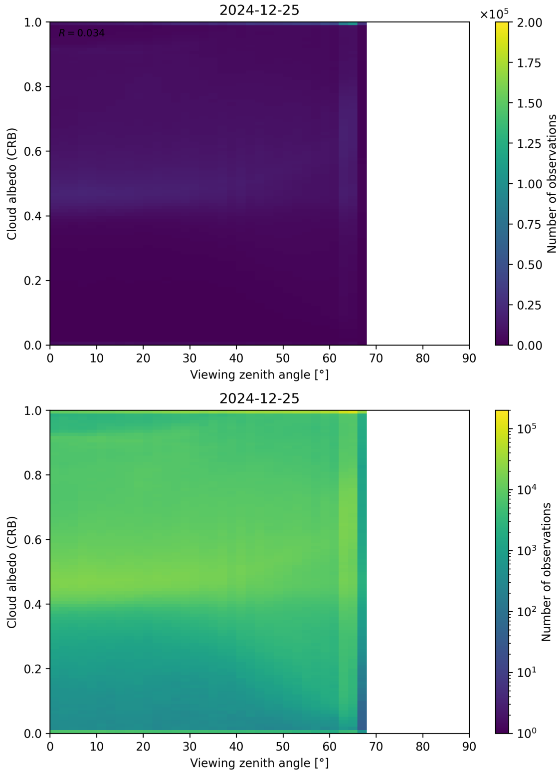
Figure 106: Scatter density plot of “Viewing zenith angle” against “Cloud albedo (CRB)” for 2024-12-24 to 2024-12-26.
