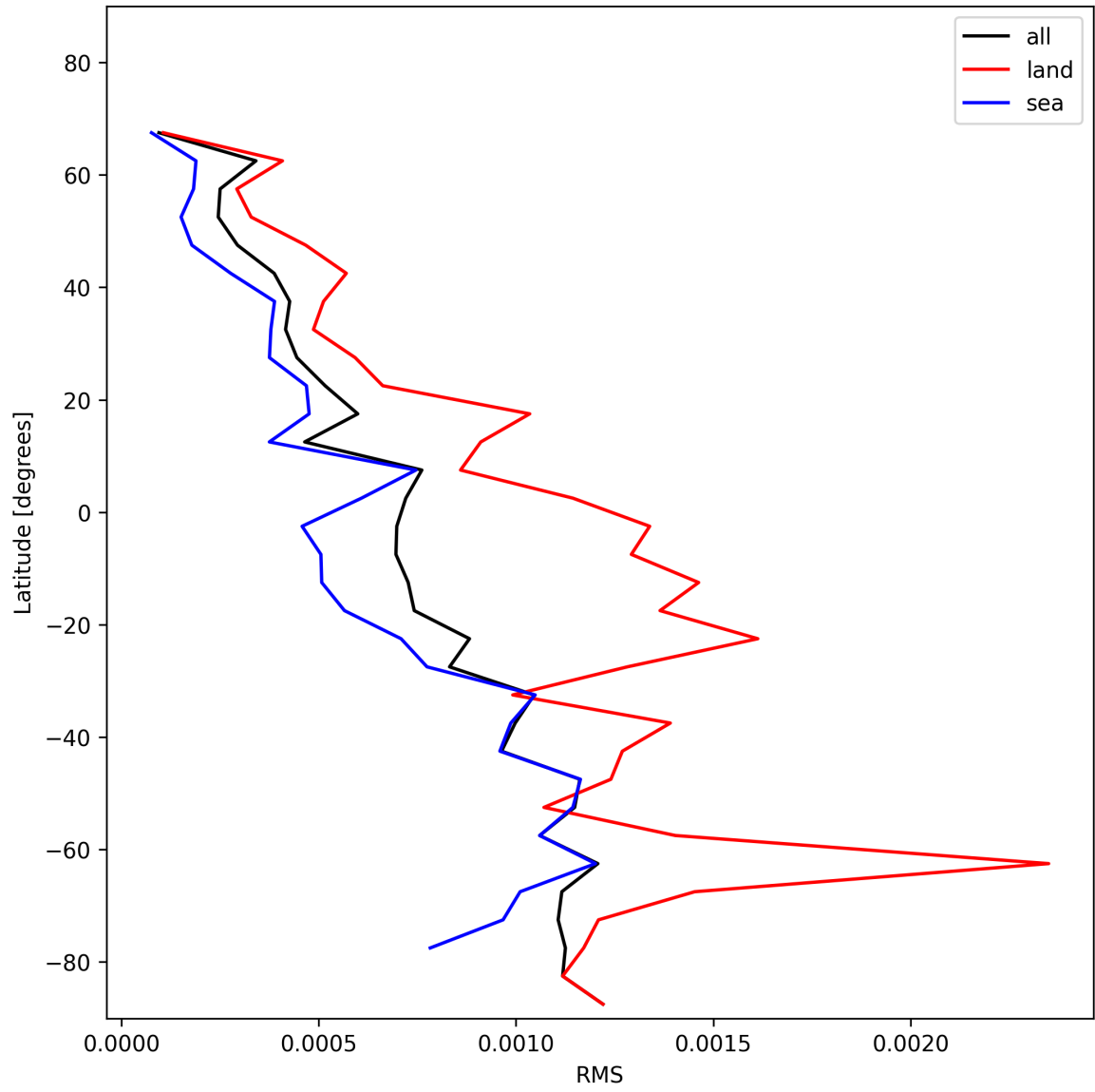
Figure 31: Zonal average of “RMS” for 2024-12-24 to 2024-12-26.
