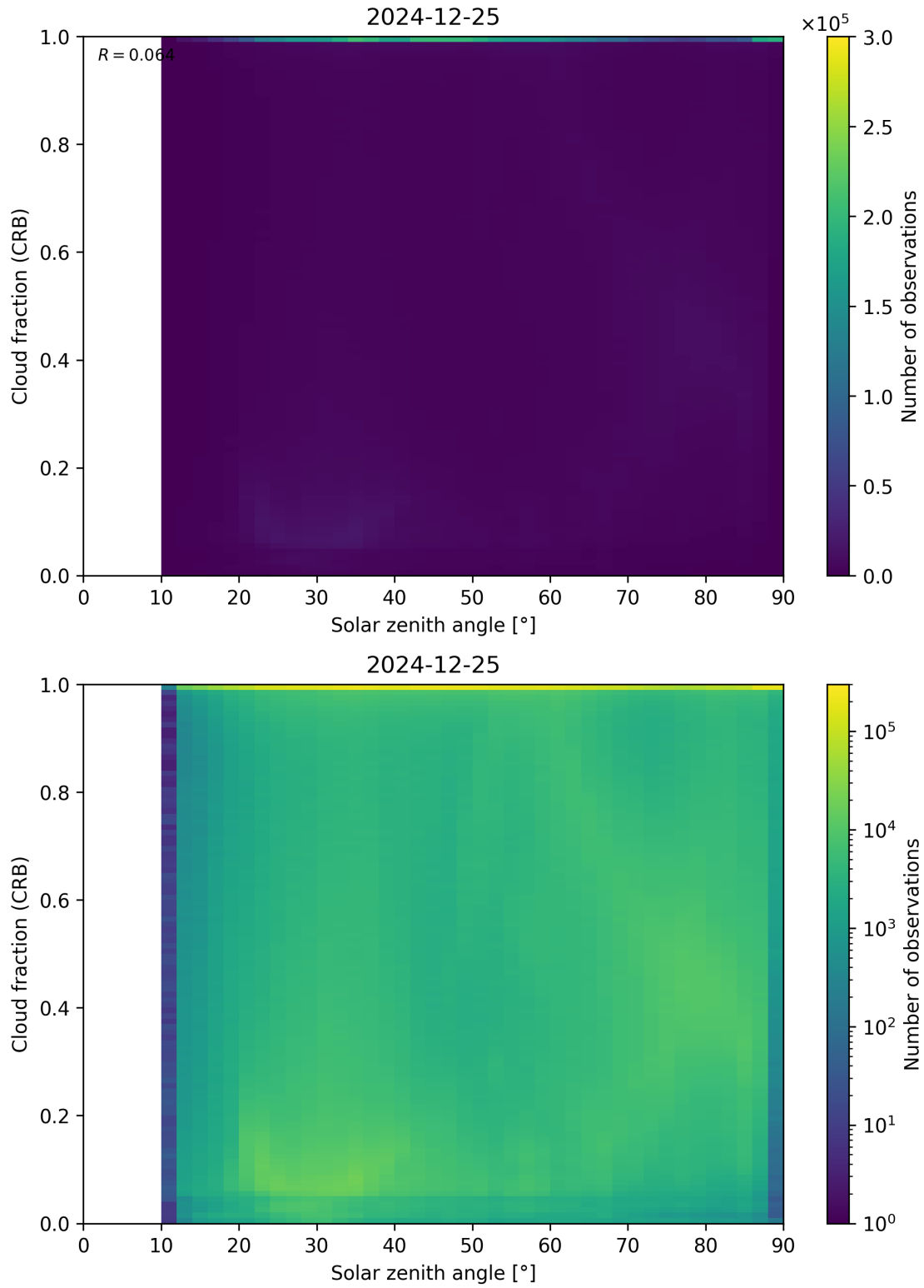
Figure 101: Scatter density plot of “Solar zenith angle” against “Cloud fraction (CRB)” for 2024-12-24 to 2024-12-26.
