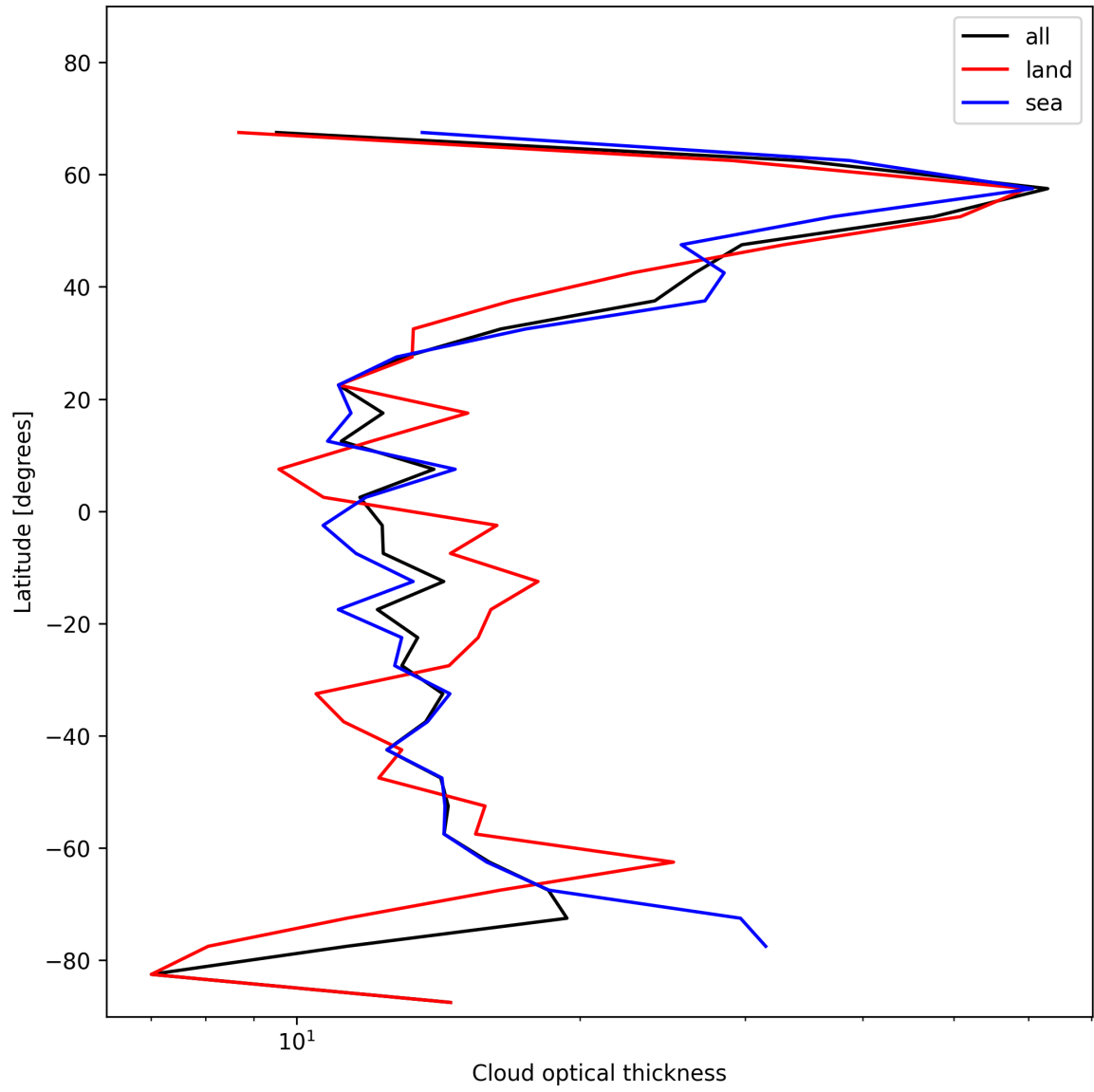
Figure 25: Zonal average of “Cloud optical thickness” for 2024-12-24 to 2024-12-26.
