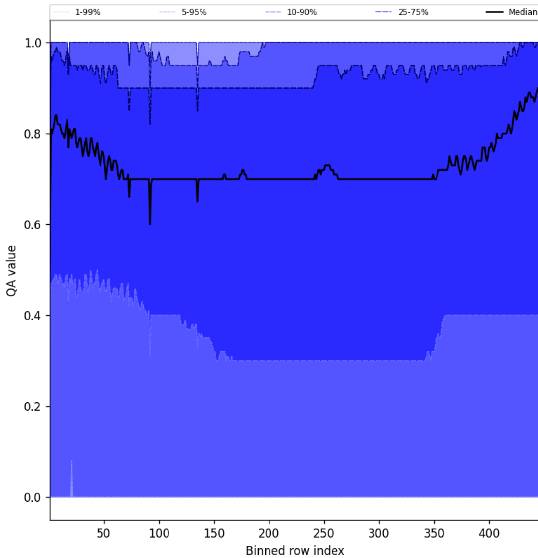
Figure 54: Along track statistics of “QA value” for 2024-12-24 to 2024-12-26
