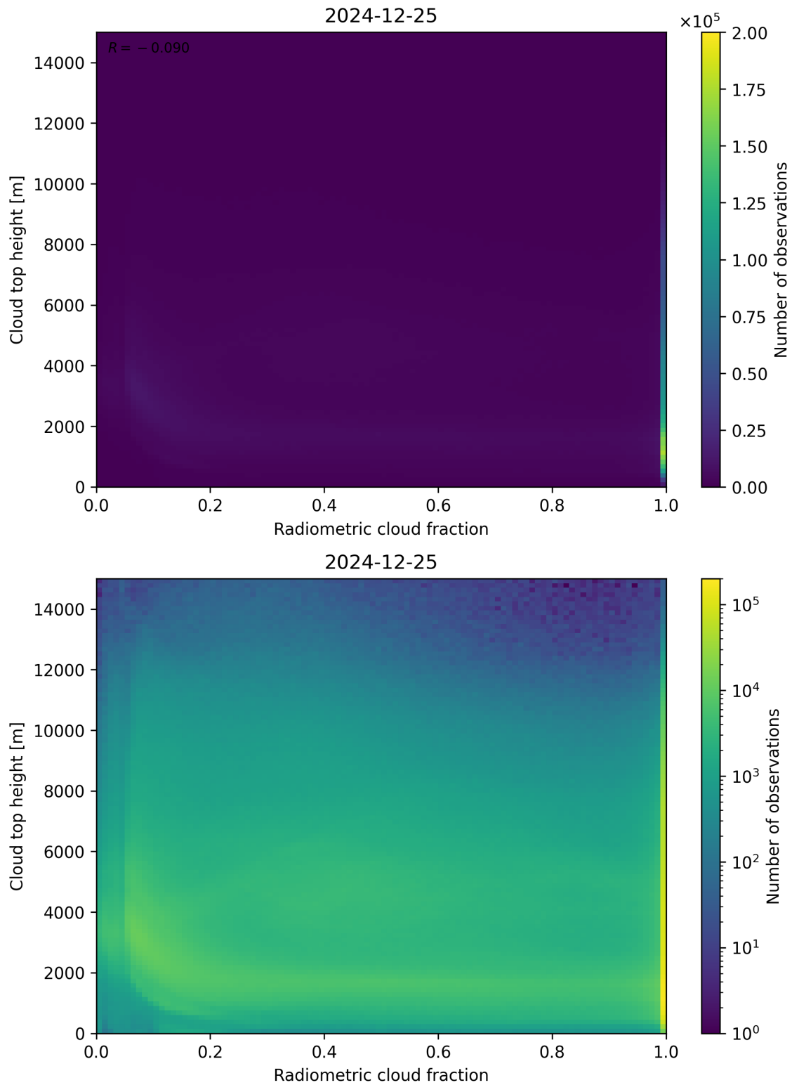
Figure 76: Scatter density plot of “Radiometric cloud fraction” against “Cloud top height” for 2024-12-24 to 2024-12-26.
