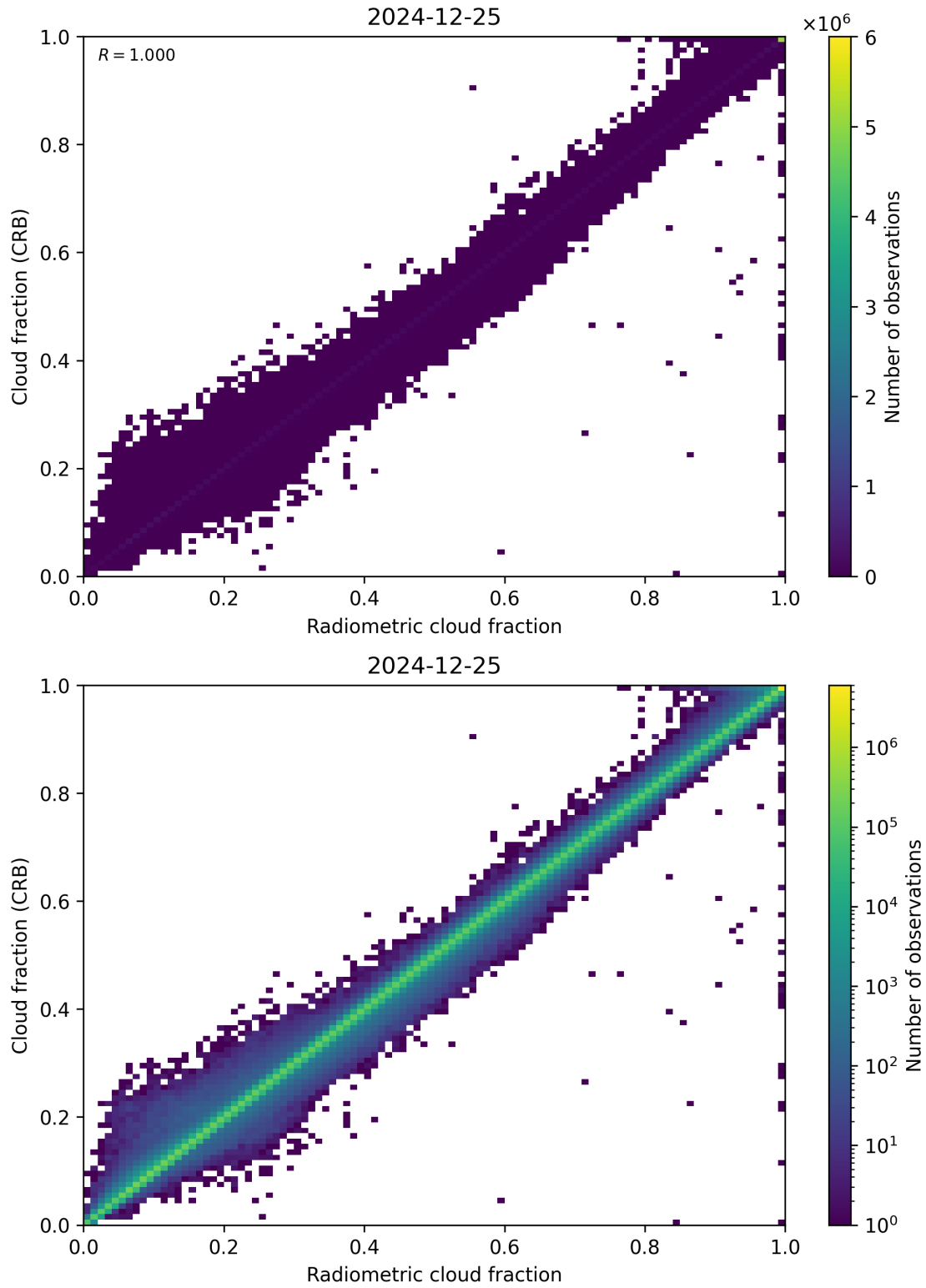
Figure 73: Scatter density plot of “Radiometric cloud fraction” against “Cloud fraction (CRB)” for 2024-12-24 to 2024-12-26.
