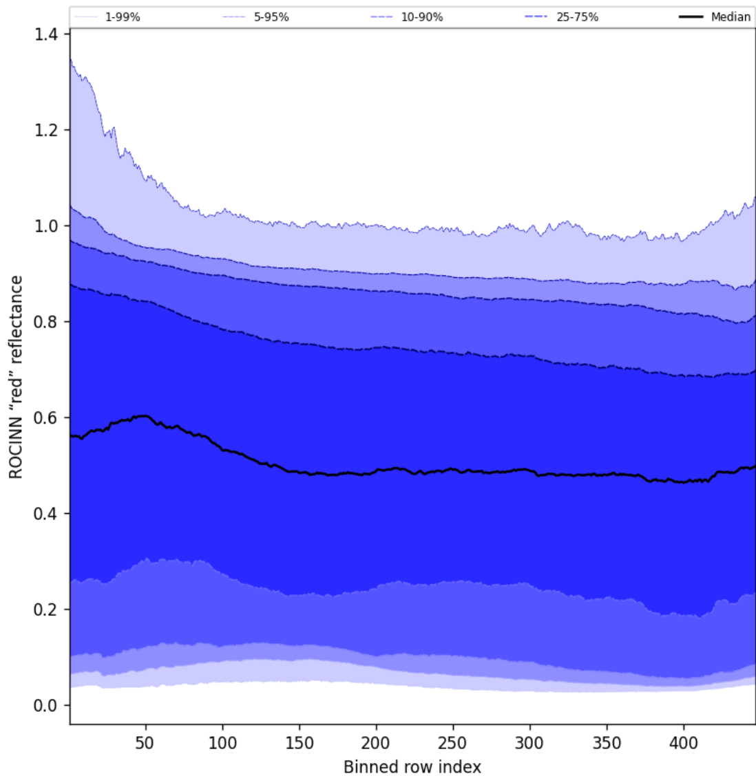
Figure 69: Along track statistics of “ROCINN “red” reflectance” for 2024-12-24 to 2024-12-26
