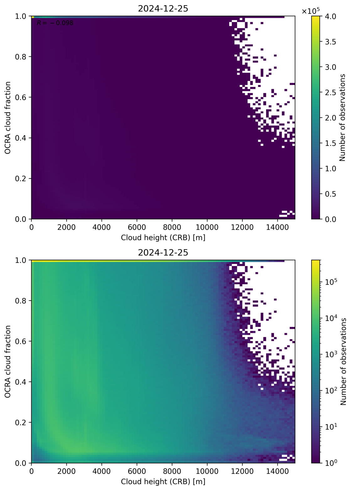
Figure 81: Scatter density plot of “Cloud height (CRB)” against “OCRA cloud fraction” for 2024-12-24 to 2024-12-26.
