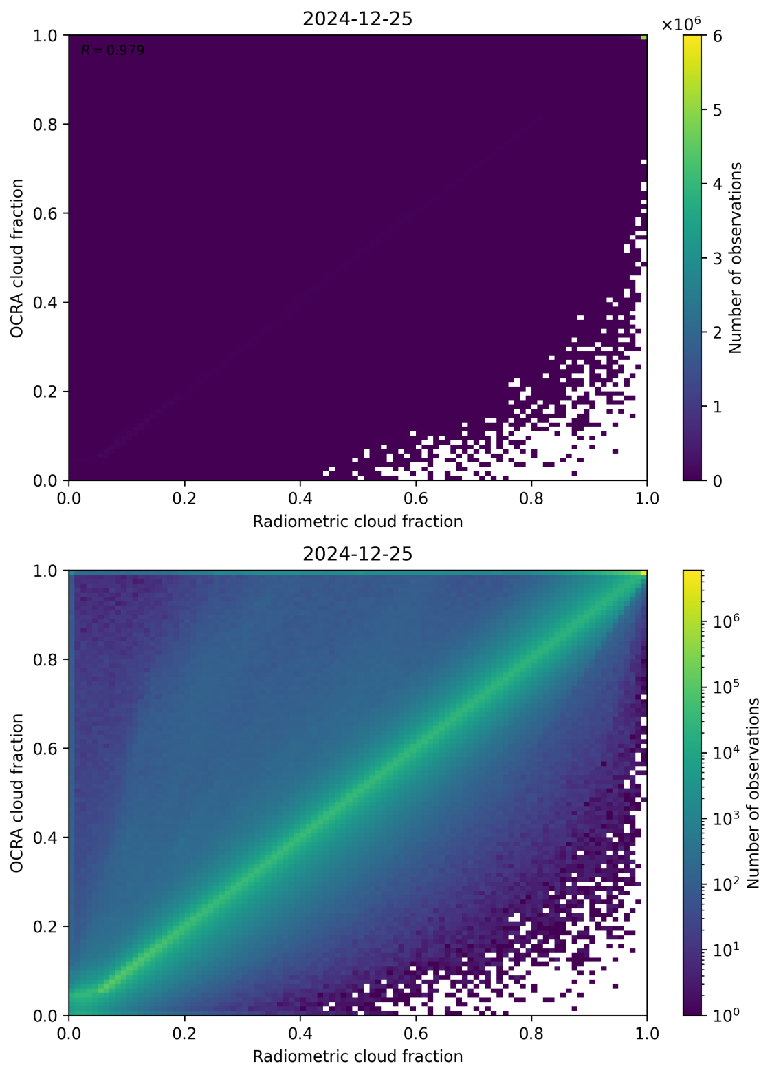
Figure 72: Scatter density plot of “Radiometric cloud fraction” against “OCRA cloud fraction” for 2024-12-24 to 2024-12-26.
