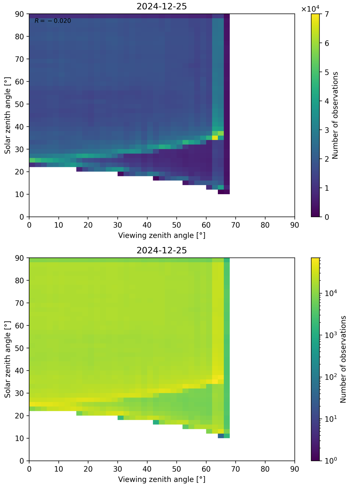
Figure 114: Scatter density plot of “Viewing zenith angle” against “Solar zenith angle” for 2024-12-24 to 2024-12-26.
