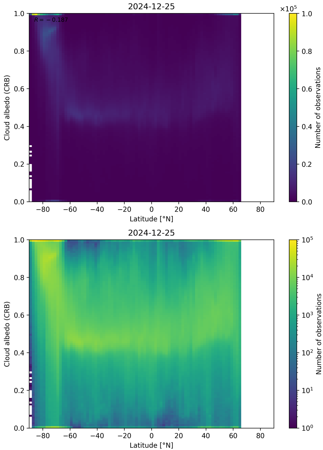
Figure 91: Scatter density plot of “Latitude” against “Cloud albedo (CRB)” for 2024-12-24 to 2024-12-26.
