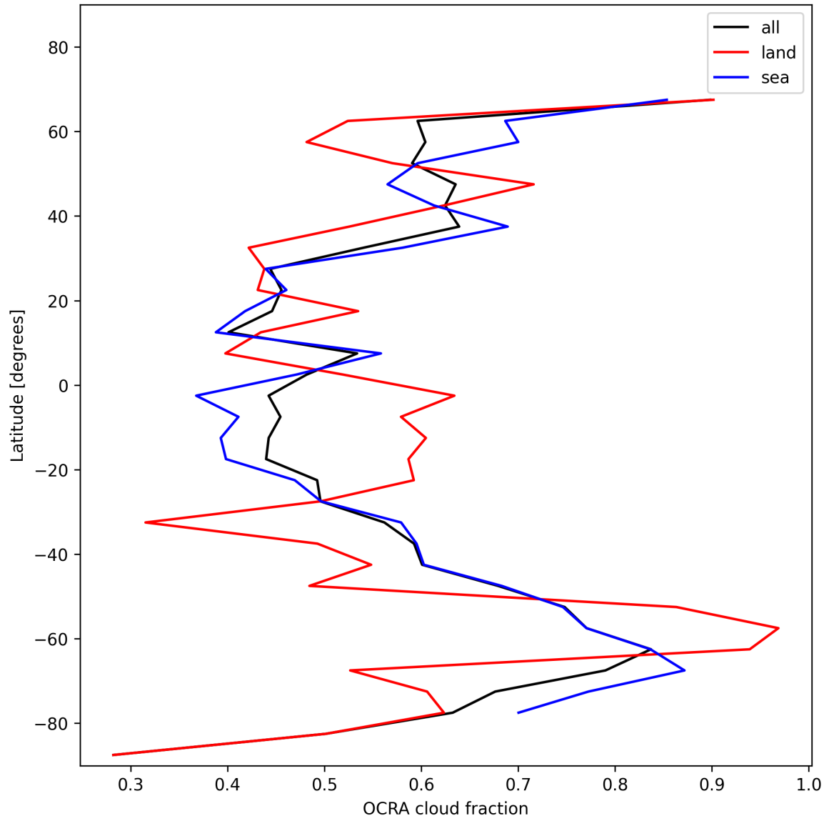
Figure 34: Zonal average of “OCRA cloud fraction” for 2024-12-24 to 2024-12-26.
