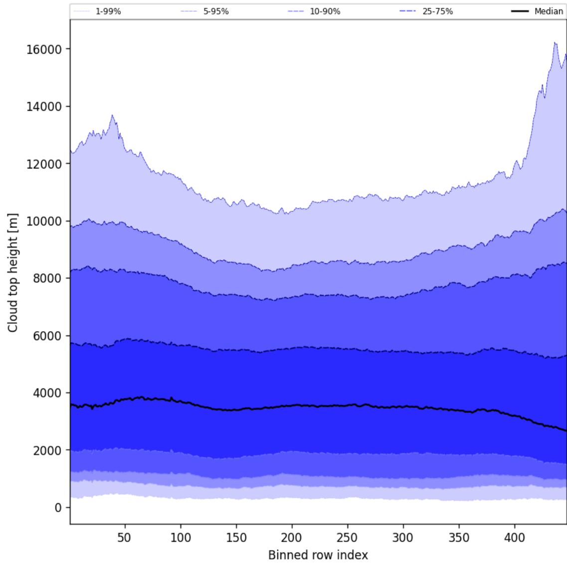
Figure 56: Along track statistics of “Cloud top height” for 2024-12-24 to 2024-12-26
