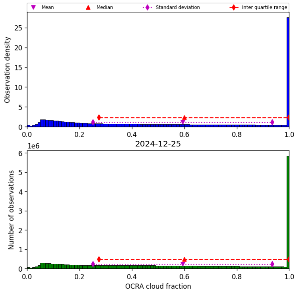
Figure 50: Histogram of “OCRA cloud fraction” for 2024-12-24 to 2024-12-26
