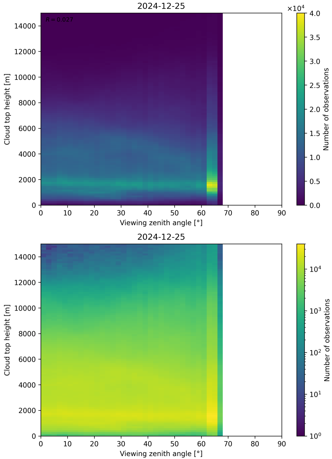
Figure 112: Scatter density plot of “Viewing zenith angle” against “Cloud top height” for 2024-12-24 to 2024-12-26.
