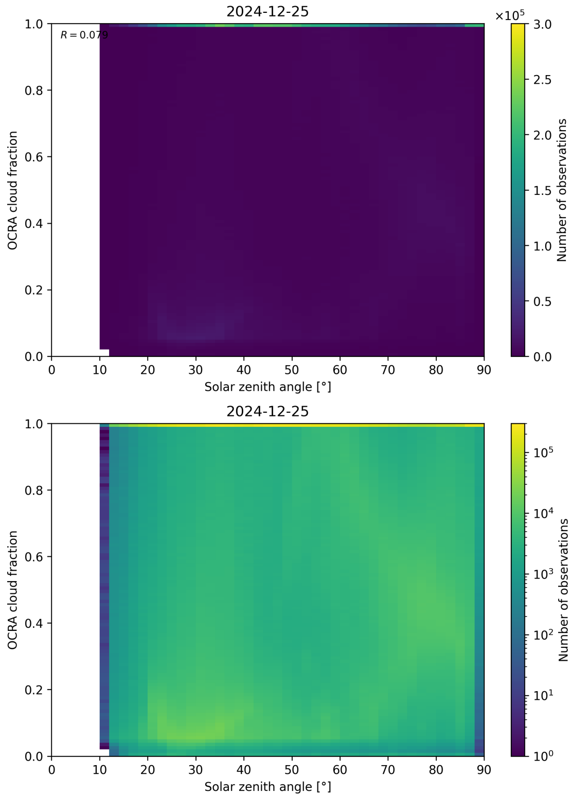
Figure 100: Scatter density plot of “Solar zenith angle” against “OCRA cloud fraction” for 2024-12-24 to 2024-12-26.
