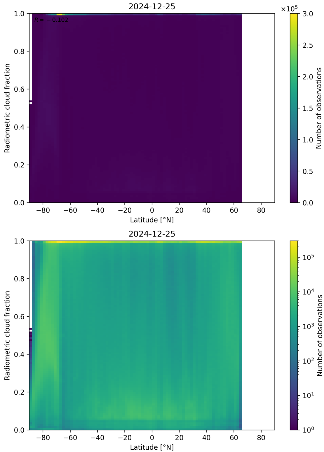
Figure 92: Scatter density plot of “Latitude” against “Radiometric cloud fraction” for 2024-12-24 to 2024-12-26.
