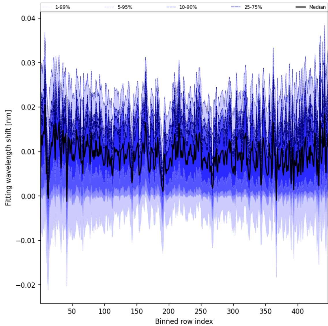
Figure 65: Along track statistics of “Fitting wavelength shift” for 2024-12-24 to 2024-12-26
