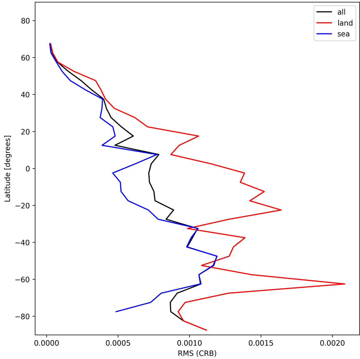
Figure 32: Zonal average of “RMS (CRB)” for 2024-12-24 to 2024-12-26.
