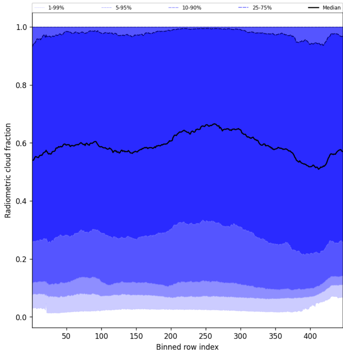
Figure 55: Along track statistics of “Radiometric cloud fraction” for 2024-12-24 to 2024-12-26
