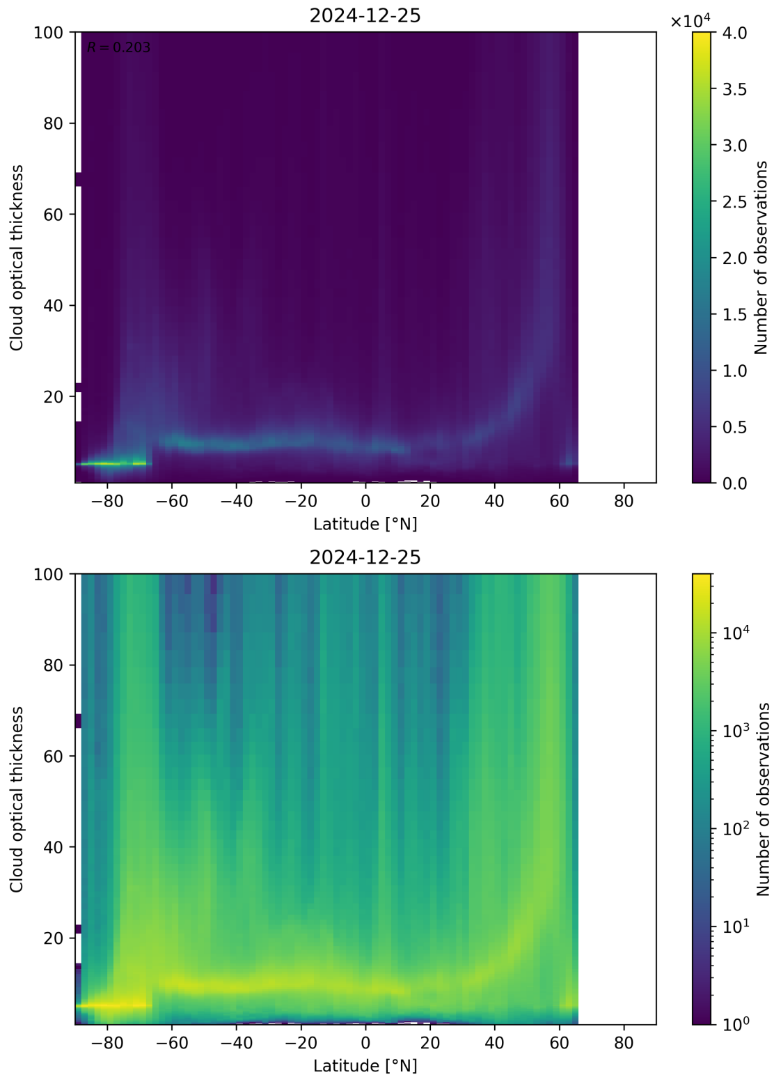
Figure 96: Scatter density plot of “Latitude” against “Cloud optical thickness” for 2024-12-24 to 2024-12-26.
