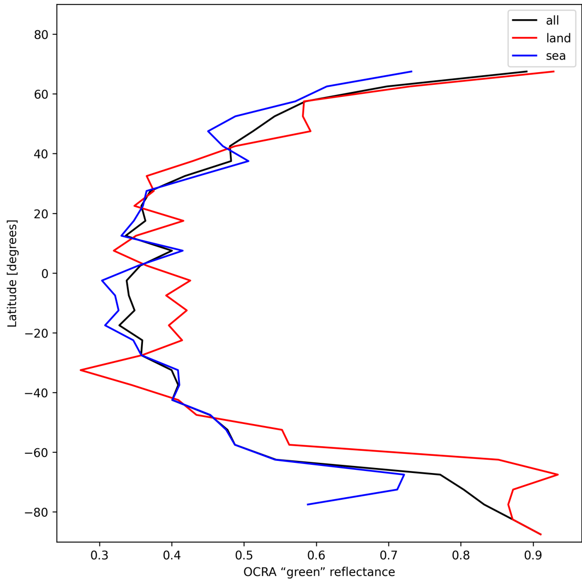
Figure 36: Zonal average of “OCRA “green” reflectance” for 2024-12-24 to 2024-12-26.
