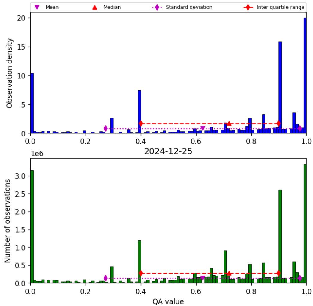
Figure 38: Histogram of “QA value” for 2024-12-24 to 2024-12-26
