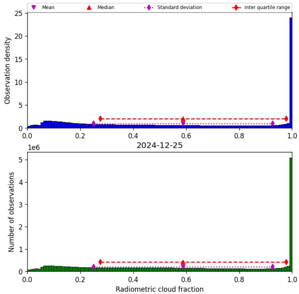
Figure 39: Histogram of “Radiometric cloud fraction” for 2024-12-24 to 2024-12-26
