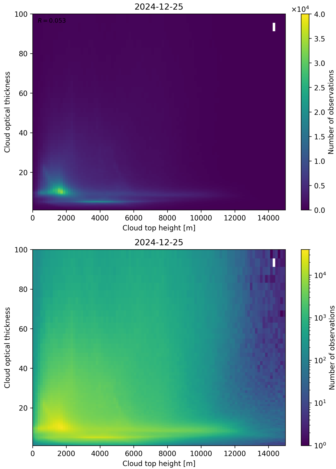
Figure 90: Scatter density plot of “Cloud top height” against “Cloud optical thickness” for 2024-12-24 to 2024-12-26.
