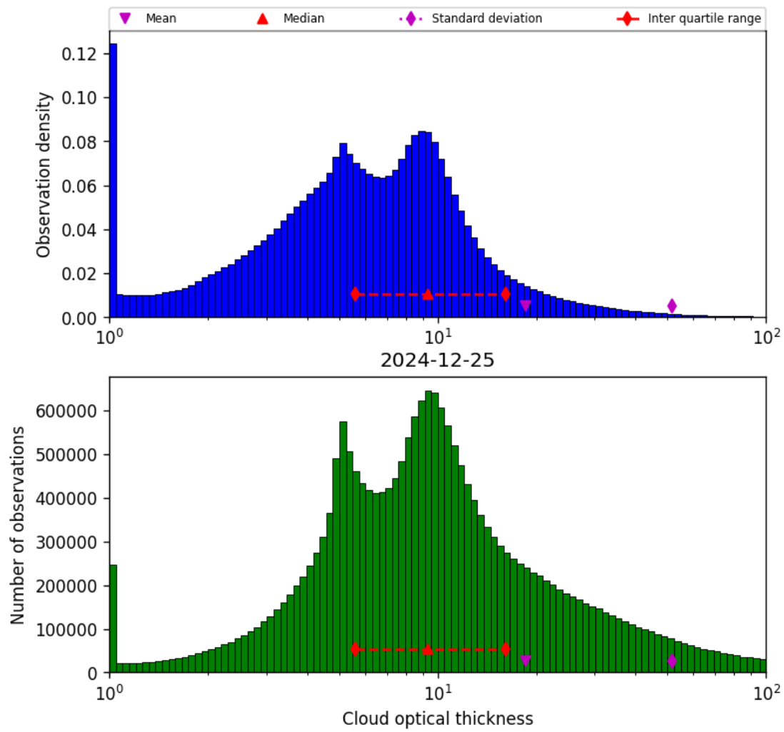
Figure 41: Histogram of “Cloud optical thickness” for 2024-12-24 to 2024-12-26
