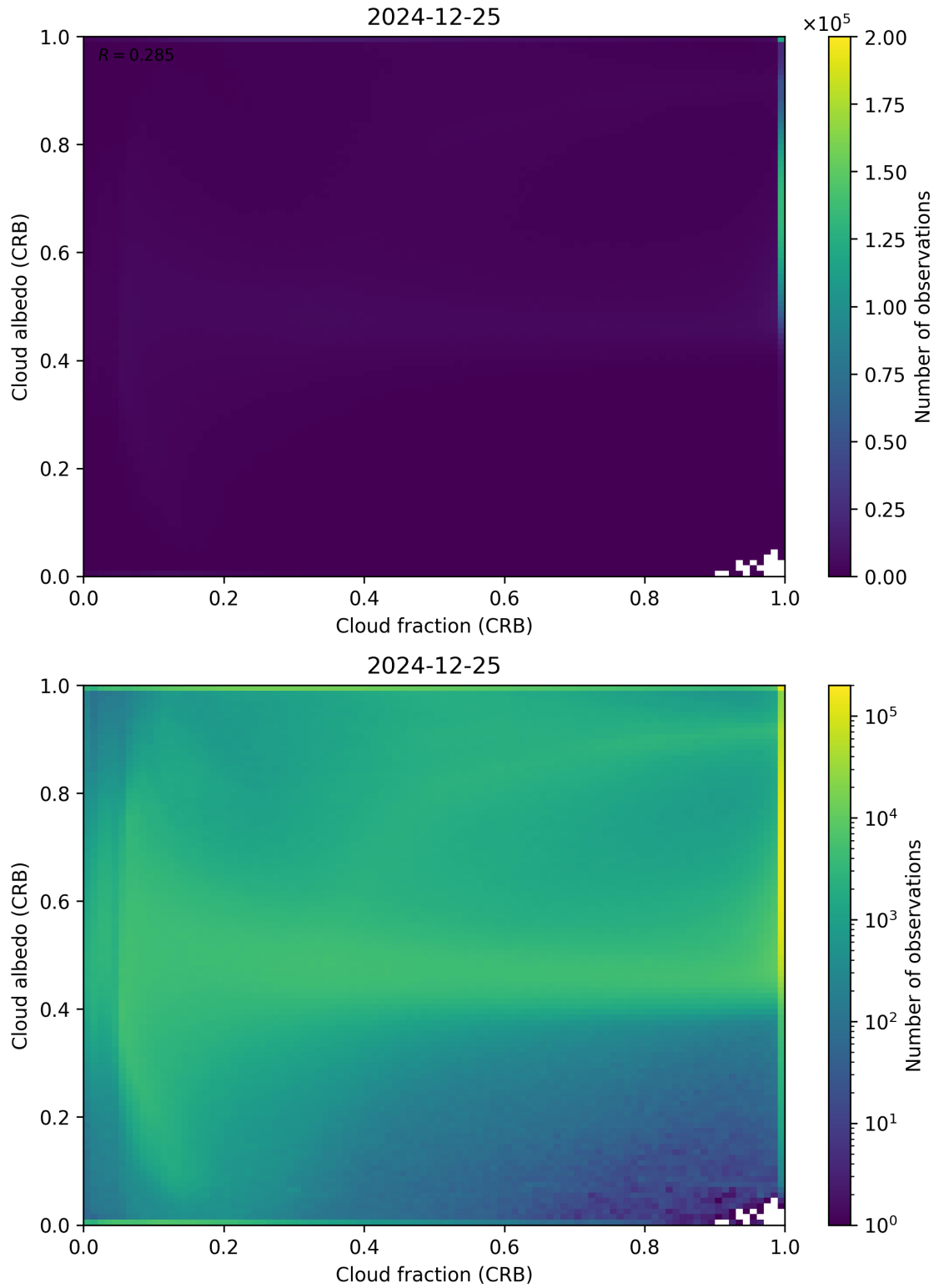
Figure 77: Scatter density plot of “Cloud fraction (CRB)” against “Cloud albedo (CRB)” for 2024-12-24 to 2024-12-26.
