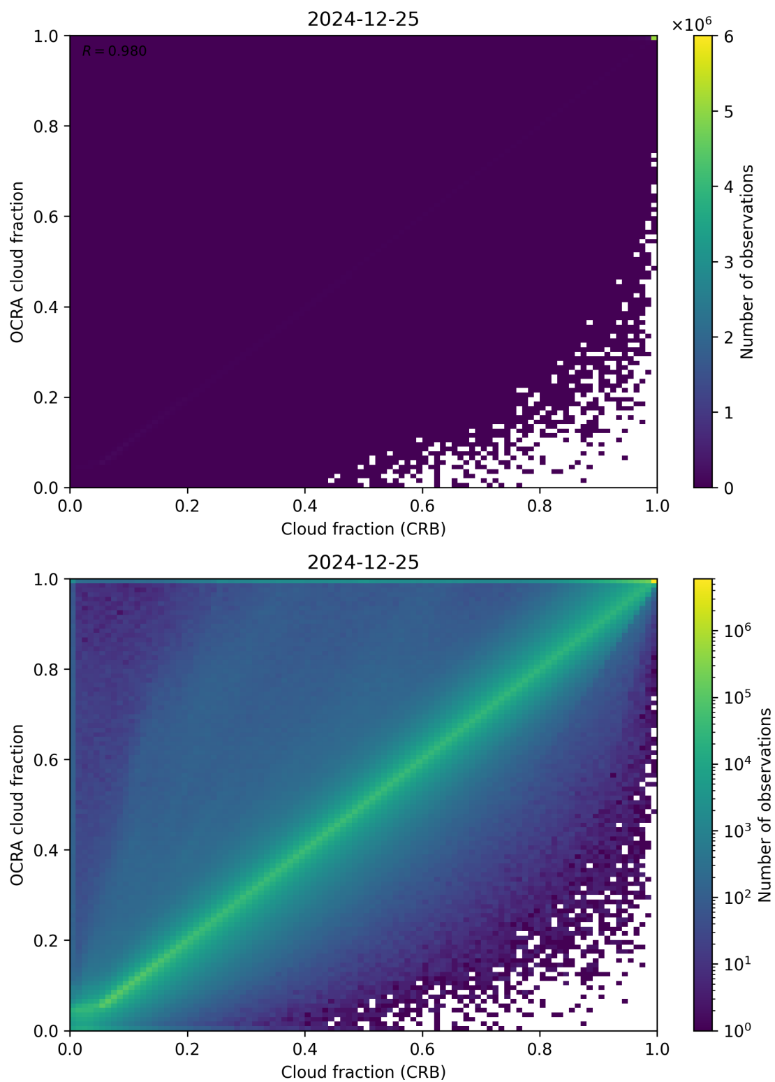
Figure 78: Scatter density plot of “Cloud fraction (CRB)” against “OCRA cloud fraction” for 2024-12-24 to 2024-12-26.
