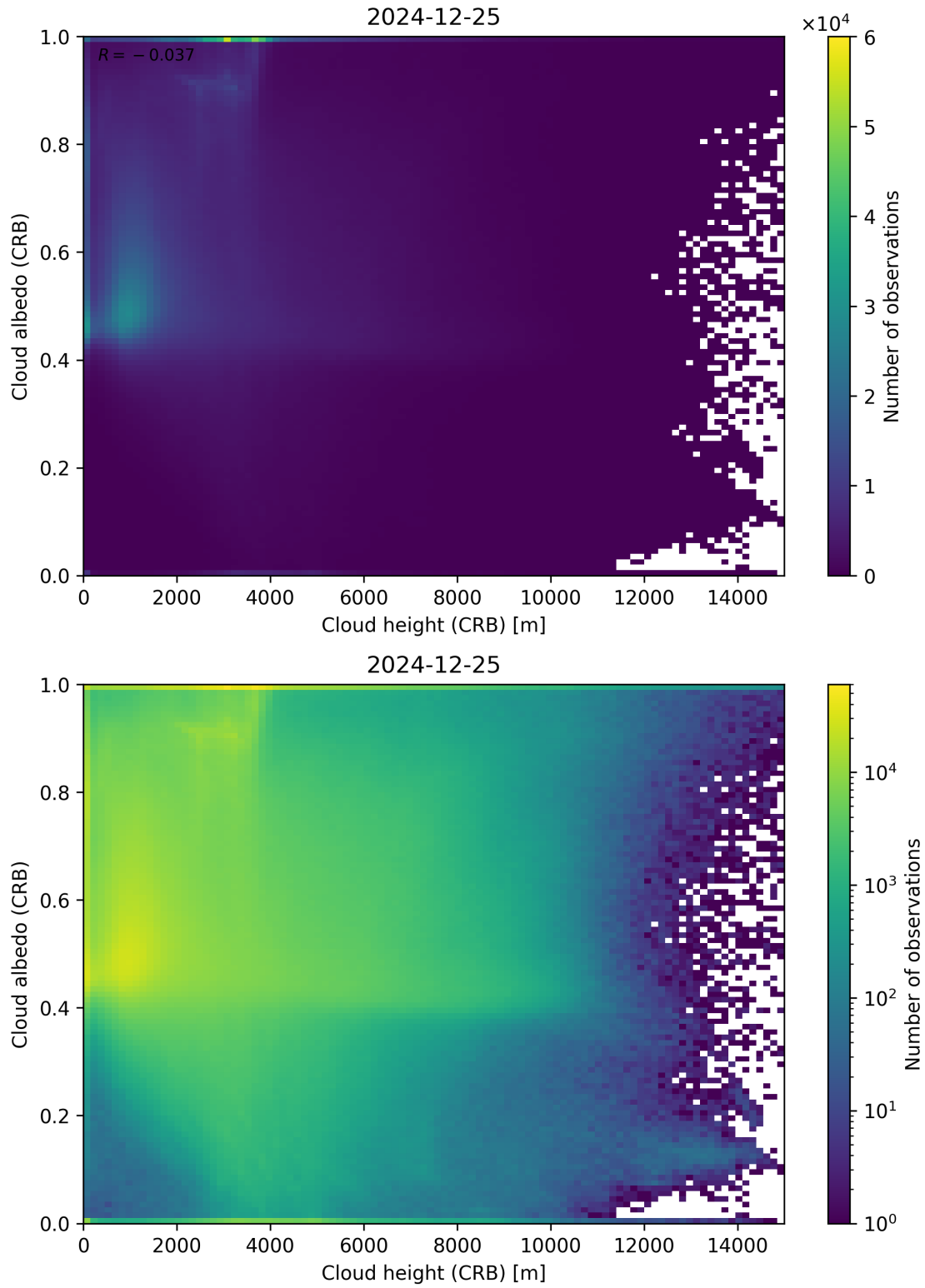
Figure 80: Scatter density plot of “Cloud height (CRB)” against “Cloud albedo (CRB)” for 2024-12-24 to 2024-12-26.
