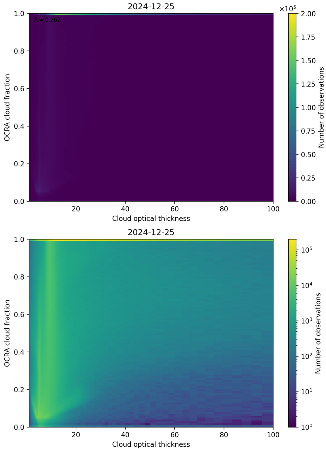
Figure 83: Scatter density plot of “Cloud optical thickness” against “OCRA cloud fraction” for 2024-12-24 to 2024-12-26.
