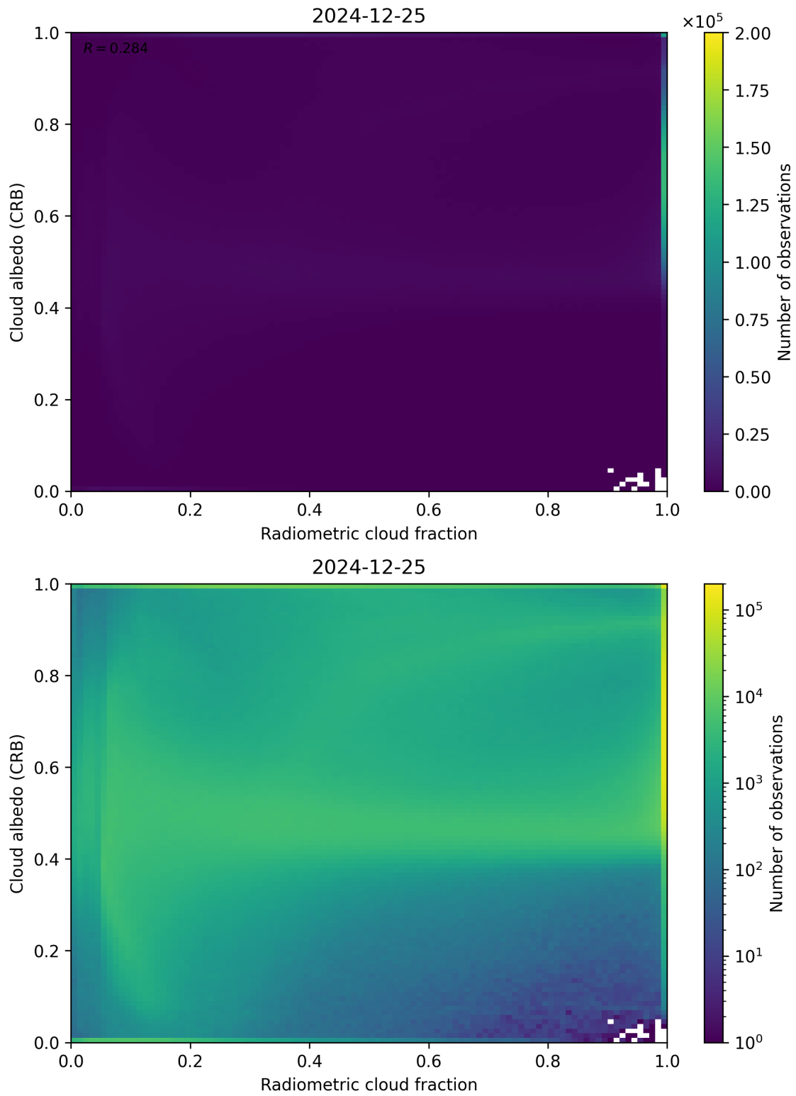
Figure 71: Scatter density plot of “Radiometric cloud fraction” against “Cloud albedo (CRB)” for 2024-12-24 to 2024-12-26.
