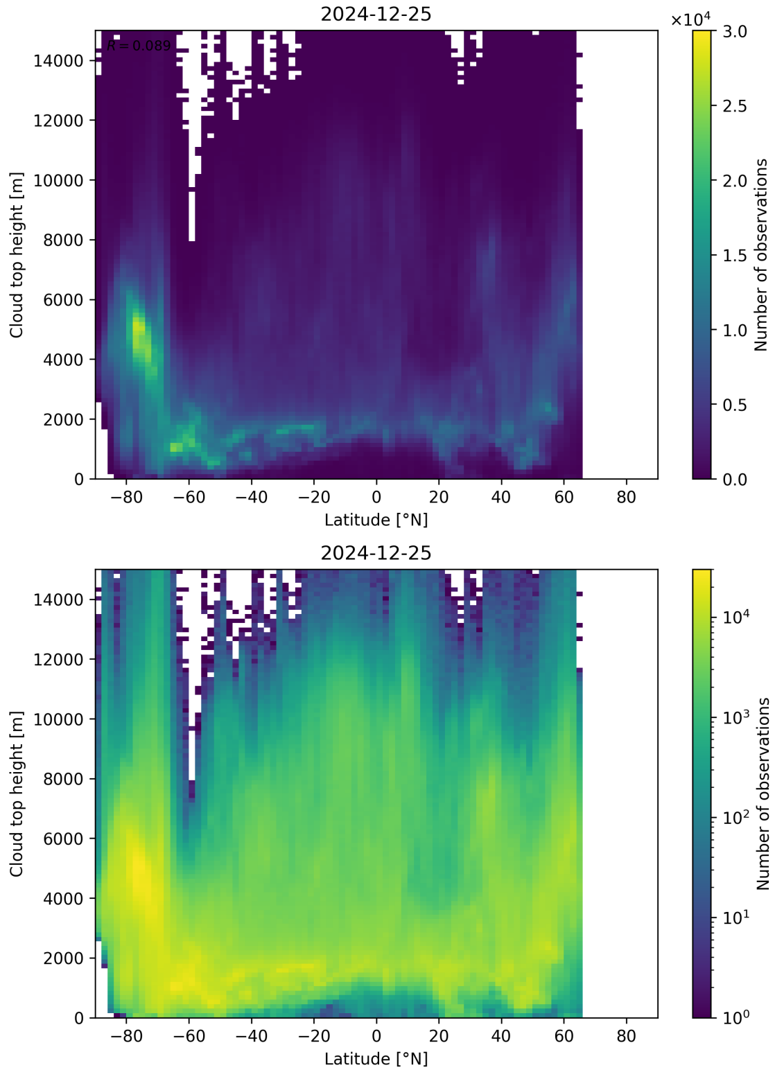
Figure 97: Scatter density plot of “Latitude” against “Cloud top height” for 2024-12-24 to 2024-12-26.
