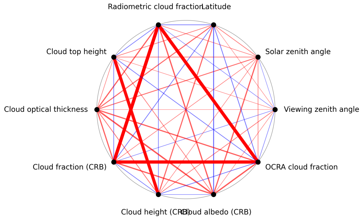
Figure 1: Map of correlation graph for 2024-12-24 to 2024-12-26.
