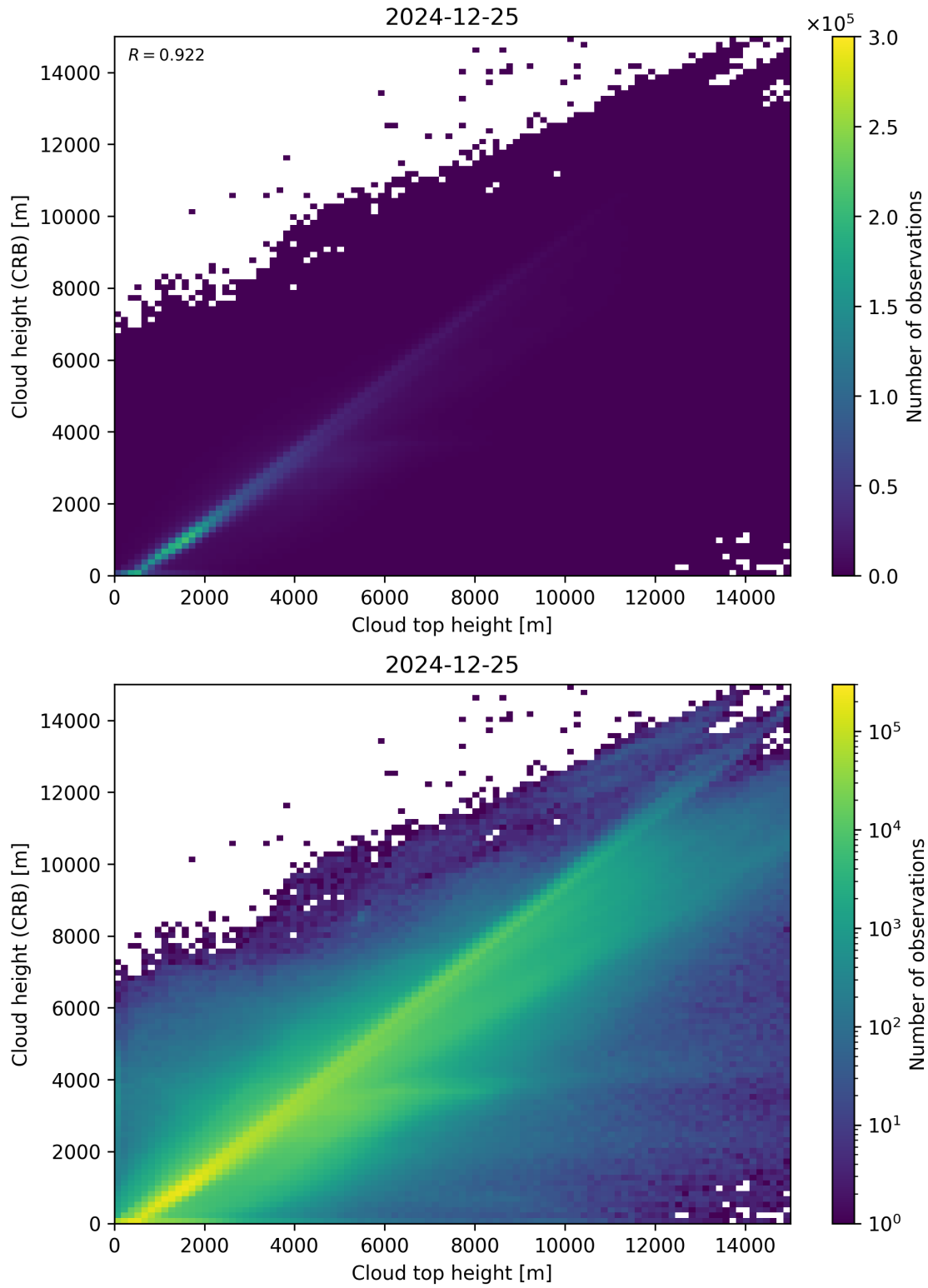
Figure 89: Scatter density plot of “Cloud top height” against “Cloud height (CRB)” for 2024-12-24 to 2024-12-26.
