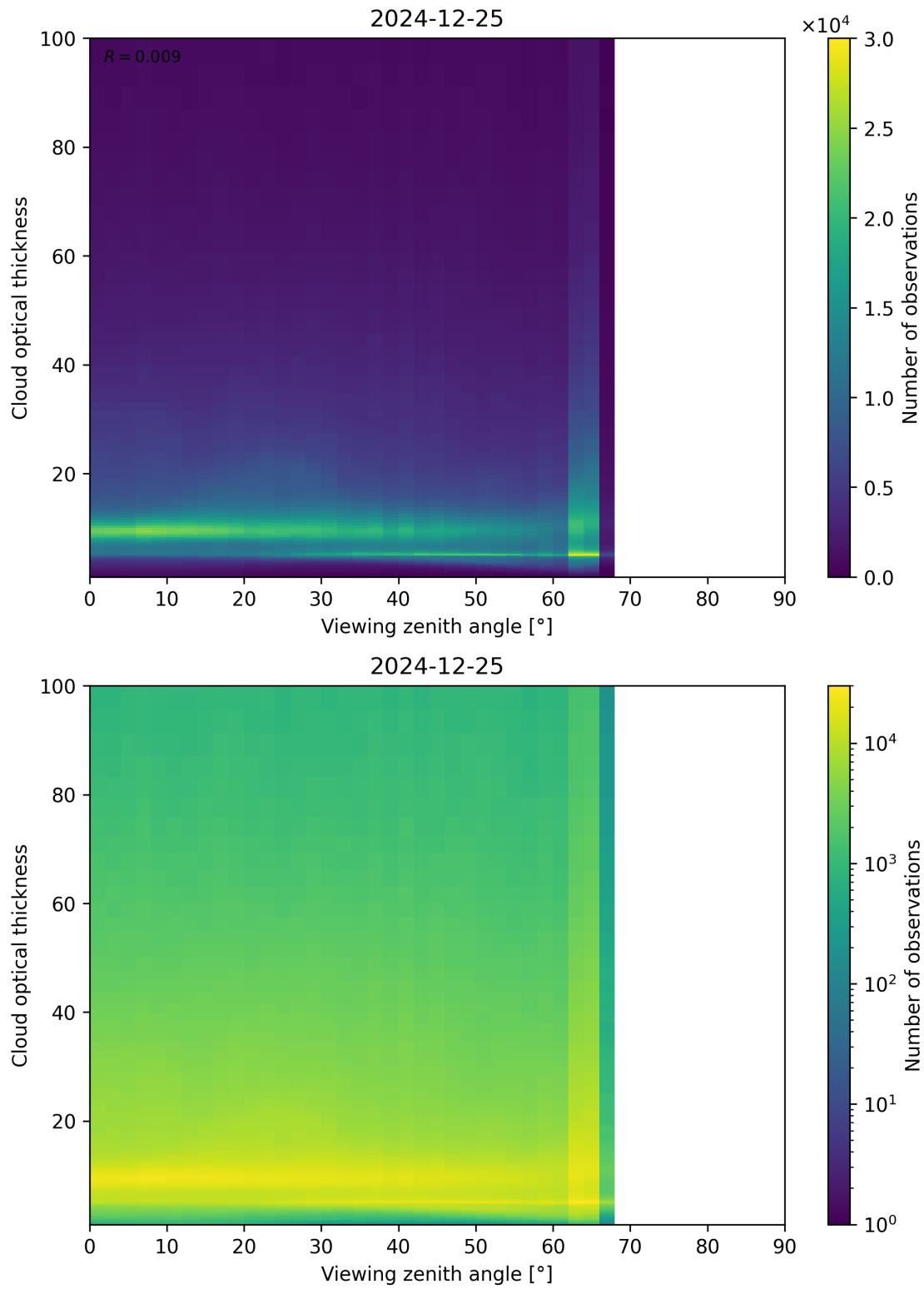
Figure 111: Scatter density plot of “Viewing zenith angle” against “Cloud optical thickness” for 2024-12-24 to 2024-12-26.
