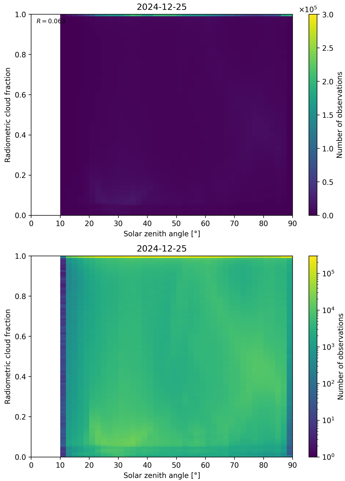
Figure 99: Scatter density plot of “Solar zenith angle” against “Radiometric cloud fraction” for 2024-12-24 to 2024-12-26.
