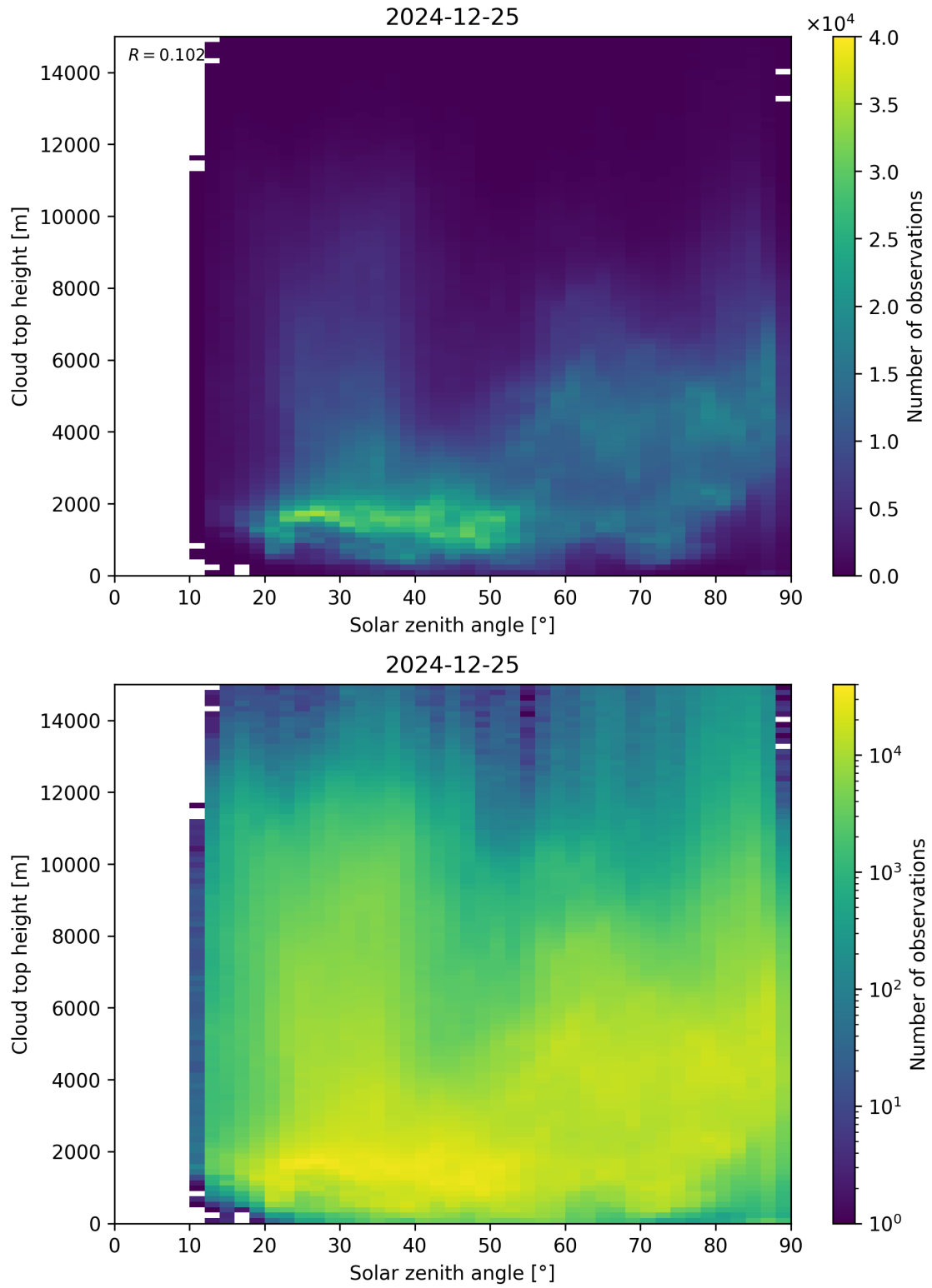
Figure 104: Scatter density plot of “Solar zenith angle” against “Cloud top height” for 2024-12-24 to 2024-12-26.
