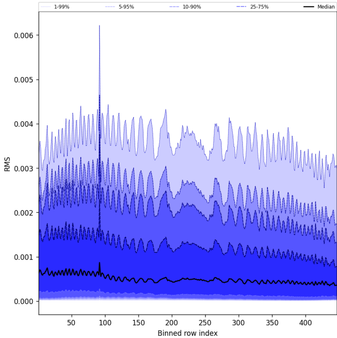
Figure 63: Along track statistics of “RMS” for 2024-12-24 to 2024-12-26
