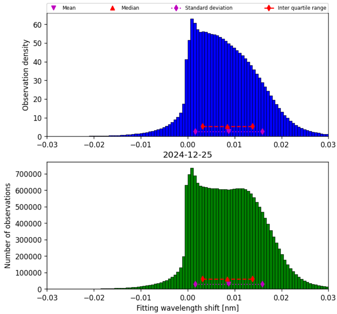
Figure 49: Histogram of “Fitting wavelength shift” for 2024-12-24 to 2024-12-26
