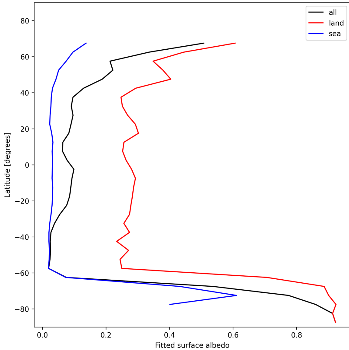
Figure 29: Zonal average of “Fitted surface albedo” for 2024-12-24 to 2024-12-26.
