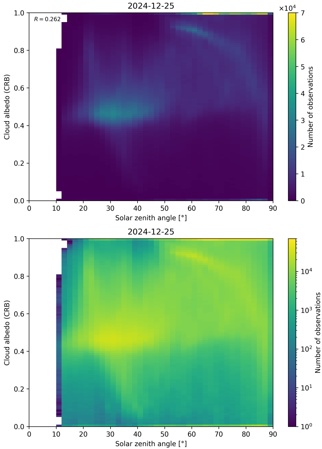
Figure 98: Scatter density plot of “Solar zenith angle” against “Cloud albedo (CRB)” for 2024-12-24 to 2024-12-26.
