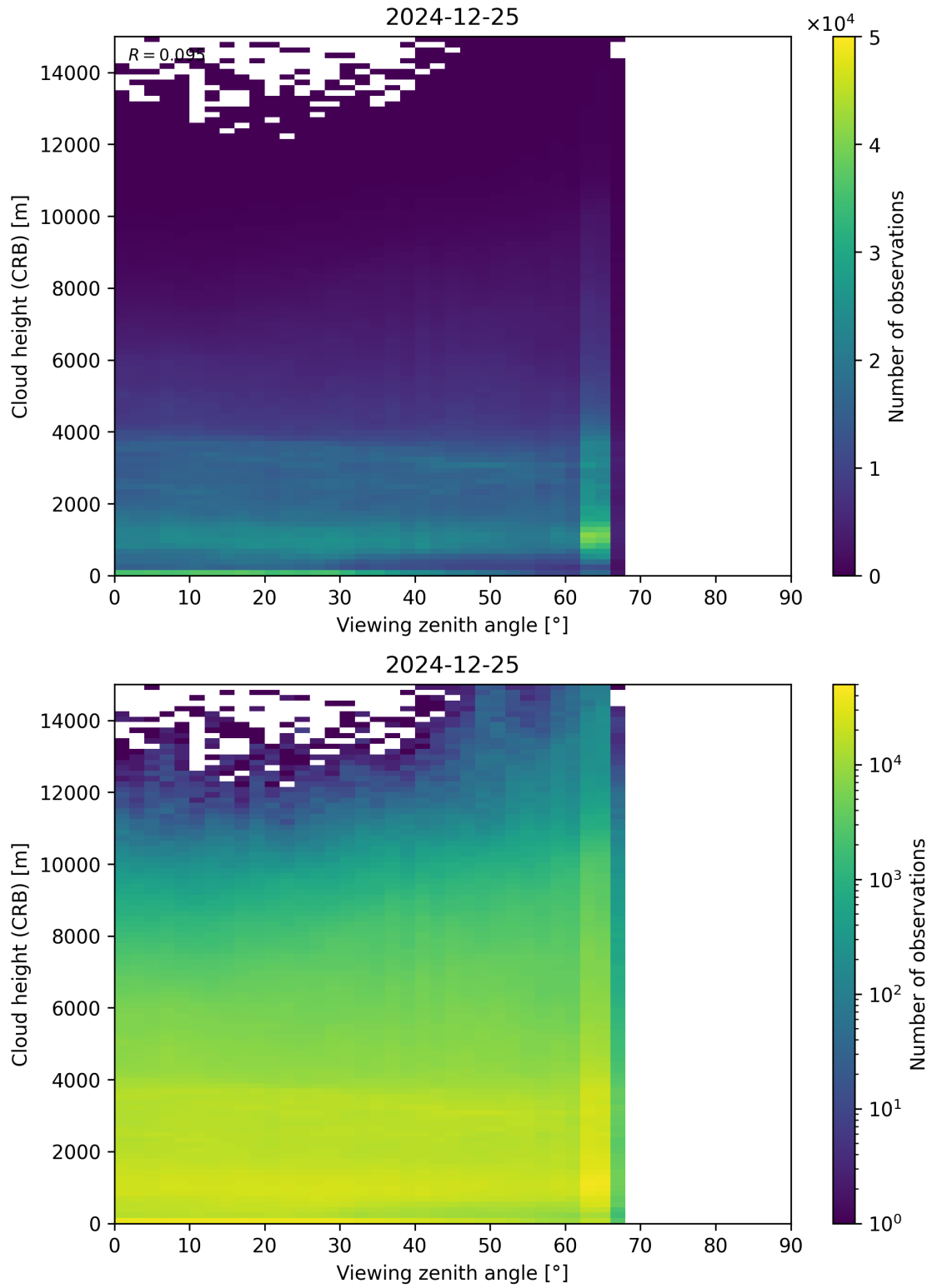
Figure 110: Scatter density plot of “Viewing zenith angle” against “Cloud height (CRB)” for 2024-12-24 to 2024-12-26.
