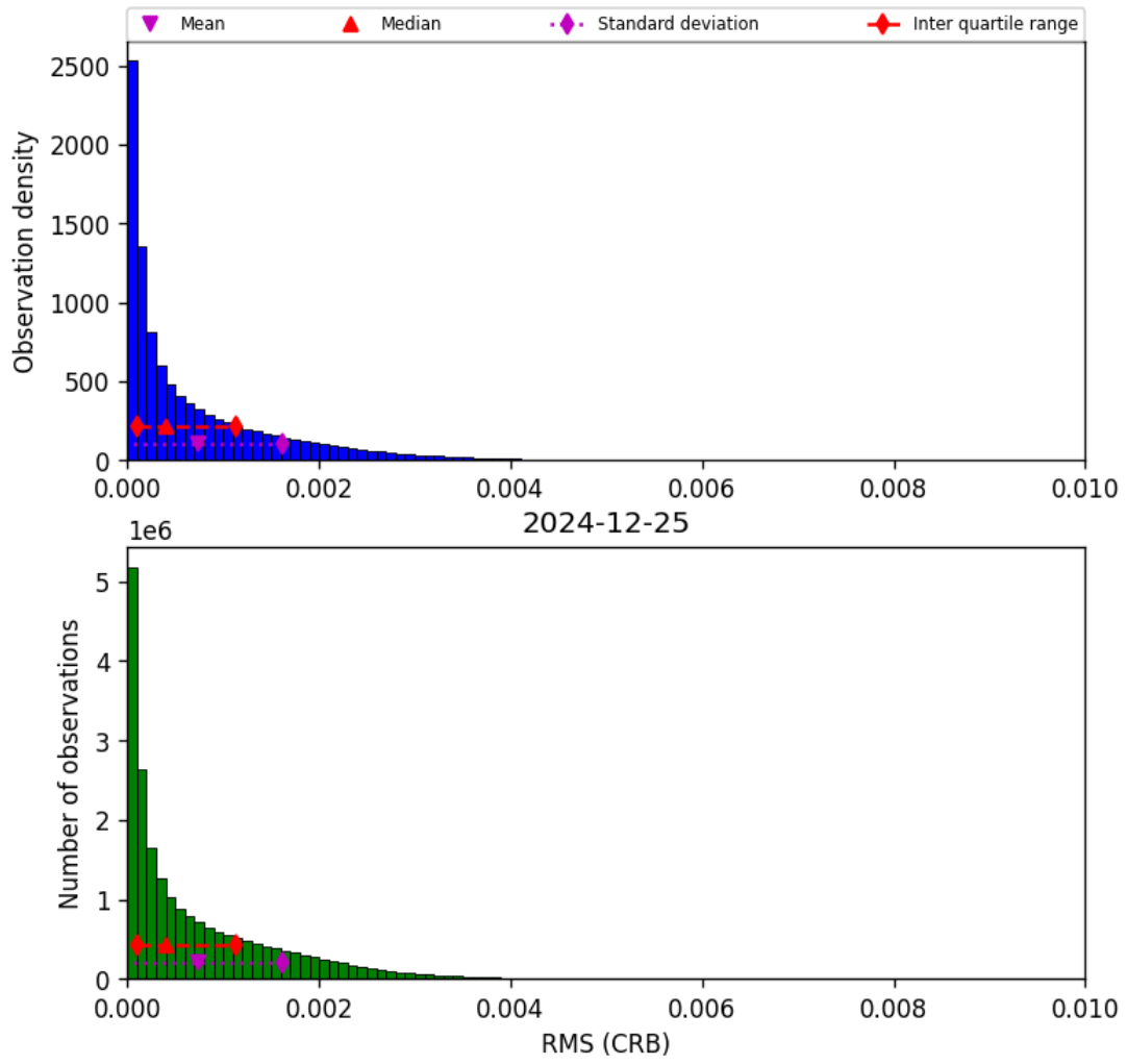
Figure 48: Histogram of “RMS (CRB)” for 2024-12-24 to 2024-12-26
