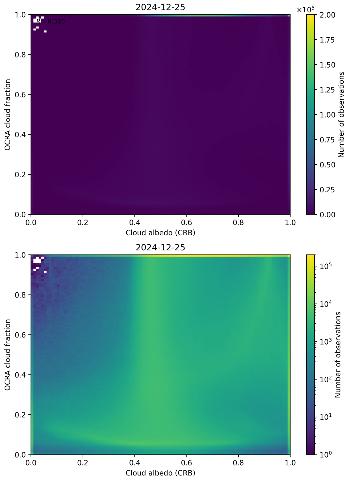
Figure 70: Scatter density plot of “Cloud albedo (CRB)” against “OCRA cloud fraction” for 2024-12-24 to 2024-12-26.
