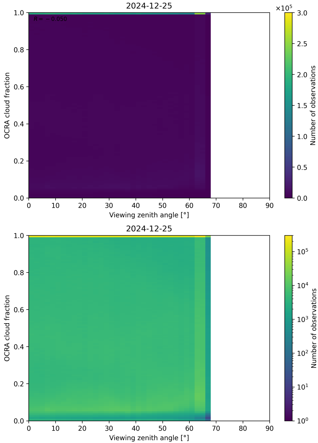
Figure 108: Scatter density plot of “Viewing zenith angle” against “OCRA cloud fraction” for 2024-12-24 to 2024-12-26.
