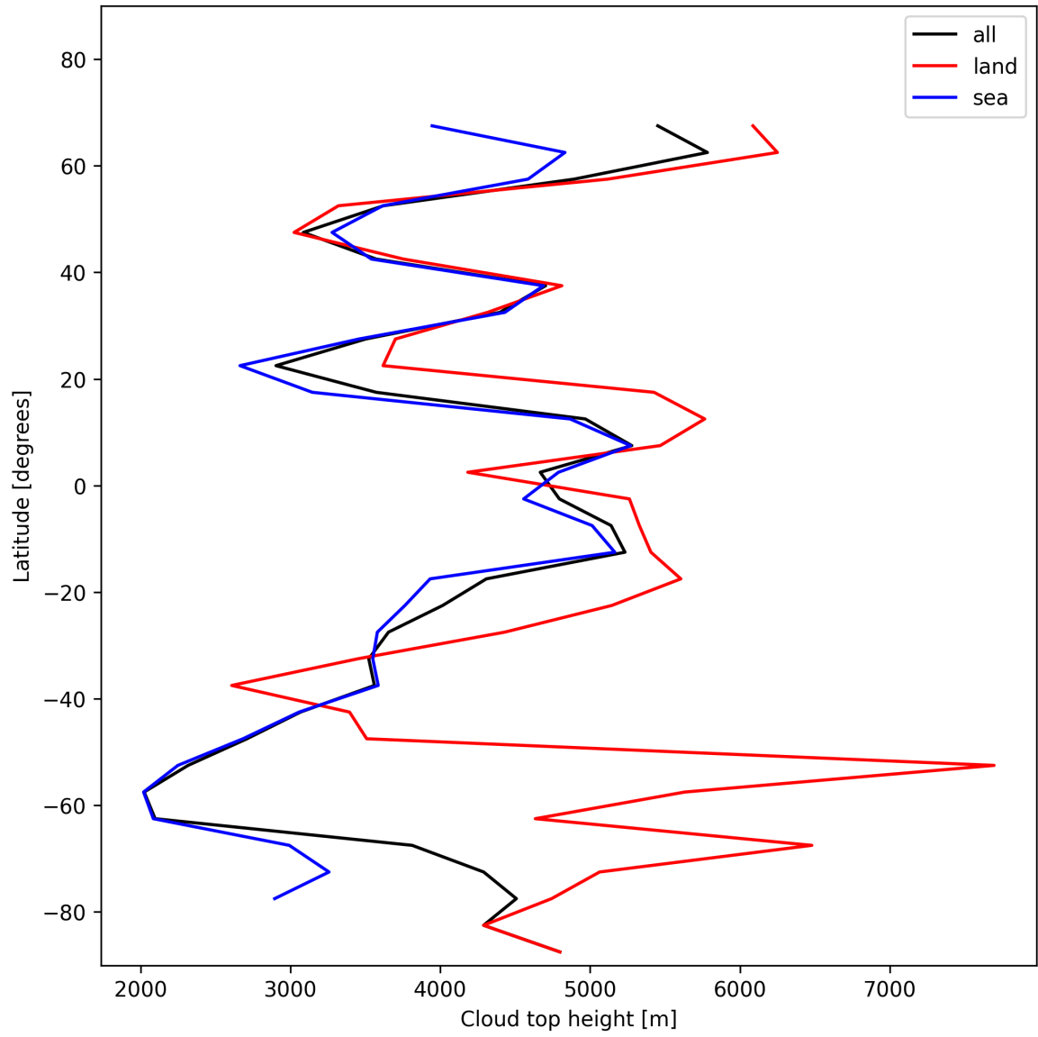
Figure 24: Zonal average of “Cloud top height” for 2024-12-24 to 2024-12-26.
