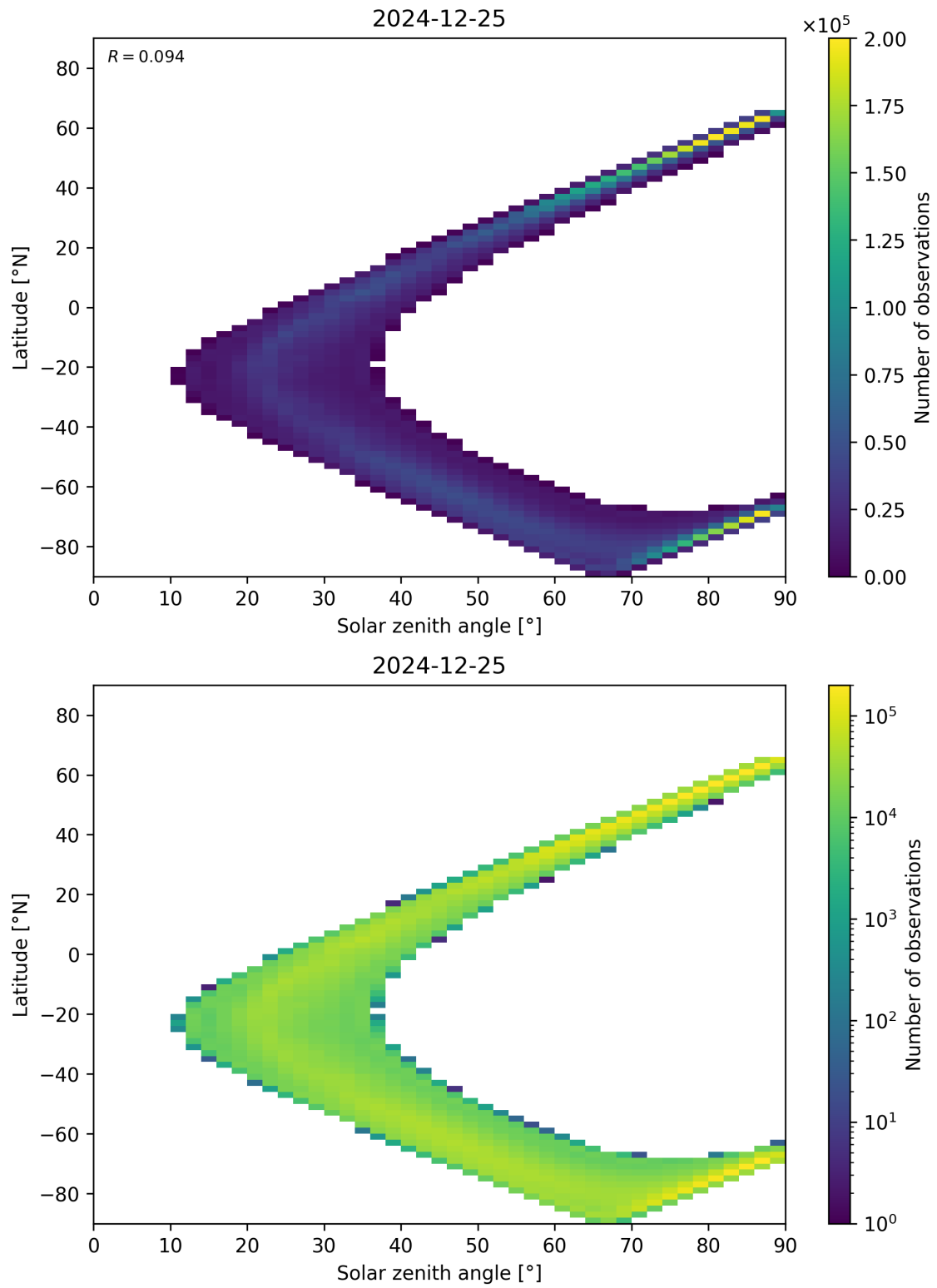
Figure 105: Scatter density plot of “Solar zenith angle” against “Latitude” for 2024-12-24 to 2024-12-26.
