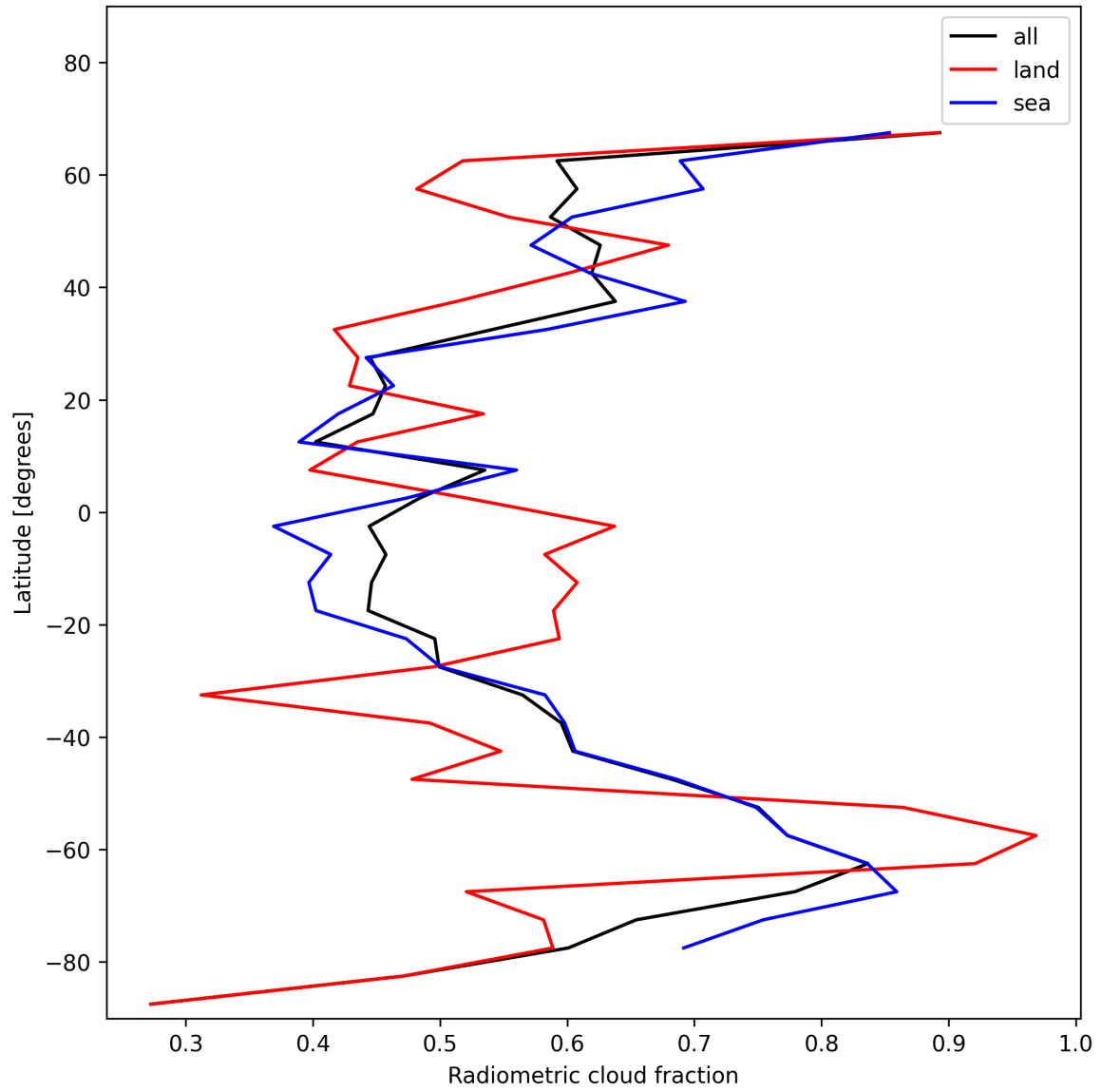
Figure 23: Zonal average of “Radiometric cloud fraction” for 2024-12-24 to 2024-12-26.
