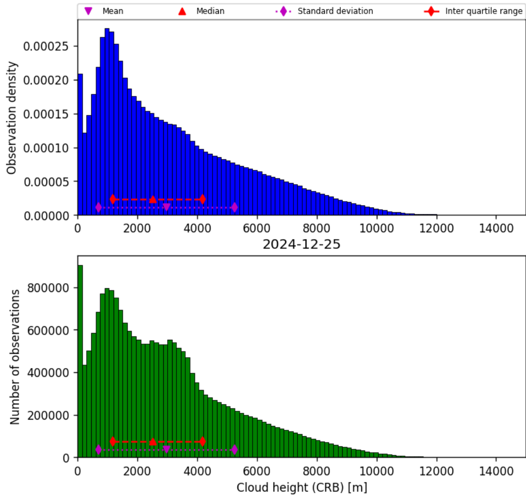
Figure 43: Histogram of “Cloud height (CRB)” for 2024-12-24 to 2024-12-26
