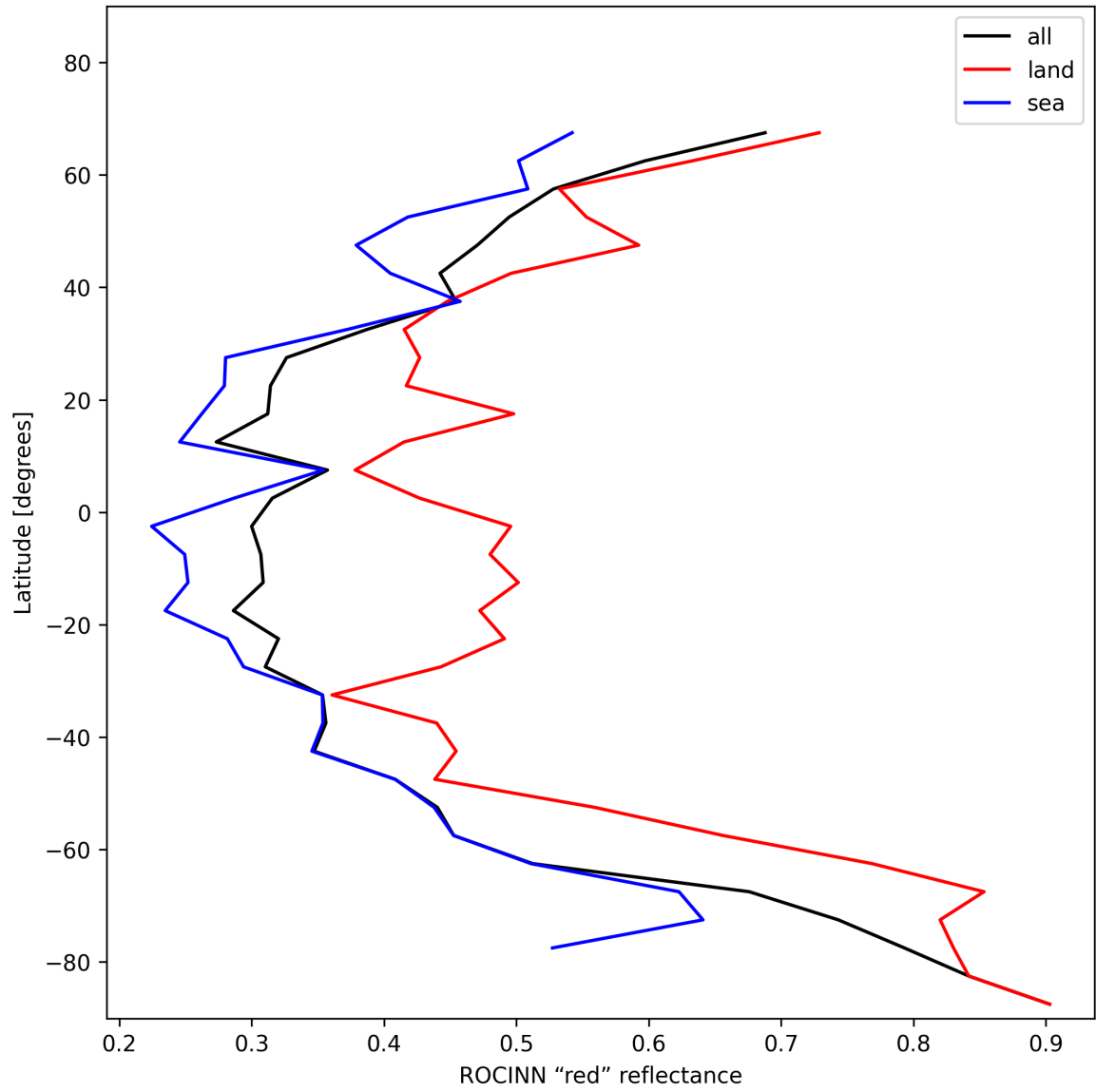
Figure 37: Zonal average of “ROCINN “red” reflectance” for 2024-12-24 to 2024-12-26.
