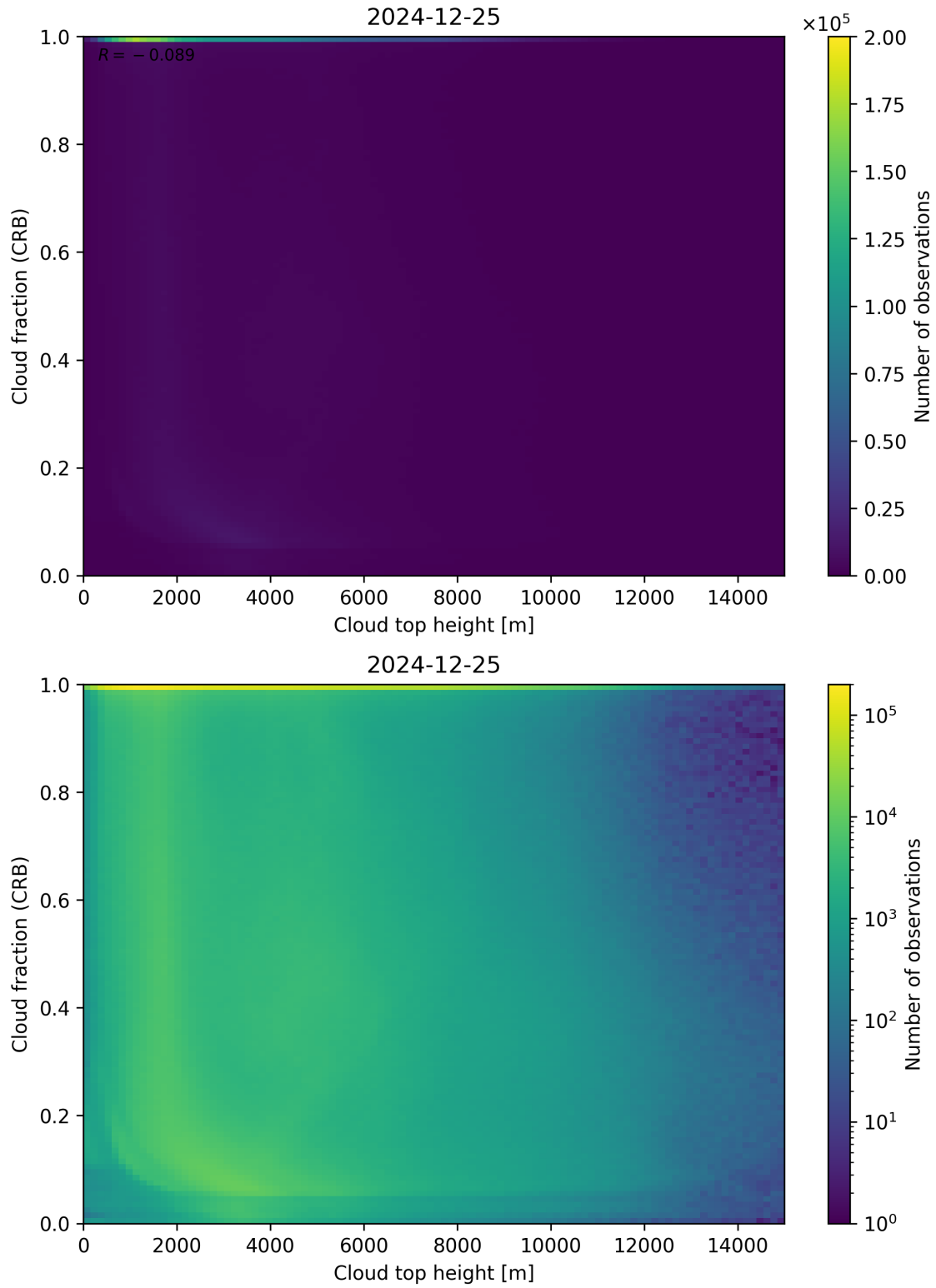
Figure 88: Scatter density plot of “Cloud top height” against “Cloud fraction (CRB)” for 2024-12-24 to 2024-12-26.
