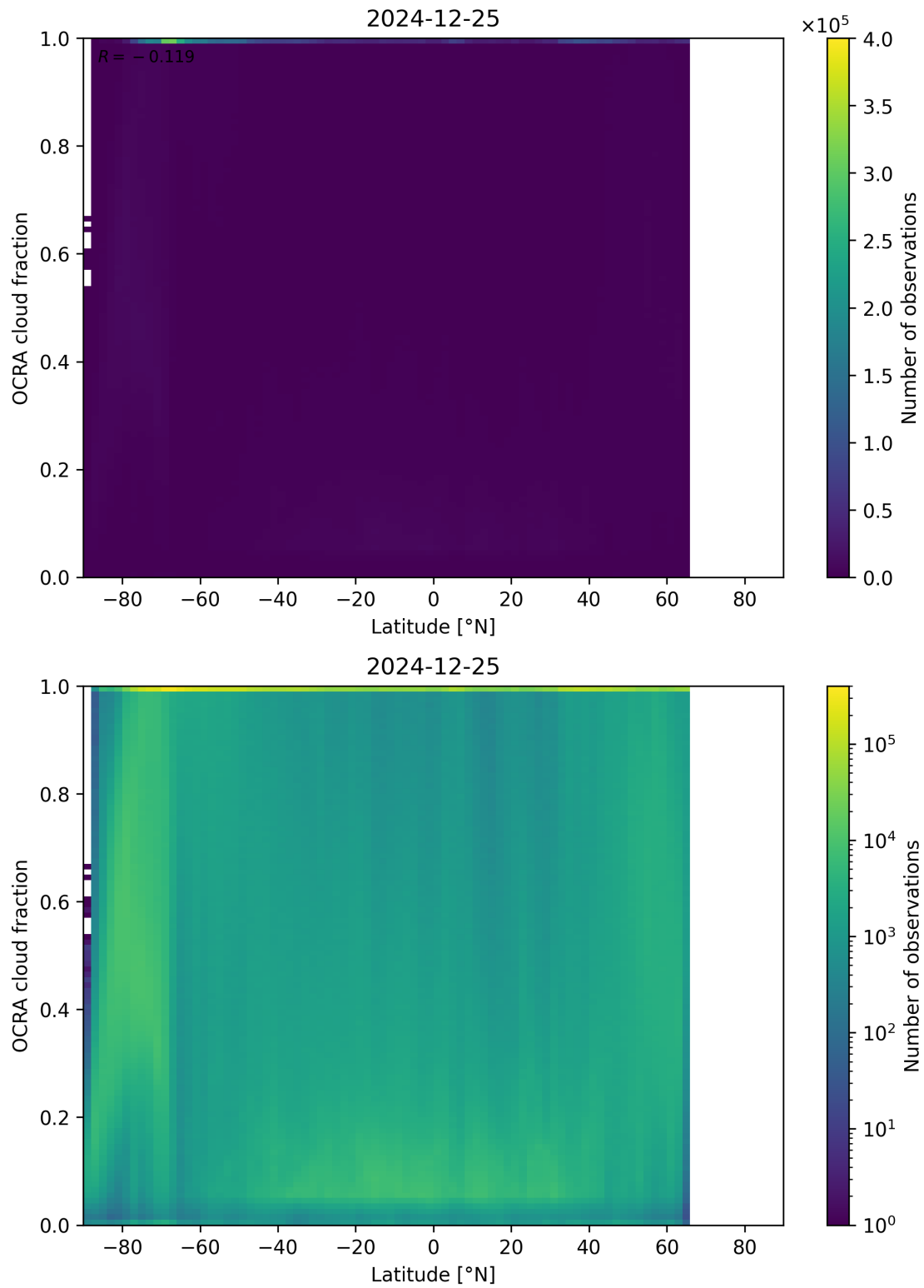
Figure 93: Scatter density plot of “Latitude” against “OCRA cloud fraction” for 2024-12-24 to 2024-12-26.
