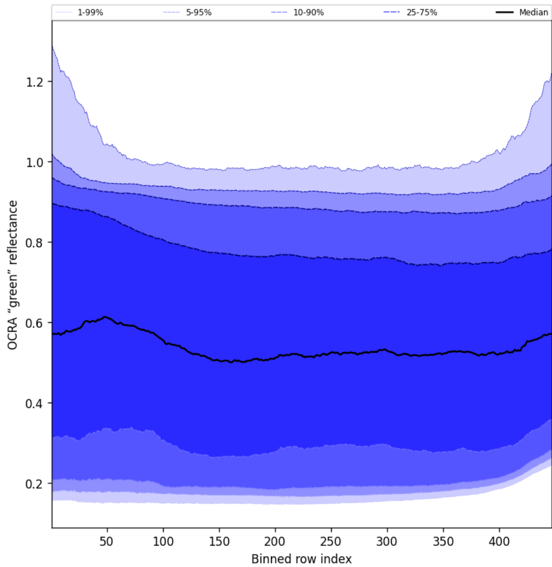
Figure 68: Along track statistics of “OCRA “green” reflectance” for 2024-12-24 to 2024-12-26
