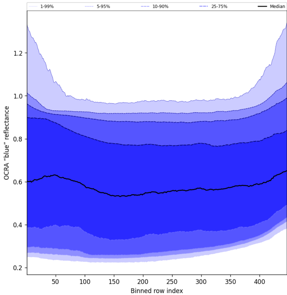
Figure 67: Along track statistics of “OCRA “blue” reflectance” for 2024-12-24 to 2024-12-26
