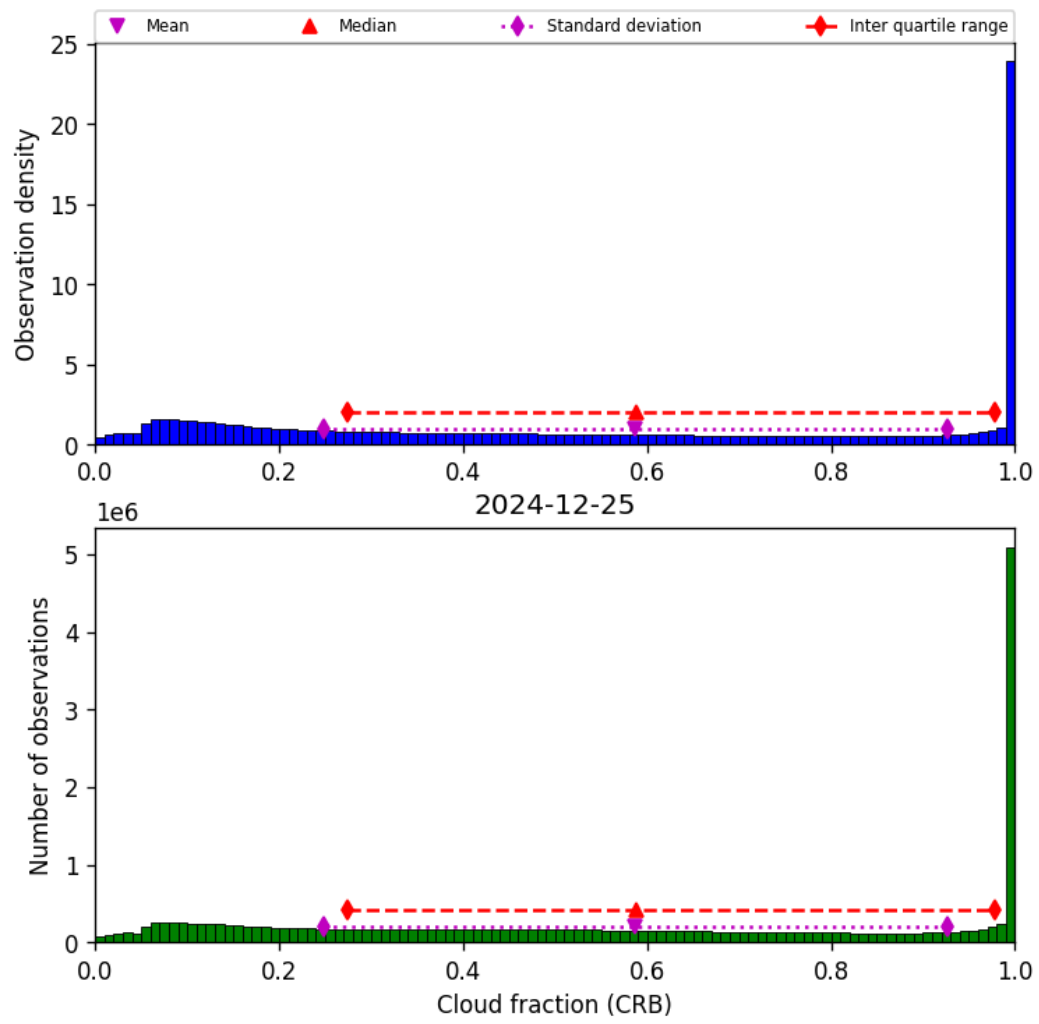
Figure 42: Histogram of “Cloud fraction (CRB)” for 2024-12-24 to 2024-12-26
