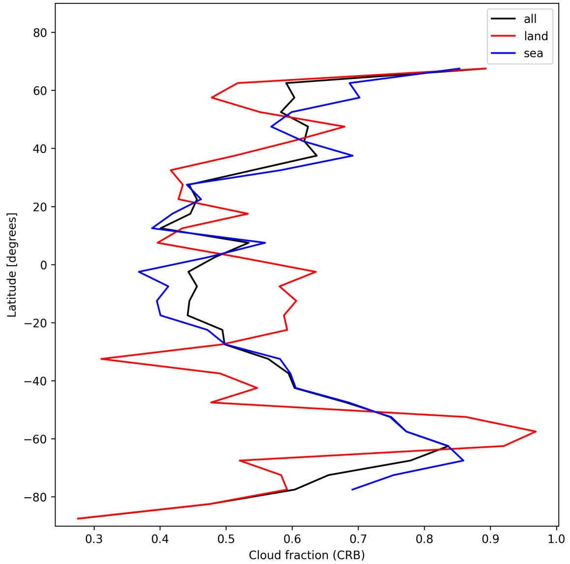
Figure 26: Zonal average of “Cloud fraction (CRB)” for 2024-12-24 to 2024-12-26.
