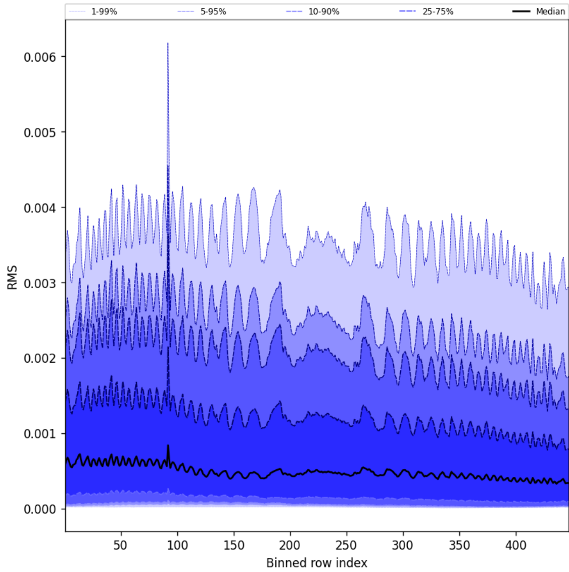
Figure 63: Along track statistics of “RMS” for 2024-12-25 to 2024-12-27
