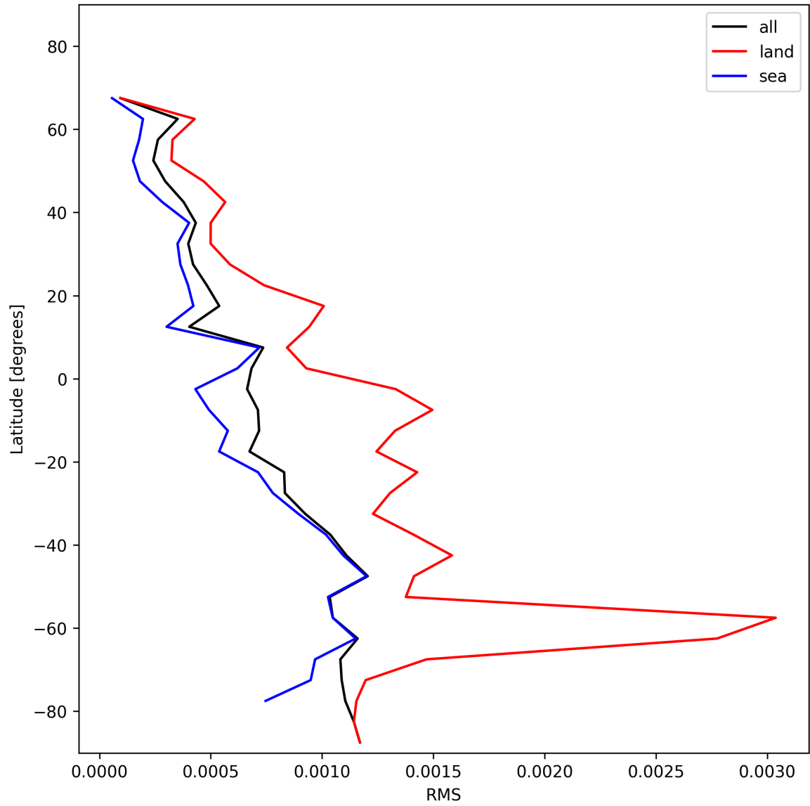
Figure 31: Zonal average of “RMS” for 2024-12-25 to 2024-12-27.
