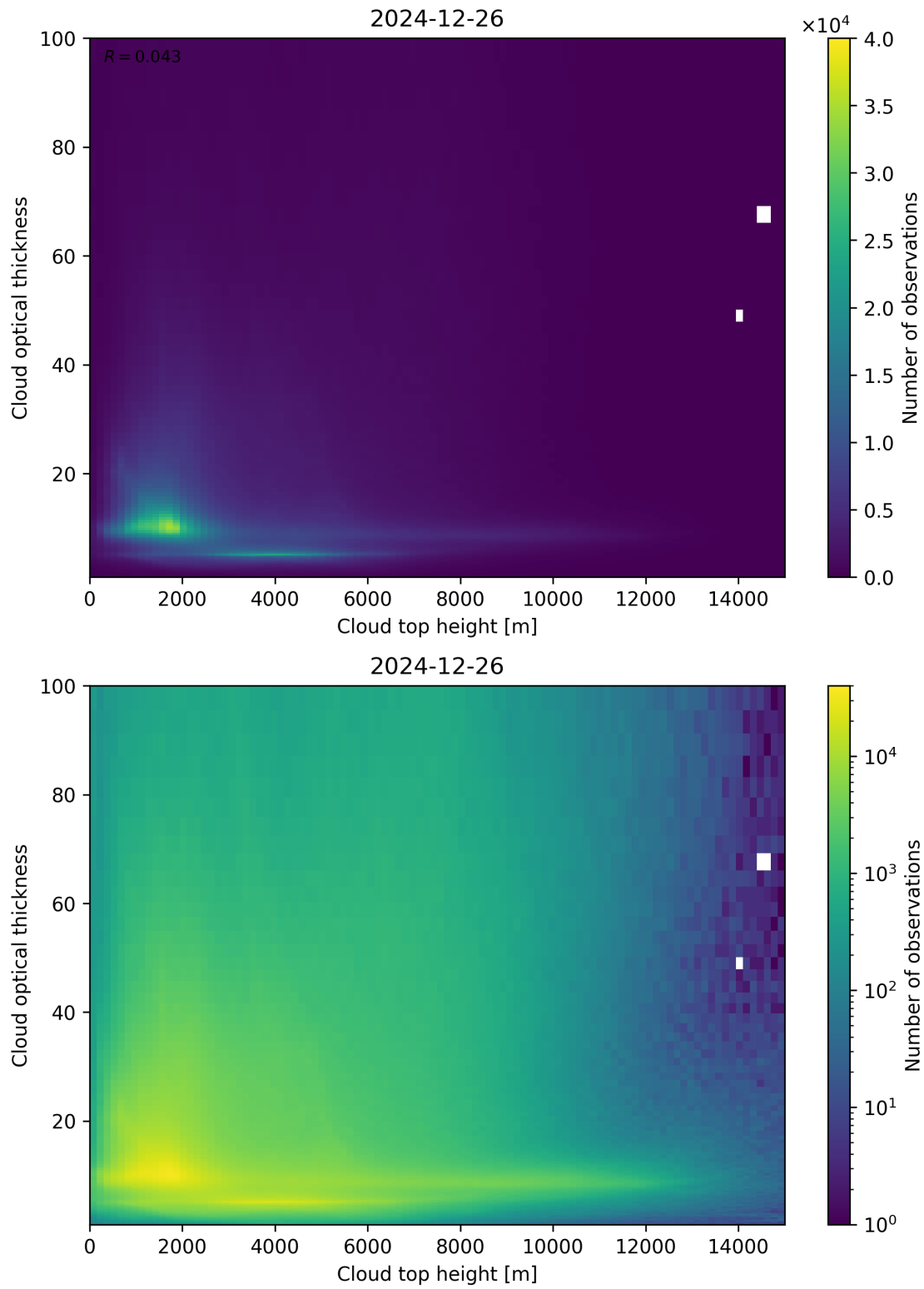
Figure 90: Scatter density plot of “Cloud top height” against “Cloud optical thickness” for 2024-12-25 to 2024-12-27.
