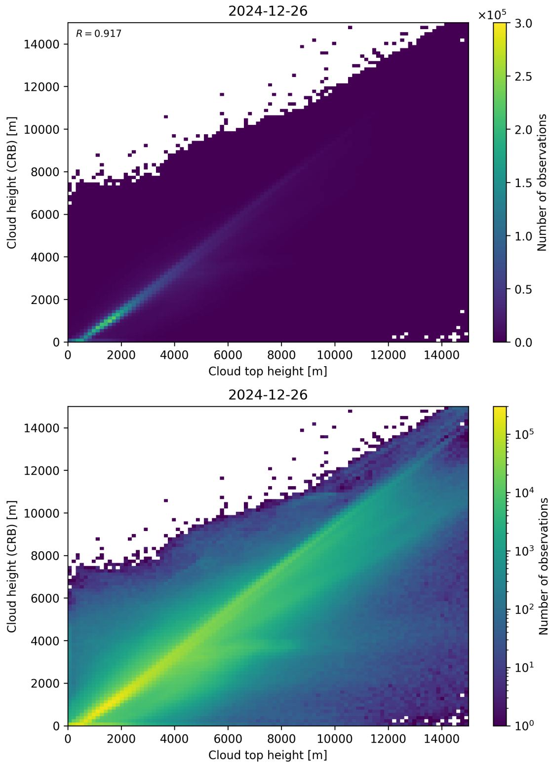
Figure 89: Scatter density plot of “Cloud top height” against “Cloud height (CRB)” for 2024-12-25 to 2024-12-27.
