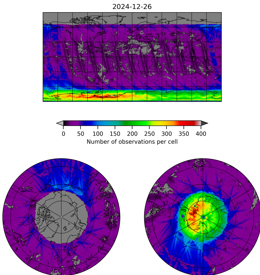
Figure 21: Map of the number of observations for 2024-12-25 to 2024-12-27
