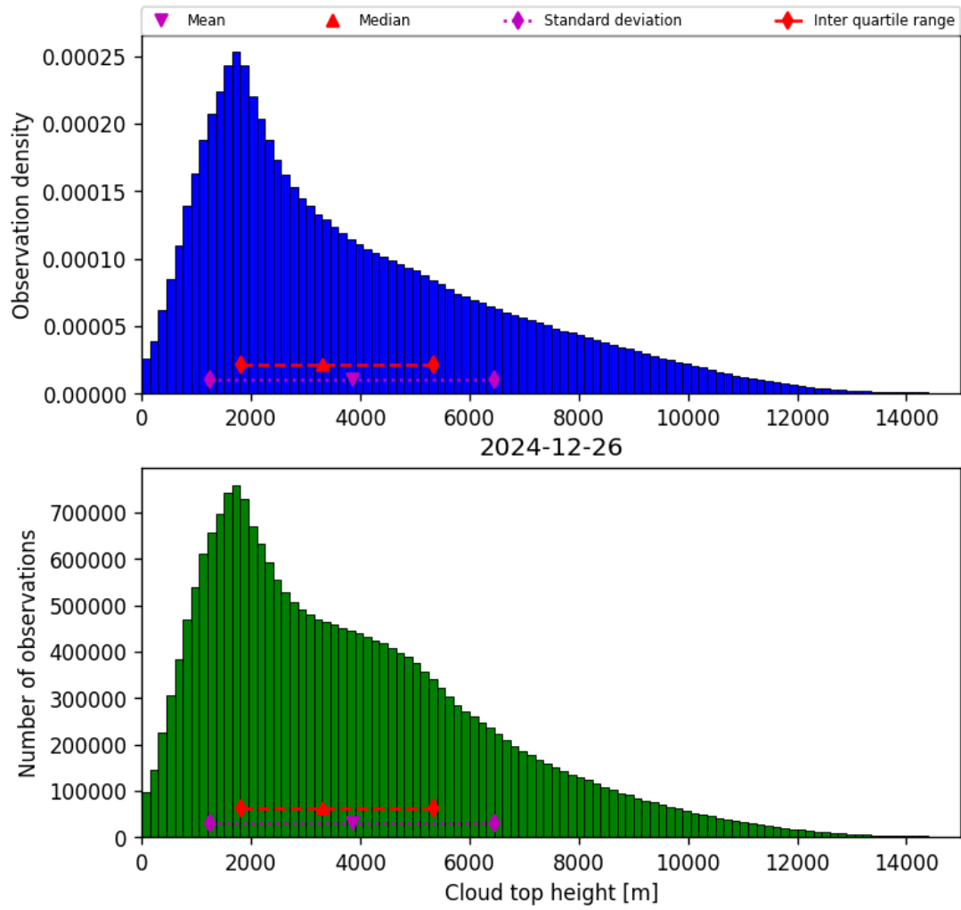
Figure 40: Histogram of “Cloud top height” for 2024-12-25 to 2024-12-27
