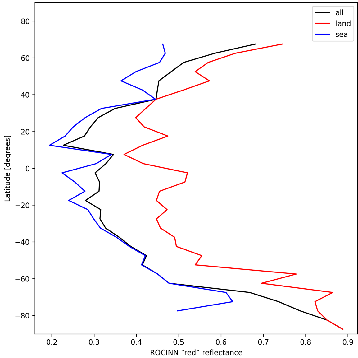
Figure 37: Zonal average of “ROCINN “red” reflectance” for 2024-12-25 to 2024-12-27.
