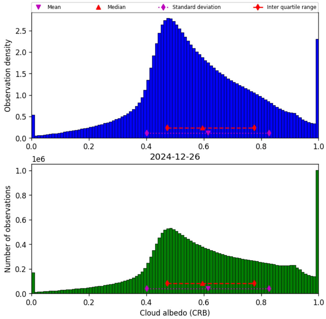
Figure 44: Histogram of “Cloud albedo (CRB)” for 2024-12-25 to 2024-12-27
