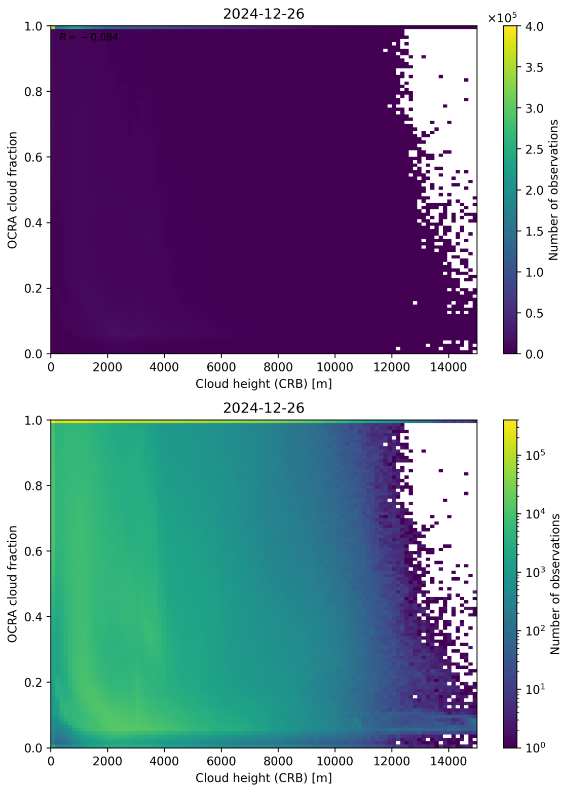
Figure 81: Scatter density plot of “Cloud height (CRB)” against “OCRA cloud fraction” for 2024-12-25 to 2024-12-27.
