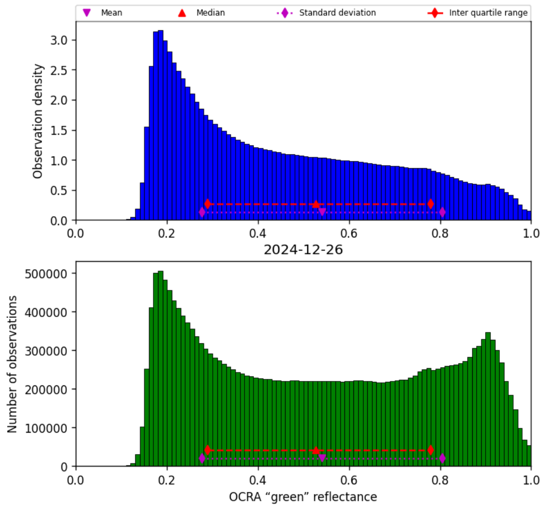
Figure 52: Histogram of “OCRA “green” reflectance” for 2024-12-25 to 2024-12-27
