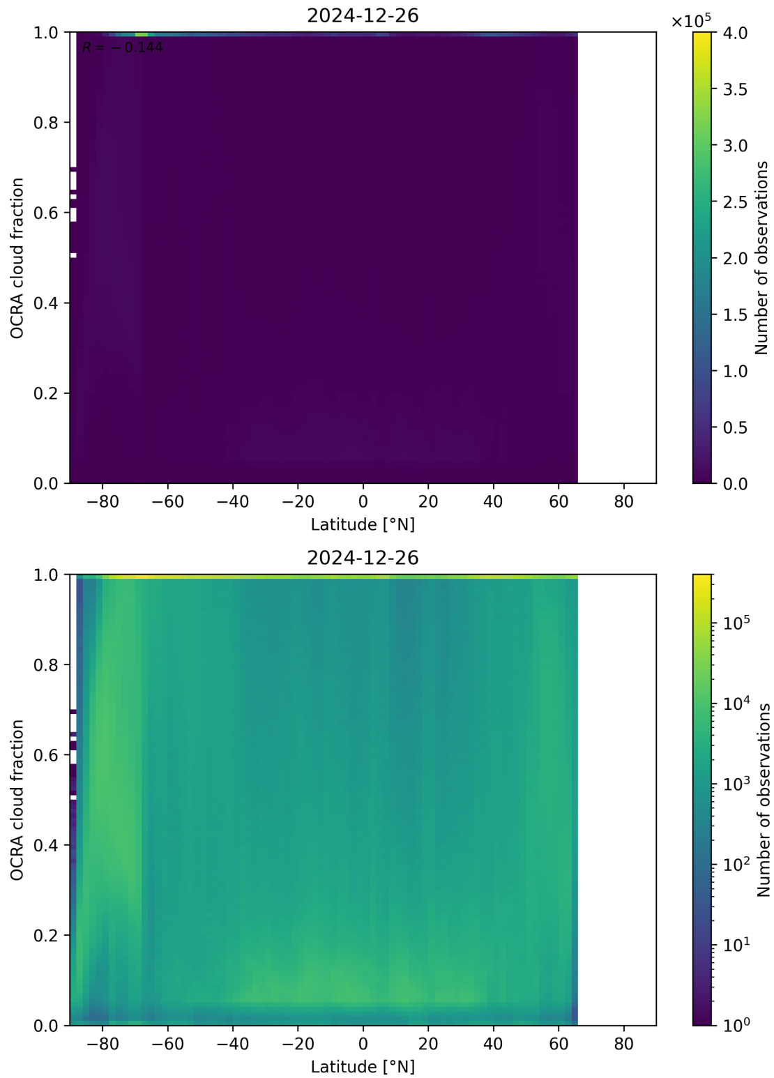
Figure 93: Scatter density plot of “Latitude” against “OCRA cloud fraction” for 2024-12-25 to 2024-12-27.
