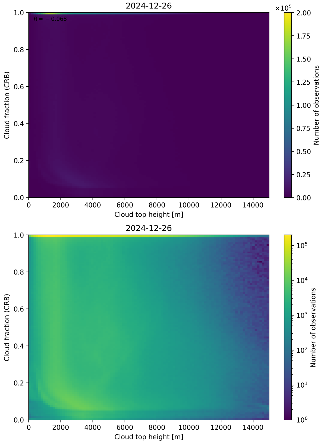
Figure 88: Scatter density plot of “Cloud top height” against “Cloud fraction (CRB)” for 2024-12-25 to 2024-12-27.
