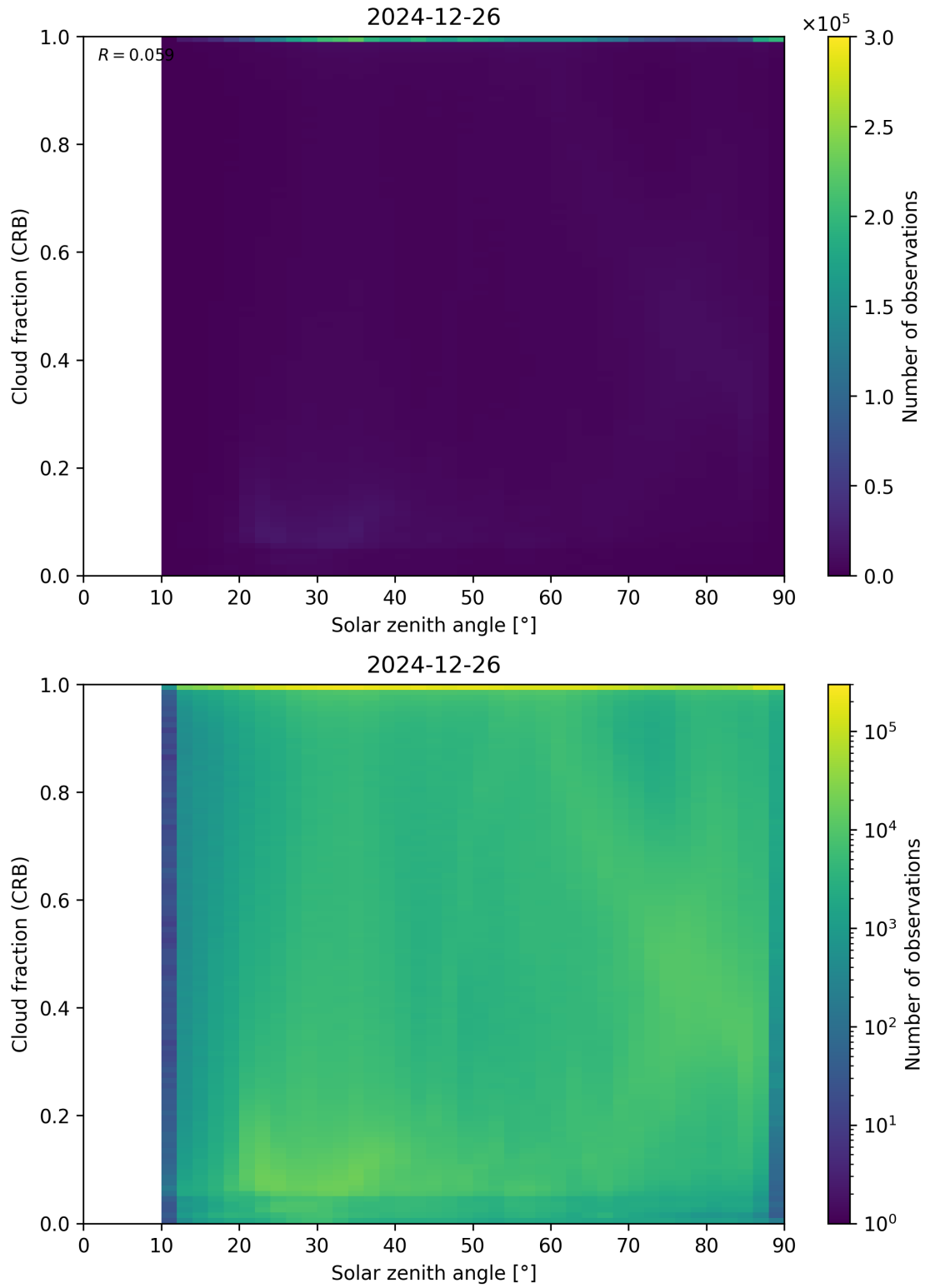
Figure 101: Scatter density plot of “Solar zenith angle” against “Cloud fraction (CRB)” for 2024-12-25 to 2024-12-27.
