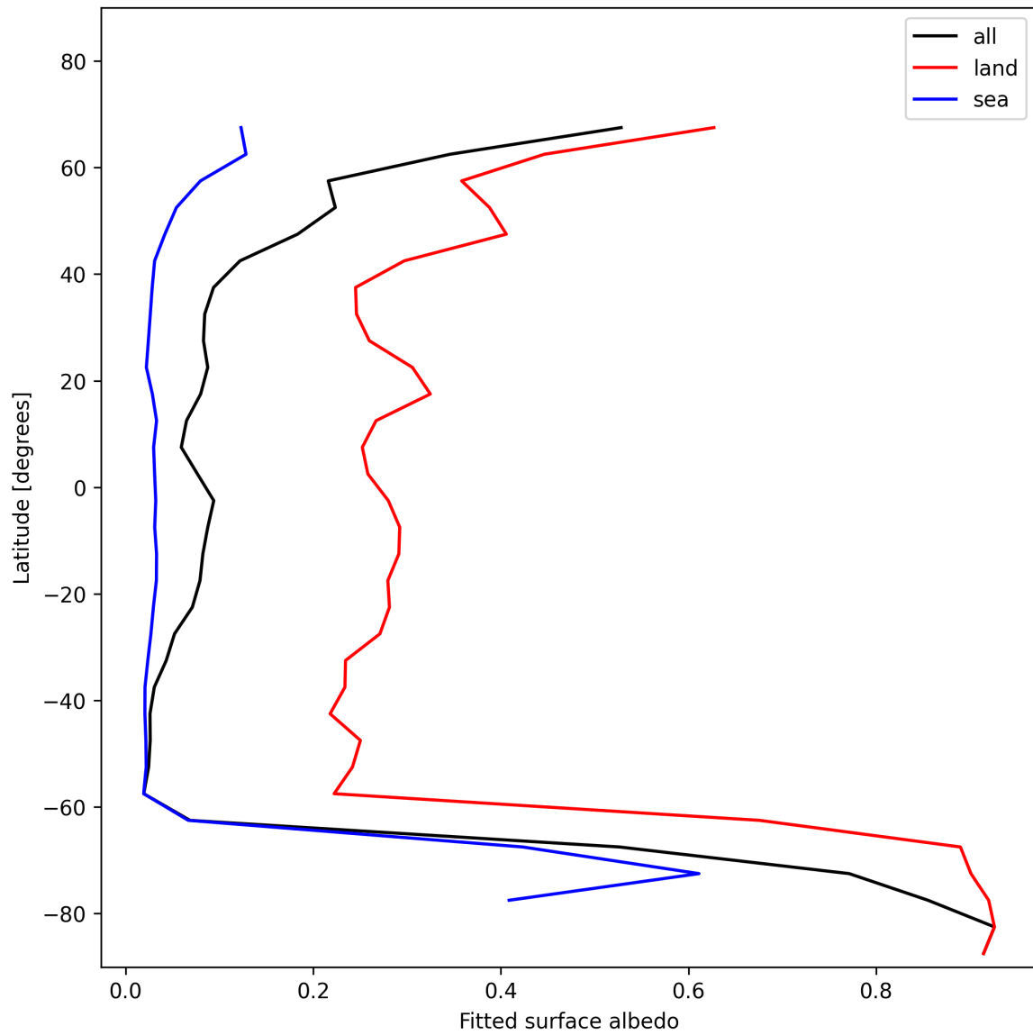
Figure 29: Zonal average of “Fitted surface albedo” for 2024-12-25 to 2024-12-27.
