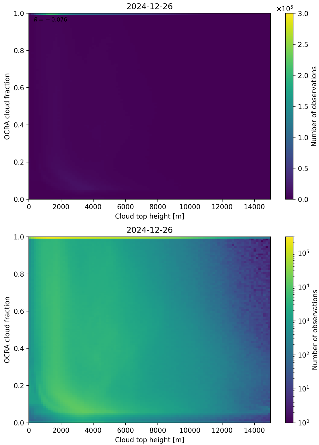
Figure 87: Scatter density plot of “Cloud top height” against “OCRA cloud fraction” for 2024-12-25 to 2024-12-27.
