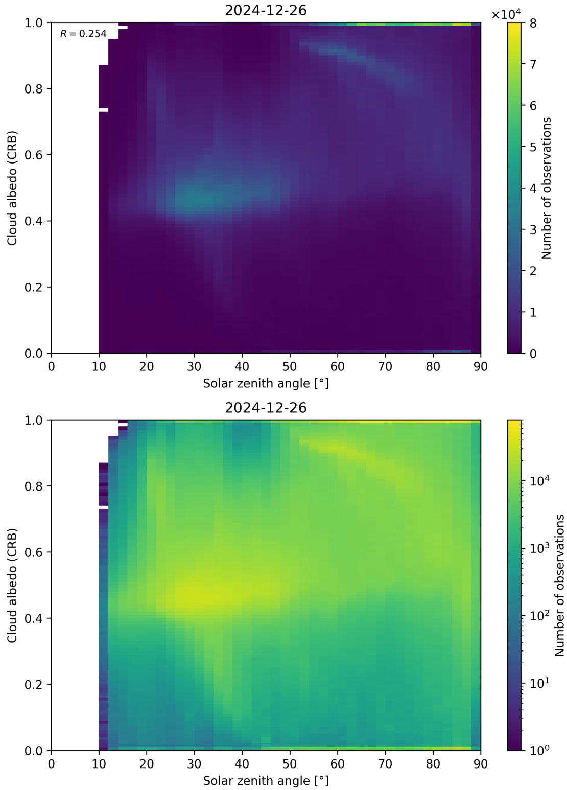
Figure 98: Scatter density plot of “Solar zenith angle” against “Cloud albedo (CRB)” for 2024-12-25 to 2024-12-27.
