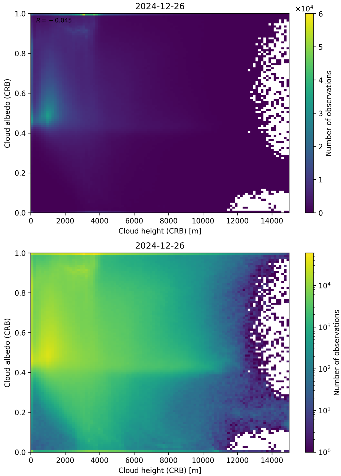
Figure 80: Scatter density plot of “Cloud height (CRB)” against “Cloud albedo (CRB)” for 2024-12-25 to 2024-12-27.
