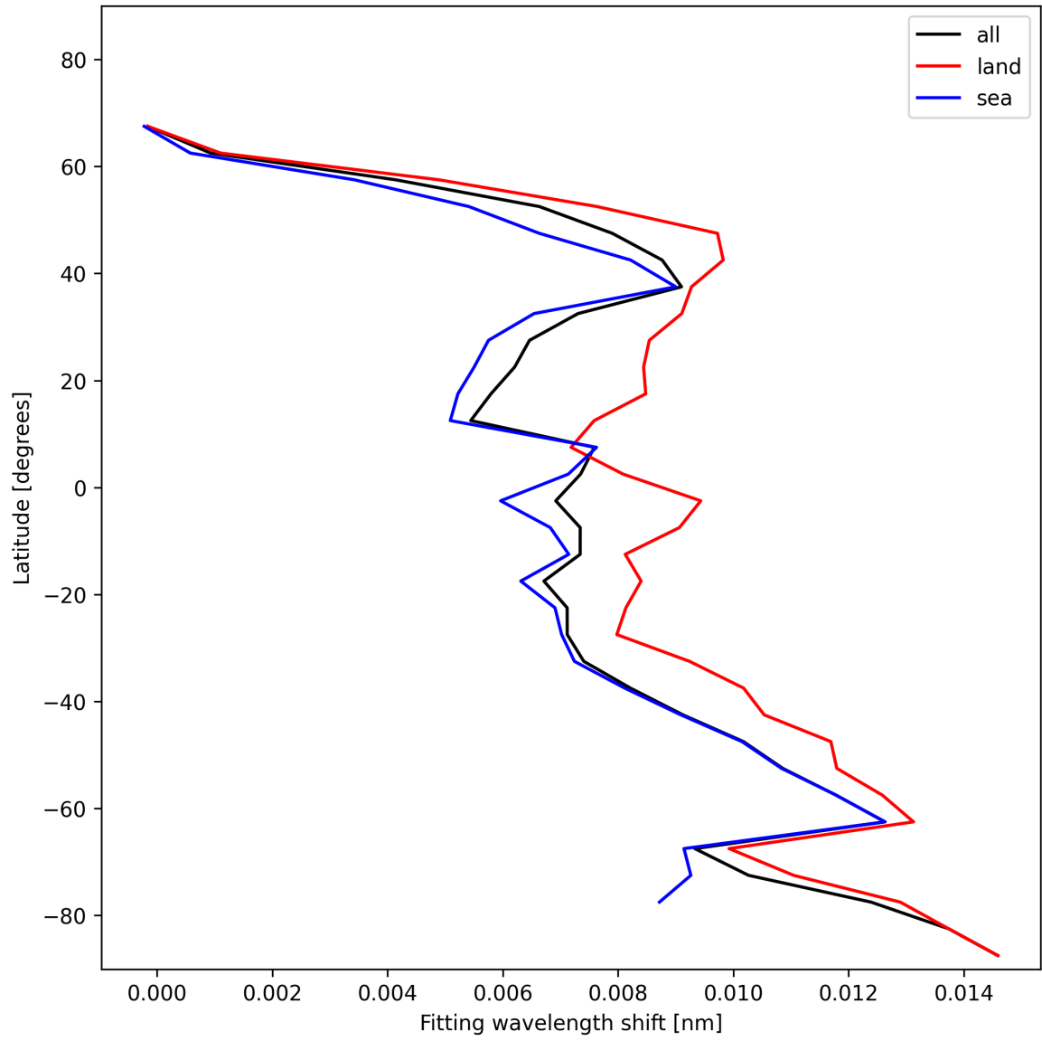
Figure 33: Zonal average of “Fitting wavelength shift” for 2024-12-25 to 2024-12-27.
