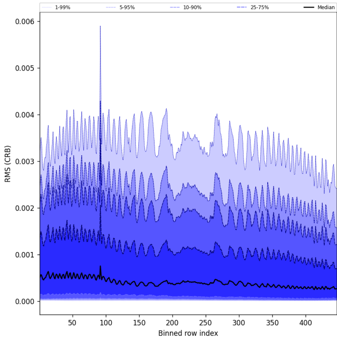
Figure 64: Along track statistics of “RMS (CRB)” for 2024-12-25 to 2024-12-27
