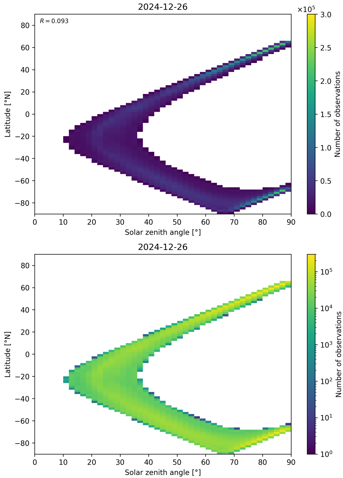
Figure 105: Scatter density plot of “Solar zenith angle” against “Latitude” for 2024-12-25 to 2024-12-27.
