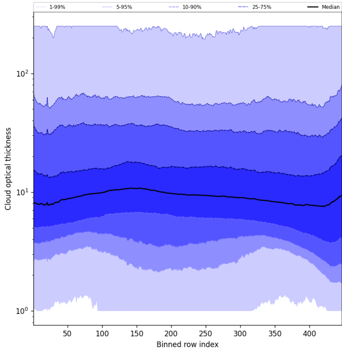
Figure 57: Along track statistics of “Cloud optical thickness” for 2024-12-25 to 2024-12-27
