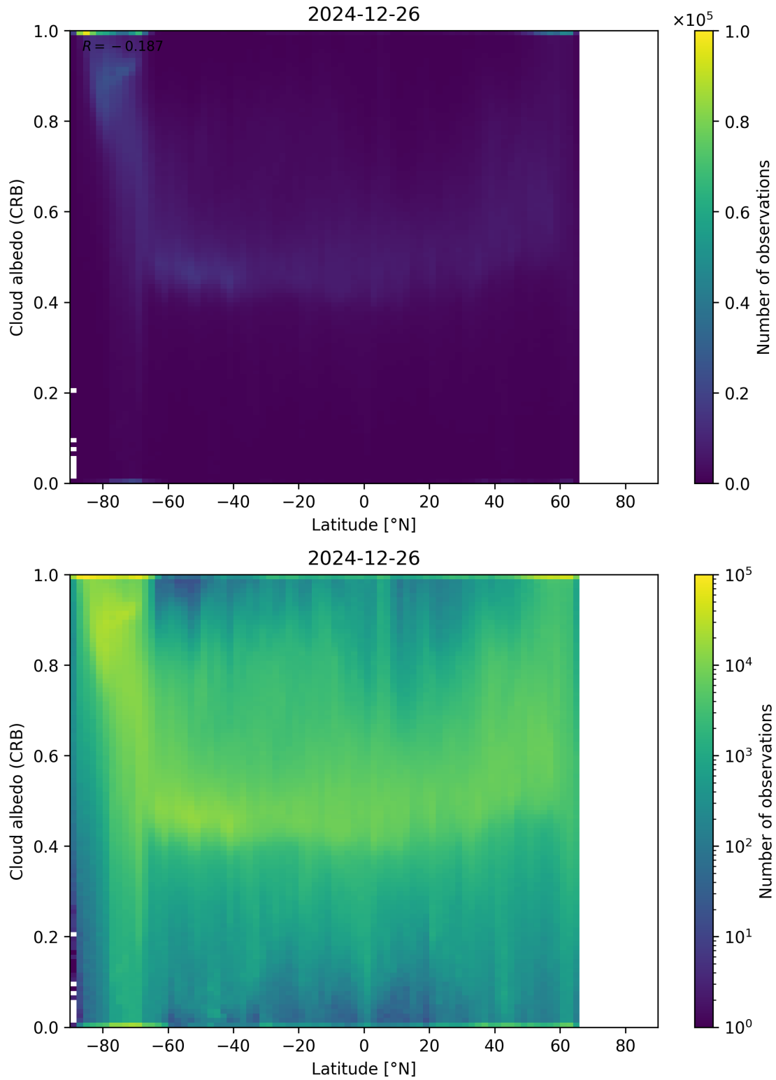
Figure 91: Scatter density plot of “Latitude” against “Cloud albedo (CRB)” for 2024-12-25 to 2024-12-27.
