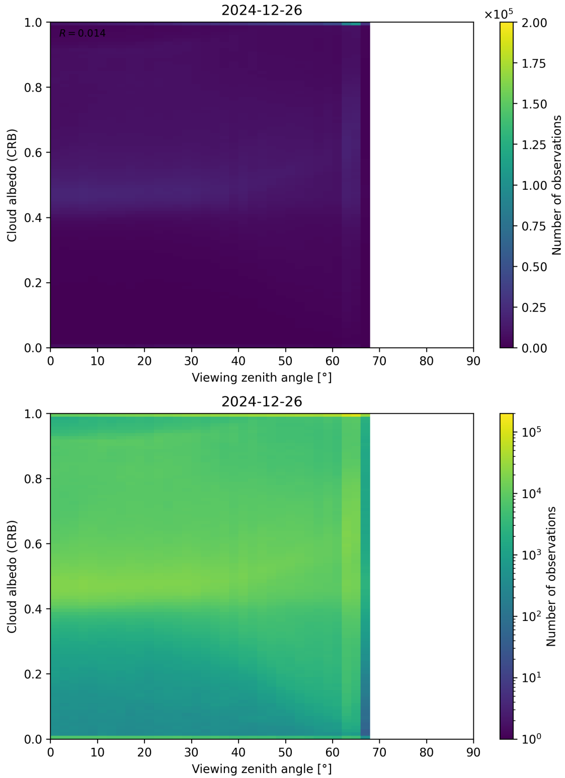
Figure 106: Scatter density plot of “Viewing zenith angle” against “Cloud albedo (CRB)” for 2024-12-25 to 2024-12-27.
