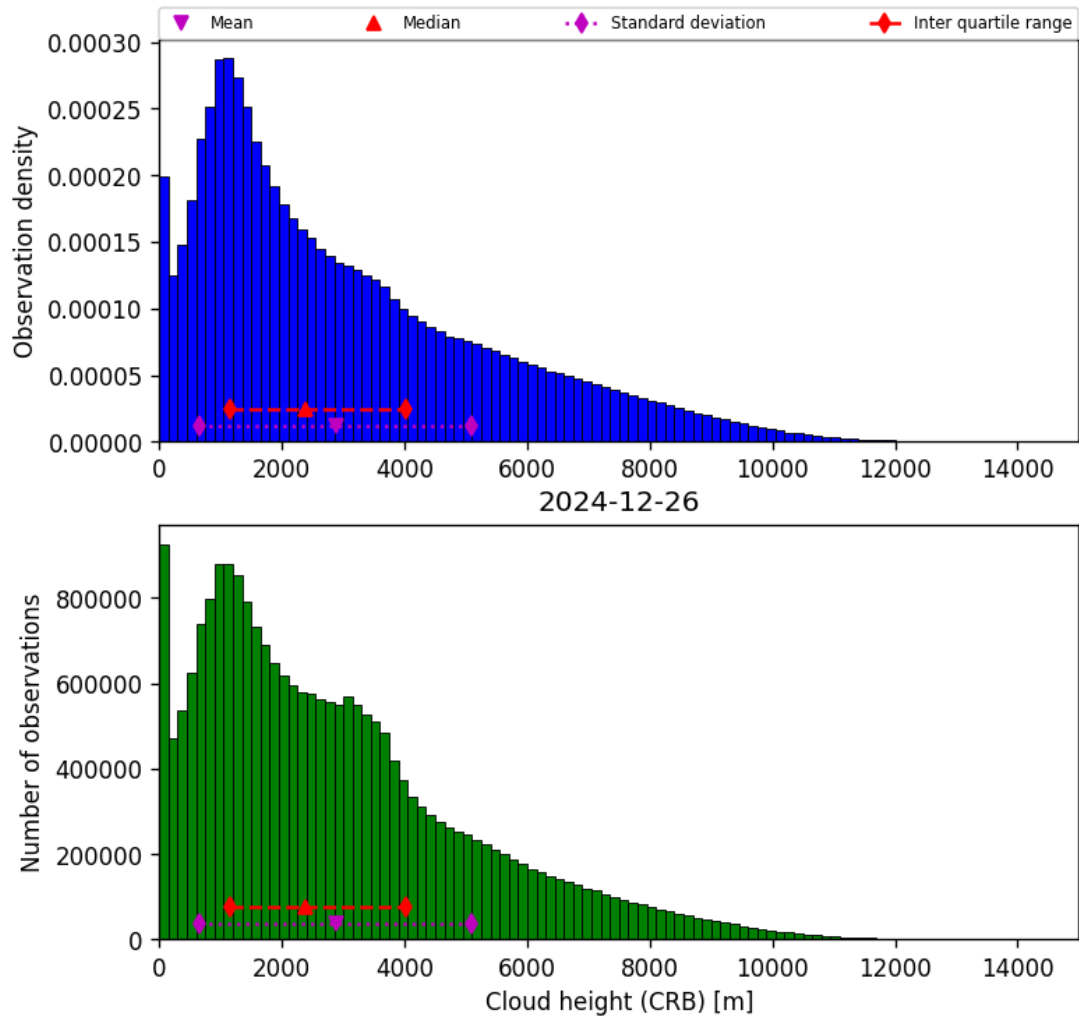
Figure 43: Histogram of “Cloud height (CRB)” for 2024-12-25 to 2024-12-27
