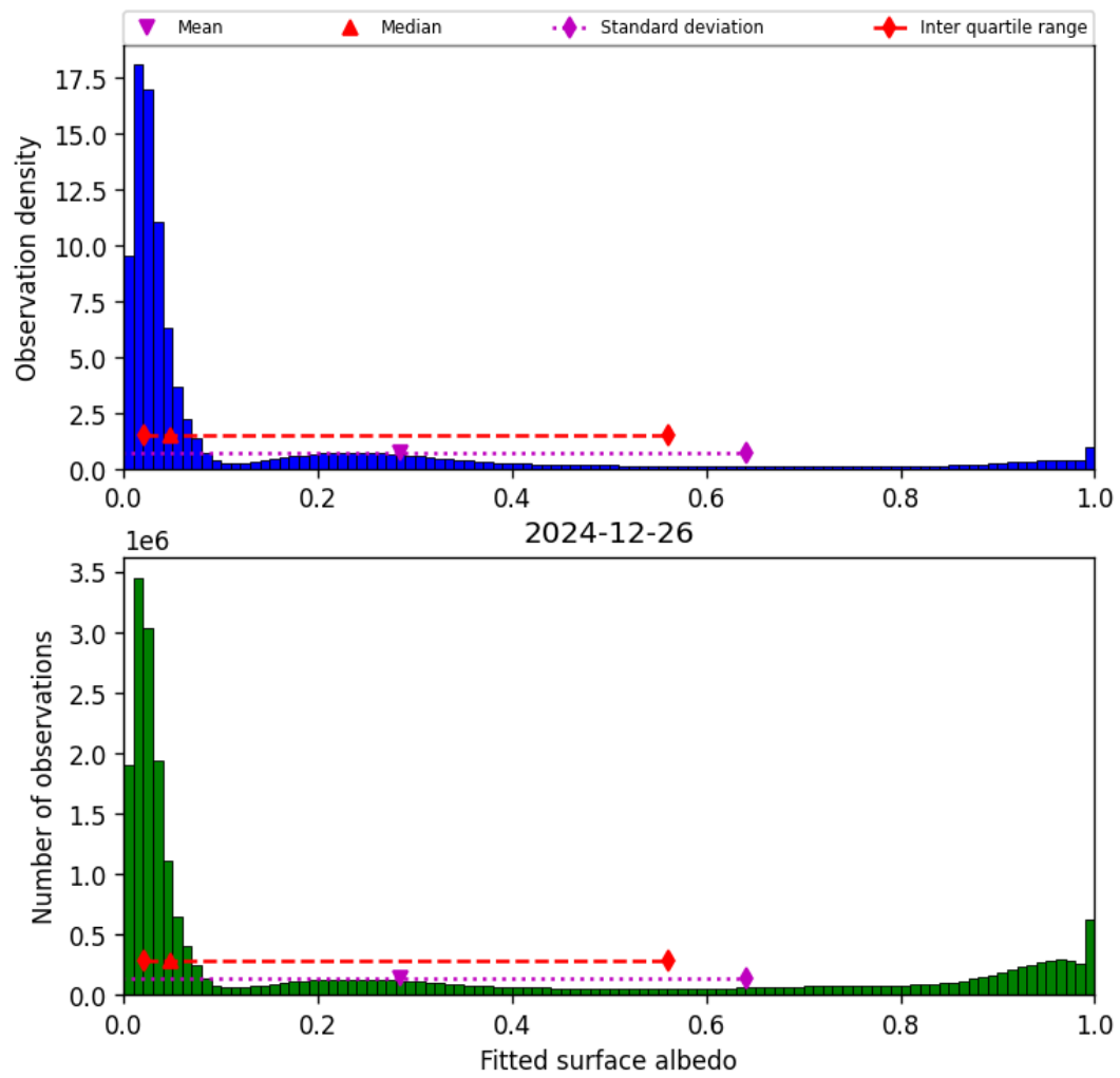
Figure 45: Histogram of “Fitted surface albedo” for 2024-12-25 to 2024-12-27
