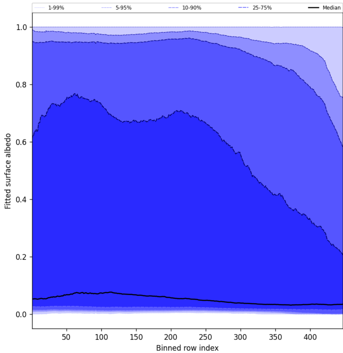
Figure 61: Along track statistics of “Fitted surface albedo” for 2024-12-25 to 2024-12-27
