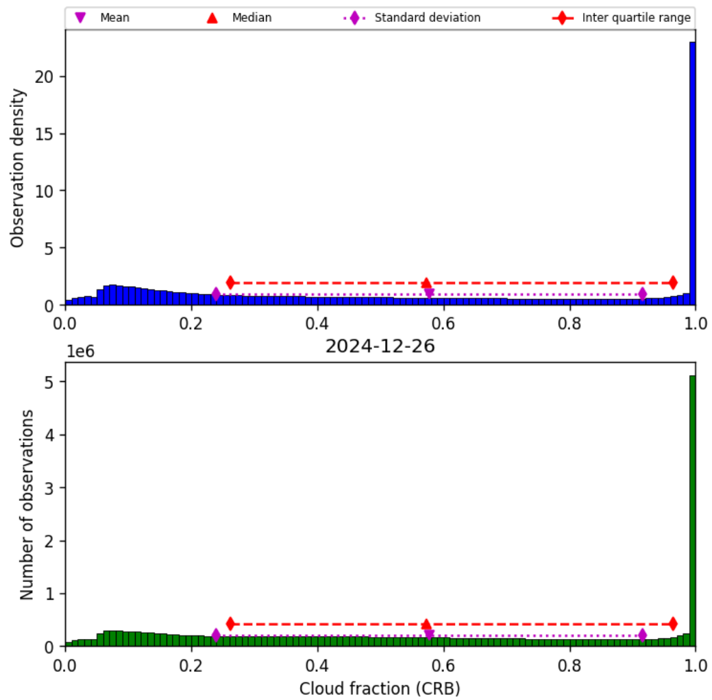
Figure 42: Histogram of “Cloud fraction (CRB)” for 2024-12-25 to 2024-12-27
