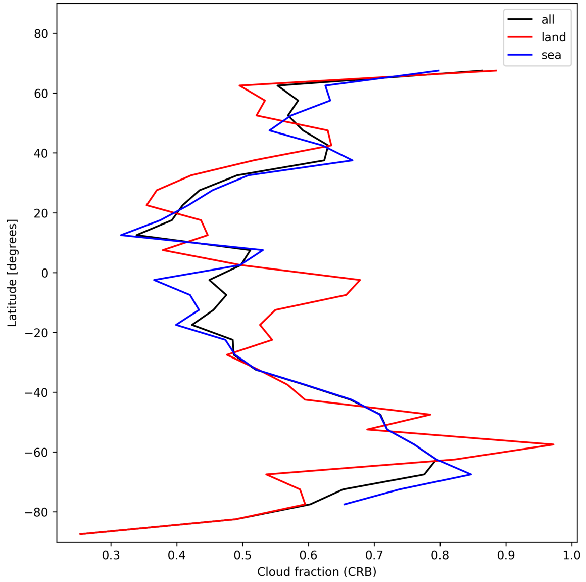
Figure 26: Zonal average of “Cloud fraction (CRB)” for 2024-12-25 to 2024-12-27.
