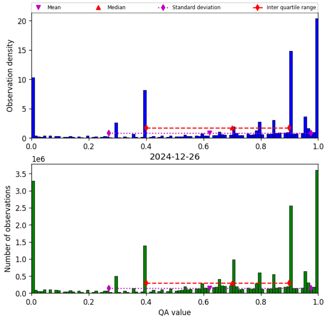
Figure 38: Histogram of “QA value” for 2024-12-25 to 2024-12-27
