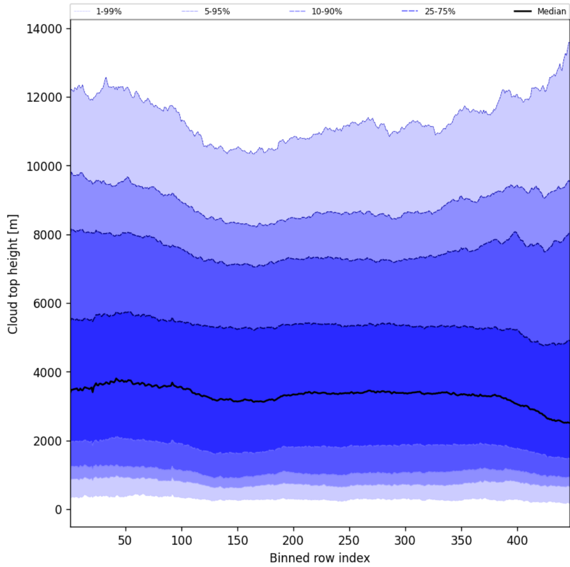
Figure 56: Along track statistics of “Cloud top height” for 2024-12-25 to 2024-12-27
