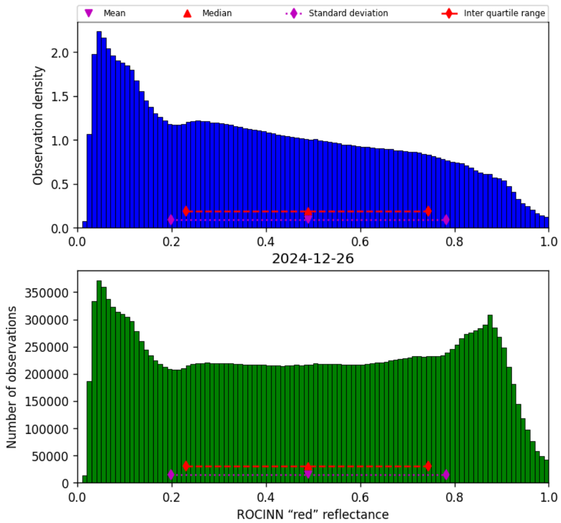
Figure 53: Histogram of “ROCINN “red” reflectance” for 2024-12-25 to 2024-12-27
