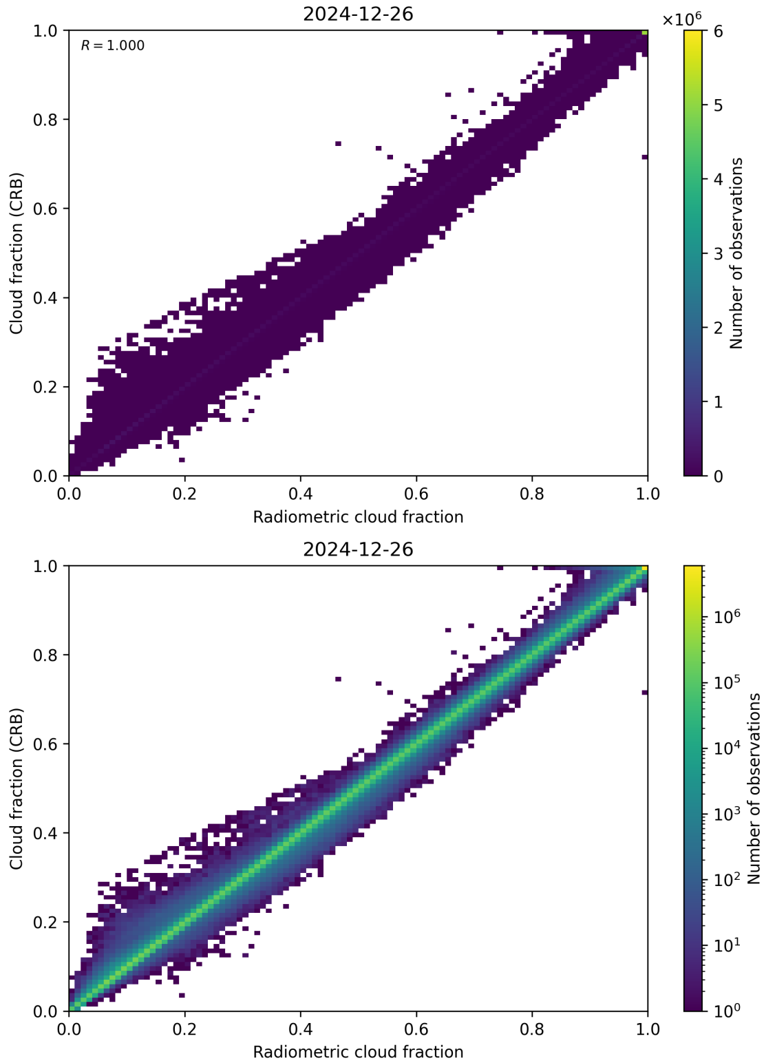
Figure 73: Scatter density plot of “Radiometric cloud fraction” against “Cloud fraction (CRB)” for 2024-12-25 to 2024-12-27.
