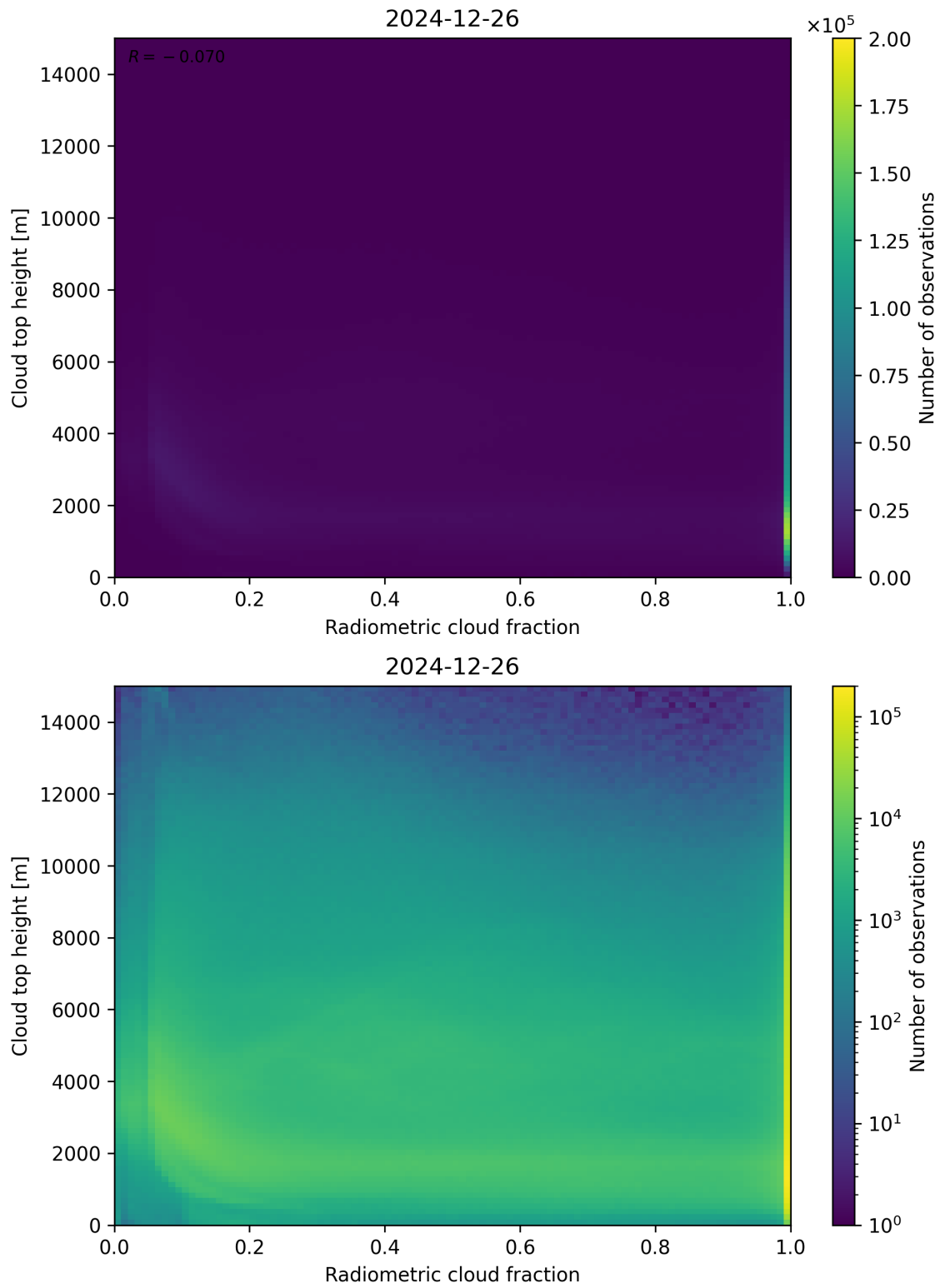
Figure 76: Scatter density plot of “Radiometric cloud fraction” against “Cloud top height” for 2024-12-25 to 2024-12-27.
