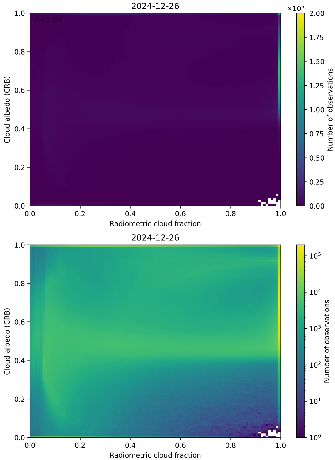
Figure 71: Scatter density plot of “Radiometric cloud fraction” against “Cloud albedo (CRB)” for 2024-12-25 to 2024-12-27.
