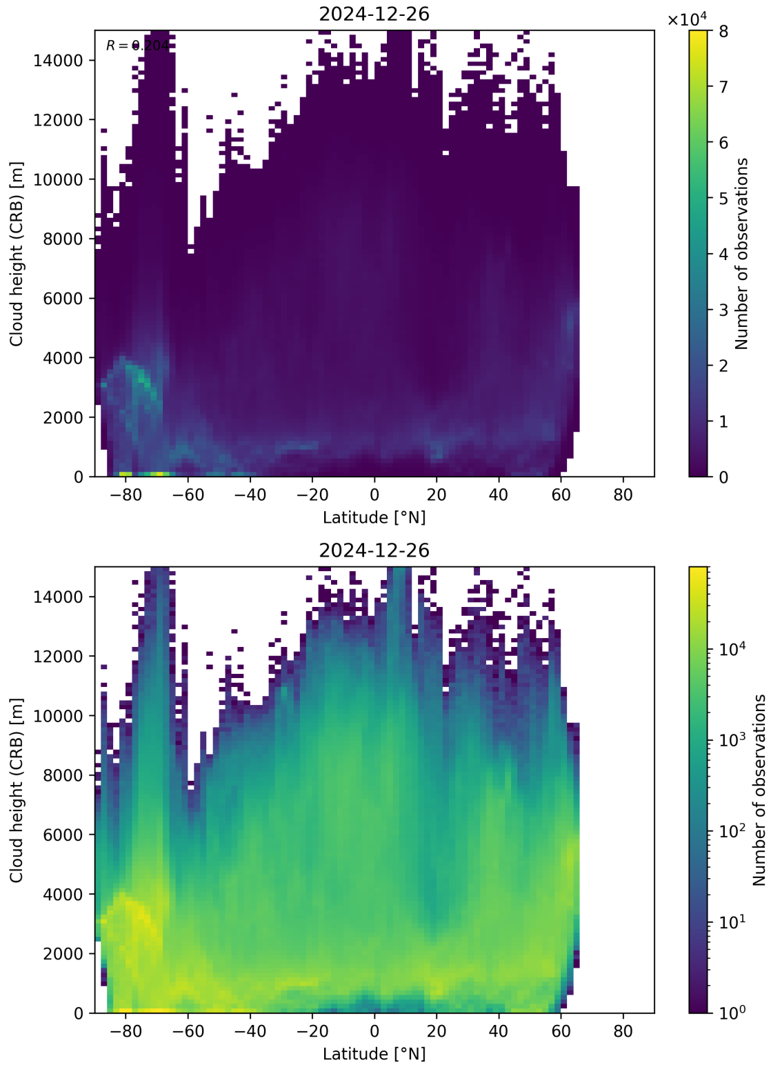
Figure 95: Scatter density plot of “Latitude” against “Cloud height (CRB)” for 2024-12-25 to 2024-12-27.
