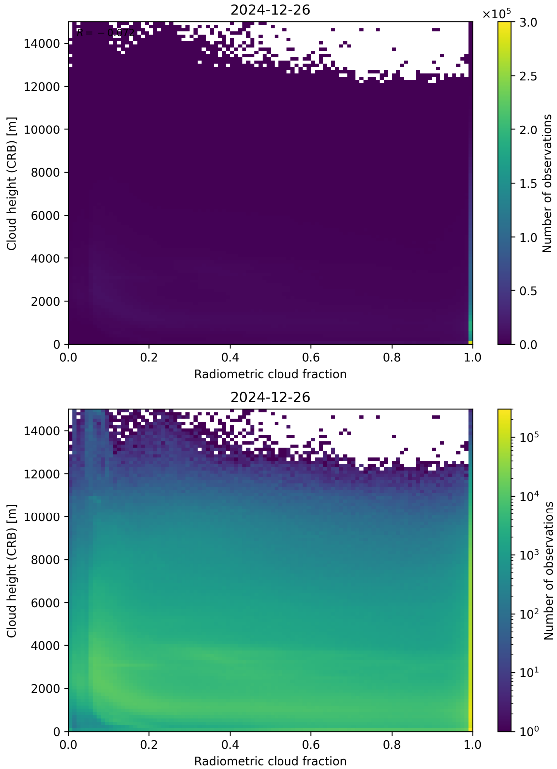
Figure 74: Scatter density plot of “Radiometric cloud fraction” against “Cloud height (CRB)” for 2024-12-25 to 2024-12-27.
