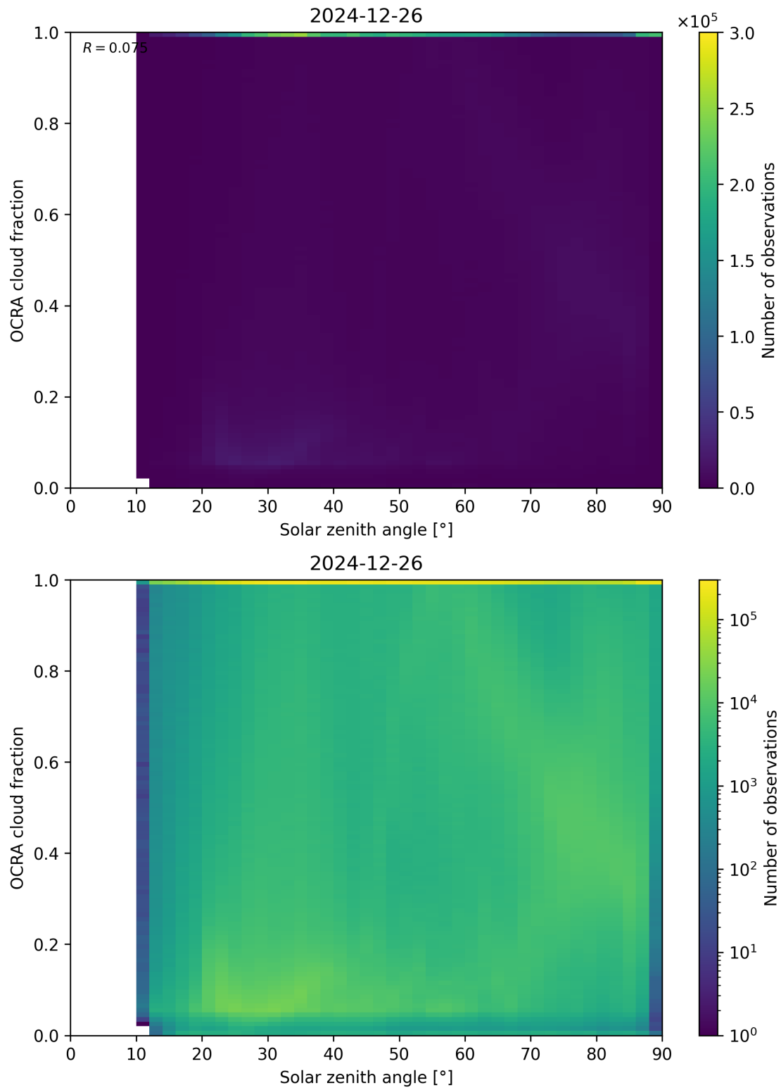
Figure 100: Scatter density plot of “Solar zenith angle” against “OCRA cloud fraction” for 2024-12-25 to 2024-12-27.
