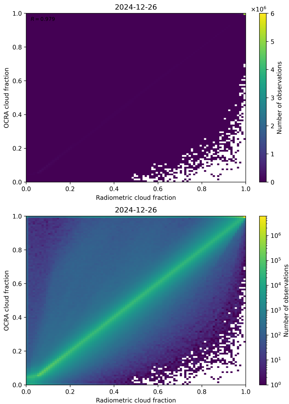
Figure 72: Scatter density plot of “Radiometric cloud fraction” against “OCRA cloud fraction” for 2024-12-25 to 2024-12-27.
