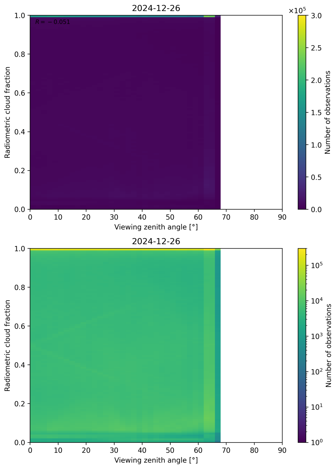
Figure 107: Scatter density plot of “Viewing zenith angle” against “Radiometric cloud fraction” for 2024-12-25 to 2024-12-27.
