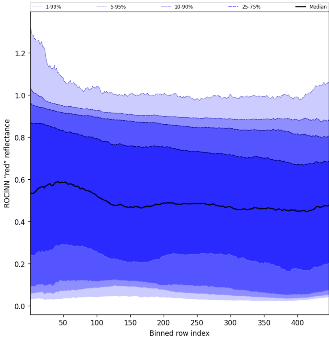
Figure 69: Along track statistics of “ROCINN “red” reflectance” for 2024-12-25 to 2024-12-27
