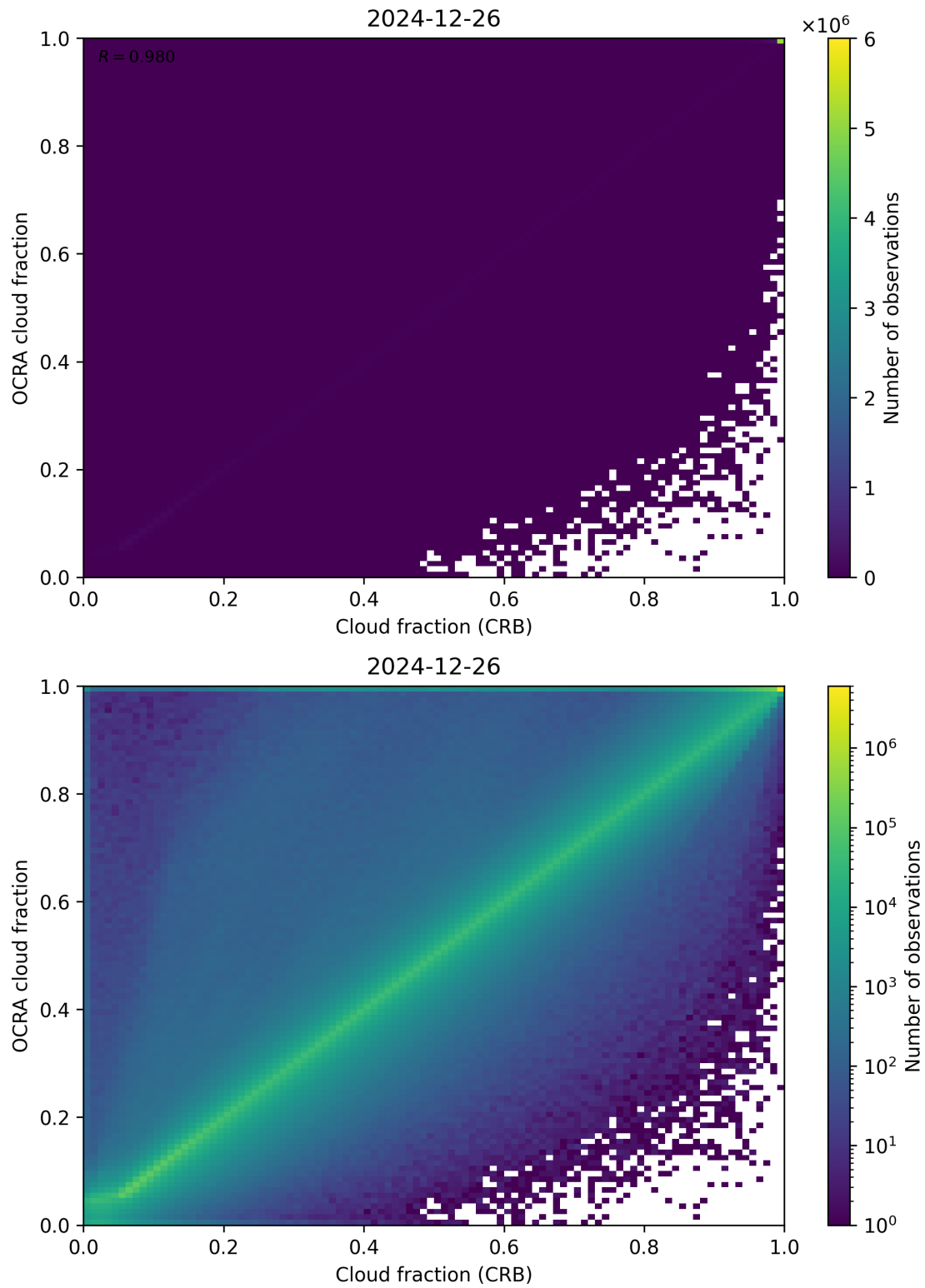
Figure 78: Scatter density plot of “Cloud fraction (CRB)” against “OCRA cloud fraction” for 2024-12-25 to 2024-12-27.
