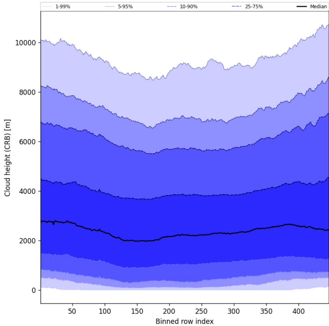
Figure 59: Along track statistics of “Cloud height (CRB)” for 2024-12-25 to 2024-12-27
