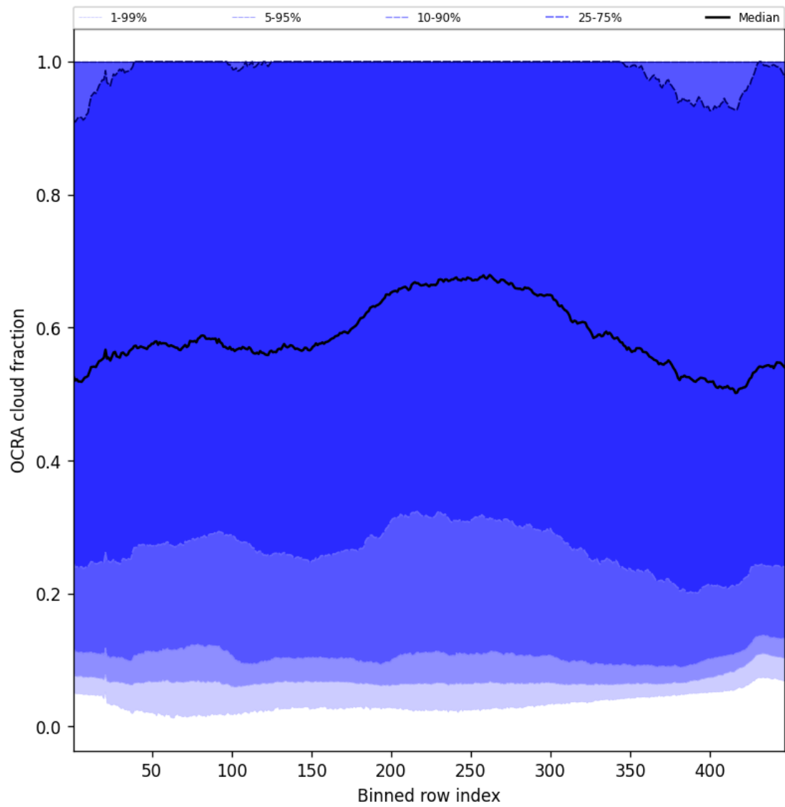
Figure 66: Along track statistics of “OCRA cloud fraction” for 2024-12-25 to 2024-12-27
