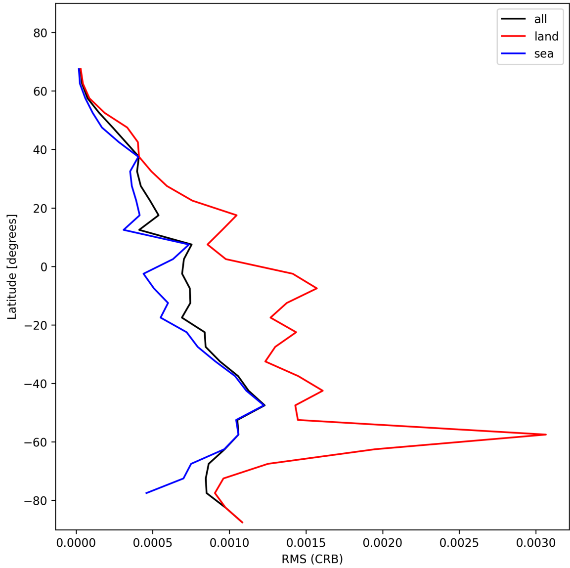
Figure 32: Zonal average of “RMS (CRB)” for 2024-12-25 to 2024-12-27.
