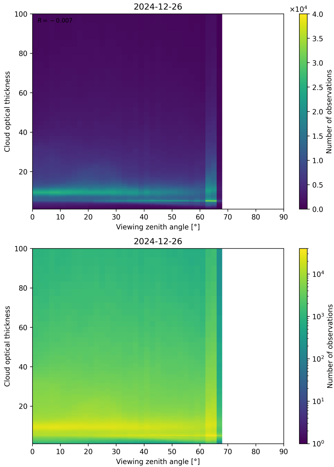
Figure 111: Scatter density plot of “Viewing zenith angle” against “Cloud optical thickness” for 2024-12-25 to 2024-12-27.
