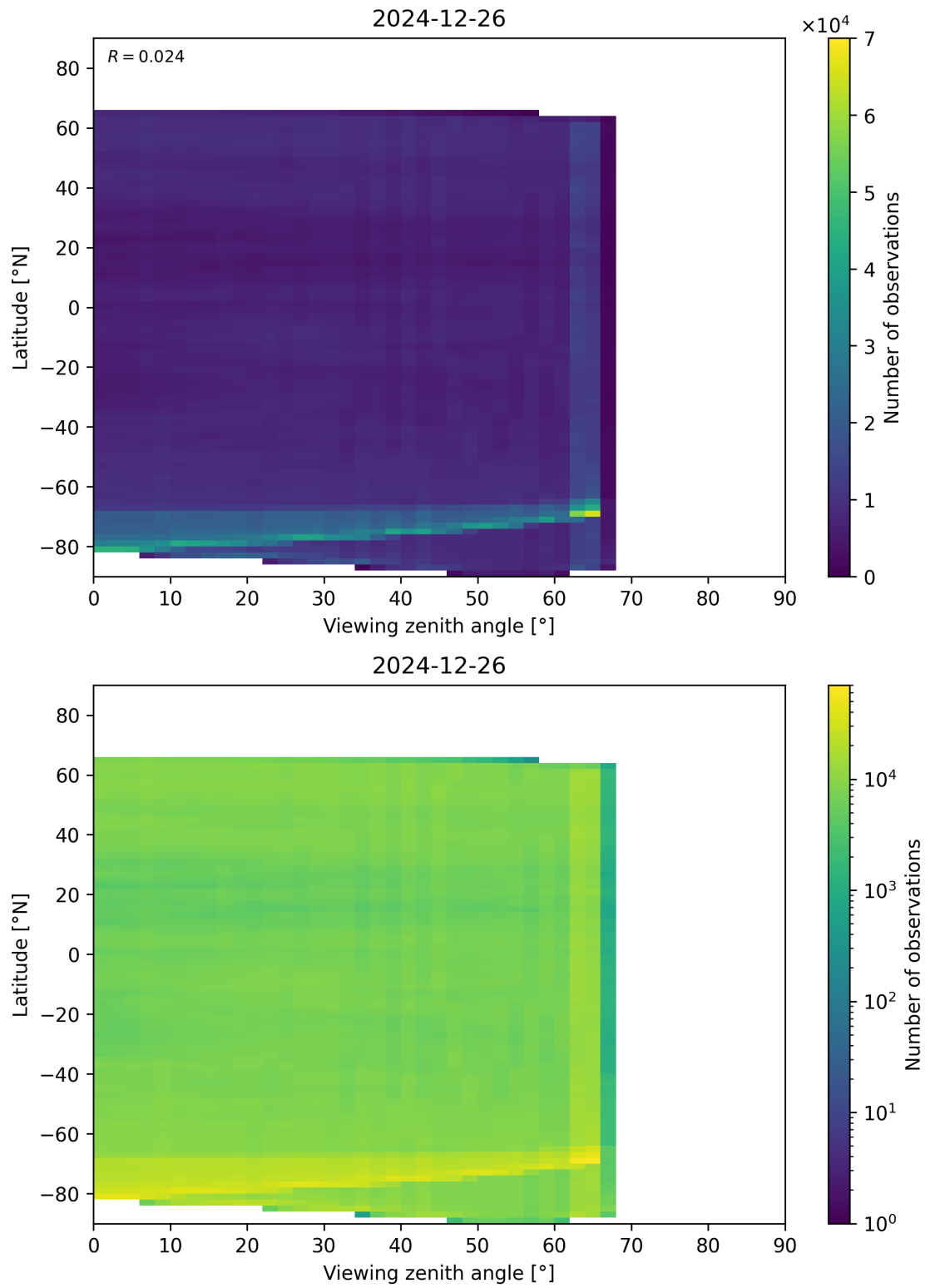
Figure 113: Scatter density plot of “Viewing zenith angle” against “Latitude” for 2024-12-25 to 2024-12-27.
