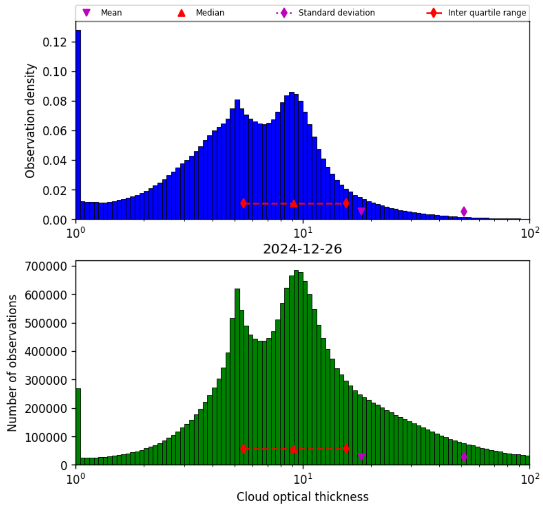
Figure 41: Histogram of “Cloud optical thickness” for 2024-12-25 to 2024-12-27
