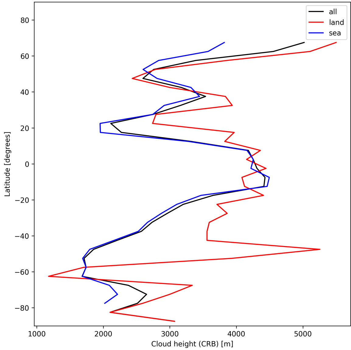
Figure 27: Zonal average of “Cloud height (CRB)” for 2024-12-25 to 2024-12-27.
