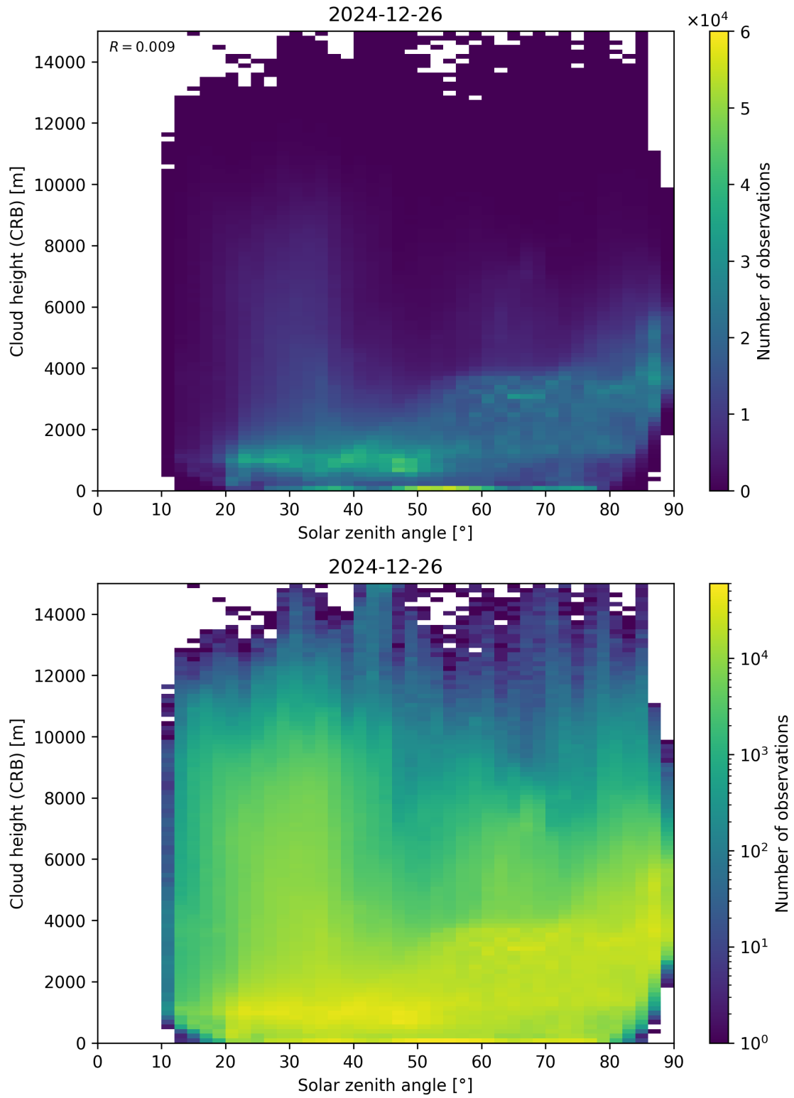
Figure 102: Scatter density plot of “Solar zenith angle” against “Cloud height (CRB)” for 2024-12-25 to 2024-12-27.
