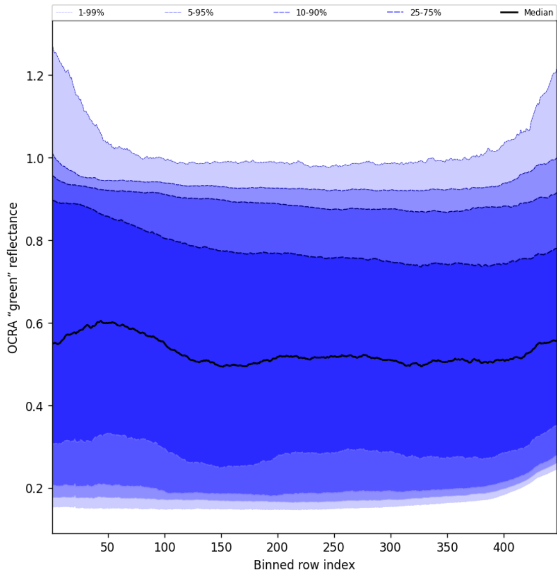
Figure 68: Along track statistics of "OCRA "green" reflectance" for 2024-12-25 to 2024-12-27
