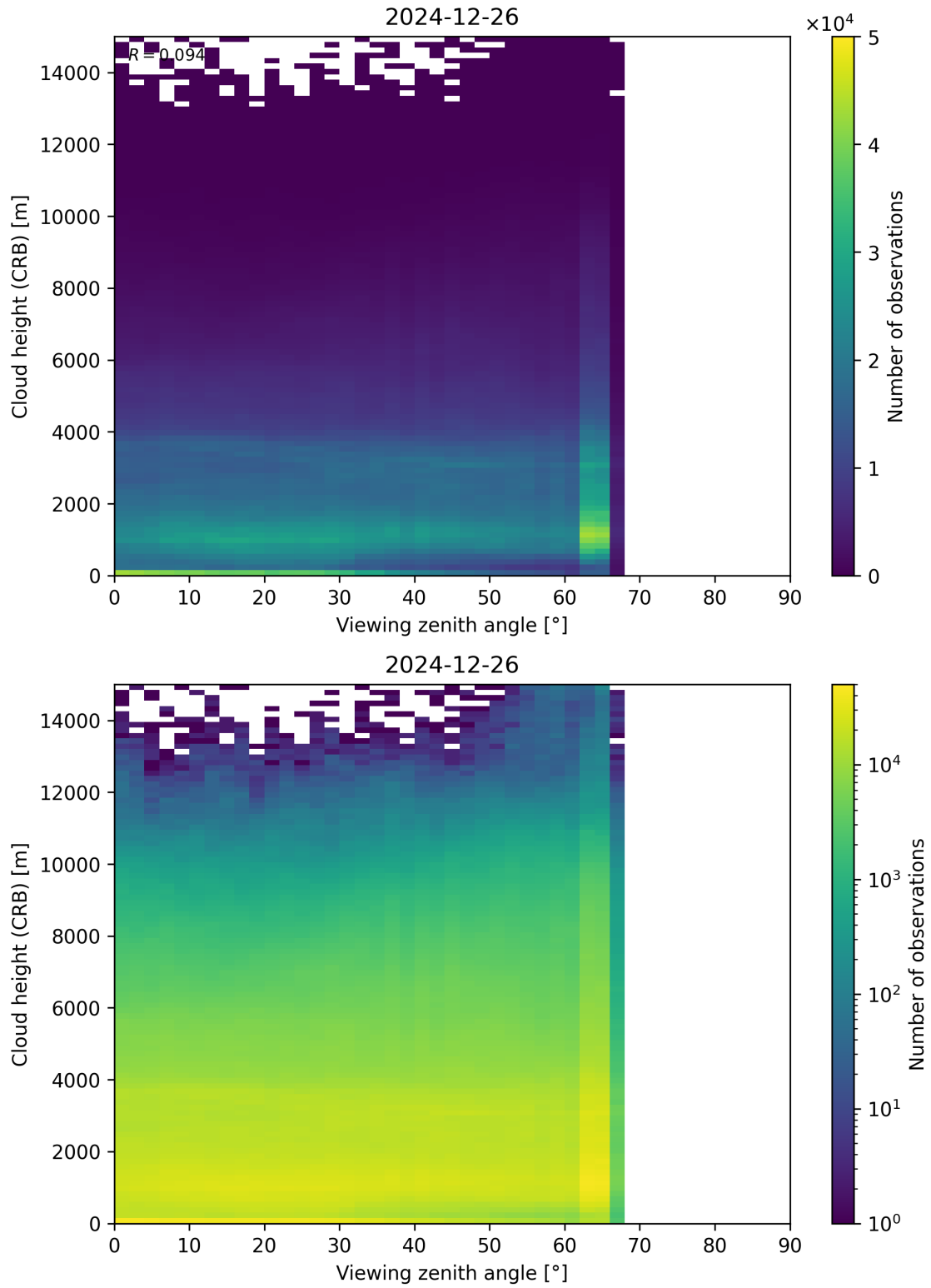
Figure 110: Scatter density plot of “Viewing zenith angle” against “Cloud height (CRB)” for 2024-12-25 to 2024-12-27.
