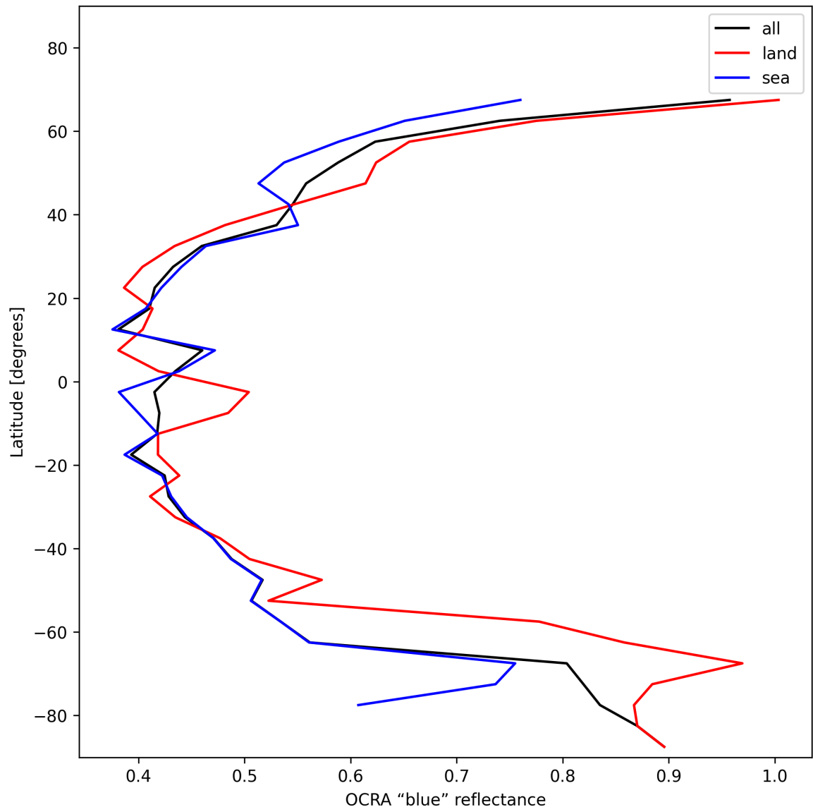
Figure 35: Zonal average of “OCRA “blue” reflectance” for 2024-12-25 to 2024-12-27.
