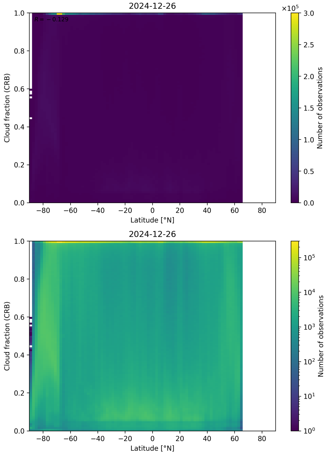
Figure 94: Scatter density plot of “Latitude” against “Cloud fraction (CRB)” for 2024-12-25 to 2024-12-27.
