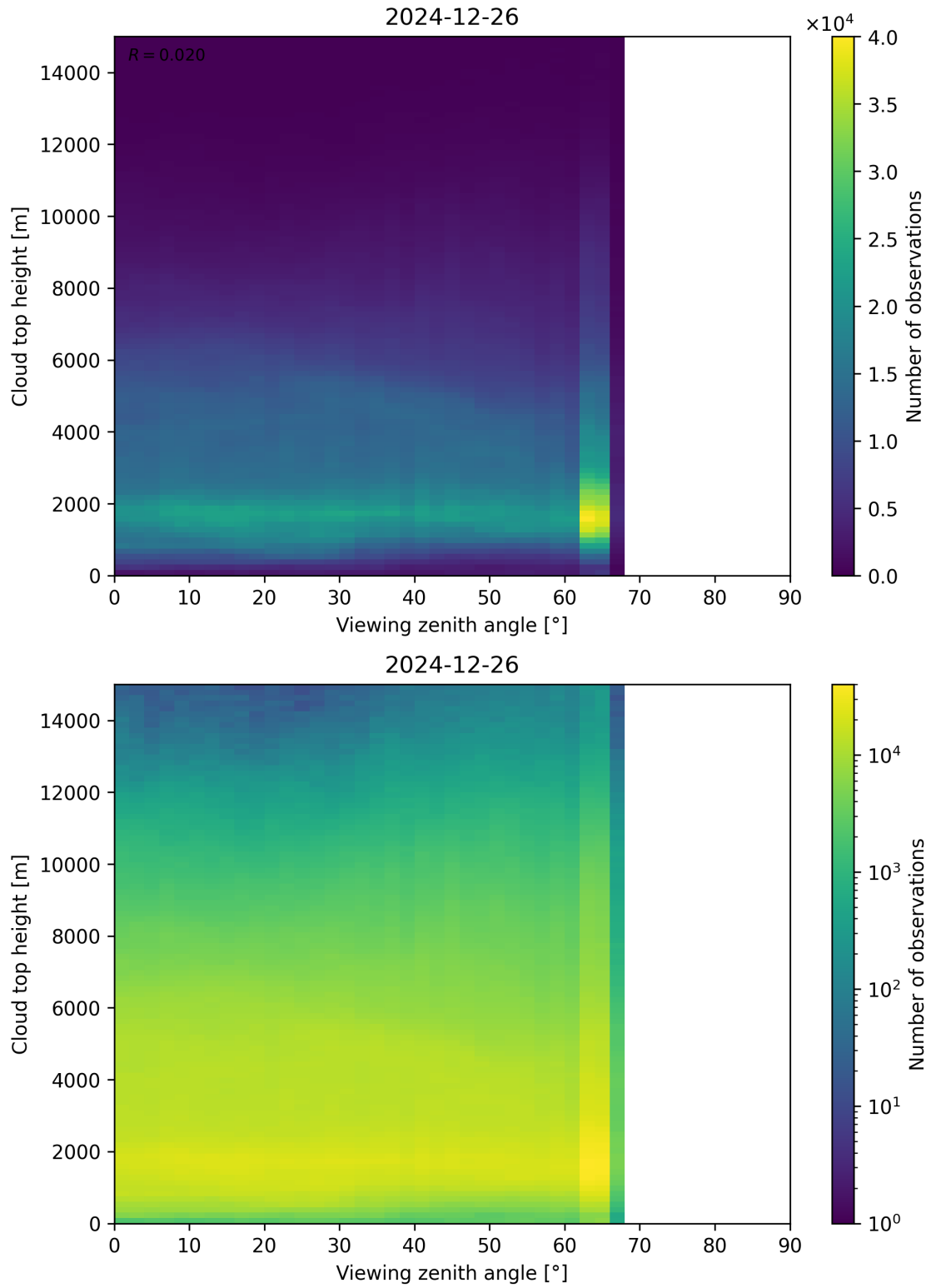
Figure 112: Scatter density plot of “Viewing zenith angle” against “Cloud top height” for 2024-12-25 to 2024-12-27.
