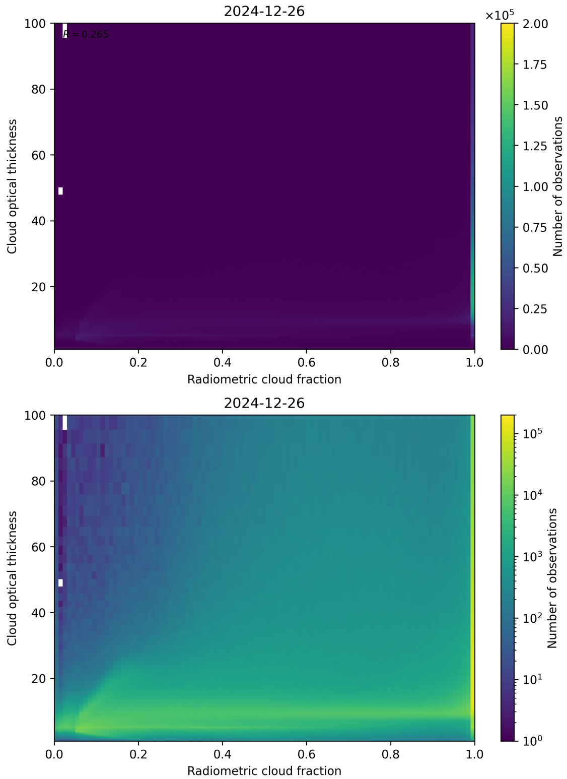
Figure 75: Scatter density plot of “Radiometric cloud fraction” against “Cloud optical thickness” for 2024-12-25 to 2024-12-27.
