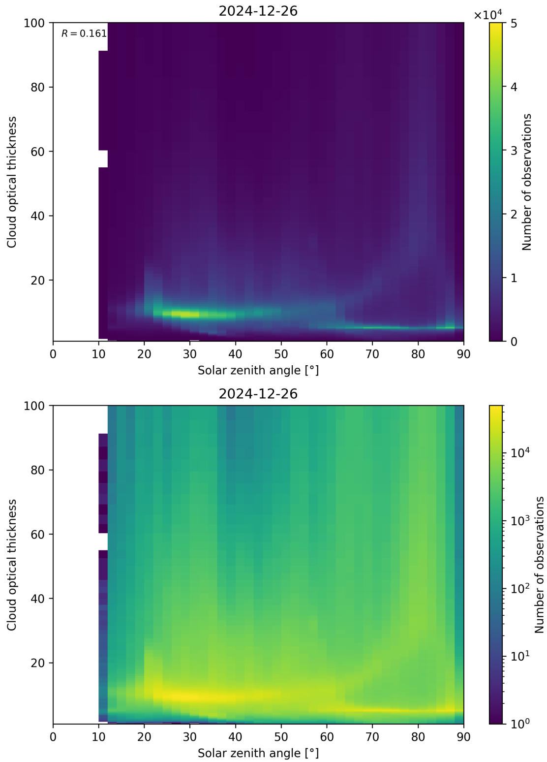
Figure 103: Scatter density plot of “Solar zenith angle” against “Cloud optical thickness” for 2024-12-25 to 2024-12-27.
