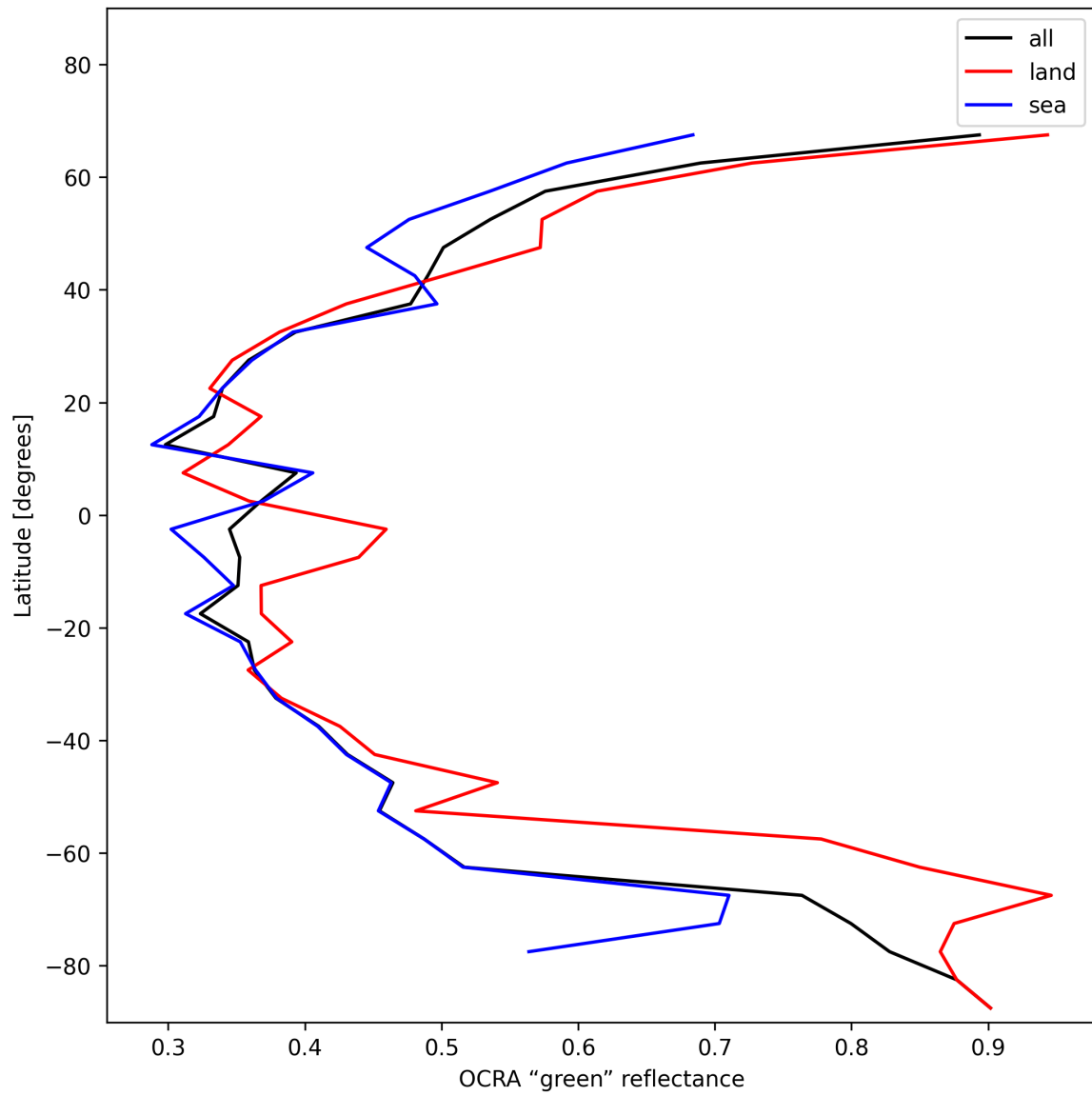
Figure 36: Zonal average of “OCRA “green” reflectance” for 2024-12-25 to 2024-12-27.
