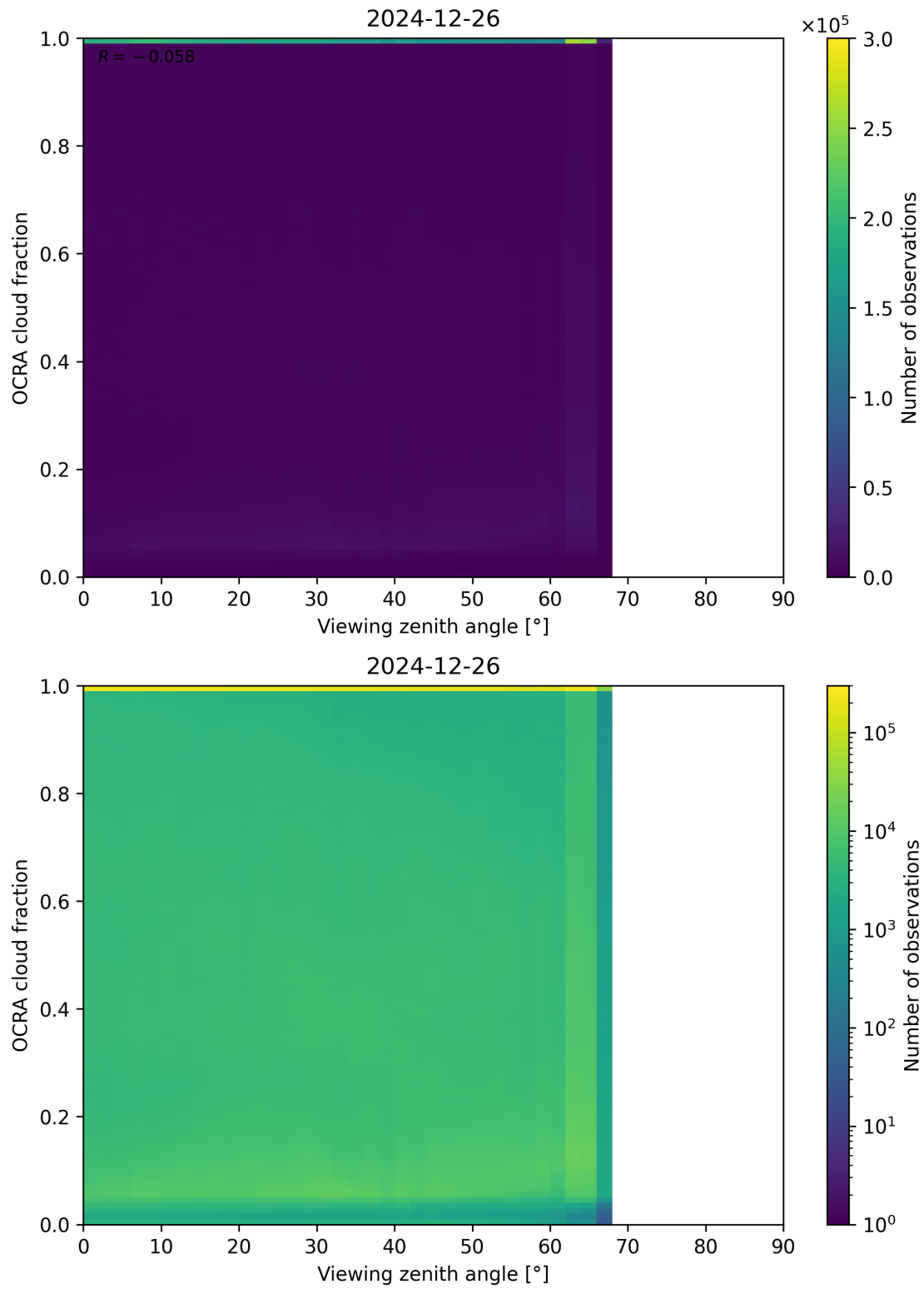
Figure 108: Scatter density plot of “Viewing zenith angle” against “OCRA cloud fraction” for 2024-12-25 to 2024-12-27.
