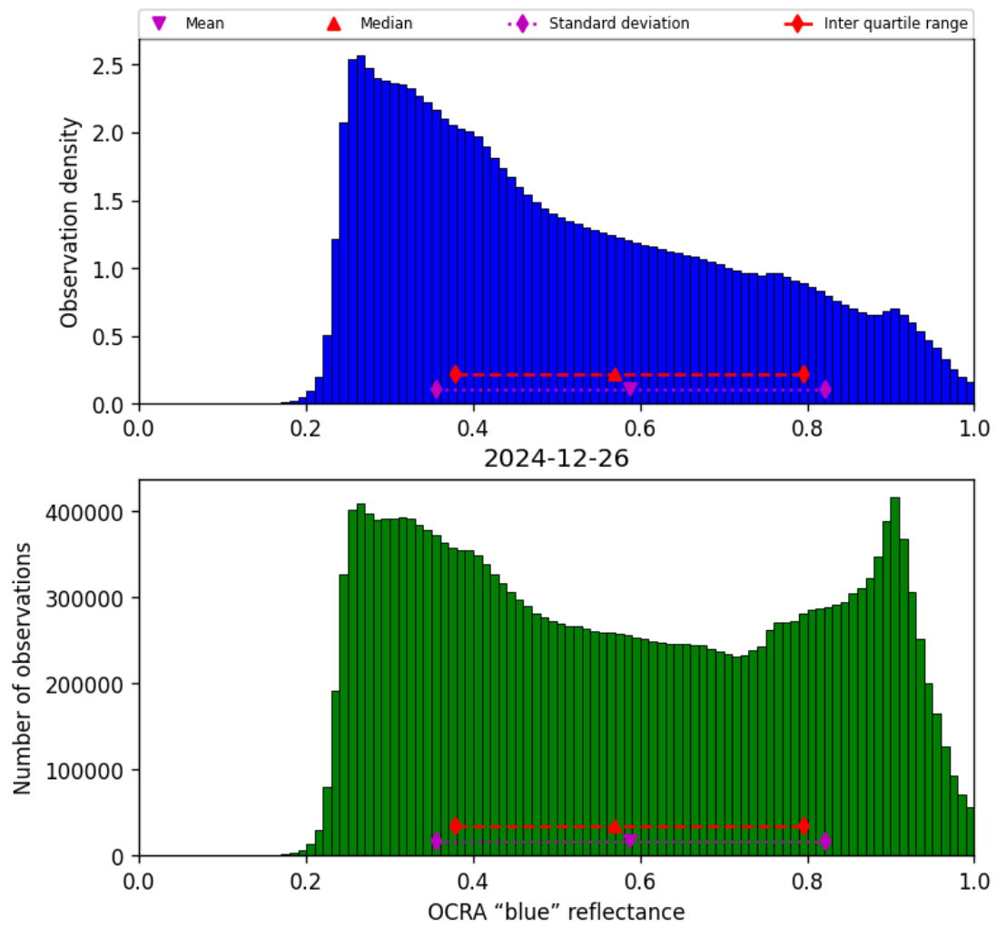
Figure 51: Histogram of “OCRA “blue” reflectance” for 2024-12-25 to 2024-12-27
