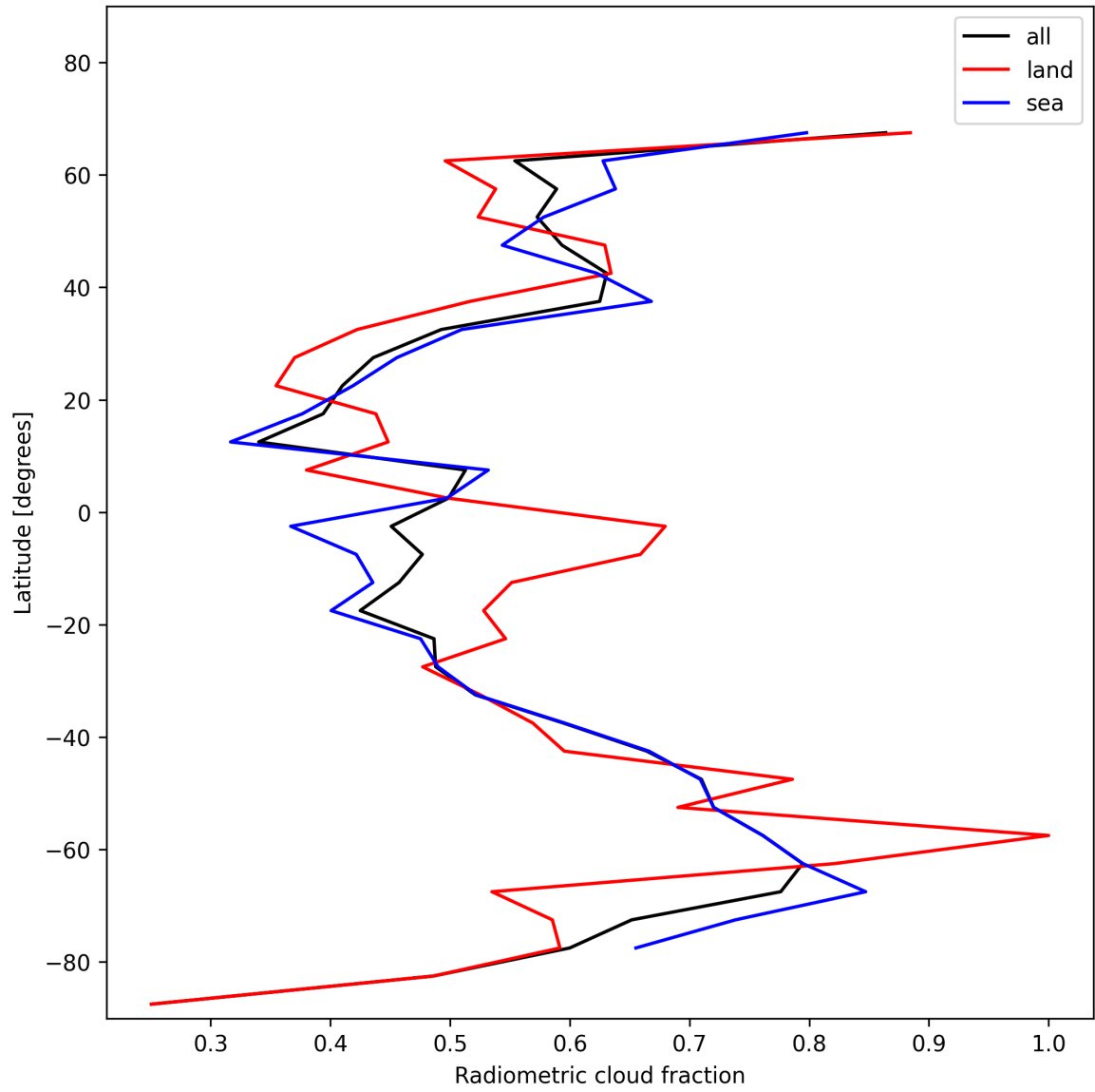
Figure 23: Zonal average of “Radiometric cloud fraction” for 2024-12-25 to 2024-12-27.
