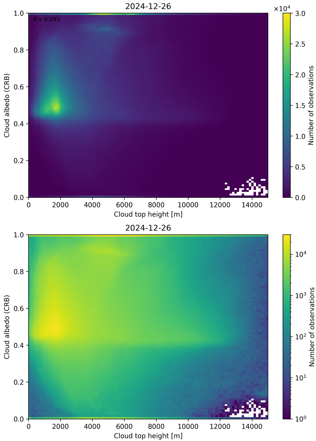
Figure 86: Scatter density plot of “Cloud top height” against “Cloud albedo (CRB)” for 2024-12-25 to 2024-12-27.
