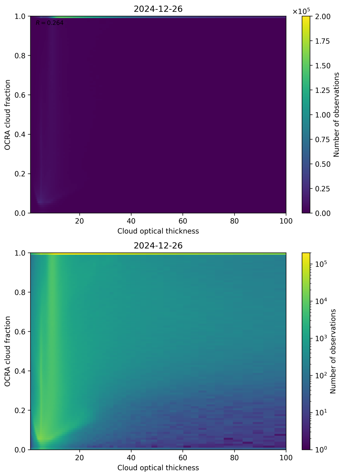
Figure 83: Scatter density plot of “Cloud optical thickness” against “OCRA cloud fraction” for 2024-12-25 to 2024-12-27.
