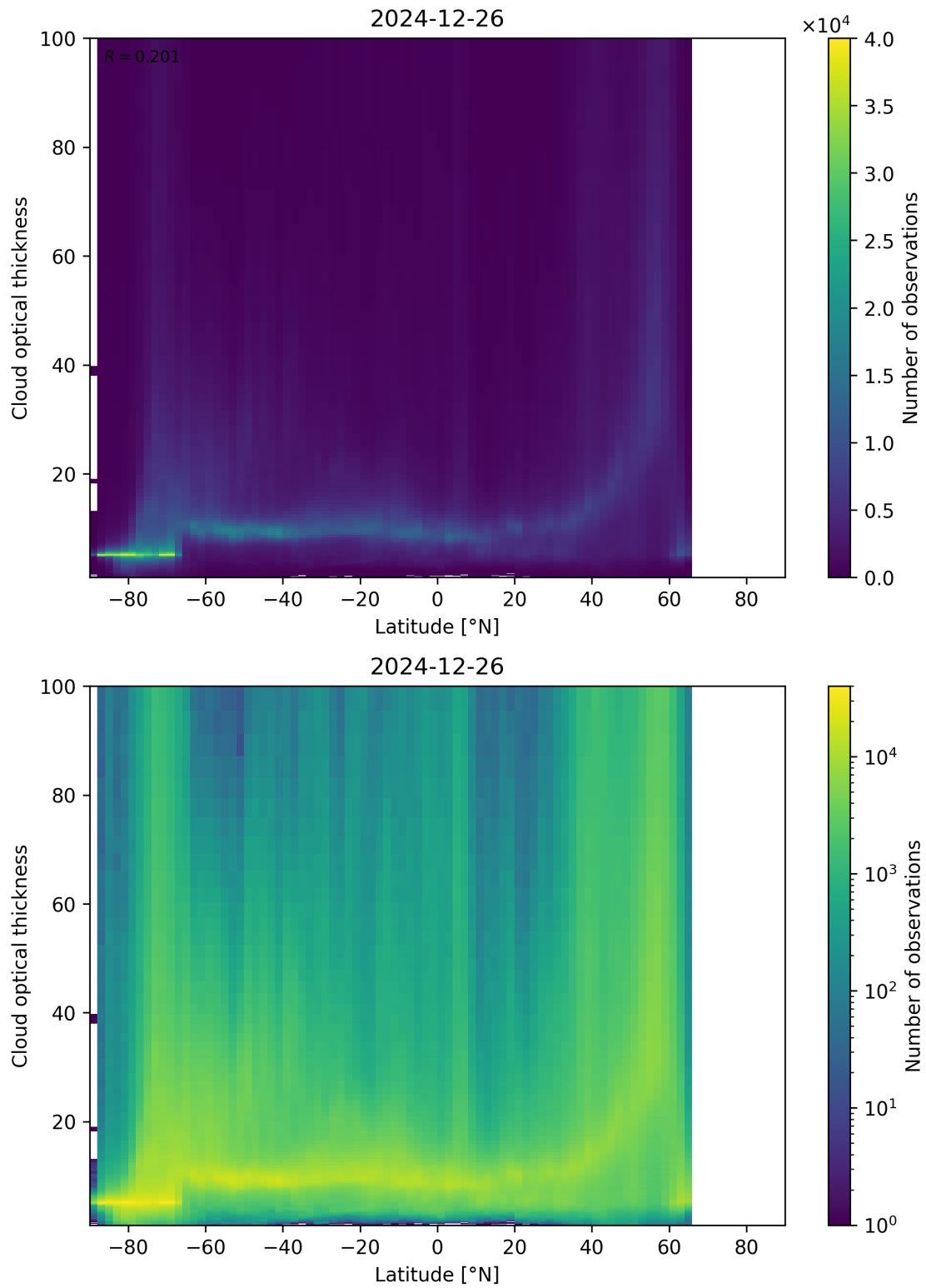
Figure 96: Scatter density plot of “Latitude” against “Cloud optical thickness” for 2024-12-25 to 2024-12-27.
