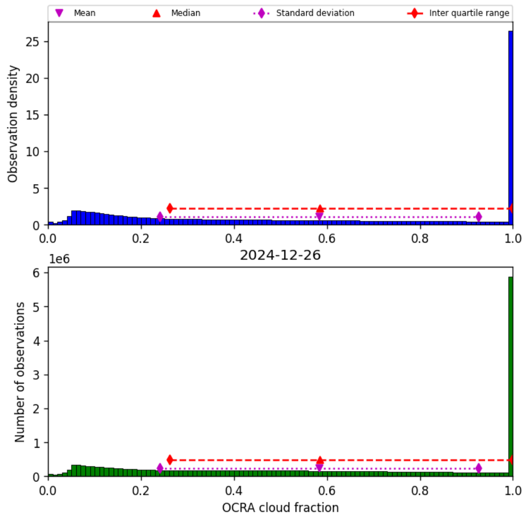
Figure 50: Histogram of “OCRA cloud fraction” for 2024-12-25 to 2024-12-27
