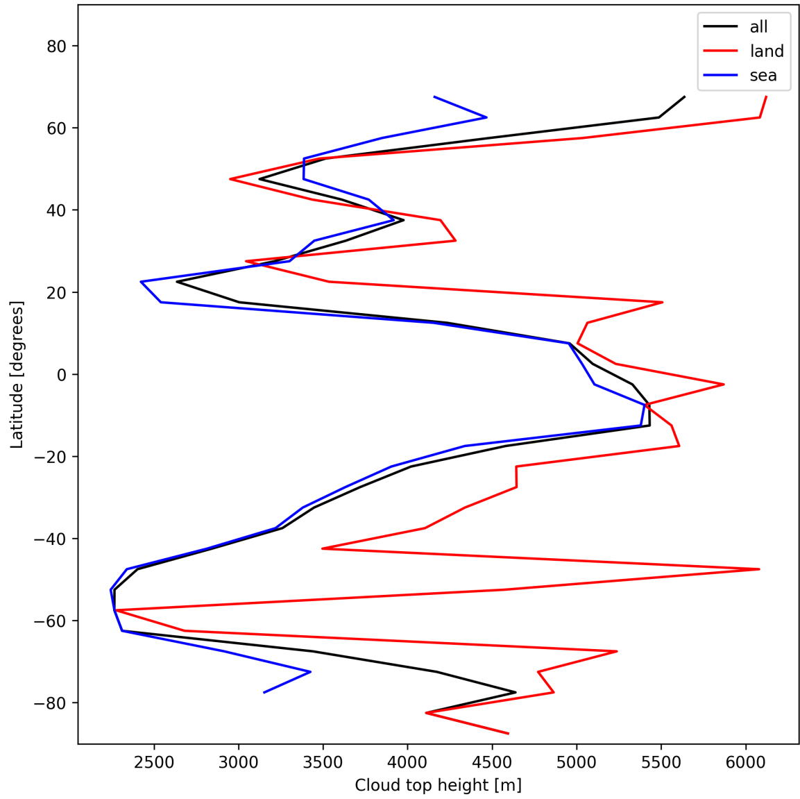
Figure 24: Zonal average of “Cloud top height” for 2024-12-25 to 2024-12-27.
