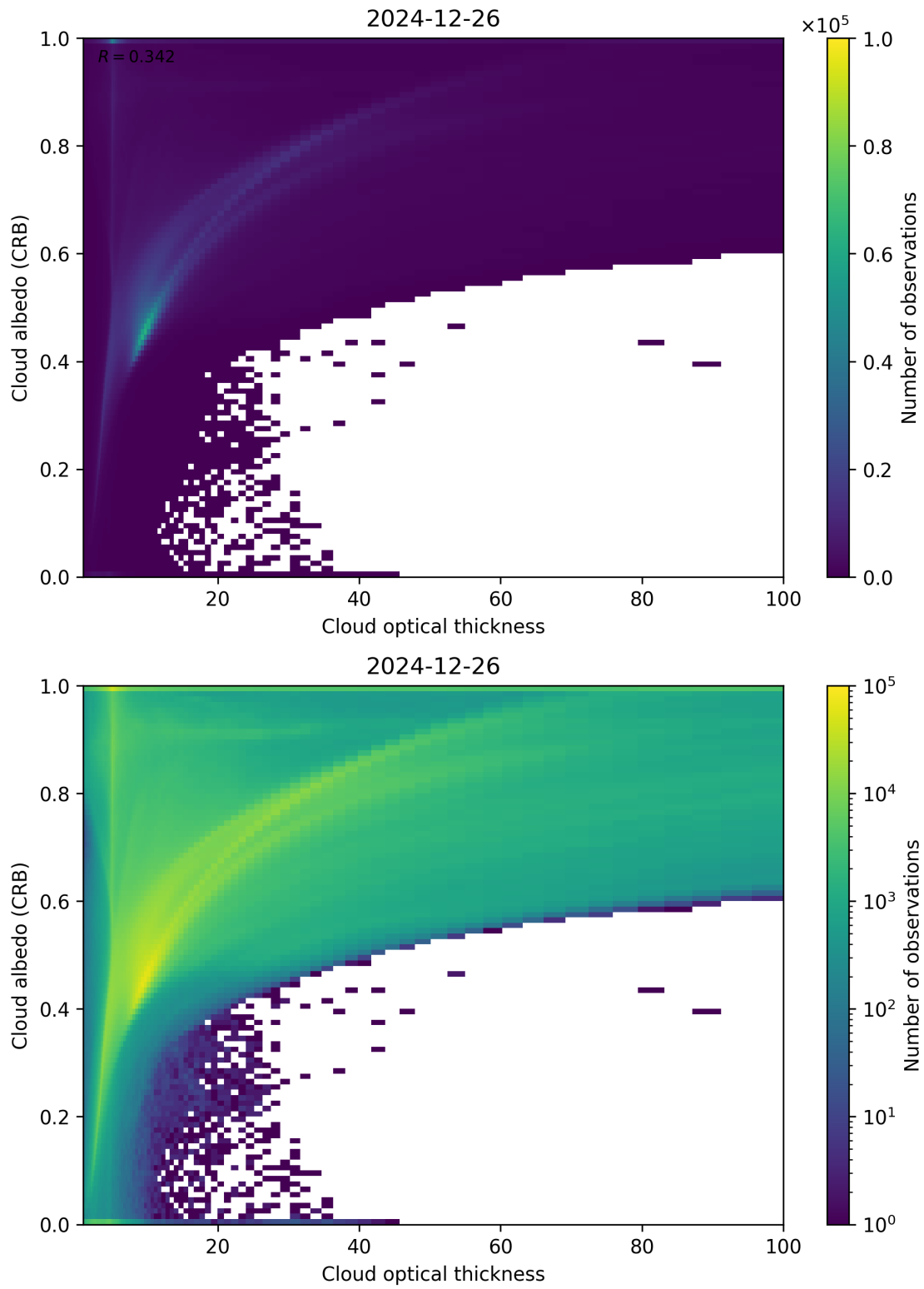
Figure 82: Scatter density plot of “Cloud optical thickness” against “Cloud albedo (CRB)” for 2024-12-25 to 2024-12-27.
