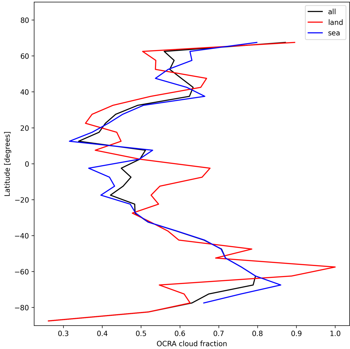
Figure 34: Zonal average of “OCRA cloud fraction” for 2024-12-25 to 2024-12-27.
