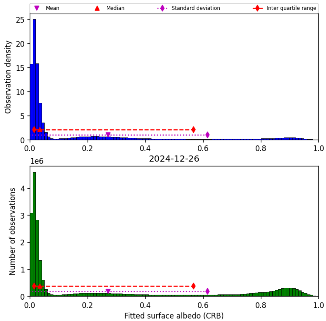
Figure 46: Histogram of “Fitted surface albedo (CRB)” for 2024-12-25 to 2024-12-27
