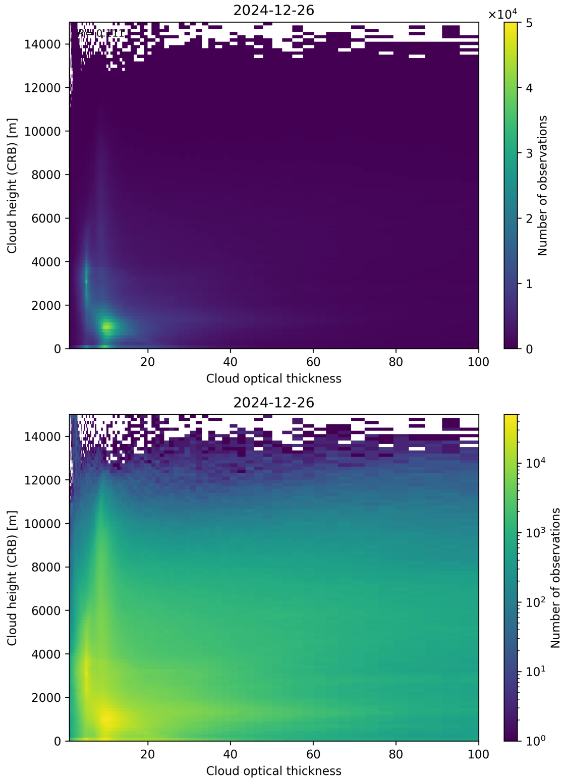
Figure 85: Scatter density plot of “Cloud optical thickness” against “Cloud height (CRB)” for 2024-12-25 to 2024-12-27.
