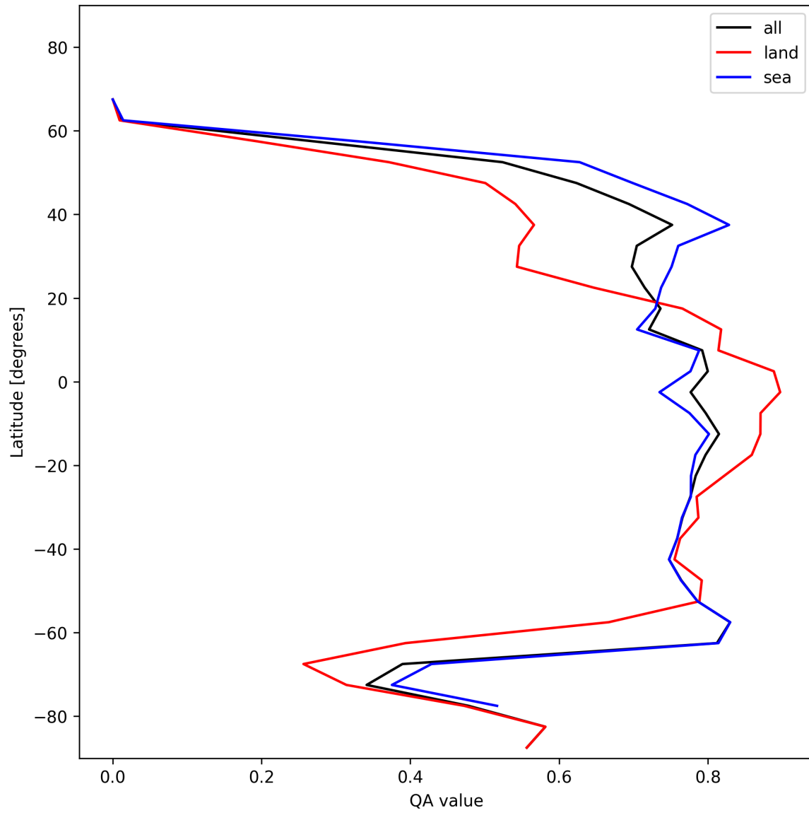
Figure 22: Zonal average of “QA value” for 2024-12-25 to 2024-12-27.
