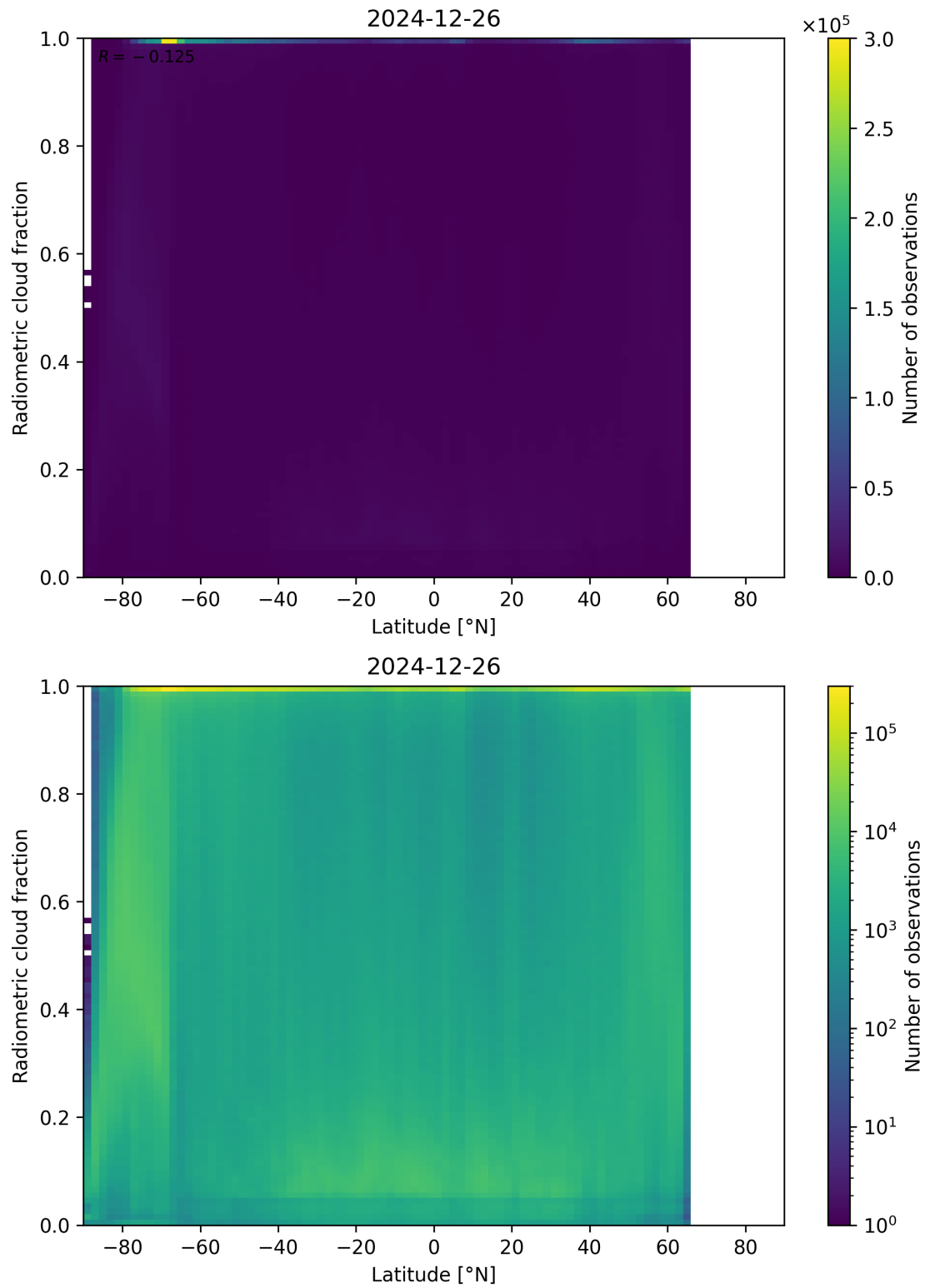
Figure 92: Scatter density plot of “Latitude” against “Radiometric cloud fraction” for 2024-12-25 to 2024-12-27.
