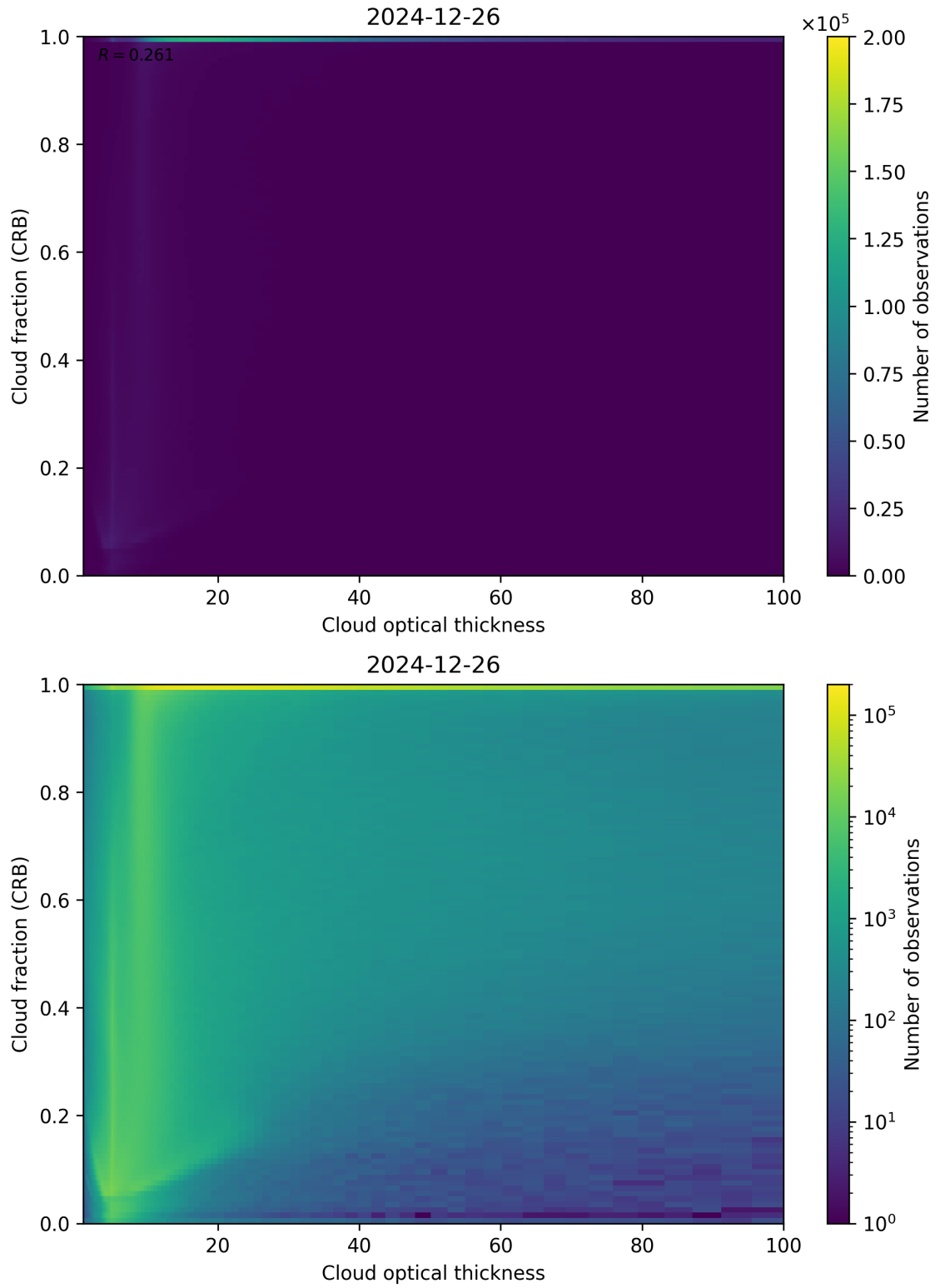
Figure 84: Scatter density plot of “Cloud optical thickness” against “Cloud fraction (CRB)” for 2024-12-25 to 2024-12-27.
