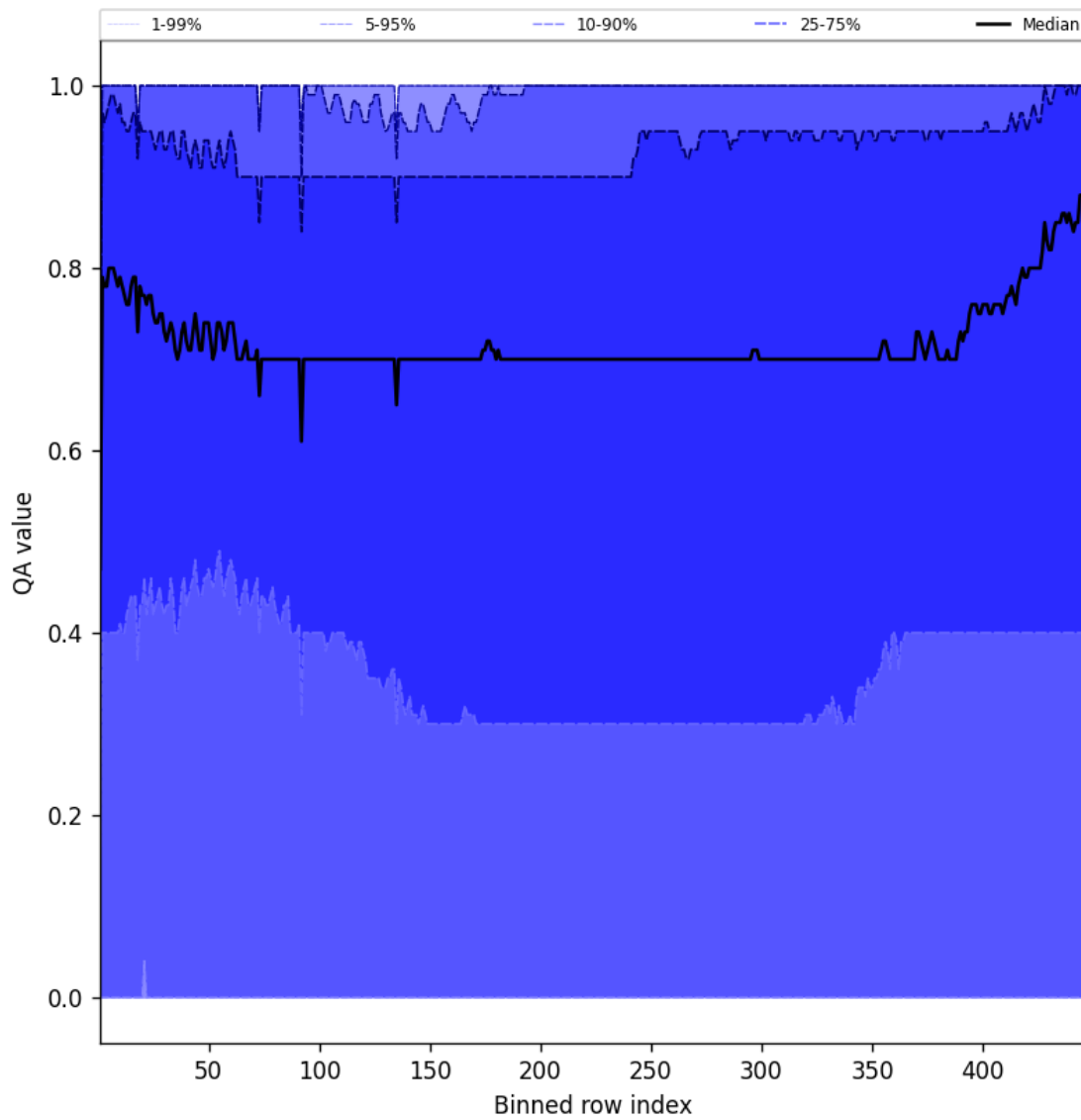
Figure 54: Along track statistics of “QA value” for 2024-12-25 to 2024-12-27
