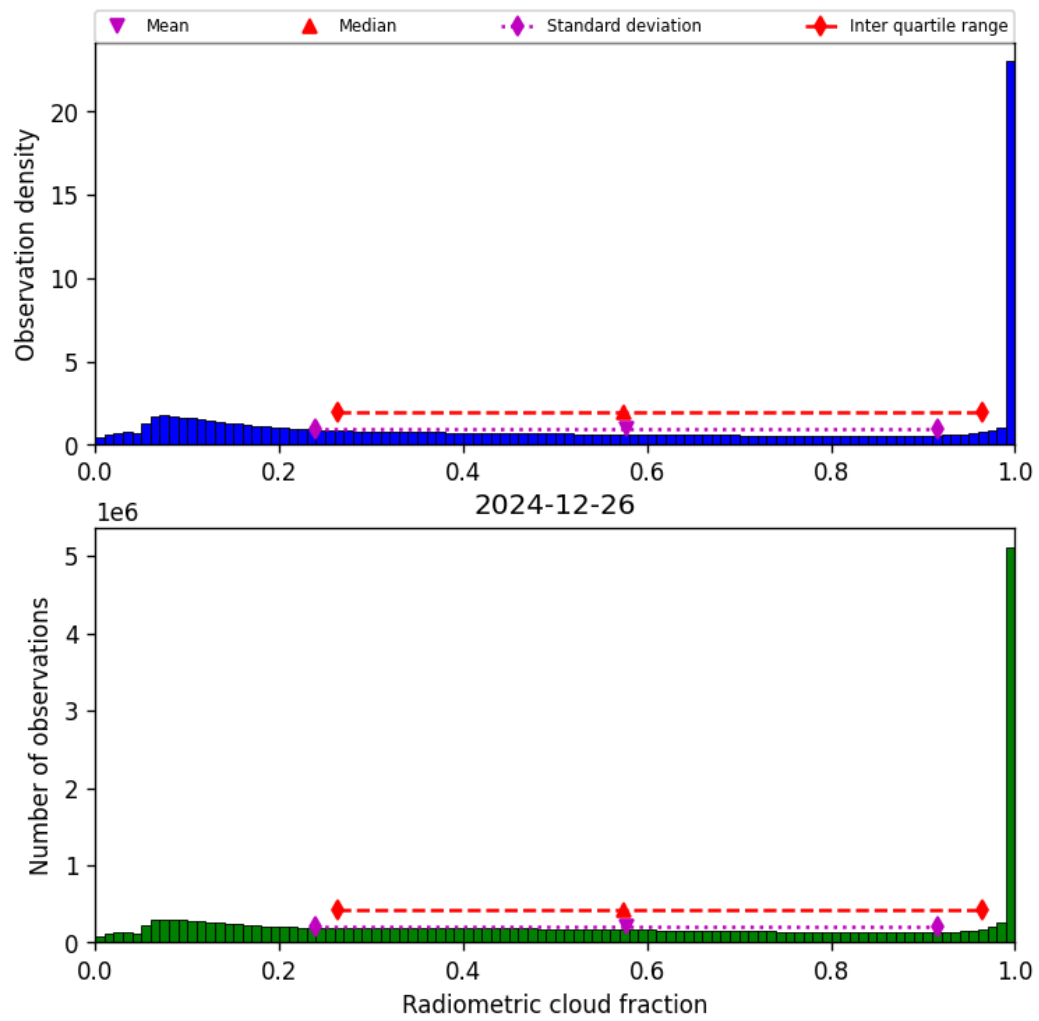
Figure 39: Histogram of “Radiometric cloud fraction” for 2024-12-25 to 2024-12-27
