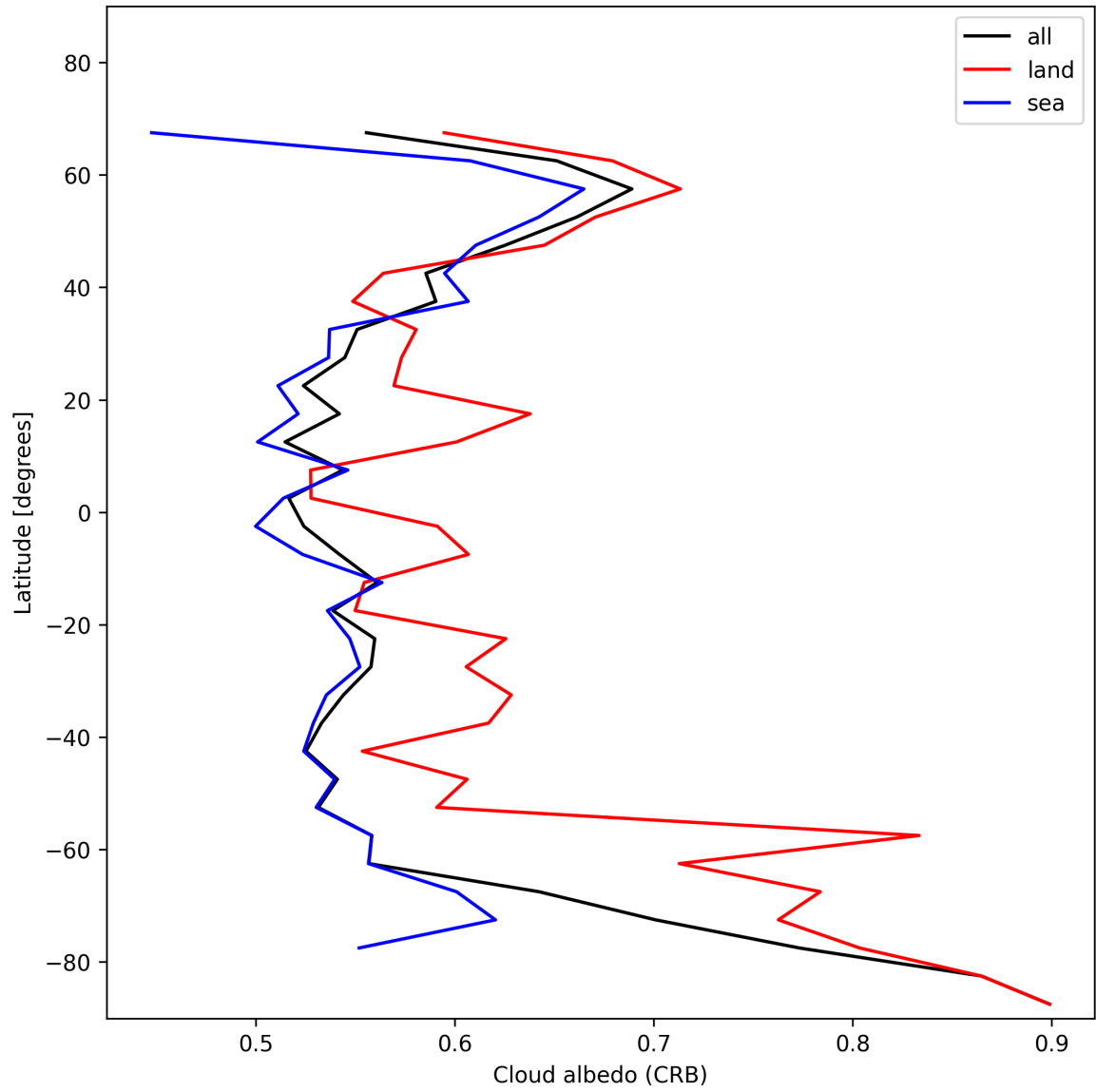
Figure 28: Zonal average of “Cloud albedo (CRB)” for 2024-12-25 to 2024-12-27.
