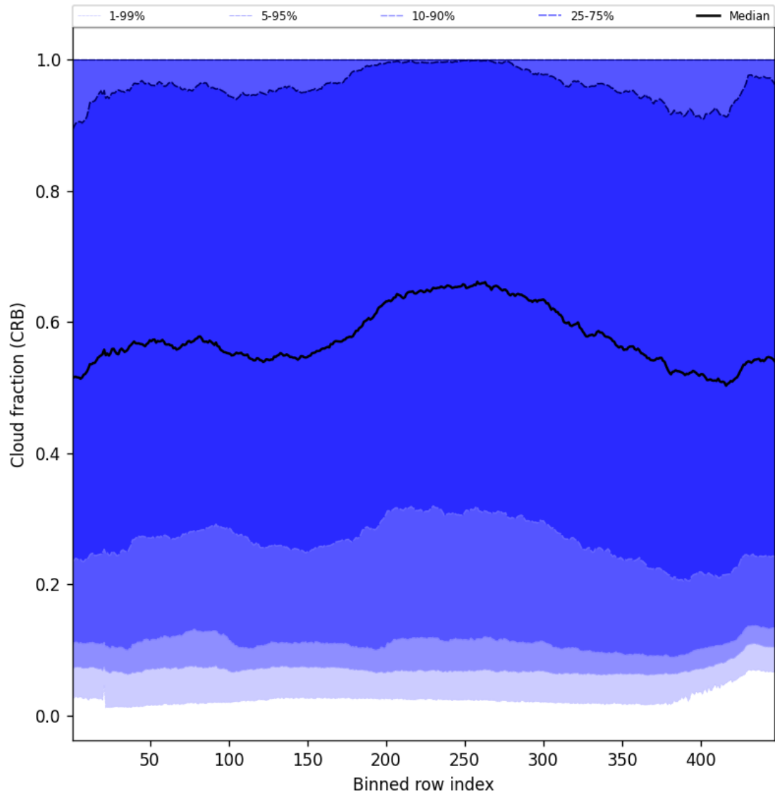
Figure 58: Along track statistics of “Cloud fraction (CRB)” for 2024-12-25 to 2024-12-27
