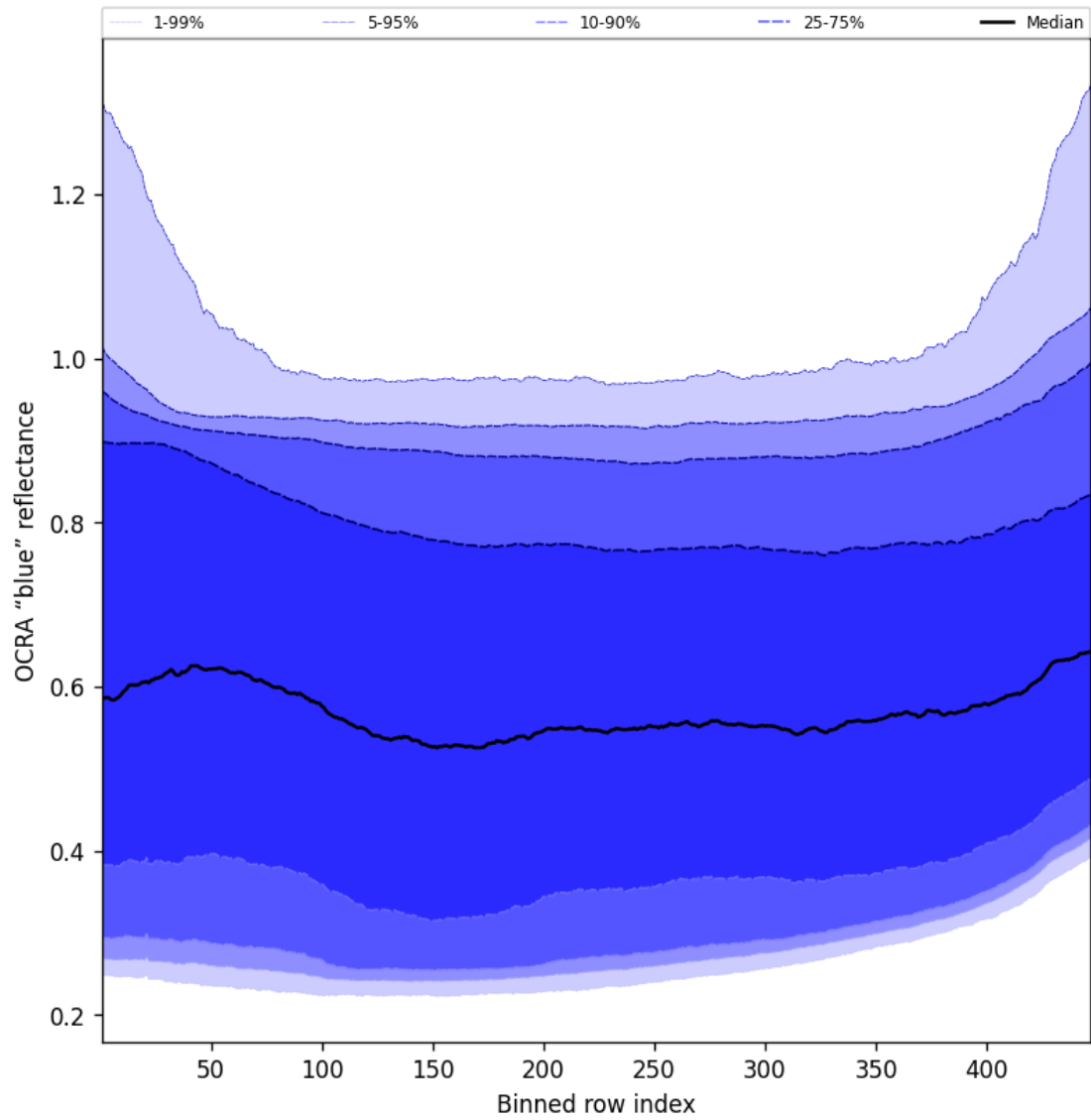
Figure 67: Along track statistics of “OCRA “blue” reflectance” for 2024-12-25 to 2024-12-27
