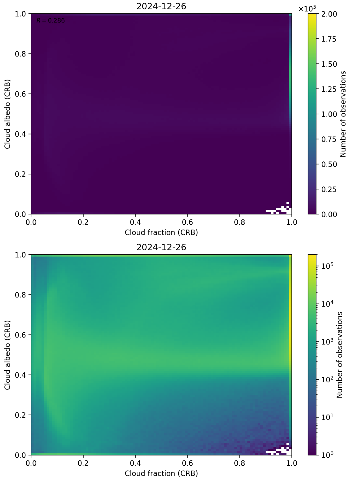
Figure 77: Scatter density plot of “Cloud fraction (CRB)” against “Cloud albedo (CRB)” for 2024-12-25 to 2024-12-27.
