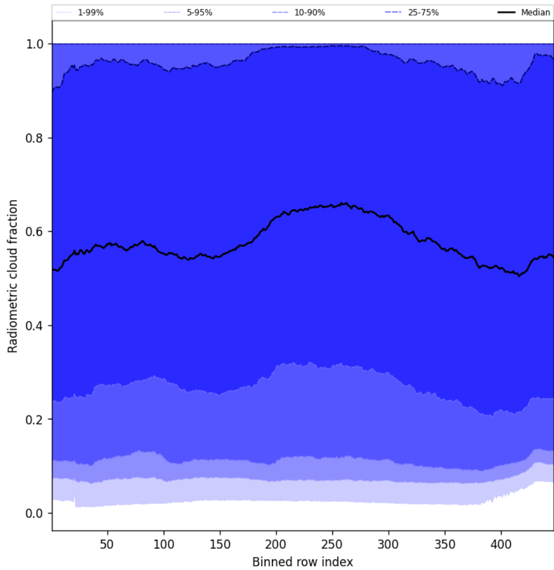
Figure 55: Along track statistics of “Radiometric cloud fraction” for 2024-12-25 to 2024-12-27
