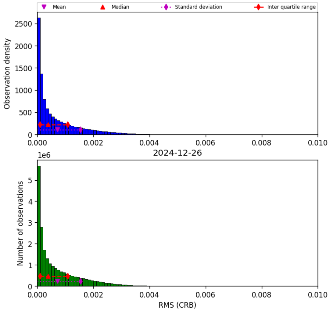
Figure 48: Histogram of “RMS (CRB)” for 2024-12-25 to 2024-12-27
