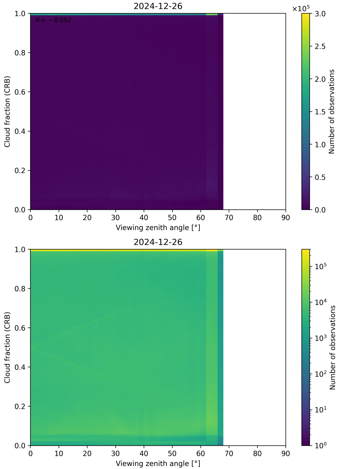
Figure 109: Scatter density plot of “Viewing zenith angle” against “Cloud fraction (CRB)” for 2024-12-25 to 2024-12-27.
