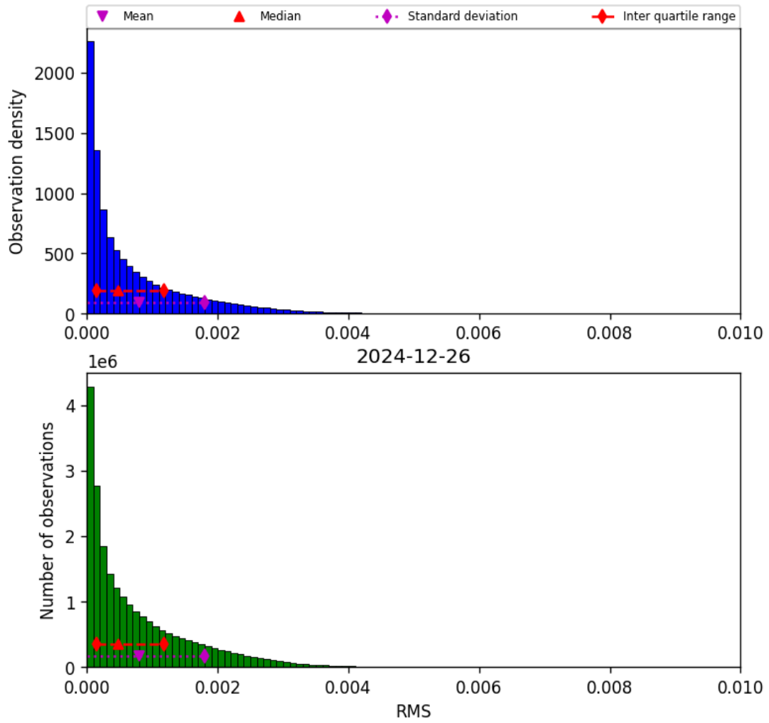
Figure 47: Histogram of “RMS” for 2024-12-25 to 2024-12-27
