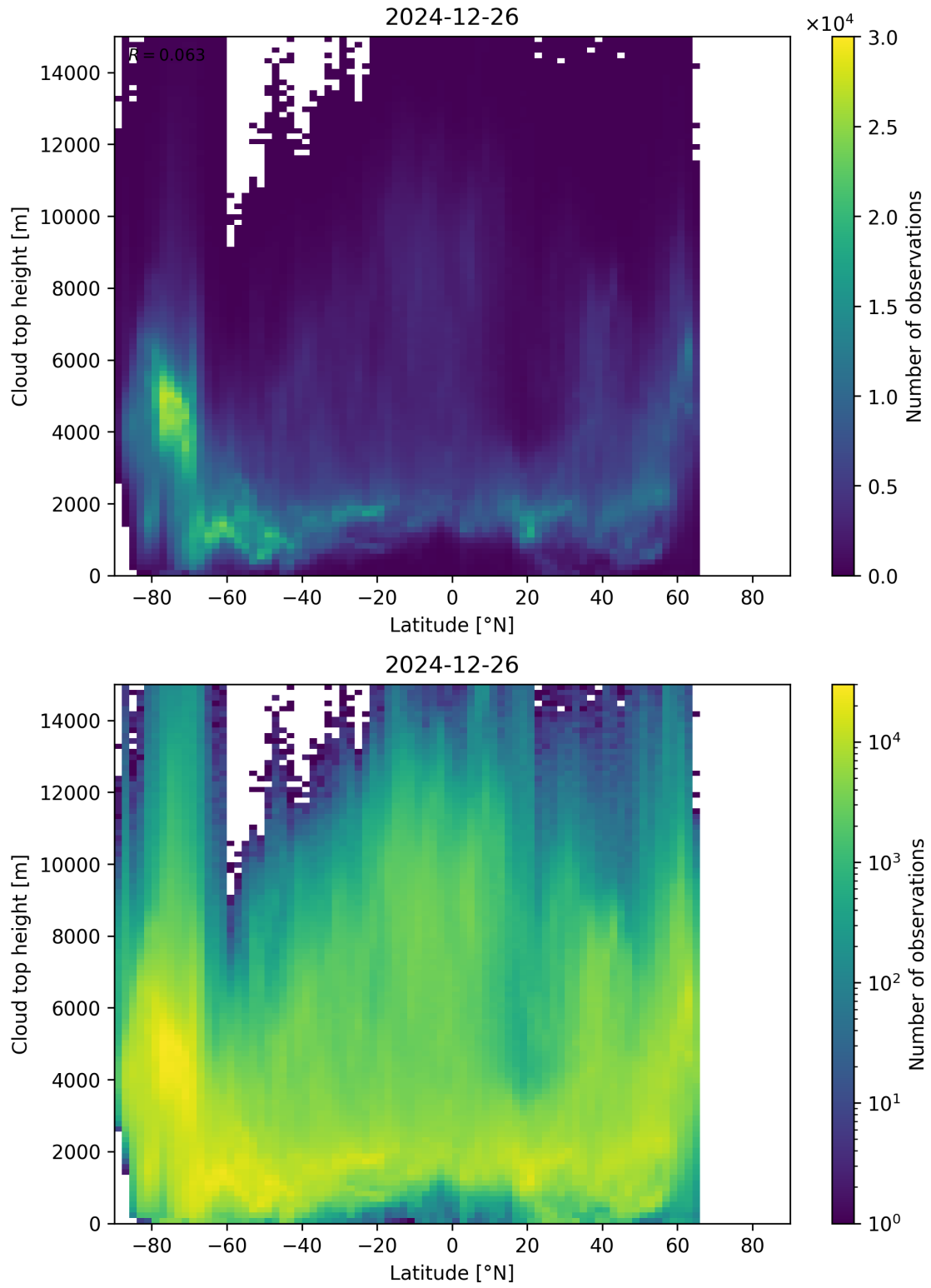
Figure 97: Scatter density plot of “Latitude” against “Cloud top height” for 2024-12-25 to 2024-12-27.
