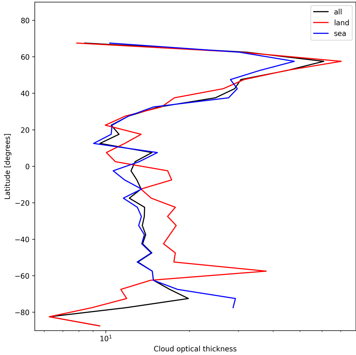
Figure 25: Zonal average of “Cloud optical thickness” for 2024-12-25 to 2024-12-27.
