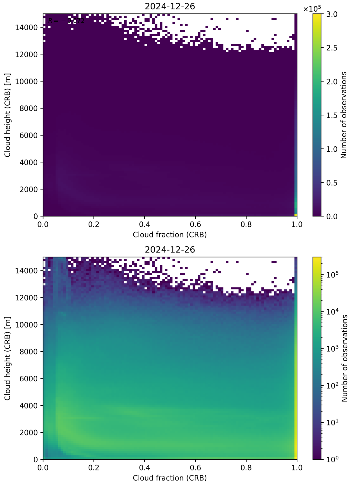
Figure 79: Scatter density plot of “Cloud fraction (CRB)” against “Cloud height (CRB)” for 2024-12-25 to 2024-12-27.
