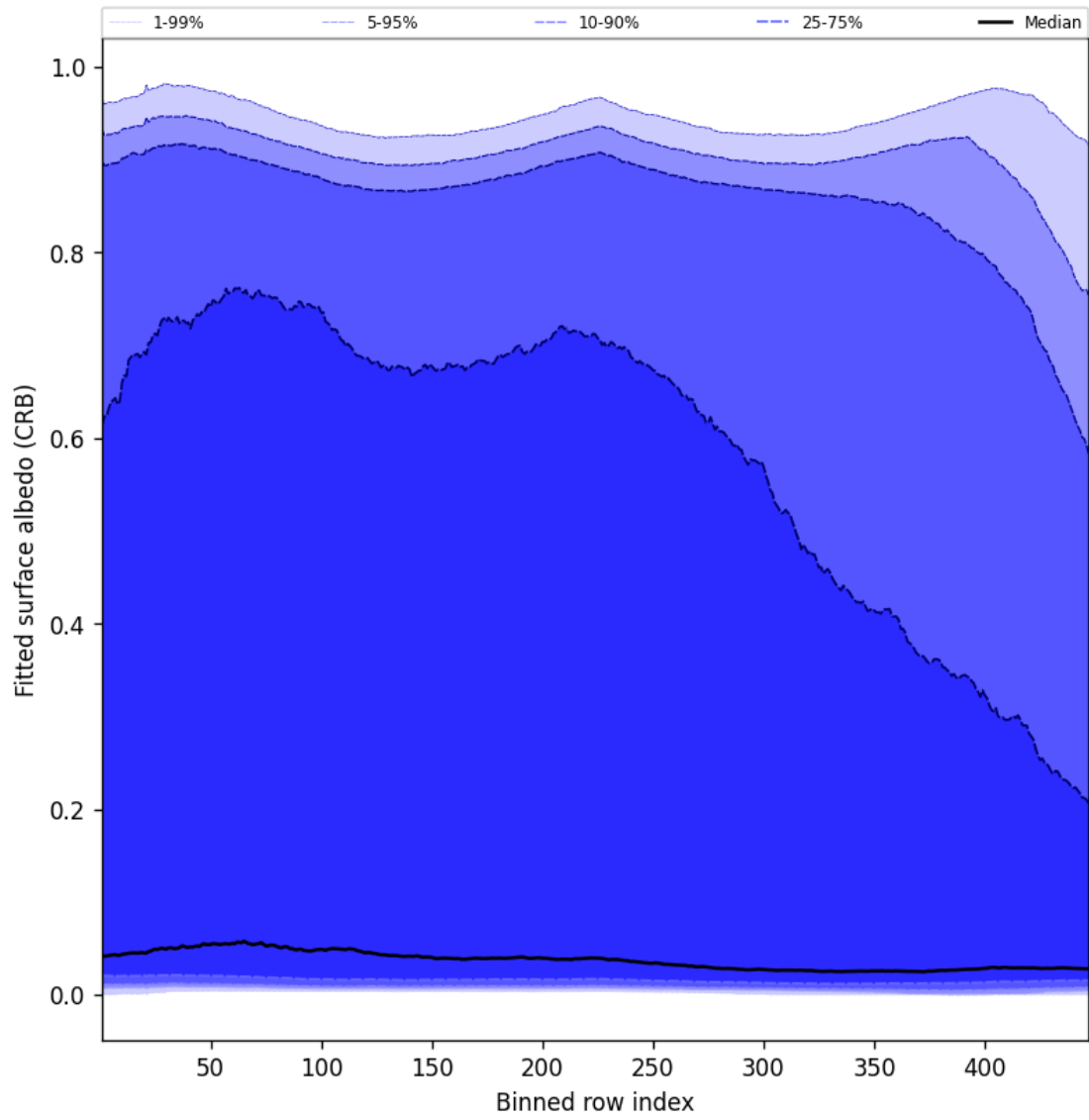
Figure 62: Along track statistics of “Fitted surface albedo (CRB)” for 2024-12-25 to 2024-12-27
