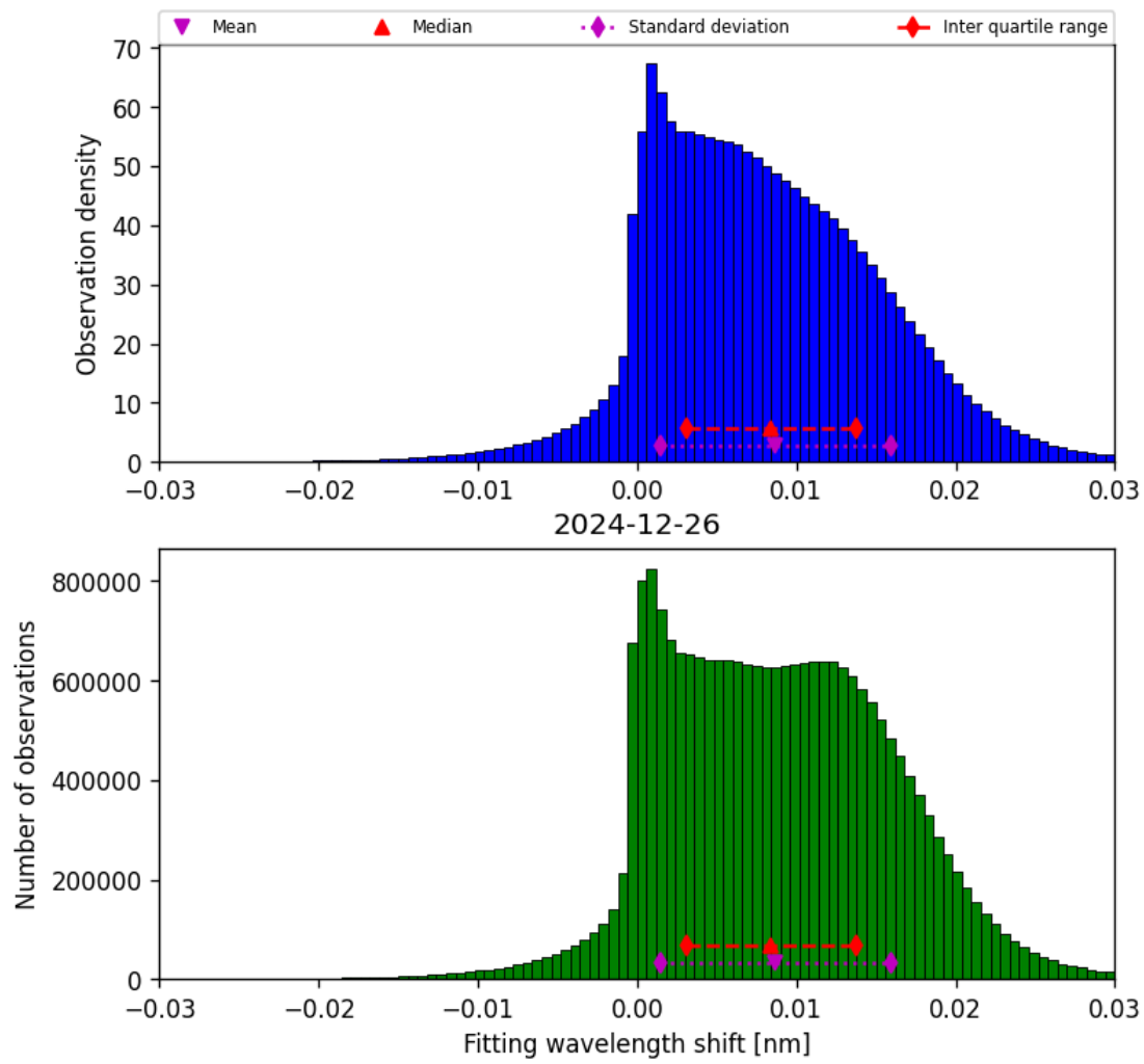
Figure 49: Histogram of “Fitting wavelength shift” for 2024-12-25 to 2024-12-27
