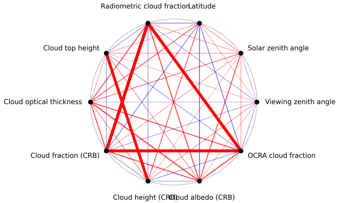
Figure 1: Map of correlation graph for 2024-12-25 to 2024-12-27.
