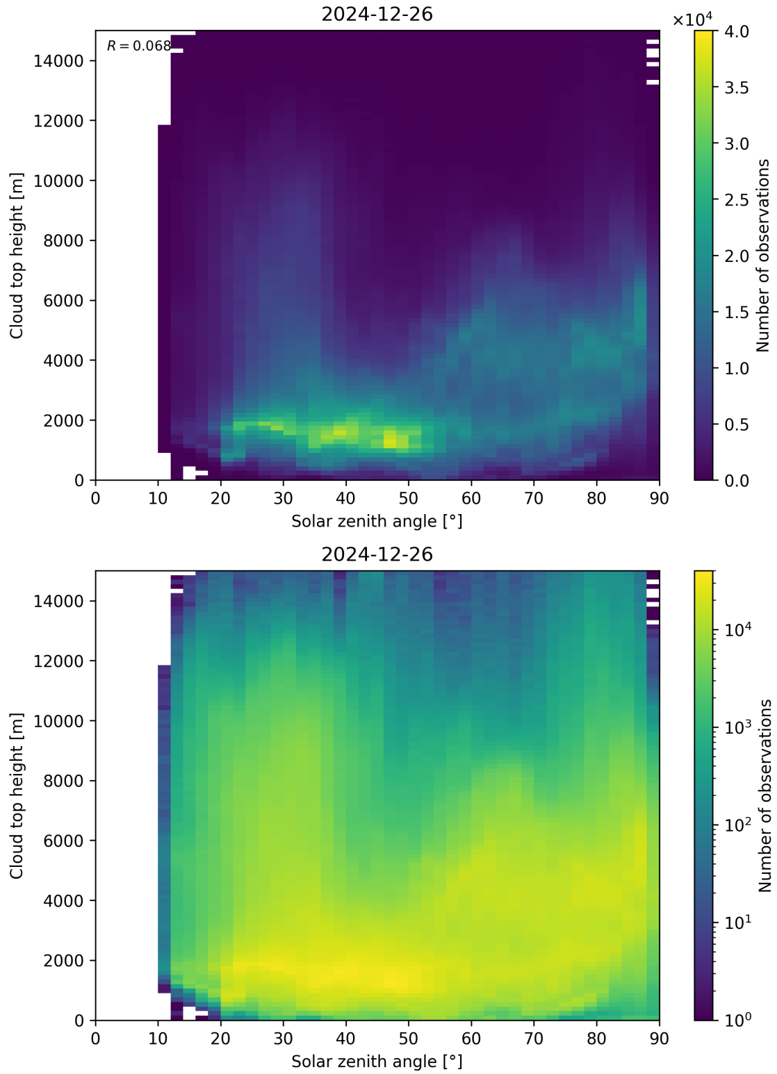
Figure 104: Scatter density plot of “Solar zenith angle” against “Cloud top height” for 2024-12-25 to 2024-12-27.
