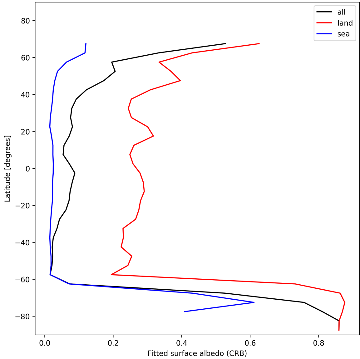
Figure 30: Zonal average of “Fitted surface albedo (CRB)” for 2024-12-25 to 2024-12-27.
