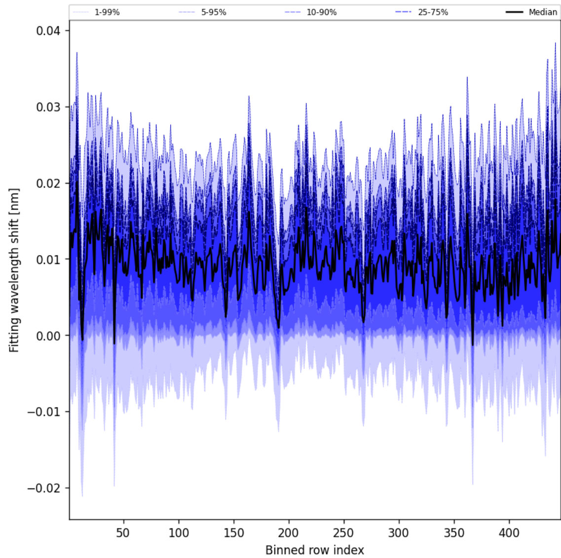
Figure 65: Along track statistics of “Fitting wavelength shift” for 2024-12-25 to 2024-12-27
