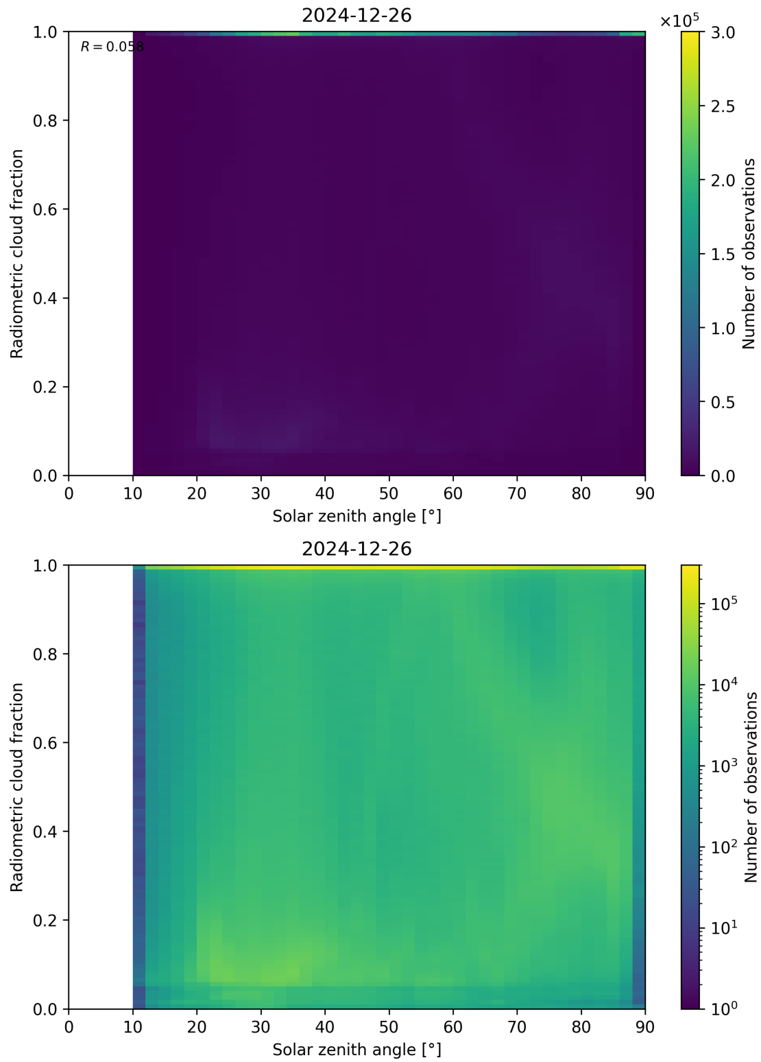
Figure 99: Scatter density plot of “Solar zenith angle” against “Radiometric cloud fraction” for 2024-12-25 to 2024-12-27.
