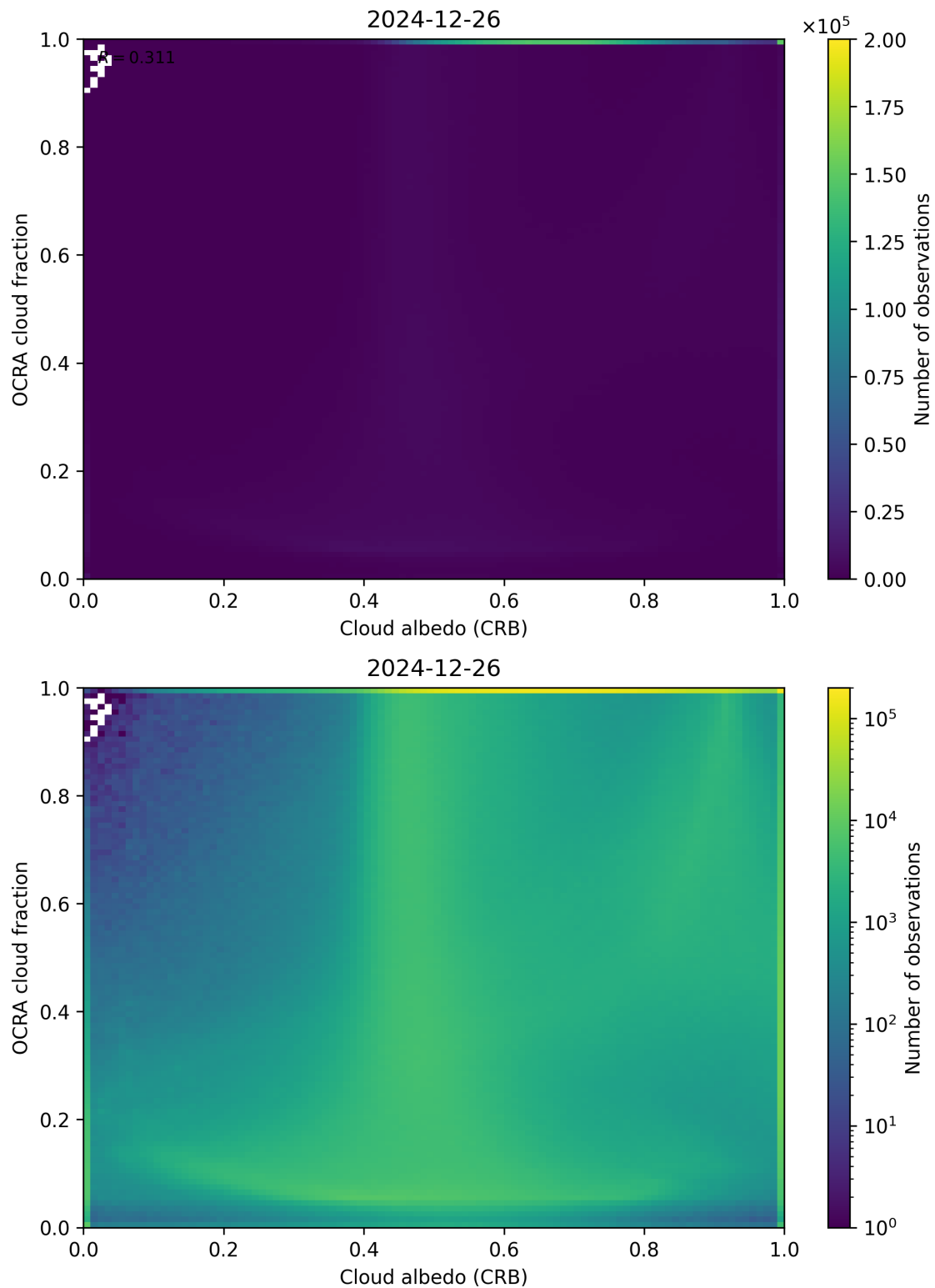
Figure 70: Scatter density plot of “Cloud albedo (CRB)” against “OCRA cloud fraction” for 2024-12-25 to 2024-12-27.
