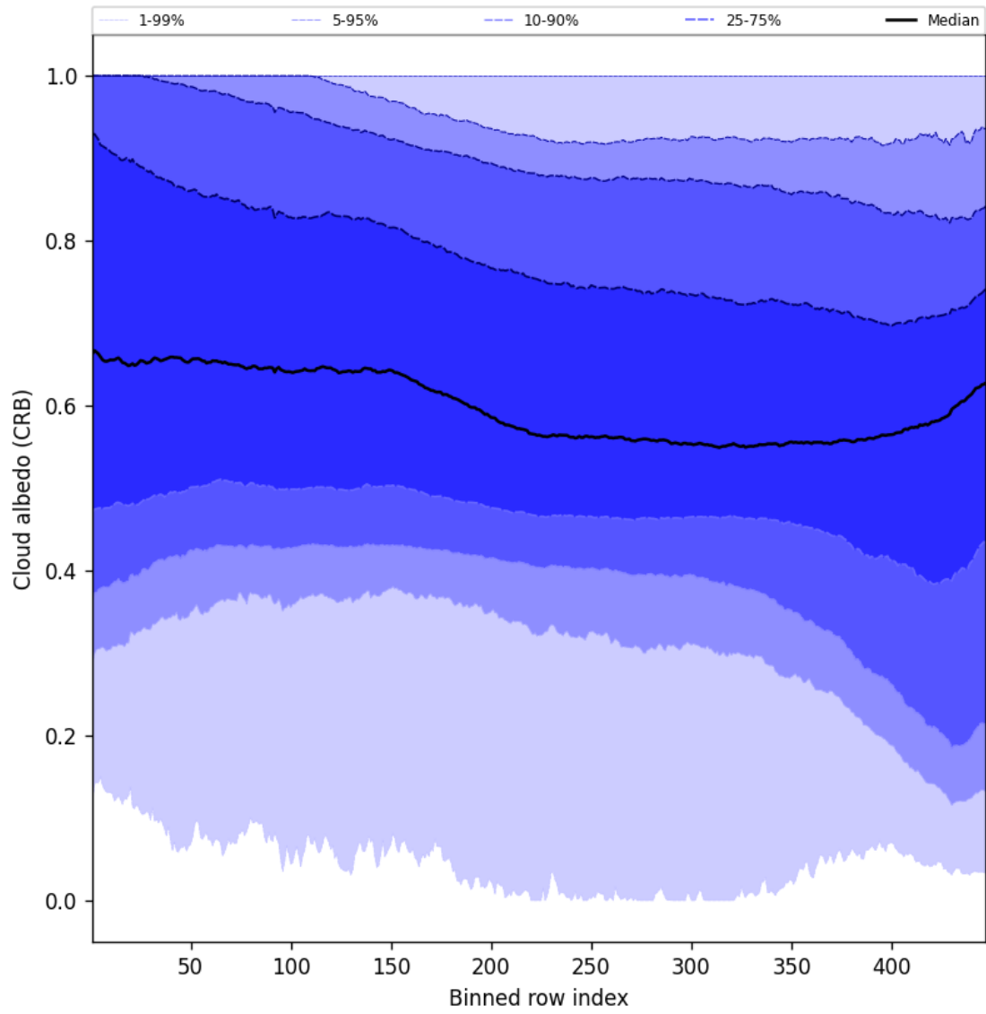
Figure 60: Along track statistics of “Cloud albedo (CRB)” for 2024-12-25 to 2024-12-27
