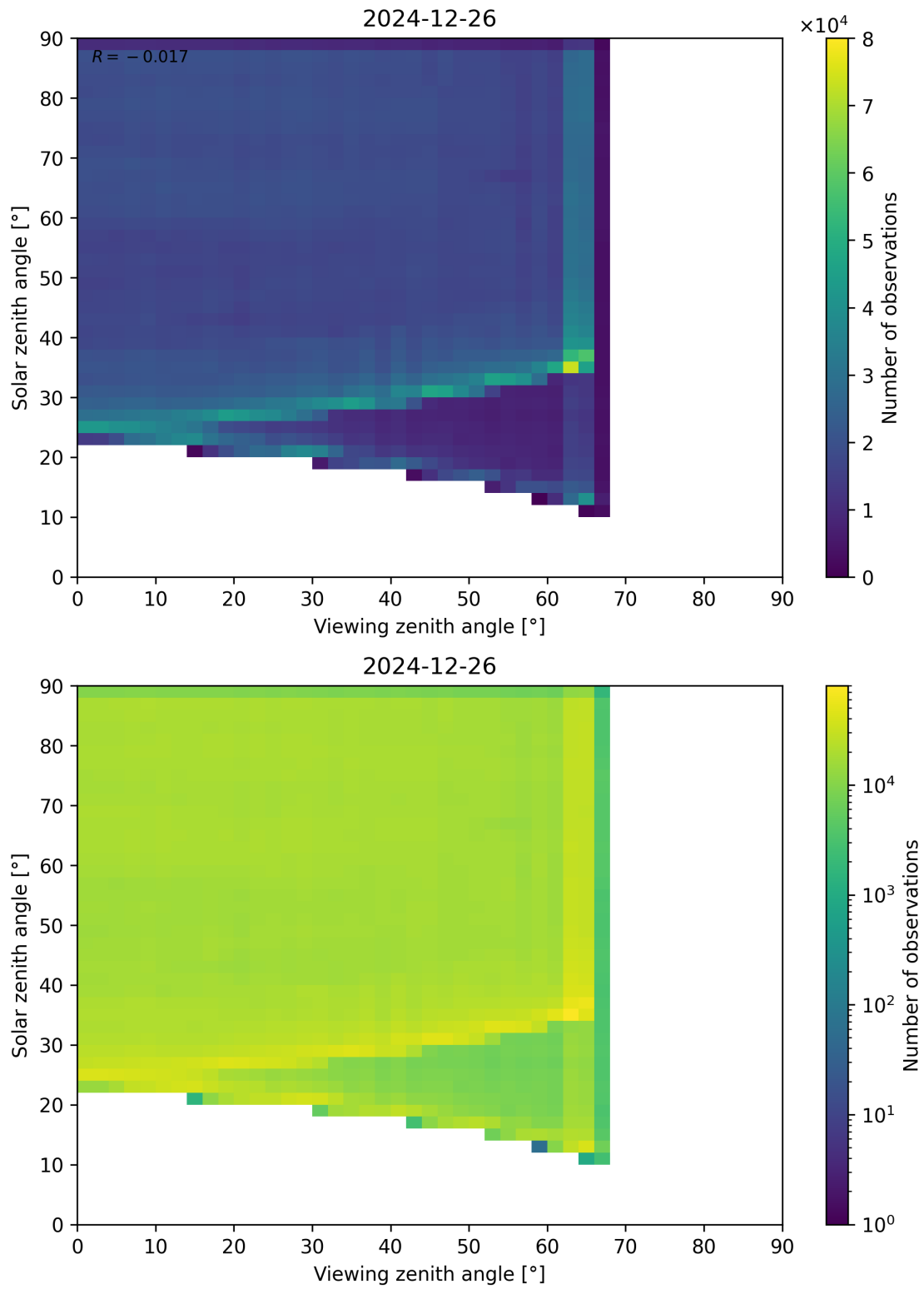
Figure 114: Scatter density plot of “Viewing zenith angle” against “Solar zenith angle” for 2024-12-25 to 2024-12-27.
