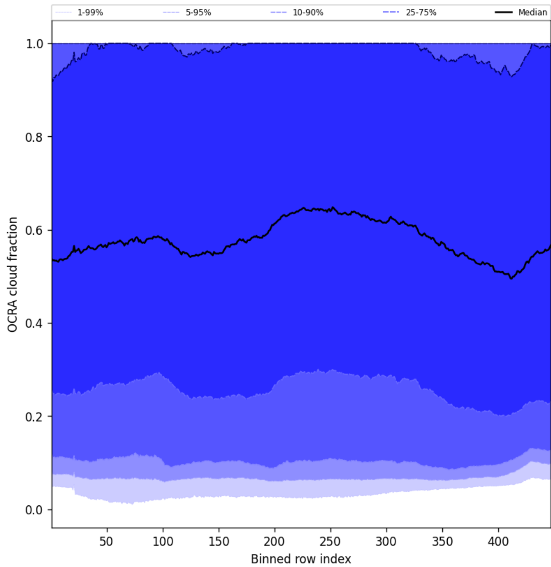
Figure 66: Along track statistics of “OCRA cloud fraction” for 2024-12-27 to 2024-12-28
