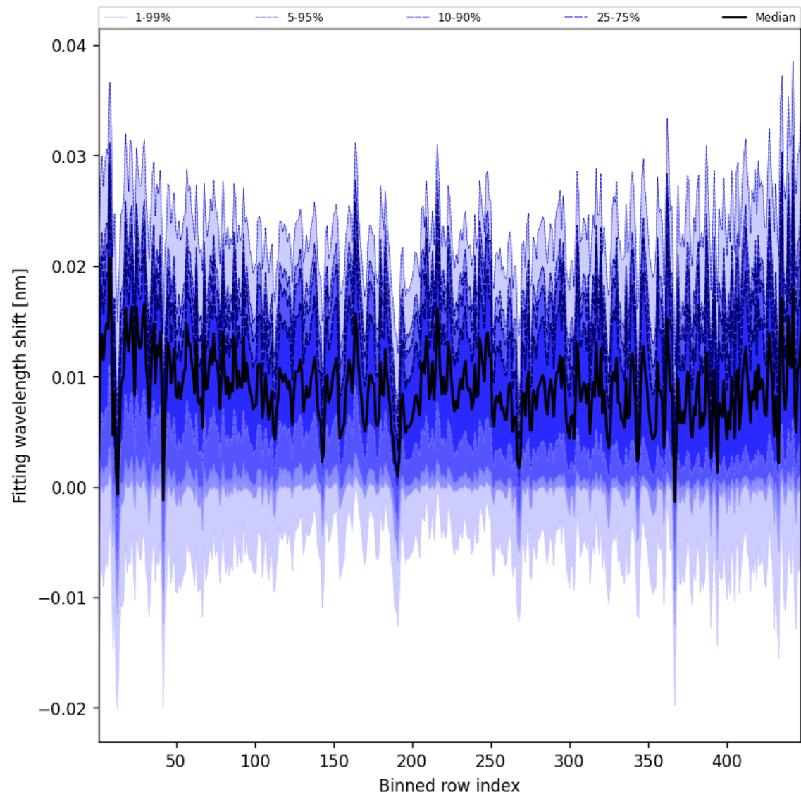
Figure 65: Along track statistics of “Fitting wavelength shift” for 2024-12-27 to 2024-12-28
