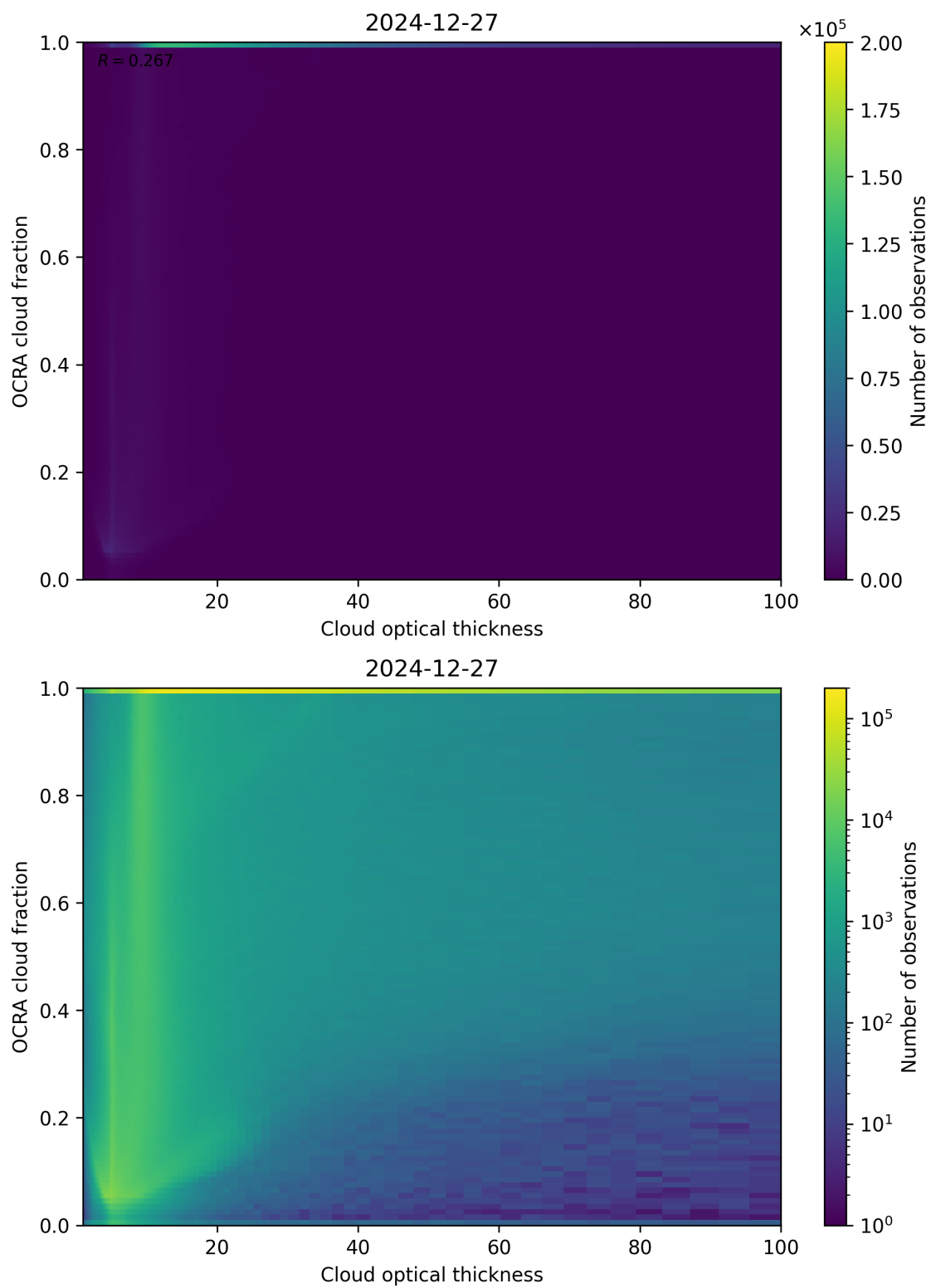
Figure 83: Scatter density plot of “Cloud optical thickness” against “OCRA cloud fraction” for 2024-12-27 to 2024-12-28.
