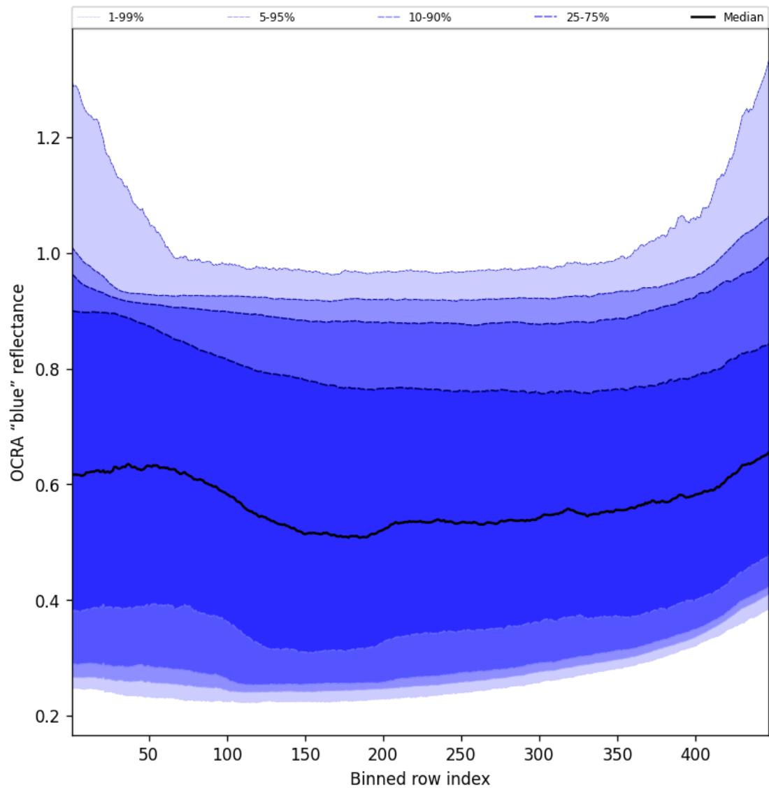
Figure 67: Along track statistics of “OCRA “blue” reflectance” for 2024-12-27 to 2024-12-28
