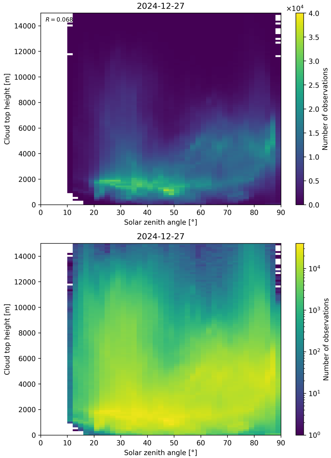
Figure 104: Scatter density plot of “Solar zenith angle” against “Cloud top height” for 2024-12-27 to 2024-12-28.
