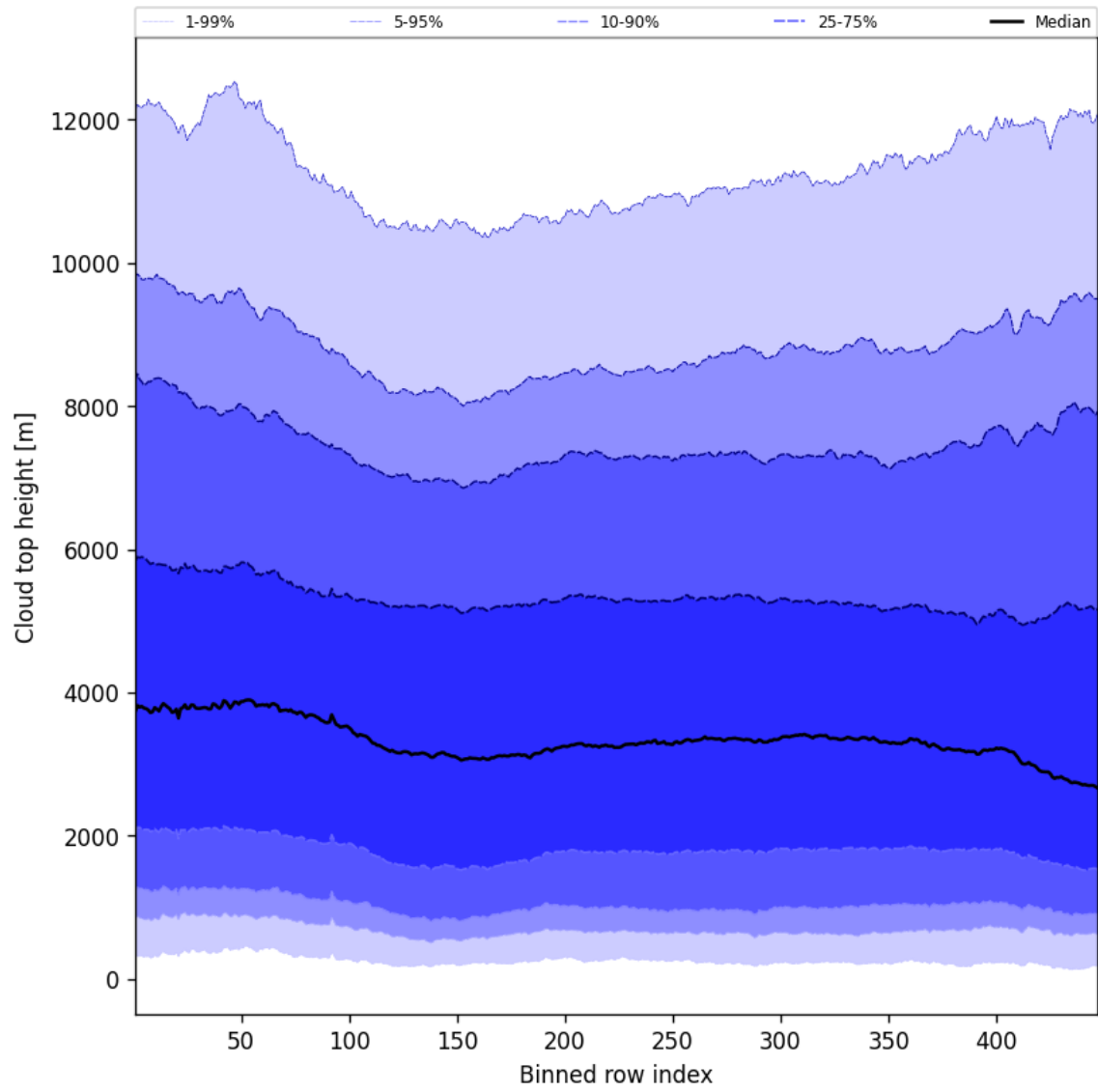
Figure 56: Along track statistics of “Cloud top height” for 2024-12-27 to 2024-12-28
