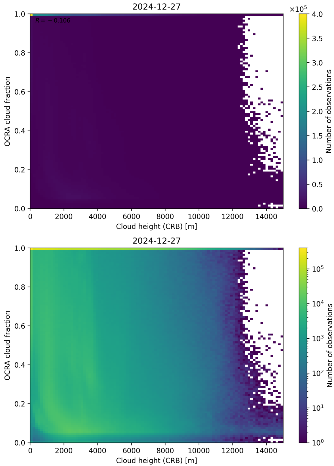
Figure 81: Scatter density plot of “Cloud height (CRB)” against “OCRA cloud fraction” for 2024-12-27 to 2024-12-28.
