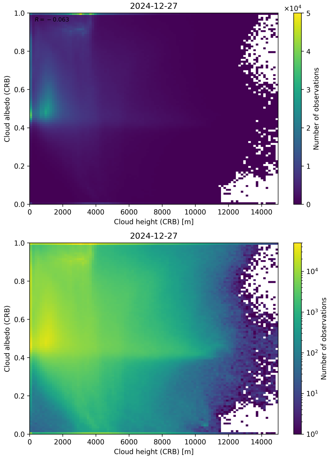
Figure 80: Scatter density plot of “Cloud height (CRB)” against “Cloud albedo (CRB)” for 2024-12-27 to 2024-12-28.
