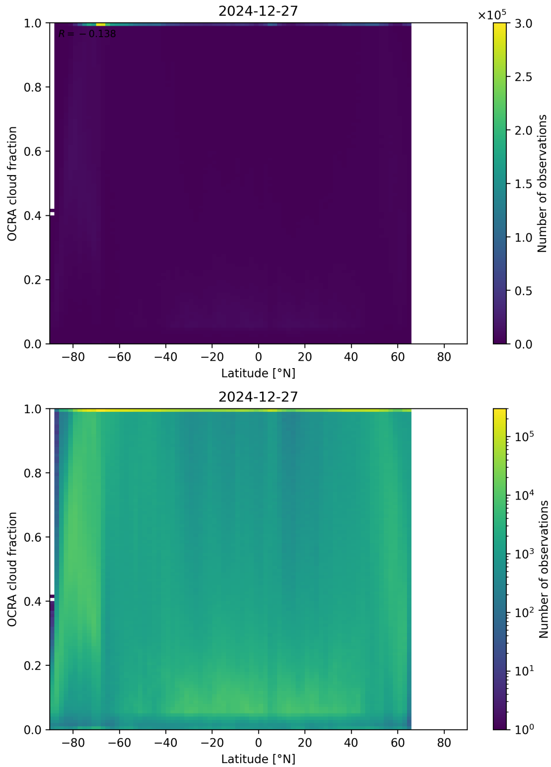
Figure 93: Scatter density plot of “Latitude” against “OCRA cloud fraction” for 2024-12-27 to 2024-12-28.
