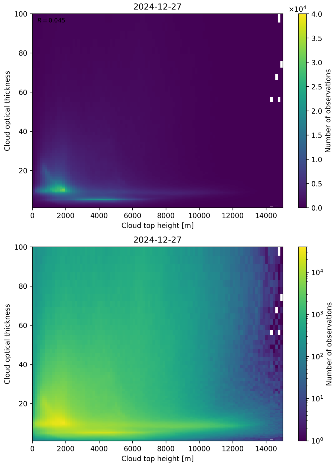
Figure 90: Scatter density plot of “Cloud top height” against “Cloud optical thickness” for 2024-12-27 to 2024-12-28.
