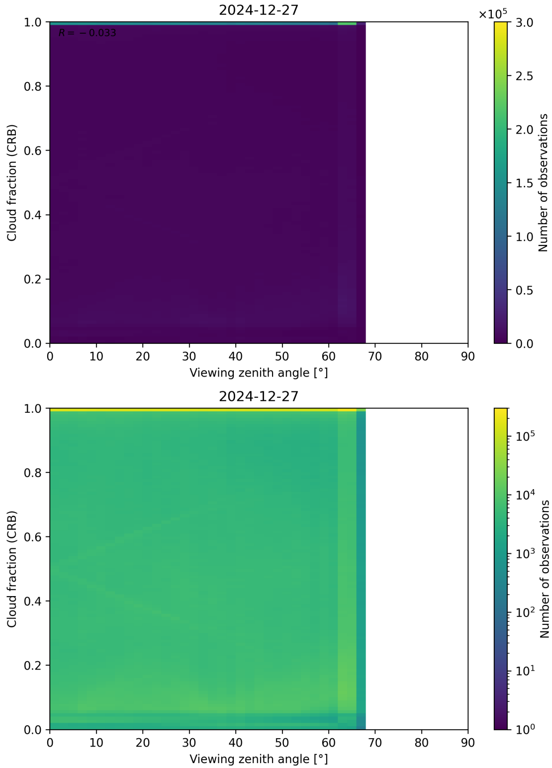
Figure 109: Scatter density plot of “Viewing zenith angle” against “Cloud fraction (CRB)” for 2024-12-27 to 2024-12-28.
