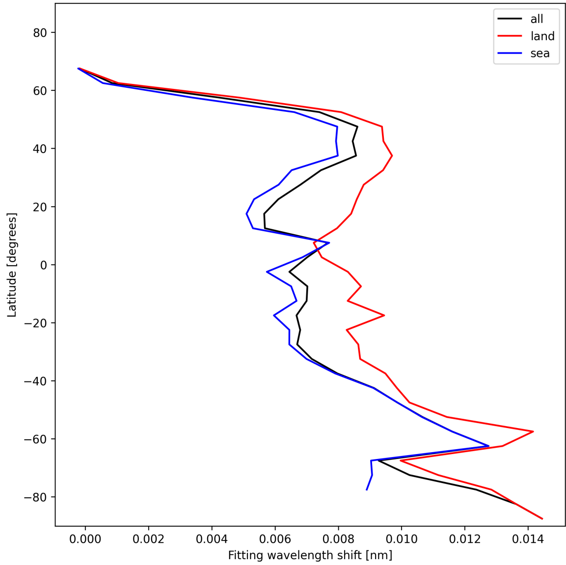
Figure 33: Zonal average of “Fitting wavelength shift” for 2024-12-27 to 2024-12-28.
