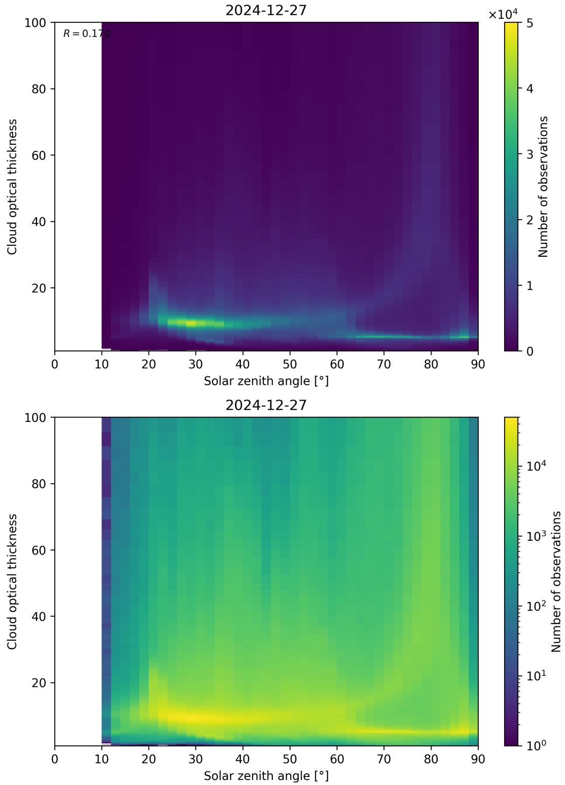
Figure 103: Scatter density plot of “Solar zenith angle” against “Cloud optical thickness” for 2024-12-27 to 2024-12-28.
