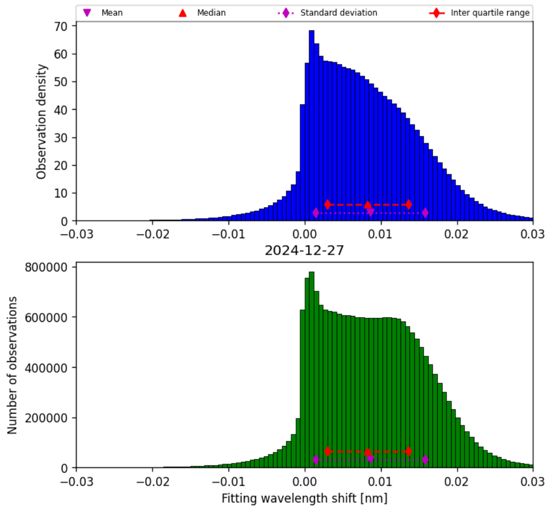
Figure 49: Histogram of “Fitting wavelength shift” for 2024-12-27 to 2024-12-28
