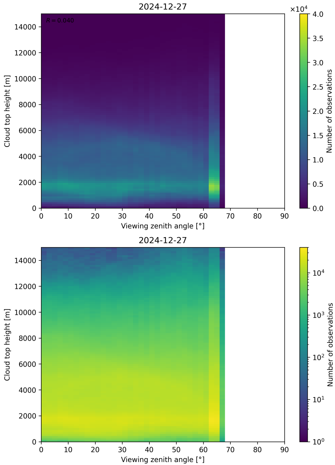
Figure 112: Scatter density plot of “Viewing zenith angle” against “Cloud top height” for 2024-12-27 to 2024-12-28.
