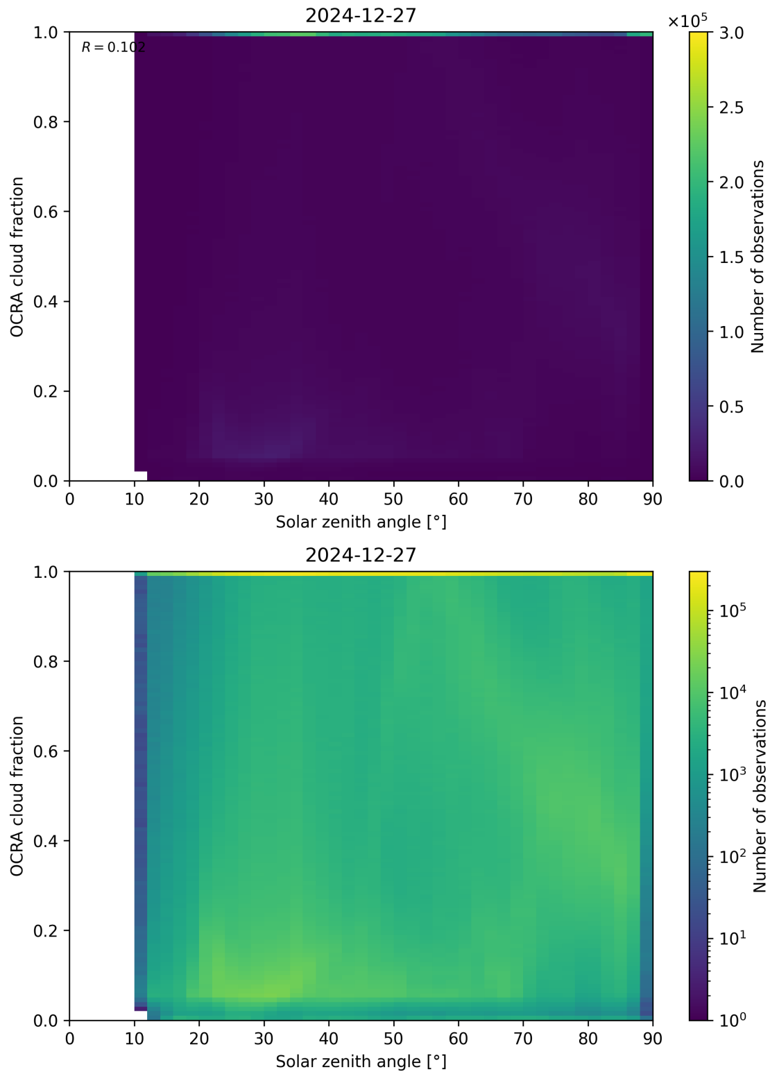
Figure 100: Scatter density plot of “Solar zenith angle” against “OCRA cloud fraction” for 2024-12-27 to 2024-12-28.
