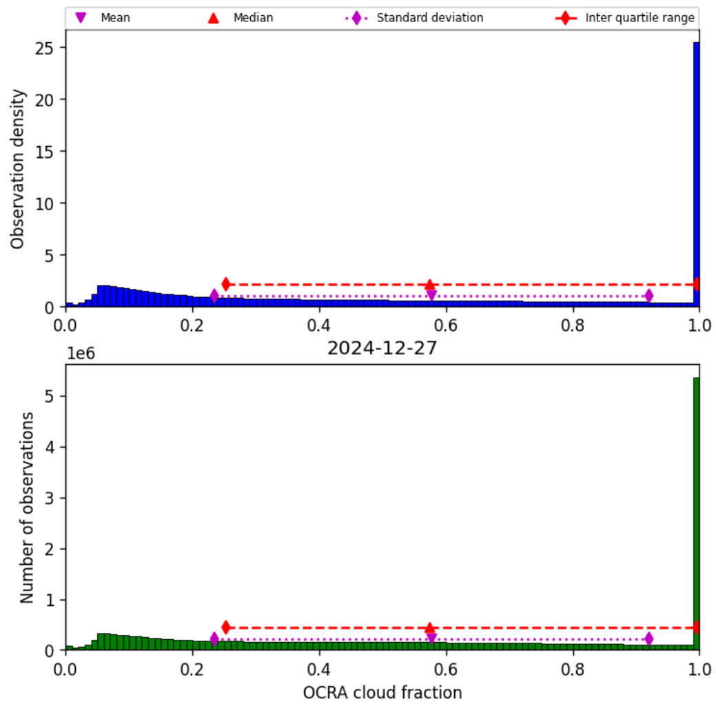
Figure 50: Histogram of “OCRA cloud fraction” for 2024-12-27 to 2024-12-28
