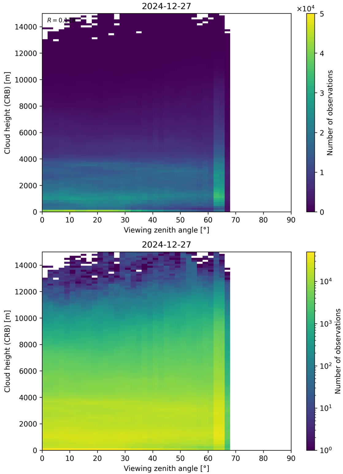
Figure 110: Scatter density plot of “Viewing zenith angle” against “Cloud height (CRB)” for 2024-12-27 to 2024-12-28.
