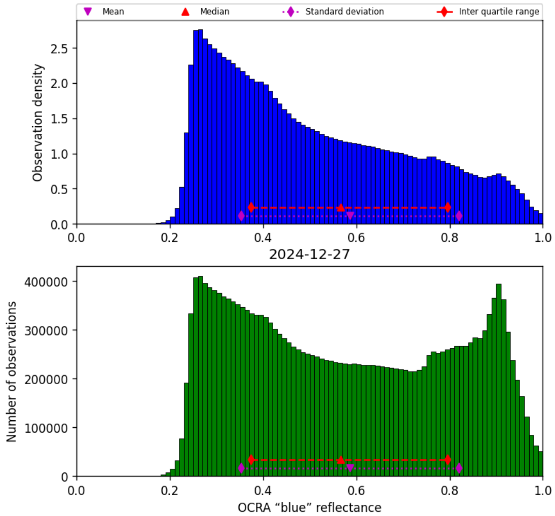
Figure 51: Histogram of “OCRA “blue” reflectance” for 2024-12-27 to 2024-12-28
