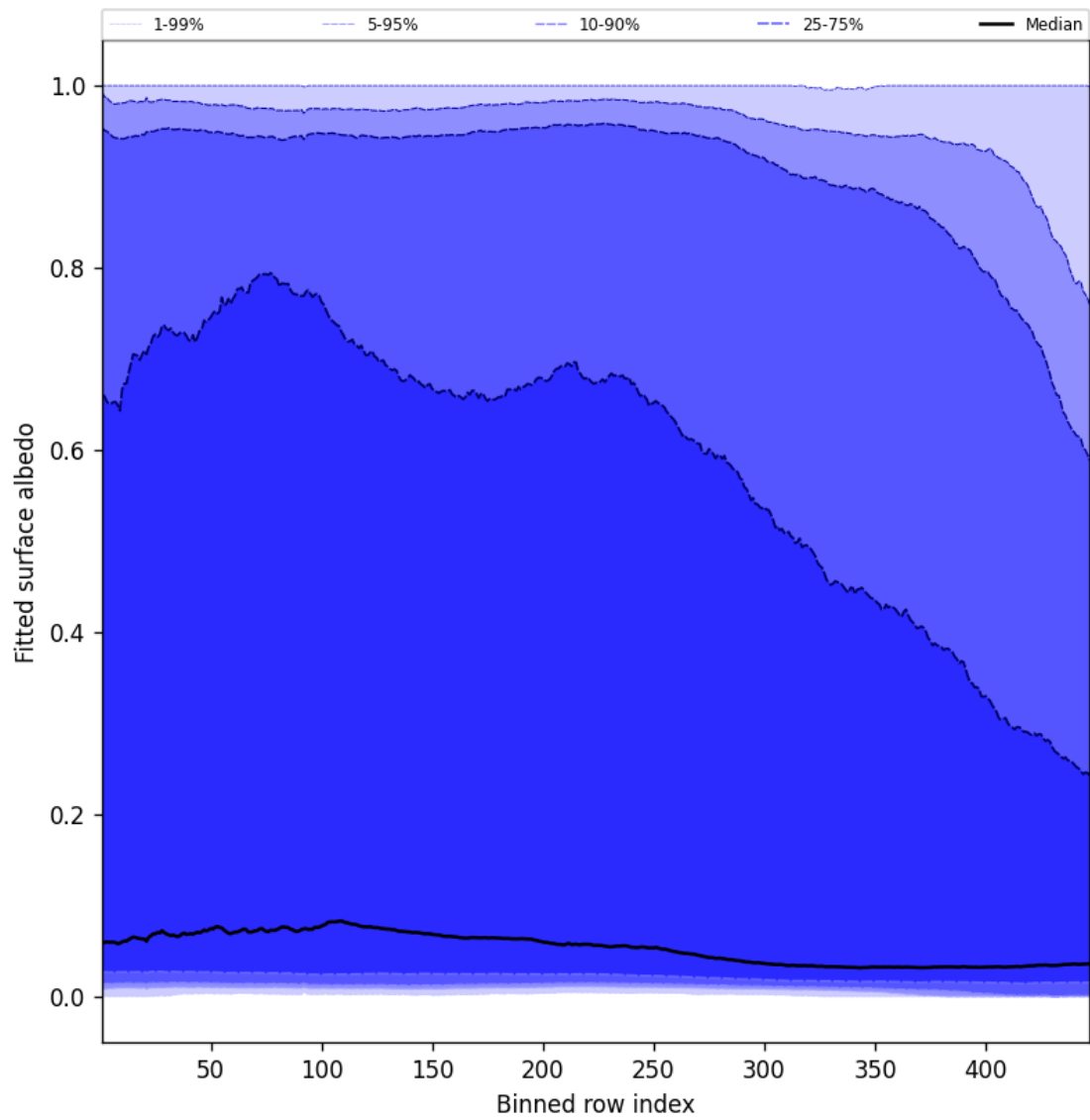
Figure 61: Along track statistics of “Fitted surface albedo” for 2024-12-27 to 2024-12-28
