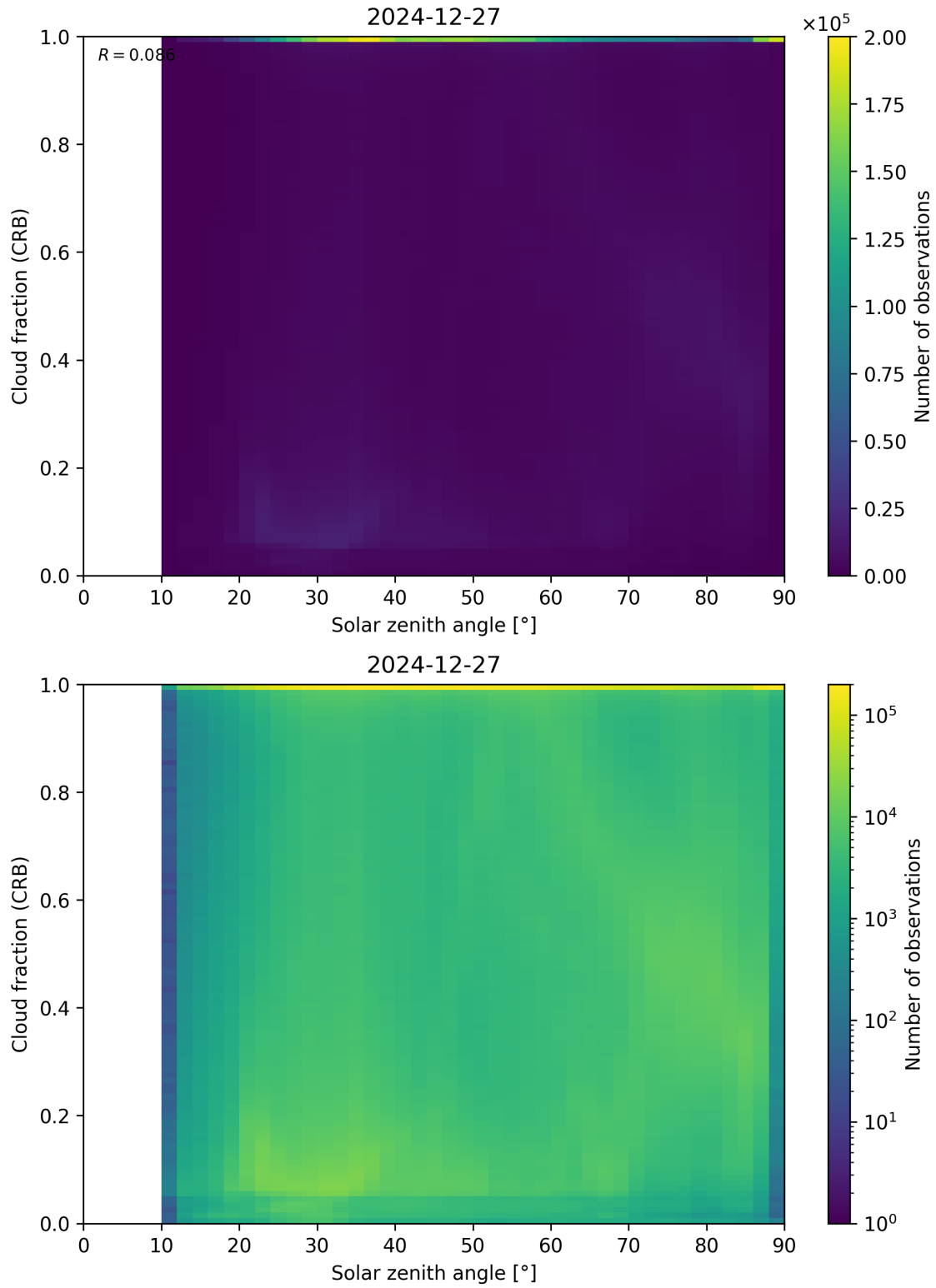
Figure 101: Scatter density plot of “Solar zenith angle” against “Cloud fraction (CRB)” for 2024-12-27 to 2024-12-28.
