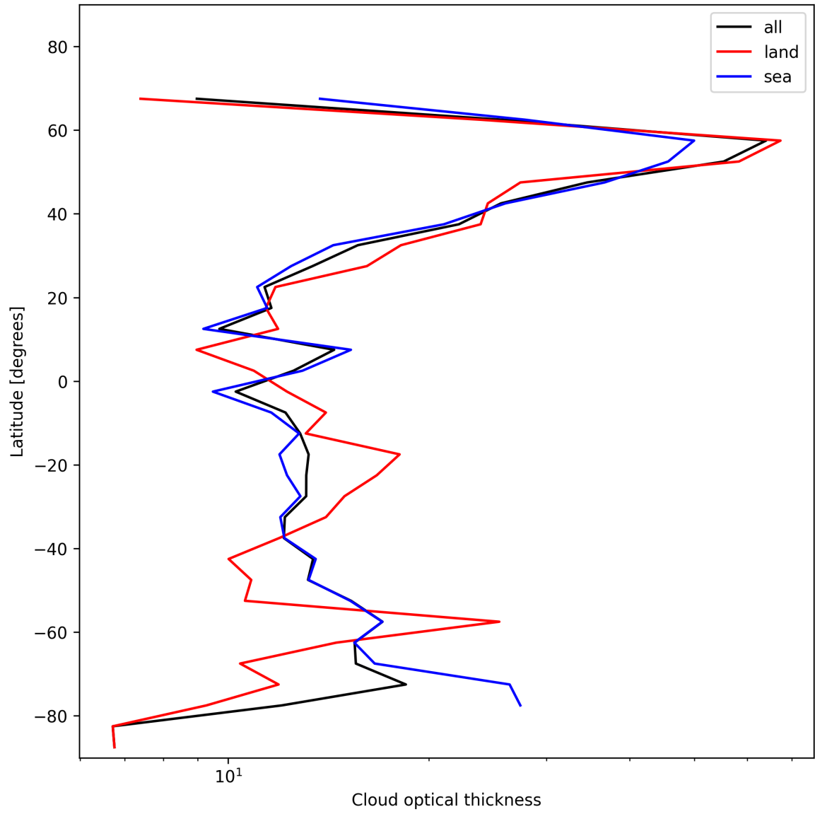
Figure 25: Zonal average of “Cloud optical thickness” for 2024-12-27 to 2024-12-28.
