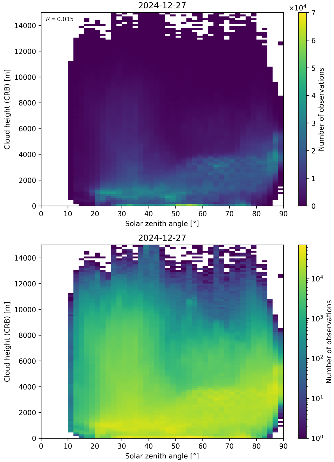
Figure 102: Scatter density plot of “Solar zenith angle” against “Cloud height (CRB)” for 2024-12-27 to 2024-12-28.
