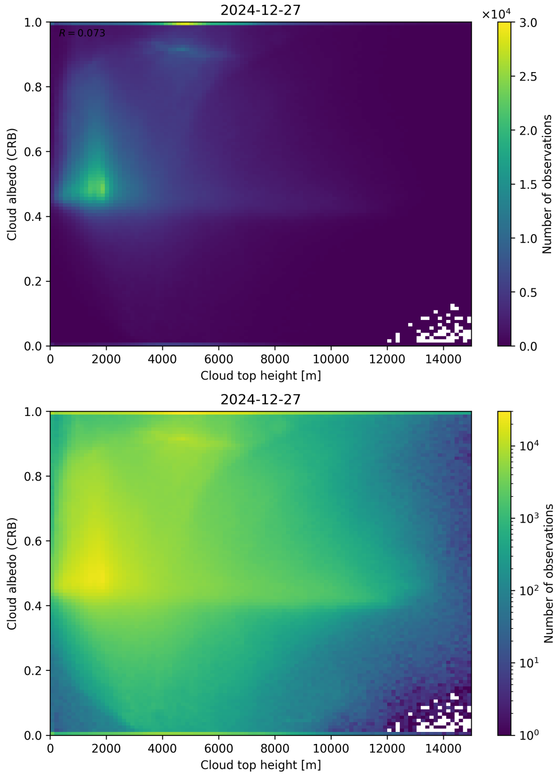
Figure 86: Scatter density plot of “Cloud top height” against “Cloud albedo (CRB)” for 2024-12-27 to 2024-12-28.
