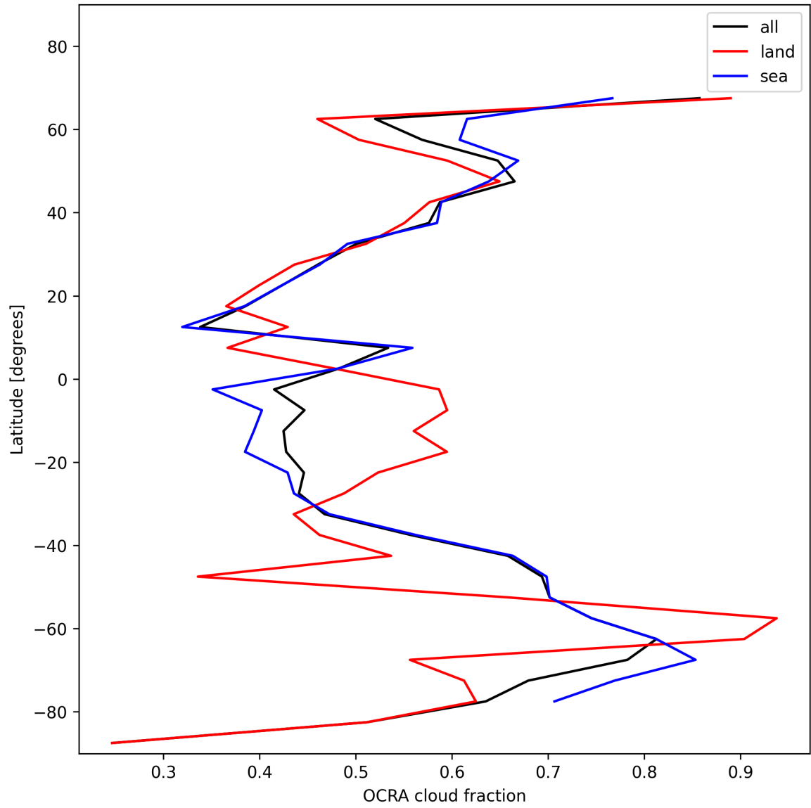
Figure 34: Zonal average of “OCRA cloud fraction” for 2024-12-27 to 2024-12-28.
