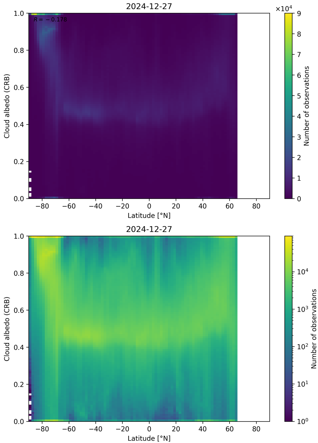
Figure 91: Scatter density plot of “Latitude” against “Cloud albedo (CRB)” for 2024-12-27 to 2024-12-28.
