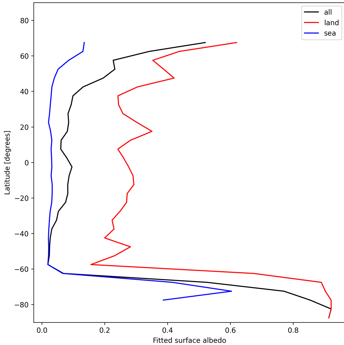
Figure 29: Zonal average of “Fitted surface albedo” for 2024-12-27 to 2024-12-28.
