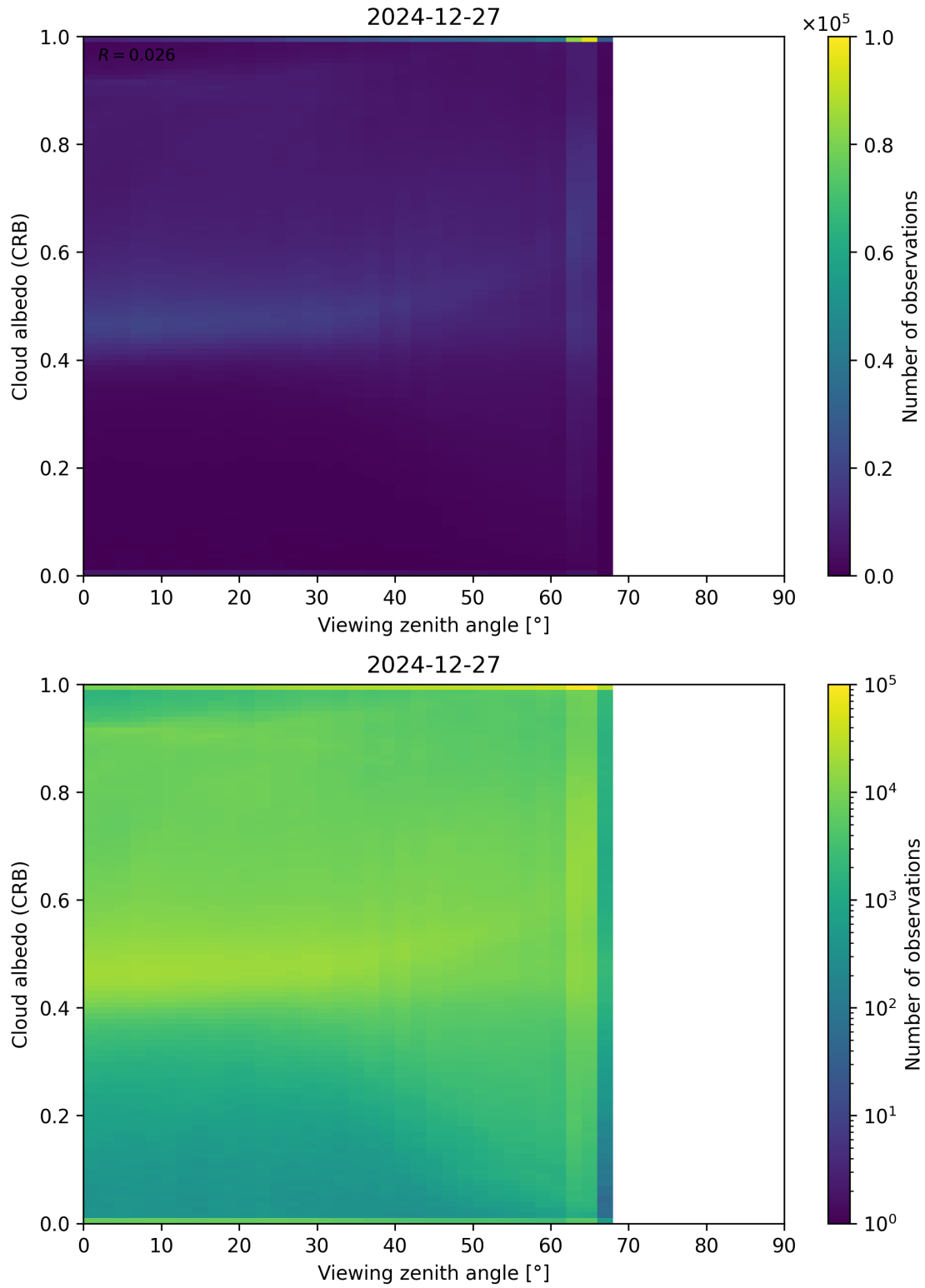
Figure 106: Scatter density plot of “Viewing zenith angle” against “Cloud albedo (CRB)” for 2024-12-27 to 2024-12-28.
