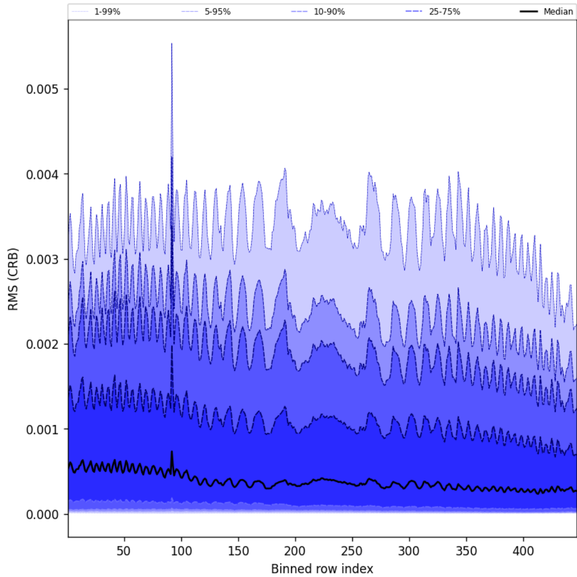
Figure 64: Along track statistics of “RMS (CRB)” for 2024-12-27 to 2024-12-28
