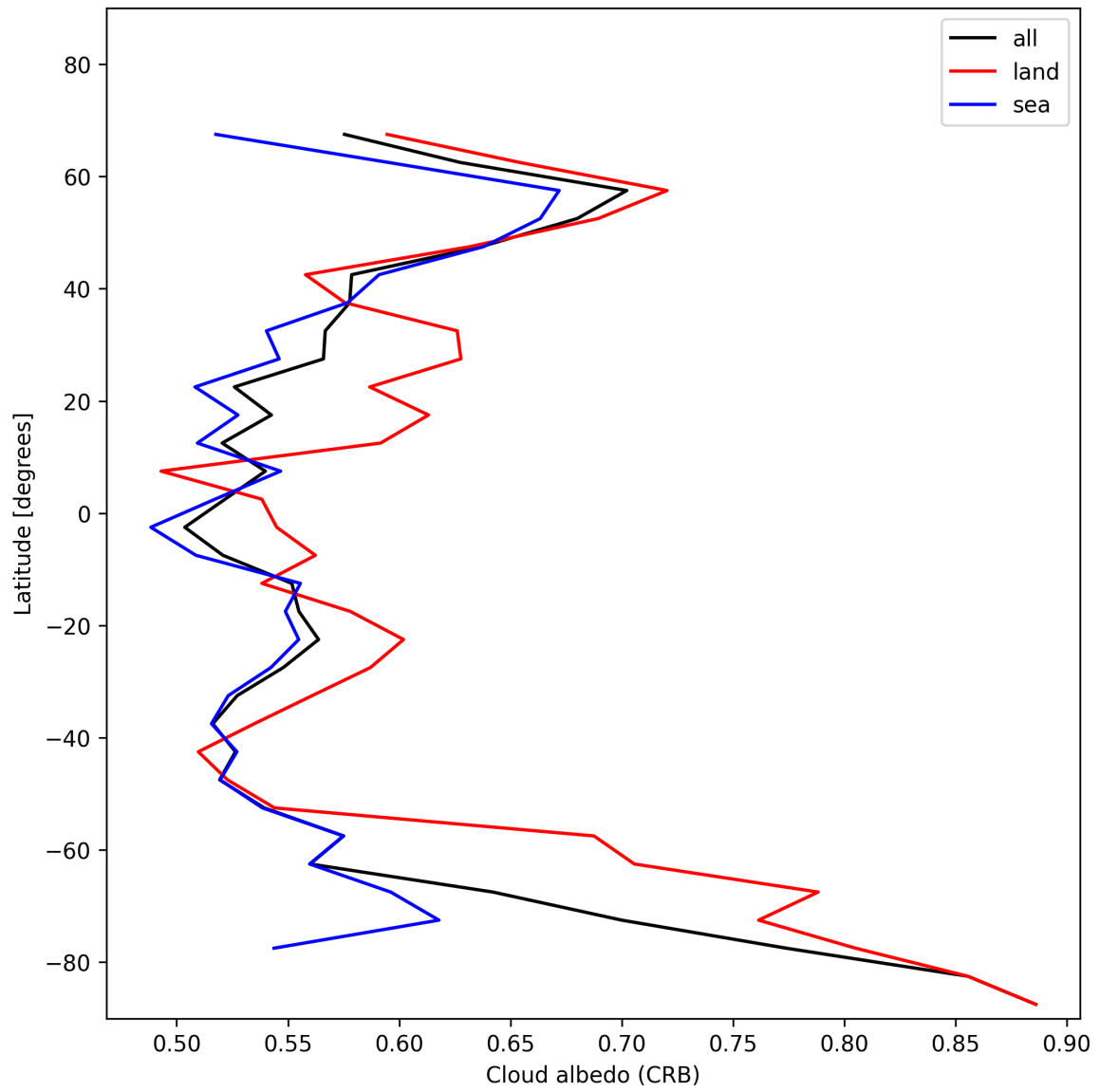
Figure 28: Zonal average of “Cloud albedo (CRB)” for 2024-12-27 to 2024-12-28.
