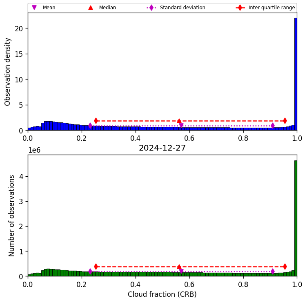
Figure 42: Histogram of “Cloud fraction (CRB)” for 2024-12-27 to 2024-12-28
