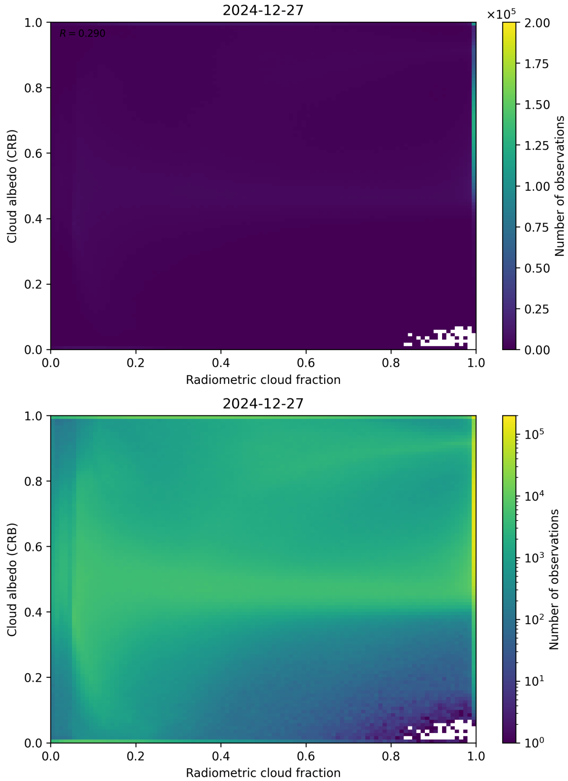
Figure 71: Scatter density plot of “Radiometric cloud fraction” against “Cloud albedo (CRB)” for 2024-12-27 to 2024-12-28.
