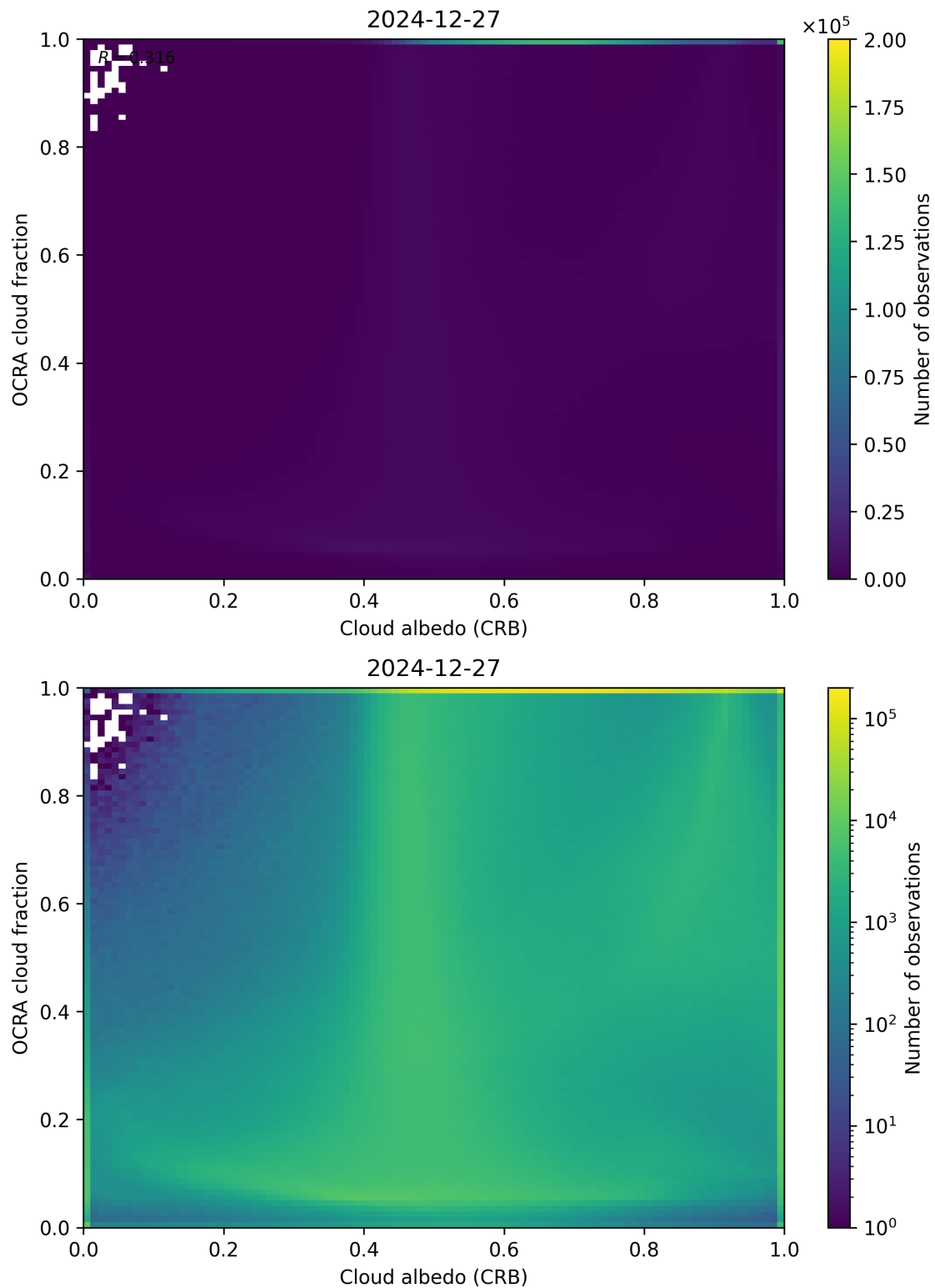
Figure 70: Scatter density plot of “Cloud albedo (CRB)” against “OCRA cloud fraction” for 2024-12-27 to 2024-12-28.
