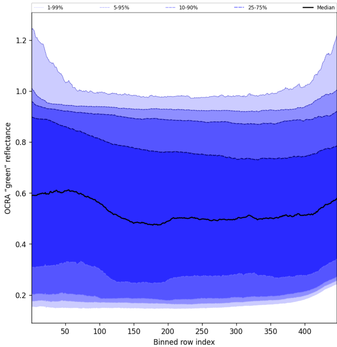
Figure 68: Along track statistics of “OCRA “green” reflectance” for 2024-12-27 to 2024-12-28
