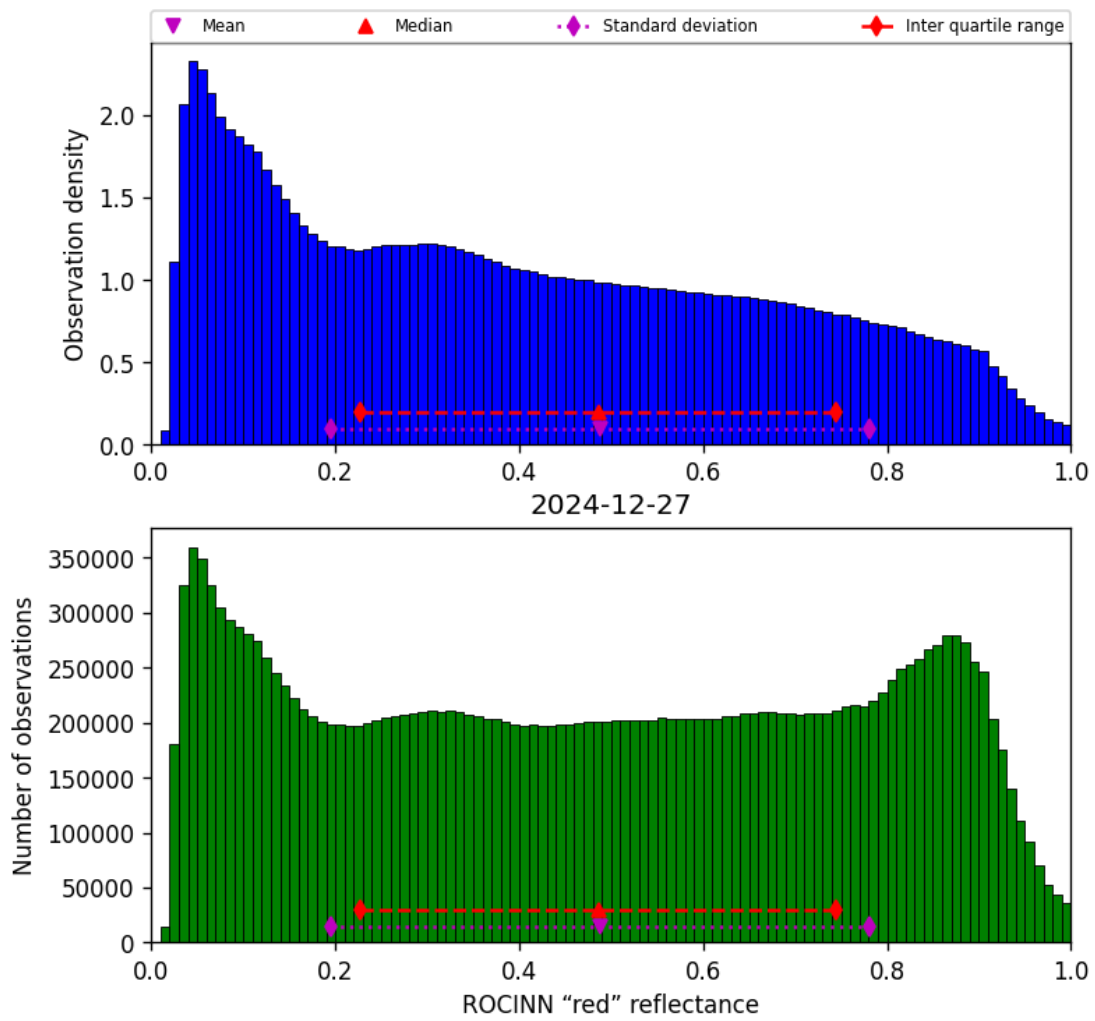
Figure 53: Histogram of “ROCINN “red” reflectance” for 2024-12-27 to 2024-12-28
