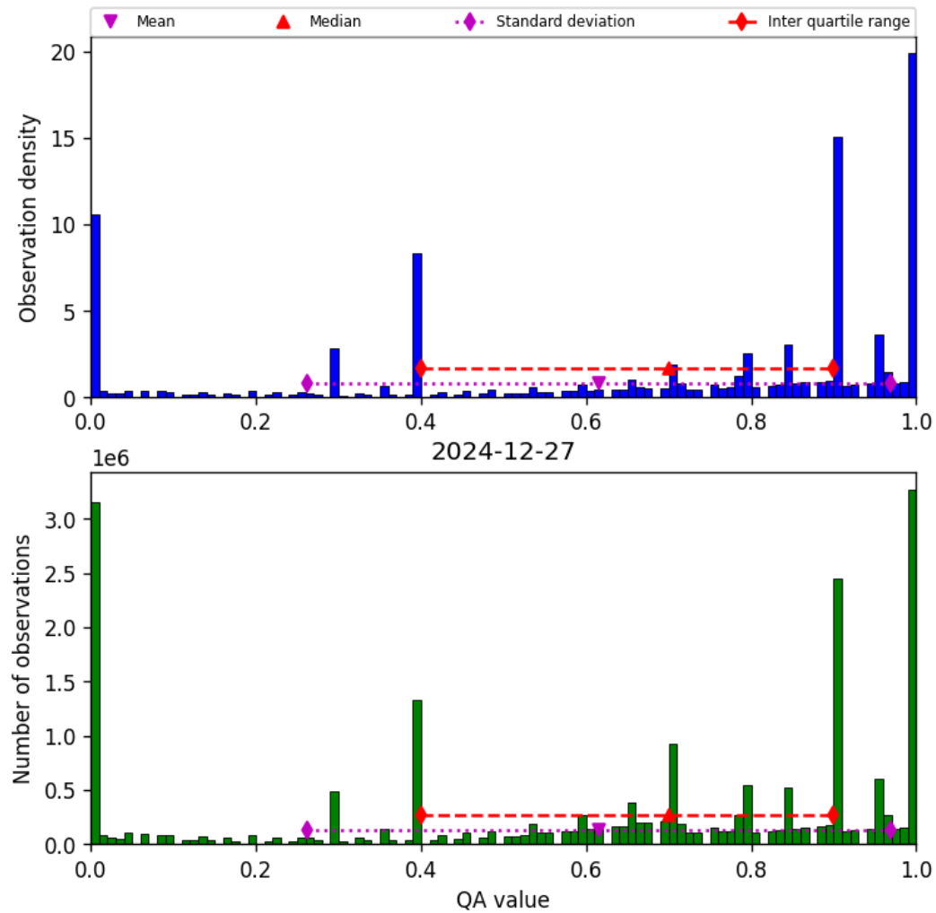
Figure 38: Histogram of “QA value” for 2024-12-27 to 2024-12-28
