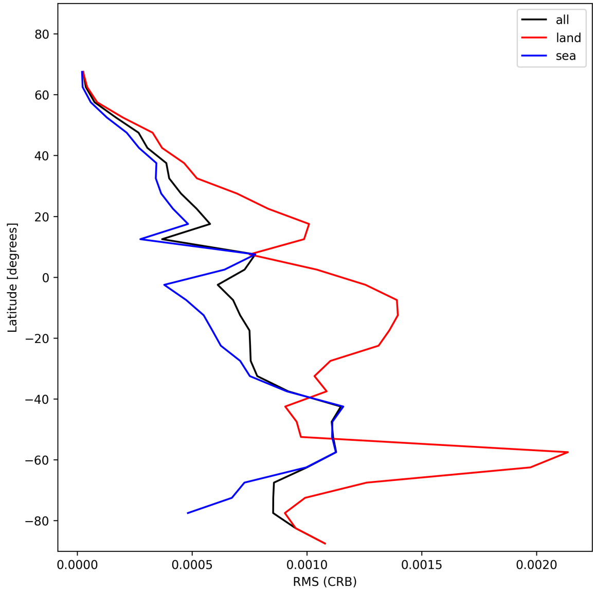
Figure 32: Zonal average of “RMS (CRB)” for 2024-12-27 to 2024-12-28.
