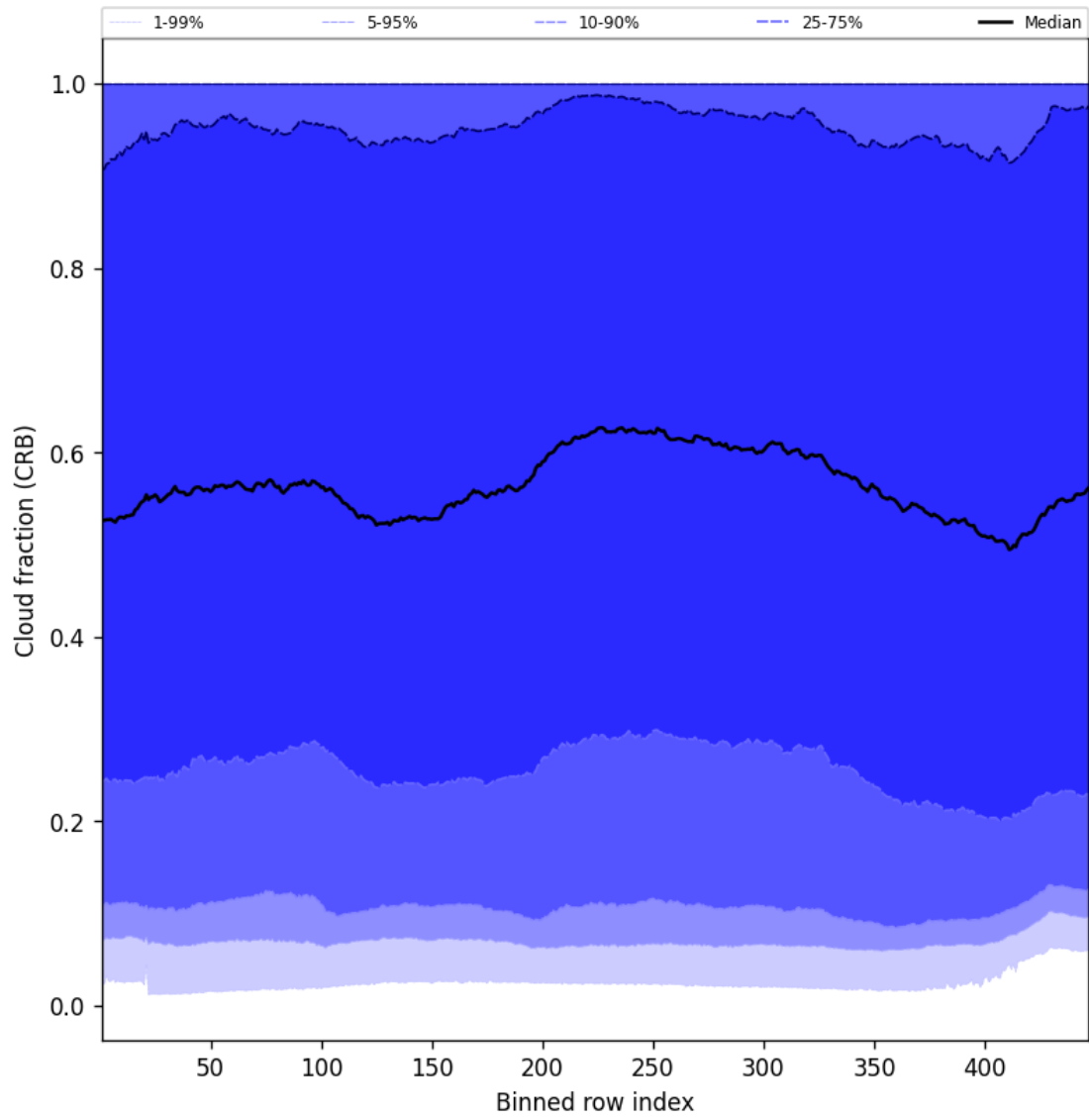
Figure 58: Along track statistics of “Cloud fraction (CRB)” for 2024-12-27 to 2024-12-28
