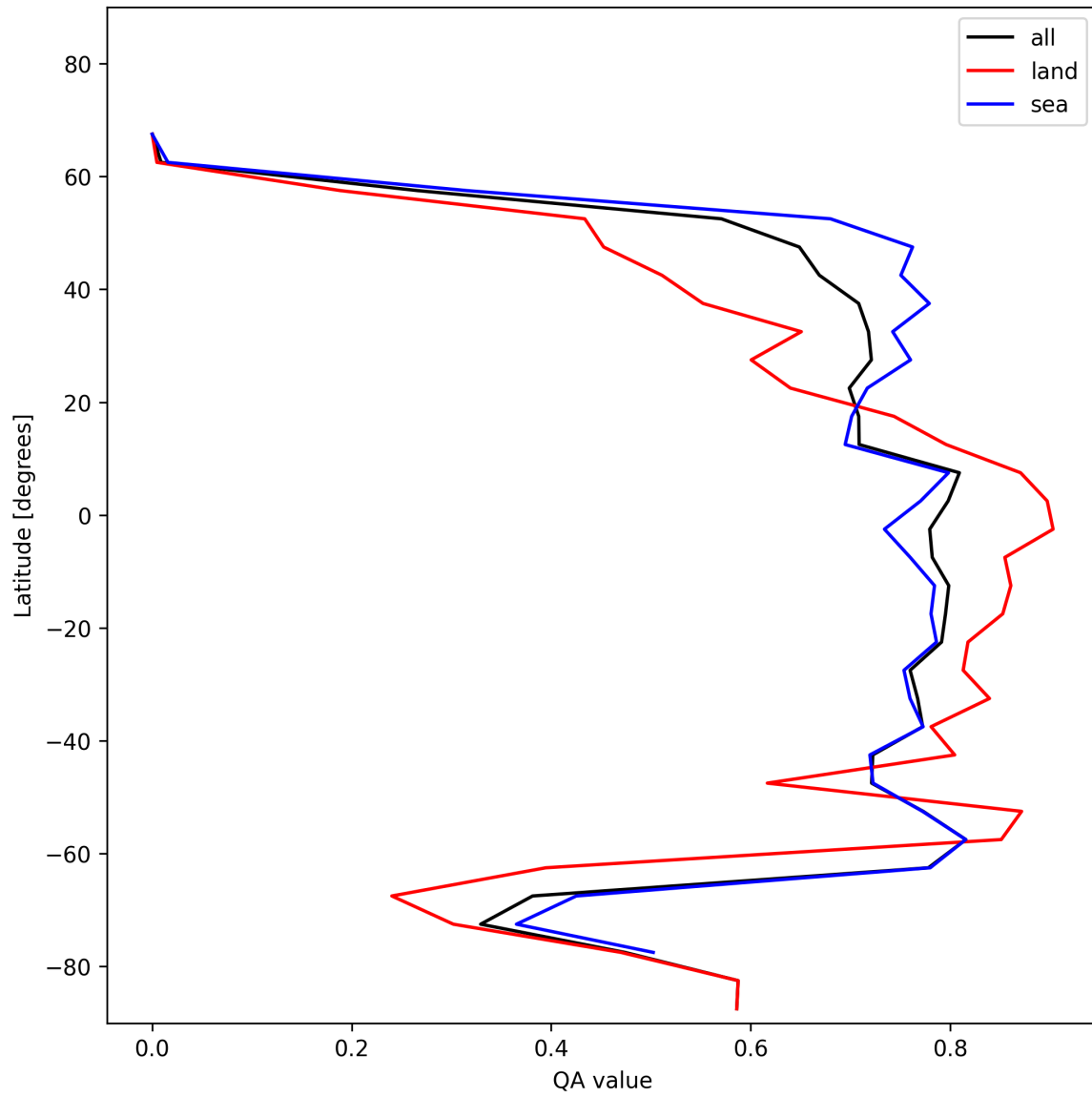
Figure 22: Zonal average of “QA value” for 2024-12-27 to 2024-12-28.
