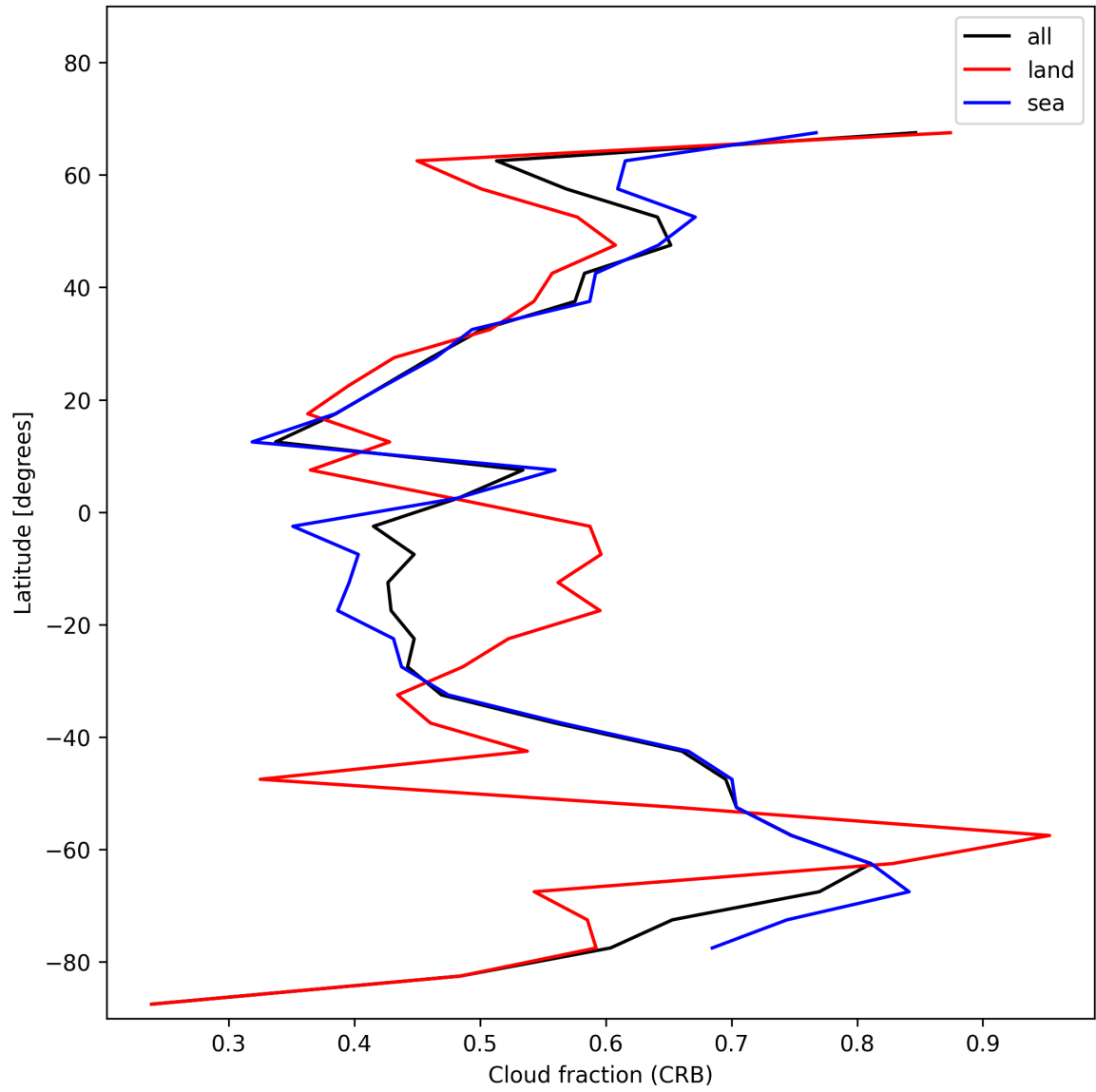
Figure 26: Zonal average of “Cloud fraction (CRB)” for 2024-12-27 to 2024-12-28.
