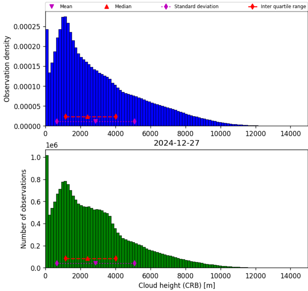
Figure 43: Histogram of “Cloud height (CRB)” for 2024-12-27 to 2024-12-28
