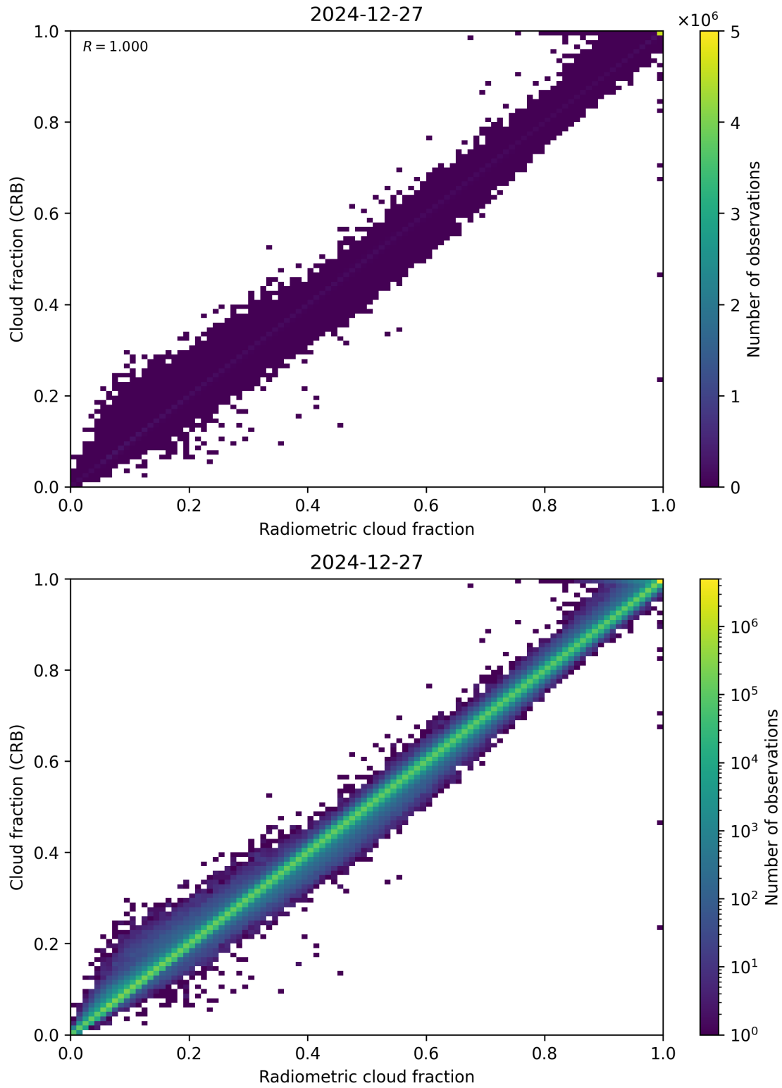
Figure 73: Scatter density plot of “Radiometric cloud fraction” against “Cloud fraction (CRB)” for 2024-12-27 to 2024-12-28.
