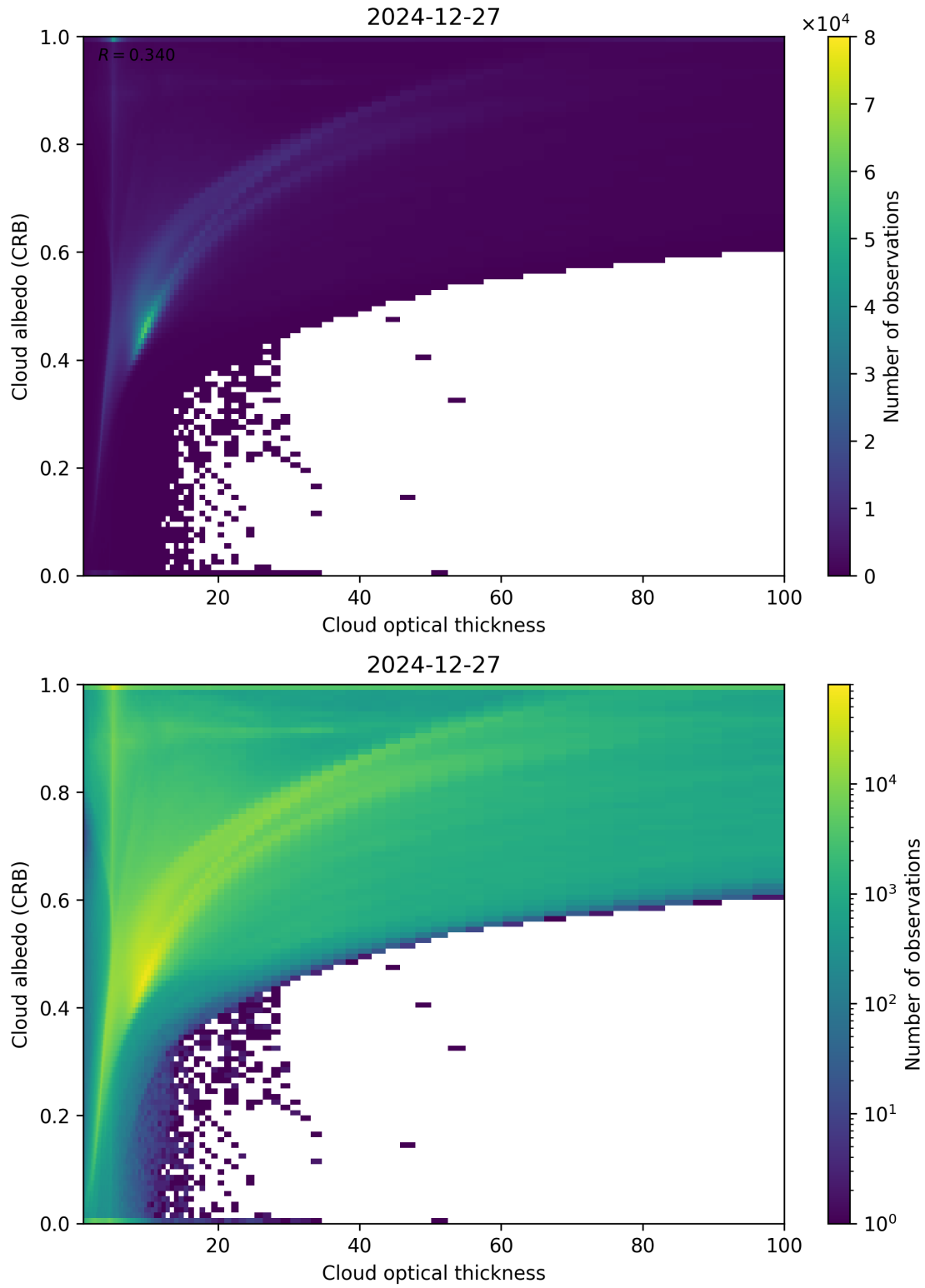
Figure 82: Scatter density plot of “Cloud optical thickness” against “Cloud albedo (CRB)” for 2024-12-27 to 2024-12-28.
