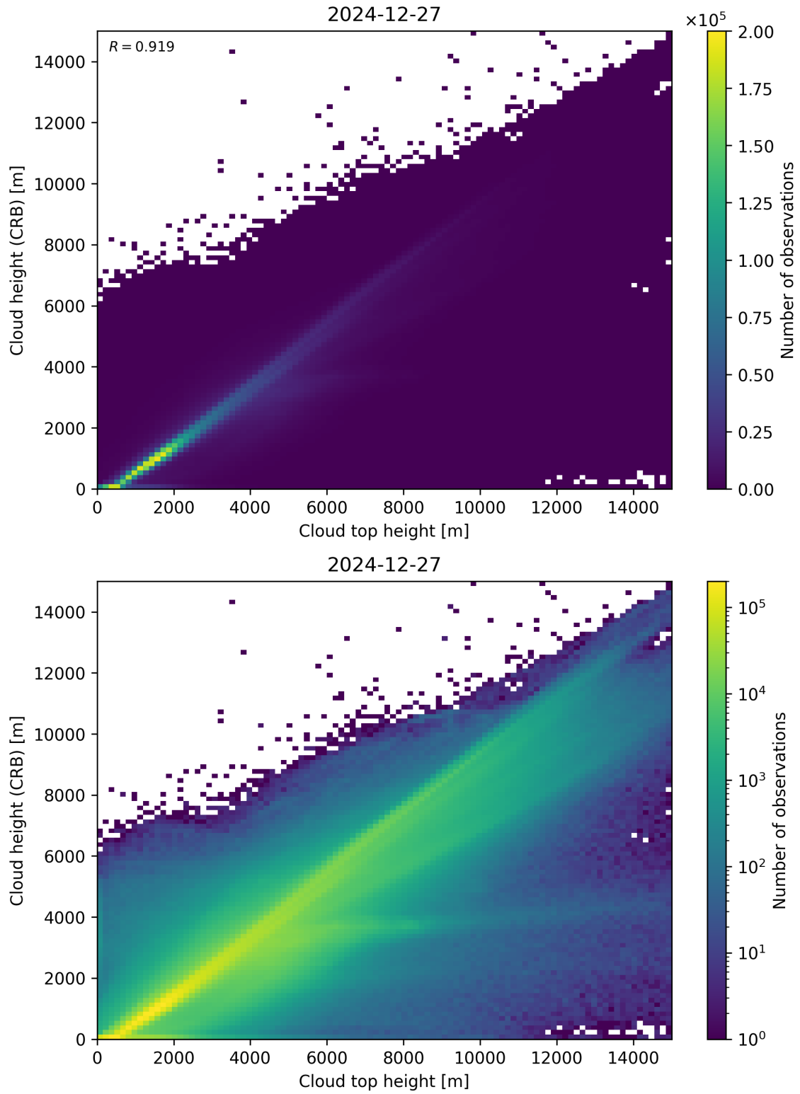
Figure 89: Scatter density plot of “Cloud top height” against “Cloud height (CRB)” for 2024-12-27 to 2024-12-28.
