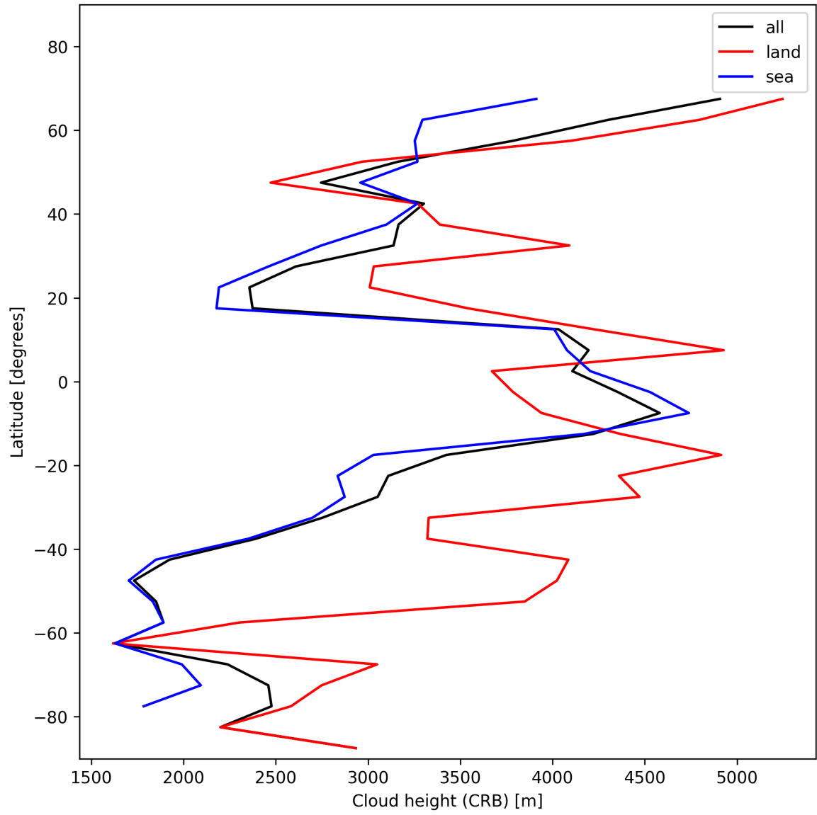
Figure 27: Zonal average of “Cloud height (CRB)” for 2024-12-27 to 2024-12-28.
