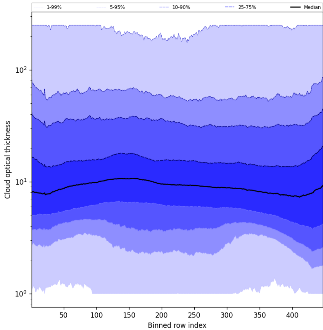
Figure 57: Along track statistics of “Cloud optical thickness” for 2024-12-27 to 2024-12-28
