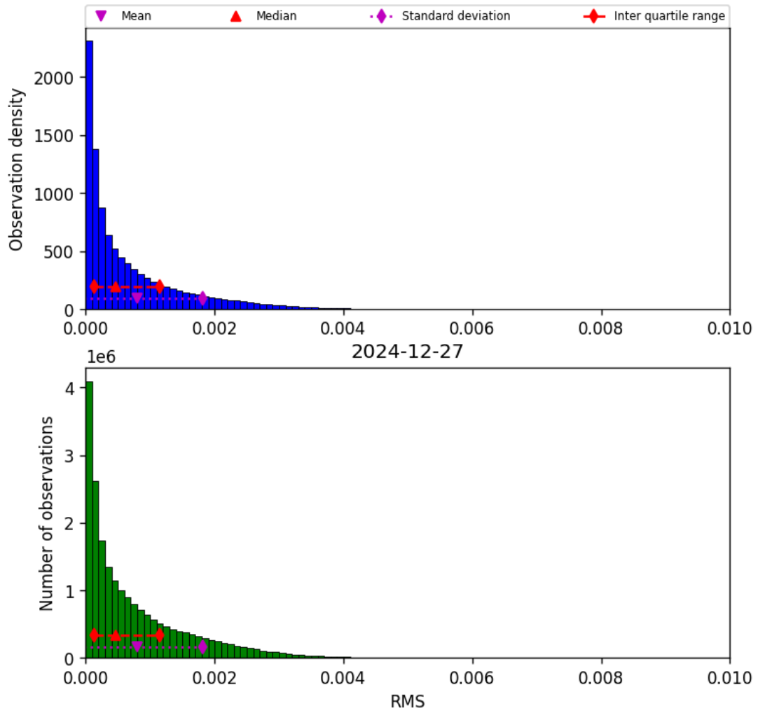
Figure 47: Histogram of “RMS” for 2024-12-27 to 2024-12-28
