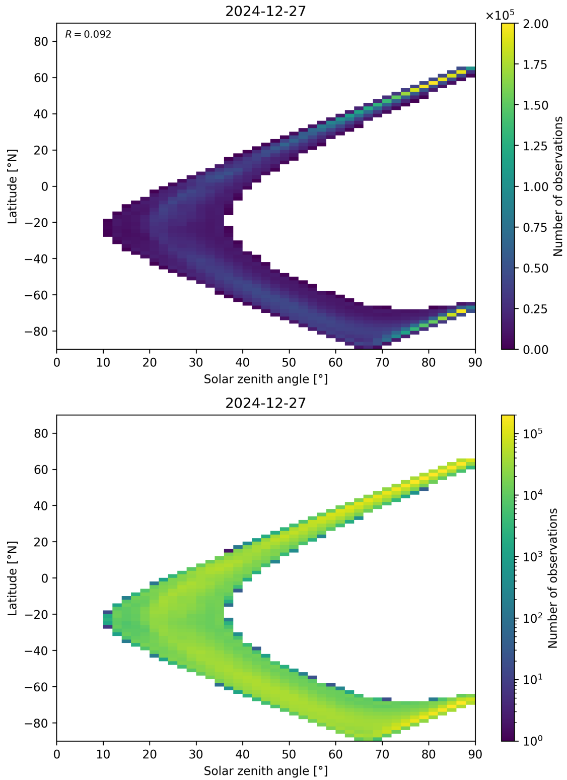
Figure 105: Scatter density plot of “Solar zenith angle” against “Latitude” for 2024-12-27 to 2024-12-28.
