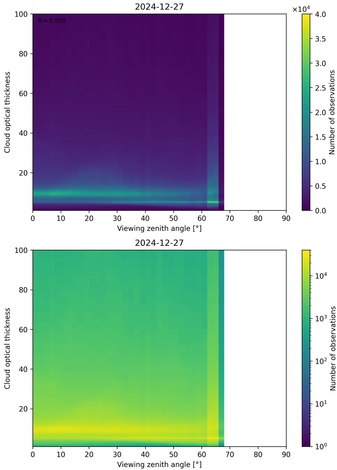
Figure 111: Scatter density plot of “Viewing zenith angle” against “Cloud optical thickness” for 2024-12-27 to 2024-12-28.
