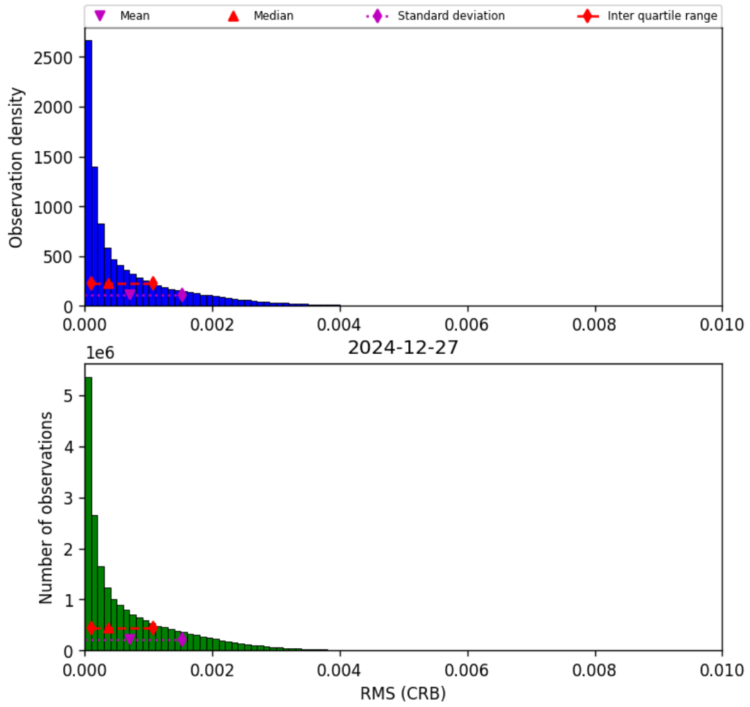
Figure 48: Histogram of “RMS (CRB)” for 2024-12-27 to 2024-12-28
