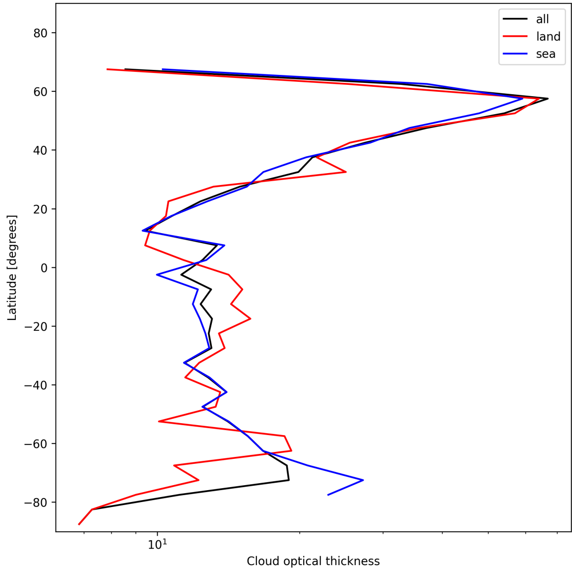
Figure 25: Zonal average of “Cloud optical thickness” for 2024-12-27 to 2024-12-29.
