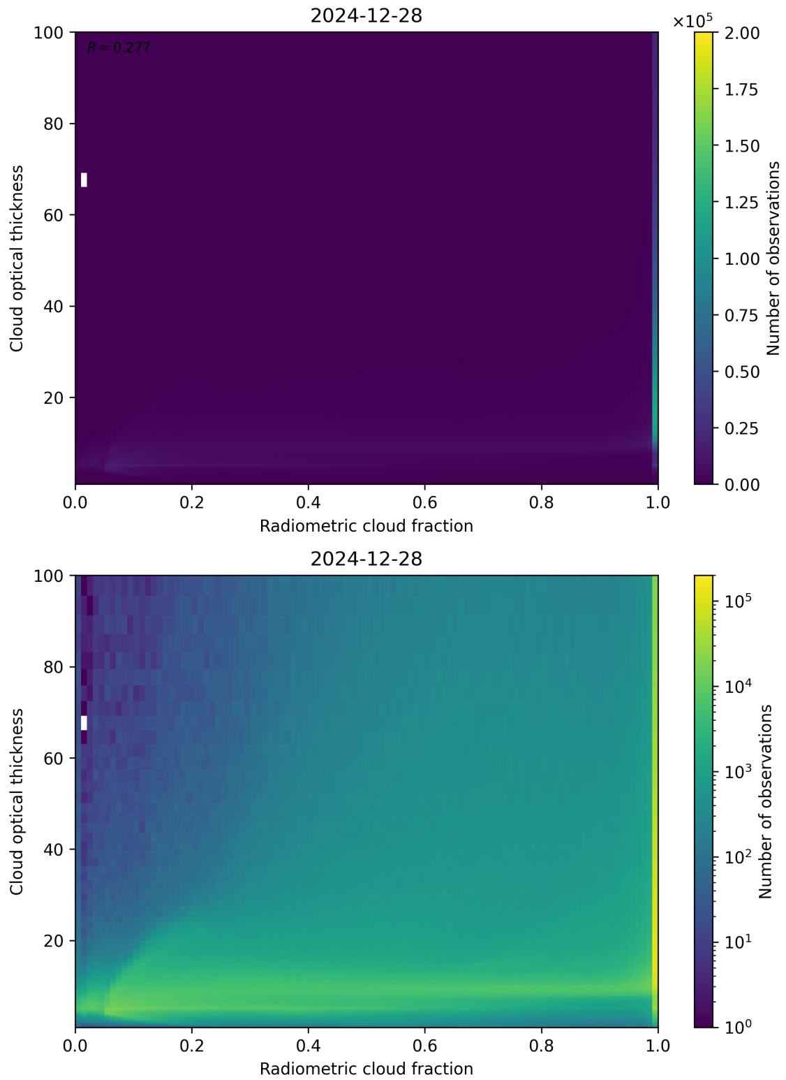
Figure 75: Scatter density plot of “Radiometric cloud fraction” against “Cloud optical thickness” for 2024-12-27 to 2024-12-29.
