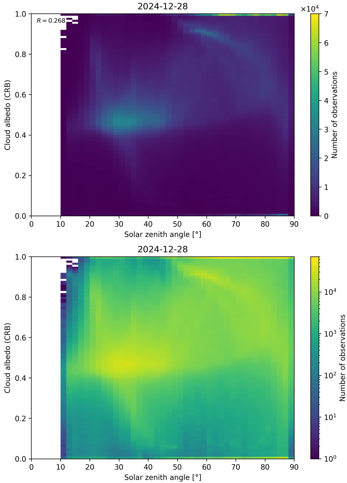
Figure 98: Scatter density plot of “Solar zenith angle” against “Cloud albedo (CRB)” for 2024-12-27 to 2024-12-29.
