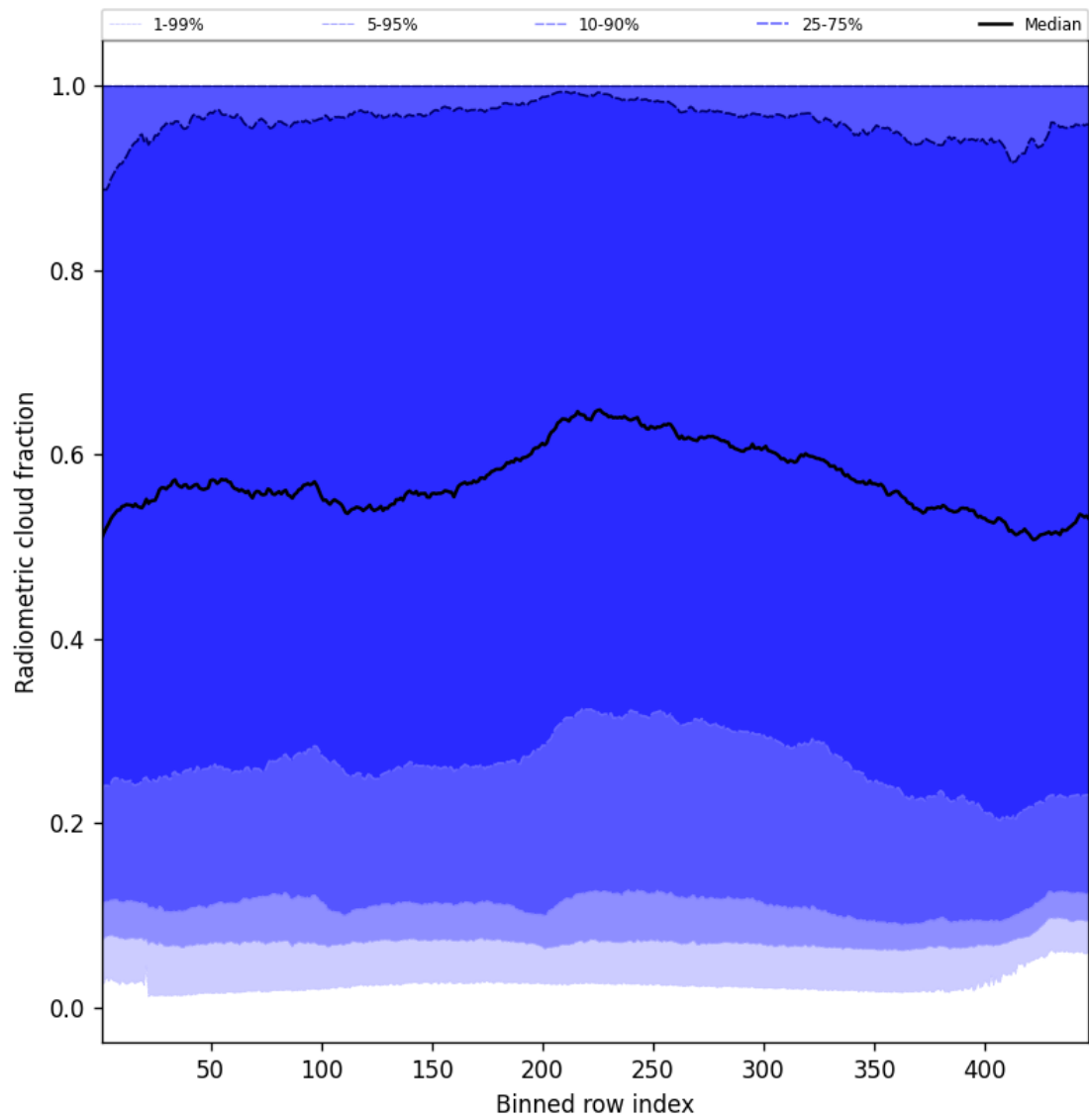
Figure 55: Along track statistics of “Radiometric cloud fraction” for 2024-12-27 to 2024-12-29
