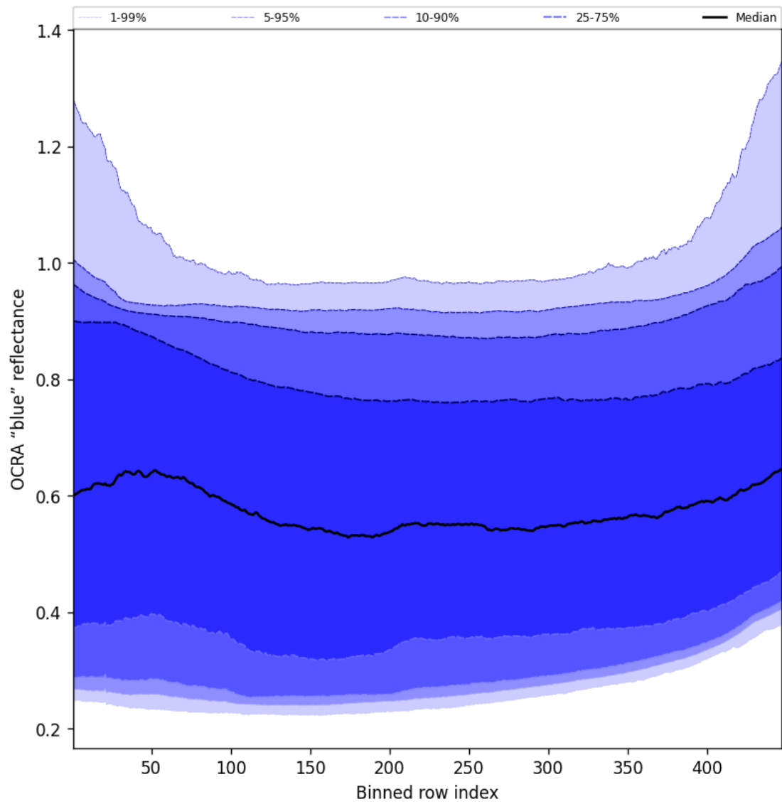
Figure 67: Along track statistics of “OCRA “blue” reflectance” for 2024-12-27 to 2024-12-29
