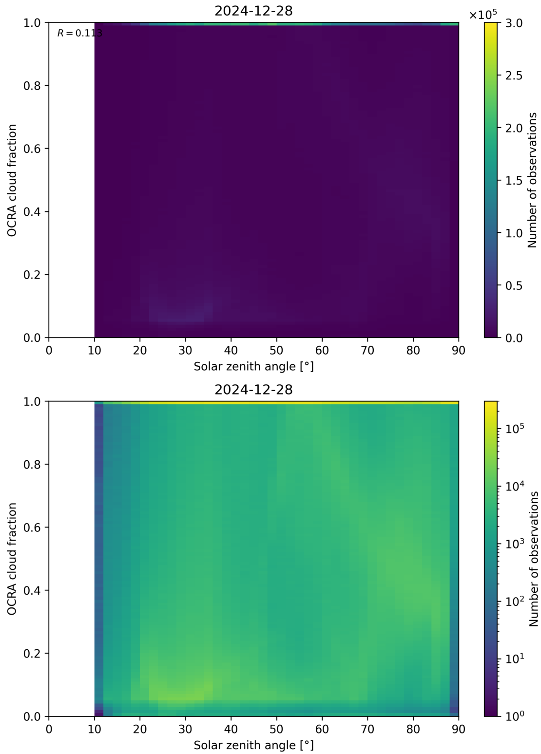
Figure 100: Scatter density plot of “Solar zenith angle” against “OCRA cloud fraction” for 2024-12-27 to 2024-12-29.
