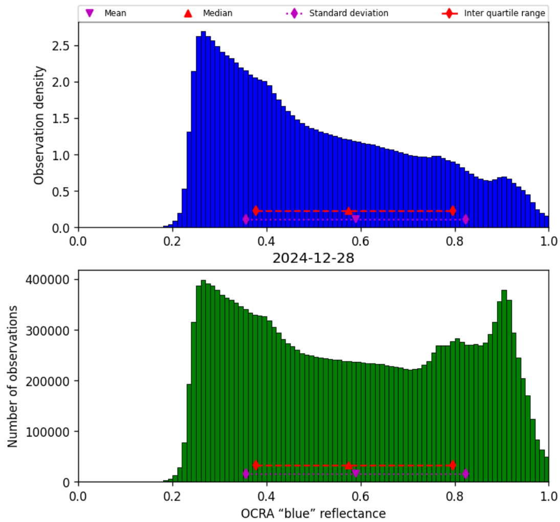
Figure 51: Histogram of “OCRA “blue” reflectance” for 2024-12-27 to 2024-12-29
