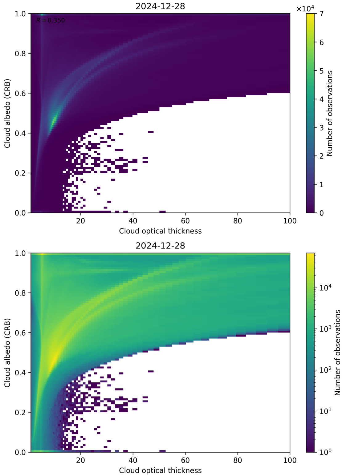
Figure 82: Scatter density plot of “Cloud optical thickness” against “Cloud albedo (CRB)” for 2024-12-27 to 2024-12-29.
