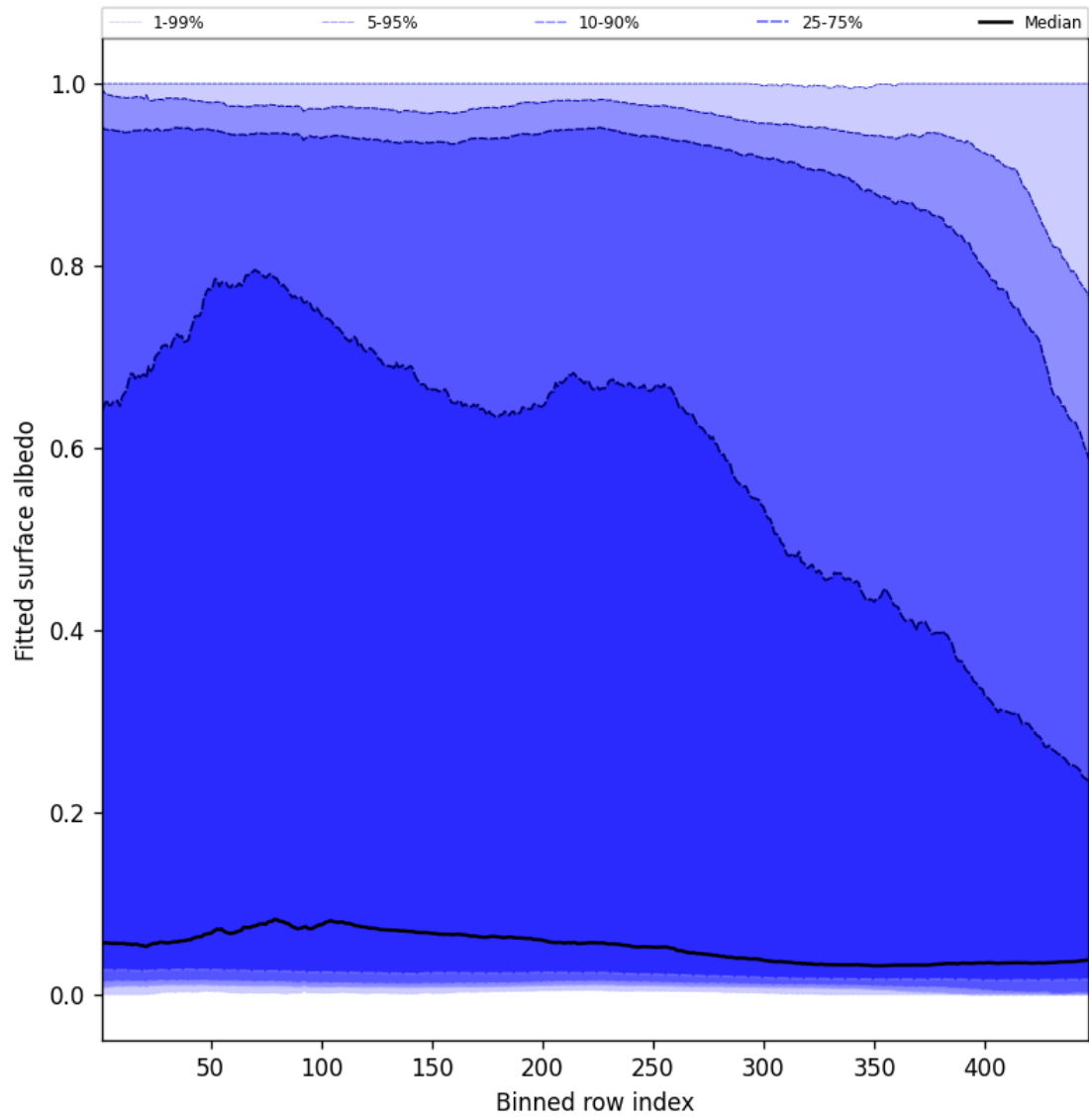
Figure 61: Along track statistics of “Fitted surface albedo” for 2024-12-27 to 2024-12-29
