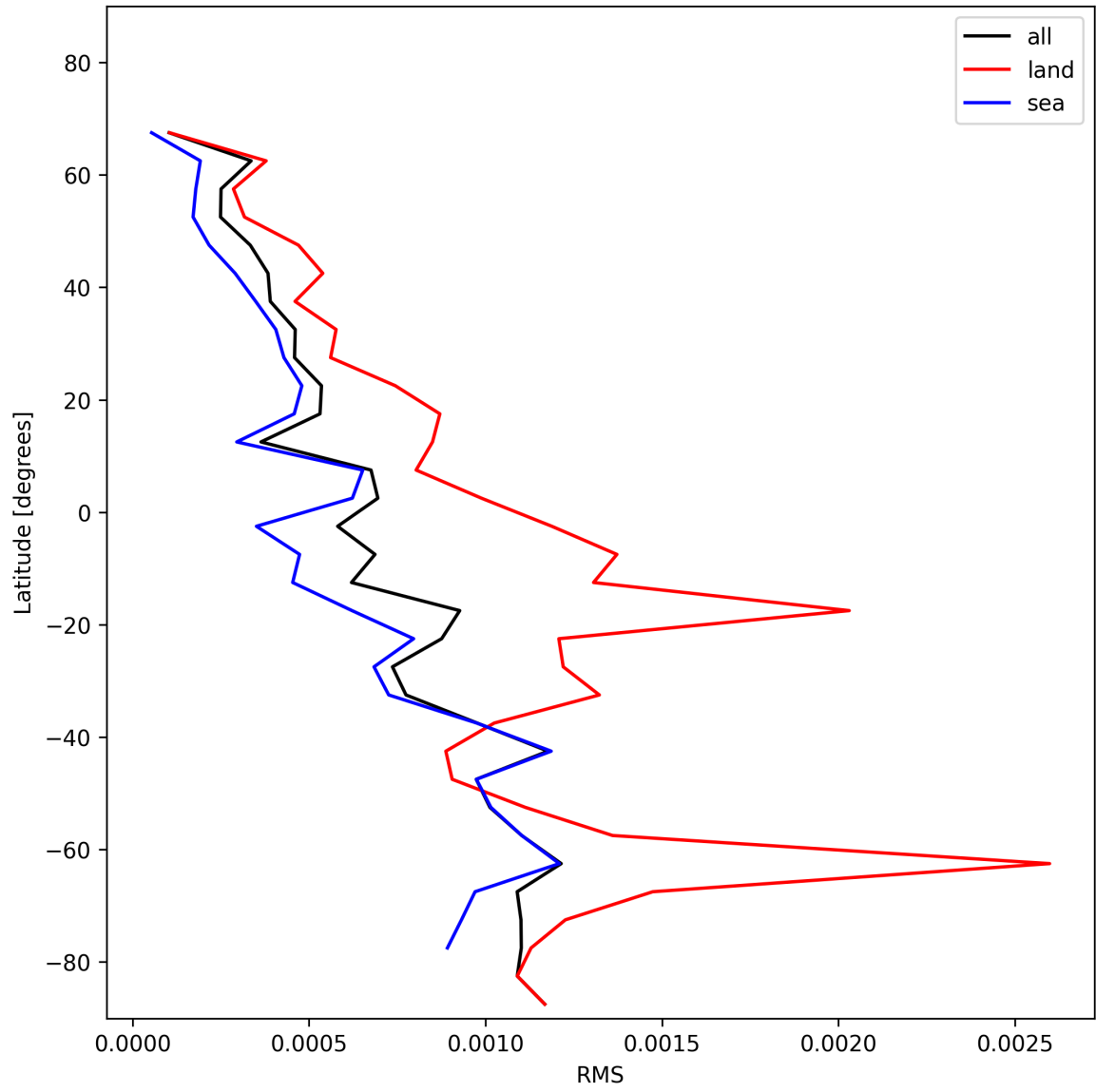
Figure 31: Zonal average of “RMS” for 2024-12-27 to 2024-12-29.
