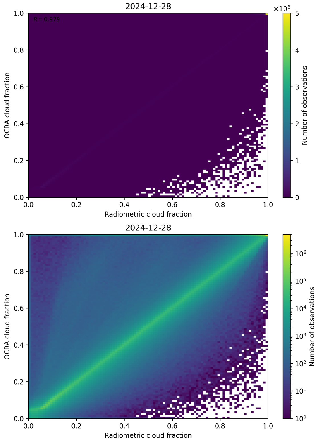
Figure 72: Scatter density plot of “Radiometric cloud fraction” against “OCRA cloud fraction” for 2024-12-27 to 2024-12-29.
