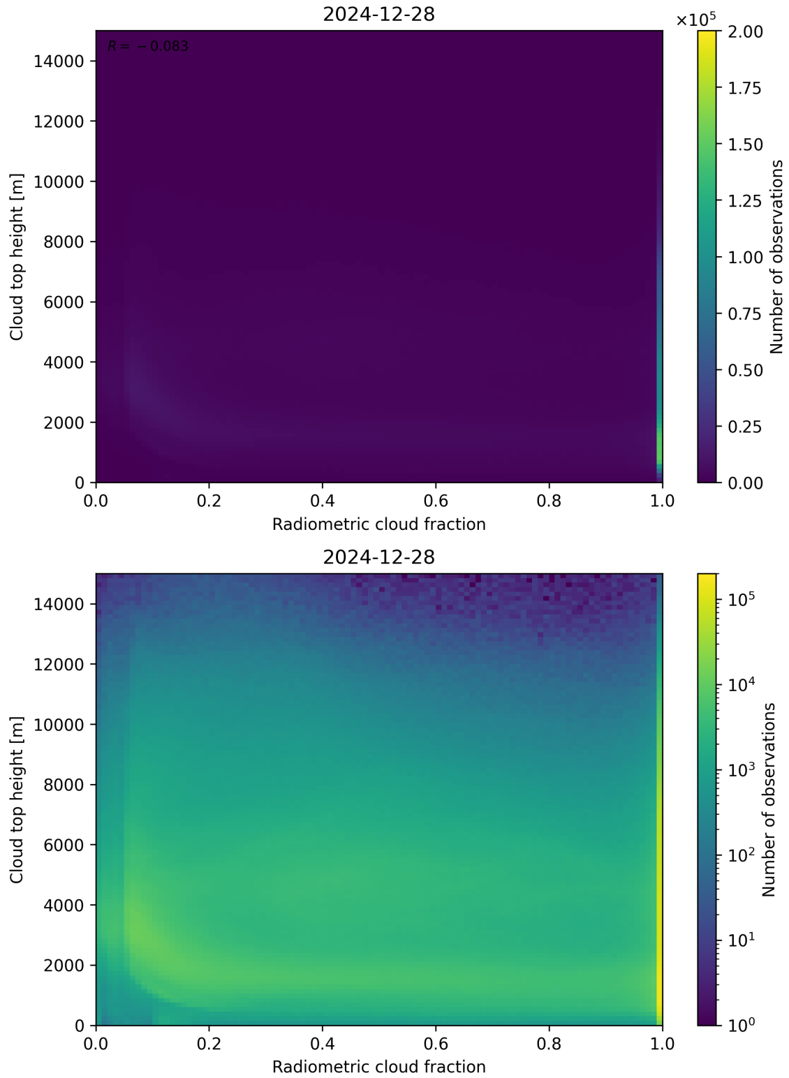
Figure 76: Scatter density plot of “Radiometric cloud fraction” against “Cloud top height” for 2024-12-27 to 2024-12-29.
