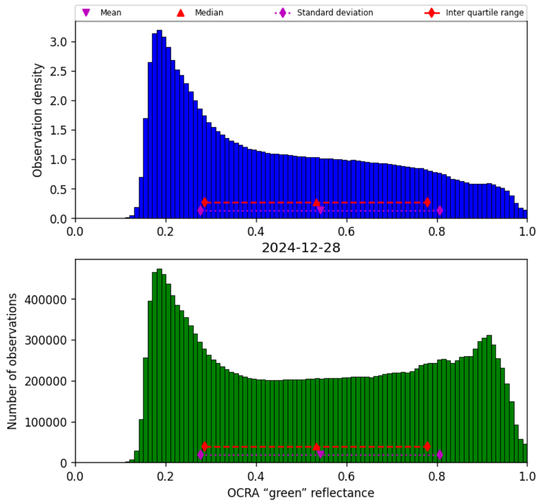
Figure 52: Histogram of “OCRA “green” reflectance” for 2024-12-27 to 2024-12-29
