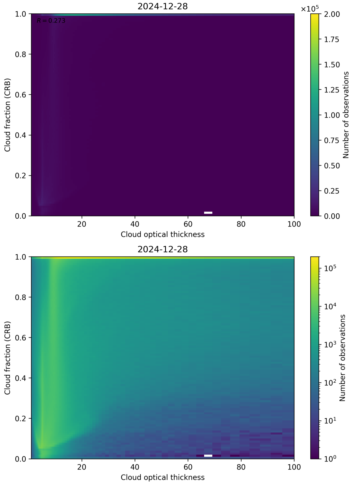
Figure 84: Scatter density plot of “Cloud optical thickness” against “Cloud fraction (CRB)” for 2024-12-27 to 2024-12-29.
