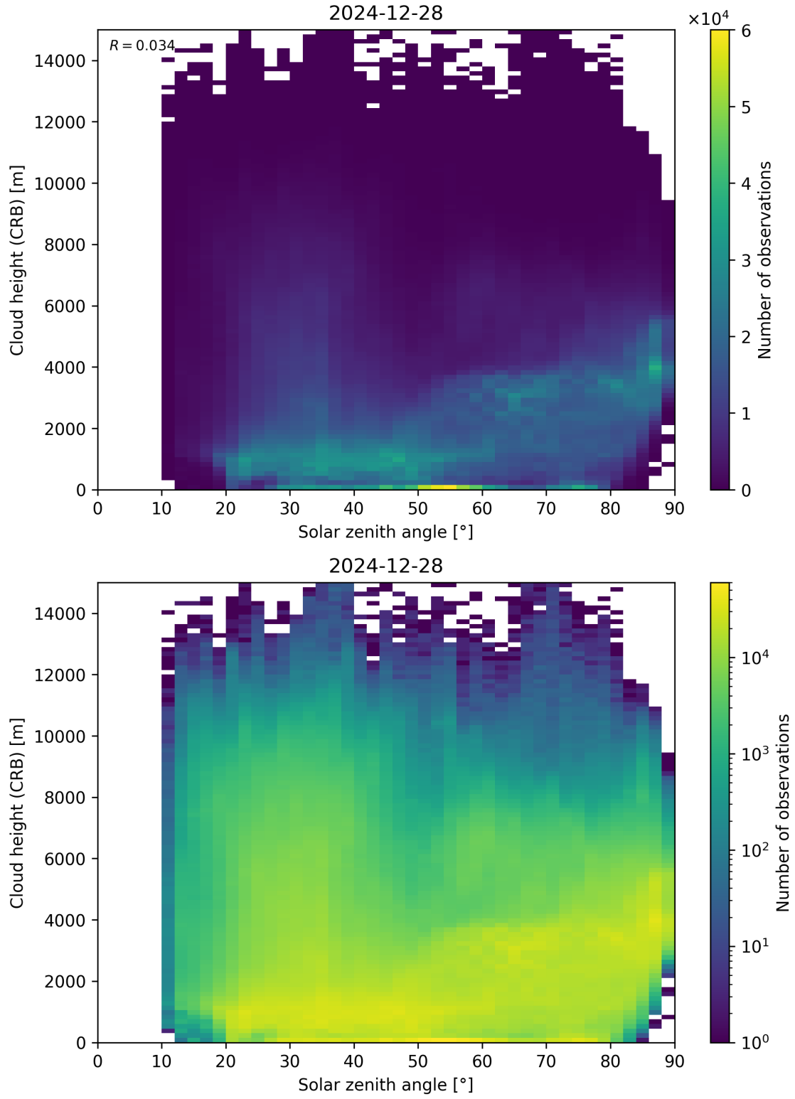
Figure 102: Scatter density plot of “Solar zenith angle” against “Cloud height (CRB)” for 2024-12-27 to 2024-12-29.
