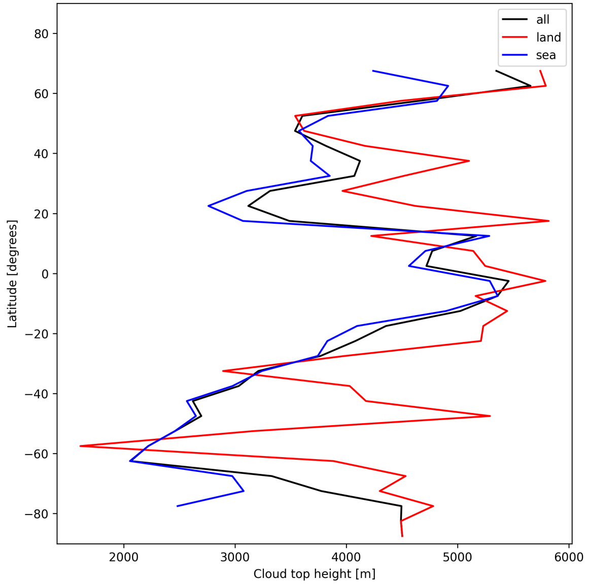
Figure 24: Zonal average of “Cloud top height” for 2024-12-27 to 2024-12-29.
