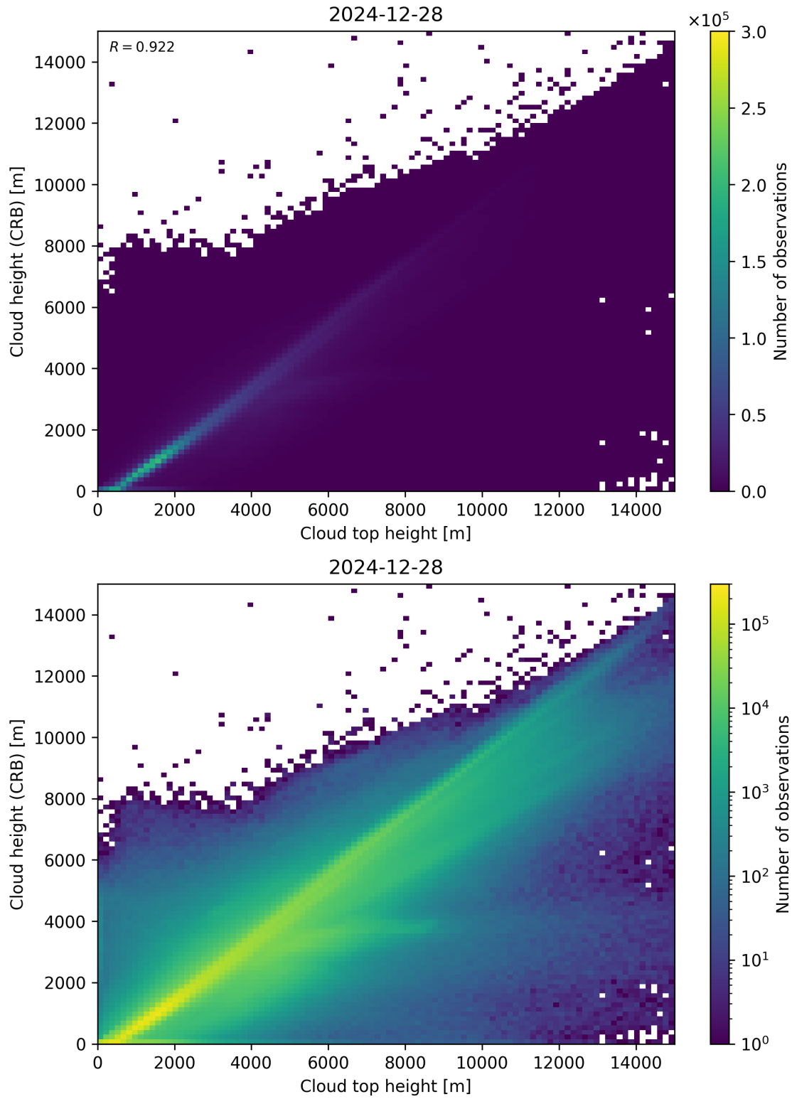
Figure 89: Scatter density plot of “Cloud top height” against “Cloud height (CRB)” for 2024-12-27 to 2024-12-29.
