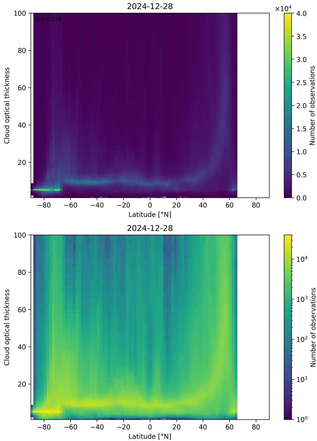
Figure 96: Scatter density plot of “Latitude” against “Cloud optical thickness” for 2024-12-27 to 2024-12-29.
