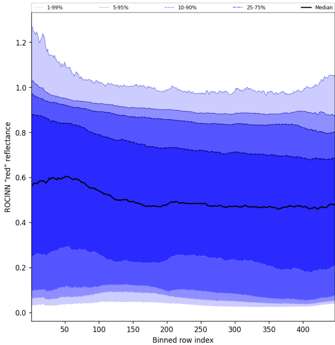
Figure 69: Along track statistics of “ROCINN “red” reflectance” for 2024-12-27 to 2024-12-29
