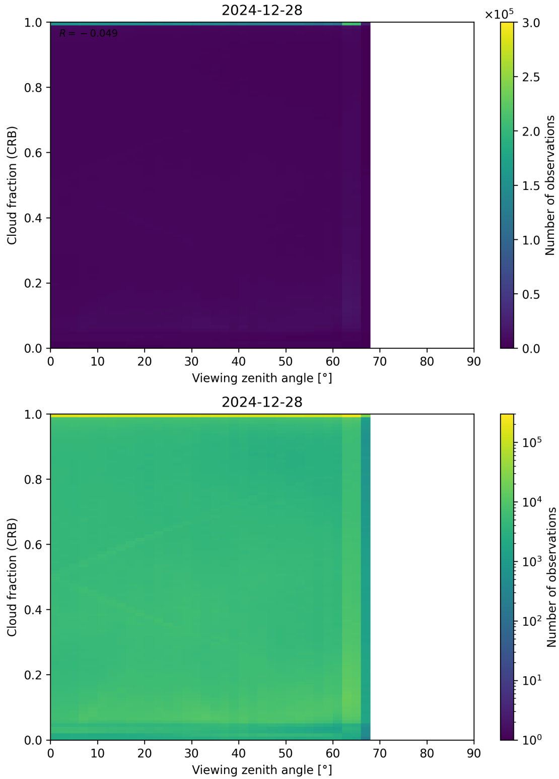
Figure 109: Scatter density plot of “Viewing zenith angle” against “Cloud fraction (CRB)” for 2024-12-27 to 2024-12-29.
