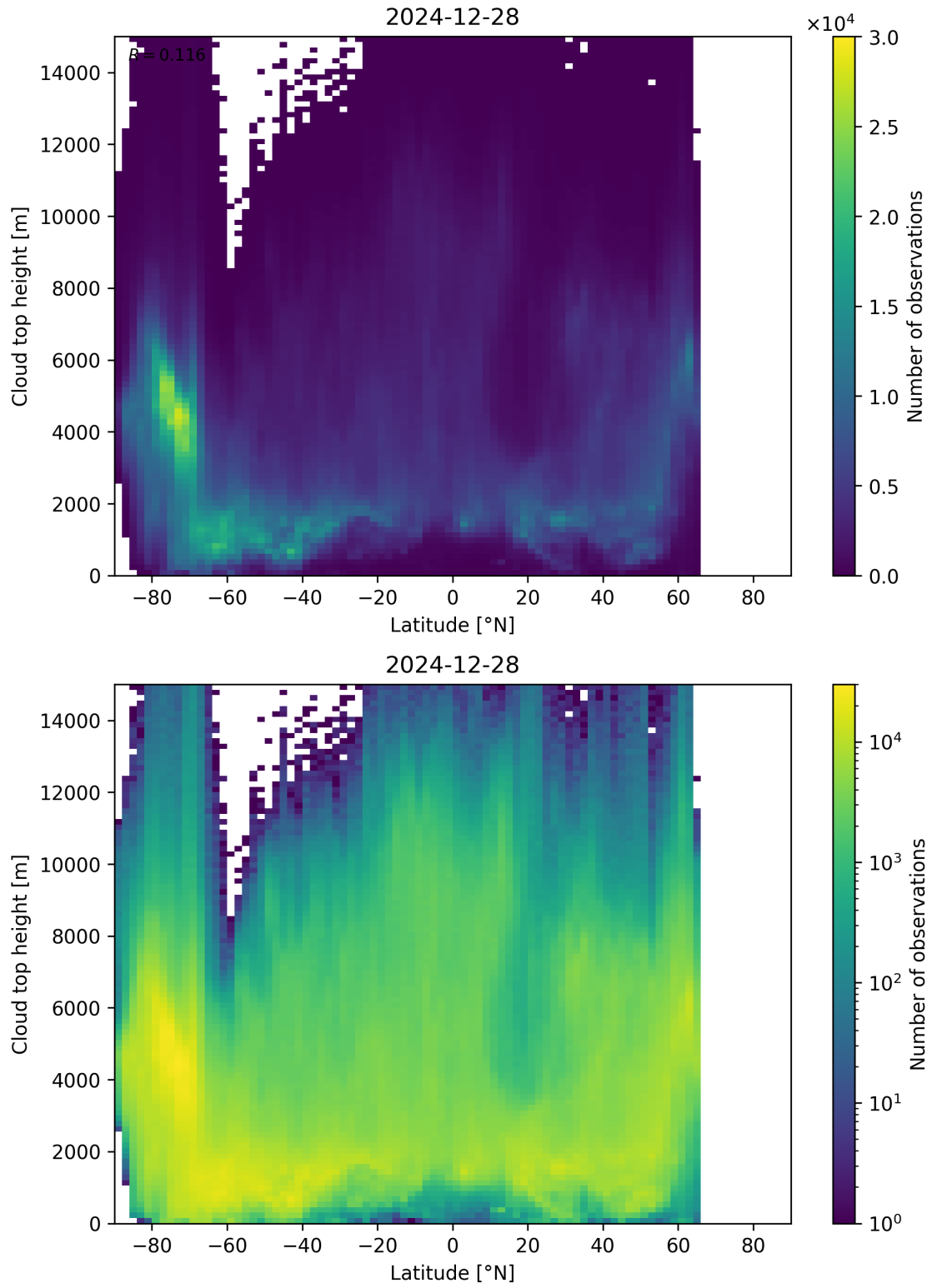
Figure 97: Scatter density plot of “Latitude” against “Cloud top height” for 2024-12-27 to 2024-12-29.
