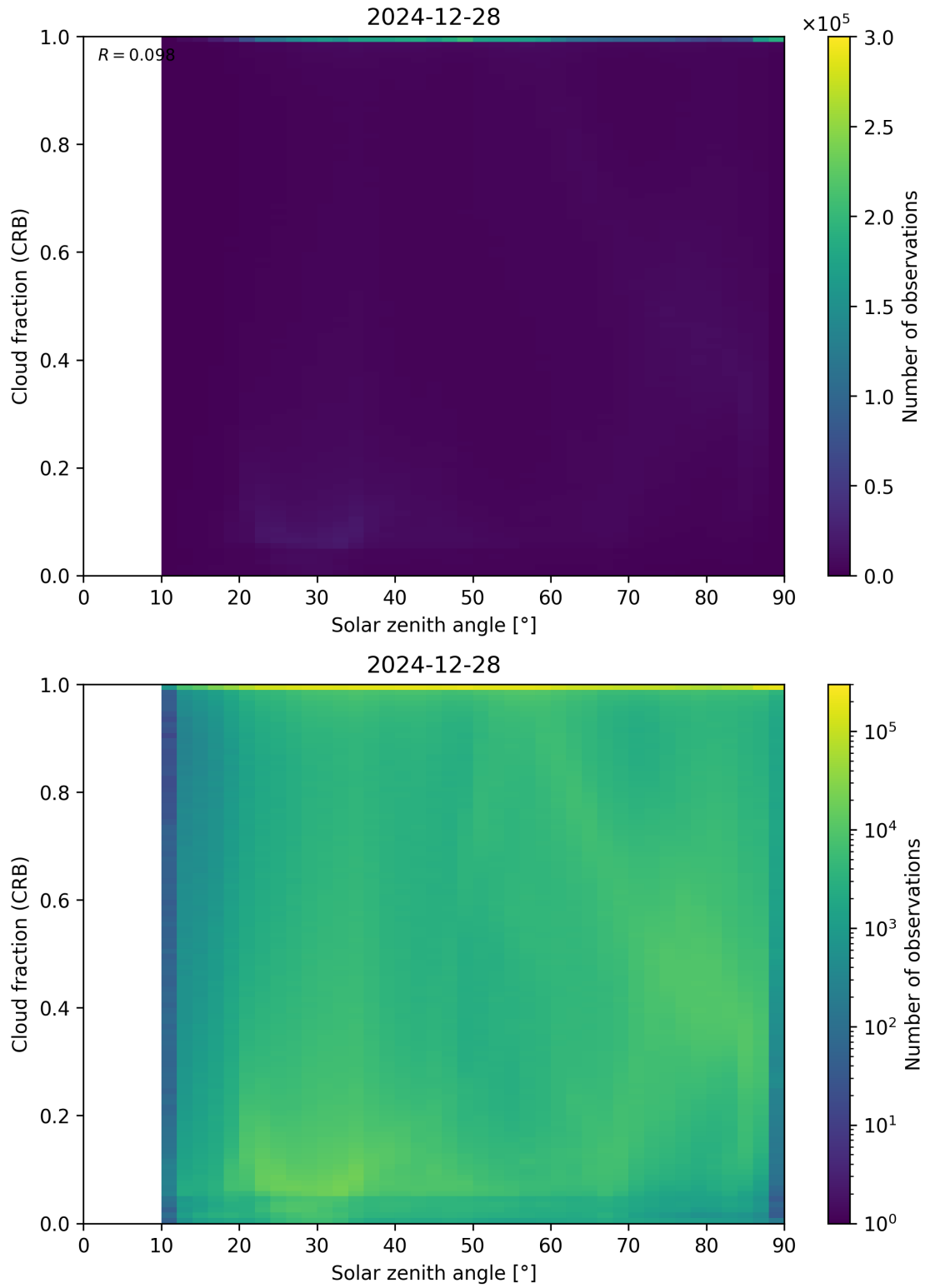
Figure 101: Scatter density plot of “Solar zenith angle” against “Cloud fraction (CRB)” for 2024-12-27 to 2024-12-29.
