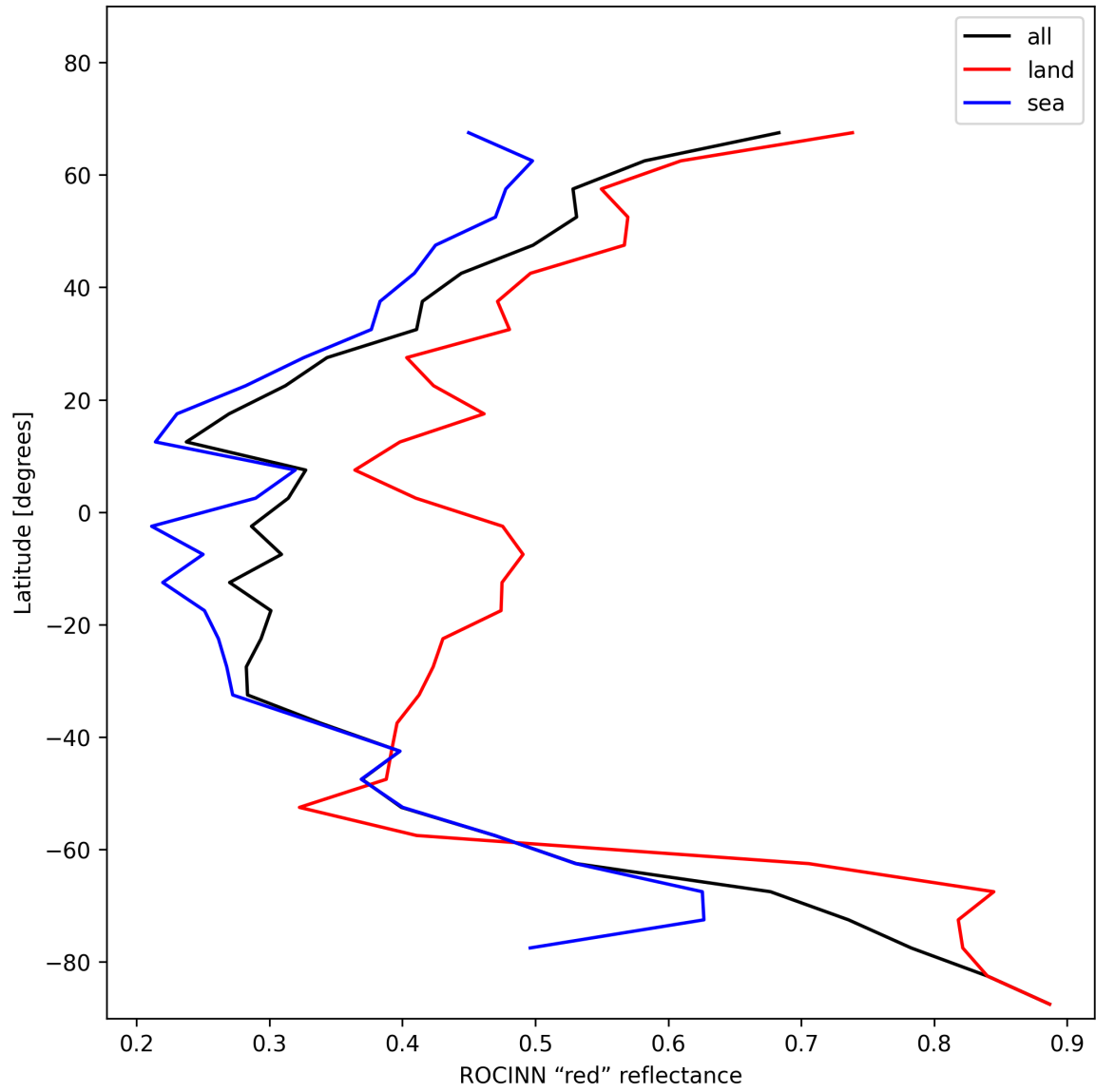
Figure 37: Zonal average of “ROCINN “red” reflectance” for 2024-12-27 to 2024-12-29.
