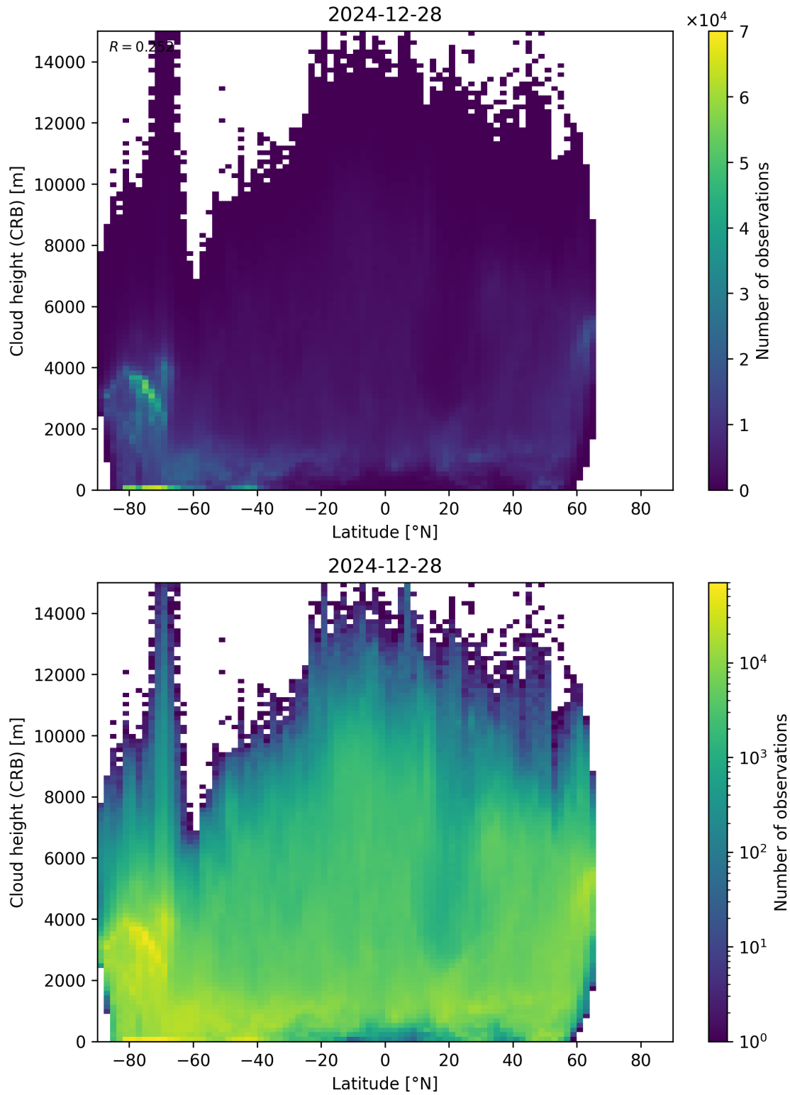
Figure 95: Scatter density plot of “Latitude” against “Cloud height (CRB)” for 2024-12-27 to 2024-12-29.
