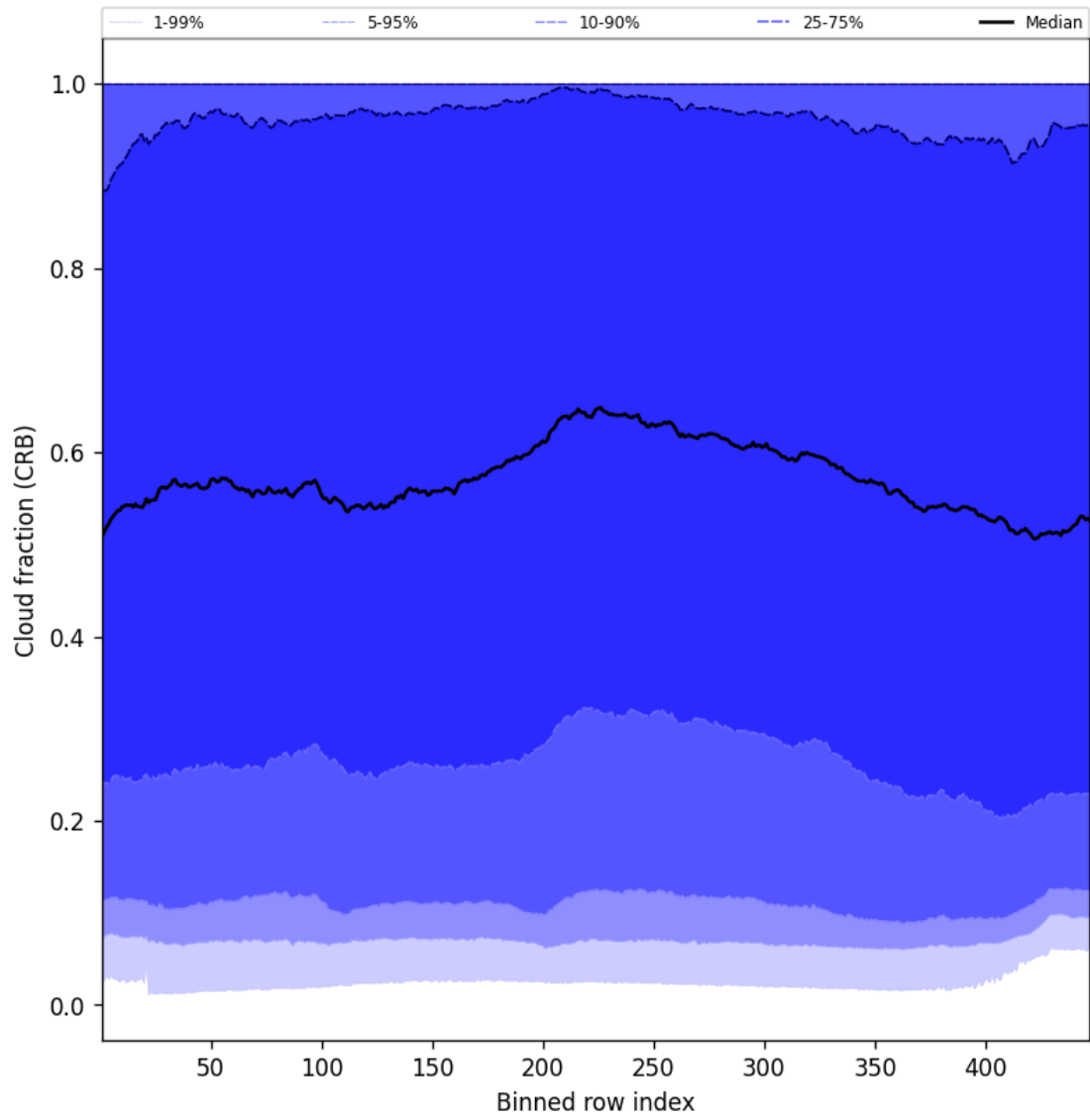
Figure 58: Along track statistics of “Cloud fraction (CRB)” for 2024-12-27 to 2024-12-29
