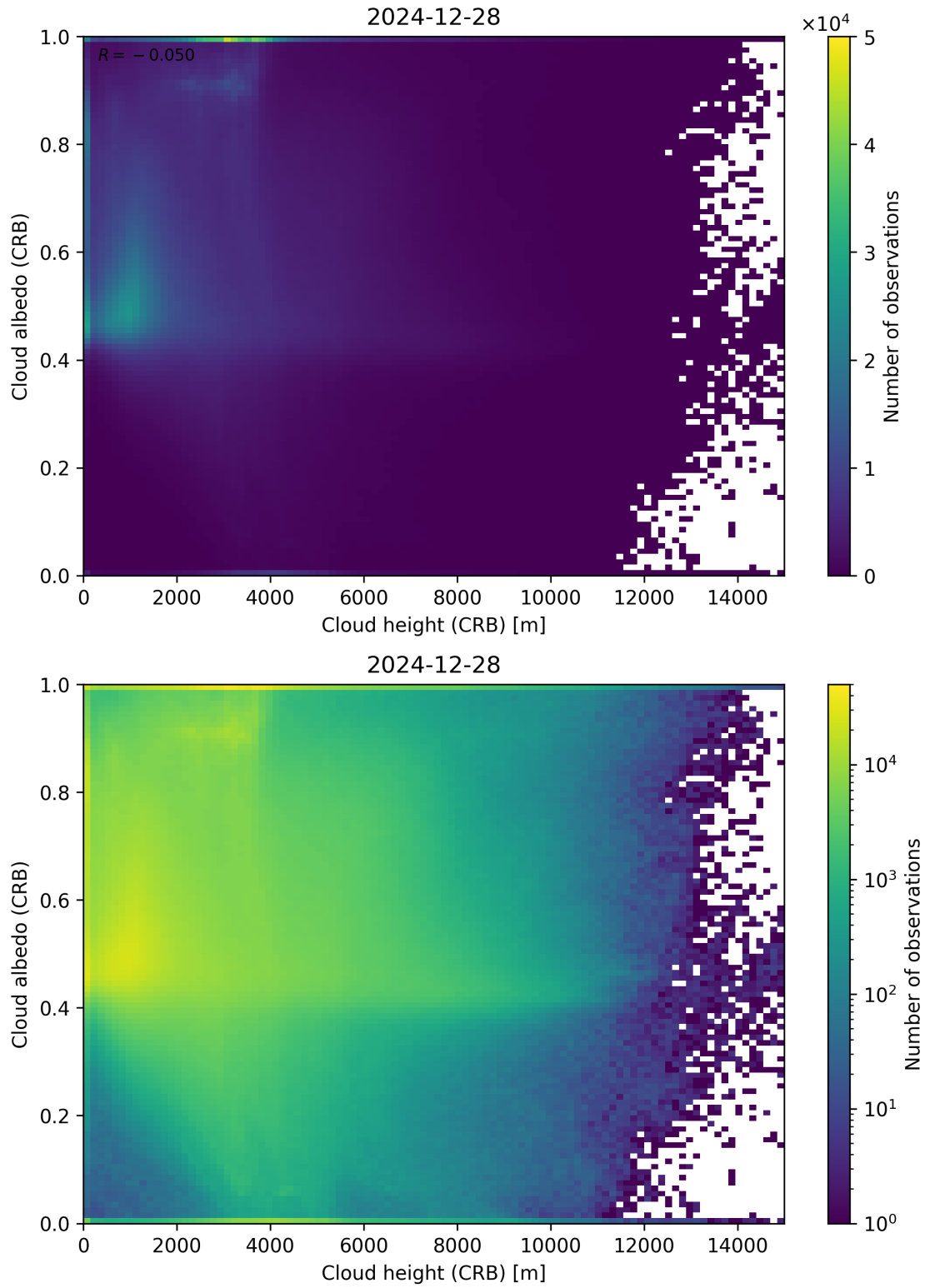
Figure 80: Scatter density plot of “Cloud height (CRB)” against “Cloud albedo (CRB)” for 2024-12-27 to 2024-12-29.
