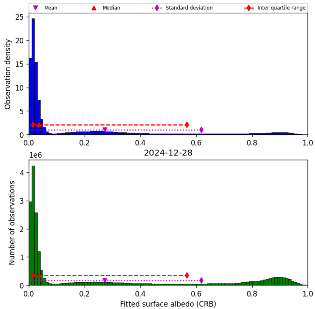
Figure 46: Histogram of “Fitted surface albedo (CRB)” for 2024-12-27 to 2024-12-29
