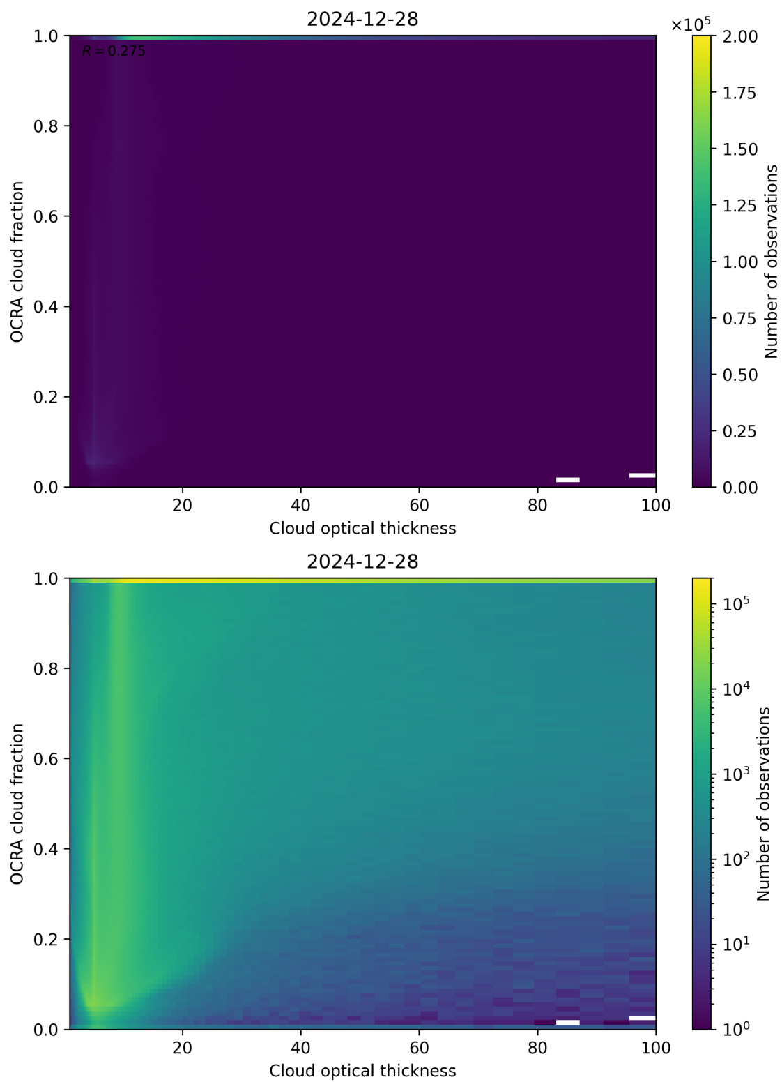
Figure 83: Scatter density plot of “Cloud optical thickness” against “OCRA cloud fraction” for 2024-12-27 to 2024-12-29.
