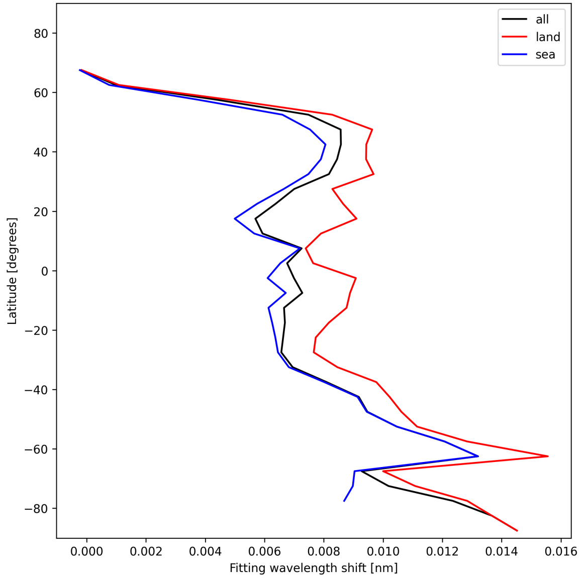
Figure 33: Zonal average of “Fitting wavelength shift” for 2024-12-27 to 2024-12-29.
