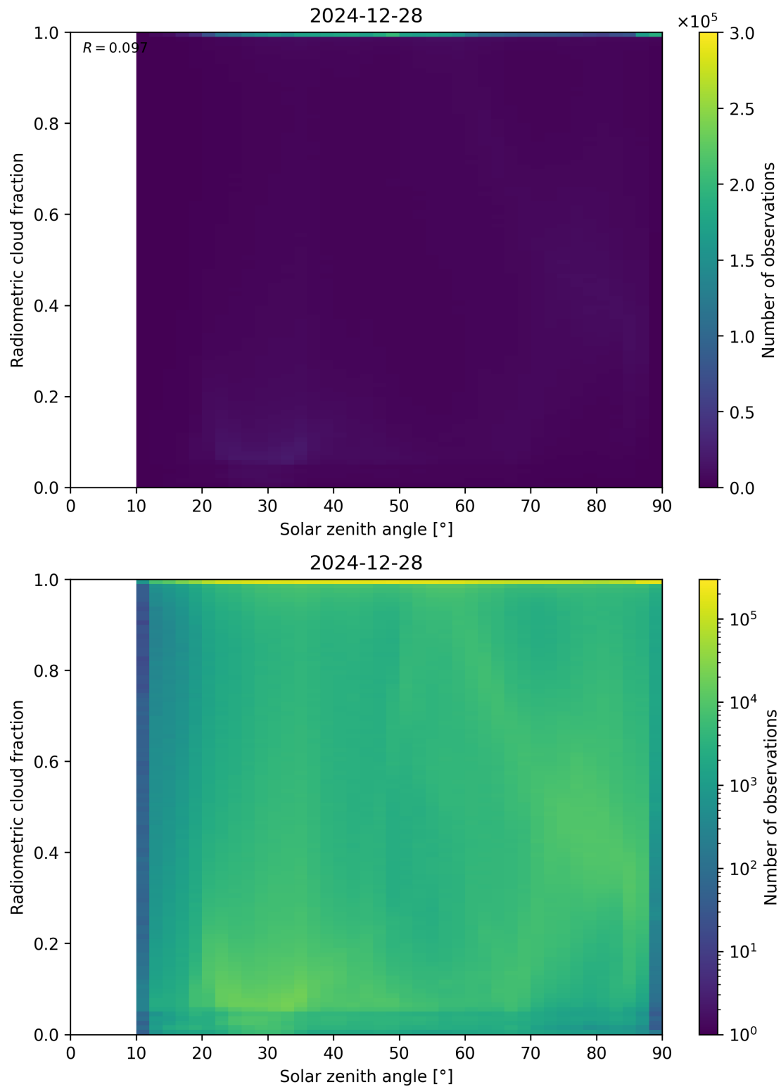
Figure 99: Scatter density plot of “Solar zenith angle” against “Radiometric cloud fraction” for 2024-12-27 to 2024-12-29.
