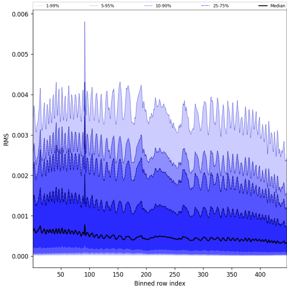
Figure 63: Along track statistics of “RMS” for 2024-12-27 to 2024-12-29
