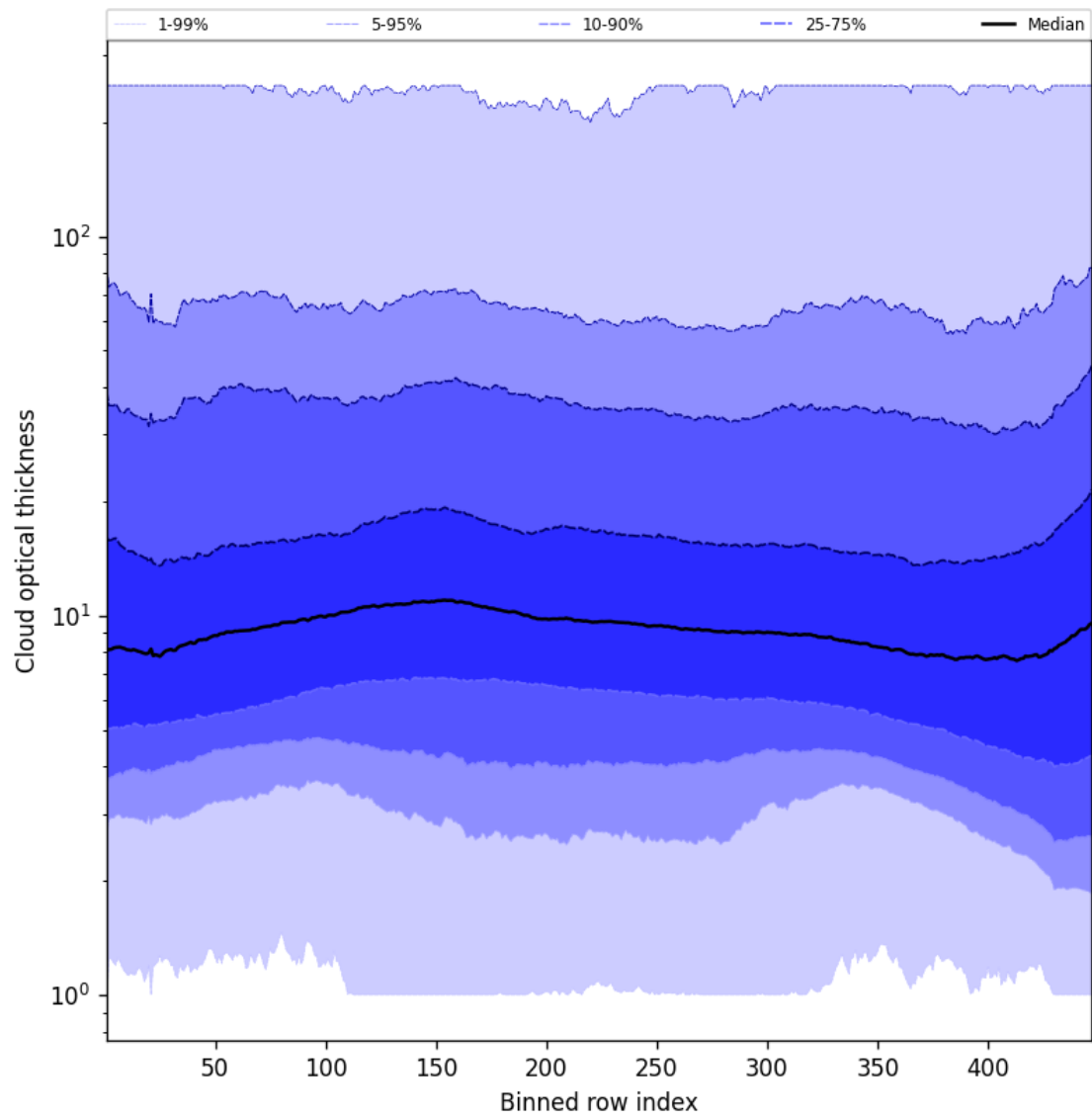
Figure 57: Along track statistics of “Cloud optical thickness” for 2024-12-27 to 2024-12-29
