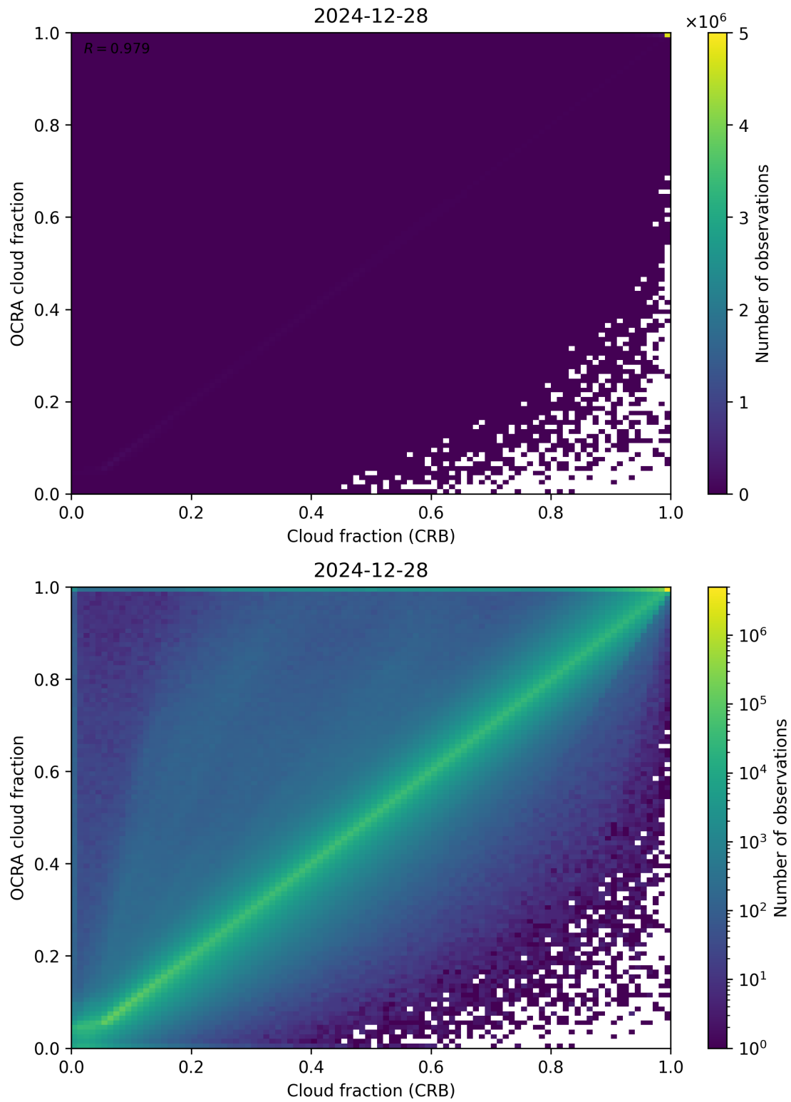
Figure 78: Scatter density plot of “Cloud fraction (CRB)” against “OCRA cloud fraction” for 2024-12-27 to 2024-12-29.
