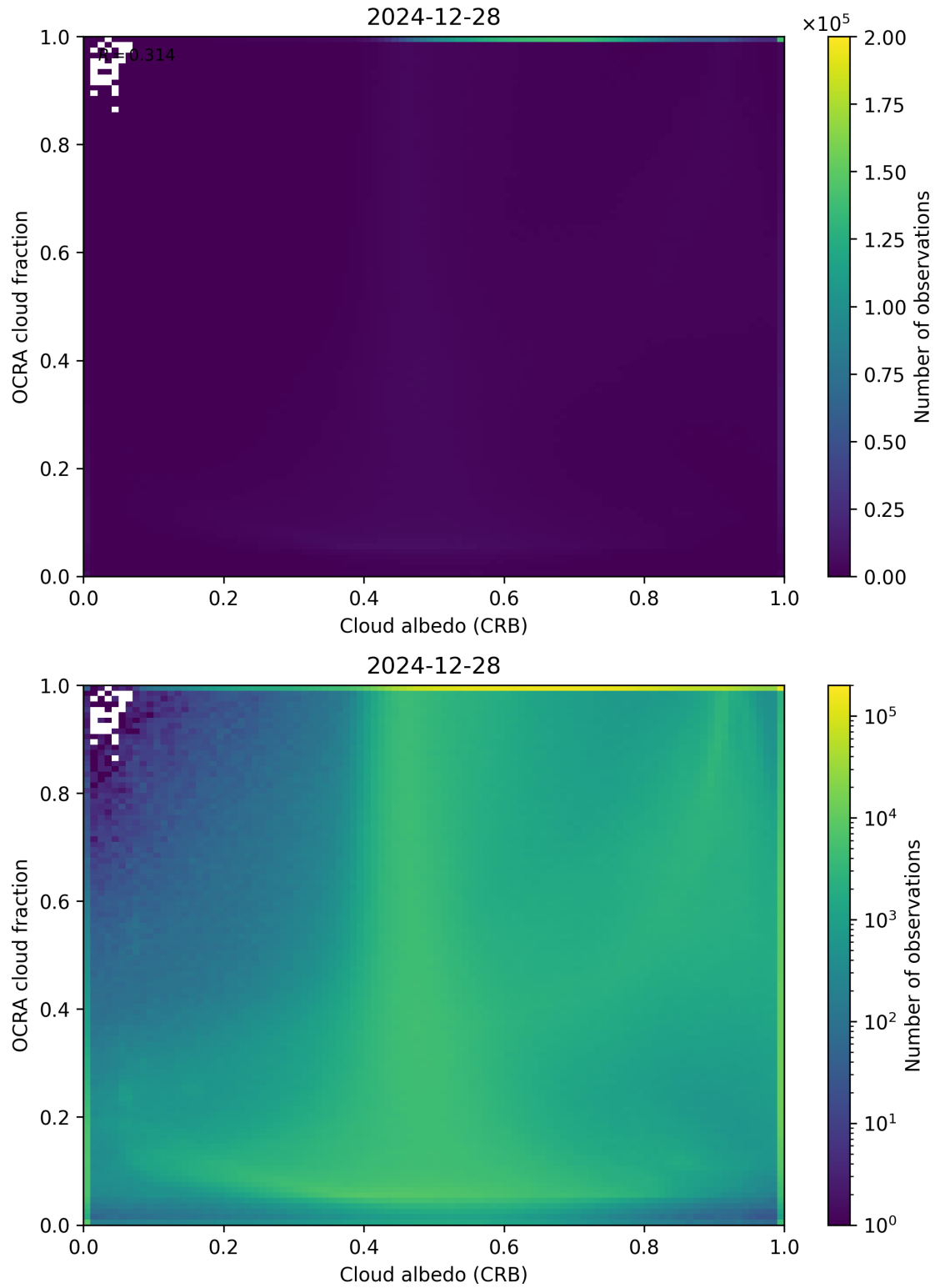
Figure 70: Scatter density plot of “Cloud albedo (CRB)” against “OCRA cloud fraction” for 2024-12-27 to 2024-12-29.
