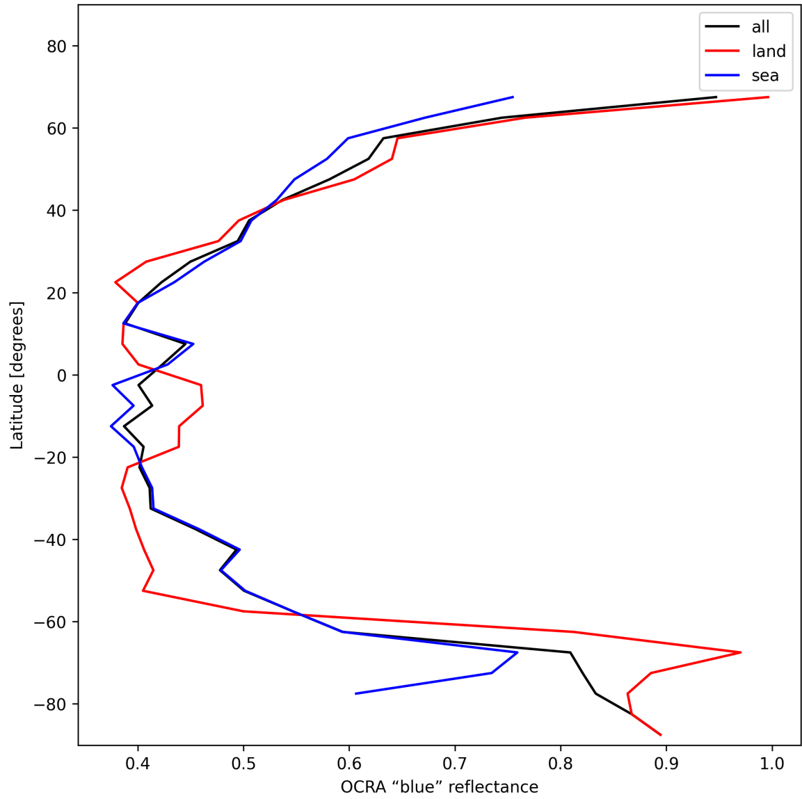
Figure 35: Zonal average of “OCRA “blue” reflectance” for 2024-12-27 to 2024-12-29.
