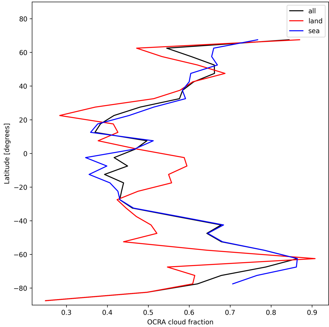
Figure 34: Zonal average of “OCRA cloud fraction” for 2024-12-27 to 2024-12-29.
