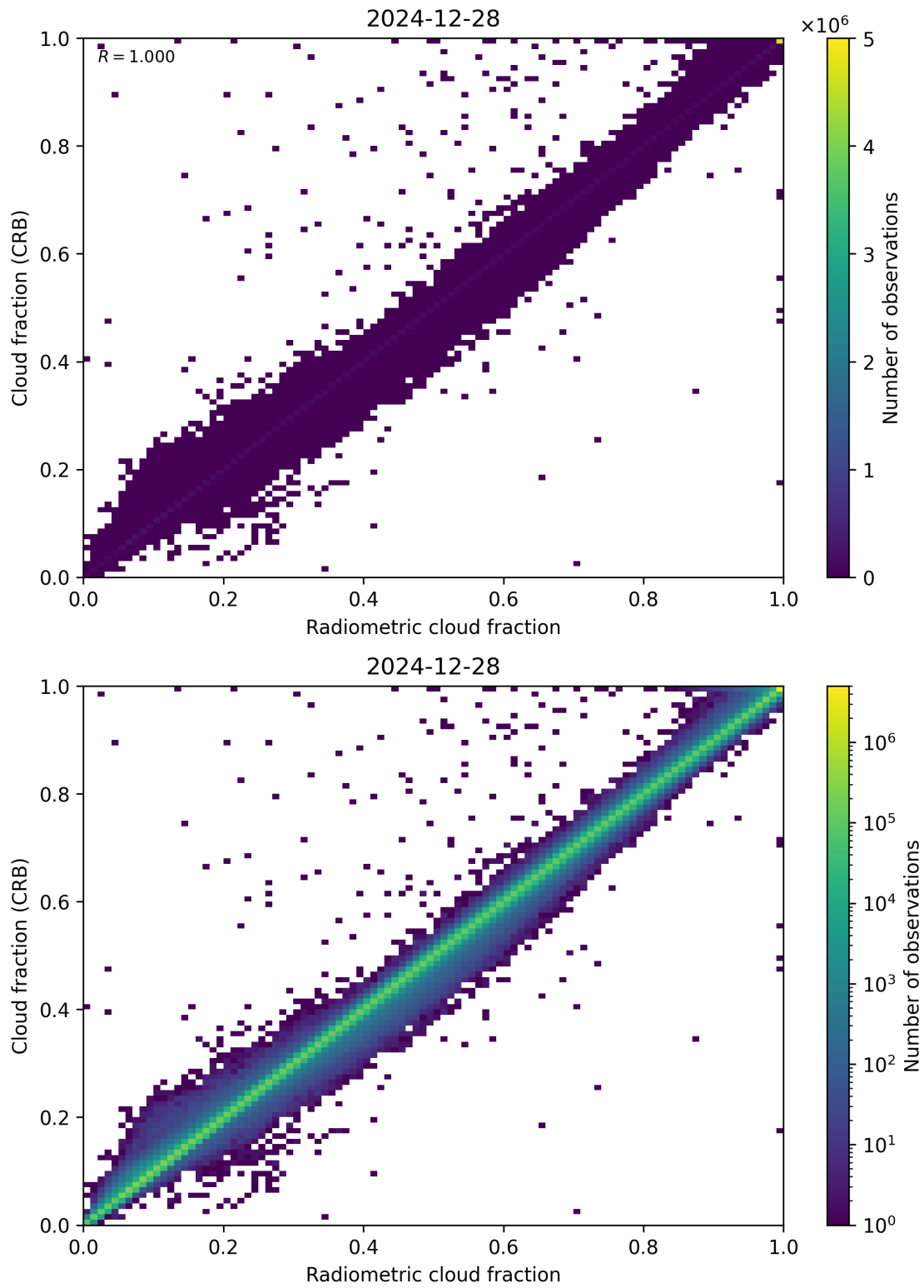
Figure 73: Scatter density plot of “Radiometric cloud fraction” against “Cloud fraction (CRB)” for 2024-12-27 to 2024-12-29.
