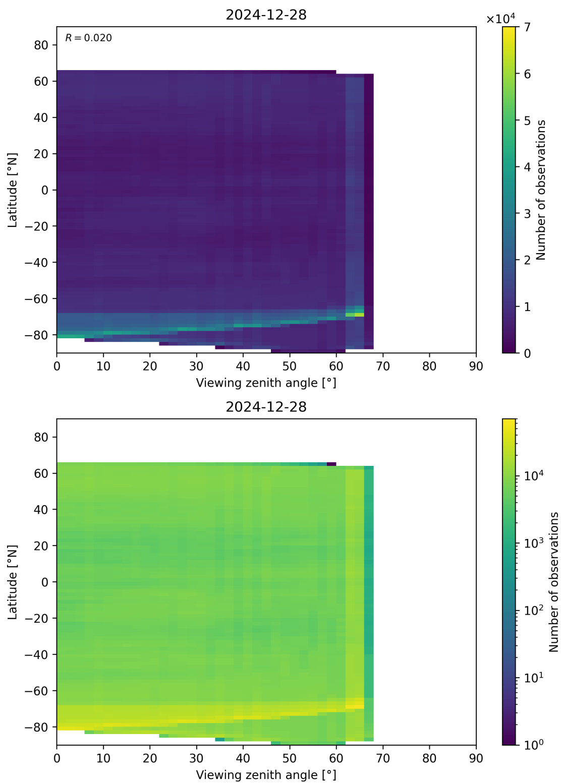
Figure 113: Scatter density plot of “Viewing zenith angle” against “Latitude” for 2024-12-27 to 2024-12-29.
