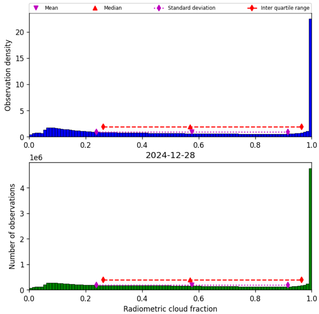
Figure 39: Histogram of “Radiometric cloud fraction” for 2024-12-27 to 2024-12-29
