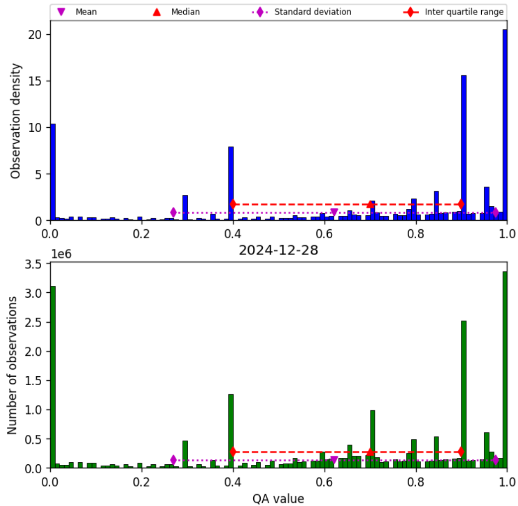
Figure 38: Histogram of “QA value” for 2024-12-27 to 2024-12-29
