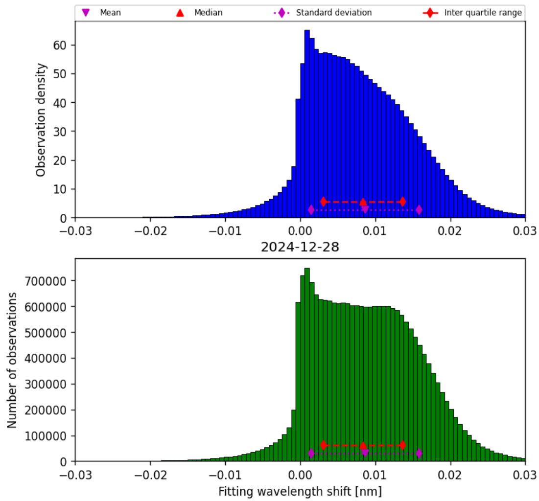
Figure 49: Histogram of “Fitting wavelength shift” for 2024-12-27 to 2024-12-29
