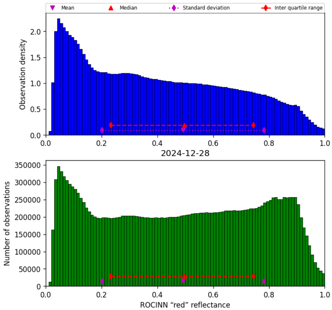
Figure 53: Histogram of “ROCINN “red” reflectance” for 2024-12-27 to 2024-12-29
