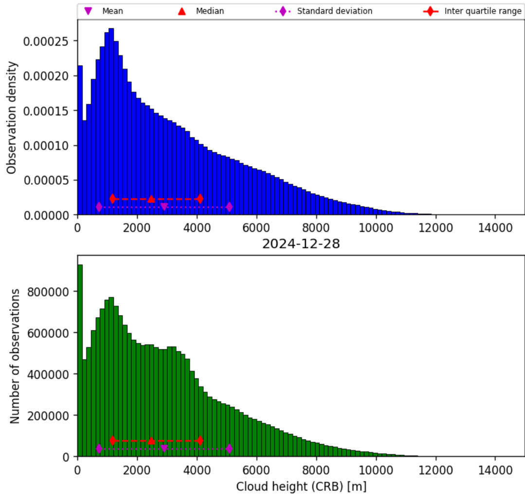
Figure 43: Histogram of “Cloud height (CRB)” for 2024-12-27 to 2024-12-29
