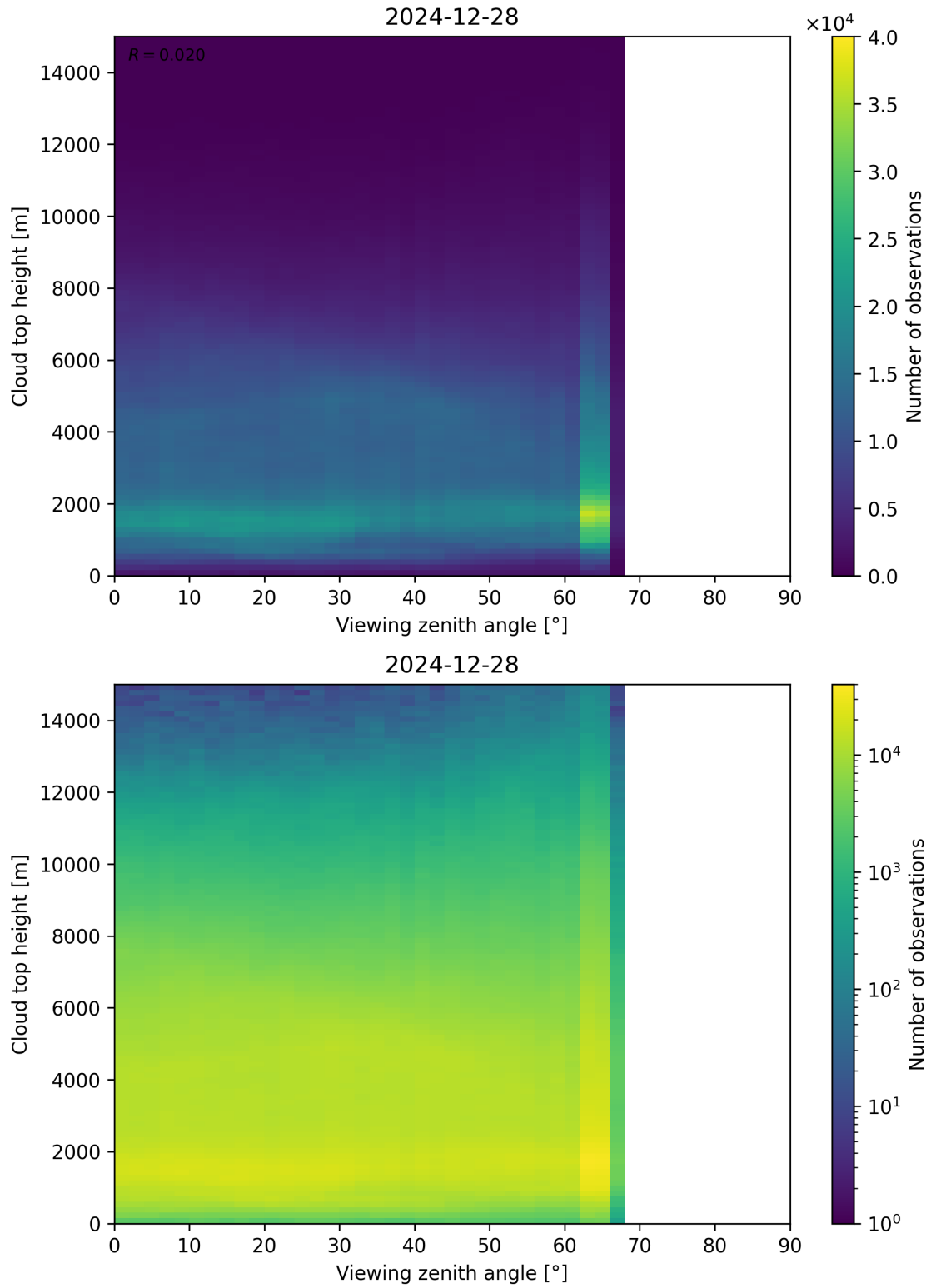
Figure 112: Scatter density plot of “Viewing zenith angle” against “Cloud top height” for 2024-12-27 to 2024-12-29.
