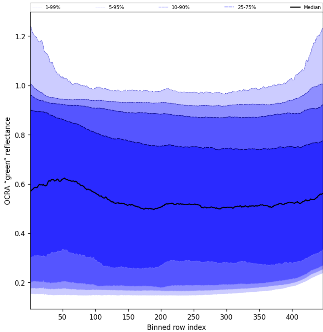
Figure 68: Along track statistics of “OCRA “green” reflectance” for 2024-12-27 to 2024-12-29
