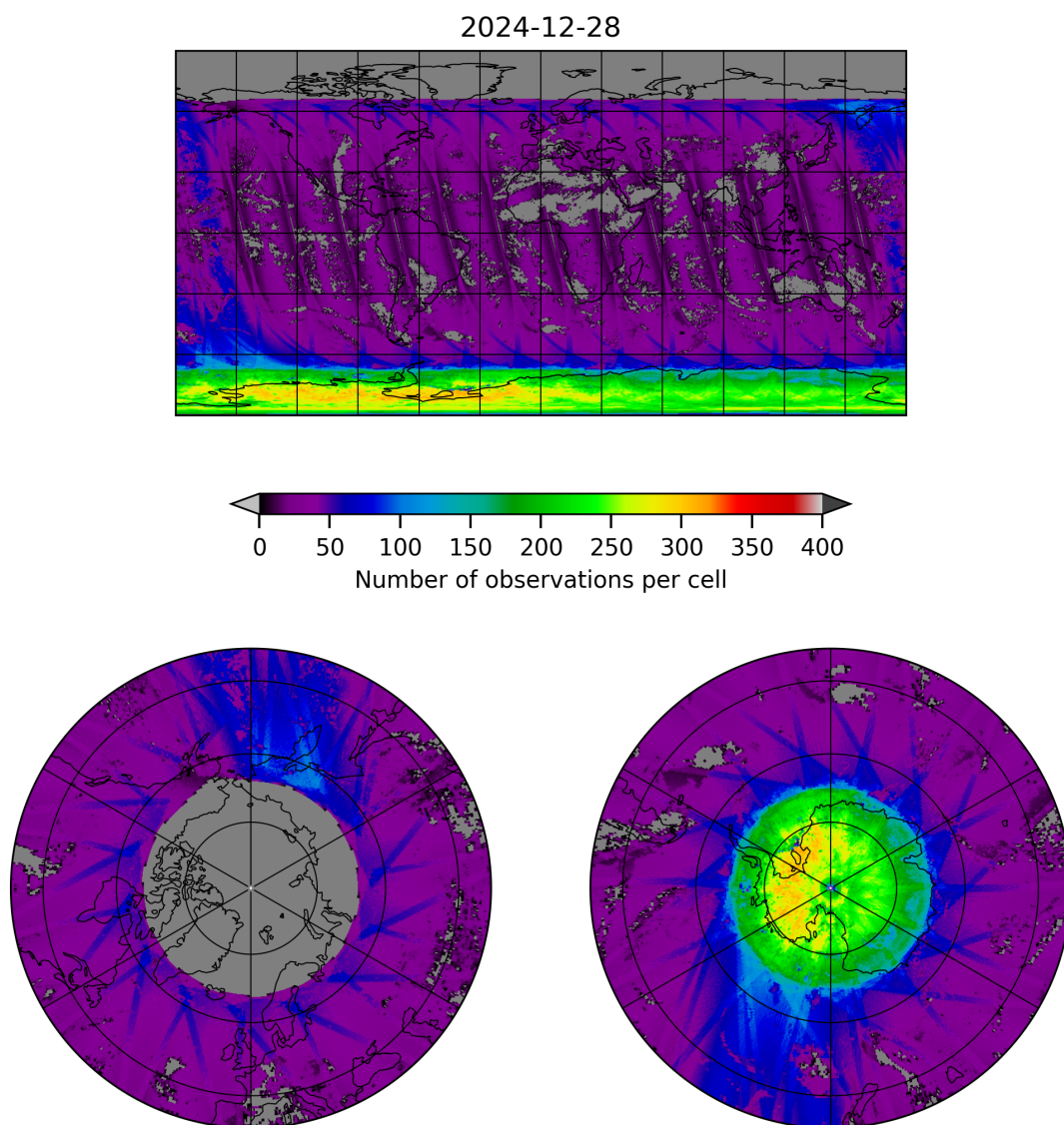
Figure 21: Map of the number of observations for 2024-12-27 to 2024-12-29
