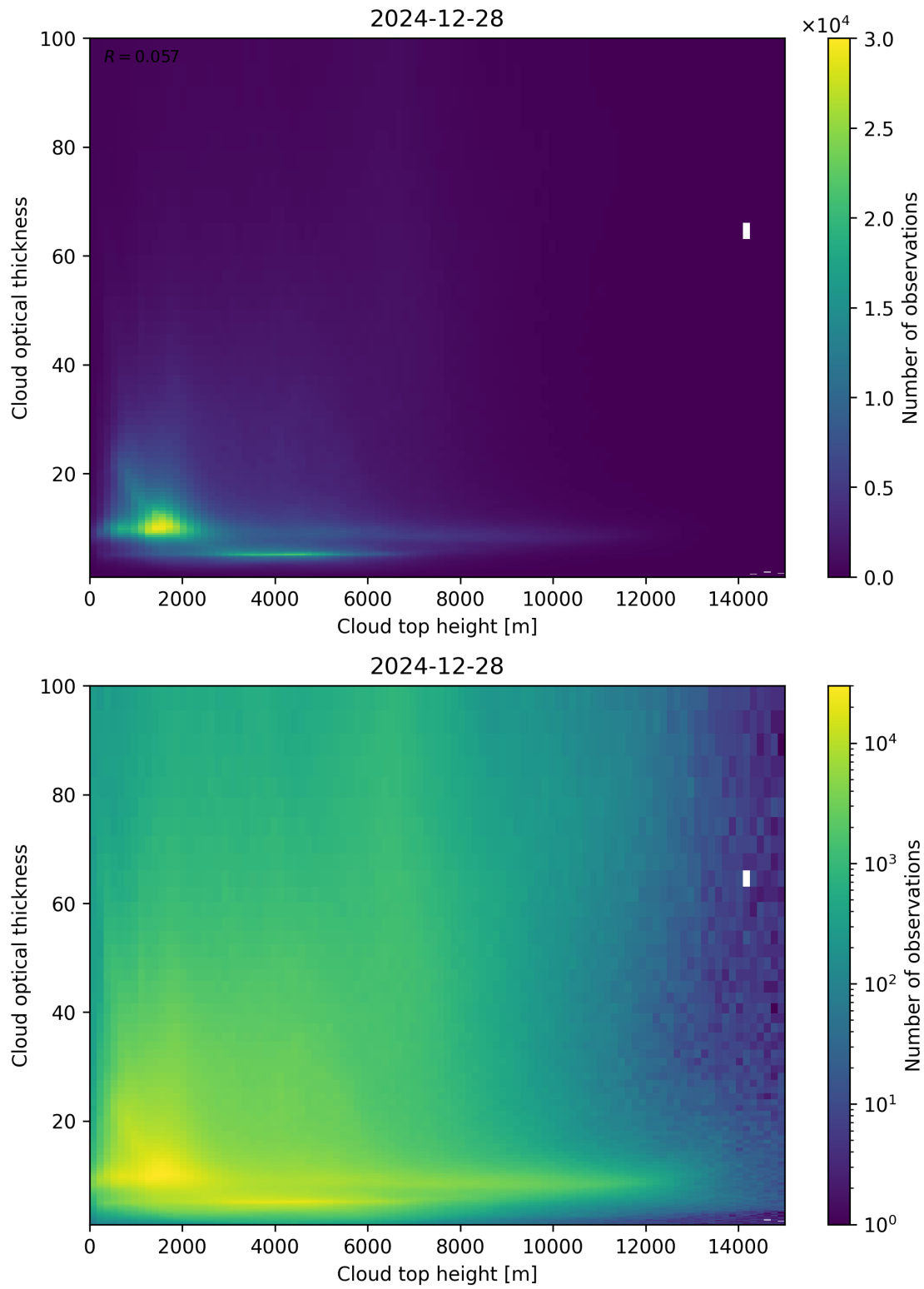
Figure 90: Scatter density plot of “Cloud top height” against “Cloud optical thickness” for 2024-12-27 to 2024-12-29.
