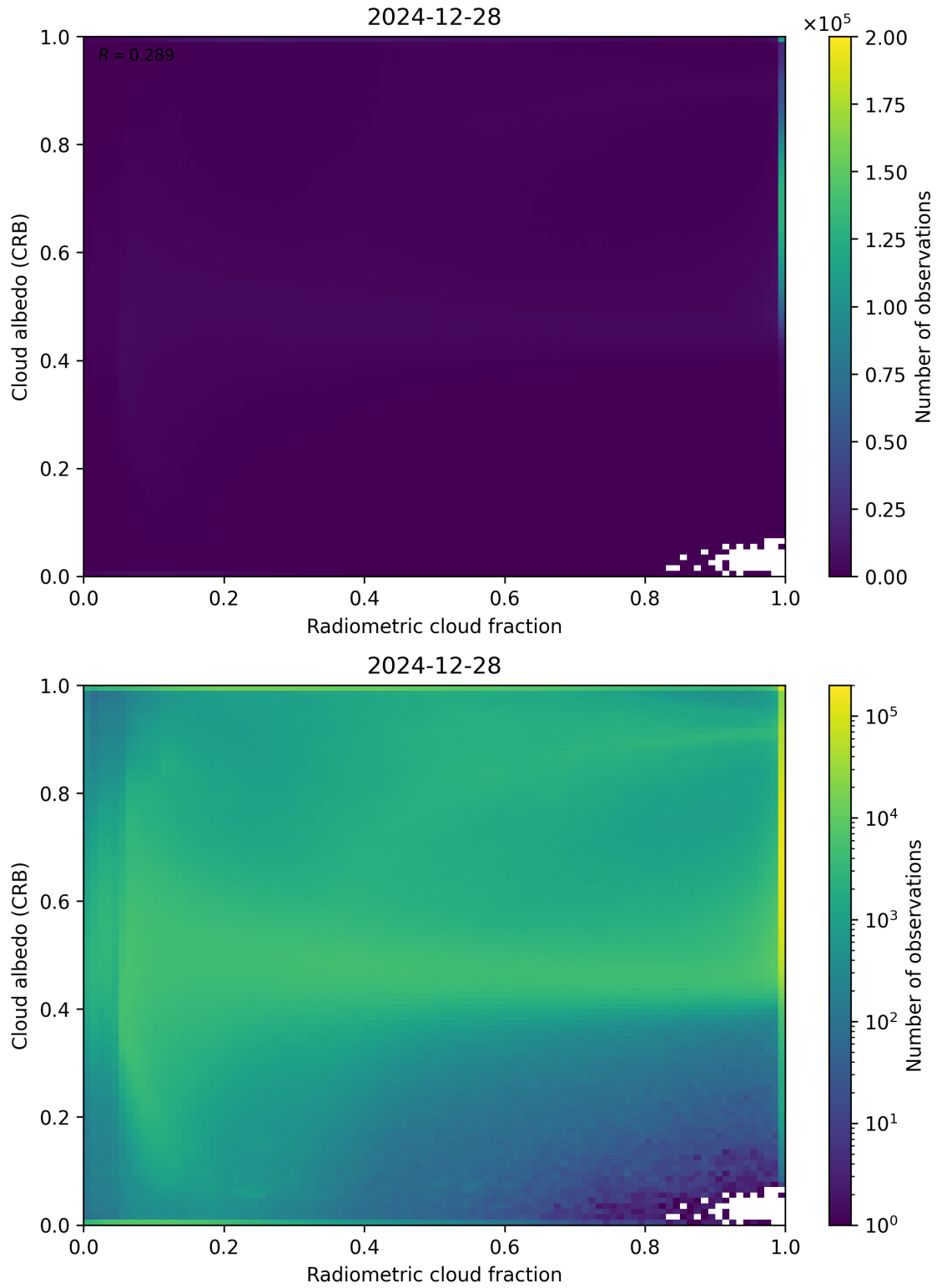
Figure 71: Scatter density plot of “Radiometric cloud fraction” against “Cloud albedo (CRB)” for 2024-12-27 to 2024-12-29.
