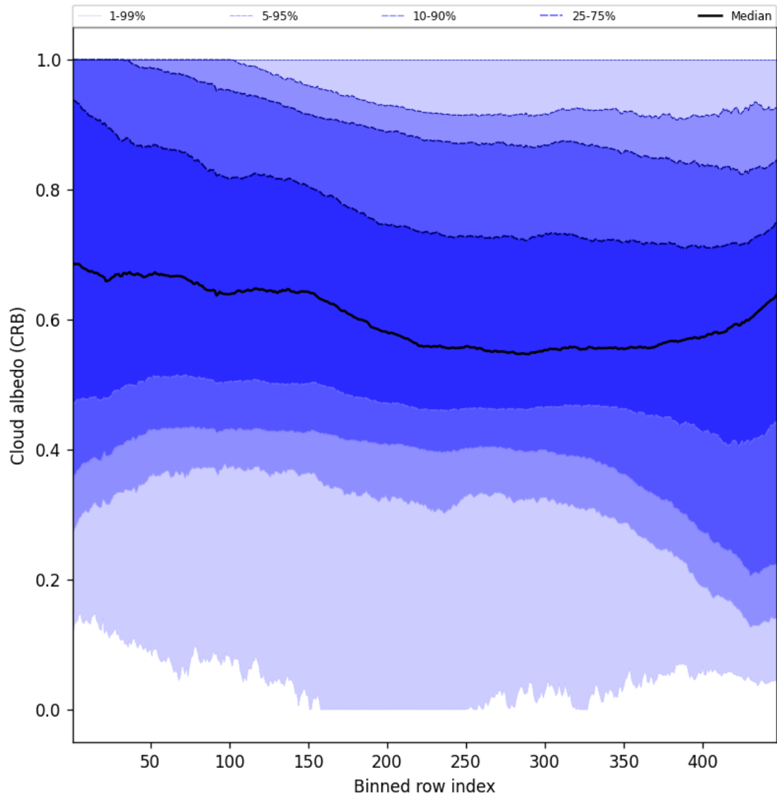
Figure 60: Along track statistics of “Cloud albedo (CRB)” for 2024-12-27 to 2024-12-29
