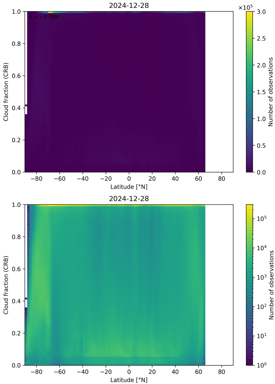
Figure 94: Scatter density plot of “Latitude” against “Cloud fraction (CRB)” for 2024-12-27 to 2024-12-29.
