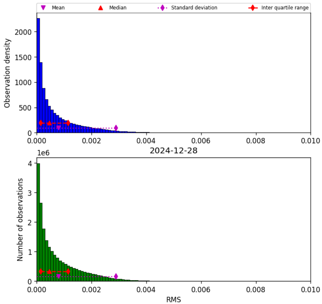
Figure 47: Histogram of “RMS” for 2024-12-27 to 2024-12-29
