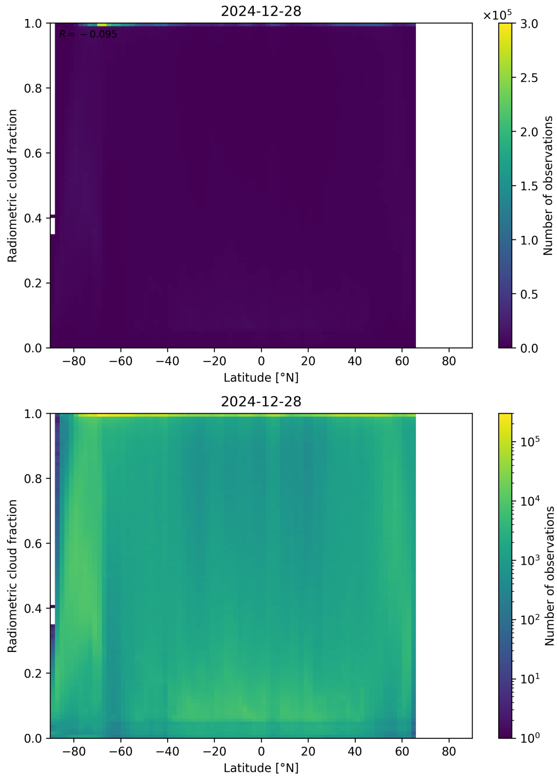
Figure 92: Scatter density plot of “Latitude” against “Radiometric cloud fraction” for 2024-12-27 to 2024-12-29.
