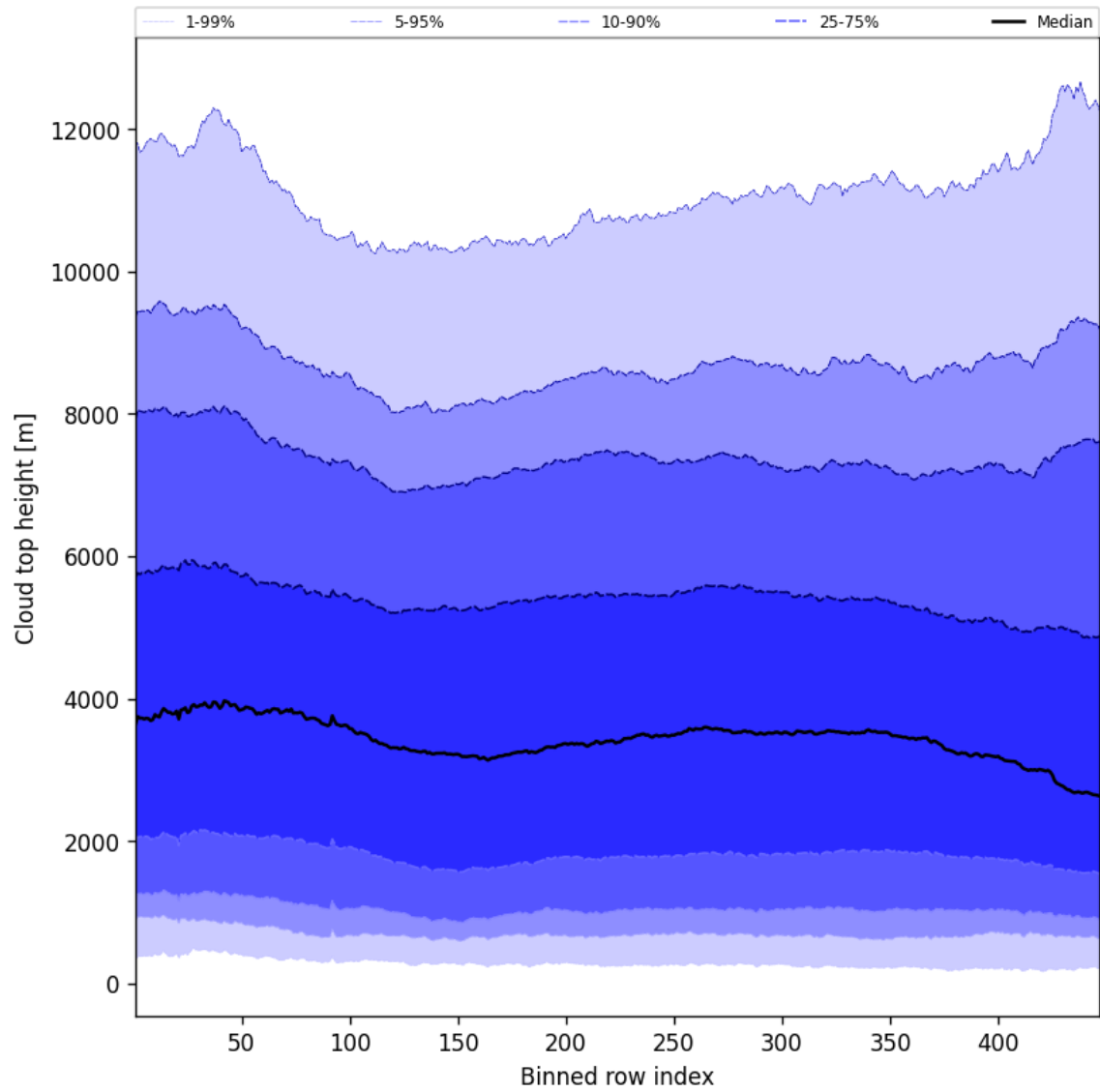
Figure 56: Along track statistics of “Cloud top height” for 2024-12-27 to 2024-12-29
