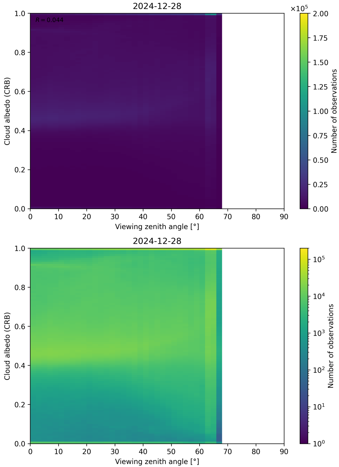
Figure 106: Scatter density plot of “Viewing zenith angle” against “Cloud albedo (CRB)” for 2024-12-27 to 2024-12-29.
