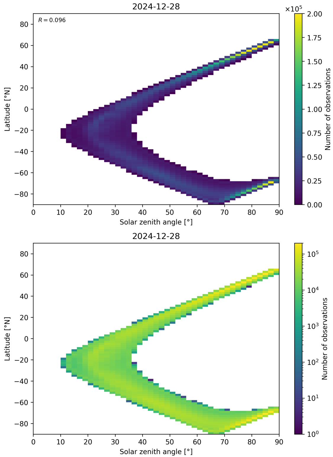
Figure 105: Scatter density plot of “Solar zenith angle” against “Latitude” for 2024-12-27 to 2024-12-29.
