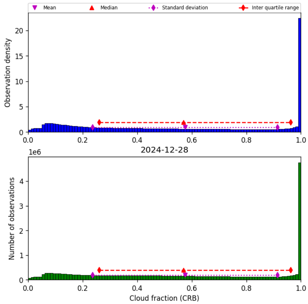
Figure 42: Histogram of “Cloud fraction (CRB)” for 2024-12-27 to 2024-12-29
