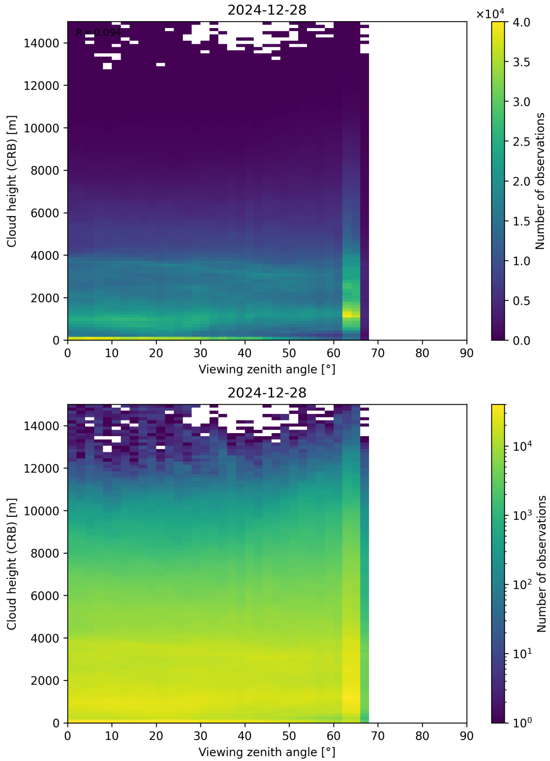
Figure 110: Scatter density plot of “Viewing zenith angle” against “Cloud height (CRB)” for 2024-12-27 to 2024-12-29.
