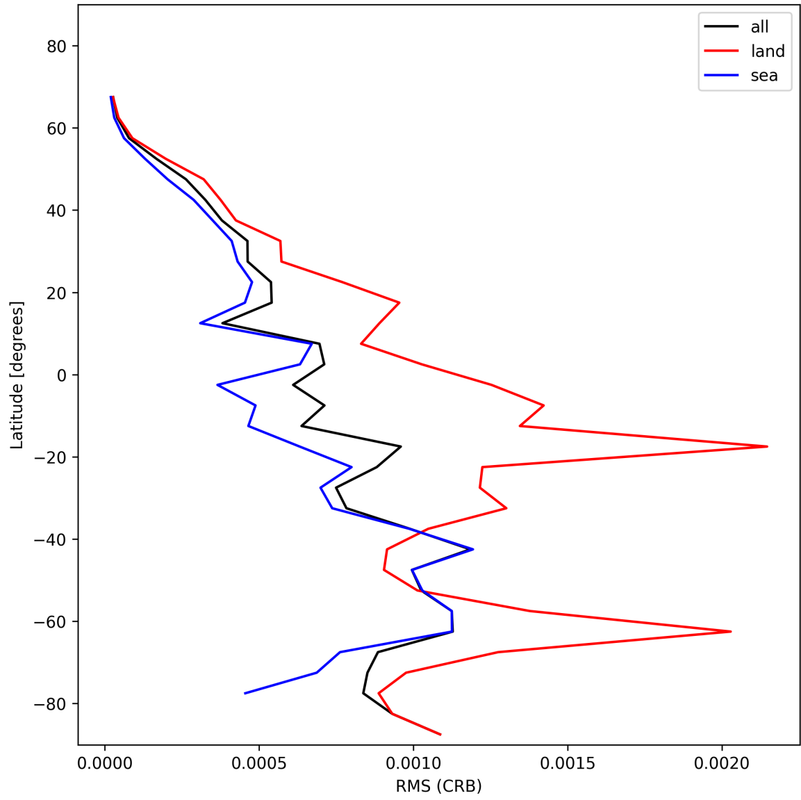
Figure 32: Zonal average of “RMS (CRB)” for 2024-12-27 to 2024-12-29.
