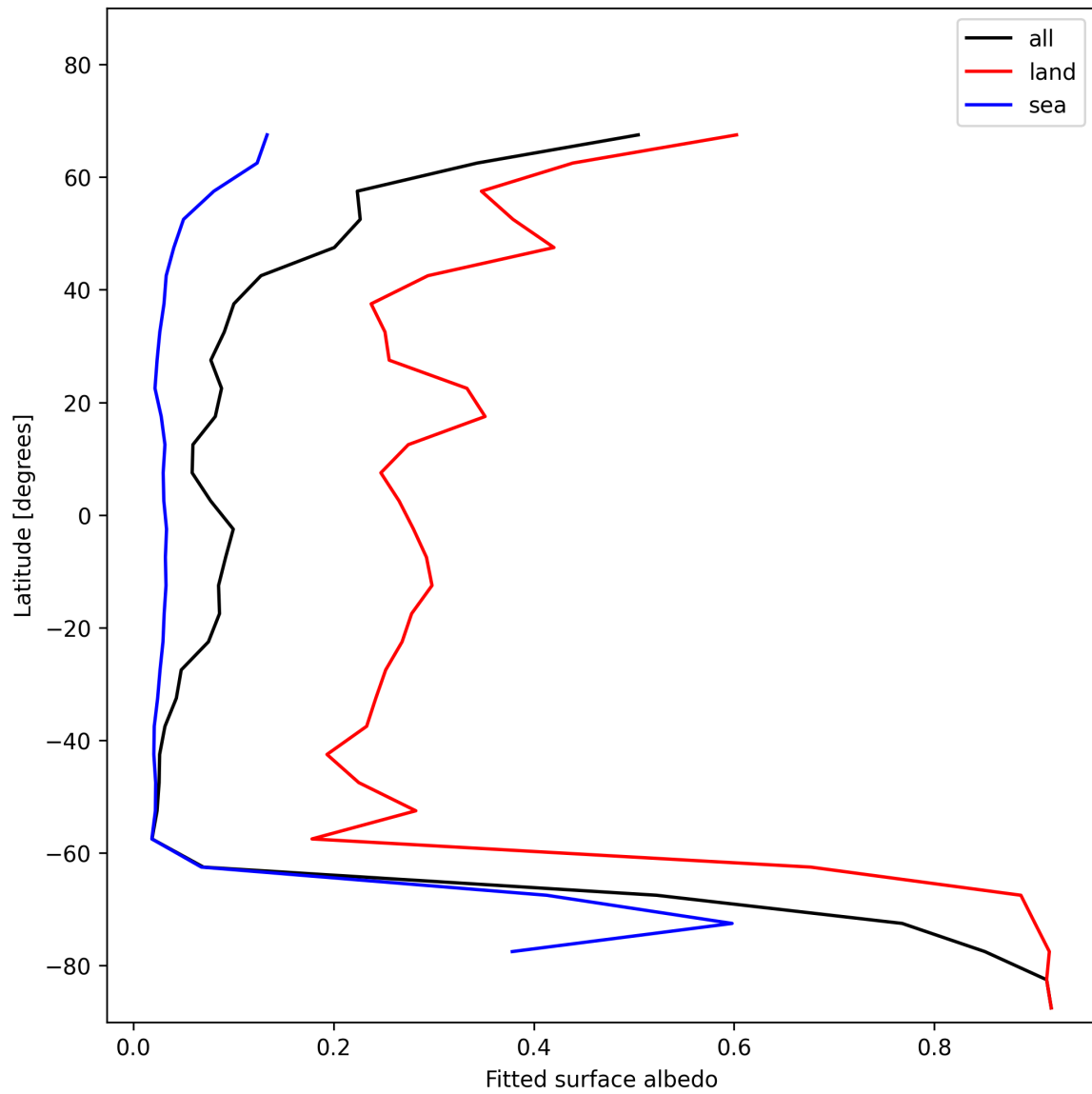
Figure 29: Zonal average of “Fitted surface albedo” for 2024-12-27 to 2024-12-29.
