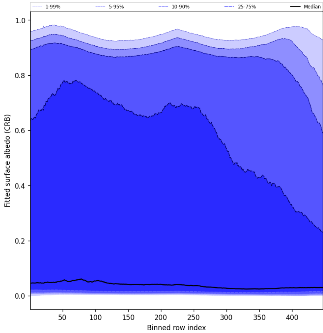
Figure 62: Along track statistics of “Fitted surface albedo (CRB)” for 2024-12-27 to 2024-12-29
