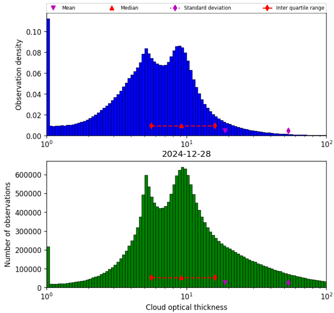
Figure 41: Histogram of “Cloud optical thickness” for 2024-12-27 to 2024-12-29
