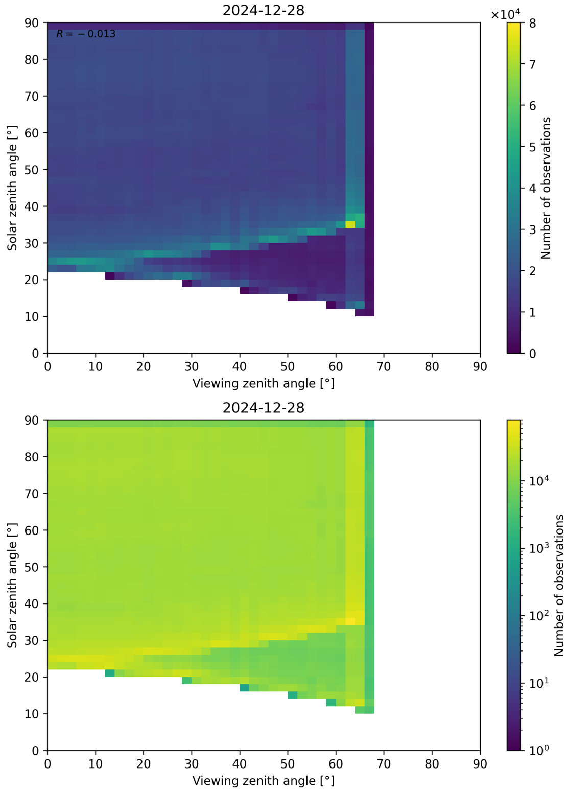
Figure 114: Scatter density plot of “Viewing zenith angle” against “Solar zenith angle” for 2024-12-27 to 2024-12-29.
