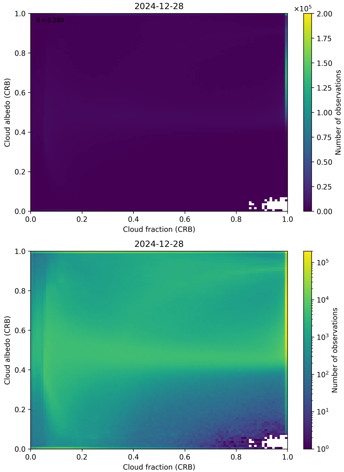
Figure 77: Scatter density plot of “Cloud fraction (CRB)” against “Cloud albedo (CRB)” for 2024-12-27 to 2024-12-29.
