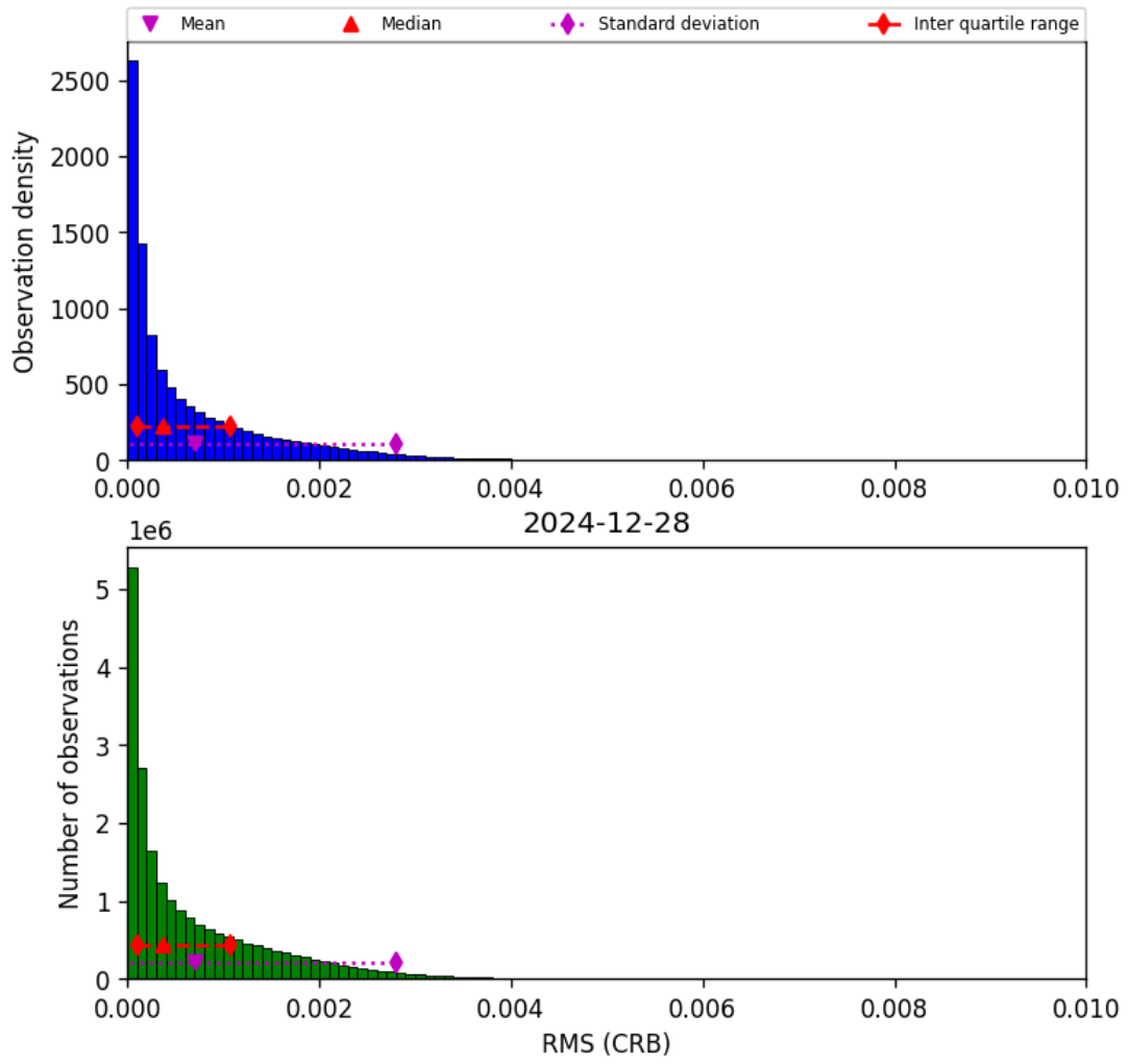
Figure 48: Histogram of “RMS (CRB)” for 2024-12-27 to 2024-12-29
