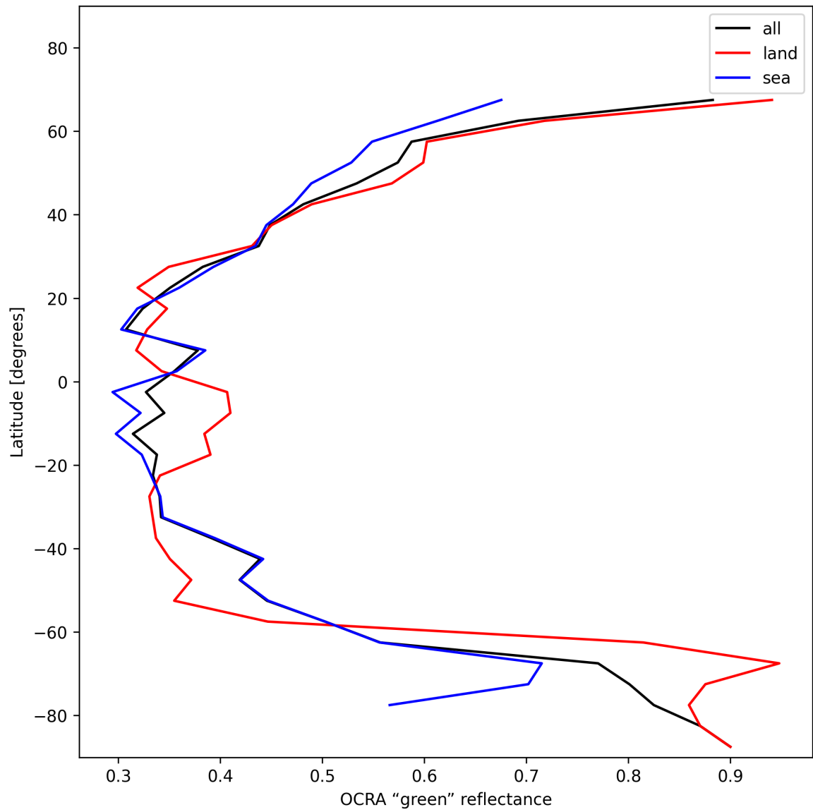
Figure 36: Zonal average of “OCRA “green” reflectance” for 2024-12-27 to 2024-12-29.
