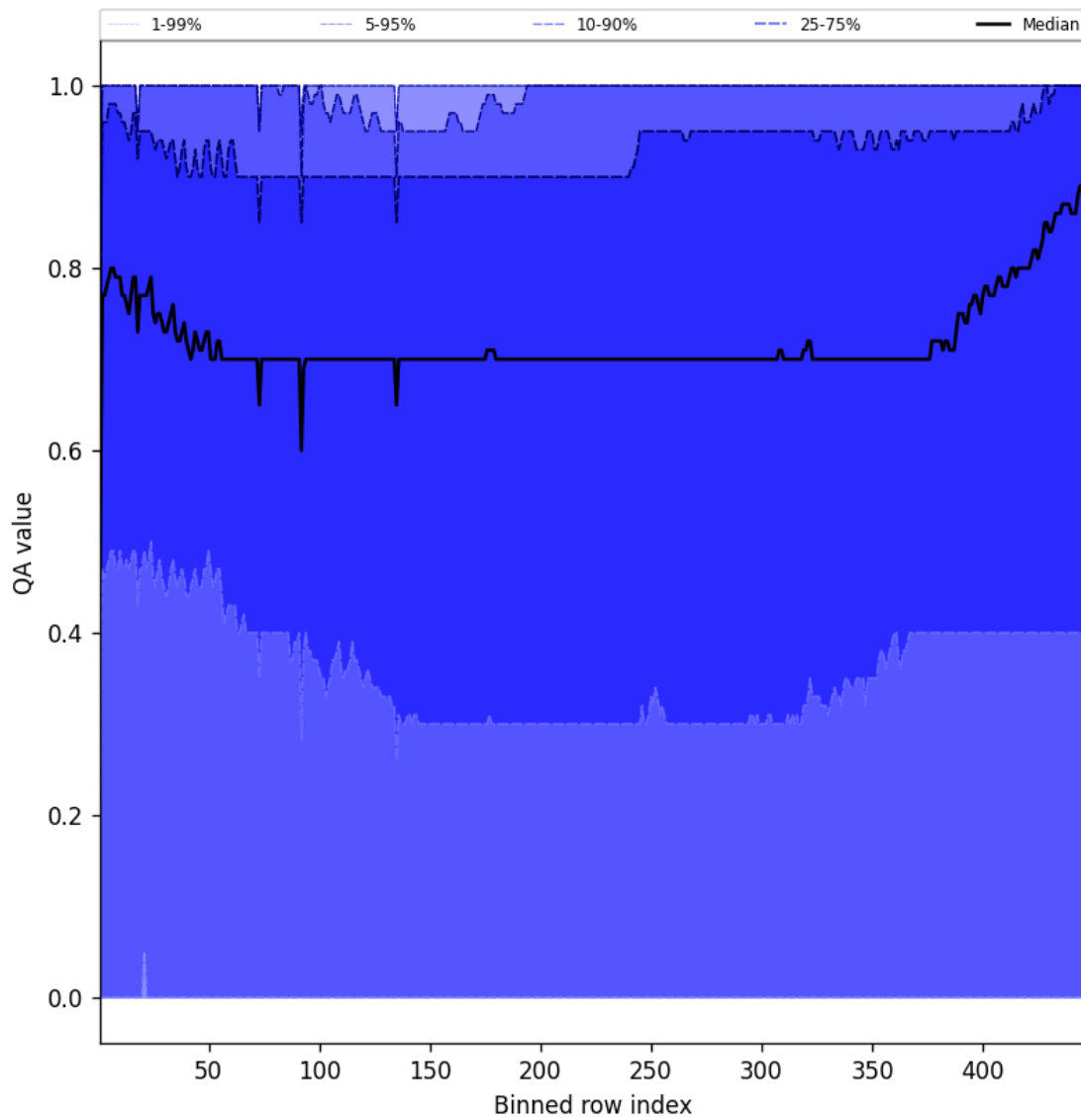
Figure 54: Along track statistics of “QA value” for 2024-12-27 to 2024-12-29
