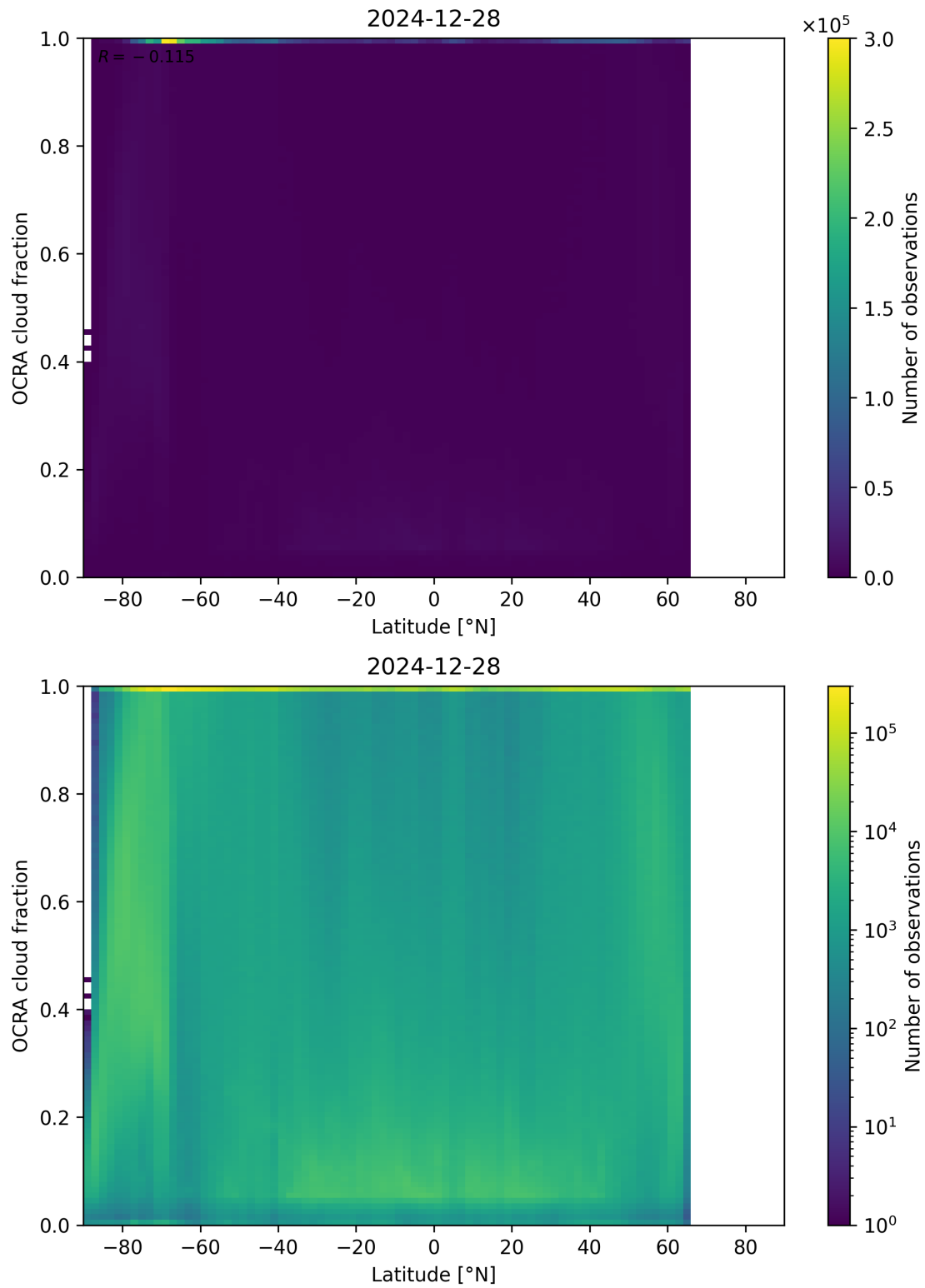
Figure 93: Scatter density plot of “Latitude” against “OCRA cloud fraction” for 2024-12-27 to 2024-12-29.
