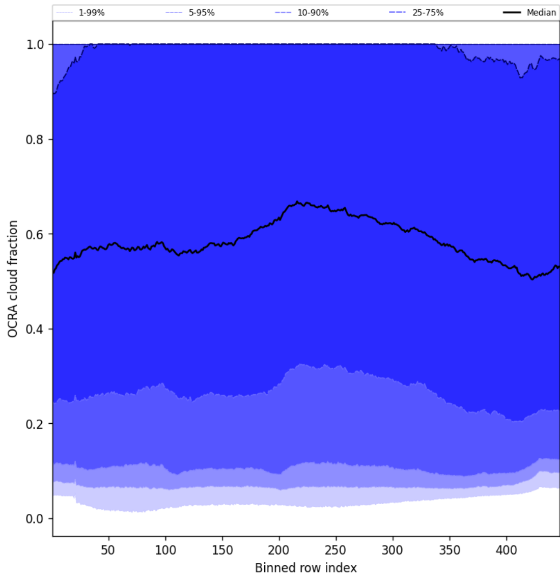
Figure 66: Along track statistics of “OCRA cloud fraction” for 2024-12-27 to 2024-12-29
