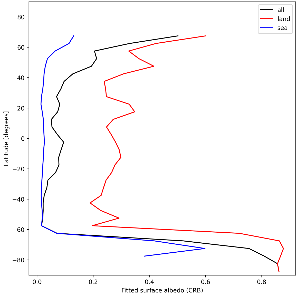
Figure 30: Zonal average of “Fitted surface albedo (CRB)” for 2024-12-27 to 2024-12-29.
