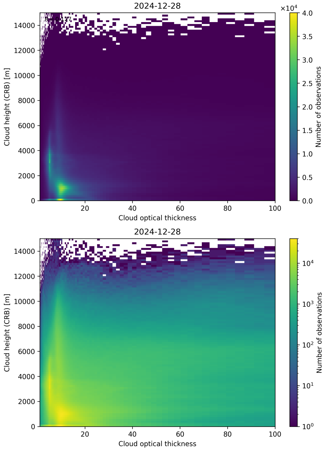
Figure 85: Scatter density plot of “Cloud optical thickness” against “Cloud height (CRB)” for 2024-12-27 to 2024-12-29.
