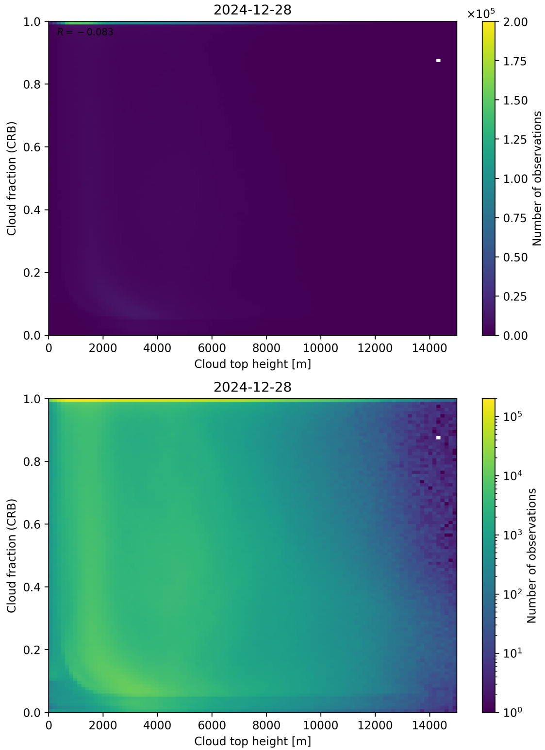
Figure 88: Scatter density plot of “Cloud top height” against “Cloud fraction (CRB)” for 2024-12-27 to 2024-12-29.
