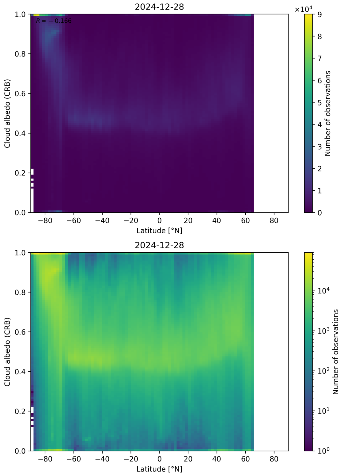
Figure 91: Scatter density plot of “Latitude” against “Cloud albedo (CRB)” for 2024-12-27 to 2024-12-29.
