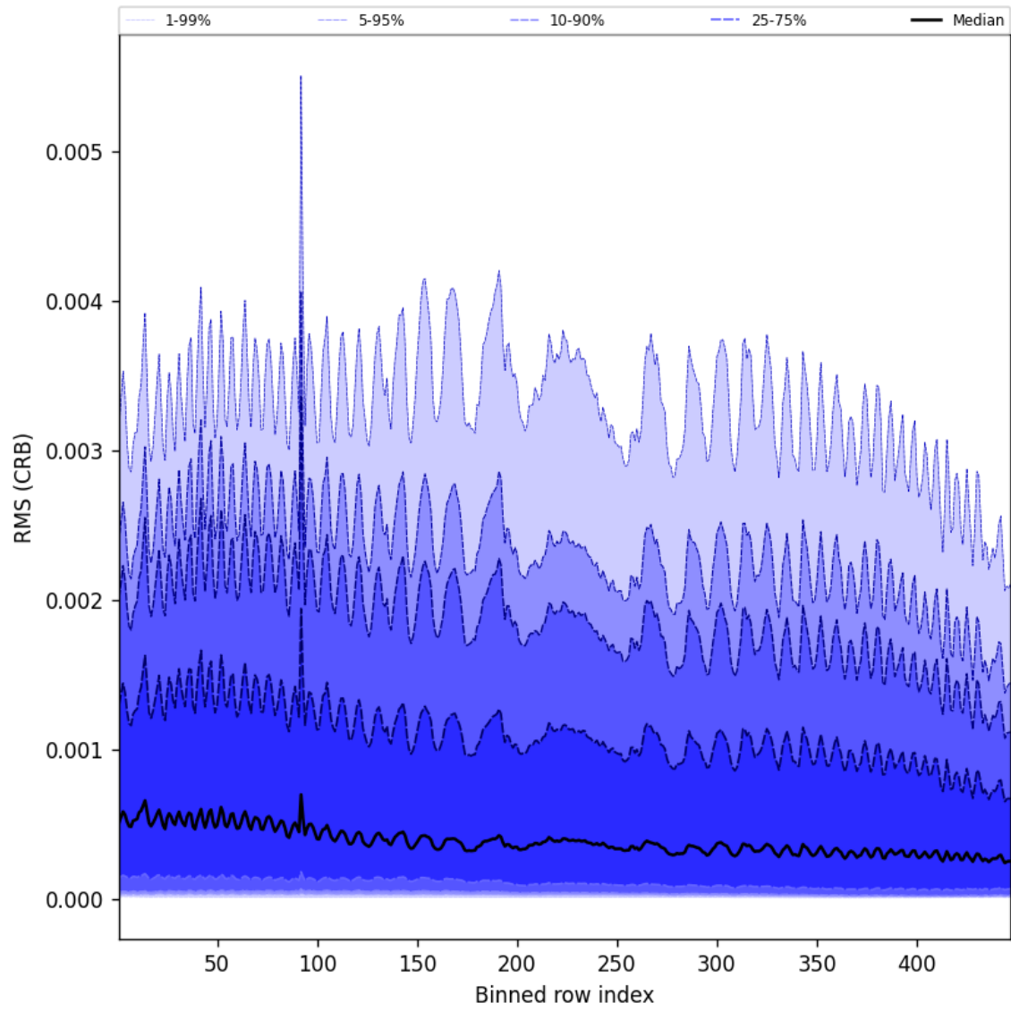
Figure 64: Along track statistics of “RMS (CRB)” for 2024-12-27 to 2024-12-29
