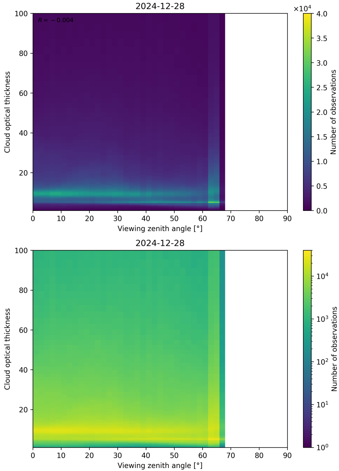
Figure 111: Scatter density plot of “Viewing zenith angle” against “Cloud optical thickness” for 2024-12-27 to 2024-12-29.
