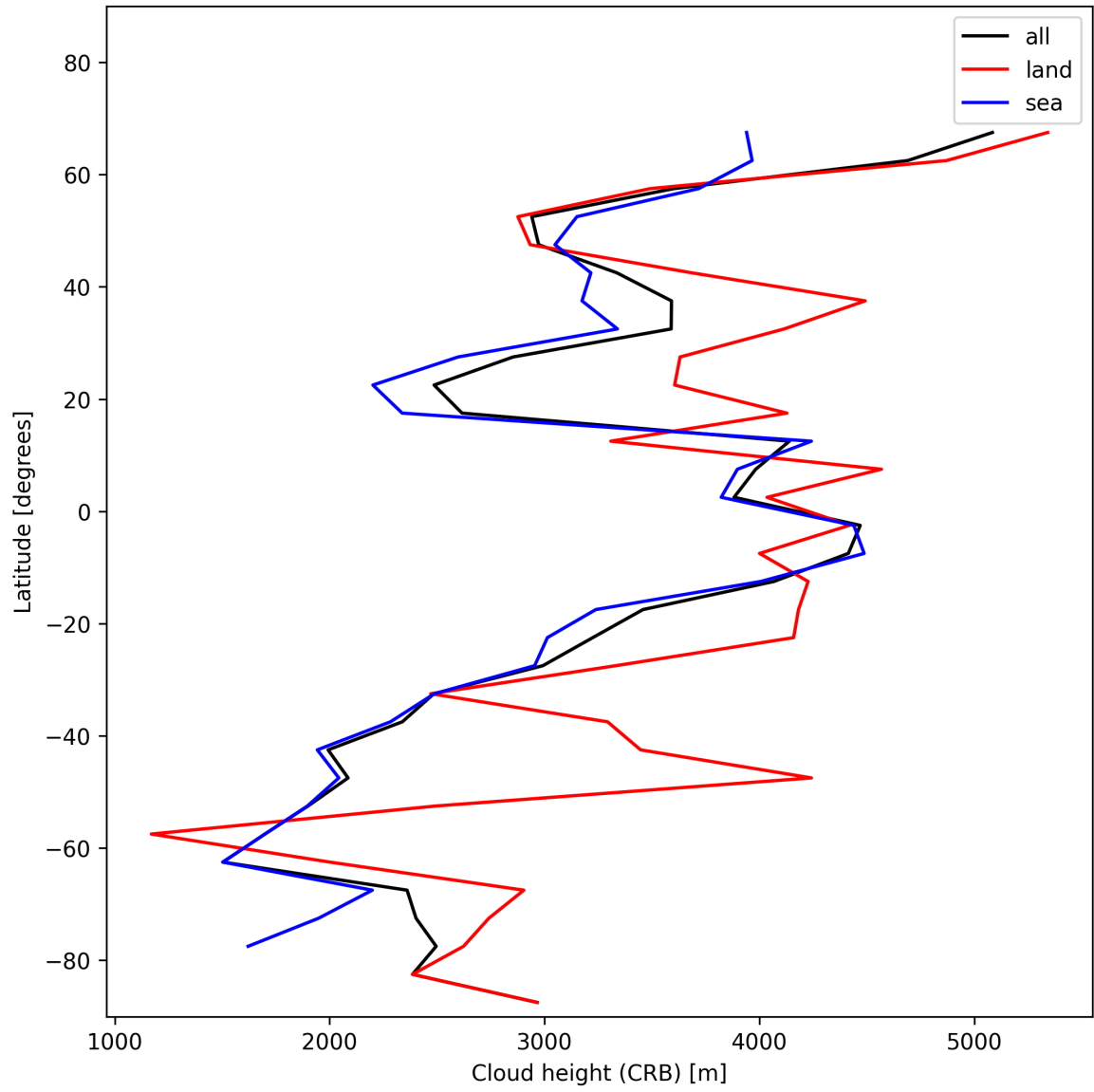
Figure 27: Zonal average of “Cloud height (CRB)” for 2024-12-27 to 2024-12-29.
