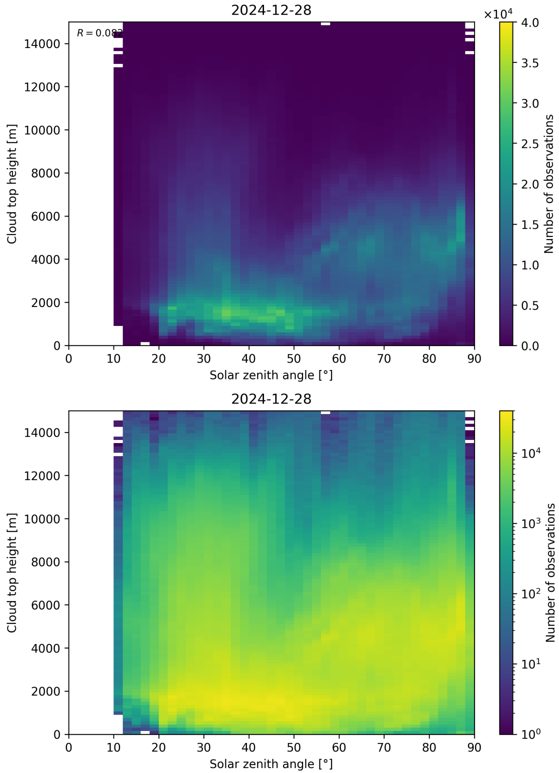
Figure 104: Scatter density plot of “Solar zenith angle” against “Cloud top height” for 2024-12-27 to 2024-12-29.
