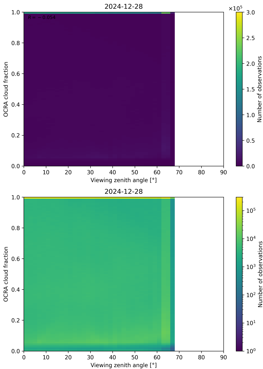
Figure 108: Scatter density plot of “Viewing zenith angle” against “OCRA cloud fraction” for 2024-12-27 to 2024-12-29.
