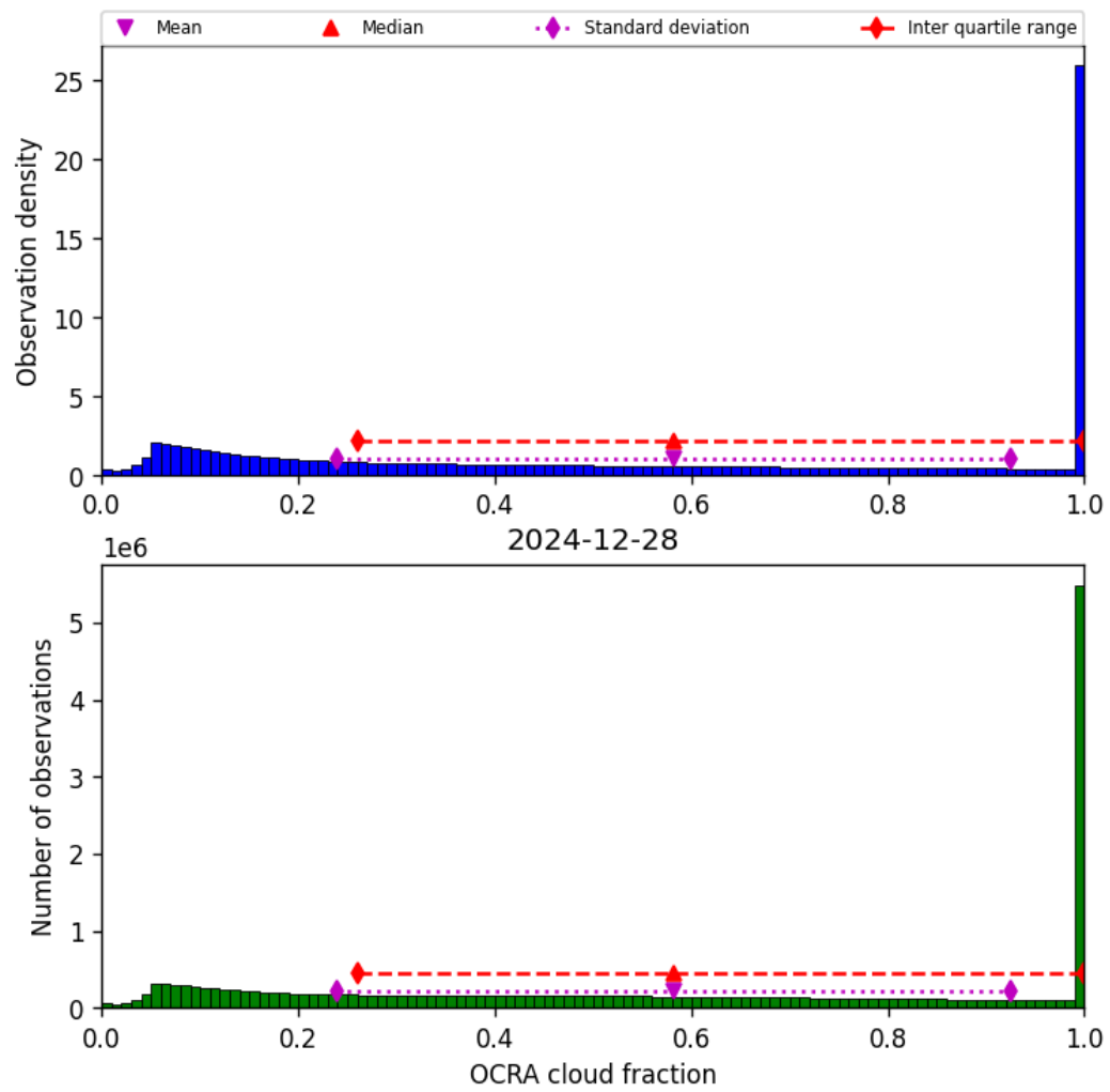
Figure 50: Histogram of “OCRA cloud fraction” for 2024-12-27 to 2024-12-29
