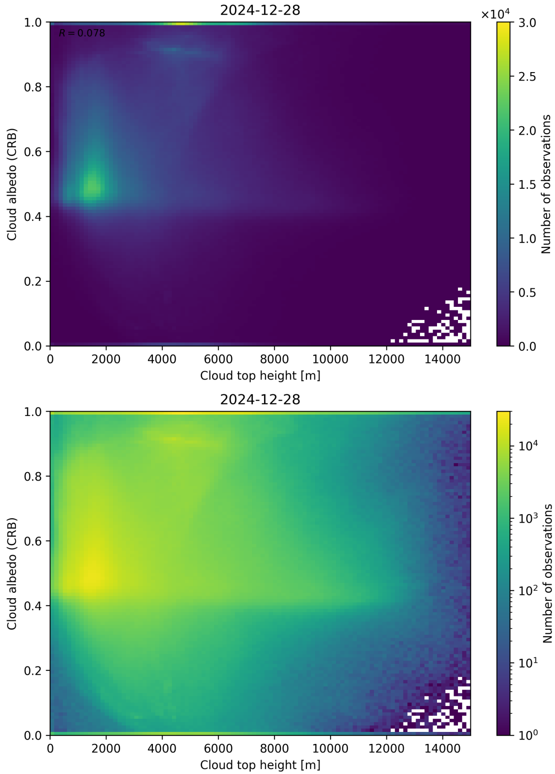
Figure 86: Scatter density plot of “Cloud top height” against “Cloud albedo (CRB)” for 2024-12-27 to 2024-12-29.
