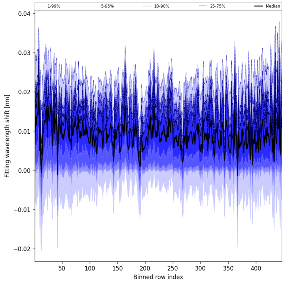
Figure 65: Along track statistics of “Fitting wavelength shift” for 2024-12-27 to 2024-12-29
