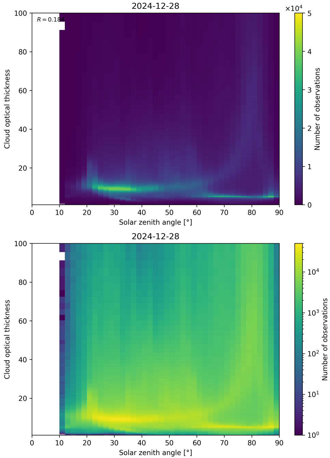
Figure 103: Scatter density plot of “Solar zenith angle” against “Cloud optical thickness” for 2024-12-27 to 2024-12-29.
