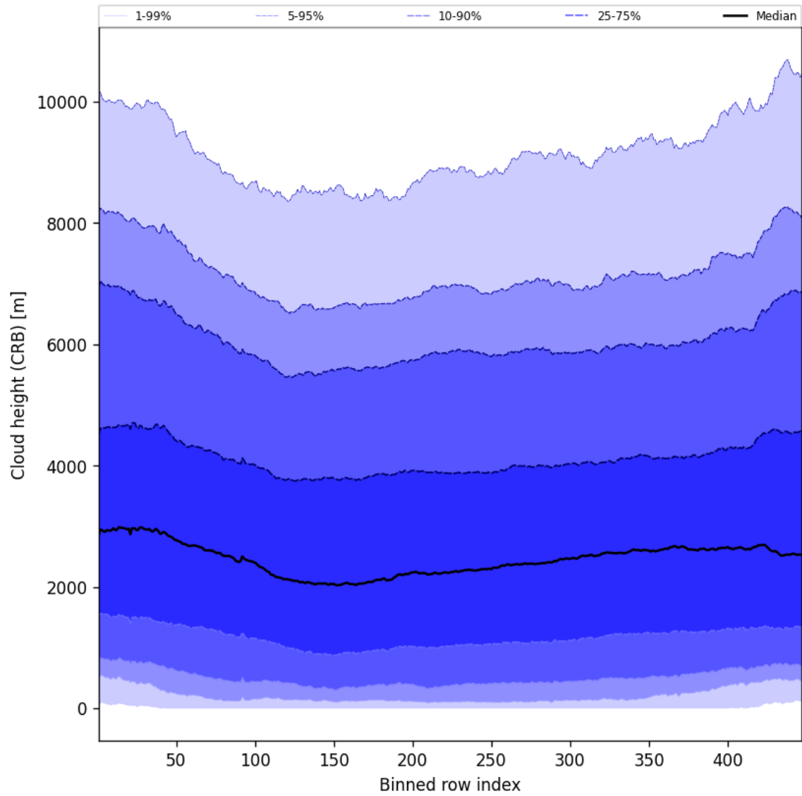
Figure 59: Along track statistics of “Cloud height (CRB)” for 2024-12-27 to 2024-12-29
