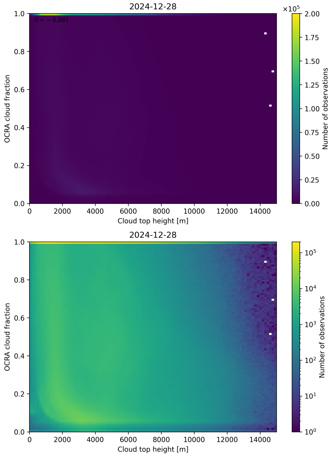
Figure 87: Scatter density plot of “Cloud top height” against “OCRA cloud fraction” for 2024-12-27 to 2024-12-29.
