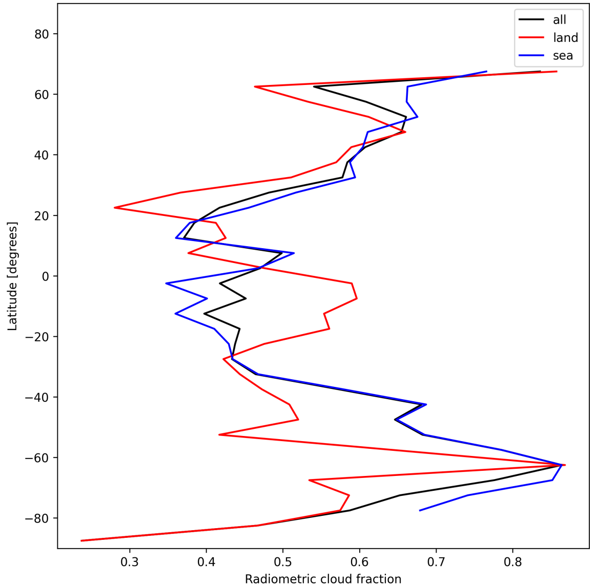
Figure 23: Zonal average of “Radiometric cloud fraction” for 2024-12-27 to 2024-12-29.
