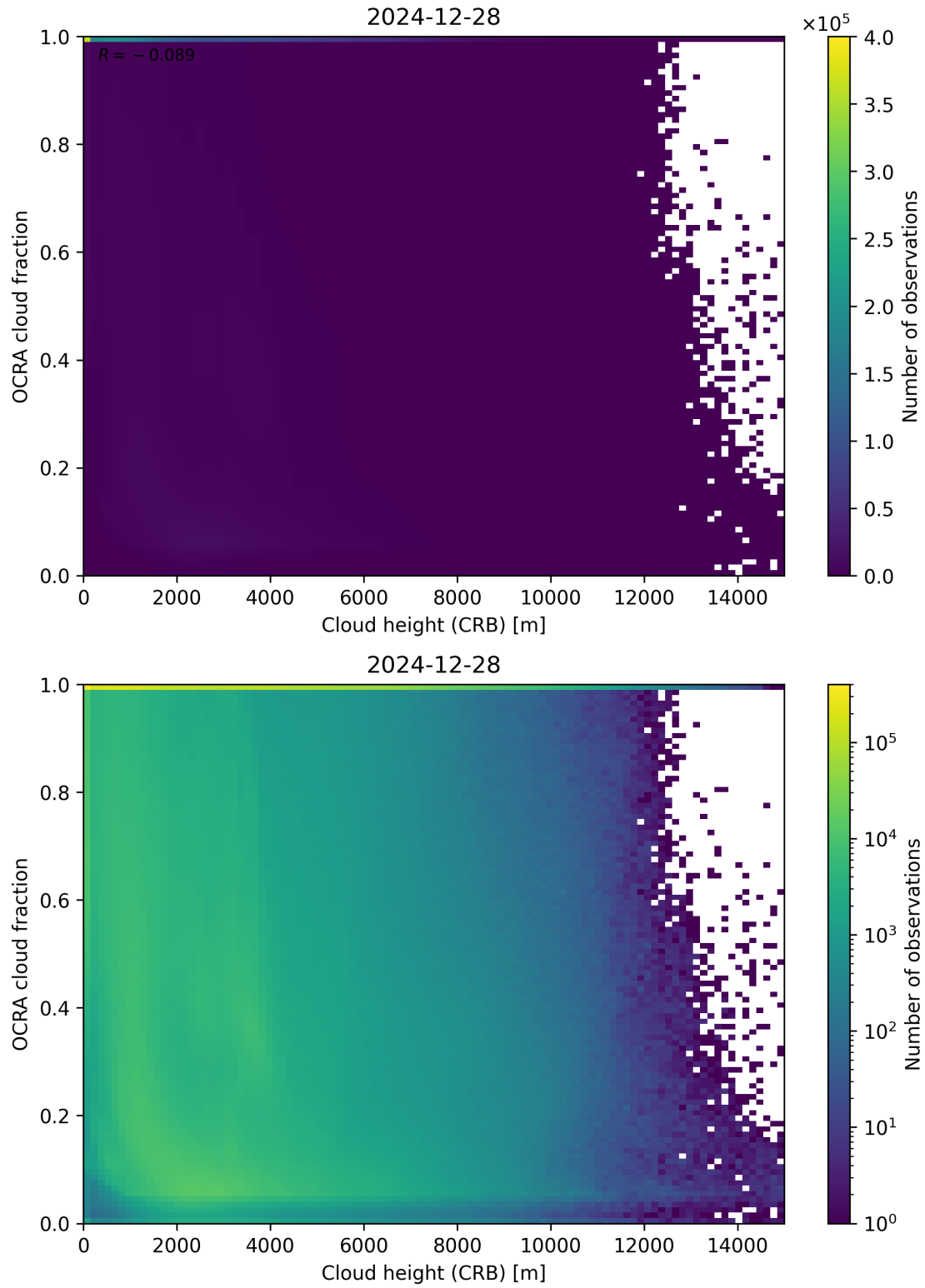
Figure 81: Scatter density plot of “Cloud height (CRB)” against “OCRA cloud fraction” for 2024-12-27 to 2024-12-29.
