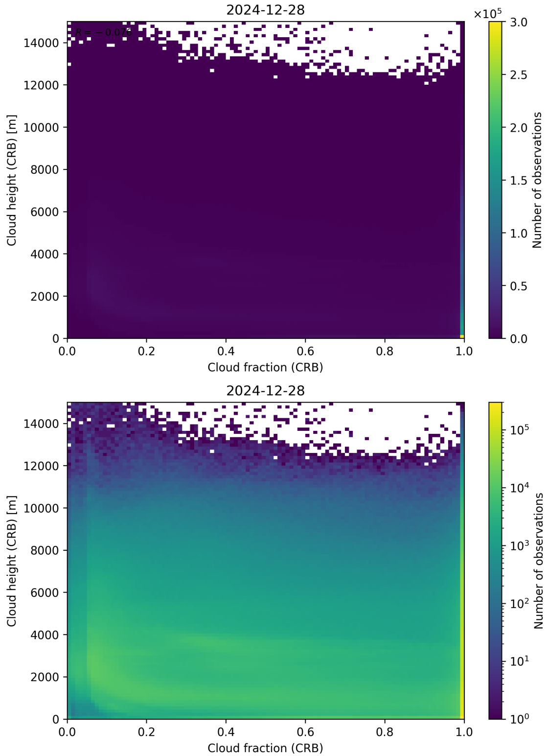
Figure 79: Scatter density plot of “Cloud fraction (CRB)” against “Cloud height (CRB)” for 2024-12-27 to 2024-12-29.
