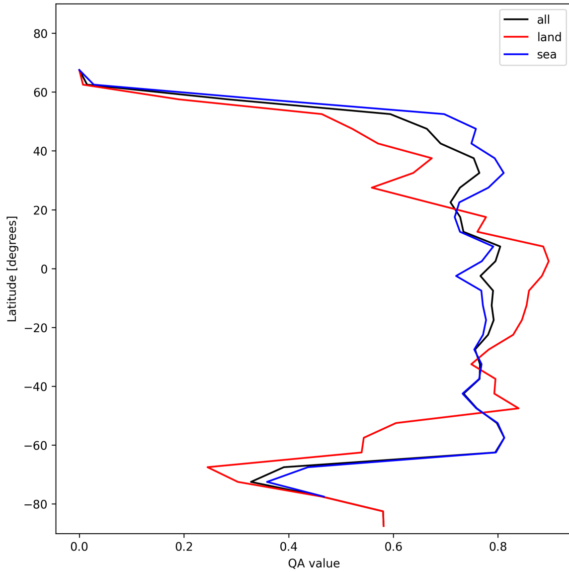
Figure 22: Zonal average of “QA value” for 2024-12-27 to 2024-12-29.
