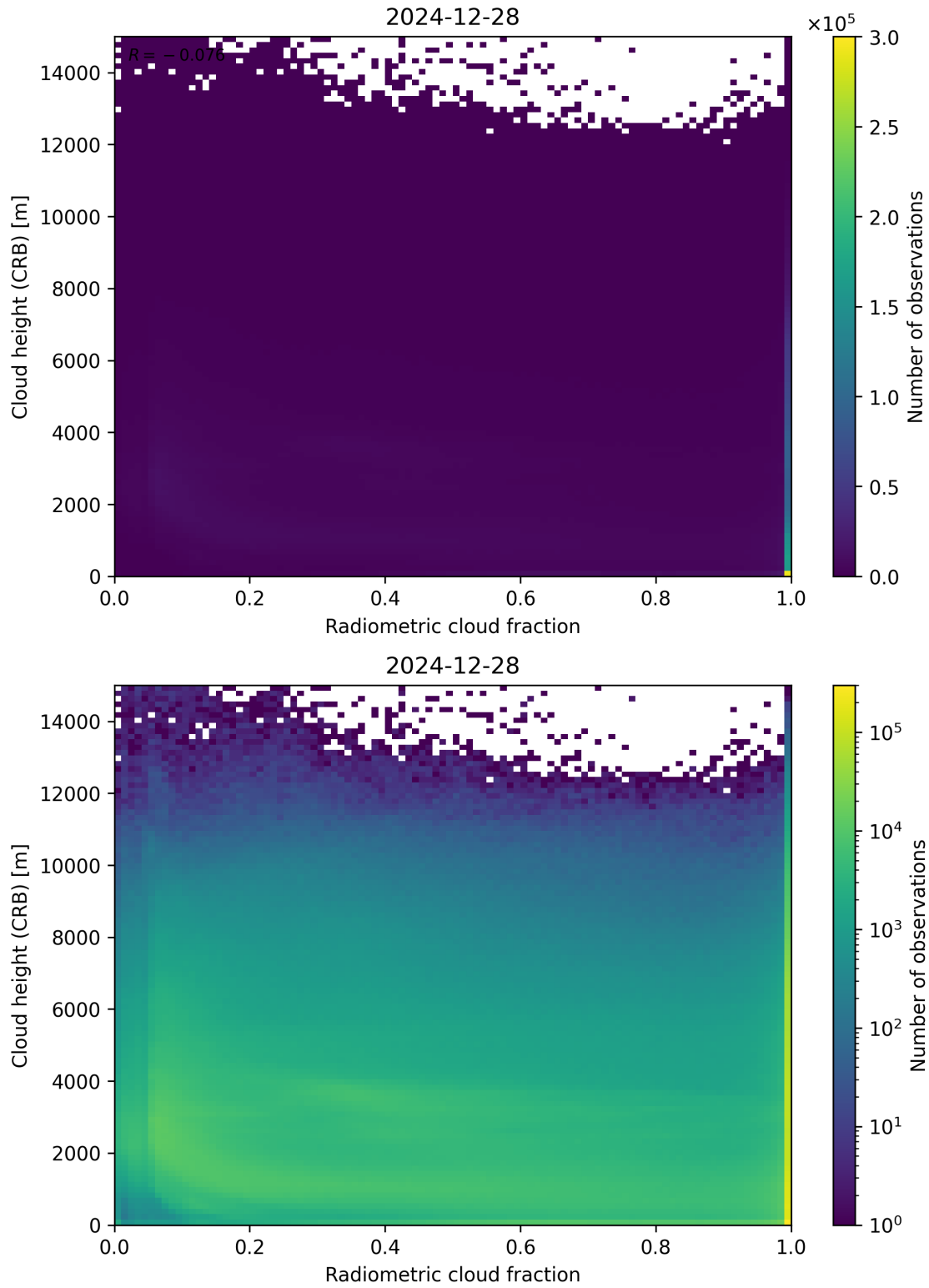
Figure 74: Scatter density plot of “Radiometric cloud fraction” against “Cloud height (CRB)” for 2024-12-27 to 2024-12-29.
