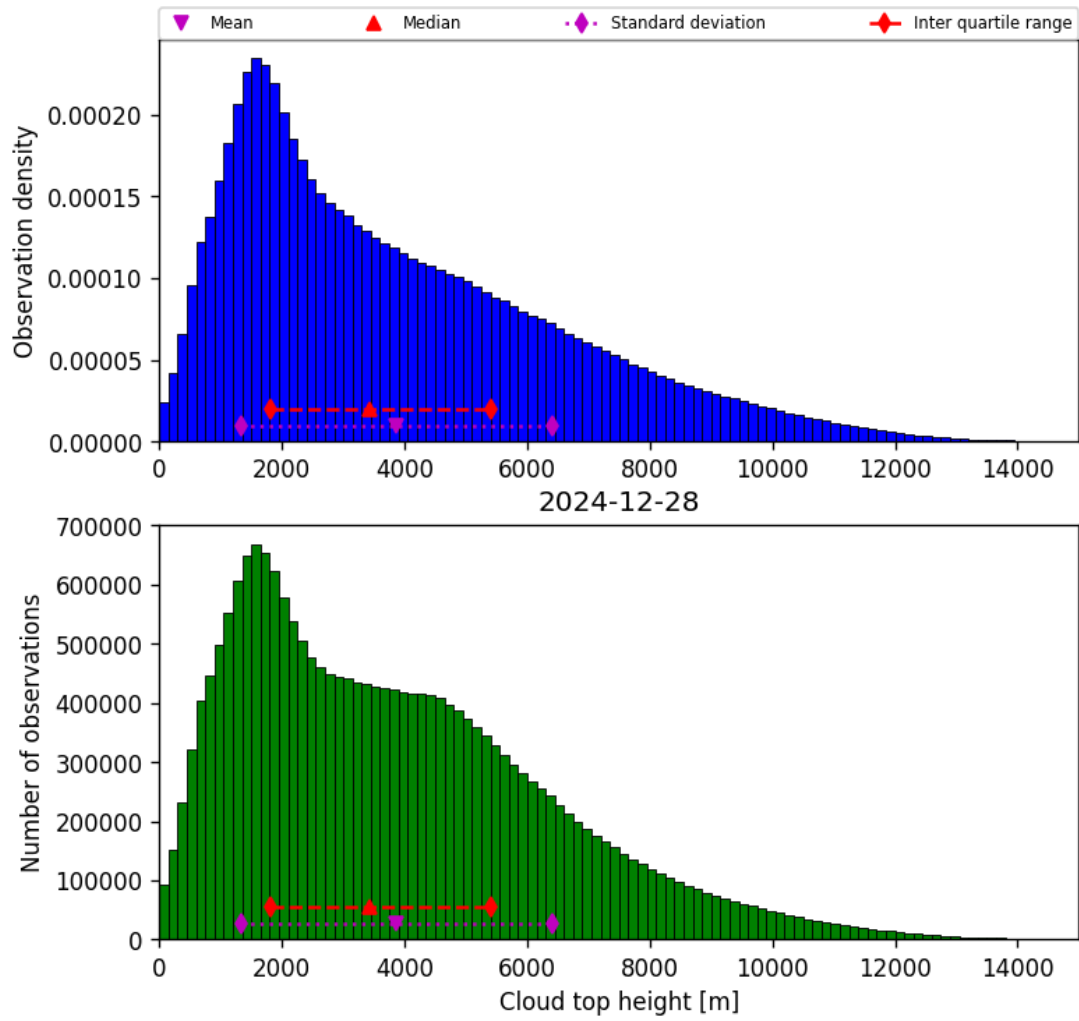
Figure 40: Histogram of “Cloud top height” for 2024-12-27 to 2024-12-29
