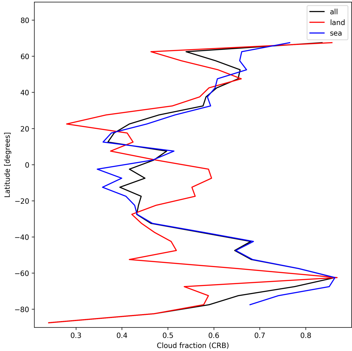
Figure 26: Zonal average of “Cloud fraction (CRB)” for 2024-12-27 to 2024-12-29.
