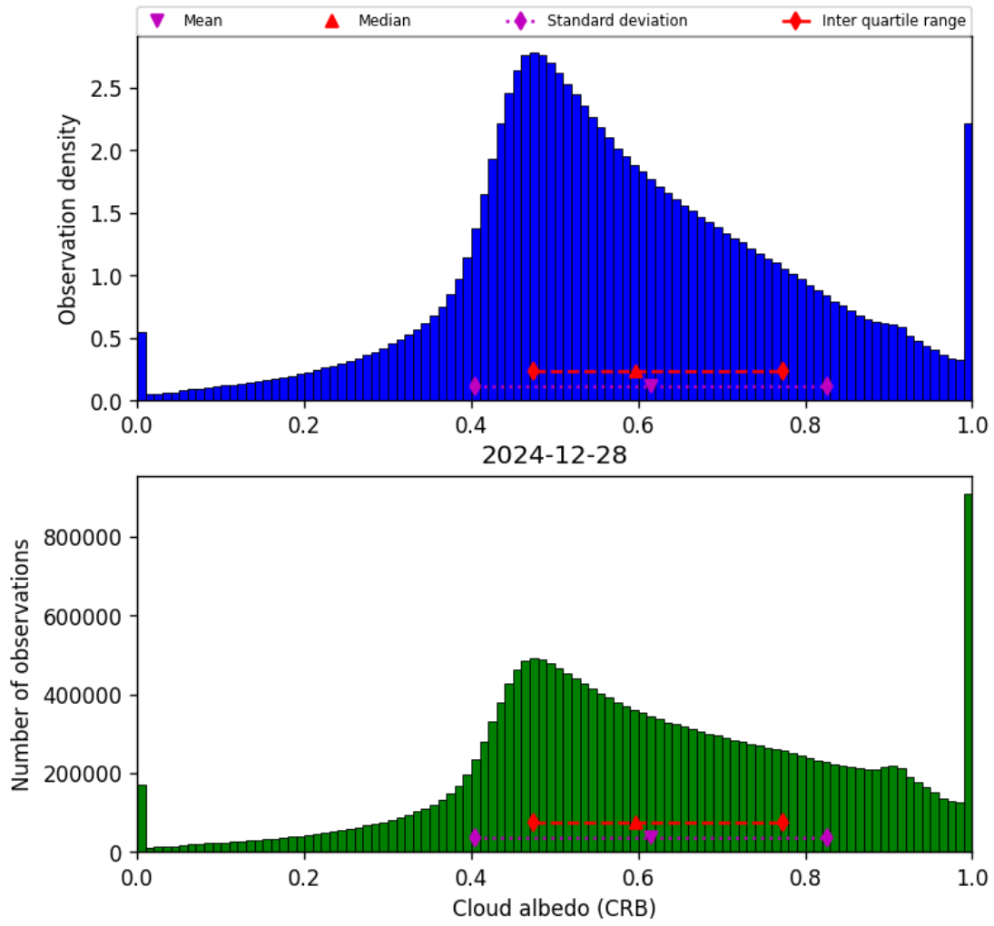
Figure 44: Histogram of “Cloud albedo (CRB)” for 2024-12-27 to 2024-12-29
