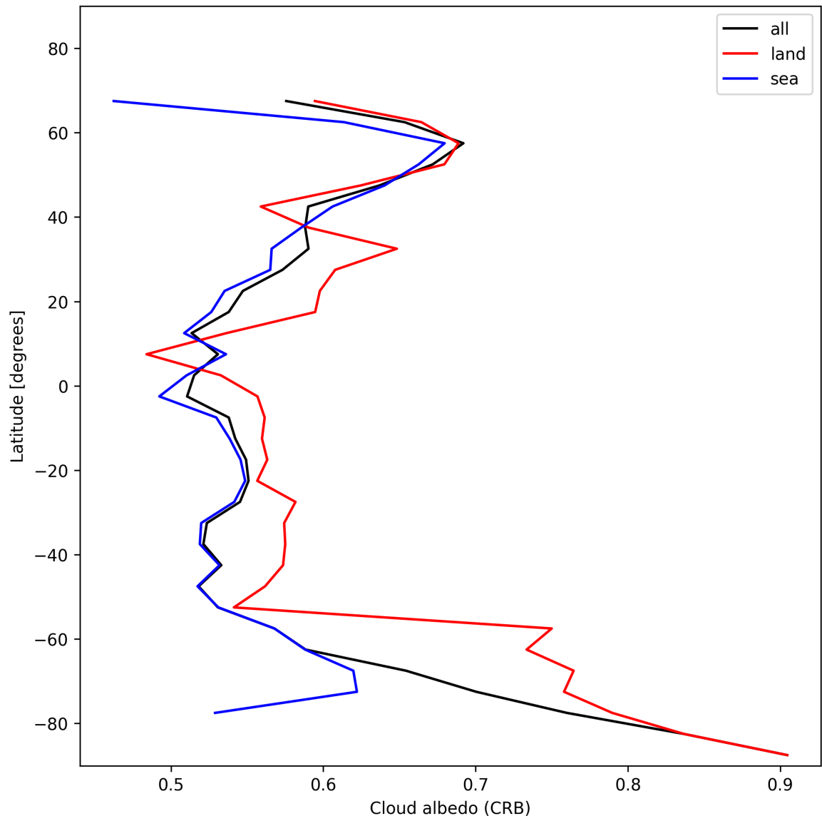
Figure 28: Zonal average of “Cloud albedo (CRB)” for 2024-12-27 to 2024-12-29.
