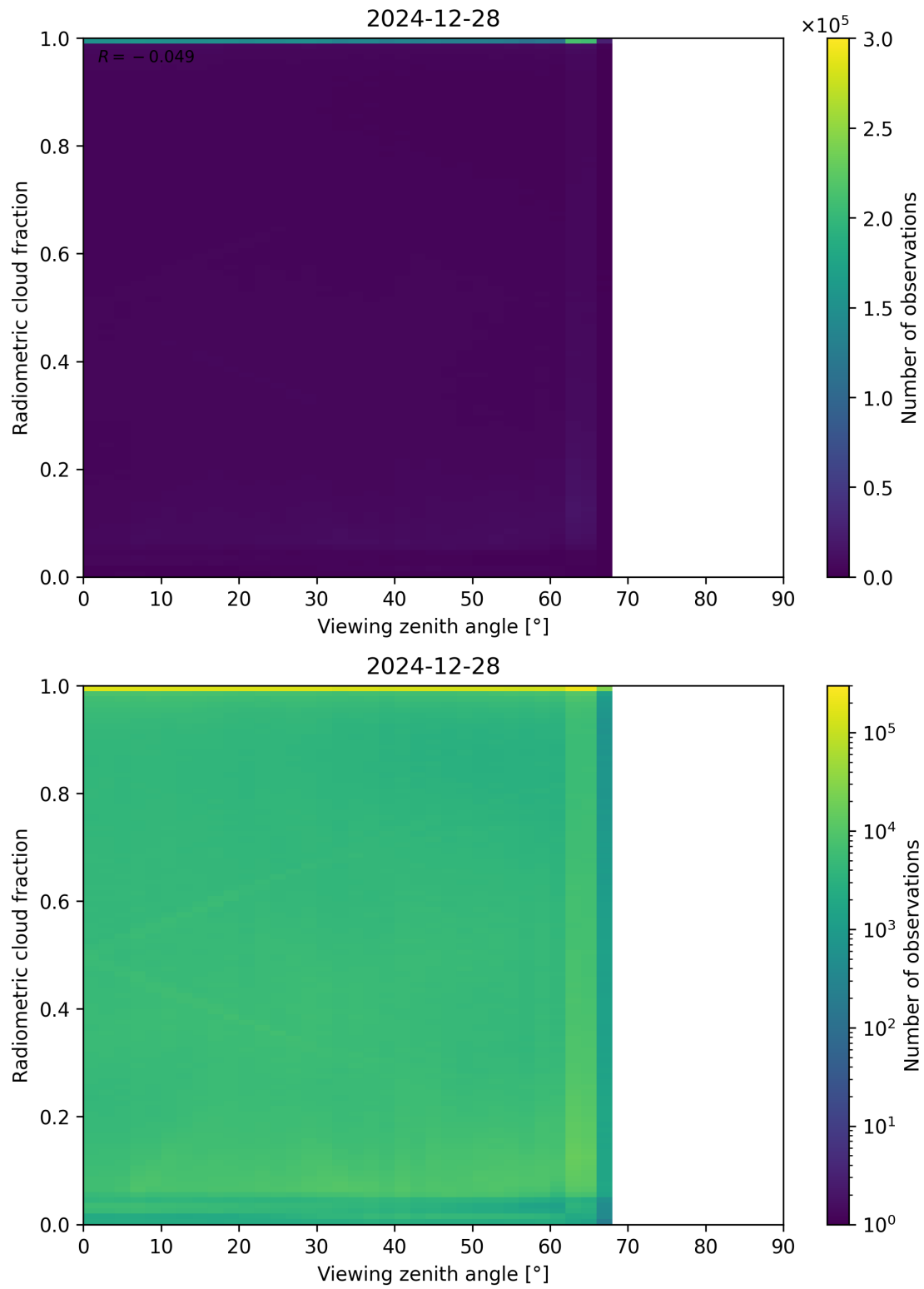
Figure 107: Scatter density plot of “Viewing zenith angle” against “Radiometric cloud fraction” for 2024-12-27 to 2024-12-29.
