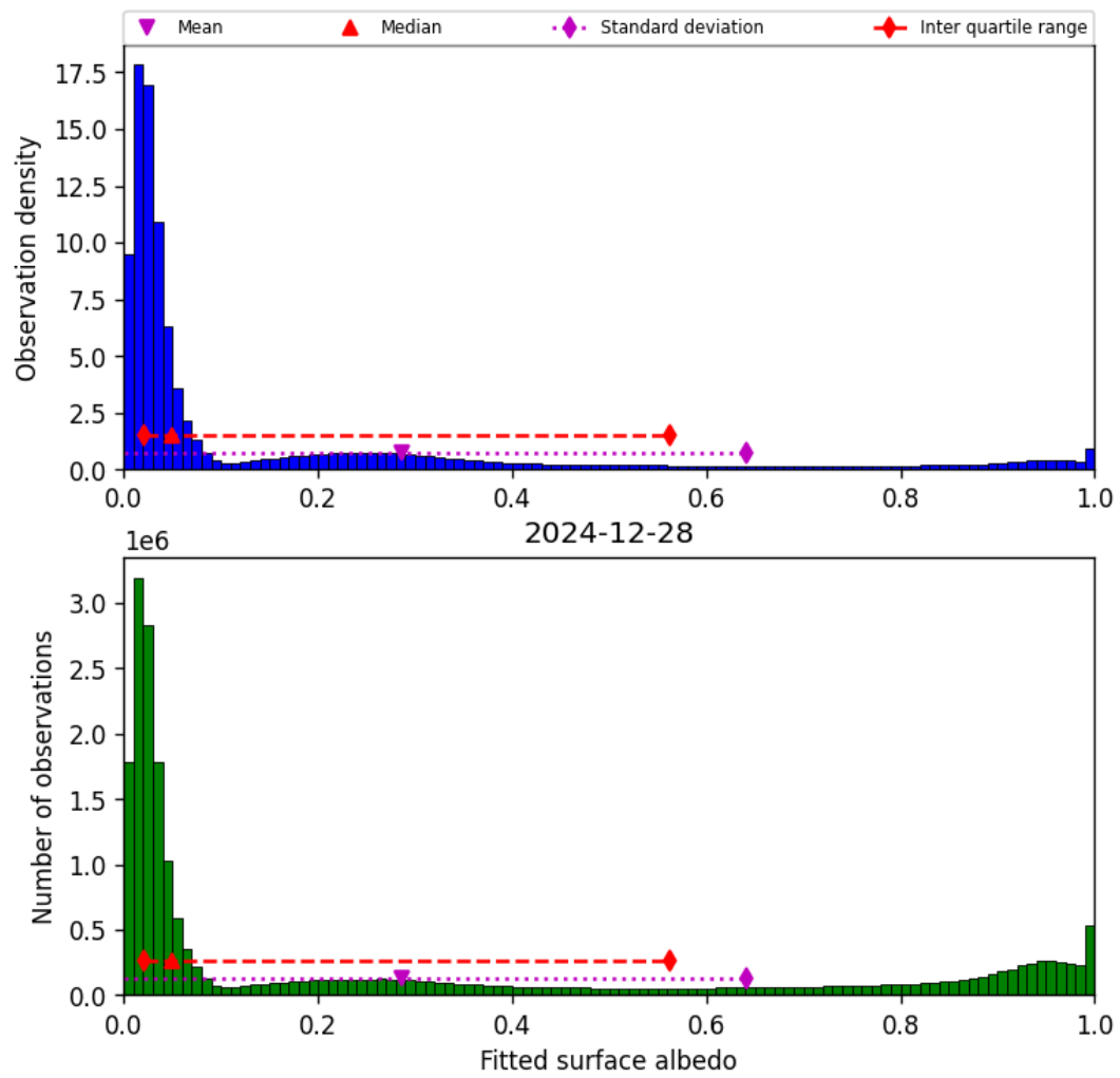
Figure 45: Histogram of “Fitted surface albedo” for 2024-12-27 to 2024-12-29
