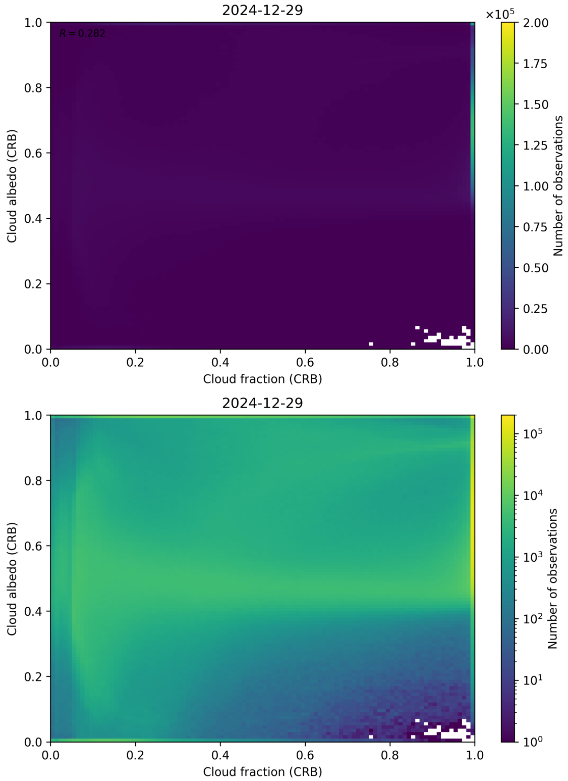
Figure 77: Scatter density plot of “Cloud fraction (CRB)” against “Cloud albedo (CRB)” for 2024-12-28 to 2024-12-30.
