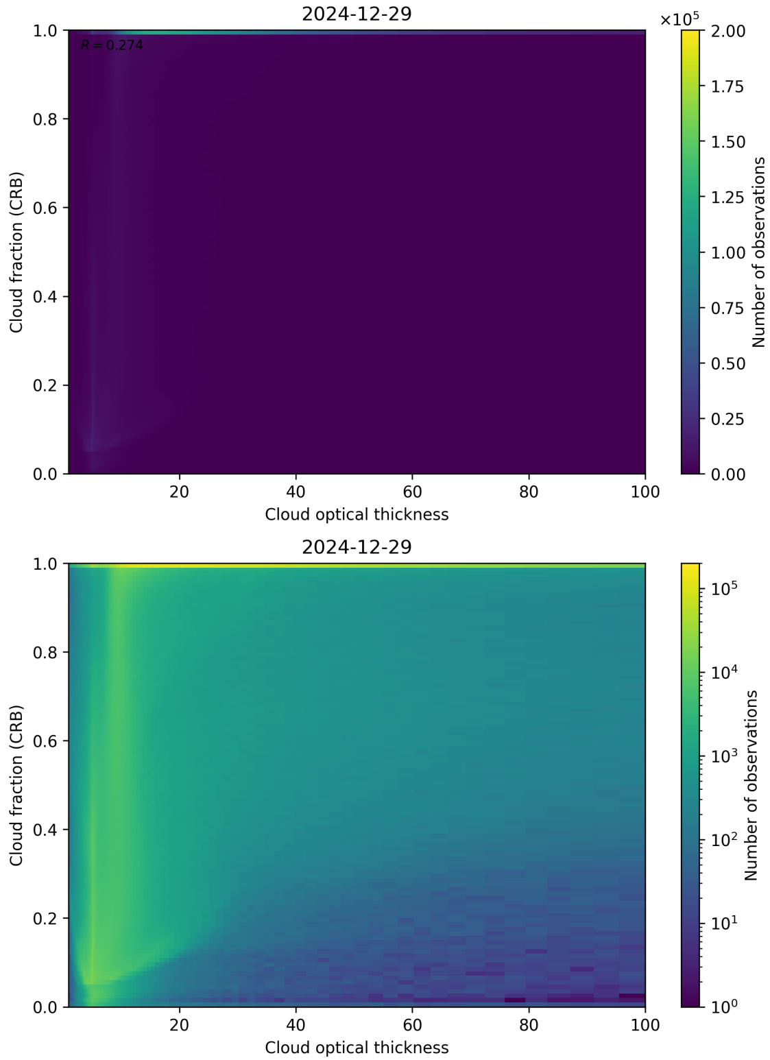
Figure 84: Scatter density plot of “Cloud optical thickness” against “Cloud fraction (CRB)” for 2024-12-28 to 2024-12-30.
