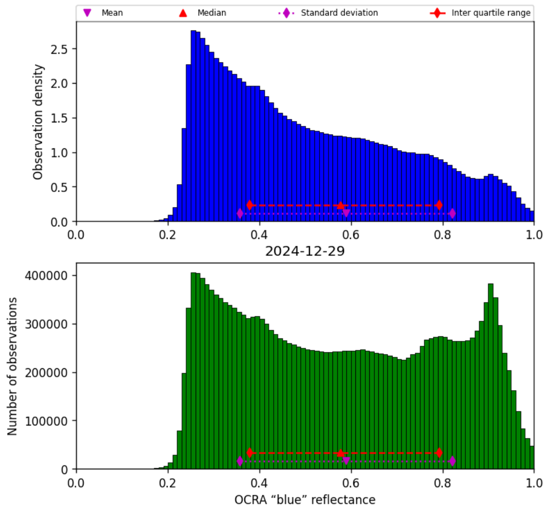
Figure 51: Histogram of “OCRA “blue” reflectance” for 2024-12-28 to 2024-12-30
