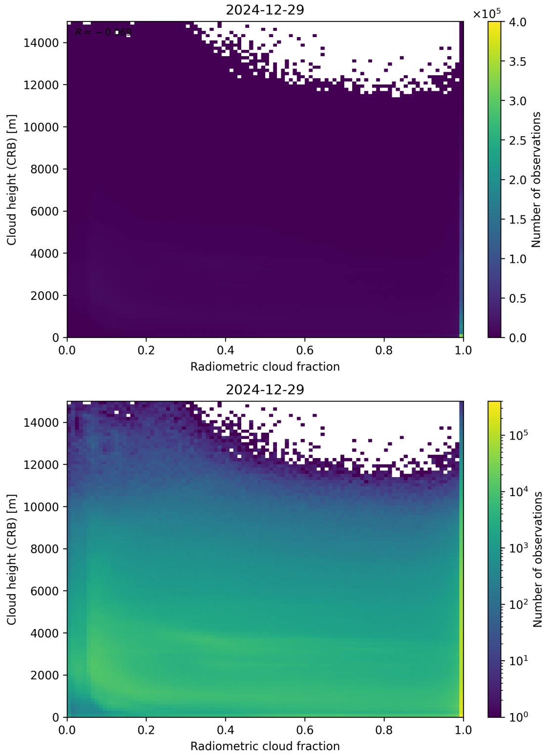
Figure 74: Scatter density plot of “Radiometric cloud fraction” against “Cloud height (CRB)” for 2024-12-28 to 2024-12-30.
