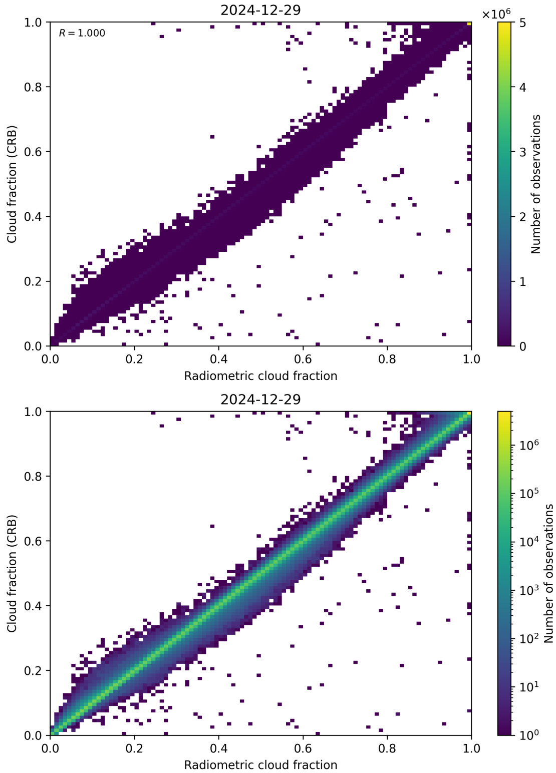
Figure 73: Scatter density plot of “Radiometric cloud fraction” against “Cloud fraction (CRB)” for 2024-12-28 to 2024-12-30.
