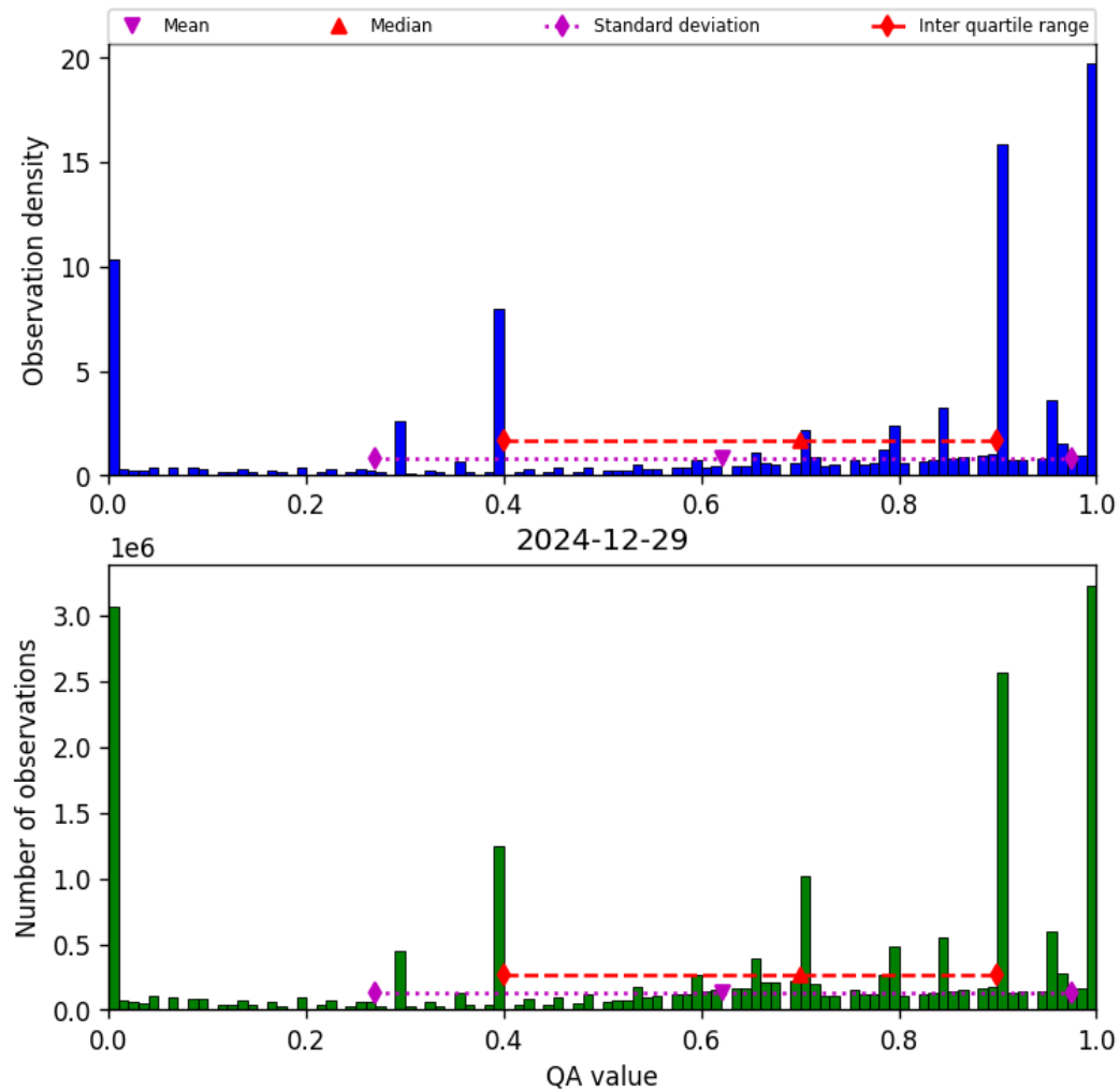
Figure 38: Histogram of “QA value” for 2024-12-28 to 2024-12-30
