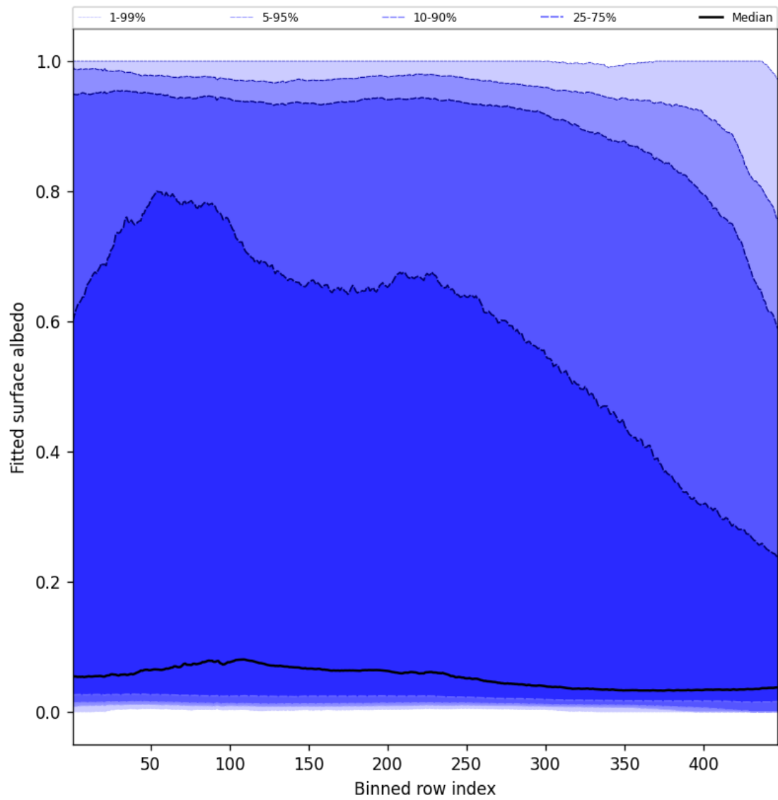
Figure 61: Along track statistics of “Fitted surface albedo” for 2024-12-28 to 2024-12-30
