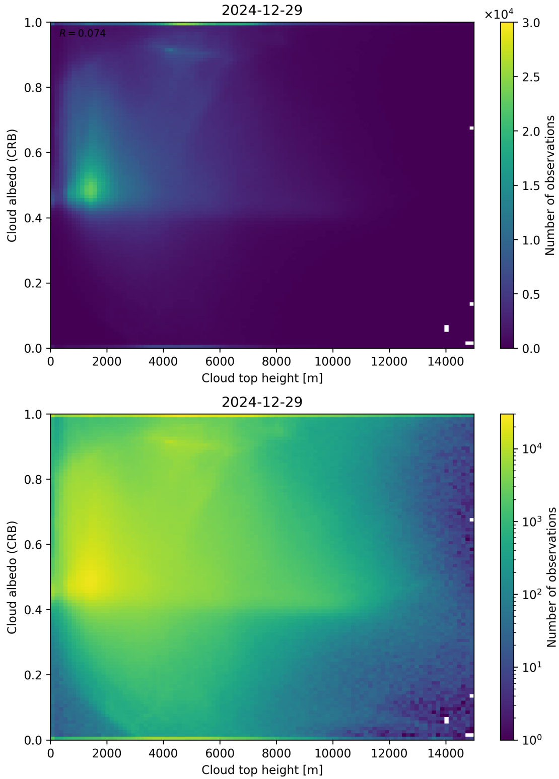
Figure 86: Scatter density plot of “Cloud top height” against “Cloud albedo (CRB)” for 2024-12-28 to 2024-12-30.
