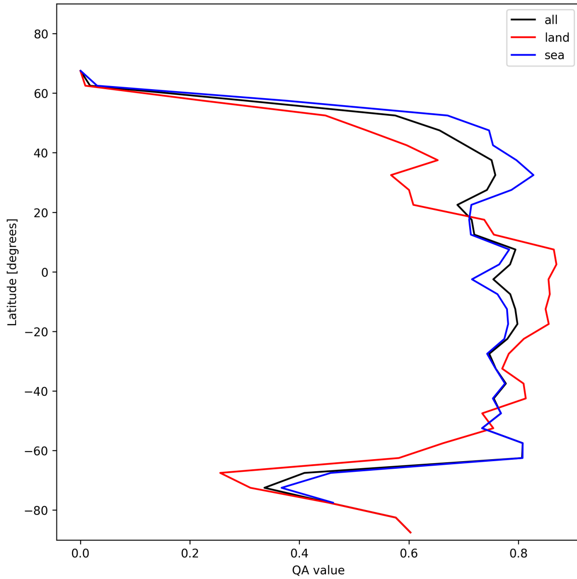
Figure 22: Zonal average of “QA value” for 2024-12-28 to 2024-12-30.
