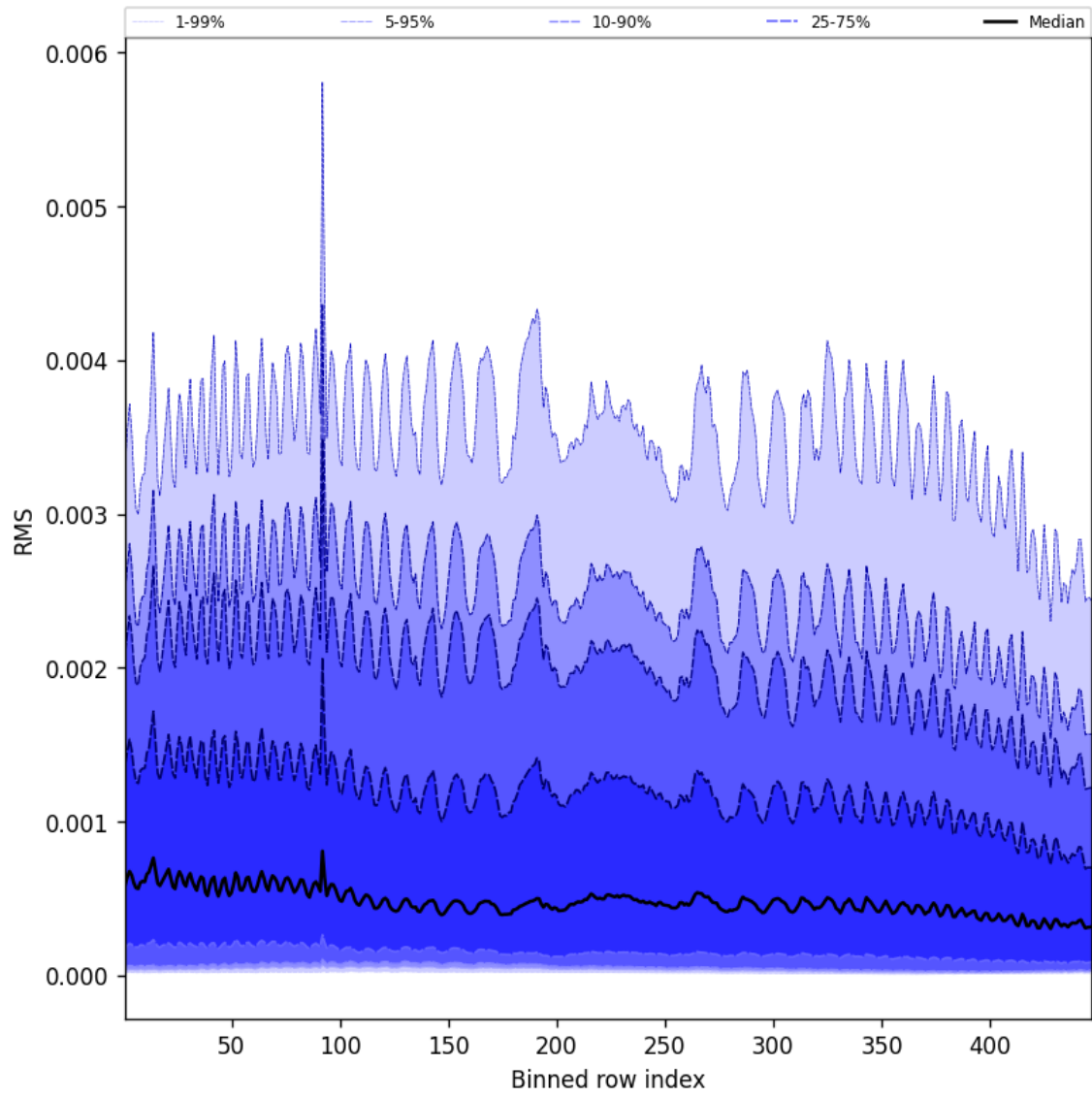
Figure 63: Along track statistics of “RMS” for 2024-12-28 to 2024-12-30
