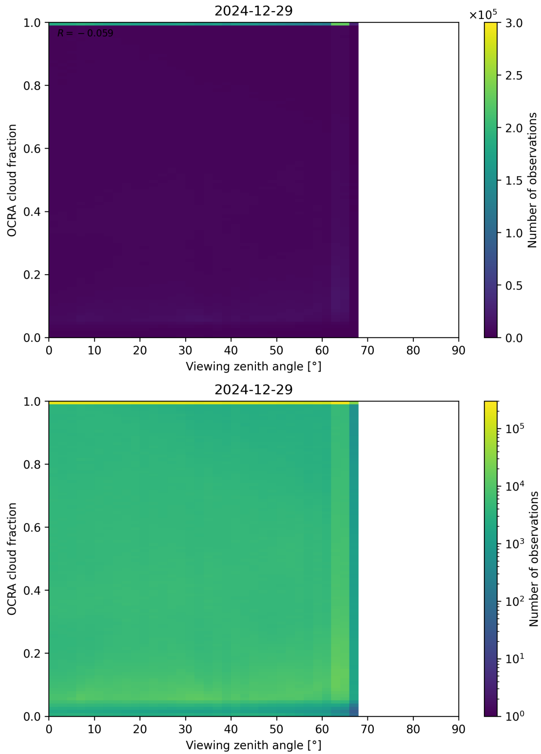
Figure 108: Scatter density plot of “Viewing zenith angle” against “OCRA cloud fraction” for 2024-12-28 to 2024-12-30.
