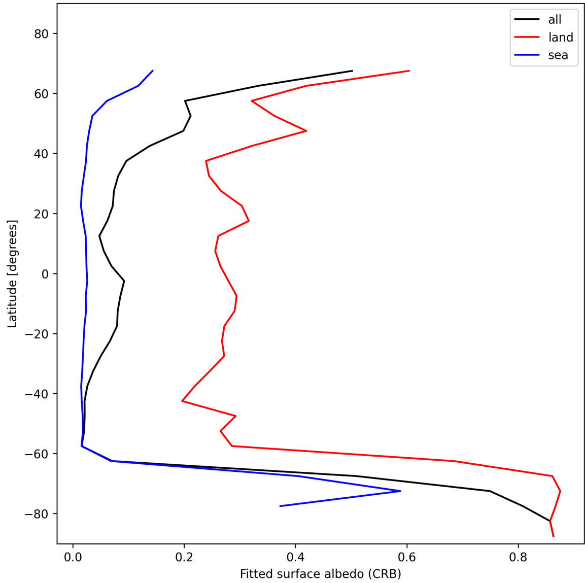
Figure 30: Zonal average of “Fitted surface albedo (CRB)” for 2024-12-28 to 2024-12-30.
