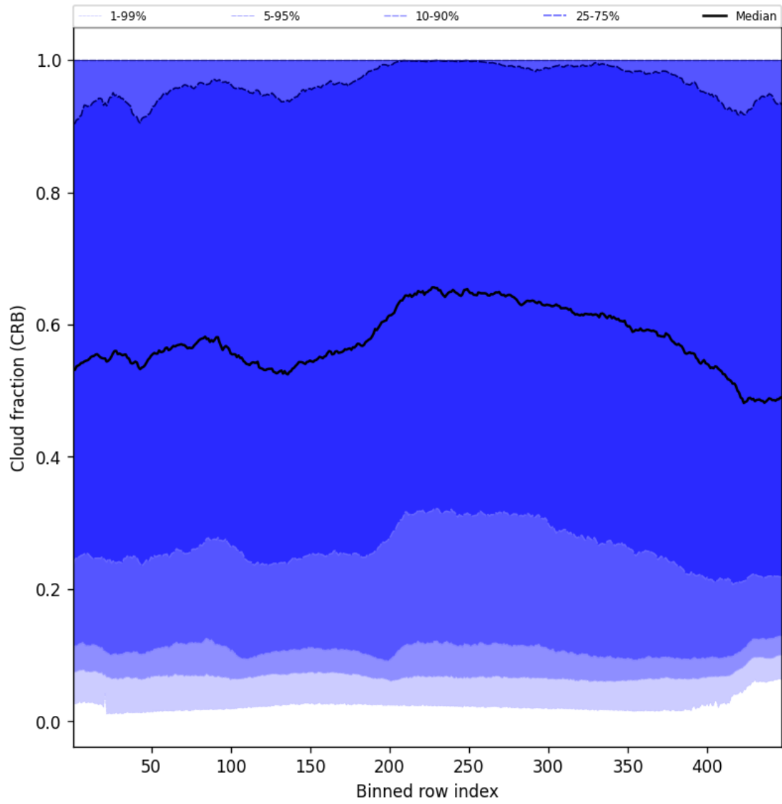
Figure 58: Along track statistics of “Cloud fraction (CRB)” for 2024-12-28 to 2024-12-30
