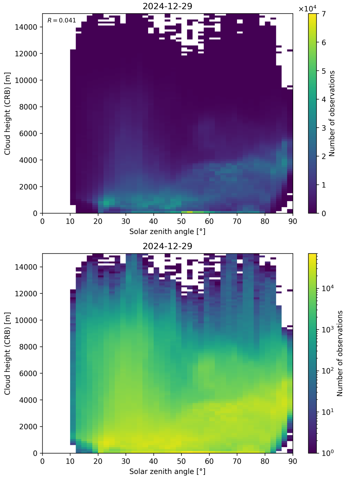
Figure 102: Scatter density plot of “Solar zenith angle” against “Cloud height (CRB)” for 2024-12-28 to 2024-12-30.
