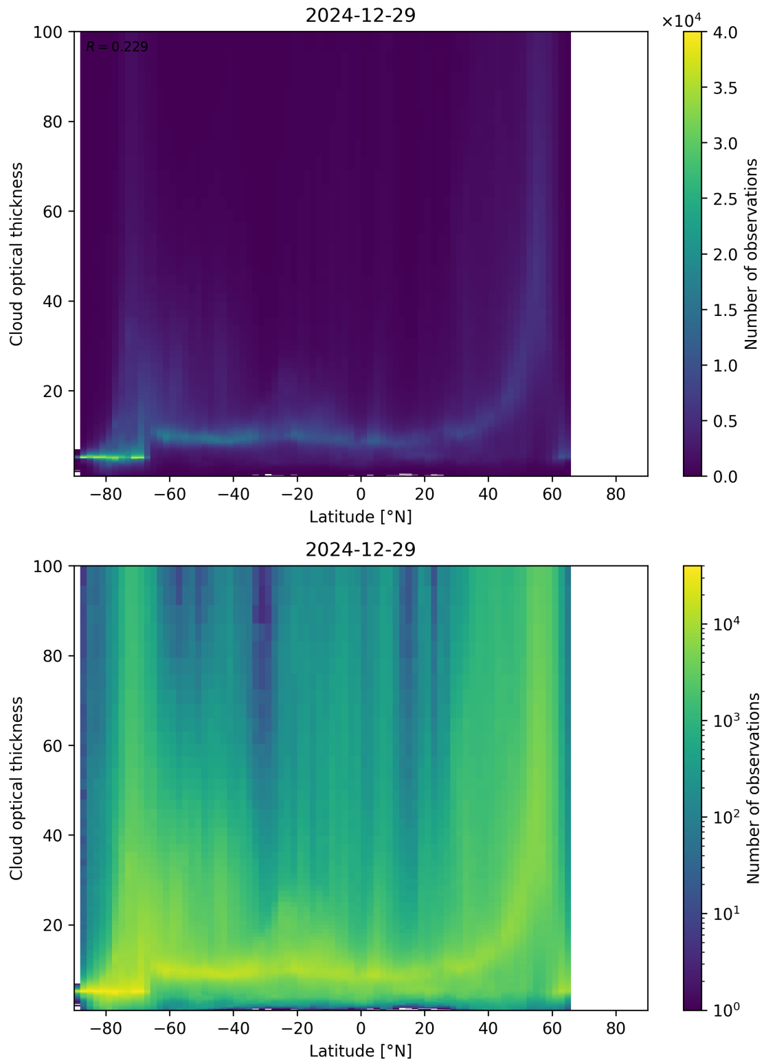
Figure 96: Scatter density plot of “Latitude” against “Cloud optical thickness” for 2024-12-28 to 2024-12-30.
