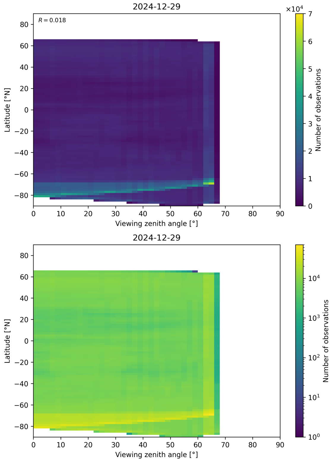
Figure 113: Scatter density plot of “Viewing zenith angle” against “Latitude” for 2024-12-28 to 2024-12-30.
