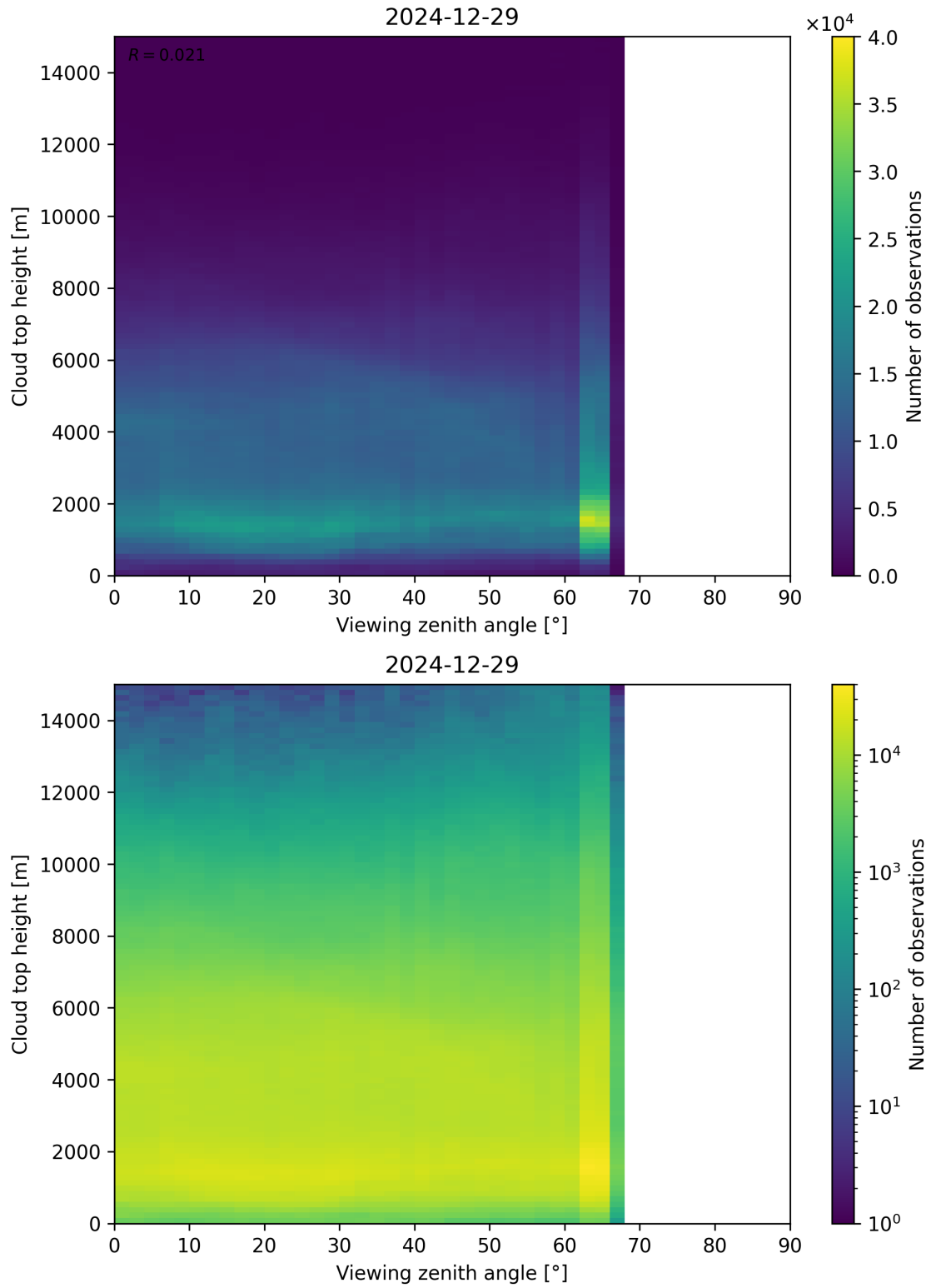
Figure 112: Scatter density plot of “Viewing zenith angle” against “Cloud top height” for 2024-12-28 to 2024-12-30.
