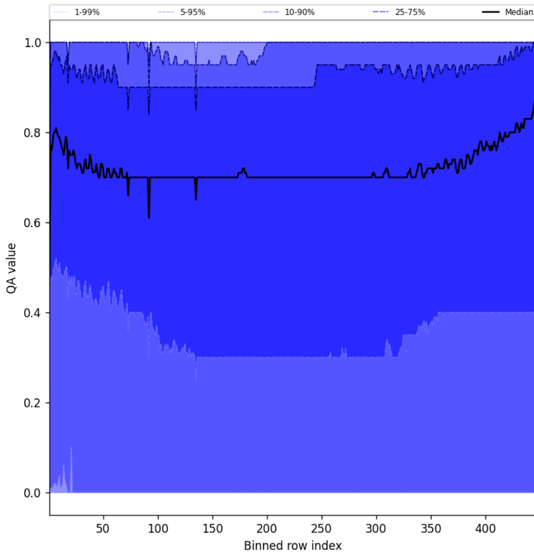
Figure 54: Along track statistics of “QA value” for 2024-12-28 to 2024-12-30
