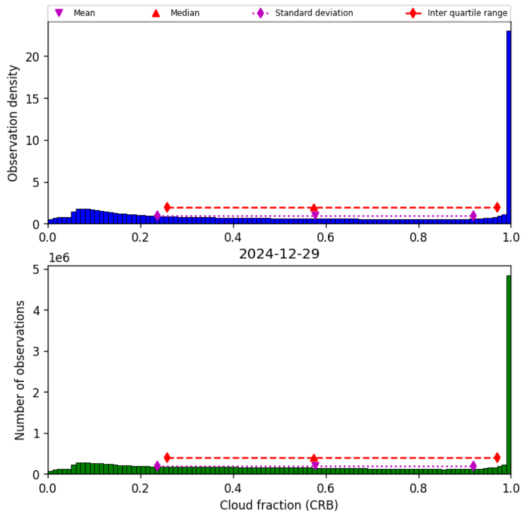
Figure 42: Histogram of “Cloud fraction (CRB)” for 2024-12-28 to 2024-12-30
