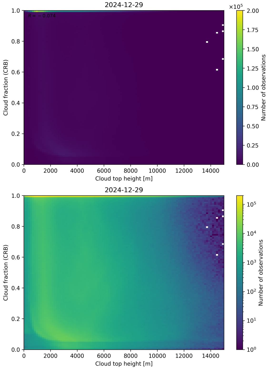
Figure 88: Scatter density plot of “Cloud top height” against “Cloud fraction (CRB)” for 2024-12-28 to 2024-12-30.
