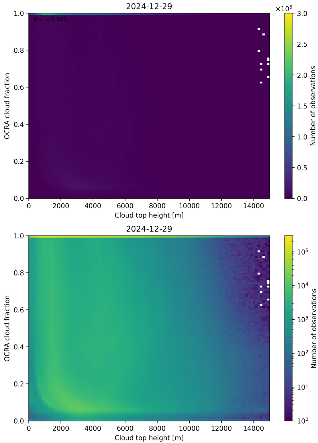
Figure 87: Scatter density plot of “Cloud top height” against “OCRA cloud fraction” for 2024-12-28 to 2024-12-30.
