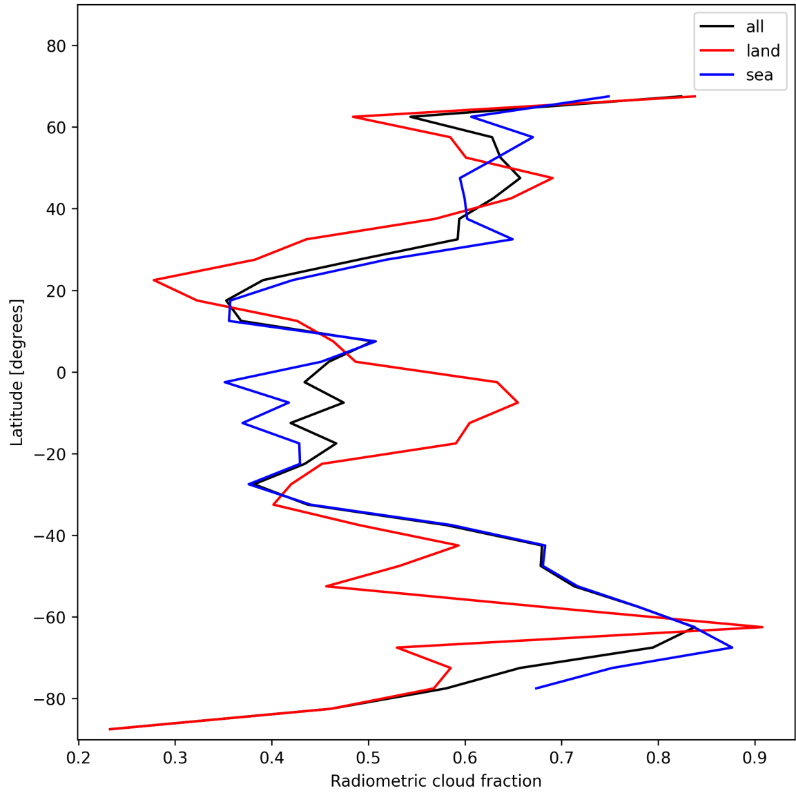
Figure 23: Zonal average of “Radiometric cloud fraction” for 2024-12-28 to 2024-12-30.
