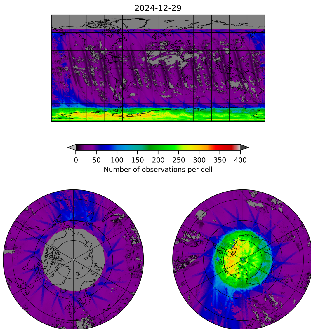
Figure 21: Map of the number of observations for 2024-12-28 to 2024-12-30
