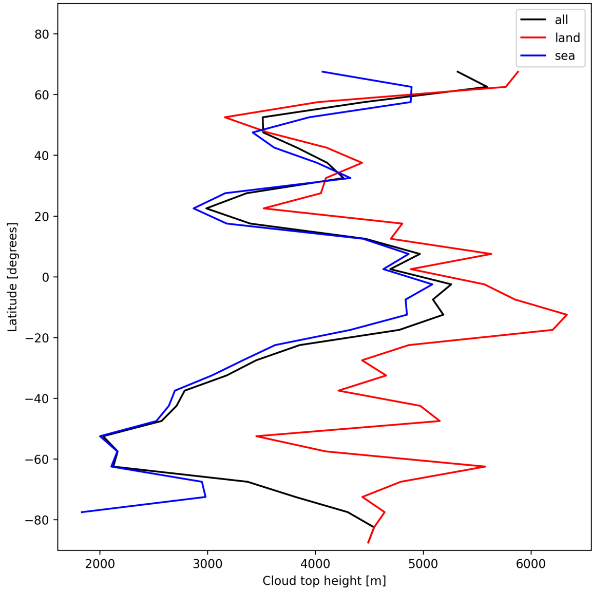
Figure 24: Zonal average of “Cloud top height” for 2024-12-28 to 2024-12-30.
