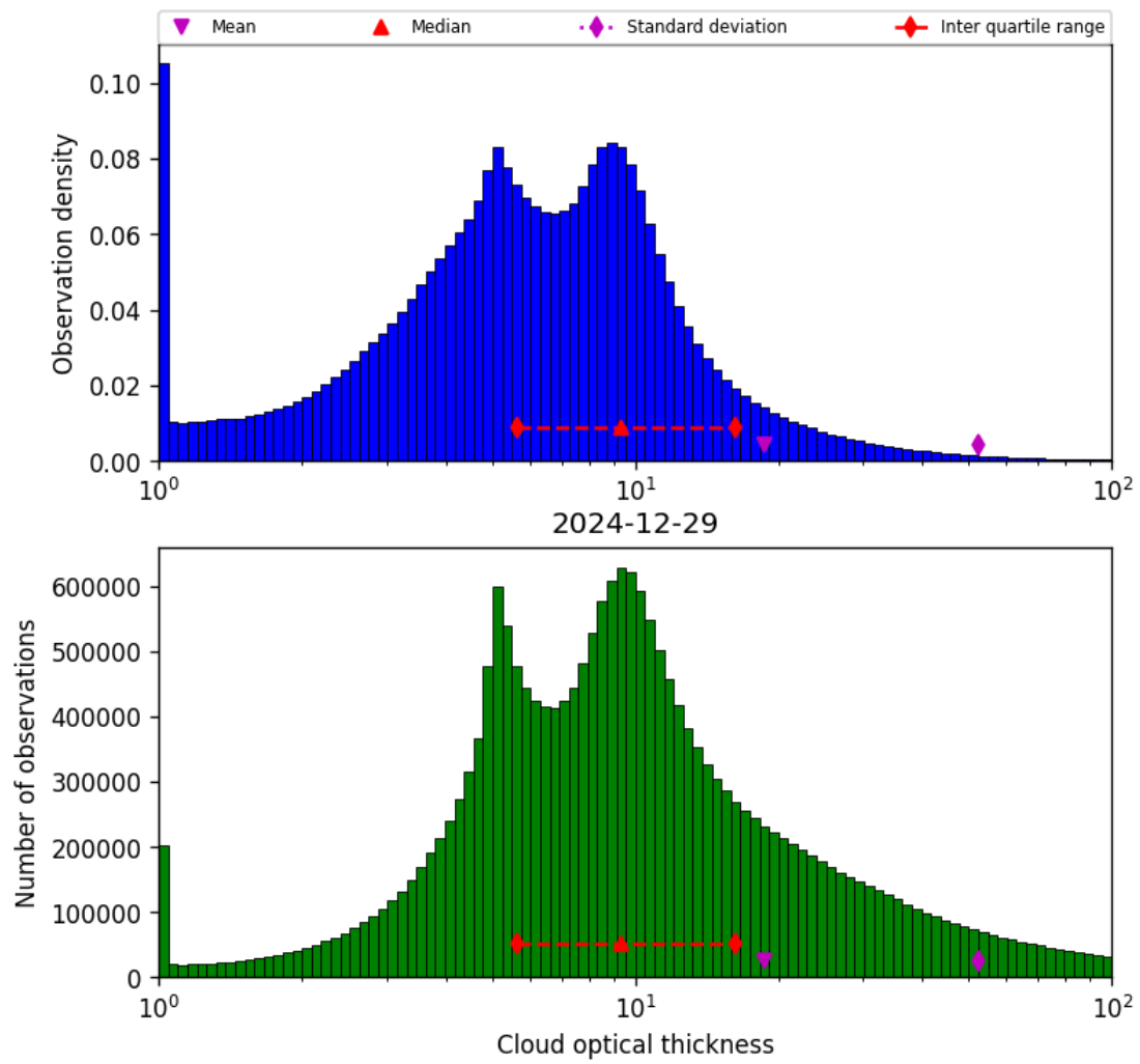
Figure 41: Histogram of “Cloud optical thickness” for 2024-12-28 to 2024-12-30
