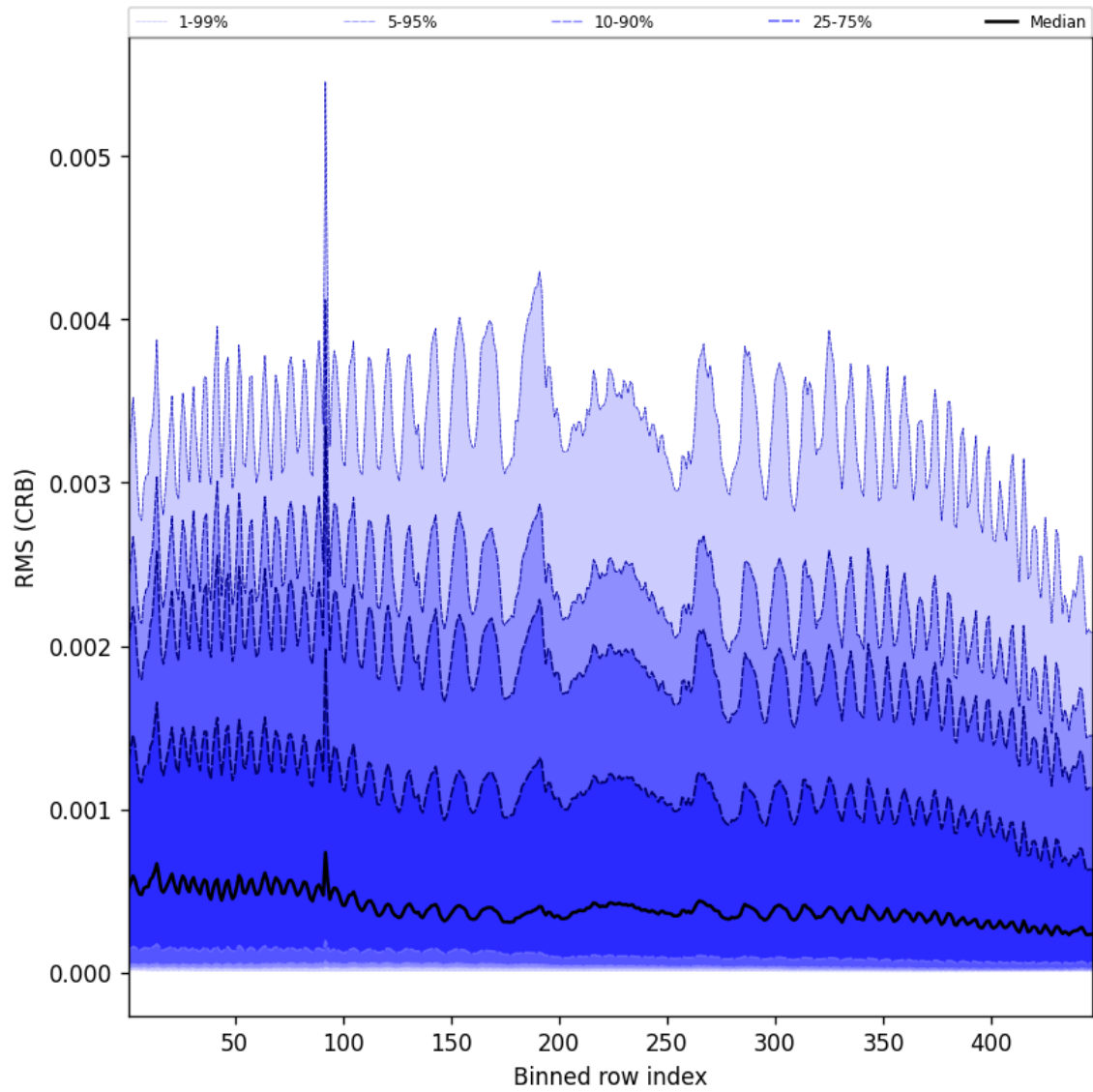
Figure 64: Along track statistics of “RMS (CRB)” for 2024-12-28 to 2024-12-30
