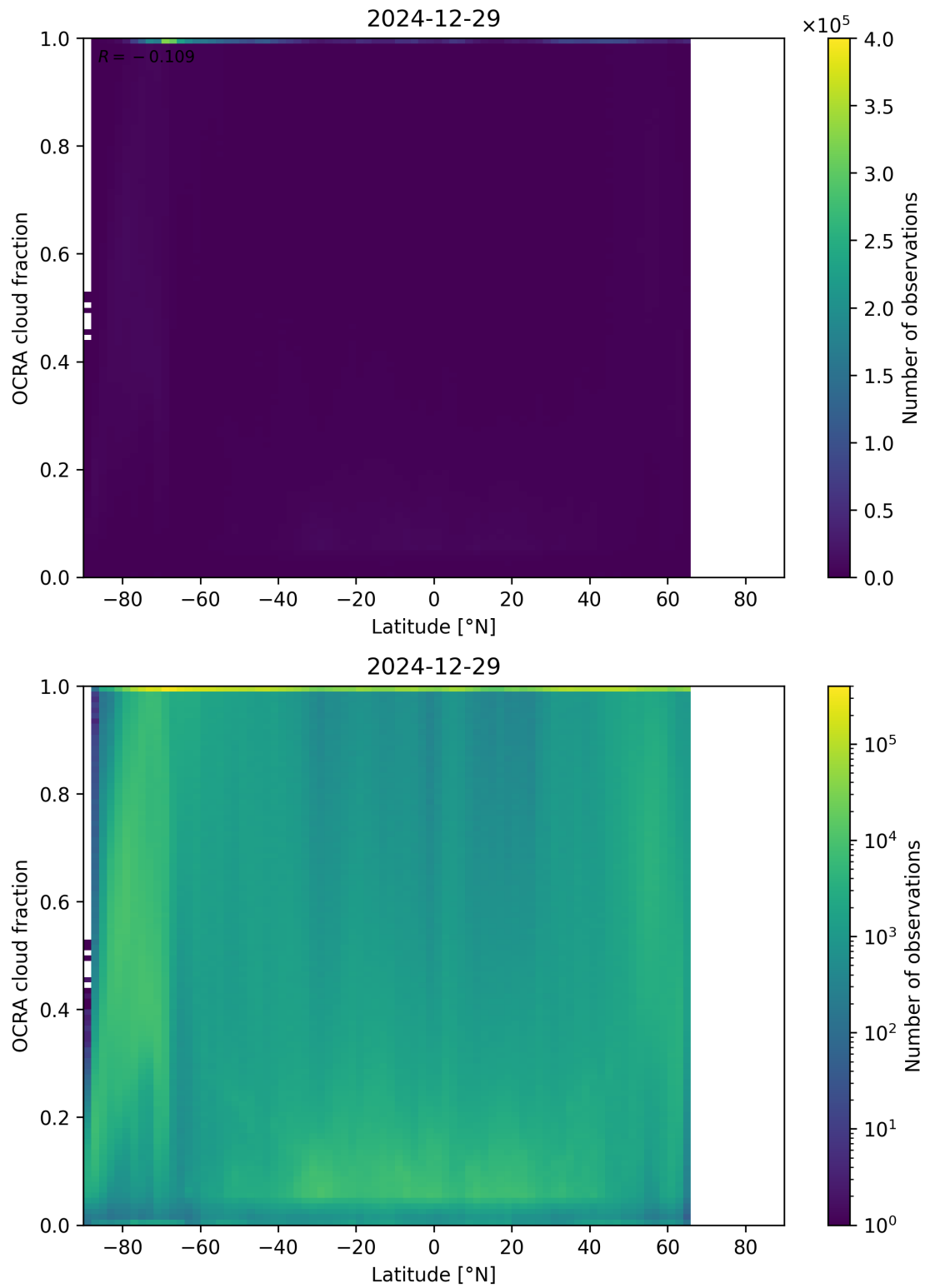
Figure 93: Scatter density plot of “Latitude” against “OCRA cloud fraction” for 2024-12-28 to 2024-12-30.
