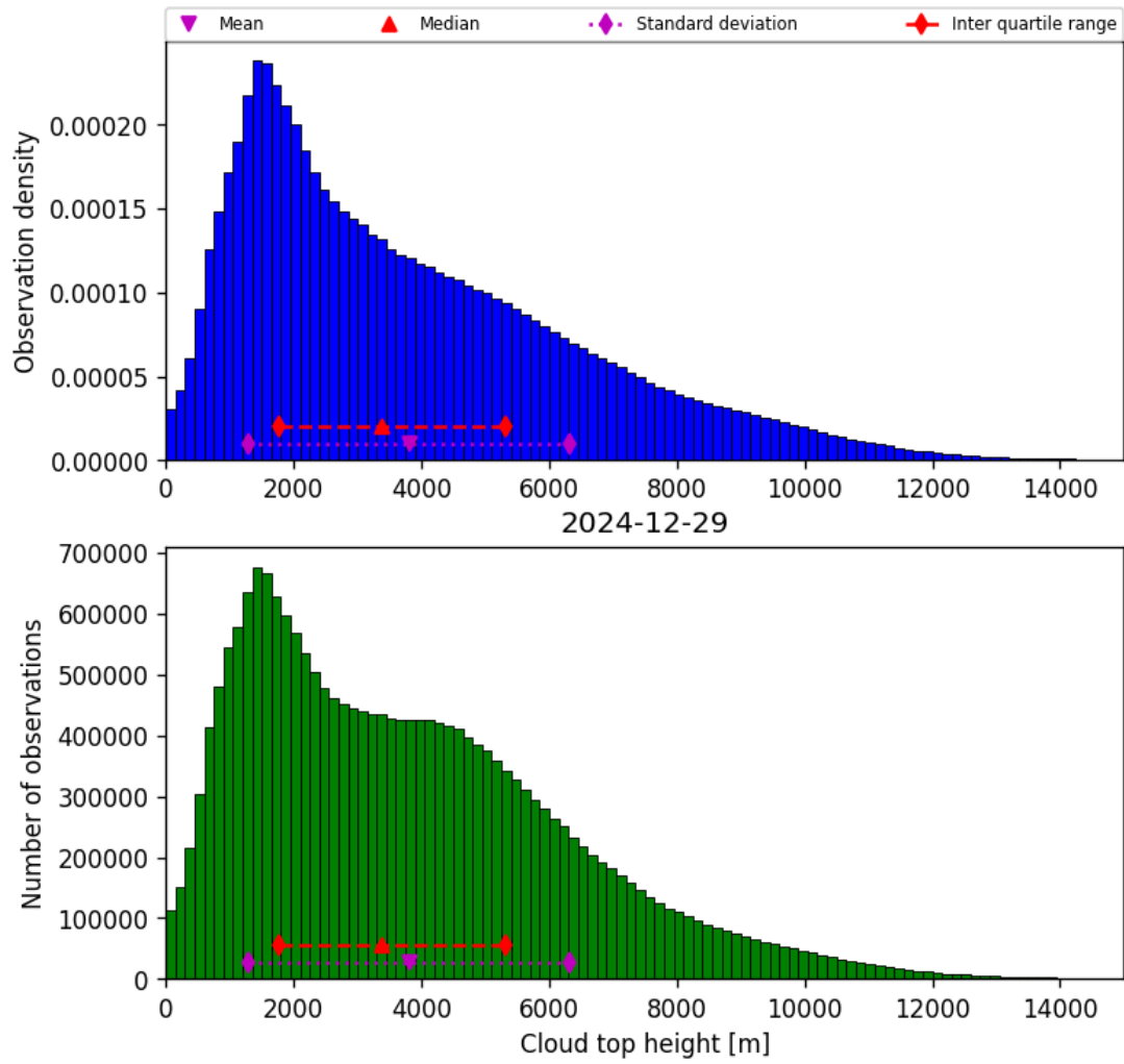
Figure 40: Histogram of “Cloud top height” for 2024-12-28 to 2024-12-30
