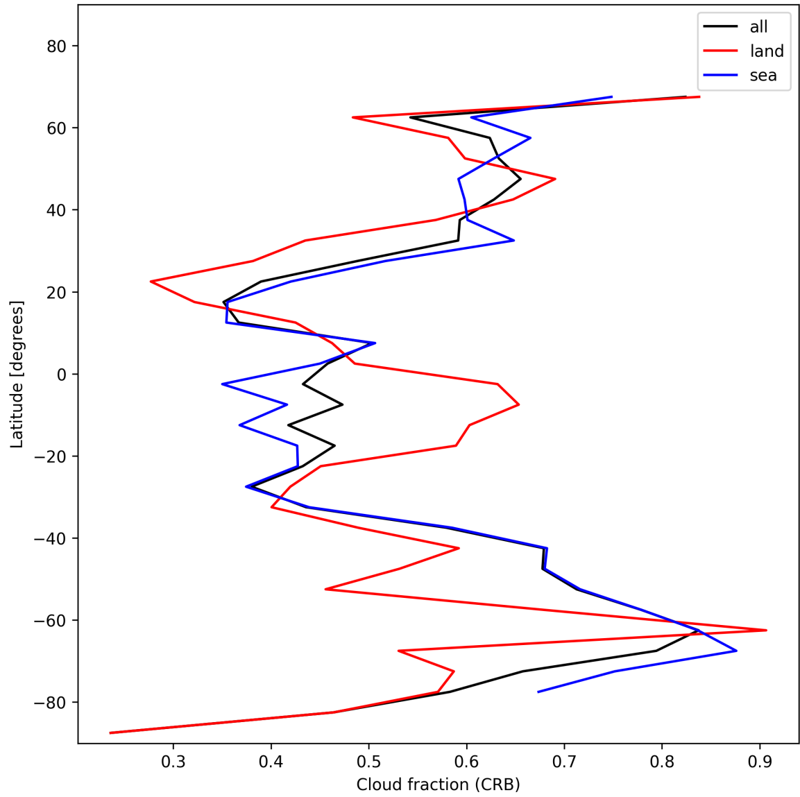
Figure 26: Zonal average of “Cloud fraction (CRB)” for 2024-12-28 to 2024-12-30.
