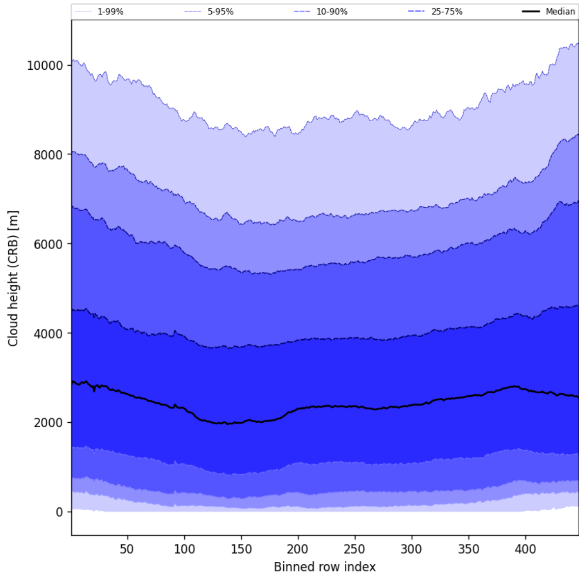
Figure 59: Along track statistics of “Cloud height (CRB)” for 2024-12-28 to 2024-12-30
