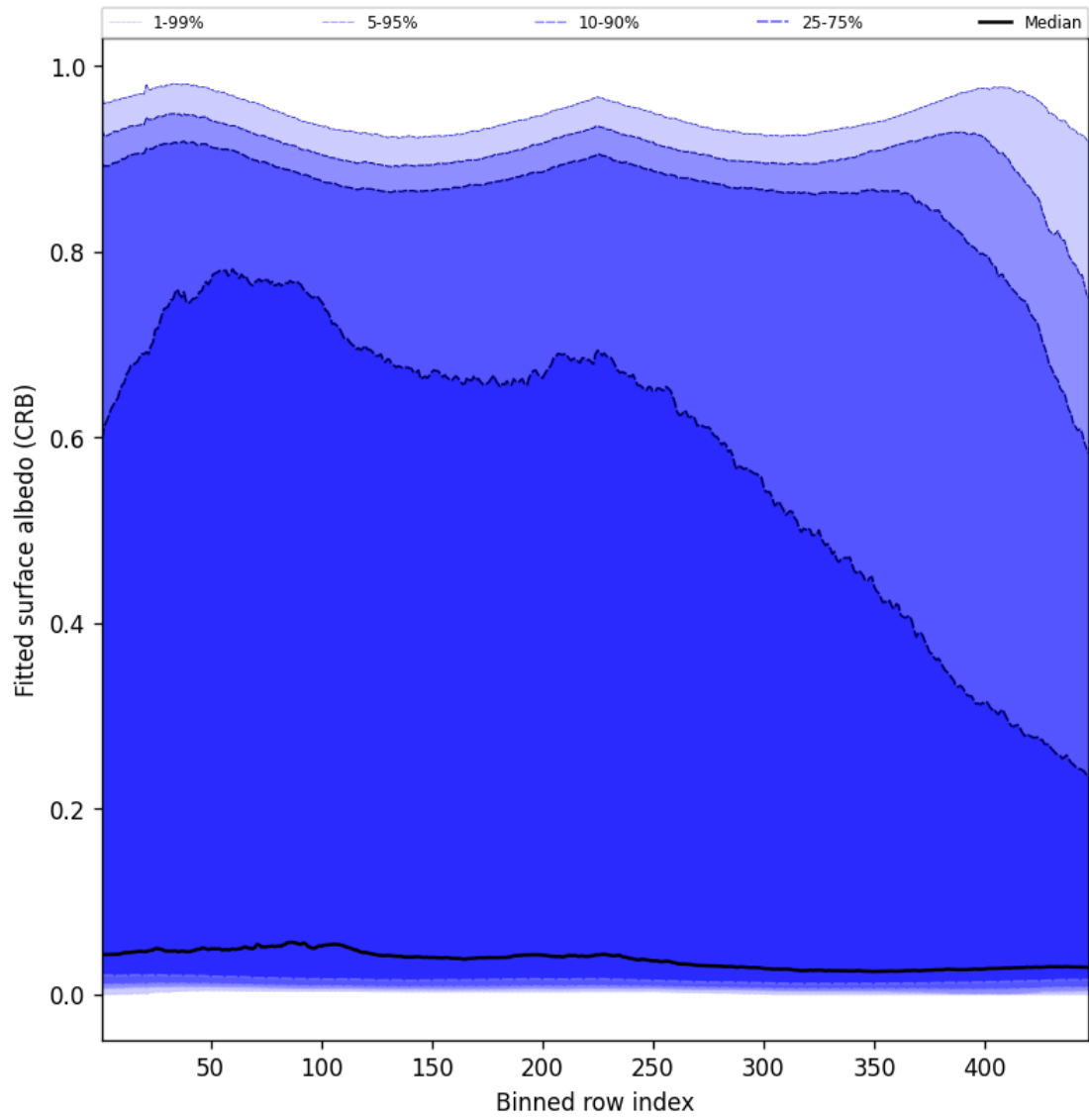
Figure 62: Along track statistics of “Fitted surface albedo (CRB)” for 2024-12-28 to 2024-12-30
