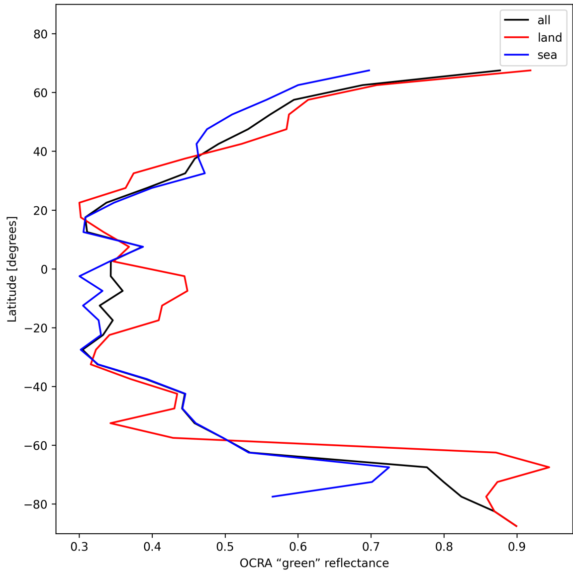
Figure 36: Zonal average of “OCRA “green” reflectance” for 2024-12-28 to 2024-12-30.
