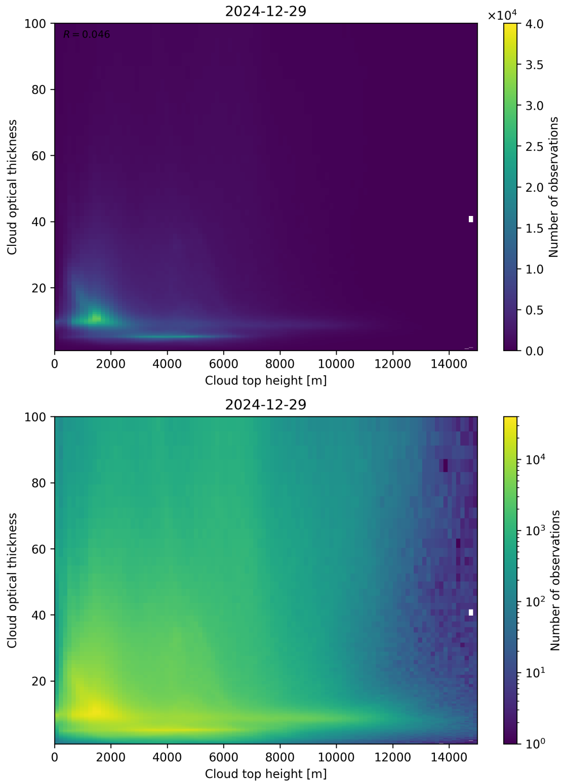
Figure 90: Scatter density plot of “Cloud top height” against “Cloud optical thickness” for 2024-12-28 to 2024-12-30.
