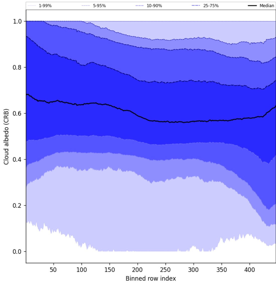
Figure 60: Along track statistics of “Cloud albedo (CRB)” for 2024-12-28 to 2024-12-30
