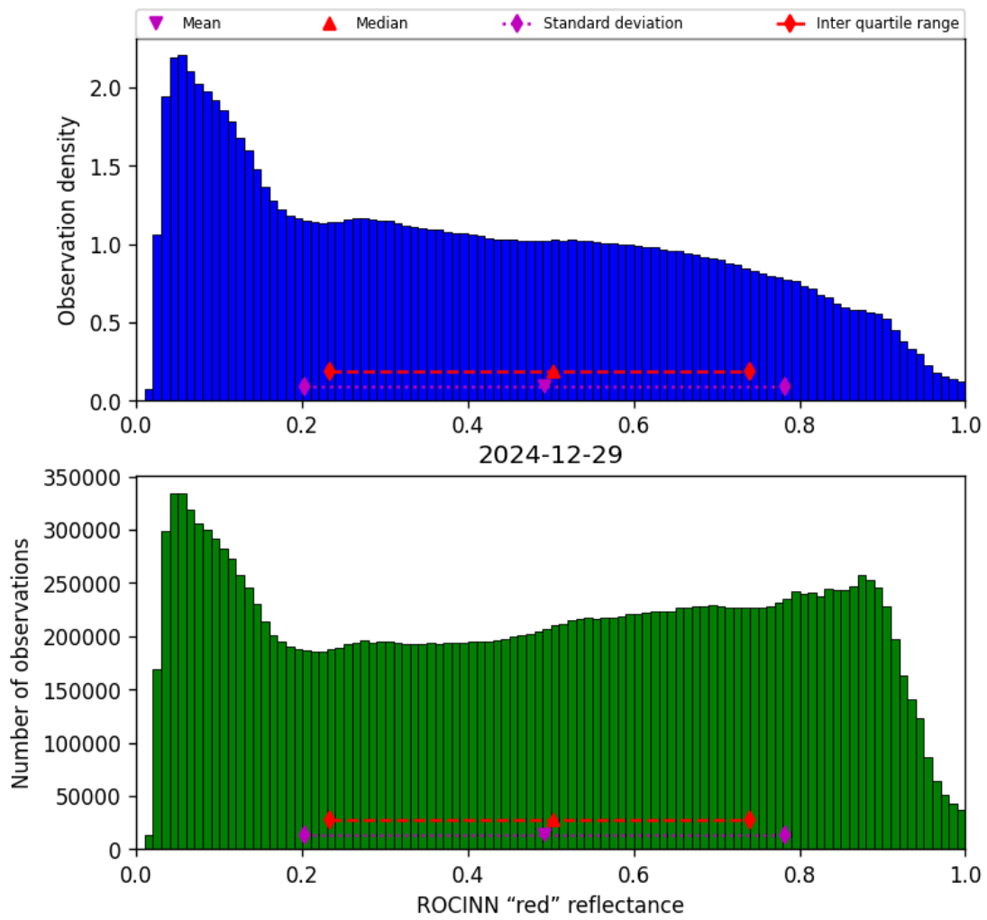
Figure 53: Histogram of “ROCINN “red” reflectance” for 2024-12-28 to 2024-12-30
