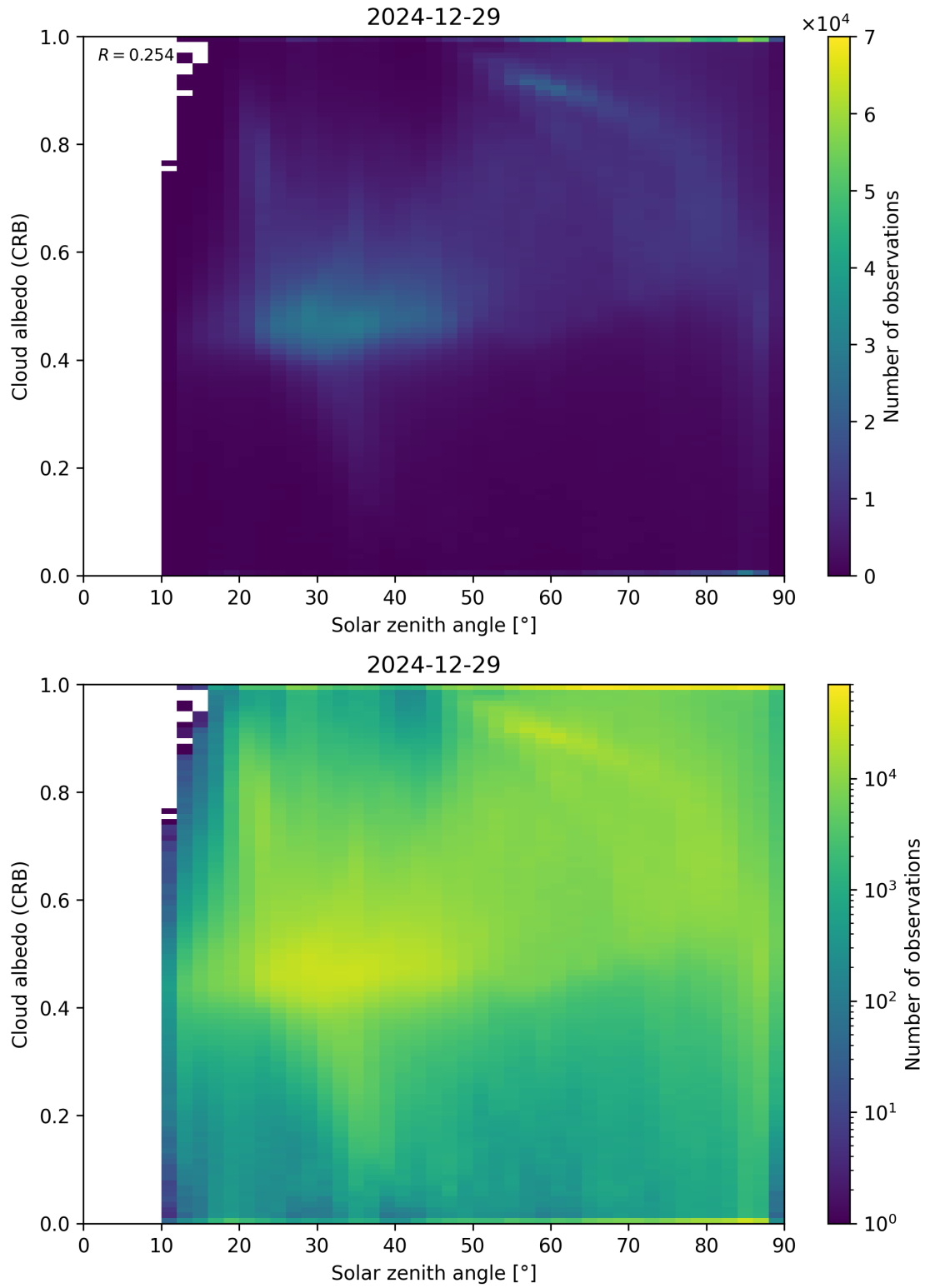
Figure 98: Scatter density plot of “Solar zenith angle” against “Cloud albedo (CRB)” for 2024-12-28 to 2024-12-30.
