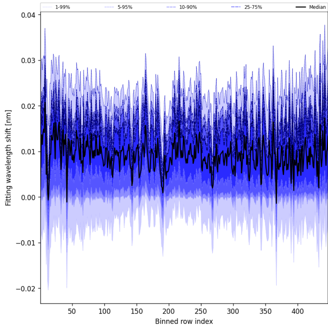
Figure 65: Along track statistics of “Fitting wavelength shift” for 2024-12-28 to 2024-12-30
