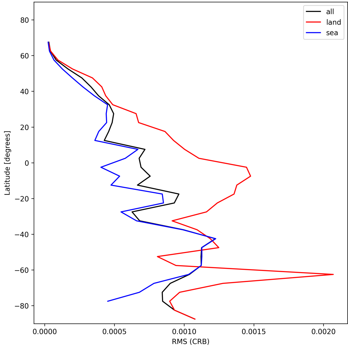
Figure 32: Zonal average of “RMS (CRB)” for 2024-12-28 to 2024-12-30.
