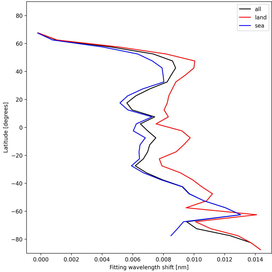
Figure 33: Zonal average of “Fitting wavelength shift” for 2024-12-28 to 2024-12-30.
