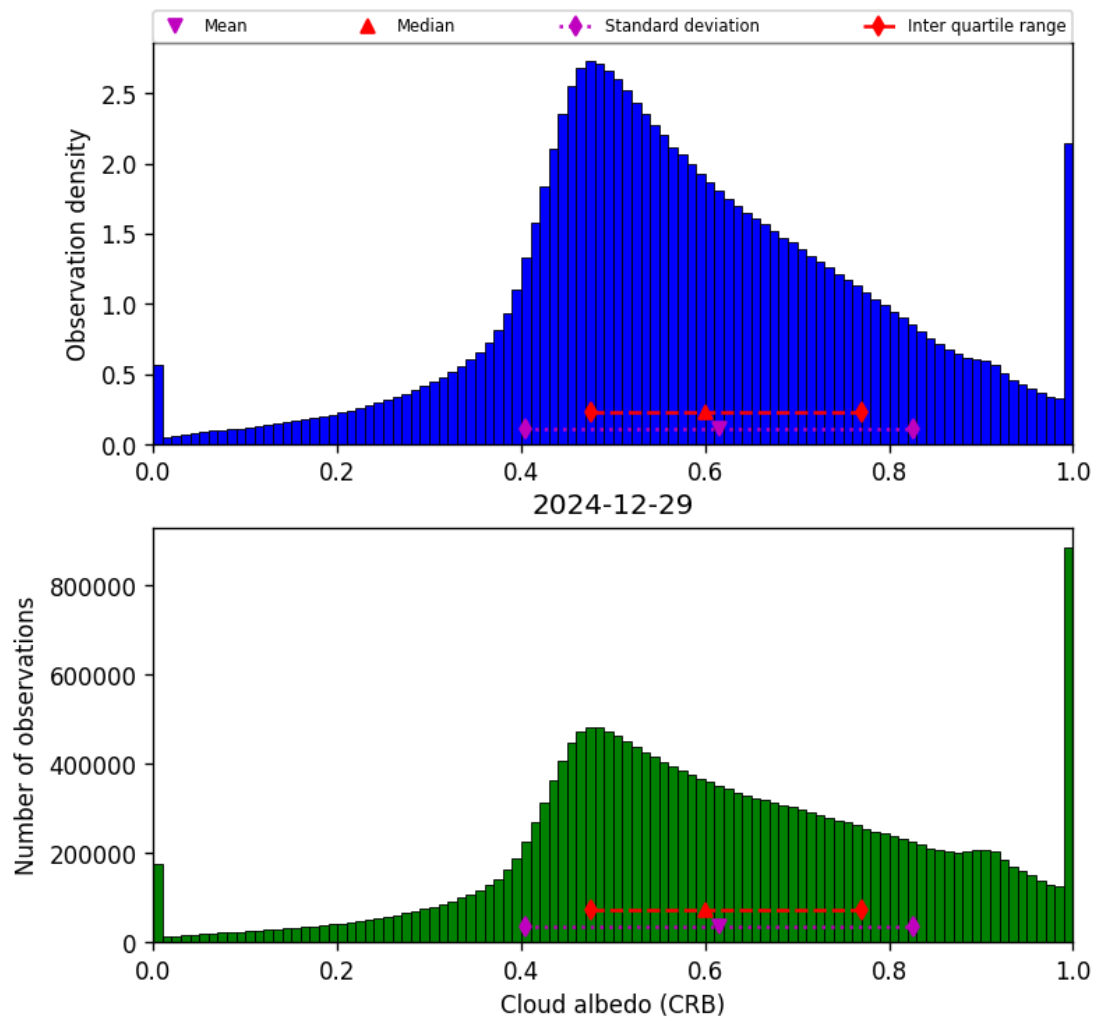
Figure 44: Histogram of “Cloud albedo (CRB)” for 2024-12-28 to 2024-12-30
