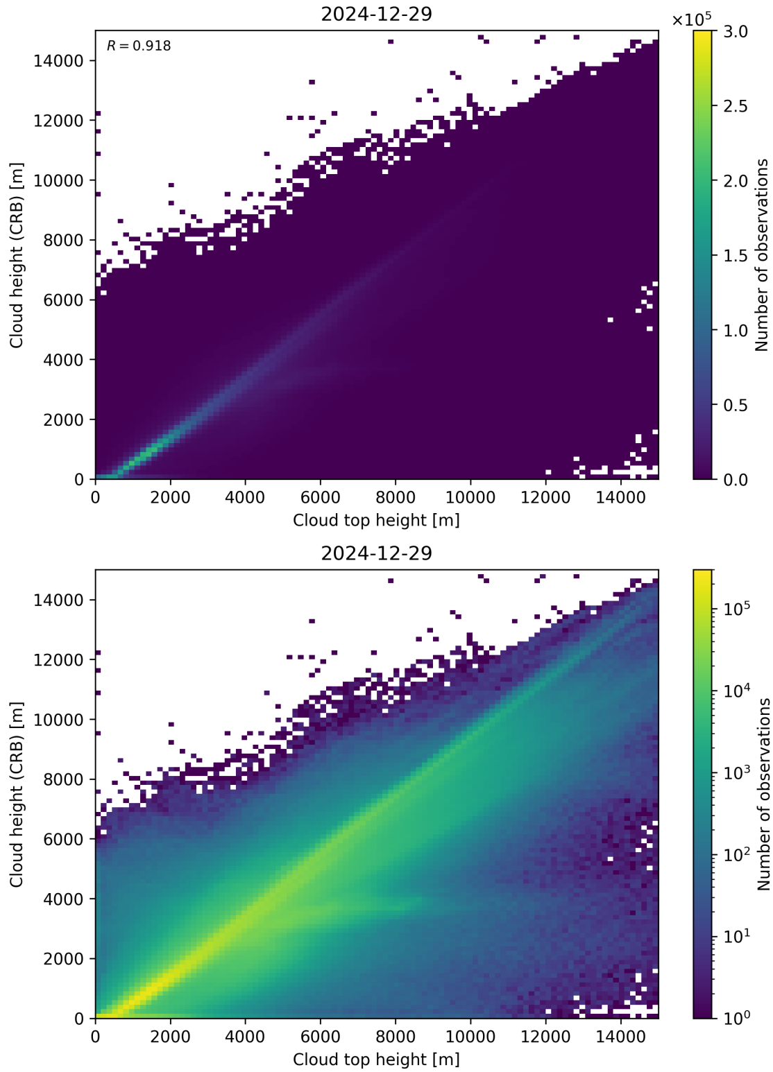
Figure 89: Scatter density plot of “Cloud top height” against “Cloud height (CRB)” for 2024-12-28 to 2024-12-30.
