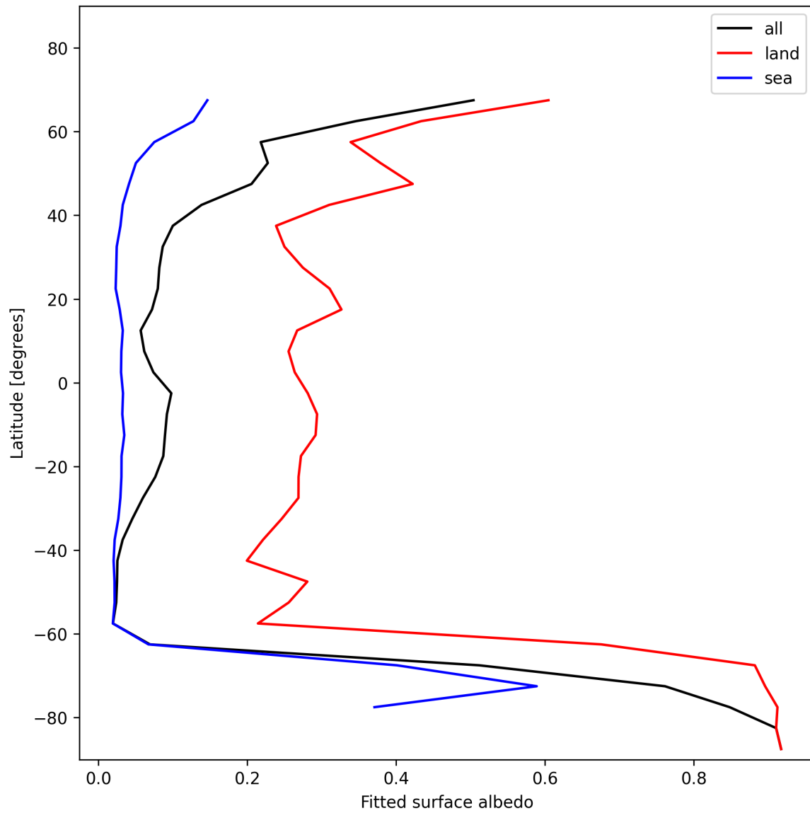
Figure 29: Zonal average of “Fitted surface albedo” for 2024-12-28 to 2024-12-30.
