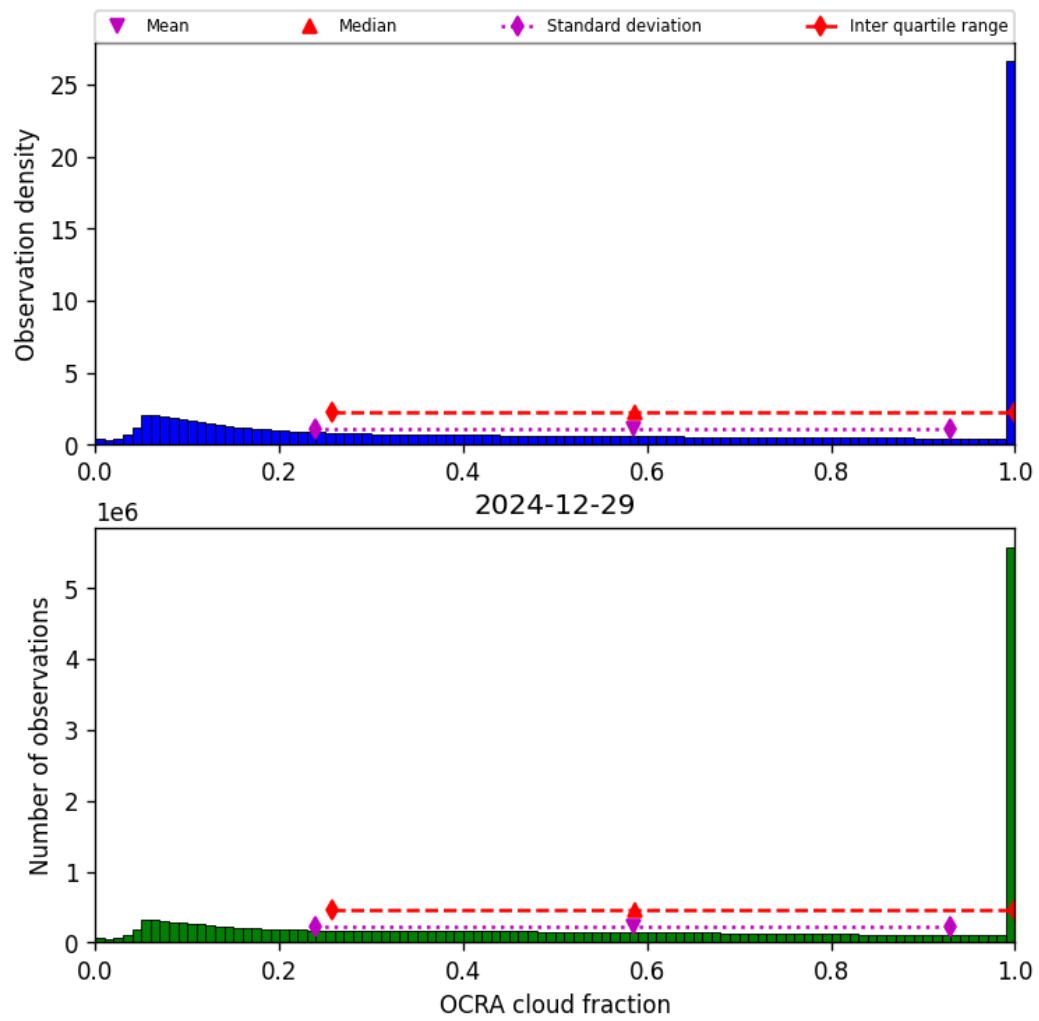
Figure 50: Histogram of “OCRA cloud fraction” for 2024-12-28 to 2024-12-30
