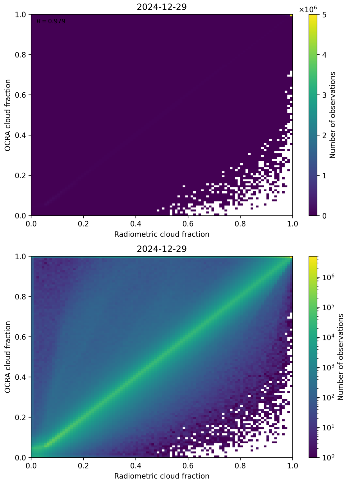
Figure 72: Scatter density plot of “Radiometric cloud fraction” against “OCRA cloud fraction” for 2024-12-28 to 2024-12-30.
