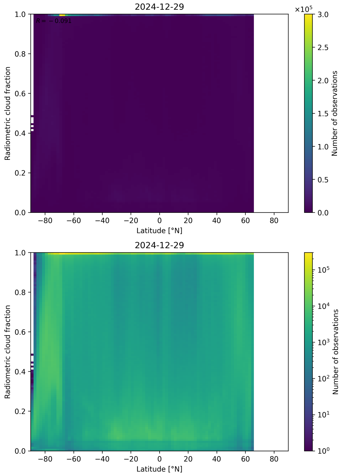
Figure 92: Scatter density plot of “Latitude” against “Radiometric cloud fraction” for 2024-12-28 to 2024-12-30.
