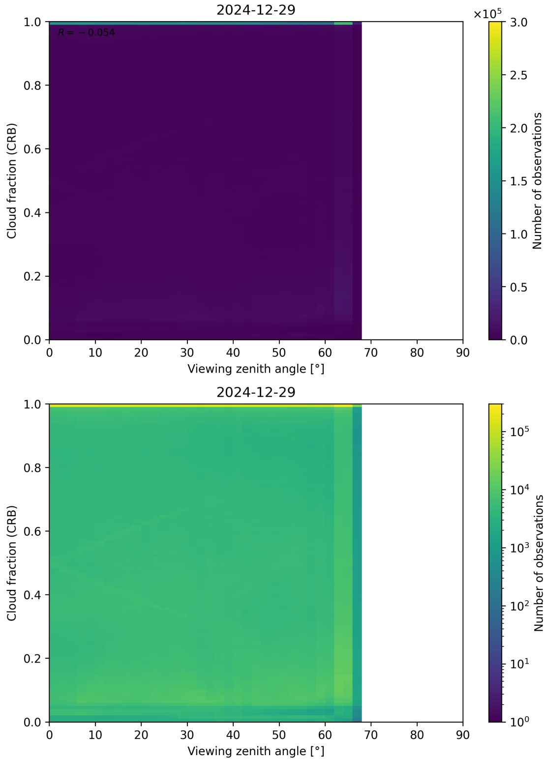
Figure 109: Scatter density plot of “Viewing zenith angle” against “Cloud fraction (CRB)” for 2024-12-28 to 2024-12-30.
