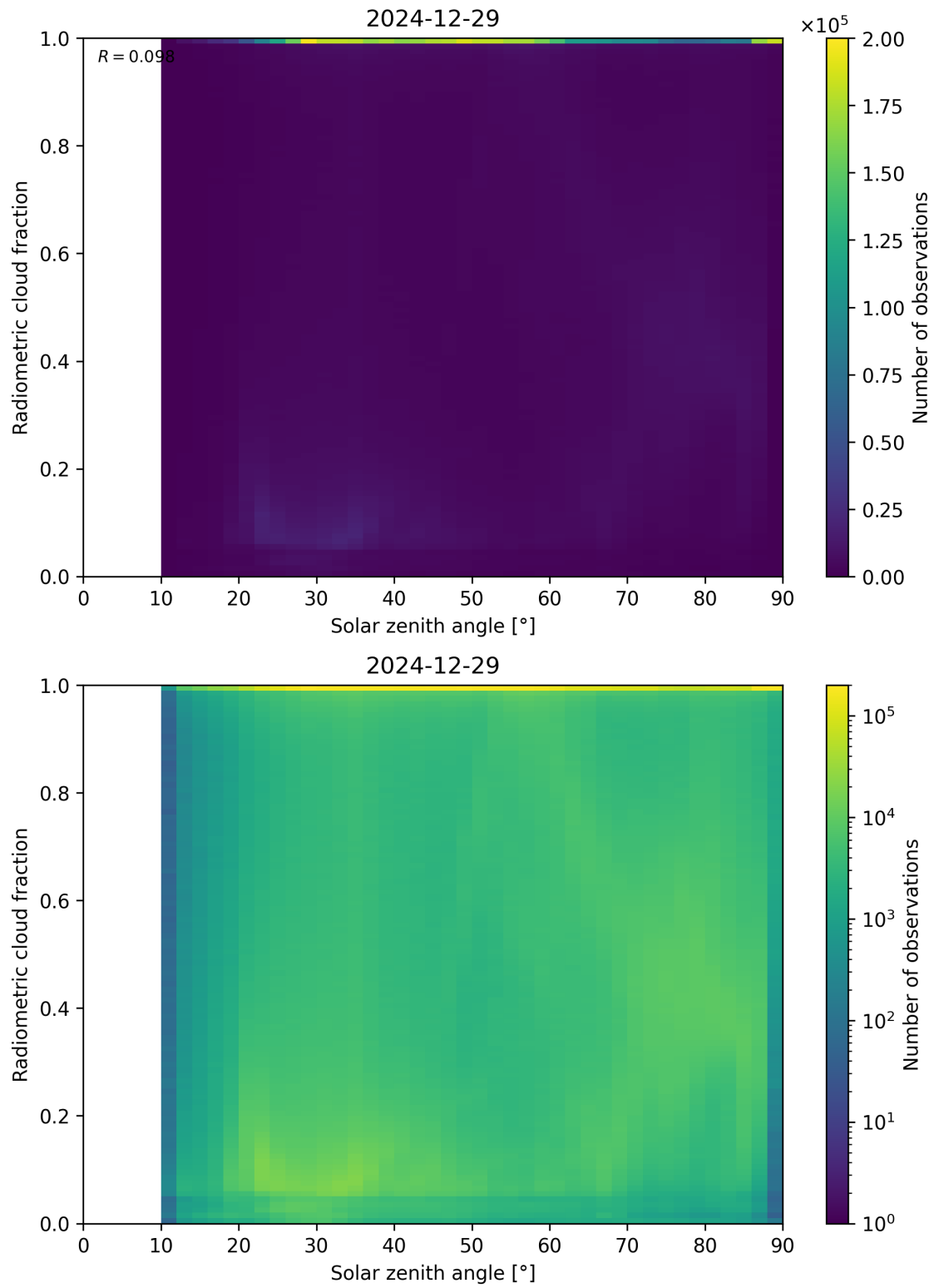
Figure 99: Scatter density plot of “Solar zenith angle” against “Radiometric cloud fraction” for 2024-12-28 to 2024-12-30.
