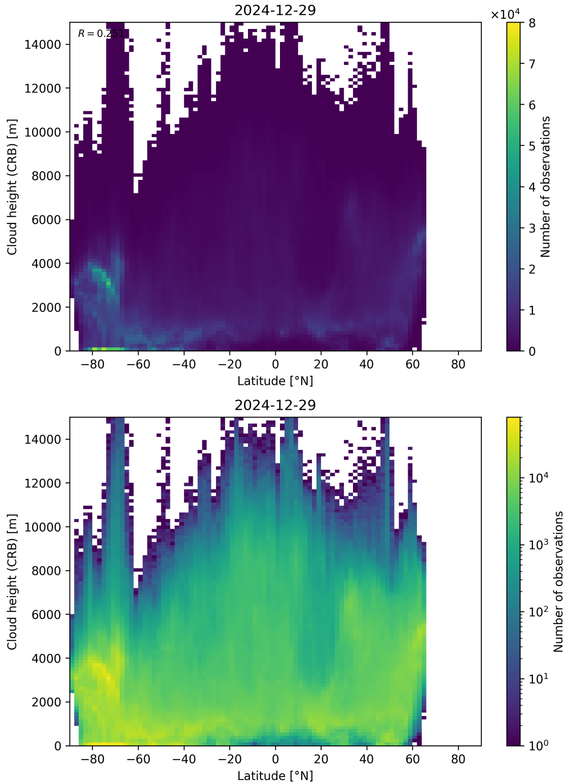
Figure 95: Scatter density plot of “Latitude” against “Cloud height (CRB)” for 2024-12-28 to 2024-12-30.
