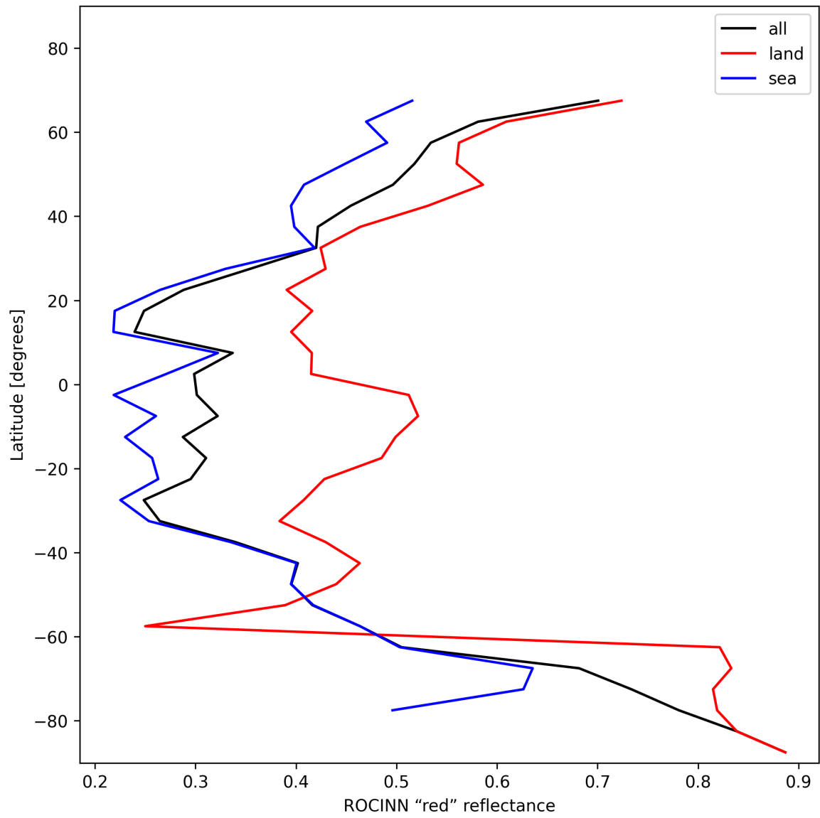
Figure 37: Zonal average of “ROCINN “red” reflectance” for 2024-12-28 to 2024-12-30.
