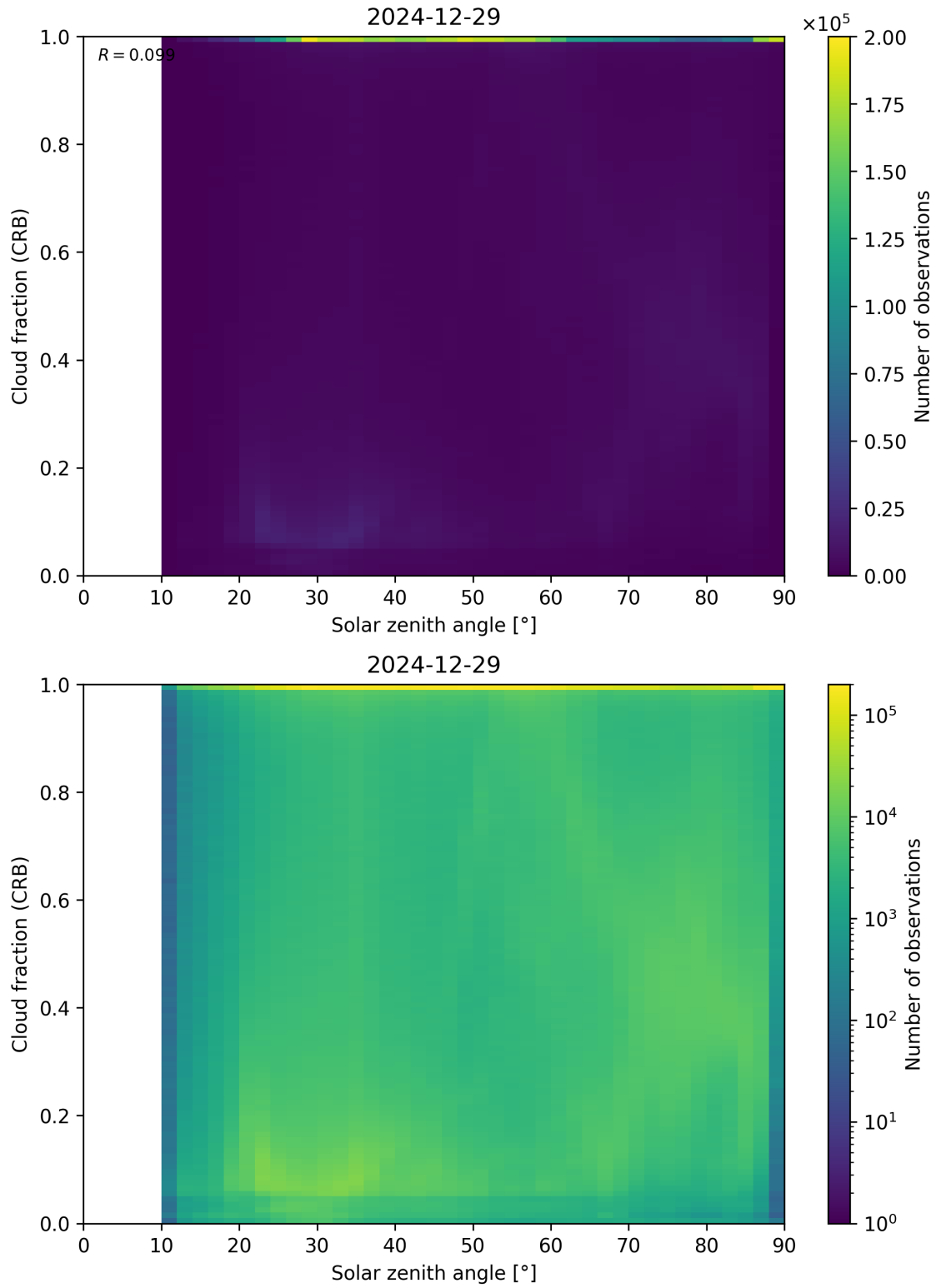
Figure 101: Scatter density plot of “Solar zenith angle” against “Cloud fraction (CRB)” for 2024-12-28 to 2024-12-30.
