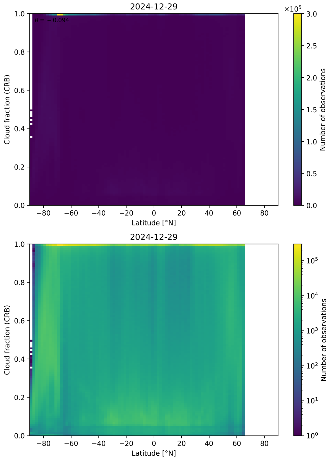
Figure 94: Scatter density plot of “Latitude” against “Cloud fraction (CRB)” for 2024-12-28 to 2024-12-30.
