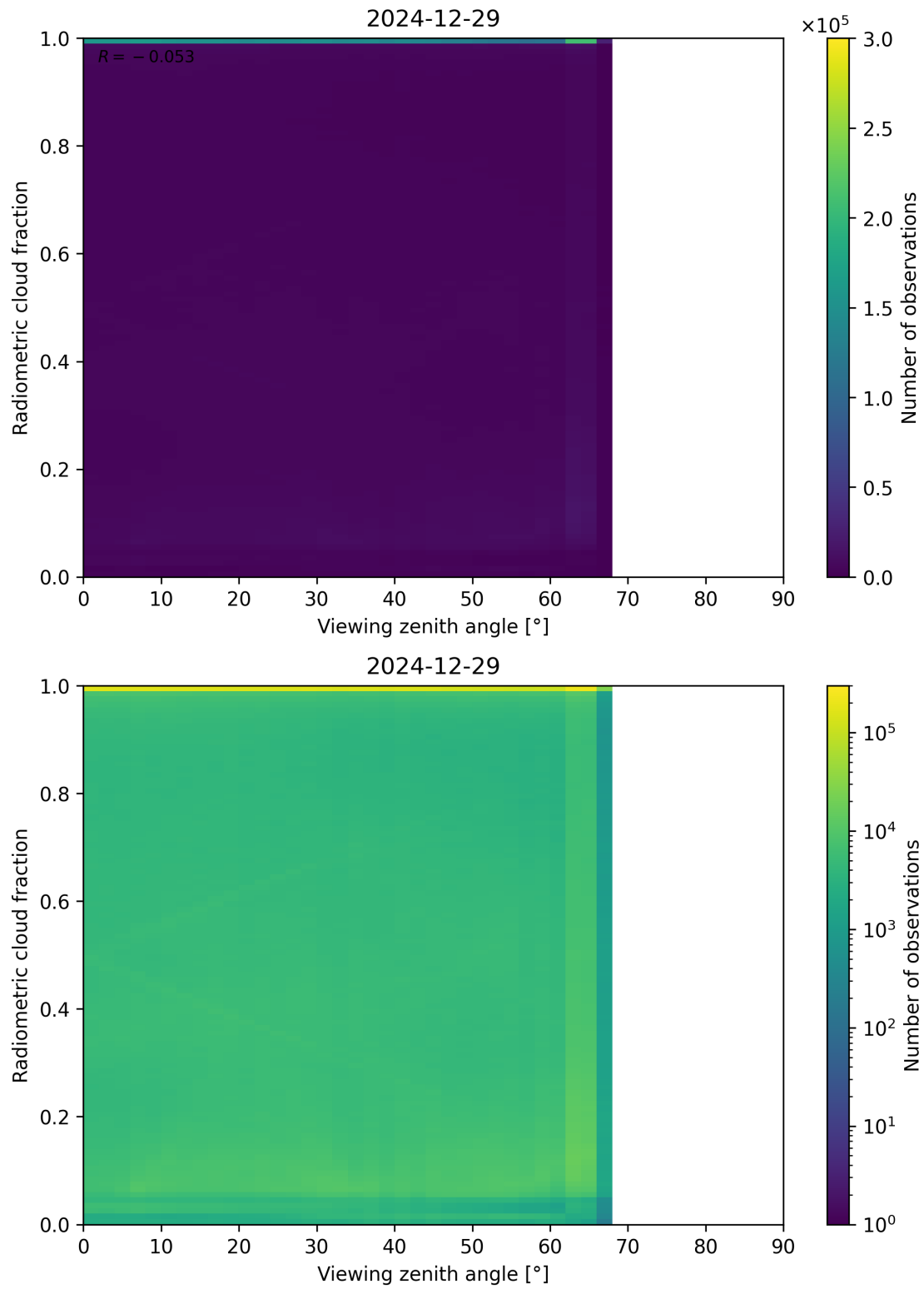
Figure 107: Scatter density plot of “Viewing zenith angle” against “Radiometric cloud fraction” for 2024-12-28 to 2024-12-30.
