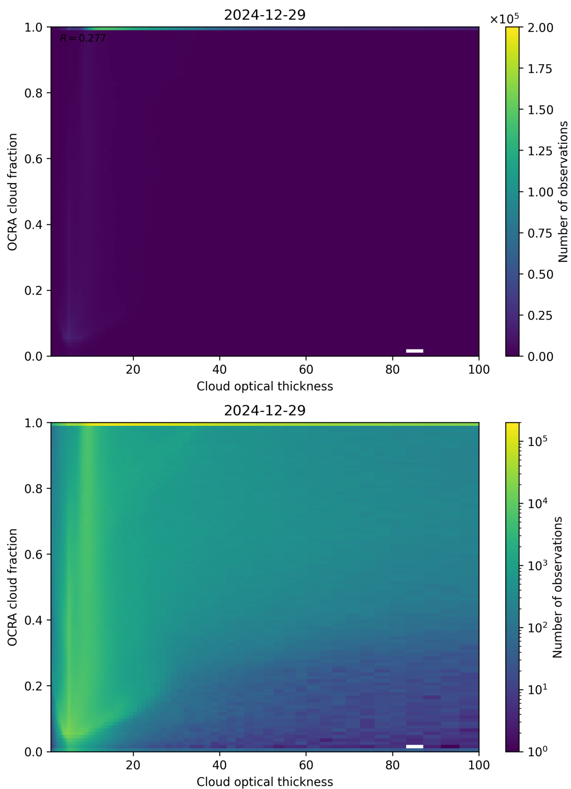
Figure 83: Scatter density plot of “Cloud optical thickness” against “OCRA cloud fraction” for 2024-12-28 to 2024-12-30.
