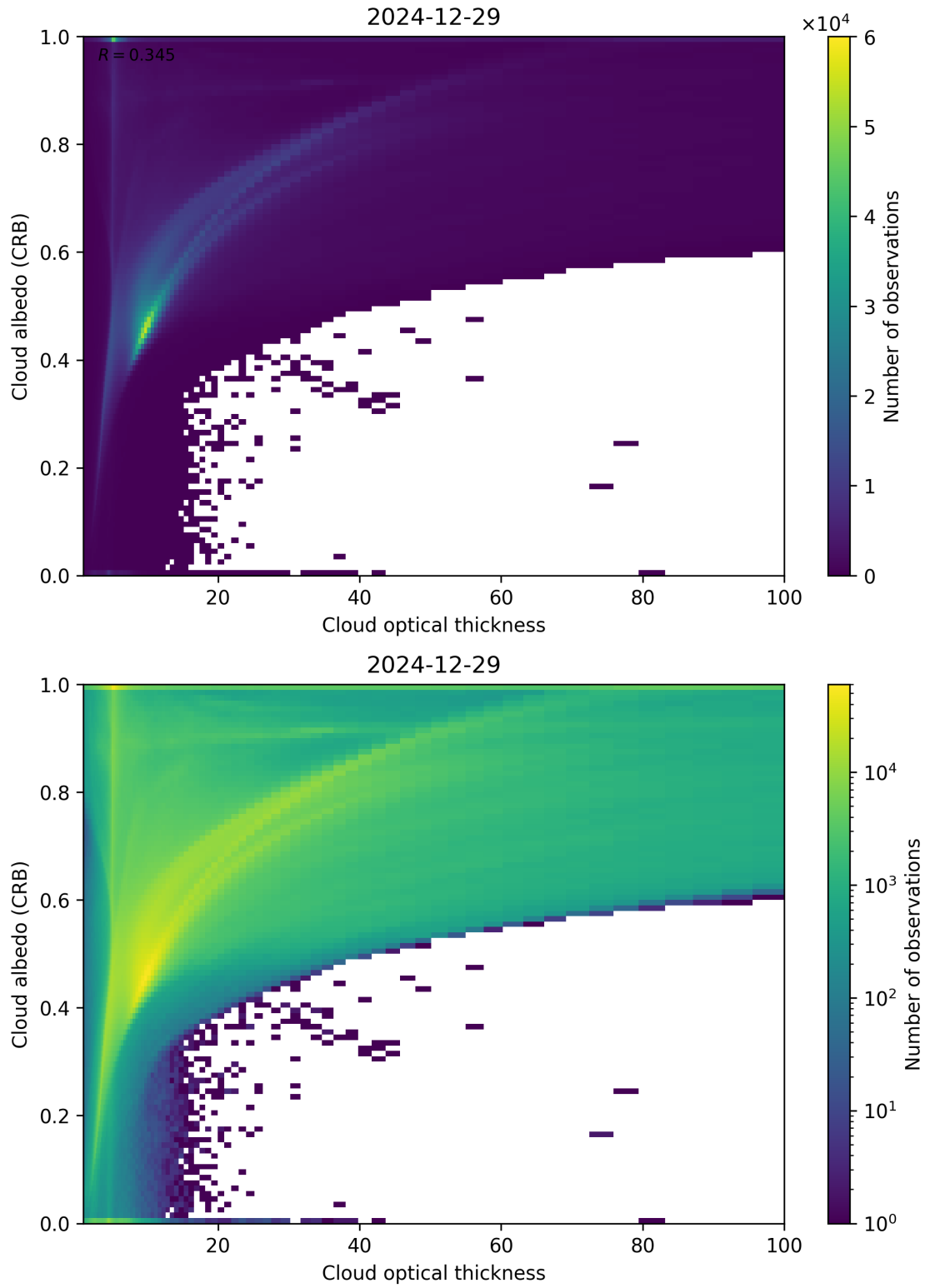
Figure 82: Scatter density plot of “Cloud optical thickness” against “Cloud albedo (CRB)” for 2024-12-28 to 2024-12-30.
