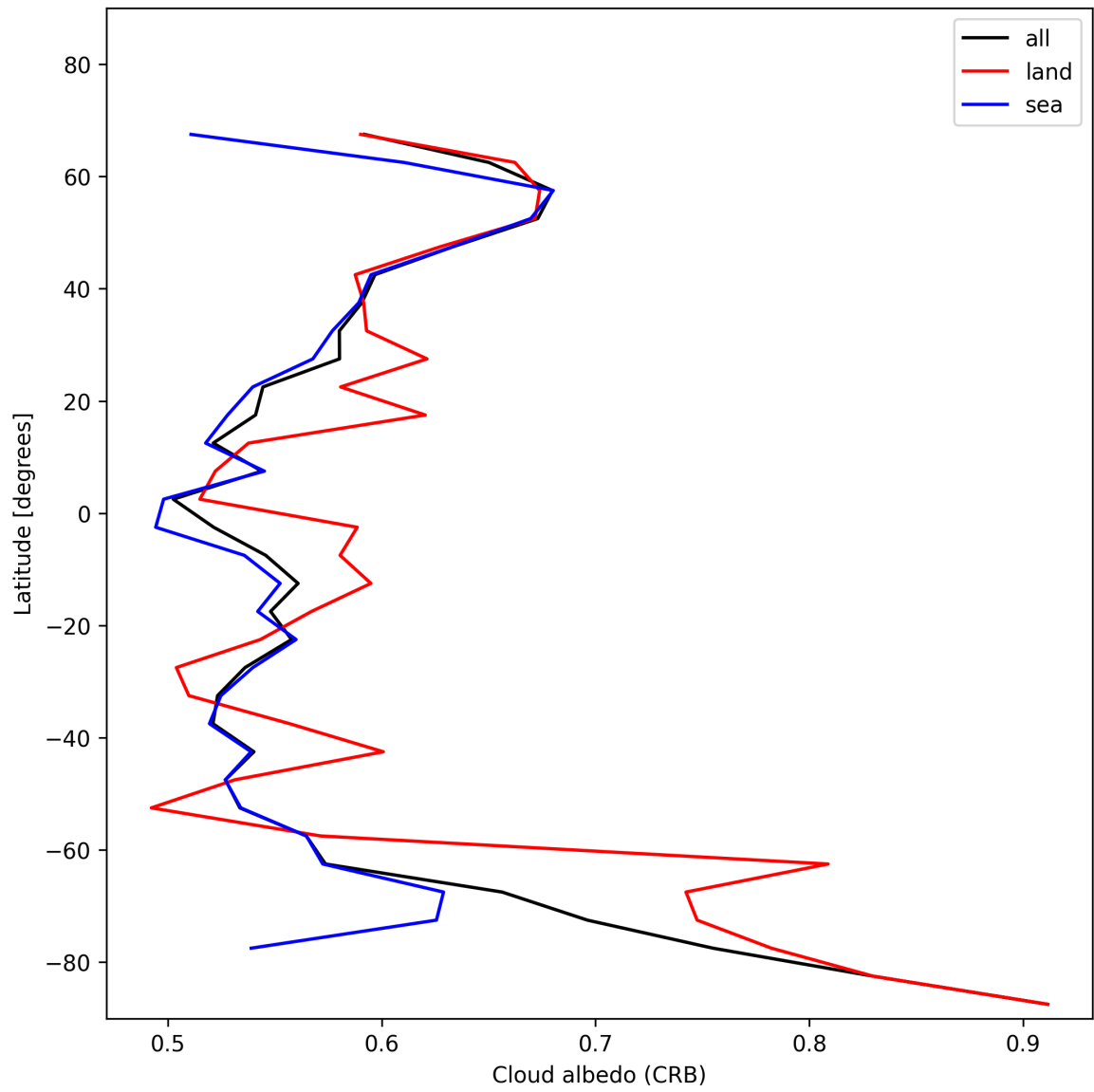
Figure 28: Zonal average of “Cloud albedo (CRB)” for 2024-12-28 to 2024-12-30.
