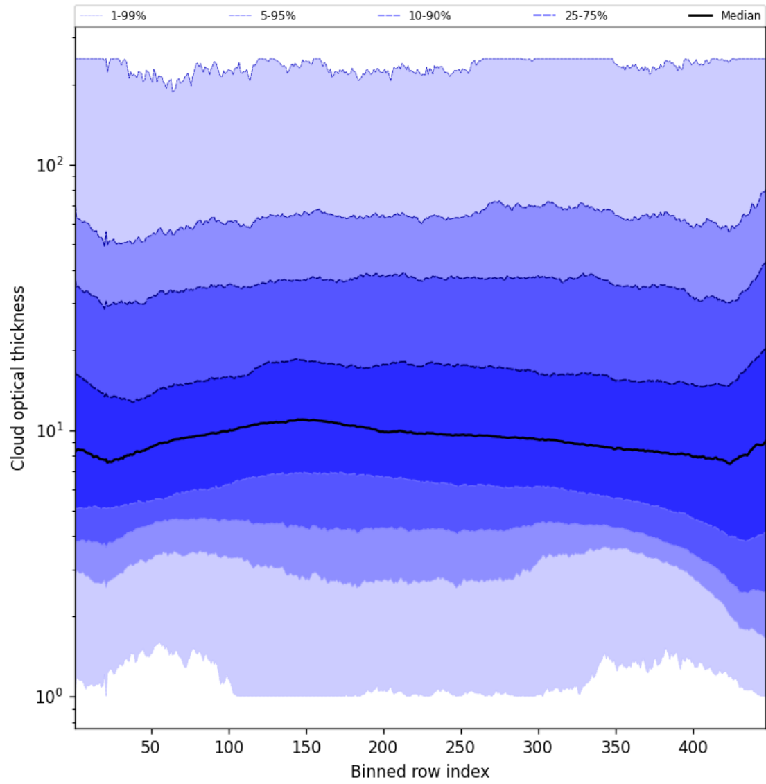
Figure 57: Along track statistics of “Cloud optical thickness” for 2024-12-28 to 2024-12-30
