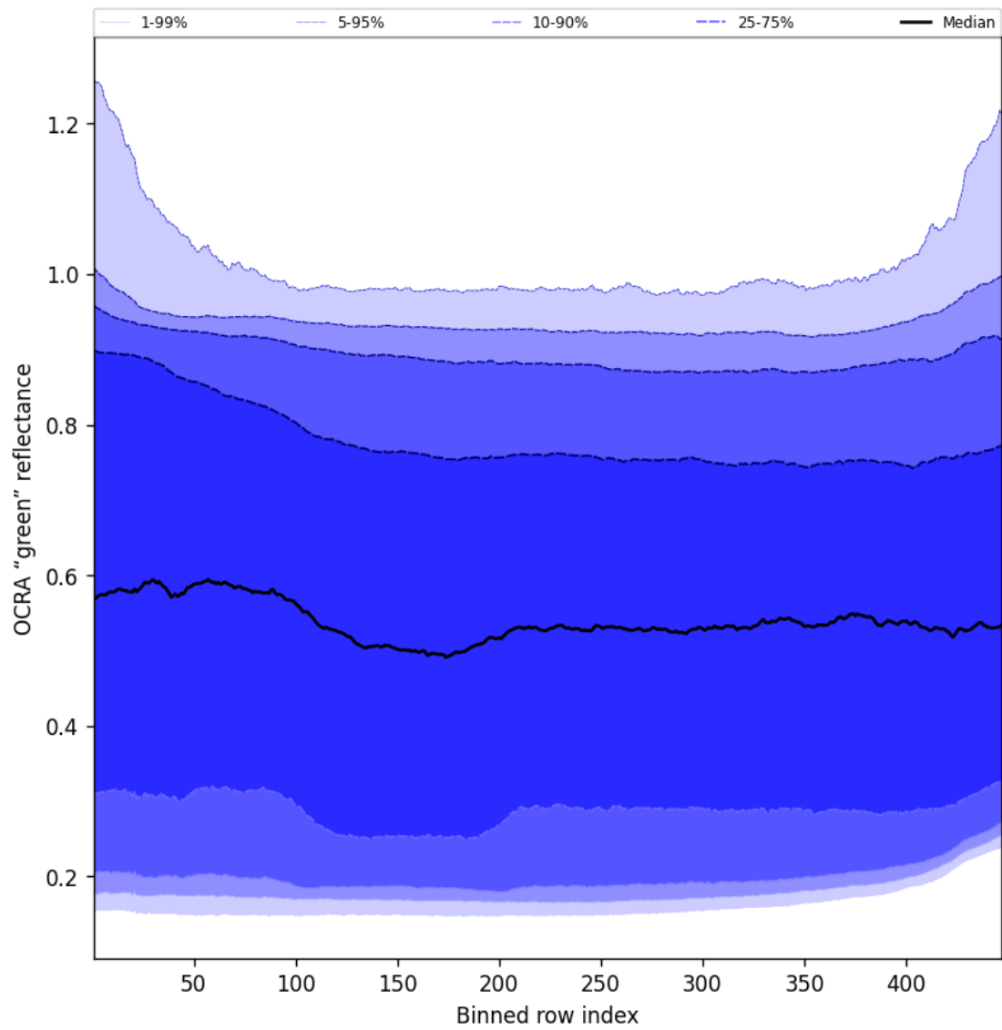
Figure 68: Along track statistics of "OCRA "green" reflectance" for 2024-12-28 to 2024-12-30
