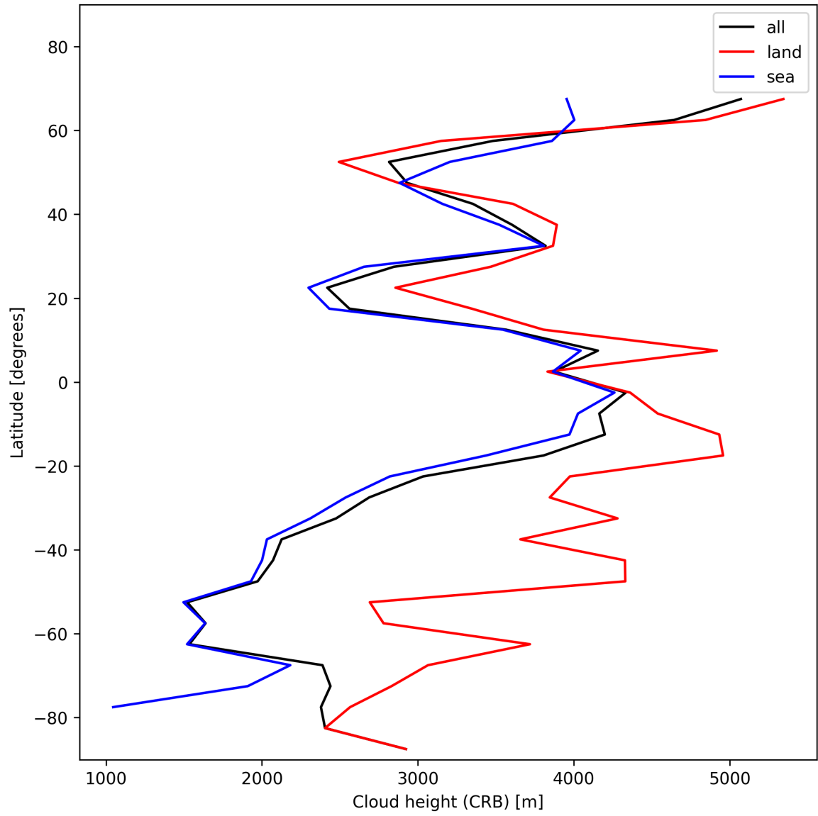
Figure 27: Zonal average of “Cloud height (CRB)” for 2024-12-28 to 2024-12-30.
