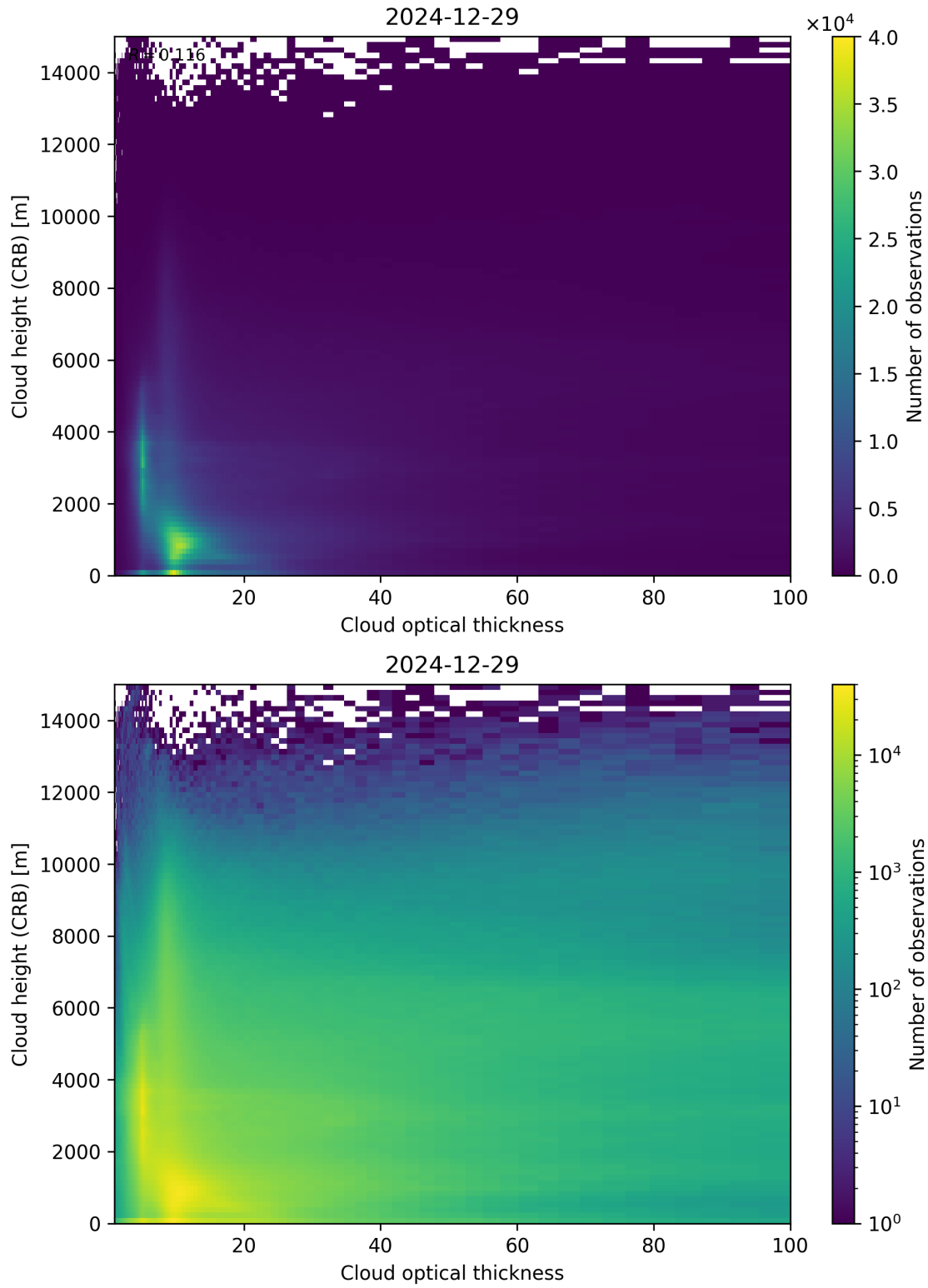
Figure 85: Scatter density plot of “Cloud optical thickness” against “Cloud height (CRB)” for 2024-12-28 to 2024-12-30.
