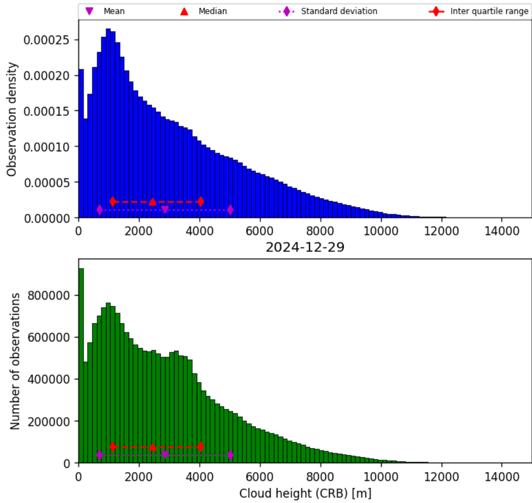
Figure 43: Histogram of “Cloud height (CRB)” for 2024-12-28 to 2024-12-30
