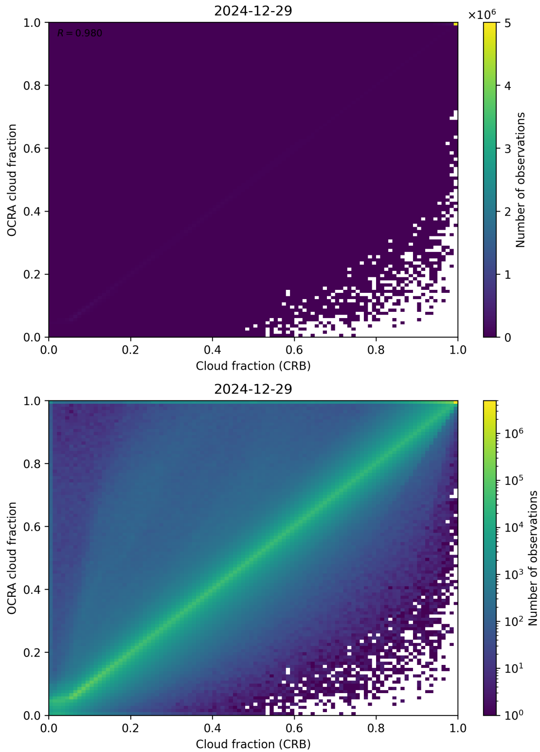
Figure 78: Scatter density plot of “Cloud fraction (CRB)” against “OCRA cloud fraction” for 2024-12-28 to 2024-12-30.
