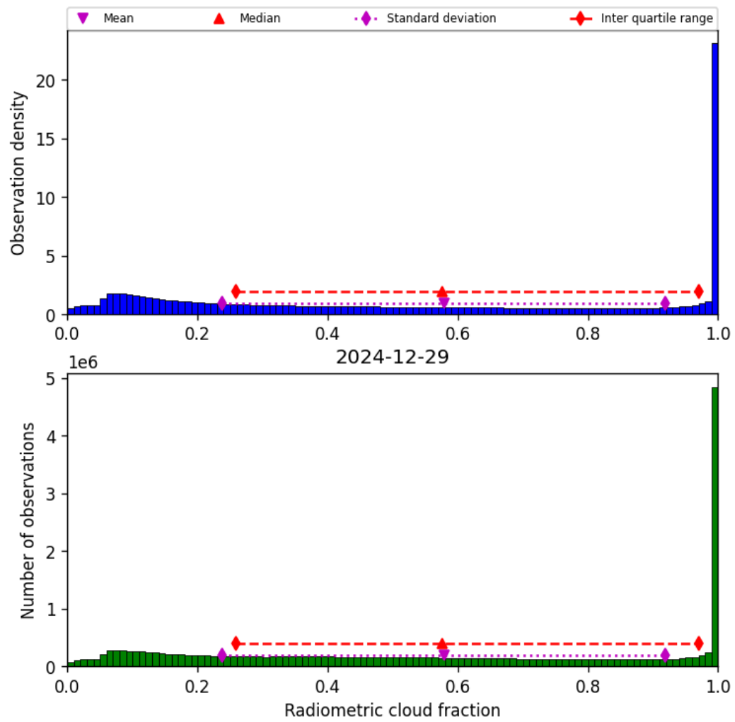
Figure 39: Histogram of “Radiometric cloud fraction” for 2024-12-28 to 2024-12-30
