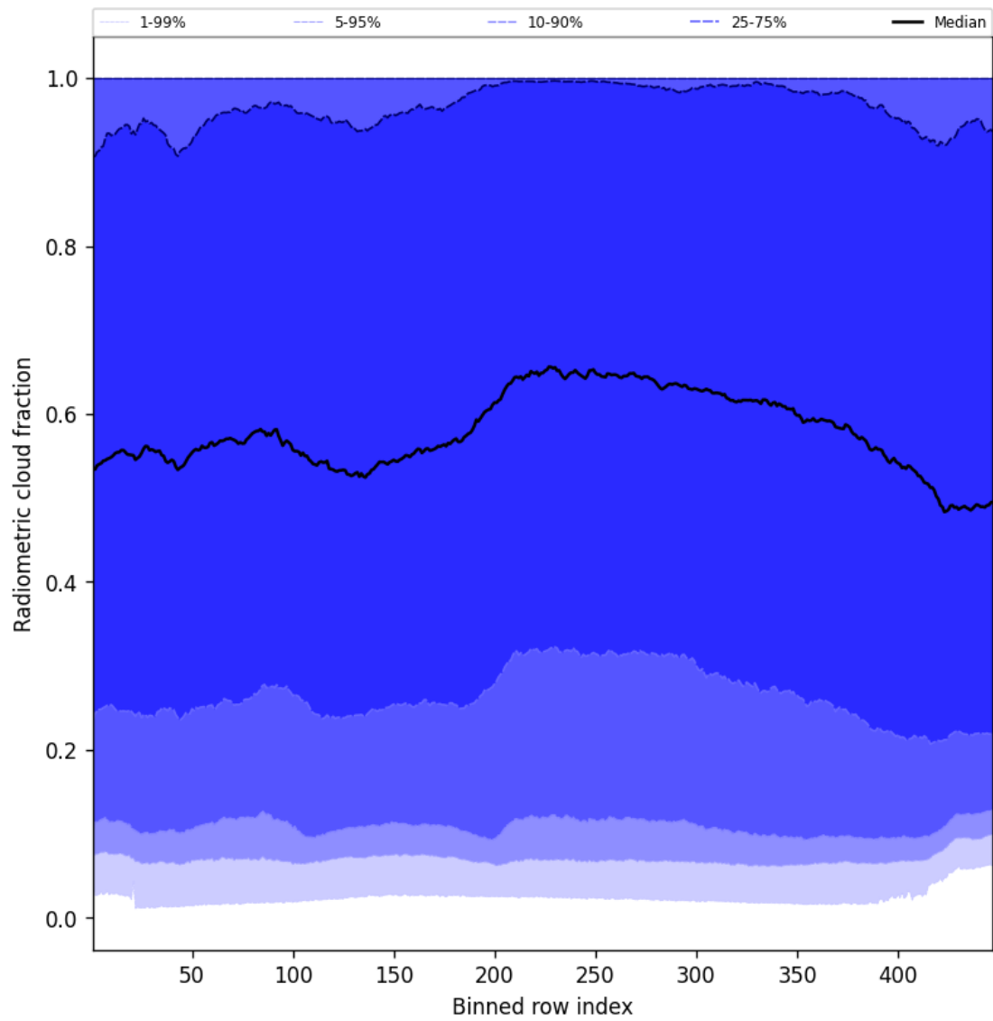
Figure 55: Along track statistics of “Radiometric cloud fraction” for 2024-12-28 to 2024-12-30
