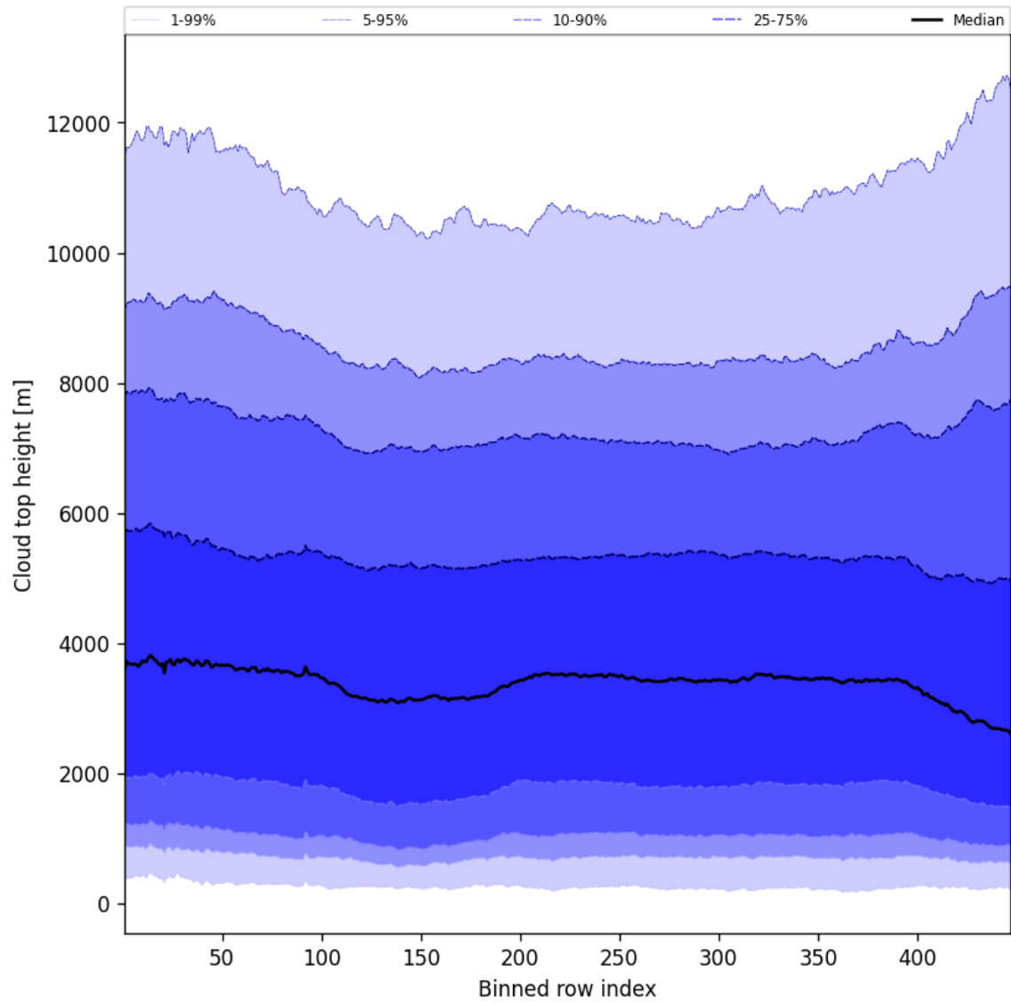
Figure 56: Along track statistics of “Cloud top height” for 2024-12-28 to 2024-12-30
