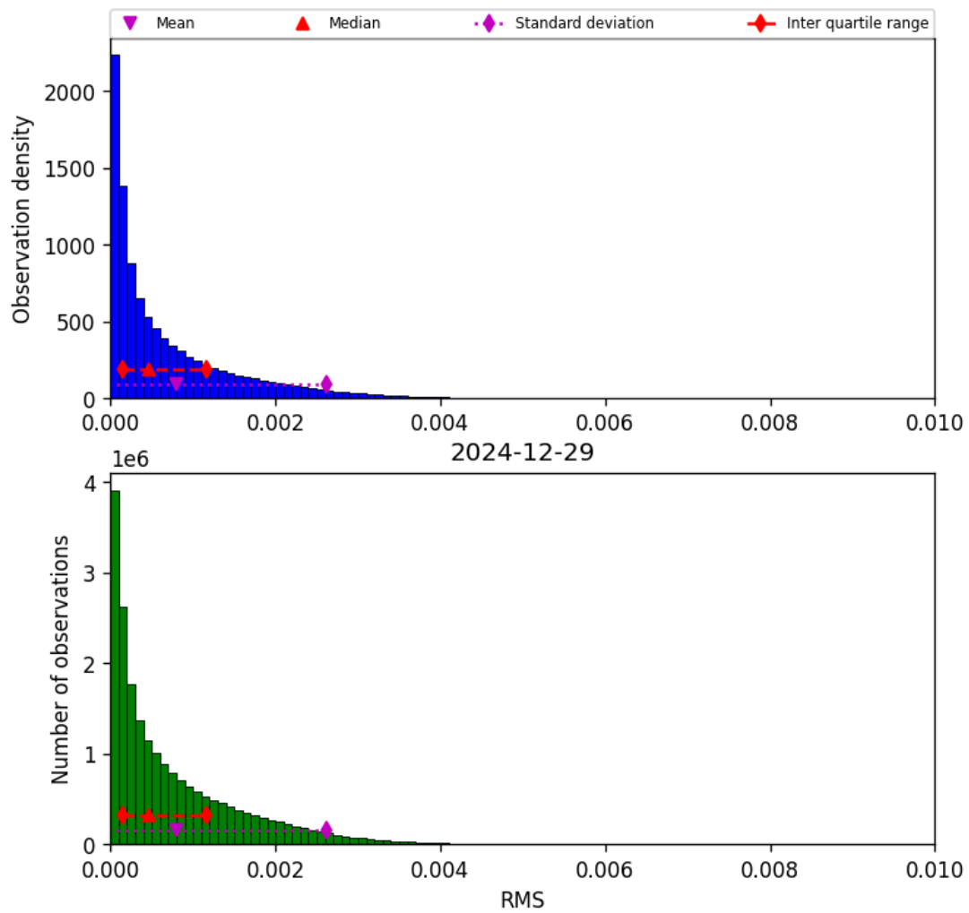
Figure 47: Histogram of “RMS” for 2024-12-28 to 2024-12-30
