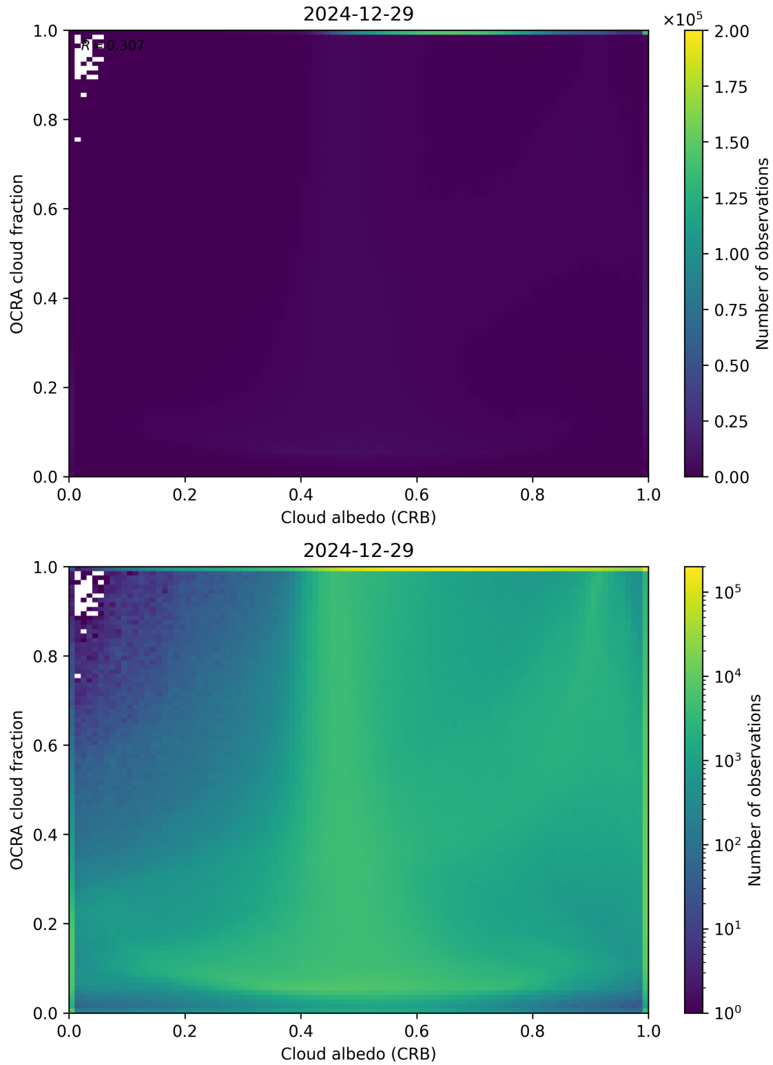
Figure 70: Scatter density plot of “Cloud albedo (CRB)” against “OCRA cloud fraction” for 2024-12-28 to 2024-12-30.
