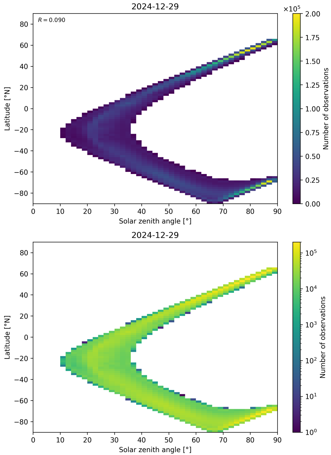
Figure 105: Scatter density plot of “Solar zenith angle” against “Latitude” for 2024-12-28 to 2024-12-30.
