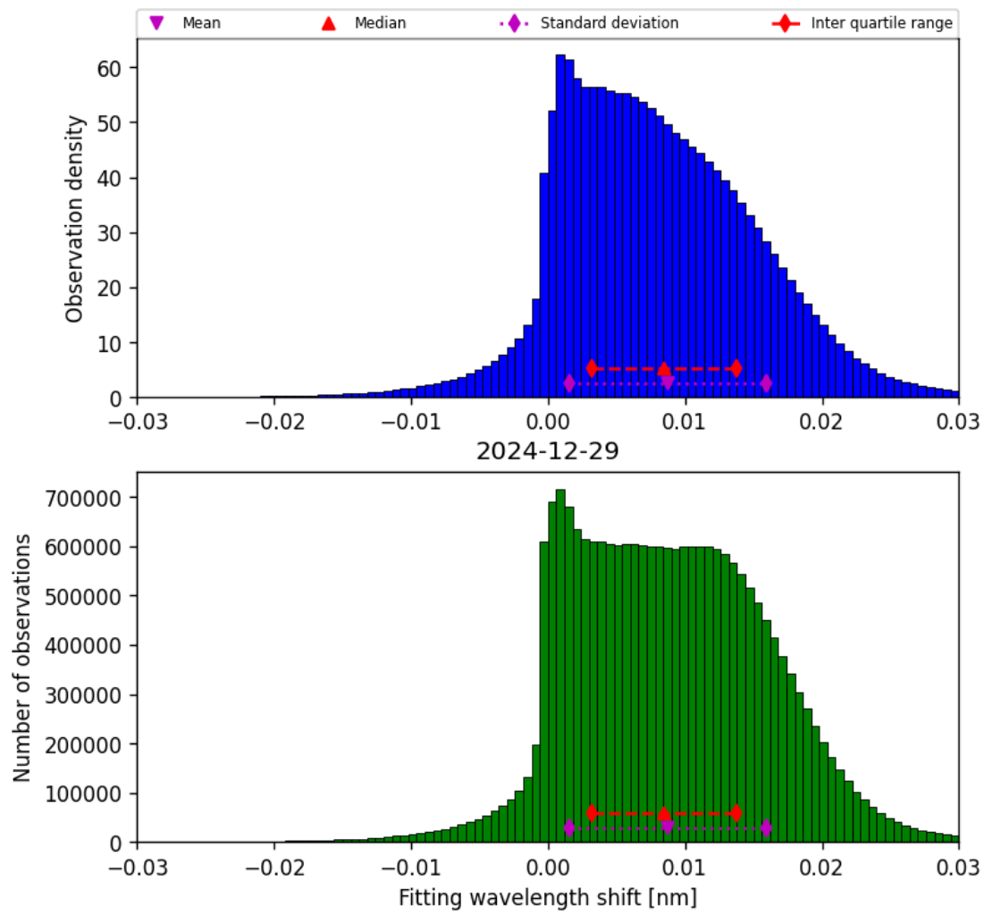
Figure 49: Histogram of “Fitting wavelength shift” for 2024-12-28 to 2024-12-30
