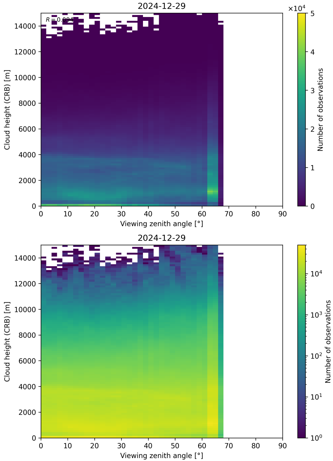
Figure 110: Scatter density plot of “Viewing zenith angle” against “Cloud height (CRB)” for 2024-12-28 to 2024-12-30.
