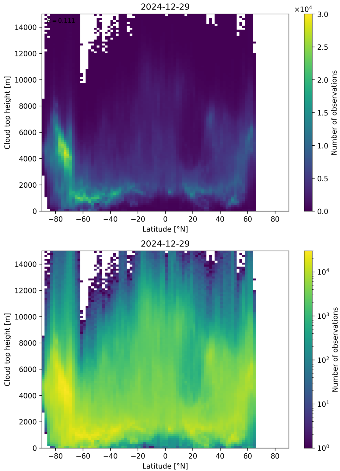
Figure 97: Scatter density plot of “Latitude” against “Cloud top height” for 2024-12-28 to 2024-12-30.
