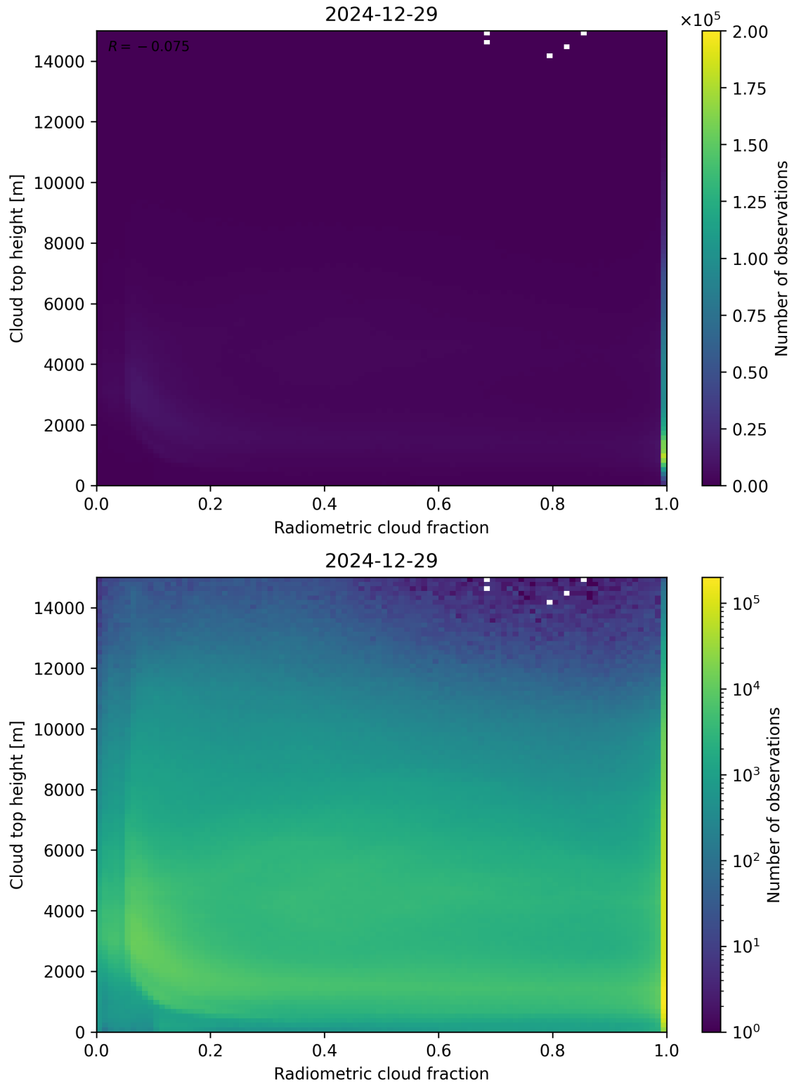
Figure 76: Scatter density plot of “Radiometric cloud fraction” against “Cloud top height” for 2024-12-28 to 2024-12-30.
