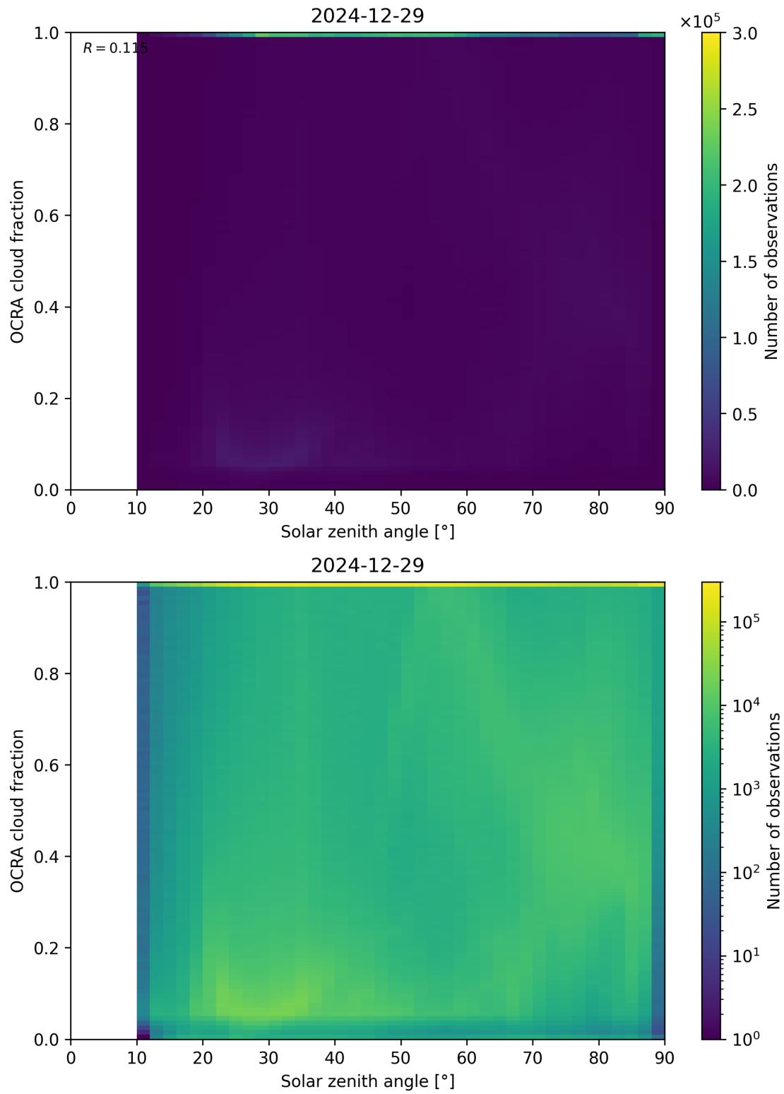
Figure 100: Scatter density plot of “Solar zenith angle” against “OCRA cloud fraction” for 2024-12-28 to 2024-12-30.
