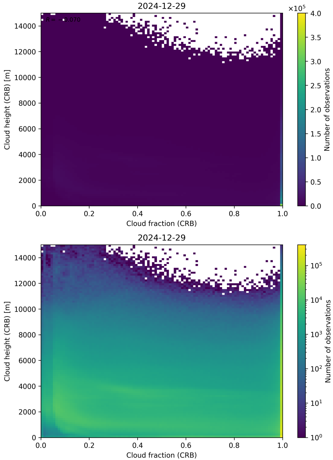
Figure 79: Scatter density plot of “Cloud fraction (CRB)” against “Cloud height (CRB)” for 2024-12-28 to 2024-12-30.
