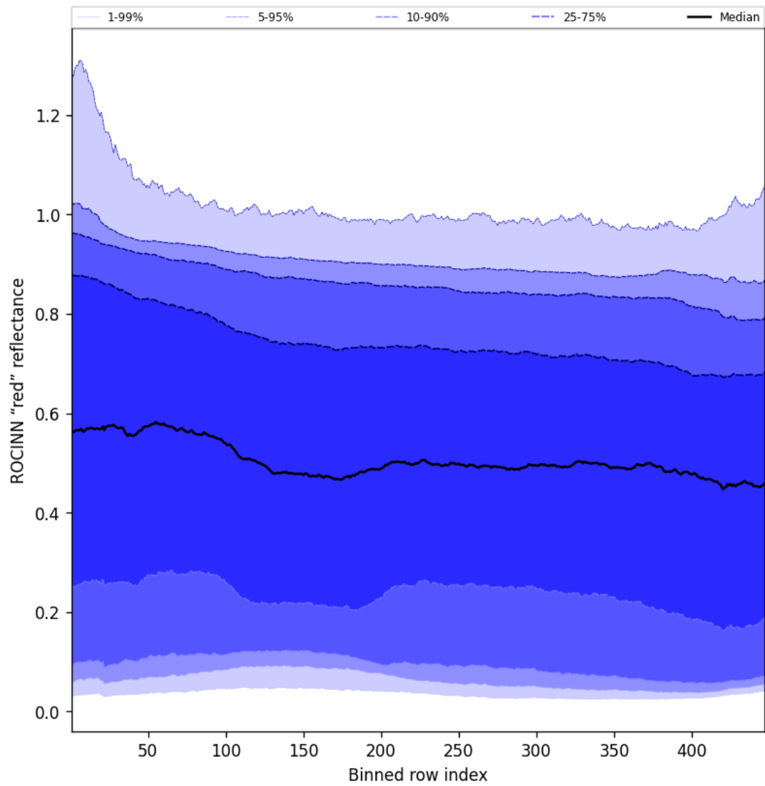
Figure 69: Along track statistics of “ROCINN “red” reflectance” for 2024-12-28 to 2024-12-30
