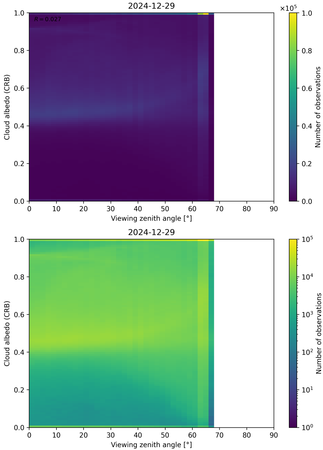
Figure 106: Scatter density plot of “Viewing zenith angle” against “Cloud albedo (CRB)” for 2024-12-28 to 2024-12-30.
