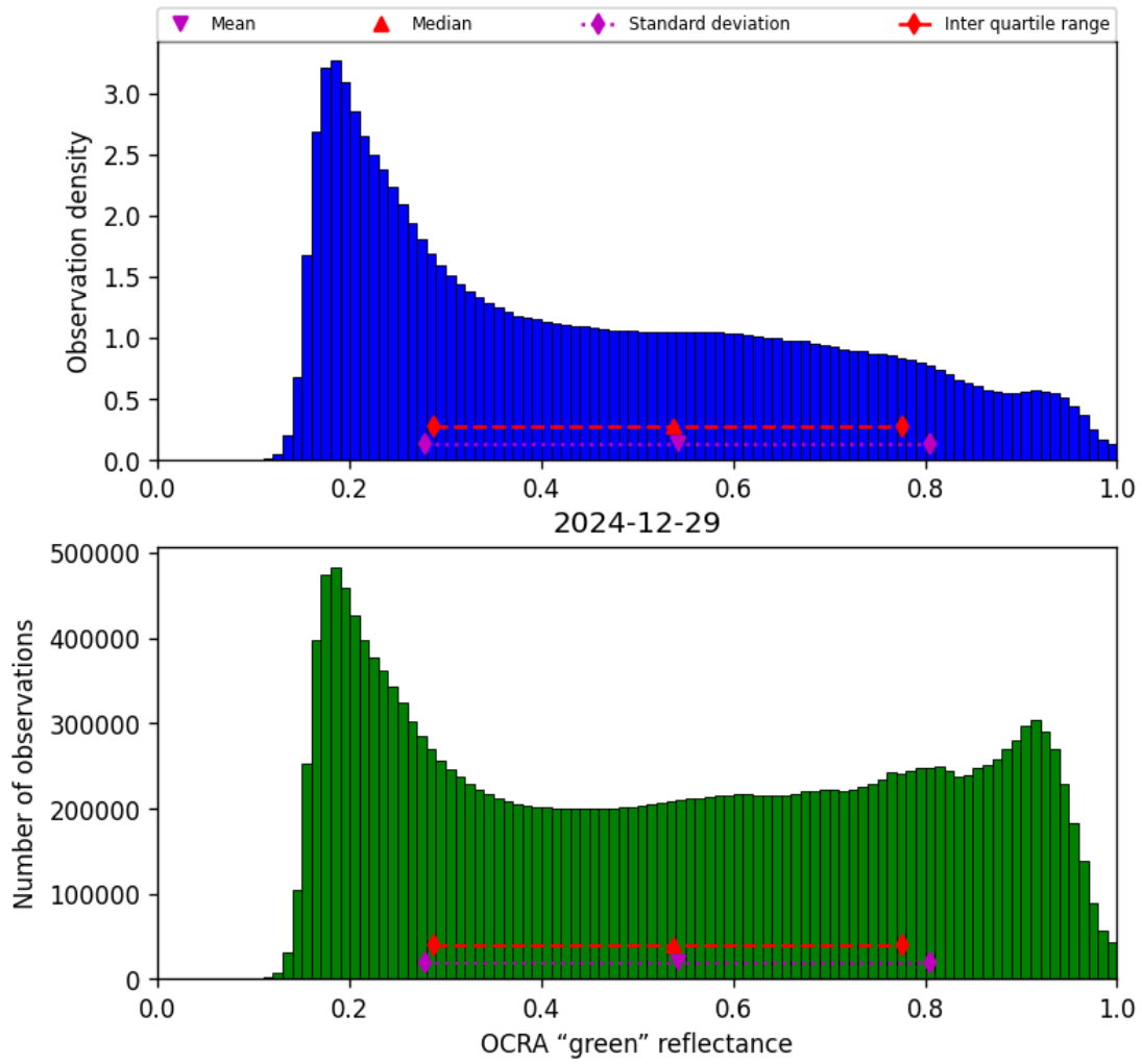
Figure 52: Histogram of “OCRA “green” reflectance” for 2024-12-28 to 2024-12-30
