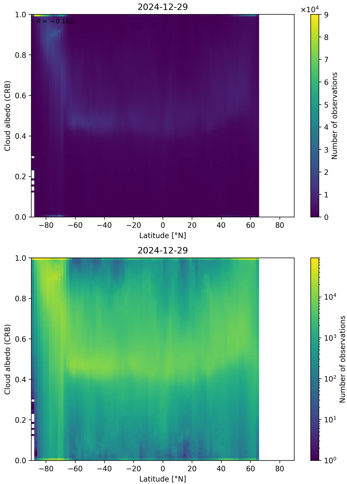
Figure 91: Scatter density plot of “Latitude” against “Cloud albedo (CRB)” for 2024-12-28 to 2024-12-30.
