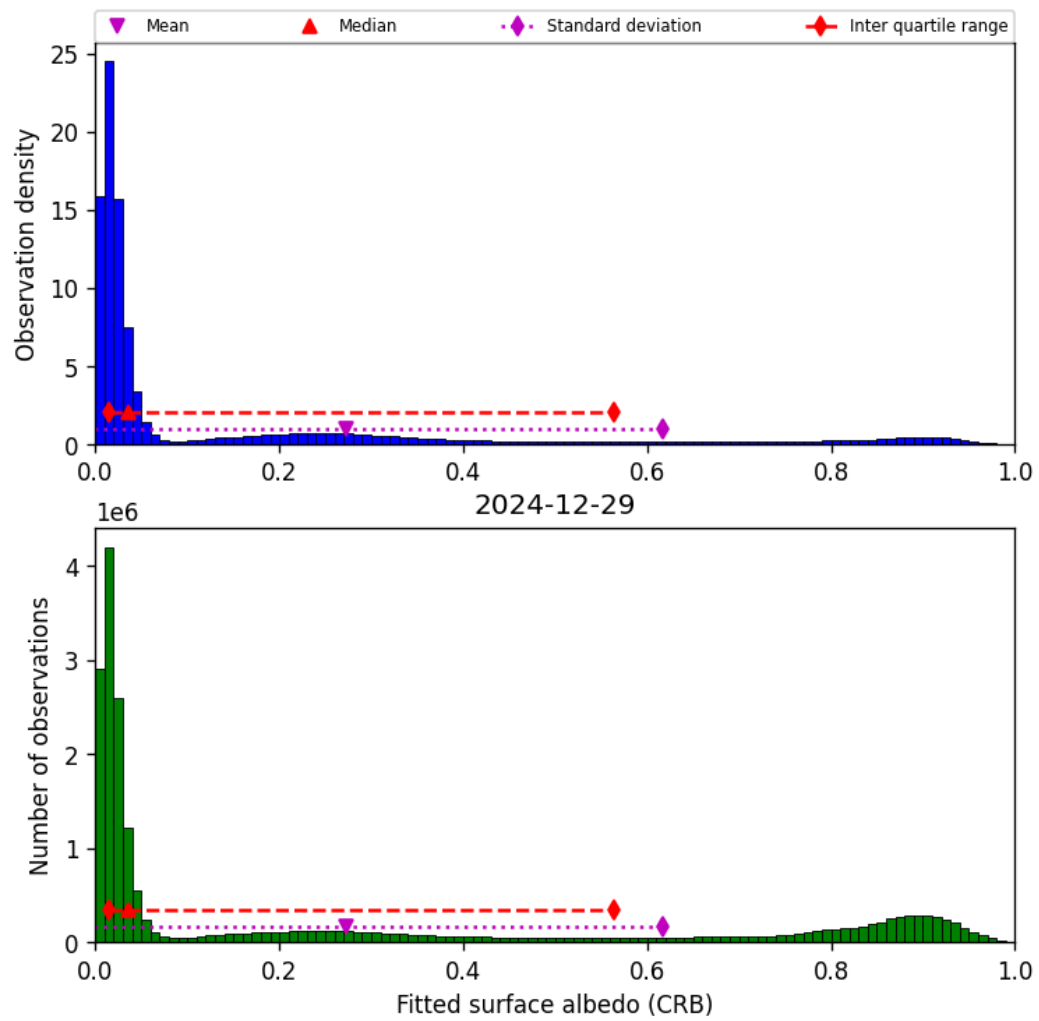
Figure 46: Histogram of “Fitted surface albedo (CRB)” for 2024-12-28 to 2024-12-30
