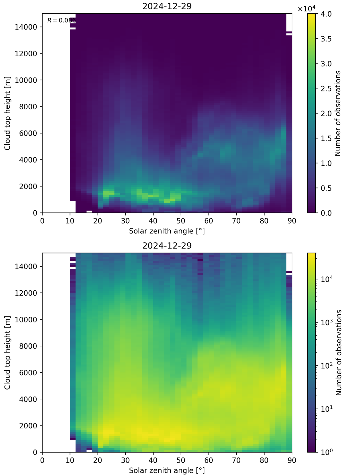
Figure 104: Scatter density plot of “Solar zenith angle” against “Cloud top height” for 2024-12-28 to 2024-12-30.
