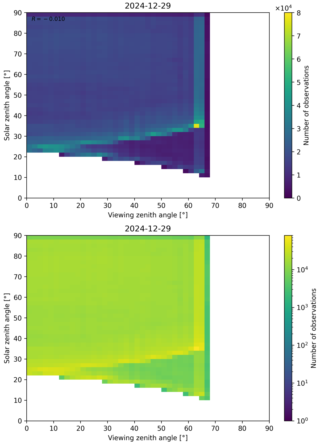
Figure 114: Scatter density plot of “Viewing zenith angle” against “Solar zenith angle” for 2024-12-28 to 2024-12-30.
