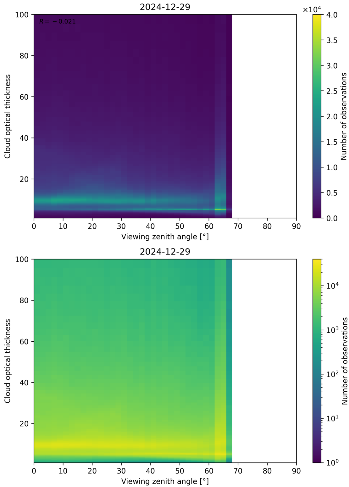
Figure 111: Scatter density plot of “Viewing zenith angle” against “Cloud optical thickness” for 2024-12-28 to 2024-12-30.
