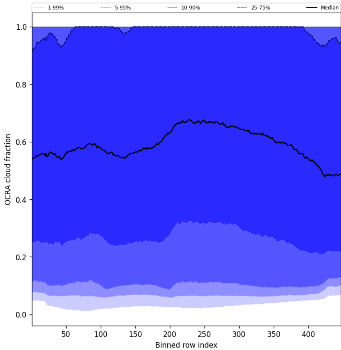
Figure 66: Along track statistics of “OCRA cloud fraction” for 2024-12-28 to 2024-12-30
