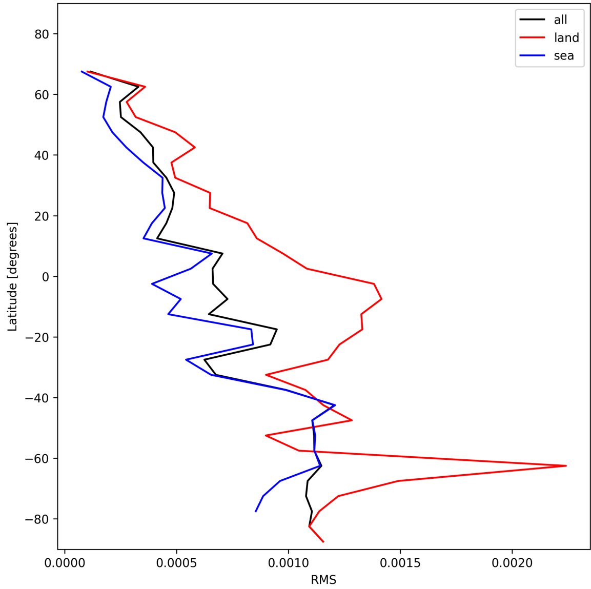
Figure 31: Zonal average of “RMS” for 2024-12-28 to 2024-12-30.
