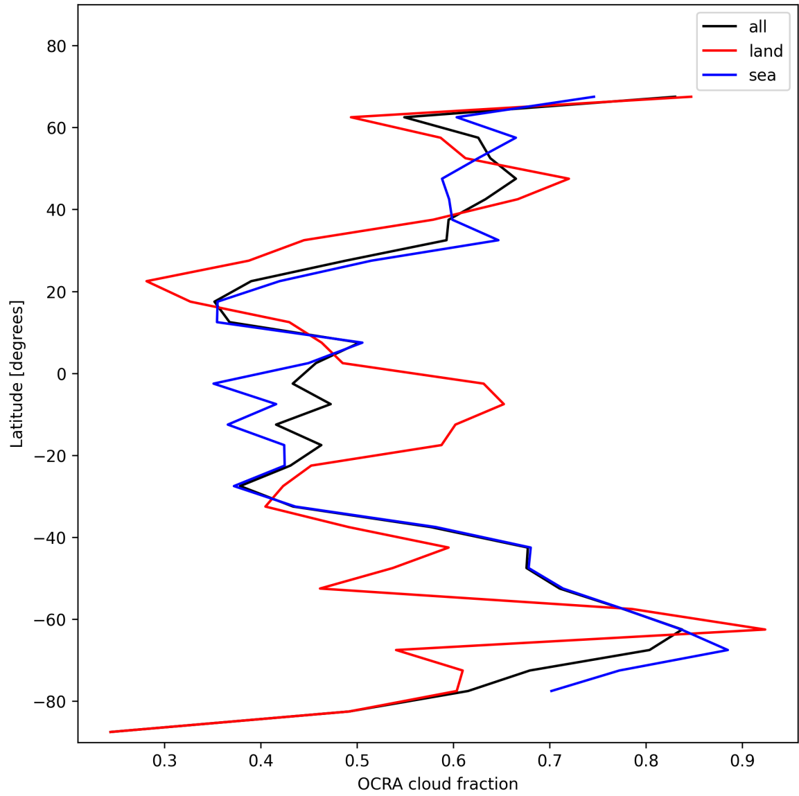
Figure 34: Zonal average of “OCRA cloud fraction” for 2024-12-28 to 2024-12-30.
