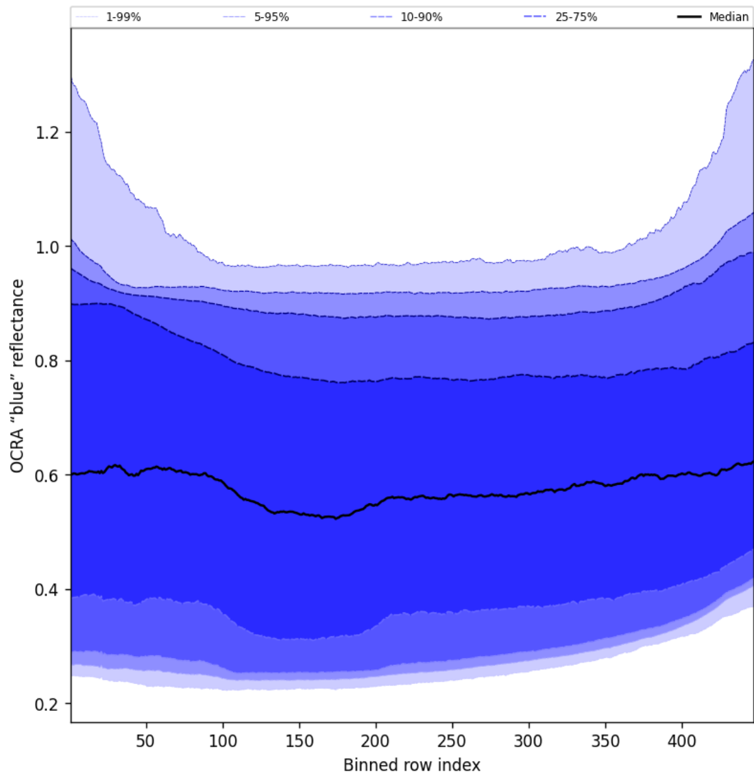
Figure 67: Along track statistics of "OCRA "blue" reflectance" for 2024-12-28 to 2024-12-30
