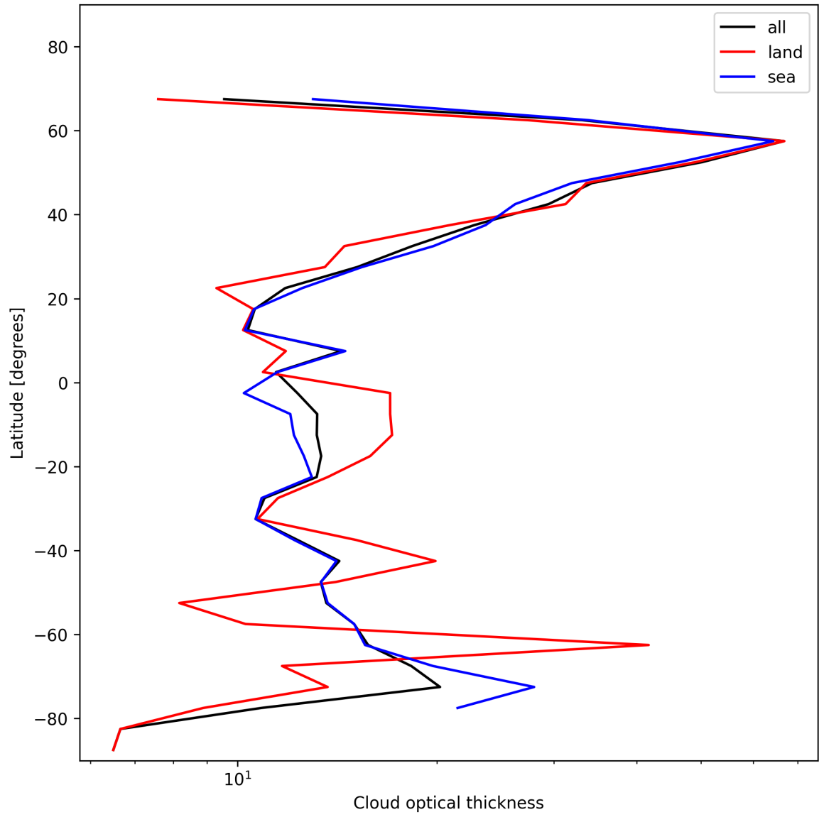
Figure 25: Zonal average of “Cloud optical thickness” for 2024-12-28 to 2024-12-30.
