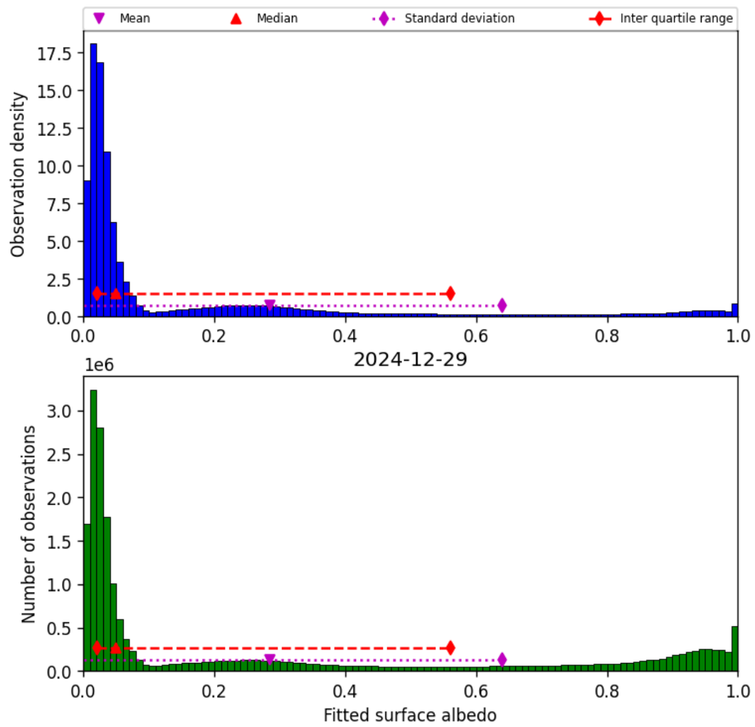
Figure 45: Histogram of “Fitted surface albedo” for 2024-12-28 to 2024-12-30
