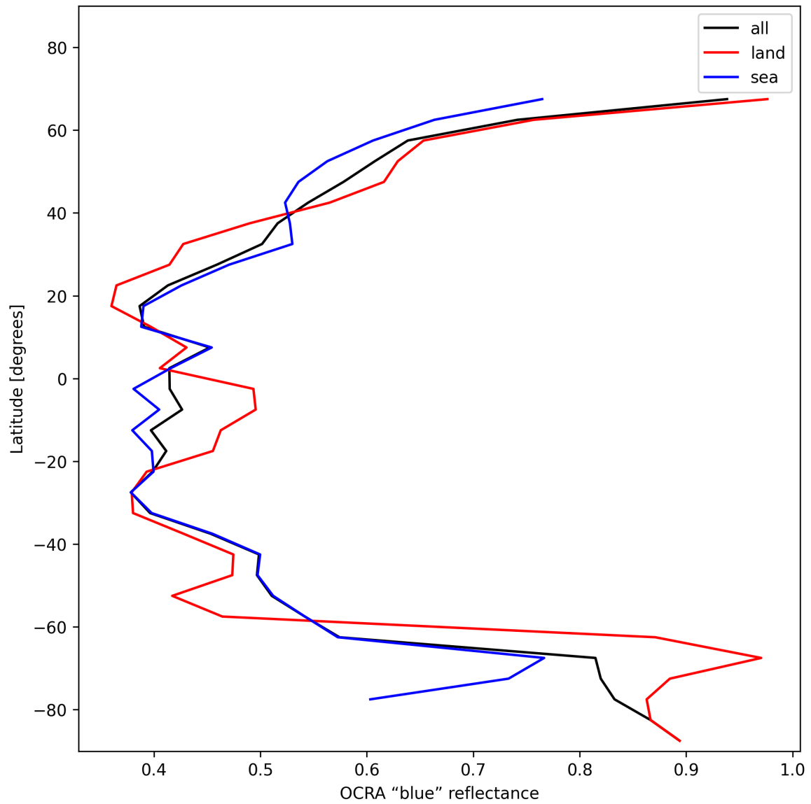
Figure 35: Zonal average of "OCRA "blue" reflectance" for 2024-12-28 to 2024-12-30.
