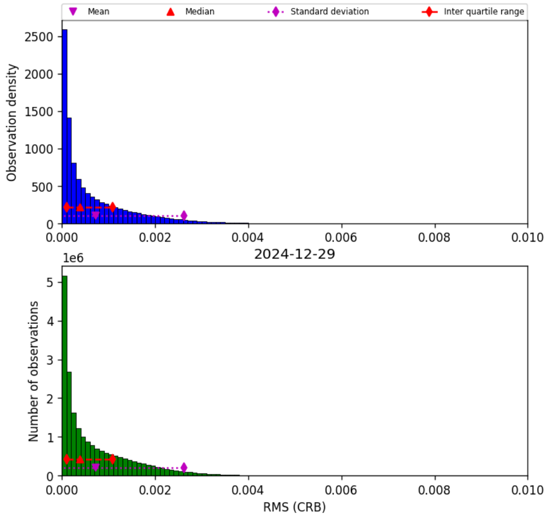
Figure 48: Histogram of “RMS (CRB)” for 2024-12-28 to 2024-12-30
