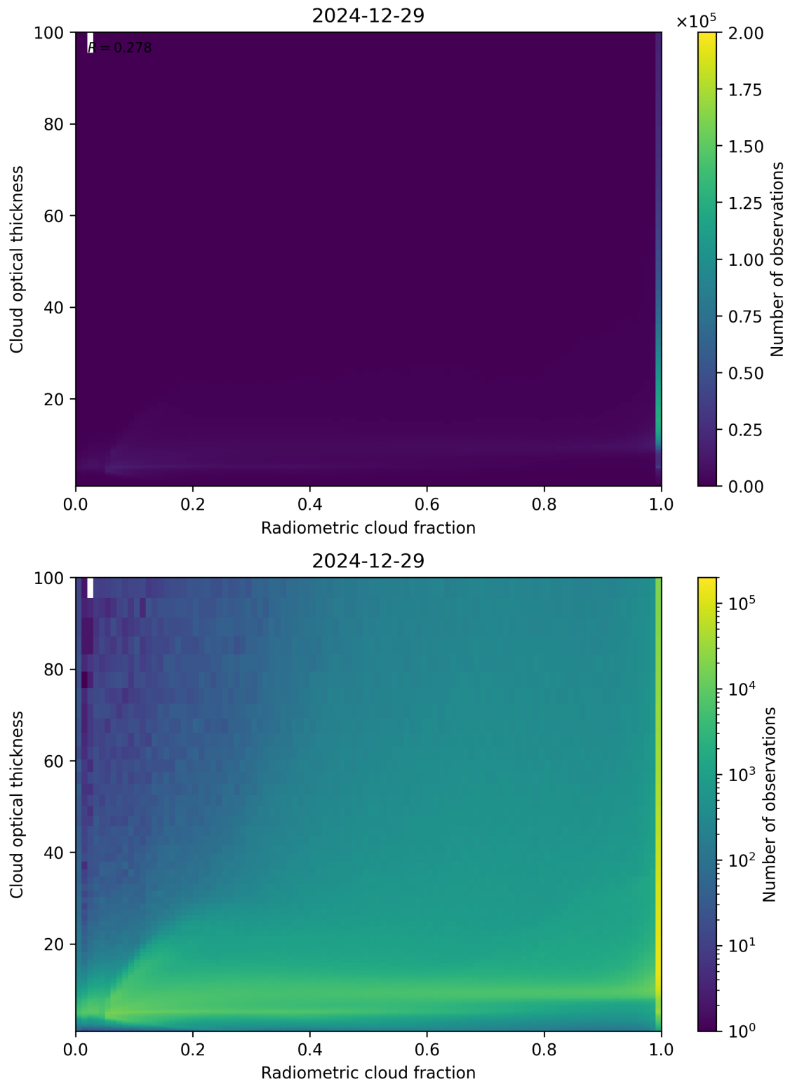
Figure 75: Scatter density plot of “Radiometric cloud fraction” against “Cloud optical thickness” for 2024-12-28 to 2024-12-30.
