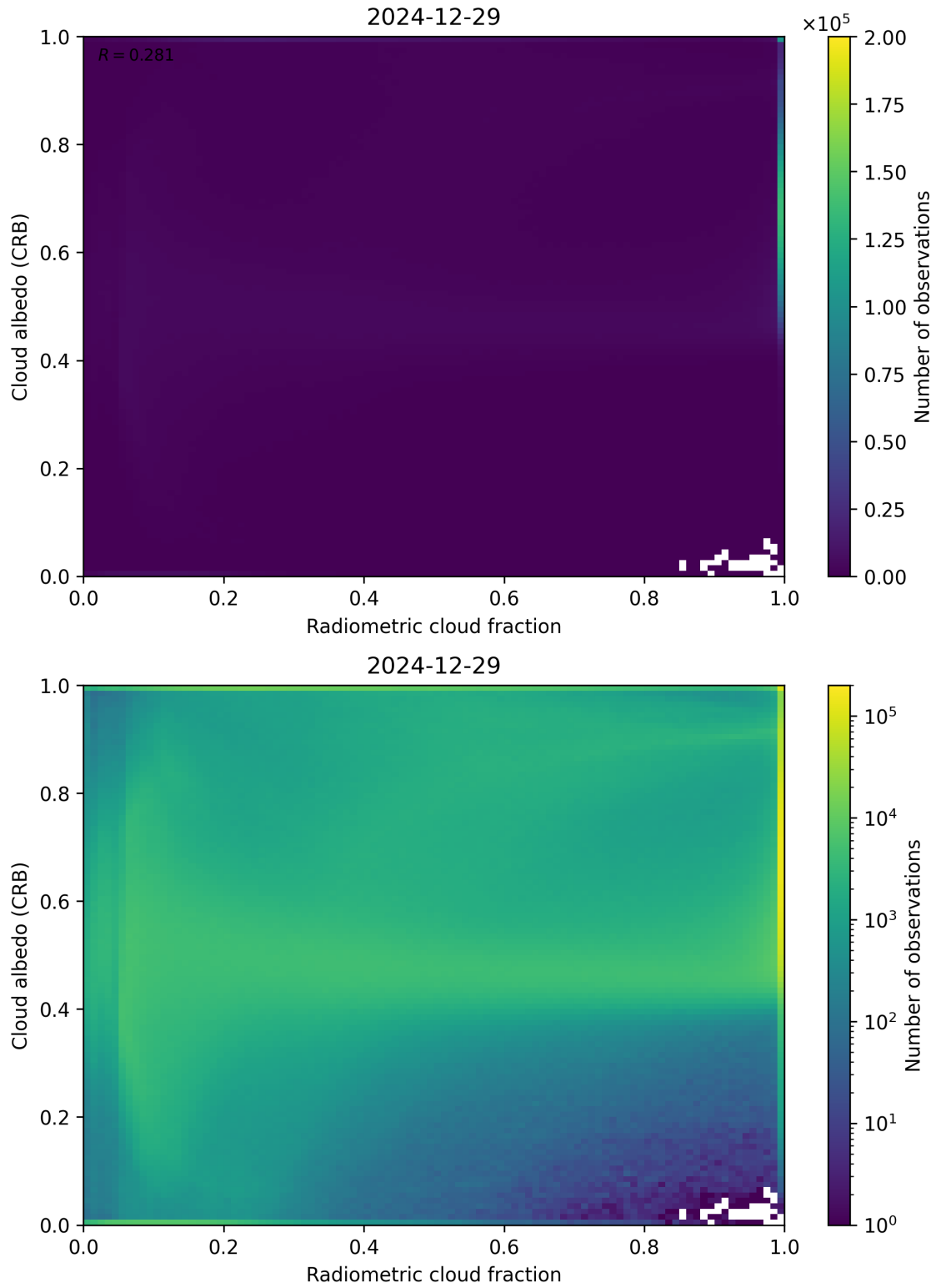
Figure 71: Scatter density plot of “Radiometric cloud fraction” against “Cloud albedo (CRB)” for 2024-12-28 to 2024-12-30.
