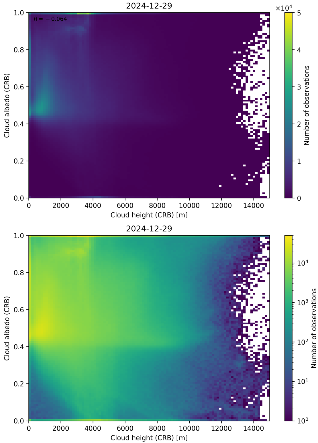
Figure 80: Scatter density plot of “Cloud height (CRB)” against “Cloud albedo (CRB)” for 2024-12-28 to 2024-12-30.
