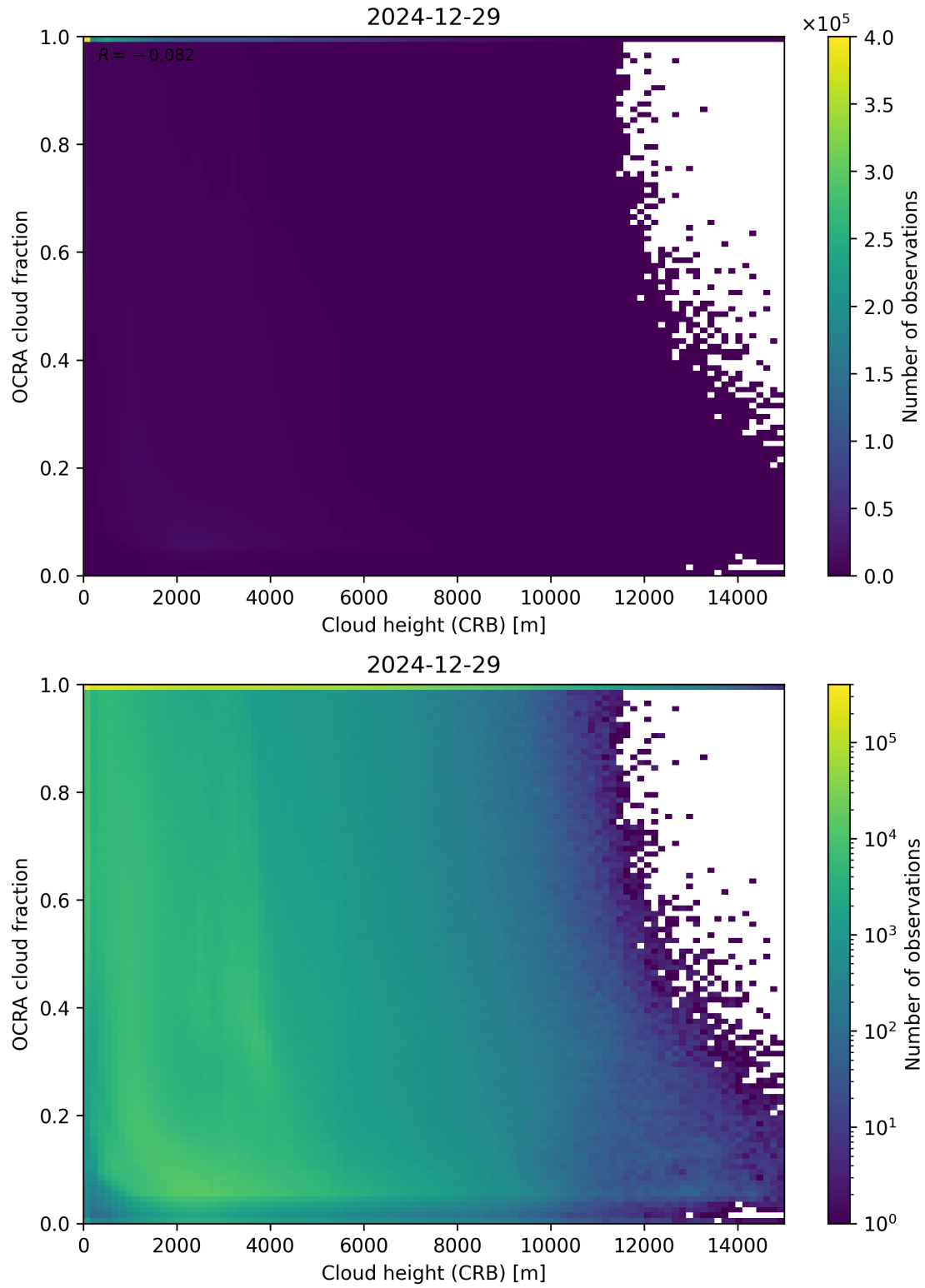
Figure 81: Scatter density plot of “Cloud height (CRB)” against “OCRA cloud fraction” for 2024-12-28 to 2024-12-30.
