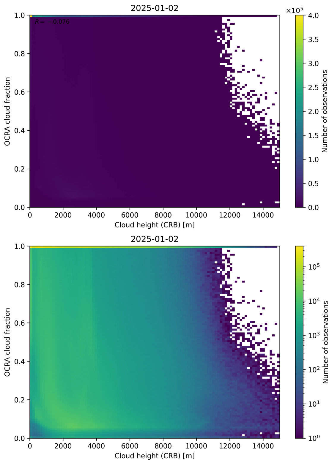
Figure 81: Scatter density plot of “Cloud height (CRB)” against “OCRA cloud fraction” for 2025-01-01 to 2025-01-03.
