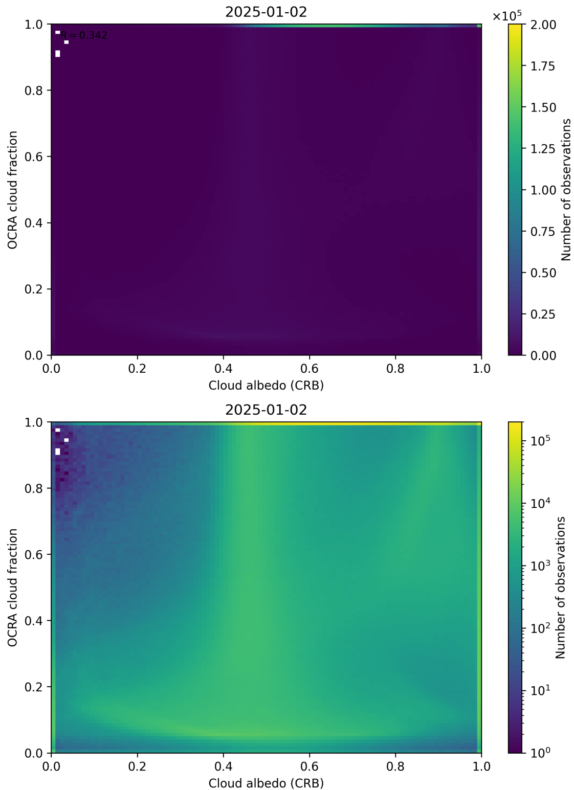
Figure 70: Scatter density plot of “Cloud albedo (CRB)” against “OCRA cloud fraction” for 2025-01-01 to 2025-01-03.
