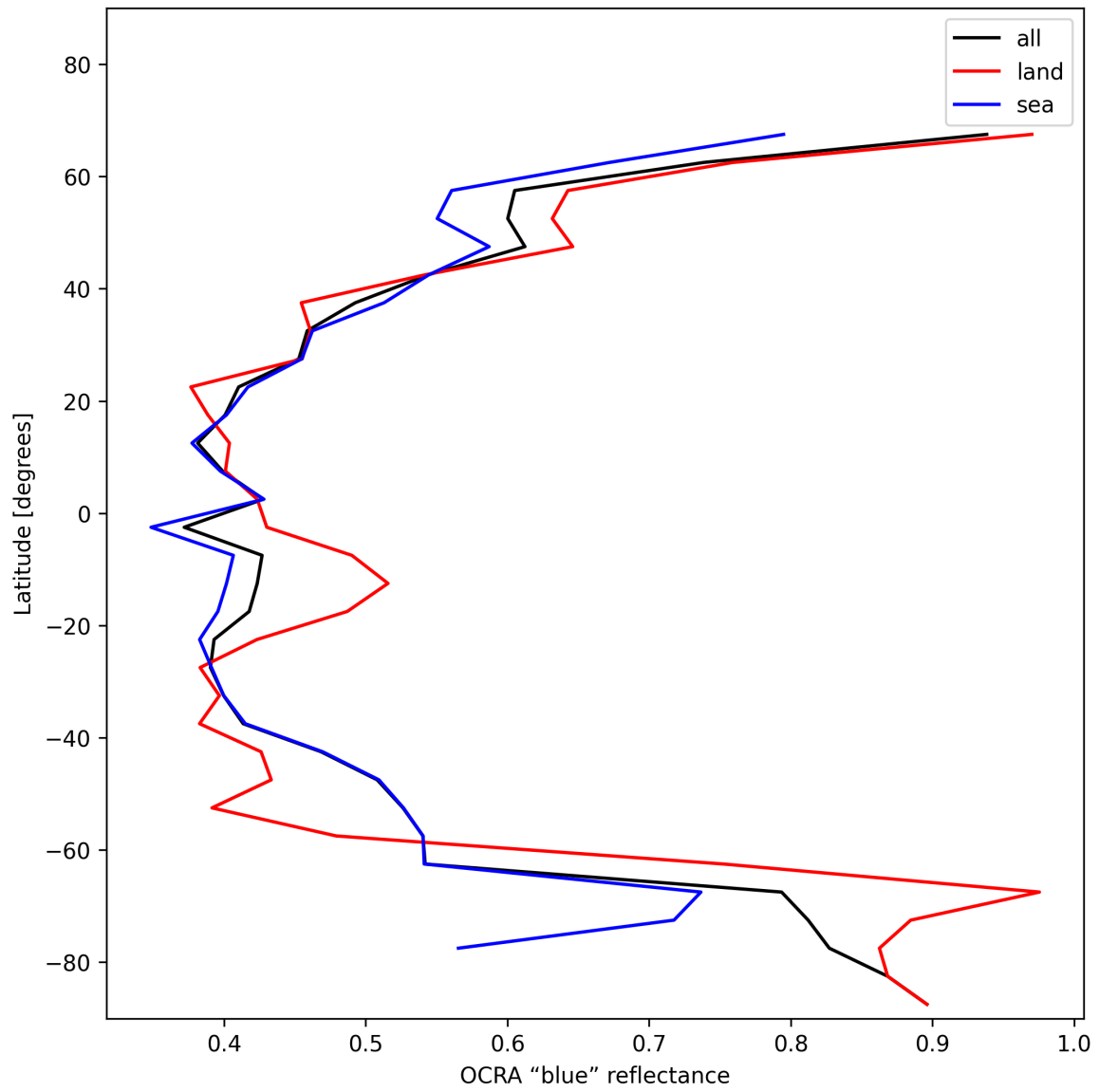
Figure 35: Zonal average of “OCRA “blue” reflectance” for 2025-01-01 to 2025-01-03.
