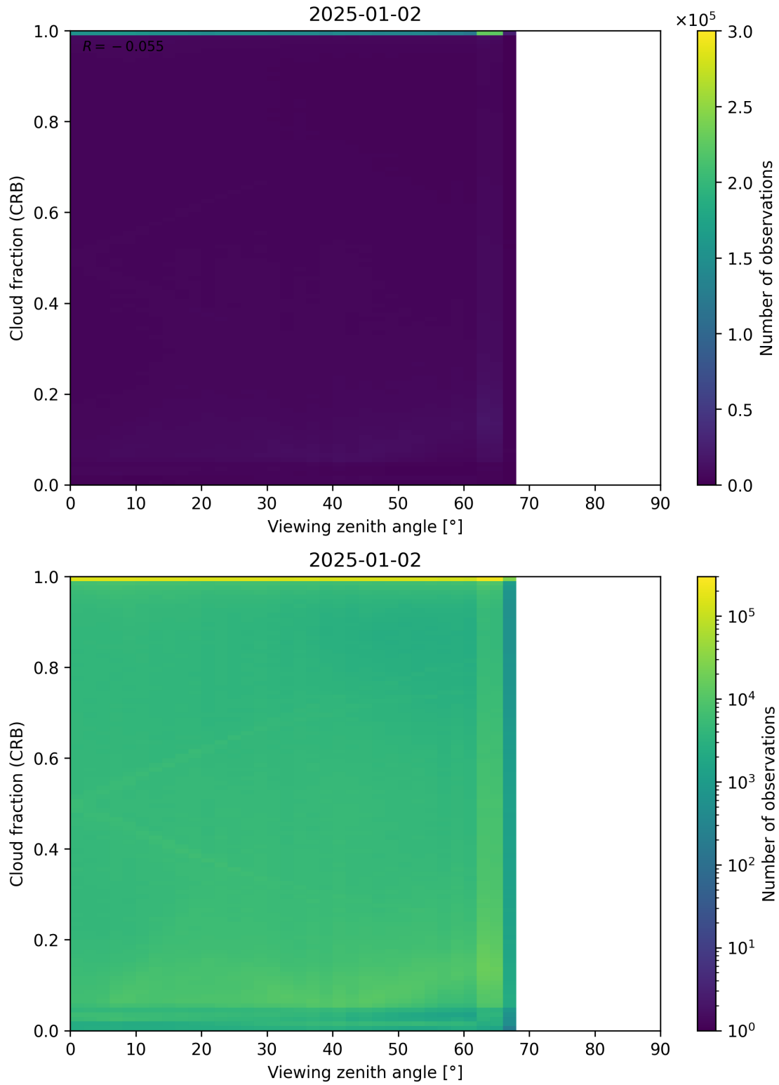
Figure 109: Scatter density plot of “Viewing zenith angle” against “Cloud fraction (CRB)” for 2025-01-01 to 2025-01-03.
