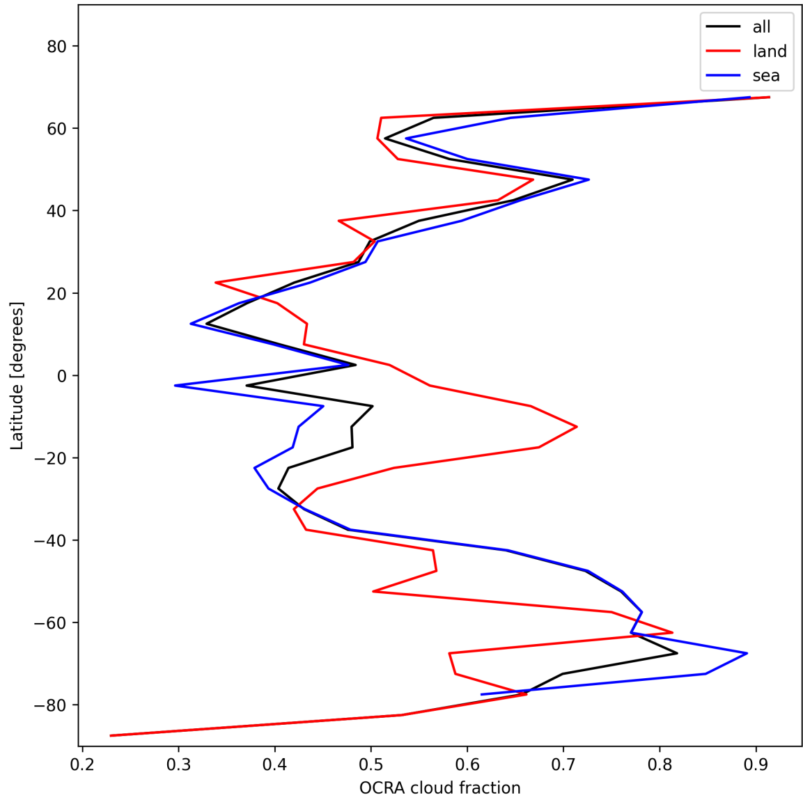
Figure 34: Zonal average of “OCRA cloud fraction” for 2025-01-01 to 2025-01-03.
