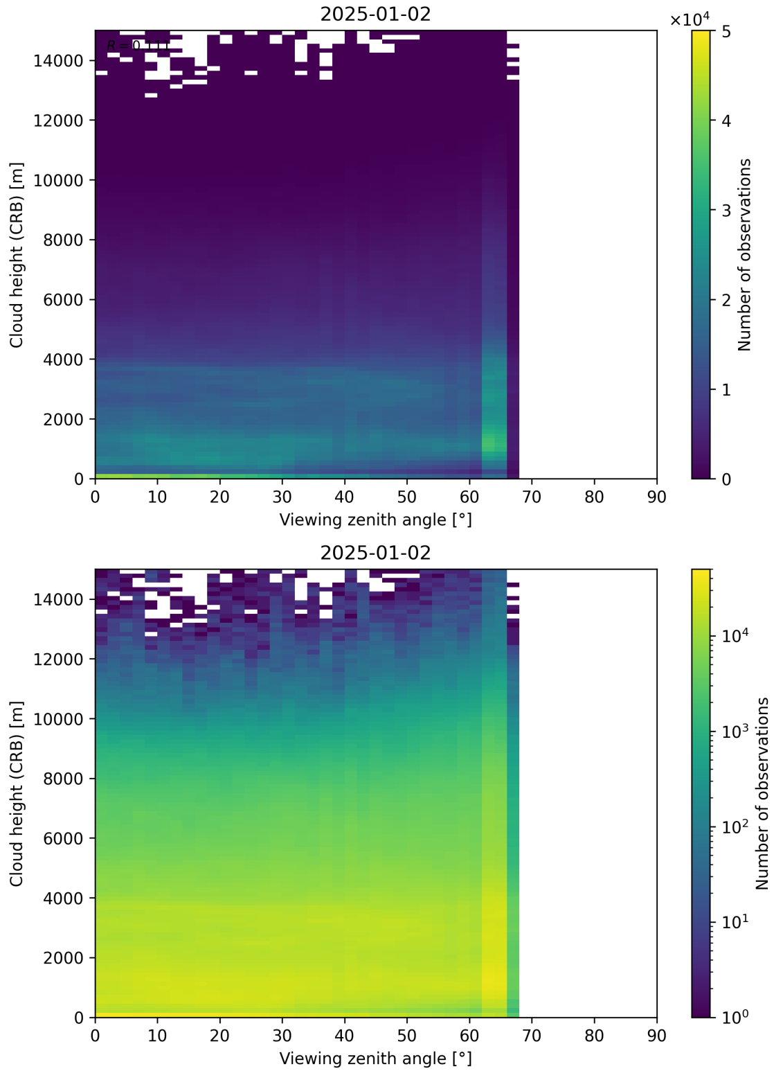
Figure 110: Scatter density plot of “Viewing zenith angle” against “Cloud height (CRB)” for 2025-01-01 to 2025-01-03.
