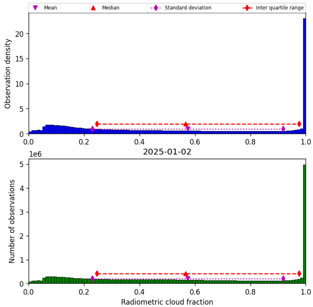
Figure 39: Histogram of "Radiometric cloud fraction" for 2025-01-01 to 2025-01-03
