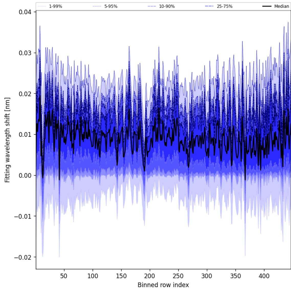
Figure 65: Along track statistics of “Fitting wavelength shift” for 2025-01-01 to 2025-01-03
