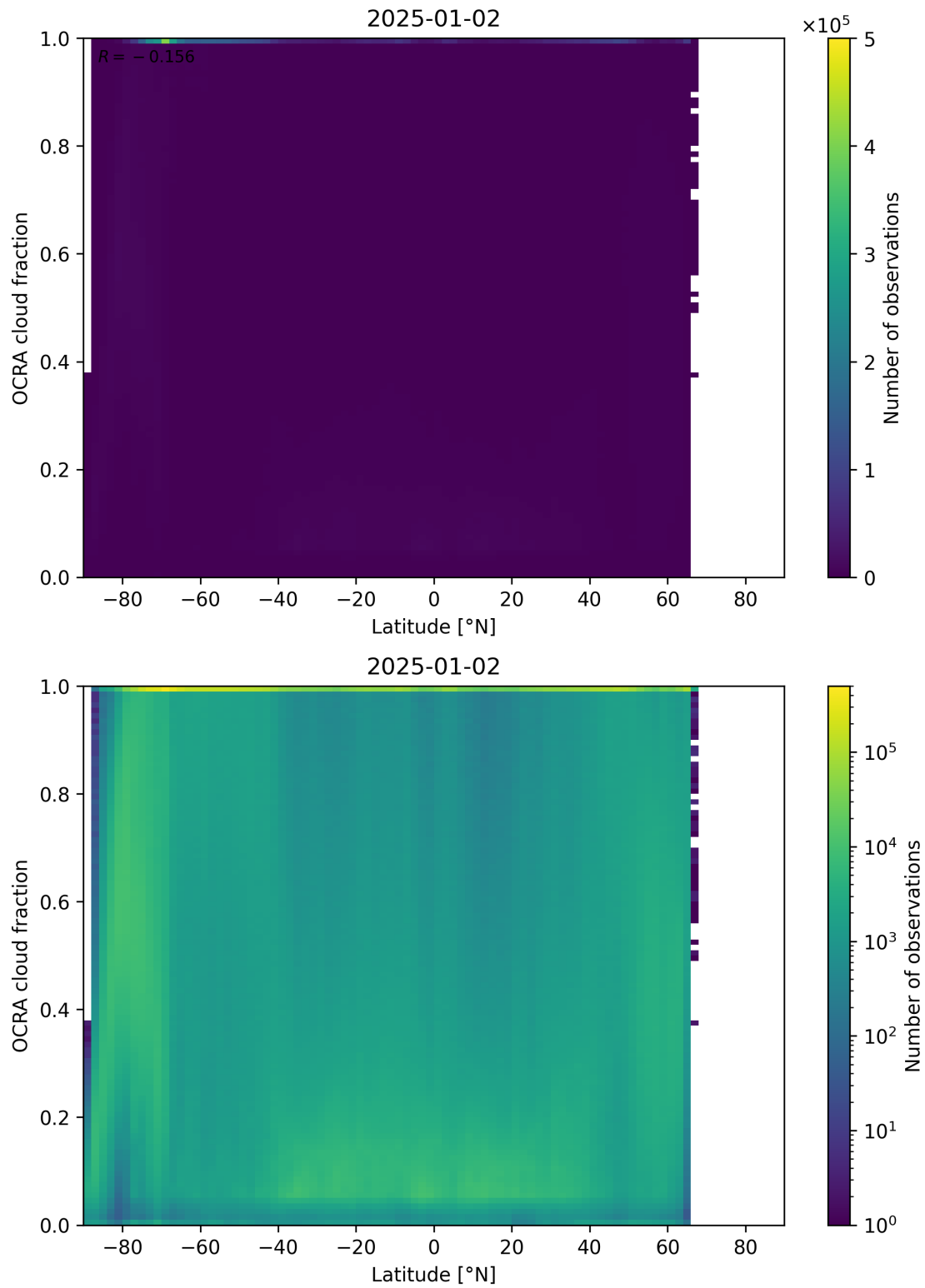
Figure 93: Scatter density plot of “Latitude” against “OCRA cloud fraction” for 2025-01-01 to 2025-01-03.
