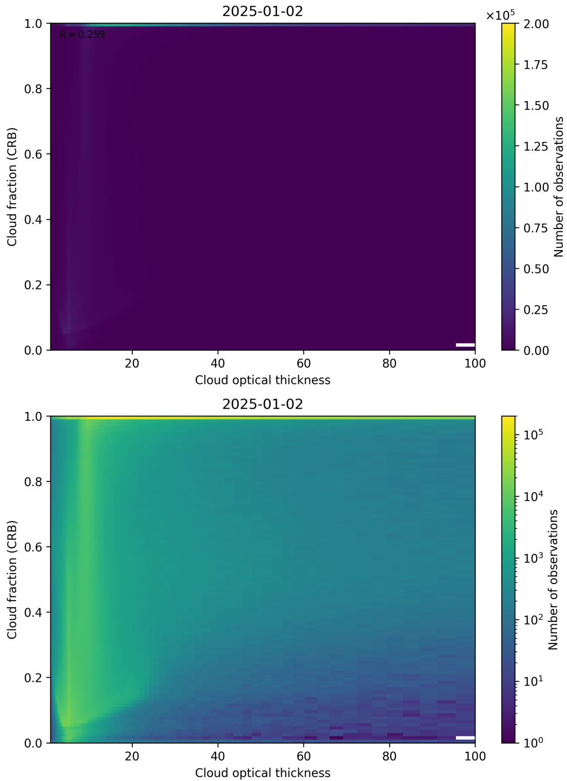
Figure 84: Scatter density plot of “Cloud optical thickness” against “Cloud fraction (CRB)” for 2025-01-01 to 2025-01-03.
