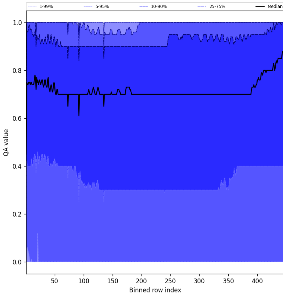
Figure 54: Along track statistics of “QA value” for 2025-01-01 to 2025-01-03
