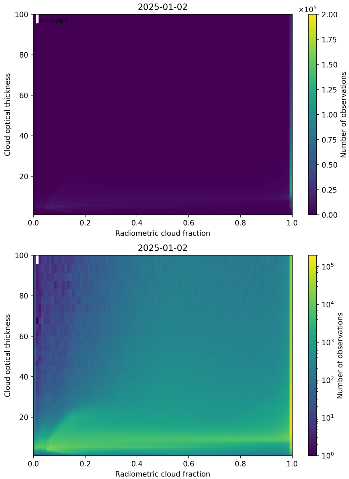
Figure 75: Scatter density plot of “Radiometric cloud fraction” against “Cloud optical thickness” for 2025-01-01 to 2025-01-03.
