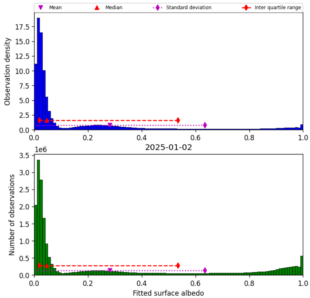
Figure 45: Histogram of “Fitted surface albedo” for 2025-01-01 to 2025-01-03
