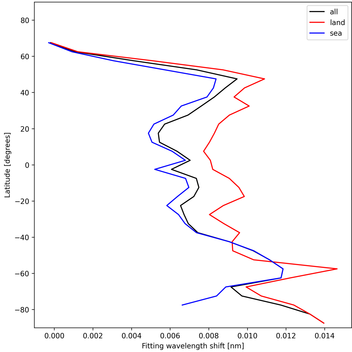
Figure 33: Zonal average of “Fitting wavelength shift” for 2025-01-01 to 2025-01-03.
