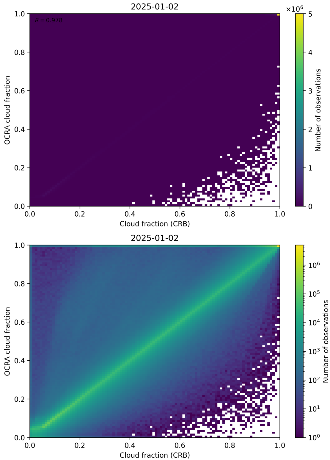
Figure 78: Scatter density plot of “Cloud fraction (CRB)” against “OCRA cloud fraction” for 2025-01-01 to 2025-01-03.
