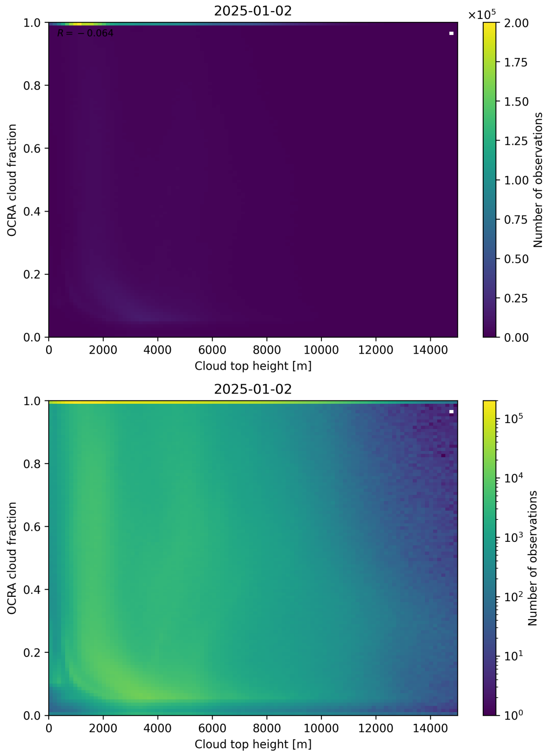
Figure 87: Scatter density plot of “Cloud top height” against “OCRA cloud fraction” for 2025-01-01 to 2025-01-03.
