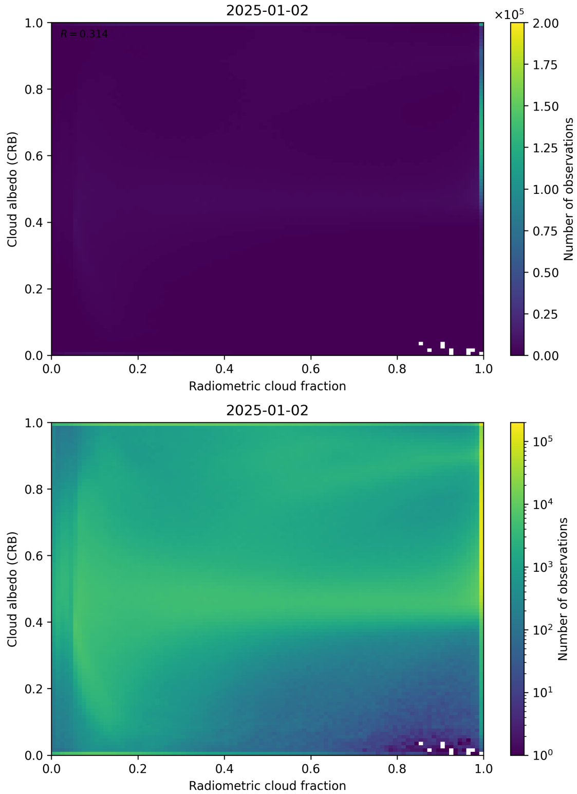
Figure 71: Scatter density plot of “Radiometric cloud fraction” against “Cloud albedo (CRB)” for 2025-01-01 to 2025-01-03.
