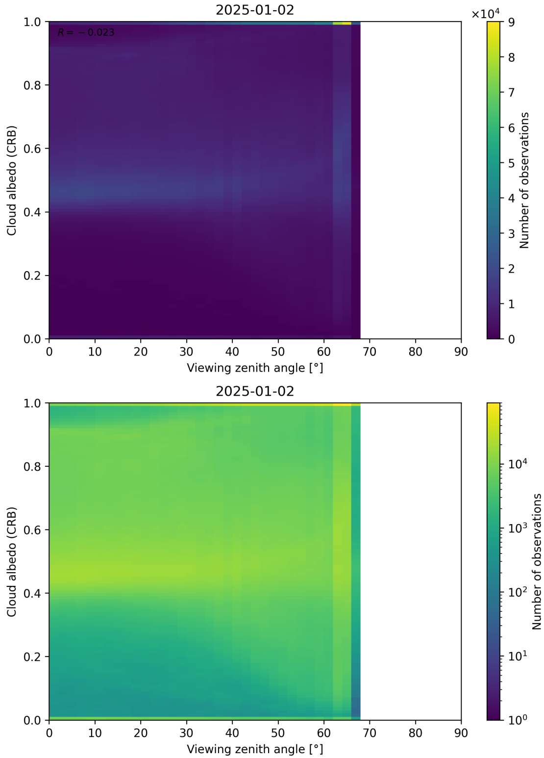
Figure 106: Scatter density plot of “Viewing zenith angle” against “Cloud albedo (CRB)” for 2025-01-01 to 2025-01-03.
