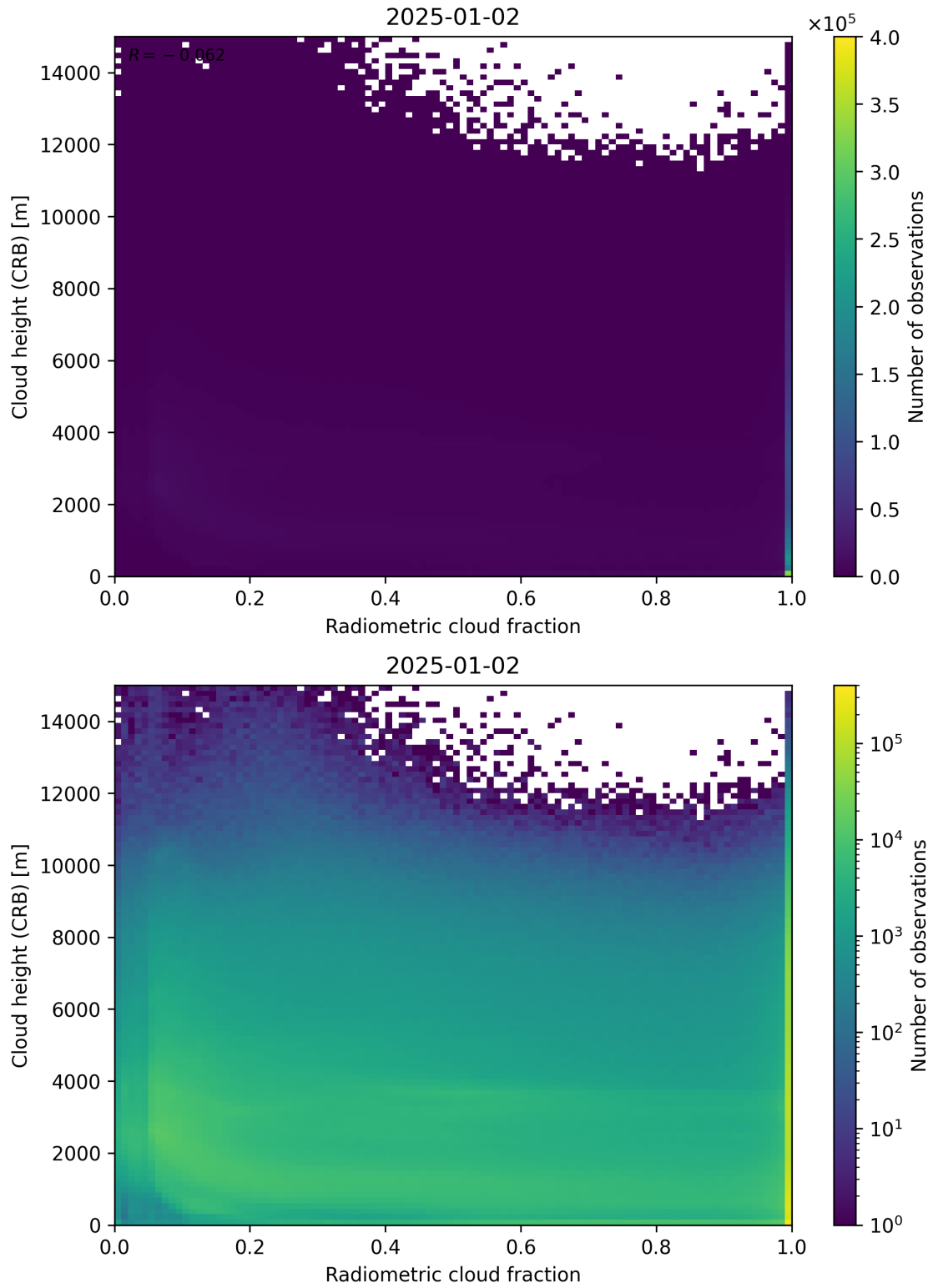
Figure 74: Scatter density plot of “Radiometric cloud fraction” against “Cloud height (CRB)” for 2025-01-01 to 2025-01-03.
