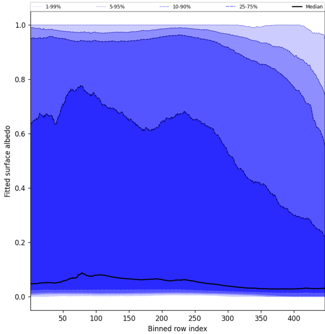
Figure 61: Along track statistics of “Fitted surface albedo” for 2025-01-01 to 2025-01-03
