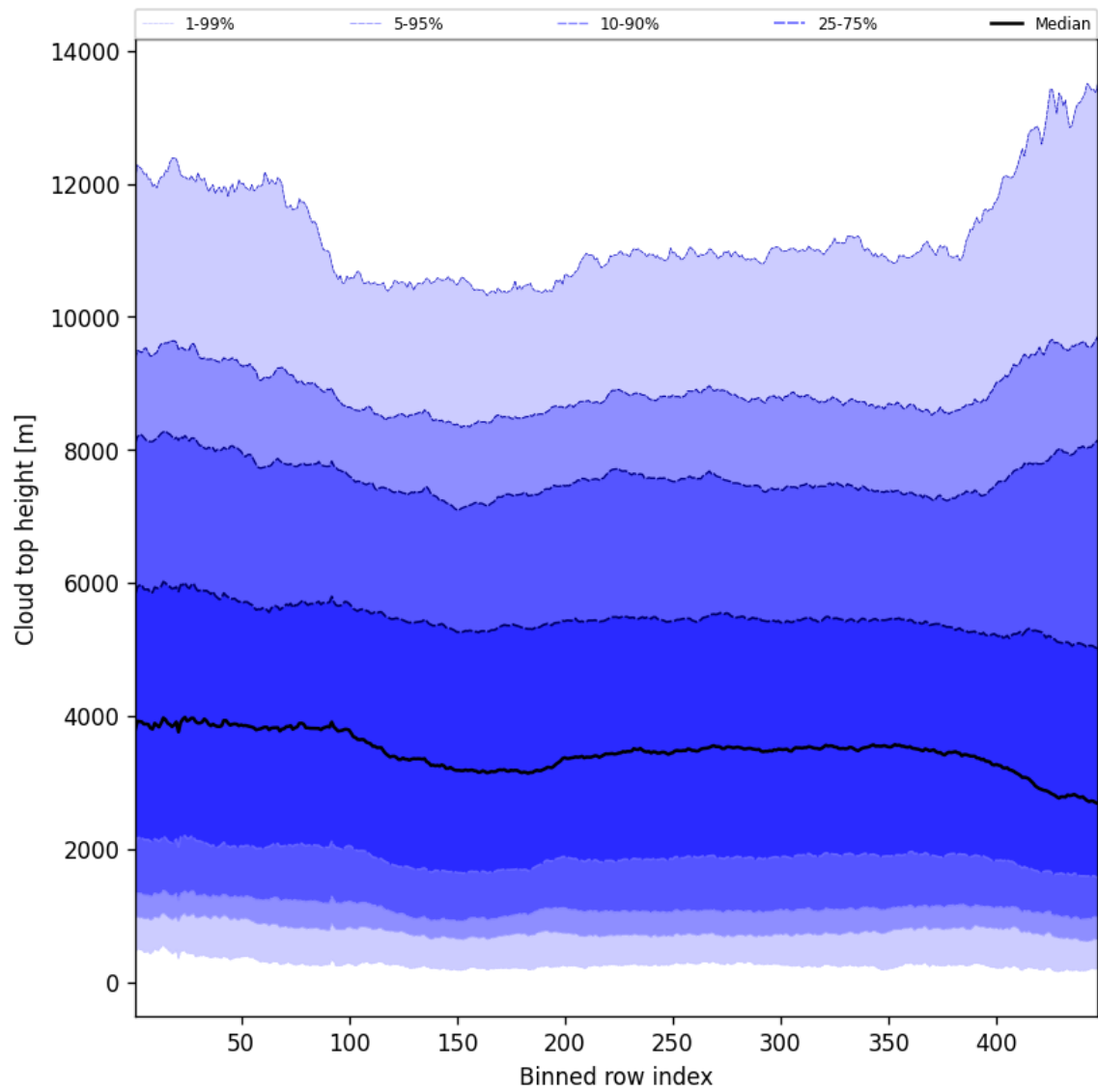
Figure 56: Along track statistics of “Cloud top height” for 2025-01-01 to 2025-01-03
