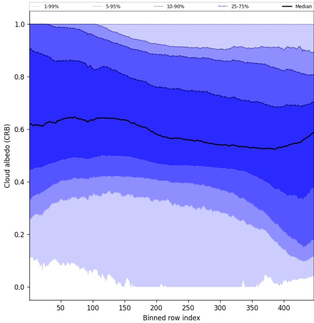
Figure 60: Along track statistics of “Cloud albedo (CRB)” for 2025-01-01 to 2025-01-03
