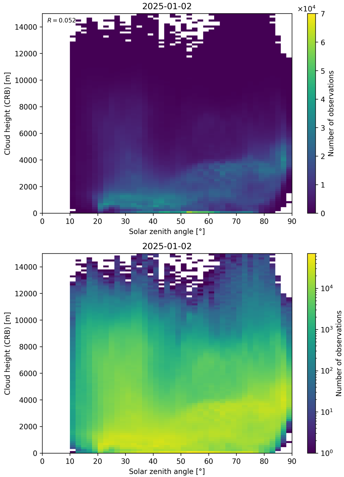
Figure 102: Scatter density plot of “Solar zenith angle” against “Cloud height (CRB)” for 2025-01-01 to 2025-01-03.
