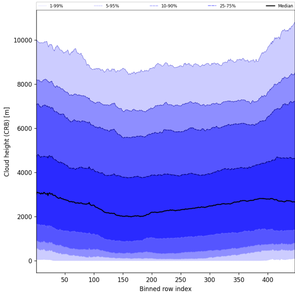
Figure 59: Along track statistics of “Cloud height (CRB)” for 2025-01-01 to 2025-01-03
