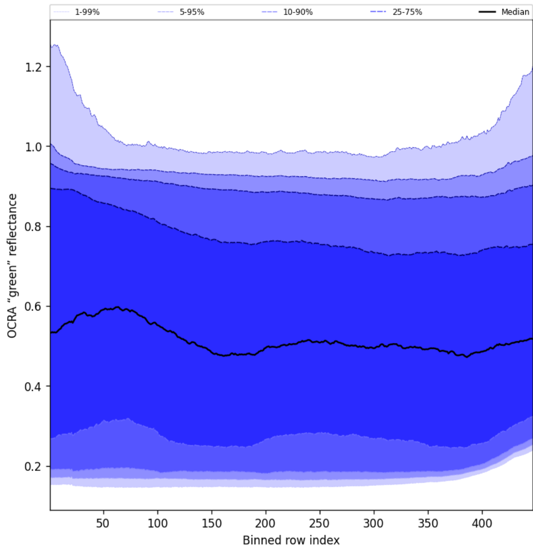
Figure 68: Along track statistics of "OCRA "green" reflectance" for 2025-01-01 to 2025-01-03
