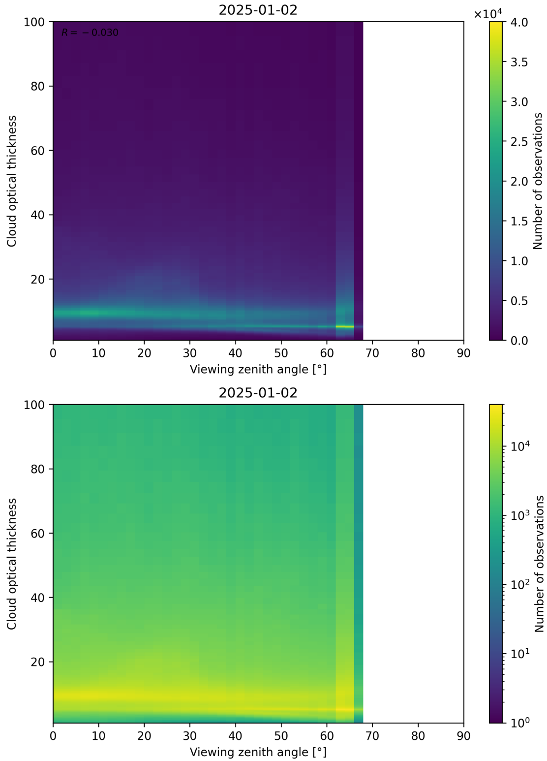
Figure 111: Scatter density plot of “Viewing zenith angle” against “Cloud optical thickness” for 2025-01-01 to 2025-01-03.
