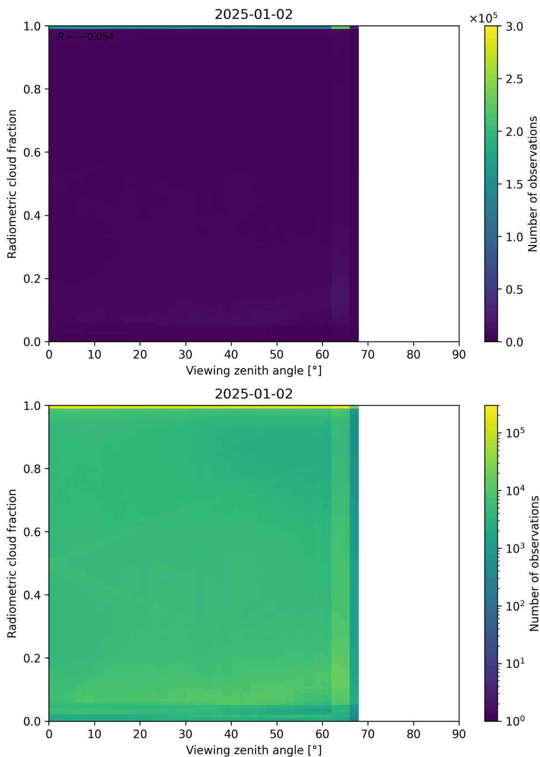
Figure 107: Scatter density plot of “Viewing zenith angle” against “Radiometric cloud fraction” for 2025-01-01 to 2025-01-03.
