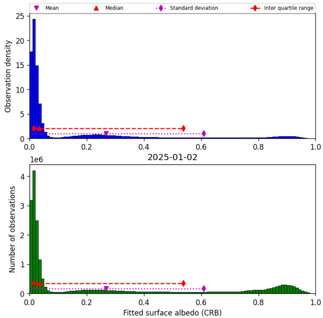
Figure 46: Histogram of “Fitted surface albedo (CRB)” for 2025-01-01 to 2025-01-03
