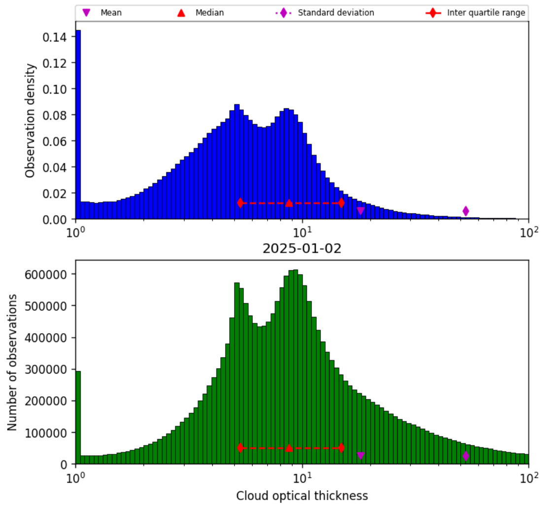
Figure 41: Histogram of “Cloud optical thickness” for 2025-01-01 to 2025-01-03
