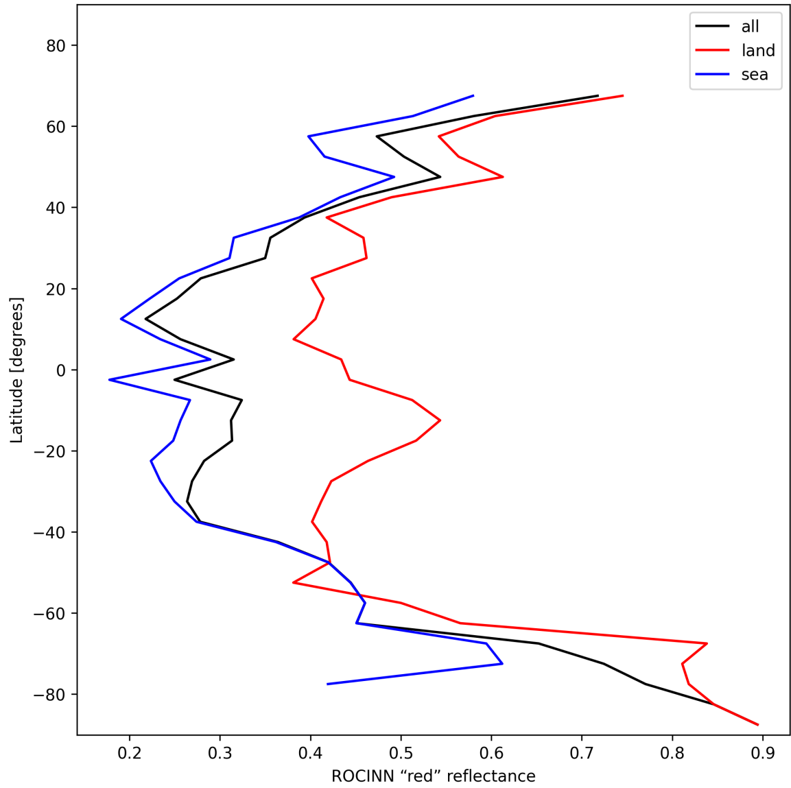
Figure 37: Zonal average of “ROCINN “red” reflectance” for 2025-01-01 to 2025-01-03.
