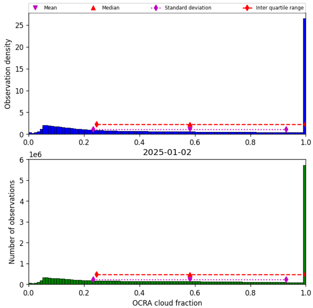
Figure 50: Histogram of “OCRA cloud fraction” for 2025-01-01 to 2025-01-03
