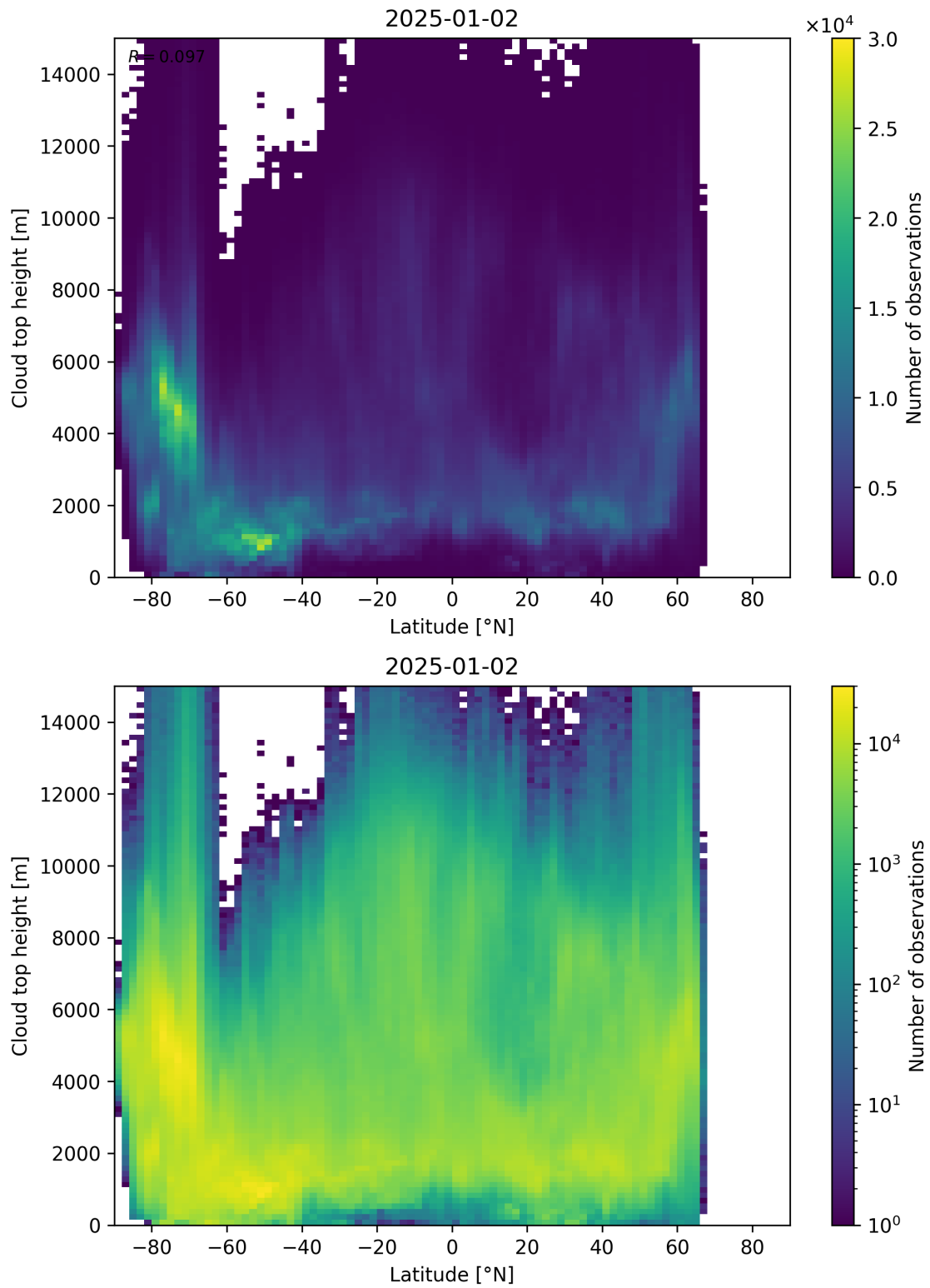
Figure 97: Scatter density plot of “Latitude” against “Cloud top height” for 2025-01-01 to 2025-01-03.
