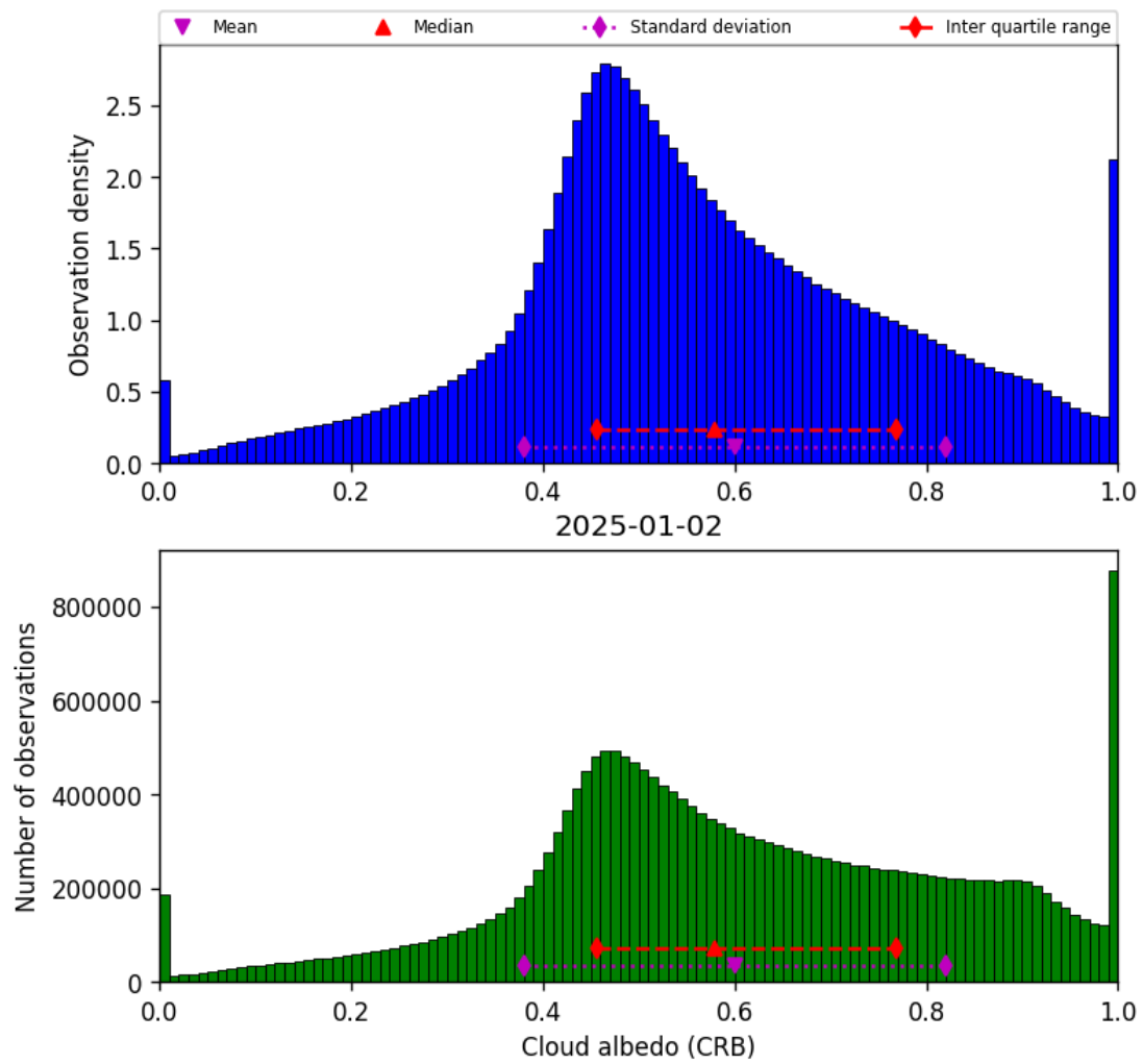
Figure 44: Histogram of “Cloud albedo (CRB)” for 2025-01-01 to 2025-01-03
