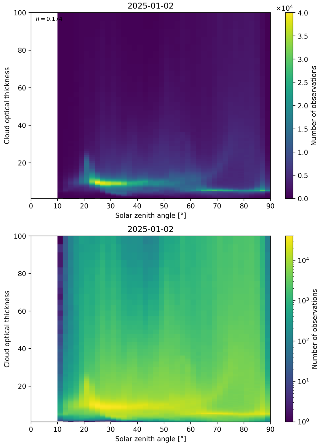
Figure 103: Scatter density plot of “Solar zenith angle” against “Cloud optical thickness” for 2025-01-01 to 2025-01-03.
