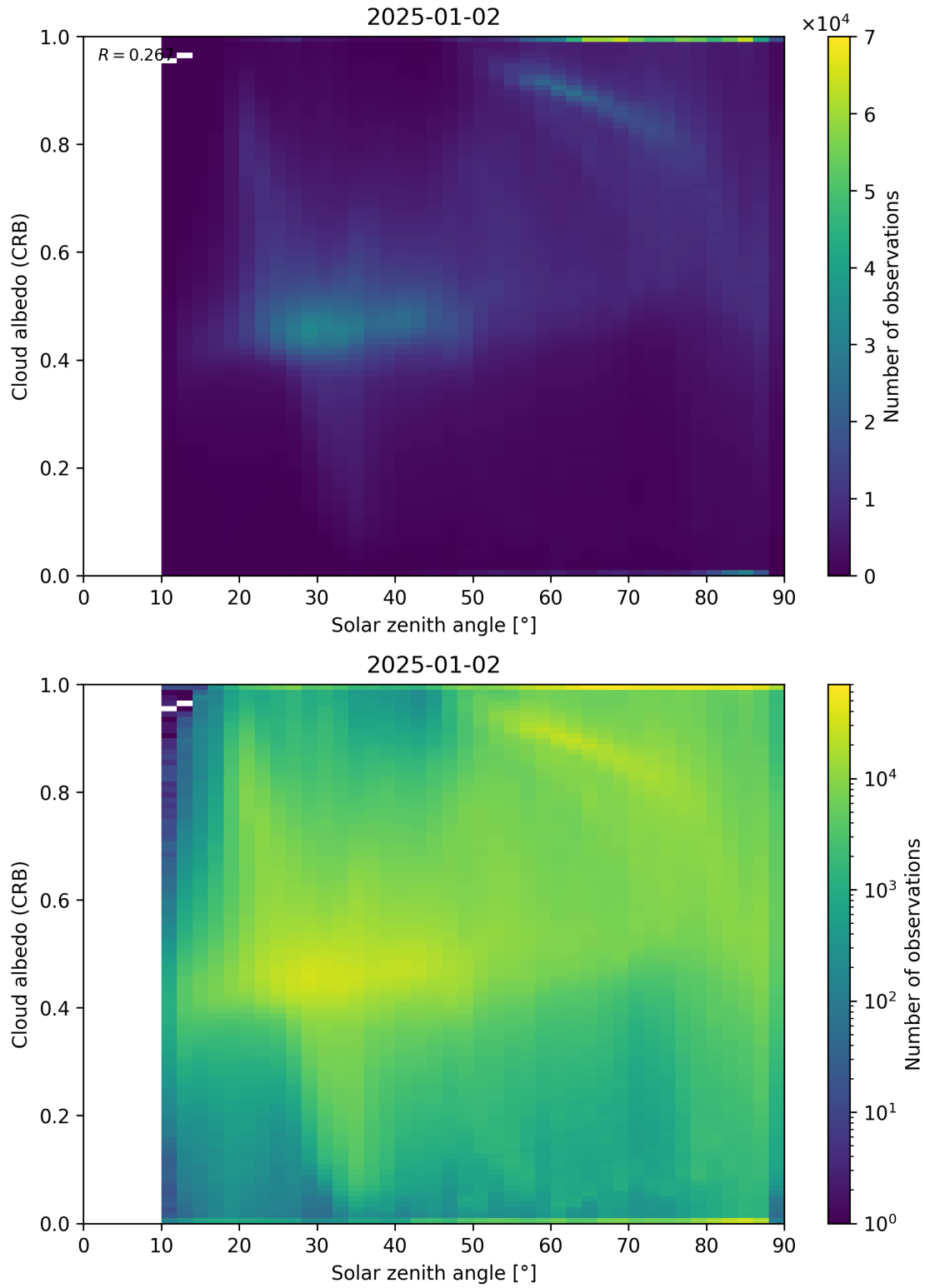
Figure 98: Scatter density plot of “Solar zenith angle” against “Cloud albedo (CRB)” for 2025-01-01 to 2025-01-03.
