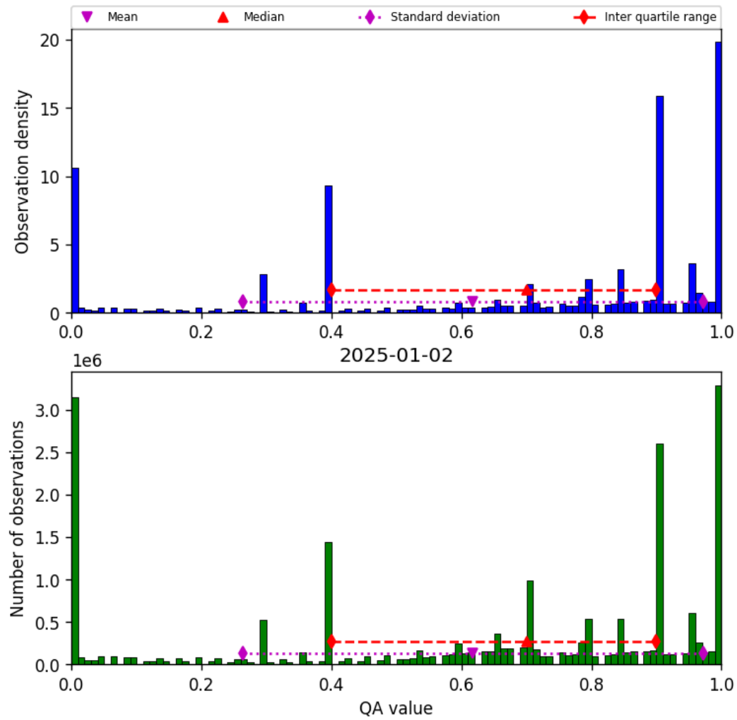
Figure 38: Histogram of “QA value” for 2025-01-01 to 2025-01-03
