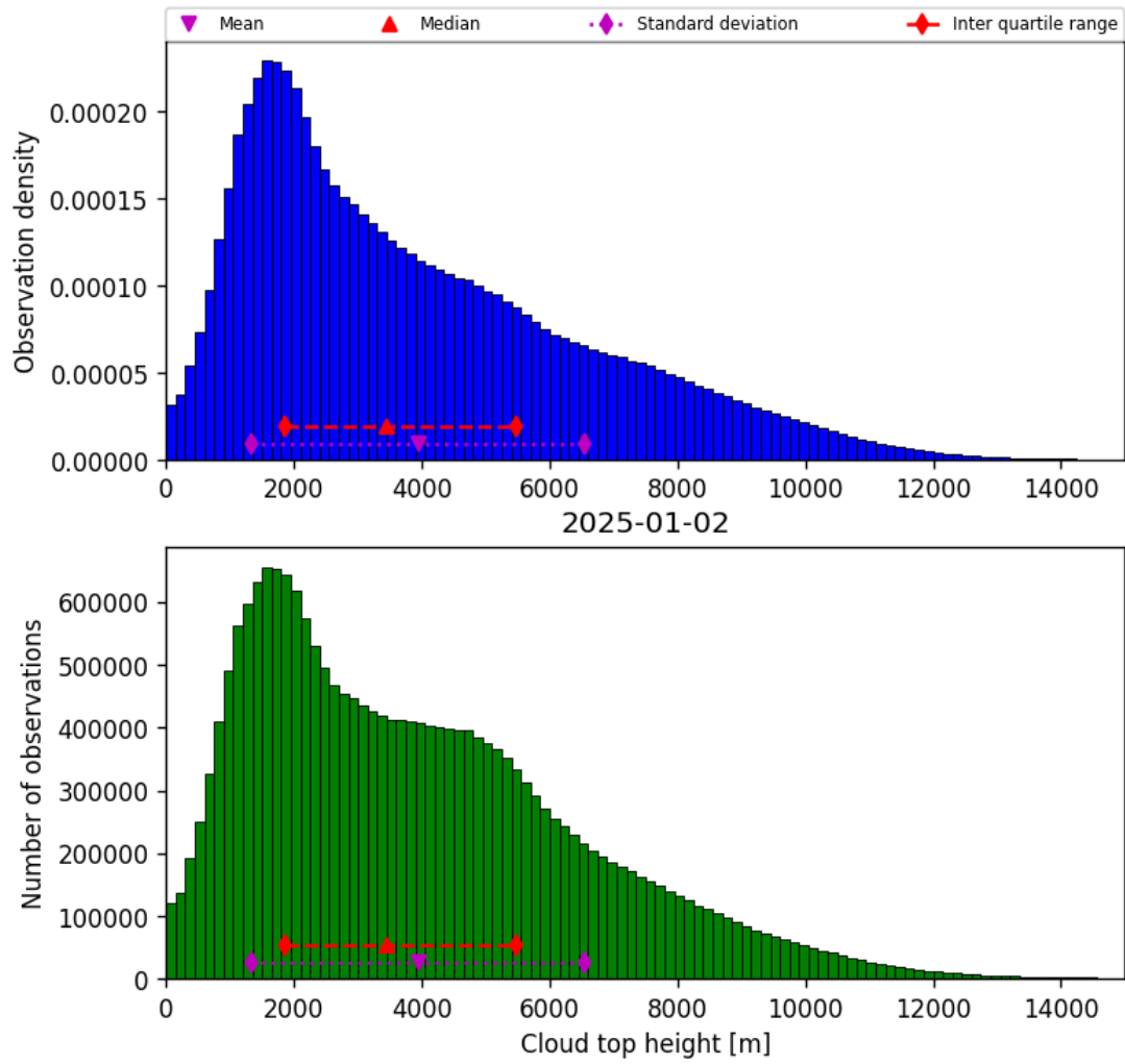
Figure 40: Histogram of “Cloud top height” for 2025-01-01 to 2025-01-03
