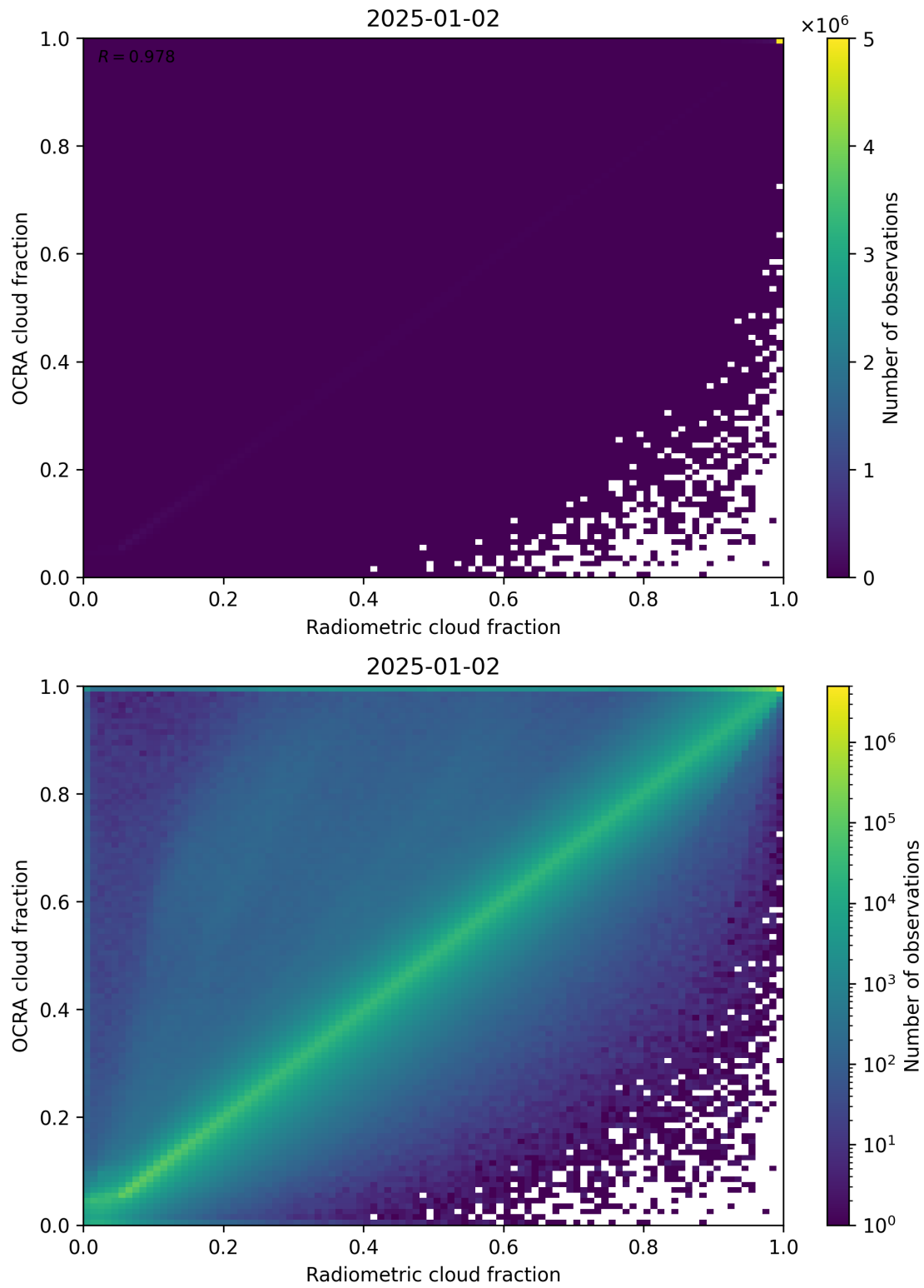
Figure 72: Scatter density plot of “Radiometric cloud fraction” against “OCRA cloud fraction” for 2025-01-01 to 2025-01-03.
