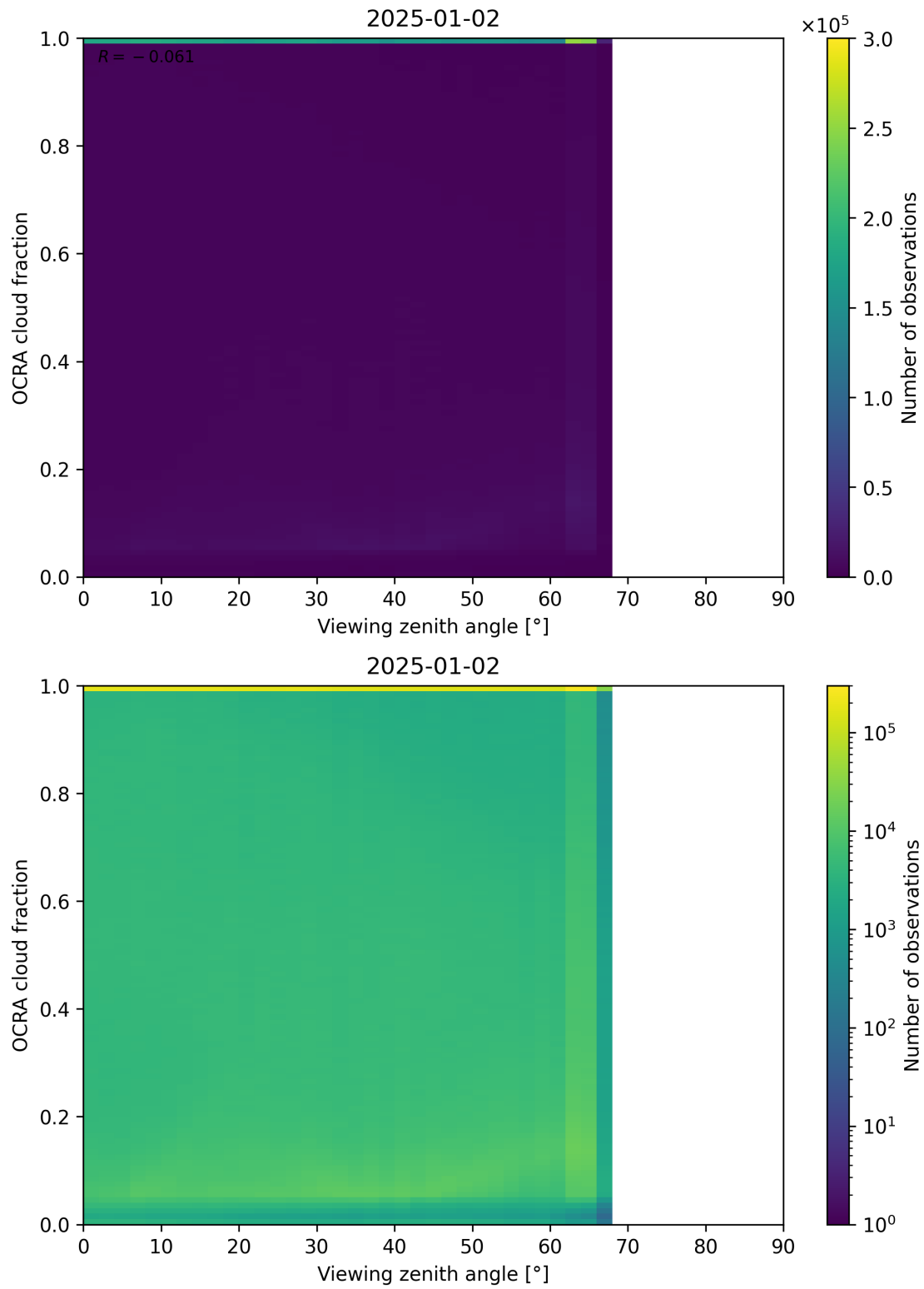
Figure 108: Scatter density plot of “Viewing zenith angle” against “OCRA cloud fraction” for 2025-01-01 to 2025-01-03.
