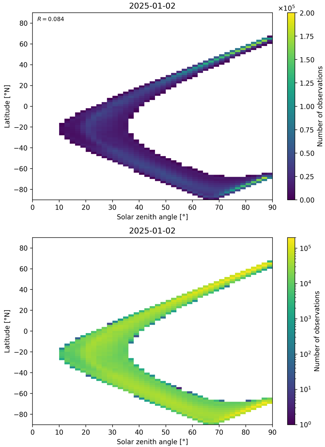
Figure 105: Scatter density plot of “Solar zenith angle” against “Latitude” for 2025-01-01 to 2025-01-03.
