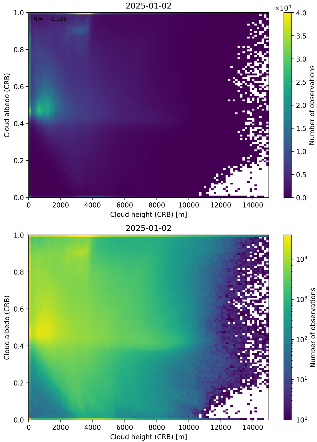
Figure 80: Scatter density plot of “Cloud height (CRB)” against “Cloud albedo (CRB)” for 2025-01-01 to 2025-01-03.
