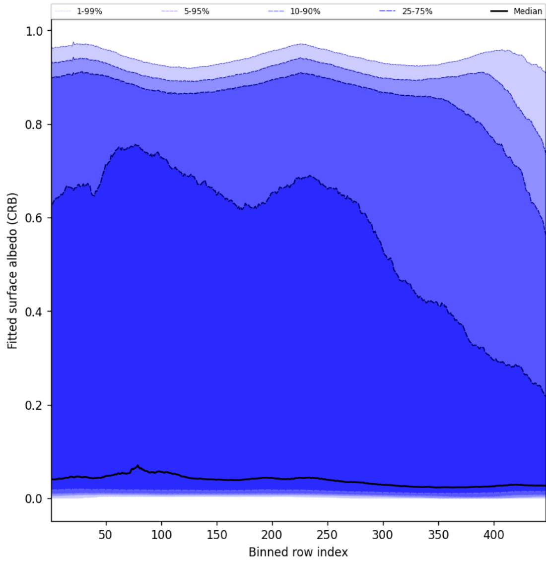
Figure 62: Along track statistics of “Fitted surface albedo (CRB)” for 2025-01-01 to 2025-01-03
