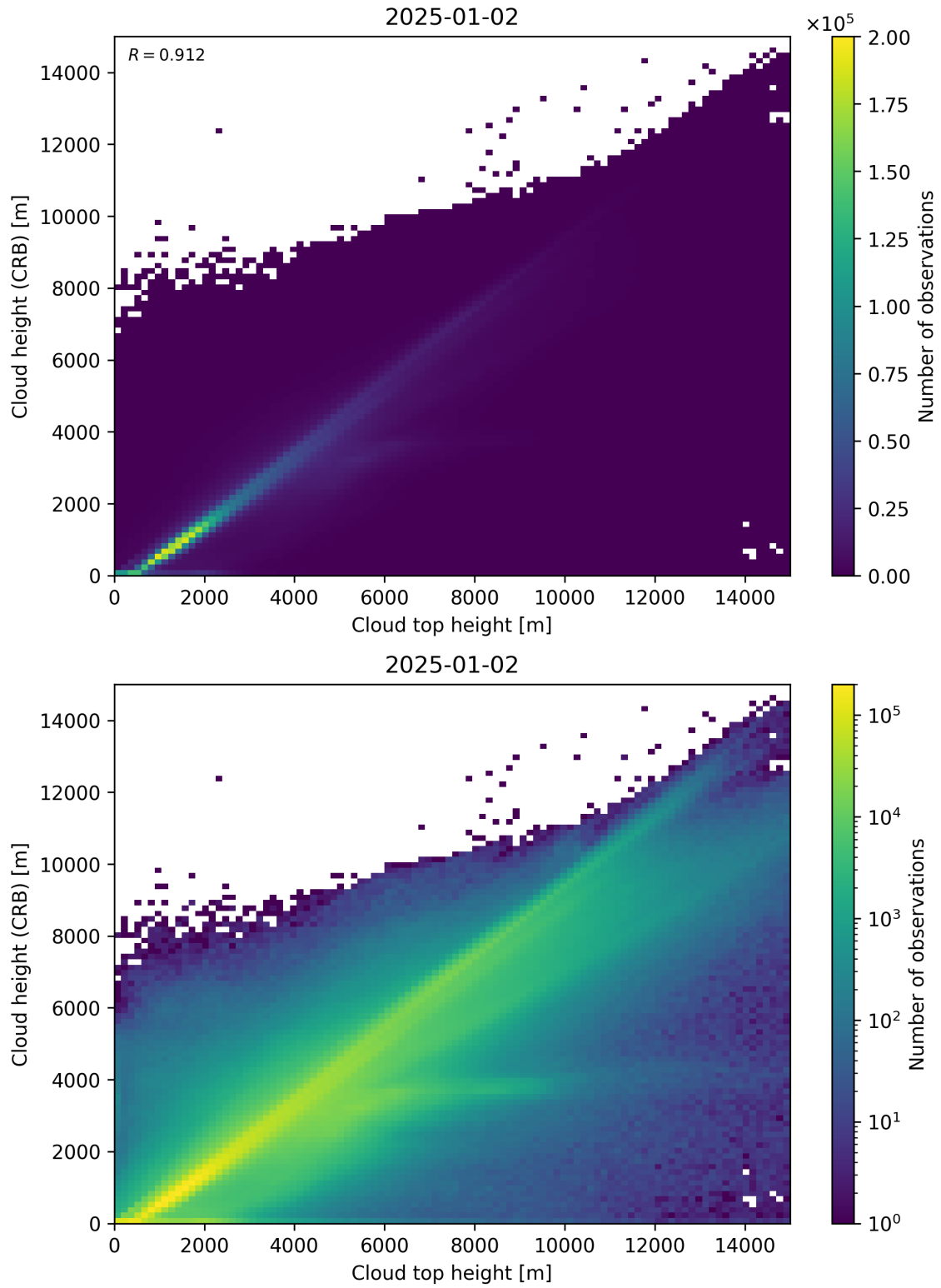
Figure 89: Scatter density plot of “Cloud top height” against “Cloud height (CRB)” for 2025-01-01 to 2025-01-03.
