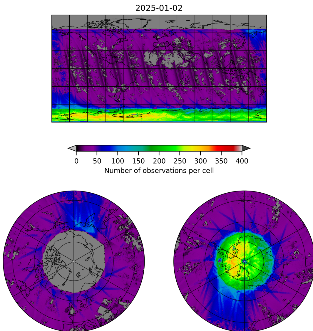
Figure 21: Map of the number of observations for 2025-01-01 to 2025-01-03
