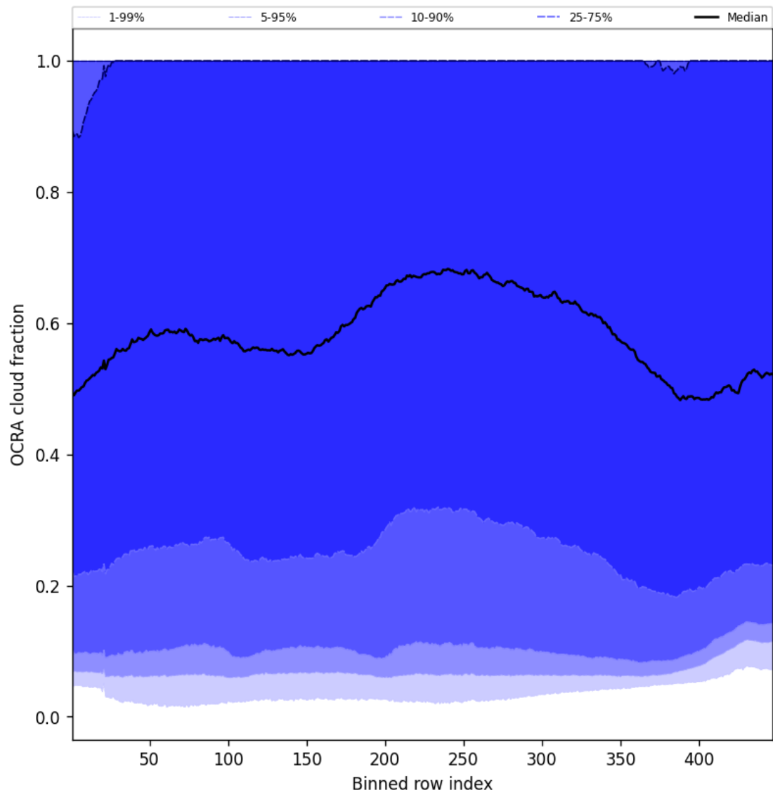
Figure 66: Along track statistics of “OCRA cloud fraction” for 2025-01-01 to 2025-01-03
