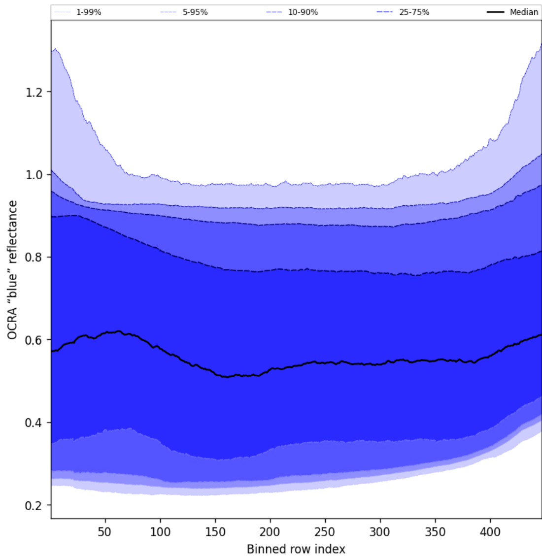
Figure 67: Along track statistics of “OCRA “blue” reflectance” for 2025-01-01 to 2025-01-03
