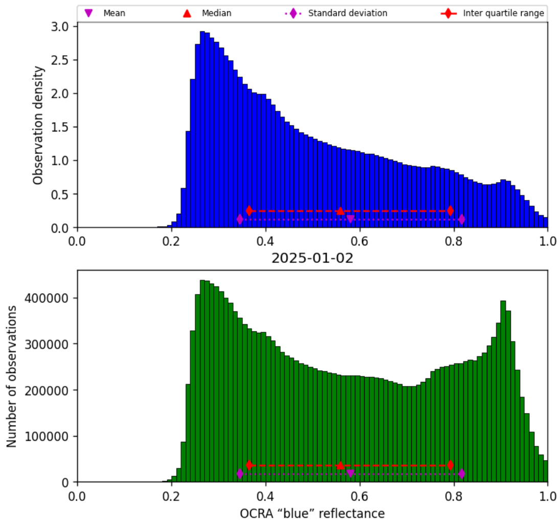
Figure 51: Histogram of “OCRA “blue” reflectance” for 2025-01-01 to 2025-01-03
