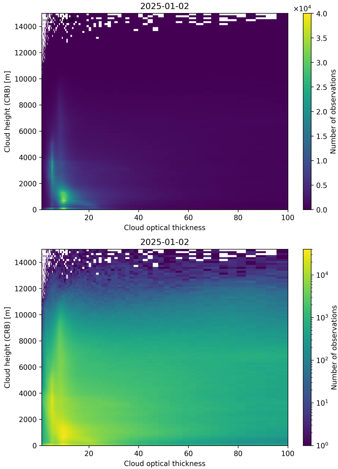
Figure 85: Scatter density plot of “Cloud optical thickness” against “Cloud height (CRB)” for 2025-01-01 to 2025-01-03.
