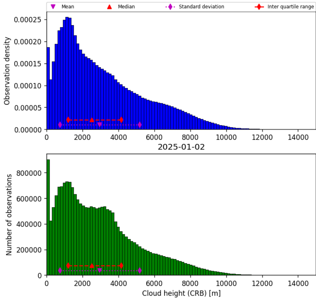
Figure 43: Histogram of “Cloud height (CRB)” for 2025-01-01 to 2025-01-03
