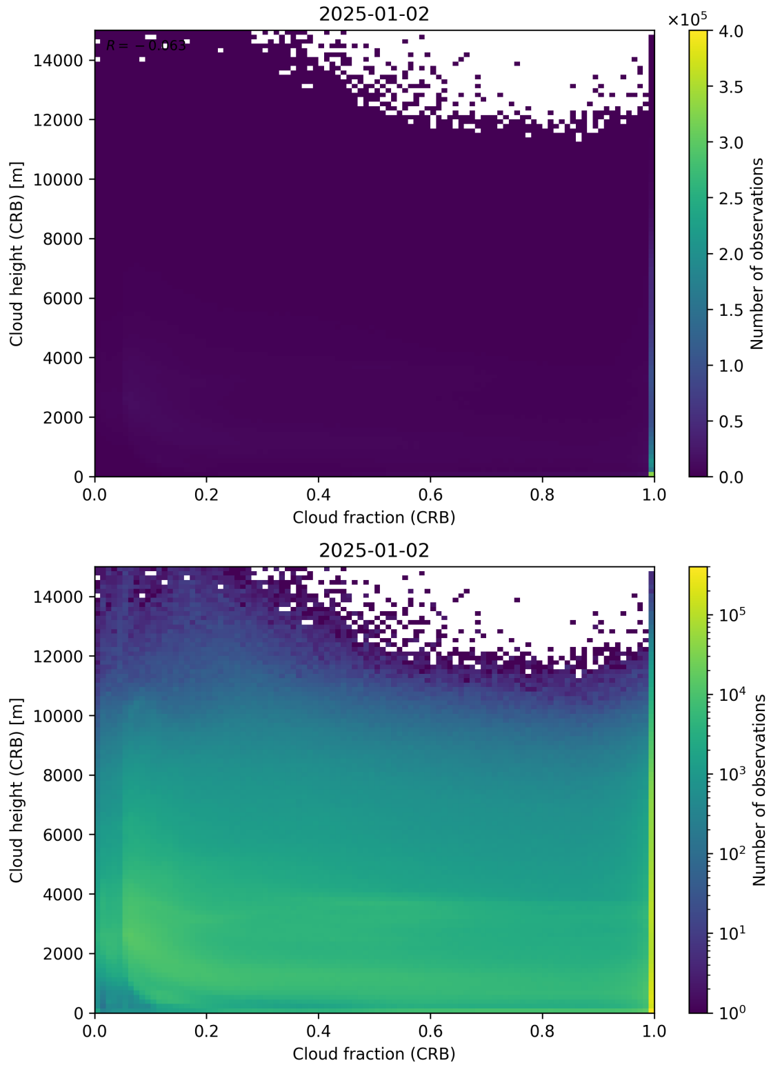
Figure 79: Scatter density plot of “Cloud fraction (CRB)” against “Cloud height (CRB)” for 2025-01-01 to 2025-01-03.
