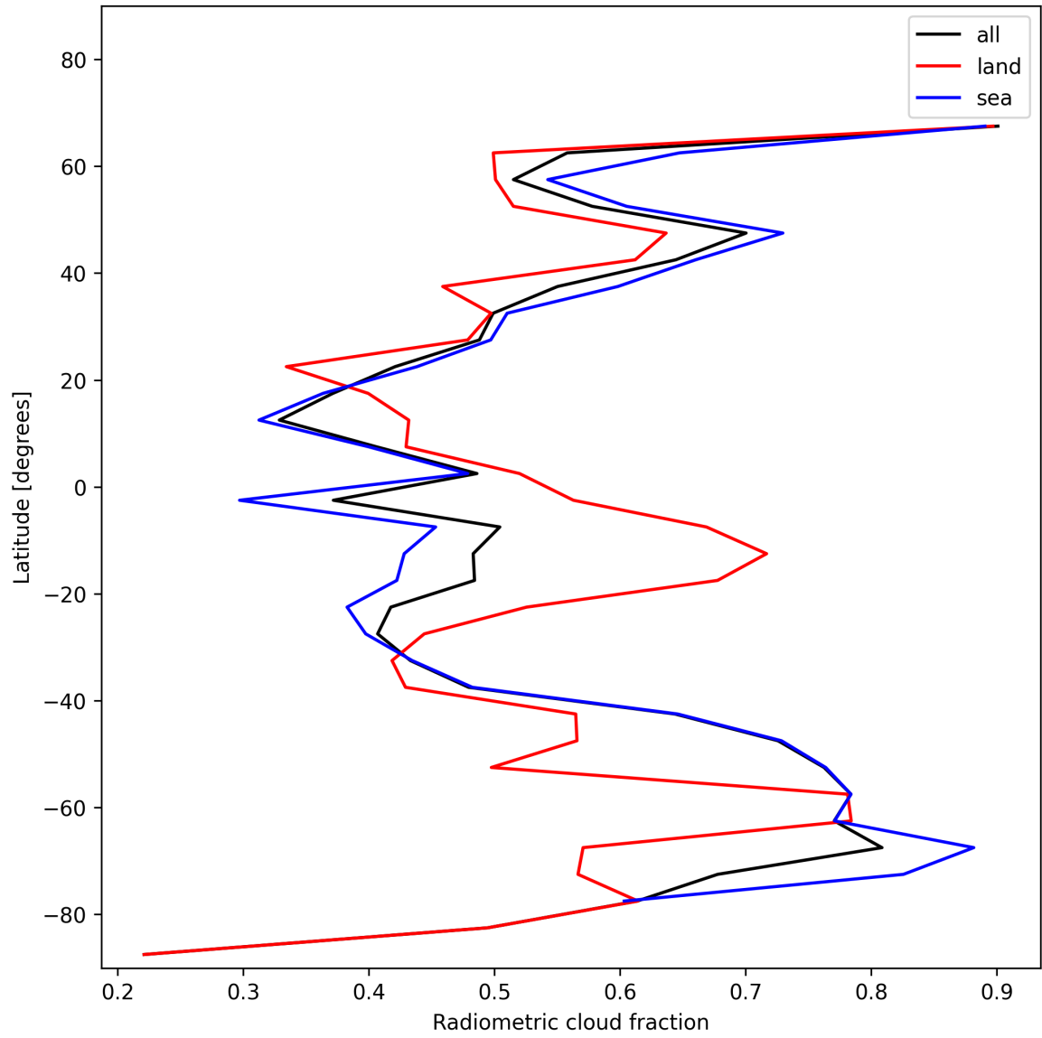
Figure 23: Zonal average of “Radiometric cloud fraction” for 2025-01-01 to 2025-01-03.
