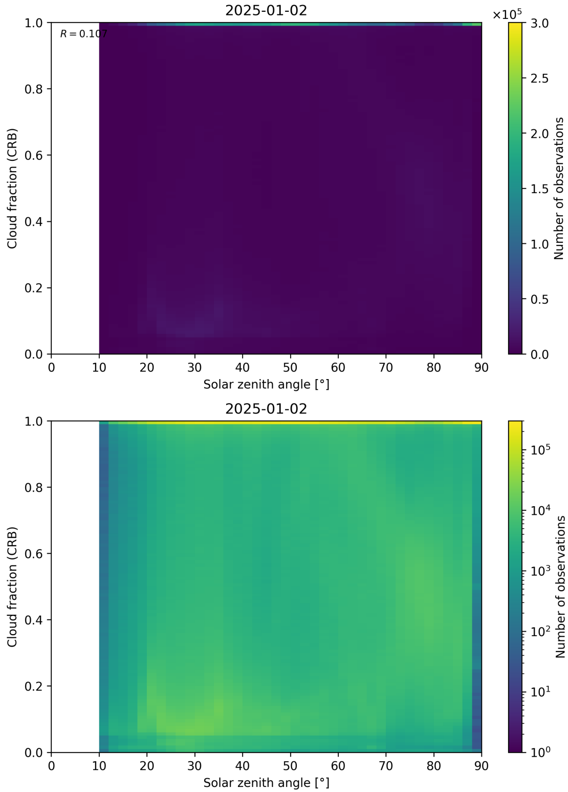
Figure 101: Scatter density plot of “Solar zenith angle” against “Cloud fraction (CRB)” for 2025-01-01 to 2025-01-03.
