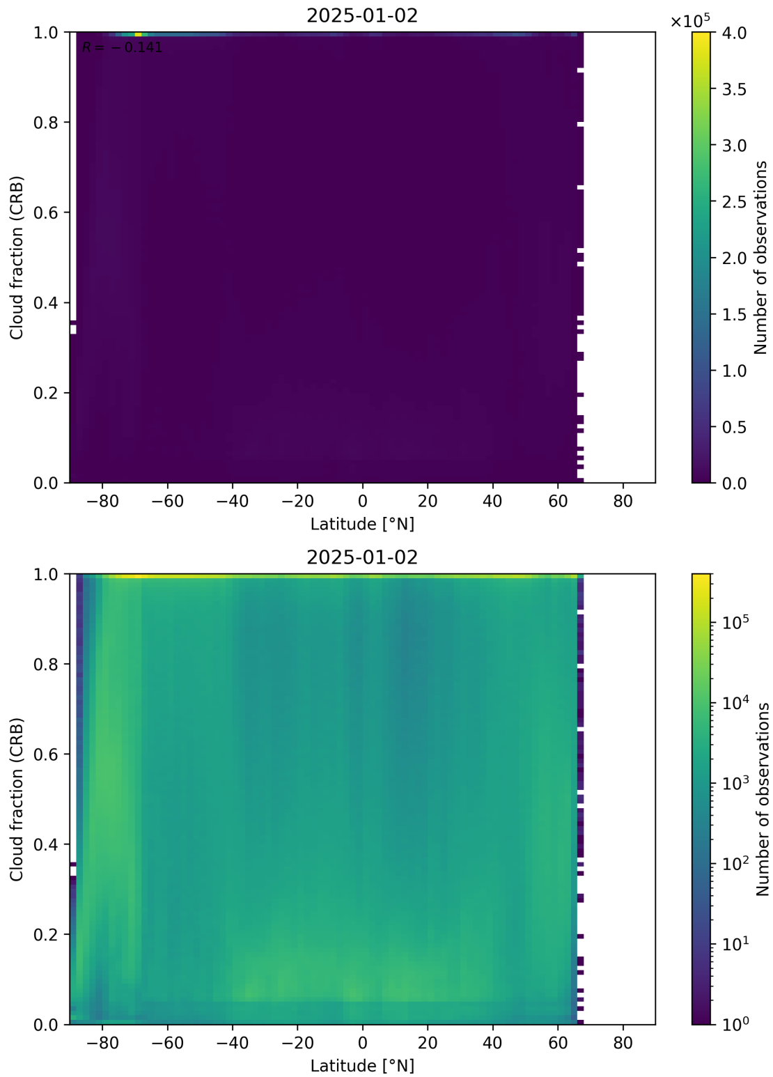
Figure 94: Scatter density plot of “Latitude” against “Cloud fraction (CRB)” for 2025-01-01 to 2025-01-03.
