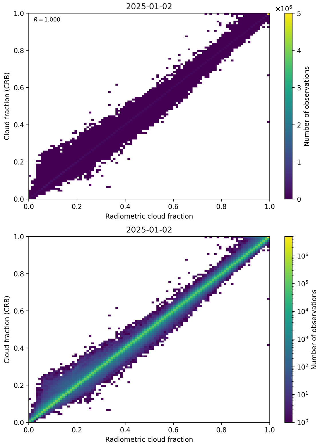
Figure 73: Scatter density plot of “Radiometric cloud fraction” against “Cloud fraction (CRB)” for 2025-01-01 to 2025-01-03.
