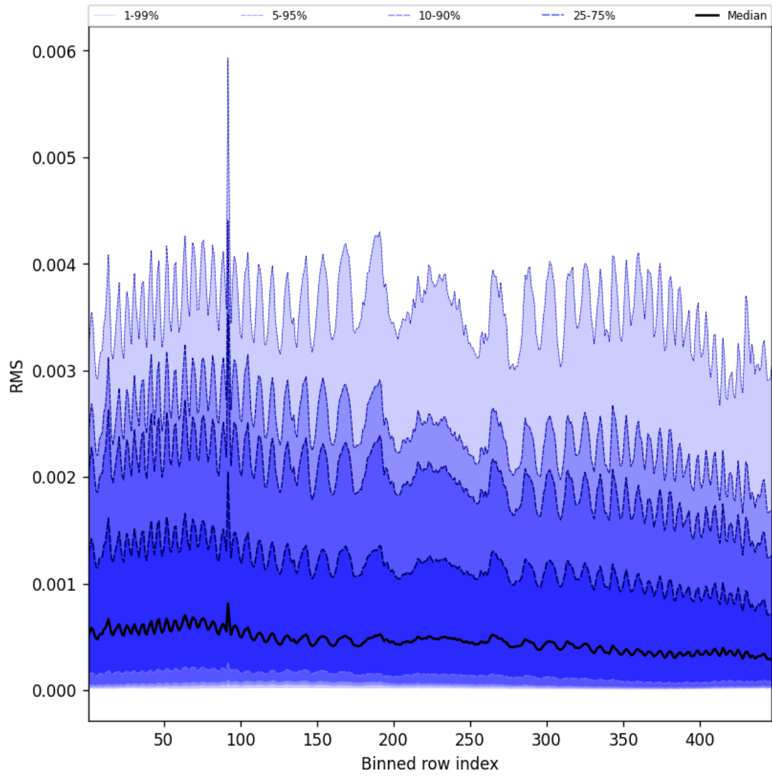
Figure 63: Along track statistics of “RMS” for 2025-01-01 to 2025-01-03
