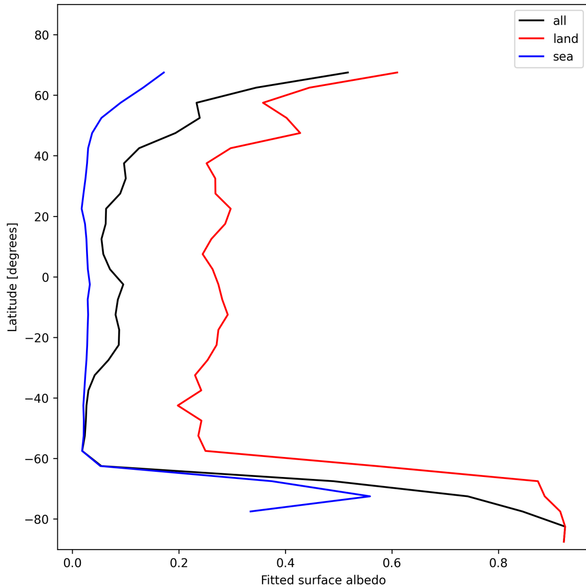
Figure 29: Zonal average of “Fitted surface albedo” for 2025-01-01 to 2025-01-03.
