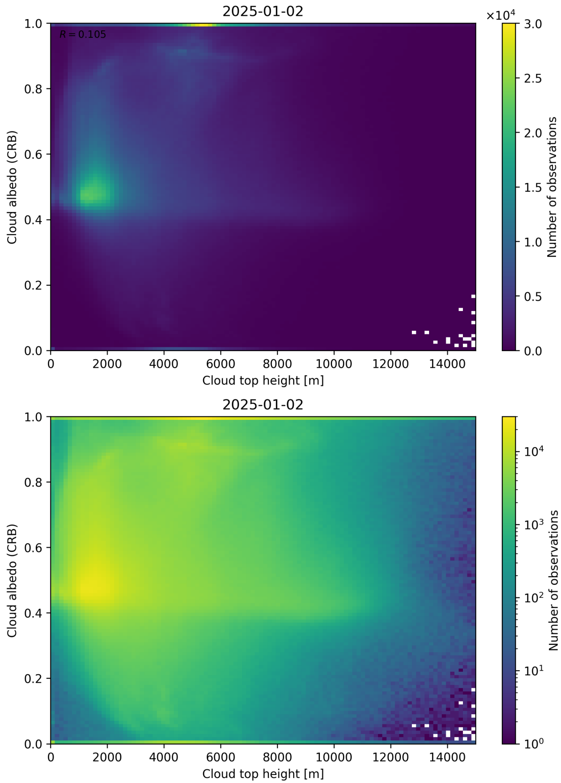
Figure 86: Scatter density plot of “Cloud top height” against “Cloud albedo (CRB)” for 2025-01-01 to 2025-01-03.
