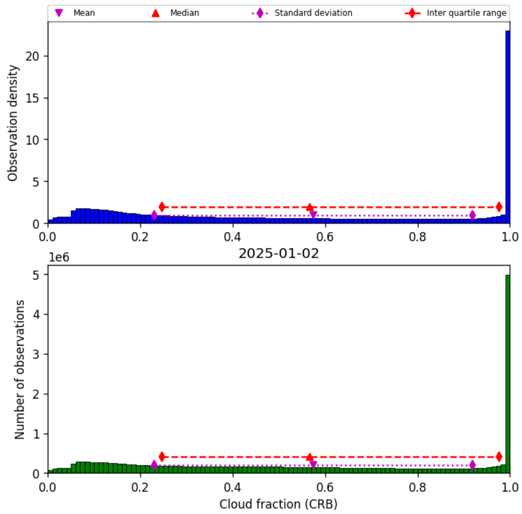
Figure 42: Histogram of “Cloud fraction (CRB)” for 2025-01-01 to 2025-01-03
