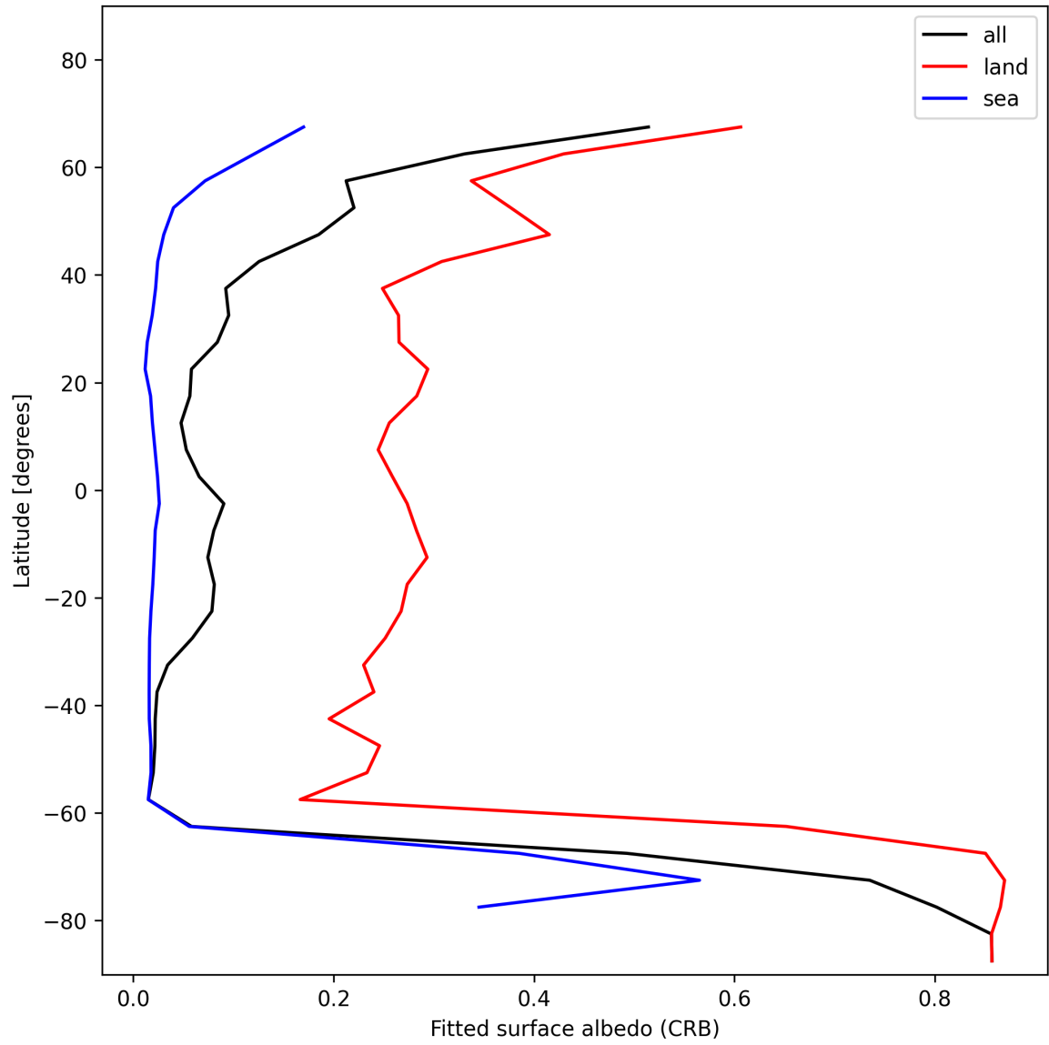
Figure 30: Zonal average of “Fitted surface albedo (CRB)” for 2025-01-01 to 2025-01-03.
