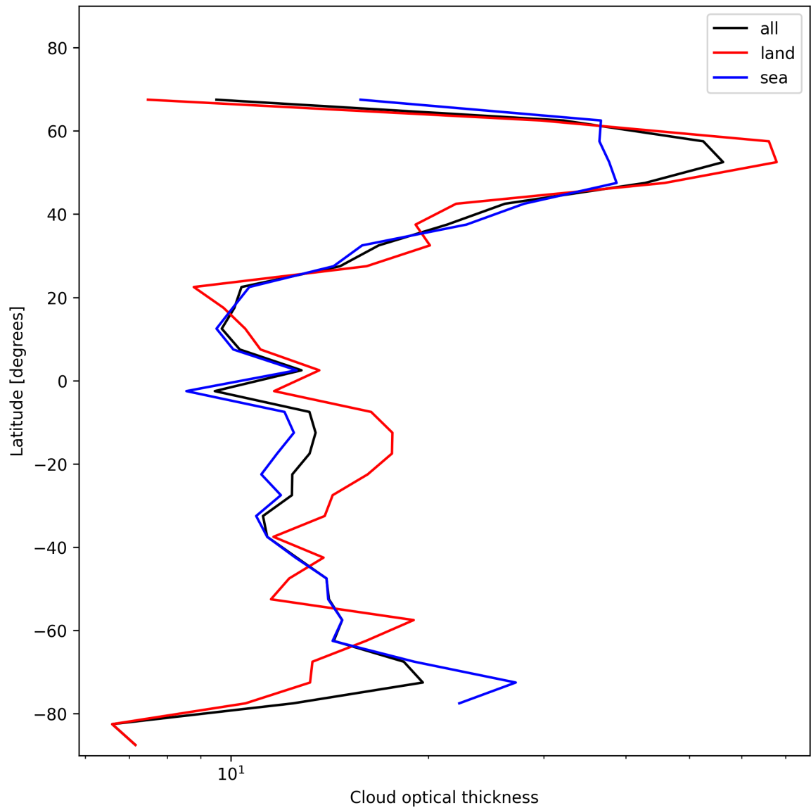
Figure 25: Zonal average of “Cloud optical thickness” for 2025-01-01 to 2025-01-03.
