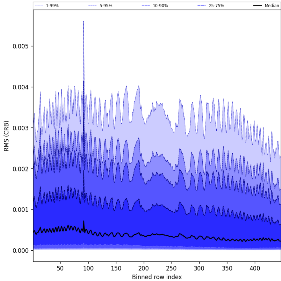
Figure 64: Along track statistics of “RMS (CRB)” for 2025-01-01 to 2025-01-03
