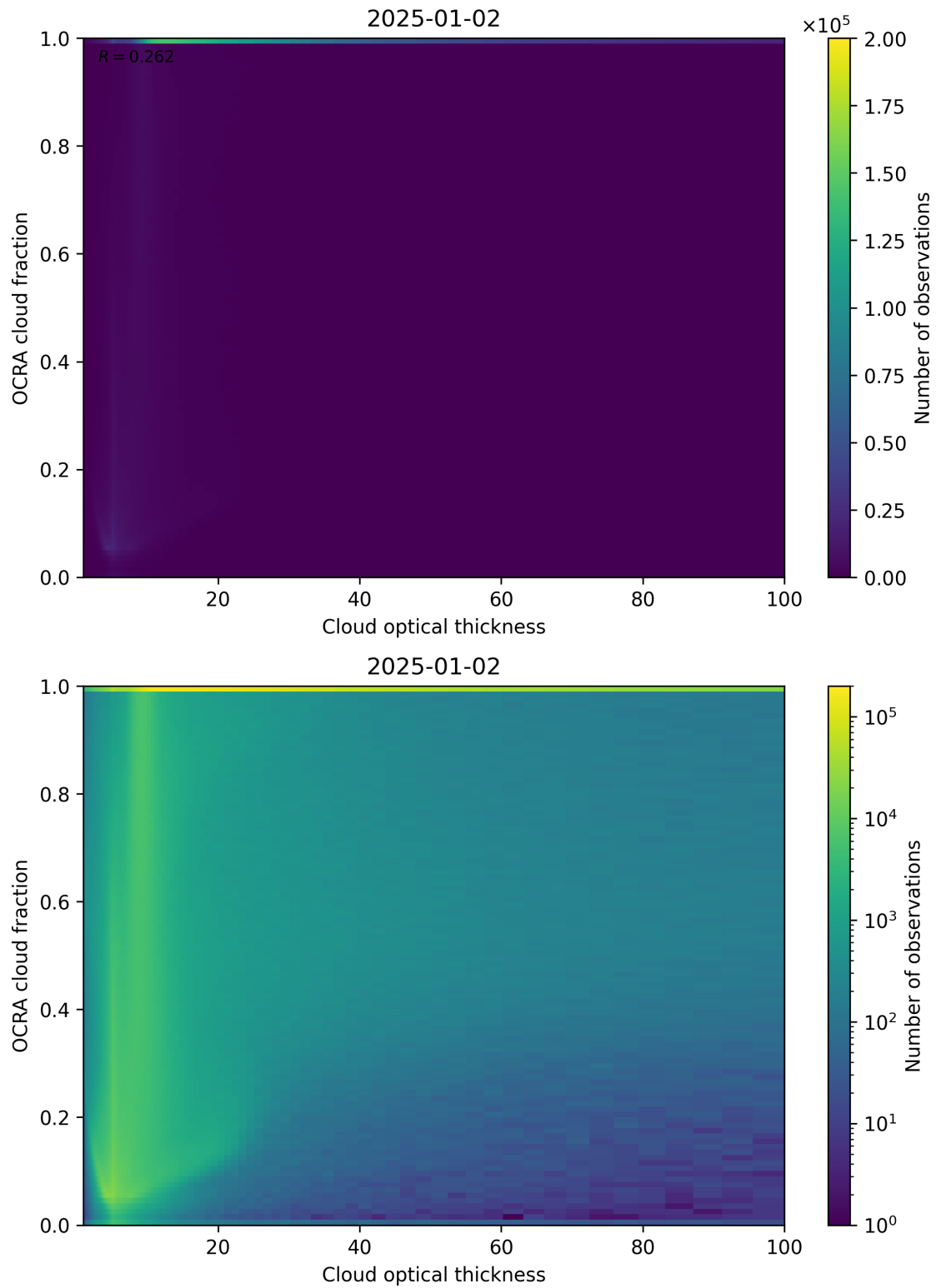
Figure 83: Scatter density plot of “Cloud optical thickness” against “OCRA cloud fraction” for 2025-01-01 to 2025-01-03.
