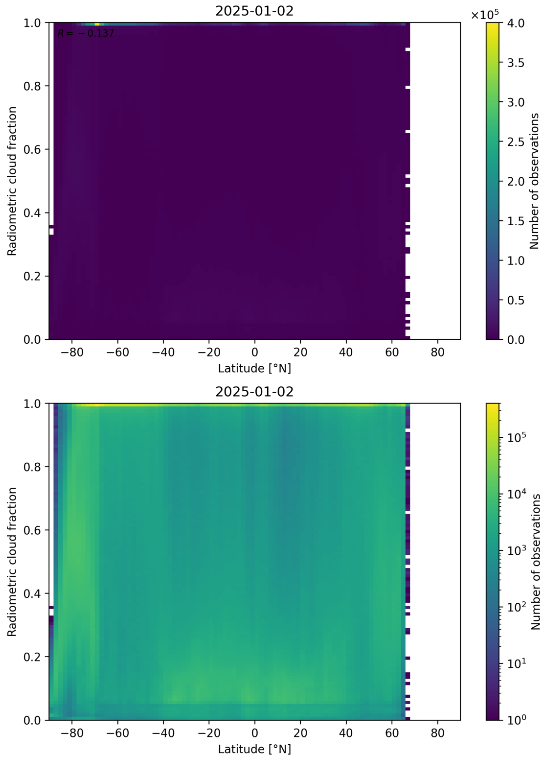
Figure 92: Scatter density plot of “Latitude” against “Radiometric cloud fraction” for 2025-01-01 to 2025-01-03.
