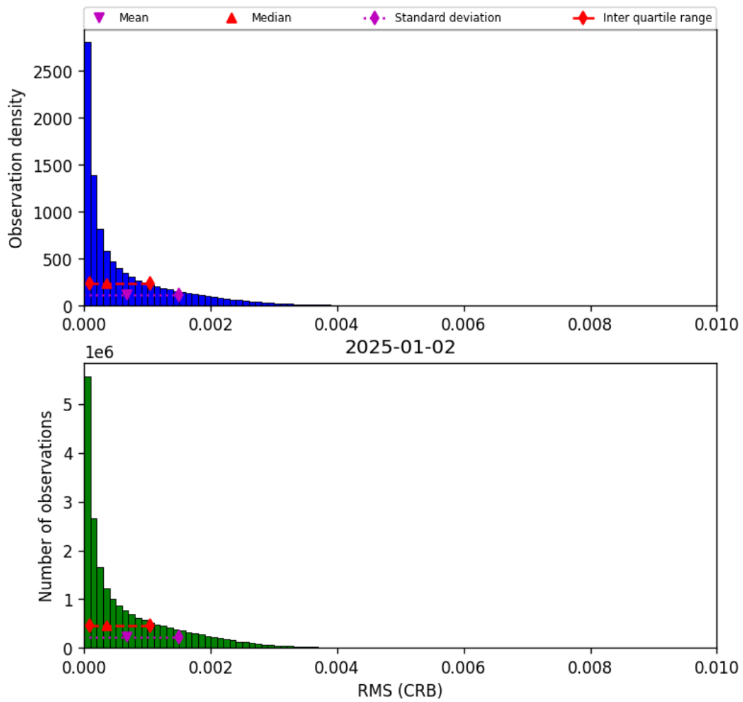
Figure 48: Histogram of “RMS (CRB)” for 2025-01-01 to 2025-01-03
