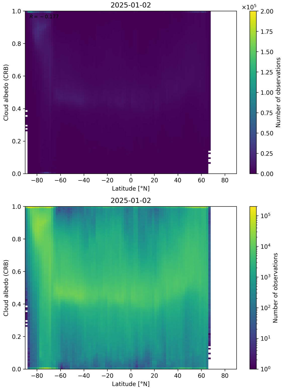
Figure 91: Scatter density plot of “Latitude” against “Cloud albedo (CRB)” for 2025-01-01 to 2025-01-03.
