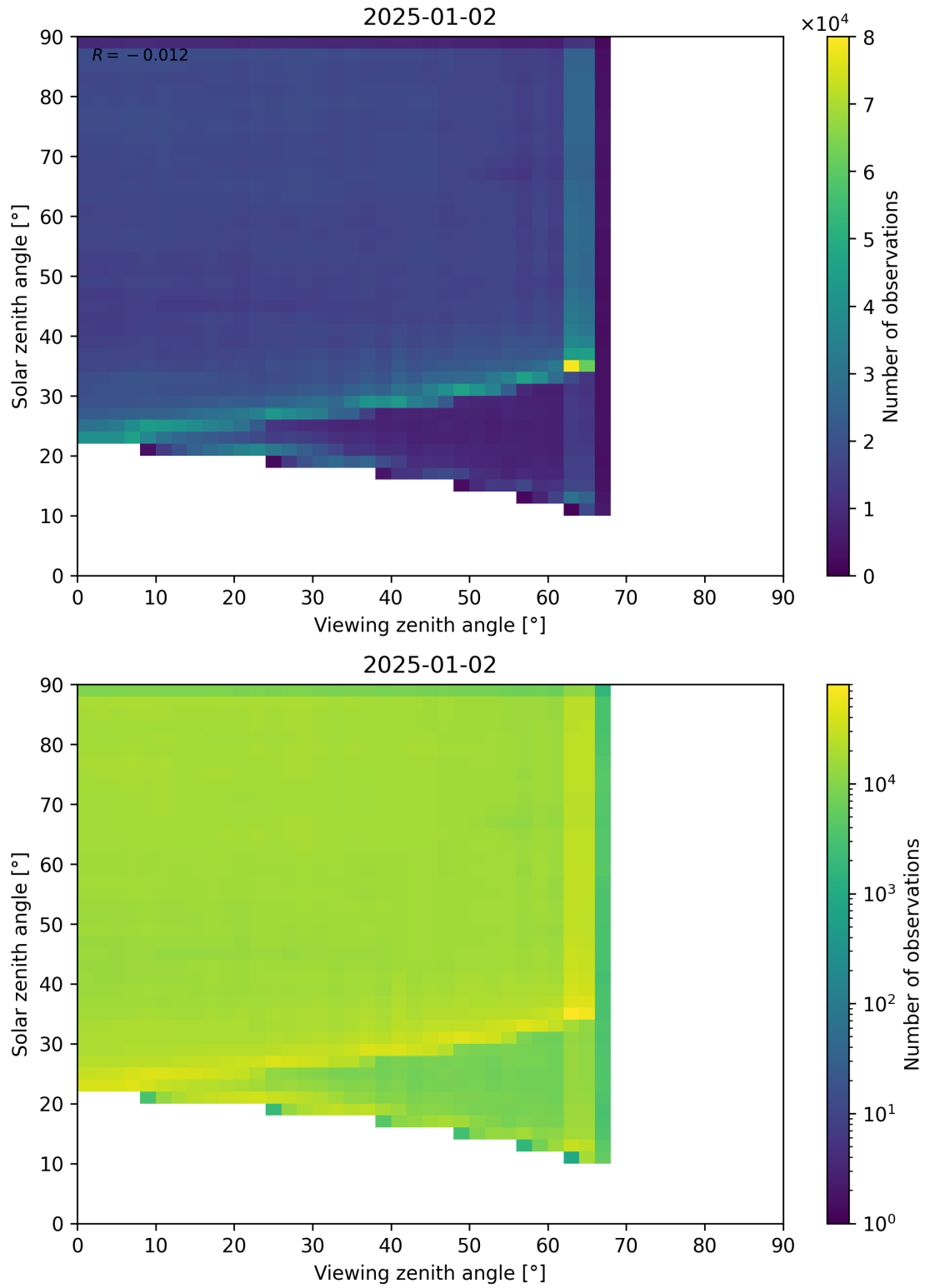
Figure 114: Scatter density plot of “Viewing zenith angle” against “Solar zenith angle” for 2025-01-01 to 2025-01-03.
