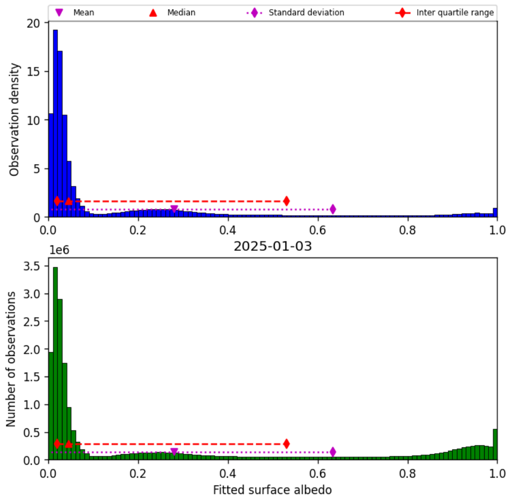
Figure 45: Histogram of “Fitted surface albedo” for 2025-01-02 to 2025-01-04
