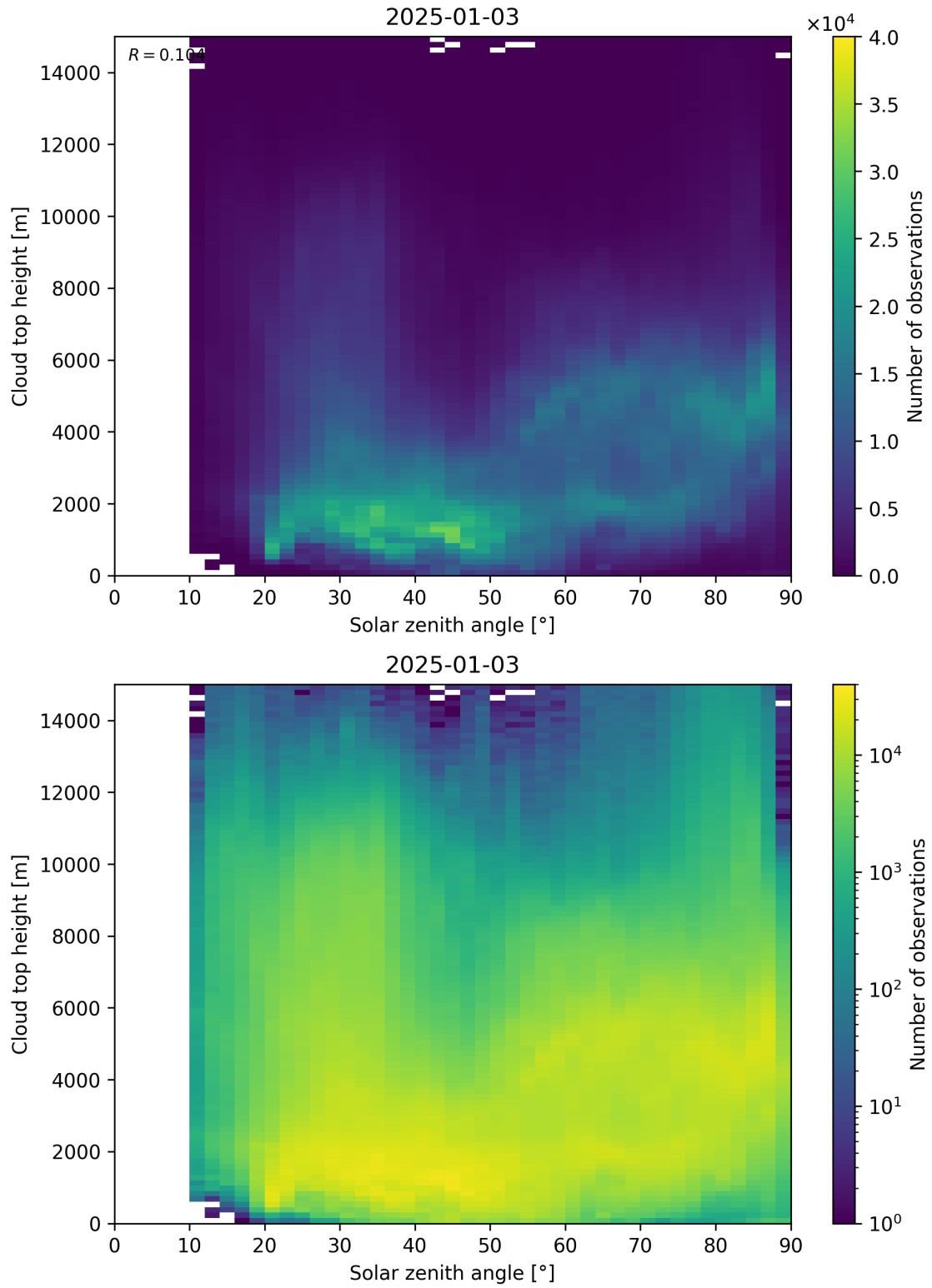
Figure 104: Scatter density plot of “Solar zenith angle” against “Cloud top height” for 2025-01-02 to 2025-01-04.
