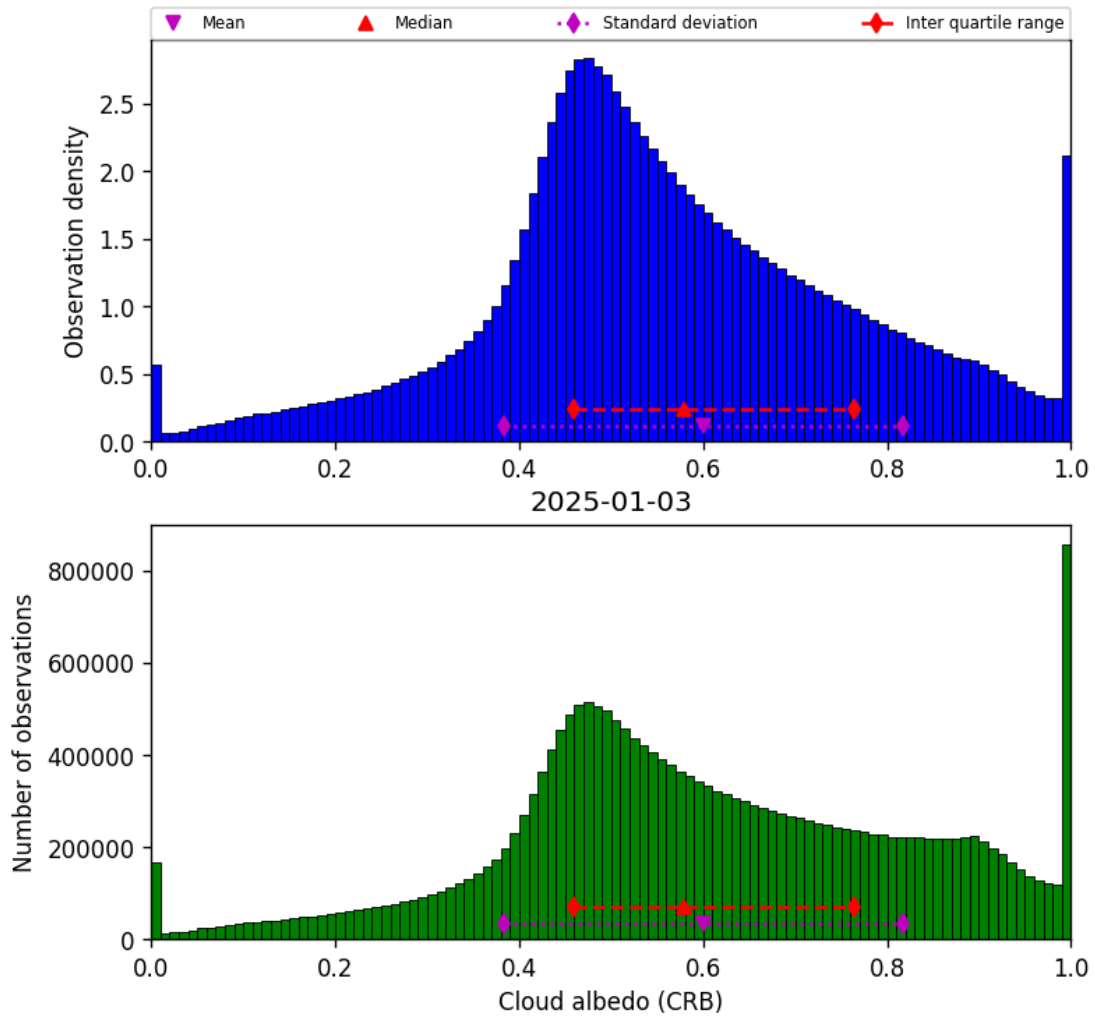
Figure 44: Histogram of “Cloud albedo (CRB)” for 2025-01-02 to 2025-01-04
