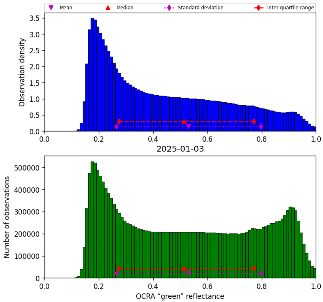
Figure 52: Histogram of “OCRA “green” reflectance” for 2025-01-02 to 2025-01-04
