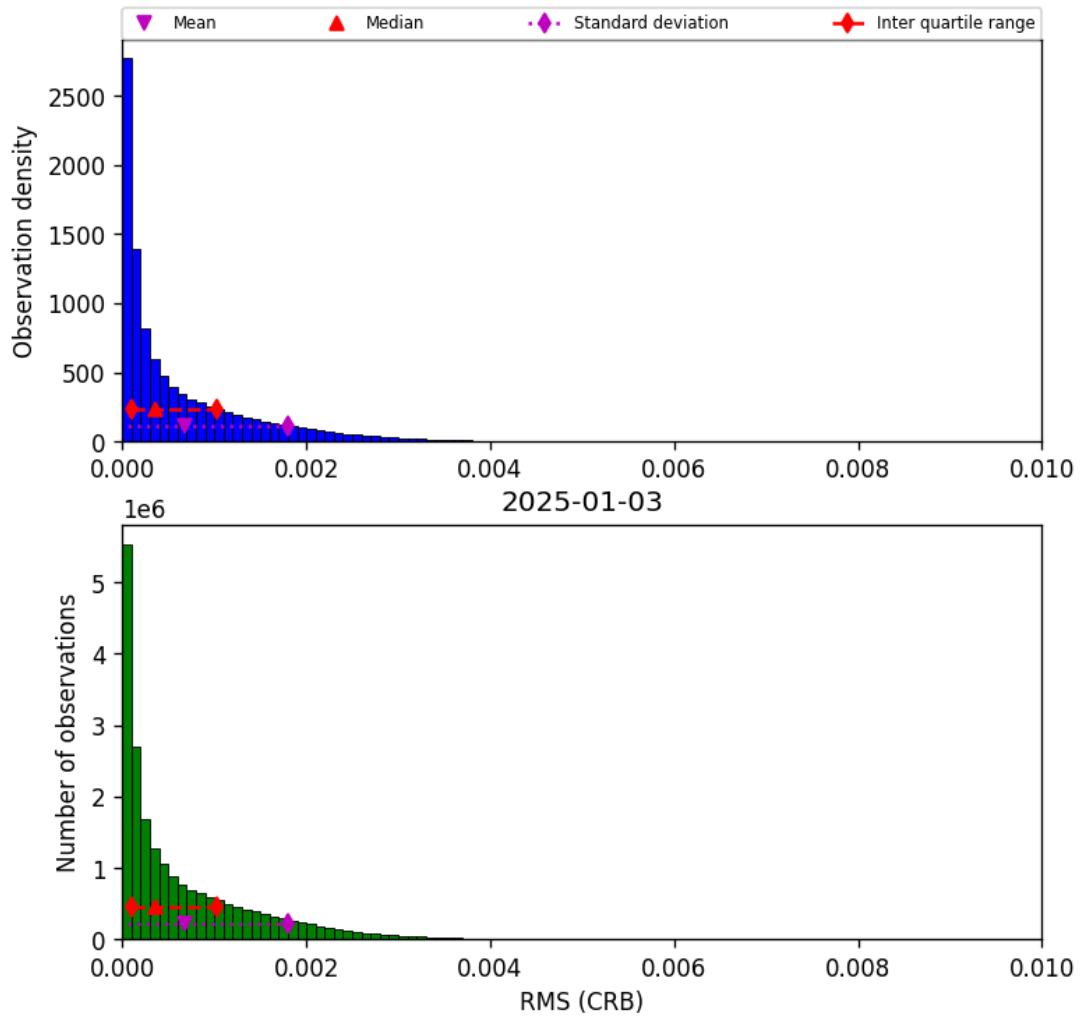
Figure 48: Histogram of “RMS (CRB)” for 2025-01-02 to 2025-01-04
