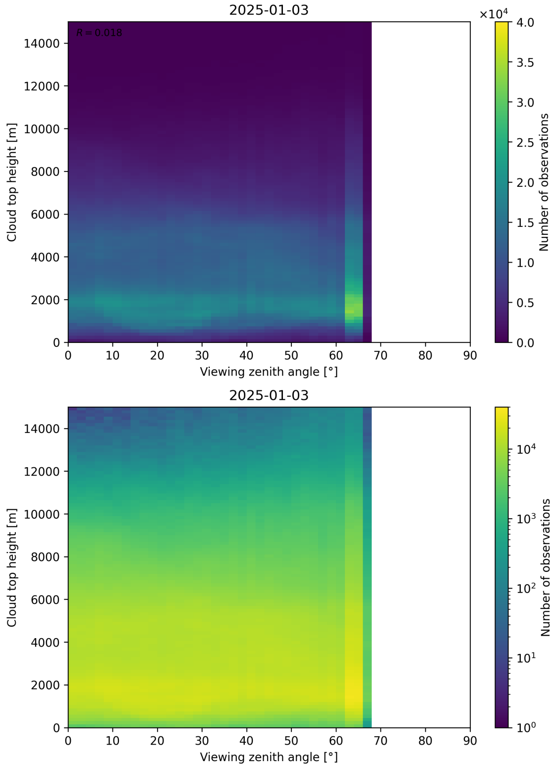
Figure 112: Scatter density plot of “Viewing zenith angle” against “Cloud top height” for 2025-01-02 to 2025-01-04.
