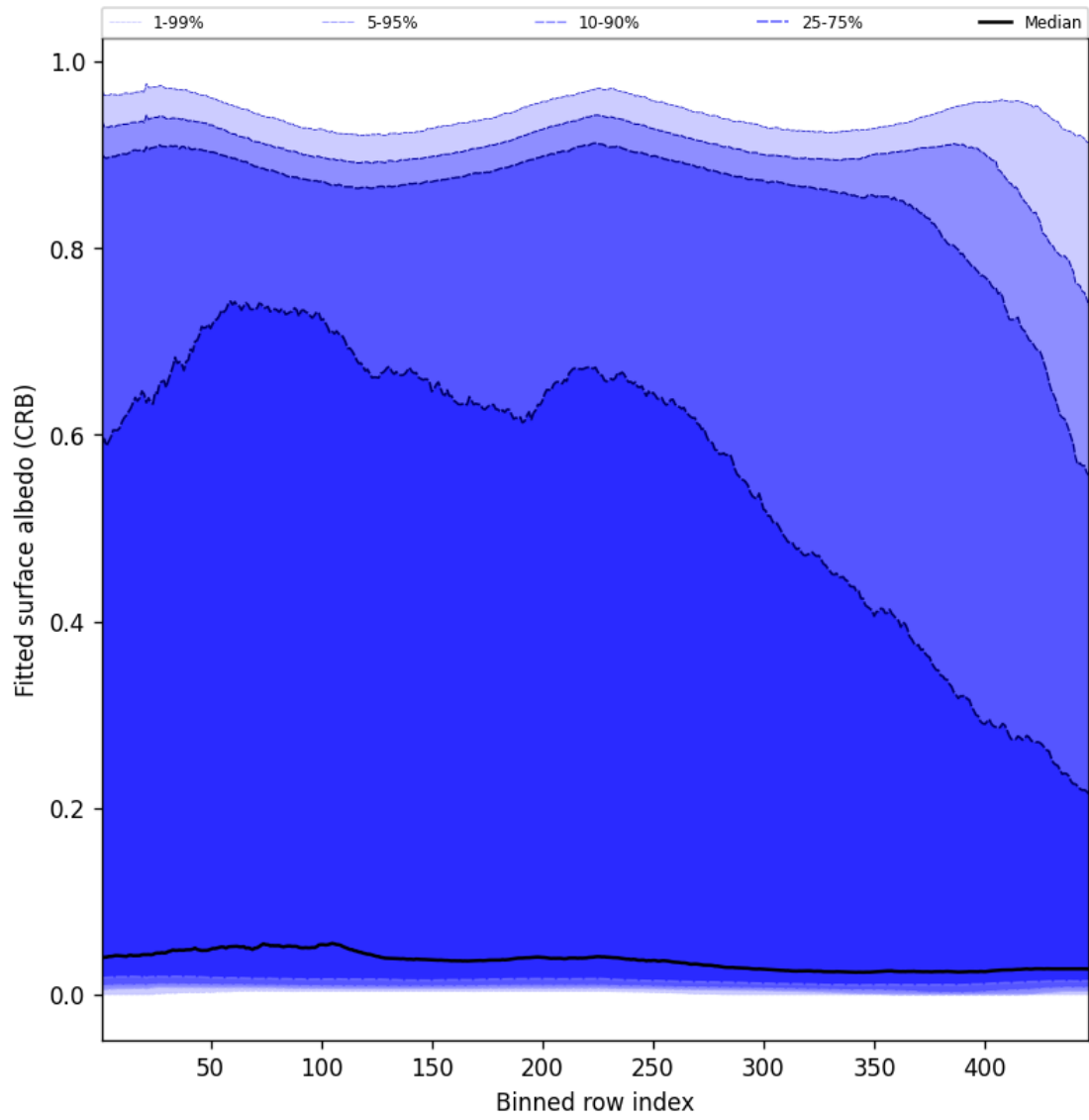
Figure 62: Along track statistics of “Fitted surface albedo (CRB)” for 2025-01-02 to 2025-01-04
