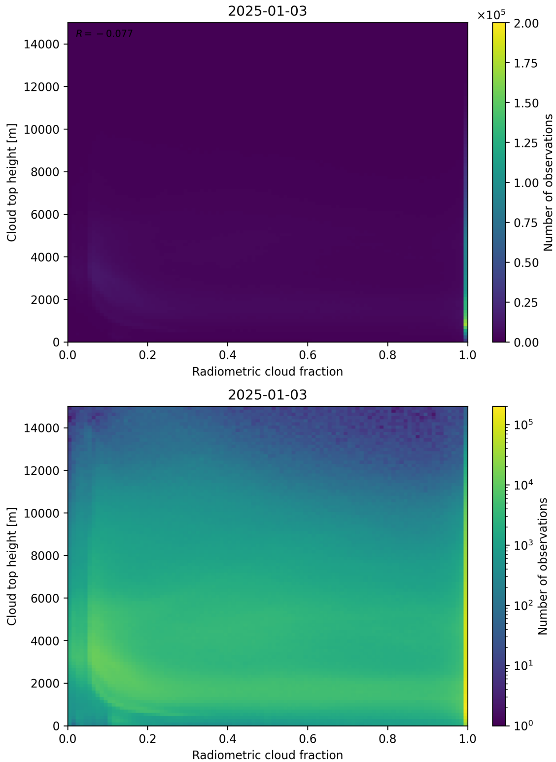
Figure 76: Scatter density plot of “Radiometric cloud fraction” against “Cloud top height” for 2025-01-02 to 2025-01-04.
