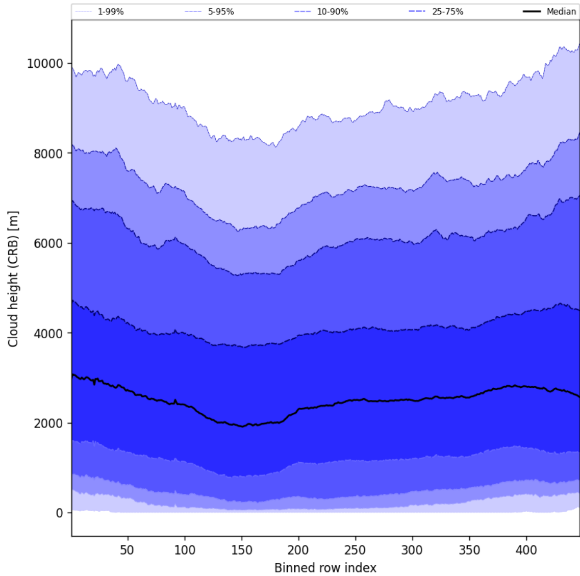
Figure 59: Along track statistics of “Cloud height (CRB)” for 2025-01-02 to 2025-01-04
