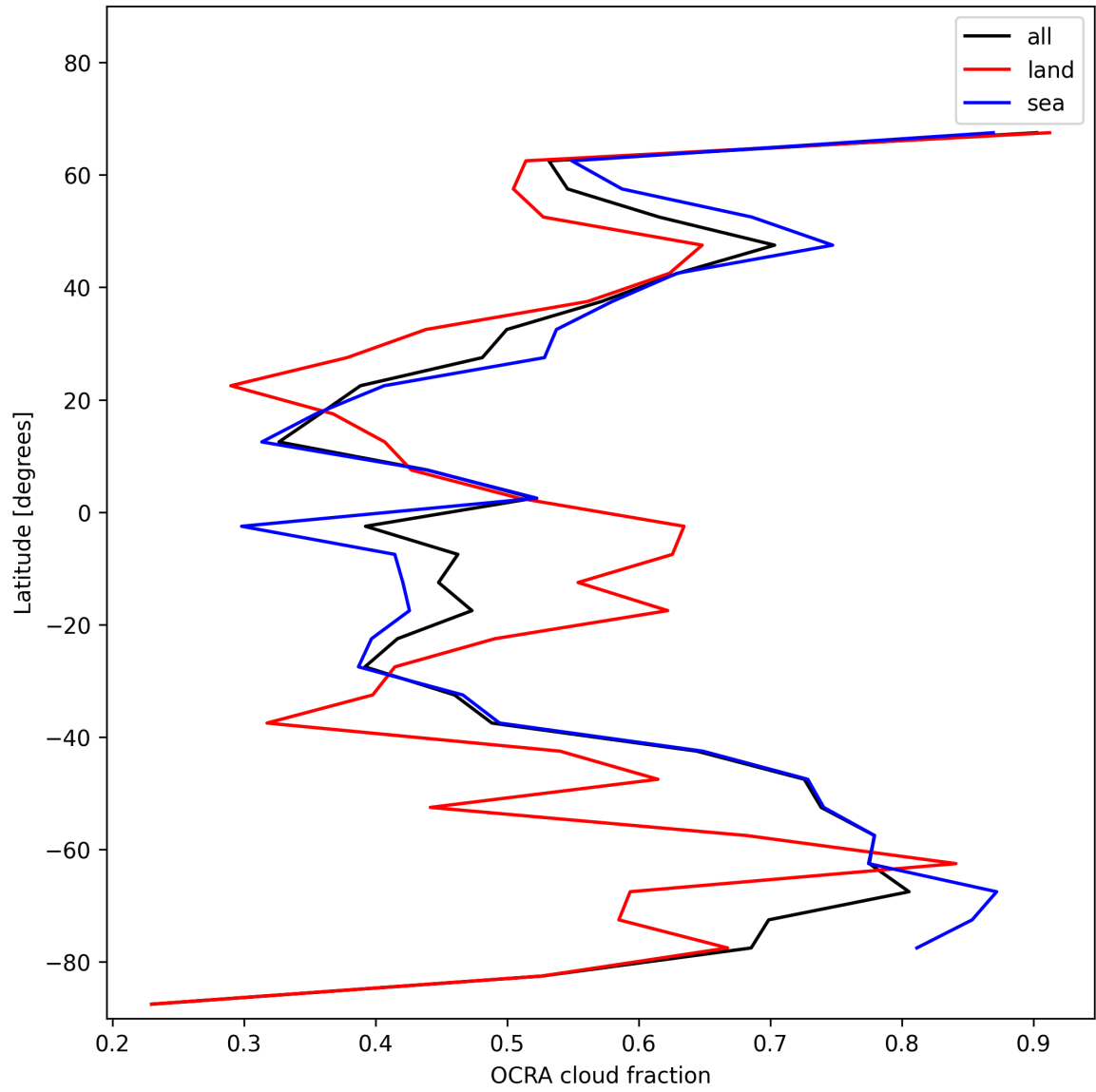
Figure 34: Zonal average of “OCRA cloud fraction” for 2025-01-02 to 2025-01-04.
