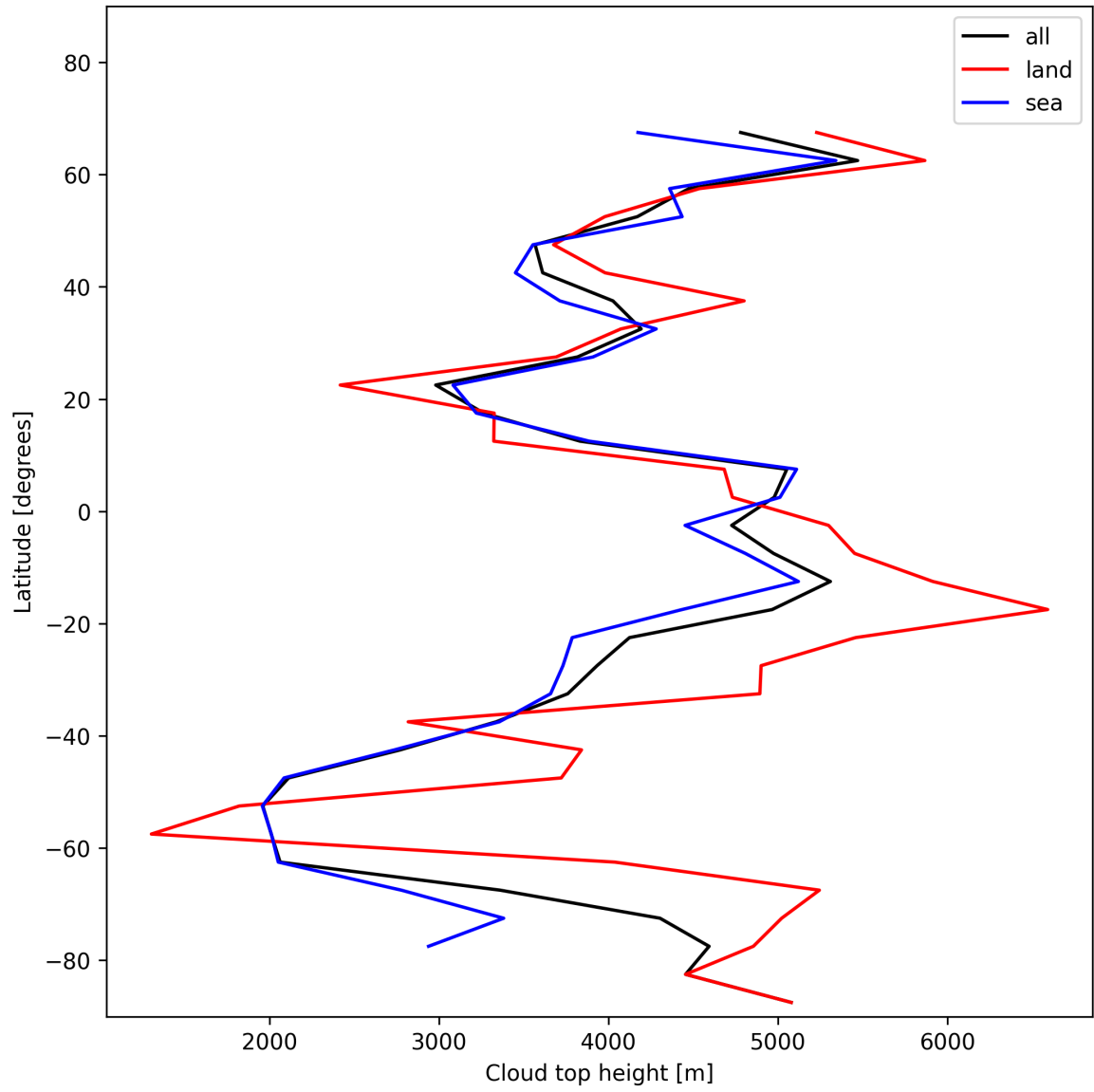
Figure 24: Zonal average of “Cloud top height” for 2025-01-02 to 2025-01-04.
