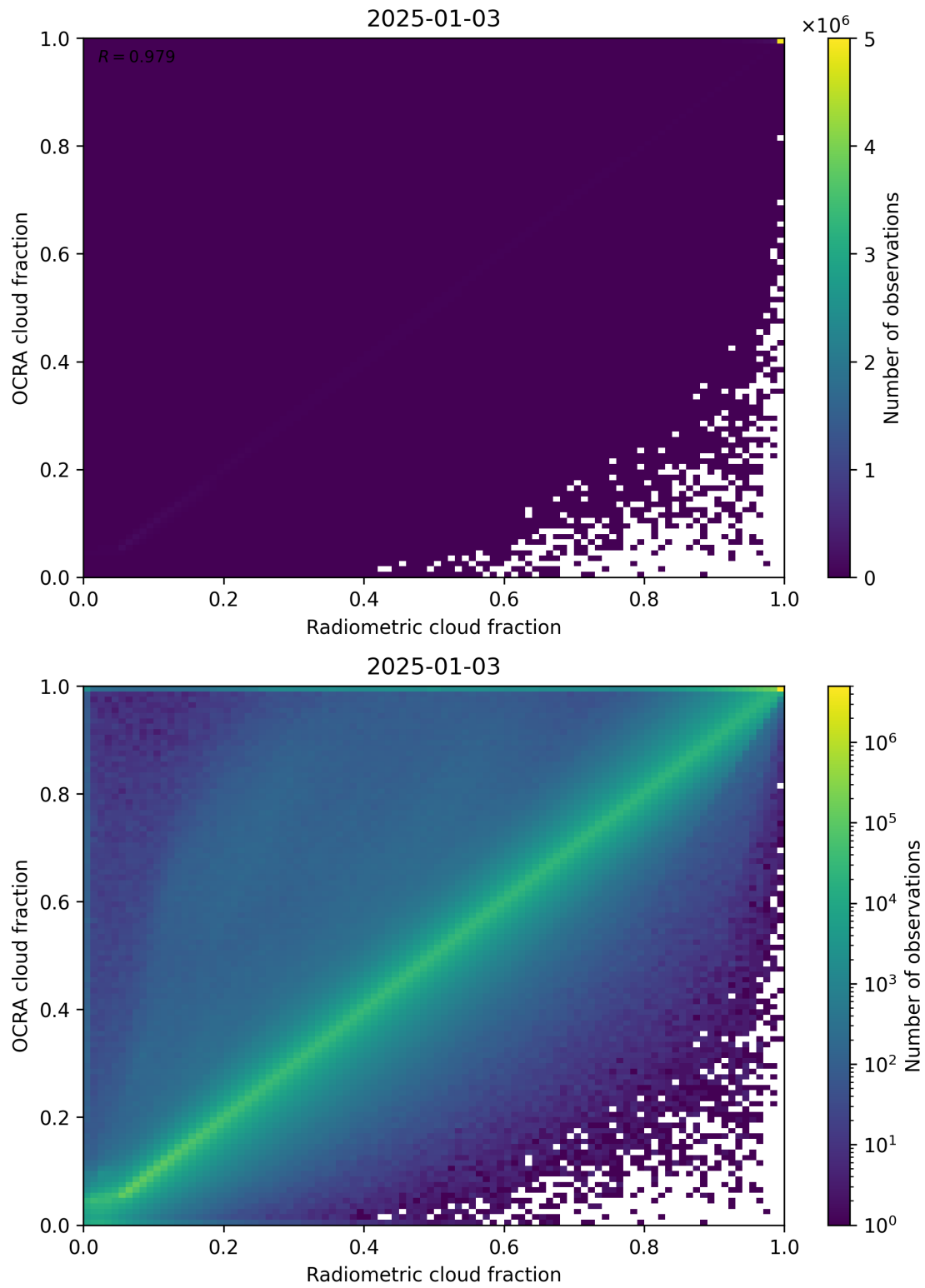
Figure 72: Scatter density plot of “Radiometric cloud fraction” against “OCRA cloud fraction” for 2025-01-02 to 2025-01-04.
