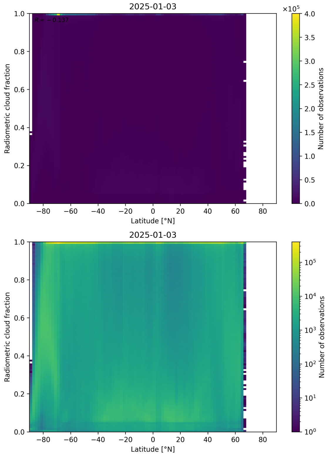
Figure 92: Scatter density plot of “Latitude” against “Radiometric cloud fraction” for 2025-01-02 to 2025-01-04.
