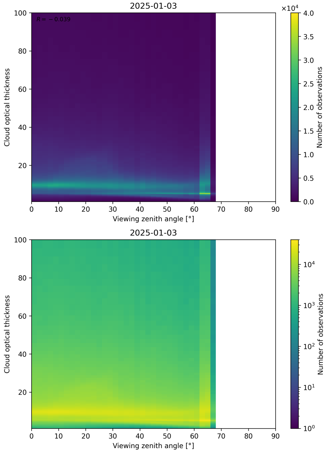
Figure 111: Scatter density plot of “Viewing zenith angle” against “Cloud optical thickness” for 2025-01-02 to 2025-01-04.
