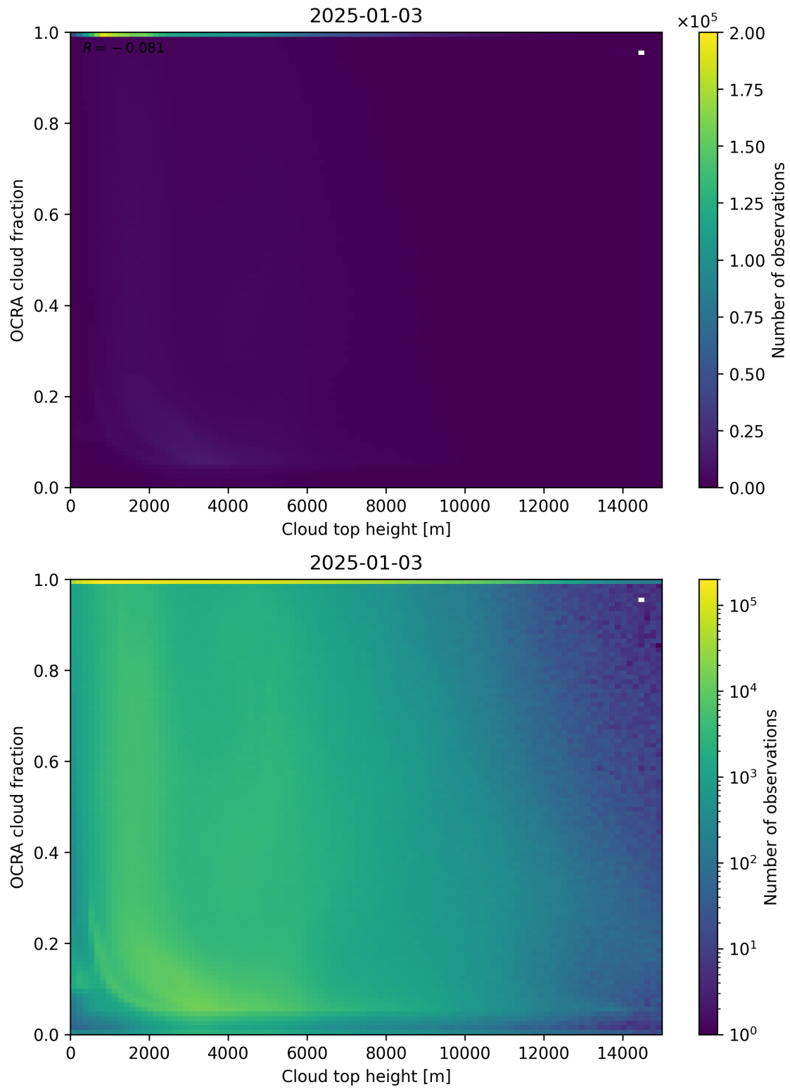
Figure 87: Scatter density plot of “Cloud top height” against “OCRA cloud fraction” for 2025-01-02 to 2025-01-04.
