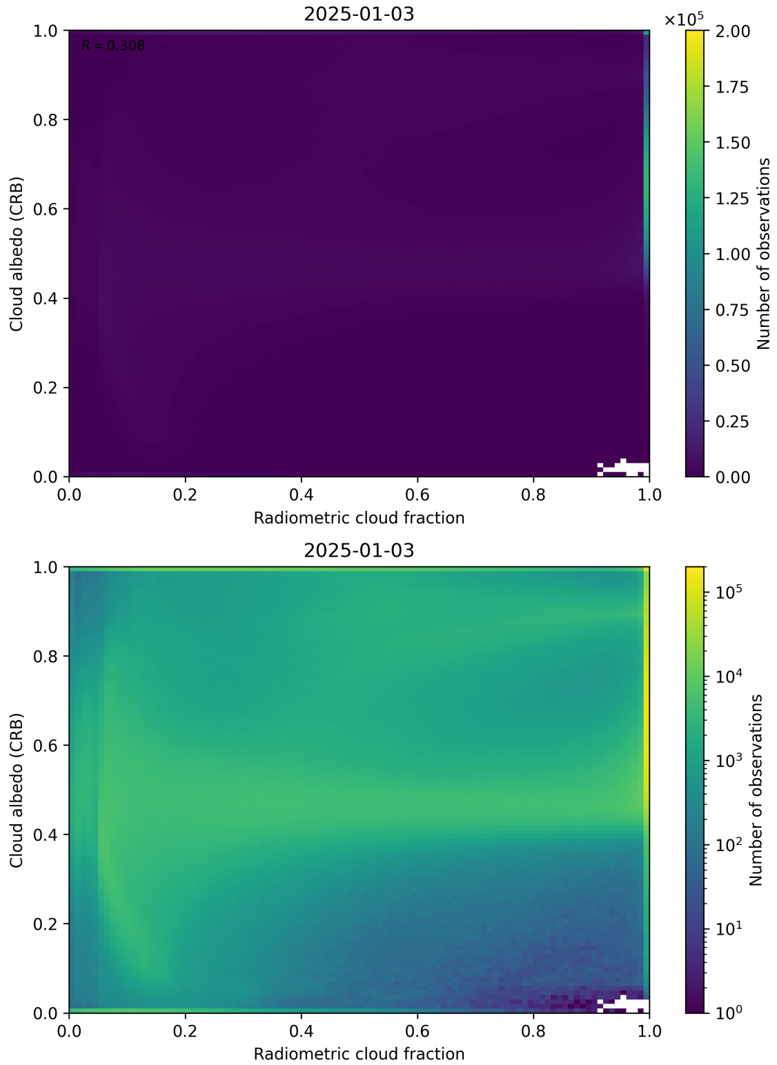
Figure 71: Scatter density plot of “Radiometric cloud fraction” against “Cloud albedo (CRB)” for 2025-01-02 to 2025-01-04.
