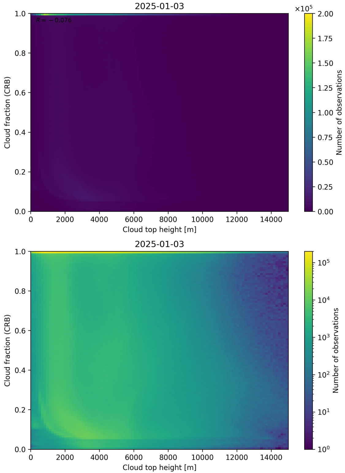
Figure 88: Scatter density plot of “Cloud top height” against “Cloud fraction (CRB)” for 2025-01-02 to 2025-01-04.
