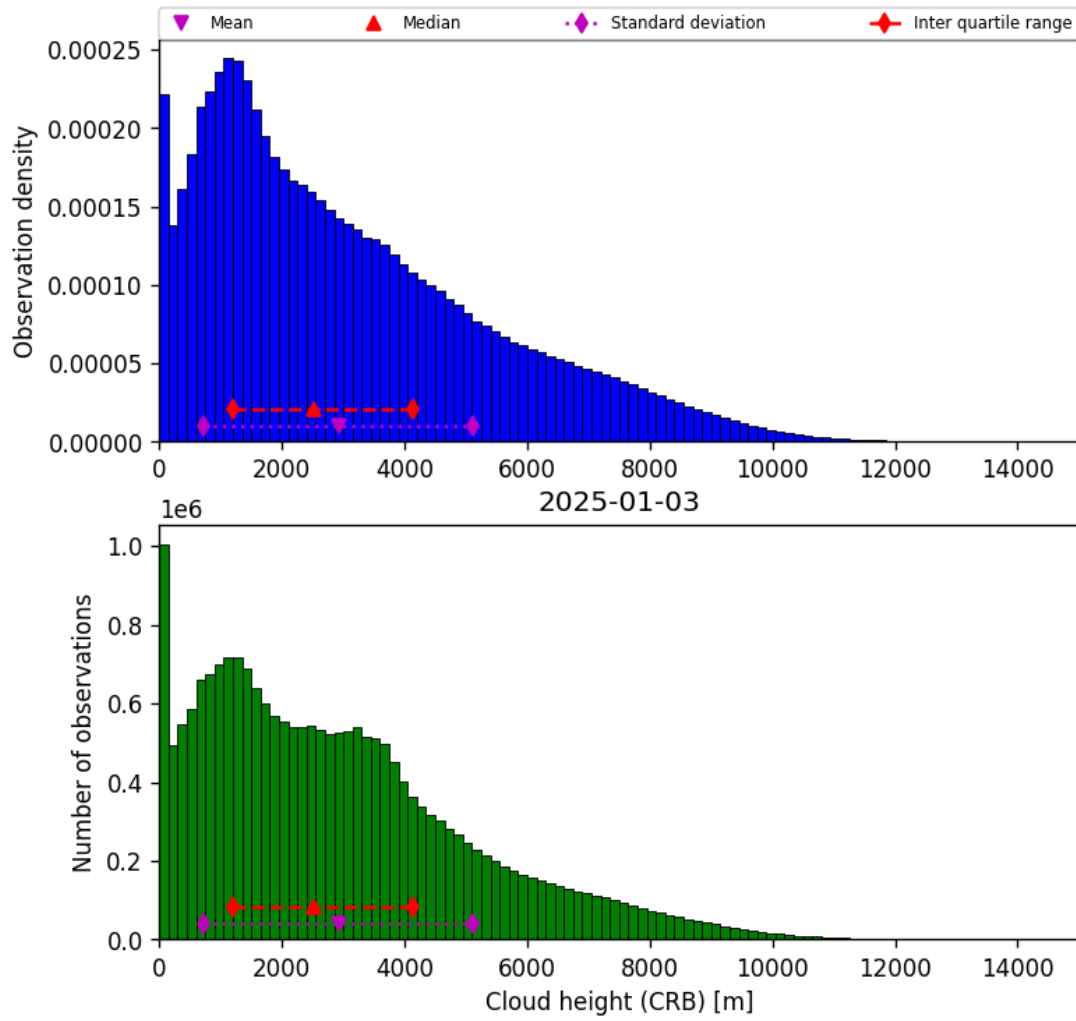
Figure 43: Histogram of “Cloud height (CRB)” for 2025-01-02 to 2025-01-04
