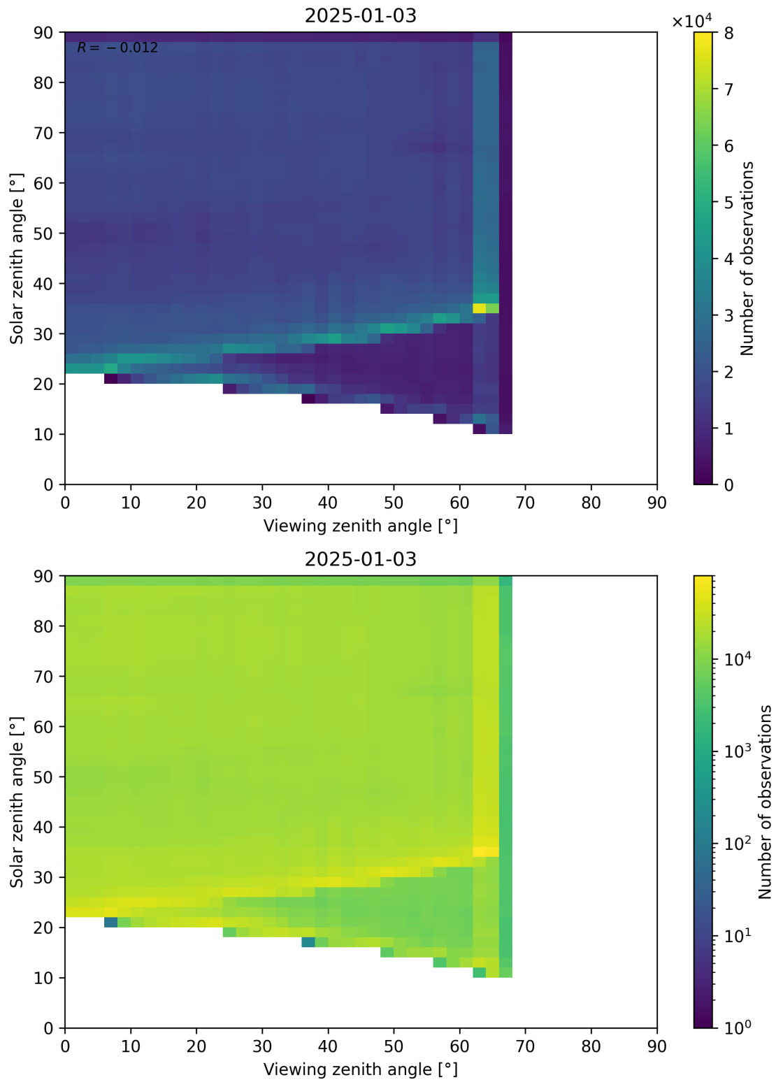
Figure 114: Scatter density plot of “Viewing zenith angle” against “Solar zenith angle” for 2025-01-02 to 2025-01-04.
