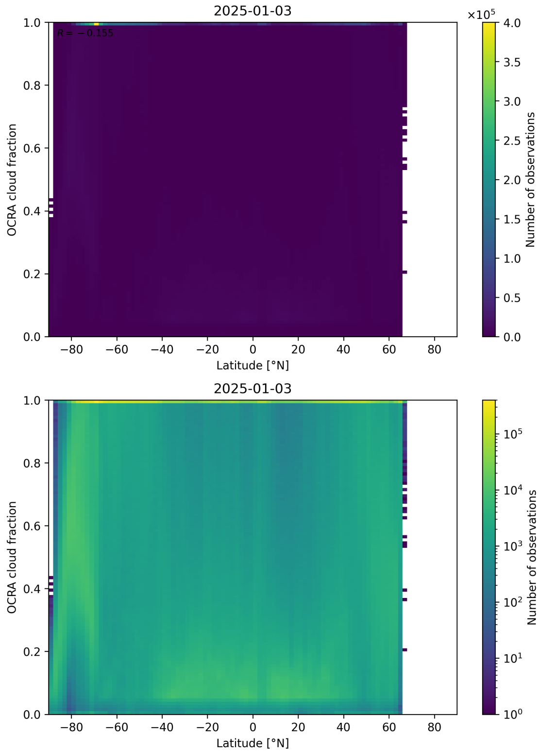
Figure 93: Scatter density plot of “Latitude” against “OCRA cloud fraction” for 2025-01-02 to 2025-01-04.
