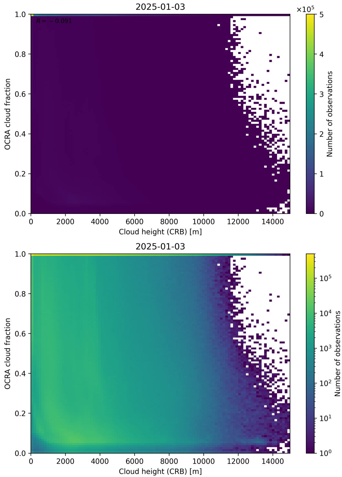
Figure 81: Scatter density plot of “Cloud height (CRB)” against “OCRA cloud fraction” for 2025-01-02 to 2025-01-04.
