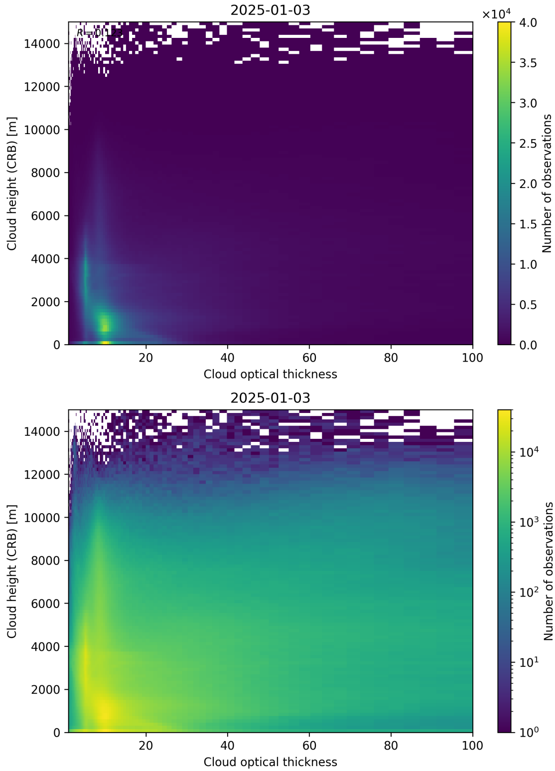
Figure 85: Scatter density plot of “Cloud optical thickness” against “Cloud height (CRB)” for 2025-01-02 to 2025-01-04.
