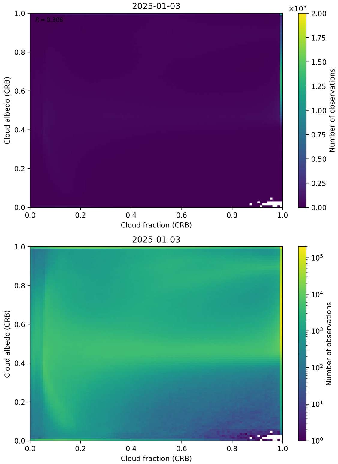
Figure 77: Scatter density plot of “Cloud fraction (CRB)” against “Cloud albedo (CRB)” for 2025-01-02 to 2025-01-04.
