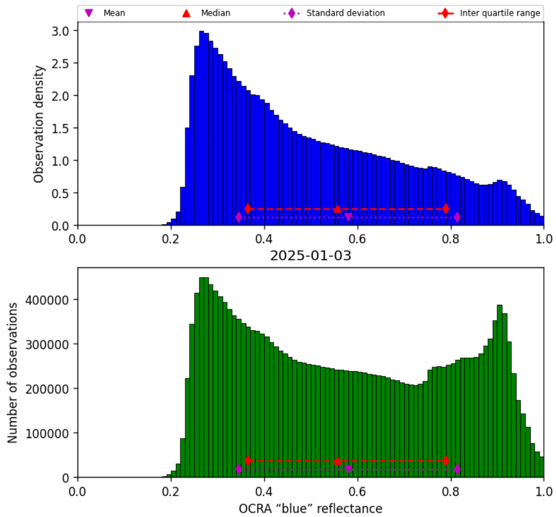
Figure 51: Histogram of “OCRA “blue” reflectance” for 2025-01-02 to 2025-01-04
