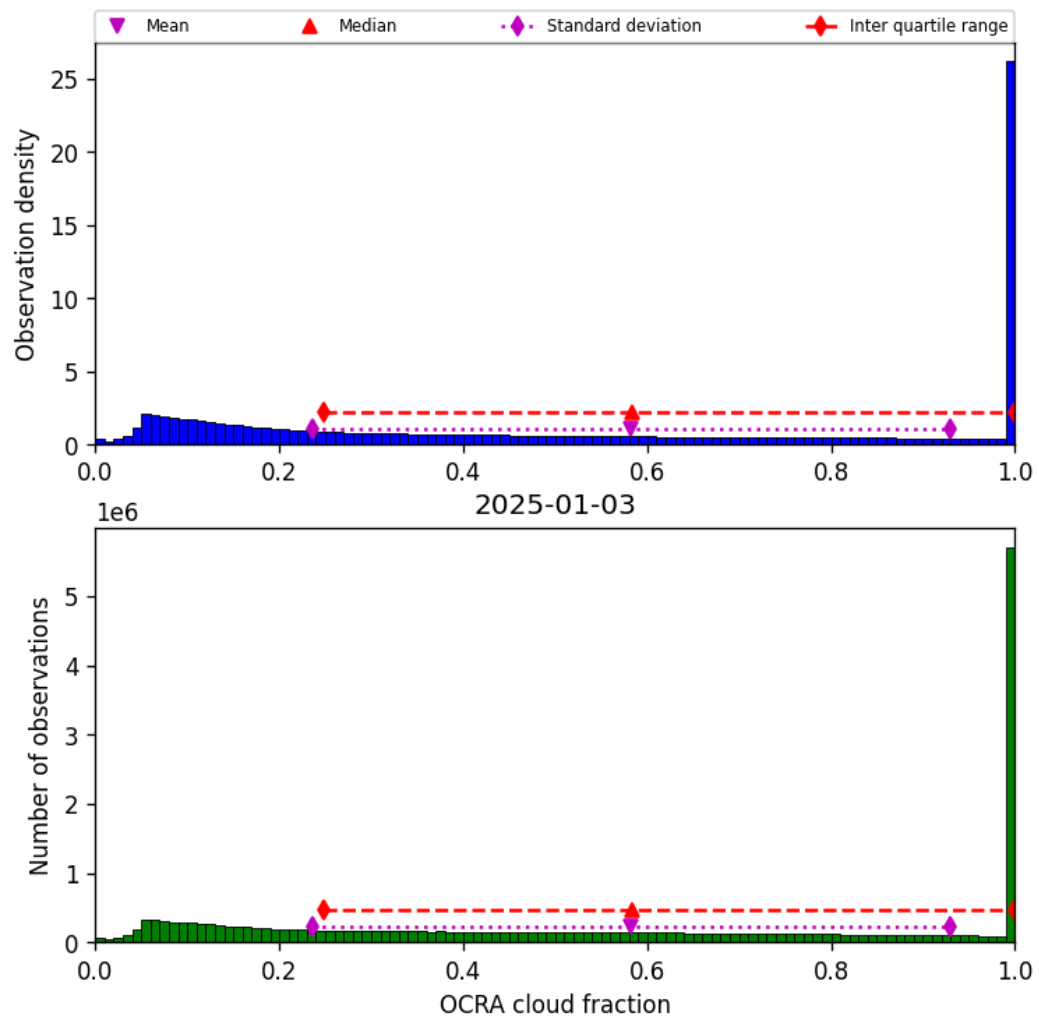
Figure 50: Histogram of “OCRA cloud fraction” for 2025-01-02 to 2025-01-04
