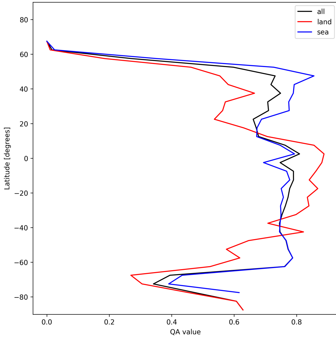
Figure 22: Zonal average of “QA value” for 2025-01-02 to 2025-01-04.
