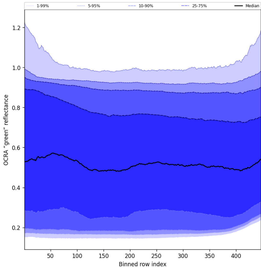
Figure 68: Along track statistics of "OCRA "green" reflectance" for 2025-01-02 to 2025-01-04
