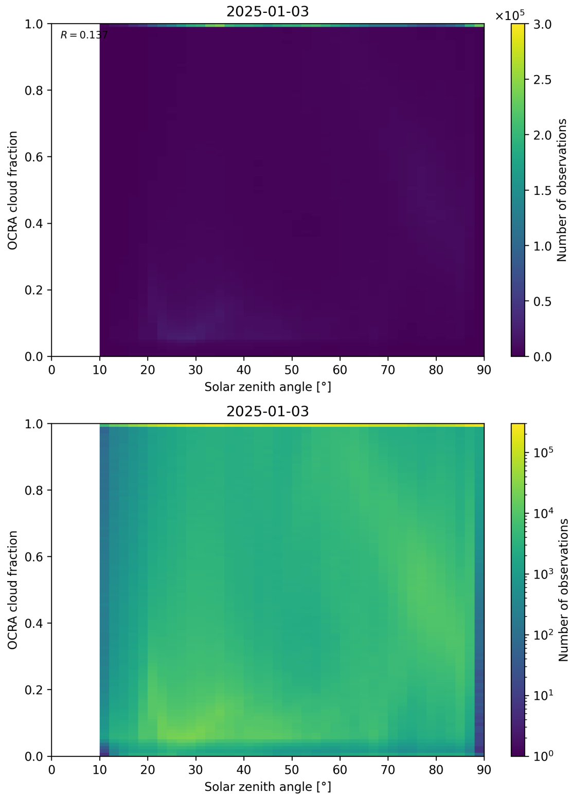
Figure 100: Scatter density plot of “Solar zenith angle” against “OCRA cloud fraction” for 2025-01-02 to 2025-01-04.
