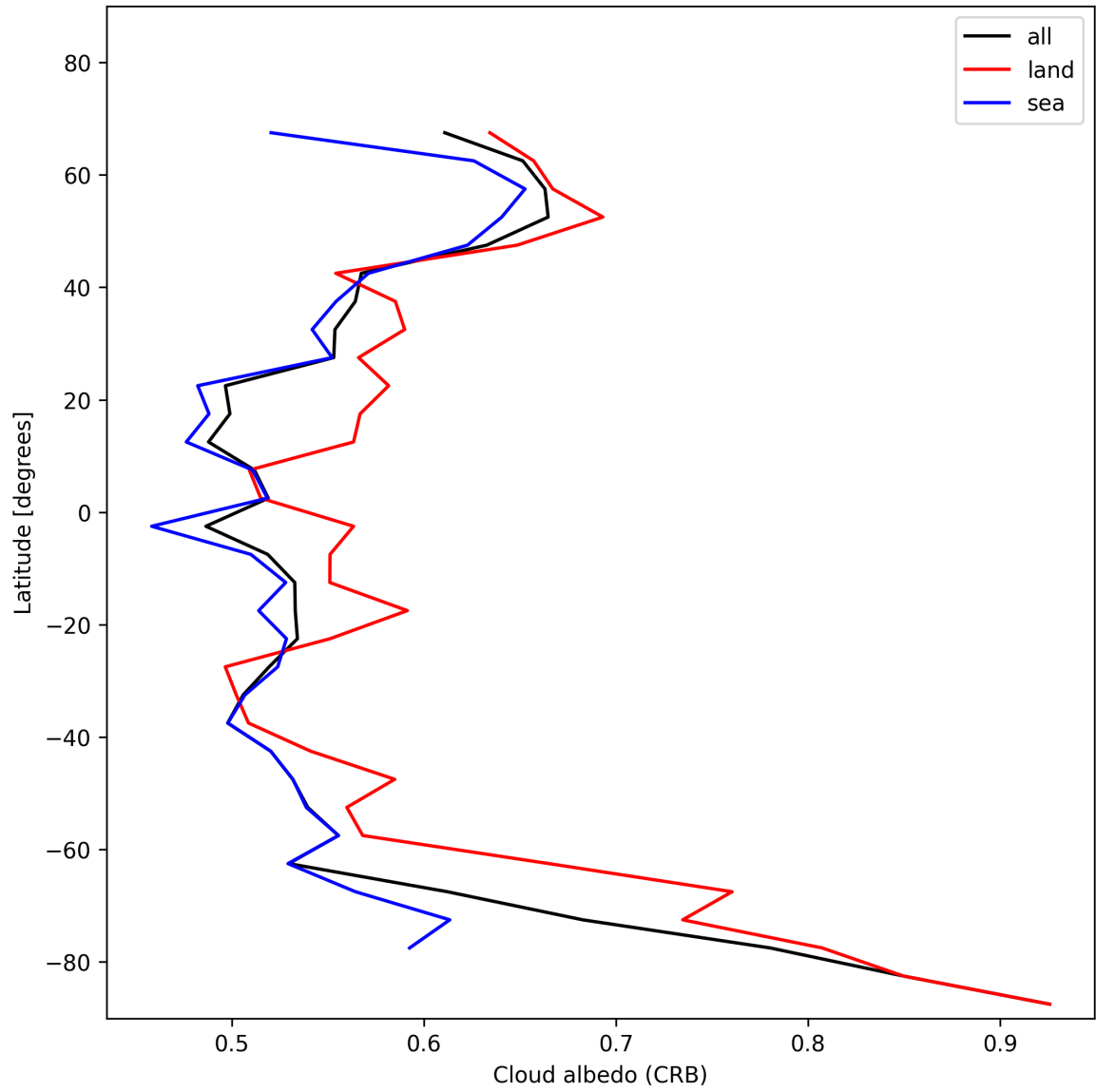
Figure 28: Zonal average of “Cloud albedo (CRB)” for 2025-01-02 to 2025-01-04.
