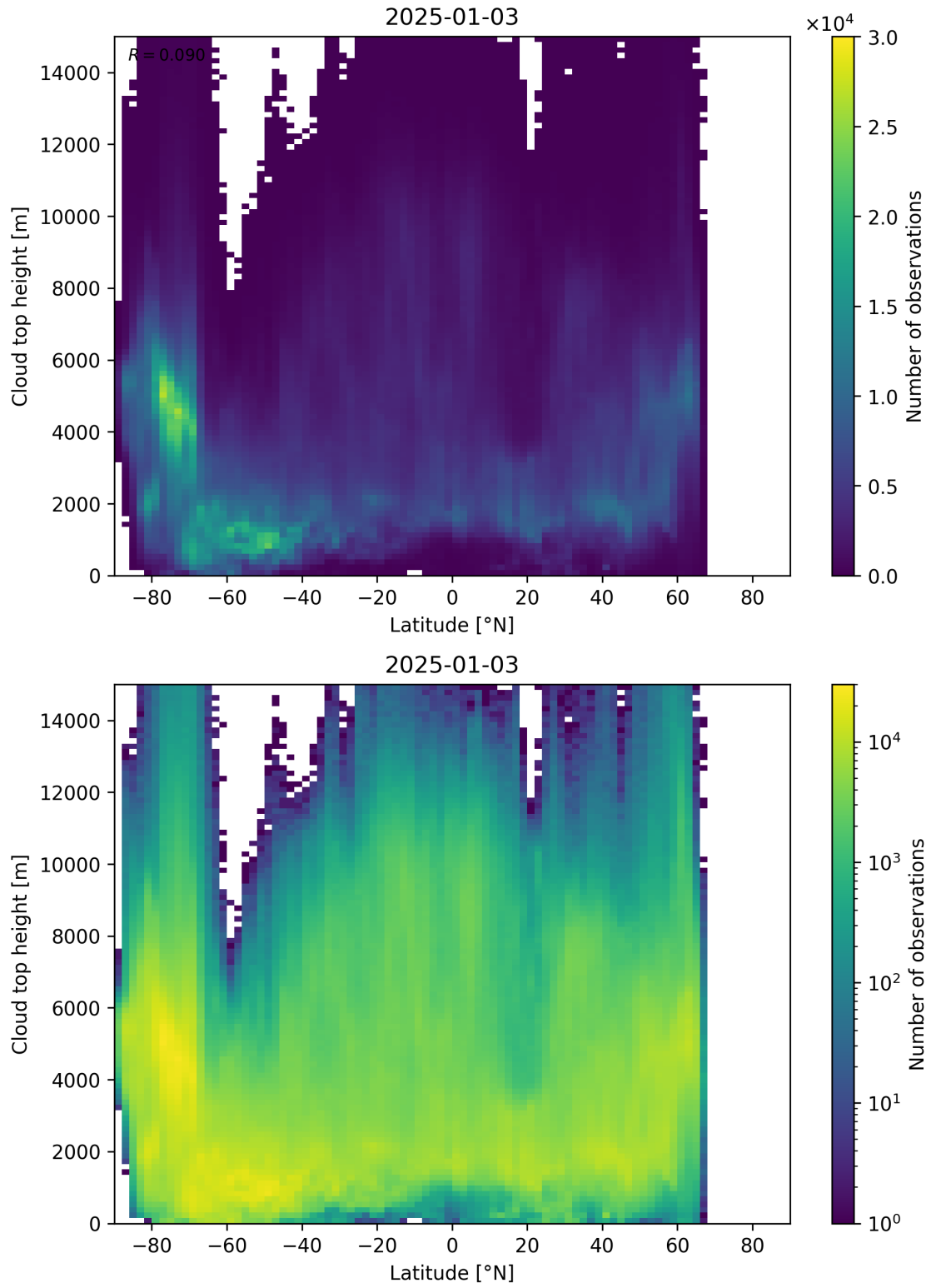
Figure 97: Scatter density plot of “Latitude” against “Cloud top height” for 2025-01-02 to 2025-01-04.
