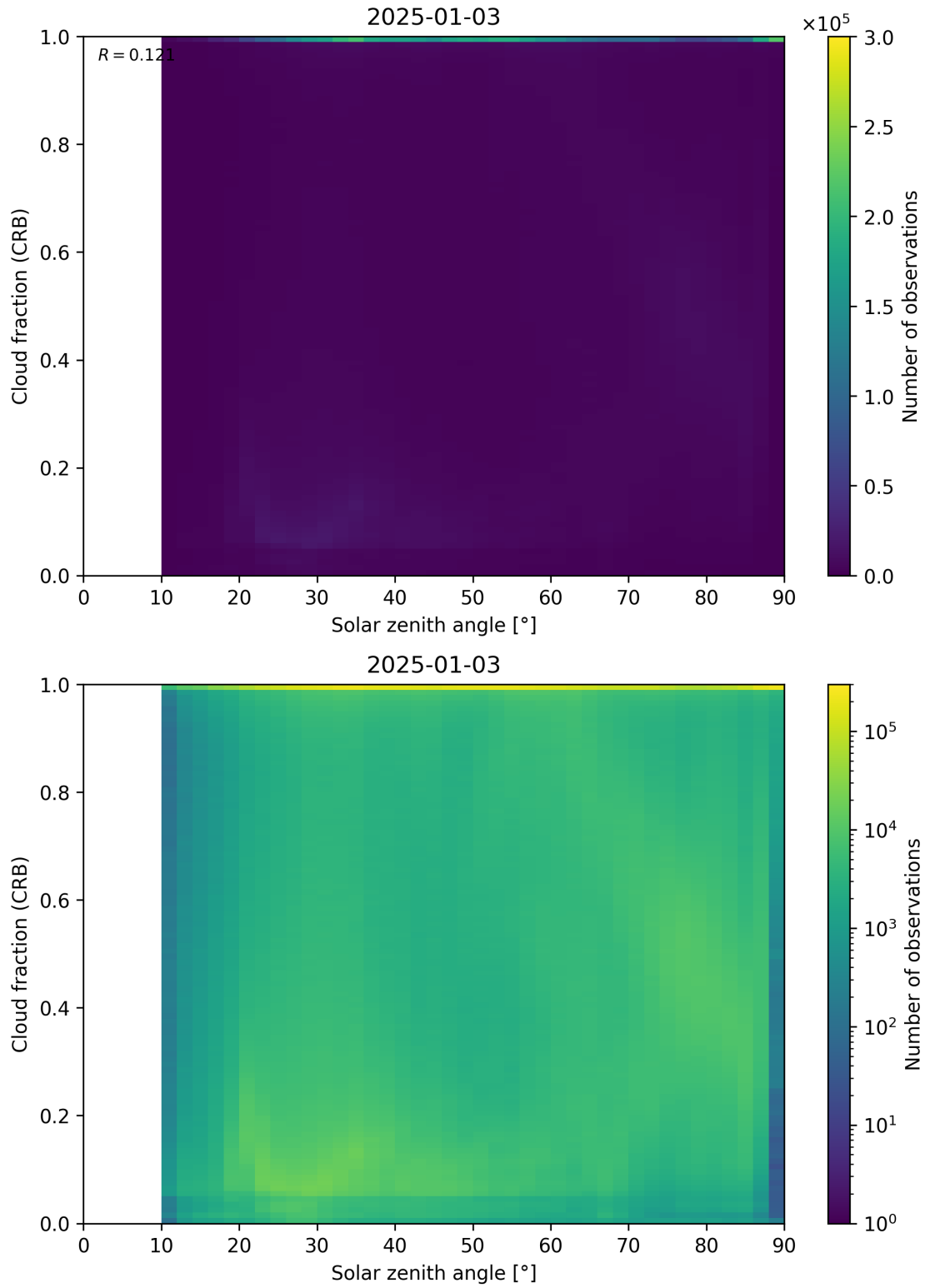
Figure 101: Scatter density plot of “Solar zenith angle” against “Cloud fraction (CRB)” for 2025-01-02 to 2025-01-04.
