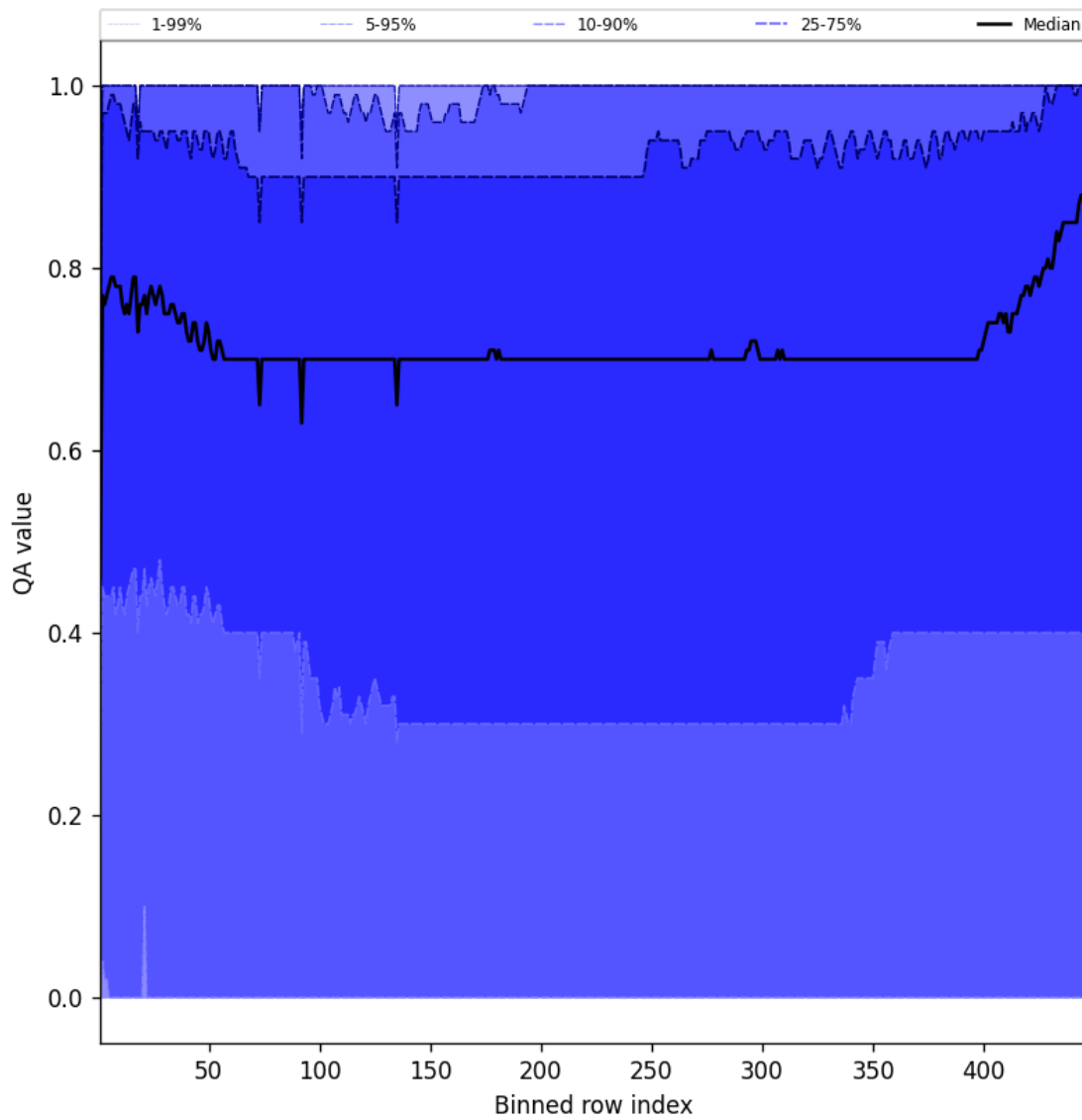
Figure 54: Along track statistics of “QA value” for 2025-01-02 to 2025-01-04
