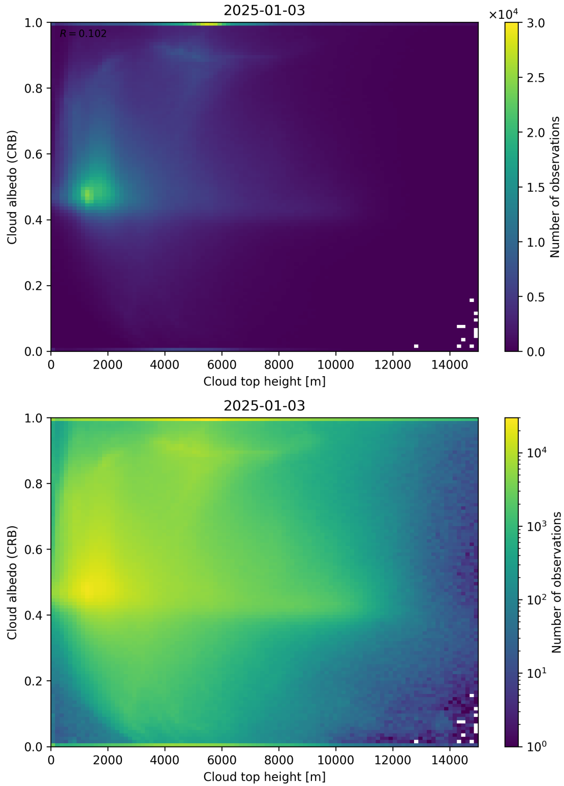
Figure 86: Scatter density plot of “Cloud top height” against “Cloud albedo (CRB)” for 2025-01-02 to 2025-01-04.
