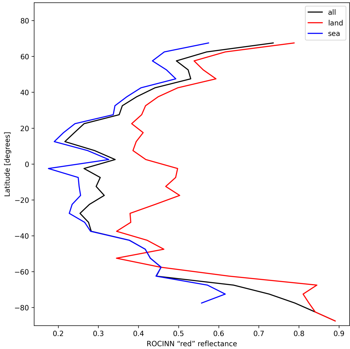
Figure 37: Zonal average of “ROCINN “red” reflectance” for 2025-01-02 to 2025-01-04.
