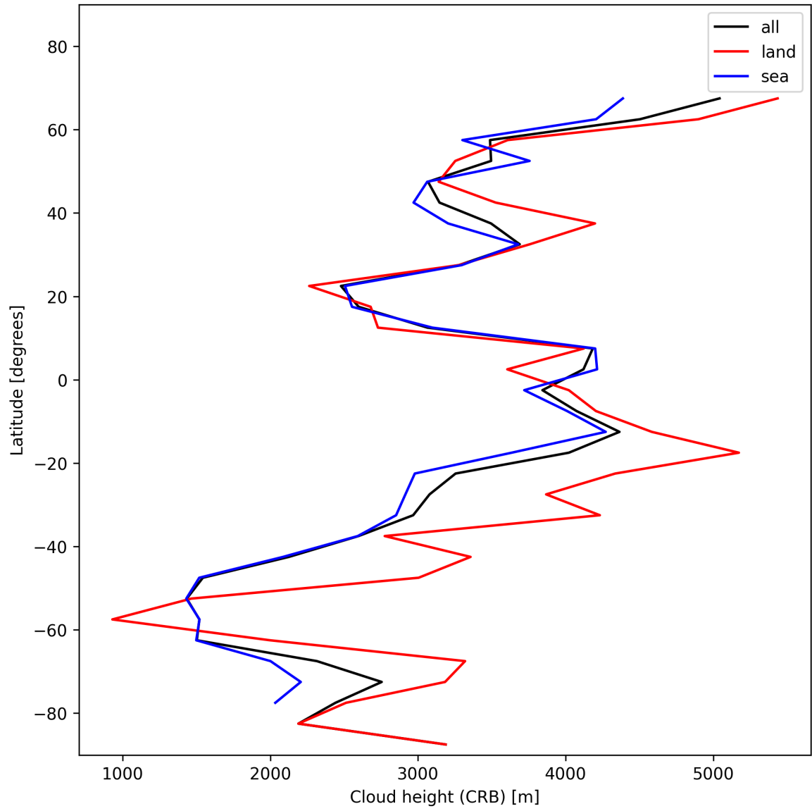
Figure 27: Zonal average of “Cloud height (CRB)” for 2025-01-02 to 2025-01-04.
