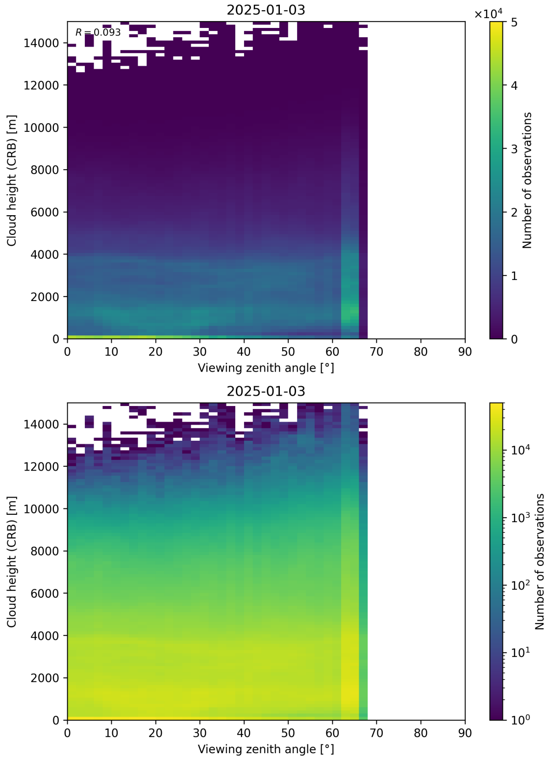
Figure 110: Scatter density plot of “Viewing zenith angle” against “Cloud height (CRB)” for 2025-01-02 to 2025-01-04.
