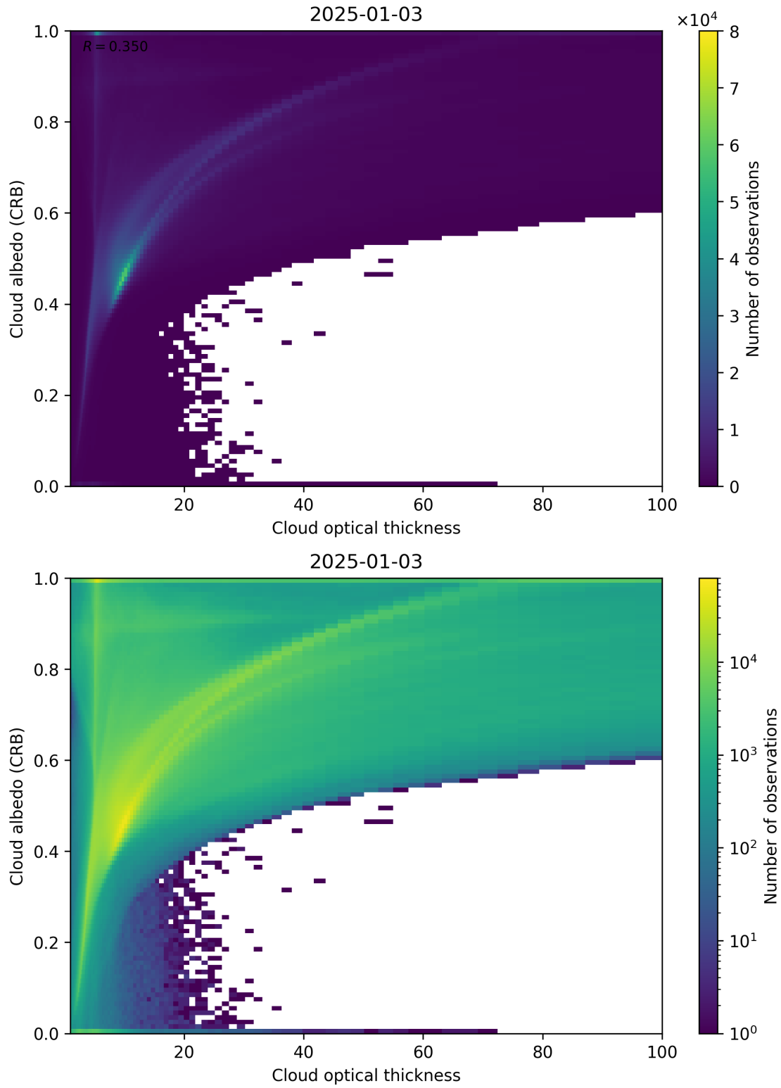
Figure 82: Scatter density plot of “Cloud optical thickness” against “Cloud albedo (CRB)” for 2025-01-02 to 2025-01-04.
