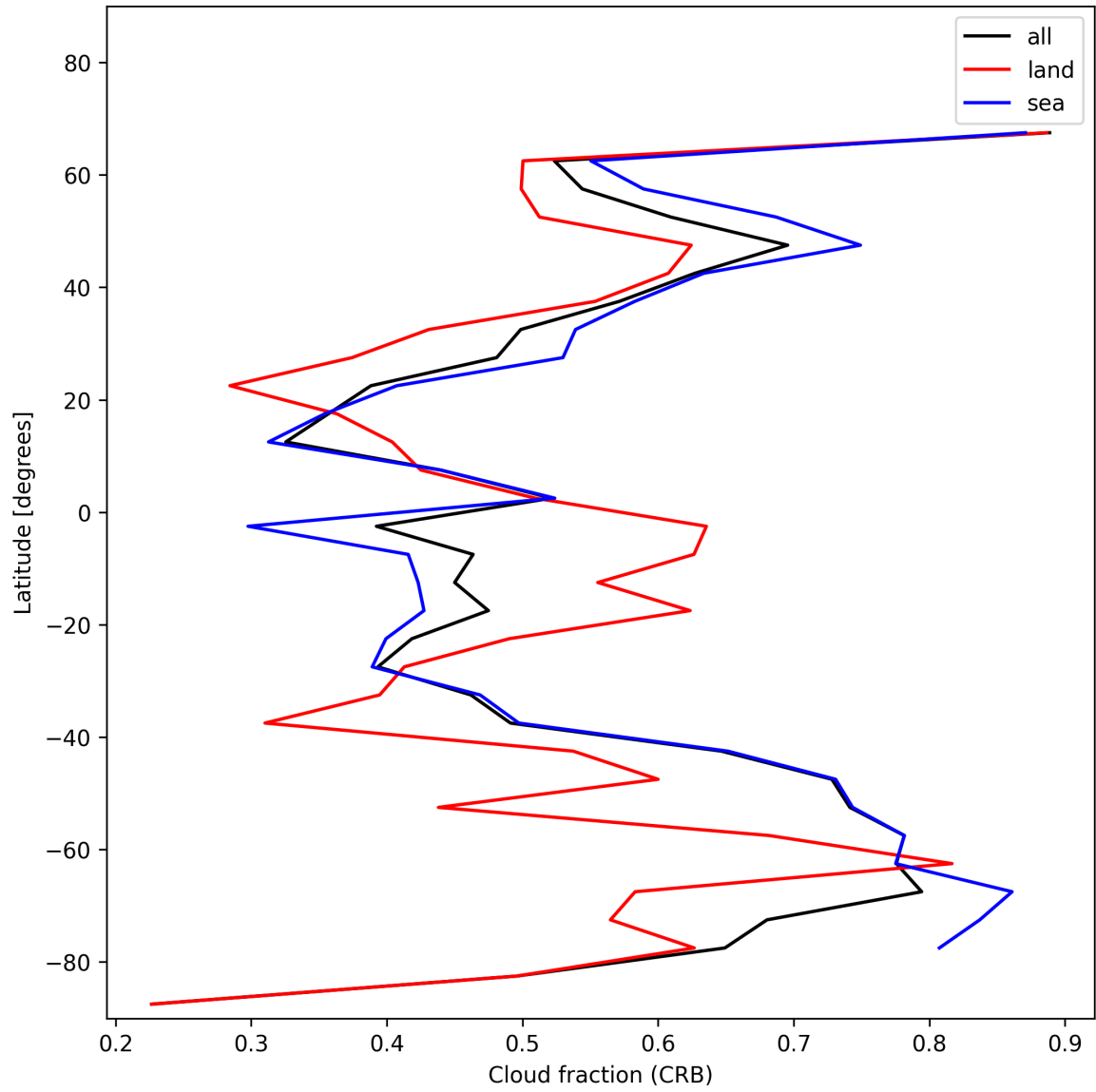
Figure 26: Zonal average of “Cloud fraction (CRB)” for 2025-01-02 to 2025-01-04.
