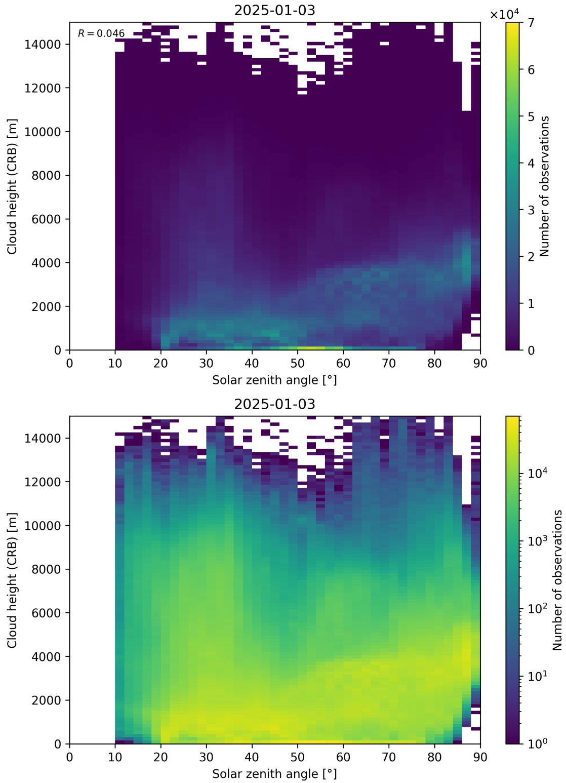
Figure 102: Scatter density plot of “Solar zenith angle” against “Cloud height (CRB)” for 2025-01-02 to 2025-01-04.
