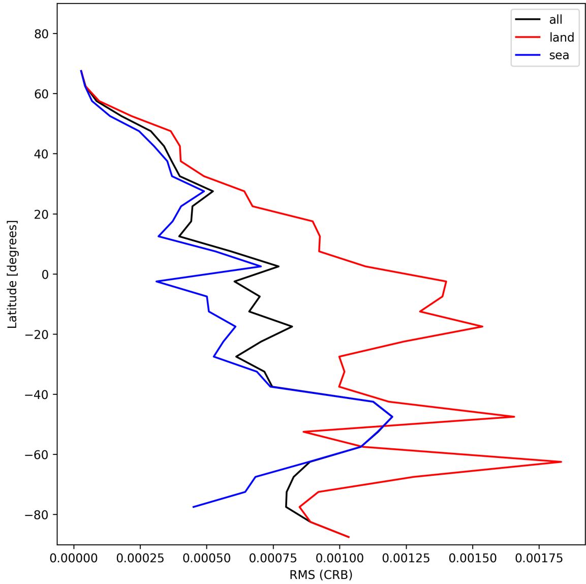
Figure 32: Zonal average of “RMS (CRB)” for 2025-01-02 to 2025-01-04.
