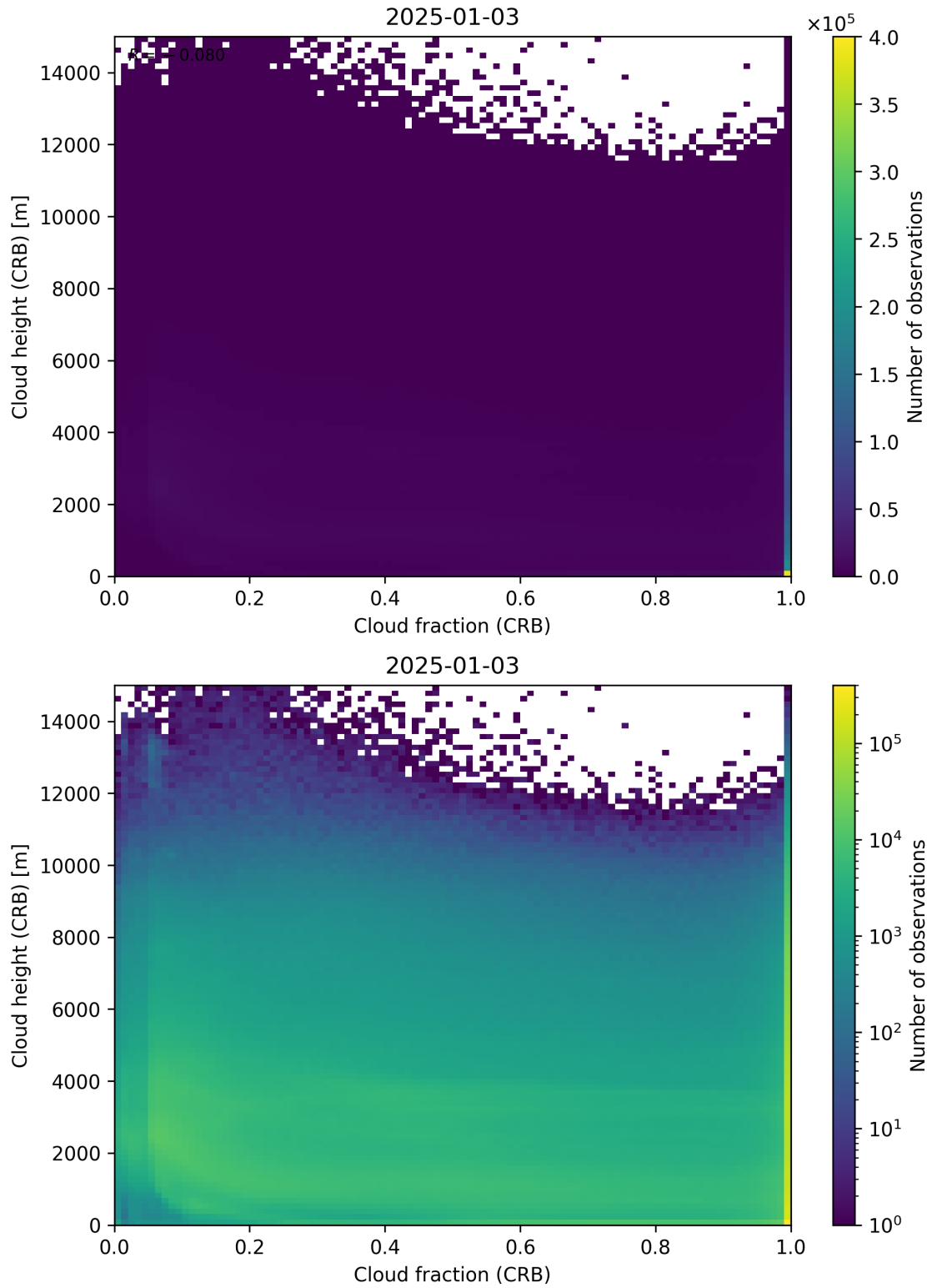
Figure 79: Scatter density plot of “Cloud fraction (CRB)” against “Cloud height (CRB)” for 2025-01-02 to 2025-01-04.
