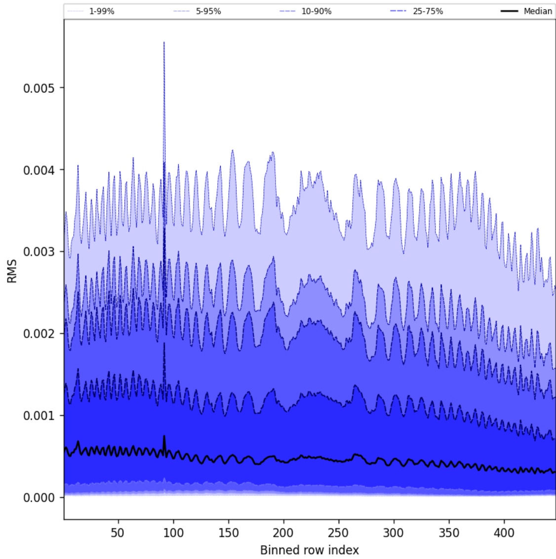
Figure 63: Along track statistics of “RMS” for 2025-01-02 to 2025-01-04
