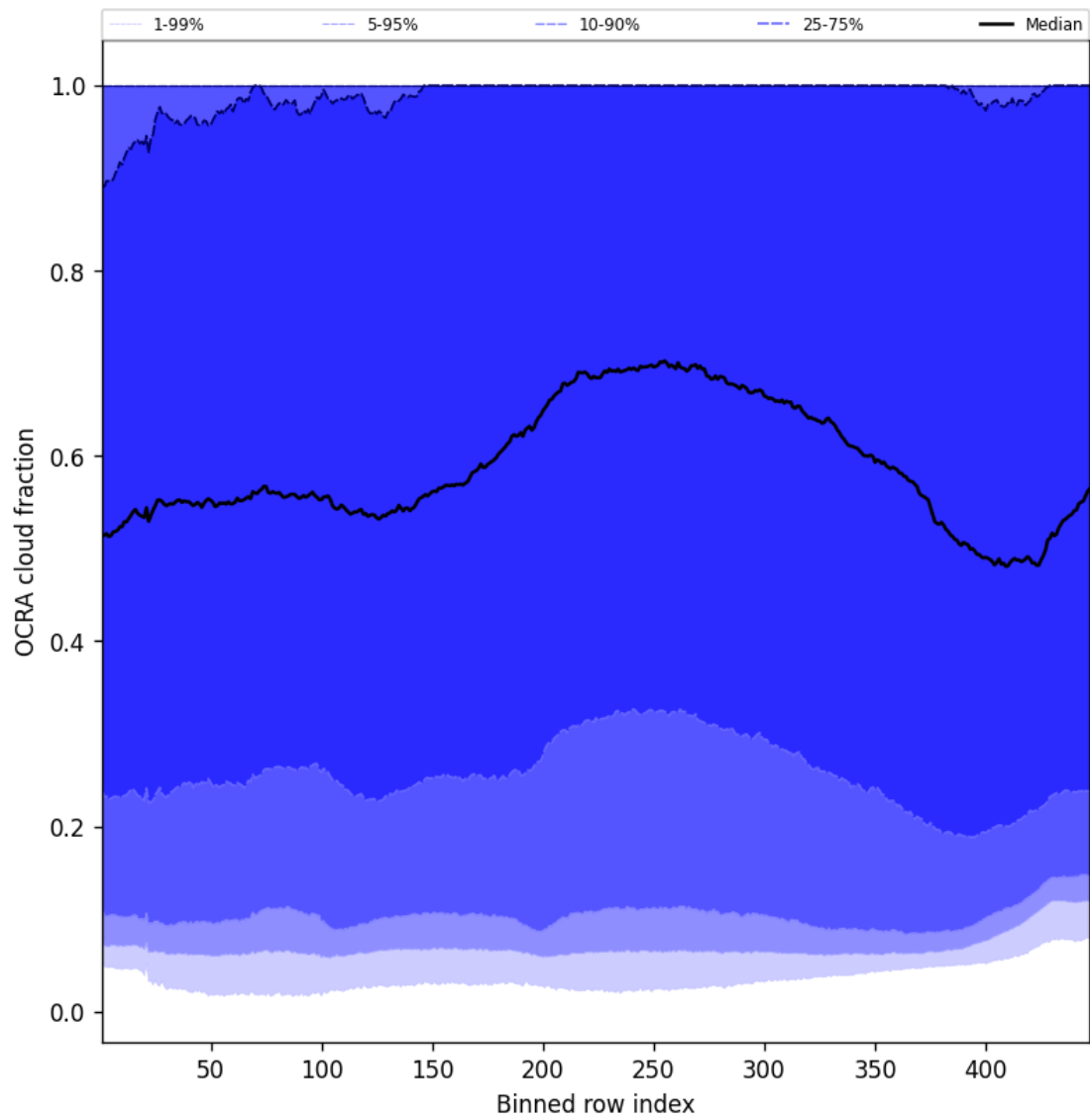
Figure 66: Along track statistics of “OCRA cloud fraction” for 2025-01-02 to 2025-01-04
