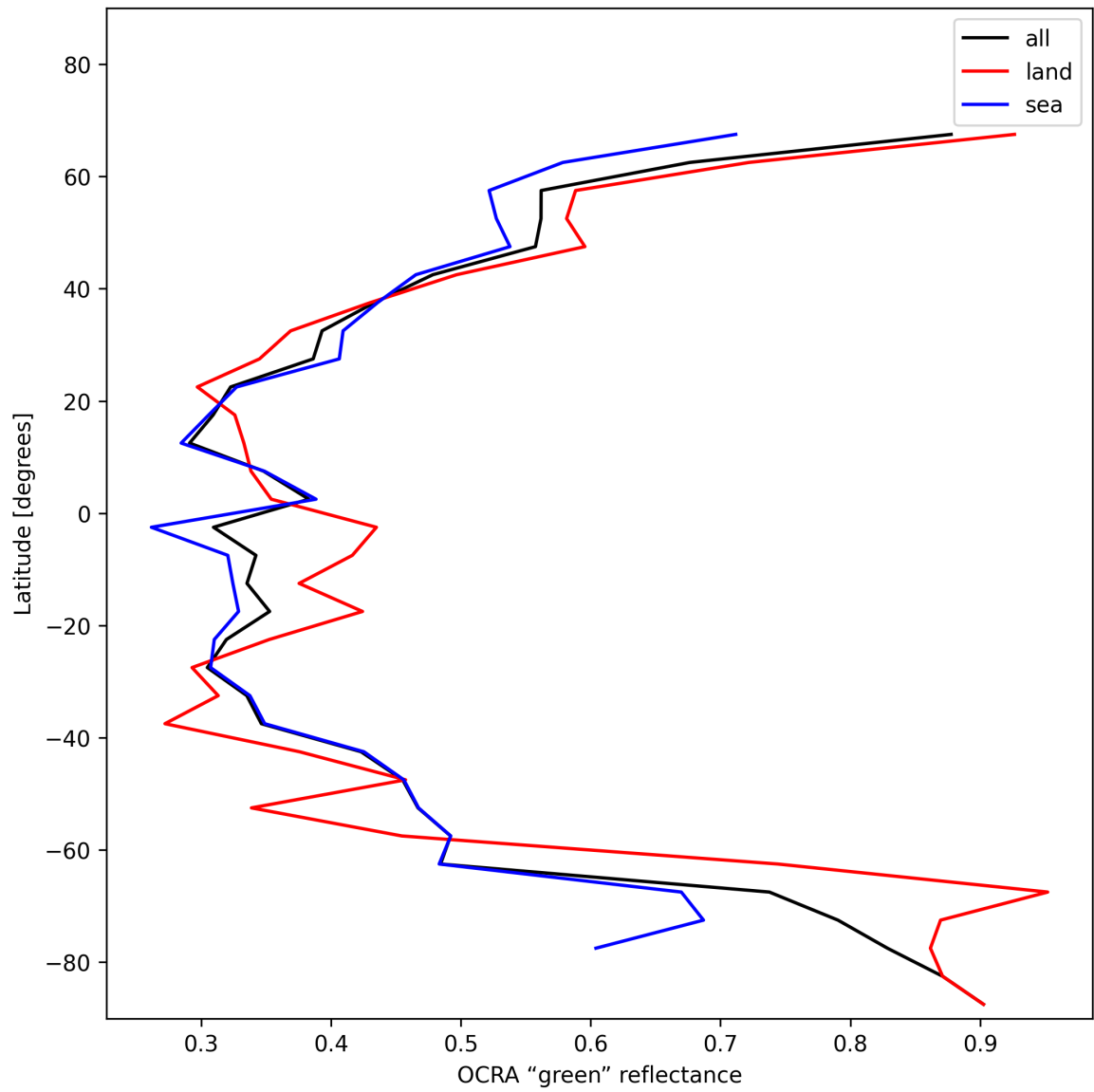
Figure 36: Zonal average of “OCRA “green” reflectance” for 2025-01-02 to 2025-01-04.
