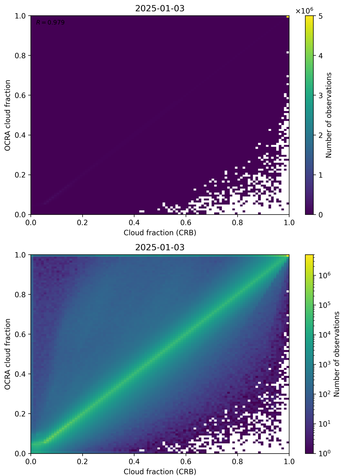
Figure 78: Scatter density plot of “Cloud fraction (CRB)” against “OCRA cloud fraction” for 2025-01-02 to 2025-01-04.
