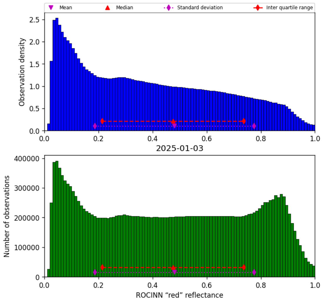
Figure 53: Histogram of “ROCINN “red” reflectance” for 2025-01-02 to 2025-01-04
