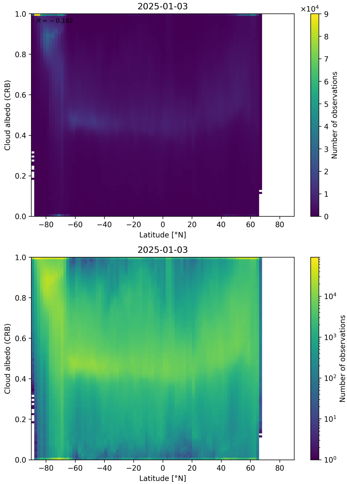
Figure 91: Scatter density plot of “Latitude” against “Cloud albedo (CRB)” for 2025-01-02 to 2025-01-04.
