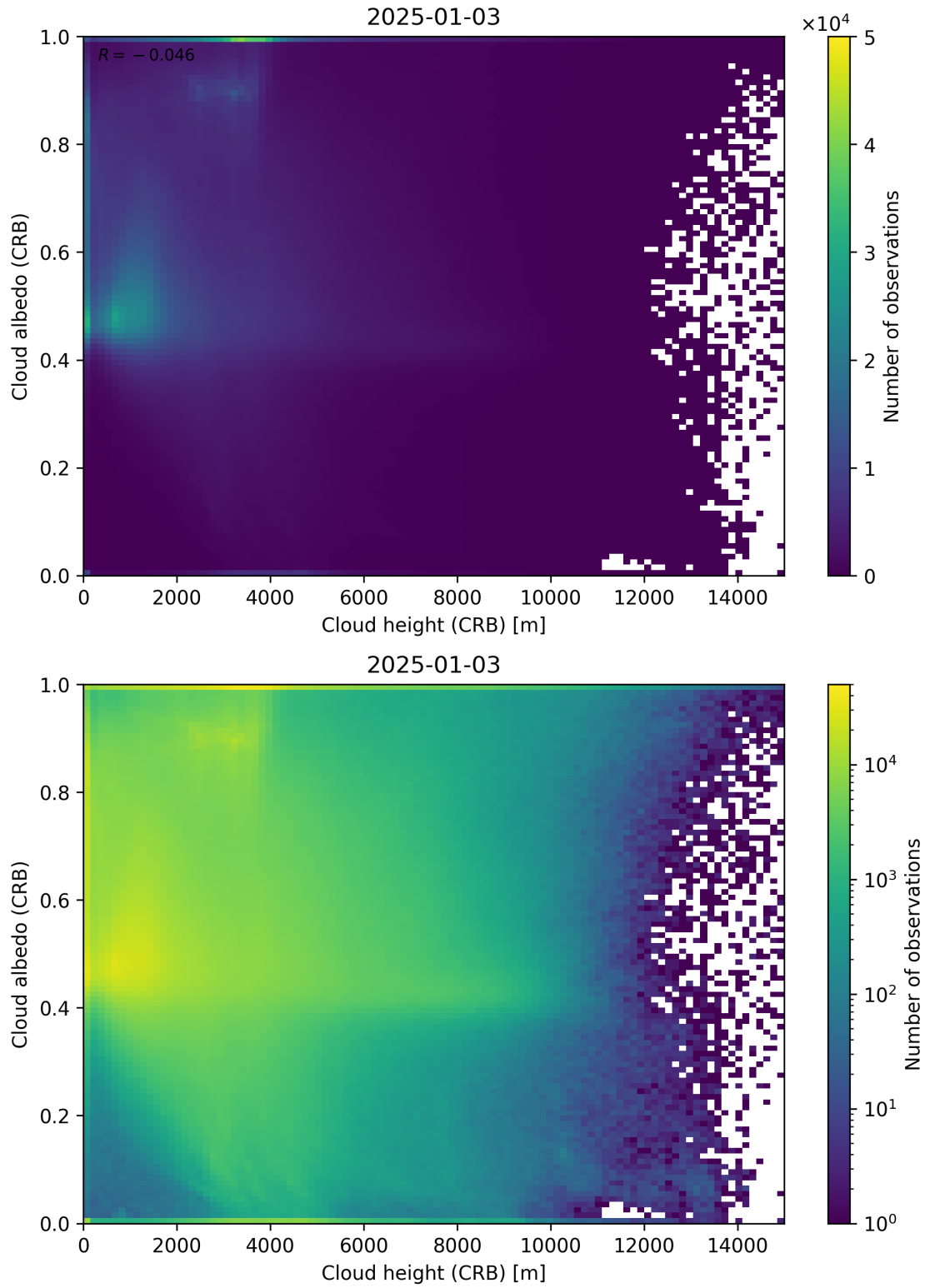
Figure 80: Scatter density plot of “Cloud height (CRB)” against “Cloud albedo (CRB)” for 2025-01-02 to 2025-01-04.
