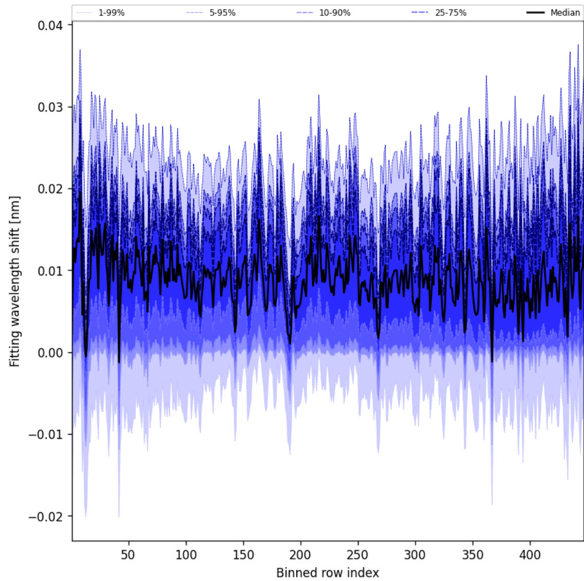
Figure 65: Along track statistics of “Fitting wavelength shift” for 2025-01-02 to 2025-01-04
