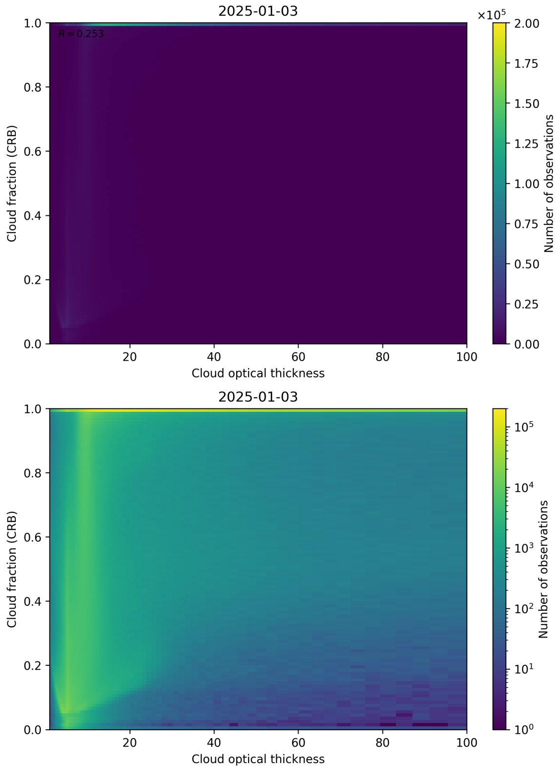
Figure 84: Scatter density plot of “Cloud optical thickness” against “Cloud fraction (CRB)” for 2025-01-02 to 2025-01-04.
