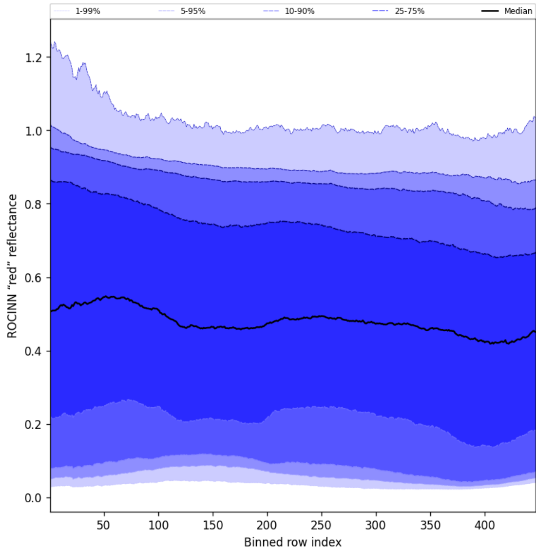
Figure 69: Along track statistics of “ROCINN “red” reflectance” for 2025-01-02 to 2025-01-04
