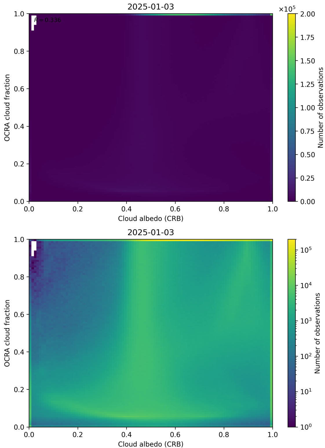
Figure 70: Scatter density plot of “Cloud albedo (CRB)” against “OCRA cloud fraction” for 2025-01-02 to 2025-01-04.
