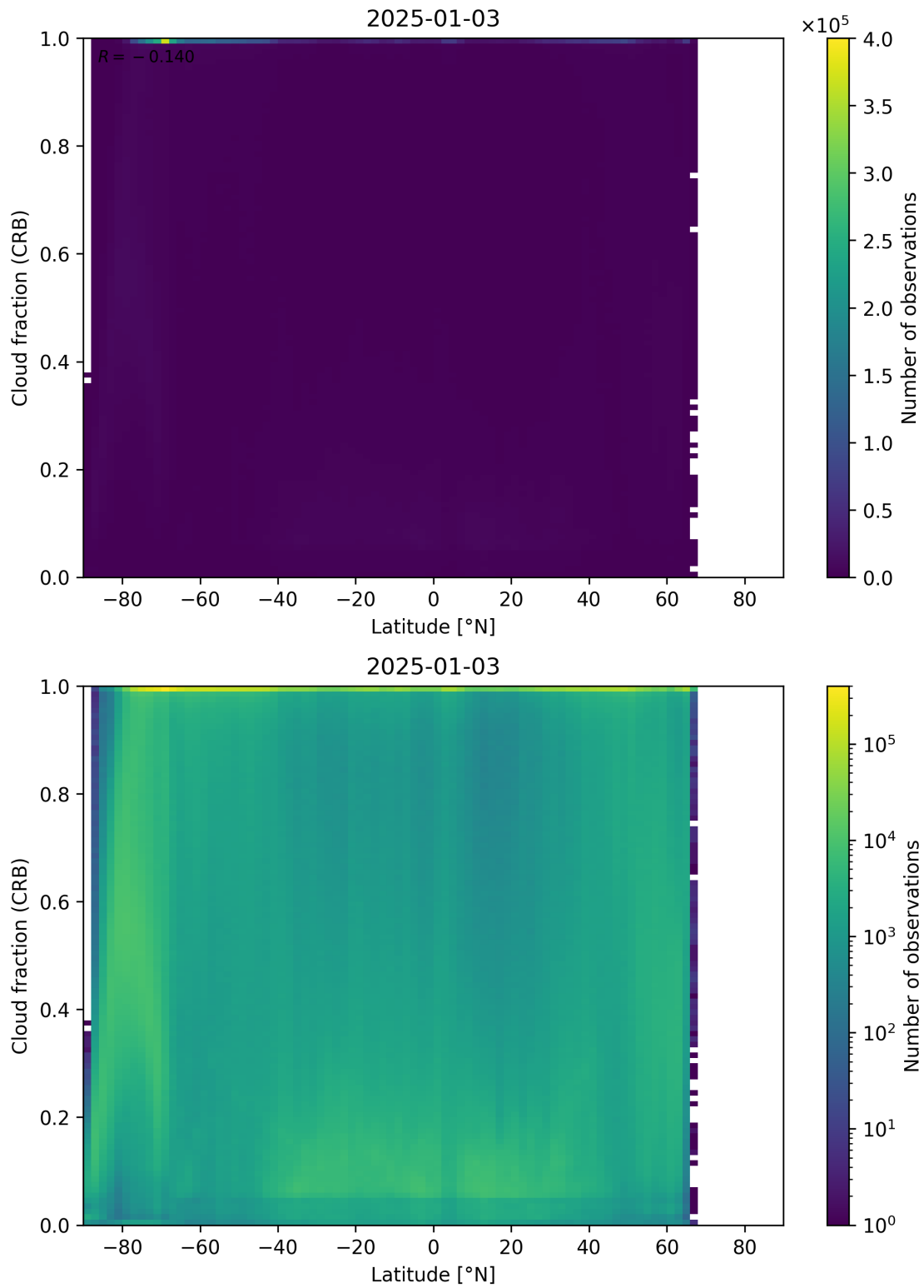
Figure 94: Scatter density plot of “Latitude” against “Cloud fraction (CRB)” for 2025-01-02 to 2025-01-04.
