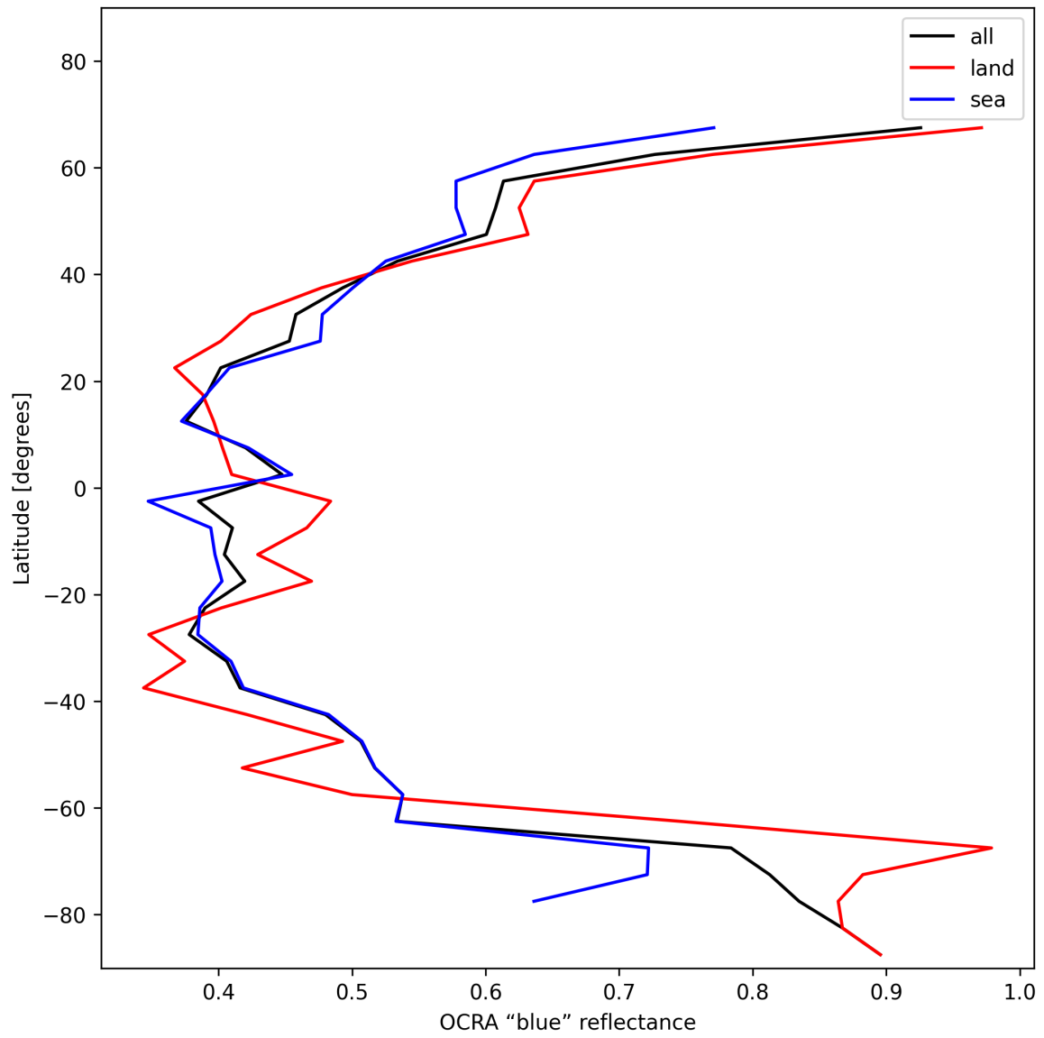
Figure 35: Zonal average of “OCRA “blue” reflectance” for 2025-01-02 to 2025-01-04.
