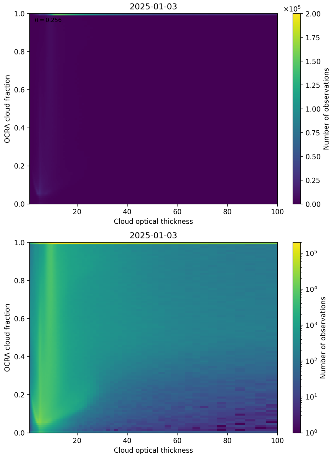
Figure 83: Scatter density plot of “Cloud optical thickness” against “OCRA cloud fraction” for 2025-01-02 to 2025-01-04.
