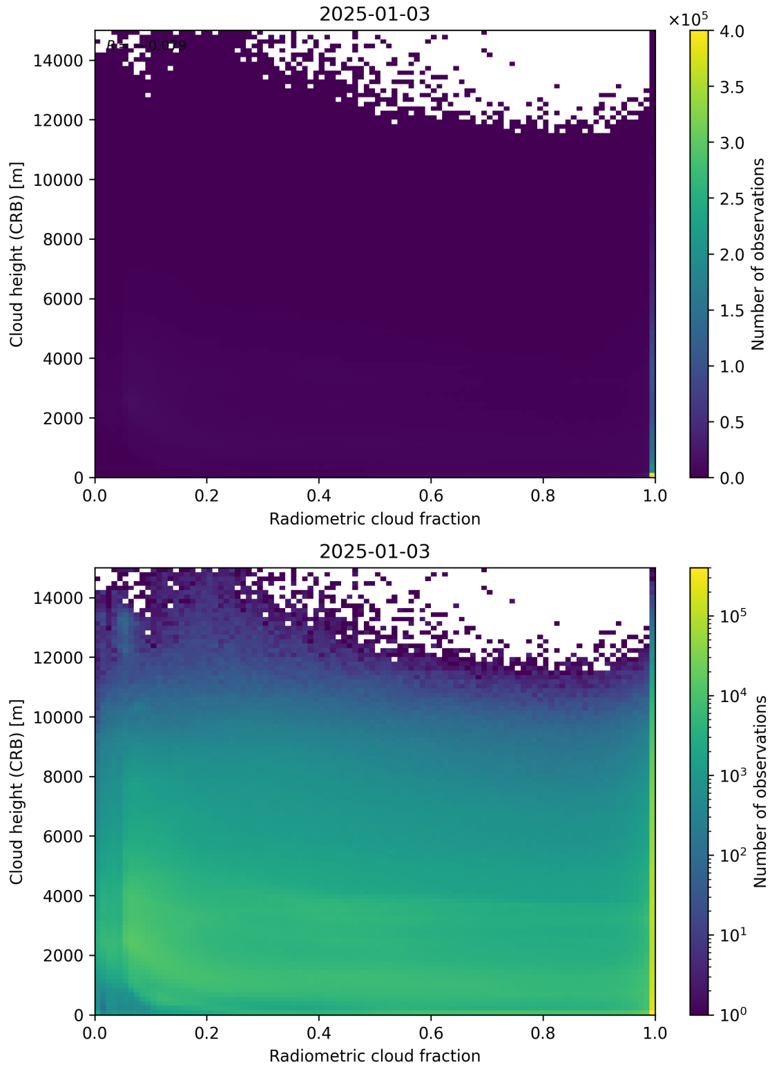
Figure 74: Scatter density plot of “Radiometric cloud fraction” against “Cloud height (CRB)” for 2025-01-02 to 2025-01-04.
