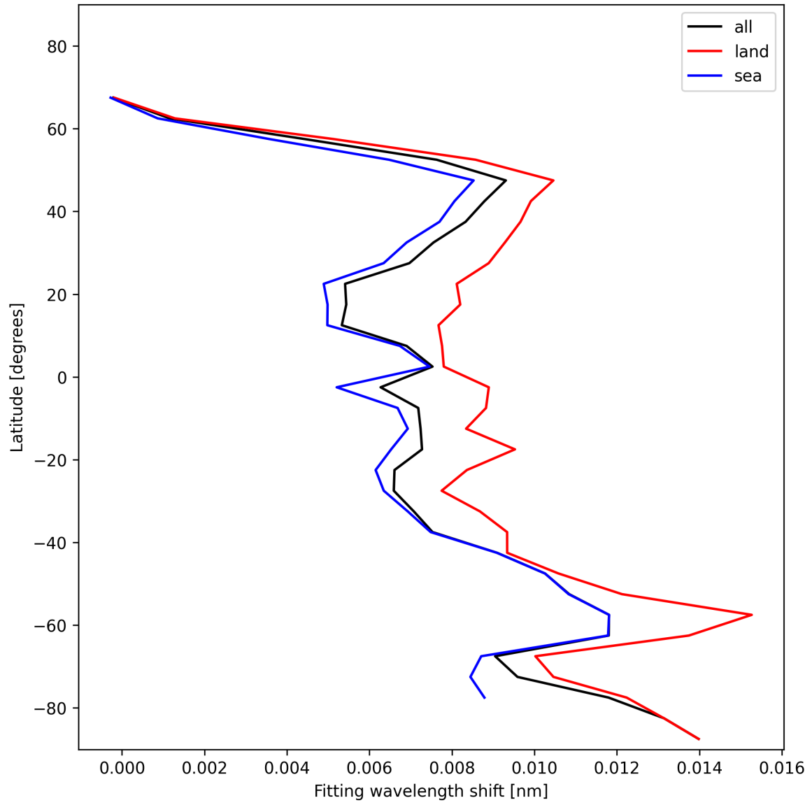
Figure 33: Zonal average of “Fitting wavelength shift” for 2025-01-02 to 2025-01-04.
