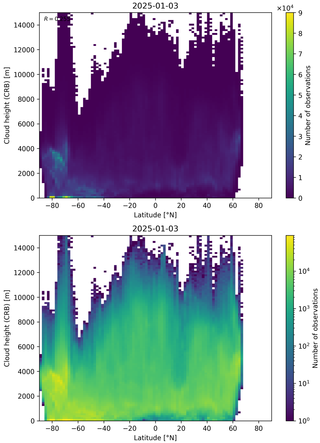
Figure 95: Scatter density plot of “Latitude” against “Cloud height (CRB)” for 2025-01-02 to 2025-01-04.
