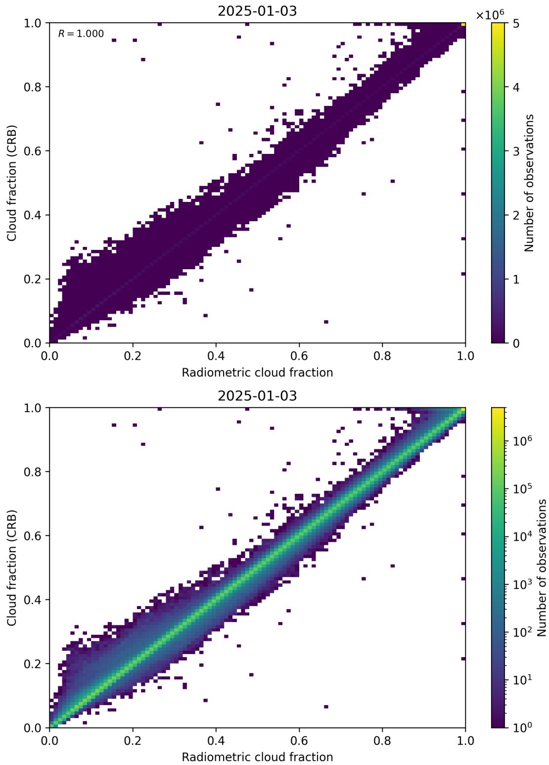
Figure 73: Scatter density plot of “Radiometric cloud fraction” against “Cloud fraction (CRB)” for 2025-01-02 to 2025-01-04.
