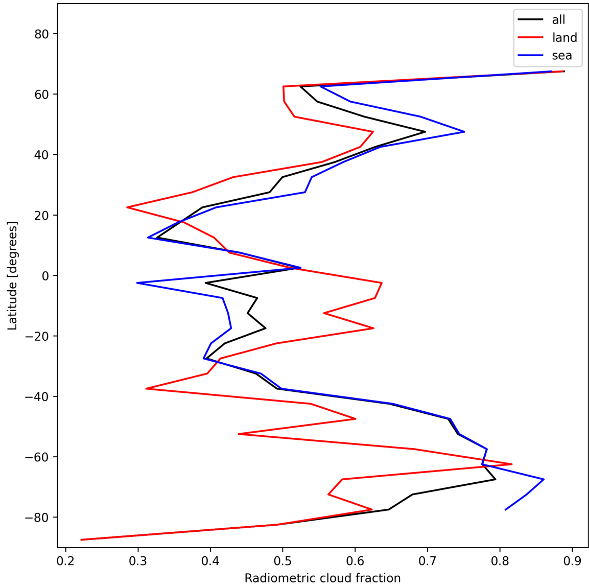
Figure 23: Zonal average of “Radiometric cloud fraction” for 2025-01-02 to 2025-01-04.
