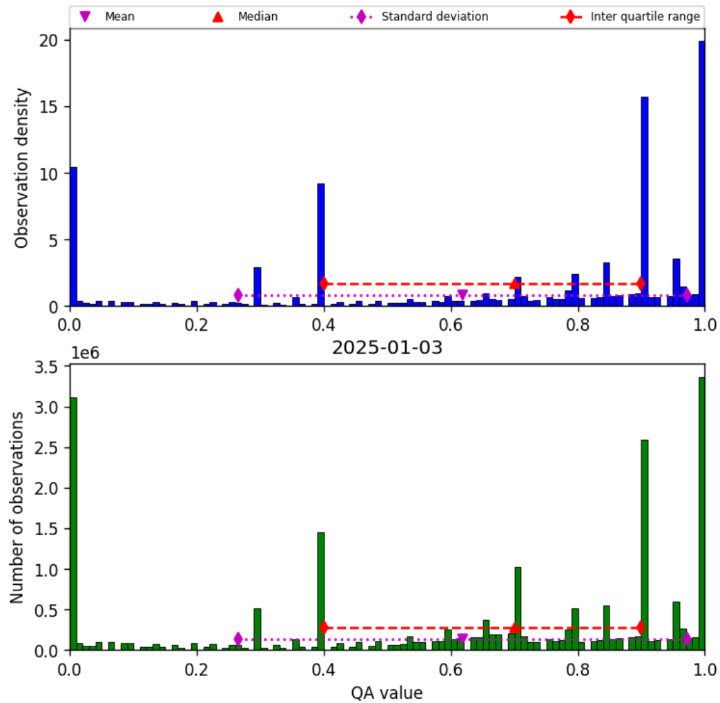
Figure 38: Histogram of “QA value” for 2025-01-02 to 2025-01-04
