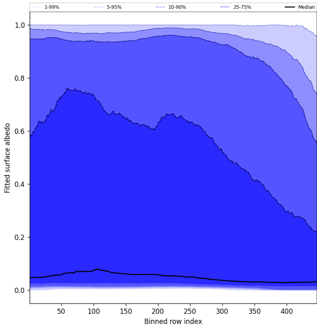
Figure 61: Along track statistics of “Fitted surface albedo” for 2025-01-02 to 2025-01-04
