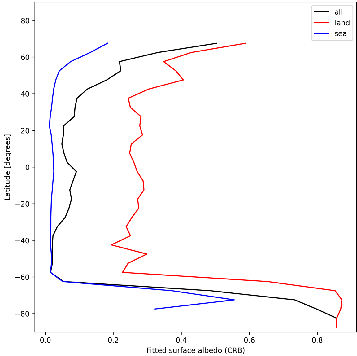
Figure 30: Zonal average of “Fitted surface albedo (CRB)” for 2025-01-02 to 2025-01-04.
