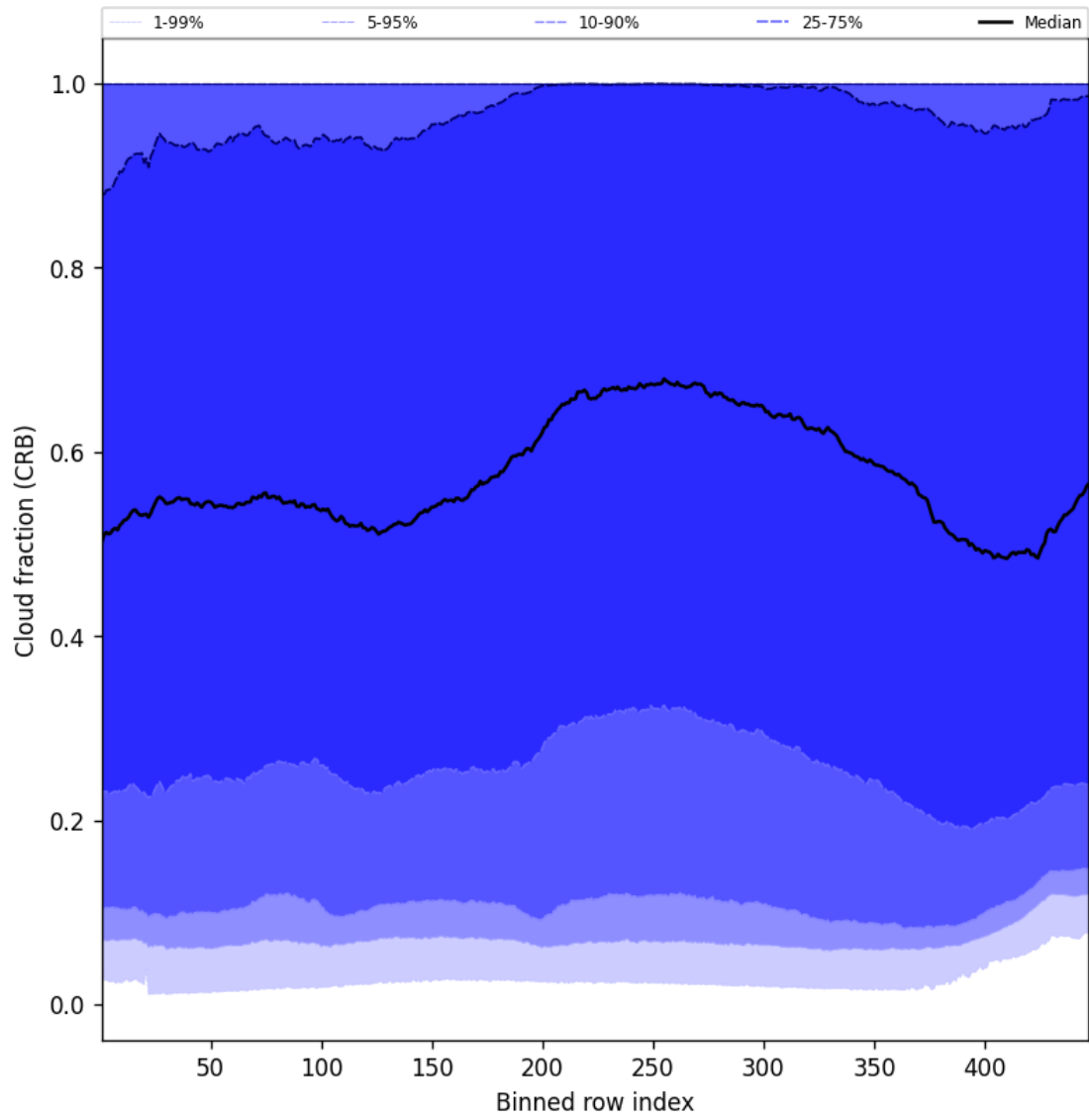
Figure 58: Along track statistics of “Cloud fraction (CRB)” for 2025-01-02 to 2025-01-04
