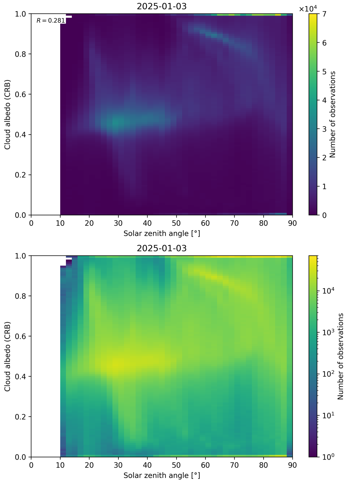
Figure 98: Scatter density plot of “Solar zenith angle” against “Cloud albedo (CRB)” for 2025-01-02 to 2025-01-04.
