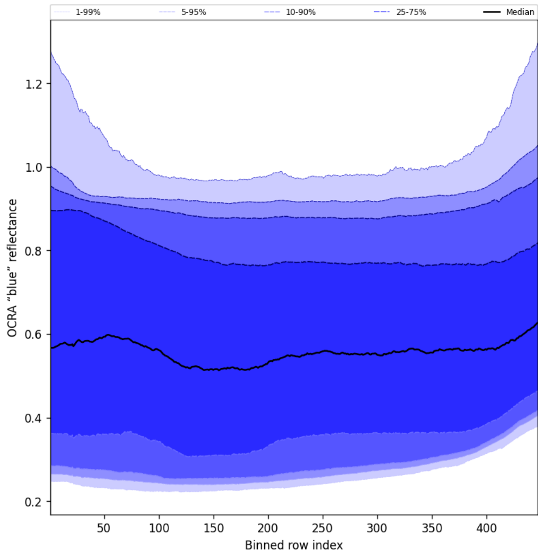
Figure 67: Along track statistics of "OCRA "blue" reflectance" for 2025-01-02 to 2025-01-04
