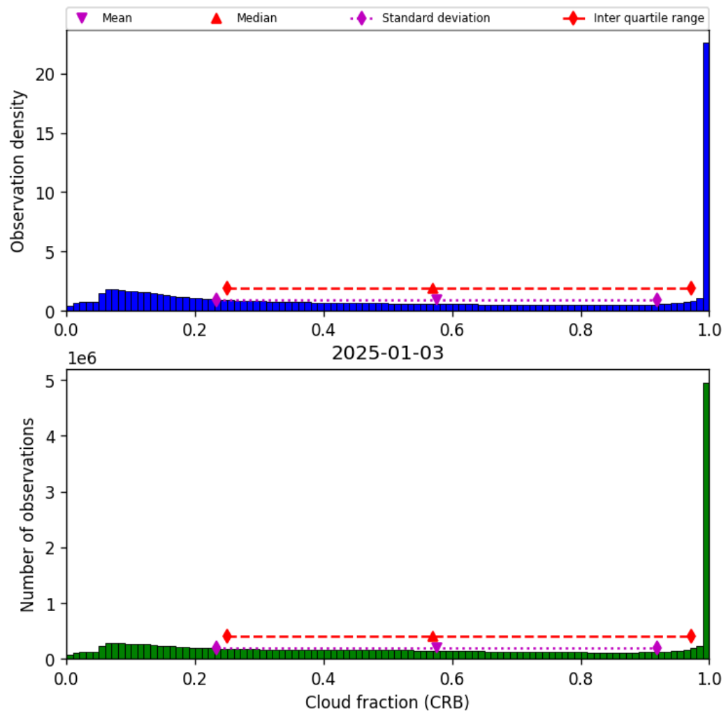
Figure 42: Histogram of “Cloud fraction (CRB)” for 2025-01-02 to 2025-01-04
