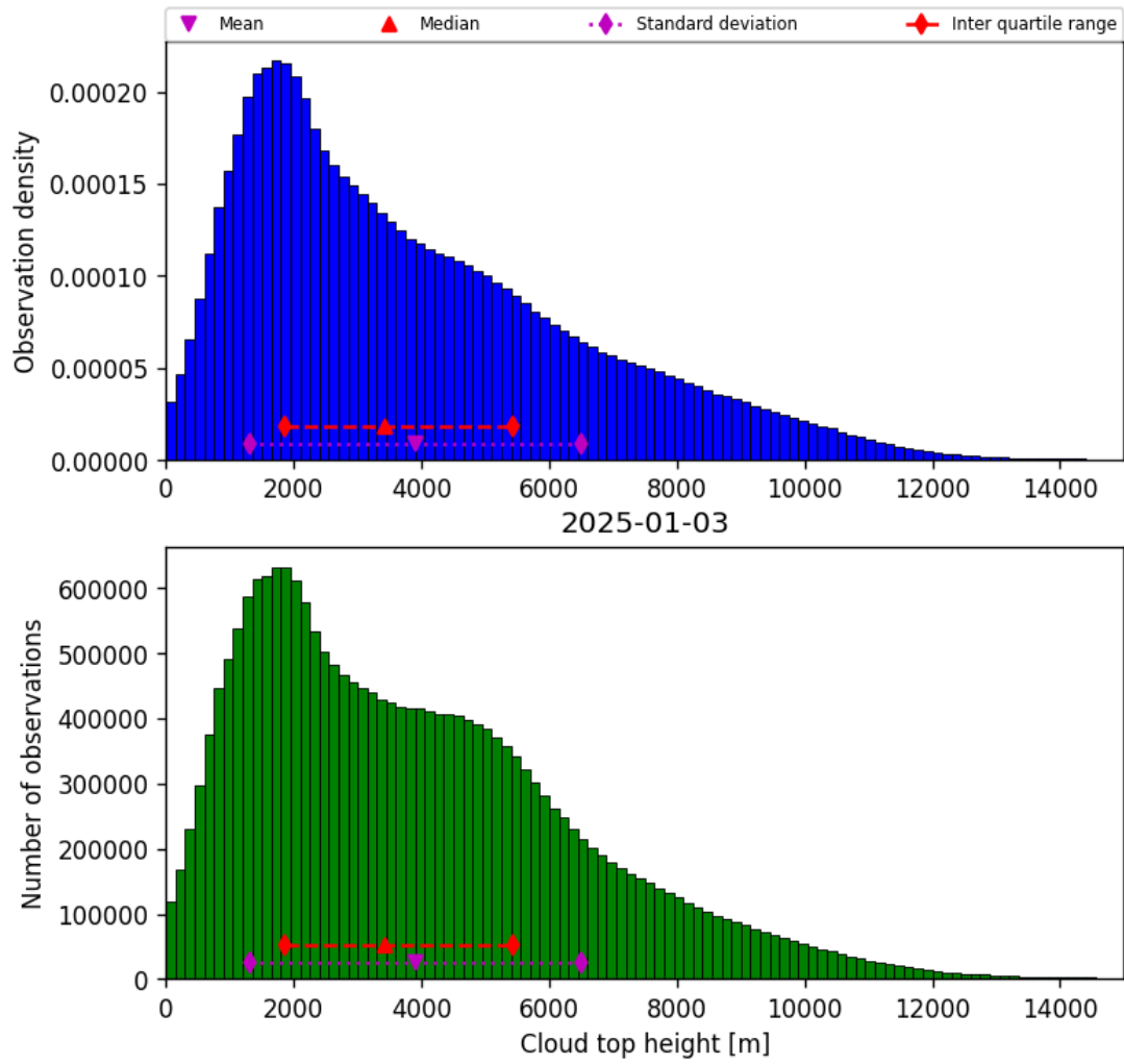
Figure 40: Histogram of “Cloud top height” for 2025-01-02 to 2025-01-04
