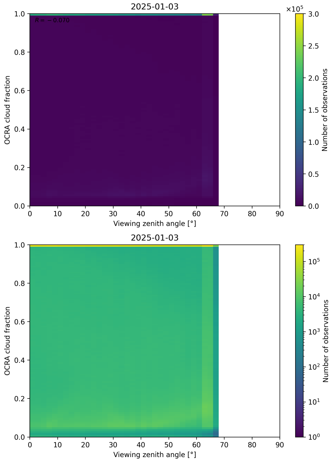
Figure 108: Scatter density plot of “Viewing zenith angle” against “OCRA cloud fraction” for 2025-01-02 to 2025-01-04.
