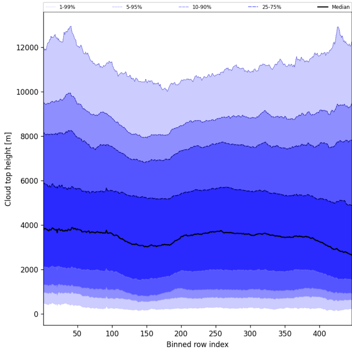
Figure 56: Along track statistics of “Cloud top height” for 2025-01-02 to 2025-01-04
