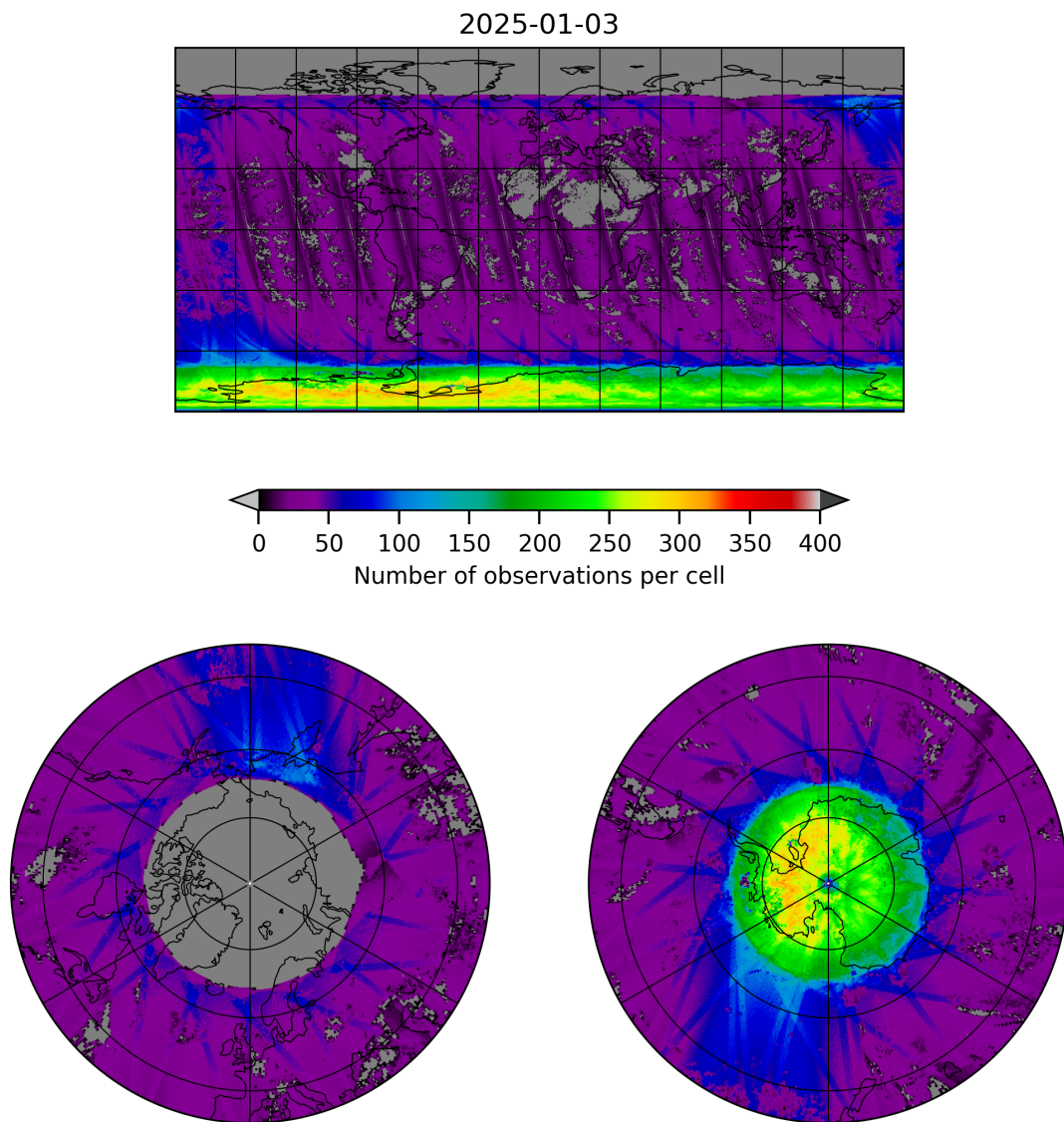
Figure 21: Map of the number of observations for 2025-01-02 to 2025-01-04
