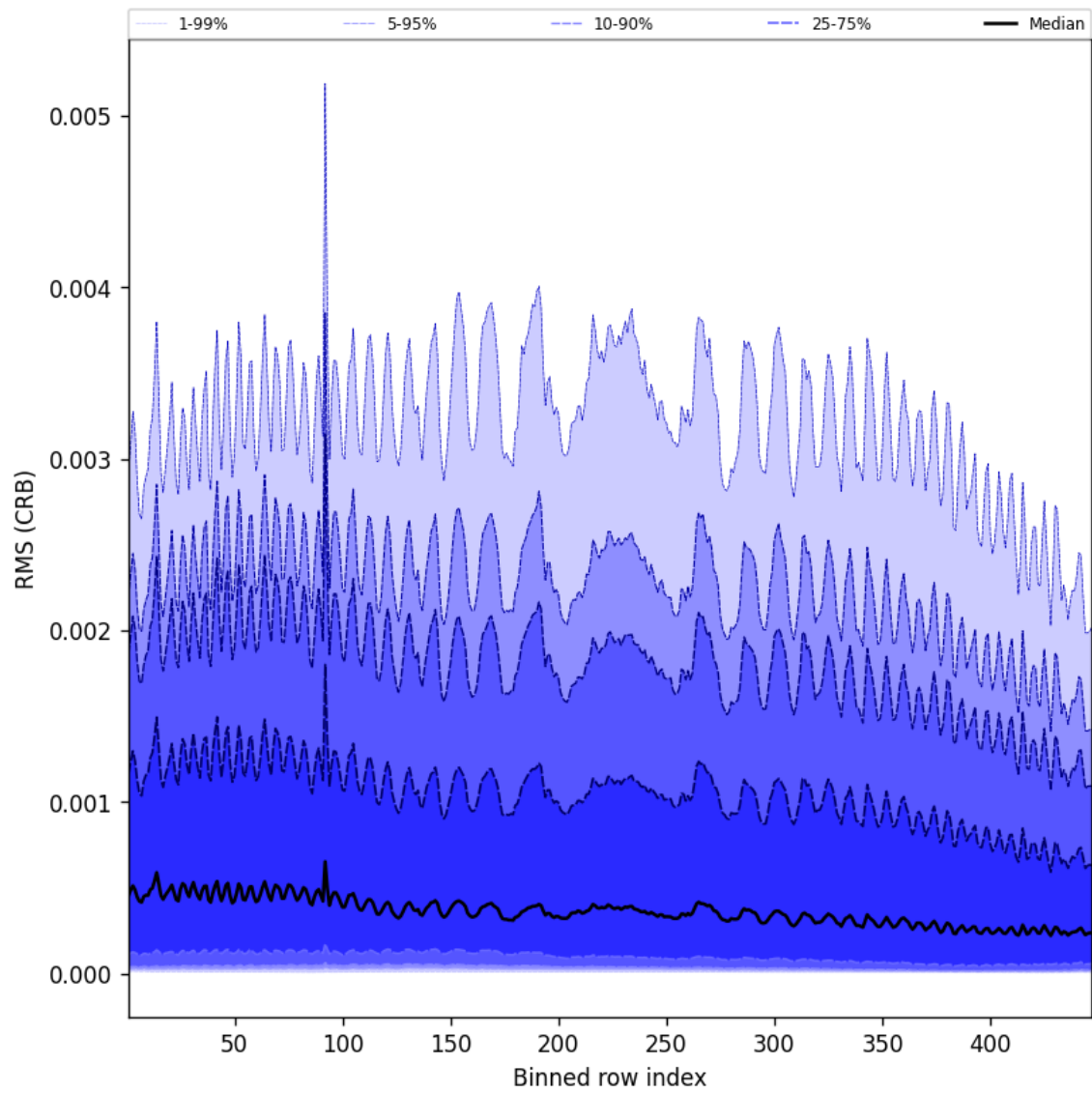
Figure 64: Along track statistics of “RMS (CRB)” for 2025-01-02 to 2025-01-04
