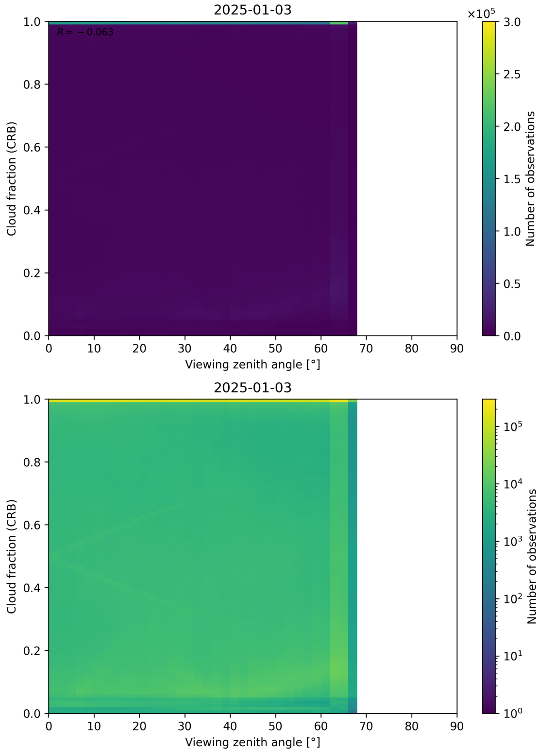
Figure 109: Scatter density plot of “Viewing zenith angle” against “Cloud fraction (CRB)” for 2025-01-02 to 2025-01-04.
