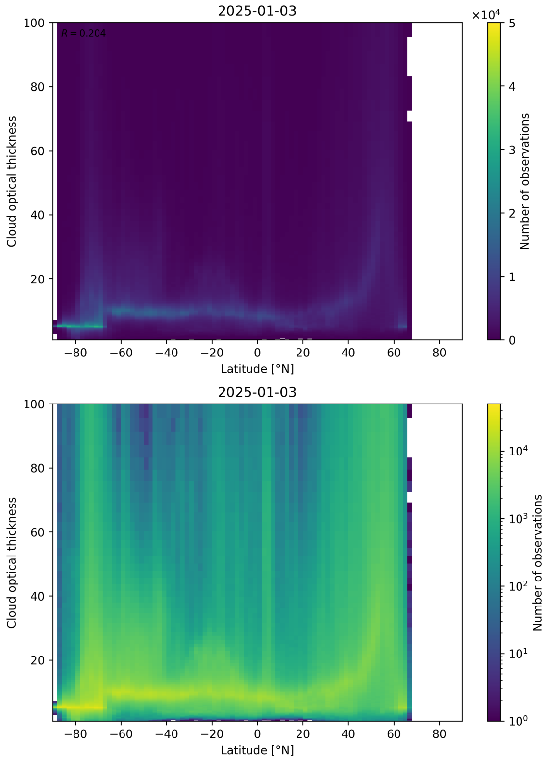
Figure 96: Scatter density plot of “Latitude” against “Cloud optical thickness” for 2025-01-02 to 2025-01-04.
