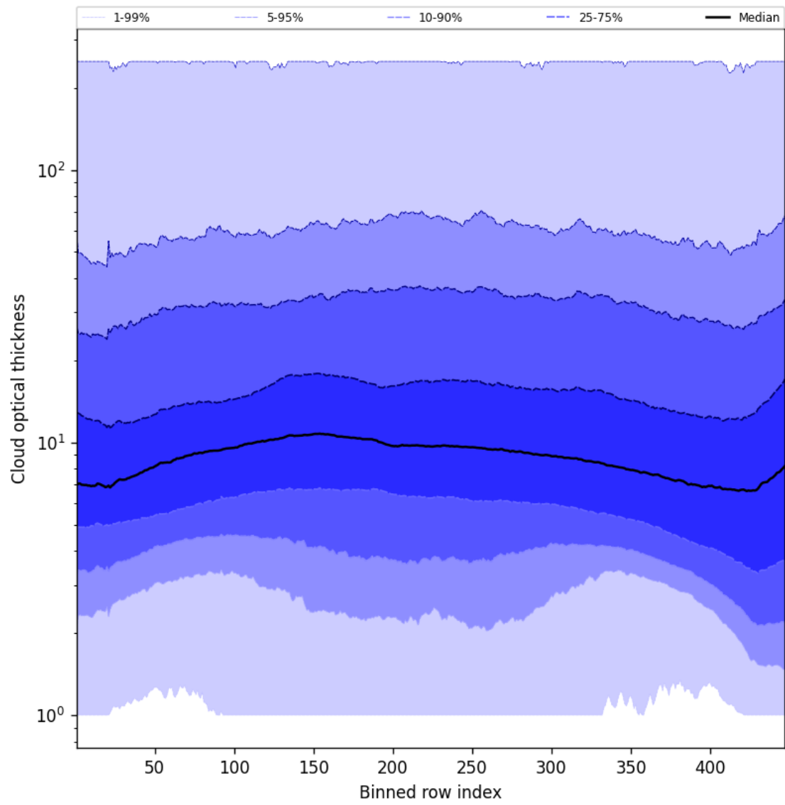
Figure 57: Along track statistics of “Cloud optical thickness” for 2025-01-02 to 2025-01-04
