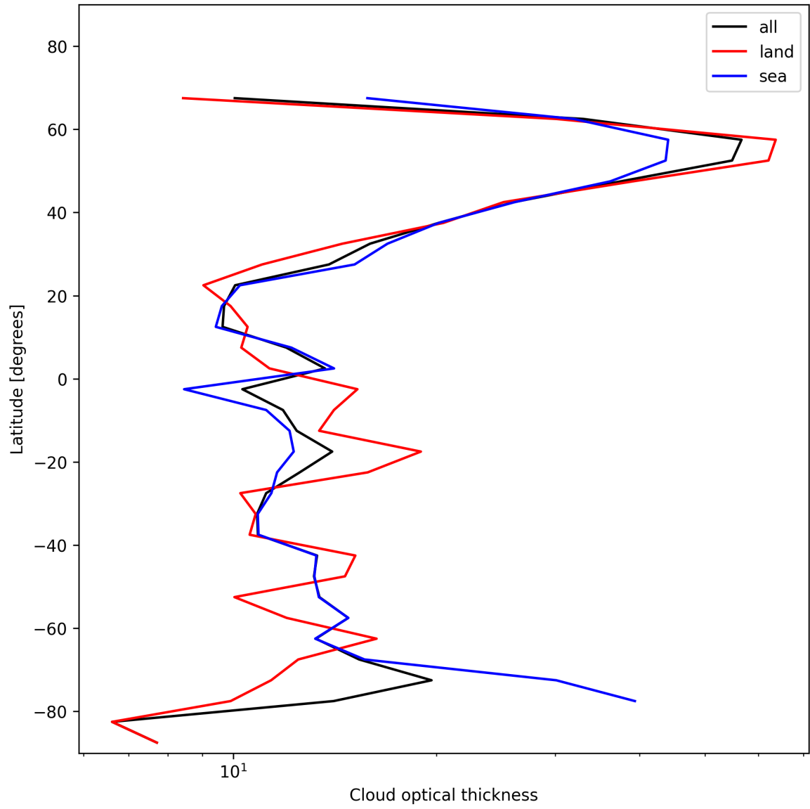
Figure 25: Zonal average of “Cloud optical thickness” for 2025-01-02 to 2025-01-04.
