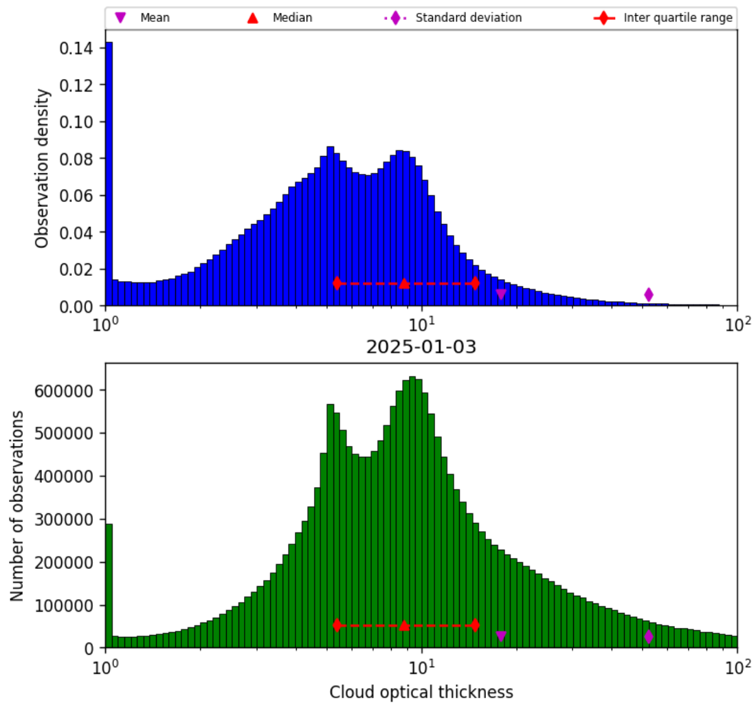
Figure 41: Histogram of “Cloud optical thickness” for 2025-01-02 to 2025-01-04
