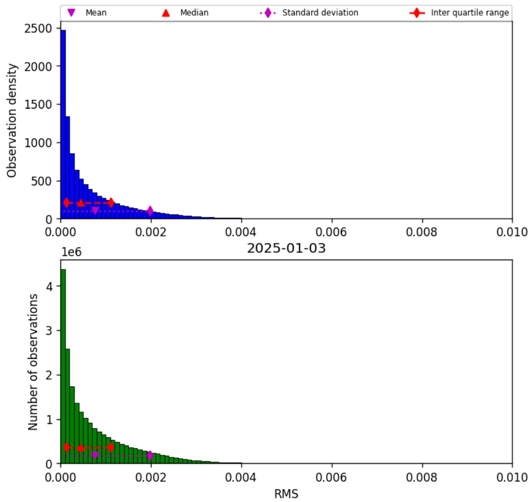
Figure 47: Histogram of “RMS” for 2025-01-02 to 2025-01-04
