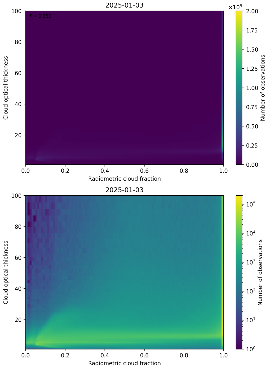
Figure 75: Scatter density plot of “Radiometric cloud fraction” against “Cloud optical thickness” for 2025-01-02 to 2025-01-04.
