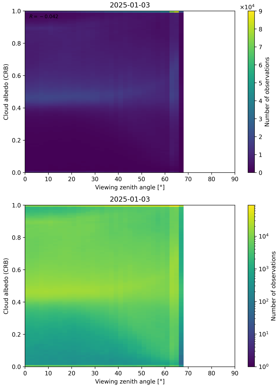
Figure 106: Scatter density plot of “Viewing zenith angle” against “Cloud albedo (CRB)” for 2025-01-02 to 2025-01-04.
