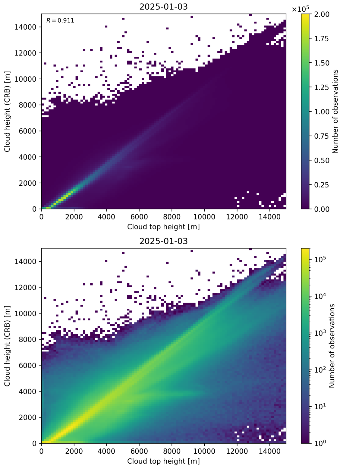
Figure 89: Scatter density plot of “Cloud top height” against “Cloud height (CRB)” for 2025-01-02 to 2025-01-04.
