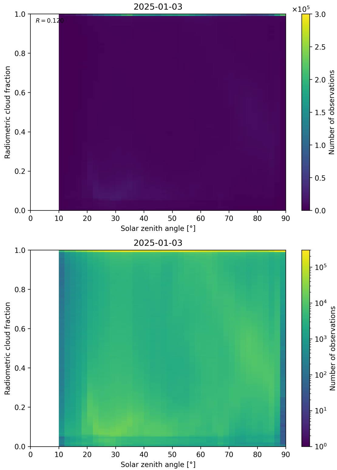
Figure 99: Scatter density plot of “Solar zenith angle” against “Radiometric cloud fraction” for 2025-01-02 to 2025-01-04.
