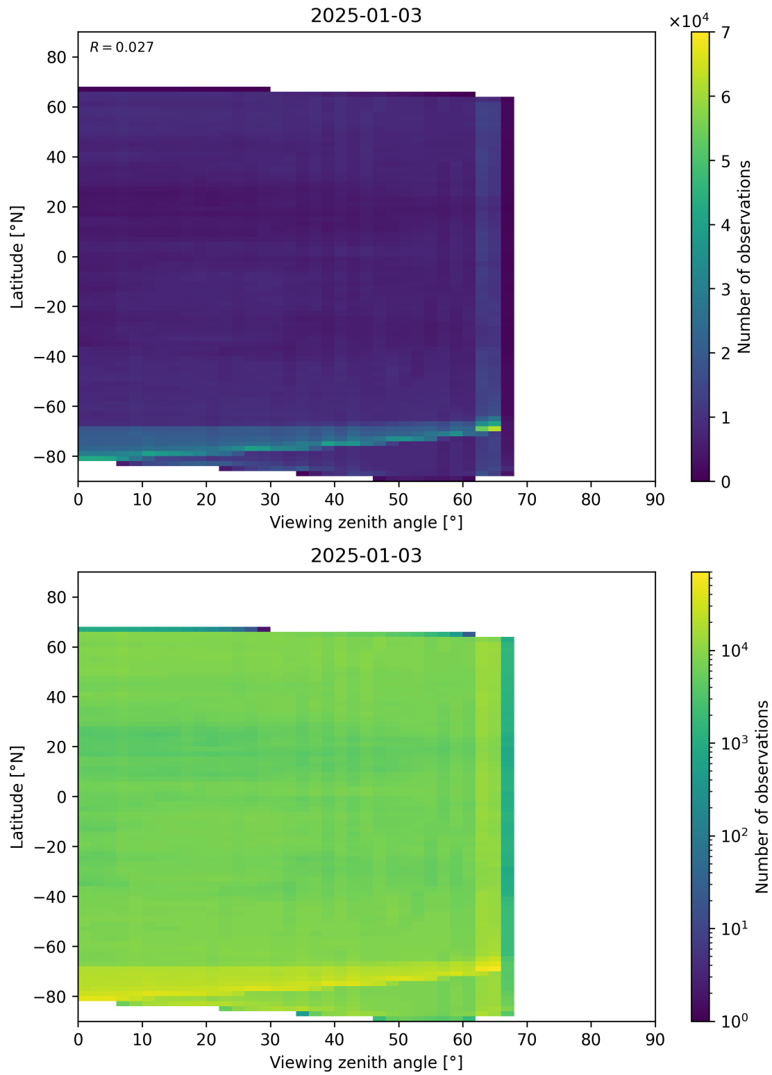
Figure 113: Scatter density plot of “Viewing zenith angle” against “Latitude” for 2025-01-02 to 2025-01-04.
