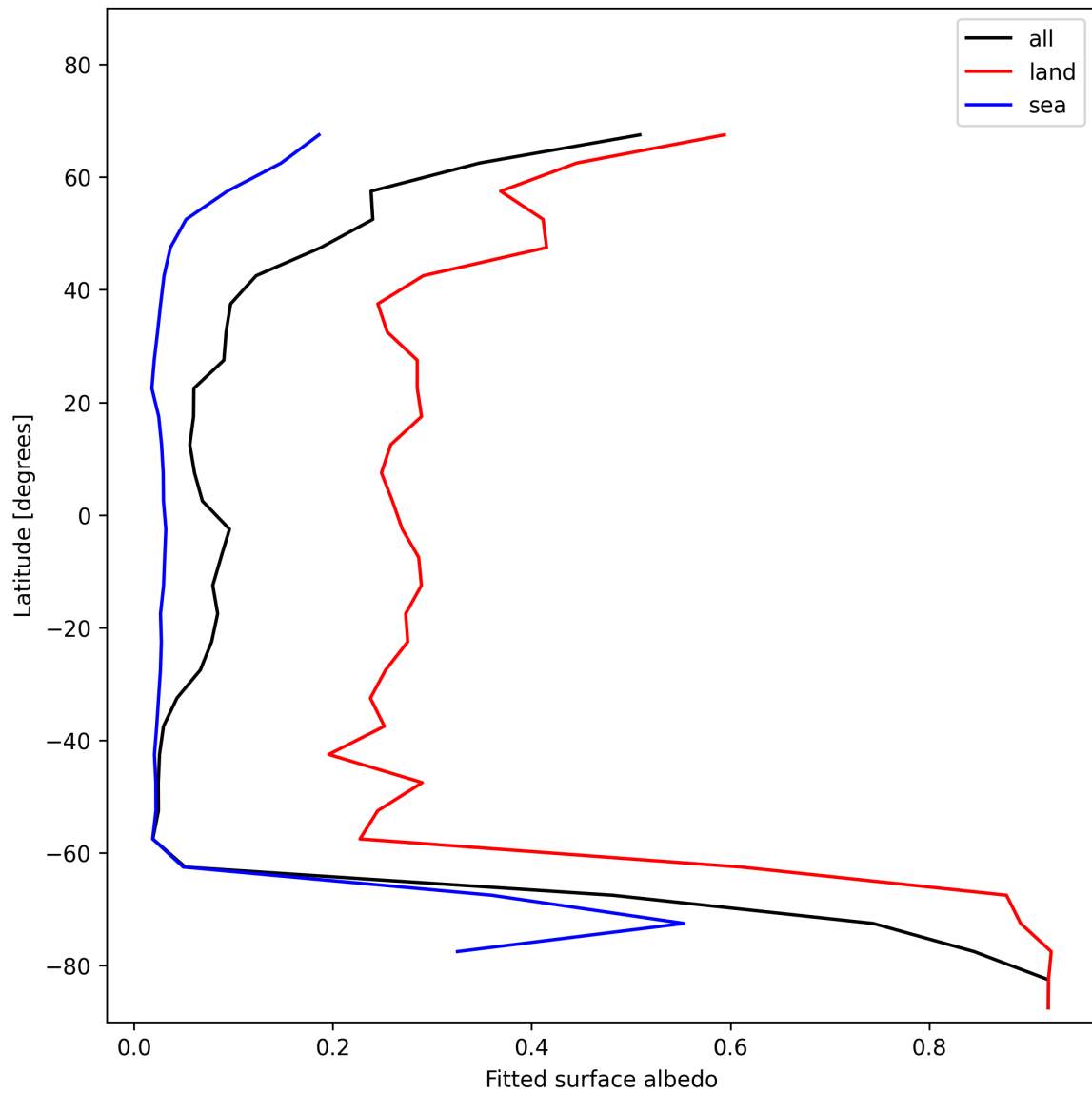
Figure 29: Zonal average of “Fitted surface albedo” for 2025-01-02 to 2025-01-04.
