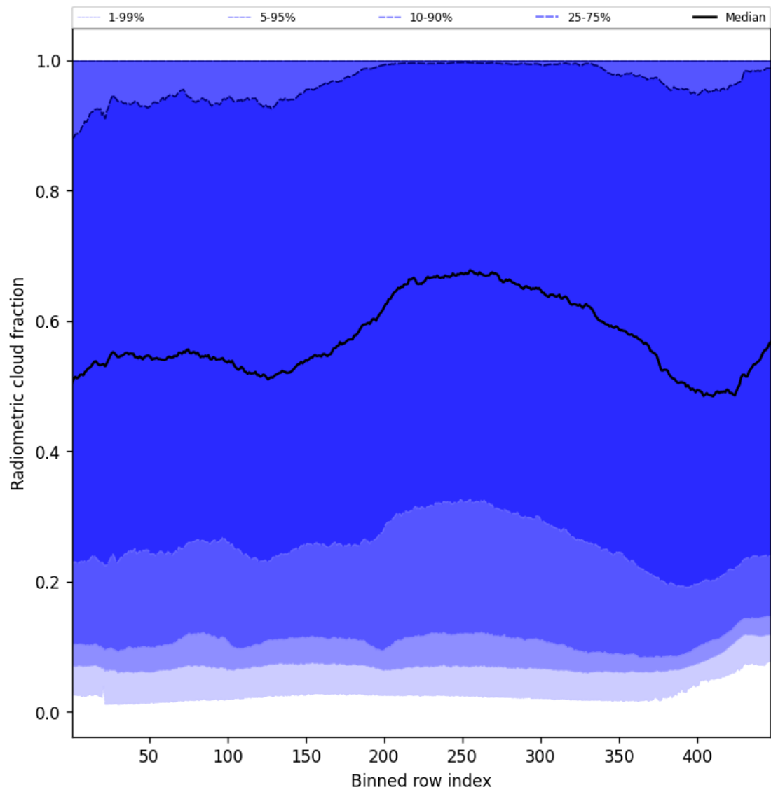
Figure 55: Along track statistics of “Radiometric cloud fraction” for 2025-01-02 to 2025-01-04
