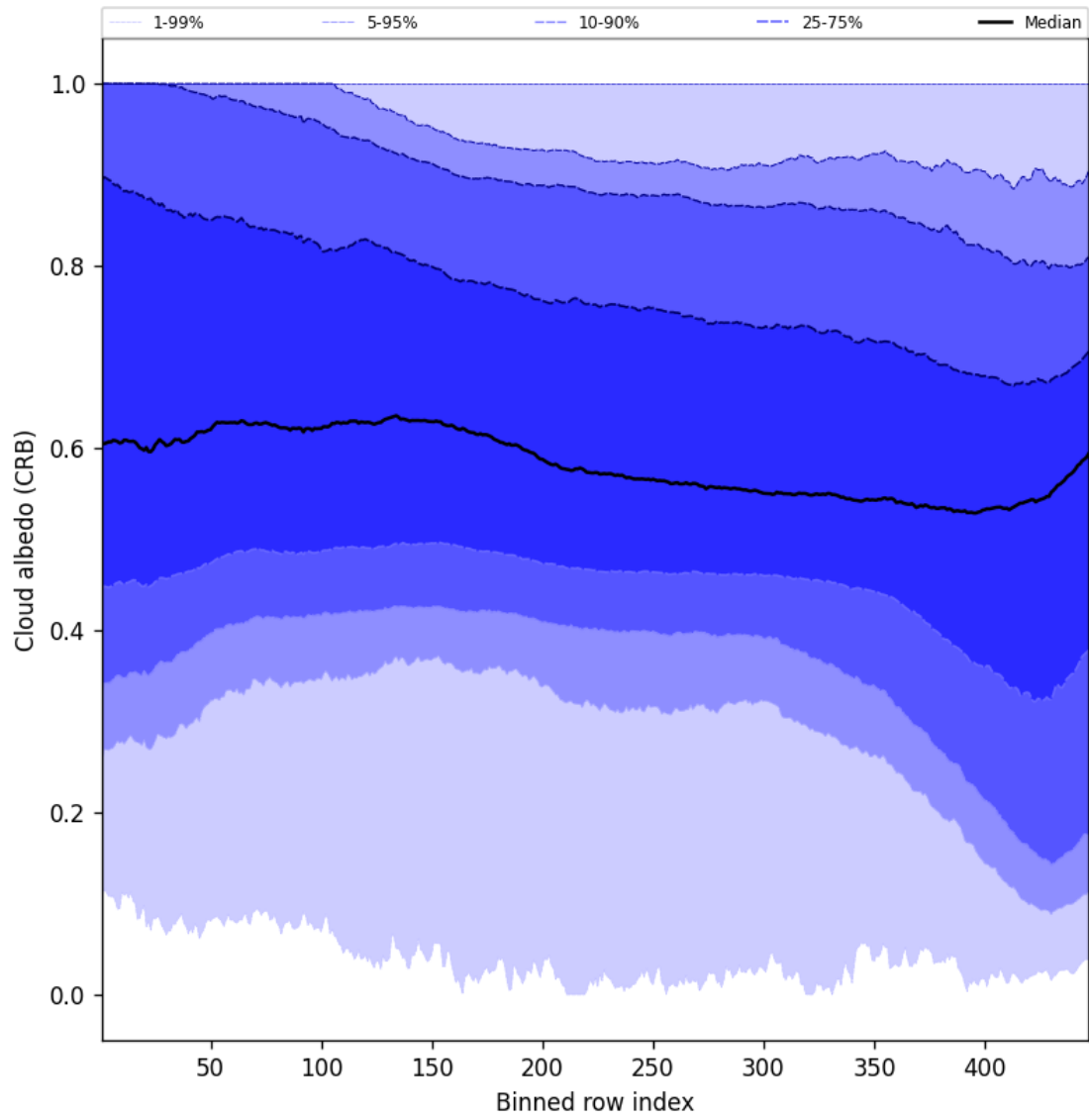
Figure 60: Along track statistics of “Cloud albedo (CRB)” for 2025-01-02 to 2025-01-04
