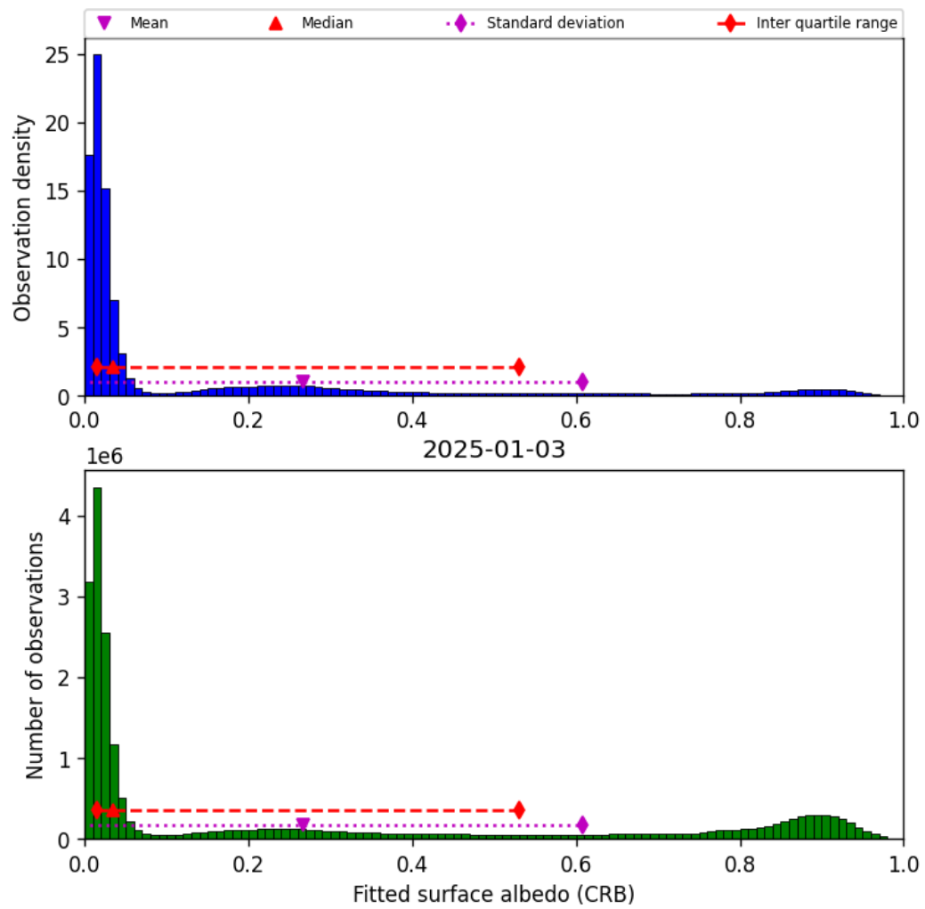
Figure 46: Histogram of “Fitted surface albedo (CRB)” for 2025-01-02 to 2025-01-04
