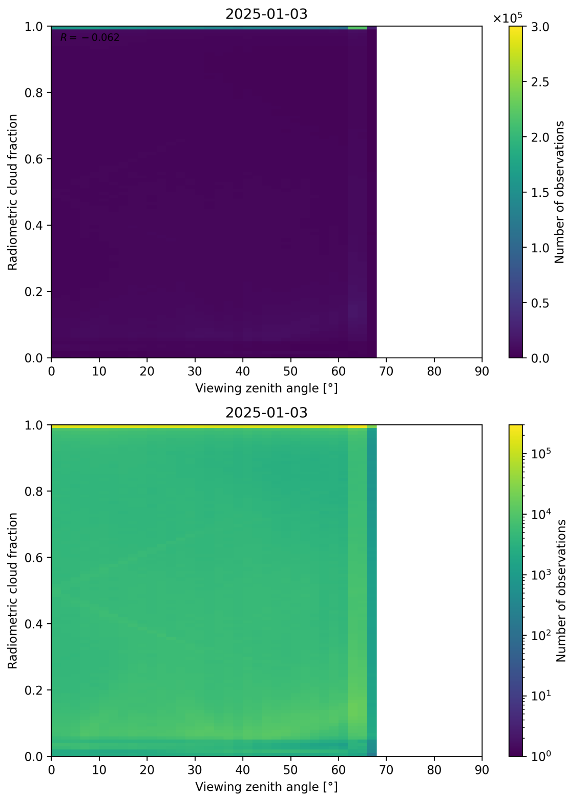
Figure 107: Scatter density plot of “Viewing zenith angle” against “Radiometric cloud fraction” for 2025-01-02 to 2025-01-04.
