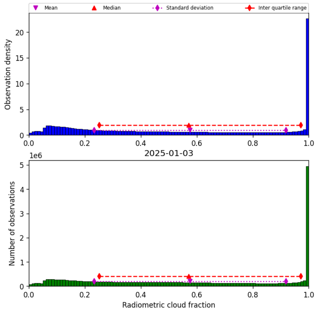
Figure 39: Histogram of “Radiometric cloud fraction” for 2025-01-02 to 2025-01-04
