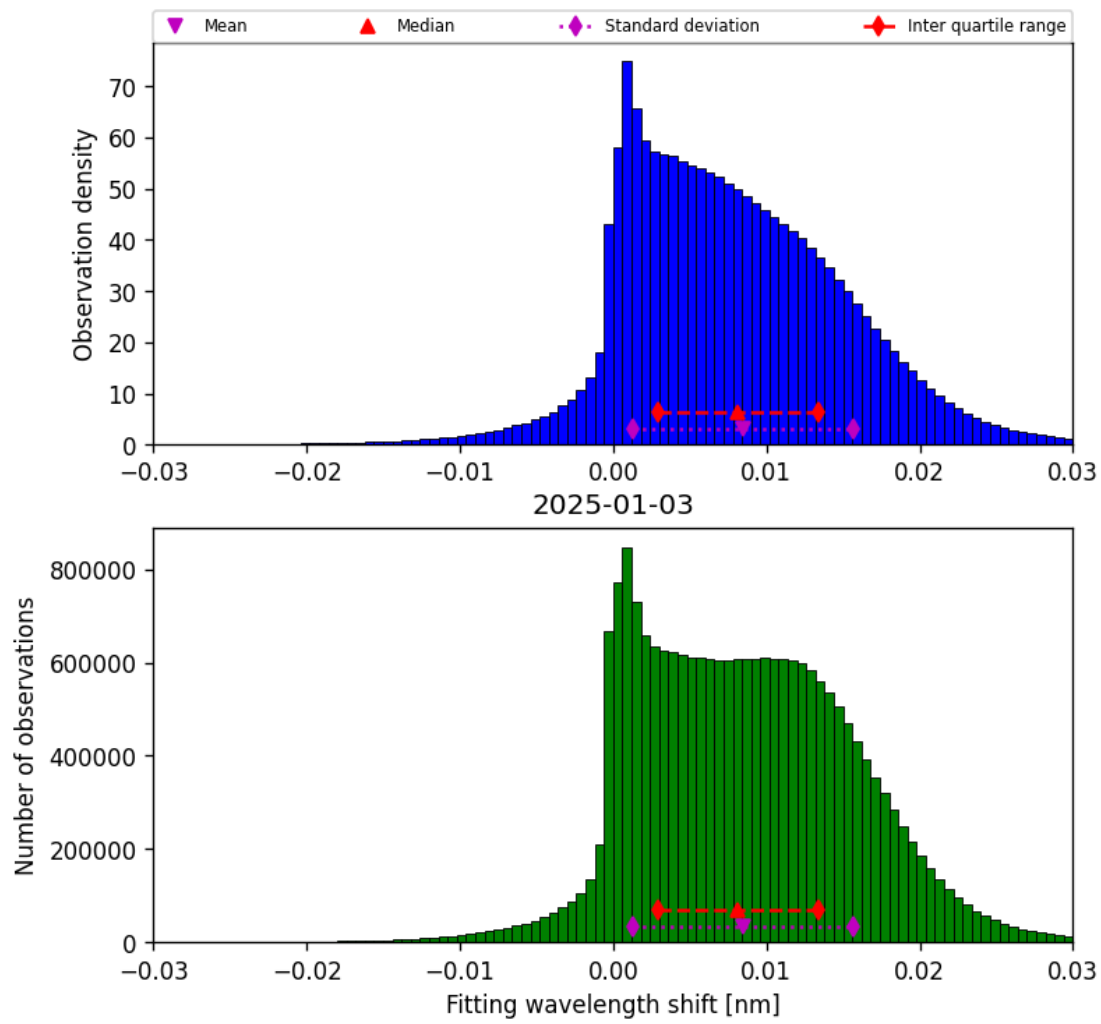
Figure 49: Histogram of “Fitting wavelength shift” for 2025-01-02 to 2025-01-04
