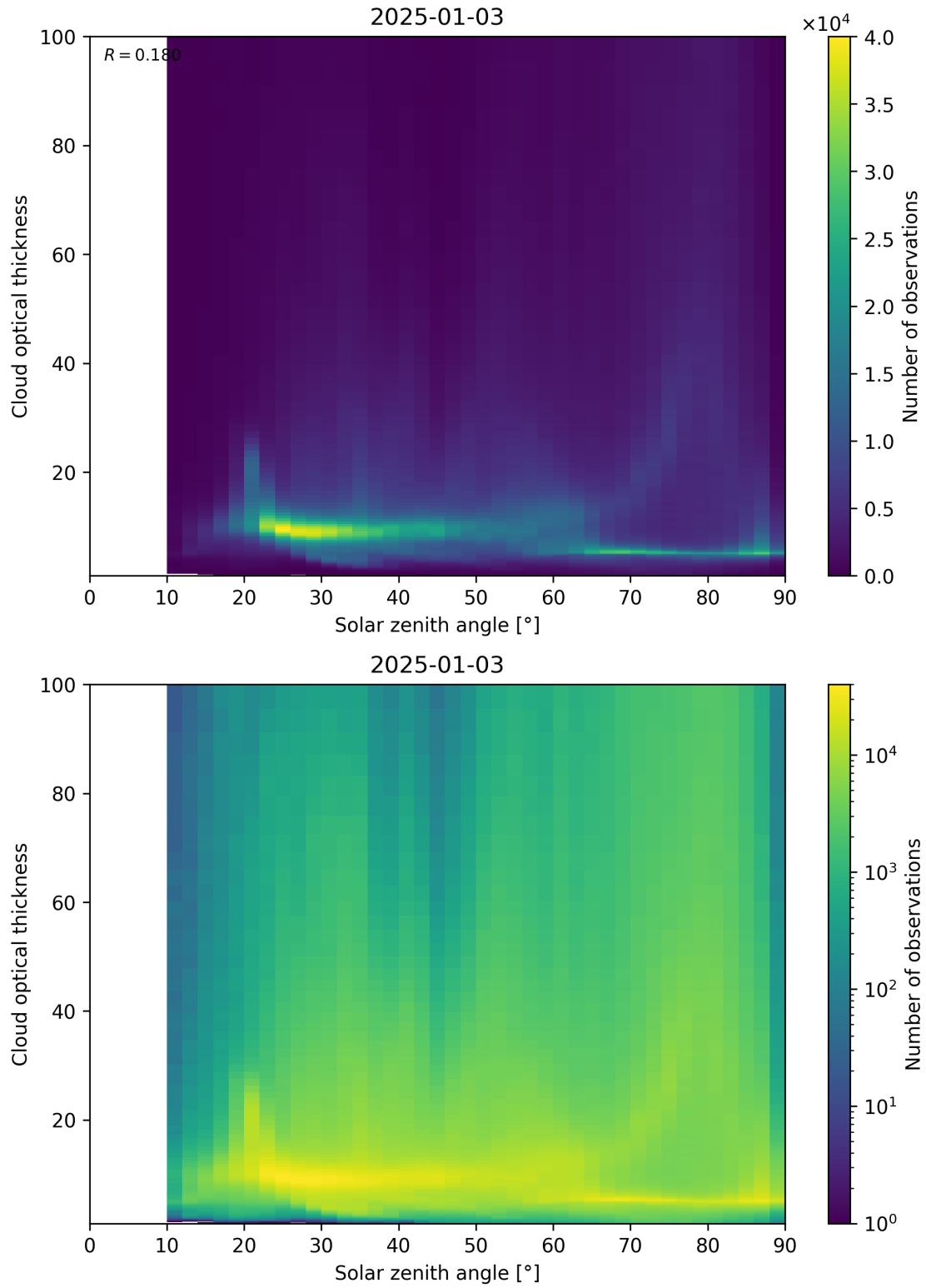
Figure 103: Scatter density plot of “Solar zenith angle” against “Cloud optical thickness” for 2025-01-02 to 2025-01-04.
