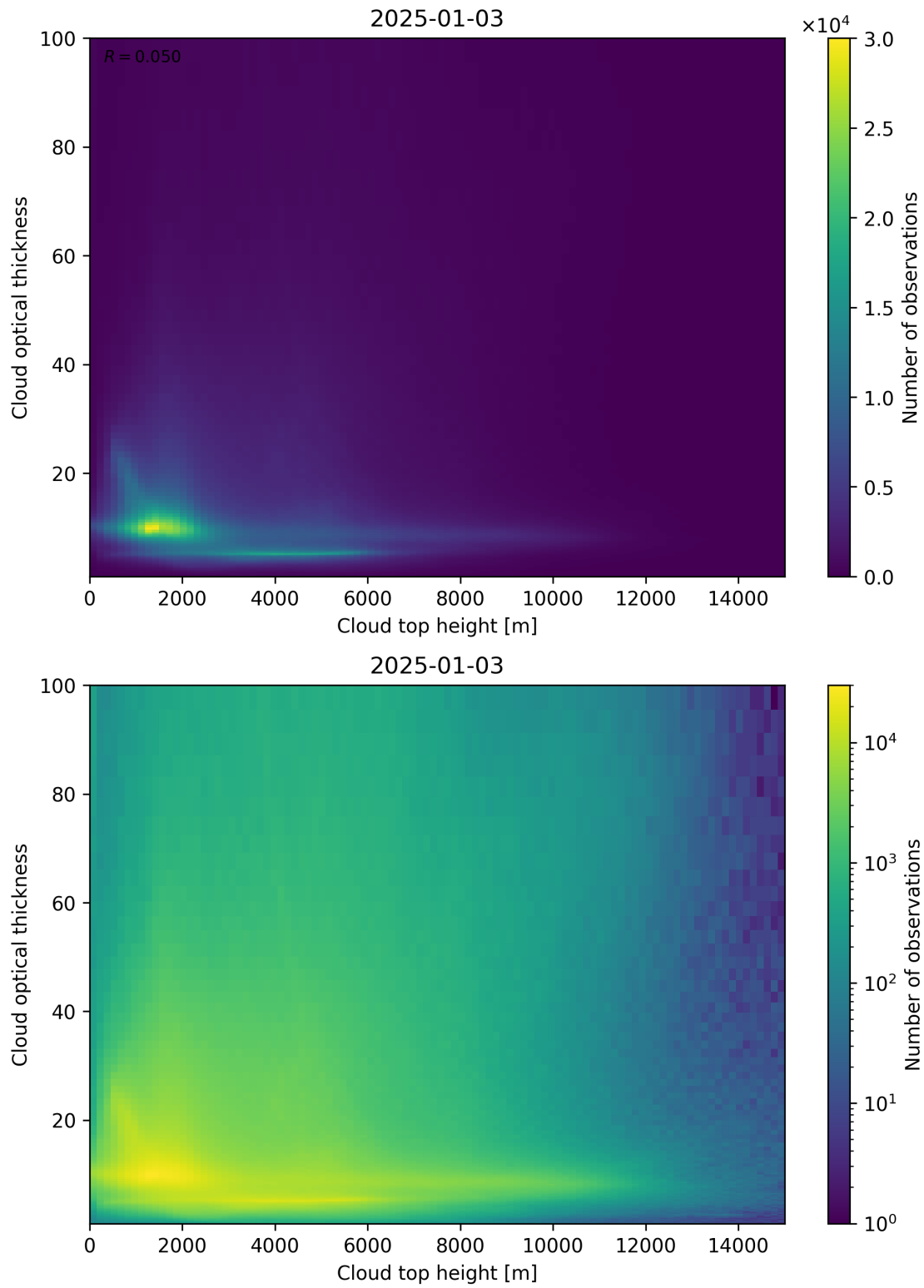
Figure 90: Scatter density plot of “Cloud top height” against “Cloud optical thickness” for 2025-01-02 to 2025-01-04.
