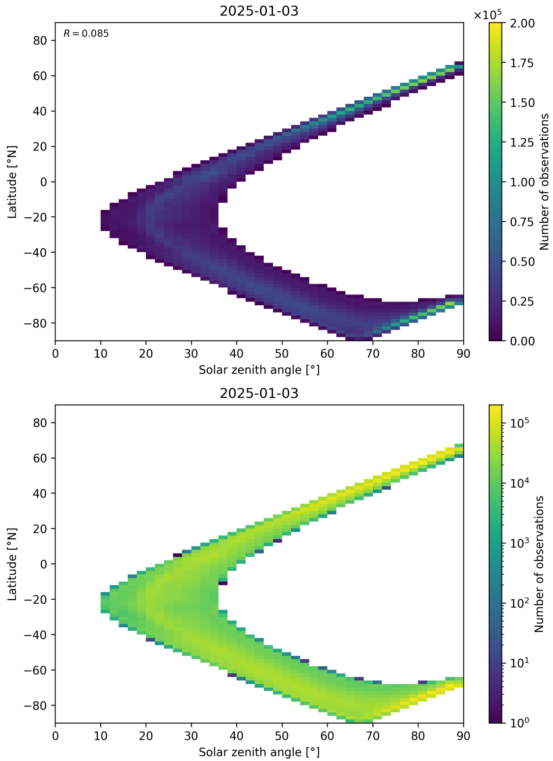
Figure 105: Scatter density plot of “Solar zenith angle” against “Latitude” for 2025-01-02 to 2025-01-04.
