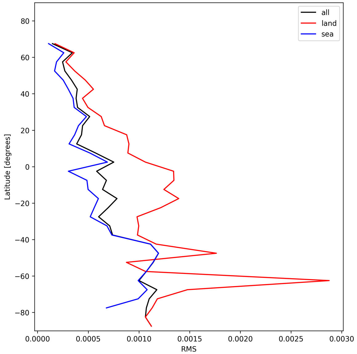
Figure 31: Zonal average of “RMS” for 2025-01-02 to 2025-01-04.
