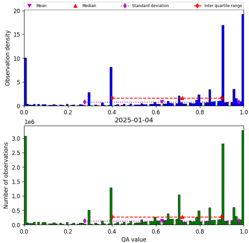
Figure 38: Histogram of “QA value” for 2025-01-03 to 2025-01-05
