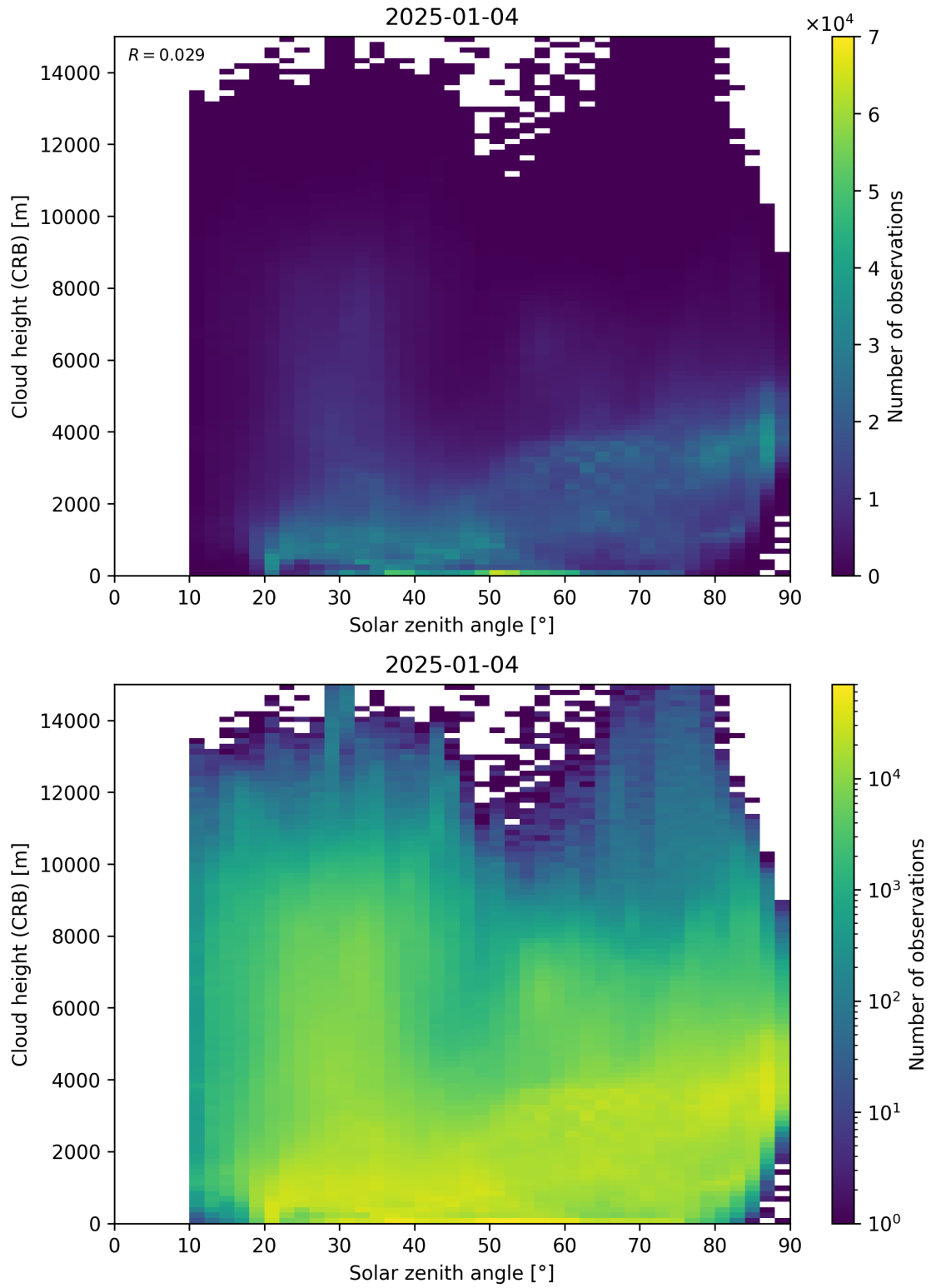
Figure 102: Scatter density plot of “Solar zenith angle” against “Cloud height (CRB)” for 2025-01-03 to 2025-01-05.
