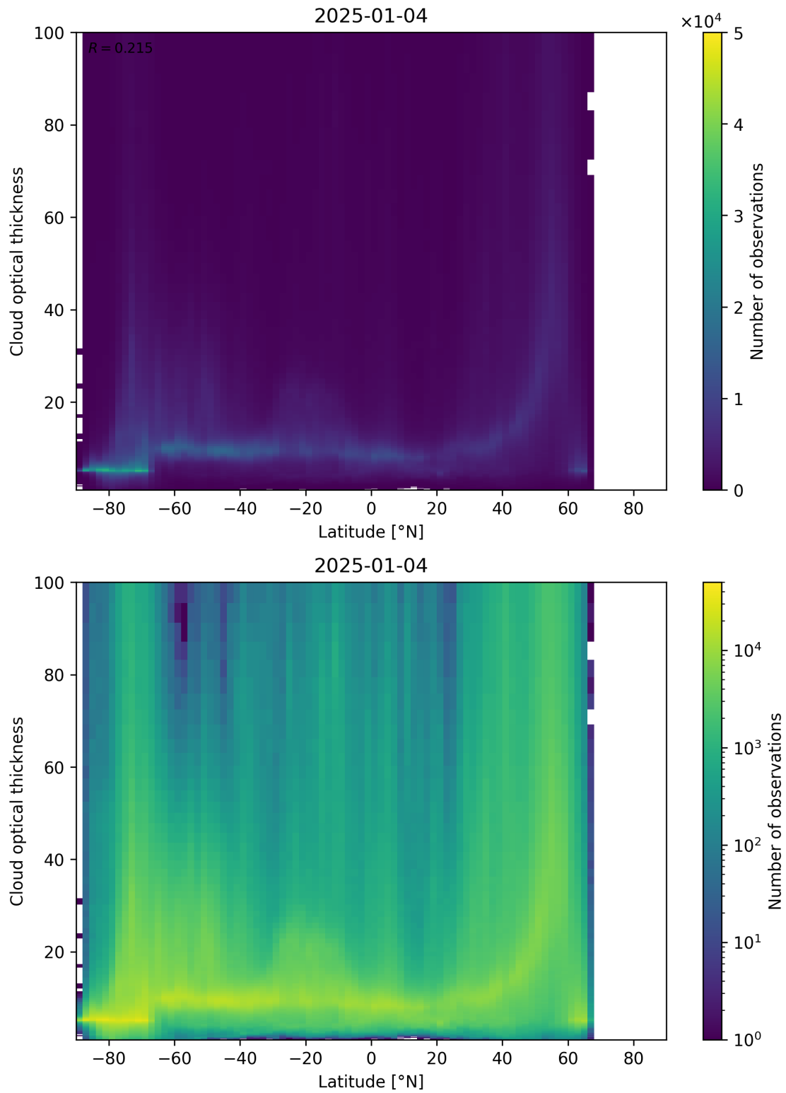
Figure 96: Scatter density plot of “Latitude” against “Cloud optical thickness” for 2025-01-03 to 2025-01-05.
