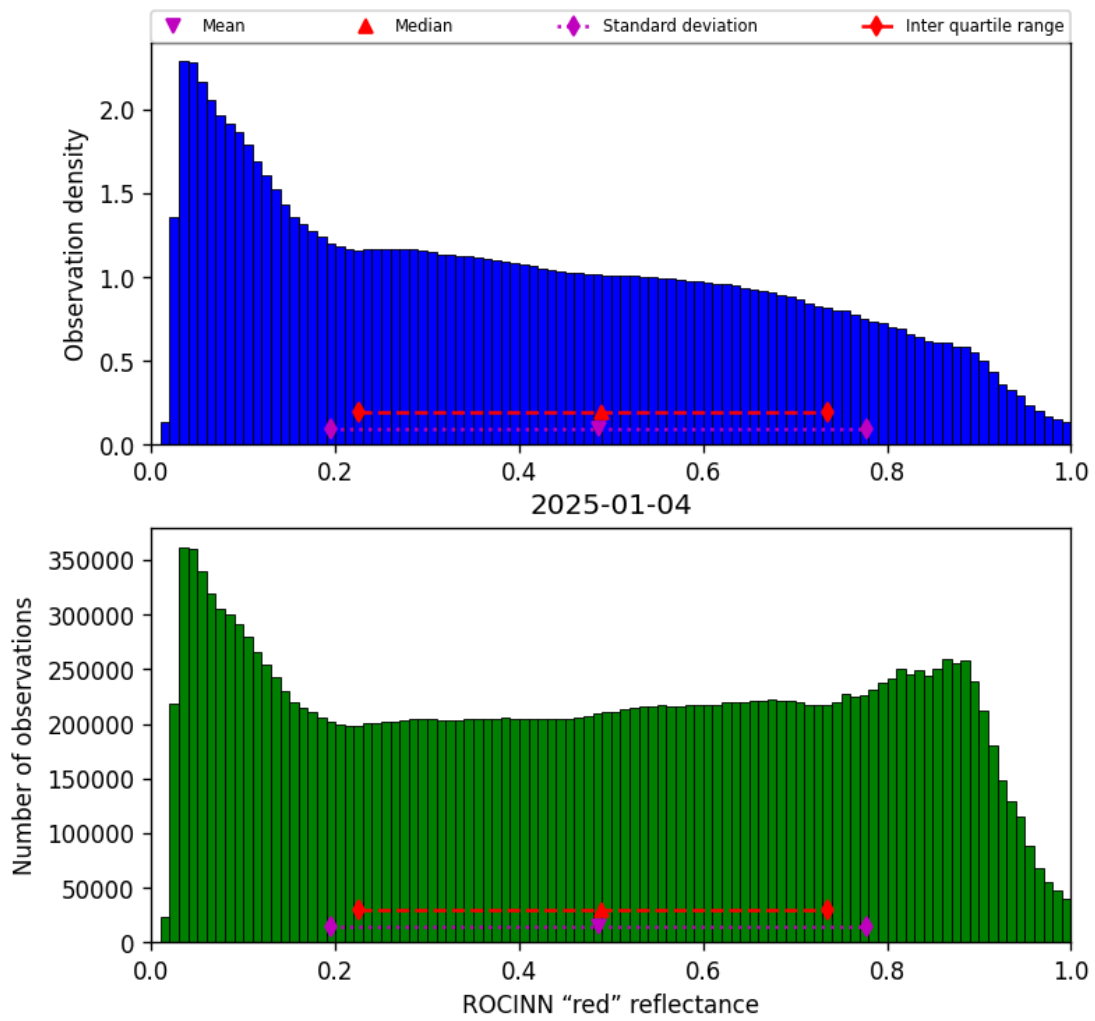
Figure 53: Histogram of “ROCINN “red” reflectance” for 2025-01-03 to 2025-01-05
