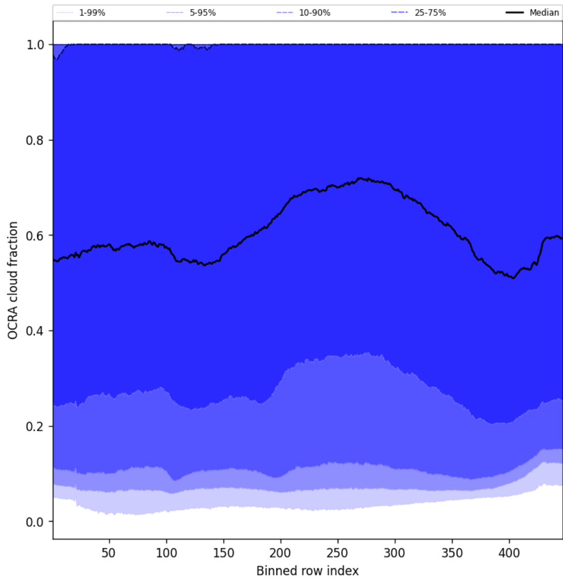
Figure 66: Along track statistics of “OCRA cloud fraction” for 2025-01-03 to 2025-01-05
