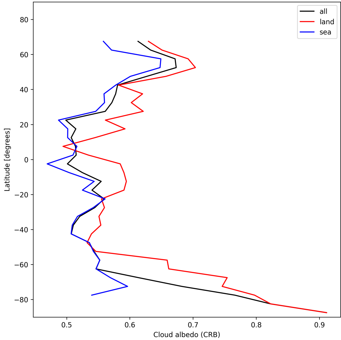
Figure 28: Zonal average of “Cloud albedo (CRB)” for 2025-01-03 to 2025-01-05.
