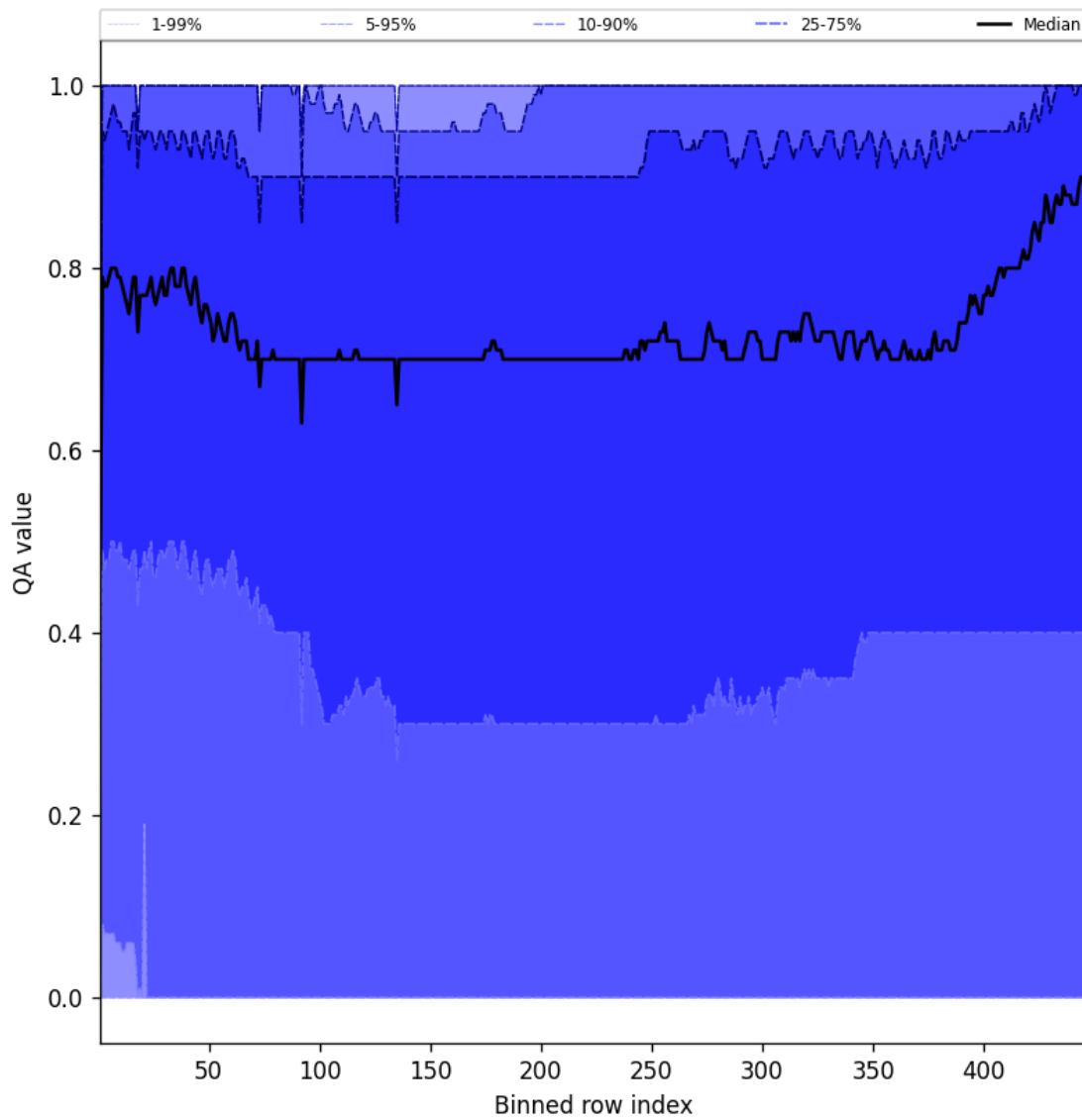
Figure 54: Along track statistics of “QA value” for 2025-01-03 to 2025-01-05
