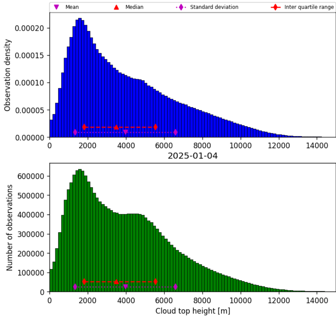
Figure 40: Histogram of “Cloud top height” for 2025-01-03 to 2025-01-05
