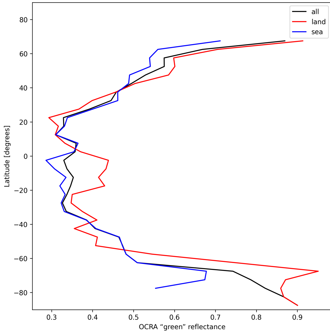
Figure 36: Zonal average of “OCRA “green” reflectance” for 2025-01-03 to 2025-01-05.
