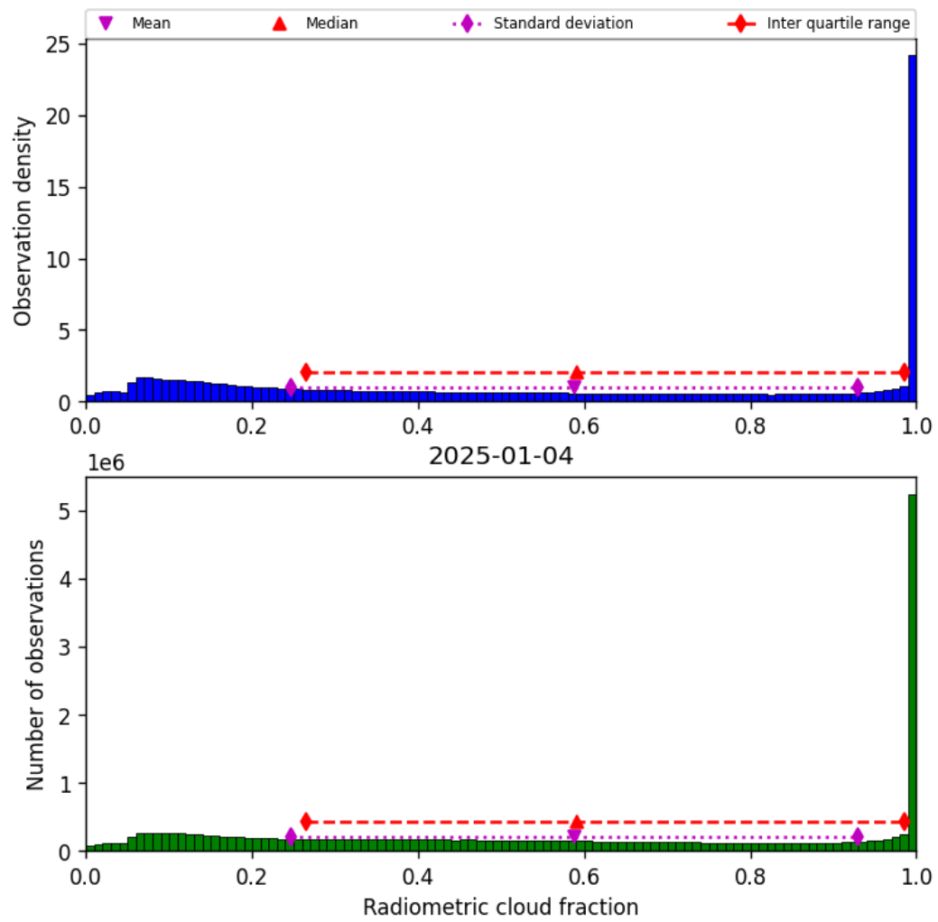
Figure 39: Histogram of “Radiometric cloud fraction” for 2025-01-03 to 2025-01-05
