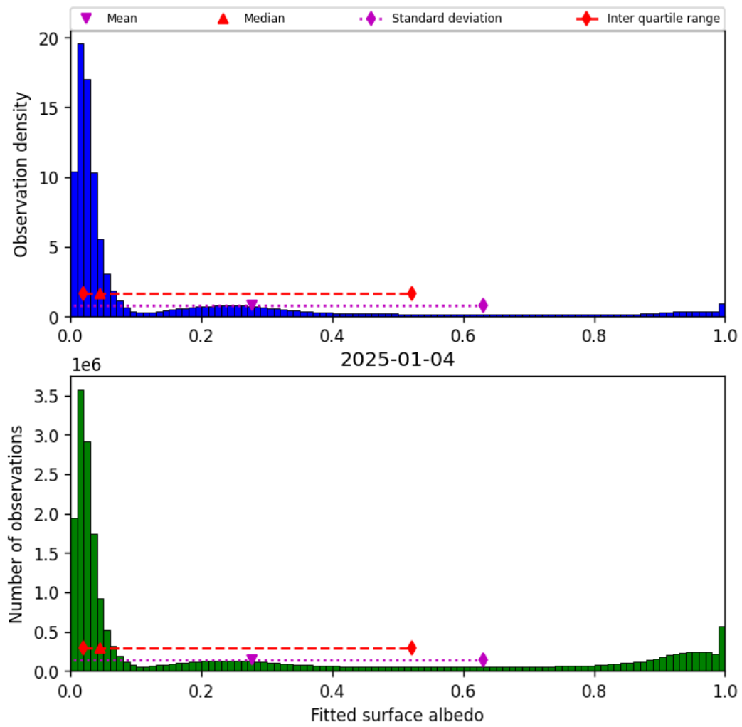
Figure 45: Histogram of “Fitted surface albedo” for 2025-01-03 to 2025-01-05
