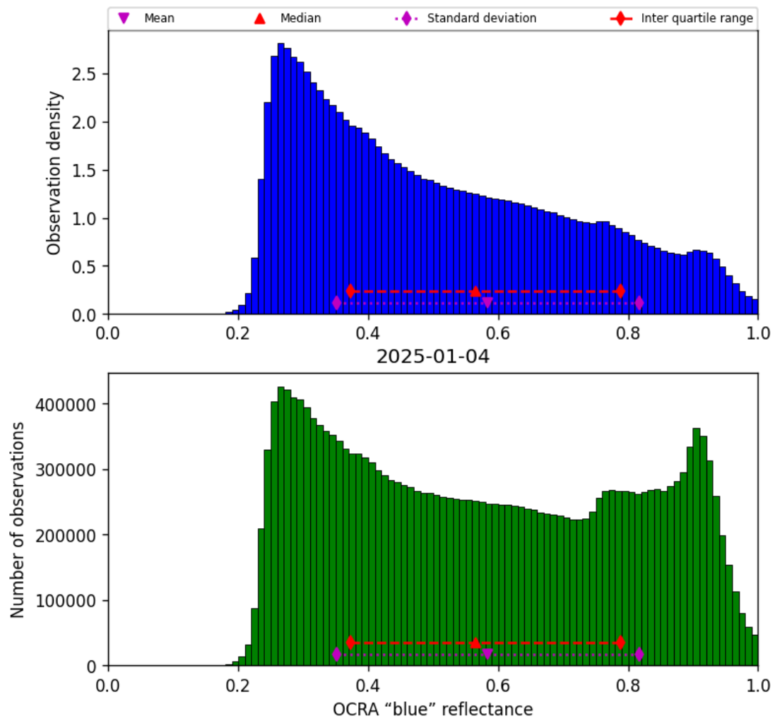
Figure 51: Histogram of “OCRA “blue” reflectance” for 2025-01-03 to 2025-01-05
