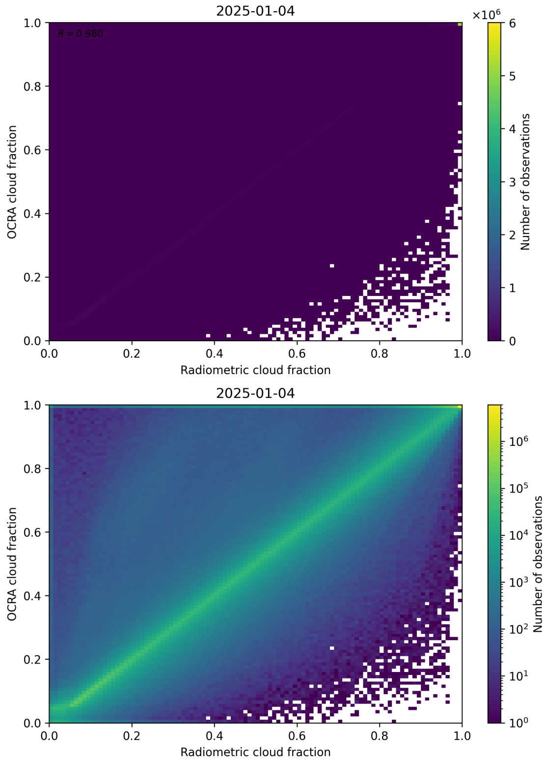
Figure 72: Scatter density plot of “Radiometric cloud fraction” against “OCRA cloud fraction” for 2025-01-03 to 2025-01-05.
