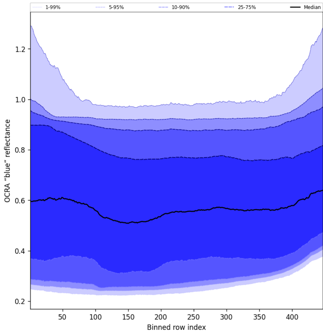
Figure 67: Along track statistics of "OCRA "blue" reflectance" for 2025-01-03 to 2025-01-05
