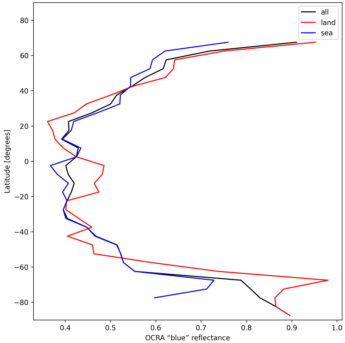
Figure 35: Zonal average of “OCRA “blue” reflectance” for 2025-01-03 to 2025-01-05.
