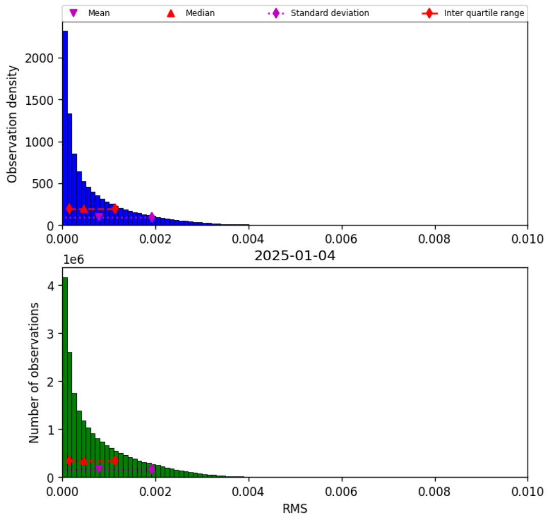
Figure 47: Histogram of “RMS” for 2025-01-03 to 2025-01-05
