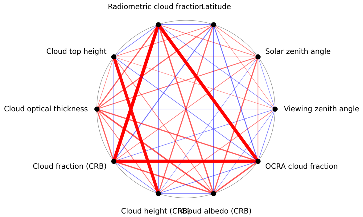
Figure 1: Map of correlation graph for 2025-01-04 to 2025-01-06.
