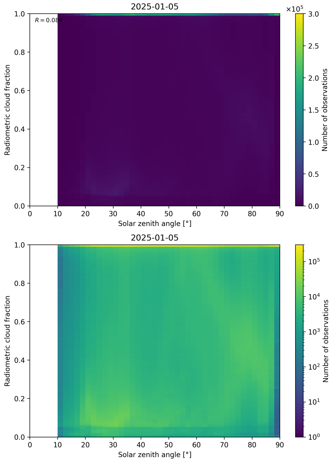
Figure 99: Scatter density plot of “Solar zenith angle” against “Radiometric cloud fraction” for 2025-01-04 to 2025-01-06.
