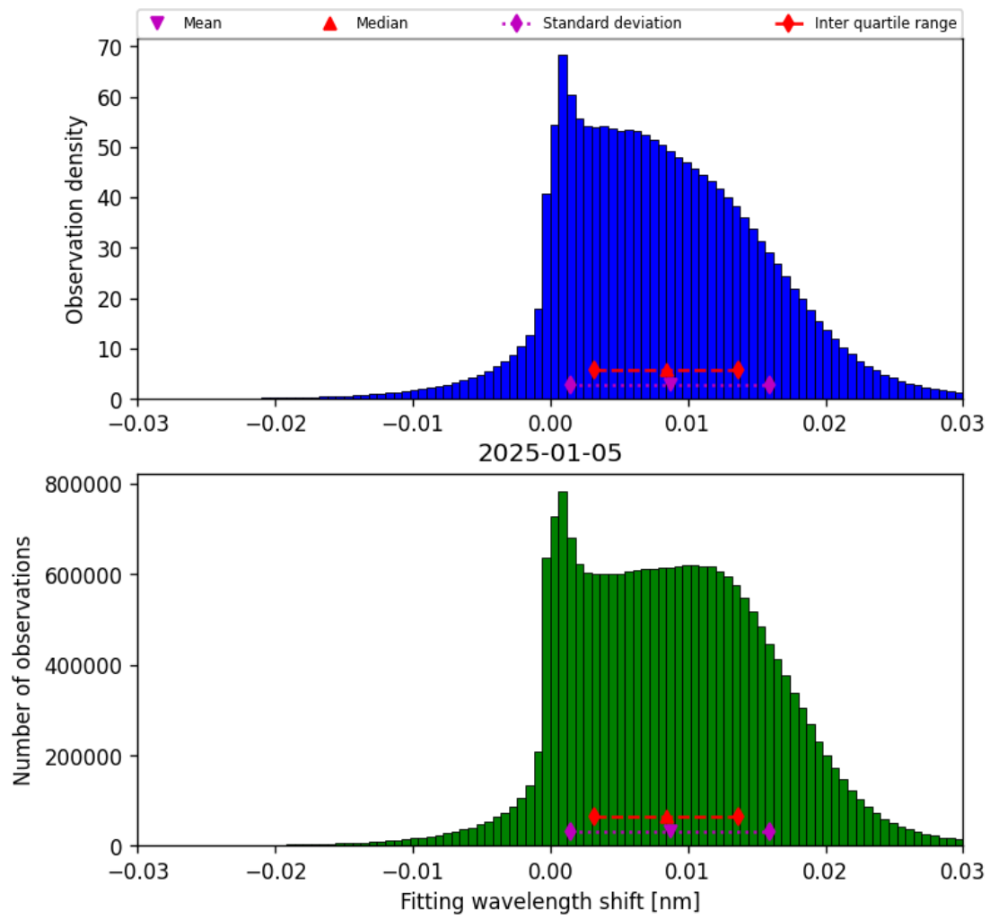
Figure 49: Histogram of “Fitting wavelength shift” for 2025-01-04 to 2025-01-06
