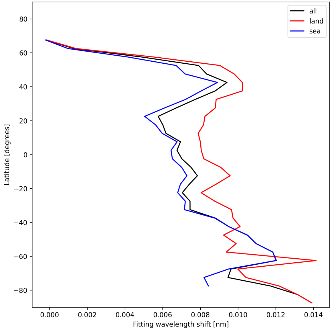
Figure 33: Zonal average of “Fitting wavelength shift” for 2025-01-04 to 2025-01-06.
