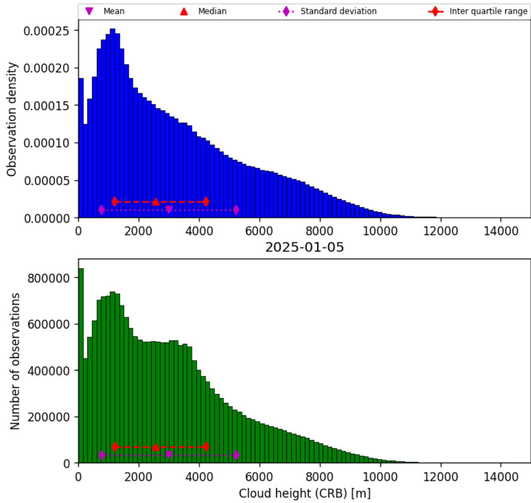
Figure 43: Histogram of “Cloud height (CRB)” for 2025-01-04 to 2025-01-06
