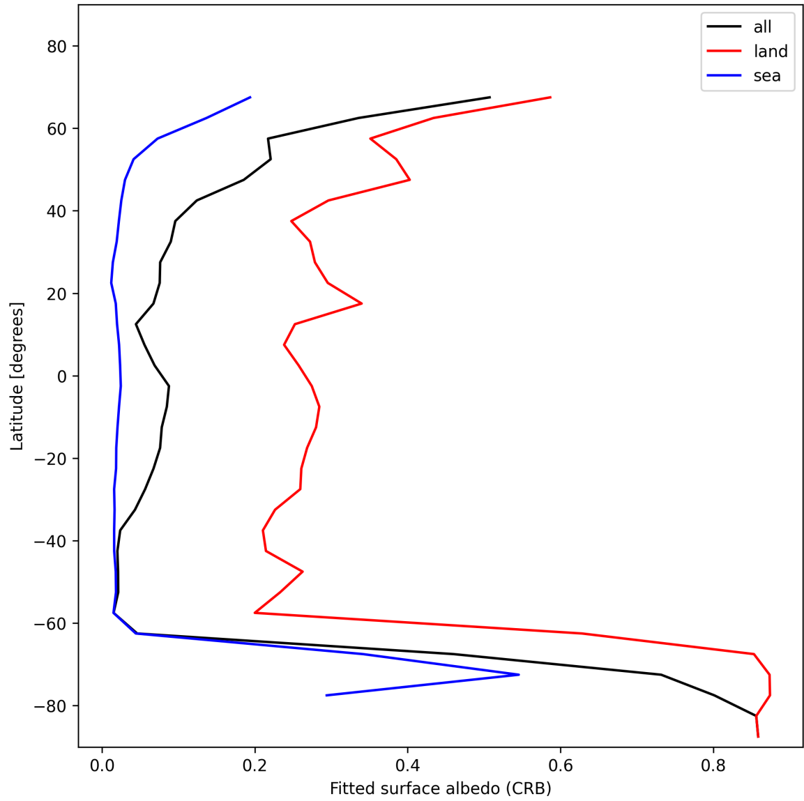
Figure 30: Zonal average of “Fitted surface albedo (CRB)” for 2025-01-04 to 2025-01-06.
