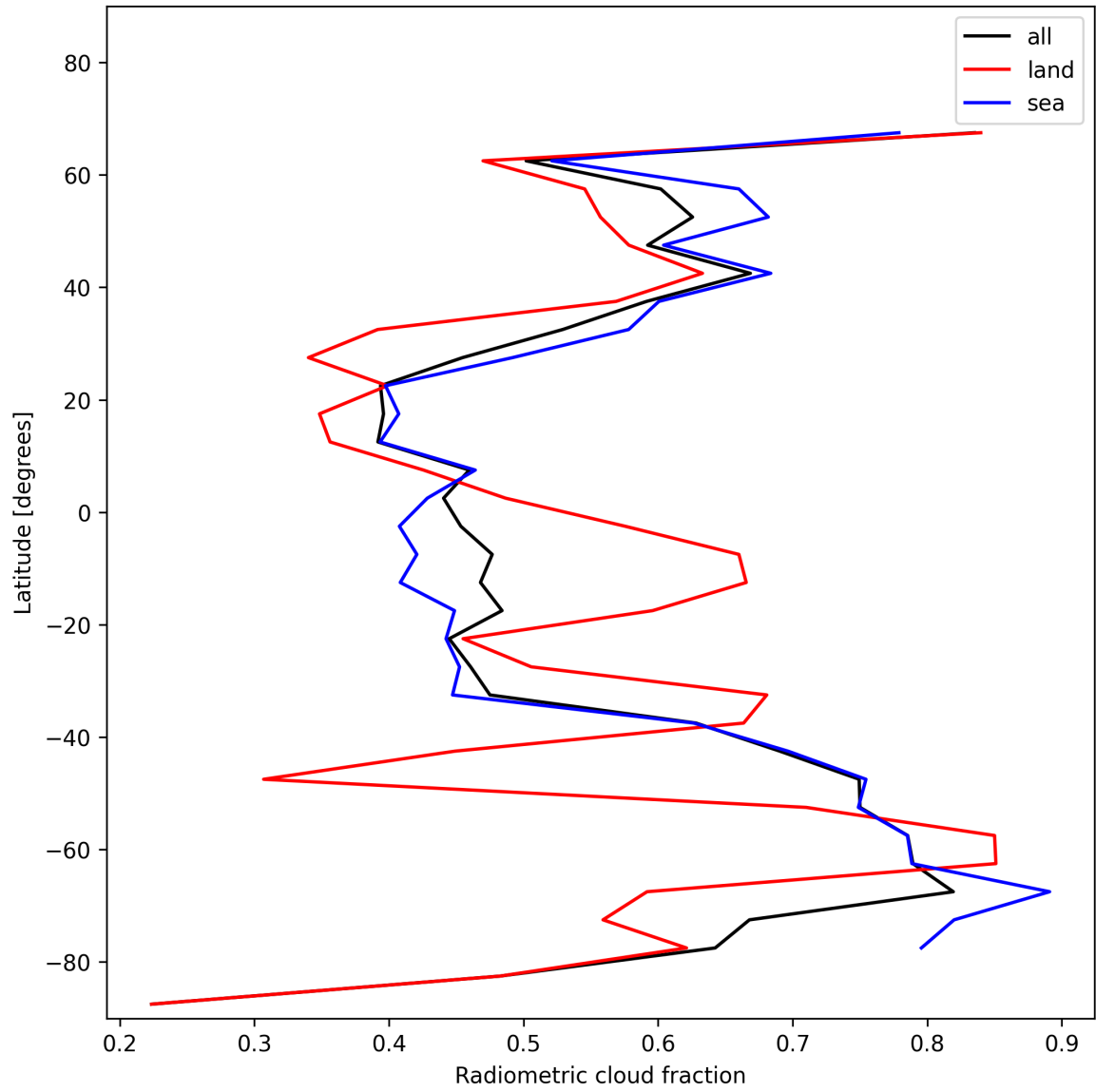
Figure 23: Zonal average of “Radiometric cloud fraction” for 2025-01-04 to 2025-01-06.
