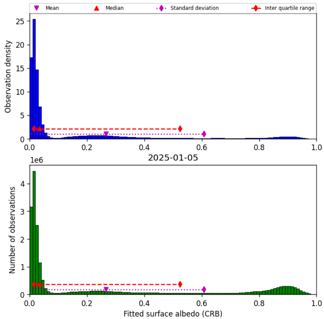
Figure 46: Histogram of “Fitted surface albedo (CRB)” for 2025-01-04 to 2025-01-06
